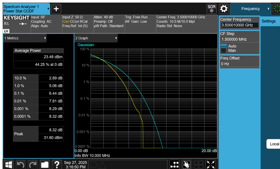
Plot 7-287. PAR Plot (NR Band n77 DoD-Band - 10MHz DFT-s-OFDM 256-QAM - Full RB)
