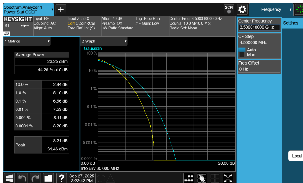
Plot 7-307. PAR Plot (NR Band n77 DoD-Band - 30MHz DFT-s-OFDM 256-QAM - Full RB)
