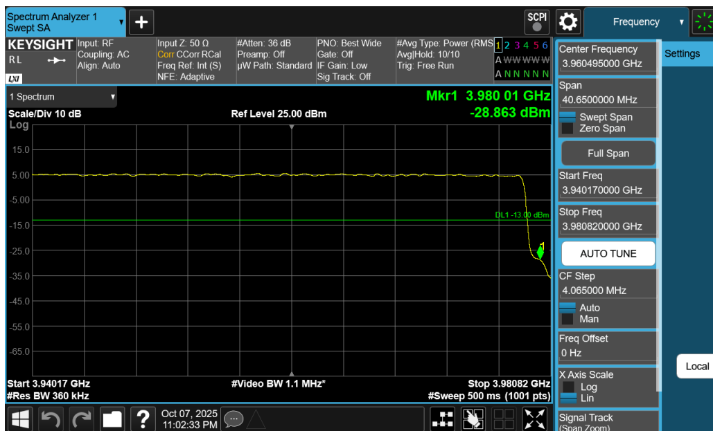
Plot 7-268. Upper Band Edge Plot (NR Band n77 C-Band - 80MHz DFT-s-OFDM QPSK – Full RB)
