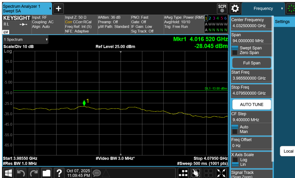
Plot 7-276. Extended Upper Band Edge Plot (NR Band n77 C-Band - 90MHz DFT-s-OFDM QPSK – Full RB)
