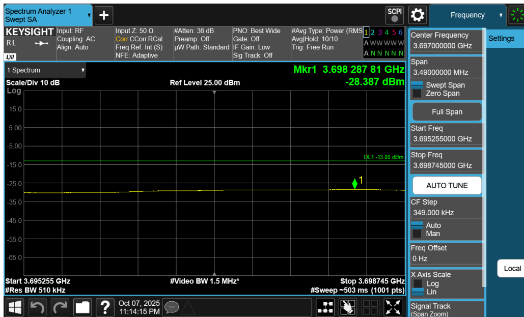
Plot 7-278. Extended Lower Band Edge Plot (NR Band n77 C-Band - 100MHz DFT-s-OFDM QPSK – Full RB)
