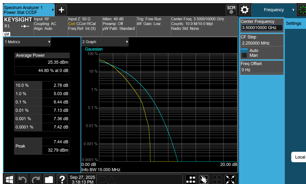
Plot 7-291. PAR Plot (NR Band n77 DoD-Band - 15MHz DFT-s-OFDM 64-QAM - Full RB)
