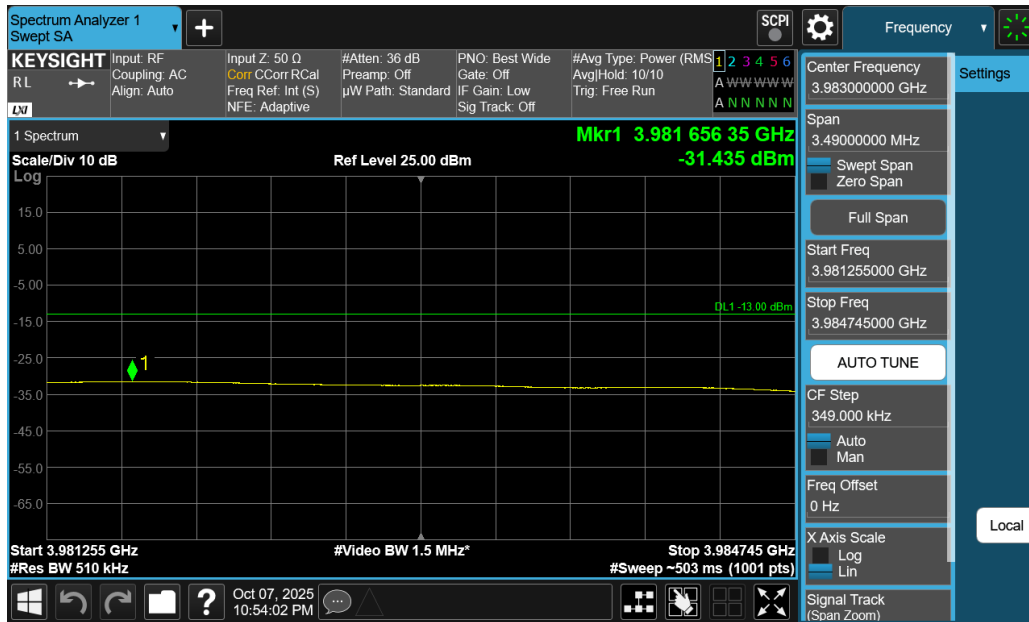
Plot 7-263. Extended Upper Band Edge Plot (NR Band n77 C-Band - 70MHz DFT-s-OFDM QPSK – Full RB)
