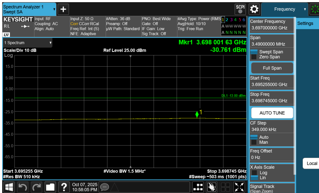
Plot 7-266. Extended Lower Band Edge Plot (NR Band n77 C-Band - 80MHz DFT-s-OFDM QPSK – Full RB)
