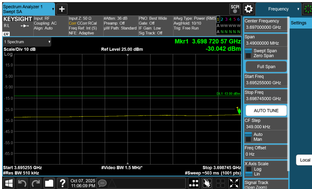
Plot 7-272. Extended Lower Band Edge Plot (NR Band n77 C-Band - 90MHz DFT-s-OFDM QPSK – Full RB)
