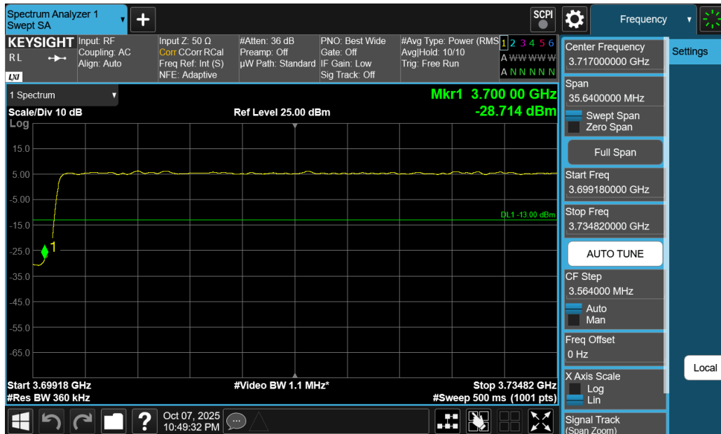
Plot 7-261. Lower Band Edge Plot (NR Band n77 C-Band - 70MHz DFT-s-OFDM QPSK – Full RB)
