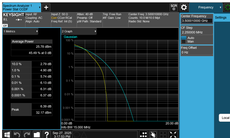
Plot 7-290. PAR Plot (NR Band n77 DoD-Band - 15MHz DFT-s-OFDM 16-QAM - Full RB)
