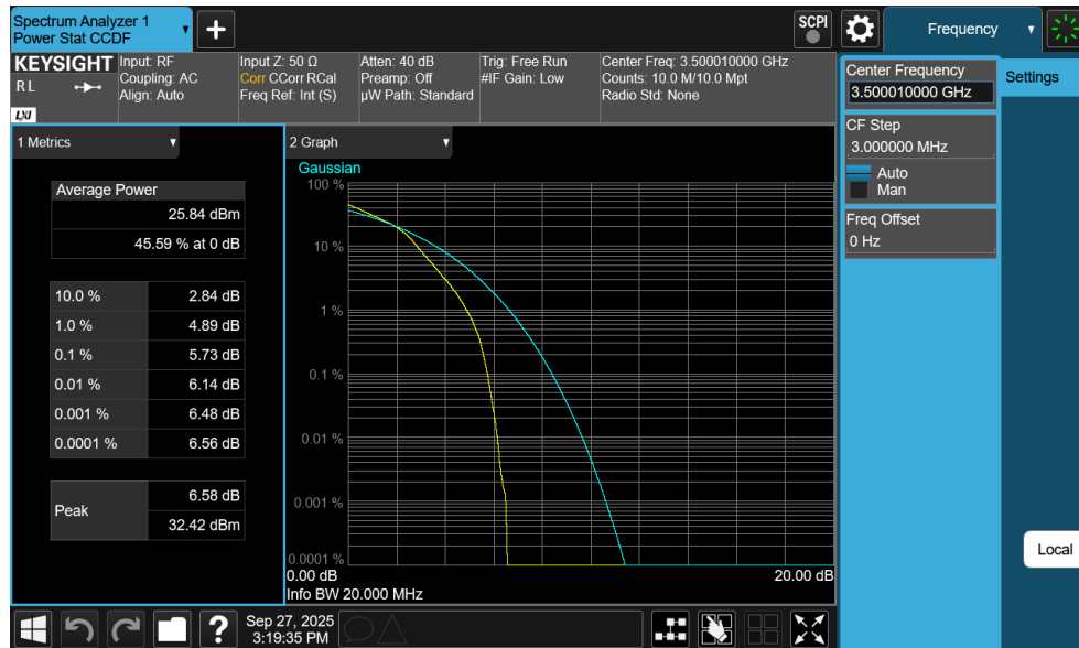
Plot 7-295. PAR Plot (NR Band n77 DoD-Band - 20MHz DFT-s-OFDM 16-QAM - Full RB)
