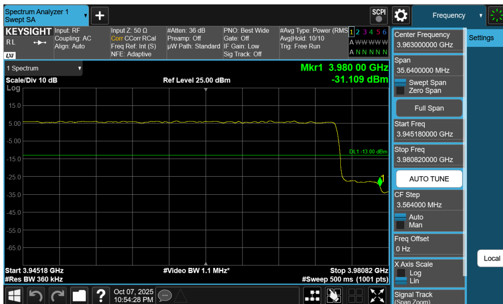
Plot 7-262. Upper Band Edge Plot (NR Band n77 C-Band - 70MHz DFT-s-OFDM QPSK – Full RB)
