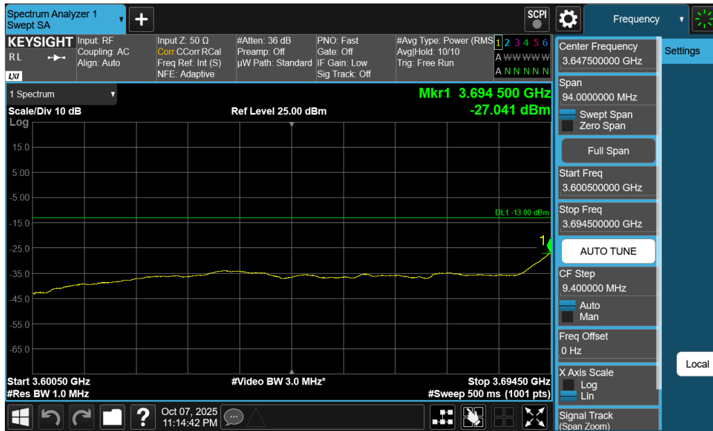
Plot 7-277. Extended Lower Band Edge Plot (NR Band n77 C-Band - 100MHz DFT-s-OFDM QPSK – Full RB)
