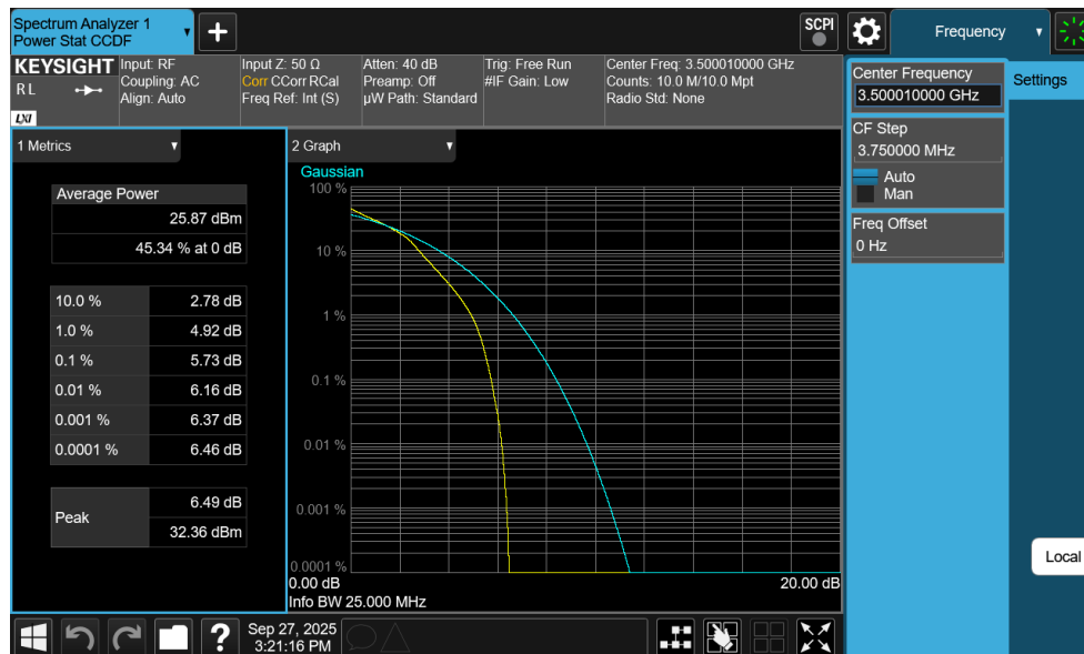
Plot 7-300. PAR Plot (NR Band n77 DoD-Band - 25MHz DFT-s-OFDM 16-QAM - Full RB)
