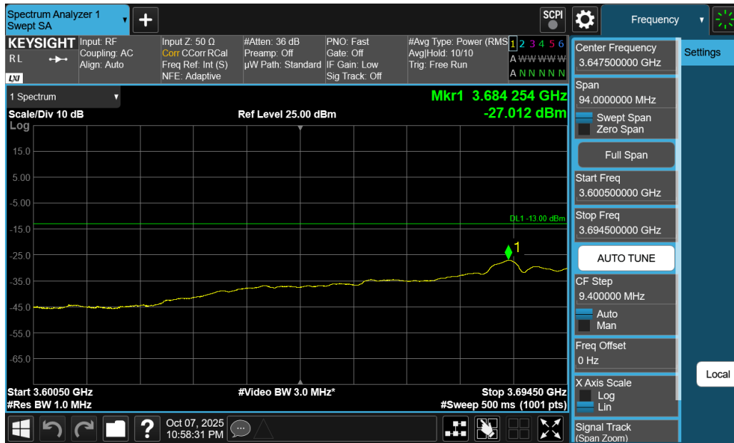
Plot 7-265. Extended Lower Band Edge Plot (NR Band n77 C-Band - 80MHz DFT-s-OFDM QPSK – Full RB)
