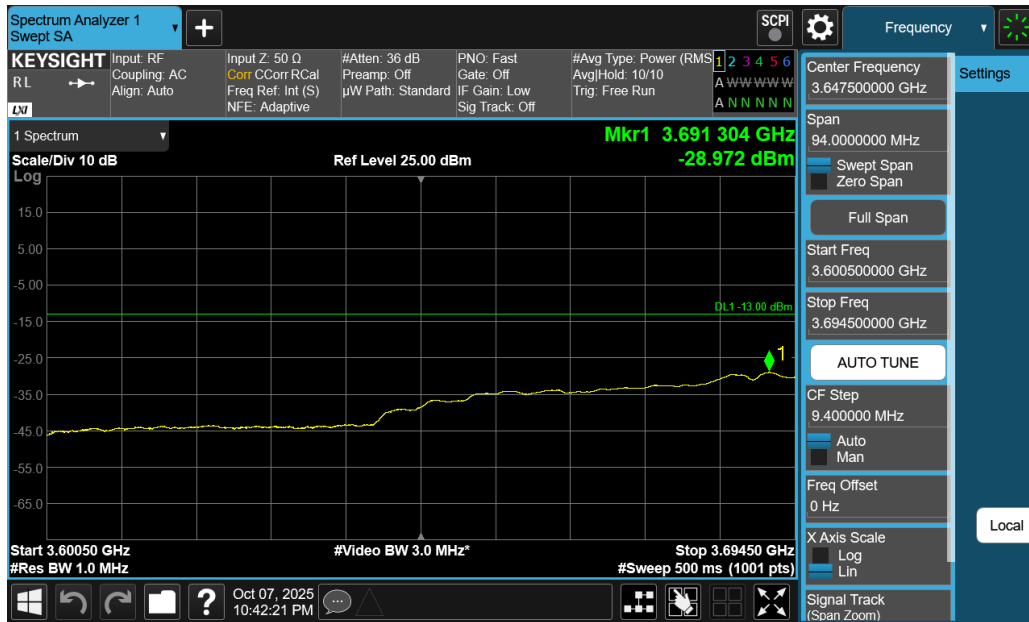
Plot 7-253. Extended Lower Band Edge Plot (NR Band n77 C-Band - 60MHz DFT-s-OFDM QPSK – Full RB)
