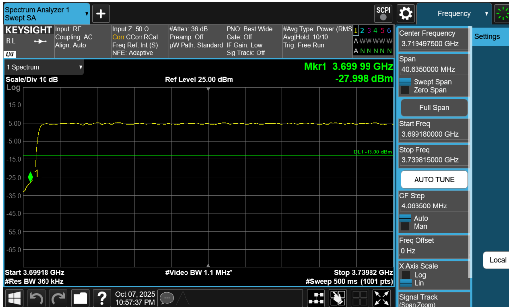
Plot 7-267. Lower Band Edge Plot (NR Band n77 C-Band - 80MHz DFT-s-OFDM QPSK – Full RB)
