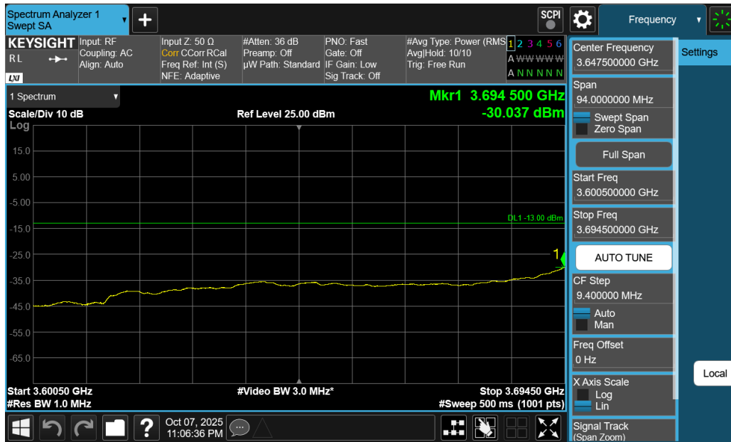
Plot 7-271. Extended Lower Band Edge Plot (NR Band n77 C-Band - 90MHz DFT-s-OFDM QPSK – Full RB)
