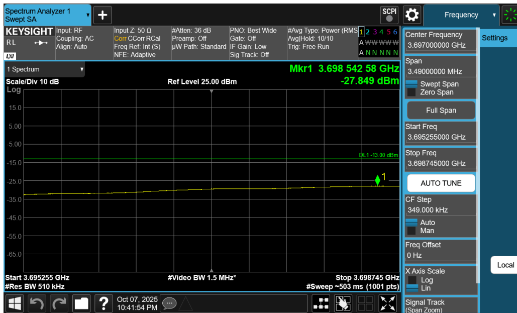
Plot 7-254. Extended Lower Band Edge Plot (NR Band n77 C-Band - 60MHz DFT-s-OFDM QPSK – Full RB)
