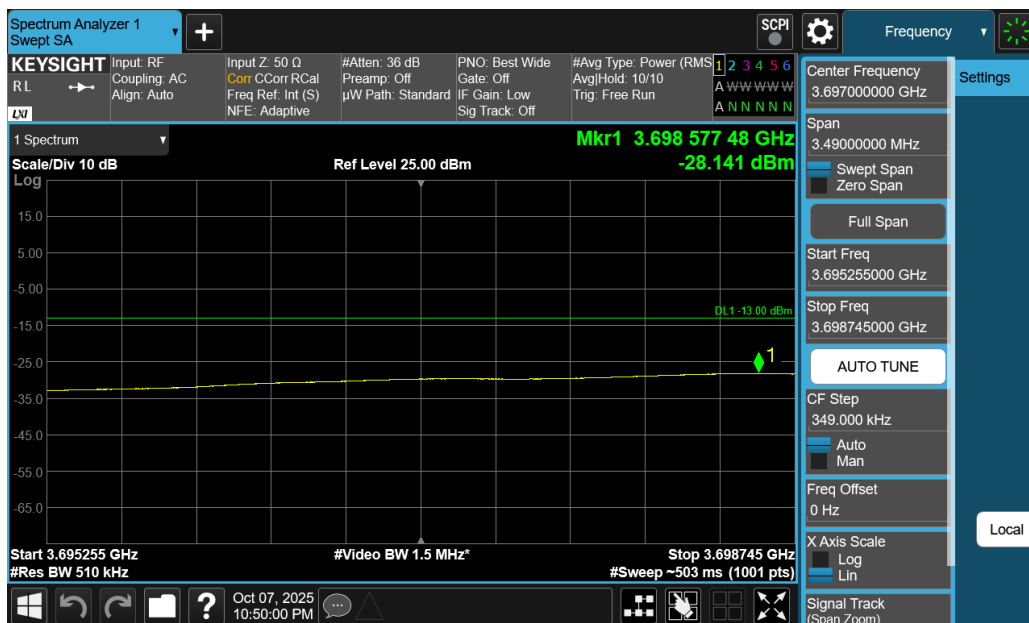
Plot 7-260. Extended Lower Band Edge Plot (NR Band n77 C-Band - 70MHz DFT-s-OFDM QPSK – Full RB)
