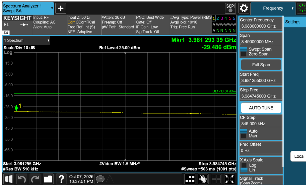
Plot 7-251. Extended Upper Band Edge Plot (NR Band n77 C-Band - 50MHz DFT-s-OFDM QPSK – Full RB)
