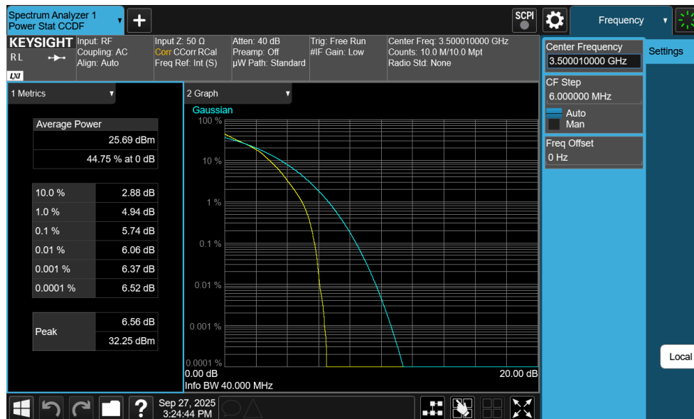
Plot 7-310. PAR Plot (NR Band n77 DoD-Band - 40MHz DFT-s-OFDM 16-QAM - Full RB)
