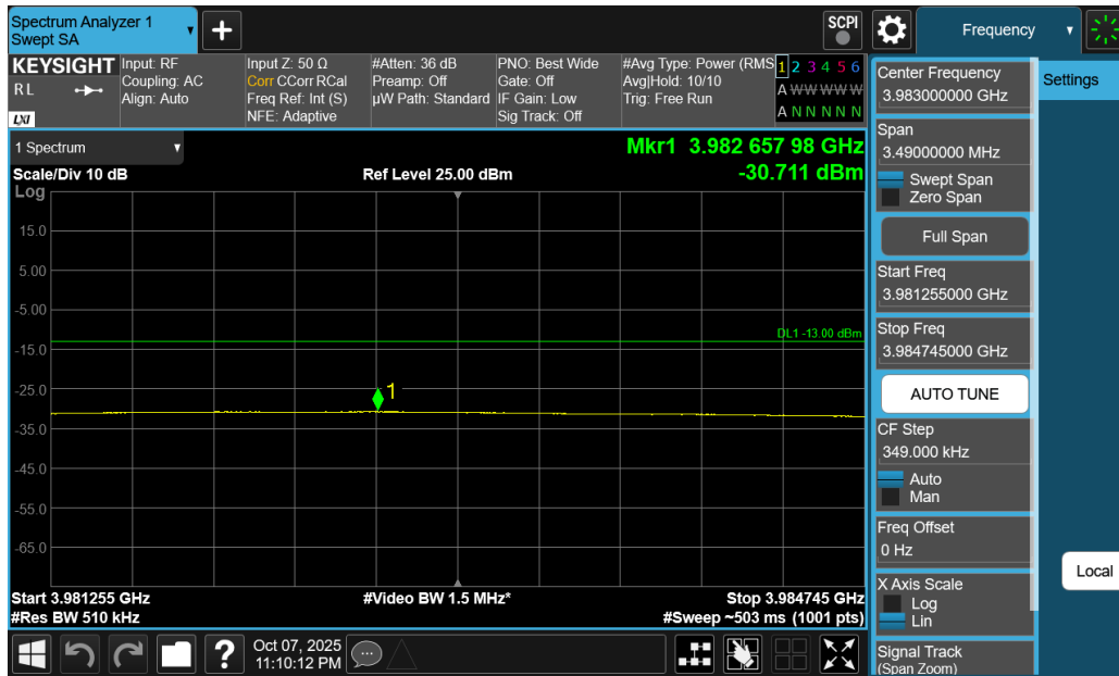
Plot 7-275. Extended Upper Band Edge Plot (NR Band n77 C-Band - 90MHz DFT-s-OFDM QPSK – Full RB)
