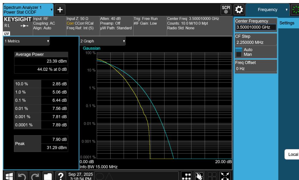
Plot 7-292. PAR Plot (NR Band n77 DoD-Band - 15MHz DFT-s-OFDM 256-QAM - Full RB)
