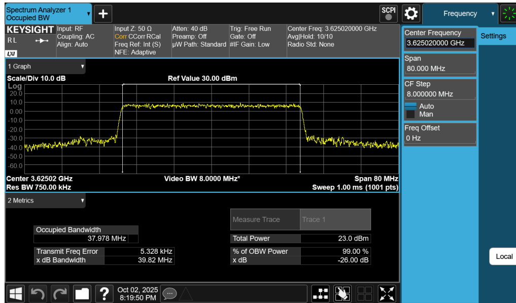
Plot 7-55. Occupied Bandwidth Plot (NR Band n48 - 40MHz CP-OFDM 16-QAM - Full RB Configuration)
