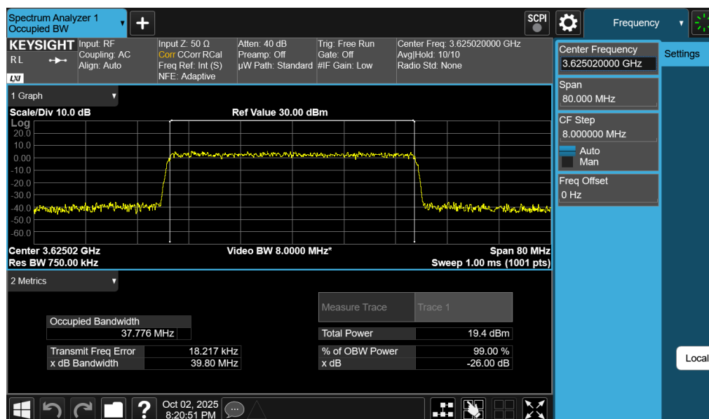
Plot 7-57. Occupied Bandwidth Plot (NR Band n48 - 40MHz CP-OFDM 256-QAM - Full RB Configuration)
