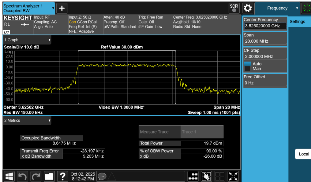
Plot 7-37. Occupied Bandwidth Plot (NR Band n48 - 10MHz CP-OFDM 256-QAM - Full RB Configuration)
