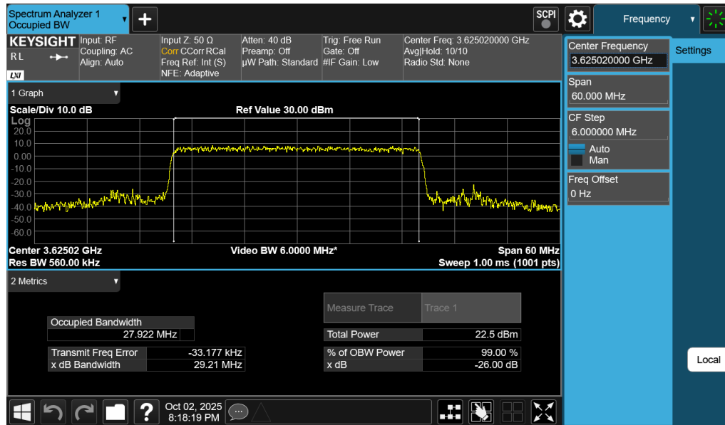
Plot 7-51. Occupied Bandwidth Plot (NR Band n48 - 30MHz CP-OFDM 64-QAM - Full RB Configuration)
