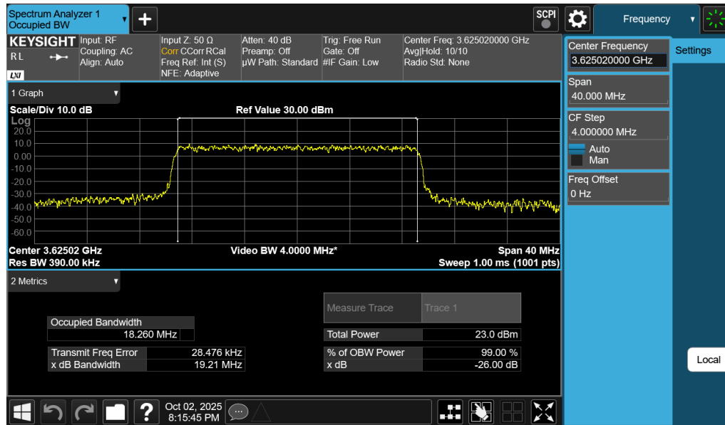
Plot 7-45. Occupied Bandwidth Plot (NR Band n48 - 20MHz CP-OFDM 16-QAM - Full RB Configuration)
