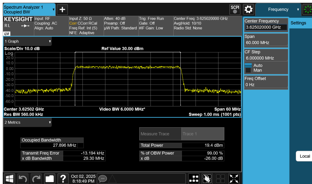
Plot 7-52. Occupied Bandwidth Plot (NR Band n48 - 30MHz CP-OFDM 256-QAM - Full RB Configuration)
