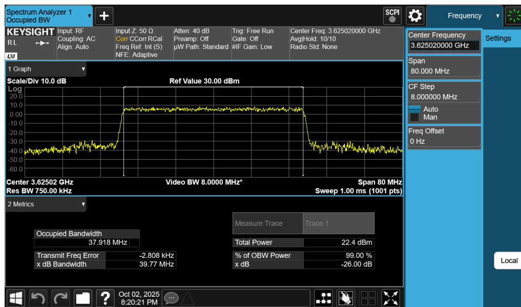
Plot 7-56. Occupied Bandwidth Plot (NR Band n48 - 40MHz CP-OFDM 64-QAM - Full RB Configuration)
