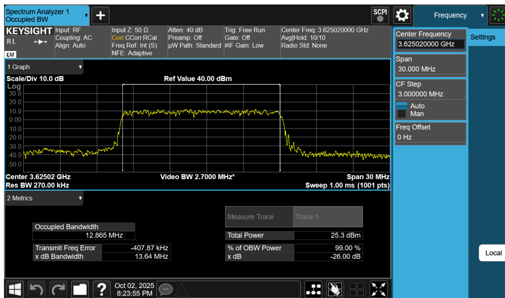
Plot 7-38. Occupied Bandwidth Plot (NR Band n48 - 15MHz DFT-s-OFDM \pi/2 BPSK - Full RB Configuration)
