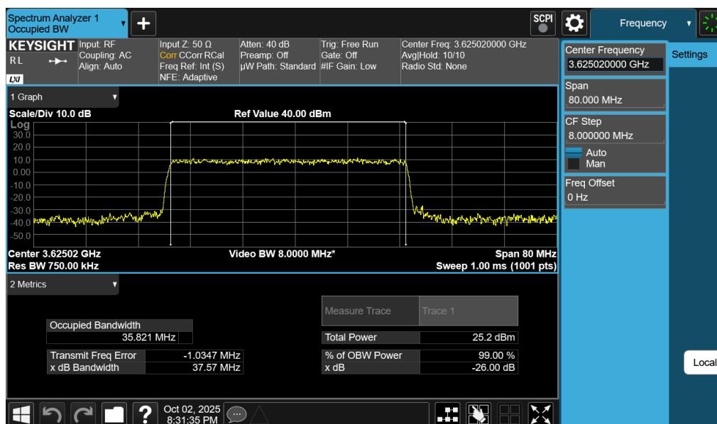
Plot 7-53. Occupied Bandwidth Plot (NR Band n48 - 40MHz DFT-s-OFDM \pi/2 BPSK - Full RB Configuration)
