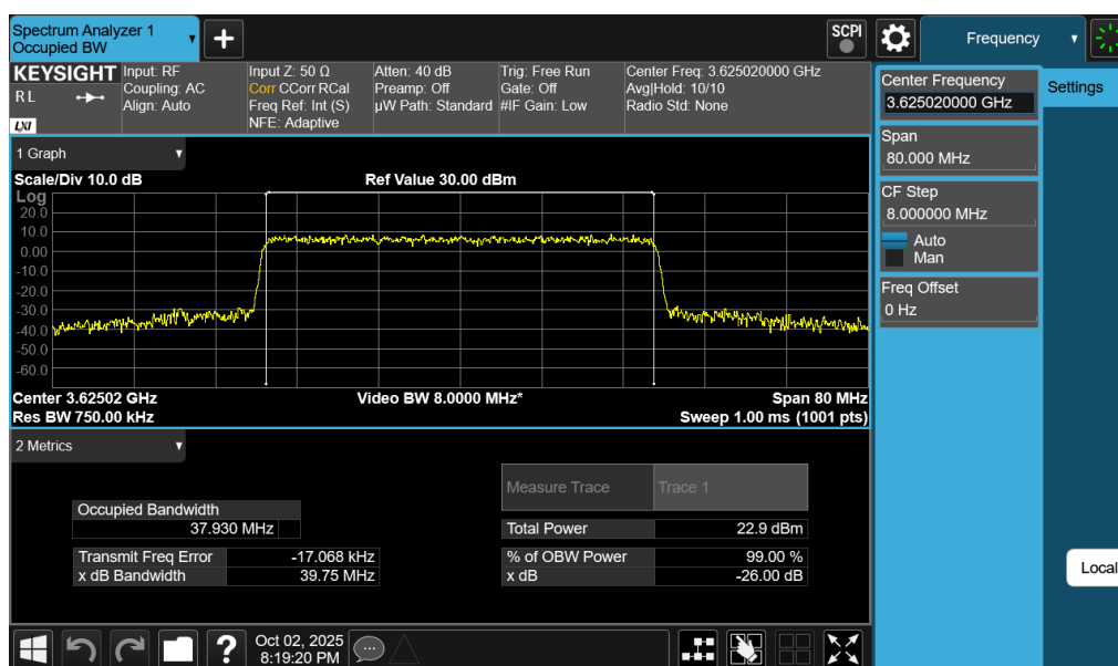
Plot 7-54. Occupied Bandwidth Plot (NR Band n48 - 40MHz CP-OFDM QPSK - Full RB Configuration)
