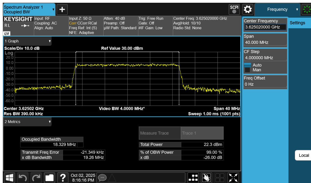
Plot 7-46. Occupied Bandwidth Plot (NR Band n48 - 20MHz CP-OFDM 64-QAM - Full RB Configuration)
