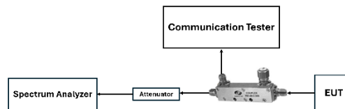
Figure 7-5. LTE Test Instrument & Measurement Setup
