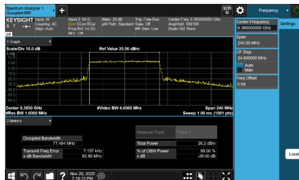
Plot 7-59 26dB BW & 99% OBW Antenna 1b (80MHz BW 802.11be(SU) - Ch.87)
