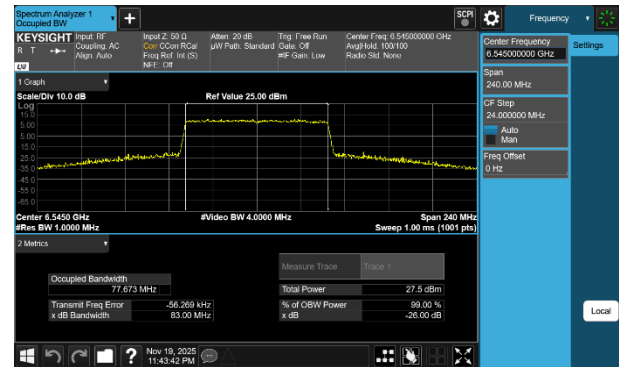
Plot 7-11 26dB BW & 99% OBW Antenna 3c (80MHz BW 802.11be(SU) - Ch.119)
