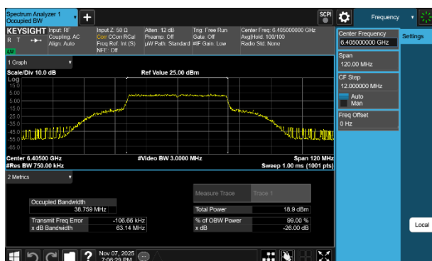
Plot 7-14 26dB BW & 99% OBW Antenna 3c (40MHz BW 802.11be(SU) - Ch.91)
