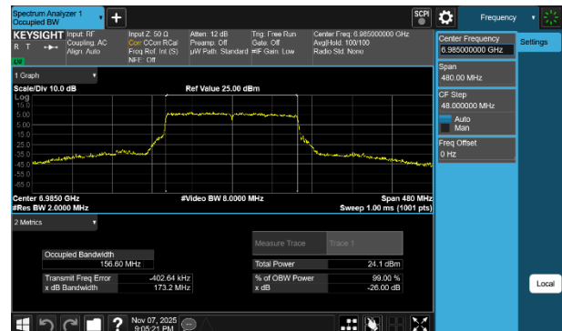
Plot 7-28 26dB BW & 99% OBW Antenna 3c (160MHz BW 802.11be(SU) - Ch.207)
