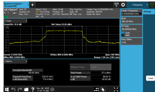
Plot 7-44 26dB BW & 99% OBW Antenna 3a (160MHz BW 802.11be(SU) - Ch.79)
