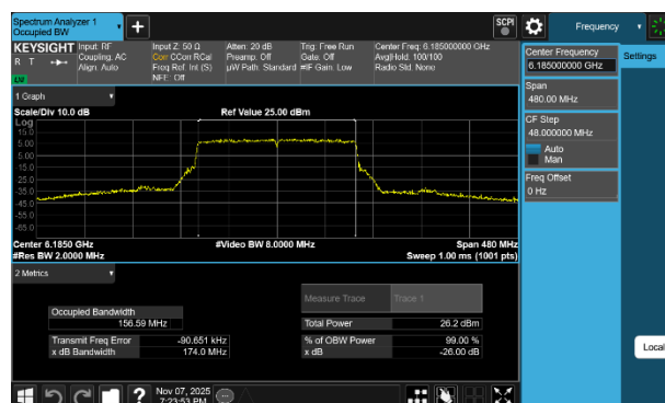
Plot 7-16 26dB BW & 99% OBW Antenna 3c (160MHz BW 802.11be(SU) - Ch.47)
