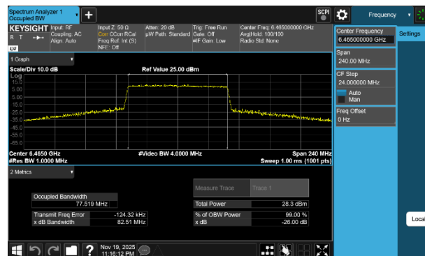
Plot 7-7 26dB BW & 99% OBW Antenna 3c (80MHz BW 802.11be(SU) - Ch.103)
