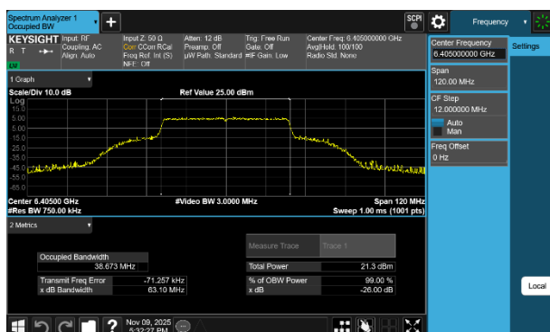
Plot 7-70 26dB BW & 99% OBW Antenna 1b (40MHz BW 802.11be(SU) - Ch.91)
