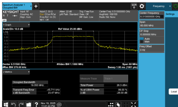
Plot 7-5 26dB BW & 99% OBW Antenna 3c (20MHz BW 802.11be(SU) - Ch.113)
