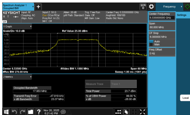
Plot 7-65 26dB BW & 99% OBW Antenna 1b (20MHz BW 802.11a - Ch.117)
