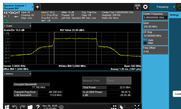
Plot 7-71 26dB BW & 99% OBW Antenna 1b (80MHz BW 802.11be(SU) - Ch.7)
