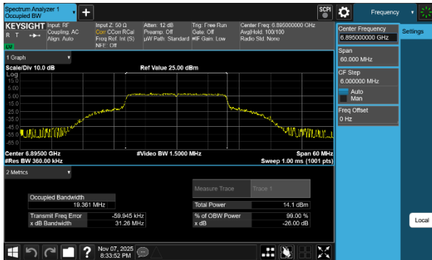
Plot 7-25 26dB BW & 99% OBW Antenna 3c (20MHz BW 802.11be(SU) - Ch.189)
