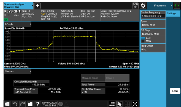
Plot 7-20 26dB BW & 99% OBW Antenna 3c (160MHz BW 802.11be(SU) - Ch.111)
