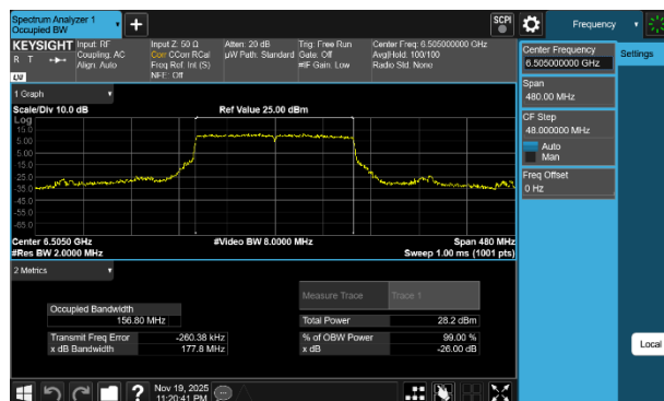
Plot 7-8 26dB BW & 99% OBW Antenna 3c (160MHz BW 802.11be(SU) - Ch.111)
