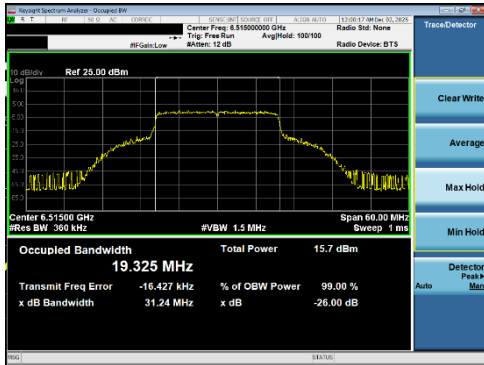
Plot 7-17 26dB BW & 99% OBW Antenna 3c (20MHz BW 802.11be(SU) - Ch.113)
