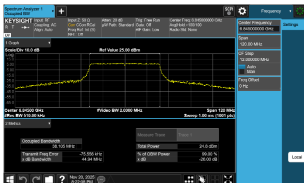
Plot 7-66 26dB BW & 99% OBW Antenna 1b (40MHz BW 802.11be(SU) - Ch.179)
