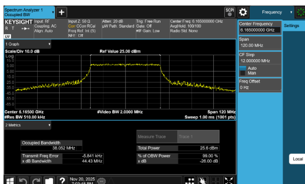
Plot 7-58 26dB BW & 99% OBW Antenna 1b (40MHz BW 802.11be(SU) - Ch.43)
