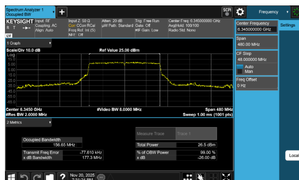
Plot 7-60 26dB BW & 99% OBW Antenna 1b (160MHz BW 802.11be(SU) - Ch.79)
