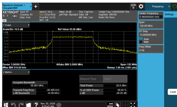
Plot 7-30 26dB BW & 99% OBW Antenna 3a (40MHz BW 802.11be(SU) - Ch.3)
