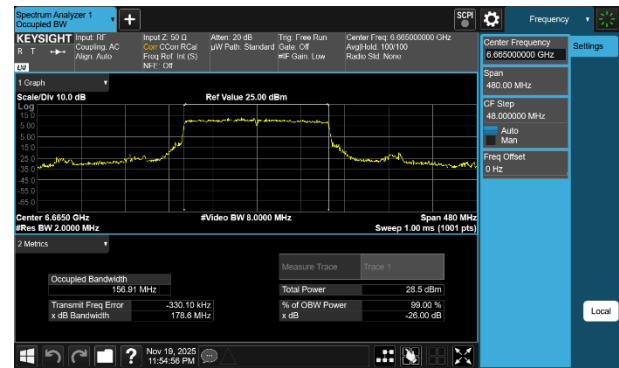
Plot 7-12 26dB BW & 99% OBW Antenna 3c (160MHz BW 802.11be(SU) - Ch.143)
