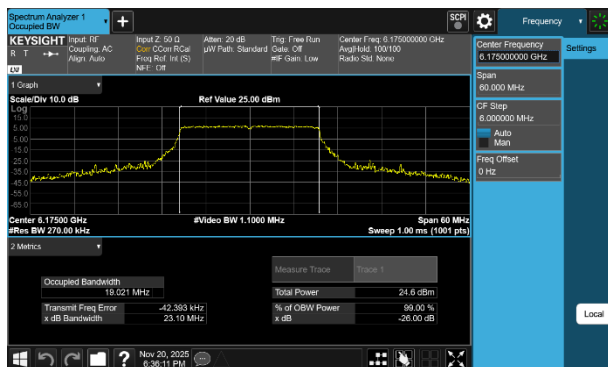
Plot 7-57 26dB BW & 99% OBW Antenna 1b (20MHz BW 802.11be(SU) - Ch.45)
