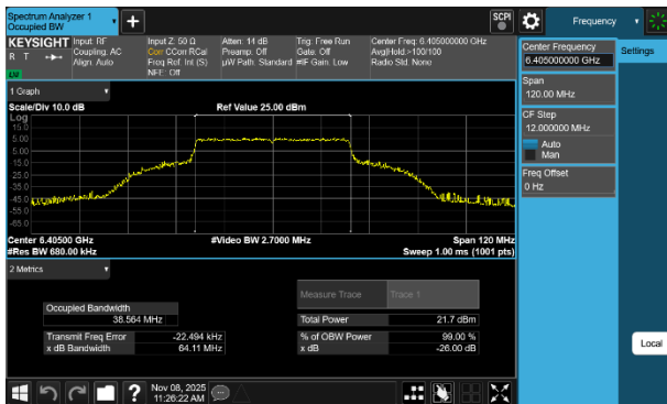
Plot 7-42 26dB BW & 99% OBW Antenna 3a (40MHz BW 802.11be(SU) - Ch.91)
