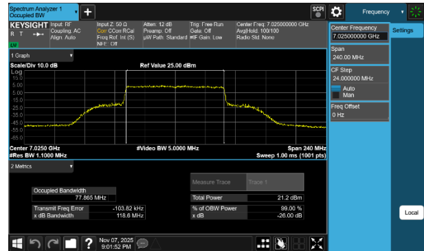
Plot 7-27 26dB BW & 99% OBW Antenna 3c (80MHz BW 802.11be(SU) - Ch.215)
