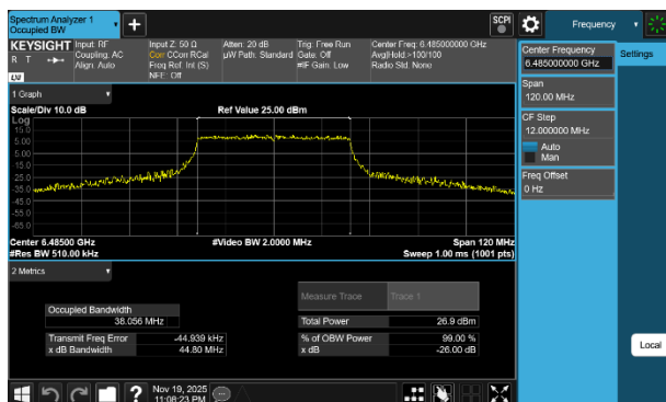
Plot 7-6 26dB BW & 99% OBW Antenna 3c (40MHz BW 802.11be(SU) - Ch.107)
