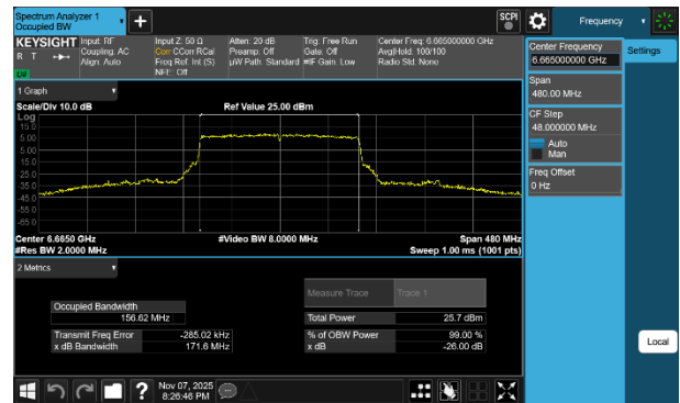
Plot 7-24 26dB BW & 99% OBW Antenna 3c (160MHz BW 802.11be(SU) - Ch.143)
