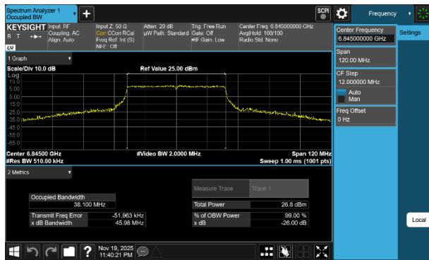
Plot 7-10 26dB BW & 99% OBW Antenna 3c (40MHz BW 802.11be(SU) - Ch.179)
