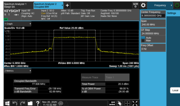
Plot 7-19 26dB BW & 99% OBW Antenna 3a (80MHz BW 802.11be(SU) - Ch.87)
