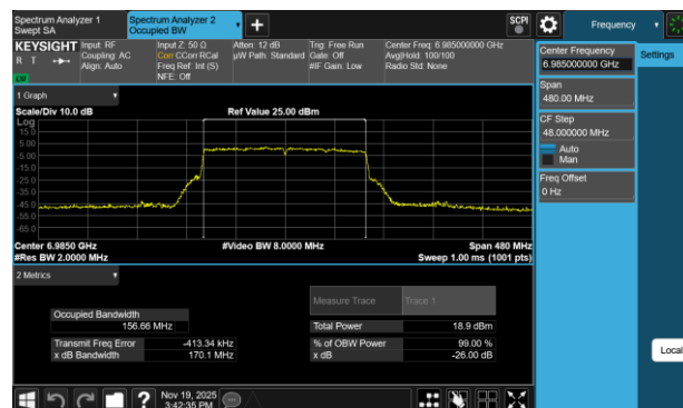
Plot 7-16 26dB BW & 99% OBW Antenna 3c (160MHz BW 802.11be(SU) - Ch.207)
