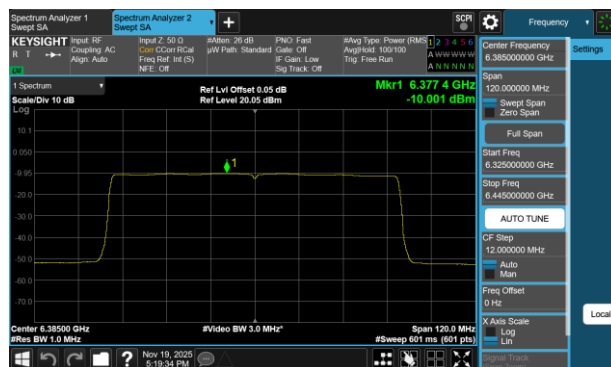
Plot 7-51 PSD Antenna 3c (80MHz BW 802.11be(SU) - Ch.87)
