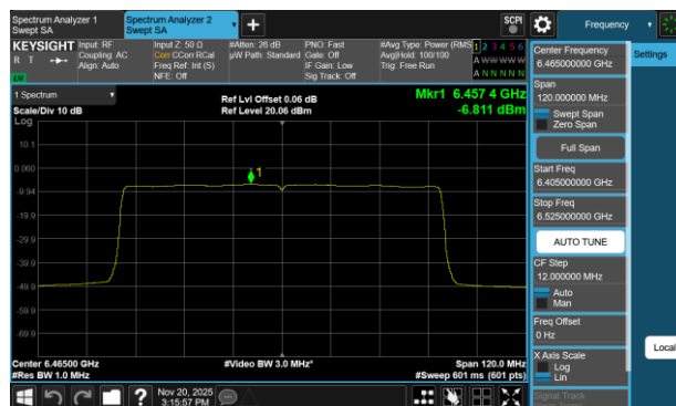
Plot 7-71 PSD Antenna 3a (80MHz BW 802.11be(SU) - Ch.103)
