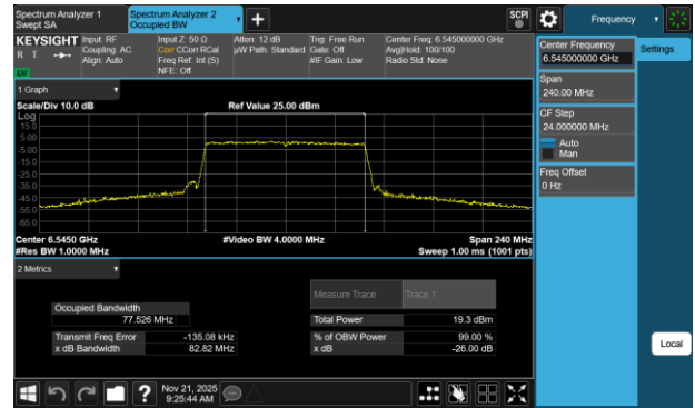
Plot 7-43 26dB BW & 99% OBW Antenna 1b (80MHz BW 802.11be(SU) - Ch.119)
