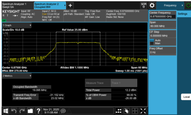
Plot 7-41 26dB BW & 99% OBW Antenna 1b (20MHz BW 802.11be(SU) - Ch.185)
