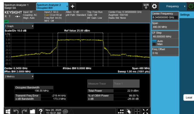
Plot 7-20 26dB BW & 99% OBW Antenna 3a (160MHz BW 802.11be(SU) - Ch.79)
