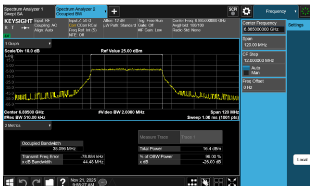
Plot 7-46 26dB BW & 99% OBW Antenna 1b (40MHz BW 802.11be(SU) - Ch.187)
