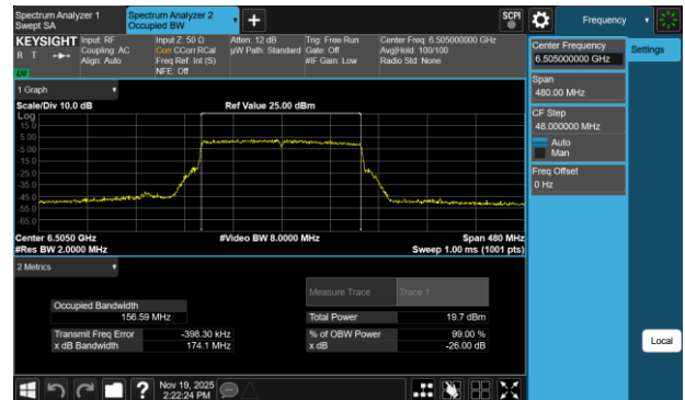
Plot 7-8 26dB BW & 99% OBW Antenna 3c (160MHz BW 802.11be(SU) - Ch.111)
