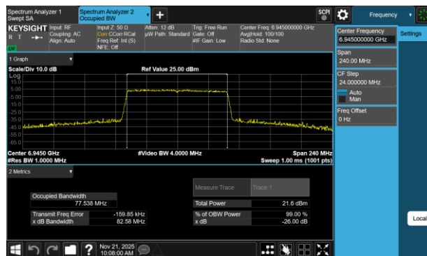
Plot 7-47 26dB BW & 99% OBW Antenna 1b (80MHz BW 802.11be(SU) - Ch.199)
