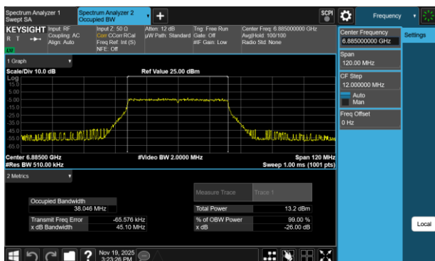
Plot 7-14 26dB BW & 99% OBW Antenna 3c (40MHz BW 802.11be(SU) - Ch.187)
