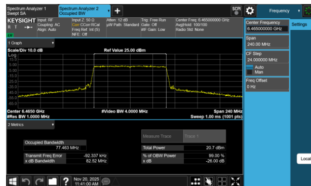
Plot 7-23 26dB BW & 99% OBW Antenna 3a (80MHz BW 802.11be(SU) - Ch.103)
