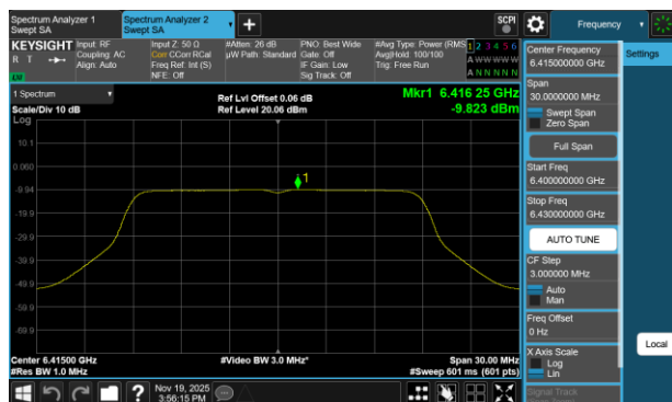
Plot 7-49 PSD Antenna 3c (20MHz BW 802.11a - Ch.93)
