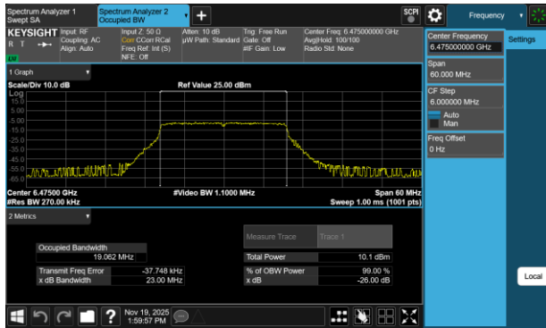
Plot 7-5 26dB BW & 99% OBW Antenna 3c (20MHz BW 802.11be(SU) - Ch.105)
