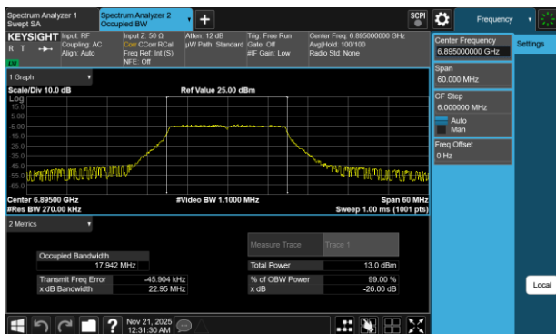
Plot 7-45 26dB BW & 99% OBW Antenna 1b (20MHz BW 802.11a - Ch.189)
