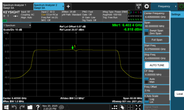
Plot 7-66 PSD Antenna 3a (40MHz BW 802.11be(SU) - Ch.91)
