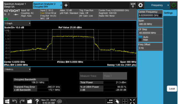
Plot 7-44 26dB BW & 99% OBW Antenna 1b (160MHz BW 802.11be(SU) - Ch.175)
