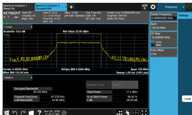
Plot 7-22 26dB BW & 99% OBW Antenna 3a (40MHz BW 802.11be(SU) - Ch.107)
