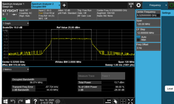
Plot 7-6 26dB BW & 99% OBW Antenna 3c (40MHz BW 802.11be(SU) - Ch.115)
