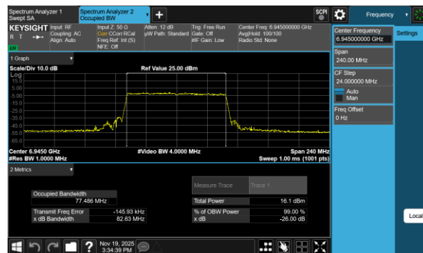
Plot 7-15 26dB BW & 99% OBW Antenna 3c (80MHz BW 802.11be(SU) - Ch.199)
