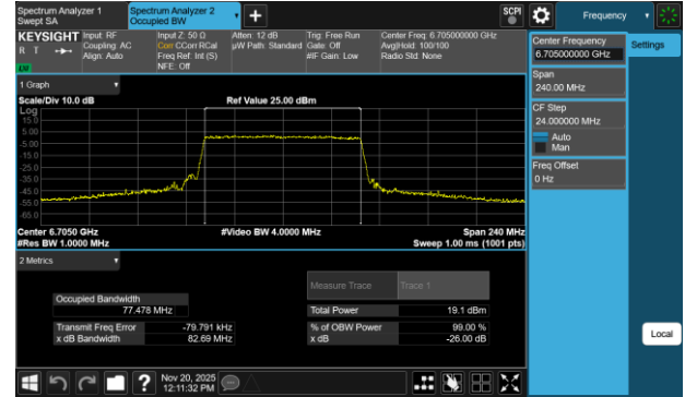
Plot 7-27 26dB BW & 99% OBW Antenna 3a (80MHz BW 802.11be(SU) - Ch.151)
