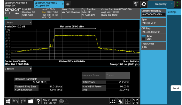
Plot 7-39 26dB BW & 99% OBW Antenna 1b (80MHz BW 802.11be(SU) - Ch.103)
