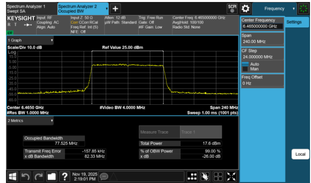
Plot 7-7 26dB BW & 99% OBW Antenna 3c (80MHz BW 802.11be(SU) - Ch.103)
