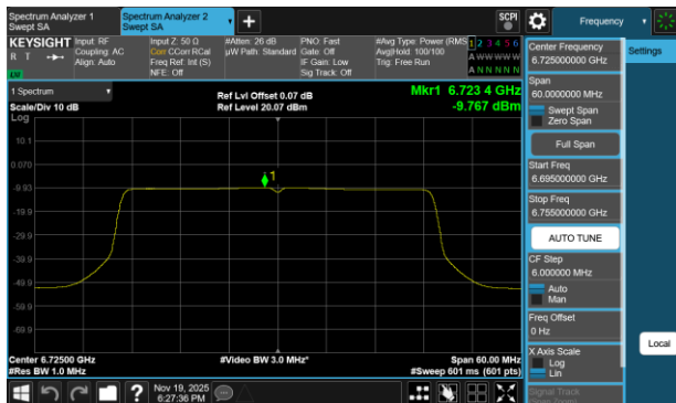
Plot 7-58 PSD Antenna 3c (40MHz BW 802.11be(SU) - Ch.155)
