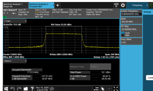
Plot 7-11 26dB BW & 99% OBW Antenna 3c (80MHz BW 802.11be(SU) - Ch.183)
