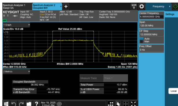
Plot 7-10 26dB BW & 99% OBW Antenna 3c (40MHz BW 802.11be(SU) - Ch.123)
