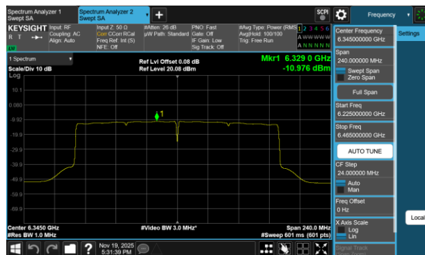
Plot 7-52 PSD Antenna 3c (160MHz BW 802.11be(SU) - Ch.79)
