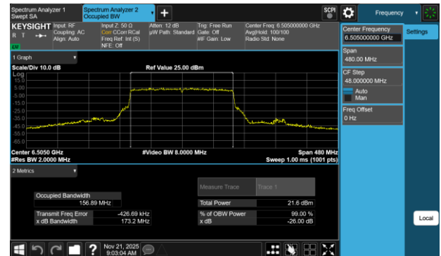
Plot 7-40 26dB BW & 99% OBW Antenna 1b (160MHz BW 802.11be(SU) - Ch.111)
