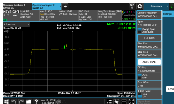
Plot 7-59 PSD Antenna 3c (80MHz BW 802.11be(SU) - Ch.151)
