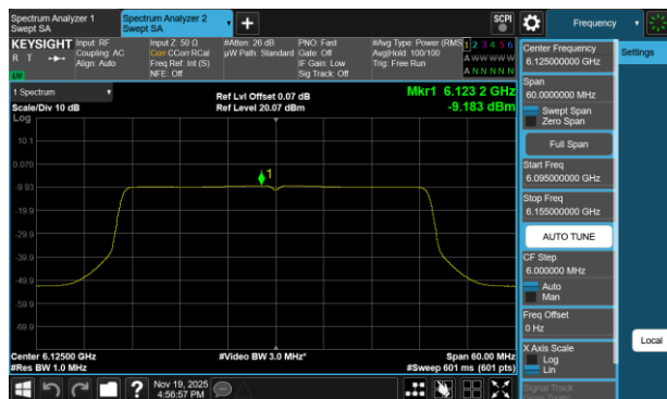
Plot 7-50 PSD Antenna 3c (40MHz BW 802.11be(SU) - Ch.35)
