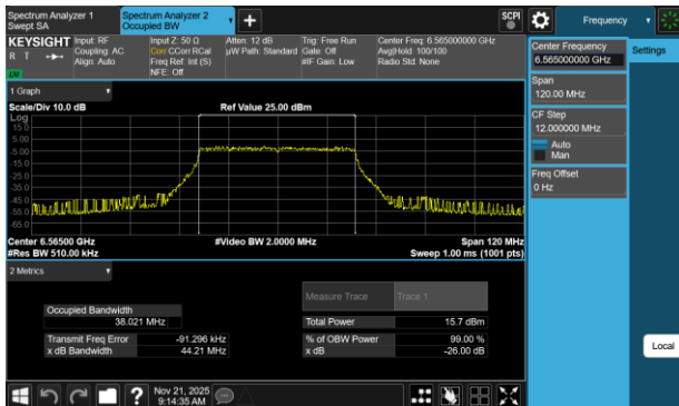
Plot 7-42 26dB BW & 99% OBW Antenna 1b (40MHz BW 802.11be(SU) - Ch.123)
