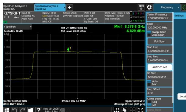
Plot 7-67 PSD Antenna 3a (80MHz BW 802.11be(SU) - Ch.87)
