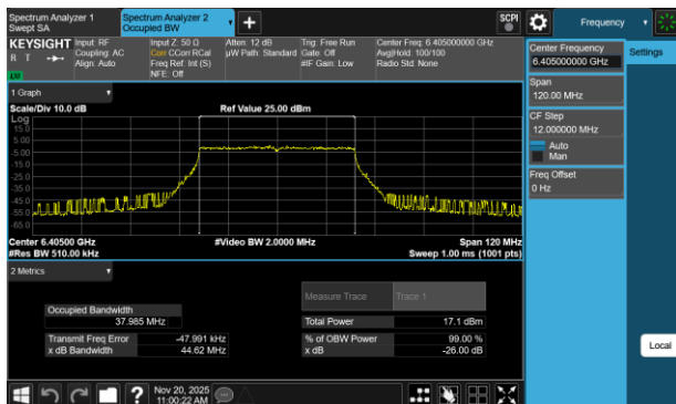
Plot 7-18 26dB BW & 99% OBW Antenna 3a (40MHz BW 802.11be(SU) - Ch.91)
