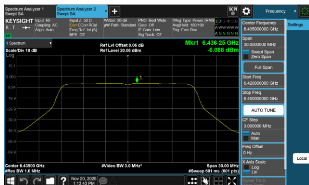
Plot 7-69 PSD Antenna 3a (20MHz BW 802.11a - Ch.97)
