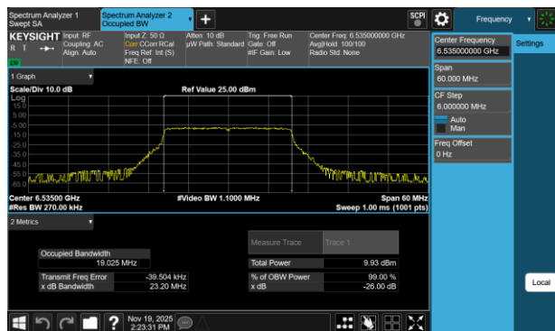
Plot 7-9 26dB BW & 99% OBW Antenna 3c (20MHz BW 802.11be(SU) - Ch.117)
