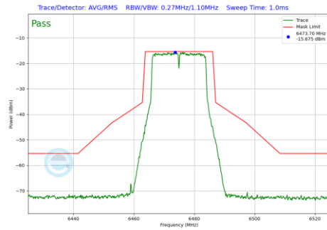
Plot 7-165 In-Band Emission Plot Antenna 3c (20MHz BW 802.11a (UNII Band 6) - Ch.105)
