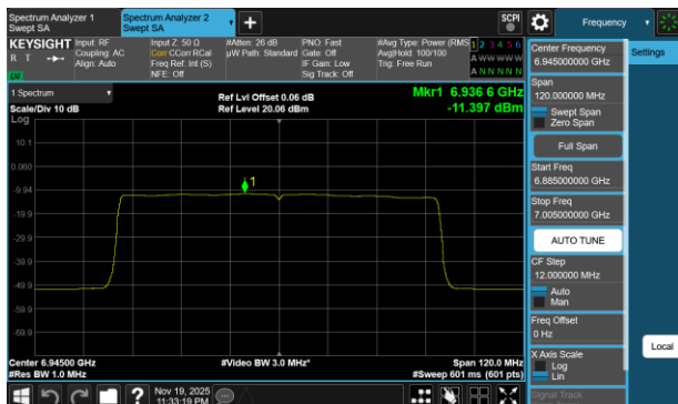
Plot 7-123 PSD SDM Primary Antenna 3c (80MHz BW 802.11be(SU) - Ch.199)
