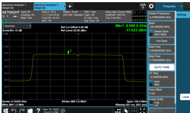
Plot 7-147 PSD CDD Diversity Antenna 3c (80MHz BW 802.11be(SU) - Ch.151)
