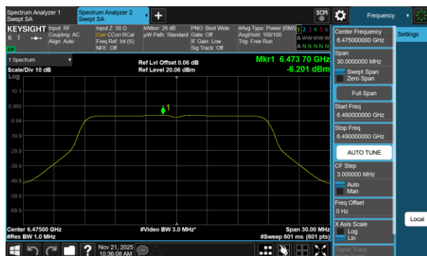
Plot 7-85 PSD Antenna 1b (20MHz BW 802.11a - Ch.105)
