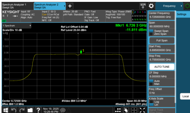
Plot 7-146 PSD CDD Diversity Antenna 3c (40MHz BW 802.11be(SU) - Ch.155)
