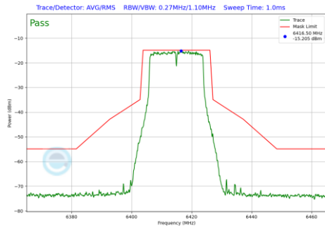
Plot 7-161 In-Band Emission Plot Antenna 3c (20MHz BW 802.11a (UNII Band 5) - Ch.93)
