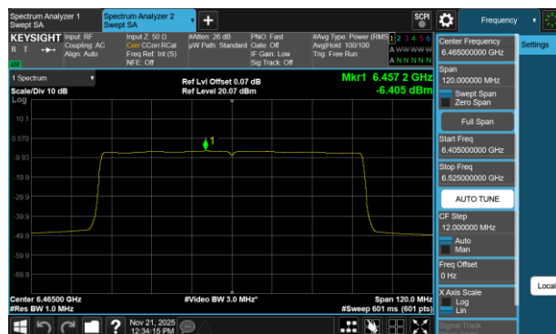
Plot 7-87 PSD Antenna 1b (80MHz BW 802.11be(SU) - Ch.103)
