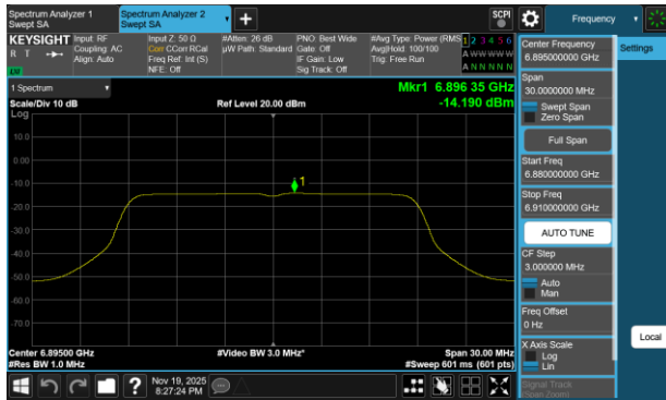
Plot 7-121 PSD CDD Primary Antenna 3c (20MHz BW 802.11a - Ch.189)
