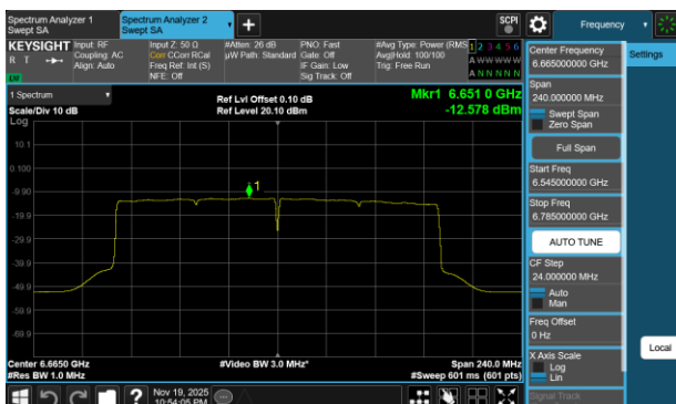
Plot 7-116 PSD SDM Primary Antenna 3c (160MHz BW 802.11be(SU) - Ch.143)
