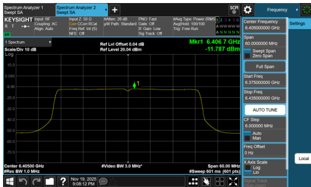
Plot 7-130 PSD CDD Diversity Antenna 3c (40MHz BW 802.11be(SU) - Ch.91)
