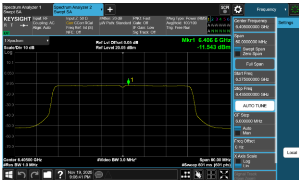
Plot 7-98 PSD SDM Primary Antenna 3c (40MHz BW 802.11be(SU) - Ch.91)
