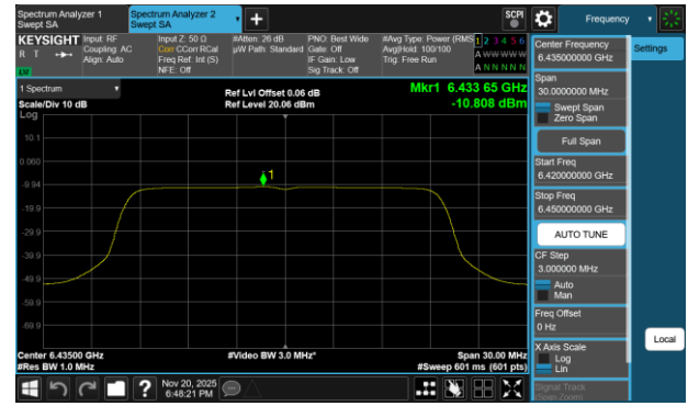
Plot 7-109 PSD SDM Primary Antenna 3a (20MHz BW 802.11be(SU) - Ch.97)
