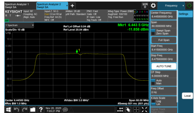
Plot 7-110 PSD SDM Primary Antenna 3a (40MHz BW 802.11be(SU) - Ch.99)
