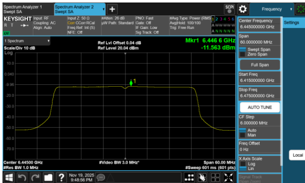
Plot 7-106 PSD SDM Primary Antenna 3c (40MHz BW 802.11be(SU) - Ch.99)
