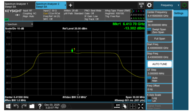
Plot 7-133 PSD CDD Diversity Antenna 1b (20MHz BW 802.11a - Ch.93)
