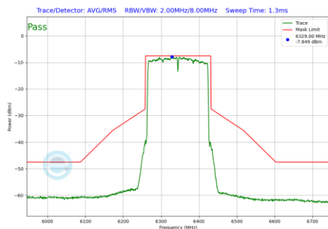
Plot 7-164 In-Band Emission Plot Antenna 3c (160MHz BW 802.11be(SU) (UNII Band 5) - Ch.79)
