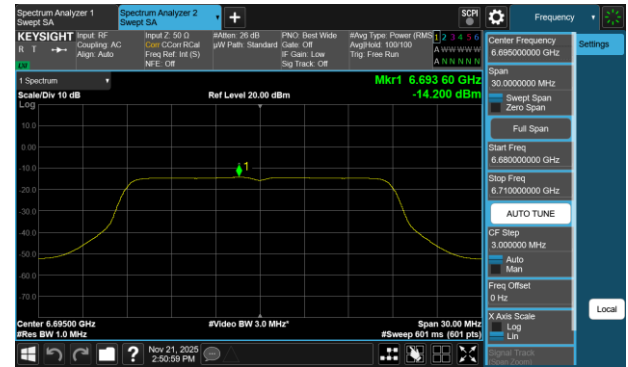
Plot 7-149 PSD CDD Diversity Antenna 1b (20MHz BW 802.11a - Ch.149)
