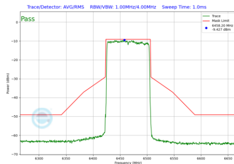
Plot 7-167 In-Band Emission Plot Antenna 3c (80MHz BW 802.11be(SU) (UNII Band 6) - Ch.103)
