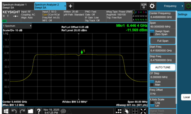
Plot 7-138 PSD CDD Diversity Antenna 3c (40MHz BW 802.11be(SU) - Ch.99)
