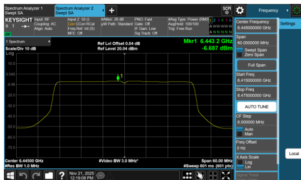
Plot 7-86 PSD Antenna 1b (40MHz BW 802.11be(SU) - Ch.99)
