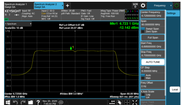
Plot 7-118 PSD SDM Primary Antenna 3a (40MHz BW 802.11be(SU) - Ch.155)
