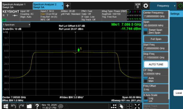
Plot 7-122 PSD SDM Primary Antenna 3c (40MHz BW 802.11be(SU) - Ch.227)
