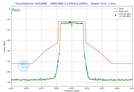
Plot 7-166 In-Band Emission Plot Antenna 3c (40MHz BW 802.11be(SU) (UNII Band 6) - Ch.115)
