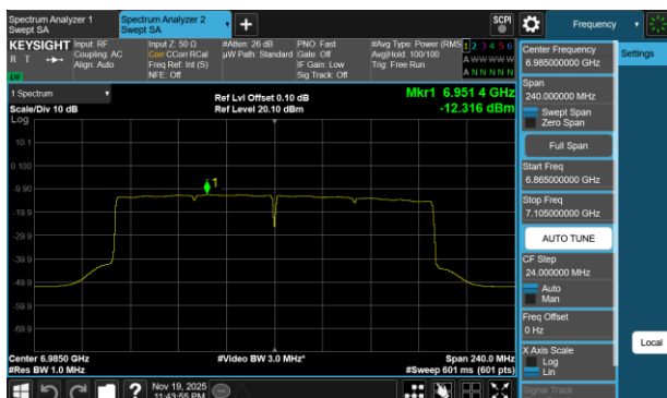
Plot 7-124 PSD SDM Primary Antenna 3c (160MHz BW 802.11be(SU) - Ch.207)
