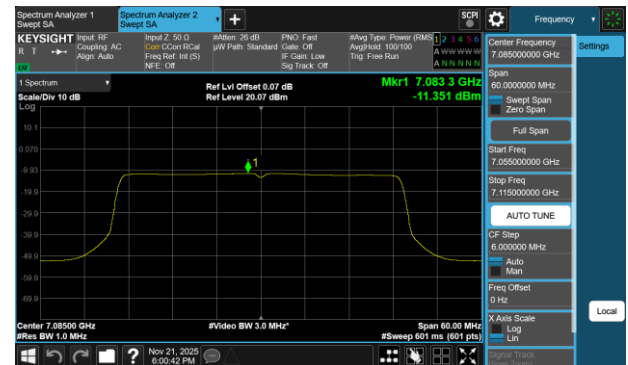
Plot 7-158 PSD CDD Diversity Antenna 1b (40MHz BW 802.11be(SU) - Ch.227)
