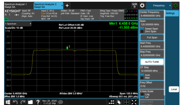
Plot 7-111 PSD SDM Primary Antenna 3a (80MHz BW 802.11be(SU) - Ch.103)
