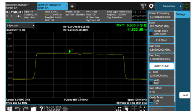
Plot 7-159 PSD CDD Diversity Antenna 1b (80MHz BW 802.11be(SU) - Ch.199)
