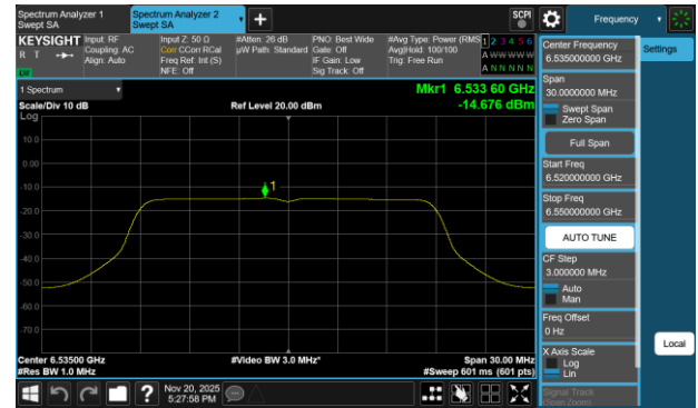
Plot 7-117 PSD CDD Primary Antenna 3a (20MHz BW 802.11a - Ch.117)
