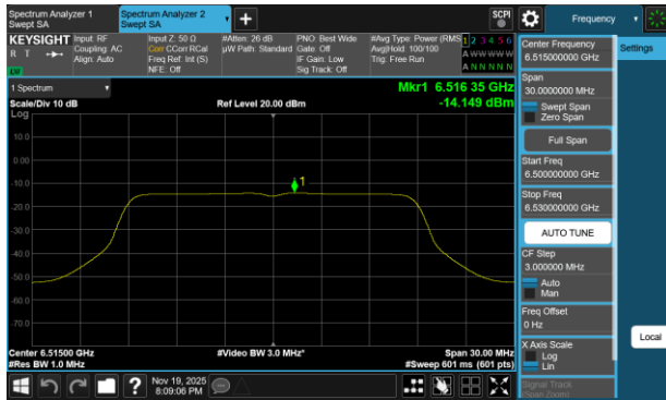
Plot 7-137 PSD CDD Diversity Antenna 3c (20MHz BW 802.11a - Ch.113)
