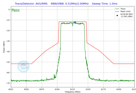
Plot 7-162 In-Band Emission Plot Antenna 3c (40MHz BW 802.11be(SU) (UNII Band 5) - Ch.35)
