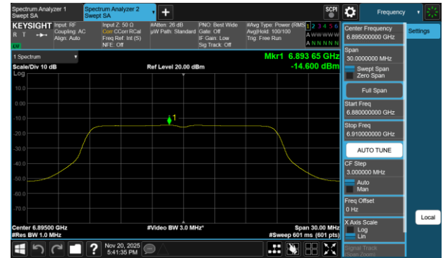
Plot 7-125 PSD CDD Primary Antenna 3a (20MHz BW 802.11a - Ch.189)
