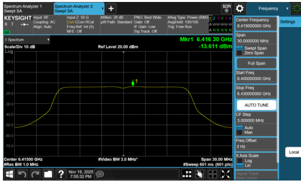
Plot 7-129 PSD CDD Diversity Antenna 3c (20MHz BW 802.11a - Ch.93)
