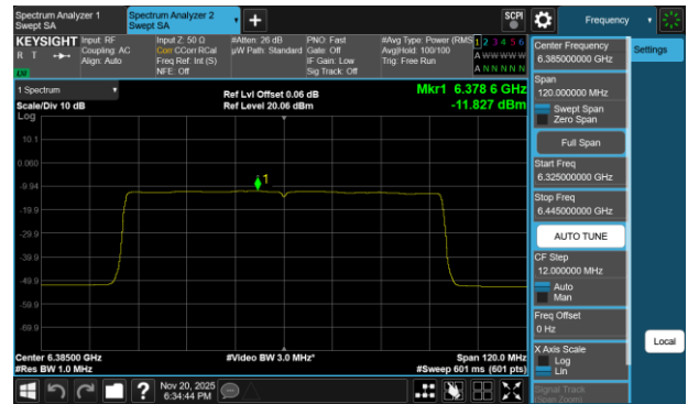
Plot 7-103 PSD SDM Primary Antenna 3a (80MHz BW 802.11be(SU) - Ch.87)
