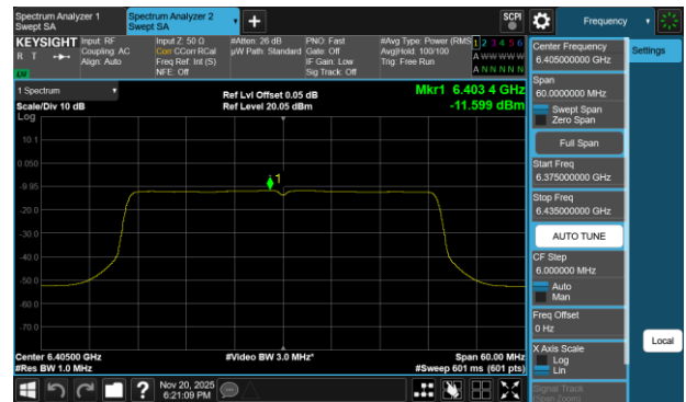
Plot 7-102 PSD SDM Primary Antenna 3a (40MHz BW 802.11be(SU) - Ch.91)
