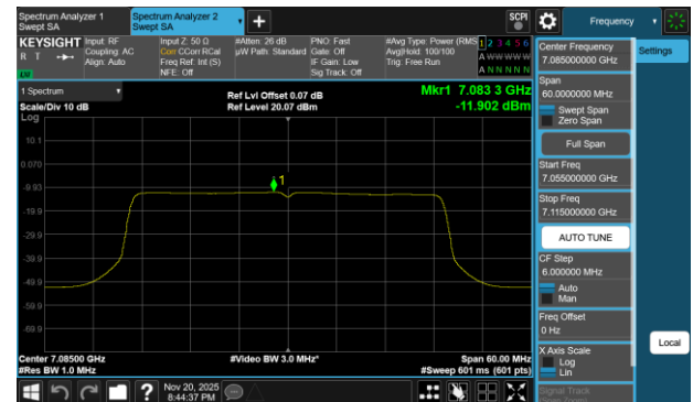
Plot 7-126 PSD SDM Primary Antenna 3a (40MHz BW 802.11be(SU) - Ch.227)
