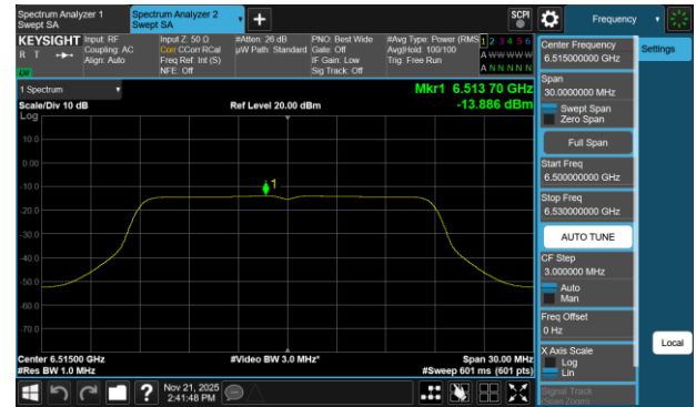
Plot 7-141 PSD CDD Diversity Antenna 1b (20MHz BW 802.11a - Ch.113)
