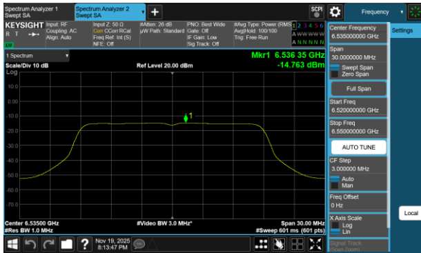
Plot 7-113 PSD CDD Primary Antenna 3c (20MHz BW 802.11a - Ch.117)
