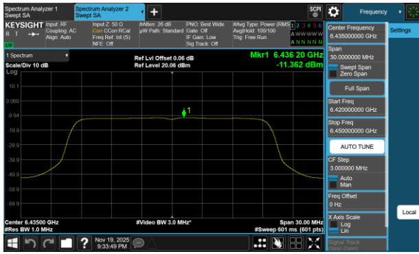
Plot 7-105 PSD SDM Primary Antenna 3c (20MHz BW 802.11be(SU) - Ch.97)
