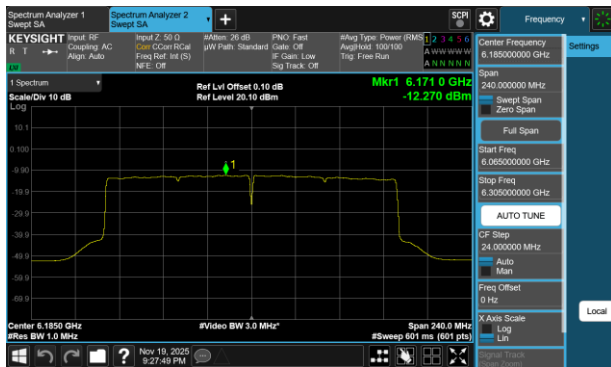
Plot 7-132 PSD CDD Diversity Antenna 3c (160MHz BW 802.11be(SU) - Ch.47)
