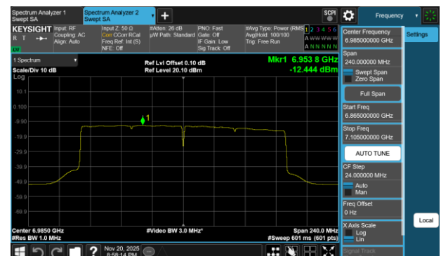
Plot 7-128 PSD SDM Primary Antenna 3a (160MHz BW 802.11be(SU) - Ch.207)
