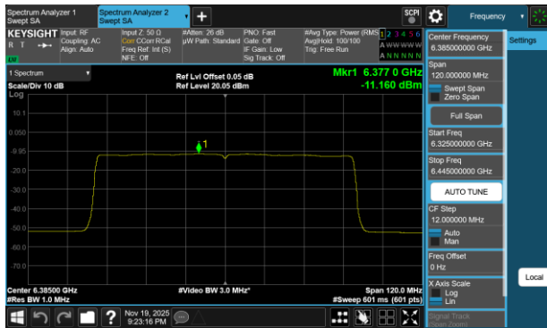
Plot 7-131 PSD CDD Diversity Antenna 3c (80MHz BW 802.11be(SU) - Ch.87)
