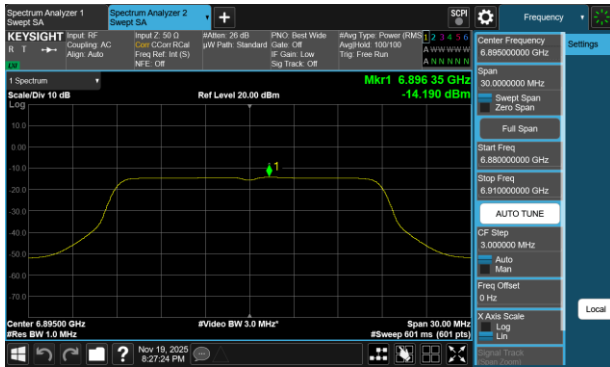
Plot 7-153 PSD CDD Diversity Antenna 3c (20MHz BW 802.11a - Ch.189)
