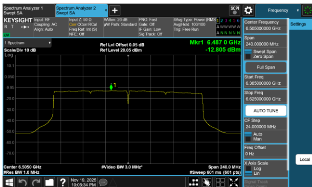
Plot 7-108 PSD SDM Primary Antenna 3c (160MHz BW 802.11be(SU) - Ch.111)
