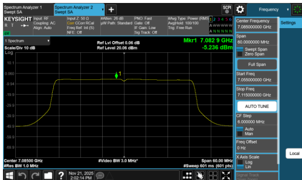
Plot 7-94 PSD Antenna 1b (40MHz BW 802.11be(SU) - Ch.227)
