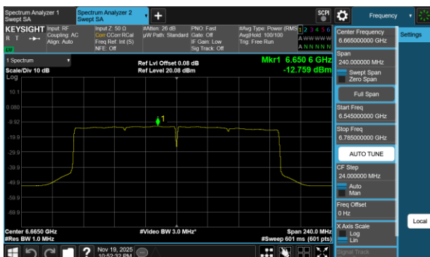
Plot 7-148 PSD CDD Diversity Antenna 3c (160MHz BW 802.11be(SU) - Ch.143)
