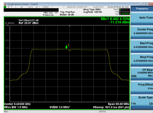
Plot 7-142 PSD CDD Diversity Antenna 1b (40MHz BW 802.11be(SU) - Ch.99)
