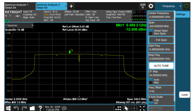
Plot 7-112 PSD SDM Primary Antenna 3a (160MHz BW 802.11be(SU) - Ch.111)
