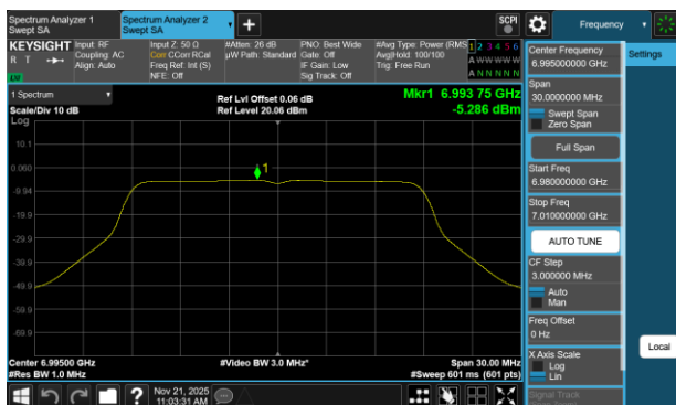
Plot 7-93 PSD Antenna 1b (20MHz BW 802.11a - Ch.209)
