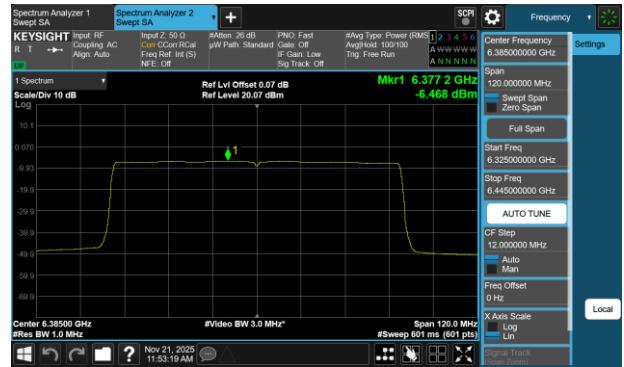
Plot 7-83 PSD Antenna 1b (80MHz BW 802.11b(SU) - Ch.87)
