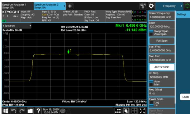
Plot 7-107 PSD SDM Primary Antenna 3c (80MHz BW 802.11be(SU) - Ch.103)
