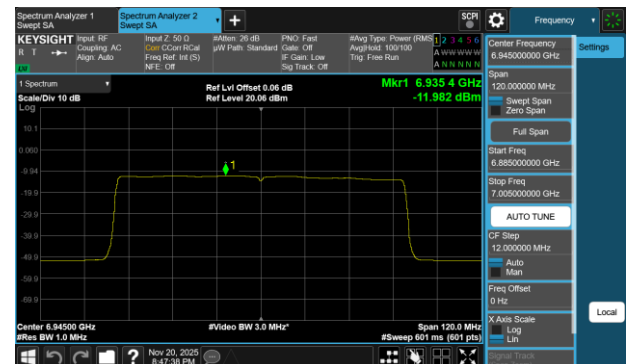
Plot 7-127 PSD SDM Primary Antenna 3a (80MHz BW 802.11be(SU) - Ch.199)
