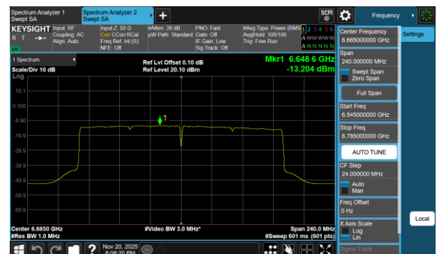
Plot 7-120 PSD SDM Primary Antenna 3a (160MHz BW 802.11be(SU) - Ch.143)
