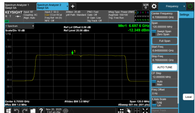
Plot 7-119 PSD SDM Primary Antenna 3a (80MHz BW 802.11be(SU) - Ch.151)
