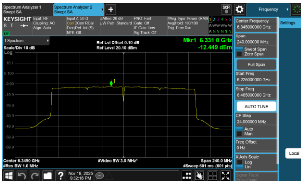
Plot 7-100 PSD SDM Primary Antenna 3c (160MHz BW 802.11be(SU) - Ch.79)
