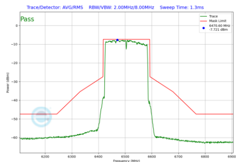
Plot 7-168 In-Band Emission Plot Antenna 3c (160MHz BW 802.11be(SU) (UNII Band 6) - Ch.111)
