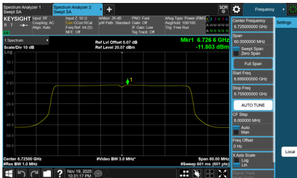
Plot 7-114 PSD SDM Primary Antenna 3c (40MHz BW 802.11be(SU) - Ch.155)
