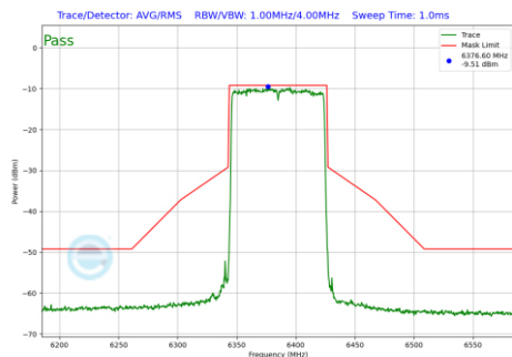
Plot 7-163 In-Band Emission Plot Antenna 3c (80MHz BW 802.11be(SU) (UNII Band 5) - Ch.87)
