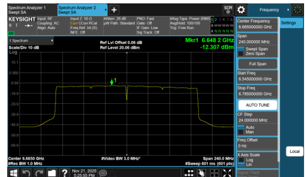
Plot 7-152 PSD CDD Diversity Antenna 1b (160MHz BW 802.11be(SU) - Ch.143)
