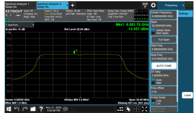
Plot 7-157 PSD CDD Diversity Antenna 1b (20MHz BW 802.11a - Ch.189)
