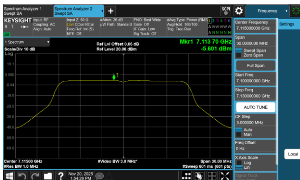
Plot 7-77 PSD Antenna 3a (20MHz BW 802.11a - Ch.233)
