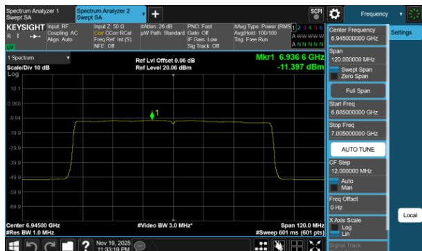
Plot 7-155 PSD CDD Diversity Antenna 3c (80MHz BW 802.11be(SU) - Ch.199)
