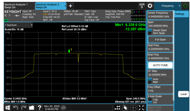
Plot 7-104 PSD SDM Primary Antenna 3a (160MHz BW 802.11be(SU) - Ch.79)
