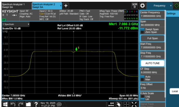
Plot 7-154 PSD CDD Diversity Antenna 3c (40MHz BW 802.11be(SU) - Ch.227)
