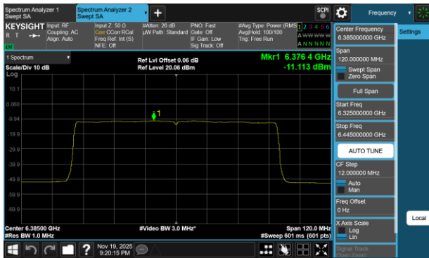
Plot 7-99 PSD SDM Primary Antenna 3c (80MHz BW 802.11be(SU) - Ch.87)
