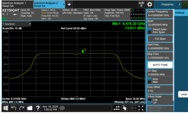
Plot 7-97 PSD CDD Primary Antenna 3c (20MHz BW 802.11a - Ch.93)
