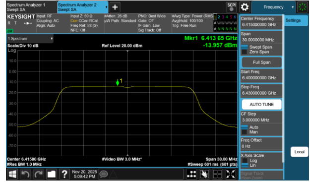
Plot 7-101 PSD CDD Primary Antenna 3a (20MHz BW 802.11a - Ch.93)
