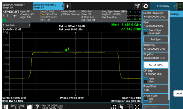
Plot 7-139 PSD CDD Diversity Antenna 3c (80MHz BW 802.11be(SU) - Ch.103)
