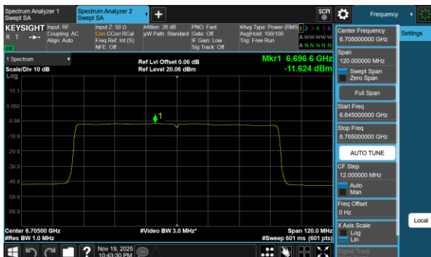
Plot 7-115 PSD SDM Primary Antenna 3c (80MHz BW 802.11be(SU) - Ch.151)
