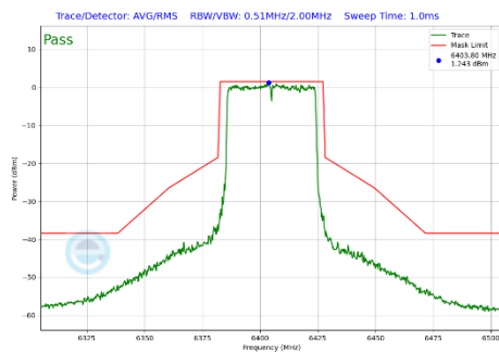
Plot 7-282 In-Band Emission Plot Antenna 3c (40MHz BW 802.11be(SU) (UNII Band 5) - Ch.91)
