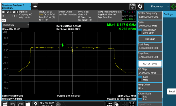
Plot 7-244 PSD CDD Diversity Antenna 3c (160MHz BW 802.11be(SU) - Ch.143)
