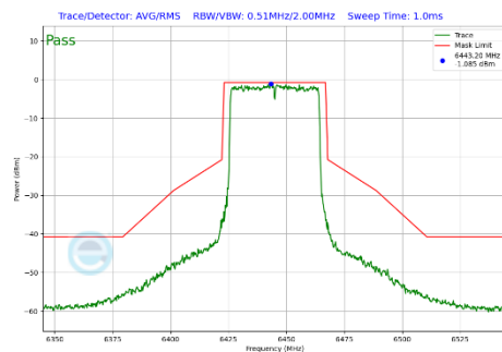
Plot 7-314 In-Band Emission Plot Antenna 3a (40MHz BW 802.11be(SU) (UNII Band 6) - Ch.99)
