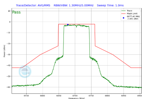
Plot 7-331 In-Band Emission Plot Antenna 3a (80MHz BW 802.11be(SU) (UNII Band 7) - Ch.151)
