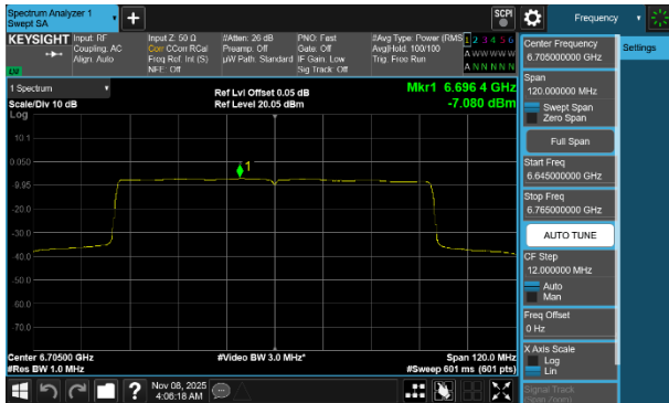
Plot 7-267 PSD CDD Diversity Antenna 3c (80MHz BW 802.11be(SU) - Ch.151)
