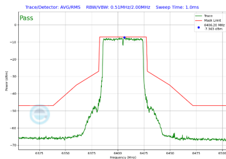
Plot 7-294 In-Band Emission Plot Antenna 3c (40MHz BW 802.11be(SU) (UNII Band 5) - Ch.91)
