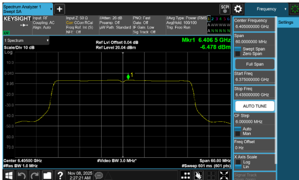
Plot 7-250 PSD CDD Diversity Antenna 3c (40MHz BW 802.11be(SU) - Ch.91)
