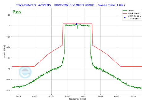
Plot 7-290 In-Band Emission Plot Antenna 3c (40MHz BW 802.11be(SU) (UNII Band 7) - Ch.123)
