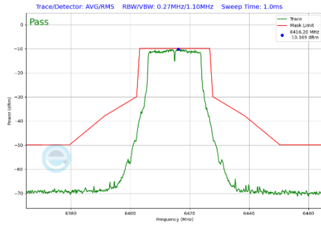
Plot 7-293 In-Band Emission Plot Antenna 3c (20MHz BW 802.11a (UNII Band 5) - Ch.93)
