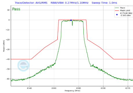
Plot 7-337 In-Band Emission Plot Antenna 1b (20MHz BW 802.11a (UNII Band 5) - Ch.45)
