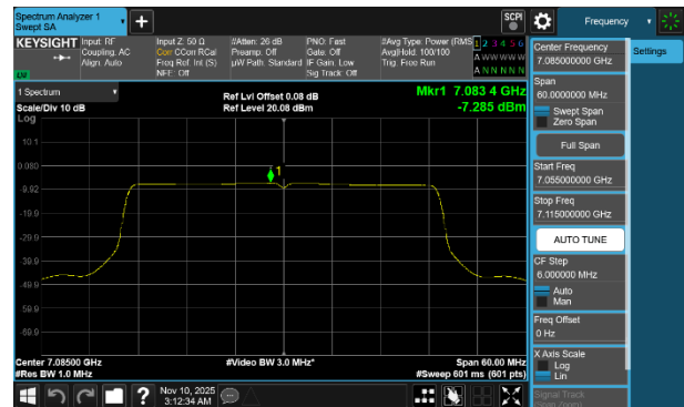
Plot 7-278 PSD CDD Diversity Antenna 1b (40MHz BW 802.11be(SU) - Ch.227)
