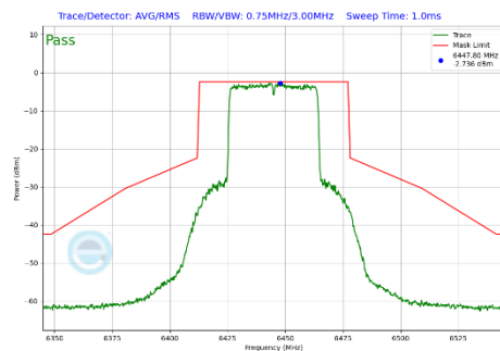
Plot 7-354 In-Band Emission Plot Antenna 1b (40MHz BW 802.11be(SU) (UNII Band 6) - Ch.99)
