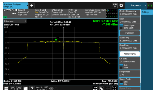
Plot 7-256 PSD CDD Diversity Antenna 1b (160MHz BW 802.11be(SU) - Ch.47)
