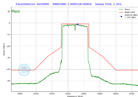
Plot 7-296 In-Band Emission Plot Antenna 3c (160MHz BW 802.11be(SU) (UNII Band 5) - Ch.79)
