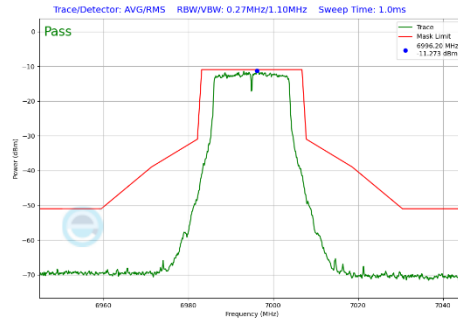
Plot 7-305 In-Band Emission Plot Antenna 3c (20MHz BW 802.11a (UNII Band 8) - Ch.209)
