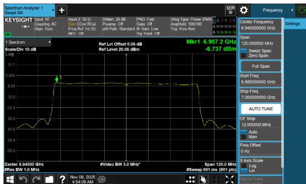
Plot 7-275 PSD CDD Diversity Antenna 3c (80MHz BW 802.11be(SU) - Ch.199)
