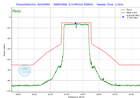
Plot 7-322 In-Band Emission Plot Antenna 3a (40MHz BW 802.11be(SU) (UNII Band 5) - Ch.43)
