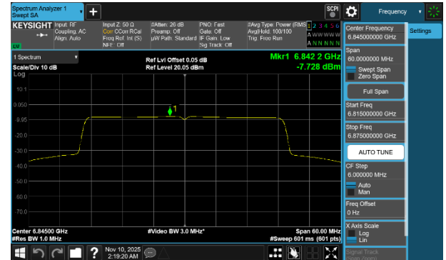
Plot 7-270 PSD CDD Diversity Antenna 1b (40MHz BW 802.11be(SU) - Ch.179)
