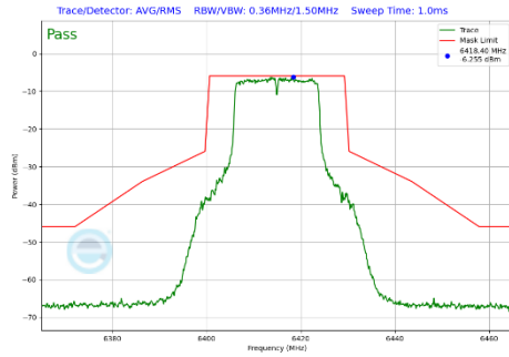
Plot 7-349 In-Band Emission Plot Antenna 1b (20MHz BW 802.11a (UNII Band 5) - Ch.93)
