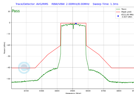
Plot 7-356 In-Band Emission Plot Antenna 1b (160MHz BW 802.11be(SU) (UNII Band 6) - Ch.111)
