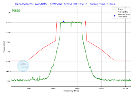
Plot 7-329 In-Band Emission Plot Antenna 3a (20MHz BW 802.11a (UNII Band 7) - Ch.185)
