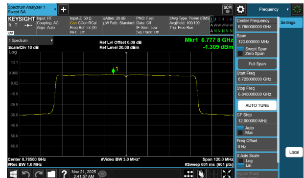
Plot 7-247 PSD CDD Diversity Antenna 1b (80MHz BW 802.11be(SU) - Ch.167)
