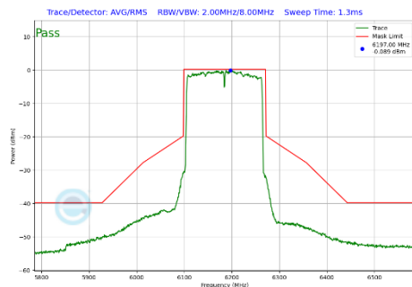
Plot 7-324 In-Band Emission Plot Antenna 3a (160MHz BW 802.11be(SU) (UNII Band 5) - Ch.47)
