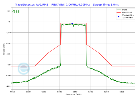
Plot 7-339 In-Band Emission Plot Antenna 1b (80MHz BW 802.11be(SU) (UNII Band 5) - Ch.39)
