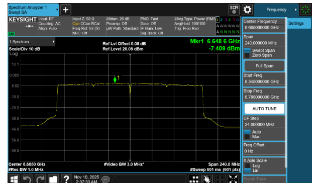
Plot 7-272 PSD CDD Diversity Antenna 1b (160MHz BW 802.11be(SU) - Ch.143)
