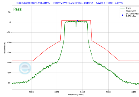
Plot 7-285 In-Band Emission Plot Antenna 3c (20MHz BW 802.11a (UNII Band 6) - Ch.97)
