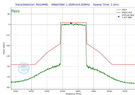
Plot 7-283 In-Band Emission Plot Antenna 3c (80MHz BW 802.11be(SU) (UNII Band 5) - Ch.87)
