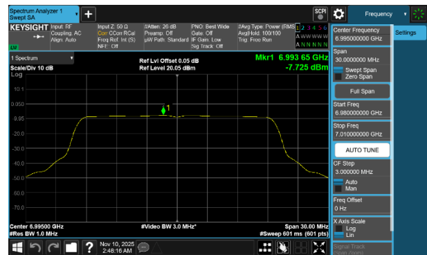
Plot 7-277 PSD CDD Diversity Antenna 1b (20MHz BW 802.11be(SU) - Ch.209)
