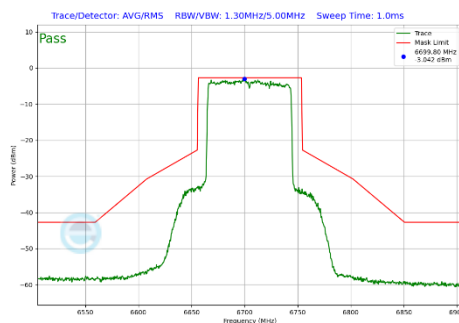
Plot 7-303 In-Band Emission Plot Antenna 3c (80MHz BW 802.11be(SU) (UNII Band 7) - Ch.151)
