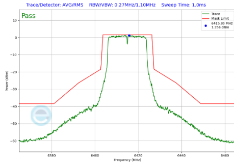
Plot 7-281 In-Band Emission Plot Antenna 3c (20MHz BW 802.11a (UNII Band 5) - Ch.93)
