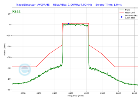
Plot 7-287 In-Band Emission Plot Antenna 3c (80MHz BW 802.11be(SU) (UNII Band 6) - Ch.103)
