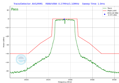
Plot 7-317 In-Band Emission Plot Antenna 3a (20MHz BW 802.11a (UNII Band 7) - Ch.117)
