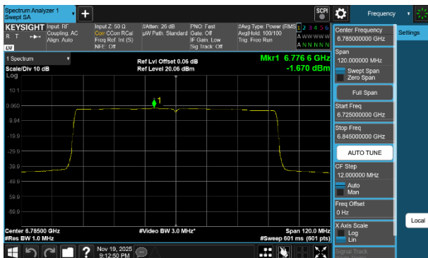
Plot 7-243 PSD CDD Diversity Antenna 3c (80MHz BW 802.11be(SU) - Ch.167)
