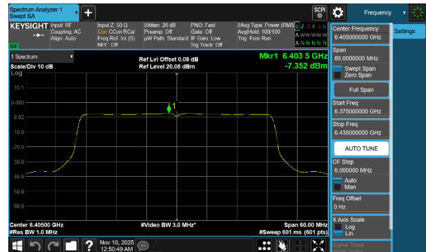
Plot 7-254 PSD CDD Diversity Antenna 1b (40MHz BW 802.11be(SU) - Ch.91)
