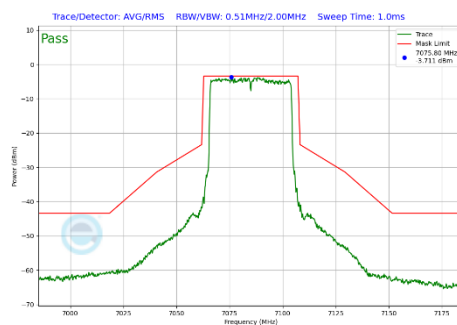
Plot 7-334 In-Band Emission Plot Antenna 3a (40MHz BW 802.11be(SU) (UNII Band 8) - Ch.227)
