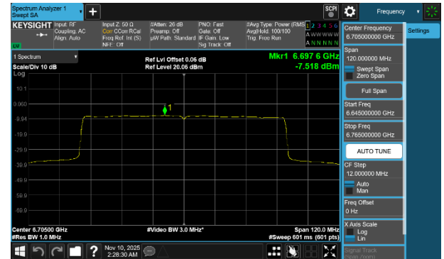
Plot 7-271 PSD CDD Diversity Antenna 1b (80MHz BW 802.11be(SU) - Ch.151)
