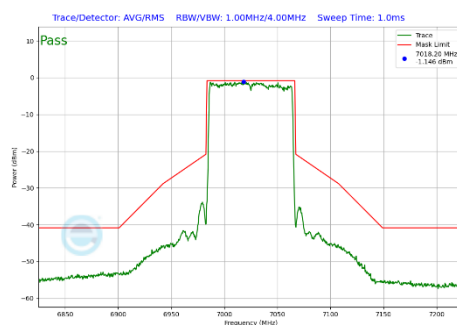
Plot 7-335 In-Band Emission Plot Antenna 3a (80MHz BW 802.11be(SU) (UNII Band 8) - Ch.215)
