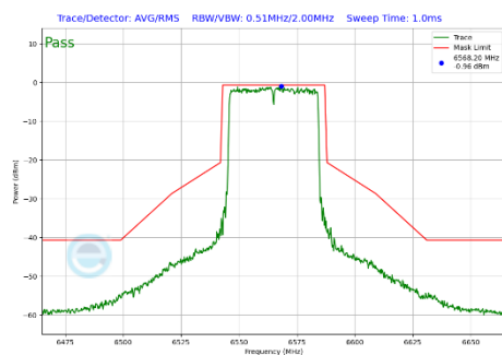
Plot 7-318 In-Band Emission Plot Antenna 3a (40MHz BW 802.11be(SU) (UNII Band 7) - Ch.123)
