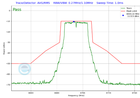
Plot 7-301 In-Band Emission Plot Antenna 3c (20MHz BW 802.11a (UNII Band 7) - Ch.149)
