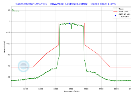
Plot 7-300 In-Band Emission Plot Antenna 3c (160MHz BW 802.11be(SU) (UNII Band 6) - Ch.111)
