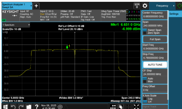
Plot 7-268 PSD CDD Diversity Antenna 3c (160MHz BW 802.11be(SU) - Ch.143)
