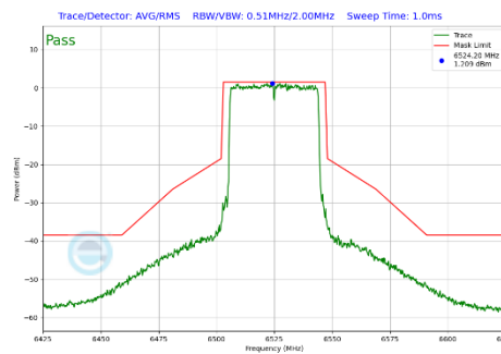
Plot 7-286 In-Band Emission Plot Antenna 3c (40MHz BW 802.11be(SU) (UNII Band 6) - Ch.115)
