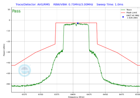
Plot 7-350 In-Band Emission Plot Antenna 1b (40MHz BW 802.11be(SU) (UNII Band 5) - Ch.91)
