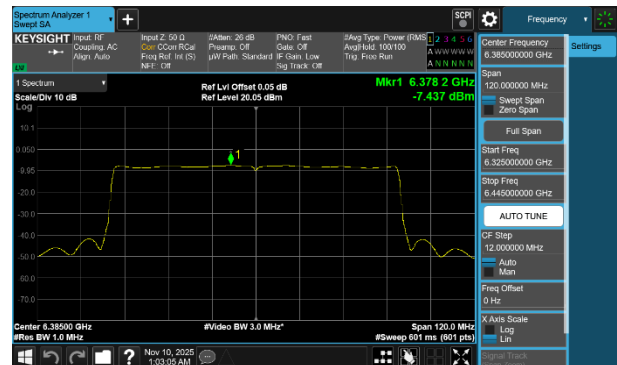
Plot 7-255 PSD CDD Diversity Antenna 1b (80MHz BW 802.11be(SU) - Ch.87)
