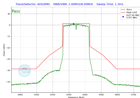
Plot 7-284 In-Band Emission Plot Antenna 3c (160MHz BW 802.11be(SU) (UNII Band 5) - Ch.79)
