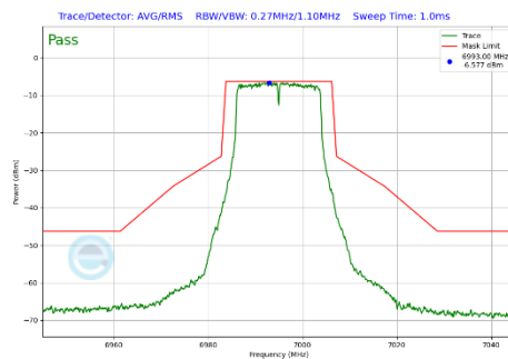
Plot 7-333 In-Band Emission Plot Antenna 3a (20MHz BW 802.11a (UNII Band 8) - Ch.209)
