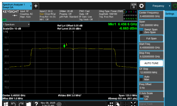
Plot 7-259 PSD CDD Diversity Antenna 3c (80MHz BW 802.11be(SU) - Ch.103)
