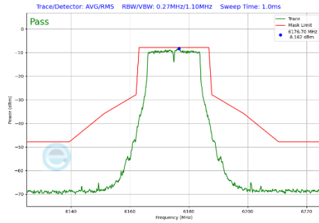
Plot 7-321 In-Band Emission Plot Antenna 3a (20MHz BW 802.11a (UNII Band 5) - Ch.45)
