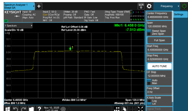
Plot 7-263 PSD CDD Diversity Antenna 1b (80MHz BW 802.11be(SU) - Ch.103)
