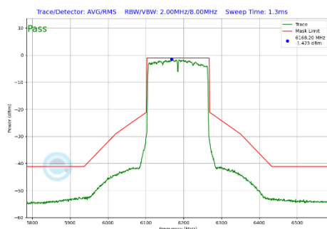
Plot 7-340 In-Band Emission Plot Antenna 1b (160MHz BW 802.11be(SU) (UNII Band 5) - Ch.47)
