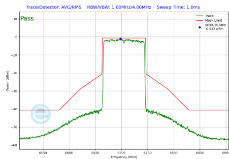
Plot 7-319 In-Band Emission Plot Antenna 3a (80MHz BW 802.11be(SU) (UNII Band 7) - Ch.151)
