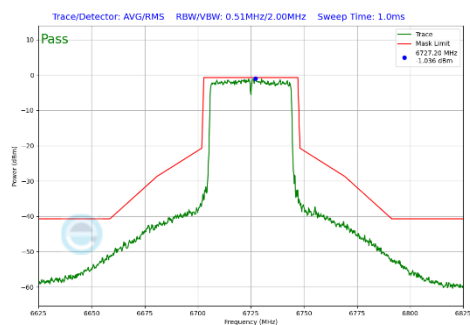
Plot 7-346 In-Band Emission Plot Antenna 1b (40MHz BW 802.11be(SU) (UNII Band 7) - Ch.155)
