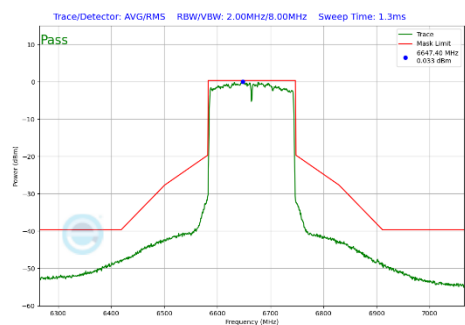
Plot 7-348 In-Band Emission Plot Antenna 1b (160MHz BW 802.11be(SU) (UNII Band 7) - Ch.143)
