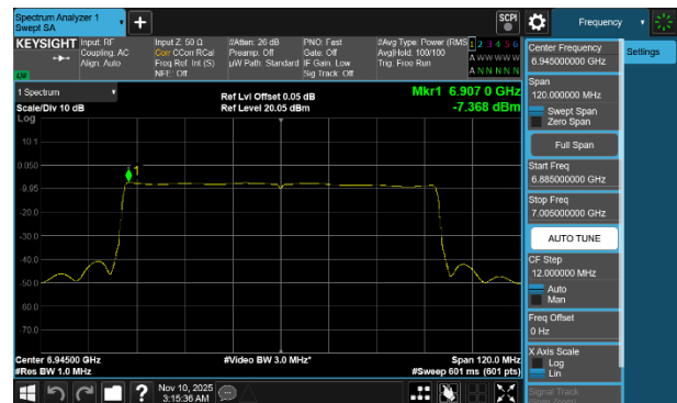
Plot 7-279 PSD CDD Diversity Antenna 1b (80MHz BW 802.11be(SU) - Ch.199)
