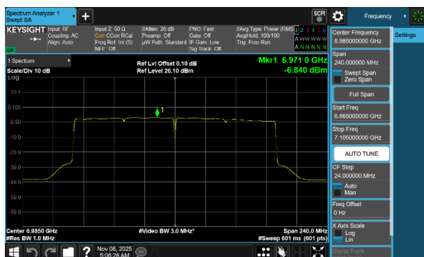
Plot 7-276 PSD CDD Diversity Antenna 3c (160MHz BW 802.11be(SU) - Ch.207)
