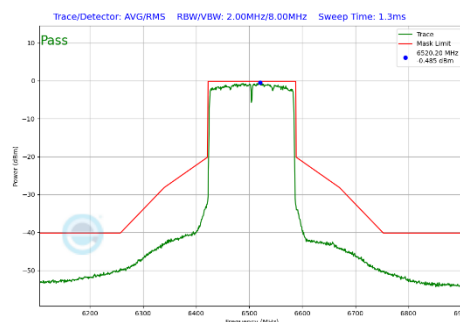
Plot 7-344 In-Band Emission Plot Antenna 1b (160MHz BW 802.11be(SU) (UNII Band 6) - Ch.111)
