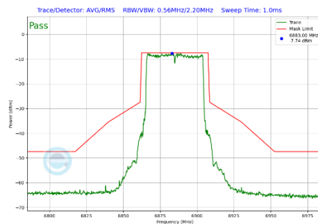
Plot 7-306 In-Band Emission Plot Antenna 3c (40MHz BW 802.11be(SU) (UNII Band 8) - Ch.187)
