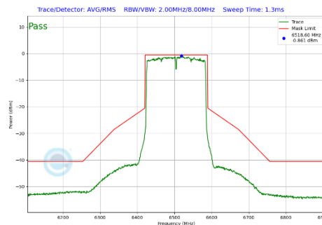
Plot 7-316 In-Band Emission Plot Antenna 3a (160MHz BW 802.11be(SU) (UNII Band 6) - Ch.111)
