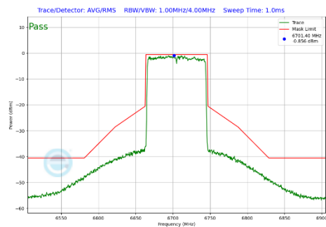
Plot 7-347 In-Band Emission Plot Antenna 1b (80MHz BW 802.11be(SU) (UNII Band 7) - Ch.151)
