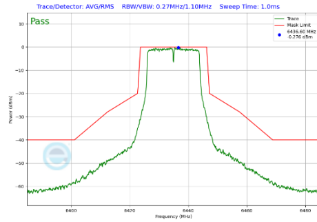
Plot 7-313 In-Band Emission Plot Antenna 3a (20MHz BW 802.11a (UNII Band 6) - Ch.97)
