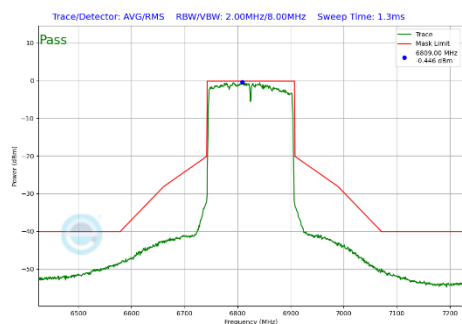
Plot 7-332 In-Band Emission Plot Antenna 3a (160MHz BW 802.11be(SU) (UNII Band 7) - Ch.175)
