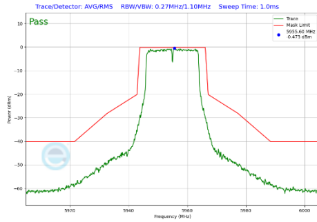
Plot 7-309 In-Band Emission Plot Antenna 3a (20MHz BW 802.11a (UNII Band 5) - Ch.1)
