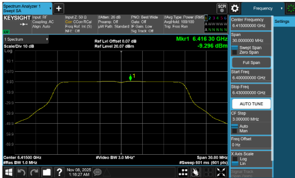
Plot 7-249 PSD CDD Diversity Antenna 3c (20MHz BW 802.11a - Ch.93)
