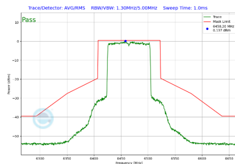
Plot 7-327 In-Band Emission Plot Antenna 3a (80MHz BW 802.11be(SU) (UNII Band 6) - Ch.103)
