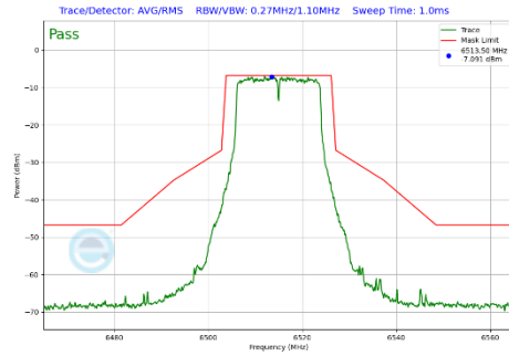
Plot 7-353 In-Band Emission Plot Antenna 1b (20MHz BW 802.11a (UNII Band 6) - Ch.113)
