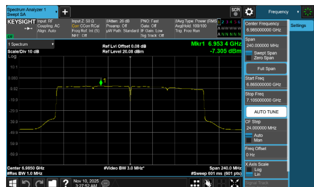
Plot 7-280 PSD CDD Diversity Antenna 1b (160MHz BW 802.11be(SU) - Ch.207)
