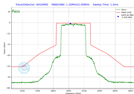
Plot 7-355 In-Band Emission Plot Antenna 1b (80MHz BW 802.11be(SU) (UNII Band 6) - Ch.103)
