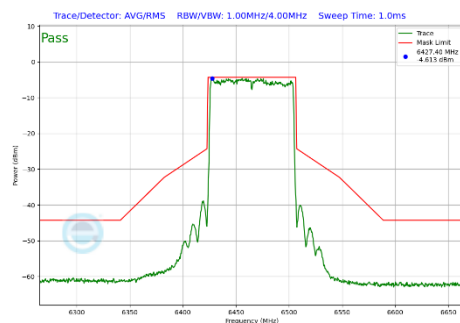
Plot 7-299 In-Band Emission Plot Antenna 3c (80MHz BW 802.11be(SU) (UNII Band 6) - Ch.103)
