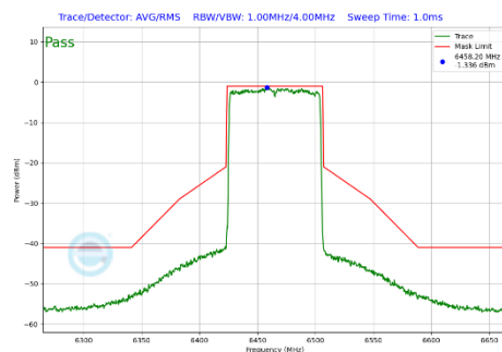
Plot 7-315 In-Band Emission Plot Antenna 3a (80MHz BW 802.11be(SU) (UNII Band 6) - Ch.103)
