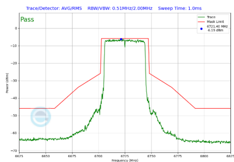
Plot 7-330 In-Band Emission Plot Antenna 3a (40MHz BW 802.11be(SU) (UNII Band 7) - Ch.155)
