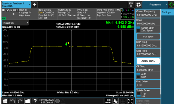
Plot 7-266 PSD CDD Diversity Antenna 3c (40MHz BW 802.11be(SU) - Ch.179)
