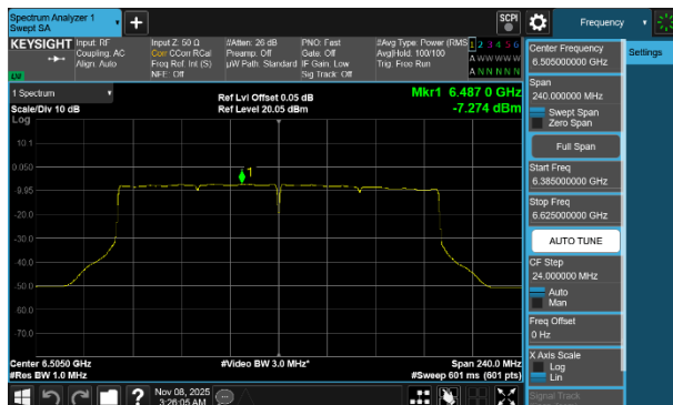
Plot 7-260 PSD CDD Diversity Antenna 3c (160MHz BW 802.11be(SU) - Ch.111)
