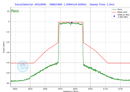
Plot 7-311 In-Band Emission Plot Antenna 3a (80MHz BW 802.11be(SU) (UNII Band 5) - Ch.7)
