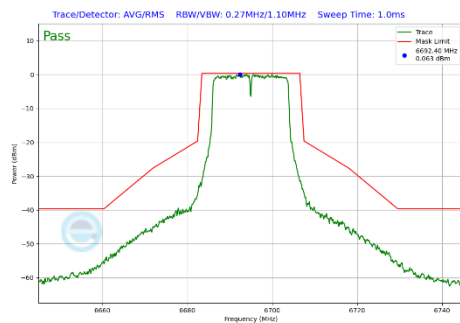
Plot 7-345 In-Band Emission Plot Antenna 1b (20MHz BW 802.11a (UNII Band 7) - Ch.149)
