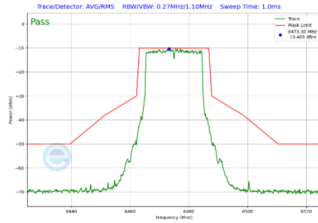
Plot 7-297 In-Band Emission Plot Antenna 3c (20MHz BW 802.11be(SU) (UNII Band 6) - Ch.105)
