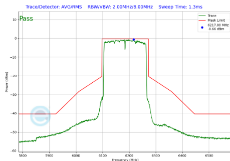
Plot 7-352 In-Band Emission Plot Antenna 1b (160MHz BW 802.11be(SU) (UNII Band 5) - Ch.47)
