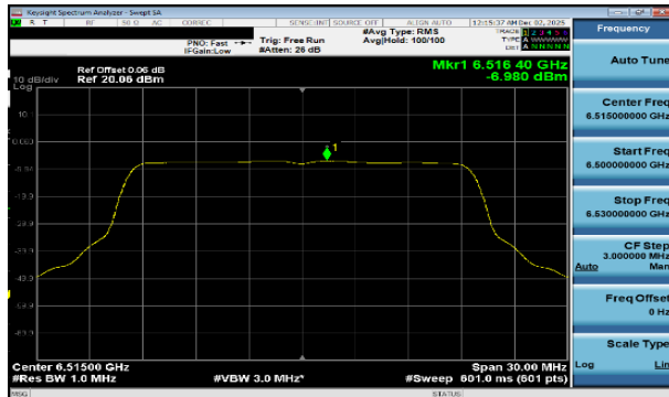
Plot 7-257 PSD CDD Diversity Antenna 3c (20MHz BW 802.11be(SU) - Ch.113)
