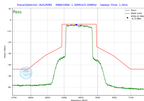
Plot 7-307 In-Band Emission Plot Antenna 3c (80MHz BW 802.11be(SU) (UNII Band 8) - Ch.199)
