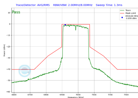
Plot 7-336 In-Band Emission Plot Antenna 3a (160MHz BW 802.11be(SU) (UNII Band 8) - Ch.207)
