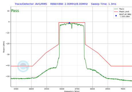
Plot 7-304 In-Band Emission Plot Antenna 3c (160MHz BW 802.11be(SU) (UNII Band 7) - Ch.143)
