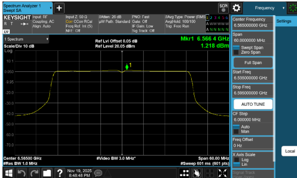
Plot 7-242 PSD CDD Diversity Antenna 3c (40MHz BW 802.11be(SU) - Ch.123)
