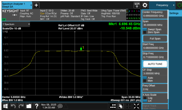
Plot 7-265 PSD CDD Diversity Antenna 3c (20MHz BW 802.11a - Ch.149)
