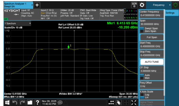
Plot 7-253 PSD CDD Diversity Antenna 1b (20MHz BW 802.11a - Ch.93)
