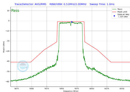
Plot 7-310 In-Band Emission Plot Antenna 3a (40MHz BW 802.11be(SU) (UNII Band 5) - Ch.3)
