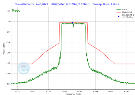
Plot 7-338 In-Band Emission Plot Antenna 1b (40MHz BW 802.11be(SU) (UNII Band 5) - Ch.43)
