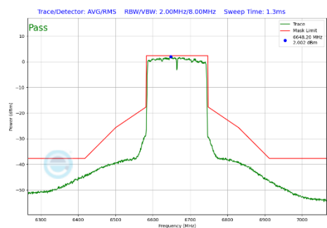
Plot 7-292 In-Band Emission Plot Antenna 3c (160MHz BW 802.11be(SU) (UNII Band 7) - Ch.143)
