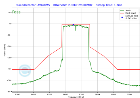
Plot 7-320 In-Band Emission Plot Antenna 3a (160MHz BW 802.11be(SU) (UNII Band 7) - Ch.143)
