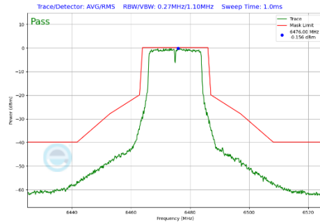
Plot 7-341 In-Band Emission Plot Antenna 1b (20MHz BW 802.11a (UNII Band 6) - Ch.105)
