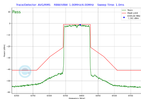
Plot 7-323 In-Band Emission Plot Antenna 3a (80MHz BW 802.11be(SU) (UNII Band 5) - Ch.87)
