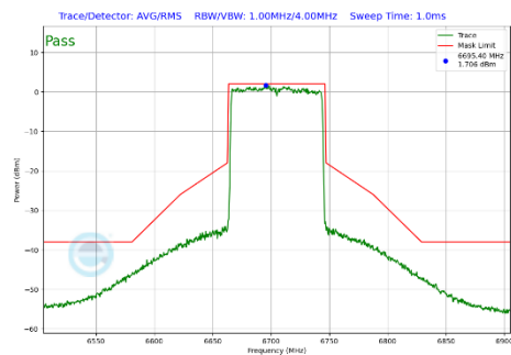
Plot 7-291 In-Band Emission Plot Antenna 3c (80MHz BW 802.11be(SU) (UNII Band 7) - Ch.151)
