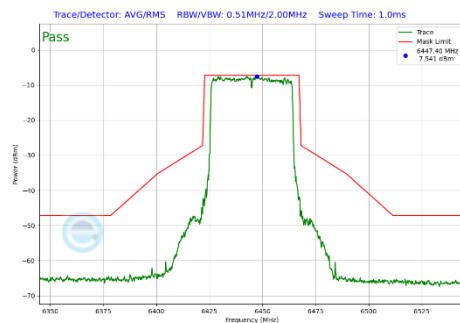
Plot 7-298 In-Band Emission Plot Antenna 3c (40MHz BW 802.11be(SU) (UNII Band 6) - Ch.99)
