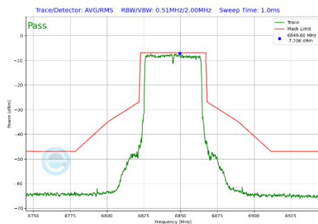
Plot 7-302 In-Band Emission Plot Antenna 3c (40MHz BW 802.11be(SU) (UNII Band 7) - Ch.179)
