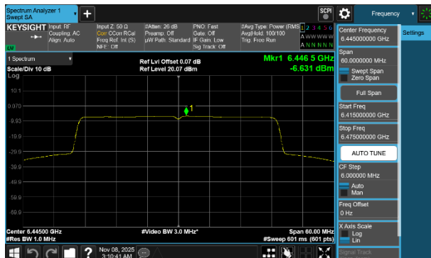
Plot 7-258 PSD CDD Diversity Antenna 3c (40MHz BW 802.11be(SU) - Ch.99)
