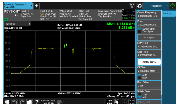
Plot 7-264 PSD CDD Diversity Antenna 1b (160MHz BW 802.11be(SU) - Ch.111)
