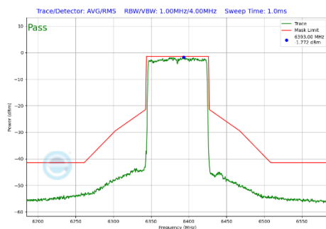
Plot 7-351 In-Band Emission Plot Antenna 1b (80MHz BW 802.11be(SU) (UNII Band 5) - Ch.87)
