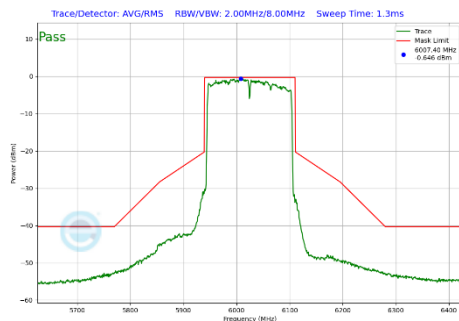
Plot 7-312 In-Band Emission Plot Antenna 3a (160MHz BW 802.11be(SU) (UNII Band 5) - Ch.15)
