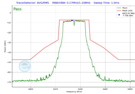
Plot 7-325 In-Band Emission Plot Antenna 3a (20MHz BW 802.11a (UNII Band 6) - Ch.97)
