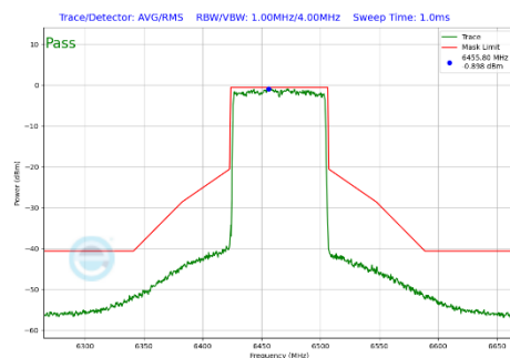
Plot 7-343 In-Band Emission Plot Antenna 1b (80MHz BW 802.11be(SU) (UNII Band 6) - Ch.103)
