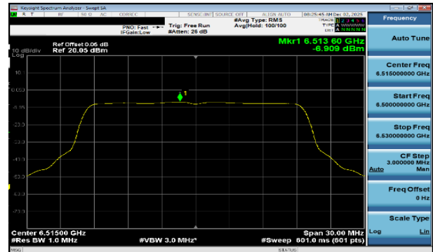
Plot 7-261 PSD CDD Diversity Antenna 1b (20MHz BW 802.11be(SU) - Ch.113)
