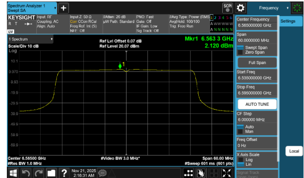
Plot 7-246 PSD CDD Diversity Antenna 1b (40MHz BW 802.11be(SU) - Ch.123)
