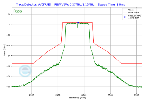
Plot 7-289 In-Band Emission Plot Antenna 3c (20MHz BW 802.11a (UNII Band 7) - Ch.117)
