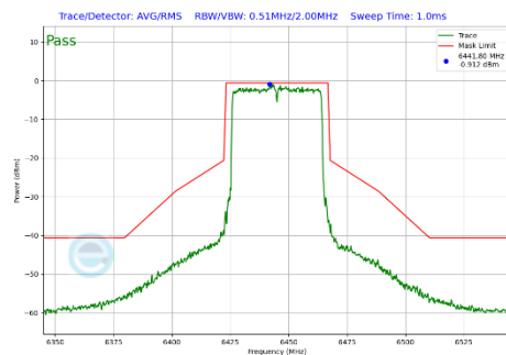
Plot 7-342 In-Band Emission Plot Antenna 1b (40MHz BW 802.11be(SU) (UNII Band 6) - Ch.99)
