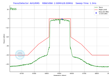
Plot 7-328 In-Band Emission Plot Antenna 3a (160MHz BW 802.11be(SU) (UNII Band 6) - Ch.111)
