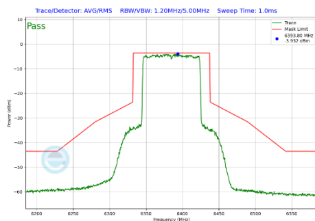
Plot 7-295 In-Band Emission Plot Antenna 3c (80MHz BW 802.11be(SU) (UNII Band 5) - Ch.87)
