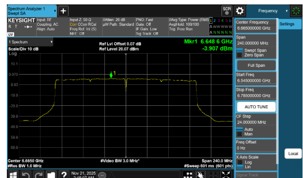
Plot 7-248 PSD CDD Diversity Antenna 1b (160MHz BW 802.11be(SU) - Ch.143)
