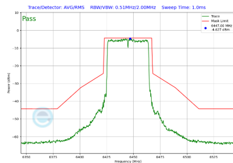
Plot 7-326 In-Band Emission Plot Antenna 3a (40MHz BW 802.11be(SU) (UNII Band 6) - Ch.99)
