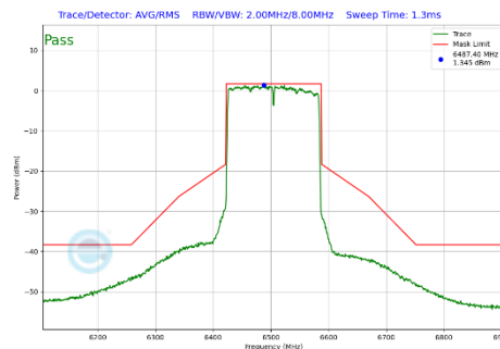
Plot 7-288 In-Band Emission Plot Antenna 3c (160MHz BW 802.11be(SU) (UNII Band 6) - Ch.111)
