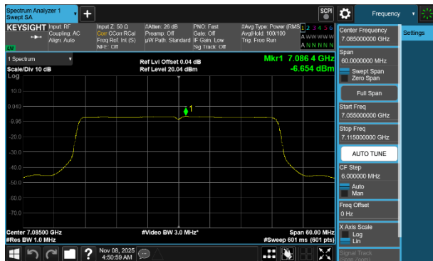
Plot 7-274 PSD CDD Diversity Antenna 3c (40MHz BW 802.11be(SU) - Ch.227)
