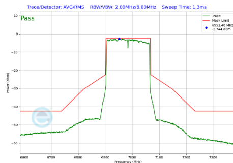
Plot 7-308 In-Band Emission Plot Antenna 3c (160MHz BW 802.11be(SU) (UNII Band 8) - Ch.207)
