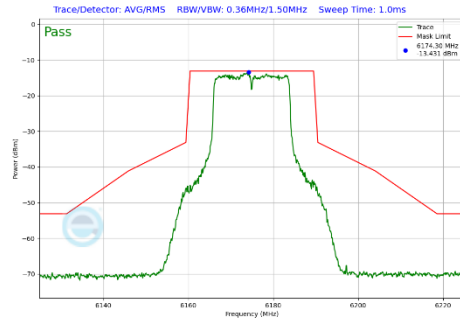
Plot 7-449 In-Band Emission Plot CDD Diversity Antenna 1b (20MHz BW 802.11a (UNII Band 5) - Ch.45)
