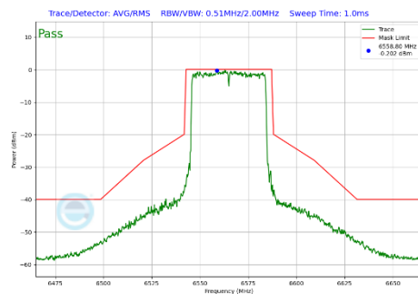
Plot 7-442 In-Band Emission Plot CDD Diversity Antenna 1b (40MHz BW 802.11be(SU) (UNII Band 7) - Ch.123)
