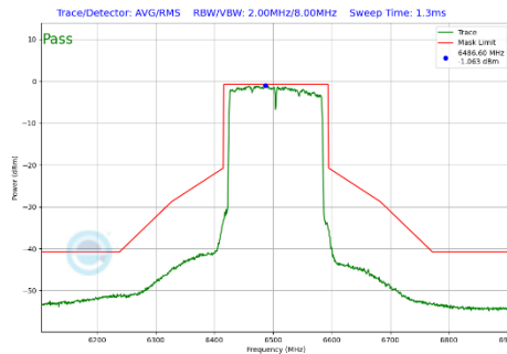
Plot 7-376 In-Band Emission Plot CDD Primary Antenna 3c (160MHz BW 802.11be(SU) (UNII Band 6) - Ch.111)
