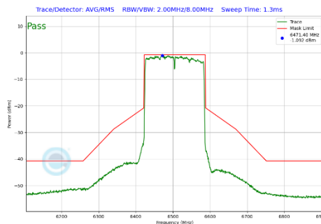
Plot 7-432 In-Band Emission Plot CDD Diversity Antenna 3c (160MHz BW 802.11be(SU) (UNII Band 6) - Ch.111)
