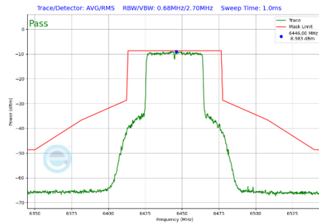
Plot 7-402 In-Band Emission Plot SDM Primary Antenna 3a (40MHz BW 802.11be(SU) (UNII Band 6) - Ch.99)
