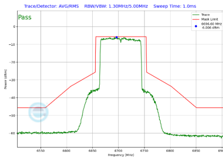
Plot 7-463 In-Band Emission Plot SDM Diversity Antenna 3c (80MHz BW 802.11be(SU) (UNII Band 7) - Ch.151)
