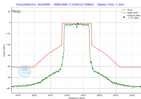
Plot 7-438 In-Band Emission Plot CDD Diversity Antenna 3c (40MHz BW 802.11be(SU) (UNII Band 7) - Ch.123)
