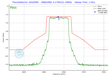
Plot 7-413 In-Band Emission Plot SDM Primary Antenna 3c (20MHz BW 802.11be(SU) (UNII Band 8) - Ch.189)
