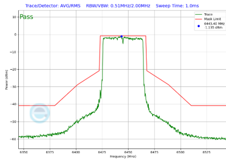
Plot 7-374 In-Band Emission Plot CDD Primary Antenna 3c (40MHz BW 802.11be(SU) (UNII Band 6) - Ch.99)
