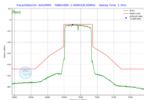
Plot 7-472 In-Band Emission Plot SDM Diversity Antenna 3c (160MHz BW 802.11be(SU) (UNII Band 8) - Ch.207)
