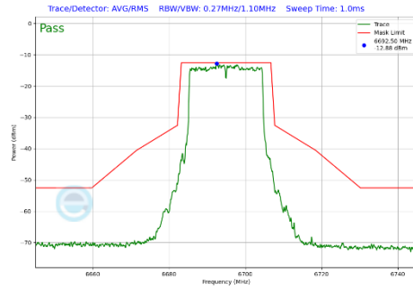
Plot 7-409 In-Band Emission Plot SDM Primary Antenna 3a (20MHz BW 802.11be(SU) (UNII Band 7) - Ch.149)
