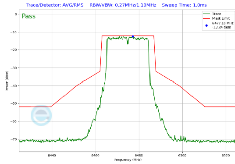
Plot 7-397 In-Band Emission Plot SDM Primary Antenna 3c (20MHz BW 802.11be(SU) (UNII Band 6) - Ch.105)
