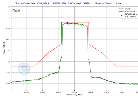
Plot 7-400 In-Band Emission Plot SDM Primary Antenna 3c (160MHz BW 802.11be(SU) (UNII Band 6) - Ch.111)
