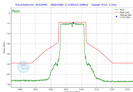
Plot 7-470 In-Band Emission Plot SDM Diversity Antenna 3c (40MHz BW 802.11be(SU) (UNII Band 8) - Ch.227)
