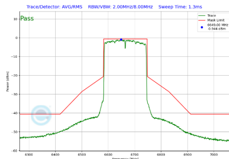
Plot 7-388 In-Band Emission Plot CDD Primary Antenna 3a (160MHz BW 802.11be(SU) (UNII Band 7) - Ch.143)
