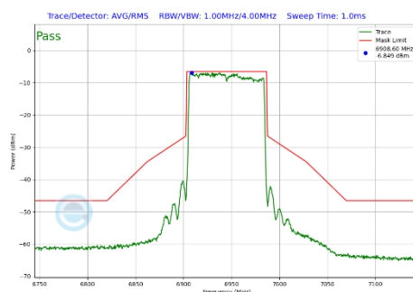
Plot 7-475 In-Band Emission Plot SDM Diversity Antenna 1b (80MHz BW 802.11be(SU) (UNII Band 8) - Ch.199)
