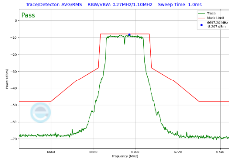
Plot 7-357 In-Band Emission Plot Antenna 1b (20MHz BW 802.11a (UNII Band 7) - Ch.149)
