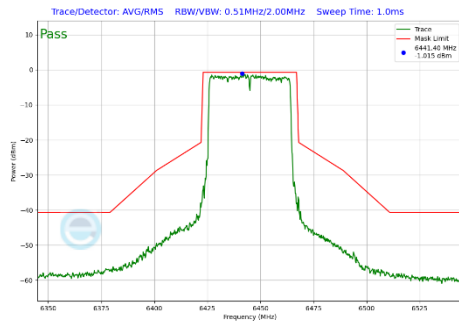
Plot 7-430 In-Band Emission Plot CDD Diversity Antenna 3c (40MHz BW 802.11be(SU) (UNII Band 6) - Ch.99)
