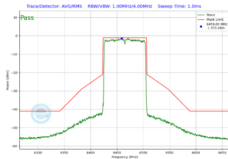
Plot 7-379 In-Band Emission Plot CDD Primary Antenna 3a (80MHz BW 802.11be(SU) (UNII Band 6) - Ch.103)
