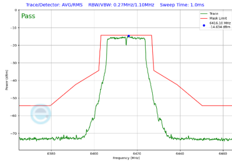
Plot 7-389 In-Band Emission Plot CDD Primary Antenna 3c (20MHz BW 802.11a (UNII Band 5) - Ch.93)
