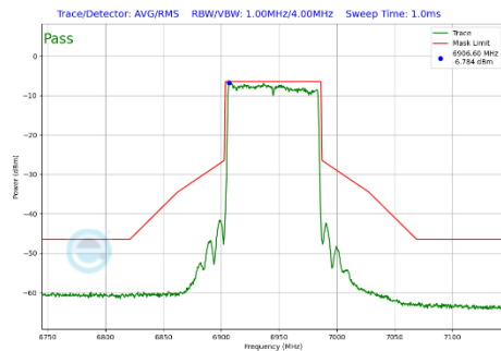
Plot 7-415 In-Band Emission Plot SDM Primary Antenna 3c (80MHz BW 802.11be(SU) (UNII Band 8) - Ch.199)
