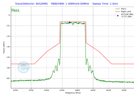
Plot 7-391 In-Band Emission Plot SDM Primary Antenna 3c (80MHz BW 802.11be(SU) (UNII Band 5) - Ch.87)
