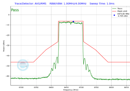
Plot 7-399 In-Band Emission Plot SDM Primary Antenna 3c (80MHz BW 802.11be(SU) (UNII Band 6) - Ch.103)
