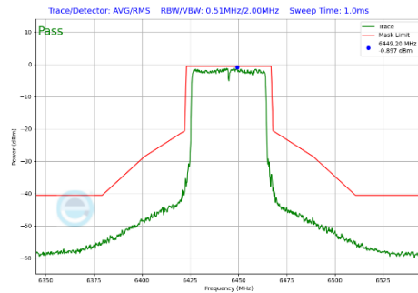
Plot 7-378 In-Band Emission Plot CDD Primary Antenna 3a (40MHz BW 802.11be(SU) (UNII Band 6) - Ch.99)
