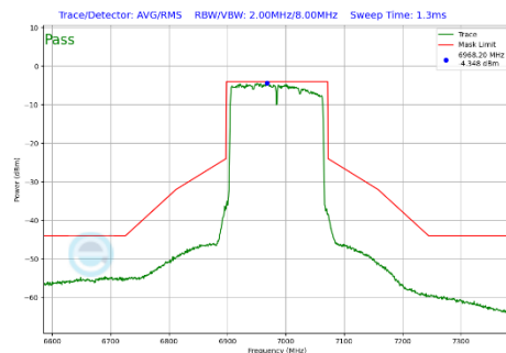
Plot 7-420 In-Band Emission Plot SDM Primary Antenna 3a (160MHz BW 802.11be(SU) (UNII Band 8) - Ch.207)
