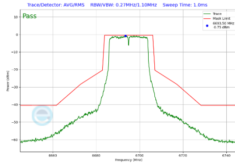
Plot 7-385 In-Band Emission Plot CDD Primary Antenna 3a (20MHz BW 802.11a (UNII Band 7) - Ch.149)
