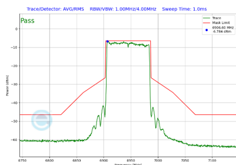
Plot 7-471 In-Band Emission Plot SDM Diversity Antenna 3c (80MHz BW 802.11be(SU) (UNII Band 8) - Ch.199)
