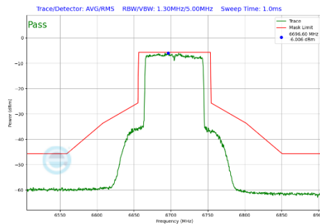
Plot 7-407 In-Band Emission Plot SDM Primary Antenna 3c (80MHz BW 802.11be(SU) (UNII Band 7) - Ch.151)
