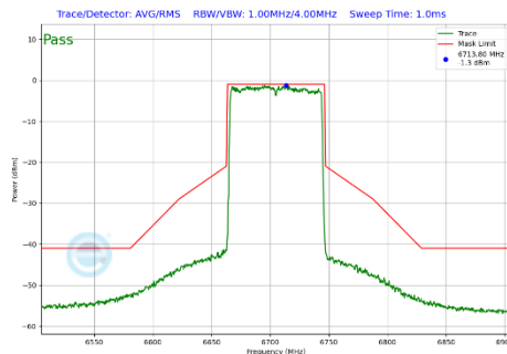
Plot 7-383 In-Band Emission Plot CDD Primary Antenna 3c (80MHz BW 802.11be(SU) (UNII Band 7) - Ch.151)
