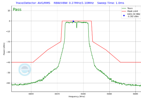
Plot 7-373 In-Band Emission Plot CDD Primary Antenna 3c (20MHz BW 802.11a (UNII Band 6) - Ch.97)
