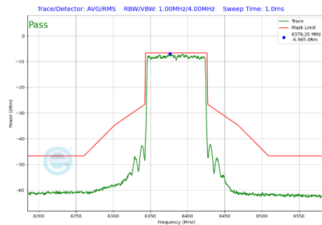
Plot 7-395 In-Band Emission Plot SDM Primary Antenna 3a (80MHz BW 802.11be(SU) (UNII Band 5) - Ch.87)
