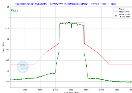
Plot 7-456 In-Band Emission Plot SDM Diversity Antenna 3c (160MHz BW 802.11be(SU) (UNII Band 6) - Ch.111)
