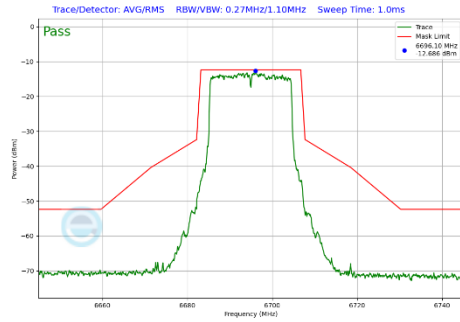
Plot 7-405 In-Band Emission Plot SDM Primary Antenna 3c (20MHz BW 802.11be(SU) (UNII Band 7) - Ch.149)
