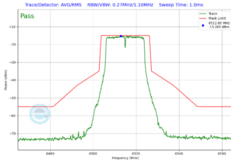
Plot 7-453 In-Band Emission Plot CDD Diversity Antenna 3c (20MHz BW 802.11a (UNII Band 6) - Ch.113)
