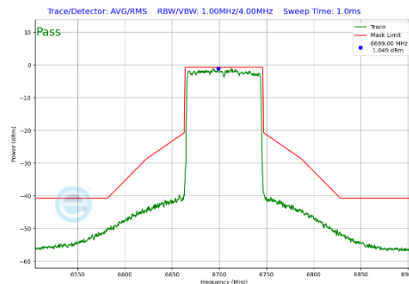
Plot 7-387 In-Band Emission Plot CDD Primary Antenna 3a (80MHz BW 802.11be(SU) (UNII Band 7) - Ch.151)
