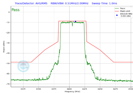
Plot 7-390 In-Band Emission Plot SDM Primary Antenna 3c (40MHz BW 802.11be(SU) (UNII Band 5) - Ch.91)
