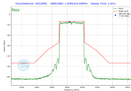
Plot 7-403 In-Band Emission Plot SDM Primary Antenna 3a (80MHz BW 802.11be(SU) (UNII Band 6) - Ch.103)
