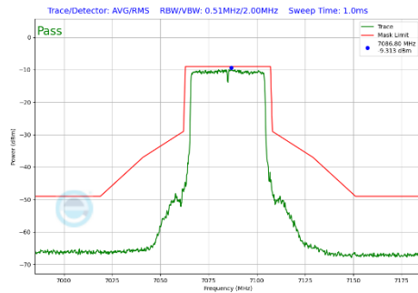
Plot 7-414 In-Band Emission Plot SDM Primary Antenna 3c (40MHz BW 802.11be(SU) (UNII Band 8) - Ch.227)
