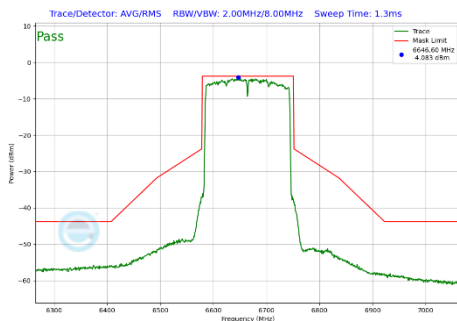
Plot 7-464 In-Band Emission Plot SDM Diversity Antenna 3c (160MHz BW 802.11be(SU) (UNII Band 7) - Ch.143)
