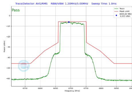
Plot 7-467 In-Band Emission Plot SDM Diversity Antenna 1b (80MHz BW 802.11be(SU) (UNII Band 7) - Ch.151)
