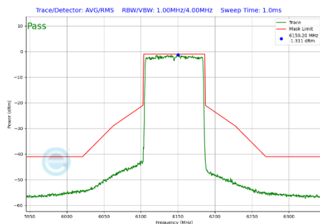
Plot 7-423 In-Band Emission Plot CDD Diversity Antenna 3c (80MHz BW 802.11be(SU) (UNII Band 5) - Ch.39)
