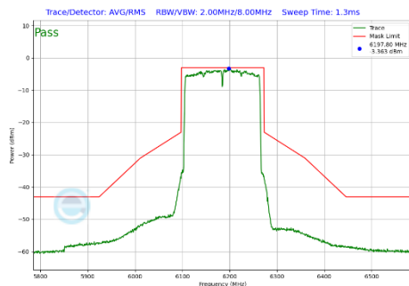
Plot 7-392 In-Band Emission Plot SDM Primary Antenna 3c (160MHz BW 802.11be(SU) (UNII Band 5) - Ch.47)
