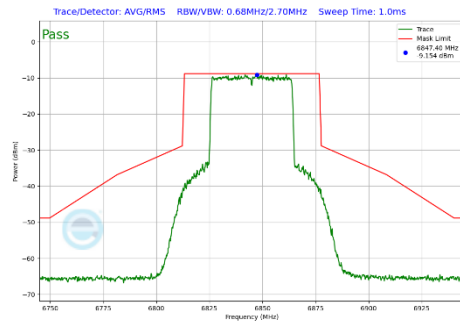
Plot 7-410 In-Band Emission Plot SDM Primary Antenna 3a (40MHz BW 802.11be(SU) (UNII Band 7) - Ch.179)
