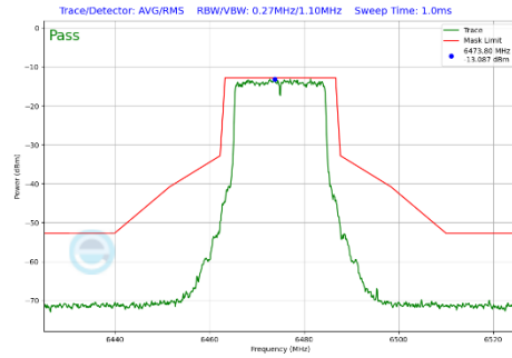
Plot 7-401 In-Band Emission Plot SDM Primary Antenna 3a (20MHz BW 802.11be(SU) (UNII Band 6) - Ch.105)
