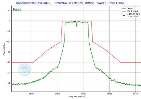
Plot 7-429 In-Band Emission Plot CDD Diversity Antenna 3c (20MHz BW 802.11a (UNII Band 6) - Ch.105)
