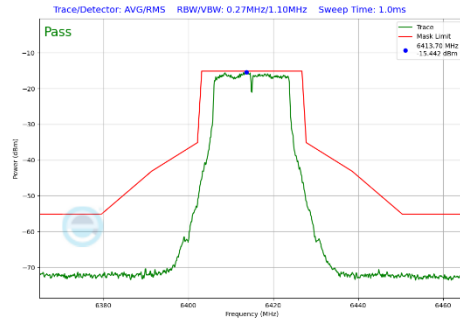
Plot 7-393 In-Band Emission Plot CDD Primary Antenna 3a (20MHz BW 802.11a (UNII Band 5) - Ch.93)
