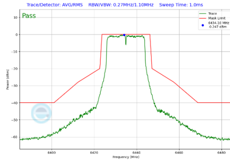
Plot 7-377 In-Band Emission Plot CDD Primary Antenna 3a (20MHz BW 802.11a (UNII Band 6) - Ch.97)
