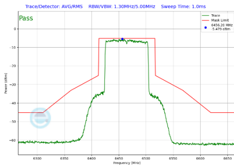
Plot 7-455 In-Band Emission Plot SDM Diversity Antenna 3c (80MHz BW 802.11be(SU) (UNII Band 6) - Ch.103)
