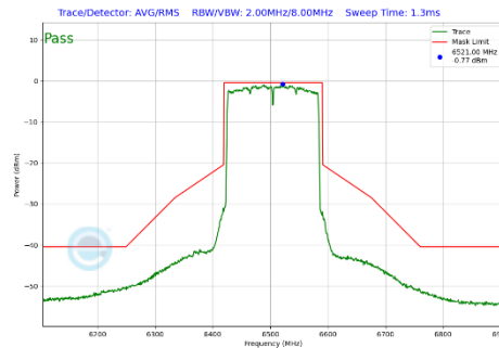
Plot 7-380 In-Band Emission Plot CDD Primary Antenna 3a (160MHz BW 802.11be(SU) (UNII Band 6) - Ch.111)
