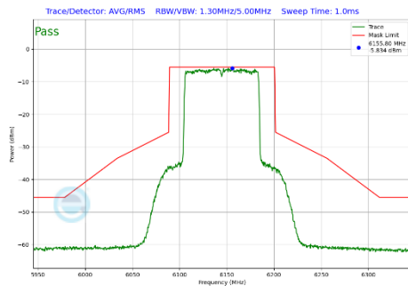
Plot 7-447 In-Band Emission Plot SDM Diversity Antenna 3c (80MHz BW 802.11be(SU) (UNII Band 5) - Ch.39)
