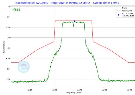
Plot 7-445 In-Band Emission Plot CDD Diversity Antenna 3c (20MHz BW 802.11a (UNII Band 5) - Ch.45)
