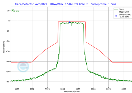
Plot 7-366 In-Band Emission Plot CDD Primary Antenna 3c (40MHz BW 802.11be(SU) (UNII Band 5) - Ch.3)
