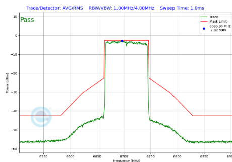
Plot 7-359 In-Band Emission Plot Antenna 1b (80MHz BW 802.11be(SU) (UNII Band 7) - Ch.151)
