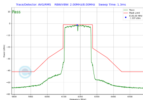
Plot 7-424 In-Band Emission Plot CDD Diversity Antenna 3c (160MHz BW 802.11be(SU) (UNII Band 5) - Ch.47)
