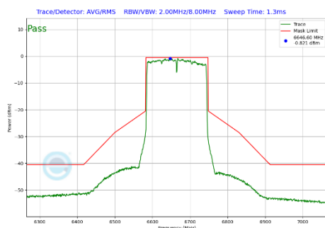
Plot 7-440 In-Band Emission Plot CDD Diversity Antenna 3c (160MHz BW 802.11be(SU) (UNII Band 7) - Ch.143)
