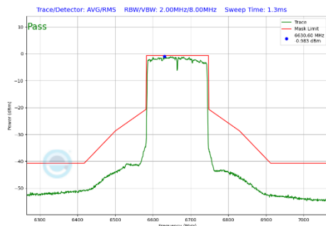
Plot 7-384 In-Band Emission Plot CDD Primary Antenna 3c (160MHz BW 802.11be(SU) (UNII Band 7) - Ch.143)
