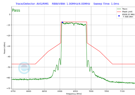
Plot 7-419 In-Band Emission Plot SDM Primary Antenna 3a (80MHz BW 802.11be(SU) (UNII Band 8) - Ch.199)
