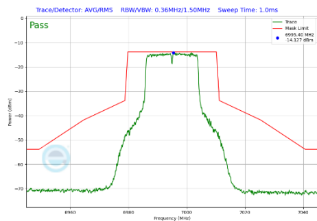
Plot 7-469 In-Band Emission Plot CDD Diversity Antenna 3c (20MHz BW 802.11a (UNII Band 8) - Ch.209)
