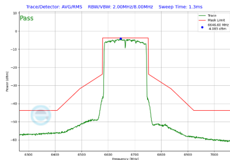
Plot 7-408 In-Band Emission Plot SDM Primary Antenna 3c (160MHz BW 802.11be(SU) (UNII Band 7) - Ch.143)
