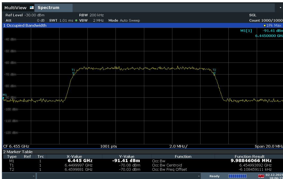
Plot 7-481. AWGN Signal – UNII 6 – 20MHz
