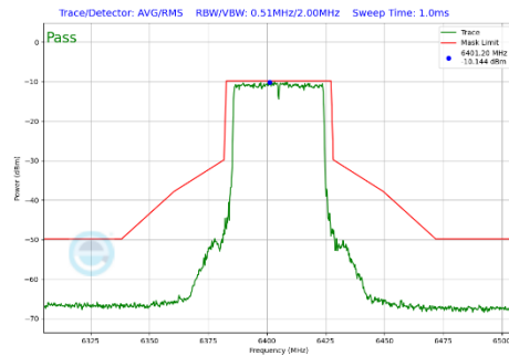
Plot 7-394 In-Band Emission Plot SDM Primary Antenna 3a (40MHz BW 802.11be(SU) (UNII Band 5) - Ch.91)
