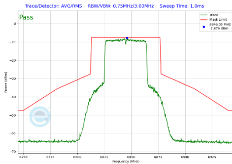
Plot 7-462 In-Band Emission Plot SDM Diversity Antenna 3c (40MHz BW 802.11be(SU) (UNII Band 7) - Ch.179)
