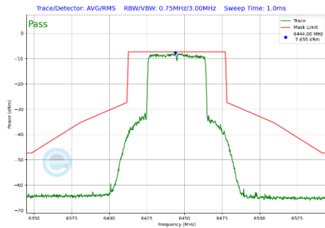
Plot 7-398 In-Band Emission Plot SDM Primary Antenna 3c (40MHz BW 802.11be(SU) (UNII Band 6) - Ch.99)
