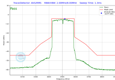
Plot 7-404 In-Band Emission Plot SDM Primary Antenna 3a (160MHz BW 802.11be(SU) (UNII Band 6) - Ch.111)
