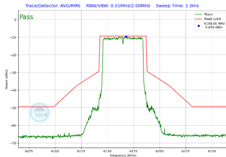
Plot 7-446 In-Band Emission Plot SDM Diversity Antenna 3c (40MHz BW 802.11be(SU) (UNII Band 5) - Ch.43)
