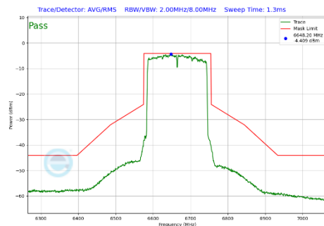
Plot 7-412 In-Band Emission Plot SDM Primary Antenna 3a (160MHz BW 802.11be(SU) (UNII Band 7) - Ch.143)
