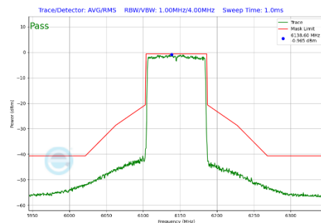
Plot 7-427 In-Band Emission Plot CDD Diversity Antenna 1b (80MHz BW 802.11be(SU) (UNII Band 5) - Ch.39)
