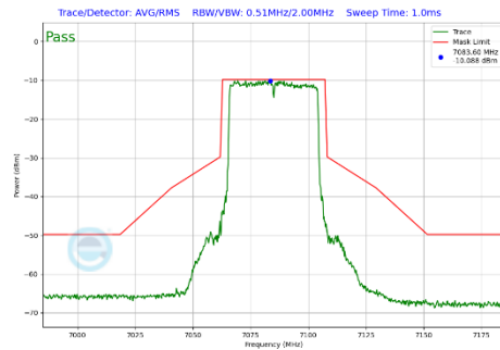
Plot 7-418 In-Band Emission Plot SDM Primary Antenna 3a (40MHz BW 802.11be(SU) (UNII Band 8) - Ch.227)
