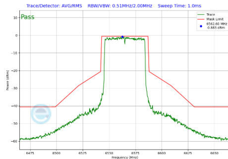
Plot 7-386 In-Band Emission Plot CDD Primary Antenna 3a (40MHz BW 802.11be(SU) (UNII Band 7) - Ch.123)
