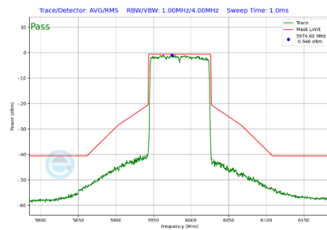
Plot 7-371 In-Band Emission Plot CDD Primary Antenna 3a (80MHz BW 802.11be(SU) (UNII Band 5) - Ch.7)
