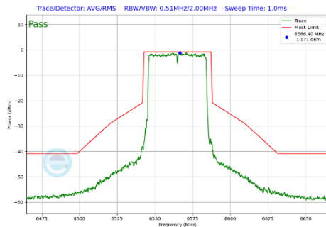
Plot 7-382 In-Band Emission Plot CDD Primary Antenna 3c (40MHz BW 802.11be(SU) (UNII Band 7) - Ch.123)
