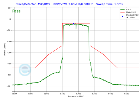
Plot 7-396 In-Band Emission Plot SDM Primary Antenna 3a (160MHz BW 802.11be(SU) (UNII Band 5) - Ch.47)
