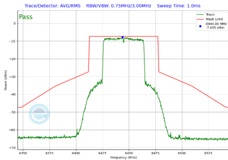
Plot 7-454 In-Band Emission Plot SDM Diversity Antenna 3c (40MHz BW 802.11be(SU) (UNII Band 6) - Ch.99)
