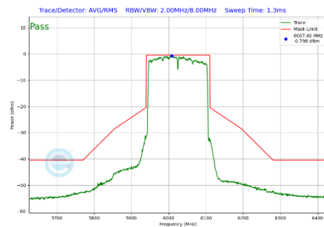
Plot 7-372 In-Band Emission Plot CDD Primary Antenna 3a (160MHz BW 802.11be(SU) (UNII Band 5) - Ch.15)
