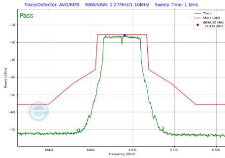
Plot 7-461 In-Band Emission Plot CDD Diversity Antenna 3c (20MHz BW 802.11a (UNII Band 7) - Ch.149)
