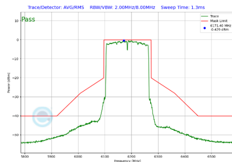
Plot 7-428 In-Band Emission Plot CDD Diversity Antenna 1b (160MHz BW 802.11be(SU) (UNII Band 5) - Ch.47)
