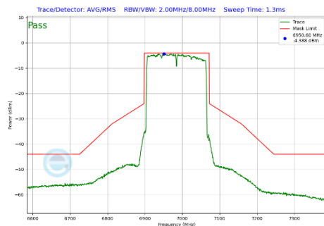
Plot 7-416 In-Band Emission Plot SDM Primary Antenna 3c (160MHz BW 802.11be(SU) (UNII Band 8) - Ch.207)
