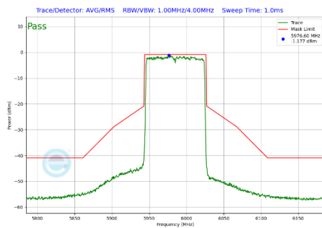
Plot 7-367 In-Band Emission Plot CDD Primary Antenna 3c (80MHz BW 802.11be(SU) (UNII Band 5) - Ch.7)
