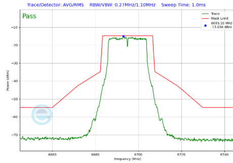
Plot 7-465 In-Band Emission Plot CDD Diversity Antenna 1b (20MHz BW 802.11a (UNII Band 7) - Ch.149)
