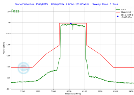
Plot 7-368 In-Band Emission Plot CDD Primary Antenna 3c (160MHz BW 802.11be(SU) (UNII Band 5) - Ch.15)
