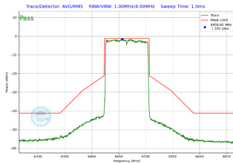
Plot 7-431 In-Band Emission Plot CDD Diversity Antenna 3c (80MHz BW 802.11be(SU) (UNII Band 6) - Ch.103)
