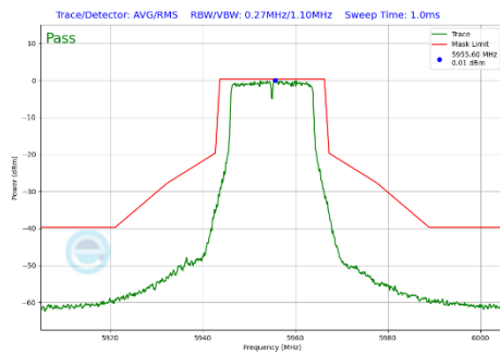
Plot 7-421 In-Band Emission Plot CDD Diversity Antenna 3c (20MHz BW 802.11a (UNII Band 5) - Ch.1)
