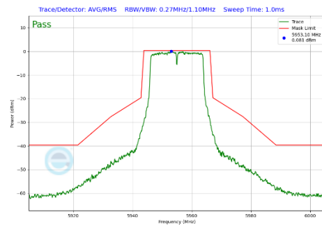
Plot 7-369 In-Band Emission Plot CDD Primary Antenna 3a (20MHz BW 802.11a (UNII Band 5) - Ch.1)
