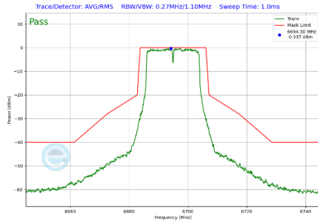
Plot 7-437 In-Band Emission Plot CDD Diversity Antenna 3c (20MHz BW 802.11a (UNII Band 7) - Ch.149)
