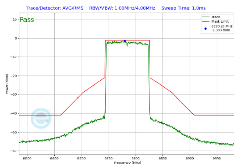
Plot 7-439 In-Band Emission Plot CDD Diversity Antenna 3c (80MHz BW 802.11be(SU) (UNII Band 7) - Ch.167)
