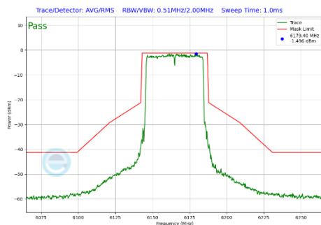
Plot 7-422 In-Band Emission Plot CDD Diversity Antenna 3c (40MHz BW 802.11be(SU) (UNII Band 5) - Ch.43)
