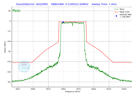
Plot 7-370 In-Band Emission Plot CDD Primary Antenna 3a (40MHz BW 802.11be(SU) (UNII Band 5) - Ch.3)
