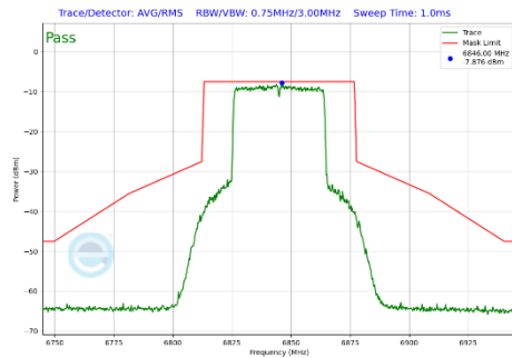
Plot 7-406 In-Band Emission Plot SDM Primary Antenna 3c (40MHz BW 802.11be(SU) (UNII Band 7) - Ch.179)
