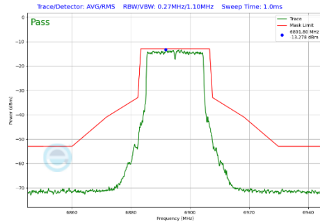
Plot 7-417 In-Band Emission Plot SDM Primary Antenna 3a (20MHz BW 802.11be(SU) (UNII Band 8) - Ch.189)
