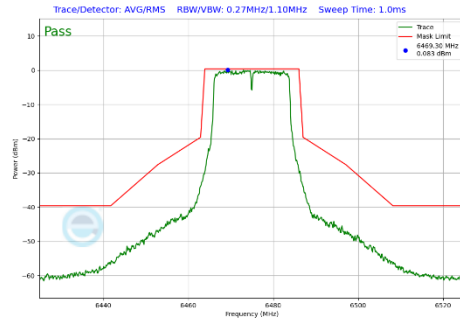
Plot 7-433 In-Band Emission Plot CDD Diversity Antenna 1b (20MHz BW 802.11a (UNII Band 6) - Ch.105)
