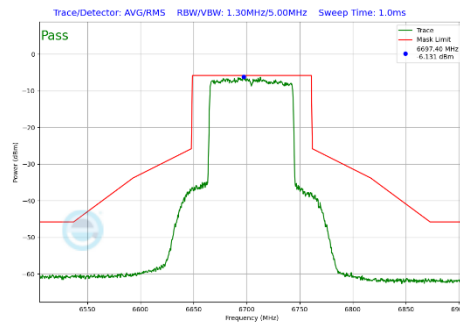
Plot 7-411 In-Band Emission Plot SDM Primary Antenna 3a (80MHz BW 802.11be(SU) (UNII Band 7) - Ch.151)
