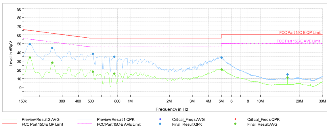
Plot 7-435. AC Line Conducted Plot with 802.11be SDM Primary – Ch.61 (L1), with AC/DC Adapter
