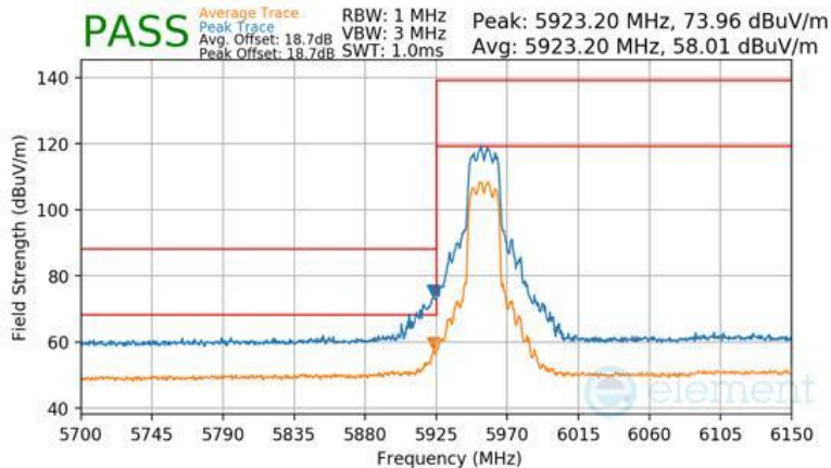
Plot 7-635 SDM Diversity Radiated Lower Band Edge (Peak & Average – UNII Band 5)
