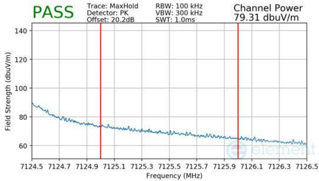
Plot 7-619 SDM Primary Radiated Integrated Band Edge (Peak – UNII Band 8)
