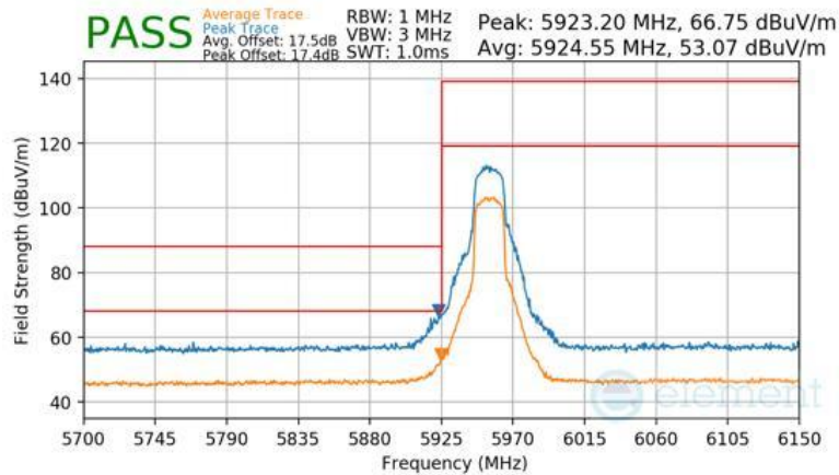
Plot 7-595 Antenna 1b Radiated Lower Band Edge (Peak & Average – UNII Band 5)
