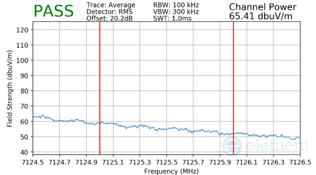
Plot 7-616 SDM Primary Radiated Integrated Band Edge (Average – UNII Band 8)
