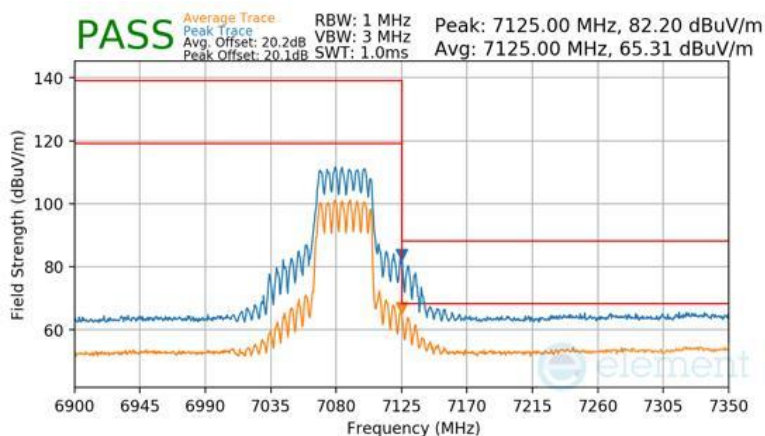
Plot 7-623 SDM Primary Radiated Upper Band Edge (Peak & Average – UNII Band 8)
