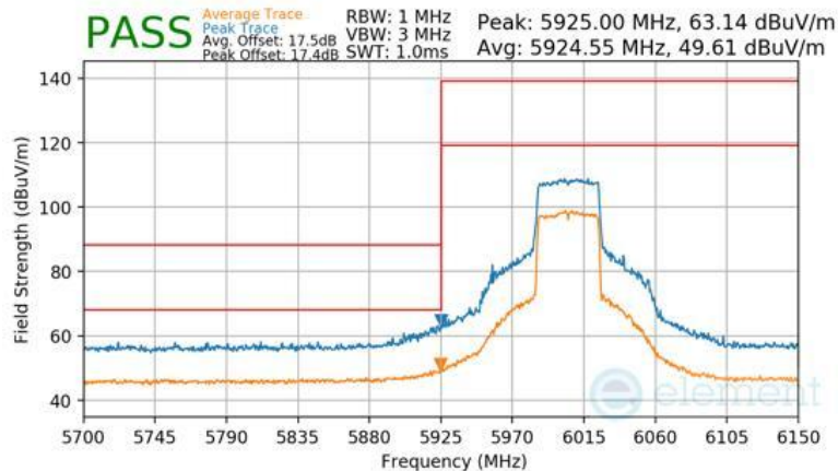
Plot 7-604 Antenna 1b Radiated Lower Band Edge (Peak & Average – UNII Band 5)
