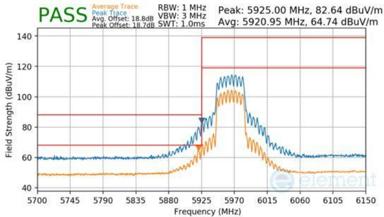
Plot 7-621 SDM Primary Radiated Lower Band Edge (Peak & Average – UNII Band 5)
