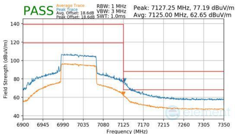
Plot 7-608 Antenna 1b Radiated Upper Band Edge (Peak & Average – UNII Band 8)
