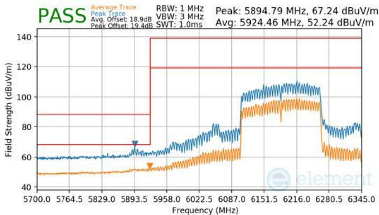
Plot 7-628 SDM Primary Radiated Lower Band Edge (Peak & Average – UNII Band 5)
