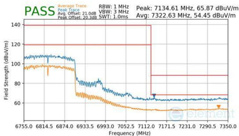
Plot 7-647 SDM Diversity Radiated Upper Band Edge (Peak & Average – UNII Band 7)
