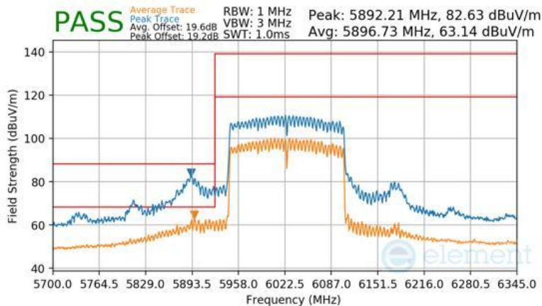
Plot 7-645 SDM Diversity Radiated Lower Band Edge (Peak & Average – UNII Band 5)
