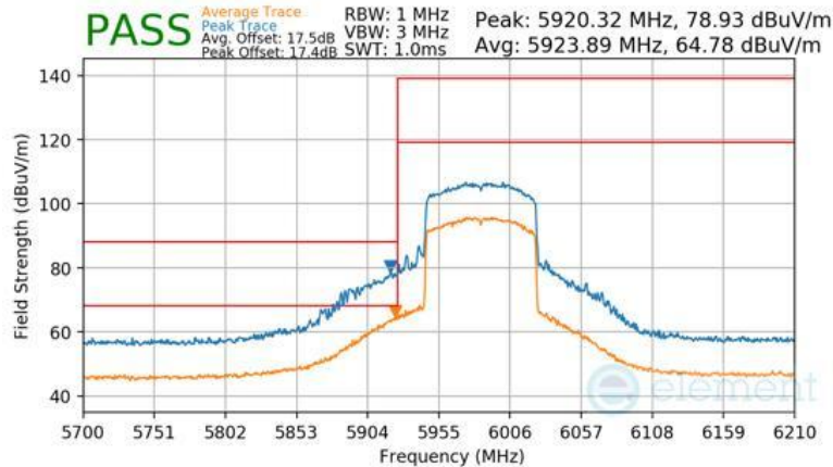
Plot 7-606 Antenna 1b Radiated Lower Band Edge (Peak & Average – UNII Band 5)
