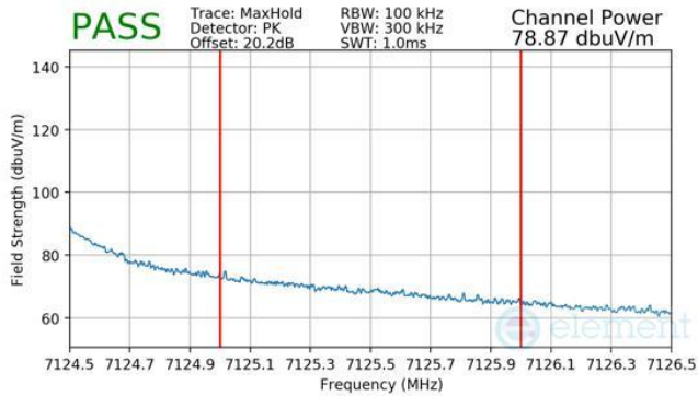
Plot 7-637 SDM Diversity Radiated Integrated Band Edge (Peak – UNII Band 8)
