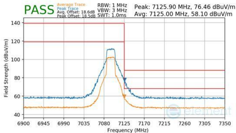
Plot 7-596 Antenna 1b Radiated Upper Band Edge (Peak & Average – UNII Band 8)
