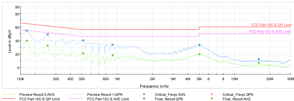
Plot 7-652. AC Line Conducted Plot with 802.11be SDM Primary – Ch. 45 (N), with AC/DC adapter
