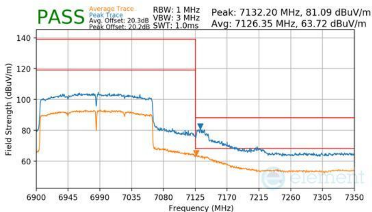
Plot 7-594 Antenna 3a Radiated Upper Band Edge (Peak & Average – UNII Band 8)
