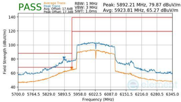
Plot 7-609 Antenna 1b Radiated Lower Band Edge (Peak & Average – UNII Band 5)
