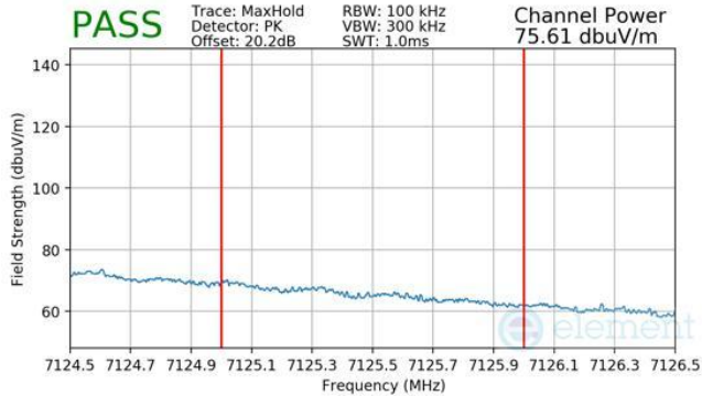
Plot 7-615 SDM Primary Radiated Integrated Band Edge (Peak – UNII Band 8)
