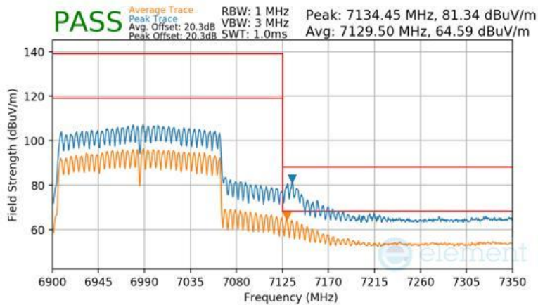
Plot 7-630 SDM Primary Radiated Upper Band Edge (Peak & Average – UNII Band 8)
