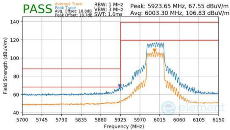
Plot 7-640 SDM Diversity Radiated Lower Band Edge (Peak & Average – UNII Band 5)
