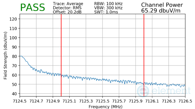
Plot 7-620 SDM Primary Radiated Integrated Band Edge (Average – UNII Band 8)
