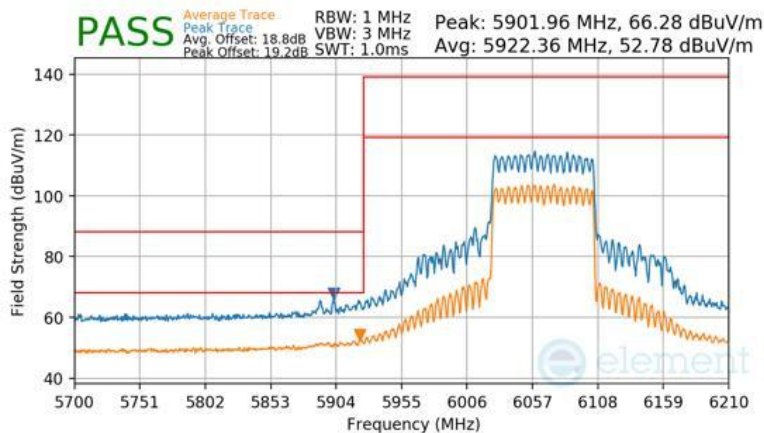
Plot 7-643 SDM Diversity Radiated Lower Band Edge (Peak & Average – UNII Band 5)
