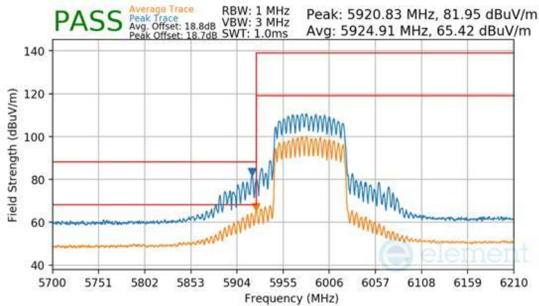
Plot 7-624 SDM Primary Radiated Lower Band Edge (Peak & Average – UNII Band 5)
