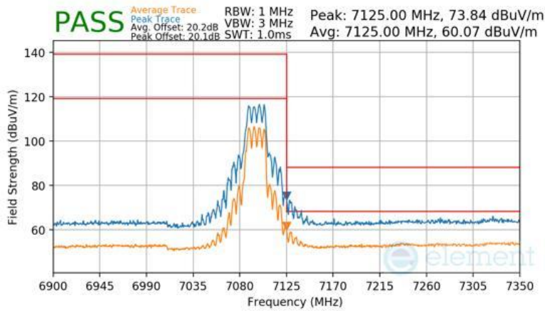
Plot 7-618 SDM Primary Radiated Upper Band Edge (Peak & Average – UNII Band 8)
