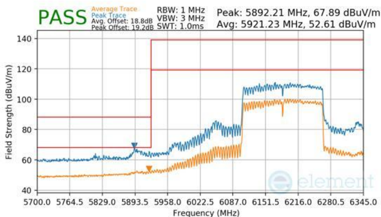
Plot 7-646 SDM Diversity Radiated Lower Band Edge (Peak & Average – UNII Band 5)
