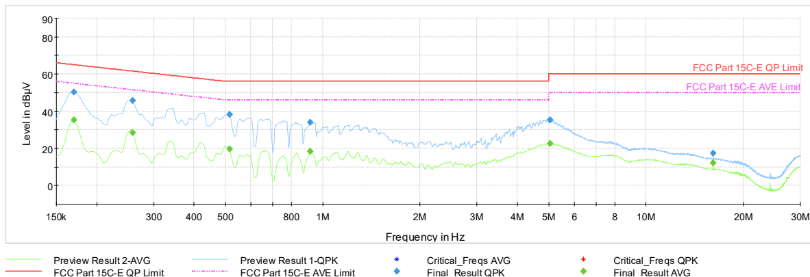
Plot 7-651. AC Line Conducted Plot with 802.11be SDM Primary – Ch.45 (L1), with AC/DC adapter
