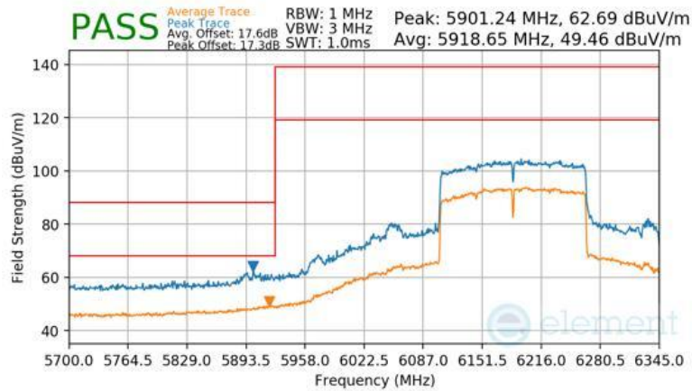
Plot 7-610 Antenna 1b Radiated Lower Band Edge (Peak & Average – UNII Band 5)
