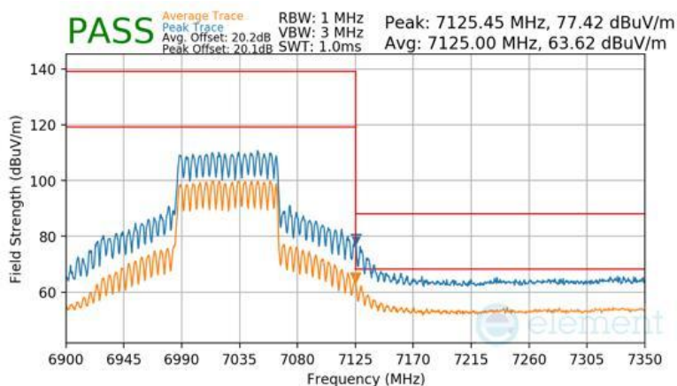
Plot 7-626 SDM Primary Radiated Upper Band Edge (Peak & Average – UNII Band 8)
