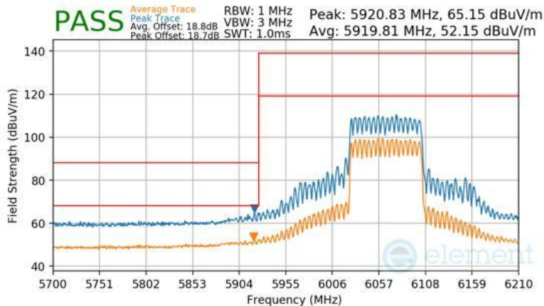
Plot 7-625 SDM Primary Radiated Lower Band Edge (Peak & Average – UNII Band 5)
