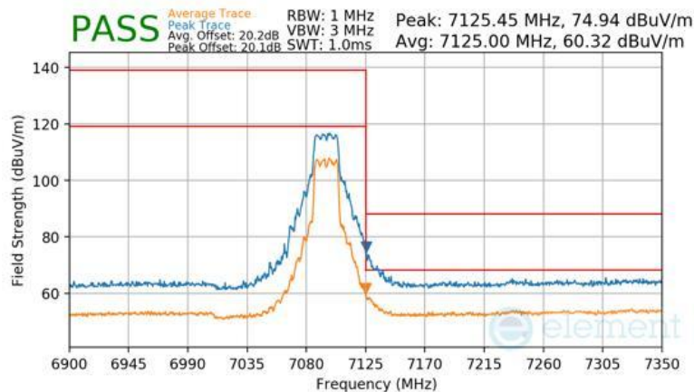
Plot 7-632 CDD Diversity Radiated Upper Band Edge (Peak & Average – UNII Band 8)
