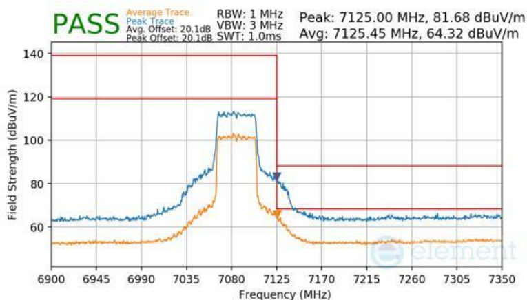
Plot 7-641 SDM Diversity Radiated Upper Band Edge (Peak & Average – UNII Band 8)
