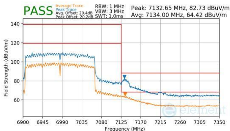
Plot 7-648 SDM Diversity Radiated Upper Band Edge (Peak & Average – UNII Band 8)
