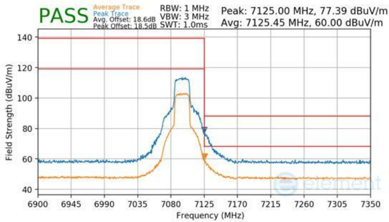
Plot 7-600 Antenna 1b Radiated Upper Band Edge (Peak & Average – UNII Band 8)
