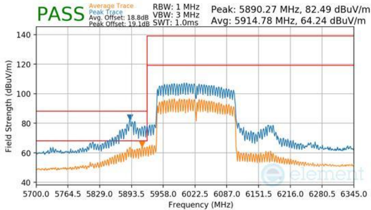
Plot 7-627 SDM Primary Radiated Lower Band Edge (Peak & Average – UNII Band 5)
