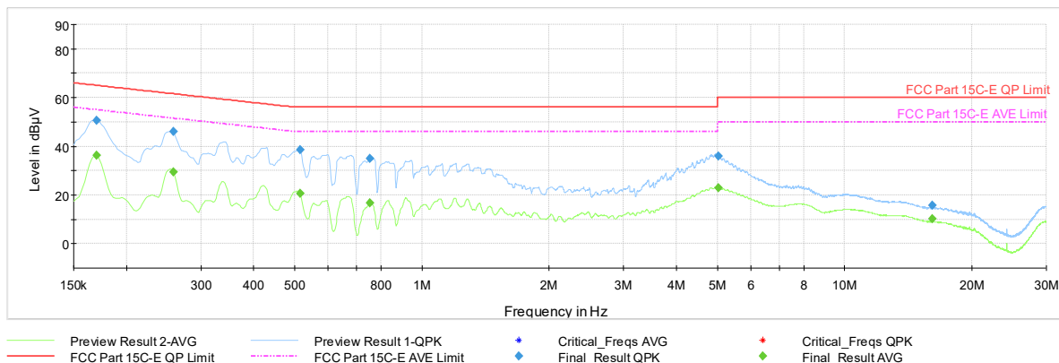
Plot 7-654. AC Line Conducted Plot with 802.11be SDM Diversity – Ch. 45 (N), with AC/DC adapter
