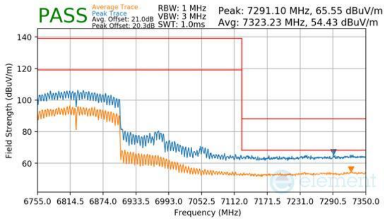
Plot 7-629 SDM Primary Radiated Upper Band Edge (Peak & Average – UNII Band 7)
