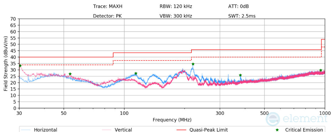
Plot 7-649. Radiated Spurious Emissions below 1GHz SDM Primary, 802.11be, Ch.45 with Charger
