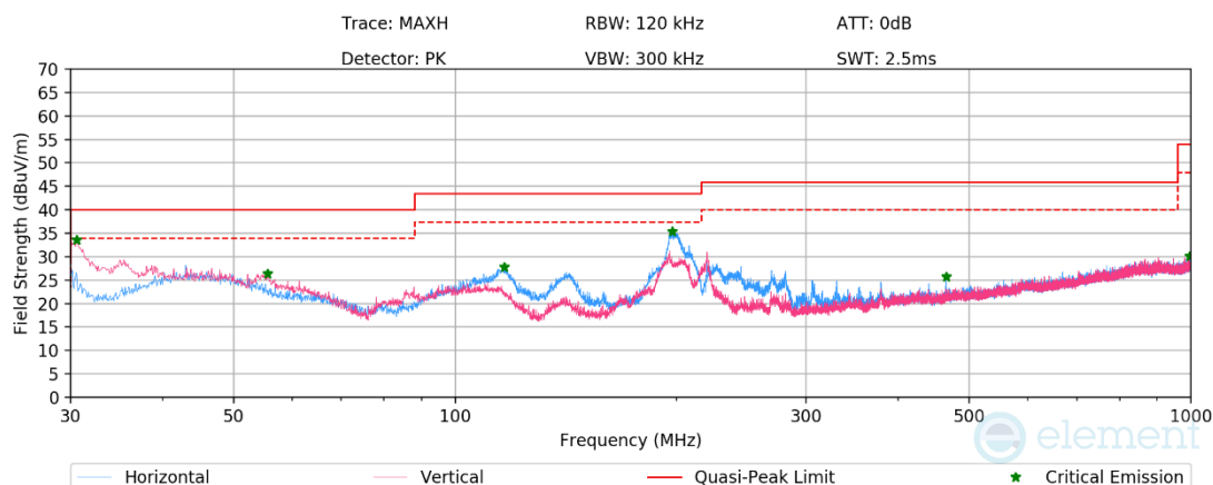
Plot 7-650. Radiated Spurious Emissions below 1GHz SDM Diversity, 802.11be, Ch.45 with Charger
