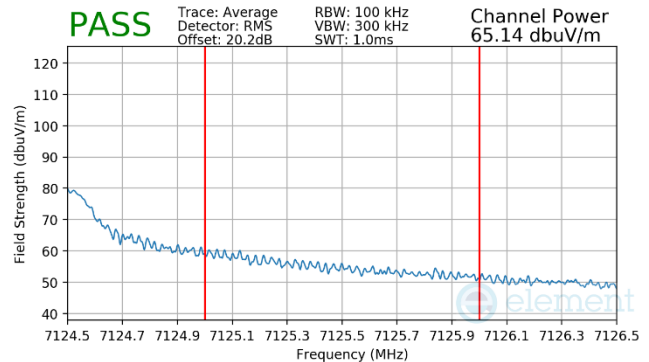
Plot 7-638 SDM Diversity Radiated Integrated Band Edge (Average – UNII Band 8)
