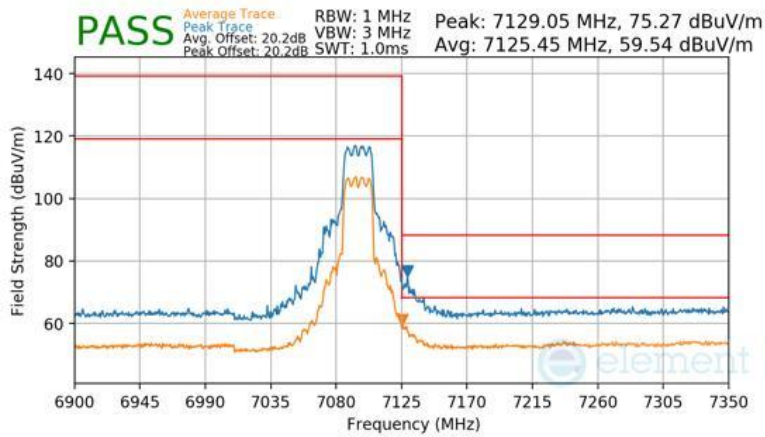
Plot 7-636 SDM Diversity Radiated Upper Band Edge (Peak & Average – UNII Band 8)
