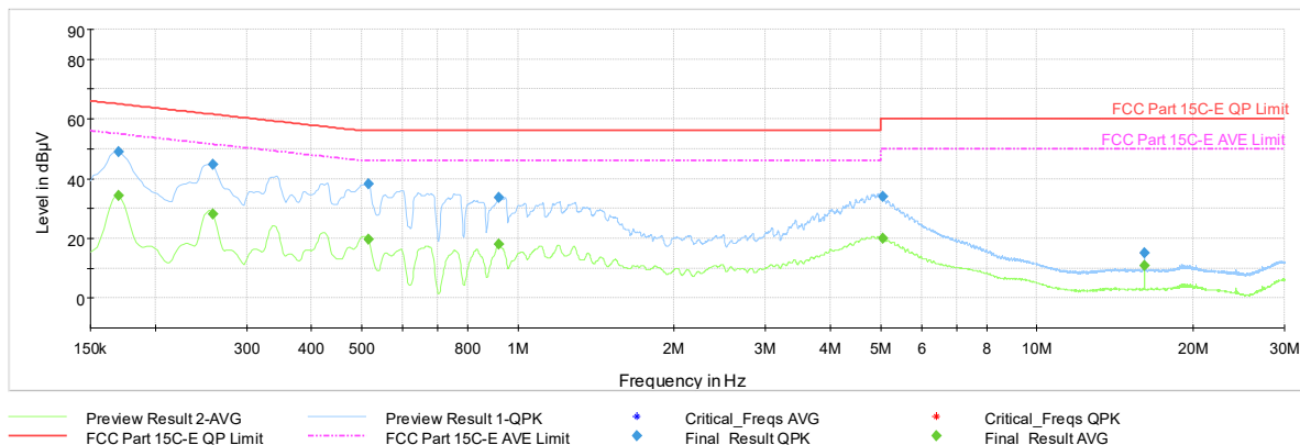
Plot 7-653. AC Line Conducted Plot with 802.11be SDM Diversity – Ch.45 (L1), with AC/DC adapter
