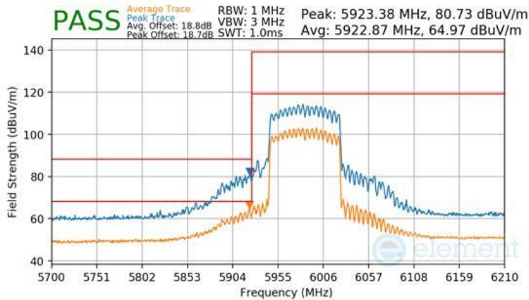
Plot 7-642 SDM Diversity Radiated Lower Band Edge (Peak & Average – UNII Band 5)
