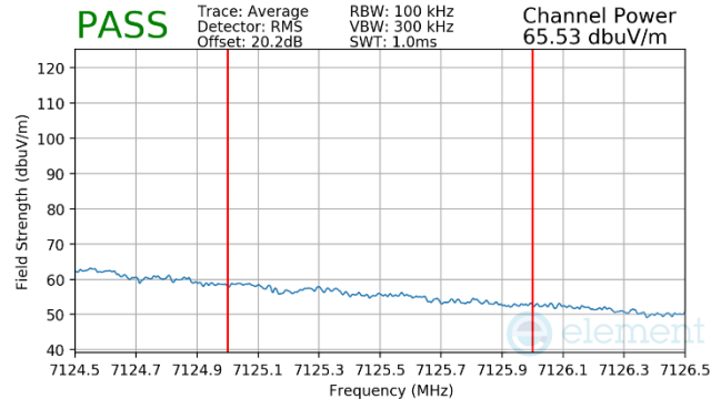
Plot 7-634 CDD Diversity Radiated Integrated Band Edge (Average – UNII Band 8)
