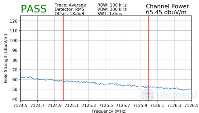
Plot 7-598 Antenna 1b Radiated Integrated Band Edge (Average – UNII Band 8)
