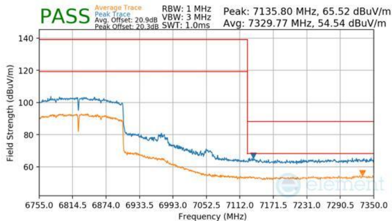
Plot 7-593 Antenna 3a Radiated Upper Band Edge (Peak & Average – UNII Band 7)
