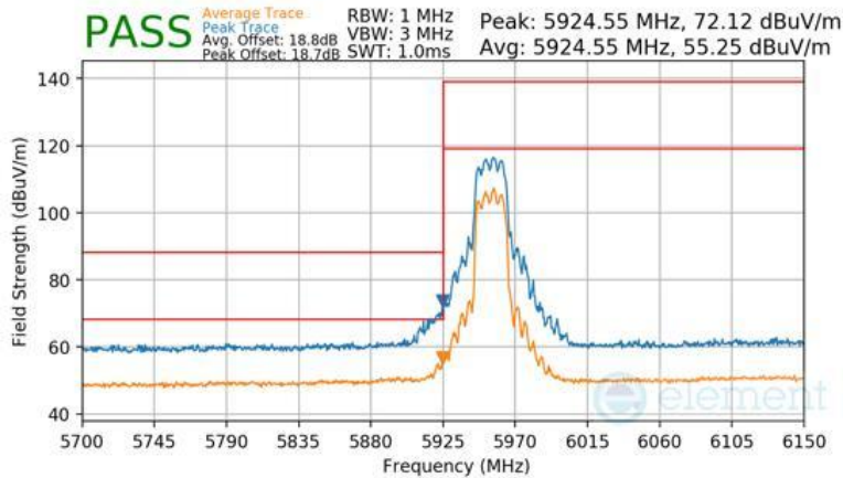
Plot 7-617 SDM Primary Radiated Lower Band Edge (Peak & Average – UNII Band 5)
