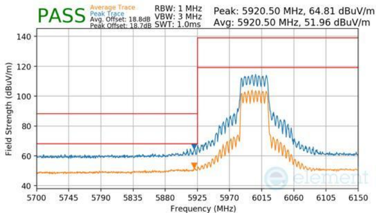
Plot 7-622 SDM Primary Radiated Lower Band Edge (Peak & Average – UNII Band 5)
