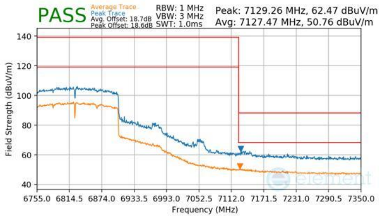
Plot 7-611 Antenna 1b Radiated Upper Band Edge (Peak & Average – UNII Band 7)
