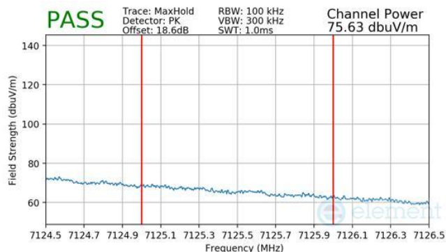
Plot 7-597 Antenna 1b Radiated Integrated Band Edge (Peak – UNII Band 8)
