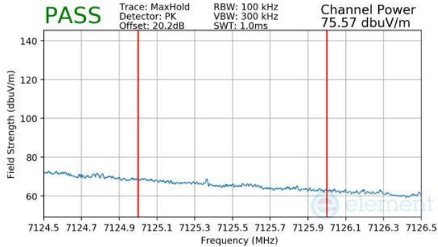
Plot 7-633 CDD Diversity Radiated Integrated Band Edge (Peak – UNII Band 8)
