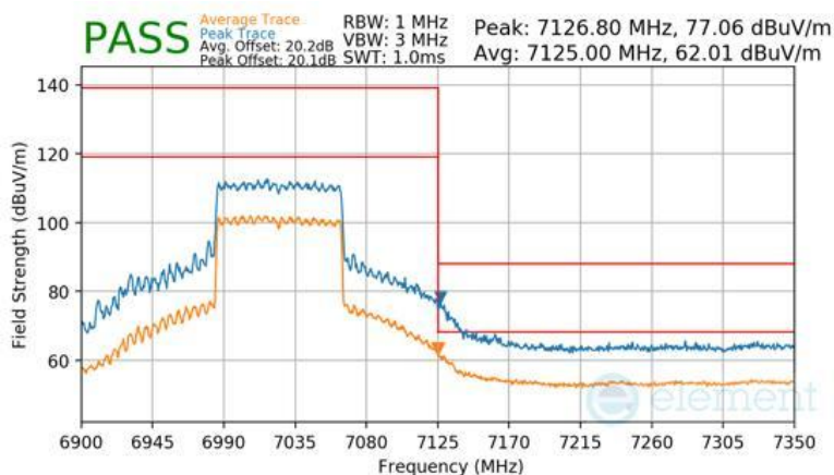
Plot 7-644 SDM Diversity Radiated Upper Band Edge (Peak & Average – UNII Band 8)
