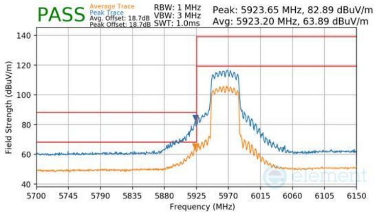
Plot 7-639 SDM Diversity Radiated Lower Band Edge (Peak & Average – UNII Band 5)
