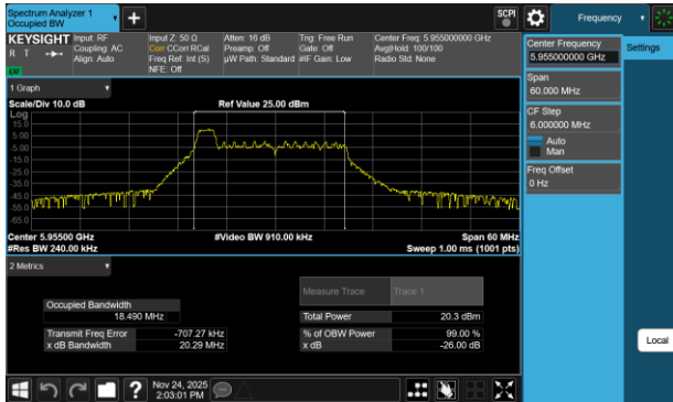
Plot 7-1 26dB BW & 99% OBW Antenna 3c (20MHz BW 802.11be(RU) RU26 Index0 - Ch.1)
