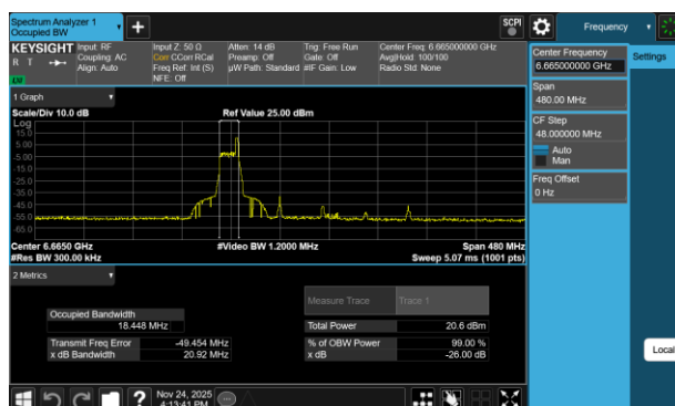
Plot 7-26 26dB BW & 99% OBW Antenna 3c (160MHz BW 802.11be(RU) RU26 Index17 - Ch.143)
