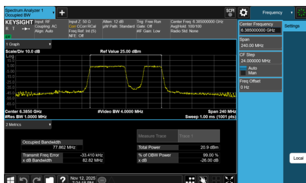
Plot 7-39 26dB BW & 99% OBW Antenna 3c (80MHz BW 802.11be(RU) RU484+242 Index92 - Ch.87)
