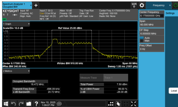
Plot 7-34 26dB BW & 99% OBW Antenna 3c (20MHz BW 802.11be(RU) RU26 Index0 - Ch.45)
