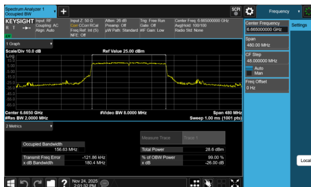
Plot 7-33 26dB BW & 99% OBW Antenna 3c (160MHz BW 802.11be(RU) RU996X2 Index68 - Ch.143)
