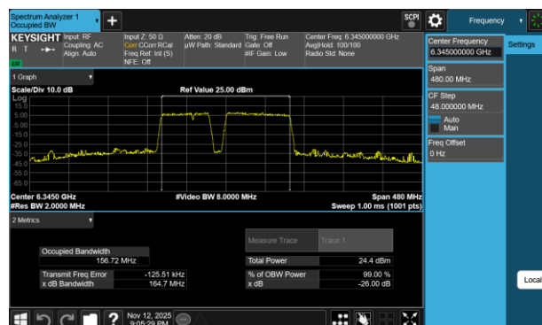
Plot 7-40 26dB BW & 99% OBW Antenna 3c (160MHz BW 802.11be(RU) RU996+484+242 Index99 - Ch.79)
