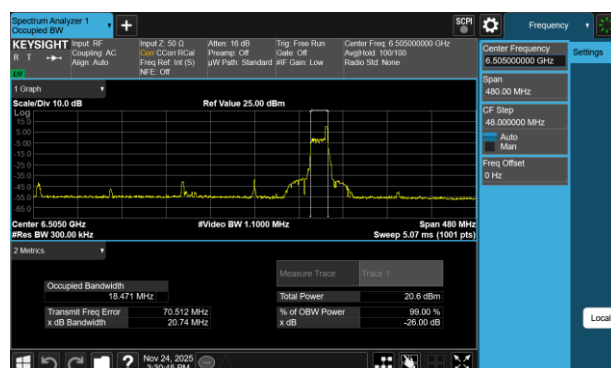
Plot 7-15 26dB BW & 99% OBW Antenna 3c (160MHz BW 802.11be(RU) RU26 Index36 - Ch.111)
