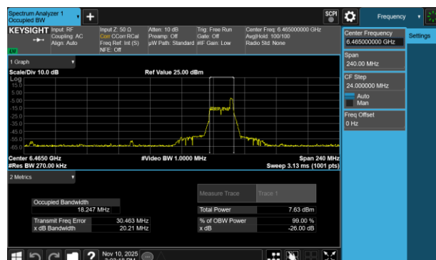
Plot 7-47 26dB BW & 99% OBW Antenna 3c (80MHz BW 802.11be(RU) RU26 Index36 - Ch.103)
