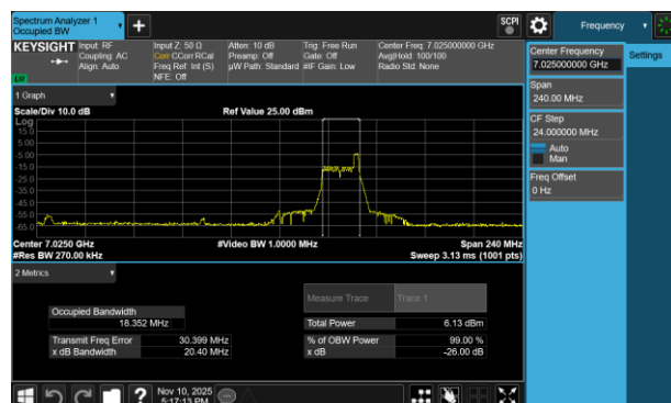
Plot 7-69 26dB BW & 99% OBW Antenna 3c (80MHz BW 802.11be(RU) RU26 Index36 - Ch.215)
