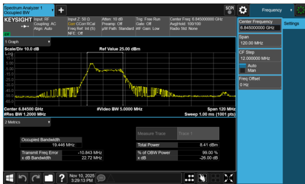
Plot 7-57 26dB BW & 99% OBW Antenna 3c (40MHz BW 802.11be(RU) RU26 Index0 - Ch.179)
