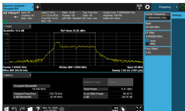
Plot 7-67 26dB BW & 99% OBW Antenna 3c (20MHz BW 802.11be(RU) RU26 Index0 - Ch.229)
