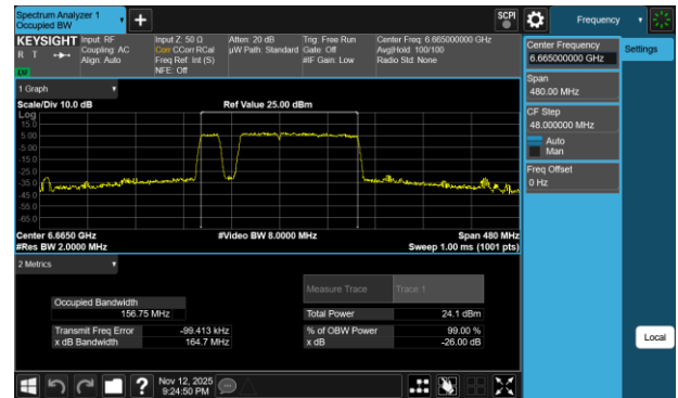
Plot 7-62 26dB BW & 99% OBW Antenna 3c (160MHz BW 802.11be(RU) RU996+484+242 Index97 - Ch.143)
