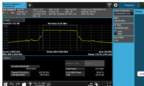
Plot 7-77 26dB BW & 99% OBW Antenna 3c (160MHz BW 802.11be(RU) RU996X2 Index68 - Ch.207)
