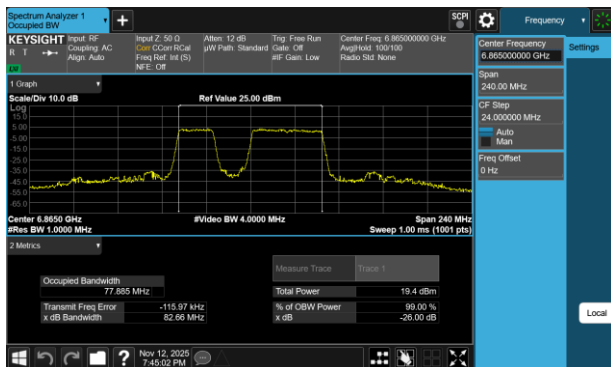
Plot 7-61 26dB BW & 99% OBW Antenna 3c (80MHz BW 802.11be(RU) RU484+242 Index91 - Ch.183)
