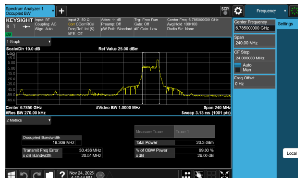
Plot 7-25 26dB BW & 99% OBW Antenna 3c (80MHz BW 802.11be(RU) RU26 Index36 - Ch.167)
