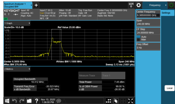
Plot 7-36 26dB BW & 99% OBW Antenna 3c (80MHz BW 802.11be(RU) RU26 Index0 - Ch.87)
