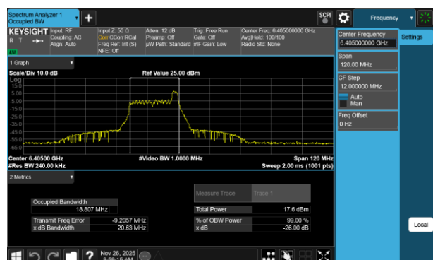
Plot 7-79 26dB BW & 99% OBW Antenna 3a (40MHz BW 802.11be(RU) RU26 Index8 - Ch.91)
