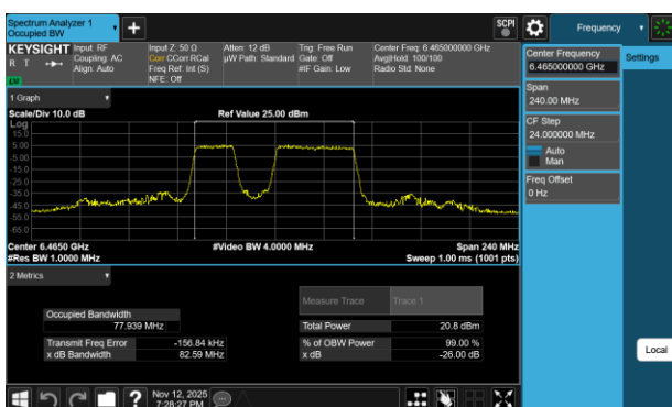
Plot 7-50 26dB BW & 99% OBW Antenna 3c (80MHz BW 802.11be(RU) RU484+242 Index91 - Ch.103)
