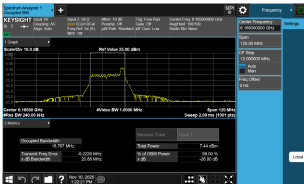
Plot 7-35 26dB BW & 99% OBW Antenna 3c (40MHz BW 802.11be(RU) RU26 Index8 - Ch.43)
