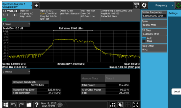
Plot 7-60 26dB BW & 99% OBW Antenna 3c (20MHz BW 802.11be(RU) RU106+26 Index82 - Ch.149)
