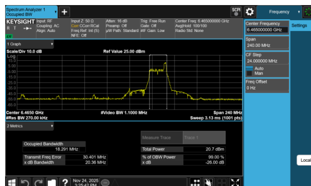
Plot 7-14 26dB BW & 99% OBW Antenna 3c (80MHz BW 802.11be(RU) RU26 Index36 - Ch.103)
