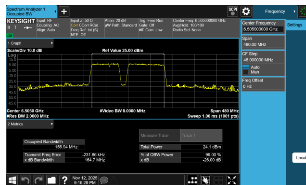
Plot 7-51 26dB BW & 99% OBW Antenna 3c (160MHz BW 802.11be(RU) RU996+484+242 Index99 - Ch.111)
