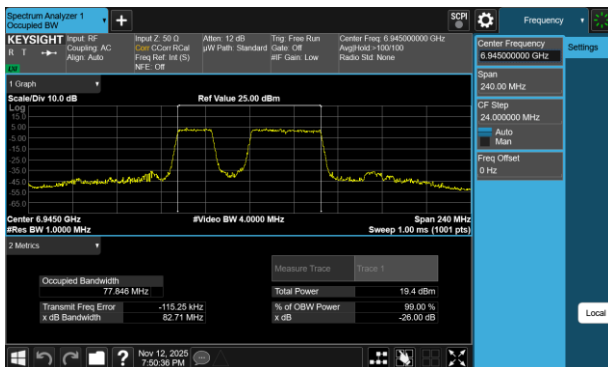
Plot 7-72 26dB BW & 99% OBW Antenna 3c (80MHz BW 802.11be(RU) RU484+242 Index91 - Ch.199)
