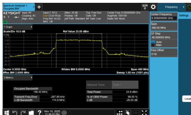
Plot 7-55 26dB BW & 99% OBW Antenna 3c (160MHz BW 802.11be(RU) RU996X2 Index68 - Ch.111)
