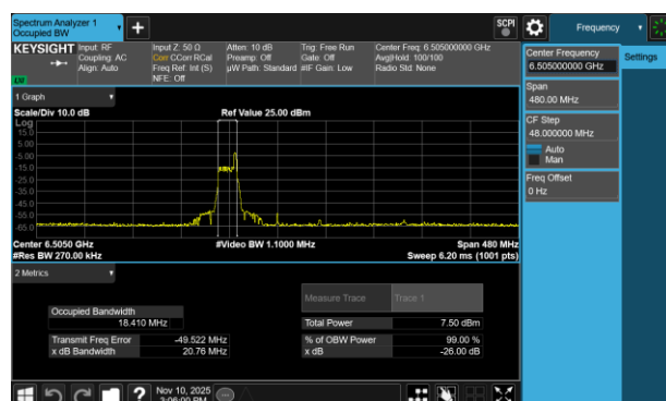
Plot 7-48 26dB BW & 99% OBW Antenna 3c (160MHz BW 802.11be(RU) RU26 Index17 - Ch.111)
