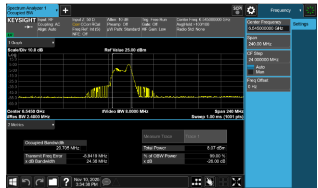
Plot 7-58 26dB BW & 99% OBW Antenna 3c (80MHz BW 802.11be(RU) RU26 Index17 - Ch.119)
