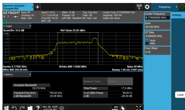
Plot 7-78 26dB BW & 99% OBW Antenna 3a (20MHz BW 802.11be(RU) RU26 Index8 - Ch.45)
