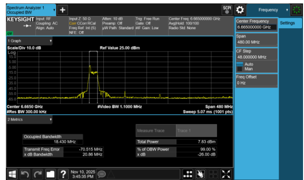
Plot 7-59 26dB BW & 99% OBW Antenna 3c (160MHz BW 802.11be(RU) RU26 Index0 - Ch.143)
