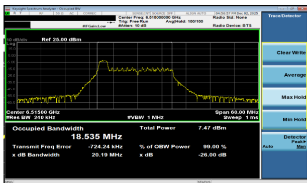
Plot 7-45 26dB BW & 99% OBW Antenna 3c (20MHz BW 802.11be(RU) RU26 Index0 - Ch.113)
