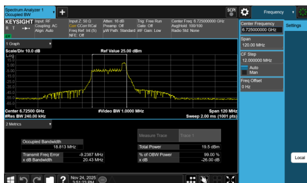
Plot 7-24 26dB BW & 99% OBW Antenna 3c (40MHz BW 802.11be(RU) RU26 Index8 - Ch.155)
