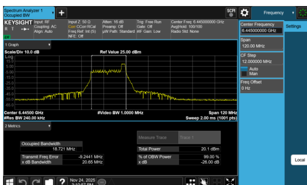
Plot 7-13 26dB BW & 99% OBW Antenna 3c (40MHz BW 802.11be(RU) RU26 Index8 - Ch.99)
