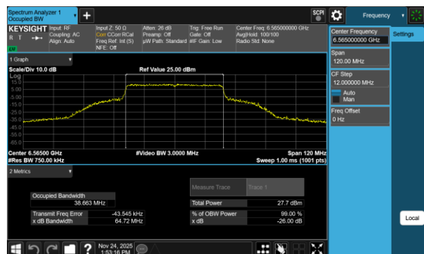
Plot 7-31 26dB BW & 99% OBW Antenna 3c (40MHz BW 802.11be(RU) RU484 Index65 - Ch.123)
