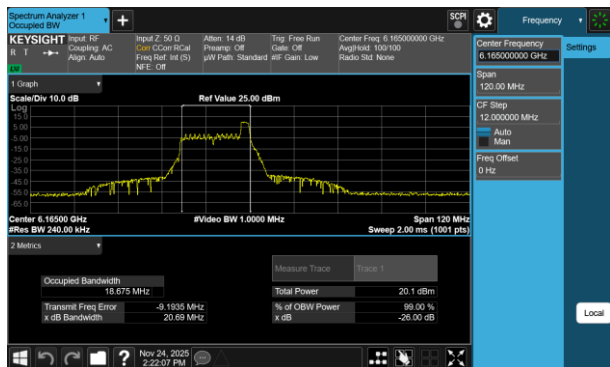
Plot 7-2 26dB BW & 99% OBW Antenna 3c (40MHz BW 802.11be(RU) RU26 Index8 - Ch.43)
