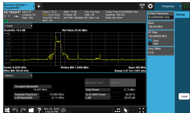
Plot 7-4 26dB BW & 99% OBW Antenna 3c (160MHz BW 802.11be(RU) RU26 Index0 - Ch.15)
