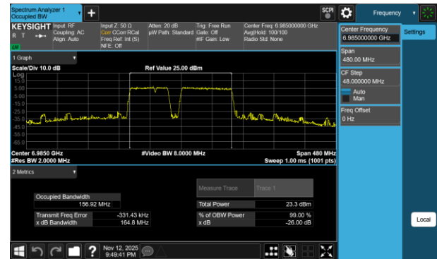
Plot 7-73 26dB BW & 99% OBW Antenna 3c (160MHz BW 802.11be(RU) RU996+484+242 Index99 - Ch.207)
