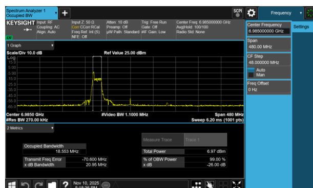
Plot 7-70 26dB BW & 99% OBW Antenna 3c (160MHz BW 802.11be(RU) RU26 Index0 - Ch.207)
