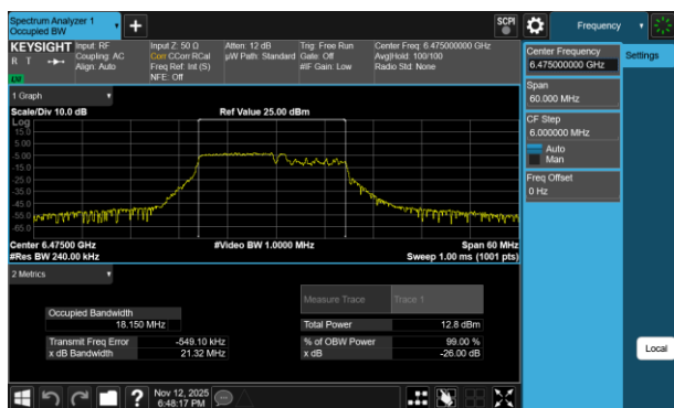
Plot 7-49 26dB BW & 99% OBW Antenna 3c (20MHz BW 802.11be(RU) RU106+26 Index82 - Ch.105)
