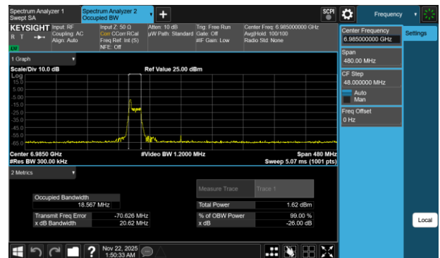
Plot 7-37 26dB BW & 99% OBW Antenna 3c (160MHz BW 802.11be(RU) RU26 Index0 - Ch.207)
