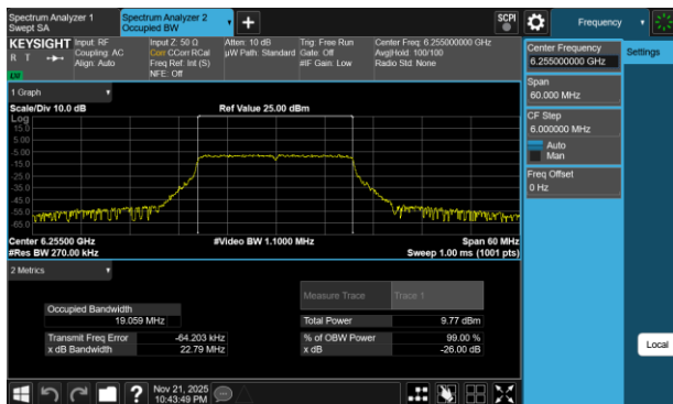
Plot 7-8 26dB BW & 99% OBW Antenna 3c (20MHz BW 802.11be(RU) RU242 Index61 - Ch.61)
