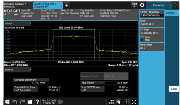
Plot 7-65 26dB BW & 99% OBW Antenna 3a (80MHz BW 802.11be(RU) RU996 Index67 - Ch.103)
