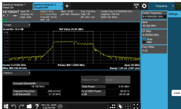
Plot 7-5 26dB BW & 99% OBW Antenna 3c (20MHz BW 802.11be(RU) RU106+26 Index82 - Ch.93)
