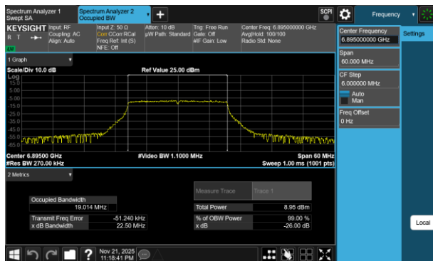
Plot 7-41 26dB BW & 99% OBW Antenna 3c (20MHz BW 802.11be(RU) RU242 Index61 - Ch.189)
