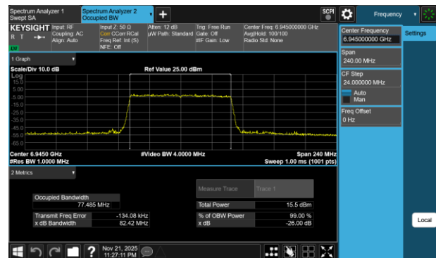
Plot 7-43 26dB BW & 99% OBW Antenna 3c (80MHz BW 802.11be(RU) RU996 Index67 - Ch.199)
