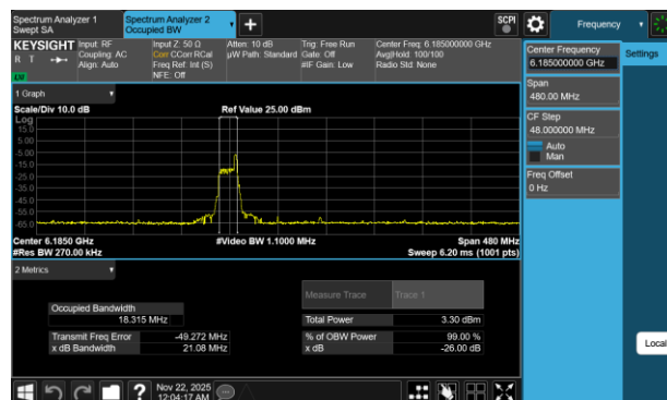
Plot 7-4 26dB BW & 99% OBW Antenna 3c (160MHz BW 802.11be(RU) RU26 Index17 - Ch.47)
