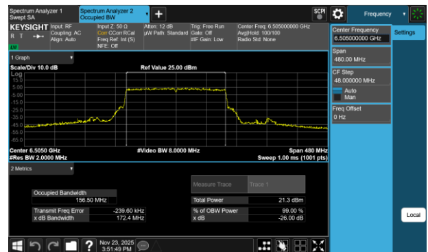
Plot 7-66 26dB BW & 99% OBW Antenna 3a (160MHz BW 802.11be(RU) RU996X2 Index68 - Ch.111)
