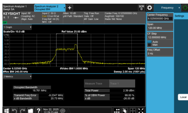
Plot 7-13 26dB BW & 99% OBW Antenna 3c (40MHz BW 802.11be(RU) RU26 Index8 - Ch.115)
