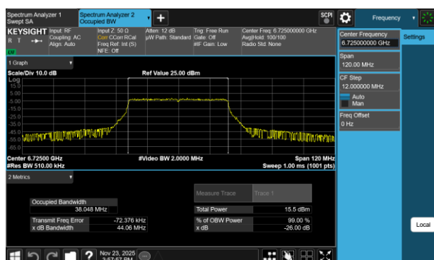
Plot 7-75 26dB BW & 99% OBW Antenna 3a (40MHz BW 802.11be(RU) RU484 Index65 - Ch.155)
