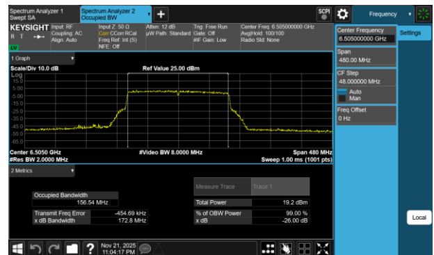
Plot 7-22 26dB BW & 99% OBW Antenna 3c (160MHz BW 802.11be(RU) RU996X2 Index68 - Ch.111)
