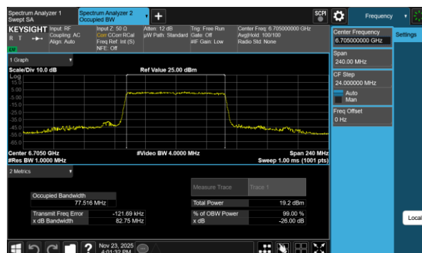
Plot 7-76 26dB BW & 99% OBW Antenna 3a (80MHz BW 802.11be(RU) RU996 Index67 - Ch.151)
