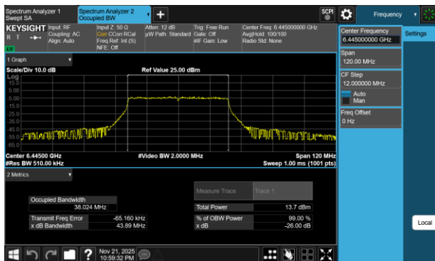
Plot 7-20 26dB BW & 99% OBW Antenna 3c (40MHz BW 802.11be(RU) RU484 Index65 - Ch.99)
