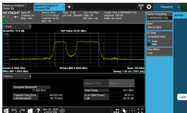
Plot 7-6 26dB BW & 99% OBW Antenna 3c (80MHz BW 802.11be(RU) RU484+242 Index91 - Ch.87)
