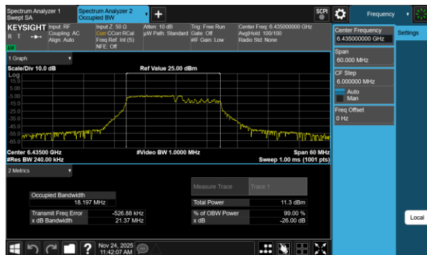
Plot 7-60 26dB BW & 99% OBW Antenna 3a (20MHz BW 802.11be(RU) RU106+26 Index82 - Ch.97)
