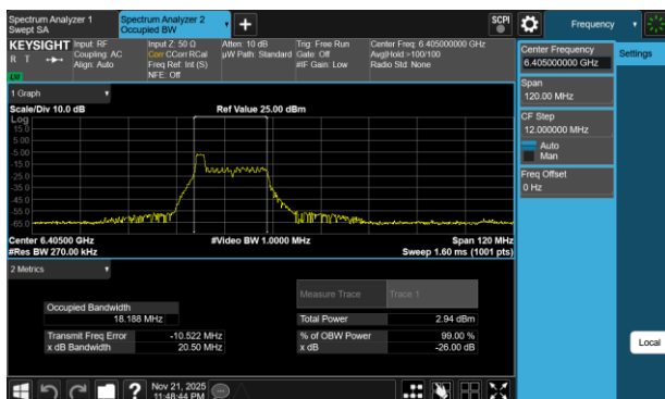
Plot 7-2 26dB BW & 99% OBW Antenna 3c (40MHz BW 802.11be(RU) RU26 Index0 - Ch.91)
