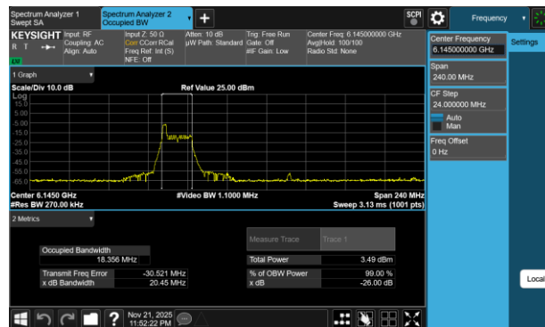
Plot 7-3 26dB BW & 99% OBW Antenna 3c (80MHz BW 802.11be(RU) RU26 Index0 - Ch.39)
