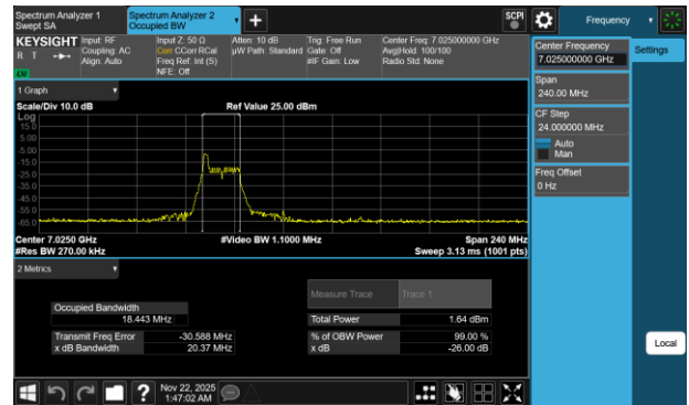
Plot 7-36 26dB BW & 99% OBW Antenna 3c (80MHz BW 802.11be(RU) RU26 Index0 - Ch.215)
