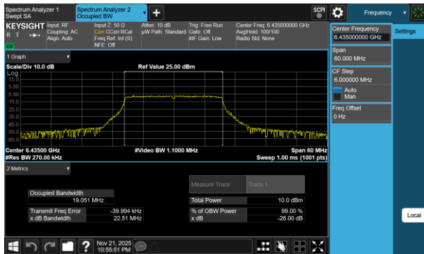
Plot 7-19 26dB BW & 99% OBW Antenna 3c (20MHz BW 802.11be(RU) RU242 Index61 - Ch.97)
