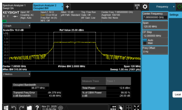
Plot 7-42 26dB BW & 99% OBW Antenna 3c (40MHz BW 802.11be(RU) RU484 Index65 - Ch.227)
