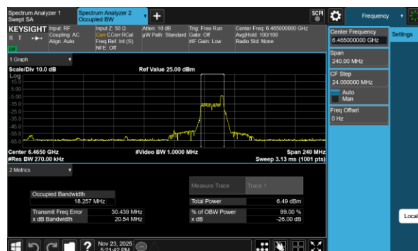
Plot 7-58 26dB BW & 99% OBW Antenna 3a (80MHz BW 802.11be(RU) RU26 Index36 - Ch.103)
