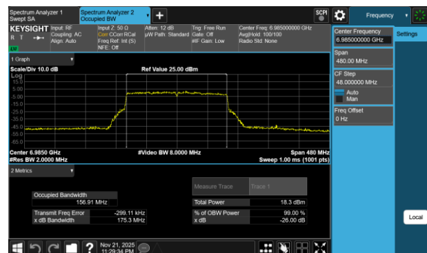
Plot 7-44 26dB BW & 99% OBW Antenna 3c (160MHz BW 802.11be(RU) RU996X2 Index68 - Ch.207)
