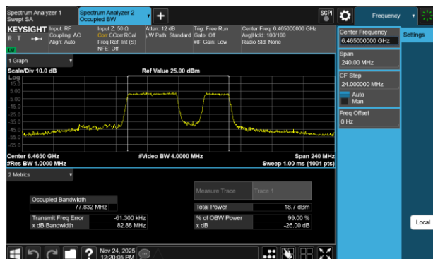
Plot 7-61 26dB BW & 99% OBW Antenna 3a (80MHz BW 802.11be(RU) RU484+242 Index92 - Ch.103)
