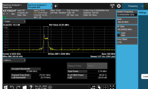
Plot 7-15 26dB BW & 99% OBW Antenna 3c (160MHz BW 802.11be(RU) RU26 Index0 - Ch.111)
