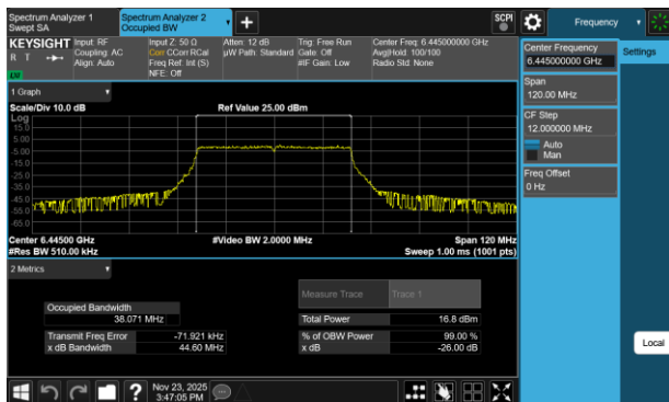
Plot 7-64 26dB BW & 99% OBW Antenna 3a (40MHz BW 802.11be(RU) RU484 Index65 - Ch.99)
