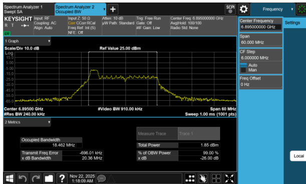
Plot 7-34 26dB BW & 99% OBW Antenna 3c (20MHz BW 802.11be(RU) RU26 Index0 - Ch.189)
