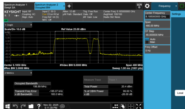
Plot 7-7 26dB BW & 99% OBW Antenna 3c (160MHz BW 802.11be(RU) RU996+484+242 Index98 - Ch.47)
