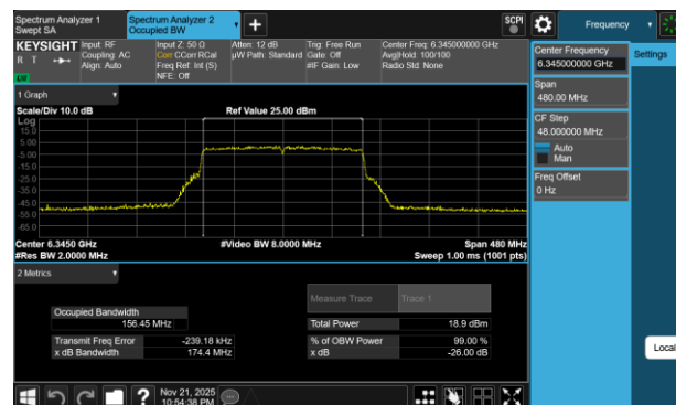
Plot 7-11 26dB BW & 99% OBW Antenna 3c (160MHz BW 802.11be(RU) RU996X2 Index68 - Ch.79)
