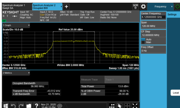
Plot 7-9 26dB BW & 99% OBW Antenna 3c (40MHz BW 802.11be(RU) RU484 Index65 - Ch.35)
