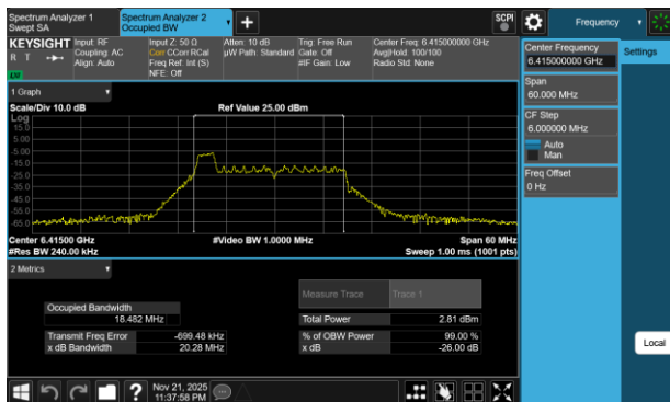
Plot 7-1 26dB BW & 99% OBW Antenna 3c (20MHz BW 802.11be(RU) RU26 Index0 - Ch.93)
