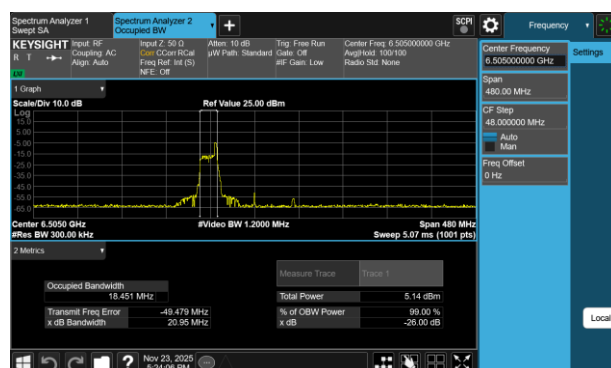
Plot 7-59 26dB BW & 99% OBW Antenna 3a (160MHz BW 802.11be(RU) RU26 Index17 - Ch.111)
