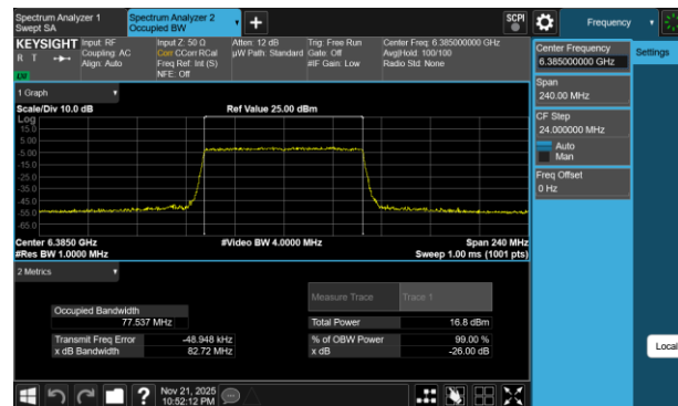
Plot 7-10 26dB BW & 99% OBW Antenna 3c (80MHz BW 802.11be(RU) RU996 Index67 - Ch.87)
