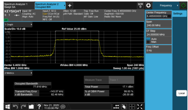
Plot 7-21 26dB BW & 99% OBW Antenna 3c (80MHz BW 802.11be(RU) RU996 Index67 - Ch.103)
