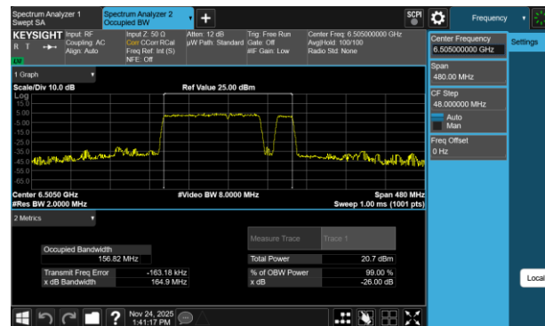
Plot 7-62 26dB BW & 99% OBW Antenna 3a (160MHz BW 802.11be(RU) RU996+484+242 Index98 - Ch.111)
