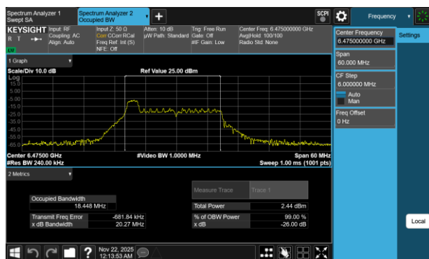
Plot 7-12 26dB BW & 99% OBW Antenna 3c (20MHz BW 802.11be(RU) RU26 Index0 - Ch.105)
