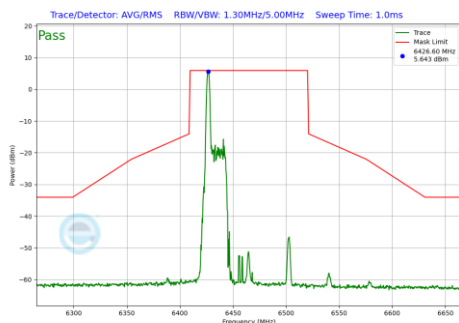
Plot 7-1019 In-Band Emission Plot CDD Primary Antenna 3a (80MHz BW 802.11be(RU) RU26 Index0 (UNII Band 6) - Ch.103)
