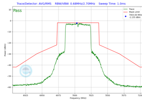
Plot 7-998 In-Band Emission Plot Antenna 1b (40MHz BW 802.11be(RU) RU484 Index65 (UNII Band 8) - Ch.211)
