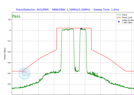
Plot 7-1038 In-Band Emission Plot CDD Primary Antenna 3a (80MHz BW 802.11be(RU) RU484+242 Index92 (UNII Band 6) - Ch.103)
