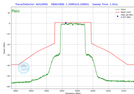
Plot 7-1045 In-Band Emission Plot CDD Primary Antenna 3c (80MHz BW 802.11be(RU) RU996 Index67 (UNII Band 5) - Ch.7)
