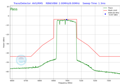
Plot 7-1110 In-Band Emission Plot SDM Primary Antenna 3c (160MHz BW 802.11be(RU) RU996+484+242 Index96 (UNII Band 8) - Ch.207)
