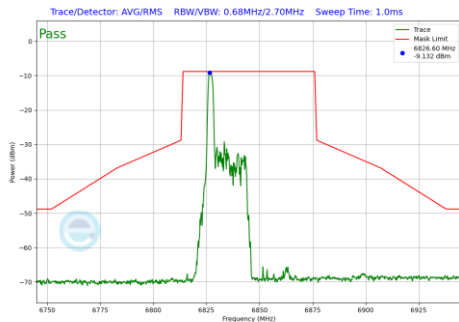
Plot 7-1076 In-Band Emission Plot SDM Primary Antenna 3c (40MHz BW 802.11be(RU) RU26 Index0 (UNII Band 7) - Ch.179)
