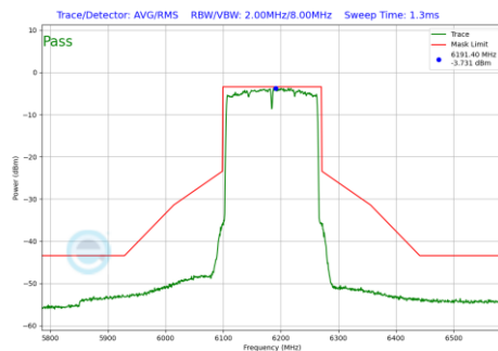
Plot 7-1125 In-Band Emission Plot SDM Primary Antenna 3c (160MHz BW 802.11be(RU) RU996X2 Index68 (UNII Band 5) - Ch.47)
