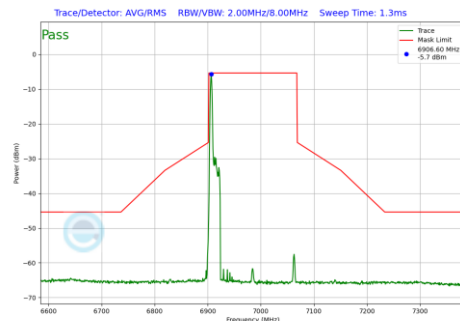
Plot 7-1082 In-Band Emission Plot SDM Primary Antenna 3c (160MHz BW 802.11be(RU) RU26 Index0 (UNII Band 8) - Ch.207)
