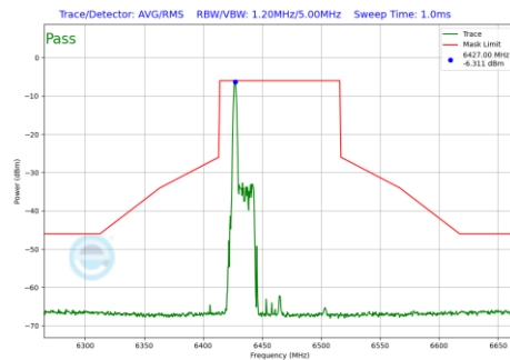
Plot 7-1073 In-Band Emission Plot SDM Primary Antenna 3c (80MHz BW 802.11be(RU) RU26 Index0 (UNII Band 6) - Ch.103)
