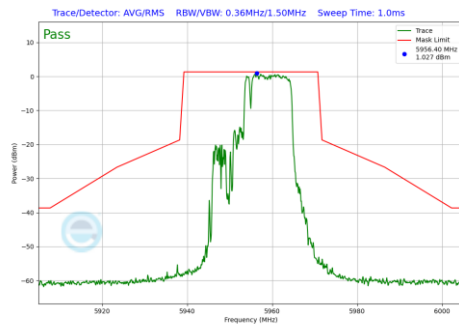
Plot 7-1025 In-Band Emission Plot CDD Primary Antenna 3c (20MHz BW 802.11be(RU) RU106+26 Index83 (UNII Band 5) - Ch.1)
