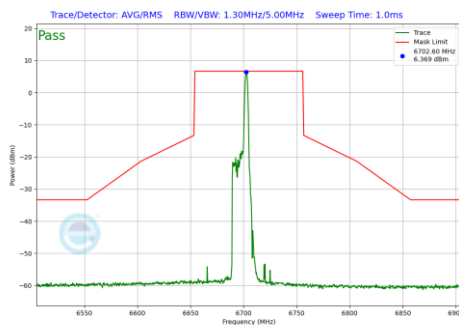
Plot 7-1011 In-Band Emission Plot CDD Primary Antenna 3c (80MHz BW 802.11be(RU) RU26 Index17 (UNII Band 7) - Ch.151)
