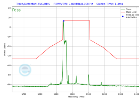
Plot 7-1016 In-Band Emission Plot CDD Primary Antenna 3a (160MHz BW 802.11be(RU) RU26 Index0 (UNII Band 5) - Ch.15)
