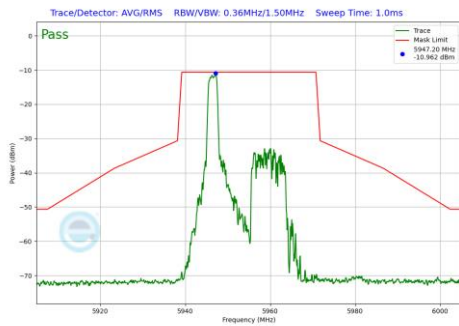
Plot 7-1067 In-Band Emission Plot SDM Primary Antenna 3c (20MHz BW 802.11be(RU) RU26 Index0 (UNII Band 5) - Ch.1)
