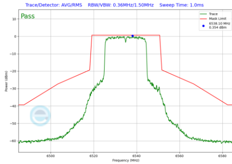
Plot 7-1051 In-Band Emission Plot CDD Primary Antenna 3c (20MHz BW 802.11be(RU) RU242 Index61 (UNII Band 7) - Ch.117)
