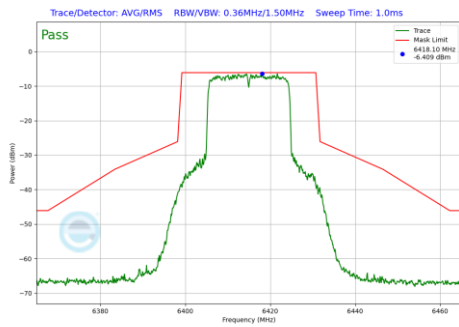
Plot 7-985 In-Band Emission Plot Antenna 1b (20MHz BW 802.11be(RU) RU242 Index61 (UNII Band 5) - Ch.93)
