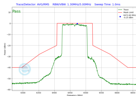
Plot 7-1049 In-Band Emission Plot CDD Primary Antenna 3c (80MHz BW 802.11be(RU) RU996 Index67 (UNII Band 6) - Ch.103)
