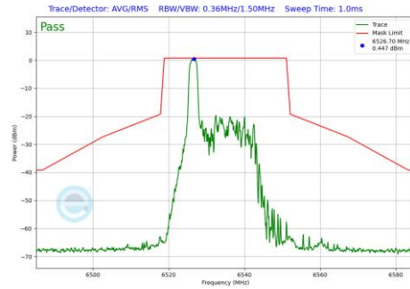
Plot 7-1021 In-Band Emission Plot CDD Primary Antenna 3a (20MHz BW 802.11be(RU) RU26 Index0 (UNII Band 7) - Ch.117)
