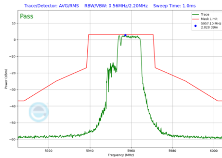
Plot 7-1034 In-Band Emission Plot CDD Primary Antenna 3a (20MHz BW 802.11be(RU) RU106+26 Index83 (UNII Band 5) - Ch.1)
