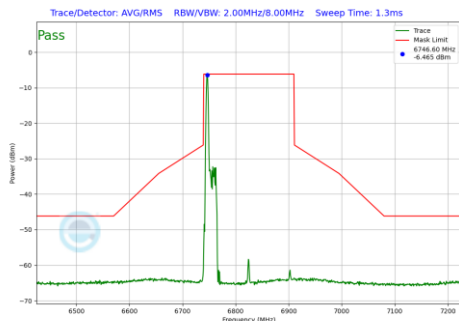
Plot 7-1078 In-Band Emission Plot SDM Primary Antenna 3c (160MHz BW 802.11be(RU) RU26 Index0 (UNII Band 7) - Ch.175)
