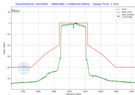
Plot 7-1046 In-Band Emission Plot CDD Primary Antenna 3c (160MHz BW 802.11be(RU) RU996X2 Index68 (UNII Band 5) - Ch.15)
