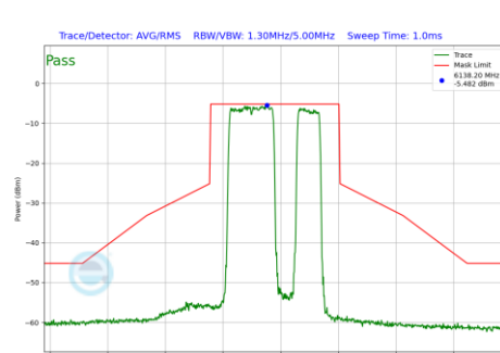
Plot 7-1112 In-Band Emission Plot SDM Primary Antenna 3a (80MHz BW 802.11be(RU) RU484+242 Index92 (UNII Band 5) - Ch.39)
