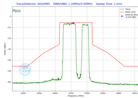
Plot 7-1103 In-Band Emission Plot SDM Primary Antenna 3c (80MHz BW 802.11be(RU) RU484+242 Index92 (UNII Band 6) - Ch.103)
