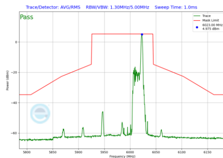
Plot 7-1015 In-Band Emission Plot CDD Primary Antenna 3a (80MHz BW 802.11be(RU) RU26 Index36 (UNII Band 5) - Ch.7)
