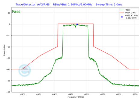
Plot 7-1061 In-Band Emission Plot CDD Primary Antenna 3a (80MHz BW 802.11be(RU) RU996 Index67 (UNII Band 6) - Ch.103)
