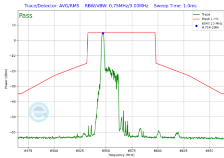
Plot 7-1010 In-Band Emission Plot CDD Primary Antenna 3c (40MHz BW 802.11be(RU) RU26 Index0 (UNII Band 7) - Ch.123)
