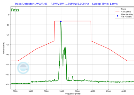
Plot 7-1069 In-Band Emission Plot SDM Primary Antenna 3c (80MHz BW 802.11be(RU) RU26 Index0 (UNII Band 5) - Ch.7)
