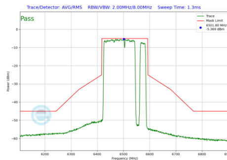
Plot 7-1104 In-Band Emission Plot SDM Primary Antenna 3c (160MHz BW 802.11be(RU) RU996+484+242 Index98 (UNII Band 6) - Ch.111)
