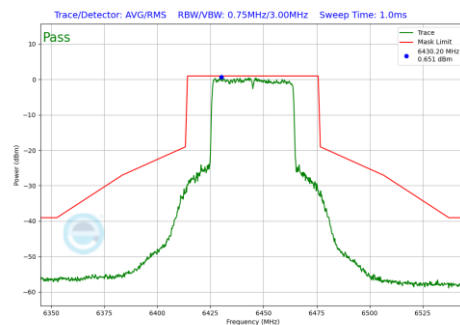
Plot 7-1048 In-Band Emission Plot CDD Primary Antenna 3c (40MHz BW 802.11be(RU) RU484 Index65 (UNII Band 6) - Ch.99)
