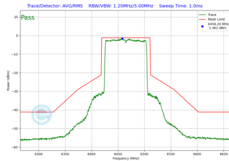
Plot 7-991 In-Band Emission Plot Antenna 1b (80MHz BW 802.11be(RU) RU996 Index67 (UNII Band 6) - Ch.103)
