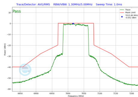
Plot 7-999 In-Band Emission Plot Antenna 1b (80MHz BW 802.11be(RU) RU996 Index67 (UNII Band 8) - Ch.215)
