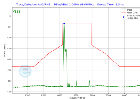
Plot 7-1074 In-Band Emission Plot SDM Primary Antenna 3c (160MHz BW 802.11be(RU) RU26 Index0 (UNII Band 6) - Ch.111)
