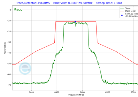
Plot 7-1142 In-Band Emission Plot SDM Primary Antenna 3a (20MHz BW 802.11be(RU) RU242 Index61 (UNII Band 6) - Ch.105)
