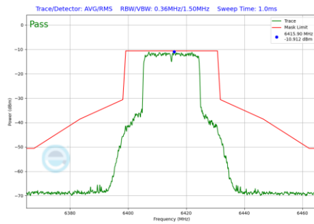
Plot 7-1122 In-Band Emission Plot SDM Primary Antenna 3c (20MHz BW 802.11be(RU) RU242 Index61 (UNII Band 5) - Ch.93)
