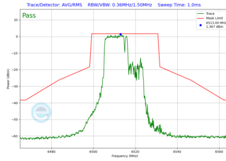
Plot 7-1037 In-Band Emission Plot CDD Primary Antenna 3a (20MHz BW 802.11be(RU) RU106+26 Index82 (UNII Band 6) - Ch.113)
