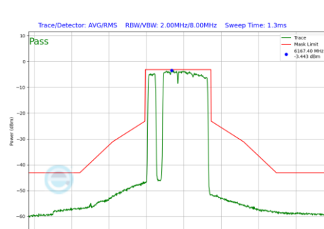
Plot 7-1113 In-Band Emission Plot SDM Primary Antenna 3a (160MHz BW 802.11be(RU) RU996+484+242 Index97 (UNII Band 5) - Ch.47)
