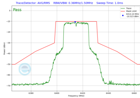
Plot 7-1138 In-Band Emission Plot SDM Primary Antenna 3a (20MHz BW 802.11be(RU) RU242 Index61 (UNII Band 5) - Ch.93)
