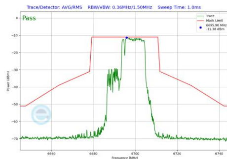
Plot 7-1105 In-Band Emission Plot SDM Primary Antenna 3c (20MHz BW 802.11be(RU) RU106+26 Index83 (UNII Band 7) - Ch.149)
