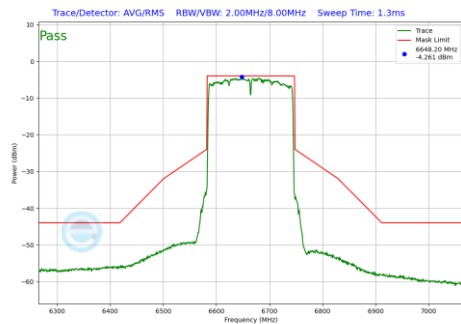
Plot 7-1133 In-Band Emission Plot SDM Primary Antenna 3c (160MHz BW 802.11be(RU) RU996X2 Index68 (UNII Band 7) - Ch.143)
