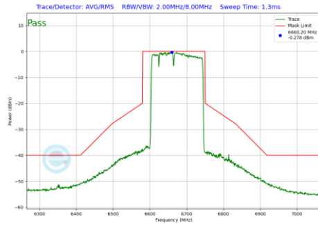
Plot 7-982 In-Band Emission Plot Antenna 1b (160MHz BW 802.11be(RU) RU996+484+242 Index96 (UNII Band 7) - Ch.143)
