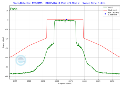
Plot 7-1052 In-Band Emission Plot CDD Primary Antenna 3c (40MHz BW 802.11be(RU) RU484 Index65 (UNII Band 7) - Ch.123)
