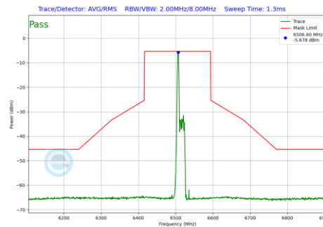
Plot 7-1090 In-Band Emission Plot SDM Primary Antenna 3a (160MHz BW 802.11be(RU) RU26 Index0 (UNII Band 6) - Ch.111)
