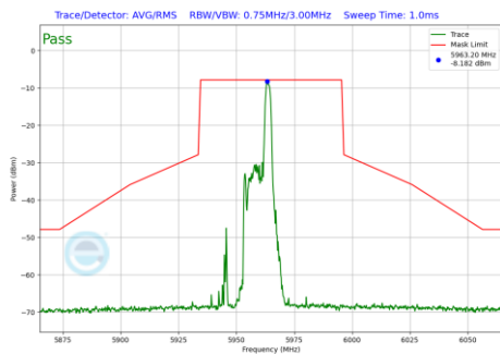
Plot 7-1068 In-Band Emission Plot SDM Primary Antenna 3c (40MHz BW 802.11be(RU) RU26 Index8 (UNII Band 5) - Ch.3)
