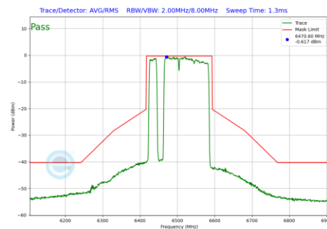
Plot 7-1030 In-Band Emission Plot CDD Primary Antenna 3c (160MHz BW 802.11be(RU) RU996+484+242 Index97 (UNII Band 6) - Ch.111)
