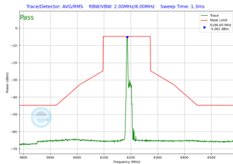
Plot 7-1086 In-Band Emission Plot SDM Primary Antenna 3a (160MHz BW 802.11be(RU) RU26 Index0 (UNII Band 5) - Ch.47)
