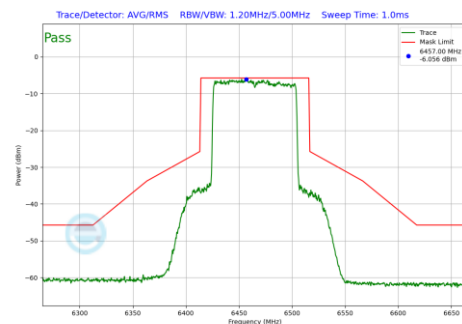
Plot 7-1128 In-Band Emission Plot SDM Primary Antenna 3c (80MHz BW 802.11be(RU) RU996 Index67 (UNII Band 6) - Ch.103)
