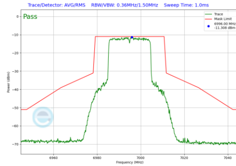
Plot 7-1134 In-Band Emission Plot SDM Primary Antenna 3c (20MHz BW 802.11be(RU) RU242 Index61 (UNII Band 8) - Ch.209)
