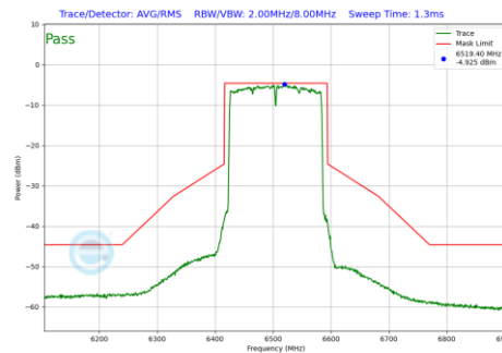
Plot 7-1145 In-Band Emission Plot SDM Primary Antenna 3a (160MHz BW 802.11be(RU) RU996X2 Index68 (UNII Band 6) - Ch.111)
