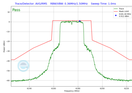
Plot 7-1043 In-Band Emission Plot CDD Primary Antenna 3c (20MHz BW 802.11be(RU) RU242 Index61 (UNII Band 5) - Ch.45)
