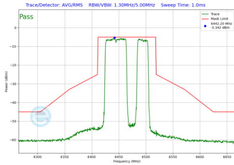
Plot 7-1115 In-Band Emission Plot SDM Primary Antenna 3a (80MHz BW 802.11be(RU) RU484+242 Index92 (UNII Band 6) - Ch.103)
