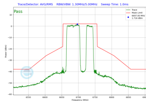
Plot 7-1032 In-Band Emission Plot CDD Primary Antenna 3c (80MHz BW 802.11be(RU) RU484+242 Index92 (UNII Band 7) - Ch.151)
