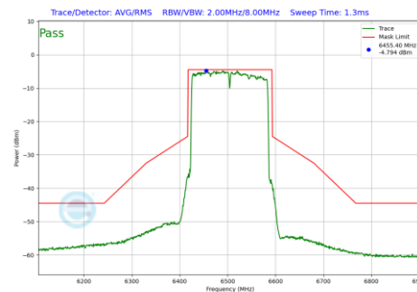
Plot 7-1129 In-Band Emission Plot SDM Primary Antenna 3c (160MHz BW 802.11be(RU) RU996X2 Index68 (UNII Band 6) - Ch.111)
