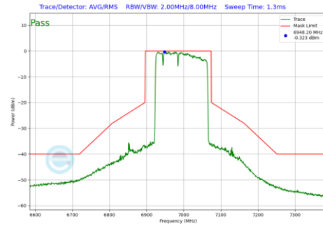
Plot 7-984 In-Band Emission Plot Antenna 1b (160MHz BW 802.11be(RU) RU996+484+242 Index96 (UNII Band 8) - Ch.207)
