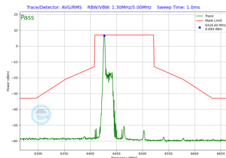
Plot 7-1007 In-Band Emission Plot CDD Primary Antenna 3c (80MHz BW 802.11be(RU) RU26 Index0 (UNII Band 6) - Ch.103)
