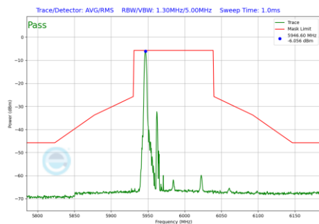
Plot 7-1085 In-Band Emission Plot SDM Primary Antenna 3a (80MHz BW 802.11be(RU) RU26 Index0 (UNII Band 5) - Ch.7)
