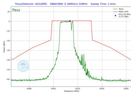
Plot 7-1028 In-Band Emission Plot CDD Primary Antenna 3c (20MHz BW 802.11be(RU) RU106+26 Index82 (UNII Band 6) - Ch.113)
