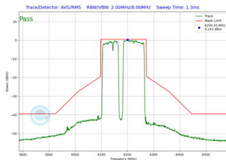
Plot 7-1027 In-Band Emission Plot CDD Primary Antenna 3c (160MHz BW 802.11be(RU) RU996+484+242 Index99 (UNII Band 5) - Ch.47)
