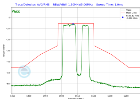
Plot 7-1118 In-Band Emission Plot SDM Primary Antenna 3a (80MHz BW 802.11be(RU) RU484+242 Index92 (UNII Band 7) - Ch.119)
