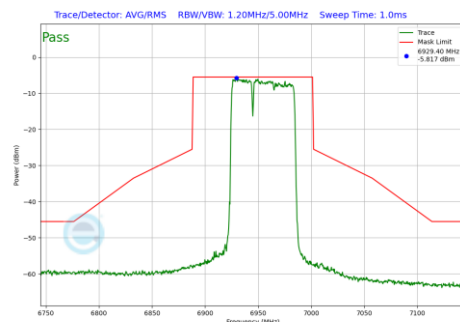
Plot 7-1120 In-Band Emission Plot SDM Primary Antenna 3a (80MHz BW 802.11be(RU) RU484+242 Index90 (UNII Band 8) - Ch.199)
