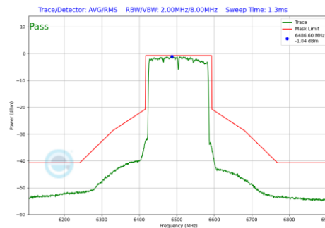
Plot 7-1050 In-Band Emission Plot CDD Primary Antenna 3c (160MHz BW 802.11be(RU) RU996X2 Index68 (UNII Band 6) - Ch.111)
