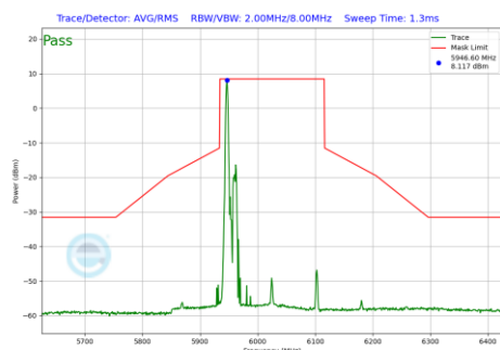
Plot 7-1004 In-Band Emission Plot CDD Primary Antenna 3c (160MHz BW 802.11be(RU) RU26 Index0 (UNII Band 5) - Ch.15)
