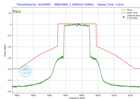
Plot 7-1057 In-Band Emission Plot CDD Primary Antenna 3a (80MHz BW 802.11be(RU) RU996 Index67 (UNII Band 5) - Ch.7)
