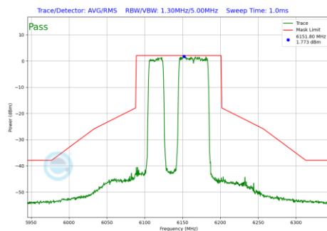
Plot 7-1026 In-Band Emission Plot CDD Primary Antenna 3c (80MHz BW 802.11be(RU) RU484+242 Index91 (UNII Band 5) - Ch.39)
