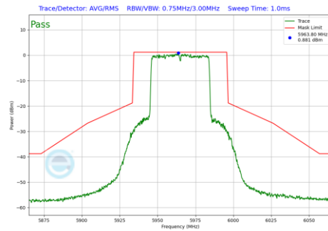
Plot 7-1056 In-Band Emission Plot CDD Primary Antenna 3a (40MHz BW 802.11be(RU) RU484 Index65 (UNII Band 5) - Ch.3)
