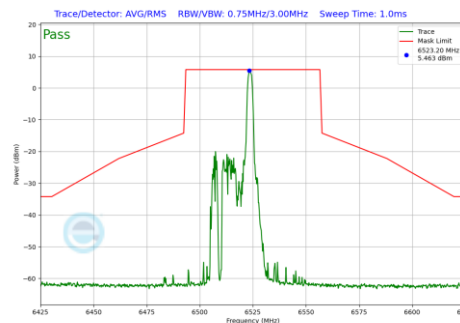
Plot 7-1006 In-Band Emission Plot CDD Primary Antenna 3c (40MHz BW 802.11be(RU) RU26 Index8 (UNII Band 6) - Ch.115)
