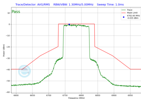
Plot 7-1053 In-Band Emission Plot CDD Primary Antenna 3c (80MHz BW 802.11be(RU) RU996 Index67 (UNII Band 7) - Ch.167)
