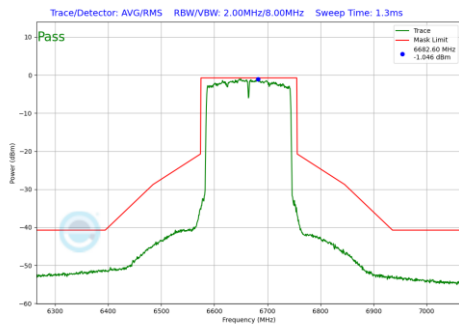
Plot 7-1054 In-Band Emission Plot CDD Primary Antenna 3c (160MHz BW 802.11be(RU) RU996X2 Index68 (UNII Band 7) - Ch.143)
