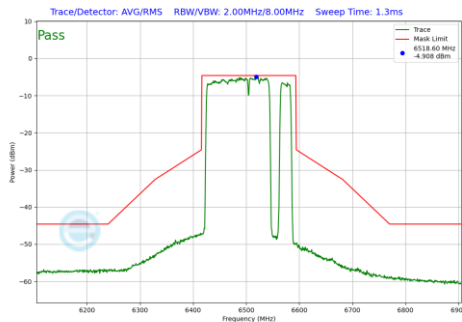
Plot 7-1116 In-Band Emission Plot SDM Primary Antenna 3a (160MHz BW 802.11be(RU) RU996+484+242 Index98 (UNII Band 6) - Ch.111)
