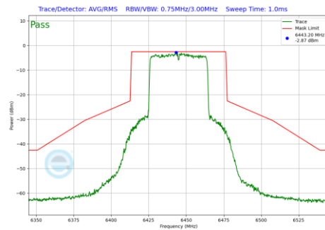
Plot 7-990 In-Band Emission Plot Antenna 1b (40MHz BW 802.11be(RU) RU484 Index65 (UNII Band 6) - Ch.99)
