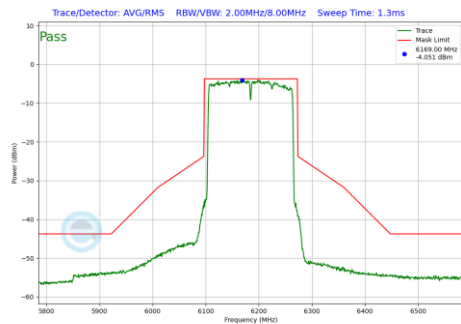
Plot 7-1141 In-Band Emission Plot SDM Primary Antenna 3a (160MHz BW 802.11be(RU) RU996X2 Index68 (UNII Band 5) - Ch.47)
