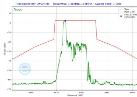
Plot 7-1005 In-Band Emission Plot CDD Primary Antenna 3c (20MHz BW 802.11be(RU) RU26 Index0 (UNII Band 6) - Ch.97)
