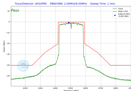
Plot 7-1062 In-Band Emission Plot CDD Primary Antenna 3a (160MHz BW 802.11be(RU) RU996X2 Index68 (UNII Band 6) - Ch.111)
