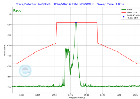
Plot 7-1072 In-Band Emission Plot SDM Primary Antenna 3c (40MHz BW 802.11be(RU) RU26 Index8 (UNII Band 6) - Ch.107)
