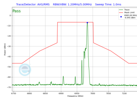
Plot 7-1097 In-Band Emission Plot SDM Primary Antenna 3a (80MHz BW 802.11be(RU) RU26 Index36 (UNII Band 8) - Ch.199)
