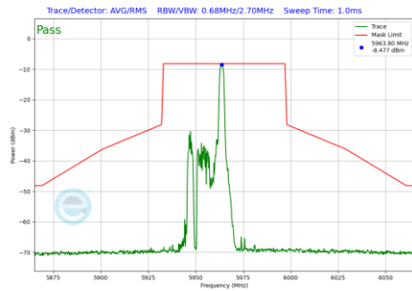
Plot 7-1084 In-Band Emission Plot SDM Primary Antenna 3a (40MHz BW 802.11be(RU) RU26 Index8 (UNII Band 5) - Ch.3)
