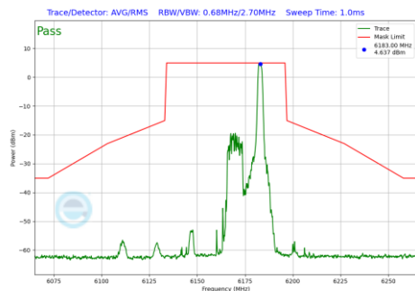
Plot 7-1002 In-Band Emission Plot CDD Primary Antenna 3c (40MHz BW 802.11be(RU) RU26 Index17 (UNII Band 5) - Ch.43)
