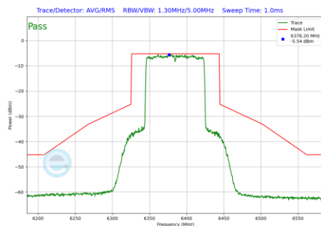
Plot 7-1124 In-Band Emission Plot SDM Primary Antenna 3c (80MHz BW 802.11be(RU) RU996 Index67 (UNII Band 5) - Ch.87)
