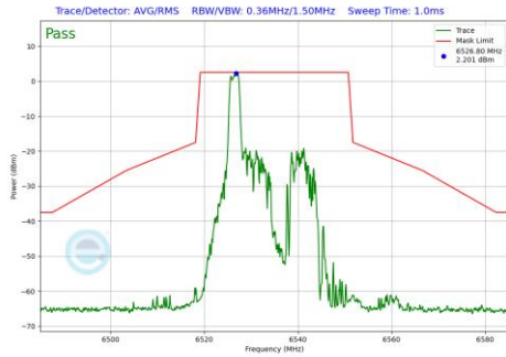
Plot 7-1009 In-Band Emission Plot CDD Primary Antenna 3c (20MHz BW 802.11be(RU) RU26 Index0 (UNII Band 7) - Ch.117)
