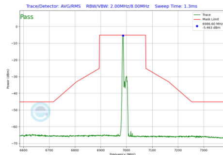
Plot 7-1098 In-Band Emission Plot SDM Primary Antenna 3a (160MHz BW 802.11be(RU) RU26 Index0 (UNII Band 8) - Ch.207)
