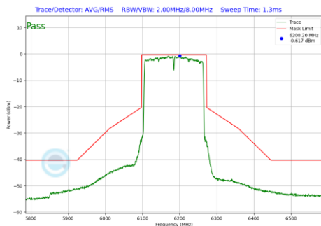
Plot 7-988 In-Band Emission Plot Antenna 1b (160MHz BW 802.11be(RU) RU996X2 Index68 (UNII Band 5) - Ch.47)
