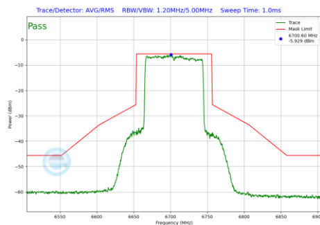
Plot 7-1132 In-Band Emission Plot SDM Primary Antenna 3c (80MHz BW 802.11be(RU) RU996 Index67 (UNII Band 7) - Ch.151)
