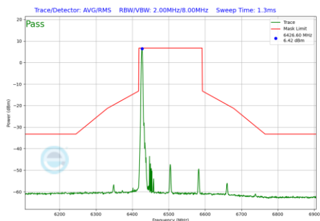
Plot 7-1020 In-Band Emission Plot CDD Primary Antenna 3a (160MHz BW 802.11be(RU) RU26 Index0 (UNII Band 6) - Ch.111)
