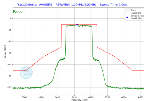
Plot 7-1144 In-Band Emission Plot SDM Primary Antenna 3a (80MHz BW 802.11be(RU) RU996 Index67 (UNII Band 6) - Ch.103)
