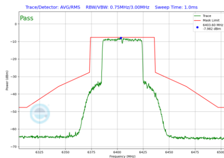
Plot 7-1123 In-Band Emission Plot SDM Primary Antenna 3c (40MHz BW 802.11be(RU) RU484 Index65 (UNII Band 5) - Ch.91)
