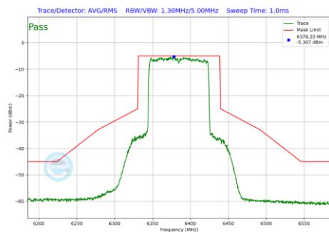
Plot 7-1140 In-Band Emission Plot SDM Primary Antenna 3a (80MHz BW 802.11be(RU) RU996 Index67 (UNII Band 5) - Ch.87)
