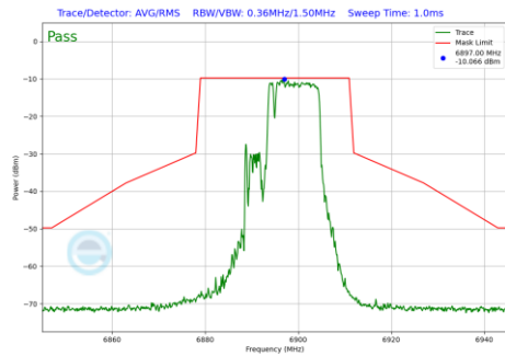
Plot 7-1108 In-Band Emission Plot SDM Primary Antenna 3c (20MHz BW 802.11be(RU) RU106+26 Index83 (UNII Band 8) - Ch.189)
