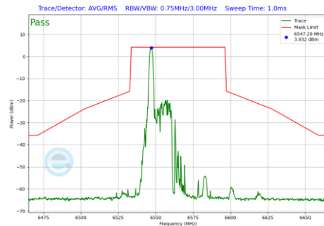
Plot 7-1022 In-Band Emission Plot CDD Primary Antenna 3a (40MHz BW 802.11be(RU) RU26 Index0 (UNII Band 7) - Ch.123)
