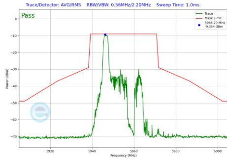
Plot 7-1083 In-Band Emission Plot SDM Primary Antenna 3a (20MHz BW 802.11be(RU) RU26 Index0 (UNII Band 5) - Ch.1)
