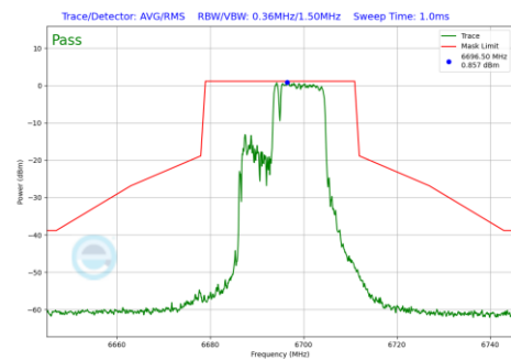
Plot 7-1031 In-Band Emission Plot CDD Primary Antenna 3c (20MHz BW 802.11be(RU) RU106+26 Index83 (UNII Band 7) - Ch.149)
