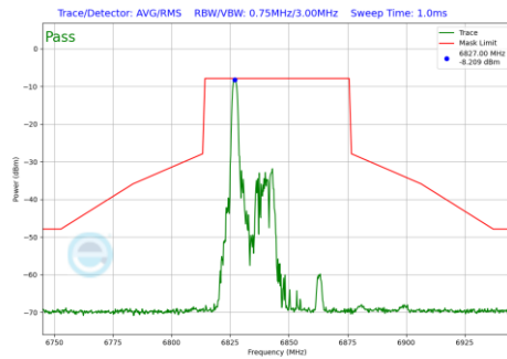
Plot 7-1092 In-Band Emission Plot SDM Primary Antenna 3a (40MHz BW 802.11be(RU) RU26 Index0 (UNII Band 7) - Ch.179)
