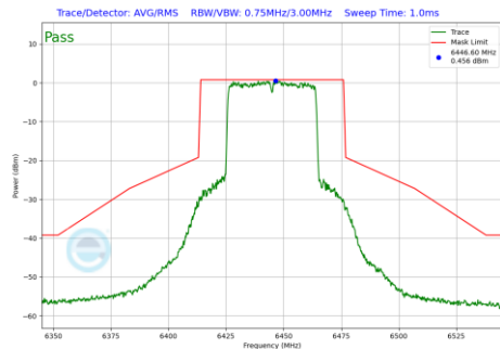
Plot 7-1060 In-Band Emission Plot CDD Primary Antenna 3a (40MHz BW 802.11be(RU) RU484 Index65 (UNII Band 6) - Ch.99)
