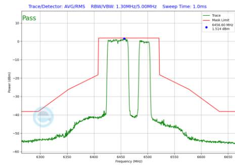
Plot 7-1029 In-Band Emission Plot CDD Primary Antenna 3c (80MHz BW 802.11be(RU) RU484+242 Index92 (UNII Band 6) - Ch.103)
