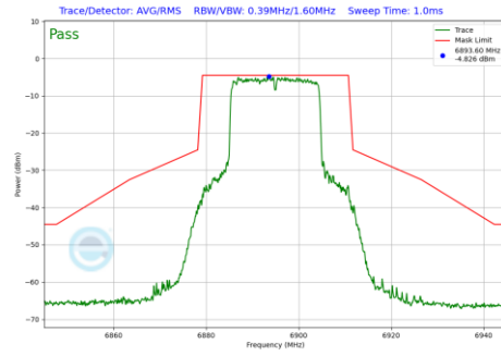
Plot 7-997 In-Band Emission Plot Antenna 1b (20MHz BW 802.11be(RU) RU242 Index61 (UNII Band 8) - Ch.189)
