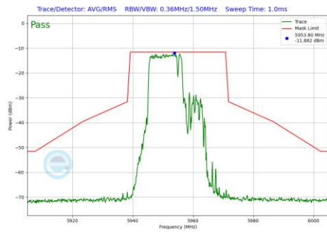
Plot 7-1099 In-Band Emission Plot SDM Primary Antenna 3c (20MHz BW 802.11be(RU) RU106+26 Index82 (UNII Band 5) - Ch.1)
