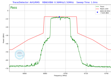
Plot 7-993 In-Band Emission Plot Antenna 1b (20MHz BW 802.11be(RU) RU242 Index61 (UNII Band 7) - Ch.149)
