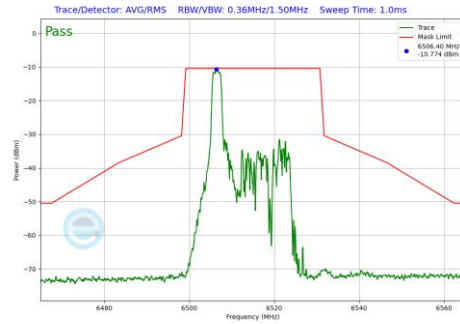
Plot 7-1087 In-Band Emission Plot SDM Primary Antenna 3a (20MHz BW 802.11be(RU) RU26 Index0 (UNII Band 6) - Ch.113)
