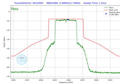
Plot 7-1143 In-Band Emission Plot SDM Primary Antenna 3a (40MHz BW 802.11be(RU) RU484 Index65 (UNII Band 6) - Ch.99)
