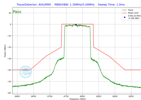
Plot 7-1065 In-Band Emission Plot CDD Primary Antenna 3a (80MHz BW 802.11be(RU) RU996 Index67 (UNII Band 7) - Ch.167)
