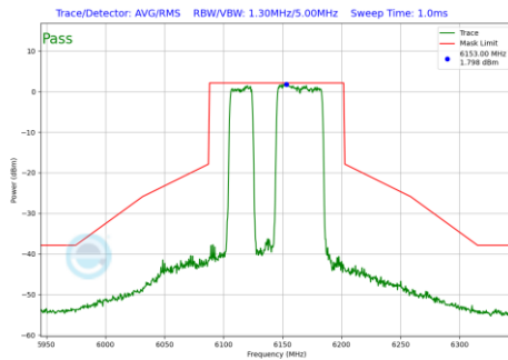
Plot 7-1035 In-Band Emission Plot CDD Primary Antenna 3a (80MHz BW 802.11be(RU) RU484+242 Index91 (UNII Band 5) - Ch.39)
