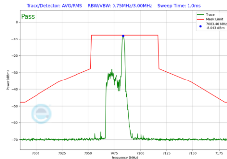
Plot 7-1080 In-Band Emission Plot SDM Primary Antenna 3c (40MHz BW 802.11be(RU) RU26 Index8 (UNII Band 8) - Ch.227)
