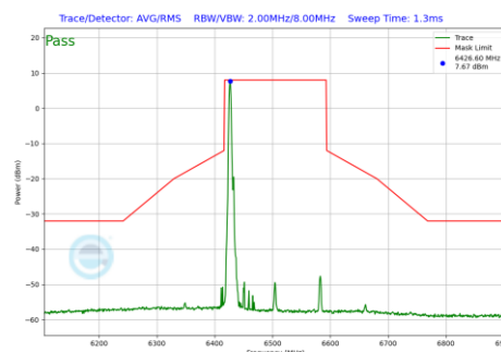
Plot 7-1008 In-Band Emission Plot CDD Primary Antenna 3c (160MHz BW 802.11be(RU) RU26 Index0 (UNII Band 6) - Ch.111)
