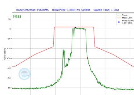
Plot 7-1040 In-Band Emission Plot CDD Primary Antenna 3a (20MHz BW 802.11be(RU) RU106+26 Index83 (UNII Band 7) - Ch.149)
