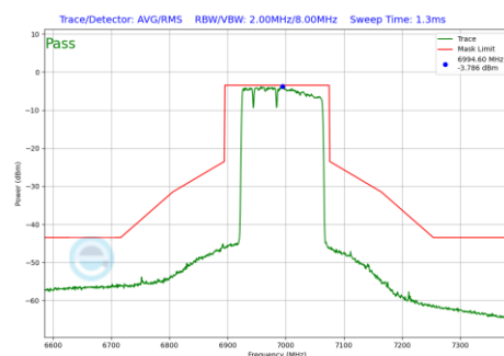
Plot 7-1121 In-Band Emission Plot SDM Primary Antenna 3a (160MHz BW 802.11be(RU) RU996+484+242 Index96 (UNII Band 8) - Ch.207)
