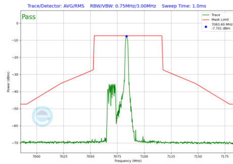
Plot 7-1096 In-Band Emission Plot SDM Primary Antenna 3a (40MHz BW 802.11be(RU) RU26 Index8 (UNII Band 8) - Ch.227)
