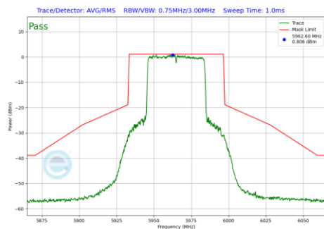
Plot 7-1044 In-Band Emission Plot CDD Primary Antenna 3c (40MHz BW 802.11be(RU) RU484 Index65 (UNII Band 5) - Ch.3)
