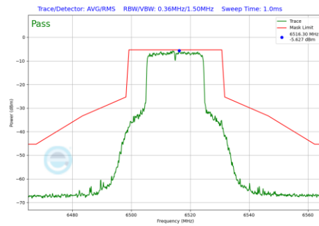
Plot 7-989 In-Band Emission Plot Antenna 1b (20MHz BW 802.11be(RU) RU242 Index61 (UNII Band 6) - Ch.113)
