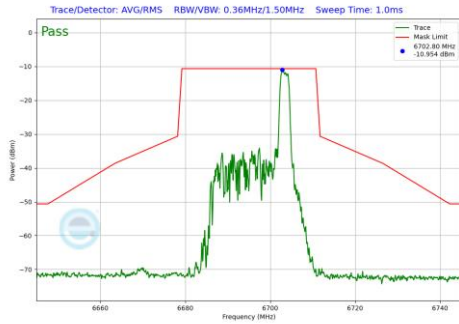
Plot 7-1075 In-Band Emission Plot SDM Primary Antenna 3c (20MHz BW 802.11be(RU) RU26 Index8 (UNII Band 7) - Ch.149)
