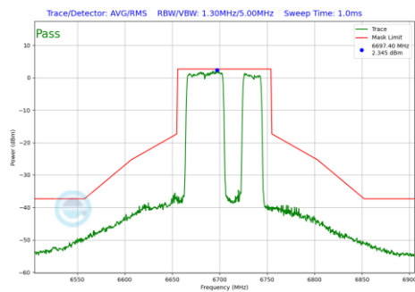
Plot 7-1041 In-Band Emission Plot CDD Primary Antenna 3a (80MHz BW 802.11be(RU) RU484+242 Index92 (UNII Band 7) - Ch.151)
