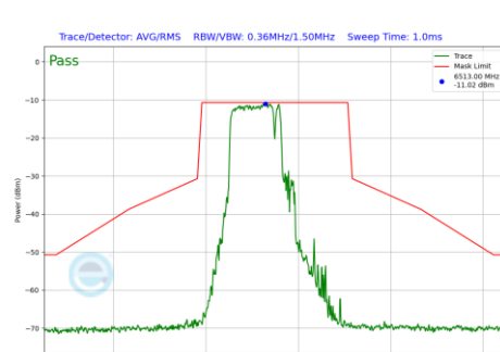
Plot 7-1114 In-Band Emission Plot SDM Primary Antenna 3a (20MHz BW 802.11be(RU) RU106+26 Index82 (UNII Band 6) - Ch.113)
