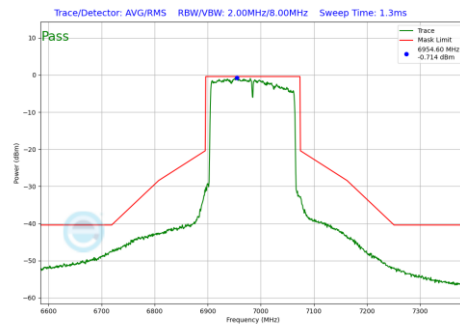
Plot 7-1000 In-Band Emission Plot Antenna 1b (160MHz BW 802.11be(RU) RU996X2 Index68 (UNII Band 8) - Ch.207)
