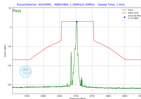
Plot 7-1023 In-Band Emission Plot CDD Primary Antenna 3a (80MHz BW 802.11be(RU) RU26 Index17 (UNII Band 7) - Ch.151)
