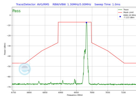
Plot 7-1081 In-Band Emission Plot SDM Primary Antenna 3c (80MHz BW 802.11be(RU) RU26 Index36 (UNII Band 8) - Ch.199)
