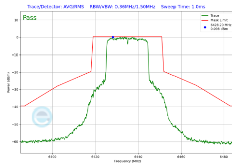
Plot 7-1047 In-Band Emission Plot CDD Primary Antenna 3c (20MHz BW 802.11be(RU) RU242 Index61 (UNII Band 6) - Ch.97)
