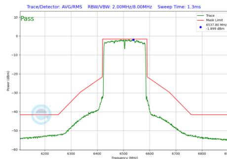
Plot 7-992 In-Band Emission Plot Antenna 1b (160MHz BW 802.11be(RU) RU996X2 Index68 (UNII Band 6) - Ch.111)
