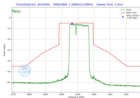
Plot 7-1109 In-Band Emission Plot SDM Primary Antenna 3c (80MHz BW 802.11be(RU) RU484+242 Index90 (UNII Band 8) - Ch.199)
