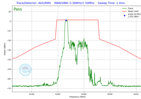
Plot 7-1013 In-Band Emission Plot CDD Primary Antenna 3a (20MHz BW 802.11be(RU) RU26 Index0 (UNII Band 5) - Ch.45)
