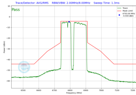
Plot 7-1107 In-Band Emission Plot SDM Primary Antenna 3c (160MHz BW 802.11be(RU) RU996+484+242 Index99 (UNII Band 7) - Ch.175)
