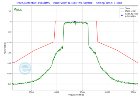
Plot 7-1063 In-Band Emission Plot CDD Primary Antenna 3a (20MHz BW 802.11be(RU) RU242 Index61 (UNII Band 7) - Ch.117)
