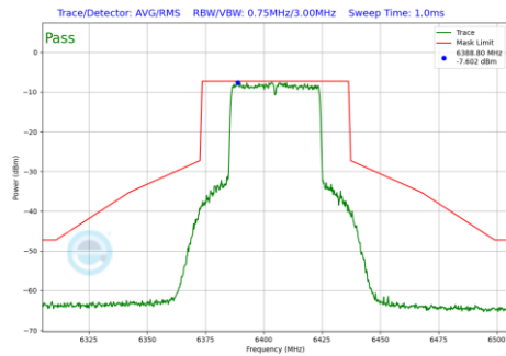
Plot 7-1139 In-Band Emission Plot SDM Primary Antenna 3a (40MHz BW 802.11be(RU) RU484 Index65 (UNII Band 5) - Ch.91)
