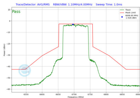
Plot 7-995 In-Band Emission Plot Antenna 1b (80MHz BW 802.11be(RU) RU996 Index67 (UNII Band 7) - Ch.151)
