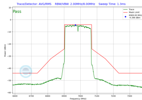
Plot 7-1137 In-Band Emission Plot SDM Primary Antenna 3c (160MHz BW 802.11be(RU) RU996X2 Index68 (UNII Band 8) - Ch.207)
