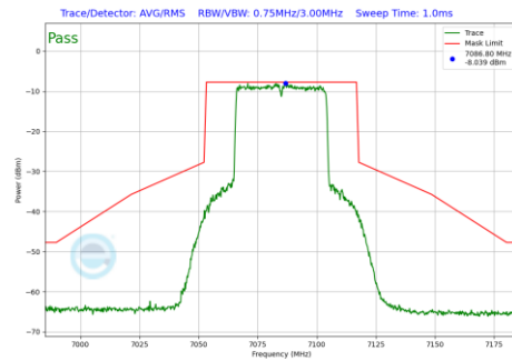
Plot 7-1135 In-Band Emission Plot SDM Primary Antenna 3c (40MHz BW 802.11be(RU) RU484 Index65 (UNII Band 8) - Ch.227)
