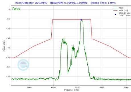
Plot 7-1091 In-Band Emission Plot SDM Primary Antenna 3a (20MHz BW 802.11be(RU) RU26 Index8 (UNII Band 7) - Ch.149)
