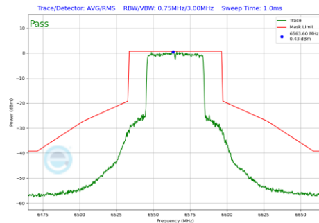
Plot 7-1064 In-Band Emission Plot CDD Primary Antenna 3a (40MHz BW 802.11be(RU) RU484 Index65 (UNII Band 7) - Ch.123)
