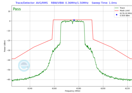
Plot 7-1055 In-Band Emission Plot CDD Primary Antenna 3a (20MHz BW 802.11be(RU) RU242 Index61 (UNII Band 5) - Ch.45)
