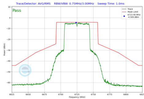
Plot 7-994 In-Band Emission Plot Antenna 1b (40MHz BW 802.11be(RU) RU484 Index65 (UNII Band 7) - Ch.155)
