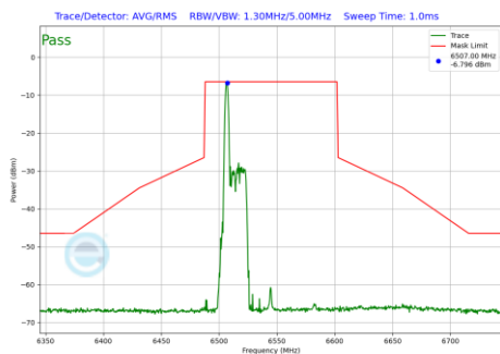
Plot 7-1077 In-Band Emission Plot SDM Primary Antenna 3c (80MHz BW 802.11be(RU) RU26 Index0 (UNII Band 7) - Ch.119)
