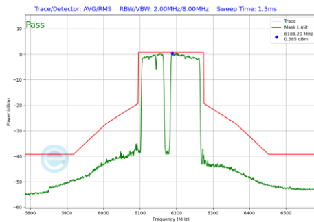
Plot 7-1036 In-Band Emission Plot CDD Primary Antenna 3a (160MHz BW 802.11be(RU) RU996+484+242 Index99 (UNII Band 5) - Ch.47)
