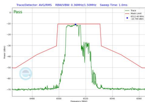
Plot 7-1102 In-Band Emission Plot SDM Primary Antenna 3c (20MHz BW 802.11be(RU) RU106+26 Index82 (UNII Band 6) - Ch.113)
