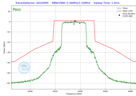
Plot 7-1059 In-Band Emission Plot CDD Primary Antenna 3a (20MHz BW 802.11be(RU) RU242 Index61 (UNII Band 6) - Ch.97)
