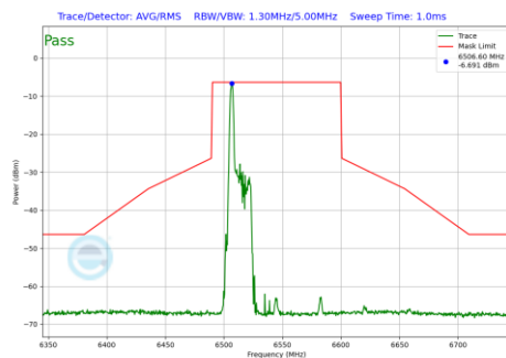
Plot 7-1093 In-Band Emission Plot SDM Primary Antenna 3a (80MHz BW 802.11be(RU) RU26 Index0 (UNII Band 7) - Ch.119)
