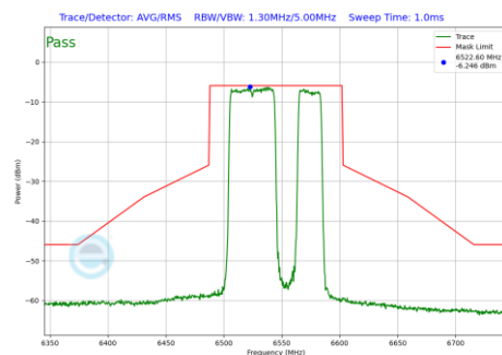
Plot 7-1106 In-Band Emission Plot SDM Primary Antenna 3c (80MHz BW 802.11be(RU) RU484+242 Index92 (UNII Band 7) - Ch.119)
