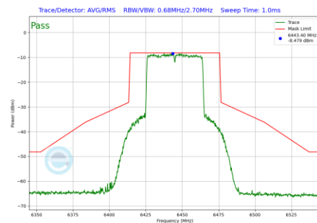
Plot 7-1127 In-Band Emission Plot SDM Primary Antenna 3c (40MHz BW 802.11be(RU) RU484 Index65 (UNII Band 6) - Ch.99)
