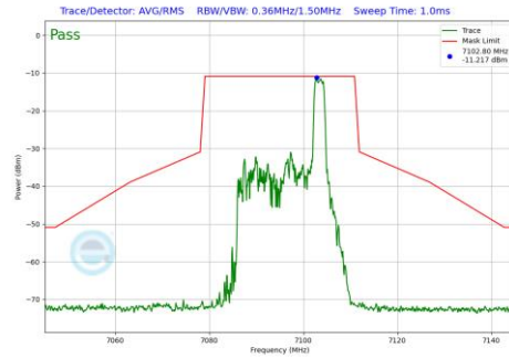
Plot 7-1079 In-Band Emission Plot SDM Primary Antenna 3c (20MHz BW 802.11be(RU) RU26 Index8 (UNII Band 8) - Ch.229)
