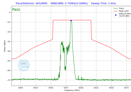
Plot 7-1088 In-Band Emission Plot SDM Primary Antenna 3a (40MHz BW 802.11be(RU) RU26 Index8 (UNII Band 6) - Ch.107)
