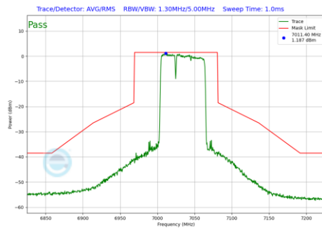
Plot 7-983 In-Band Emission Plot Antenna 1b (80MHz BW 802.11be(RU) RU484+242 Index90 (UNII Band 8) - Ch.215)
