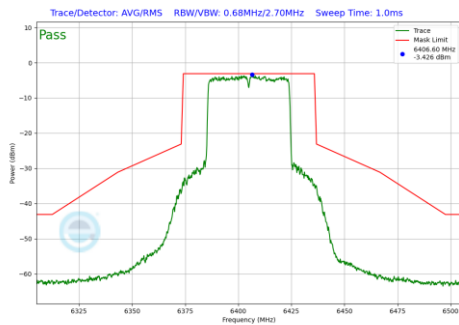
Plot 7-986 In-Band Emission Plot Antenna 1b (40MHz BW 802.11be(RU) RU484 Index65 (UNII Band 5) - Ch.91)
