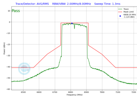
Plot 7-996 In-Band Emission Plot Antenna 1b (160MHz BW 802.11be(RU) RU996X2 Index68 (UNII Band 7) - Ch.175)
