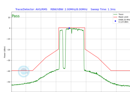
Plot 7-1039 In-Band Emission Plot CDD Primary Antenna 3a (160MHz BW 802.11be(RU) RU996+484+242 Index97 (UNII Band 6) - Ch.111)
