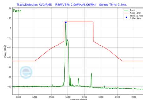
Plot 7-1024 In-Band Emission Plot CDD Primary Antenna 3a (160MHz BW 802.11be(RU) RU26 Index0 (UNII Band 7) - Ch.143)
