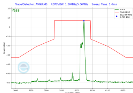
Plot 7-1003 In-Band Emission Plot CDD Primary Antenna 3c (80MHz BW 802.11be(RU) RU26 Index36 (UNII Band 5) - Ch.7)
