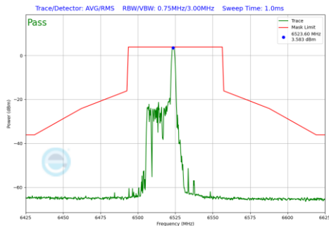
Plot 7-1018 In-Band Emission Plot CDD Primary Antenna 3a (40MHz BW 802.11be(RU) RU26 Index8 (UNII Band 6) - Ch.115)
