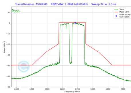
Plot 7-1042 In-Band Emission Plot CDD Primary Antenna 3a (160MHz BW 802.11be(RU) RU996+484+242 Index99 (UNII Band 7) - Ch.143)
