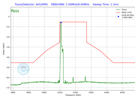
Plot 7-1070 In-Band Emission Plot SDM Primary Antenna 3c (160MHz BW 802.11be(RU) RU26 Index0 (UNII Band 5) - Ch.47)
