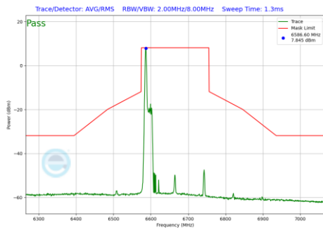
Plot 7-1012 In-Band Emission Plot CDD Primary Antenna 3c (160MHz BW 802.11be(RU) RU26 Index0 (UNII Band 7) - Ch.143)
