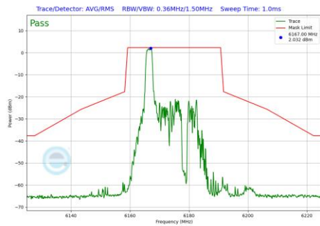
Plot 7-1001 In-Band Emission Plot CDD Primary Antenna 3c (20MHz BW 802.11be(RU) RU26 Index0 (UNII Band 5) - Ch.45)
