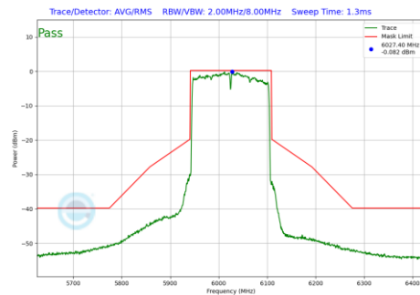
Plot 7-1058 In-Band Emission Plot CDD Primary Antenna 3a (160MHz BW 802.11be(RU) RU996X2 Index68 (UNII Band 5) - Ch.15)
