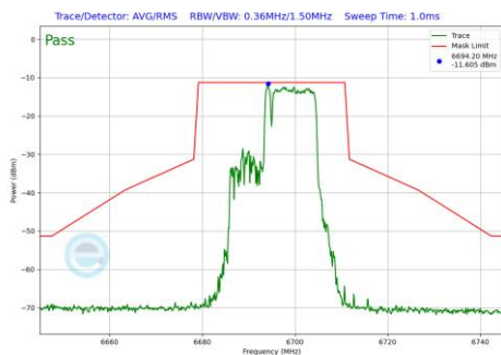
Plot 7-1117 In-Band Emission Plot SDM Primary Antenna 3a (20MHz BW 802.11be(RU) RU106+26 Index83 (UNII Band 7) - Ch.149)
