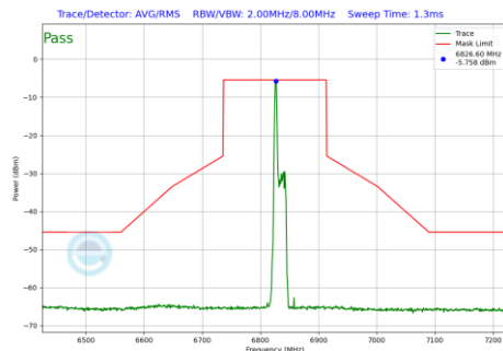
Plot 7-1094 In-Band Emission Plot SDM Primary Antenna 3a (160MHz BW 802.11be(RU) RU26 Index0 (UNII Band 7) - Ch.175)
