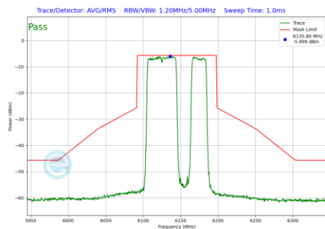
Plot 7-1100 In-Band Emission Plot SDM Primary Antenna 3c (80MHz BW 802.11be(RU) RU484+242 Index92 (UNII Band 5) - Ch.39)
