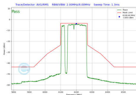
Plot 7-1101 In-Band Emission Plot SDM Primary Antenna 3c (160MHz BW 802.11be(RU) RU996+484+242 Index97 (UNII Band 5) - Ch.47)
