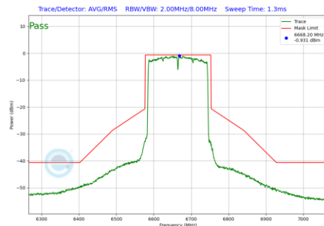
Plot 7-1066 In-Band Emission Plot CDD Primary Antenna 3a (160MHz BW 802.11be(RU) RU996X2 Index68 (UNII Band 7) - Ch.143)
