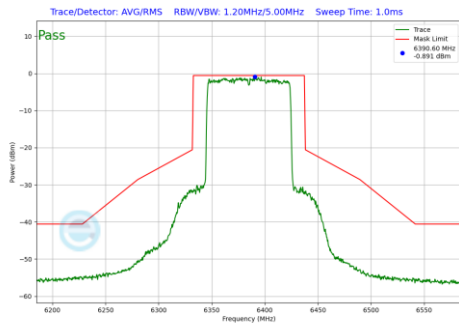
Plot 7-987 In-Band Emission Plot Antenna 1b (80MHz BW 802.11be(RU) RU996 Index67 (UNII Band 5) - Ch.87)
