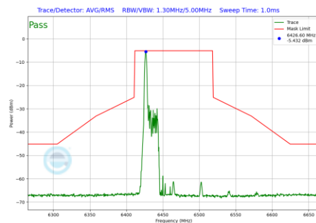
Plot 7-1089 In-Band Emission Plot SDM Primary Antenna 3a (80MHz BW 802.11be(RU) RU26 Index0 (UNII Band 6) - Ch.103)
