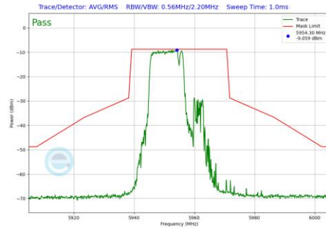
Plot 7-1111 In-Band Emission Plot SDM Primary Antenna 3a (20MHz BW 802.11be(RU) RU106+26 Index82 (UNII Band 5) - Ch.1)
