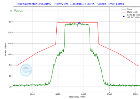
Plot 7-1126 In-Band Emission Plot SDM Primary Antenna 3c (20MHz BW 802.11be(RU) RU242 Index61 (UNII Band 6) - Ch.105)
