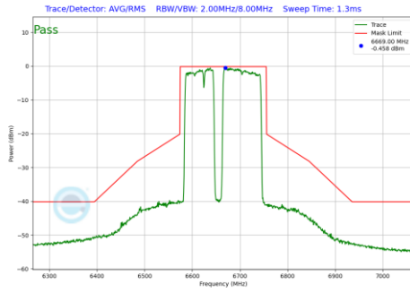
Plot 7-1033 In-Band Emission Plot CDD Primary Antenna 3c (160MHz BW 802.11be(RU) RU996+484+242 Index99 (UNII Band 7) - Ch.143)
