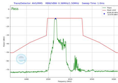
Plot 7-1071 In-Band Emission Plot SDM Primary Antenna 3c (20MHz BW 802.11be(RU) RU26 Index0 (UNII Band 6) - Ch.113)
