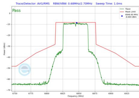
Plot 7-1131 In-Band Emission Plot SDM Primary Antenna 3c (40MHz BW 802.11be(RU) RU484 Index65 (UNII Band 7) - Ch.179)
