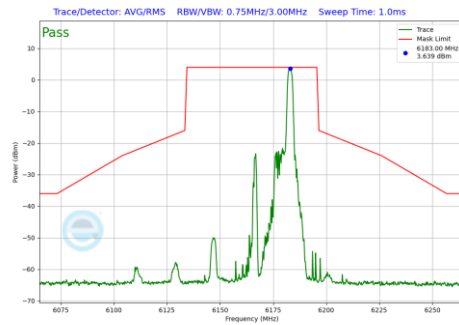
Plot 7-1014 In-Band Emission Plot CDD Primary Antenna 3a (40MHz BW 802.11be(RU) RU26 Index17 (UNII Band 5) - Ch.43)
