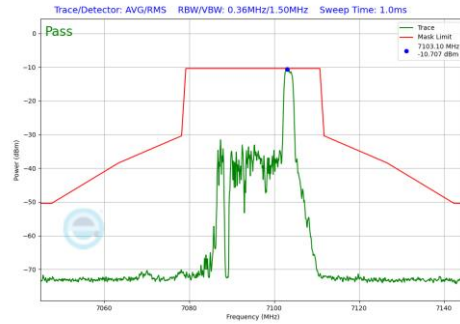
Plot 7-1095 In-Band Emission Plot SDM Primary Antenna 3a (20MHz BW 802.11be(RU) RU26 Index8 (UNII Band 8) - Ch.229)
