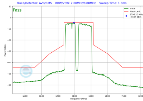
Plot 7-1119 In-Band Emission Plot SDM Primary Antenna 3a (160MHz BW 802.11be(RU) RU996+484+242 Index99 (UNII Band 7) - Ch.175)
