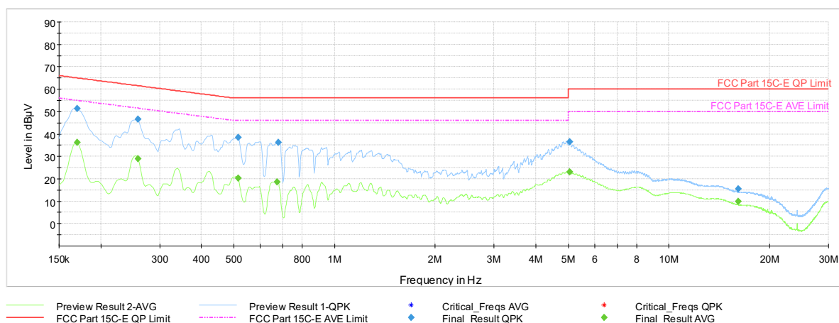
Plot 7-1159. AC Line Conducted Plot with 11be UNII Band 5 SDM Primary – RU26 – Ch.61 (N) with AC/DC Adapter
