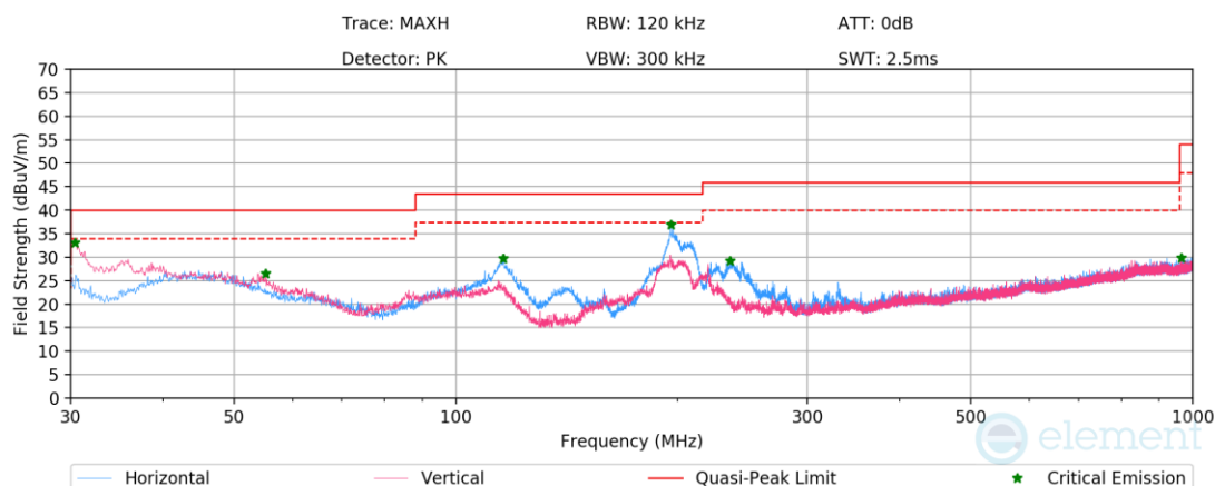
Plot 7-1157. Radiated Spurious Emissions below 1GHz SDM Diversity (802.11be – Ch.61 – RU242) with AC/DC Adapter
