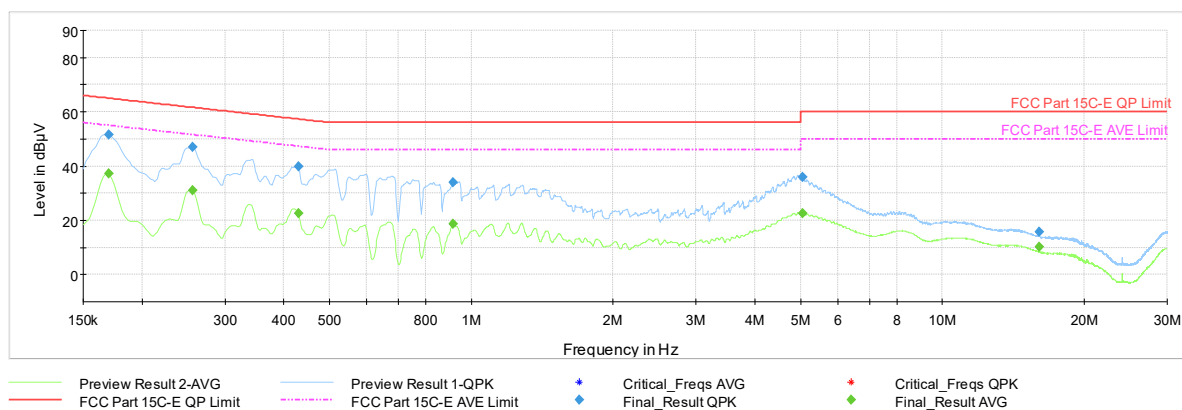
Plot 7-1165. AC Line Conducted Plot with 11be UNII Band 5 SDM Diversity – RU242 – Ch.61 (N) with AC/DC Adapter
