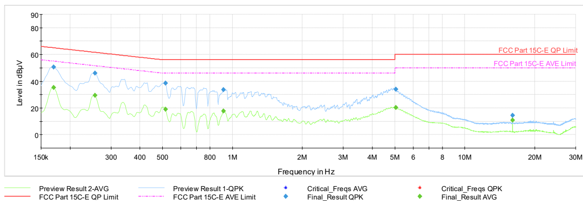
Plot 7-1162. AC Line Conducted Plot with 11be UNII Band 5 SDM Diversity – RU26 – Ch.61 (L1) with AC/DC Adapter
