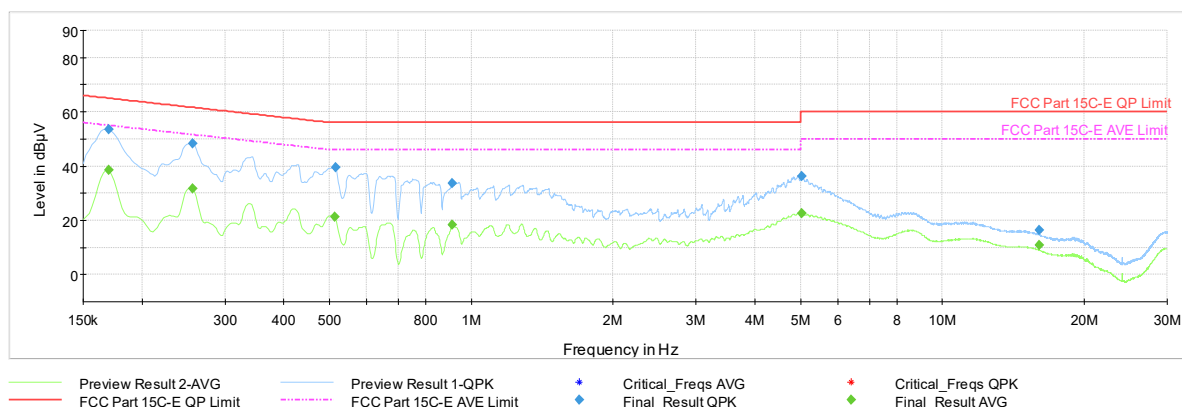
Plot 7-1163. AC Line Conducted Plot with 11be UNII Band 5 SDM Diversity – RU26 – Ch.61 (N) with AC/DC Adapter
