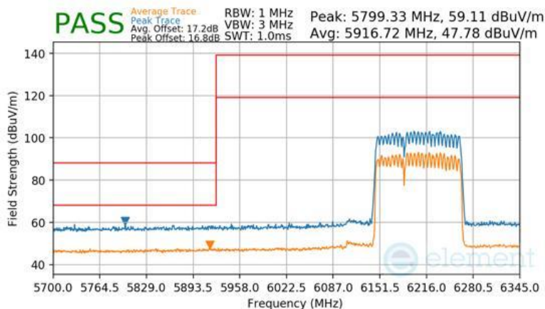
Plot 7-1128 SDM Diversity Radiated Lower Band Edge (Peak & Average – UNII Band 5) - RU996+484 (L)
