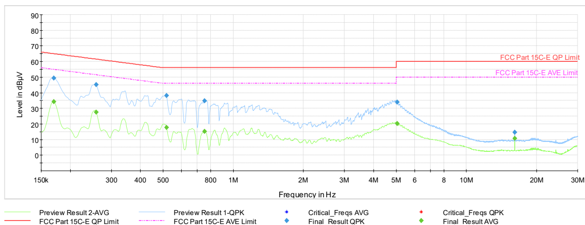
Plot 7-1158. AC Line Conducted Plot with 11be UNII Band 5 SDM Primary – RU26 – Ch.61 (L1) with AC/DC Adapter
