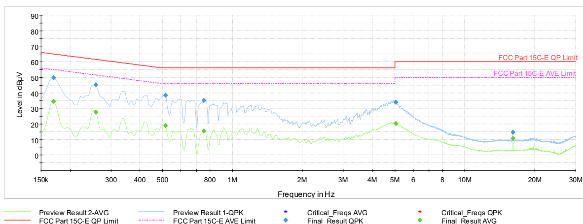
Plot 7-1160. AC Line Conducted Plot with 11be UNII Band 5 SDM Primary – RU242 – Ch.61 (L1) with AC/DC Adapter
