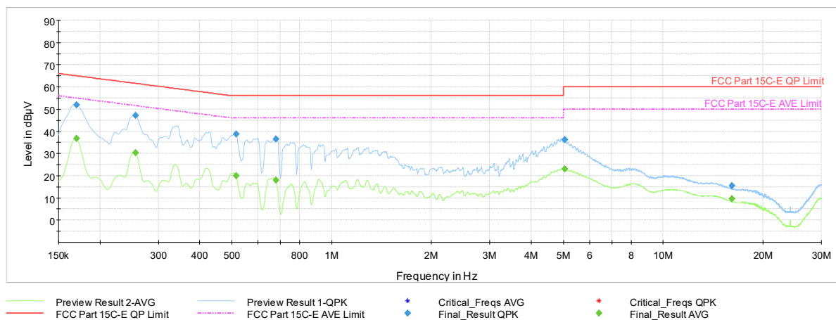
Plot 7-1161. AC Line Conducted Plot with 11be UNII Band 5 SDM Primary – RU242 – Ch.61 (N) with AC/DC Adapter
