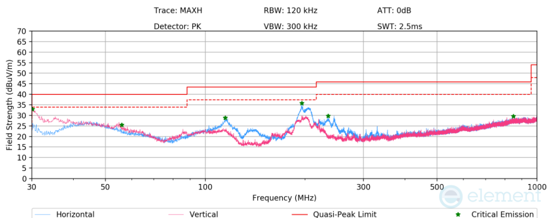
Plot 7-1154. Radiated Spurious Emissions below 1GHz SDM Primary (802.11be – Ch.61 – RU26) with AC/DC Adapter
