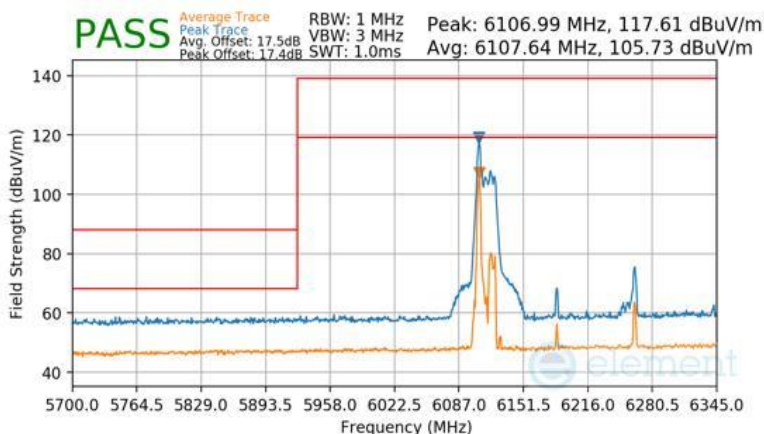
Plot 7-1125 SDM Diversity Radiated Lower Band Edge (Peak & Average – UNII Band 5) - RU26 (L)
