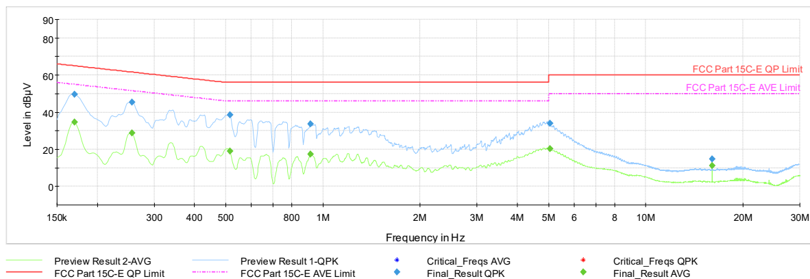
Plot 7-1164. AC Line Conducted Plot with 11be UNII Band 5 SDM Diversity – RU242 – Ch.61 (L1) with AC/DC Adapter
