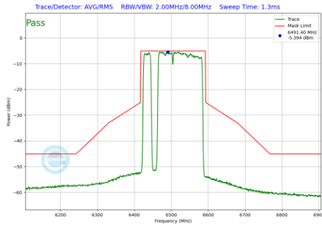
Plot 7-1268 In-Band Emission Plot SDM Diversity Antenna 3c (160MHz BW 802.11be(RU) RU996+484+242 Index97 (UNII Band 6) - Ch.111)
