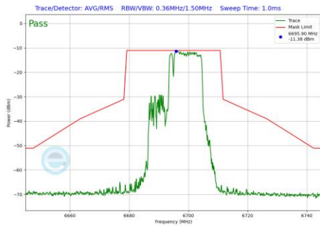
Plot 7-1269 In-Band Emission Plot SDM Diversity Antenna 3c (20MHz BW 802.11be(RU) RU106+26 Index83 (UNII Band 7) - Ch.149)
