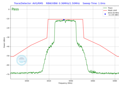
Plot 7-1278 In-Band Emission Plot SDM Diversity Antenna 1b (20MHz BW 802.11be(RU) RU242 Index61 (UNII Band 6) - Ch.97)
