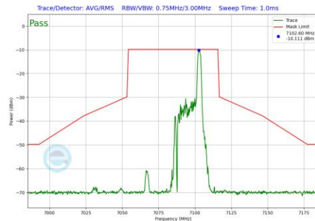
Plot 7-1233 In-Band Emission Plot SDM Diversity Antenna 1b (40MHz BW 802.11be(RU) RU26 Index17 (UNII Band 8) - Ch.227)
