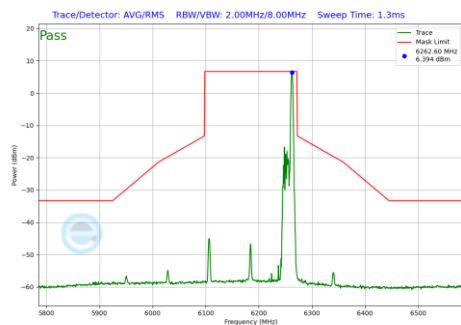
Plot 7-1157 In-Band Emission Plot CDD Diversity Antenna 1b (160MHz BW 802.11be(RU) RU26 Index36 (UNII Band 5) - Ch.47)
