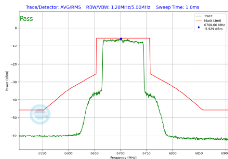
Plot 7-1300 In-Band Emission Plot SDM Diversity Antenna 3c (80MHz BW 802.11be(RU) RU996 Index67 (UNII Band 7) - Ch.151)
