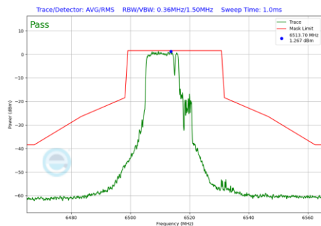
Plot 7-1181 In-Band Emission Plot CDD Diversity Antenna 1b (20MHz BW 802.11be(RU) RU106+26 Index82 (UNII Band 6) - Ch.113)
