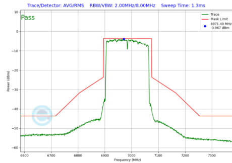
Plot 7-1153 In-Band Emission Plot SDM Primary Antenna 3a (160MHz BW 802.11be(RU) RU996X2 Index68 (UNII Band 8) - Ch.207)
