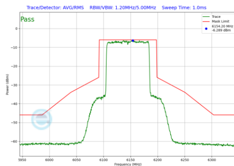
Plot 7-1292 In-Band Emission Plot SDM Diversity Antenna 3c (80MHz BW 802.11be(RU) RU996 Index67 (UNII Band 5) - Ch.39)
