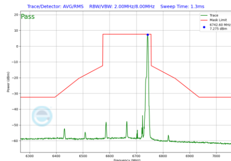
Plot 7-1177 In-Band Emission Plot CDD Diversity Antenna 3c (160MHz BW 802.11be(RU) RU26 Index36 (UNII Band 7) - Ch.143)
