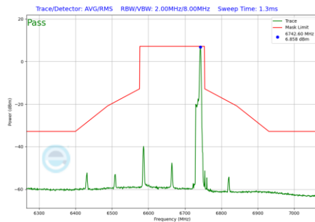
Plot 7-1165 In-Band Emission Plot CDD Diversity Antenna 1b (160MHz BW 802.11be(RU) RU26 Index36 (UNII Band 7) - Ch.143)
