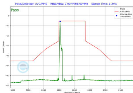
Plot 7-1239 In-Band Emission Plot SDM Diversity Antenna 3c (160MHz BW 802.11be(RU) RU26 Index0 (UNII Band 5) - Ch.47)
