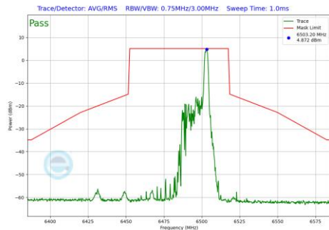
Plot 7-1171 In-Band Emission Plot CDD Diversity Antenna 3c (40MHz BW 802.11be(RU) RU26 Index17 (UNII Band 6) - Ch.107)
