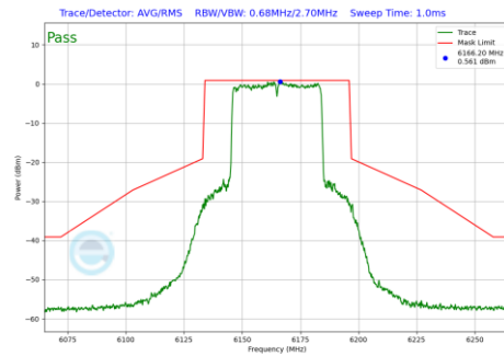
Plot 7-1209 In-Band Emission Plot CDD Diversity Antenna 3c (40MHz BW 802.11be(RU) RU484 Index65 (UNII Band 5) - Ch.43)
