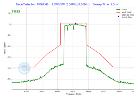
Plot 7-1183 In-Band Emission Plot CDD Diversity Antenna 1b (160MHz BW 802.11be(RU) RU996+484+242 Index96 (UNII Band 6) - Ch.111)
