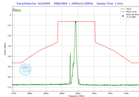
Plot 7-1234 In-Band Emission Plot SDM Diversity Antenna 1b (80MHz BW 802.11be(RU) RU26 Index17 (UNII Band 8) - Ch.199)
