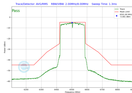
Plot 7-1281 In-Band Emission Plot SDM Diversity Antenna 1b (160MHz BW 802.11be(RU) RU996X2 Index68 (UNII Band 6) - Ch.111)
