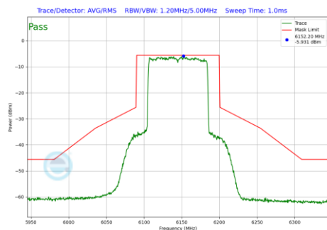
Plot 7-1276 In-Band Emission Plot SDM Diversity Antenna 1b (80MHz BW 802.11be(RU) RU996 Index67 (UNII Band 5) - Ch.39)
