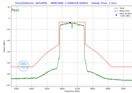
Plot 7-1149 In-Band Emission Plot SDM Primary Antenna 3a (160MHz BW 802.11be(RU) RU996X2 Index68 (UNII Band 7) - Ch.143)
