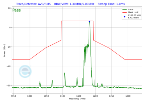
Plot 7-1156 In-Band Emission Plot CDD Diversity Antenna 1b (80MHz BW 802.11be(RU) RU26 Index36 (UNII Band 5) - Ch.39)
