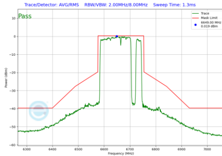
Plot 7-1186 In-Band Emission Plot CDD Diversity Antenna 1b (160MHz BW 802.11be(RU) RU996+484+242 Index98 (UNII Band 7) - Ch.143)
