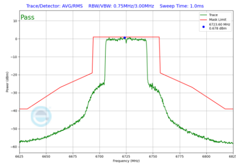
Plot 7-1205 In-Band Emission Plot CDD Diversity Antenna 1b (40MHz BW 802.11be(RU) RU484 Index65 (UNII Band 7) - Ch.155)
