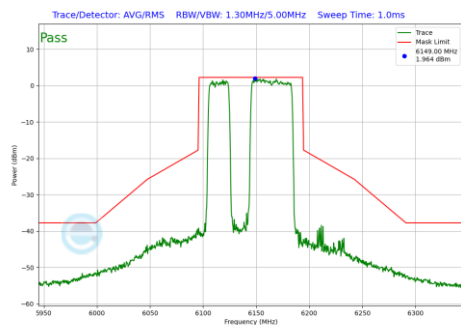
Plot 7-1179 In-Band Emission Plot CDD Diversity Antenna 1b (80MHz BW 802.11be(RU) RU484+242 Index91 (UNII Band 5) - Ch.39)
