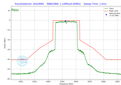
Plot 7-1202 In-Band Emission Plot CDD Diversity Antenna 1b (80MHz BW 802.11be(RU) RU996 Index67 (UNII Band 6) - Ch.103)
