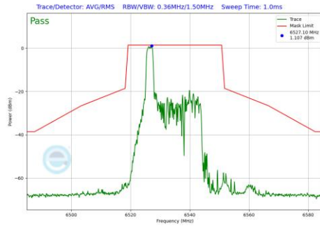
Plot 7-1162 In-Band Emission Plot CDD Diversity Antenna 1b (20MHz BW 802.11be(RU) RU26 Index0 (UNII Band 7) - Ch.117)
