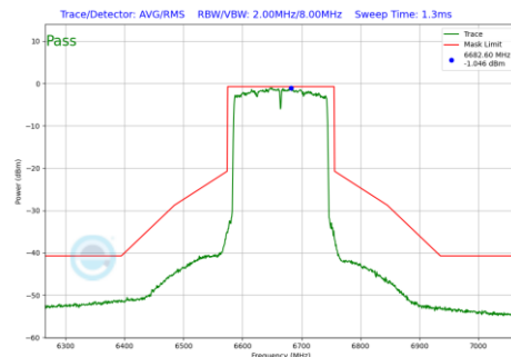
Plot 7-1219 In-Band Emission Plot CDD Diversity Antenna 3c (160MHz BW 802.11be(RU) RU996X2 Index68 (UNII Band 7) - Ch.143)
