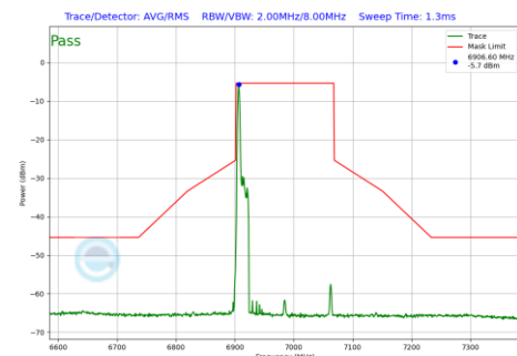
Plot 7-1251 In-Band Emission Plot SDM Diversity Antenna 3c (160MHz BW 802.11be(RU) RU26 Index0 (UNII Band 8) - Ch.207)
