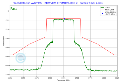
Plot 7-1283 In-Band Emission Plot SDM Diversity Antenna 1b (40MHz BW 802.11be(RU) RU484 Index65 (UNII Band 7) - Ch.155)
