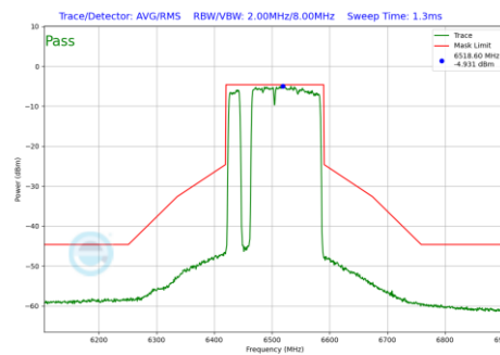
Plot 7-1257 In-Band Emission Plot SDM Diversity Antenna 1b (160MHz BW 802.11be(RU) RU996+484+242 Index97 (UNII Band 6) - Ch.111)
