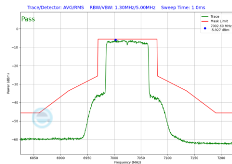
Plot 7-1304 In-Band Emission Plot SDM Diversity Antenna 3c (80MHz BW 802.11be(RU) RU996 Index67 (UNII Band 8) - Ch.215)
