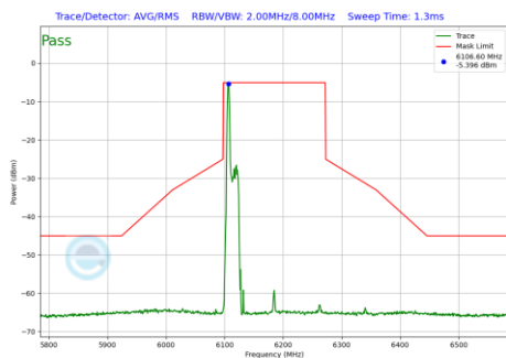
Plot 7-1223 In-Band Emission Plot SDM Diversity Antenna 1b (160MHz BW 802.11be(RU) RU26 Index0 (UNII Band 5) - Ch.47)
