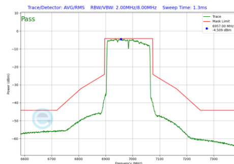
Plot 7-1289 In-Band Emission Plot SDM Diversity Antenna 1b (160MHz BW 802.11be(RU) RU996X2 Index68 (UNII Band 8) - Ch.207)
