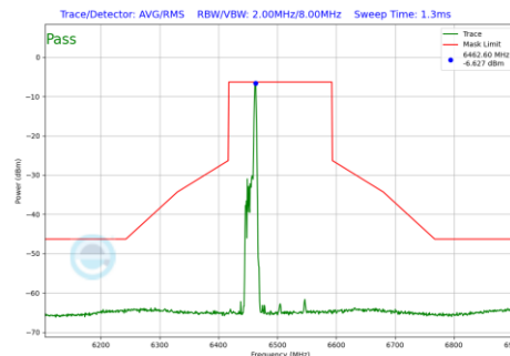
Plot 7-1243 In-Band Emission Plot SDM Diversity Antenna 3c (160MHz BW 802.11be(RU) RU26 Index17 (UNII Band 6) - Ch.111)
