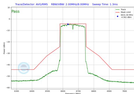
Plot 7-1285 In-Band Emission Plot SDM Diversity Antenna 1b (160MHz BW 802.11be(RU) RU996X2 Index68 (UNII Band 7) - Ch.143)
