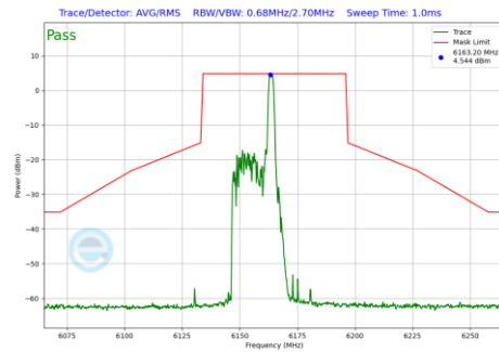
Plot 7-1167 In-Band Emission Plot CDD Diversity Antenna 3c (40MHz BW 802.11be(RU) RU26 Index8 (UNII Band 5) - Ch.43)
