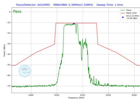
Plot 7-1255 In-Band Emission Plot SDM Diversity Antenna 1b (20MHz BW 802.11be(RU) RU106+26 Index82 (UNII Band 6) - Ch.113)
