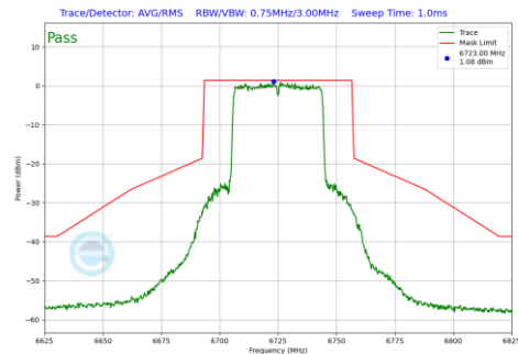
Plot 7-1217 In-Band Emission Plot CDD Diversity Antenna 3c (40MHz BW 802.11be(RU) RU484 Index65 (UNII Band 7) - Ch.155)
