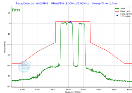
Plot 7-1191 In-Band Emission Plot CDD Diversity Antenna 3c (80MHz BW 802.11be(RU) RU484+242 Index92 (UNII Band 6) - Ch.103)
