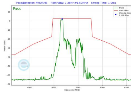
Plot 7-1174 In-Band Emission Plot CDD Diversity Antenna 3c (20MHz BW 802.11be(RU) RU26 Index0 (UNII Band 7) - Ch.117)
