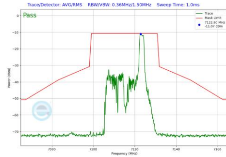
Plot 7-1248 In-Band Emission Plot SDM Diversity Antenna 3c (20MHz BW 802.11be(RU) RU26 Index8 (UNII Band 8) - Ch.233)
