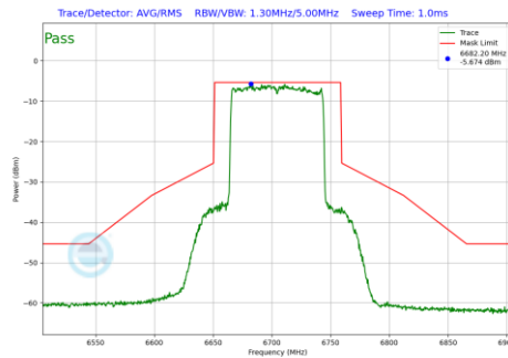
Plot 7-1148 In-Band Emission Plot SDM Primary Antenna 3a (80MHz BW 802.11be(RU) RU996 Index67 (UNII Band 7) - Ch.151)
