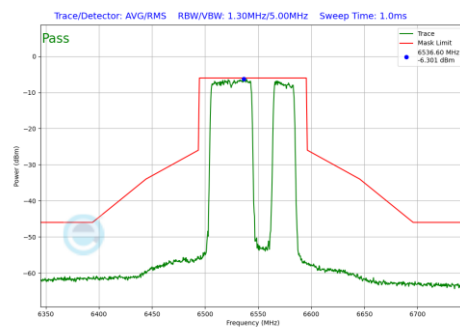
Plot 7-1259 In-Band Emission Plot SDM Diversity Antenna 1b (80MHz BW 802.11be(RU) RU484+242 Index92 (UNII Band 7) - Ch.119)
