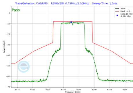
Plot 7-1291 In-Band Emission Plot SDM Diversity Antenna 3c (40MHz BW 802.11be(RU) RU484 Index65 (UNII Band 5) - Ch.43)
