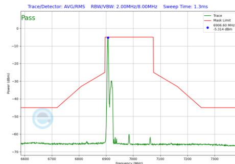
Plot 7-1235 In-Band Emission Plot SDM Diversity Antenna 1b (160MHz BW 802.11be(RU) RU26 Index0 (UNII Band 8) - Ch.207)
