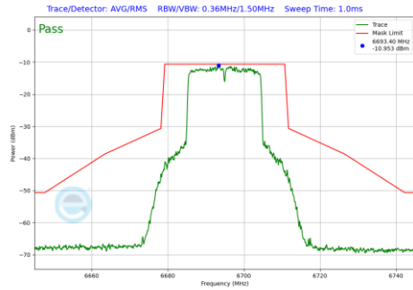
Plot 7-1298 In-Band Emission Plot SDM Diversity Antenna 3c (20MHz BW 802.11be(RU) RU242 Index61 (UNII Band 7) - Ch.149)
