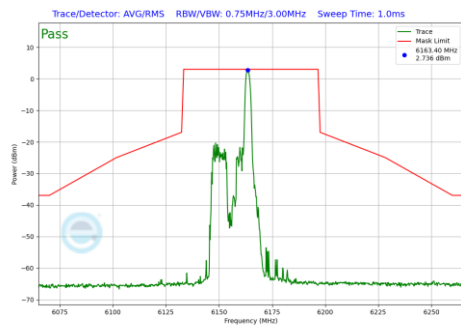
Plot 7-1155 In-Band Emission Plot CDD Diversity Antenna 1b (40MHz BW 802.11be(RU) RU26 Index8 (UNII Band 5) - Ch.43)
