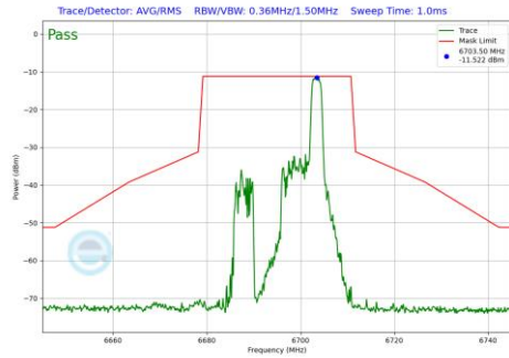
Plot 7-1228 In-Band Emission Plot SDM Diversity Antenna 1b (20MHz BW 802.11be(RU) RU26 Index8 (UNII Band 7) - Ch.149)
