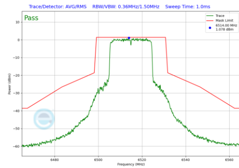
Plot 7-1200 In-Band Emission Plot CDD Diversity Antenna 1b (20MHz BW 802.11be(RU) RU242 Index61 (UNII Band 6) - Ch.113)
