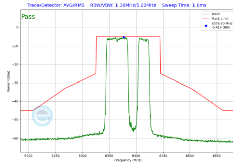
Plot 7-1264 In-Band Emission Plot SDM Diversity Antenna 3c (80MHz BW 802.11be(RU) RU484+242 Index92 (UNII Band 5) - Ch.87)
