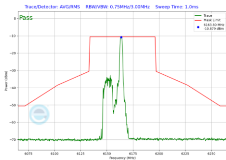
Plot 7-1221 In-Band Emission Plot SDM Diversity Antenna 1b (40MHz BW 802.11be(RU) RU26 Index8 (UNII Band 5) - Ch.43)
