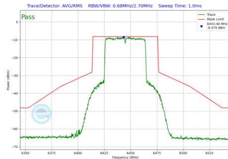
Plot 7-1295 In-Band Emission Plot SDM Diversity Antenna 3c (40MHz BW 802.11be(RU) RU484 Index65 (UNII Band 6) - Ch.99)
