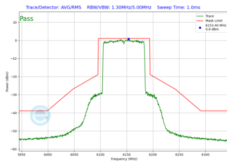
Plot 7-1198 In-Band Emission Plot CDD Diversity Antenna 1b (80MHz BW 802.11be(RU) RU996 Index67 (UNII Band 5) - Ch.39)
