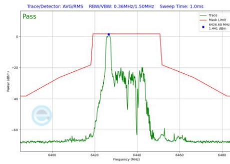
Plot 7-1158 In-Band Emission Plot CDD Diversity Antenna 1b (20MHz BW 802.11be(RU) RU26 Index0 (UNII Band 6) - Ch.97)
