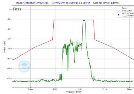
Plot 7-1232 In-Band Emission Plot SDM Diversity Antenna 1b (20MHz BW 802.11be(RU) RU26 Index8 (UNII Band 8) - Ch.229)
