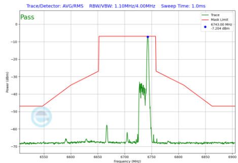
Plot 7-1230 In-Band Emission Plot SDM Diversity Antenna 1b (80MHz BW 802.11be(RU) RU26 Index36 (UNII Band 7) - Ch.151)
