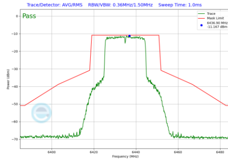
Plot 7-1294 In-Band Emission Plot SDM Diversity Antenna 3c (20MHz BW 802.11be(RU) RU242 Index61 (UNII Band 6) - Ch.97)
