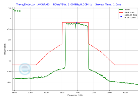
Plot 7-1273 In-Band Emission Plot SDM Diversity Antenna 3c (160MHz BW 802.11be(RU) RU996+484+242 Index96 (UNII Band 8) - Ch.207)
