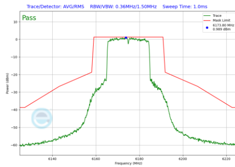
Plot 7-1196 In-Band Emission Plot CDD Diversity Antenna 1b (20MHz BW 802.11be(RU) RU242 Index61 (UNII Band 5) - Ch.45)
