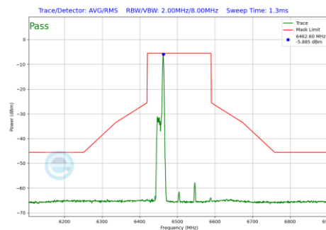
Plot 7-1227 In-Band Emission Plot SDM Diversity Antenna 1b (160MHz BW 802.11be(RU) RU26 Index17 (UNII Band 6) - Ch.111)
