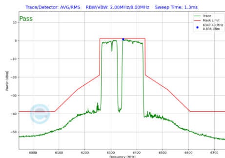
Plot 7-1180 In-Band Emission Plot CDD Diversity Antenna 1b (160MHz BW 802.11be(RU) RU996+484+242 Index99 (UNII Band 5) - Ch.79)
