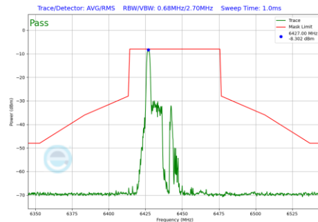
Plot 7-1241 In-Band Emission Plot SDM Diversity Antenna 3c (40MHz BW 802.11be(RU) RU26 Index0 (UNII Band 6) - Ch.99)
