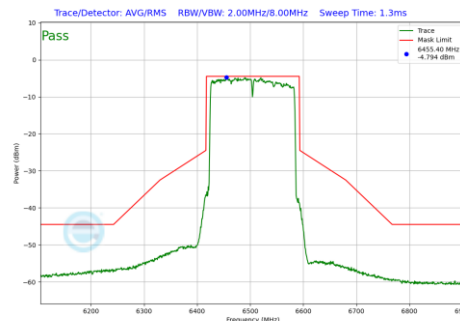
Plot 7-1297 In-Band Emission Plot SDM Diversity Antenna 3c (160MHz BW 802.11be(RU) RU996X2 Index68 (UNII Band 6) - Ch.111)
