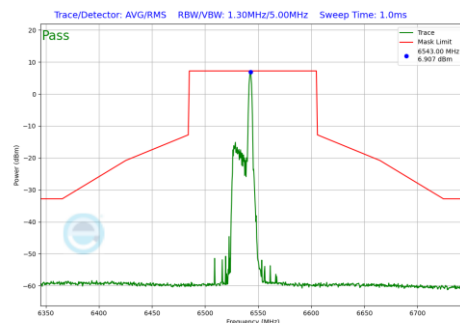
Plot 7-1176 In-Band Emission Plot CDD Diversity Antenna 3c (80MHz BW 802.11be(RU) RU26 Index17 (UNII Band 7) - Ch.119)
