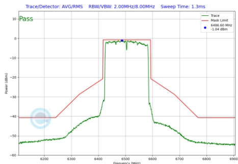
Plot 7-1215 In-Band Emission Plot CDD Diversity Antenna 3c (160MHz BW 802.11be(RU) RU996X2 Index68 (UNII Band 6) - Ch.111)
