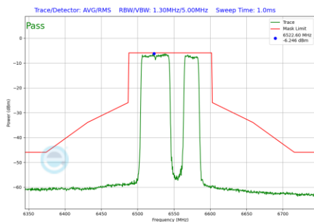
Plot 7-1270 In-Band Emission Plot SDM Diversity Antenna 3c (80MHz BW 802.11be(RU) RU484+242 Index92 (UNII Band 7) - Ch.119)
