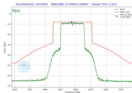
Plot 7-1279 In-Band Emission Plot SDM Diversity Antenna 1b (40MHz BW 802.11be(RU) RU484 Index65 (UNII Band 6) - Ch.99)
