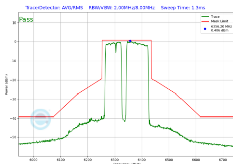
Plot 7-1189 In-Band Emission Plot CDD Diversity Antenna 3c (160MHz BW 802.11be(RU) RU996+484+242 Index99 (UNII Band 5) - Ch.79)
