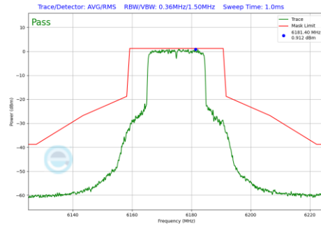
Plot 7-1208 In-Band Emission Plot CDD Diversity Antenna 3c (20MHz BW 802.11be(RU) RU242 Index61 (UNII Band 5) - Ch.45)
