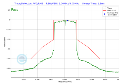
Plot 7-1203 In-Band Emission Plot CDD Diversity Antenna 1b (160MHz BW 802.11be(RU) RU996X2 Index68 (UNII Band 6) - Ch.111)
