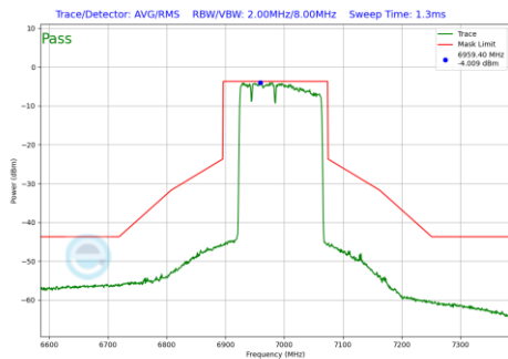
Plot 7-1262 In-Band Emission Plot SDM Diversity Antenna 1b (160MHz BW 802.11be(RU) RU996+484+242 Index96 (UNII Band 8) - Ch.207)
