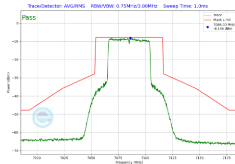
Plot 7-1287 In-Band Emission Plot SDM Diversity Antenna 1b (40MHz BW 802.11be(RU) RU484 Index65 (UNII Band 8) - Ch.227)
