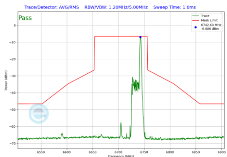
Plot 7-1246 In-Band Emission Plot SDM Diversity Antenna 3c (80MHz BW 802.11be(RU) RU26 Index36 (UNII Band 7) - Ch.151)
