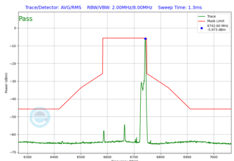
Plot 7-1247 In-Band Emission Plot SDM Diversity Antenna 3c (160MHz BW 802.11be(RU) RU26 Index36 (UNII Band 7) - Ch.143)
