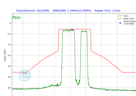
Plot 7-1267 In-Band Emission Plot SDM Diversity Antenna 3c (80MHz BW 802.11be(RU) RU484+242 Index92 (UNII Band 6) - Ch.103)
