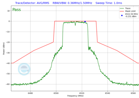
Plot 7-1212 In-Band Emission Plot CDD Diversity Antenna 3c (20MHz BW 802.11be(RU) RU242 Index61 (UNII Band 6) - Ch.113)
