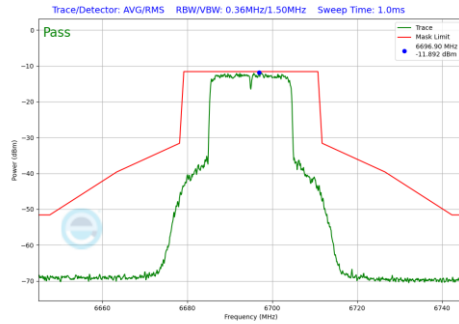
Plot 7-1146 In-Band Emission Plot SDM Primary Antenna 3a (20MHz BW 802.11be(RU) RU242 Index61 (UNII Band 7) - Ch.149)
