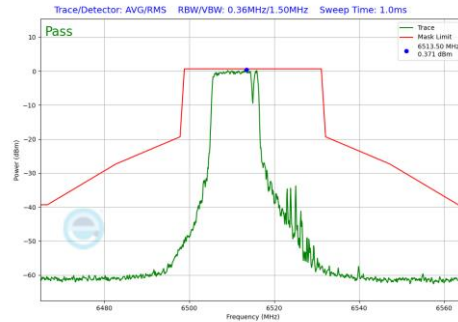
Plot 7-1190 In-Band Emission Plot CDD Diversity Antenna 3c (20MHz BW 802.11be(RU) RU106+26 Index82 (UNII Band 6) - Ch.113)
