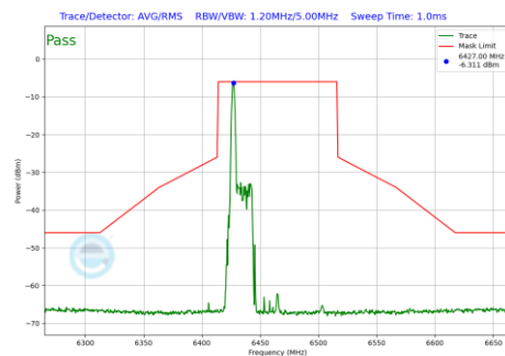
Plot 7-1242 In-Band Emission Plot SDM Diversity Antenna 3c (80MHz BW 802.11be(RU) RU26 Index0 (UNII Band 6) - Ch.103)
