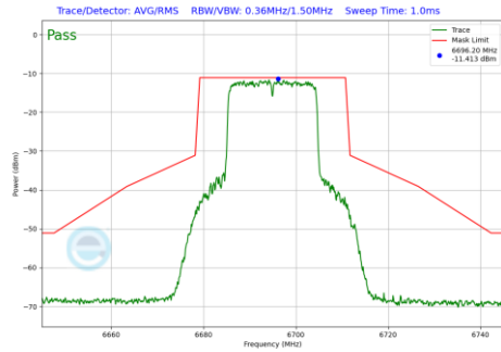
Plot 7-1282 In-Band Emission Plot SDM Diversity Antenna 1b (20MHz BW 802.11be(RU) RU242 Index61 (UNII Band 7) - Ch.149)
