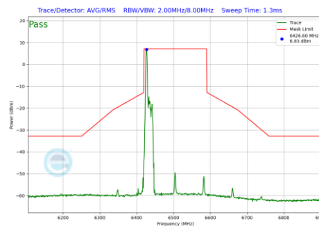
Plot 7-1161 In-Band Emission Plot CDD Diversity Antenna 1b (160MHz BW 802.11be(RU) RU26 Index0 (UNII Band 6) - Ch.111)
