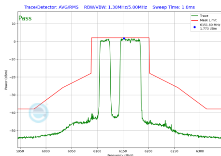
Plot 7-1188 In-Band Emission Plot CDD Diversity Antenna 3c (80MHz BW 802.11be(RU) RU484+242 Index91 (UNII Band 5) - Ch.39)
