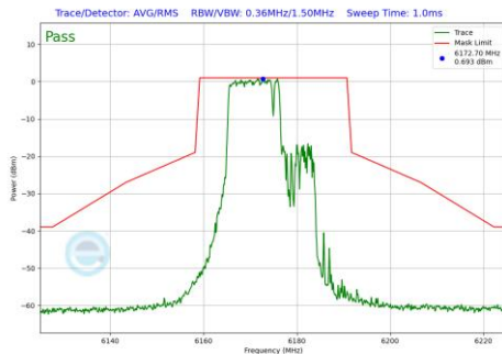
Plot 7-1187 In-Band Emission Plot CDD Diversity Antenna 3c (20MHz BW 802.11be(RU) RU106+26 Index82 (UNII Band 5) - Ch.45)
