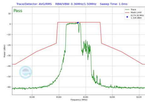
Plot 7-1178 In-Band Emission Plot CDD Diversity Antenna 1b (20MHz BW 802.11be(RU) RU106+26 Index82 (UNII Band 5) - Ch.45)
