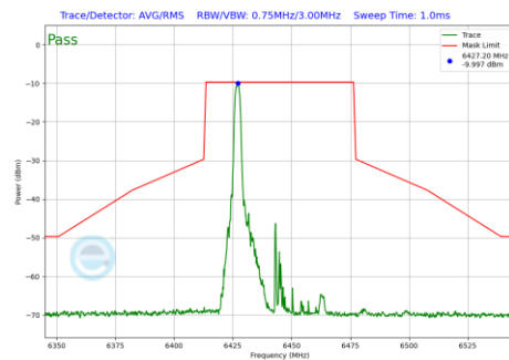
Plot 7-1225 In-Band Emission Plot SDM Diversity Antenna 1b (40MHz BW 802.11be(RU) RU26 Index0 (UNII Band 6) - Ch.99)
