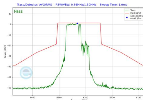
Plot 7-1193 In-Band Emission Plot CDD Diversity Antenna 3c (20MHz BW 802.11be(RU) RU106+26 Index82 (UNII Band 7) - Ch.149)
