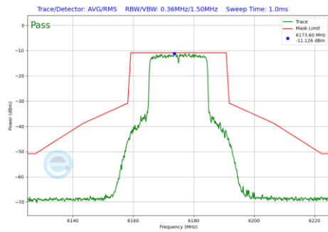
Plot 7-1274 In-Band Emission Plot SDM Diversity Antenna 1b (20MHz BW 802.11be(RU) RU242 Index61 (UNII Band 5) - Ch.45)
