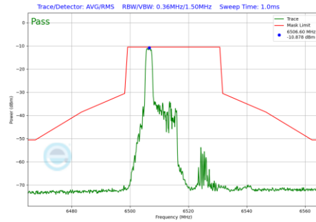
Plot 7-1240 In-Band Emission Plot SDM Diversity Antenna 3c (20MHz BW 802.11be(RU) RU26 Index0 (UNII Band 6) - Ch.113)
