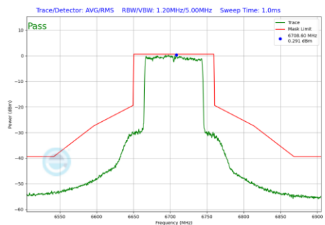
Plot 7-1206 In-Band Emission Plot CDD Diversity Antenna 1b (80MHz BW 802.11be(RU) RU996 Index67 (UNII Band 7) - Ch.151)
