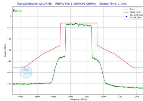
Plot 7-1152 In-Band Emission Plot SDM Primary Antenna 3a (80MHz BW 802.11be(RU) RU996 Index67 (UNII Band 8) - Ch.215)
