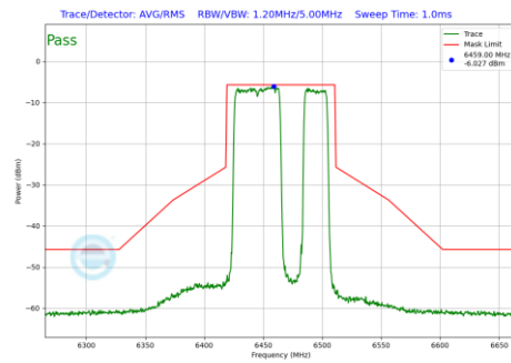
Plot 7-1256 In-Band Emission Plot SDM Diversity Antenna 1b (80MHz BW 802.11be(RU) RU484+242 Index92 (UNII Band 6) - Ch.103)
