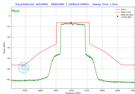
Plot 7-1284 In-Band Emission Plot SDM Diversity Antenna 1b (80MHz BW 802.11be(RU) RU996 Index67 (UNII Band 7) - Ch.151)
