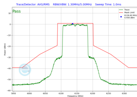
Plot 7-1210 In-Band Emission Plot CDD Diversity Antenna 3c (80MHz BW 802.11be(RU) RU996 Index67 (UNII Band 5) - Ch.39)
