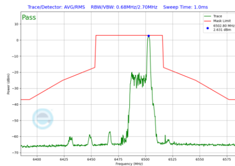
Plot 7-1159 In-Band Emission Plot CDD Diversity Antenna 1b (40MHz BW 802.11be(RU) RU26 Index17 (UNII Band 6) - Ch.107)
