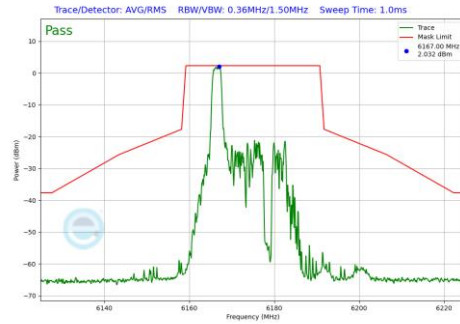
Plot 7-1166 In-Band Emission Plot CDD Diversity Antenna 3c (20MHz BW 802.11be(RU) RU26 Index0 (UNII Band 5) - Ch.45)
