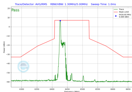
Plot 7-1172 In-Band Emission Plot CDD Diversity Antenna 3c (80MHz BW 802.11be(RU) RU26 Index0 (UNII Band 6) - Ch.103)
