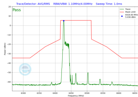
Plot 7-1160 In-Band Emission Plot CDD Diversity Antenna 1b (80MHz BW 802.11be(RU) RU26 Index0 (UNII Band 6) - Ch.103)
