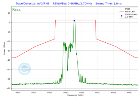
Plot 7-1163 In-Band Emission Plot CDD Diversity Antenna 1b (40MHz BW 802.11be(RU) RU26 Index8 (UNII Band 7) - Ch.123)
