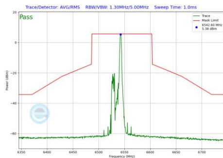
Plot 7-1164 In-Band Emission Plot CDD Diversity Antenna 1b (80MHz BW 802.11be(RU) RU26 Index17 (UNII Band 7) - Ch.119)
