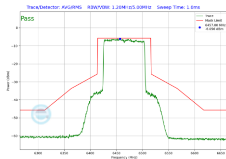
Plot 7-1296 In-Band Emission Plot SDM Diversity Antenna 3c (80MHz BW 802.11be(RU) RU996 Index67 (UNII Band 6) - Ch.103)
