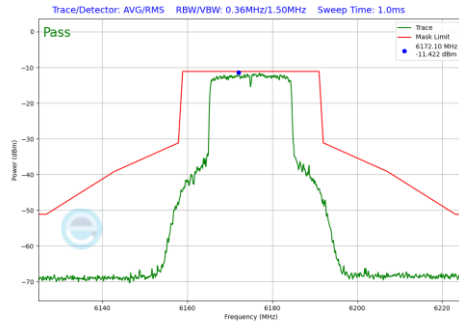
Plot 7-1290 In-Band Emission Plot SDM Diversity Antenna 3c (20MHz BW 802.11be(RU) RU242 Index61 (UNII Band 5) - Ch.45)
