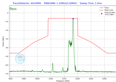
Plot 7-1222 In-Band Emission Plot SDM Diversity Antenna 1b (80MHz BW 802.11be(RU) RU26 Index36 (UNII Band 5) - Ch.39)
