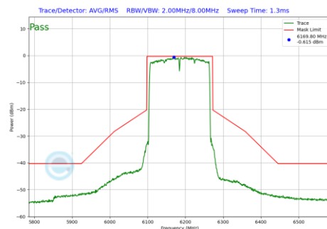
Plot 7-1211 In-Band Emission Plot CDD Diversity Antenna 3c (160MHz BW 802.11be(RU) RU996X2 Index68 (UNII Band 5) - Ch.47)
