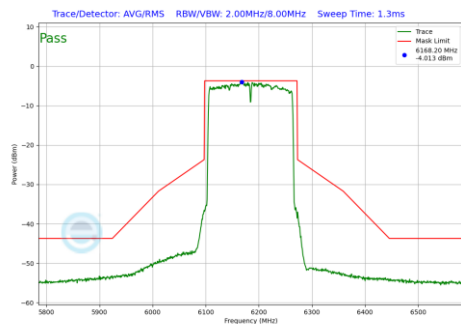
Plot 7-1277 In-Band Emission Plot SDM Diversity Antenna 1b (160MHz BW 802.11be(RU) RU996X2 Index68 (UNII Band 5) - Ch.47)
