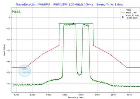
Plot 7-1253 In-Band Emission Plot SDM Diversity Antenna 1b (80MHz BW 802.11be(RU) RU484+242 Index92 (UNII Band 5) - Ch.87)
