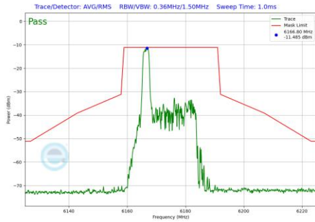
Plot 7-1236 In-Band Emission Plot SDM Diversity Antenna 3c (20MHz BW 802.11be(RU) RU26 Index0 (UNII Band 5) - Ch.45)
