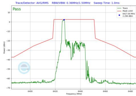
Plot 7-1170 In-Band Emission Plot CDD Diversity Antenna 3c (20MHz BW 802.11be(RU) RU26 Index0 (UNII Band 6) - Ch.97)
