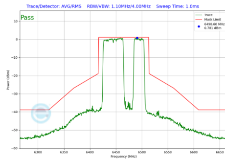
Plot 7-1182 In-Band Emission Plot CDD Diversity Antenna 1b (80MHz BW 802.11be(RU) RU484+242 Index92 (UNII Band 6) - Ch.103)
