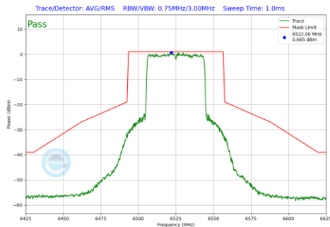
Plot 7-1213 In-Band Emission Plot CDD Diversity Antenna 3c (40MHz BW 802.11be(RU) RU484 Index65 (UNII Band 6) - Ch.115)
