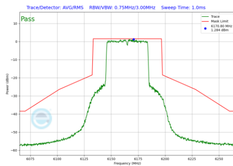
Plot 7-1197 In-Band Emission Plot CDD Diversity Antenna 1b (40MHz BW 802.11be(RU) RU484 Index65 (UNII Band 5) - Ch.43)
