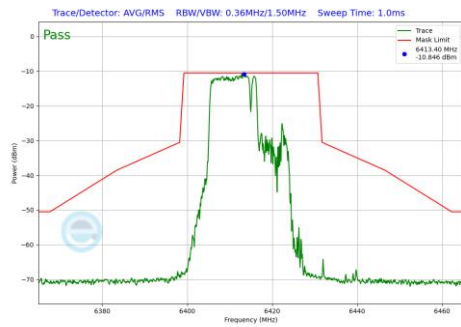
Plot 7-1252 In-Band Emission Plot SDM Diversity Antenna 1b (20MHz BW 802.11be(RU) RU106+26 Index82 (UNII Band 5) - Ch.93)
