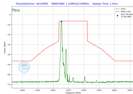
Plot 7-1226 In-Band Emission Plot SDM Diversity Antenna 1b (80MHz BW 802.11be(RU) RU26 Index0 (UNII Band 6) - Ch.103)
