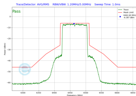
Plot 7-1280 In-Band Emission Plot SDM Diversity Antenna 1b (80MHz BW 802.11be(RU) RU996 Index67 (UNII Band 6) - Ch.103)
