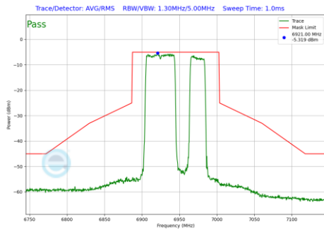
Plot 7-1261 In-Band Emission Plot SDM Diversity Antenna 1b (80MHz BW 802.11be(RU) RU484+242 Index92 (UNII Band 8) - Ch.199)
