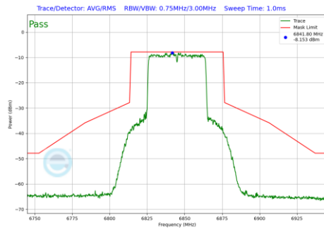
Plot 7-1147 In-Band Emission Plot SDM Primary Antenna 3a (40MHz BW 802.11be(RU) RU484 Index65 (UNII Band 7) - Ch.179)
