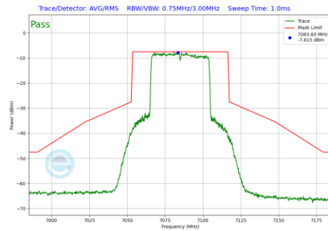
Plot 7-1151 In-Band Emission Plot SDM Primary Antenna 3a (40MHz BW 802.11be(RU) RU484 Index65 (UNII Band 8) - Ch.227)
