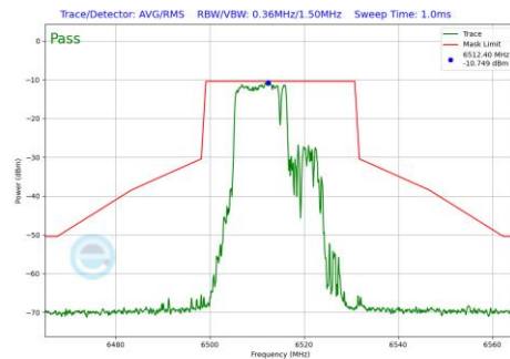
Plot 7-1266 In-Band Emission Plot SDM Diversity Antenna 3c (20MHz BW 802.11be(RU) RU106+26 Index82 (UNII Band 6) - Ch.113)
