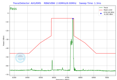
Plot 7-1231 In-Band Emission Plot SDM Diversity Antenna 1b (160MHz BW 802.11be(RU) RU26 Index36 (UNII Band 7) - Ch.143)
