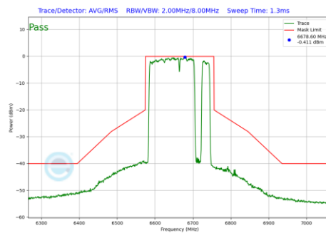
Plot 7-1195 In-Band Emission Plot CDD Diversity Antenna 3c (160MHz BW 802.11be(RU) RU996+484+242 Index98 (UNII Band 7) - Ch.143)
