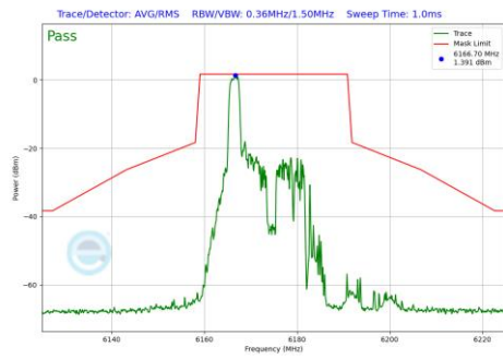
Plot 7-1154 In-Band Emission Plot CDD Diversity Antenna 1b (20MHz BW 802.11be(RU) RU26 Index0 (UNII Band 5) - Ch.45)
