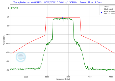
Plot 7-1150 In-Band Emission Plot SDM Primary Antenna 3a (20MHz BW 802.11be(RU) RU242 Index61 (UNII Band 8) - Ch.209)
