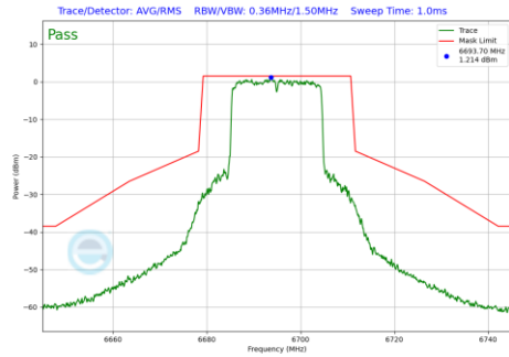
Plot 7-1204 In-Band Emission Plot CDD Diversity Antenna 1b (20MHz BW 802.11be(RU) RU242 Index61 (UNII Band 7) - Ch.149)
