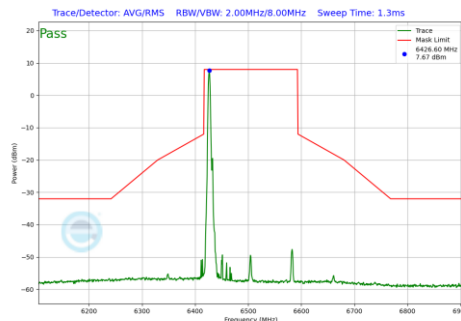
Plot 7-1173 In-Band Emission Plot CDD Diversity Antenna 3c (160MHz BW 802.11be(RU) RU26 Index0 (UNII Band 6) - Ch.111)
