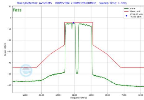
Plot 7-1271 In-Band Emission Plot SDM Diversity Antenna 3c (160MHz BW 802.11be(RU) RU996+484+242 Index99 (UNII Band 7) - Ch.175)
