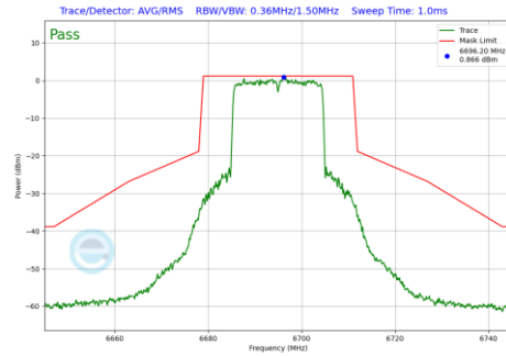
Plot 7-1216 In-Band Emission Plot CDD Diversity Antenna 3c (20MHz BW 802.11be(RU) RU242 Index61 (UNII Band 7) - Ch.149)
