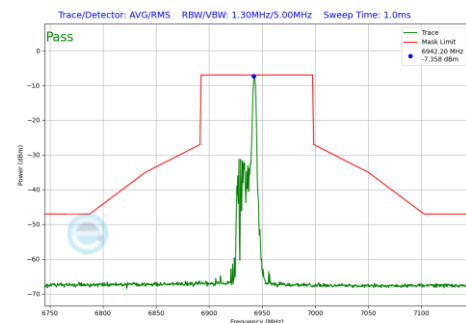
Plot 7-1250 In-Band Emission Plot SDM Diversity Antenna 3c (80MHz BW 802.11be(RU) RU26 Index17 (UNII Band 8) - Ch.199)
