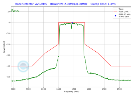
Plot 7-1199 In-Band Emission Plot CDD Diversity Antenna 1b (160MHz BW 802.11be(RU) RU996X2 Index68 (UNII Band 5) - Ch.47)
