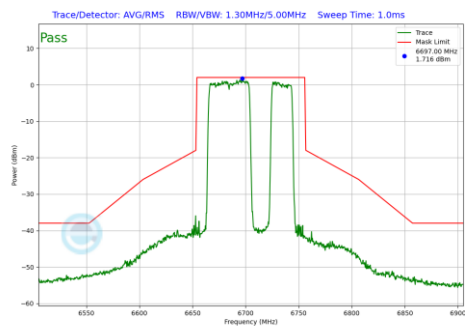
Plot 7-1194 In-Band Emission Plot CDD Diversity Antenna 3c (80MHz BW 802.11be(RU) RU484+242 Index92 (UNII Band 7) - Ch.151)
