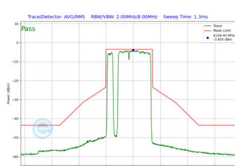
Plot 7-1265 In-Band Emission Plot SDM Diversity Antenna 3c (160MHz BW 802.11be(RU) RU996+484+242 Index97 (UNII Band 5) - Ch.47)
