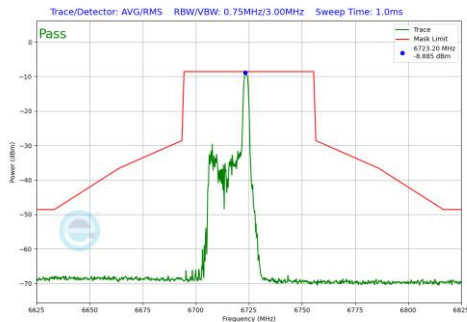
Plot 7-1245 In-Band Emission Plot SDM Diversity Antenna 3c (40MHz BW 802.11be(RU) RU26 Index8 (UNII Band 7) - Ch.155)
