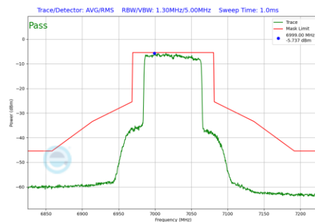
Plot 7-1288 In-Band Emission Plot SDM Diversity Antenna 1b (80MHz BW 802.11be(RU) RU996 Index67 (UNII Band 8) - Ch.215)
