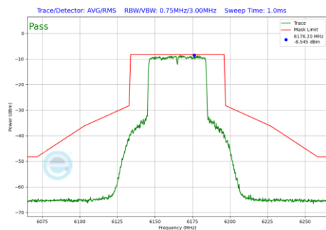
Plot 7-1275 In-Band Emission Plot SDM Diversity Antenna 1b (40MHz BW 802.11be(RU) RU484 Index65 (UNII Band 5) - Ch.43)
