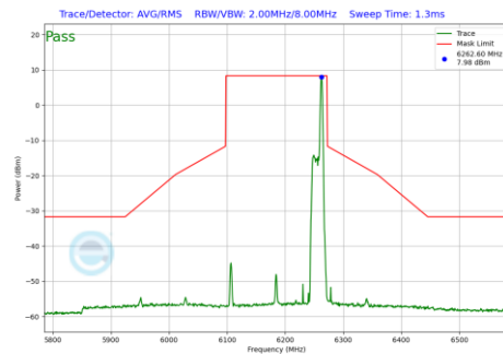
Plot 7-1169 In-Band Emission Plot CDD Diversity Antenna 3c (160MHz BW 802.11be(RU) RU26 Index36 (UNII Band 5) - Ch.47)
