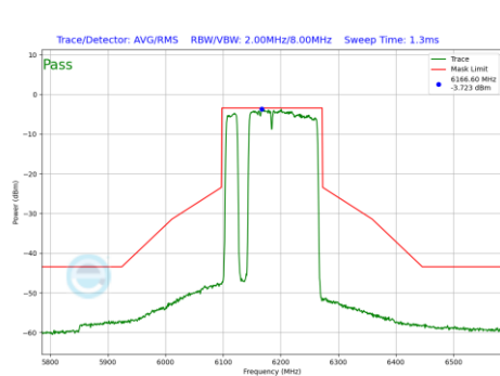
Plot 7-1254 In-Band Emission Plot SDM Diversity Antenna 1b (160MHz BW 802.11be(RU) RU996+484+242 Index97 (UNII Band 5) - Ch.47)
