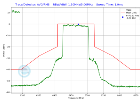
Plot 7-1214 In-Band Emission Plot CDD Diversity Antenna 3c (80MHz BW 802.11be(RU) RU996 Index67 (UNII Band 6) - Ch.103)
