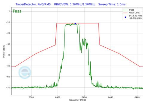
Plot 7-1263 In-Band Emission Plot SDM Diversity Antenna 3c (20MHz BW 802.11be(RU) RU106+26 Index82 (UNII Band 5) - Ch.93)
