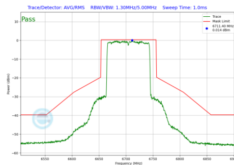
Plot 7-1218 In-Band Emission Plot CDD Diversity Antenna 3c (80MHz BW 802.11be(RU) RU996 Index67 (UNII Band 7) - Ch.151)
