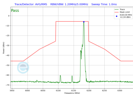
Plot 7-1238 In-Band Emission Plot SDM Diversity Antenna 3c (80MHz BW 802.11be(RU) RU26 Index36 (UNII Band 5) - Ch.39)
