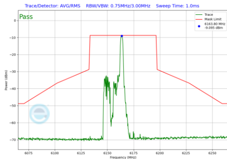
Plot 7-1237 In-Band Emission Plot SDM Diversity Antenna 3c (40MHz BW 802.11be(RU) RU26 Index8 (UNII Band 5) - Ch.43)
