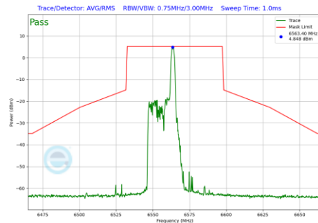
Plot 7-1175 In-Band Emission Plot CDD Diversity Antenna 3c (40MHz BW 802.11be(RU) RU26 Index8 (UNII Band 7) - Ch.123)
