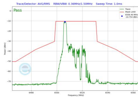
Plot 7-1224 In-Band Emission Plot SDM Diversity Antenna 1b (20MHz BW 802.11be(RU) RU26 Index0 (UNII Band 6) - Ch.113)
