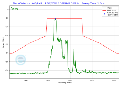
Plot 7-1220 In-Band Emission Plot SDM Diversity Antenna 1b (20MHz BW 802.11be(RU) RU26 Index0 (UNII Band 5) - Ch.45)
