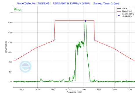
Plot 7-1249 In-Band Emission Plot SDM Diversity Antenna 3c (40MHz BW 802.11be(RU) RU26 Index17 (UNII Band 8) - Ch.227)
