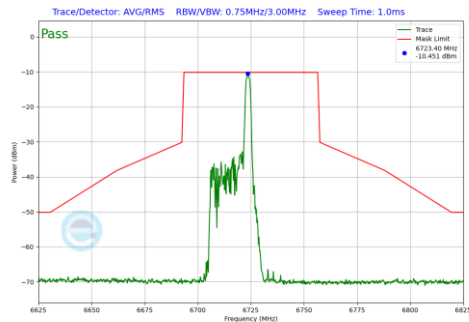
Plot 7-1229 In-Band Emission Plot SDM Diversity Antenna 1b (40MHz BW 802.11be(RU) RU26 Index8 (UNII Band 7) - Ch.155)
