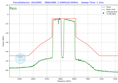
Plot 7-1260 In-Band Emission Plot SDM Diversity Antenna 1b (160MHz BW 802.11be(RU) RU996+484+242 Index99 (UNII Band 7) - Ch.175)
