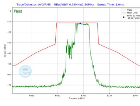
Plot 7-1258 In-Band Emission Plot SDM Diversity Antenna 1b (20MHz BW 802.11be(RU) RU106+26 Index83 (UNII Band 7) - Ch.149)
