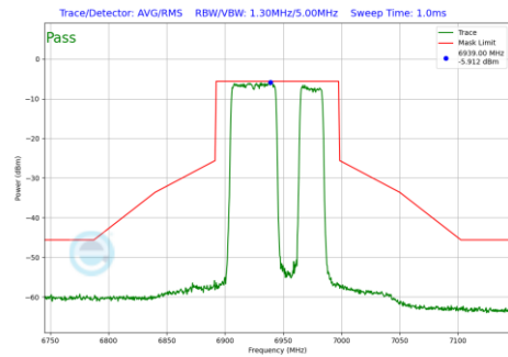
Plot 7-1272 In-Band Emission Plot SDM Diversity Antenna 3c (80MHz BW 802.11be(RU) RU484+242 Index92 (UNII Band 8) - Ch.199)
