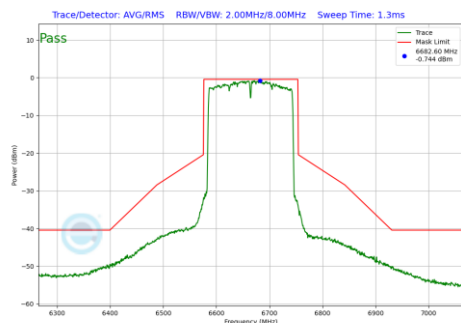
Plot 7-1207 In-Band Emission Plot CDD Diversity Antenna 1b (160MHz BW 802.11be(RU) RU996X2 Index68 (UNII Band 7) - Ch.143)
