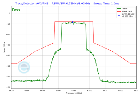
Plot 7-1299 In-Band Emission Plot SDM Diversity Antenna 3c (40MHz BW 802.11be(RU) RU484 Index65 (UNII Band 7) - Ch.155)
