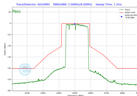
Plot 7-1192 In-Band Emission Plot CDD Diversity Antenna 3c (160MHz BW 802.11be(RU) RU996+484+242 Index96 (UNII Band 6) - Ch.111)
