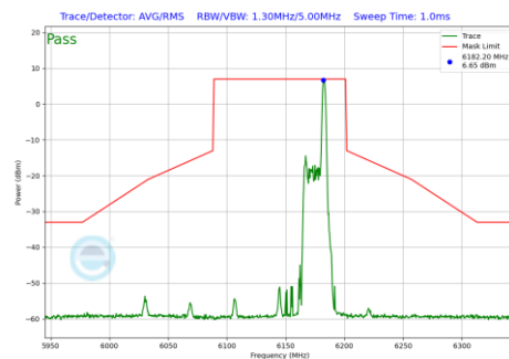
Plot 7-1168 In-Band Emission Plot CDD Diversity Antenna 3c (80MHz BW 802.11be(RU) RU26 Index36 (UNII Band 5) - Ch.39)
