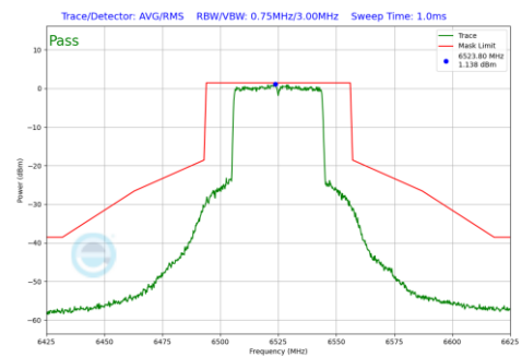
Plot 7-1201 In-Band Emission Plot CDD Diversity Antenna 1b (40MHz BW 802.11be(RU) RU484 Index65 (UNII Band 6) - Ch.115)
