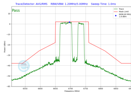
Plot 7-1185 In-Band Emission Plot CDD Diversity Antenna 1b (80MHz BW 802.11be(RU) RU484+242 Index92 (UNII Band 7) - Ch.151)
