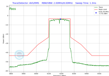
Plot 7-1293 In-Band Emission Plot SDM Diversity Antenna 3c (160MHz BW 802.11be(RU) RU996X2 Index68 (UNII Band 5) - Ch.47)
