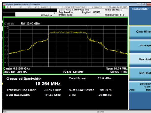
Plot 7-173 26dB BW & 99% OBW Antenna 1b (20MHz BW 802.11be(RU) RU242 Index61 - Ch.113)
