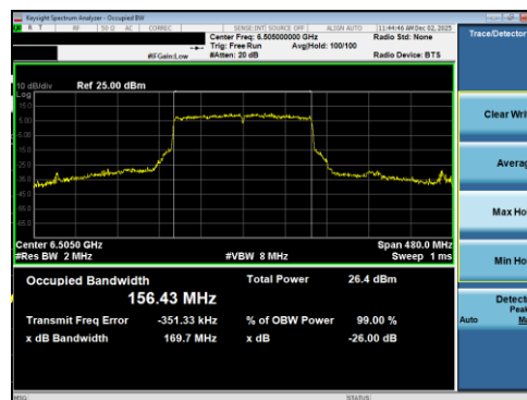
Plot 7-176 26dB BW & 99% OBW Antenna 1b (160MHz BW 802.11be(RU) RU996X2 Index68 - Ch.111)
