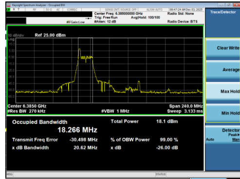
Plot 7-157 26dB BW & 99% OBW Antenna 1b (80MHz BW 802.11be(RU) RU26 Index0 - Ch.87)
