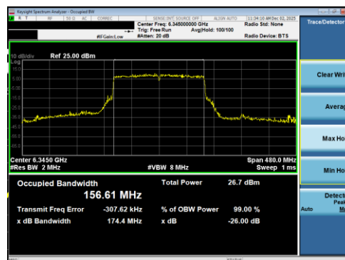
Plot 7-165 26dB BW & 99% OBW Antenna 1b (160MHz BW 802.11be(RU) RU996X2 Index68 - Ch.79)
