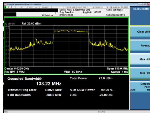
Plot 7-161 26dB BW & 99% OBW Antenna 1b (160MHz BW 802.11be(RU) RU996+484+242 Index96 - Ch.15)
