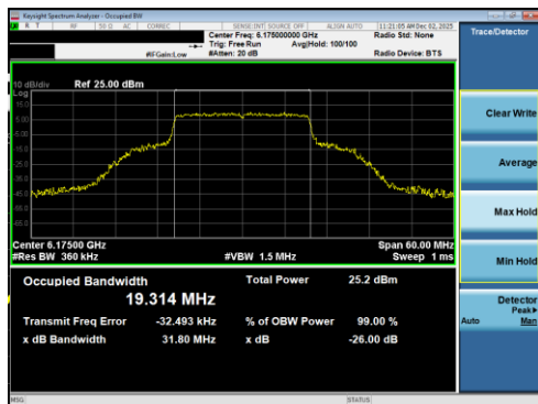
Plot 7-162 26dB BW & 99% OBW Antenna 1b (20MHz BW 802.11be(RU) RU242 Index61 - Ch.45)
