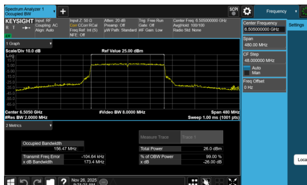
Plot 7-99 26dB BW & 99% OBW Antenna 3a (160MHz BW 802.11be(RU) RU996X2 Index68 - Ch.111)
