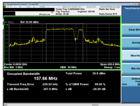
Plot 7-183 26dB BW & 99% OBW Antenna 1b (160MHz BW 802.11be(RU) RU996+484+242 Index98 - Ch.143)
