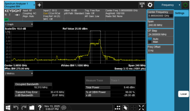
Plot 7-113 26dB BW & 99% OBW Antenna 3a (80MHz BW 802.11be(RU) RU26 Index36 - Ch.7)
