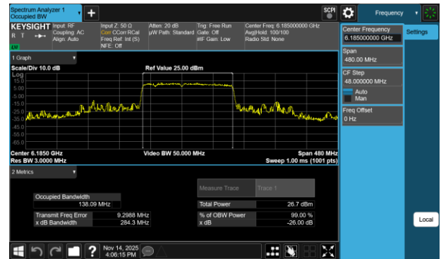
Plot 7-117 26dB BW & 99% OBW Antenna 3a (160MHz BW 802.11be(RU) RU996+484+242 Index96 - Ch.47)
