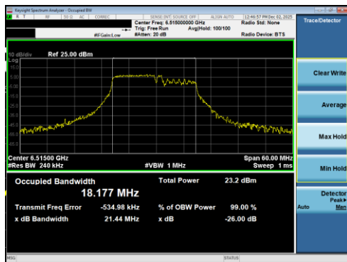
Plot 7-170 26dB BW & 99% OBW Antenna 1b (20MHz BW 802.11be(RU) RU106+26 Index82 - Ch.113)
