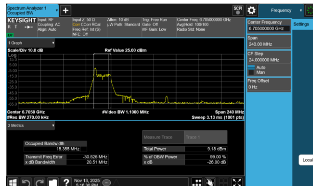
Plot 7-135 26dB BW & 99% OBW Antenna 3a (80MHz BW 802.11be(RU) RU26 Index0 - Ch.151)
