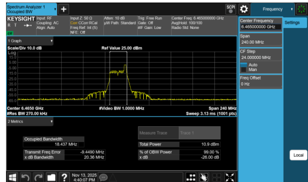
Plot 7-124 26dB BW & 99% OBW Antenna 3a (80MHz BW 802.11be(RU) RU26 Index17 - Ch.103)
