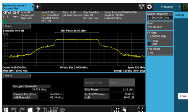
Plot 7-130 26dB BW & 99% OBW Antenna 3a (40MHz BW 802.11be(RU) RU484 Index65 - Ch.107)
