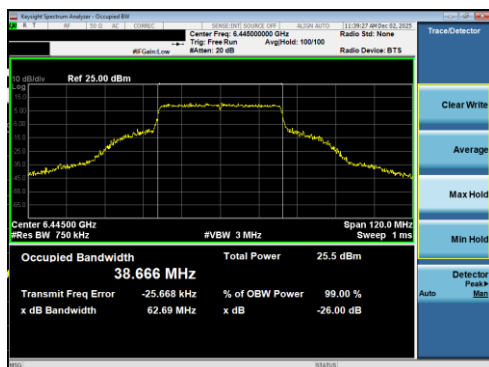
Plot 7-174 26dB BW & 99% OBW Antenna 1b (40MHz BW 802.11be(RU) RU484 Index65 - Ch.99)
