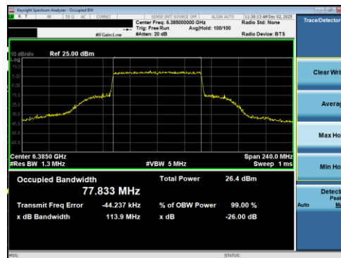
Plot 7-164 26dB BW & 99% OBW Antenna 1b (80MHz BW 802.11be(RU) RU996 Index67 - Ch.87)
