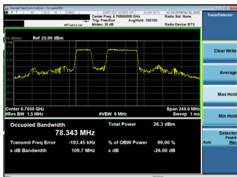
Plot 7-182 26dB BW & 99% OBW Antenna 1b (80MHz BW 802.11be(RU) RU484+242 Index91 - Ch.151)
