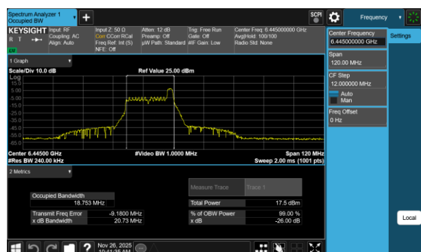
Plot 7-90 26dB BW & 99% OBW Antenna 3a (40MHz BW 802.11be(RU) RU26 Index8 - Ch.99)
