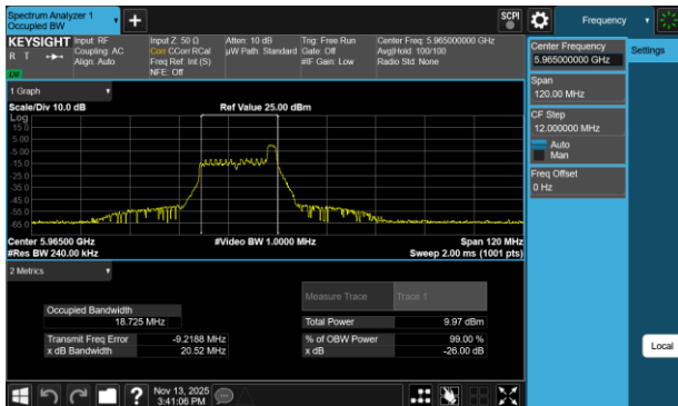
Plot 7-112 26dB BW & 99% OBW Antenna 3a (40MHz BW 802.11be(RU) RU26 Index8 - Ch.3)
