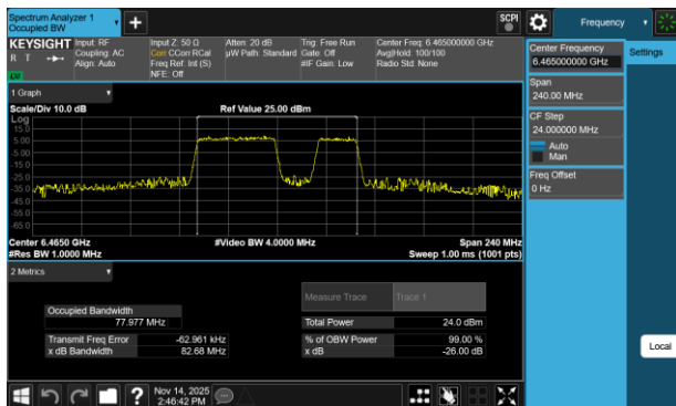
Plot 7-127 26dB BW & 99% OBW Antenna 3a (80MHz BW 802.11be(RU) RU484+242 Index92 - Ch.103)
