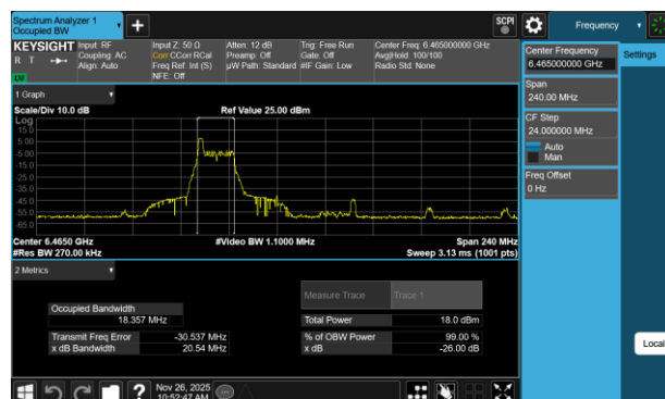
Plot 7-91 26dB BW & 99% OBW Antenna 3a (80MHz BW 802.11be(RU) RU26 Index0 - Ch.103)
