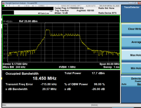
Plot 7-155 26dB BW & 99% OBW Antenna 1b (20MHz BW 802.11be(RU) RU26 Index0 - Ch.45)
