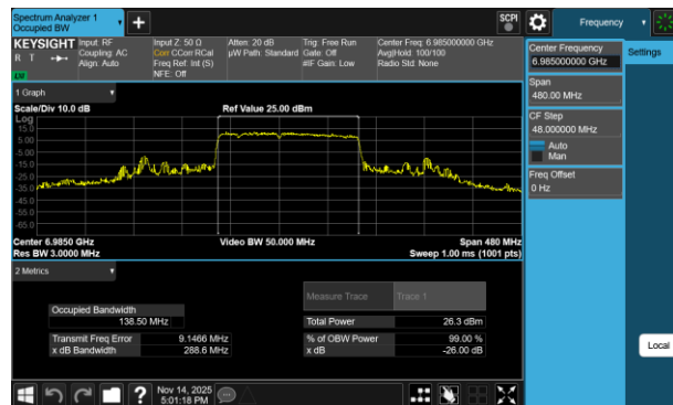
Plot 7-150 26dB BW & 99% OBW Antenna 3a (160MHz BW 802.11be(RU) RU996+484+242 Index96 - Ch.207)
