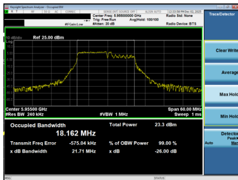
Plot 7-159 26dB BW & 99% OBW Antenna 1b (20MHz BW 802.11be(RU) RU106+26 Index82 - Ch.1)
