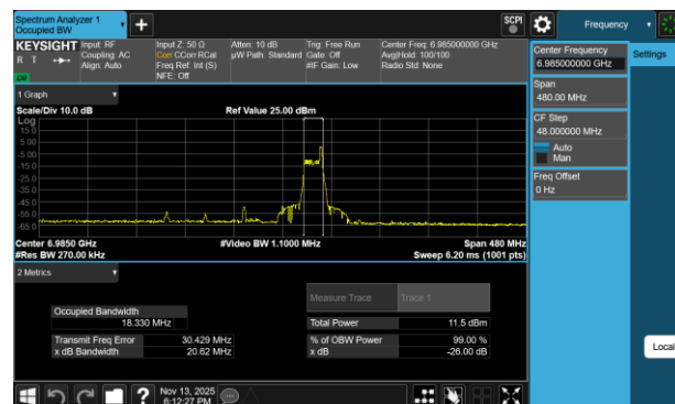
Plot 7-147 26dB BW & 99% OBW Antenna 3a (160MHz BW 802.11be(RU) RU26 Index17 - Ch.207)
