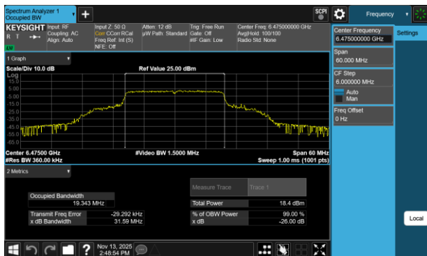
Plot 7-129 26dB BW & 99% OBW Antenna 3a (20MHz BW 802.11be(RU) RU242 Index61 - Ch.105)
