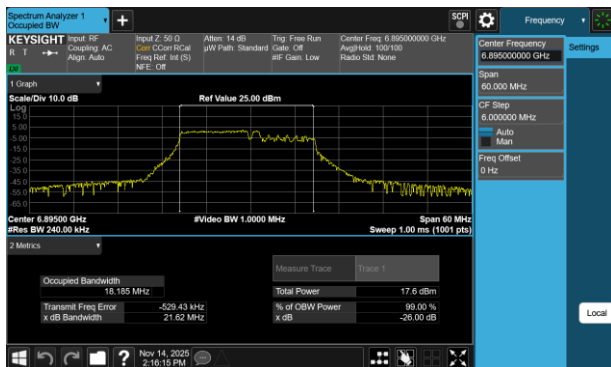
Plot 7-148 26dB BW & 99% OBW Antenna 3a (20MHz BW 802.11be(RU) RU106+26 Index82 - Ch.189)
