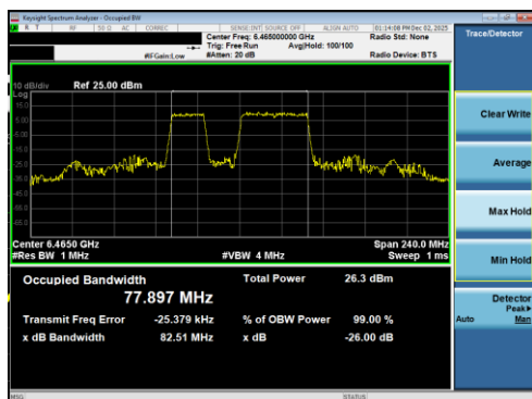
Plot 7-171 26dB BW & 99% OBW Antenna 1b (80MHz BW 802.11be(RU) RU484+242 Index91 - Ch.103)
