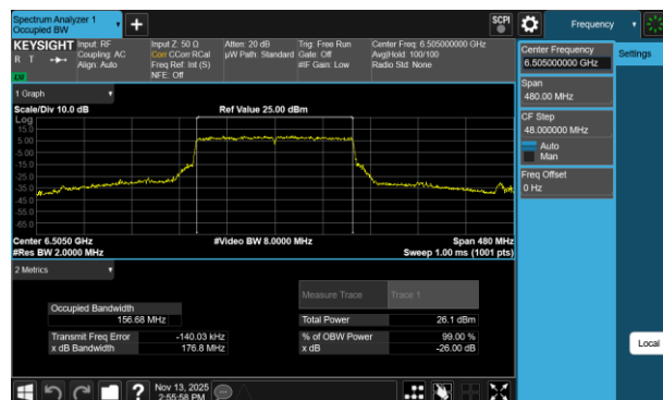
Plot 7-132 26dB BW & 99% OBW Antenna 3a (160MHz BW 802.11be(RU) RU996X2 Index68 - Ch.111)
