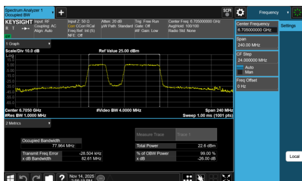
Plot 7-138 26dB BW & 99% OBW Antenna 3a (80MHz BW 802.11be(RU) RU484+242 Index91 - Ch.151)
