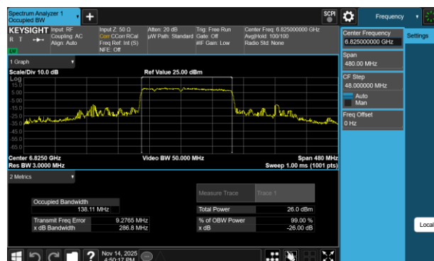
Plot 7-139 26dB BW & 99% OBW Antenna 3a (160MHz BW 802.11be(RU) RU996+484+242 Index96 - Ch.175)
