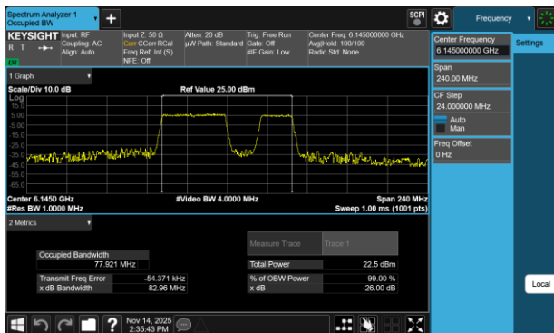
Plot 7-116 26dB BW & 99% OBW Antenna 3a (80MHz BW 802.11be(RU) RU484+242 Index92 - Ch.39)
