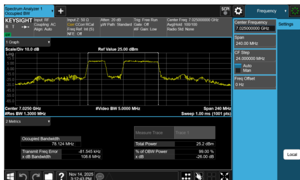
Plot 7-149 26dB BW & 99% OBW Antenna 3a (80MHz BW 802.11be(RU) RU484+242 Index91 - Ch.215)
