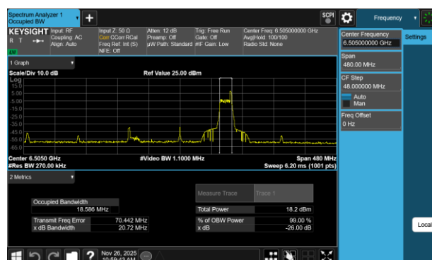
Plot 7-92 26dB BW & 99% OBW Antenna 3a (160MHz BW 802.11be(RU) RU26 Index36 - Ch.111)
