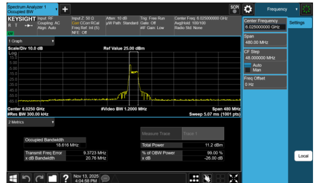
Plot 7-114 26dB BW & 99% OBW Antenna 3a (160MHz BW 802.11be(RU) RU26 Index0 - Ch.15)
