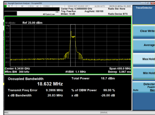
Plot 7-158 26dB BW & 99% OBW Antenna 1b (160MHz BW 802.11be(RU) RU26 Index0 - Ch.79)
