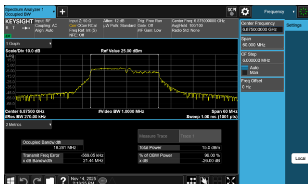
Plot 7-137 26dB BW & 99% OBW Antenna 3a (20MHz BW 802.11be(RU) RU106+26 Index82 - Ch.185)
