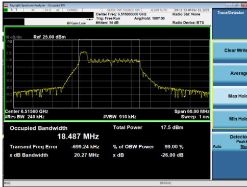
Plot 7-166 26dB BW & 99% OBW Antenna 1b (20MHz BW 802.11be(RU) RU26 Index0 - Ch.113)
