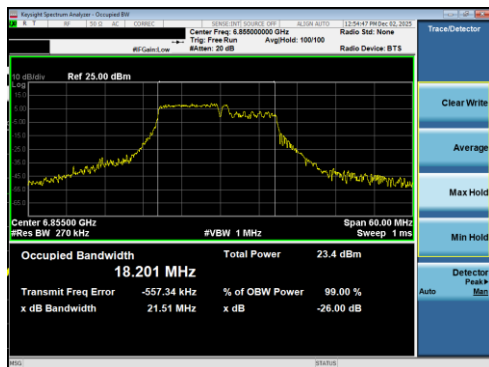
Plot 7-181 26dB BW & 99% OBW Antenna 1b (20MHz BW 802.11be(RU) RU106+26 Index82 - Ch.181)
