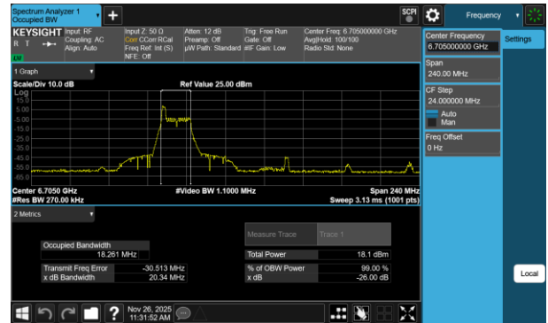
Plot 7-102 26dB BW & 99% OBW Antenna 3a (80MHz BW 802.11be(RU) RU26 Index0 - Ch.151)
