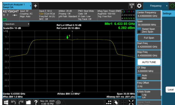
Plot 7-250 PSD Antenna 3c (20MHz BW 802.11be(RU) RU242 Index61 - Ch.97)
