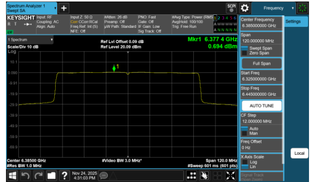
Plot 7-241 PSD Antenna 3c (80MHz BW 802.11be(RU) RU996 Index67 - Ch.87)
