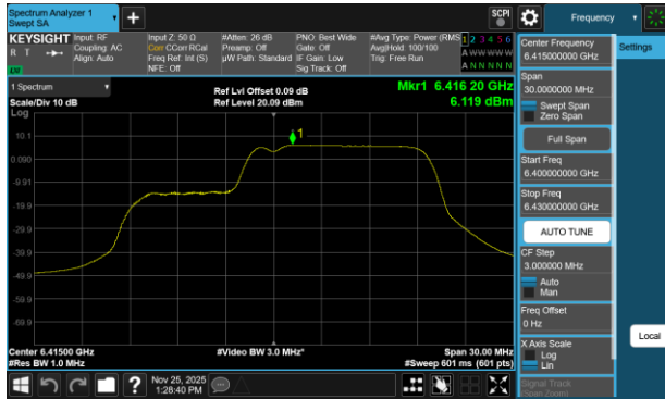
Plot 7-236 PSD Antenna 3c (20MHz BW 802.11be(RU) RU106+26 Index83 - Ch.93)
