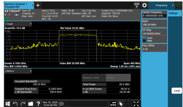
Plot 7-194 26dB BW & 99% OBW Antenna 1b (160MHz BW 802.11be(RU) RU996+484+242 Index96 - Ch.47)
