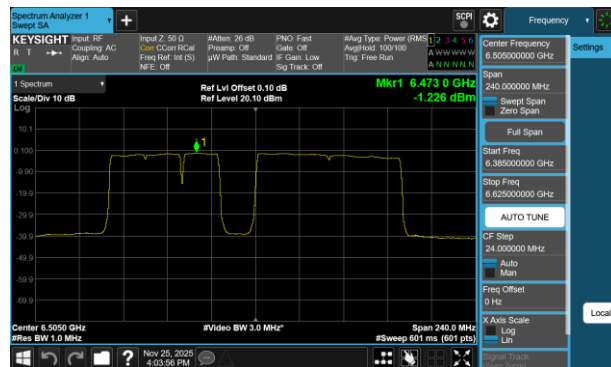
Plot 7-249 PSD Antenna 3c (160MHz BW 802.11be(RU) RU996+484+242 Index99 - Ch.111)
