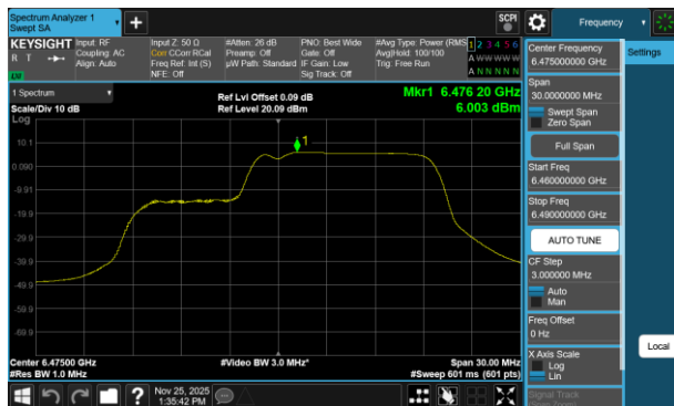
Plot 7-247 PSD Antenna 3c (20MHz BW 802.11be(RU) RU106+26 Index83 - Ch.105)
