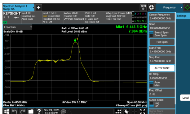
Plot 7-244 PSD Antenna 3c (40MHz BW 802.11be(RU) RU26 Index8 - Ch.99)
