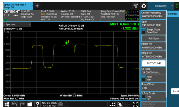
Plot 7-260 PSD Antenna 3c (160MHz BW 802.11be(RU) RU996+484+242 Index97 - Ch.143)
