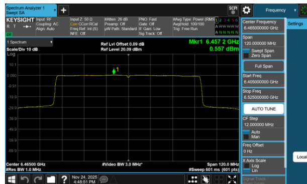
Plot 7-252 PSD Antenna 3c (80MHz BW 802.11be(RU) RU996 Index67 - Ch.103)
