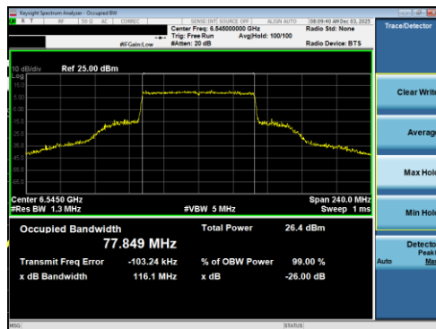
Plot 7-186 26dB BW & 99% OBW Antenna 1b (80MHz BW 802.11be(RU) RU996 Index67 - Ch.119)
