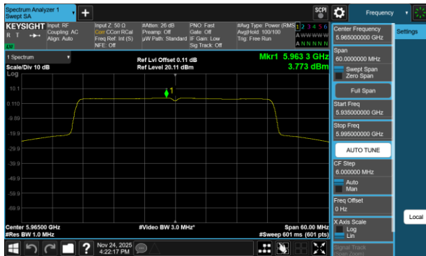
Plot 7-240 PSD Antenna 3c (40MHz BW 802.11be(RU) RU484 Index65 - Ch.3)
