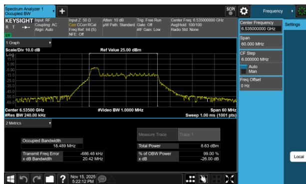
Plot 7-210 26dB BW & 99% OBW Antenna 1b (20MHz BW 802.11be(RU) RU26 Index0 - Ch.117)
