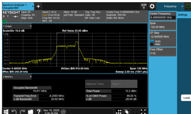
Plot 7-200 26dB BW & 99% OBW Antenna 1b (40MHz BW 802.11be(RU) RU26 Index8 - Ch.107)
