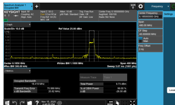
Plot 7-191 26dB BW & 99% OBW Antenna 1b (160MHz BW 802.11be(RU) RU26 Index36 - Ch.47)
