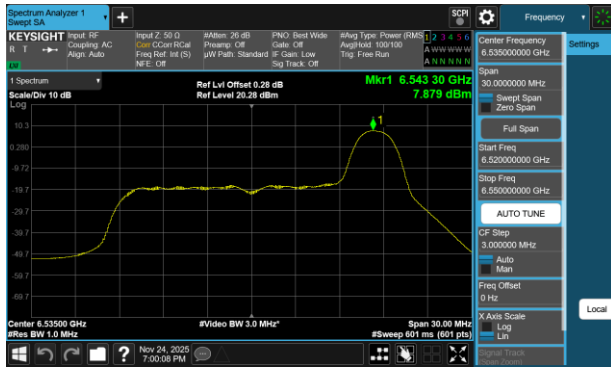
Plot 7-254 PSD Antenna 3c (20MHz BW 802.11be(RU) RU26 Index8 - Ch.117)
