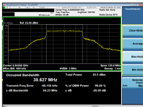
Plot 7-185 26dB BW & 99% OBW Antenna 1b (40MHz BW 802.11be(RU) RU484 Index65 - Ch.179)
