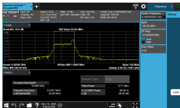
Plot 7-211 26dB BW & 99% OBW Antenna 1b (40MHz BW 802.11be(RU) RU26 Index8 - Ch.123)
