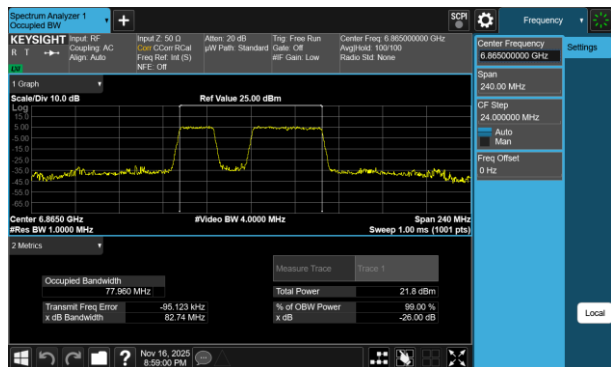
Plot 7-215 26dB BW & 99% OBW Antenna 1b (80MHz BW 802.11be(RU) RU484+242 Index91 - Ch.183)
