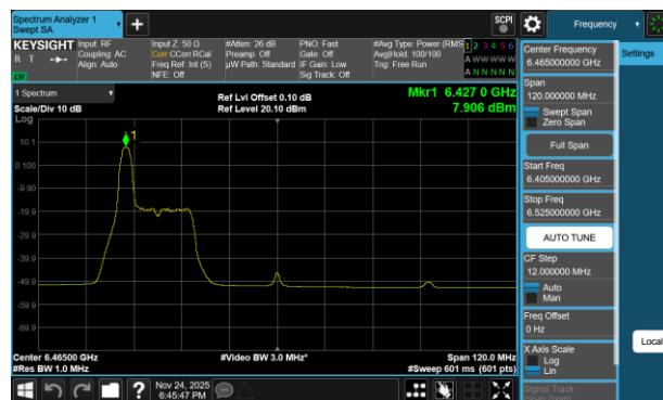
Plot 7-245 PSD Antenna 3c (80MHz BW 802.11be(RU) RU26 Index0 - Ch.103)
