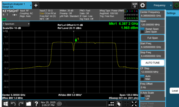
Plot 7-237 PSD Antenna 3c (80MHz BW 802.11be(RU) RU484+242 Index90 - Ch.87)
