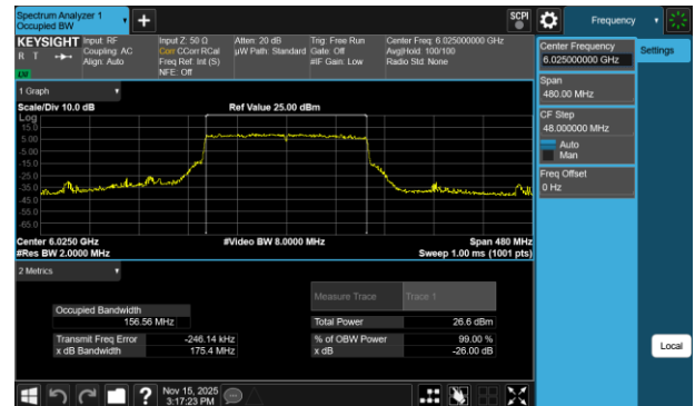
Plot 7-198 26dB BW & 99% OBW Antenna 1b (160MHz BW 802.11be(RU) RU996X2 Index68 - Ch.15)
