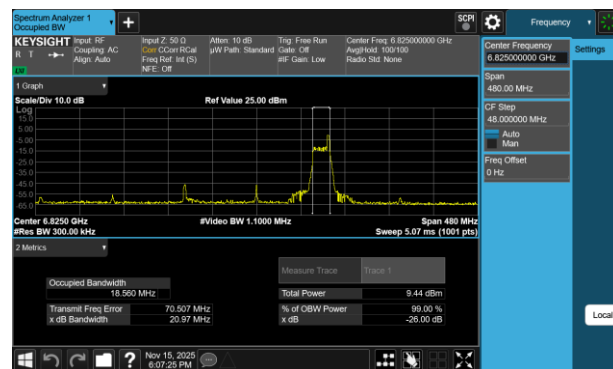
Plot 7-213 26dB BW & 99% OBW Antenna 1b (160MHz BW 802.11be(RU) RU26 Index36 - Ch.175)
