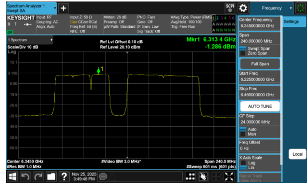
Plot 7-238 PSD Antenna 3c (160MHz BW 802.11be(RU) RU996+484+242 Index99 - Ch.79)
