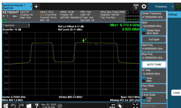
Plot 7-259 PSD Antenna 3c (80MHz BW 802.11be(RU) RU484+242 Index91 - Ch.151)
