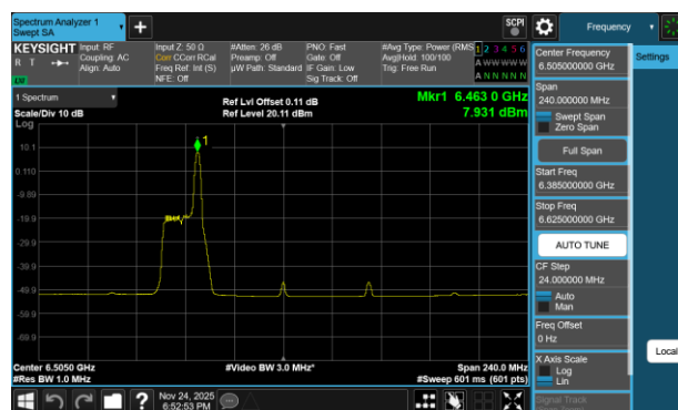
Plot 7-246 PSD Antenna 3c (160MHz BW 802.11be(RU) RU26 Index17 - Ch.111)
