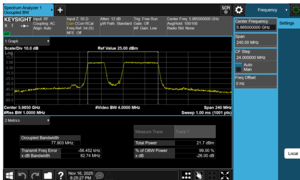
Plot 7-193 26dB BW & 99% OBW Antenna 1b (80MHz BW 802.11be(RU) RU484+242 Index91 - Ch.7)
