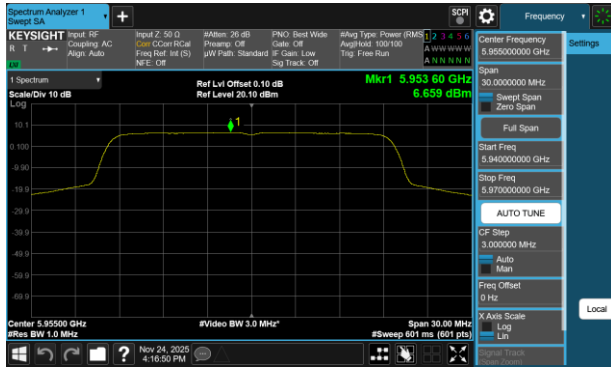
Plot 7-239 PSD Antenna 3c (20MHz BW 802.11be(RU) RU242 Index61 - Ch.1)
