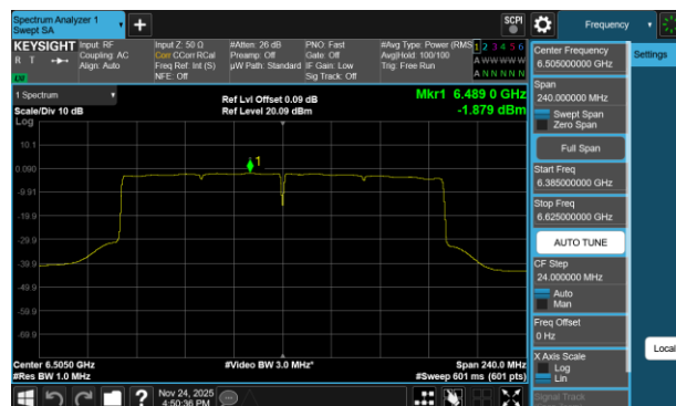
Plot 7-253 PSD Antenna 3c (160MHz BW 802.11be(RU) RU996X2 Index68 - Ch.111)
