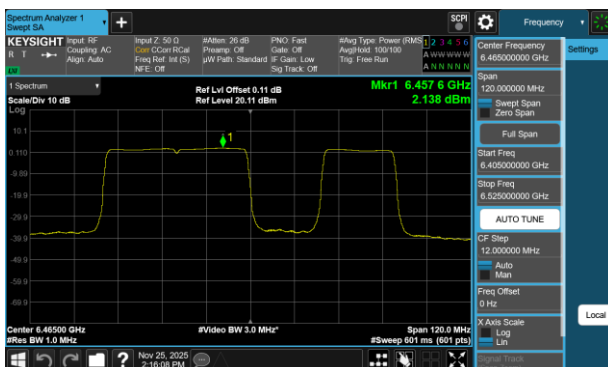
Plot 7-248 PSD Antenna 3c (80MHz BW 802.11be(RU) RU484+242 Index92 - Ch.103)
