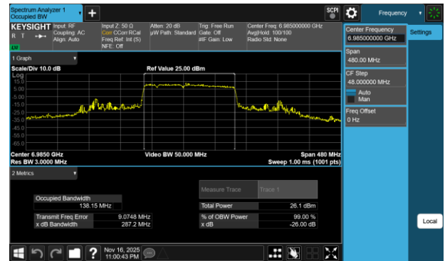
Plot 7-227 26dB BW & 99% OBW Antenna 1b (160MHz BW 802.11be(RU) RU996+484+242 Index96 - Ch.207)
