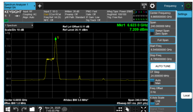
Plot 7-257 PSD Antenna 3c (160MHz BW 802.11be(RU) RU26 Index17 - Ch.143)
