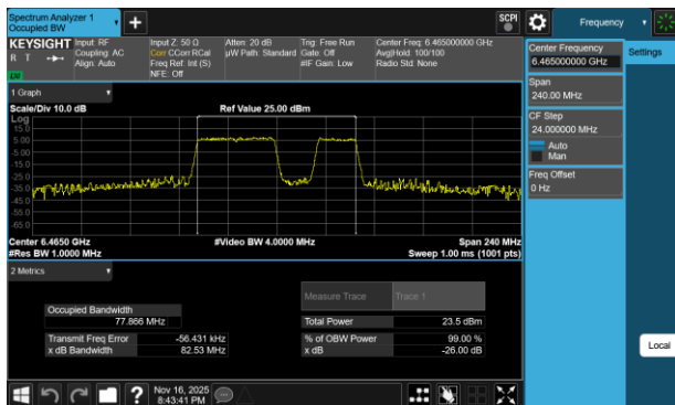
Plot 7-204 26dB BW & 99% OBW Antenna 1b (80MHz BW 802.11be(RU) RU484+242 Index92 - Ch.103)
