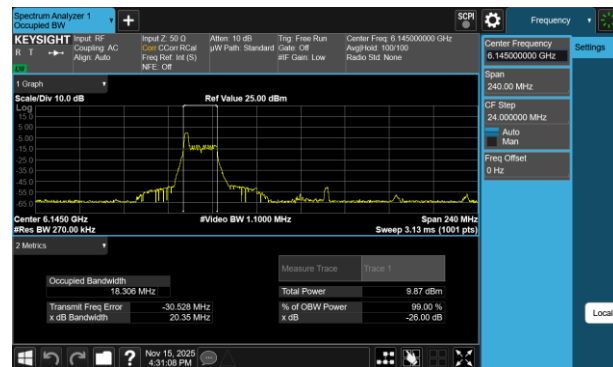
Plot 7-190 26dB BW & 99% OBW Antenna 1b (80MHz BW 802.11be(RU) RU26 Index0 - Ch.39)
