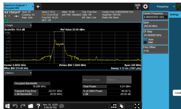
Plot 7-212 26dB BW & 99% OBW Antenna 1b (80MHz BW 802.11be(RU) RU26 Index0 - Ch.183)
