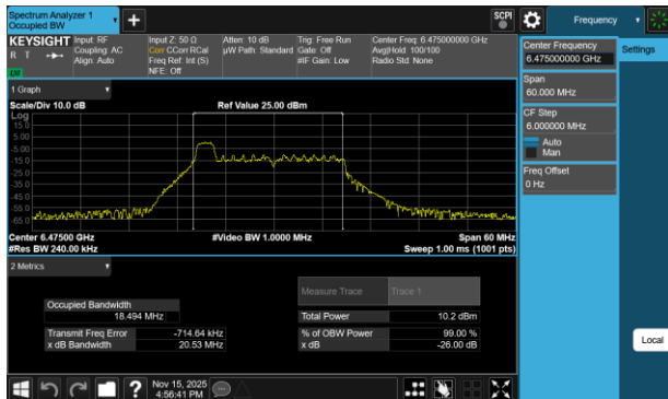
Plot 7-199 26dB BW & 99% OBW Antenna 1b (20MHz BW 802.11be(RU) RU26 Index0 - Ch.105)
