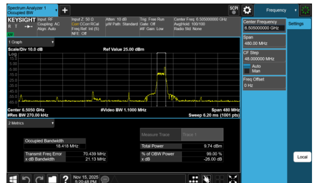
Plot 7-202 26dB BW & 99% OBW Antenna 1b (160MHz BW 802.11be(RU) RU26 Index36 - Ch.111)
