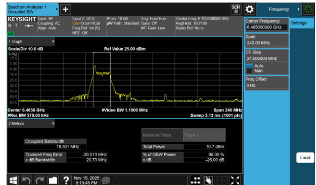
Plot 7-201 26dB BW & 99% OBW Antenna 1b (80MHz BW 802.11be(RU) RU26 Index0 - Ch.103)
