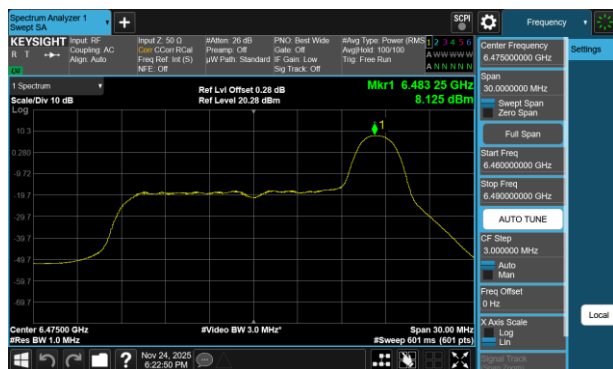
Plot 7-243 PSD Antenna 3c (20MHz BW 802.11be(RU) RU26 Index8 - Ch.105)
