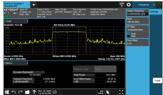
Plot 7-205 26dB BW & 99% OBW Antenna 1b (160MHz BW 802.11be(RU) RU996+484+242 Index96 - Ch.111)
