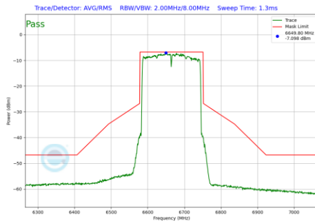
Plot 7-480 In-Band Emission Plot Antenna 3c (160MHz BW 802.11be(RU) RU996X2 Index68 (UNII Band 7) - Ch.143)
