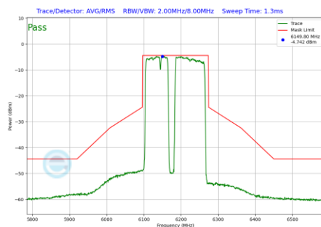
Plot 7-503 In-Band Emission Plot Antenna 3a (160MHz BW 802.11be(RU) RU996+484+242 Index99 (UNII Band 5) - Ch.47)
