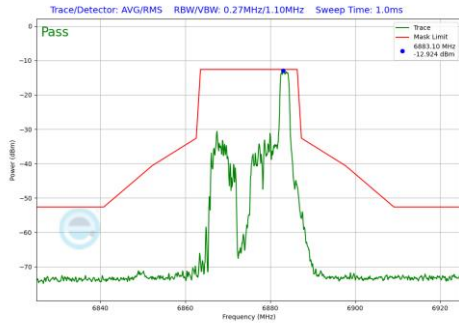
Plot 7-537 In-Band Emission Plot Antenna 1b (20MHz BW 802.11be(RU) RU26 Index8 (UNII Band 7) - Ch.185)
