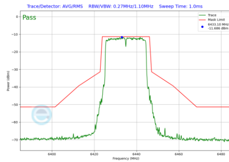
Plot 7-517 In-Band Emission Plot Antenna 3a (20MHz BW 802.11be(RU) RU242 Index61 (UNII Band 6) - Ch.97)
