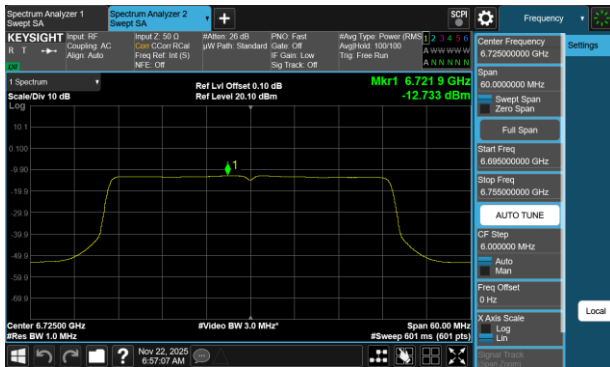
Plot 7-412 PSD SDM Diversity Antenna 3c (40MHz BW 802.11be(RU) RU484 Index65 - Ch.155)
