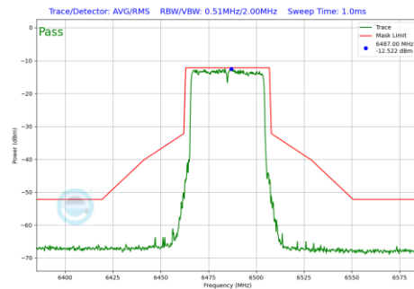
Plot 7-474 In-Band Emission Plot Antenna 3c (40MHz BW 802.11be(RU) RU484 Index65 (UNII Band 6) - Ch.107)
