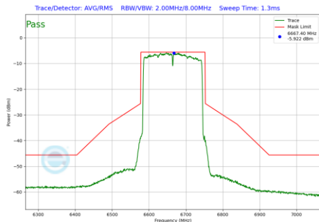
Plot 7-524 In-Band Emission Plot Antenna 3a (160MHz BW 802.11be(RU) RU996X2 Index68 (UNII Band 7) - Ch.143)
