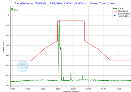
Plot 7-488 In-Band Emission Plot Antenna 3a (160MHz BW 802.11be(RU) RU26 Index0 (UNII Band 5) - Ch.47)
