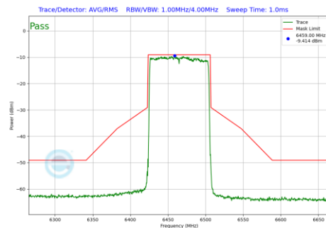
Plot 7-475 In-Band Emission Plot Antenna 3c (80MHz BW 802.11be(RU) RU996 Index67 (UNII Band 6) - Ch.103)
