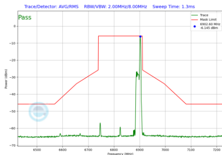
Plot 7-496 In-Band Emission Plot Antenna 3a (160MHz BW 802.11be(RU) RU26 Index36 (UNII Band 7) - Ch.175)
