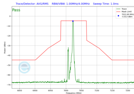
Plot 7-499 In-Band Emission Plot Antenna 3a (80MHz BW 802.11be(RU) RU26 Index17 (UNII Band 8) - Ch.215)
