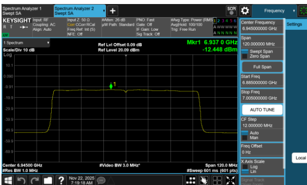
Plot 7-435 PSD SDM Diversity Antenna 3c (80MHz BW 802.11be(RU) RU996 Index67 - Ch.199)
