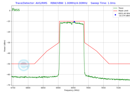
Plot 7-483 In-Band Emission Plot Antenna 3c (80MHz BW 802.11be(RU) RU996 Index67 (UNII Band 8) - Ch.199)
