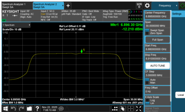
Plot 7-433 PSD SDM Diversity Antenna 3c (20MHz BW 802.11be(RU) RU242 Index61 - Ch.189)
