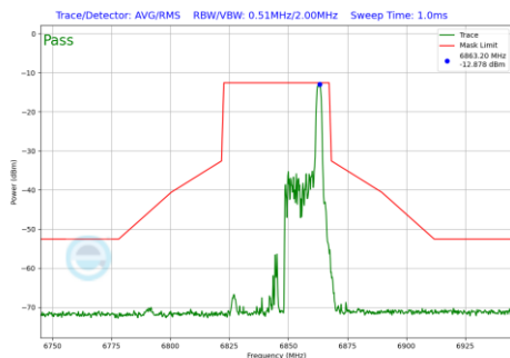
Plot 7-450 In-Band Emission Plot Antenna 3c (40MHz BW 802.11be(RU) RU26 Index17 (UNII Band 7) - Ch.179)
