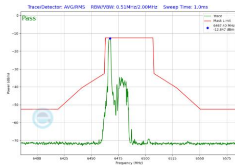
Plot 7-446 In-Band Emission Plot Antenna 3c (40MHz BW 802.11be(RU) RU26 Index0 (UNII Band 6) - Ch.107)
