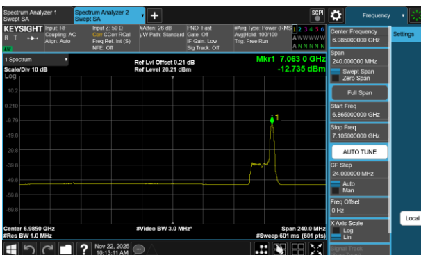
Plot 7-422 PSD SDM Diversity Antenna 3c (160MHz BW 802.11be(RU) RU26 Index36 - Ch.207)
