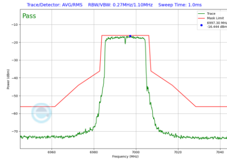
Plot 7-481 In-Band Emission Plot Antenna 3c (20MHz BW 802.11be(RU) RU242 Index61 (UNII Band 8) - Ch.209)
