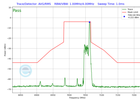
Plot 7-543 In-Band Emission Plot Antenna 1b (80MHz BW 802.11be(RU) RU26 Index36 (UNII Band 8) - Ch.215)
