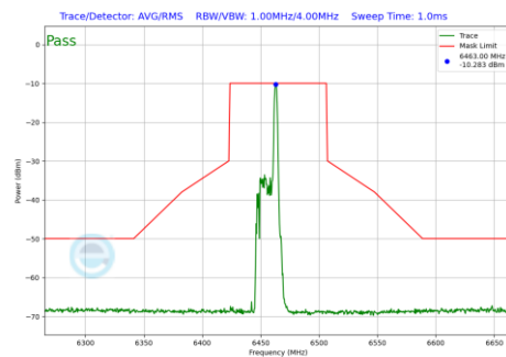
Plot 7-447 In-Band Emission Plot Antenna 3c (80MHz BW 802.11be(RU) RU26 Index17 (UNII Band 6) - Ch.103)
