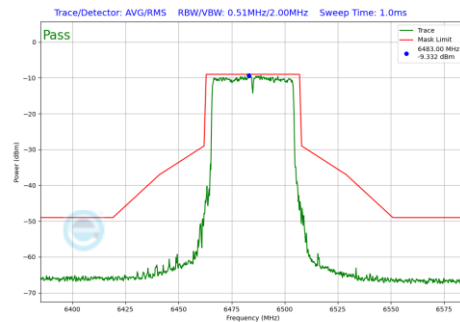
Plot 7-518 In-Band Emission Plot Antenna 3a (40MHz BW 802.11be(RU) RU484 Index65 (UNII Band 6) - Ch.107)
