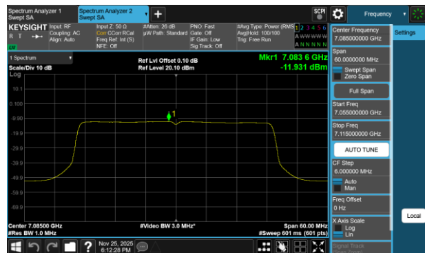
Plot 7-438 PSD SDM Diversity Antenna 1b (40MHz BW 802.11be(RU) RU484 Index65 - Ch.227)
