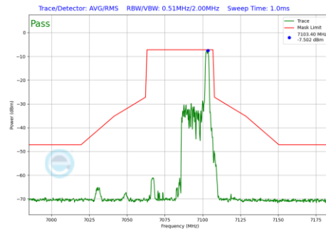
Plot 7-542 In-Band Emission Plot Antenna 1b (40MHz BW 802.11be(RU) RU26 Index17 (UNII Band 8) - Ch.227)
