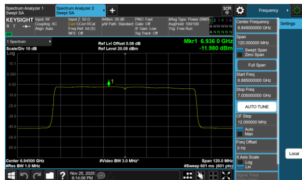
Plot 7-439 PSD SDM Diversity Antenna 1b (80MHz BW 802.11be(RU) RU996 Index67 - Ch.199)
