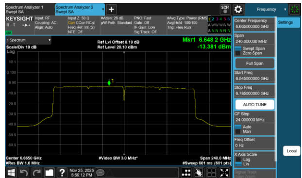
Plot 7-418 PSD SDM Diversity Antenna 1b (160MHz BW 802.11be(RU) RU996X2 Index68 - Ch.143)
