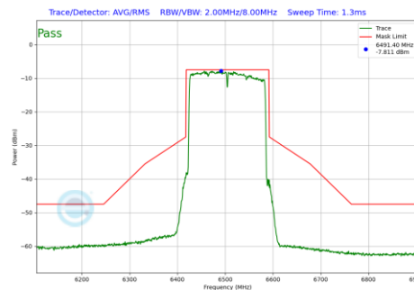
Plot 7-476 In-Band Emission Plot Antenna 3c (160MHz BW 802.11be(RU) RU996X2 Index68 (UNII Band 6) - Ch.111)
