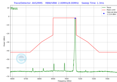
Plot 7-544 In-Band Emission Plot Antenna 1b (160MHz BW 802.11be(RU) RU26 Index36 (UNII Band 8) - Ch.207)
