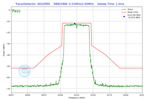
Plot 7-470 In-Band Emission Plot Antenna 3c (40MHz BW 802.11be(RU) RU484 Index65 (UNII Band 5) - Ch.35)
