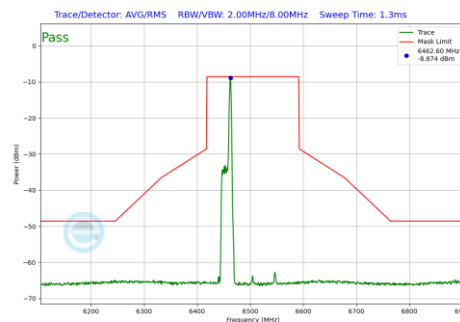
Plot 7-448 In-Band Emission Plot Antenna 3c (160MHz BW 802.11be(RU) RU26 Index17 (UNII Band 6) - Ch.111)
