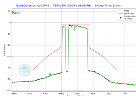
Plot 7-512 In-Band Emission Plot Antenna 3a (160MHz BW 802.11be(RU) RU996+484+242 Index97 (UNII Band 8) - Ch.207)
