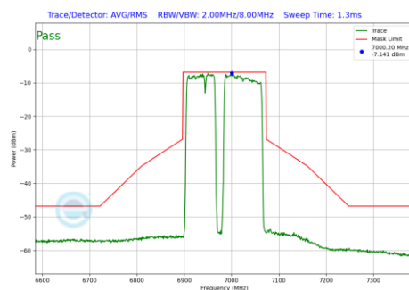
Plot 7-468 In-Band Emission Plot Antenna 3c (160MHz BW 802.11be(RU) RU996+484+242 Index99 (UNII Band 8) - Ch.207)
