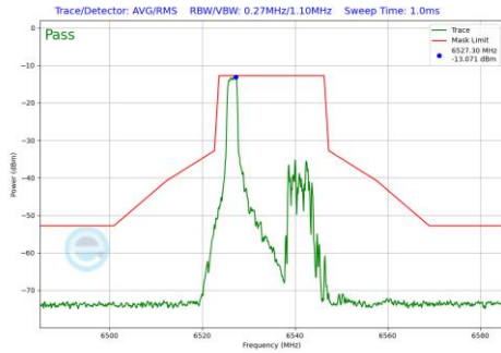
Plot 7-493 In-Band Emission Plot Antenna 3a (20MHz BW 802.11be(RU) RU26 Index0 (UNII Band 7) - Ch.117)
