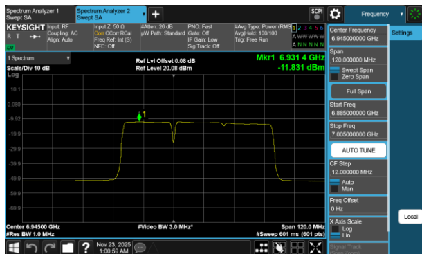
Plot 7-428 PSD SDM Diversity Antenna 3c (80MHz BW 802.11be(RU) RU484+242 Index90 - Ch.199)
