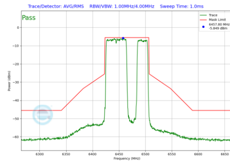
Plot 7-549 In-Band Emission Plot Antenna 1b (80MHz BW 802.11be(RU) RU484+242 Index92 (UNII Band 6) - Ch.103)
