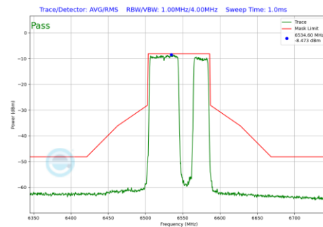
Plot 7-464 In-Band Emission Plot Antenna 3c (80MHz BW 802.11be(RU) RU484+242 Index92 (UNII Band 7) - Ch.119)
