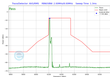
Plot 7-444 In-Band Emission Plot Antenna 3c (160MHz BW 802.11be(RU) RU26 Index0 (UNII Band 5) - Ch.47)
