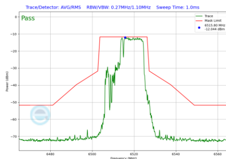
Plot 7-504 In-Band Emission Plot Antenna 3a (20MHz BW 802.11be(RU) RU106+26 Index83 (UNII Band 6) - Ch.113)
