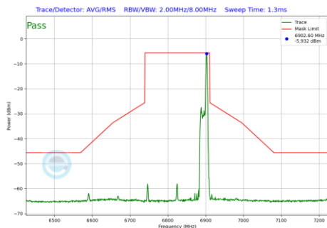
Plot 7-540 In-Band Emission Plot Antenna 1b (160MHz BW 802.11be(RU) RU26 Index36 (UNII Band 7) - Ch.175)
