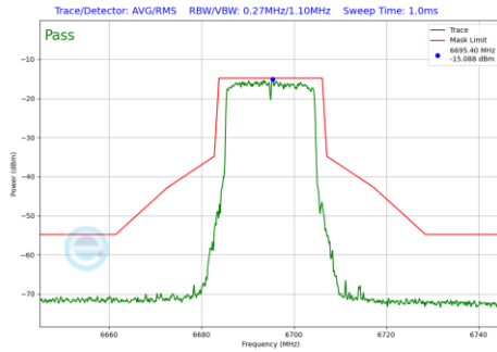
Plot 7-477 In-Band Emission Plot Antenna 3c (20MHz BW 802.11be(RU) RU242 Index61 (UNII Band 7) - Ch.149)
