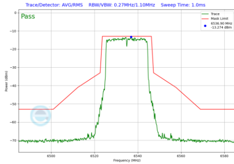
Plot 7-521 In-Band Emission Plot Antenna 3a (20MHz BW 802.11be(RU) RU242 Index61 (UNII Band 7) - Ch.117)
