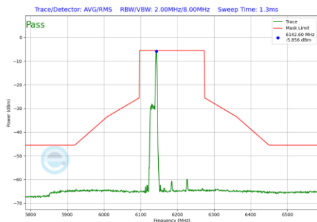
Plot 7-532 In-Band Emission Plot Antenna 1b (160MHz BW 802.11be(RU) RU26 Index17 (UNII Band 5) - Ch.47)
