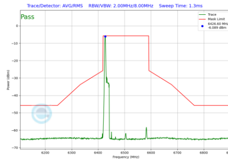
Plot 7-492 In-Band Emission Plot Antenna 3a (160MHz BW 802.11be(RU) RU26 Index0 (UNII Band 6) - Ch.111)
