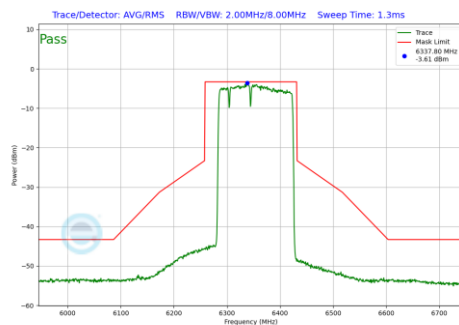
Plot 7-547 In-Band Emission Plot Antenna 1b (160MHz BW 802.11be(RU) RU996+484+242 Index96 (UNII Band 5) - Ch.79)
