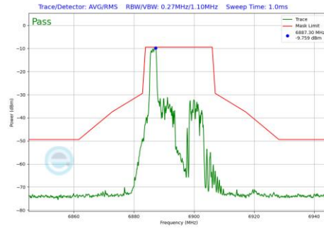
Plot 7-541 In-Band Emission Plot Antenna 1b (20MHz BW 802.11be(RU) RU26 Index0 (UNII Band 8) - Ch.189)
