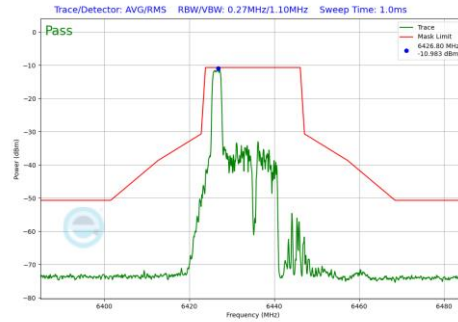
Plot 7-489 In-Band Emission Plot Antenna 3a (20MHz BW 802.11be(RU) RU26 Index0 (UNII Band 6) - Ch.97)
