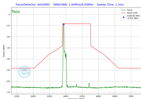
Plot 7-452 In-Band Emission Plot Antenna 3c (160MHz BW 802.11be(RU) RU26 Index0 (UNII Band 7) - Ch.143)
