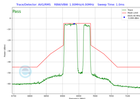
Plot 7-511 In-Band Emission Plot Antenna 3a (80MHz BW 802.11be(RU) RU484+242 Index92 (UNII Band 8) - Ch.199)
