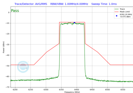
Plot 7-471 In-Band Emission Plot Antenna 3c (80MHz BW 802.11be(RU) RU996 Index67 (UNII Band 5) - Ch.87)
