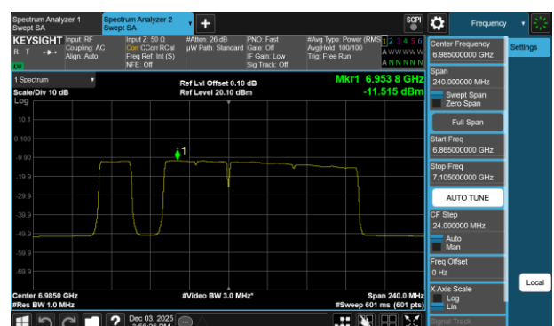
Plot 7-432 PSD SDM Diversity Antenna 1b (160MHz BW 802.11be(RU) RU996+484+242 Index97 - Ch.207)
