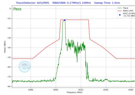
Plot 7-533 In-Band Emission Plot Antenna 1b (20MHz BW 802.11be(RU) RU26 Index0 (UNII Band 6) - Ch.113)
