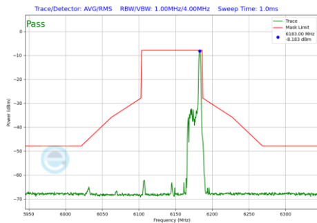
Plot 7-487 In-Band Emission Plot Antenna 3a (80MHz BW 802.11be(RU) RU26 Index36 (UNII Band 5) - Ch.39)
