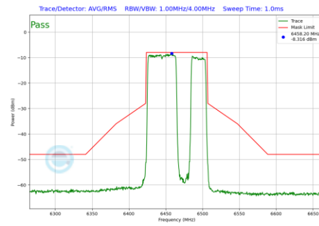
Plot 7-461 In-Band Emission Plot Antenna 3c (80MHz BW 802.11be(RU) RU484+242 Index92 (UNII Band 6) - Ch.103)
