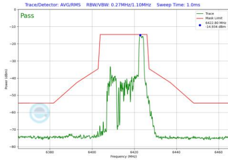
Plot 7-441 In-Band Emission Plot Antenna 3c (20MHz BW 802.11be(RU) RU26 Index8 (UNII Band 5) - Ch.93)
