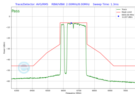
Plot 7-465 In-Band Emission Plot Antenna 3c (160MHz BW 802.11be(RU) RU996+484+242 Index97 (UNII Band 7) - Ch.143)
