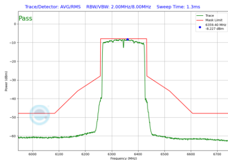
Plot 7-472 In-Band Emission Plot Antenna 3c (160MHz BW 802.11be(RU) RU996X2 Index68 (UNII Band 5) - Ch.79)
