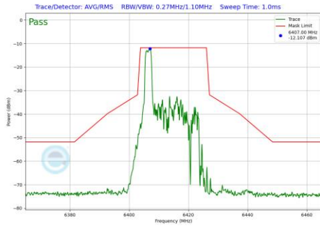
Plot 7-529 In-Band Emission Plot Antenna 1b (20MHz BW 802.11be(RU) RU26 Index0 (UNII Band 5) - Ch.93)
