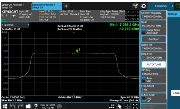
Plot 7-434 PSD SDM Diversity Antenna 3c (40MHz BW 802.11be(RU) RU484 Index65 - Ch.227)
