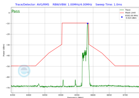
Plot 7-451 In-Band Emission Plot Antenna 3c (80MHz BW 802.11be(RU) RU26 Index36 (UNII Band 7) - Ch.119)
