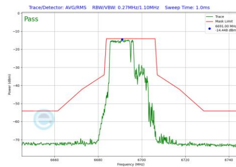
Plot 7-463 In-Band Emission Plot Antenna 3c (20MHz BW 802.11be(RU) RU106+26 Index82 (UNII Band 7) - Ch.149)
