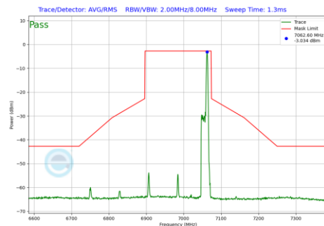
Plot 7-500 In-Band Emission Plot Antenna 3a (160MHz BW 802.11be(RU) RU26 Index36 (UNII Band 8) - Ch.207)
