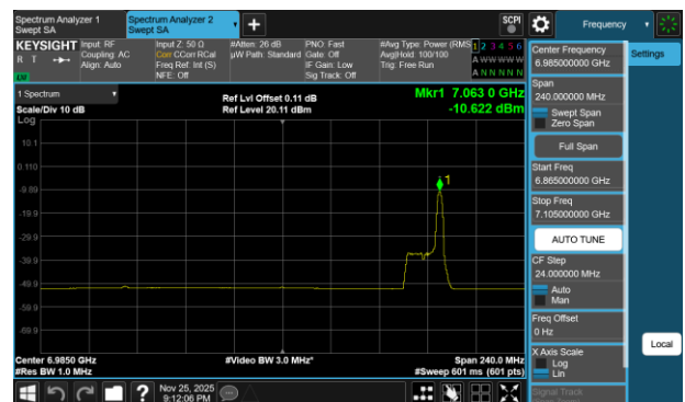
Plot 7-426 PSD SDM Diversity Antenna 1b (160MHz BW 802.11be(RU) RU26 Index36 - Ch.207)
