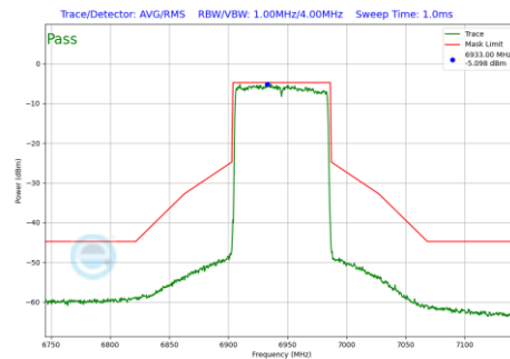
Plot 7-527 In-Band Emission Plot Antenna 3a (80MHz BW 802.11be(RU) RU996 Index67 (UNII Band 8) - Ch.199)
