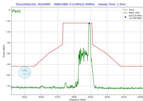
Plot 7-442 In-Band Emission Plot Antenna 3c (40MHz BW 802.11be(RU) RU26 Index17 (UNII Band 5) - Ch.91)
