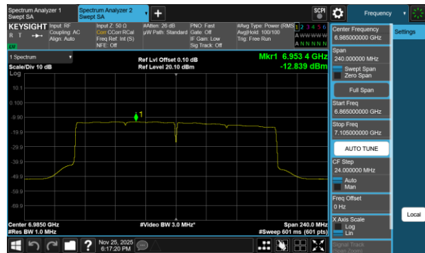
Plot 7-440 PSD SDM Diversity Antenna 1b (160MHz BW 802.11be(RU) RU996X2 Index68 - Ch.207)
