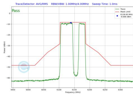
Plot 7-458 In-Band Emission Plot Antenna 3c (80MHz BW 802.11be(RU) RU484+242 Index92 (UNII Band 5) - Ch.39)
