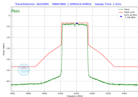
Plot 7-515 In-Band Emission Plot Antenna 3a (80MHz BW 802.11be(RU) RU996 Index67 (UNII Band 5) - Ch.39)
