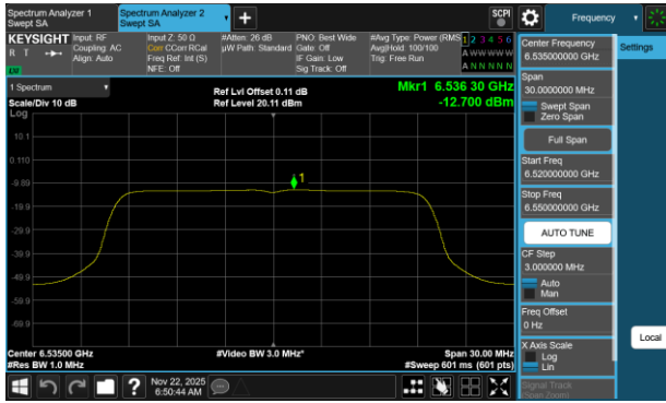
Plot 7-411 PSD SDM Diversity Antenna 3c (20MHz BW 802.11be(RU) RU242 Index61 - Ch.117)
