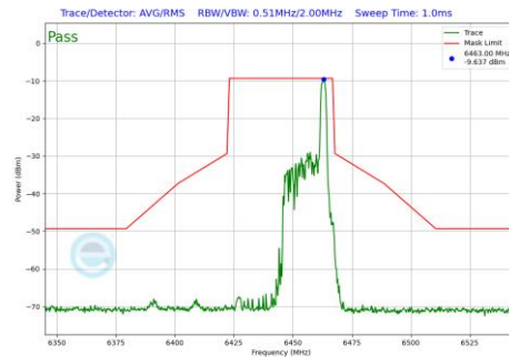
Plot 7-534 In-Band Emission Plot Antenna 1b (40MHz BW 802.11be(RU) RU26 Index17 (UNII Band 6) - Ch.99)
