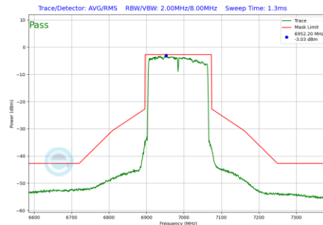
Plot 7-528 In-Band Emission Plot Antenna 3a (160MHz BW 802.11be(RU) RU996X2 Index68 (UNII Band 8) - Ch.207)
