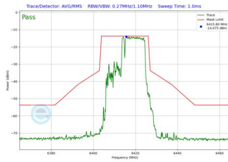
Plot 7-457 In-Band Emission Plot Antenna 3c (20MHz BW 802.11be(RU) RU106+26 Index83 (UNII Band 5) - Ch.93)
