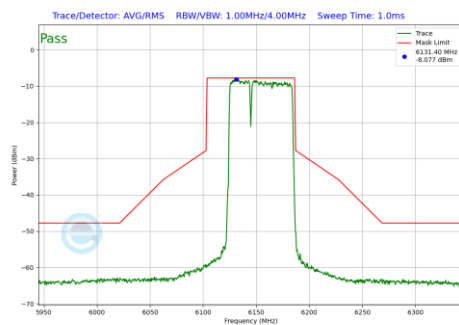
Plot 7-502 In-Band Emission Plot Antenna 3a (80MHz BW 802.11be(RU) RU484+242 Index90 (UNII Band 5) - Ch.39)
