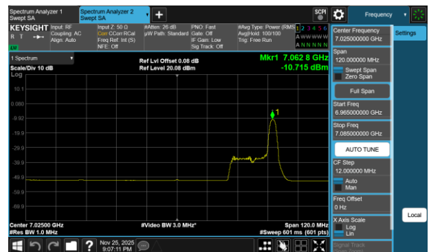
Plot 7-425 PSD SDM Diversity Antenna 1b (80MHz BW 802.11be(RU) RU26 Index36 - Ch.215)
