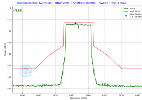
Plot 7-482 In-Band Emission Plot Antenna 3c (40MHz BW 802.11be(RU) RU484 Index65 (UNII Band 8) - Ch.187)
