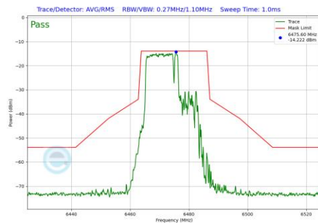
Plot 7-460 In-Band Emission Plot Antenna 3c (20MHz BW 802.11be(RU) RU106+26 Index82 (UNII Band 6) - Ch.105)
