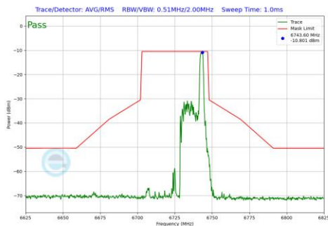
Plot 7-494 In-Band Emission Plot Antenna 3a (40MHz BW 802.11be(RU) RU26 Index17 (UNII Band 7) - Ch.155)
