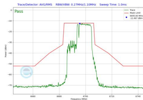
Plot 7-551 In-Band Emission Plot Antenna 1b (20MHz BW 802.11be(RU) RU106+26 Index83 (UNII Band 7) - Ch.149)
