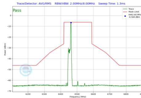
Plot 7-536 In-Band Emission Plot Antenna 1b (160MHz BW 802.11be(RU) RU26 Index17 (UNII Band 6) - Ch.111)
