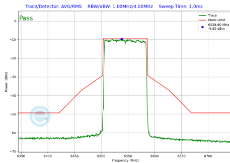
Plot 7-479 In-Band Emission Plot Antenna 3c (80MHz BW 802.11be(RU) RU996 Index67 (UNII Band 7) - Ch.119)
