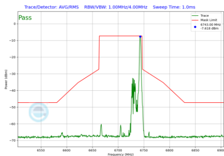
Plot 7-495 In-Band Emission Plot Antenna 3a (80MHz BW 802.11be(RU) RU26 Index36 (UNII Band 7) - Ch.151)
