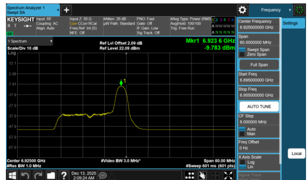
Plot 7-424 PSD SDM Diversity Antenna 1b (40MHz BW 802.11be(RU) RU26 Index8 - Ch.195)
