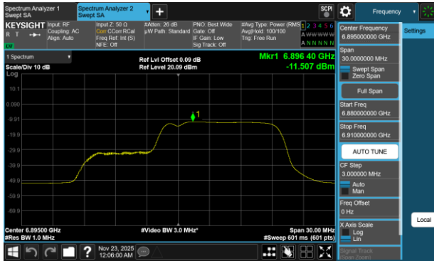
Plot 7-427 PSD SDM Diversity Antenna 3c (20MHz BW 802.11be(RU) RU106+26 Index83 - Ch.189)
