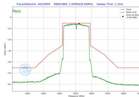
Plot 7-520 In-Band Emission Plot Antenna 3a (160MHz BW 802.11be(RU) RU996X2 Index68 (UNII Band 6) - Ch.111)
