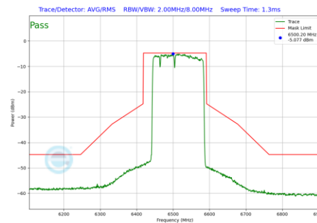
Plot 7-506 In-Band Emission Plot Antenna 3a (160MHz BW 802.11be(RU) RU996+484+242 Index96 (UNII Band 6) - Ch.111)
