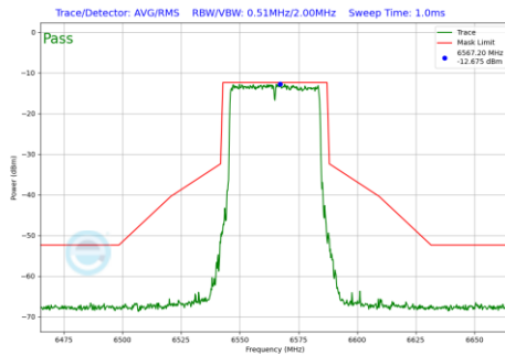
Plot 7-478 In-Band Emission Plot Antenna 3c (40MHz BW 802.11be(RU) RU484 Index65 (UNII Band 7) - Ch.123)
