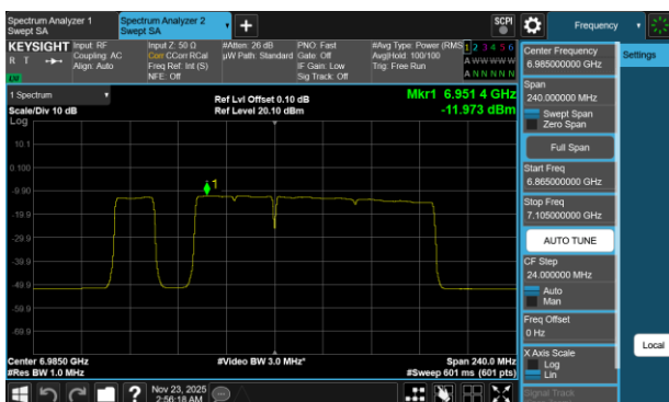
Plot 7-429 PSD SDM Diversity Antenna 3c (160MHz BW 802.11be(RU) RU996+484+242 Index97 - Ch.207)
