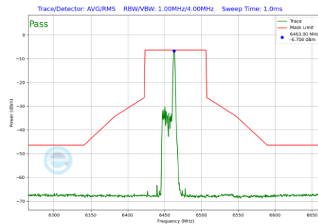
Plot 7-535 In-Band Emission Plot Antenna 1b (80MHz BW 802.11be(RU) RU26 Index17 (UNII Band 6) - Ch.103)
