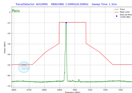
Plot 7-456 In-Band Emission Plot Antenna 3c (160MHz BW 802.11be(RU) RU26 Index17 (UNII Band 8) - Ch.207)
