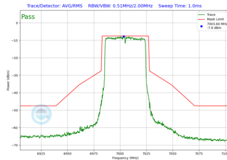
Plot 7-526 In-Band Emission Plot Antenna 3a (40MHz BW 802.11be(RU) RU484 Index65 (UNII Band 8) - Ch.211)
