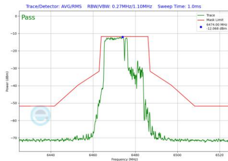
Plot 7-548 In-Band Emission Plot Antenna 1b (20MHz BW 802.11be(RU) RU106+26 Index82 (UNII Band 6) - Ch.105)
