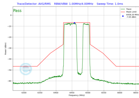
Plot 7-505 In-Band Emission Plot Antenna 3a (80MHz BW 802.11be(RU) RU484+242 Index92 (UNII Band 6) - Ch.103)
