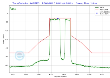
Plot 7-546 In-Band Emission Plot Antenna 1b (80MHz BW 802.11be(RU) RU484+242 Index92 (UNII Band 5) - Ch.87)
