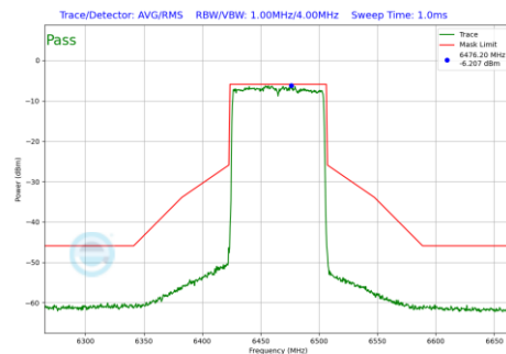
Plot 7-519 In-Band Emission Plot Antenna 3a (80MHz BW 802.11be(RU) RU996 Index67 (UNII Band 6) - Ch.103)
