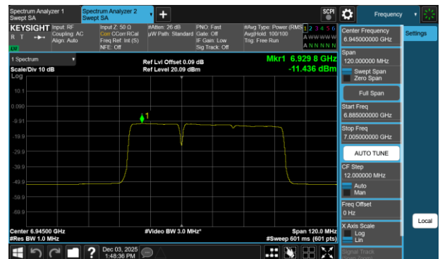
Plot 7-431 PSD SDM Diversity Antenna 1b (80MHz BW 802.11be(RU) RU484+242 Index90 - Ch.199)
