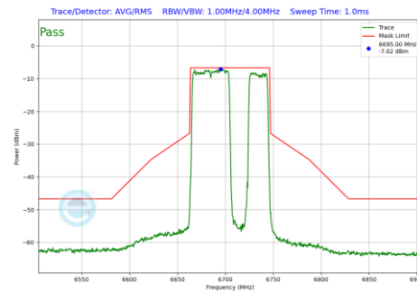
Plot 7-552 In-Band Emission Plot Antenna 1b (80MHz BW 802.11be(RU) RU484+242 Index92 (UNII Band 7) - Ch.151)
