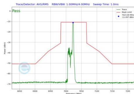
Plot 7-455 In-Band Emission Plot Antenna 3c (80MHz BW 802.11be(RU) RU26 Index17 (UNII Band 8) - Ch.215)
