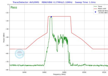
Plot 7-445 In-Band Emission Plot Antenna 3c (20MHz BW 802.11be(RU) RU26 Index0 (UNII Band 6) - Ch.105)
