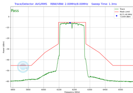
Plot 7-516 In-Band Emission Plot Antenna 3a (160MHz BW 802.11be(RU) RU996X2 Index68 (UNII Band 5) - Ch.47)
