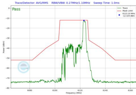
Plot 7-485 In-Band Emission Plot Antenna 3a (20MHz BW 802.11be(RU) RU26 Index8 (UNII Band 5) - Ch.33)
