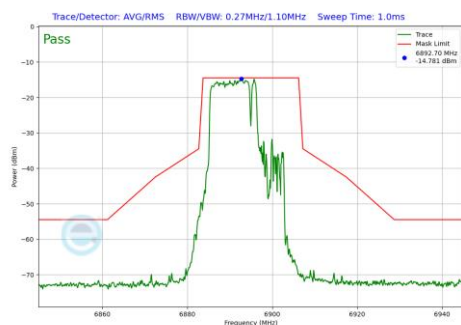
Plot 7-466 In-Band Emission Plot Antenna 3c (20MHz BW 802.11be(RU) RU106+26 Index82 (UNII Band 8) - Ch.189)
