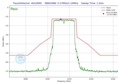
Plot 7-513 In-Band Emission Plot Antenna 3a (20MHz BW 802.11be(RU) RU242 Index61 (UNII Band 5) - Ch.33)
