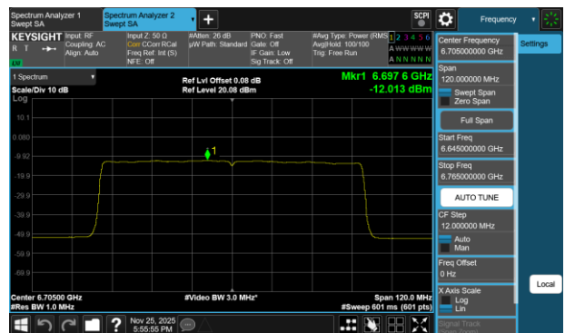
Plot 7-417 PSD SDM Diversity Antenna 1b (80MHz BW 802.11be(RU) RU996 Index67 - Ch.151)
