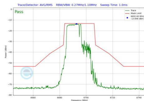
Plot 7-507 In-Band Emission Plot Antenna 3a (20MHz BW 802.11be(RU) RU106+26 Index82 (UNII Band 7) - Ch.149)
