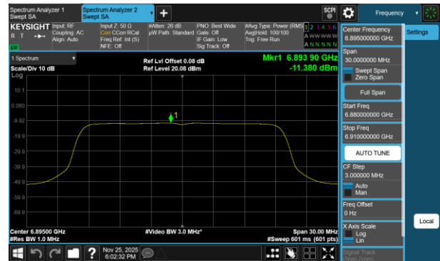
Plot 7-437 PSD SDM Diversity Antenna 1b (20MHz BW 802.11be(RU) RU242 Index61 - Ch.189)
