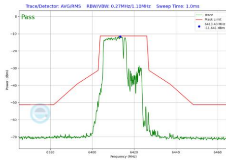
Plot 7-545 In-Band Emission Plot Antenna 1b (20MHz BW 802.11be(RU) RU106+26 Index82 (UNII Band 5) - Ch.93)
