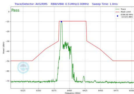
Plot 7-530 In-Band Emission Plot Antenna 1b (40MHz BW 802.11be(RU) RU26 Index0 (UNII Band 5) - Ch.91)
