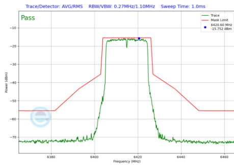
Plot 7-469 In-Band Emission Plot Antenna 3c (20MHz BW 802.11be(RU) RU242 Index61 (UNII Band 5) - Ch.93)
