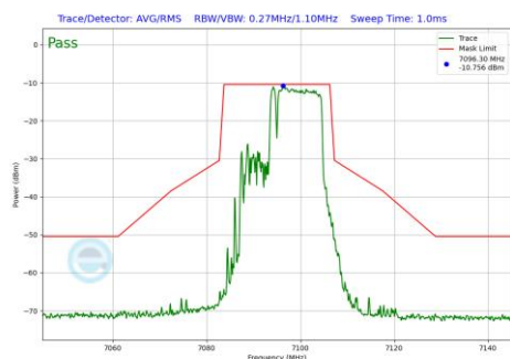
Plot 7-510 In-Band Emission Plot Antenna 3a (20MHz BW 802.11be(RU) RU106+26 Index83 (UNII Band 8) - Ch.229)
