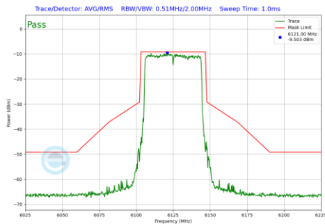
Plot 7-514 In-Band Emission Plot Antenna 3a (40MHz BW 802.11be(RU) RU484 Index65 (UNII Band 5) - Ch.35)
