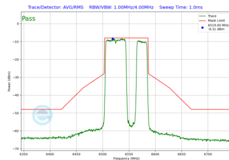
Plot 7-508 In-Band Emission Plot Antenna 3a (80MHz BW 802.11be(RU) RU484+242 Index92 (UNII Band 7) - Ch.119)
