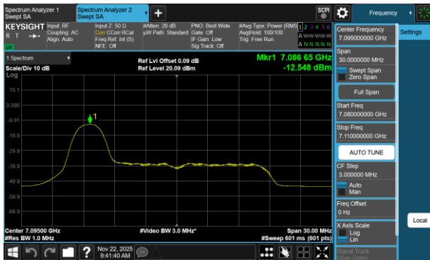
Plot 7-419 PSD SDM Diversity Antenna 3c (20MHz BW 802.11be(RU) RU26 Index0 - Ch.229)
