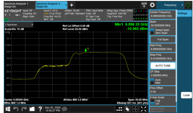
Plot 7-430 PSD SDM Diversity Antenna 1b (20MHz BW 802.11be(RU) RU106+26 Index83 - Ch.189)
