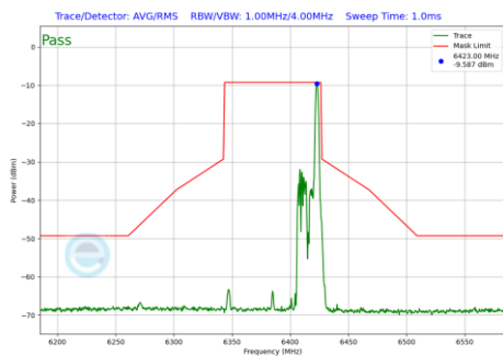
Plot 7-443 In-Band Emission Plot Antenna 3c (80MHz BW 802.11be(RU) RU26 Index36 (UNII Band 5) - Ch.87)
