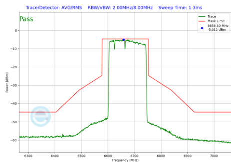
Plot 7-509 In-Band Emission Plot Antenna 3a (160MHz BW 802.11be(RU) RU996+484+242 Index96 (UNII Band 7) - Ch.143)
