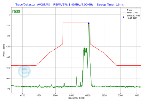
Plot 7-539 In-Band Emission Plot Antenna 1b (80MHz BW 802.11be(RU) RU26 Index36 (UNII Band 7) - Ch.183)
