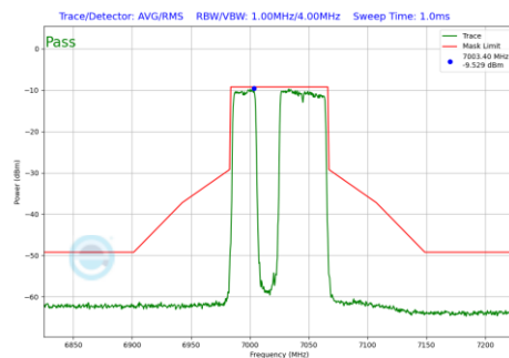
Plot 7-467 In-Band Emission Plot Antenna 3c (80MHz BW 802.11be(RU) RU484+242 Index91 (UNII Band 8) - Ch.215)
