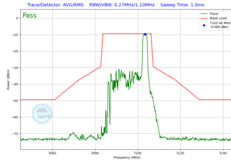
Plot 7-497 In-Band Emission Plot Antenna 3a (20MHz BW 802.11be(RU) RU26 Index8 (UNII Band 8) - Ch.229)
