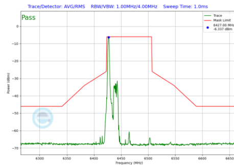
Plot 7-491 In-Band Emission Plot Antenna 3a (80MHz BW 802.11be(RU) RU26 Index0 (UNII Band 6) - Ch.103)
