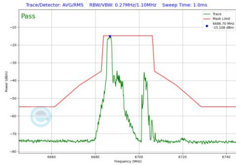
Plot 7-449 In-Band Emission Plot Antenna 3c (20MHz BW 802.11be(RU) RU26 Index0 (UNII Band 7) - Ch.149)
