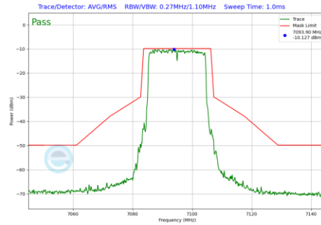
Plot 7-525 In-Band Emission Plot Antenna 3a (20MHz BW 802.11be(RU) RU242 Index61 (UNII Band 8) - Ch.229)
