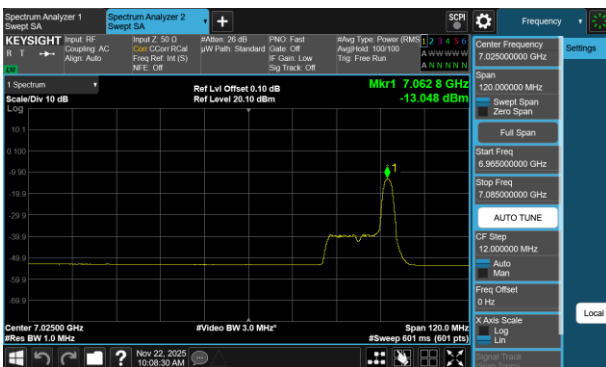
Plot 7-421 PSD SDM Diversity Antenna 3c (80MHz BW 802.11be(RU) RU26 Index36 - Ch.215)
