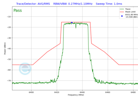
Plot 7-473 In-Band Emission Plot Antenna 3c (20MHz BW 802.11be(RU) RU242 Index61 (UNII Band 6) - Ch.97)
