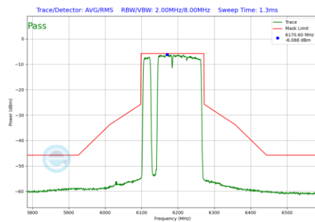
Plot 7-459 In-Band Emission Plot Antenna 3c (160MHz BW 802.11be(RU) RU996+484+242 Index97 (UNII Band 5) - Ch.47)
