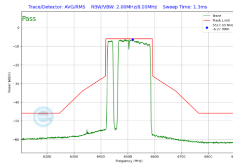
Plot 7-462 In-Band Emission Plot Antenna 3c (160MHz BW 802.11be(RU) RU996+484+242 Index97 (UNII Band 6) - Ch.111)
