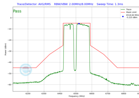
Plot 7-550 In-Band Emission Plot Antenna 1b (160MHz BW 802.11be(RU) RU996+484+242 Index99 (UNII Band 6) - Ch.111)
