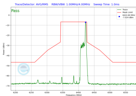
Plot 7-531 In-Band Emission Plot Antenna 1b (80MHz BW 802.11be(RU) RU26 Index36 (UNII Band 5) - Ch.87)
