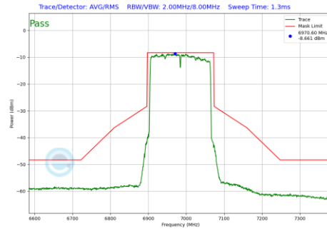
Plot 7-484 In-Band Emission Plot Antenna 3c (160MHz BW 802.11be(RU) RU996X2 Index68 (UNII Band 8) - Ch.207)
