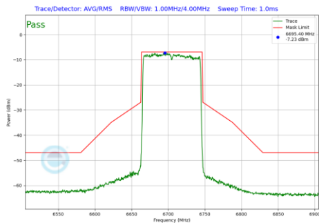
Plot 7-523 In-Band Emission Plot Antenna 3a (80MHz BW 802.11be(RU) RU996 Index67 (UNII Band 7) - Ch.151)
