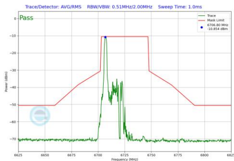
Plot 7-538 In-Band Emission Plot Antenna 1b (40MHz BW 802.11be(RU) RU26 Index0 (UNII Band 7) - Ch.155)
