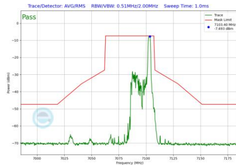
Plot 7-498 In-Band Emission Plot Antenna 3a (40MHz BW 802.11be(RU) RU26 Index17 (UNII Band 8) - Ch.227)
