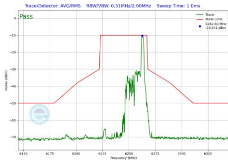
Plot 7-486 In-Band Emission Plot Antenna 3a (40MHz BW 802.11be(RU) RU26 Index17 (UNII Band 5) - Ch.59)
