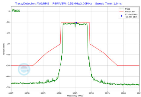
Plot 7-522 In-Band Emission Plot Antenna 3a (40MHz BW 802.11be(RU) RU484 Index65 (UNII Band 7) - Ch.155)
