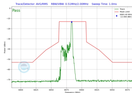
Plot 7-454 In-Band Emission Plot Antenna 3c (40MHz BW 802.11be(RU) RU26 Index8 (UNII Band 8) - Ch.187)
