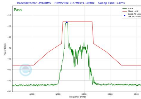
Plot 7-453 In-Band Emission Plot Antenna 3c (20MHz BW 802.11be(RU) RU26 Index0 (UNII Band 8) - Ch.189)
