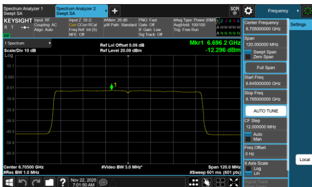
Plot 7-413 PSD SDM Diversity Antenna 3c (80MHz BW 802.11be(RU) RU996 Index67 - Ch.151)
