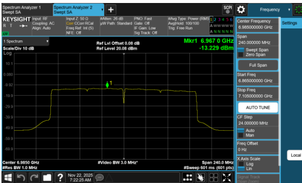
Plot 7-436 PSD SDM Diversity Antenna 3c (160MHz BW 802.11be(RU) RU996X2 Index68 - Ch.207)
