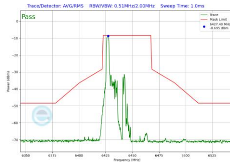
Plot 7-490 In-Band Emission Plot Antenna 3a (40MHz BW 802.11be(RU) RU26 Index0 (UNII Band 6) - Ch.99)
