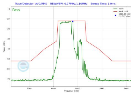
Plot 7-501 In-Band Emission Plot Antenna 3a (20MHz BW 802.11be(RU) RU106+26 Index82 (UNII Band 5) - Ch.93)
