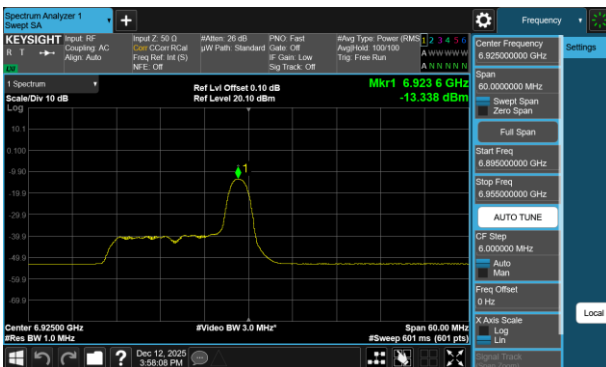
Plot 7-420 PSD SDM Diversity Antenna 3c (40MHz BW 802.11be(RU) RU26 Index8 - Ch.195)
