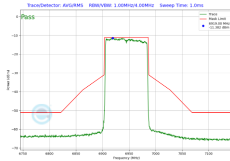
Plot 7-731 In-Band Emission Plot SDM Diversity Antenna 1b (80MHz BW 802.11be(RU) RU996 Index67 (UNII Band 8) - Ch.199)
