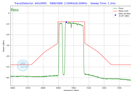
Plot 7-616 In-Band Emission Plot SDM Primary Antenna 3c (160MHz BW 802.11be(RU) RU996+484+242 Index97 (UNII Band 8) - Ch.207)
