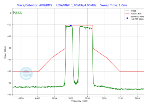
Plot 7-627 In-Band Emission Plot SDM Primary Antenna 3a (80MHz BW 802.11be(RU) RU484+242 Index91 (UNII Band 8) - Ch.215)
