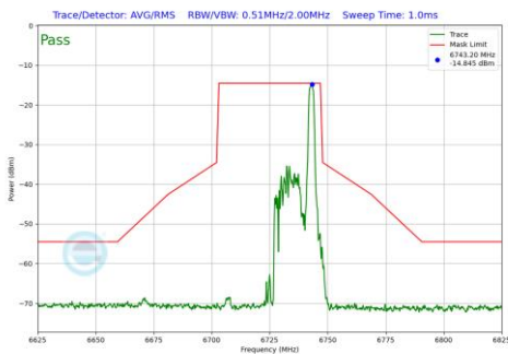
Plot 7-582 In-Band Emission Plot SDM Primary Antenna 3c (40MHz BW 802.11be(RU) RU26 Index17 (UNII Band 7) - Ch.155)
