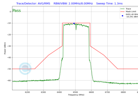
Plot 7-740 In-Band Emission Plot SDM Diversity Antenna 3c (160MHz BW 802.11be(RU) RU996X2 Index68 (UNII Band 6) - Ch.111)
