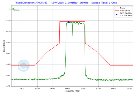
Plot 7-621 In-Band Emission Plot SDM Primary Antenna 3a (80MHz BW 802.11be(RU) RU484+242 Index90 (UNII Band 6) - Ch.103)
