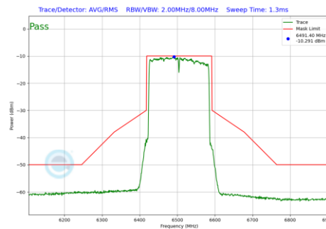
Plot 7-636 In-Band Emission Plot SDM Primary Antenna 3c (160MHz BW 802.11be(RU) RU996X2 Index68 (UNII Band 6) - Ch.111)
