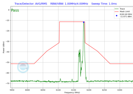
Plot 7-663 In-Band Emission Plot SDM Diversity Antenna 1b (80MHz BW 802.11be(RU) RU26 Index36 (UNII Band 5) - Ch.39)
