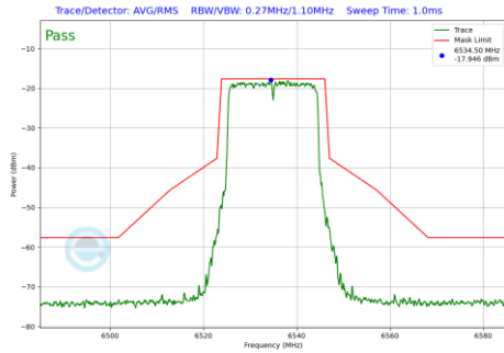
Plot 7-637 In-Band Emission Plot SDM Primary Antenna 3c (20MHz BW 802.11be(RU) RU242 Index61 (UNII Band 7) - Ch.117)
