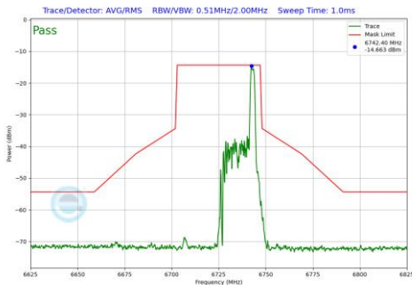
Plot 7-598 In-Band Emission Plot SDM Primary Antenna 3a (40MHz BW 802.11be(RU) RU26 Index17 (UNII Band 7) - Ch.155)
