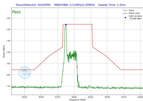
Plot 7-662 In-Band Emission Plot SDM Diversity Antenna 1b (40MHz BW 802.11be(RU) RU26 Index0 (UNII Band 5) - Ch.91)
