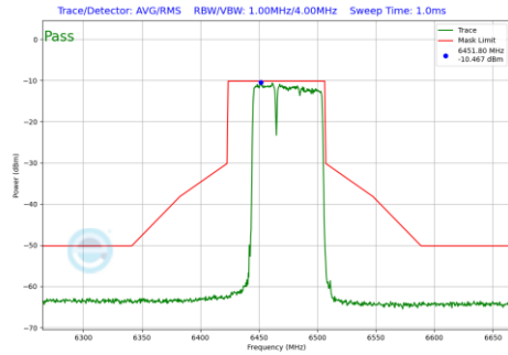
Plot 7-709 In-Band Emission Plot SDM Diversity Antenna 3c (80MHz BW 802.11be(RU) RU484+242 Index90 (UNII Band 6) - Ch.103)
