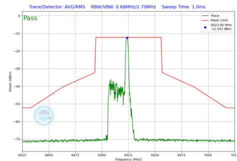
Plot 7-674 In-Band Emission Plot SDM Diversity Antenna 1b (40MHz BW 802.11be(RU) RU26 Index8 (UNII Band 8) - Ch.195)
