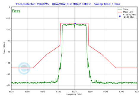
Plot 7-630 In-Band Emission Plot SDM Primary Antenna 3c (40MHz BW 802.11be(RU) RU484 Index65 (UNII Band 5) - Ch.35)
