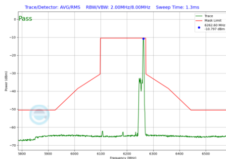
Plot 7-680 In-Band Emission Plot SDM Diversity Antenna 3c (160MHz BW 802.11be(RU) RU26 Index36 (UNII Band 5) - Ch.47)
