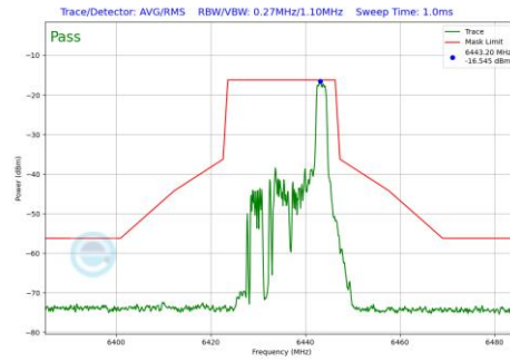
Plot 7-665 In-Band Emission Plot SDM Diversity Antenna 1b (20MHz BW 802.11be(RU) RU26 Index8 (UNII Band 6) - Ch.97)
