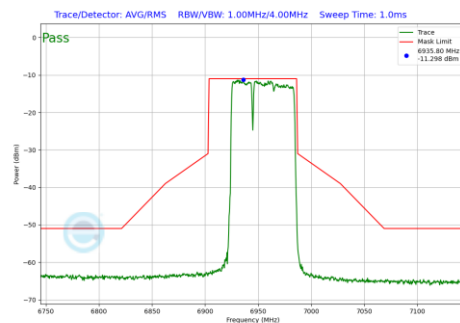
Plot 7-715 In-Band Emission Plot SDM Diversity Antenna 3c (80MHz BW 802.11be(RU) RU484+242 Index90 (UNII Band 8) - Ch.199)
