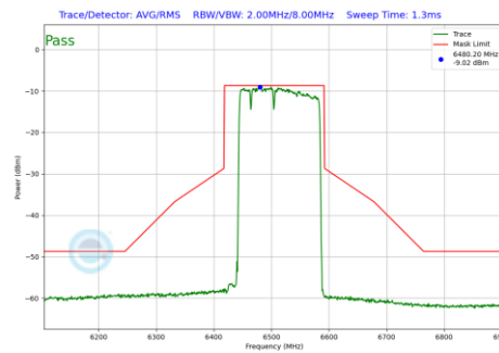
Plot 7-610 In-Band Emission Plot SDM Primary Antenna 3c (160MHz BW 802.11be(RU) RU996+484+242 Index96 (UNII Band 6) - Ch.111)
