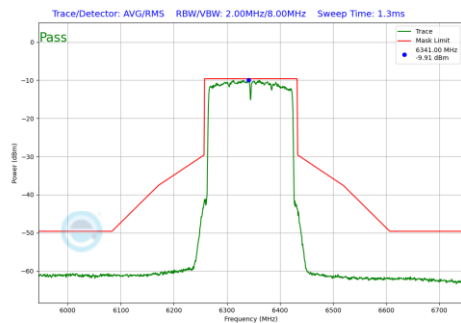
Plot 7-632 In-Band Emission Plot SDM Primary Antenna 3c (160MHz BW 802.11be(RU) RU996X2 Index68 (UNII Band 5) - Ch.79)
