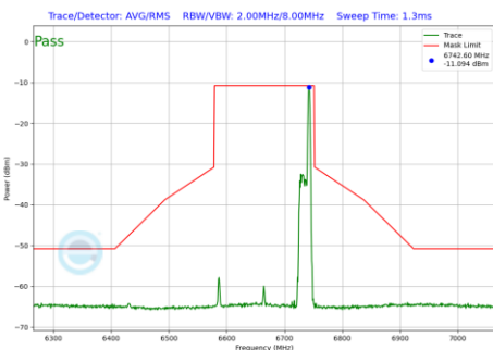
Plot 7-688 In-Band Emission Plot SDM Diversity Antenna 3c (160MHz BW 802.11be(RU) RU26 Index36 (UNII Band 7) - Ch.143)
