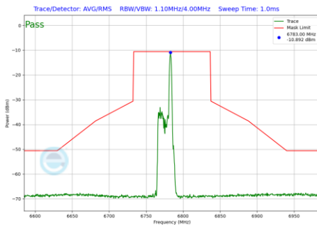
Plot 7-671 In-Band Emission Plot SDM Diversity Antenna 1b (80MHz BW 802.11be(RU) RU26 Index17 (UNII Band 7) - Ch.167)
