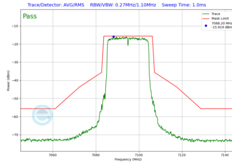
Plot 7-657 In-Band Emission Plot SDM Primary Antenna 3a (20MHz BW 802.11be(RU) RU242 Index61 (UNII Band 8) - Ch.229)
