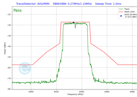
Plot 7-633 In-Band Emission Plot SDM Primary Antenna 3c (20MHz BW 802.11be(RU) RU242 Index61 (UNII Band 6) - Ch.97)
