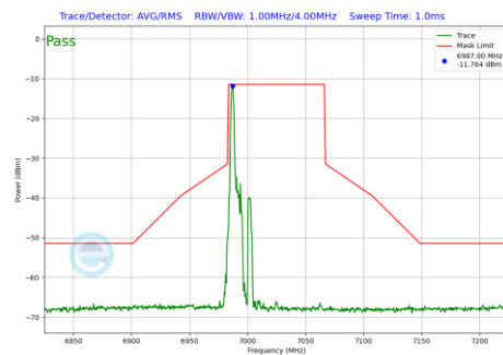
Plot 7-587 In-Band Emission Plot SDM Primary Antenna 3c (80MHz BW 802.11be(RU) RU26 Index0 (UNII Band 8) - Ch.215)
