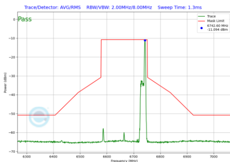
Plot 7-584 In-Band Emission Plot SDM Primary Antenna 3c (160MHz BW 802.11be(RU) RU26 Index36 (UNII Band 7) - Ch.143)
