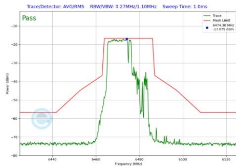
Plot 7-696 In-Band Emission Plot SDM Diversity Antenna 1b (20MHz BW 802.11be(RU) RU106+26 Index82 (UNII Band 6) - Ch.105)
