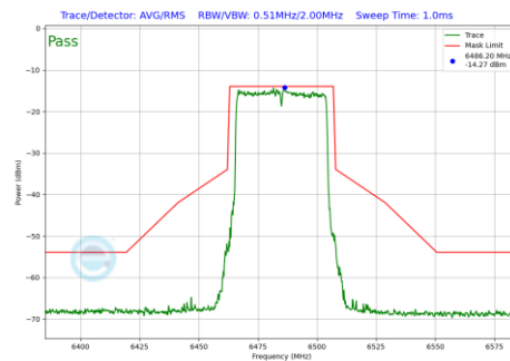
Plot 7-738 In-Band Emission Plot SDM Diversity Antenna 3c (40MHz BW 802.11be(RU) RU484 Index65 (UNII Band 6) - Ch.107)
