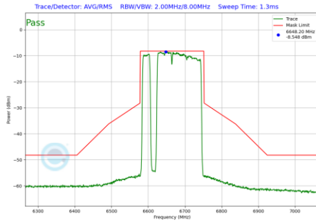
Plot 7-701 In-Band Emission Plot SDM Diversity Antenna 1b (160MHz BW 802.11be(RU) RU996+484+242 Index97 (UNII Band 7) - Ch.143)
