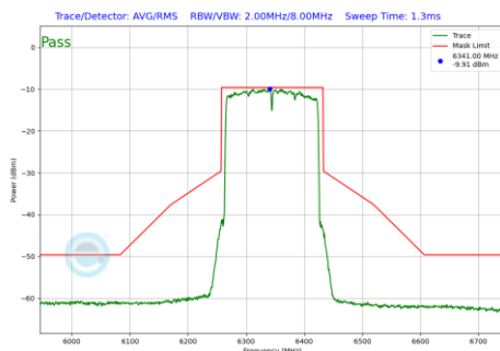
Plot 7-736 In-Band Emission Plot SDM Diversity Antenna 3c (160MHz BW 802.11be(RU) RU996X2 Index68 (UNII Band 5) - Ch.79)
