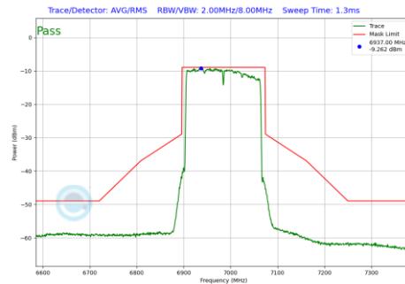
Plot 7-660 In-Band Emission Plot SDM Primary Antenna 3a (160MHz BW 802.11be(RU) RU996X2 Index68 (UNII Band 8) - Ch.207)
