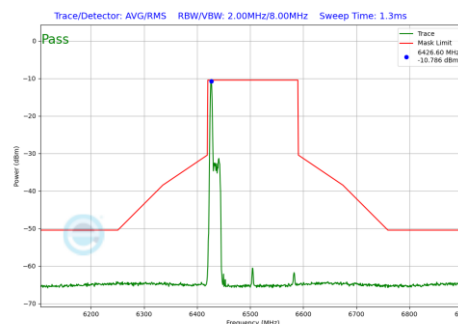
Plot 7-668 In-Band Emission Plot SDM Diversity Antenna 1b (160MHz BW 802.11be(RU) RU26 Index0 (UNII Band 6) - Ch.111)
