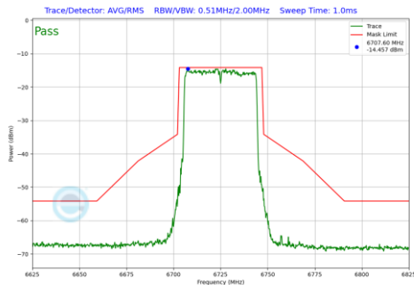
Plot 7-726 In-Band Emission Plot SDM Diversity Antenna 1b (40MHz BW 802.11be(RU) RU484 Index65 (UNII Band 7) - Ch.155)
