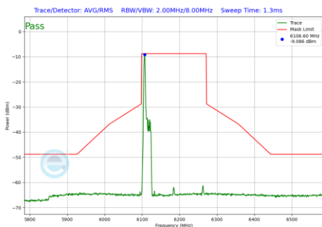
Plot 7-576 In-Band Emission Plot SDM Primary Antenna 3c (160MHz BW 802.11be(RU) RU26 Index0 (UNII Band 5) - Ch.47)
