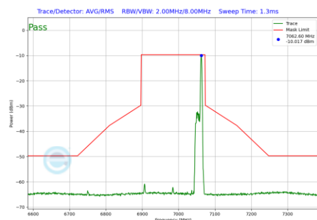
Plot 7-692 In-Band Emission Plot SDM Diversity Antenna 3c (160MHz BW 802.11be(RU) RU26 Index36 (UNII Band 8) - Ch.207)
