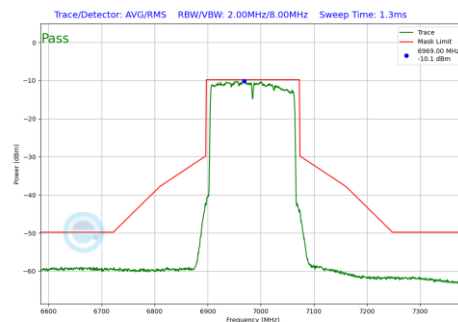
Plot 7-644 In-Band Emission Plot SDM Primary Antenna 3c (160MHz BW 802.11be(RU) RU996X2 Index68 (UNII Band 8) - Ch.207)
