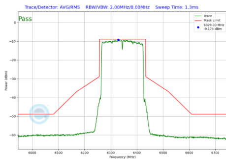
Plot 7-648 In-Band Emission Plot SDM Primary Antenna 3a (160MHz BW 802.11be(RU) RU996X2 Index68 (UNII Band 5) - Ch.79)
