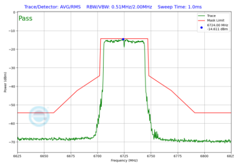
Plot 7-654 In-Band Emission Plot SDM Primary Antenna 3a (40MHz BW 802.11be(RU) RU484 Index65 (UNII Band 7) - Ch.155)
