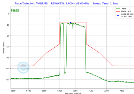
Plot 7-704 In-Band Emission Plot SDM Diversity Antenna 1b (160MHz BW 802.11be(RU) RU996+484+242 Index97 (UNII Band 8) - Ch.207)
