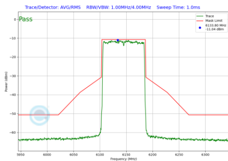
Plot 7-647 In-Band Emission Plot SDM Primary Antenna 3a (80MHz BW 802.11be(RU) RU996 Index67 (UNII Band 5) - Ch.39)
