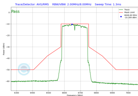
Plot 7-640 In-Band Emission Plot SDM Primary Antenna 3c (160MHz BW 802.11be(RU) RU996X2 Index68 (UNII Band 7) - Ch.143)
