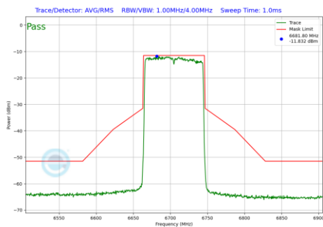
Plot 7-639 In-Band Emission Plot SDM Primary Antenna 3c (80MHz BW 802.11be(RU) RU996 Index67 (UNII Band 7) - Ch.151)
