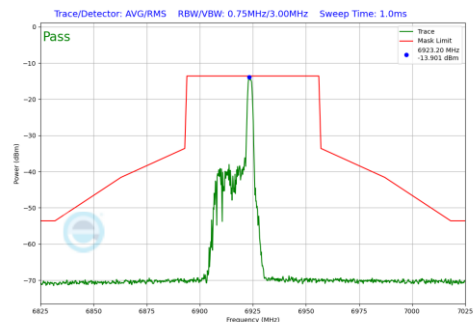
Plot 7-690 In-Band Emission Plot SDM Diversity Antenna 3c (40MHz BW 802.11be(RU) RU26 Index8 (UNII Band 8) - Ch.195)
