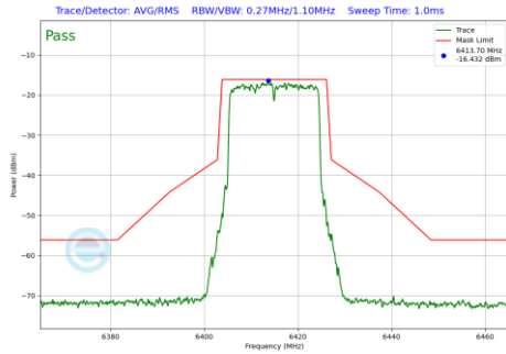
Plot 7-645 In-Band Emission Plot SDM Primary Antenna 3a (20MHz BW 802.11be(RU) RU242 Index61 (UNII Band 5) - Ch.93)
