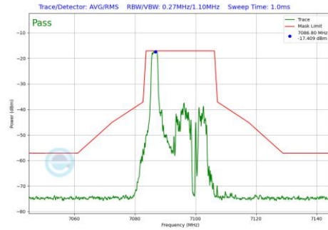
Plot 7-601 In-Band Emission Plot SDM Primary Antenna 3a (20MHz BW 802.11be(RU) RU26 Index0 (UNII Band 8) - Ch.229)
