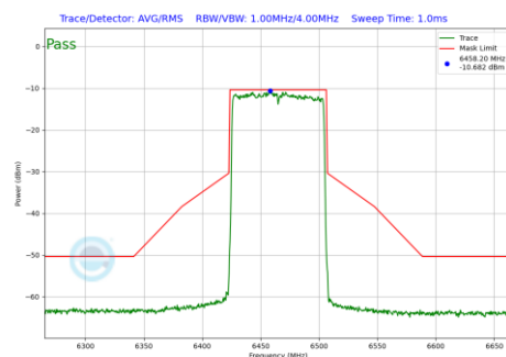
Plot 7-651 In-Band Emission Plot SDM Primary Antenna 3a (80MHz BW 802.11be(RU) RU996 Index67 (UNII Band 6) - Ch.103)
