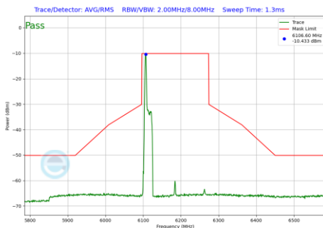
Plot 7-592 In-Band Emission Plot SDM Primary Antenna 3a (160MHz BW 802.11be(RU) RU26 Index0 (UNII Band 5) - Ch.47)
