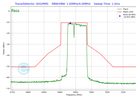
Plot 7-703 In-Band Emission Plot SDM Diversity Antenna 1b (80MHz BW 802.11be(RU) RU484+242 Index90 (UNII Band 8) - Ch.199)
