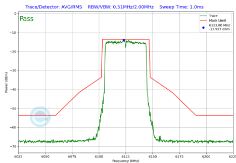
Plot 7-646 In-Band Emission Plot SDM Primary Antenna 3a (40MHz BW 802.11be(RU) RU484 Index65 (UNII Band 5) - Ch.35)
