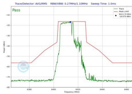
Plot 7-693 In-Band Emission Plot SDM Diversity Antenna 1b (20MHz BW 802.11be(RU) RU106+26 Index82 (UNII Band 5) - Ch.93)
