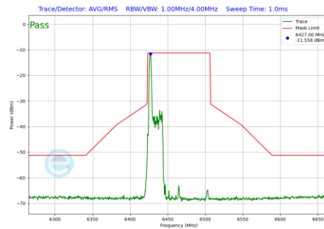
Plot 7-667 In-Band Emission Plot SDM Diversity Antenna 1b (80MHz BW 802.11be(RU) RU26 Index0 (UNII Band 6) - Ch.103)
