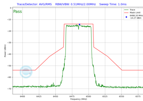
Plot 7-634 In-Band Emission Plot SDM Primary Antenna 3c (40MHz BW 802.11be(RU) RU484 Index65 (UNII Band 6) - Ch.107)
