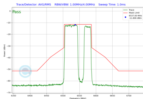
Plot 7-624 In-Band Emission Plot SDM Primary Antenna 3a (80MHz BW 802.11be(RU) RU484+242 Index92 (UNII Band 7) - Ch.119)
