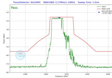
Plot 7-705 In-Band Emission Plot SDM Diversity Antenna 3c (20MHz BW 802.11be(RU) RU106+26 Index82 (UNII Band 5) - Ch.93)
