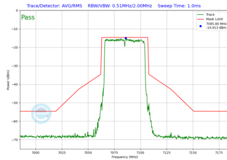
Plot 7-746 In-Band Emission Plot SDM Diversity Antenna 3c (40MHz BW 802.11be(RU) RU484 Index65 (UNII Band 8) - Ch.227)
