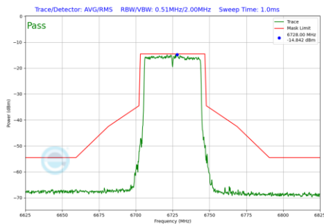
Plot 7-638 In-Band Emission Plot SDM Primary Antenna 3c (40MHz BW 802.11be(RU) RU484 Index65 (UNII Band 7) - Ch.155)
