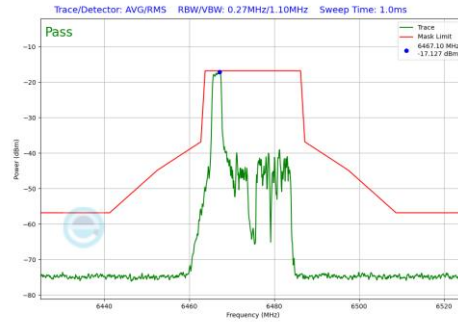
Plot 7-593 In-Band Emission Plot SDM Primary Antenna 3a (20MHz BW 802.11be(RU) RU26 Index0 (UNII Band 6) - Ch.105)
