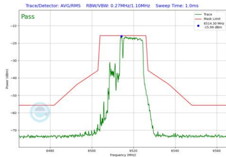
Plot 7-608 In-Band Emission Plot SDM Primary Antenna 3c (20MHz BW 802.11be(RU) RU106+26 Index83 (UNII Band 6) - Ch.113)
