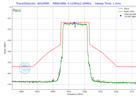
Plot 7-658 In-Band Emission Plot SDM Primary Antenna 3a (40MHz BW 802.11be(RU) RU484 Index65 (UNII Band 8) - Ch.227)
