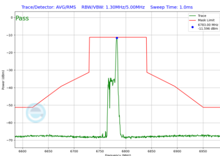
Plot 7-687 In-Band Emission Plot SDM Diversity Antenna 3c (80MHz BW 802.11be(RU) RU26 Index17 (UNII Band 7) - Ch.167)
