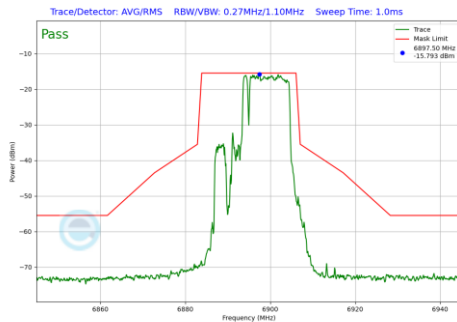
Plot 7-702 In-Band Emission Plot SDM Diversity Antenna 1b (20MHz BW 802.11be(RU) RU106+26 Index83 (UNII Band 8) - Ch.189)
