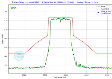
Plot 7-653 In-Band Emission Plot SDM Primary Antenna 3a (20MHz BW 802.11be(RU) RU242 Index61 (UNII Band 7) - Ch.117)
