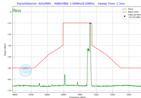
Plot 7-604 In-Band Emission Plot SDM Primary Antenna 3a (160MHz BW 802.11be(RU) RU26 Index36 (UNII Band 8) - Ch.207)
