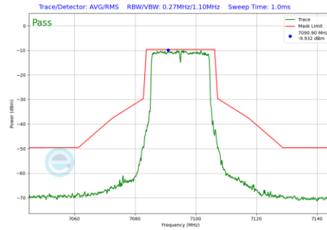
Plot 7-569 In-Band Emission Plot Antenna 1b (20MHz BW 802.11be(RU) RU242 Index61 (UNII Band 8) - Ch.229)
