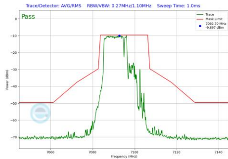
Plot 7-554 In-Band Emission Plot Antenna 1b (20MHz BW 802.11be(RU) RU106+26 Index82 (UNII Band 8) - Ch.229)
