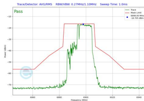
Plot 7-714 In-Band Emission Plot SDM Diversity Antenna 3c (20MHz BW 802.11be(RU) RU106+26 Index83 (UNII Band 8) - Ch.189)
