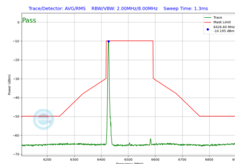
Plot 7-684 In-Band Emission Plot SDM Diversity Antenna 3c (160MHz BW 802.11be(RU) RU26 Index0 (UNII Band 6) - Ch.111)
