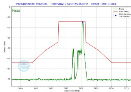
Plot 7-586 In-Band Emission Plot SDM Primary Antenna 3c (40MHz BW 802.11be(RU) RU26 Index17 (UNII Band 8) - Ch.227)
