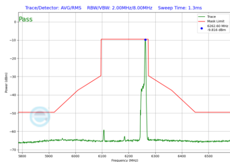
Plot 7-664 In-Band Emission Plot SDM Diversity Antenna 1b (160MHz BW 802.11be(RU) RU26 Index36 (UNII Band 5) - Ch.47)
