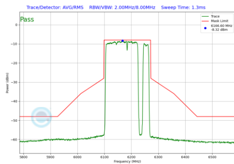
Plot 7-607 In-Band Emission Plot SDM Primary Antenna 3c (160MHz BW 802.11be(RU) RU996+484+242 Index98 (UNII Band 5) - Ch.47)
