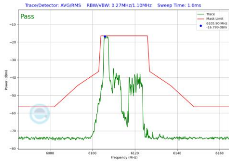
Plot 7-661 In-Band Emission Plot SDM Diversity Antenna 1b (20MHz BW 802.11be(RU) RU26 Index0 (UNII Band 5) - Ch.33)
