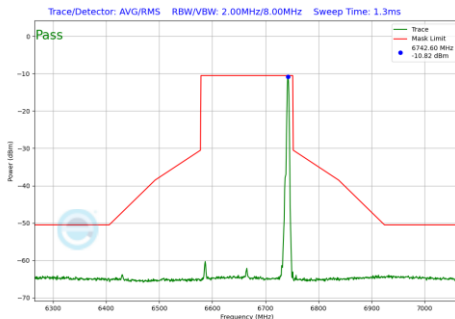
Plot 7-672 In-Band Emission Plot SDM Diversity Antenna 1b (160MHz BW 802.11be(RU) RU26 Index36 (UNII Band 7) - Ch.143)
