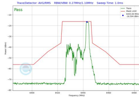
Plot 7-681 In-Band Emission Plot SDM Diversity Antenna 3c (20MHz BW 802.11be(RU) RU26 Index8 (UNII Band 6) - Ch.97)
