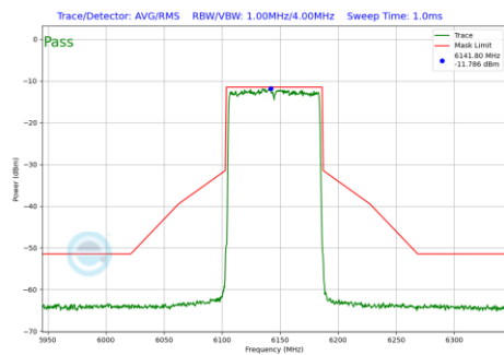
Plot 7-631 In-Band Emission Plot SDM Primary Antenna 3c (80MHz BW 802.11be(RU) RU996 Index67 (UNII Band 5) - Ch.39)
