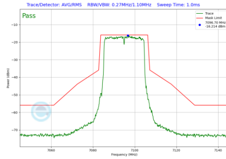
Plot 7-729 In-Band Emission Plot SDM Diversity Antenna 1b (20MHz BW 802.11be(RU) RU242 Index61 (UNII Band 8) - Ch.229)
