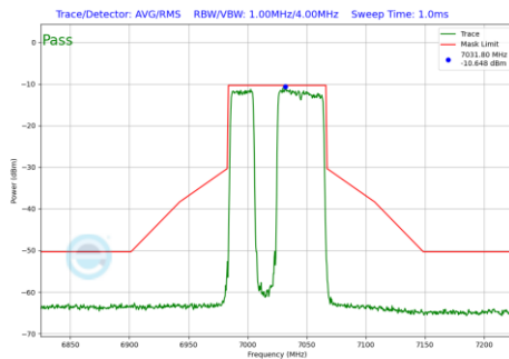
Plot 7-615 In-Band Emission Plot SDM Primary Antenna 3c (80MHz BW 802.11be(RU) RU484+242 Index91 (UNII Band 8) - Ch.215)
