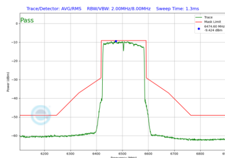
Plot 7-652 In-Band Emission Plot SDM Primary Antenna 3a (160MHz BW 802.11be(RU) RU996X2 Index68 (UNII Band 6) - Ch.111)
