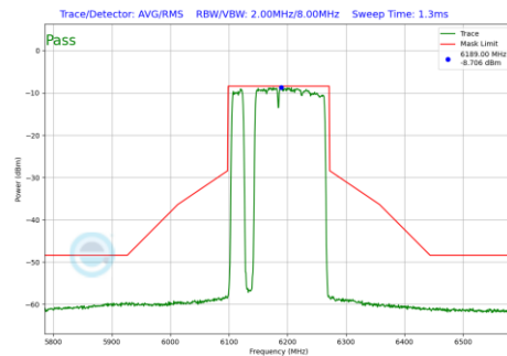
Plot 7-707 In-Band Emission Plot SDM Diversity Antenna 3c (160MHz BW 802.11be(RU) RU996+484+242 Index97 (UNII Band 5) - Ch.47)
