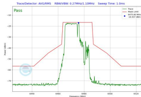
Plot 7-708 In-Band Emission Plot SDM Diversity Antenna 3c (20MHz BW 802.11be(RU) RU106+26 Index82 (UNII Band 6) - Ch.105)
