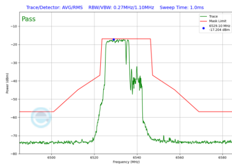
Plot 7-623 In-Band Emission Plot SDM Primary Antenna 3a (20MHz BW 802.11be(RU) RU106+26 Index82 (UNII Band 7) - Ch.117)
