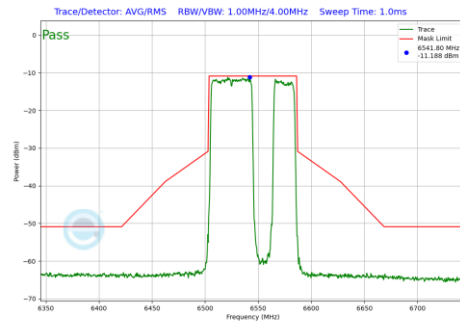
Plot 7-612 In-Band Emission Plot SDM Primary Antenna 3c (80MHz BW 802.11be(RU) RU484+242 Index92 (UNII Band 7) - Ch.119)
