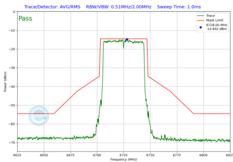
Plot 7-742 In-Band Emission Plot SDM Diversity Antenna 3c (40MHz BW 802.11be(RU) RU484 Index65 (UNII Band 7) - Ch.155)
