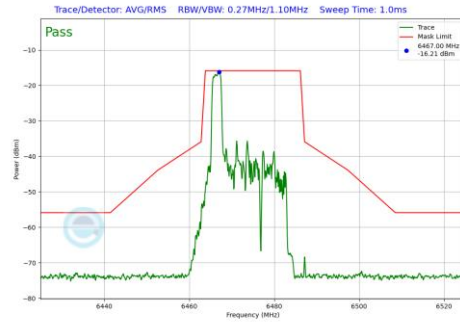
Plot 7-577 In-Band Emission Plot SDM Primary Antenna 3c (20MHz BW 802.11be(RU) RU26 Index0 (UNII Band 6) - Ch.105)
