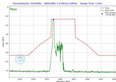
Plot 7-678 In-Band Emission Plot SDM Diversity Antenna 3c (40MHz BW 802.11be(RU) RU26 Index0 (UNII Band 5) - Ch.91)
