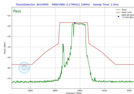
Plot 7-626 In-Band Emission Plot SDM Primary Antenna 3a (20MHz BW 802.11be(RU) RU106+26 Index83 (UNII Band 8) - Ch.189)
