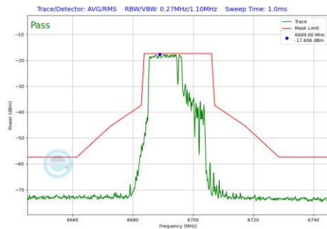
Plot 7-711 In-Band Emission Plot SDM Diversity Antenna 3c (20MHz BW 802.11be(RU) RU106+26 Index82 (UNII Band 7) - Ch.149)
