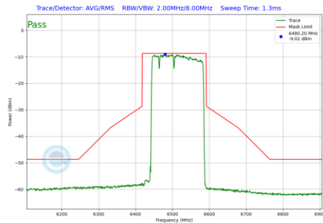
Plot 7-710 In-Band Emission Plot SDM Diversity Antenna 3c (160MHz BW 802.11be(RU) RU996+484+242 Index96 (UNII Band 6) - Ch.111)
