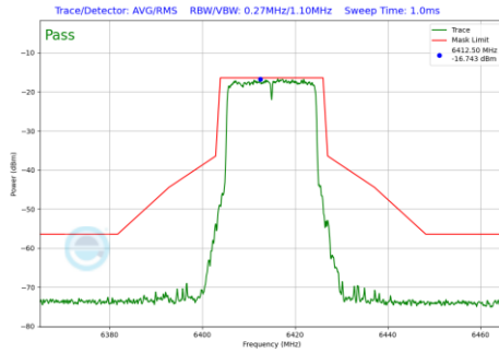
Plot 7-733 In-Band Emission Plot SDM Diversity Antenna 3c (20MHz BW 802.11be(RU) RU242 Index61 (UNII Band 5) - Ch.93)
