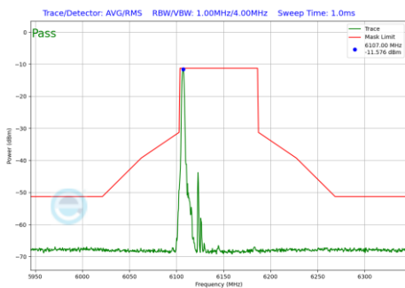
Plot 7-575 In-Band Emission Plot SDM Primary Antenna 3c (80MHz BW 802.11be(RU) RU26 Index0 (UNII Band 5) - Ch.39)
