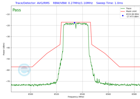
Plot 7-725 In-Band Emission Plot SDM Diversity Antenna 1b (20MHz BW 802.11be(RU) RU242 Index61 (UNII Band 7) - Ch.117)
