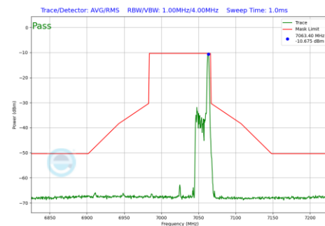
Plot 7-675 In-Band Emission Plot SDM Diversity Antenna 1b (80MHz BW 802.11be(RU) RU26 Index36 (UNII Band 8) - Ch.215)
