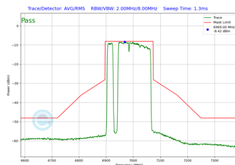
Plot 7-628 In-Band Emission Plot SDM Primary Antenna 3a (160MHz BW 802.11be(RU) RU996+484+242 Index97 (UNII Band 8) - Ch.207)
