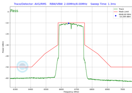
Plot 7-744 In-Band Emission Plot SDM Diversity Antenna 3c (160MHz BW 802.11be(RU) RU996X2 Index68 (UNII Band 7) - Ch.143)
