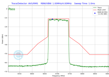
Plot 7-655 In-Band Emission Plot SDM Primary Antenna 3a (80MHz BW 802.11be(RU) RU996 Index67 (UNII Band 7) - Ch.151)
