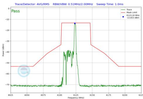
Plot 7-574 In-Band Emission Plot SDM Primary Antenna 3c (40MHz BW 802.11be(RU) RU26 Index8 (UNII Band 5) - Ch.35)
