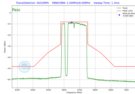
Plot 7-713 In-Band Emission Plot SDM Diversity Antenna 3c (160MHz BW 802.11be(RU) RU996+484+242 Index97 (UNII Band 7) - Ch.143)
