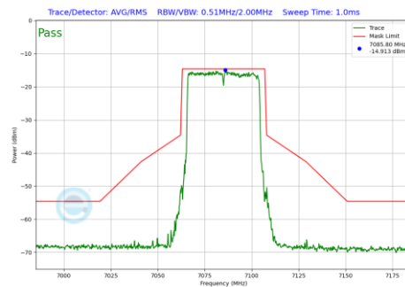
Plot 7-642 In-Band Emission Plot SDM Primary Antenna 3c (40MHz BW 802.11be(RU) RU484 Index65 (UNII Band 8) - Ch.227)
