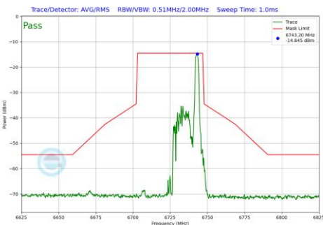
Plot 7-686 In-Band Emission Plot SDM Diversity Antenna 3c (40MHz BW 802.11be(RU) RU26 Index17 (UNII Band 7) - Ch.155)
