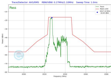
Plot 7-581 In-Band Emission Plot SDM Primary Antenna 3c (20MHz BW 802.11be(RU) RU26 Index0 (UNII Band 7) - Ch.117)
