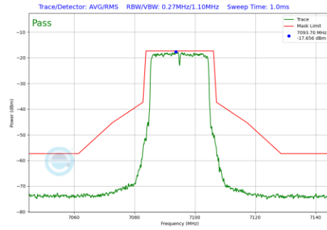
Plot 7-745 In-Band Emission Plot SDM Diversity Antenna 3c (20MHz BW 802.11be(RU) RU242 Index61 (UNII Band 8) - Ch.229)
