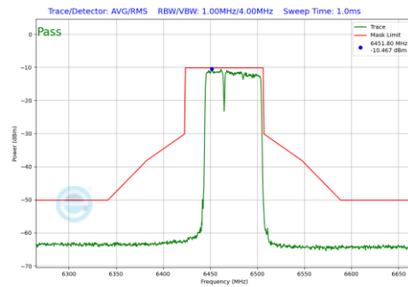
Plot 7-609 In-Band Emission Plot SDM Primary Antenna 3c (80MHz BW 802.11be(RU) RU484+242 Index90 (UNII Band 6) - Ch.103)
