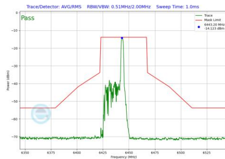
Plot 7-578 In-Band Emission Plot SDM Primary Antenna 3c (40MHz BW 802.11be(RU) RU26 Index8 (UNII Band 6) - Ch.99)
