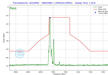
Plot 7-603 In-Band Emission Plot SDM Primary Antenna 3a (80MHz BW 802.11be(RU) RU26 Index0 (UNII Band 8) - Ch.215)
