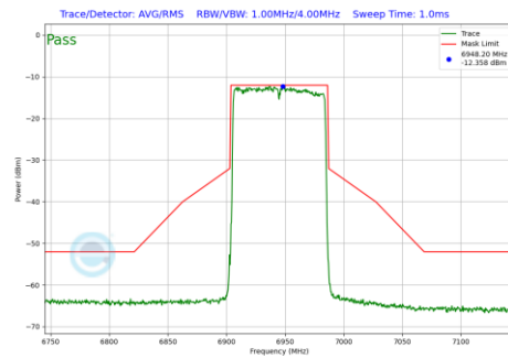
Plot 7-747 In-Band Emission Plot SDM Diversity Antenna 3c (80MHz BW 802.11be(RU) RU996 Index67 (UNII Band 8) - Ch.199)
