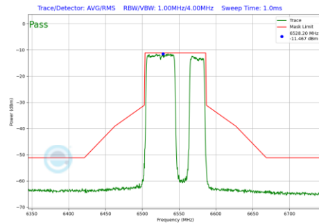
Plot 7-700 In-Band Emission Plot SDM Diversity Antenna 1b (80MHz BW 802.11be(RU) RU484+242 Index92 (UNII Band 7) - Ch.119)
