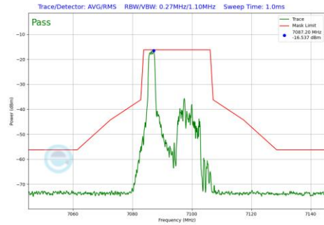
Plot 7-689 In-Band Emission Plot SDM Diversity Antenna 3c (20MHz BW 802.11be(RU) RU26 Index0 (UNII Band 8) - Ch.229)
