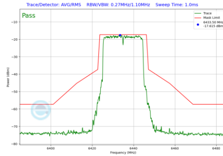
Plot 7-737 In-Band Emission Plot SDM Diversity Antenna 3c (20MHz BW 802.11be(RU) RU242 Index61 (UNII Band 6) - Ch.97)
