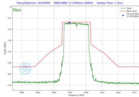
Plot 7-730 In-Band Emission Plot SDM Diversity Antenna 1b (40MHz BW 802.11be(RU) RU484 Index65 (UNII Band 8) - Ch.227)
