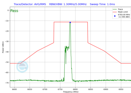
Plot 7-583 In-Band Emission Plot SDM Primary Antenna 3c (80MHz BW 802.11be(RU) RU26 Index17 (UNII Band 7) - Ch.167)
