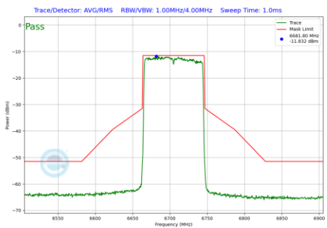
Plot 7-743 In-Band Emission Plot SDM Diversity Antenna 3c (80MHz BW 802.11be(RU) RU996 Index67 (UNII Band 7) - Ch.151)
