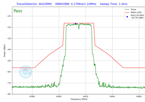
Plot 7-629 In-Band Emission Plot SDM Primary Antenna 3c (20MHz BW 802.11be(RU) RU242 Index61 (UNII Band 5) - Ch.93)
