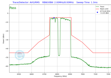
Plot 7-553 In-Band Emission Plot Antenna 1b (160MHz BW 802.11be(RU) RU996+484+242 Index99 (UNII Band 7) - Ch.175)
