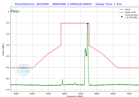
Plot 7-600 In-Band Emission Plot SDM Primary Antenna 3a (160MHz BW 802.11be(RU) RU26 Index36 (UNII Band 7) - Ch.143)
