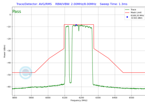
Plot 7-695 In-Band Emission Plot SDM Diversity Antenna 1b (160MHz BW 802.11be(RU) RU996+484+242 Index97 (UNII Band 5) - Ch.47)
