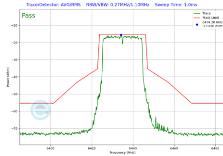
Plot 7-649 In-Band Emission Plot SDM Primary Antenna 3a (20MHz BW 802.11be(RU) RU242 Index61 (UNII Band 6) - Ch.97)
