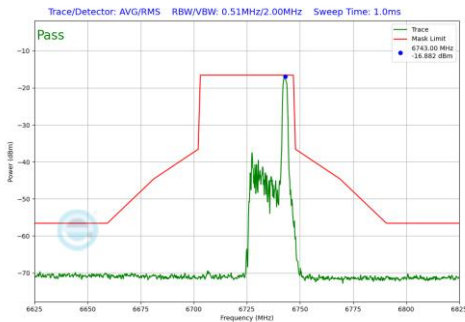
Plot 7-670 In-Band Emission Plot SDM Diversity Antenna 1b (40MHz BW 802.11be(RU) RU26 Index17 (UNII Band 7) - Ch.155)
