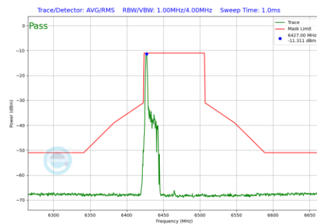
Plot 7-579 In-Band Emission Plot SDM Primary Antenna 3c (80MHz BW 802.11be(RU) RU26 Index0 (UNII Band 6) - Ch.103)
