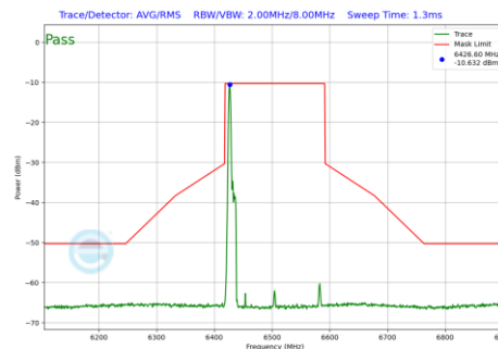
Plot 7-596 In-Band Emission Plot SDM Primary Antenna 3a (160MHz BW 802.11be(RU) RU26 Index0 (UNII Band 6) - Ch.111)
