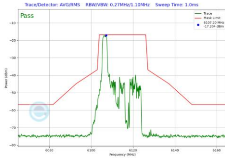
Plot 7-677 In-Band Emission Plot SDM Diversity Antenna 3c (20MHz BW 802.11be(RU) RU26 Index0 (UNII Band 5) - Ch.33)
