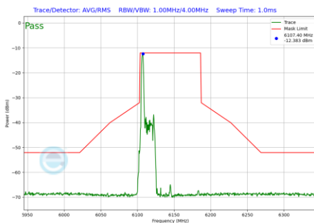
Plot 7-591 In-Band Emission Plot SDM Primary Antenna 3a (80MHz BW 802.11be(RU) RU26 Index0 (UNII Band 5) - Ch.39)
