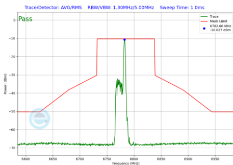
Plot 7-599 In-Band Emission Plot SDM Primary Antenna 3a (80MHz BW 802.11be(RU) RU26 Index17 (UNII Band 7) - Ch.167)
