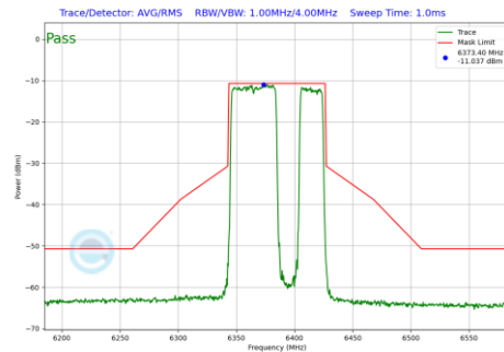
Plot 7-706 In-Band Emission Plot SDM Diversity Antenna 3c (80MHz BW 802.11be(RU) RU484+242 Index92 (UNII Band 5) - Ch.87)
