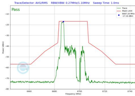
Plot 7-669 In-Band Emission Plot SDM Diversity Antenna 1b (20MHz BW 802.11be(RU) RU26 Index0 (UNII Band 7) - Ch.149)
