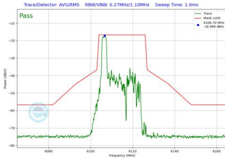
Plot 7-589 In-Band Emission Plot SDM Primary Antenna 3a (20MHz BW 802.11be(RU) RU26 Index0 (UNII Band 5) - Ch.33)
