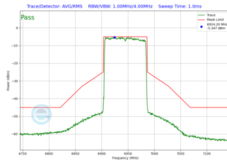
Plot 7-571 In-Band Emission Plot Antenna 1b (80MHz BW 802.11be(RU) RU996 Index67 (UNII Band 8) - Ch.199)
