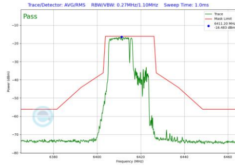
Plot 7-617 In-Band Emission Plot SDM Primary Antenna 3a (20MHz BW 802.11be(RU) RU106+26 Index82 (UNII Band 5) - Ch.93)
