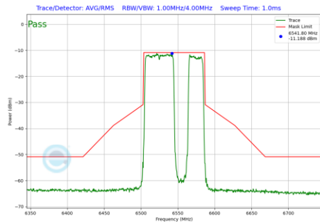
Plot 7-712 In-Band Emission Plot SDM Diversity Antenna 3c (80MHz BW 802.11be(RU) RU484+242 Index92 (UNII Band 7) - Ch.119)
