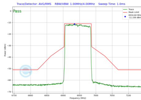
Plot 7-659 In-Band Emission Plot SDM Primary Antenna 3a (80MHz BW 802.11be(RU) RU996 Index67 (UNII Band 8) - Ch.199)
