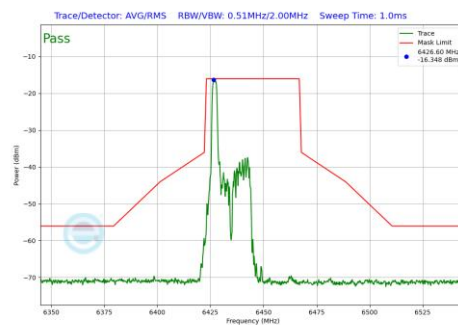
Plot 7-666 In-Band Emission Plot SDM Diversity Antenna 1b (40MHz BW 802.11be(RU) RU26 Index0 (UNII Band 6) - Ch.99)
