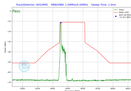
Plot 7-683 In-Band Emission Plot SDM Diversity Antenna 3c (80MHz BW 802.11be(RU) RU26 Index0 (UNII Band 6) - Ch.103)
