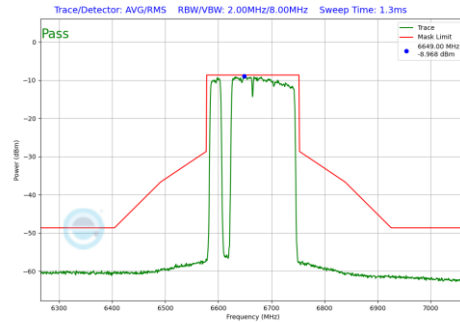
Plot 7-625 In-Band Emission Plot SDM Primary Antenna 3a (160MHz BW 802.11be(RU) RU996+484+242 Index97 (UNII Band 7) - Ch.143)
