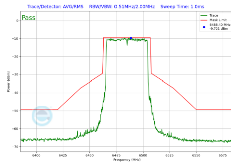
Plot 7-562 In-Band Emission Plot Antenna 1b (40MHz BW 802.11be(RU) RU484 Index65 (UNII Band 6) - Ch.107)
