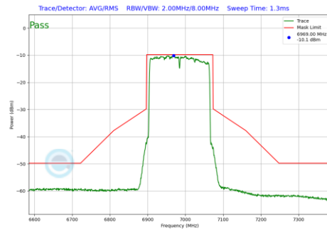
Plot 7-748 In-Band Emission Plot SDM Diversity Antenna 3c (160MHz BW 802.11be(RU) RU996X2 Index68 (UNII Band 8) - Ch.207)
