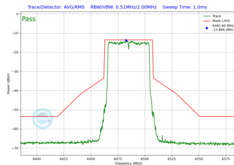
Plot 7-650 In-Band Emission Plot SDM Primary Antenna 3a (40MHz BW 802.11be(RU) RU484 Index65 (UNII Band 6) - Ch.107)
