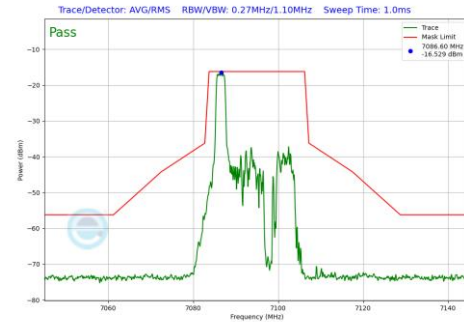
Plot 7-673 In-Band Emission Plot SDM Diversity Antenna 1b (20MHz BW 802.11be(RU) RU26 Index0 (UNII Band 8) - Ch.229)
