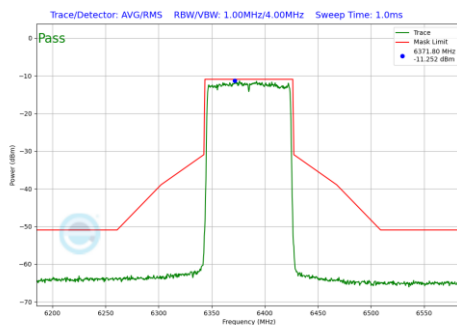
Plot 7-735 In-Band Emission Plot SDM Diversity Antenna 3c (80MHz BW 802.11be(RU) RU996 Index67 (UNII Band 5) - Ch.87)
