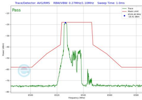
Plot 7-597 In-Band Emission Plot SDM Primary Antenna 3a (20MHz BW 802.11be(RU) RU26 Index0 (UNII Band 7) - Ch.117)
