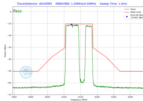
Plot 7-618 In-Band Emission Plot SDM Primary Antenna 3a (80MHz BW 802.11be(RU) RU484+242 Index92 (UNII Band 5) - Ch.39)
