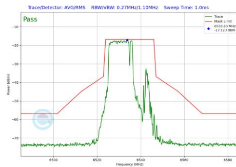
Plot 7-611 In-Band Emission Plot SDM Primary Antenna 3c (20MHz BW 802.11be(RU) RU106+26 Index82 (UNII Band 7) - Ch.117)
