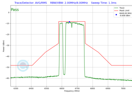
Plot 7-613 In-Band Emission Plot SDM Primary Antenna 3c (160MHz BW 802.11be(RU) RU996+484+242 Index97 (UNII Band 7) - Ch.143)
