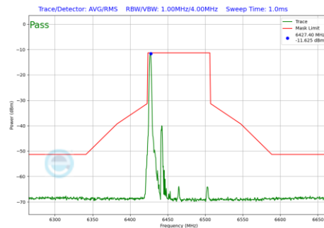
Plot 7-595 In-Band Emission Plot SDM Primary Antenna 3a (80MHz BW 802.11be(RU) RU26 Index0 (UNII Band 6) - Ch.103)
