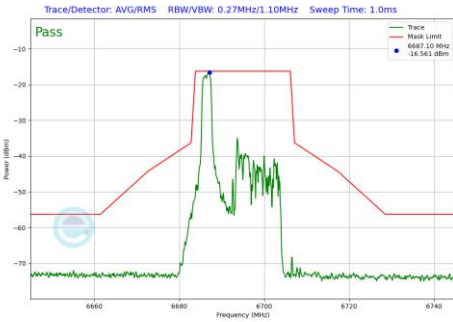
Plot 7-685 In-Band Emission Plot SDM Diversity Antenna 3c (20MHz BW 802.11be(RU) RU26 Index0 (UNII Band 7) - Ch.149)
