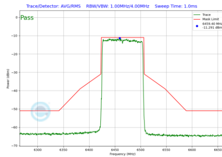
Plot 7-739 In-Band Emission Plot SDM Diversity Antenna 3c (80MHz BW 802.11be(RU) RU996 Index67 (UNII Band 6) - Ch.103)
