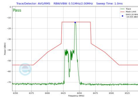
Plot 7-594 In-Band Emission Plot SDM Primary Antenna 3a (40MHz BW 802.11be(RU) RU26 Index8 (UNII Band 6) - Ch.99)
