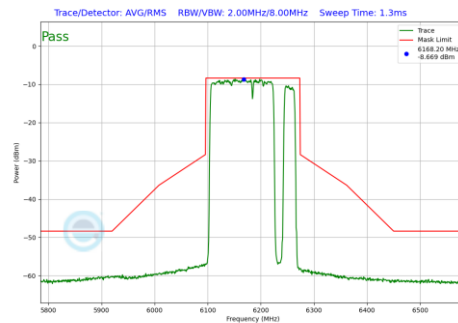
Plot 7-619 In-Band Emission Plot SDM Primary Antenna 3a (160MHz BW 802.11be(RU) RU996+484+242 Index98 (UNII Band 5) - Ch.47)
