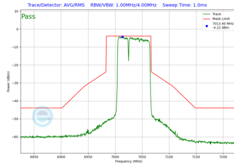
Plot 7-555 In-Band Emission Plot Antenna 1b (80MHz BW 802.11be(RU) RU484+242 Index90 (UNII Band 8) - Ch.215)
