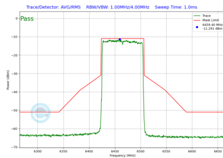
Plot 7-635 In-Band Emission Plot SDM Primary Antenna 3c (80MHz BW 802.11be(RU) RU996 Index67 (UNII Band 6) - Ch.103)
