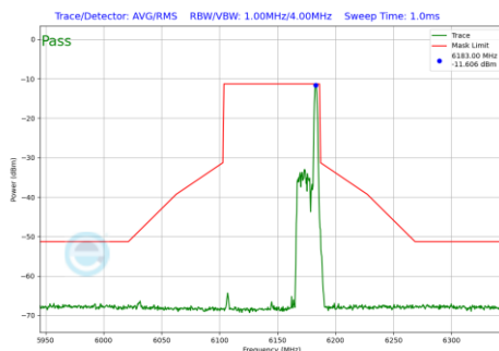
Plot 7-679 In-Band Emission Plot SDM Diversity Antenna 3c (80MHz BW 802.11be(RU) RU26 Index36 (UNII Band 5) - Ch.39)
