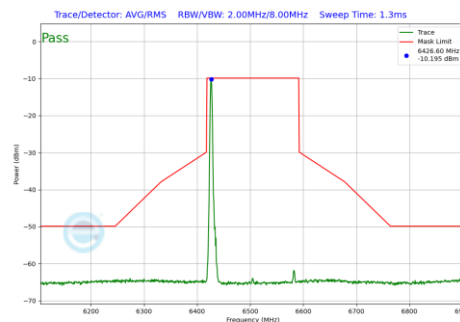
Plot 7-580 In-Band Emission Plot SDM Primary Antenna 3c (160MHz BW 802.11be(RU) RU26 Index0 (UNII Band 6) - Ch.111)
