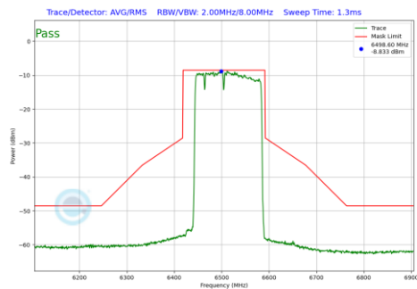
Plot 7-622 In-Band Emission Plot SDM Primary Antenna 3a (160MHz BW 802.11be(RU) RU996+484+242 Index96 (UNII Band 6) - Ch.111)
