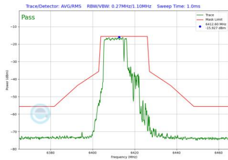
Plot 7-605 In-Band Emission Plot SDM Primary Antenna 3c (20MHz BW 802.11be(RU) RU106+26 Index82 (UNII Band 5) - Ch.93)
