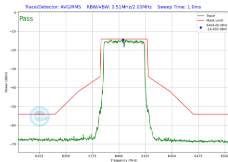
Plot 7-734 In-Band Emission Plot SDM Diversity Antenna 3c (40MHz BW 802.11be(RU) RU484 Index65 (UNII Band 5) - Ch.91)
