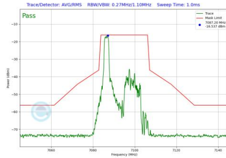
Plot 7-585 In-Band Emission Plot SDM Primary Antenna 3c (20MHz BW 802.11be(RU) RU26 Index0 (UNII Band 8) - Ch.229)
