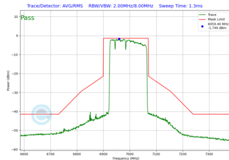
Plot 7-556 In-Band Emission Plot Antenna 1b (160MHz BW 802.11be(RU) RU996+484+242 Index96 (UNII Band 8) - Ch.207)
