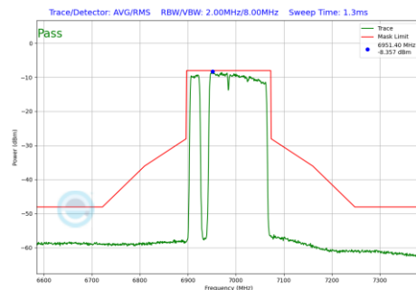
Plot 7-716 In-Band Emission Plot SDM Diversity Antenna 3c (160MHz BW 802.11be(RU) RU996+484+242 Index97 (UNII Band 8) - Ch.207)
