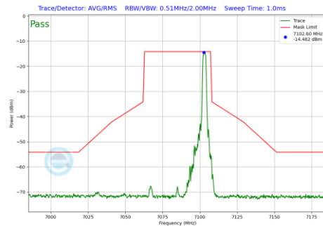
Plot 7-602 In-Band Emission Plot SDM Primary Antenna 3a (40MHz BW 802.11be(RU) RU26 Index17 (UNII Band 8) - Ch.227)
