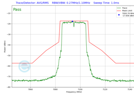
Plot 7-641 In-Band Emission Plot SDM Primary Antenna 3c (20MHz BW 802.11be(RU) RU242 Index61 (UNII Band 8) - Ch.229)
