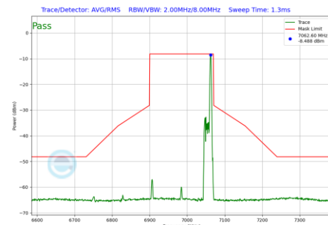
Plot 7-676 In-Band Emission Plot SDM Diversity Antenna 1b (160MHz BW 802.11be(RU) RU26 Index36 (UNII Band 8) - Ch.207)
