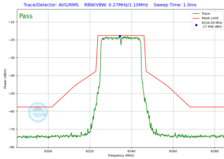
Plot 7-741 In-Band Emission Plot SDM Diversity Antenna 3c (20MHz BW 802.11be(RU) RU242 Index61 (UNII Band 7) - Ch.117)
