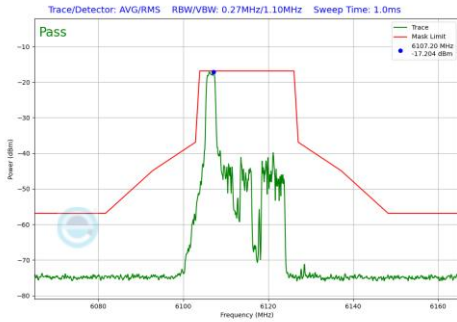
Plot 7-573 In-Band Emission Plot SDM Primary Antenna 3c (20MHz BW 802.11be(RU) RU26 Index0 (UNII Band 5) - Ch.33)
