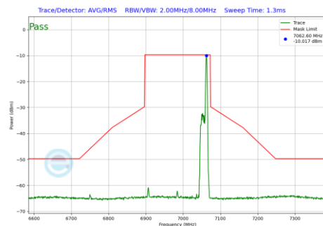
Plot 7-588 In-Band Emission Plot SDM Primary Antenna 3c (160MHz BW 802.11be(RU) RU26 Index36 (UNII Band 8) - Ch.207)
