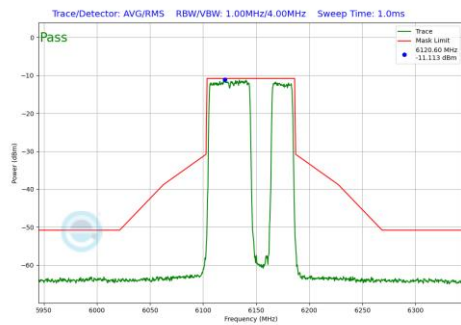
Plot 7-606 In-Band Emission Plot SDM Primary Antenna 3c (80MHz BW 802.11be(RU) RU484+242 Index92 (UNII Band 5) - Ch.39)
