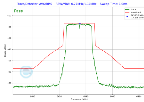
Plot 7-721 In-Band Emission Plot SDM Diversity Antenna 1b (20MHz BW 802.11be(RU) RU242 Index61 (UNII Band 6) - Ch.97)
