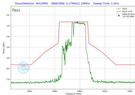
Plot 7-614 In-Band Emission Plot SDM Primary Antenna 3c (20MHz BW 802.11be(RU) RU106+26 Index83 (UNII Band 8) - Ch.189)
