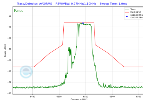
Plot 7-620 In-Band Emission Plot SDM Primary Antenna 3a (20MHz BW 802.11be(RU) RU106+26 Index83 (UNII Band 6) - Ch.113)
