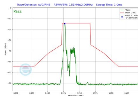
Plot 7-682 In-Band Emission Plot SDM Diversity Antenna 3c (40MHz BW 802.11be(RU) RU26 Index0 (UNII Band 6) - Ch.99)
