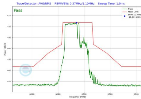
Plot 7-699 In-Band Emission Plot SDM Diversity Antenna 1b (20MHz BW 802.11be(RU) RU106+26 Index82 (UNII Band 7) - Ch.149)
