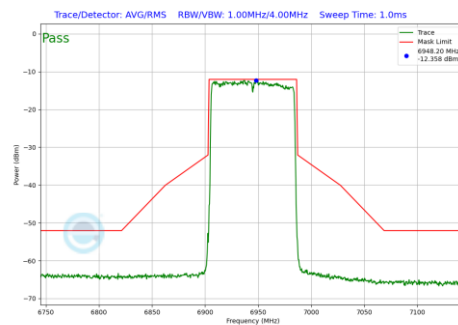
Plot 7-643 In-Band Emission Plot SDM Primary Antenna 3c (80MHz BW 802.11be(RU) RU996 Index67 (UNII Band 8) - Ch.199)
