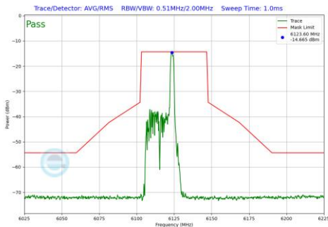
Plot 7-590 In-Band Emission Plot SDM Primary Antenna 3a (40MHz BW 802.11be(RU) RU26 Index8 (UNII Band 5) - Ch.35)
