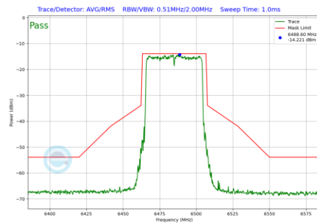
Plot 7-722 In-Band Emission Plot SDM Diversity Antenna 1b (40MHz BW 802.11be(RU) RU484 Index65 (UNII Band 6) - Ch.107)
