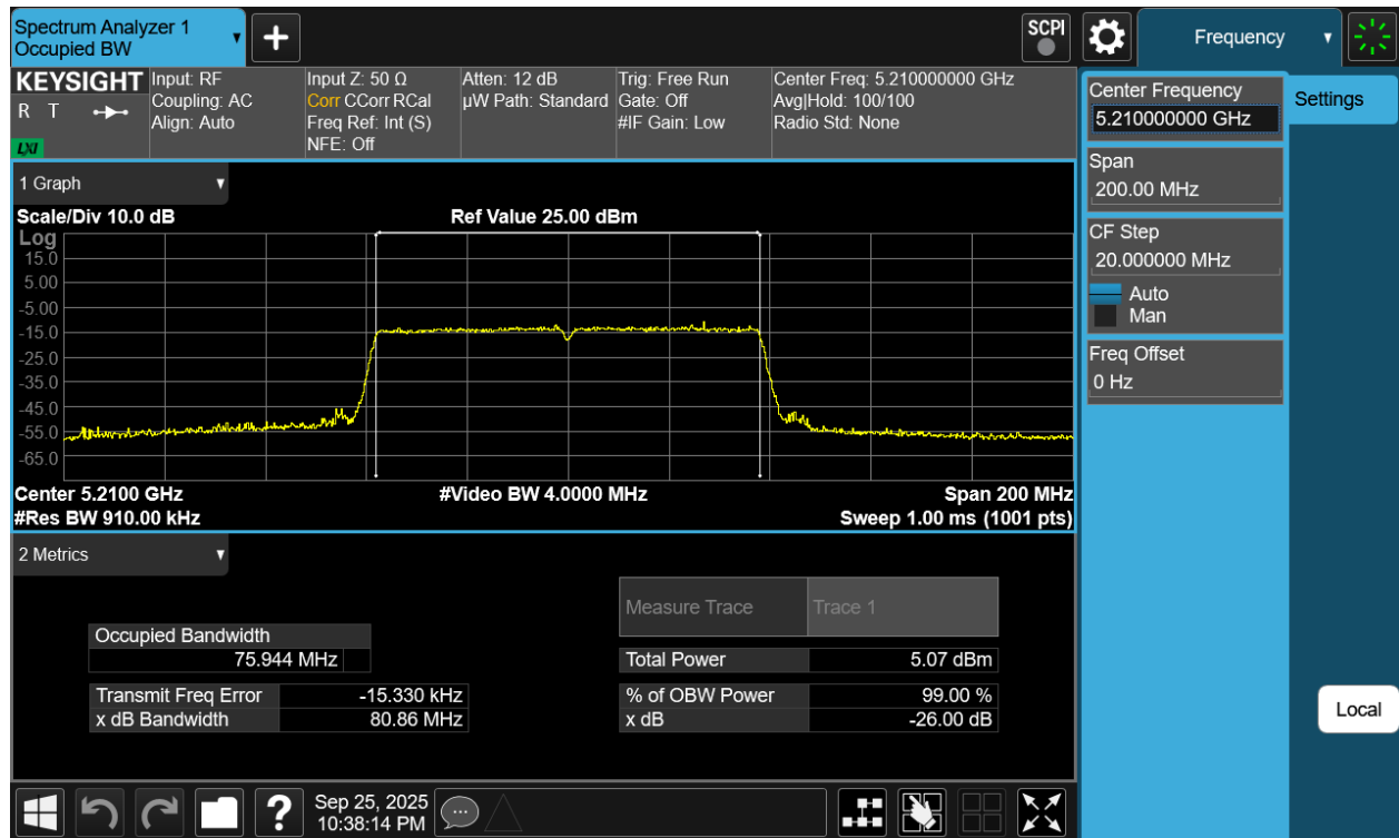
Plot 7-3 26dB BW & 99% OBW Antenna 3c (80MHz BW 802.11ac - Ch.42)
