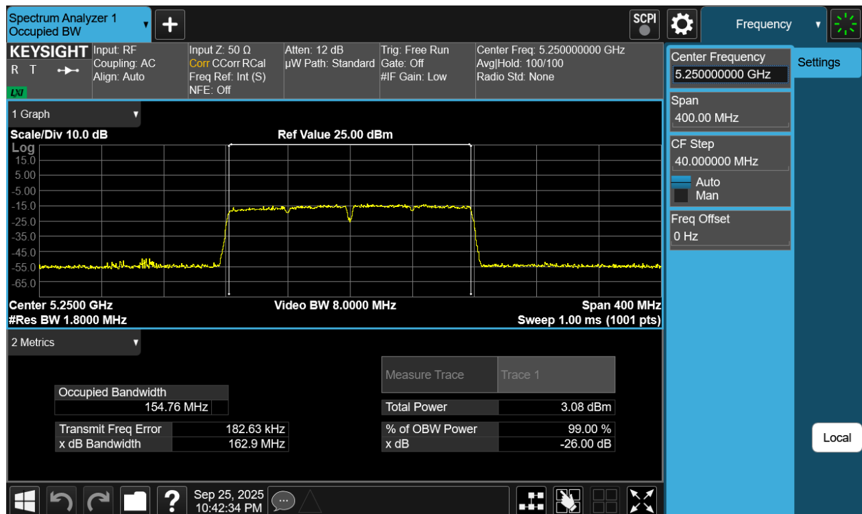
Plot 7-4 26dB BW & 99% OBW Antenna 3c (160MHz BW 802.11ac - Ch.50)
