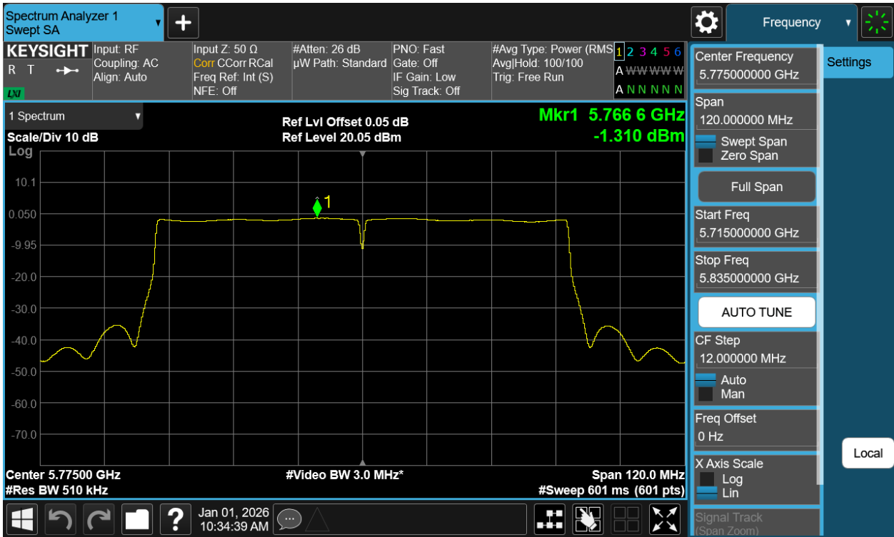
Plot 7-28 PSD Antenna 3c (80MHz BW 802.11ac - Ch.155)
