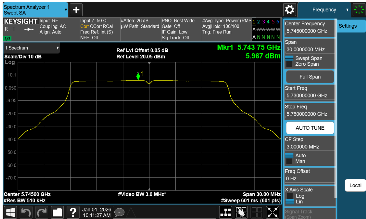
Plot 7-26 PSD Antenna 3c (20MHz BW 802.11n - Ch.149)
