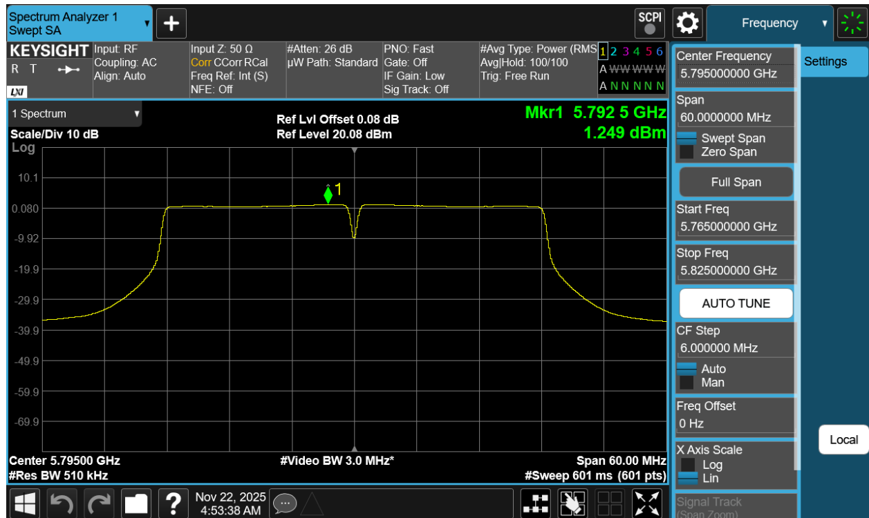
Plot 7-38 PSD Antenna 3a (40MHz BW 802.11n - Ch.159)
