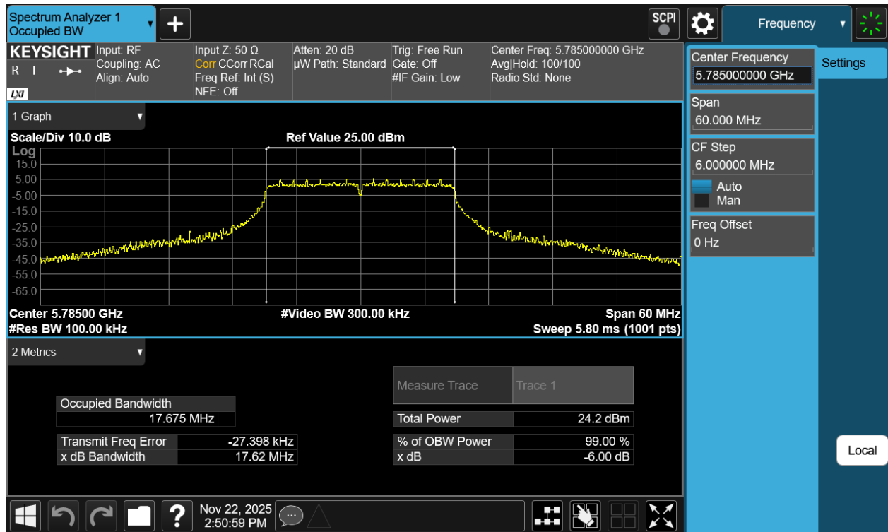
Plot 7-19 6dB OBW Antenna 1b (20MHz BW 802.11a - Ch.157)
