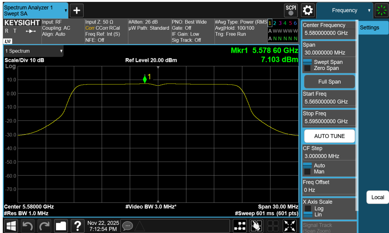
Plot 7-44 PSD Antenna 1b (20MHz BW 802.11a - Ch.116)
