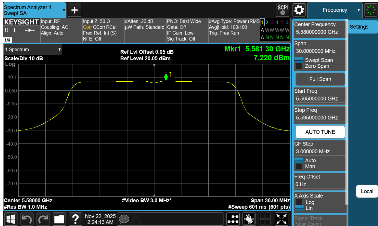
Plot 7-33 PSD Antenna 3a (20MHz BW 802.11a - Ch.116)
