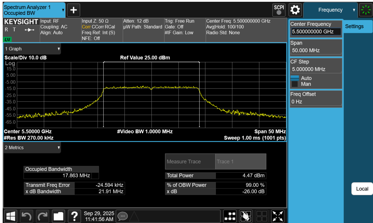
Plot 7-5 26dB BW & 99% OBW Antenna 3a (20MHz BW 802.11n - Ch.100)
