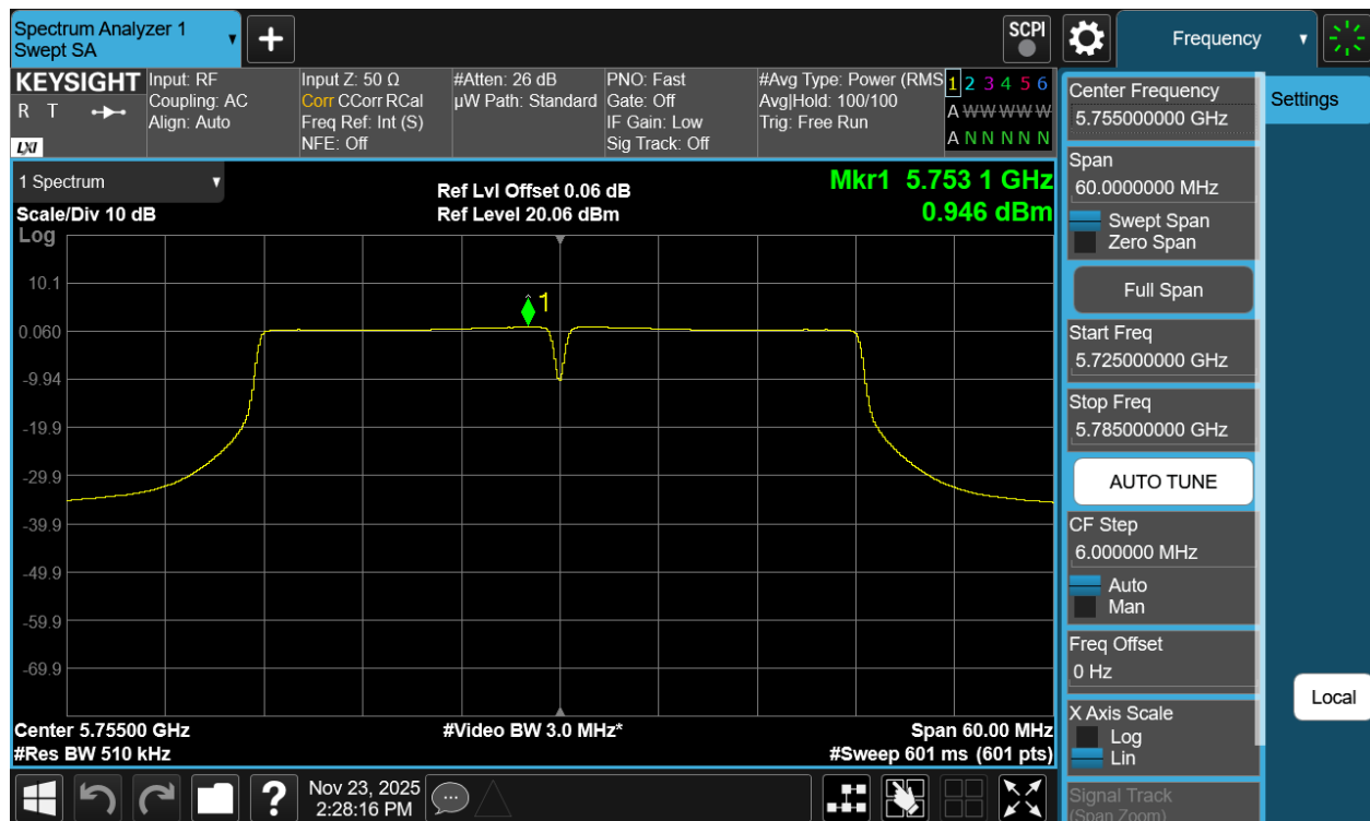
Plot 7-49 PSD Antenna 1b (40MHz BW 802.11n - Ch.151)
