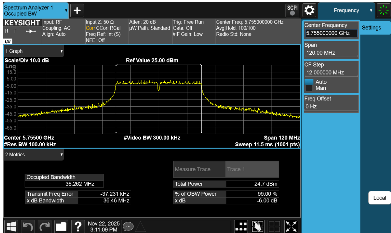
Plot 7-20 6dB OBW Antenna 1b (40MHz BW 802.11n - Ch.151)
