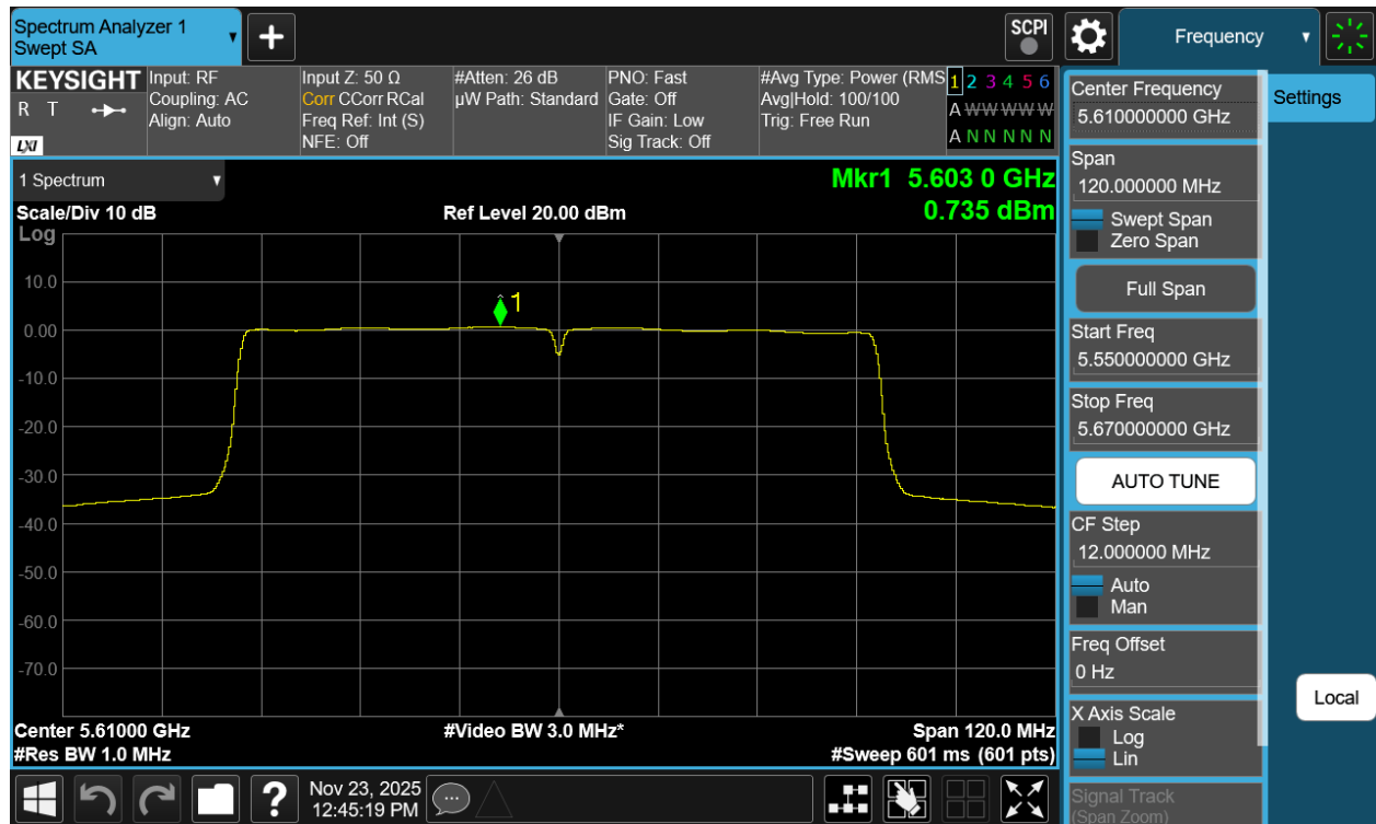
Plot 7-46 PSD Antenna 1b (80MHz BW 802.11ac - Ch.122)
