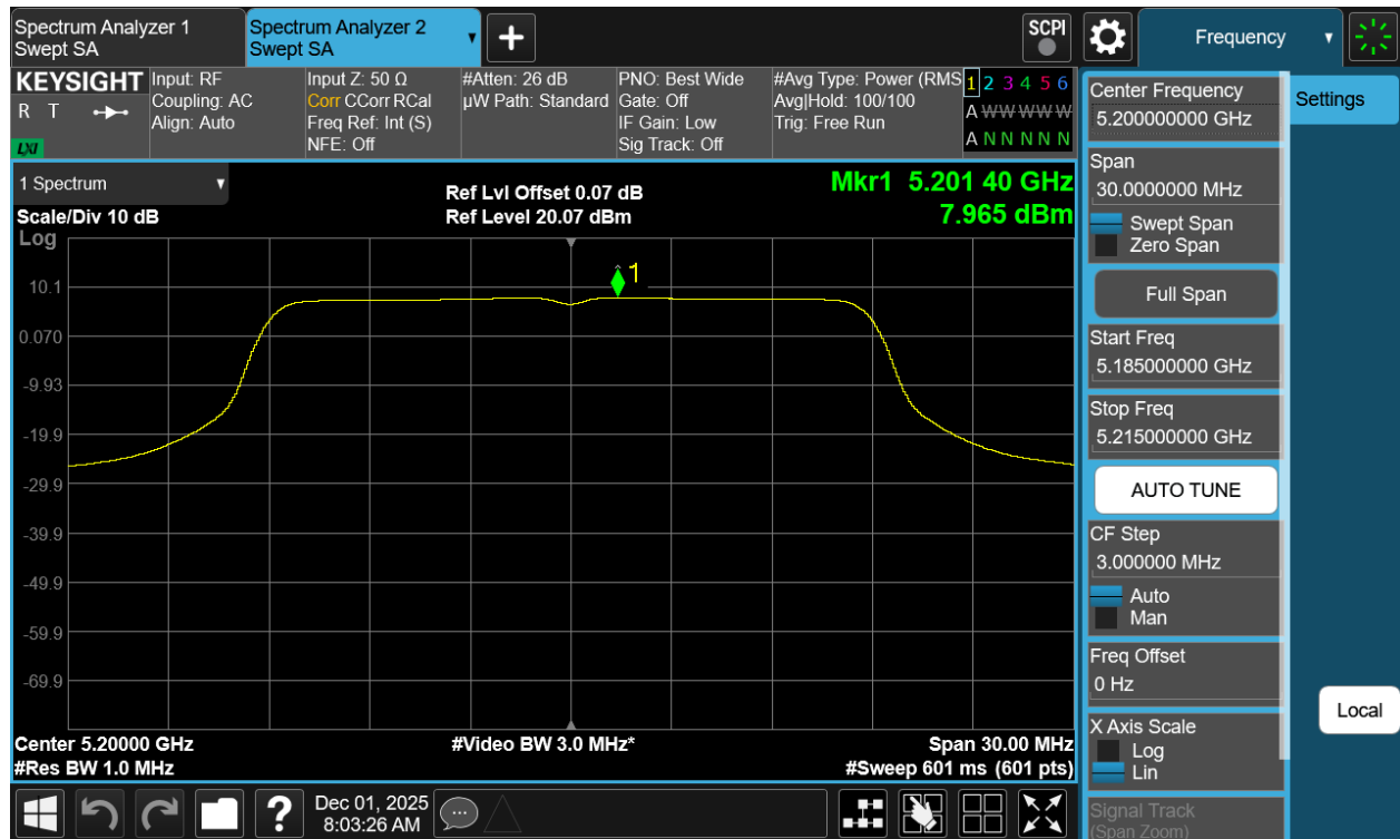
Plot 7-29 PSD Antenna 3c (20MHz BW 802.11a - Ch.40)
