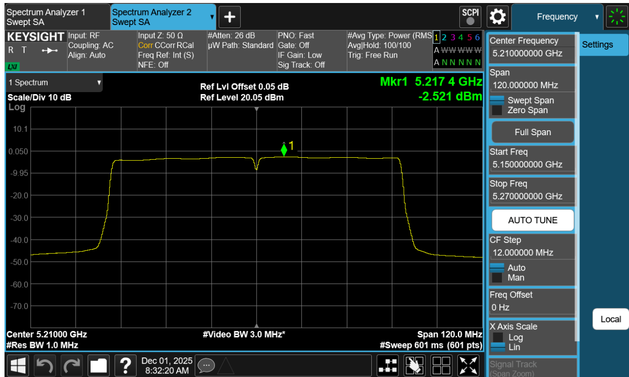
Plot 7-31 PSD Antenna 3c (80MHz BW 802.11ac - Ch.42)
