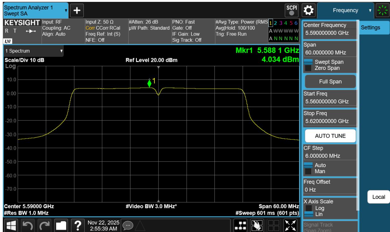
Plot 7-34 PSD Antenna 3a (40MHz BW 802.11n - Ch.118)
