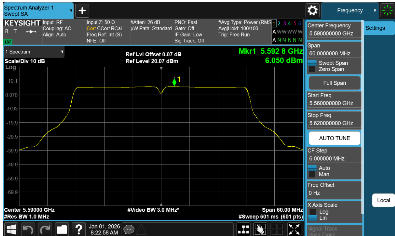
Plot 7-23 PSD Antenna 3c (40MHz BW 802.11n - Ch.118)
