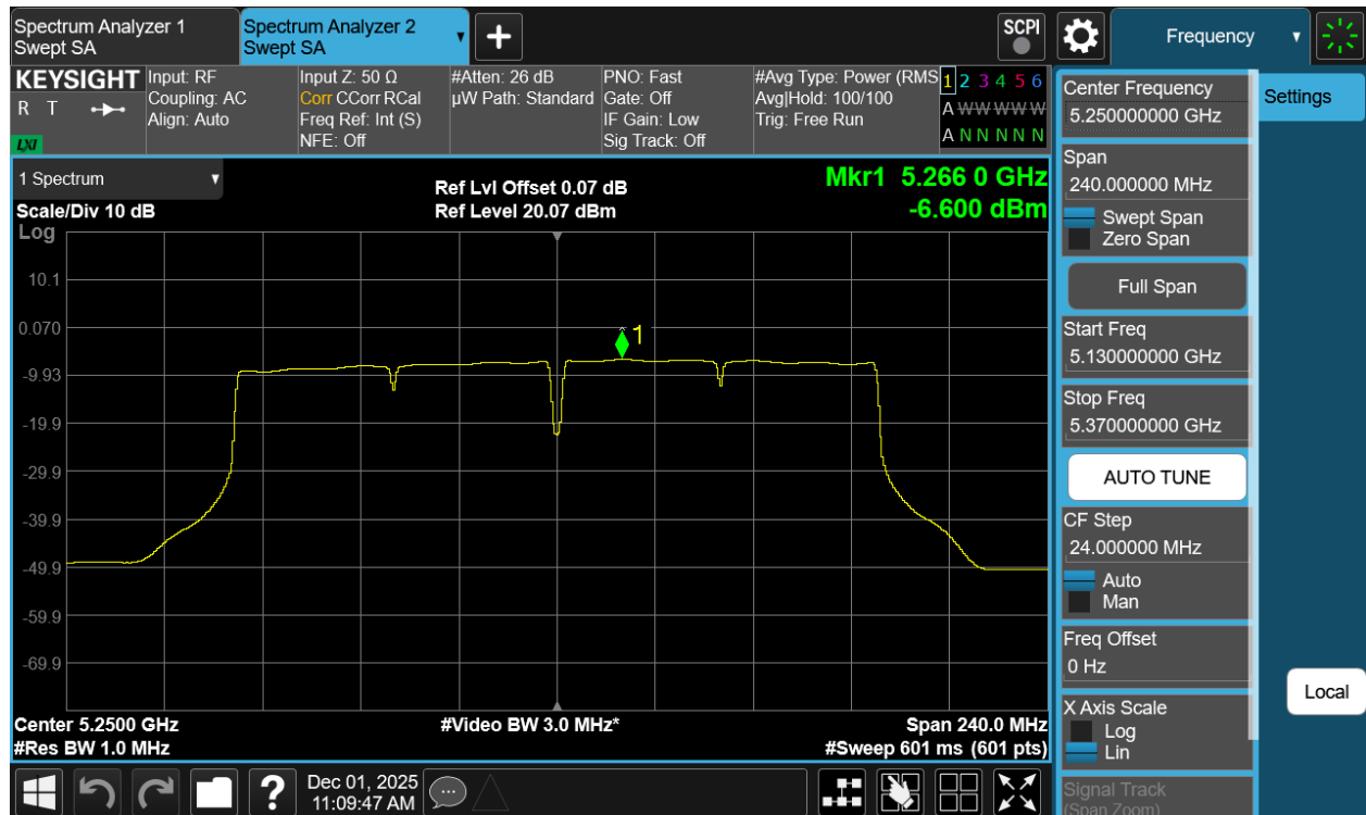
Plot 7-43 PSD Antenna 3a (160MHz BW 802.11ac - Ch.50)
