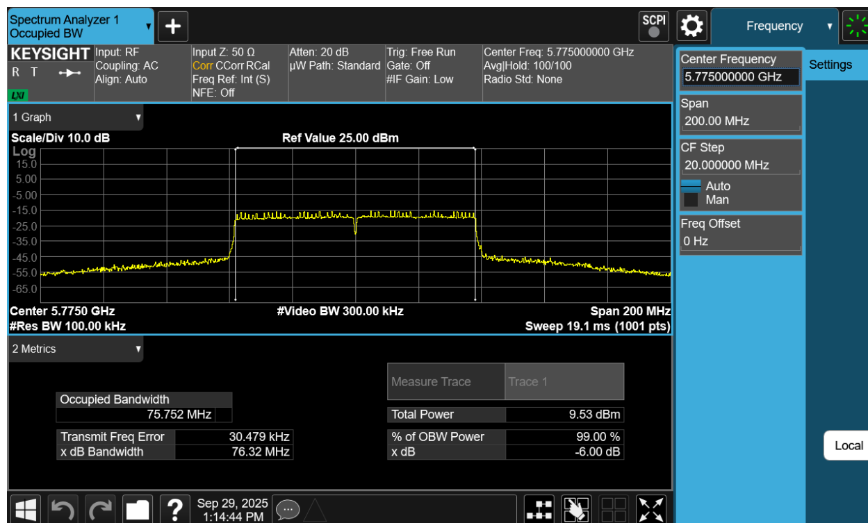
Plot 7-18 6dB OBW Antenna 3a (80MHz BW 802.11ac - Ch.155)
