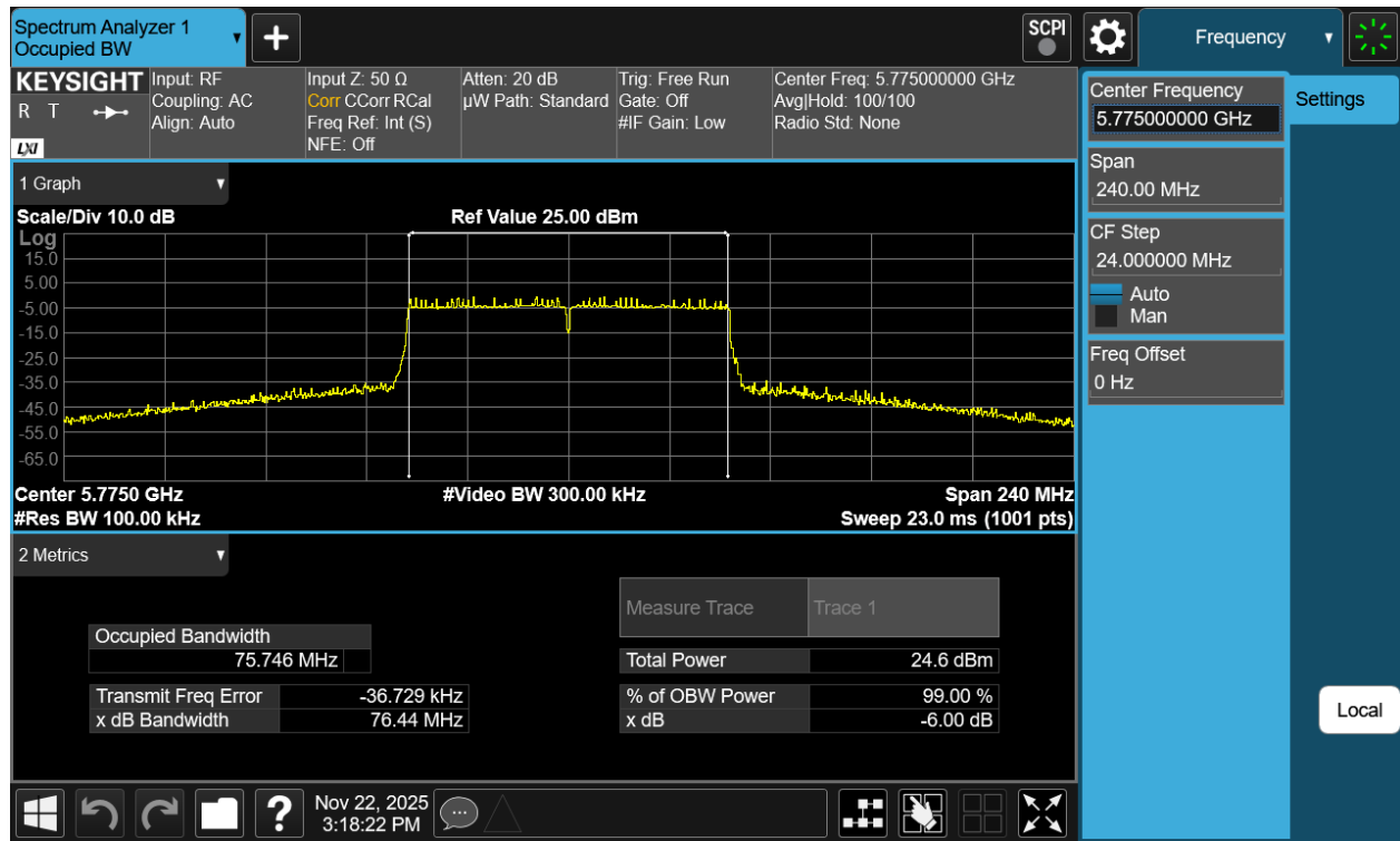
Plot 7-21 6dB OBW Antenna 1b (80MHz BW 802.11ac - Ch.155)
