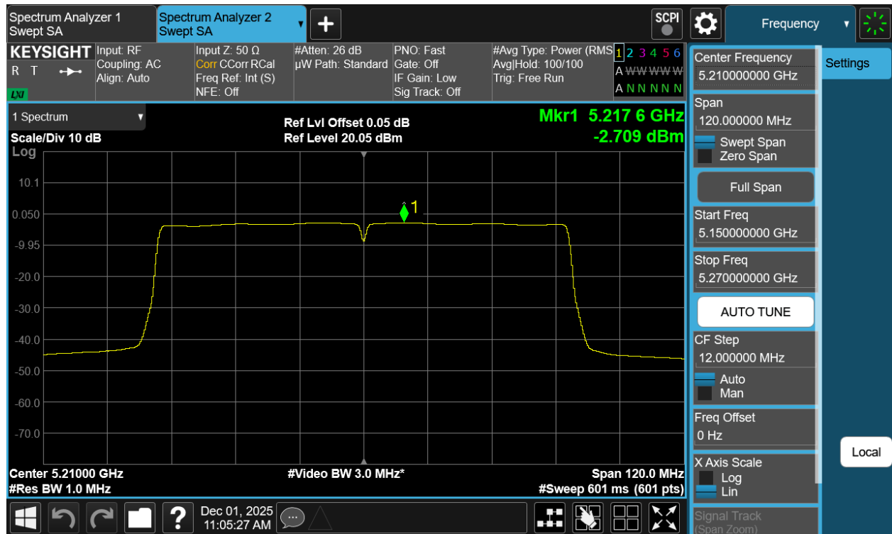
Plot 7-42 PSD Antenna 3a (80MHz BW 802.11ac - Ch.42)
