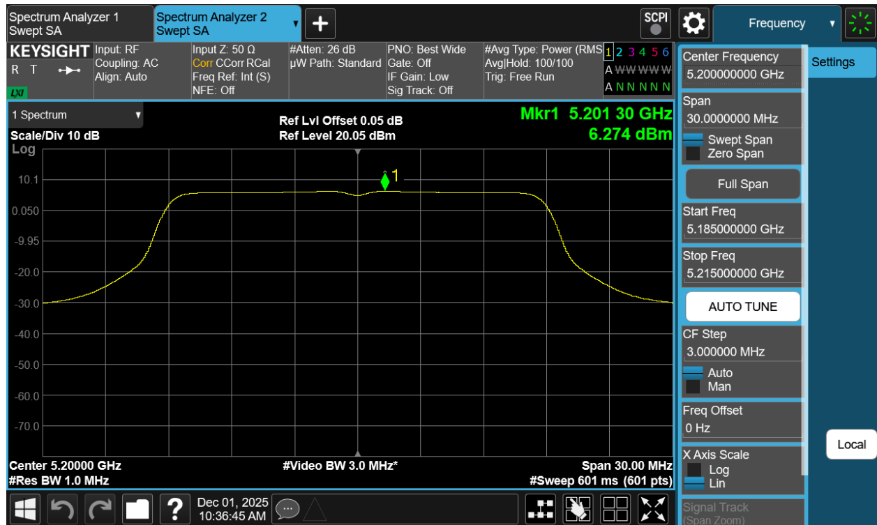
Plot 7-40 PSD Antenna 3a (20MHz BW 802.11a - Ch.40)
