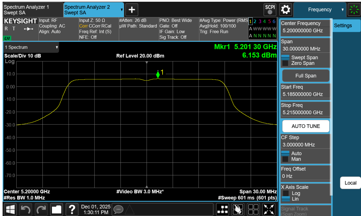
Plot 7-51 PSD Antenna 1b (20MHz BW 802.11a - Ch.40)
