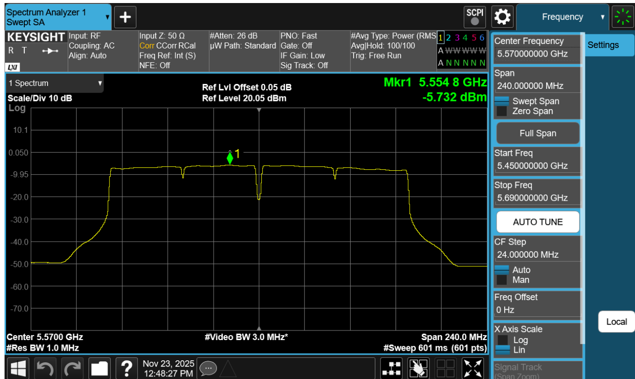
Plot 7-47 PSD Antenna 1b (160MHz BW 802.11ac - Ch.114)
