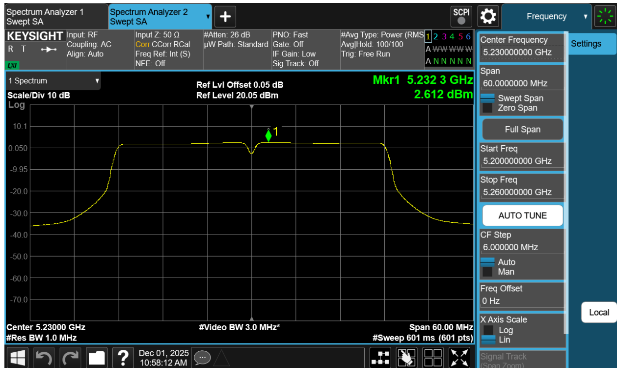
Plot 7-41 PSD Antenna 3a (40MHz BW 802.11n - Ch.46)
