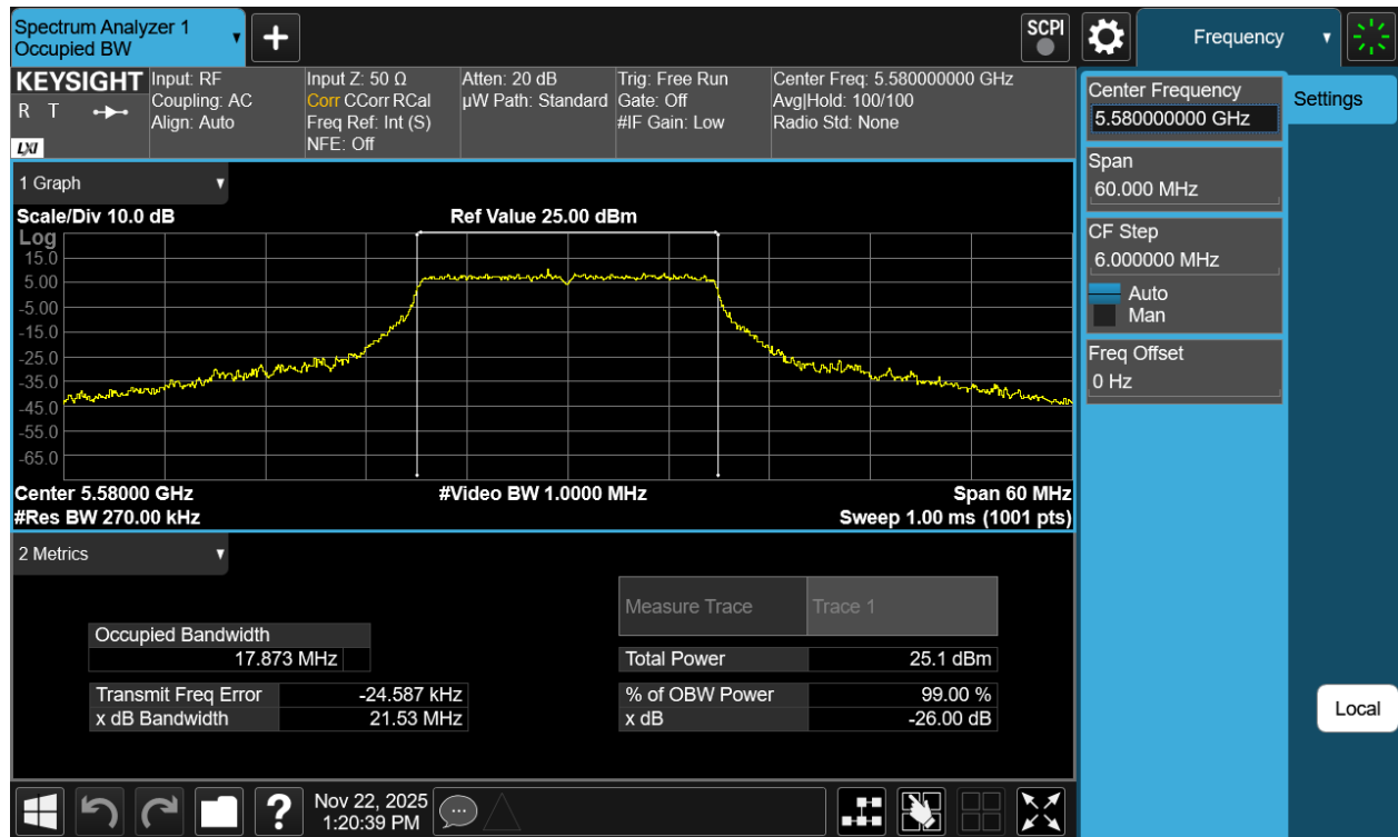
Plot 7-9 26dB BW & 99% OBW Antenna 1b (20MHz BW 802.11a - Ch.116)
