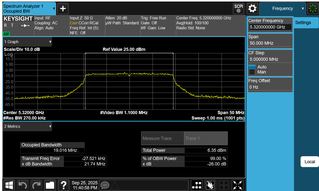
Plot 7-1 26dB BW & 99% OBW Antenna 3c (20MHz BW 802.11be(SU) - Ch.64)
