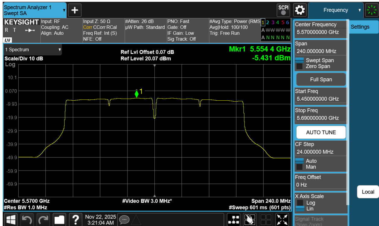
Plot 7-36 PSD Antenna 3a (160MHz BW 802.11ac - Ch.114)
