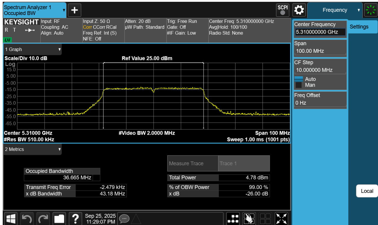
Plot 7-2 26dB BW & 99% OBW Antenna 3c (40MHz BW 802.11n - Ch.62)
