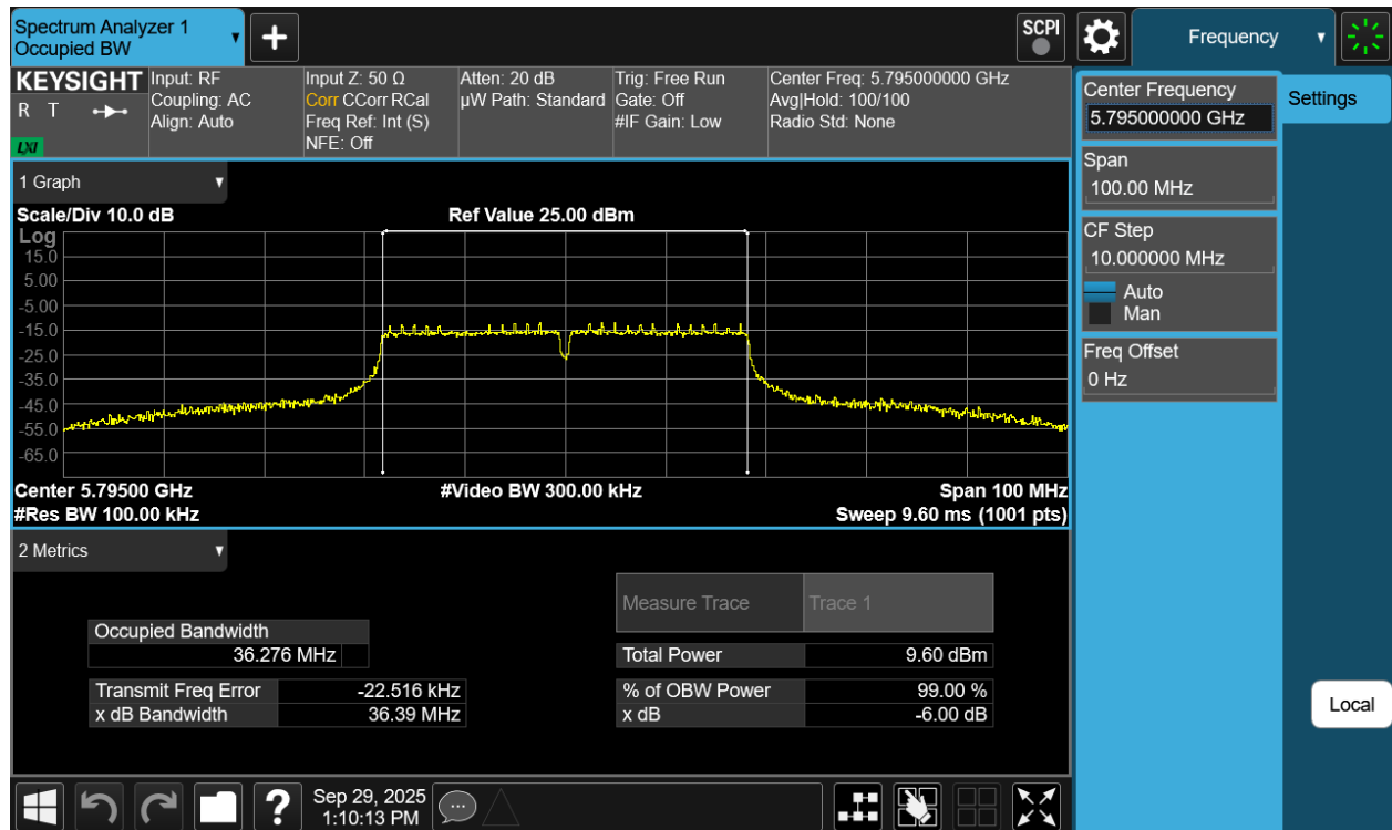
Plot 7-17 6dB OBW Antenna 3a (40MHz BW 802.11n - Ch.159)
