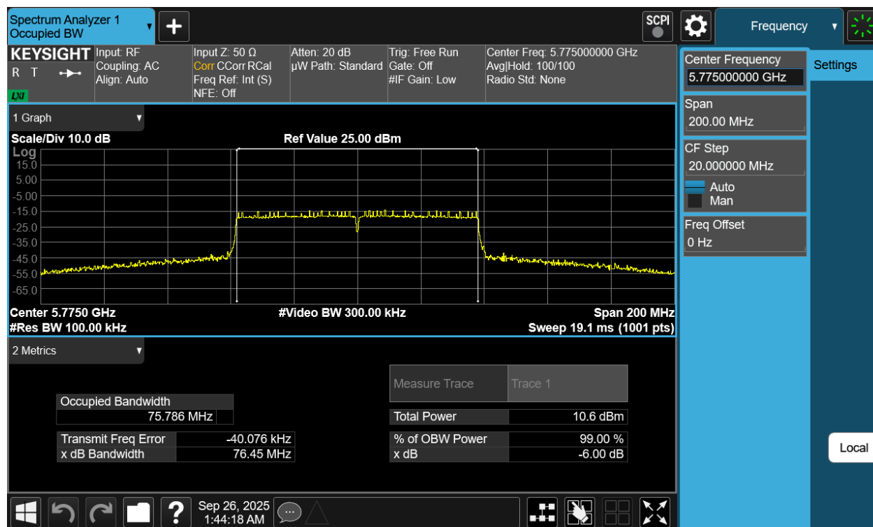
Plot 7-15 6dB OBW Antenna 3c (80MHz BW 802.11ac - Ch.155)
