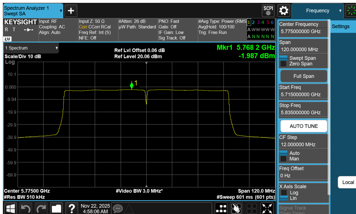
Plot 7-39 PSD Antenna 3a (80MHz BW 802.11ac - Ch.155)
