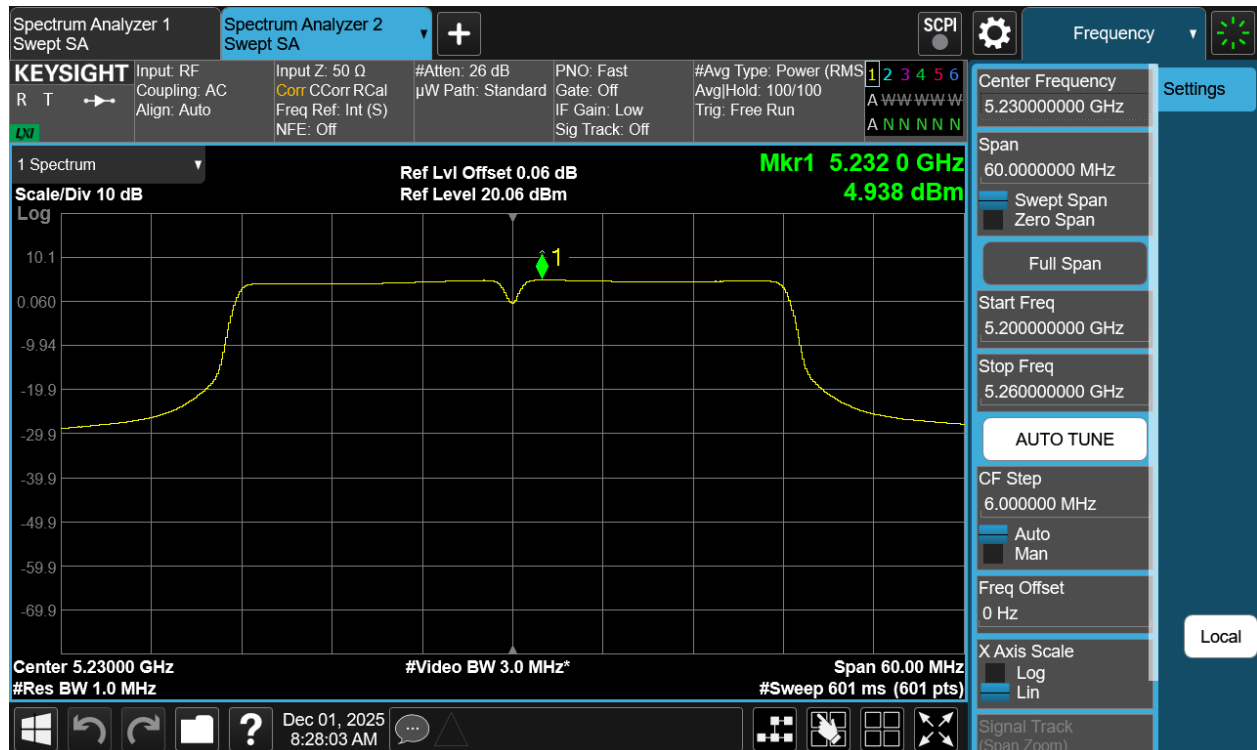
Plot 7-30 PSD Antenna 3c (40MHz BW 802.11n - Ch.46)
