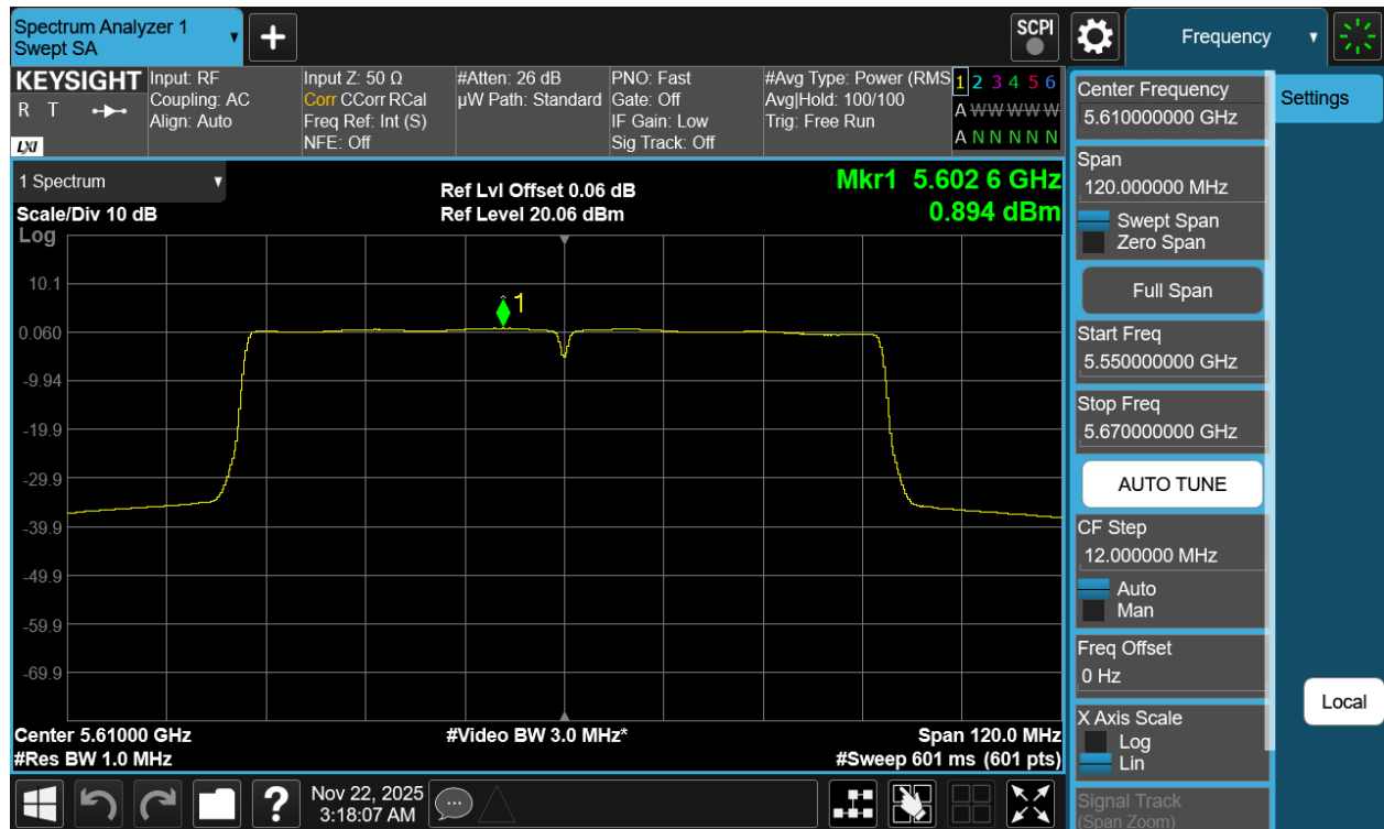
Plot 7-35 PSD Antenna 3a (80MHz BW 802.11ac - Ch.122)
