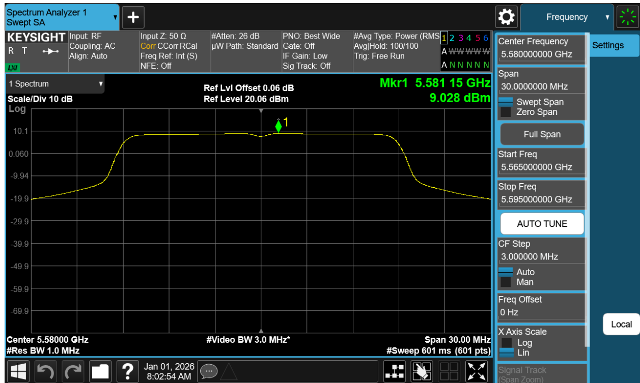
Plot 7-22 PSD Antenna 3c (20MHz BW 802.11a - Ch.116)
