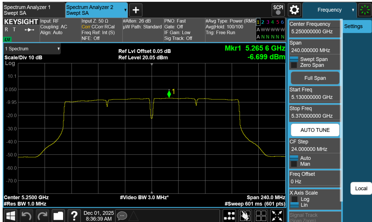
Plot 7-32 PSD Antenna 3c (160MHz BW 802.11ac - Ch.50)
