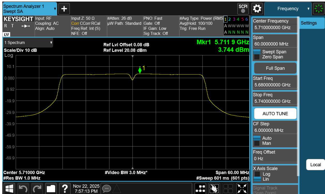
Plot 7-45 PSD Antenna 1b (40MHz BW 802.11n - Ch.142)
