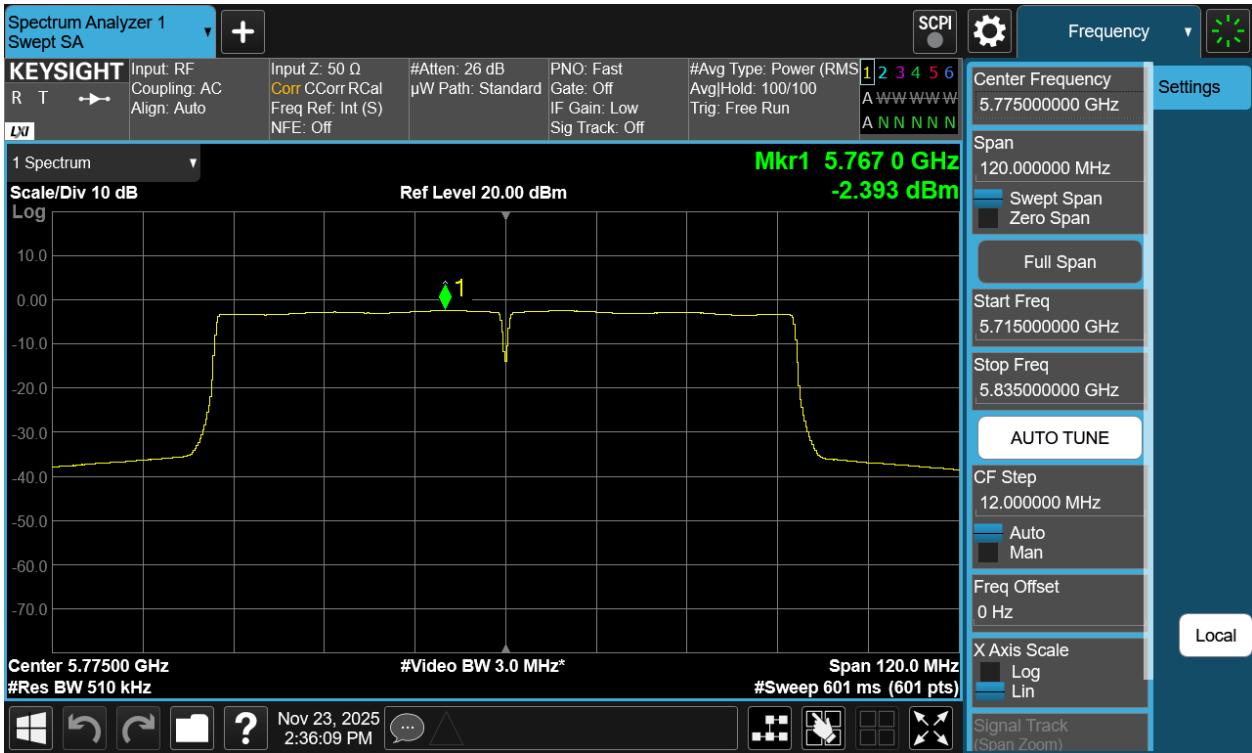
Plot 7-50 PSD Antenna 1b (80MHz BW 802.11ac - Ch.155)
