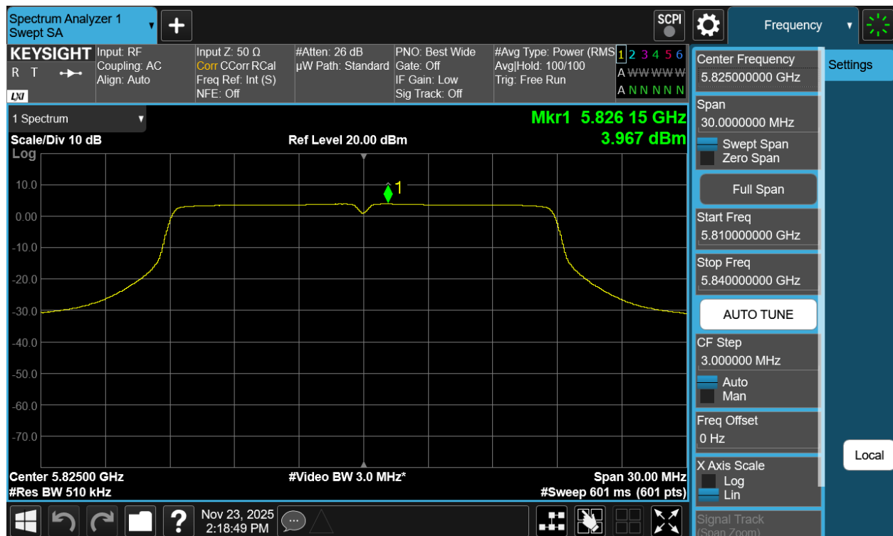
Plot 7-48 PSD Antenna 1b (20MHz BW 802.11n - Ch.165)
