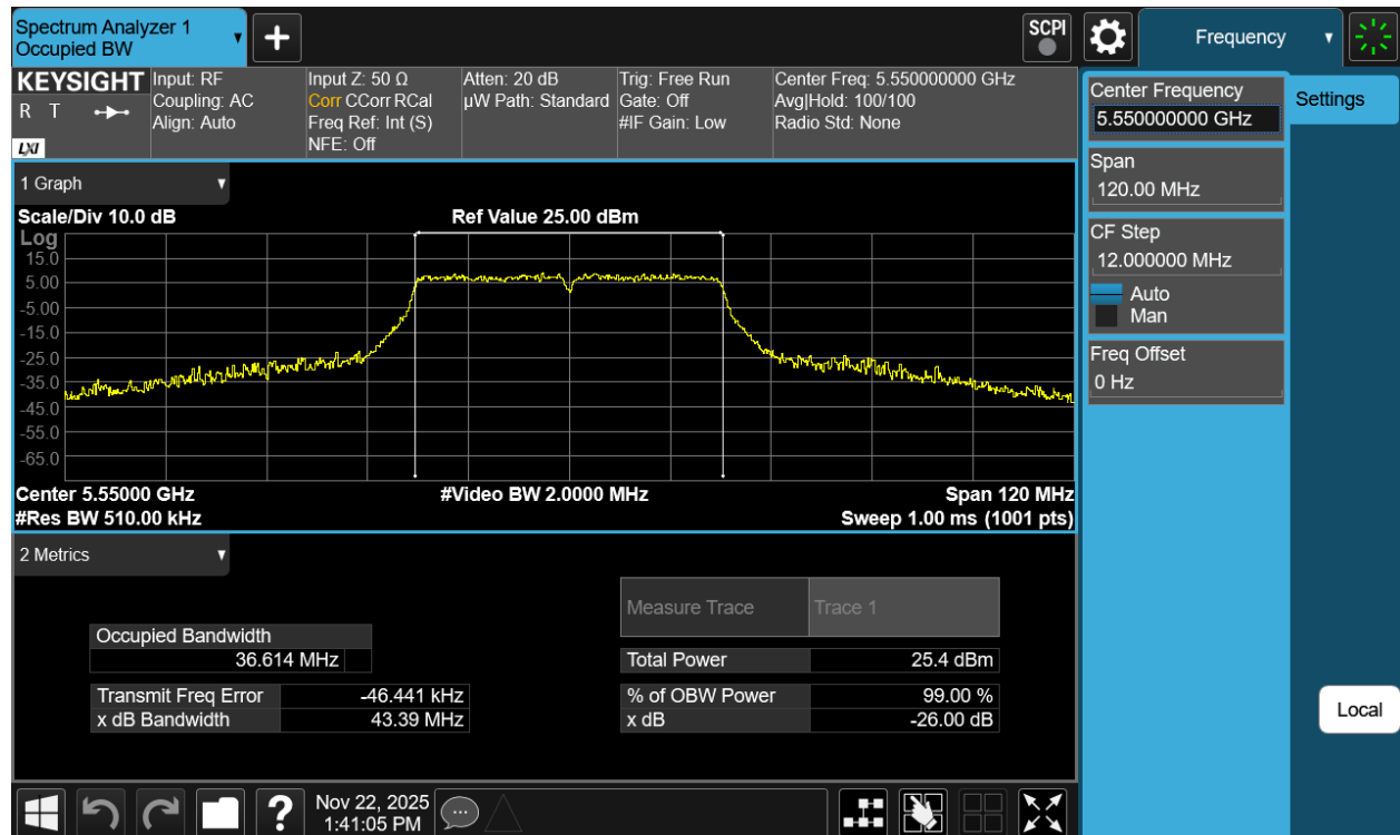
Plot 7-10 26dB BW & 99% OBW Antenna 1b (40MHz BW 802.11n - Ch.110)
