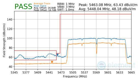
Plot 7-230. Antenna 3c (Peak & Average, Ch.114, 802.11ac, MCS9)
