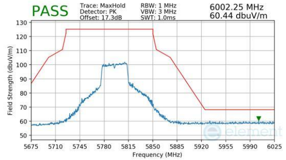
Plot 7-266. Antenna 3a (Peak, Ch.159, 802.11n, MCS7)
