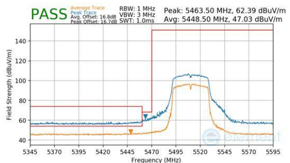
Plot 7-324. Antenna 1b (Peak & Average, Ch.102, 802.11n, MCS7)
