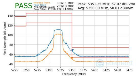
Plot 7-302. Antenna 1b (Peak & Average, Ch.64, 802.11n, MCS7)
