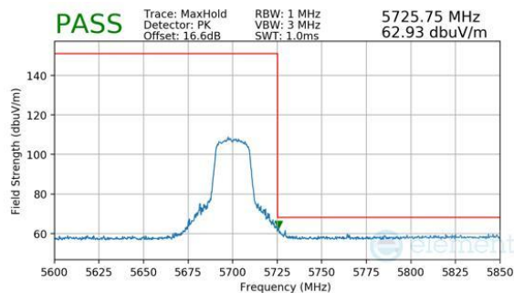
Plot 7-317. Antenna 1b (Peak, Ch.140, 802.11be(SU), MCS11)
