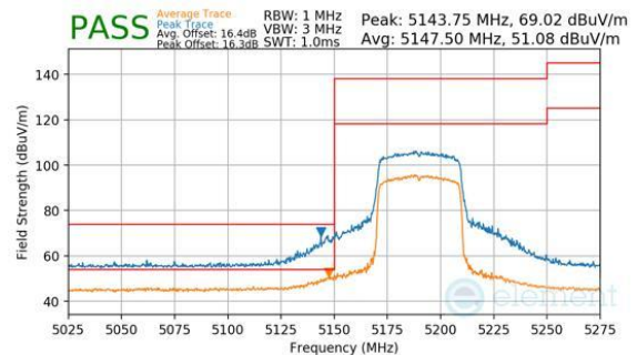
Plot 7-330. Antenna 1b (Peak & Average, Ch.38, 802.11be(SU), MCS11)
