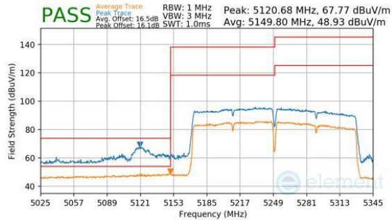
Plot 7-354. Antenna 1b (Peak & Average, Ch.50, 802.11ac, MCS9)
