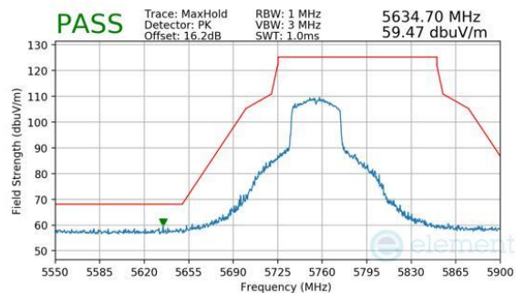
Plot 7-338. Antenna 1b (Peak, Ch.151, 802.11be(SU), MCS11)
