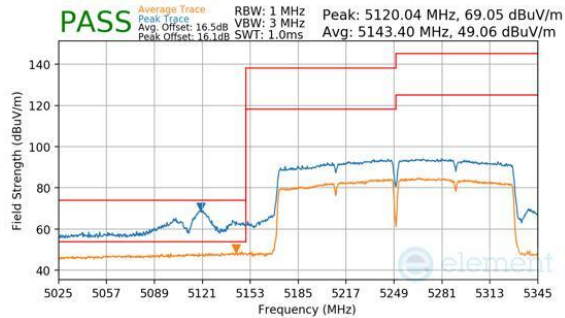
Plot 7-291. Antenna 3a (Peak & Average, Ch.50, 802.11ac, MCS9)
