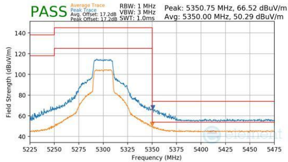
Plot 7-311. Antenna 1b (Peak & Average, Ch.60, 802.11be(SU), MCS11)
