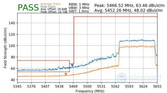
Plot 7-224. Antenna 3c (Peak & Average, Ch.122, 802.11be(SU), MCS11)
