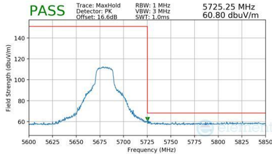
Plot 7-305. Antenna 1b (Peak, Ch.136, 802.11n, MCS7)
