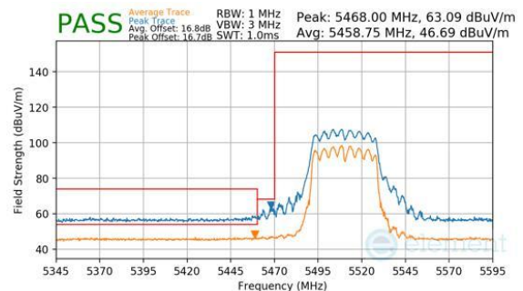
Plot 7-390. CDD Primary (Peak & Average, Ch.102, 802.11n, MCS7)
