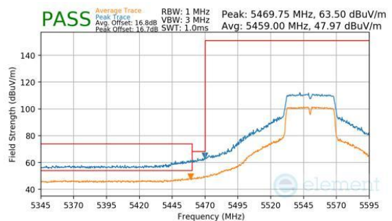
Plot 7-325. Antenna 1b (Peak & Average, Ch.110, 802.11n, MCS7)
