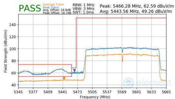
Plot 7-234. Antenna 3c (Peak & Average, Ch.114, 802.11be(SU), MCS11)
