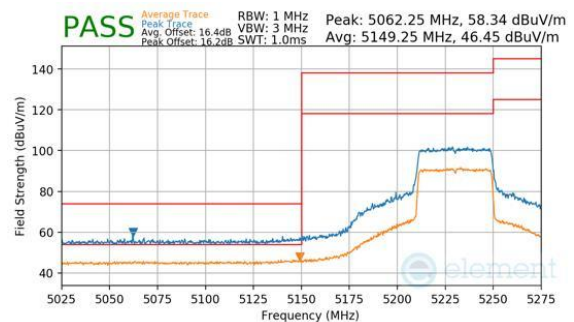
Plot 7-268. Antenna 3a (Peak & Average, Ch.46, 802.11be(SU), MCS11)
