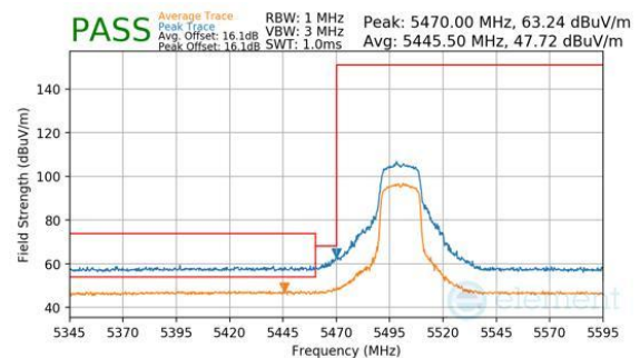
Plot 7-240. Antenna 3a (Peak & Average, Ch.100, 802.11n, MCS7)
