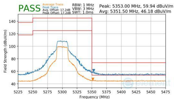
Plot 7-238. Antenna 3a (Peak & Average, Ch.60, 802.11n, MCS7)
