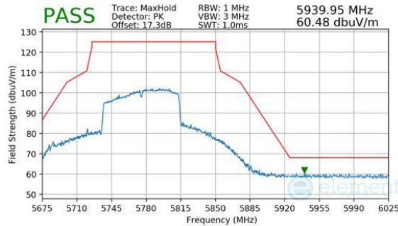
Plot 7-283. Antenna 3a (Peak, Ch.155, 802.11ac, MCS9)
