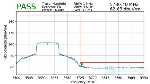
Plot 7-281. Antenna 3a (Peak, Ch.122, 802.11ac, MCS9)
