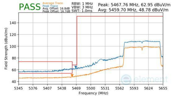
Plot 7-217. Antenna 3c (Peak & Average, Ch.122, 802.11ac, MCS9)
