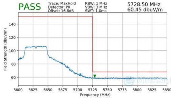
Plot 7-263. Antenna 3a (Peak, Ch.126, 802.11n, MCS7)
