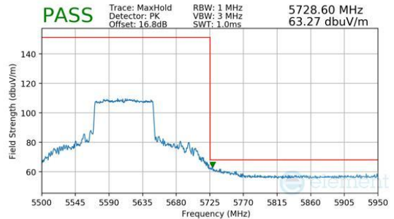
Plot 7-225. Antenna 3c (Peak, Ch.122, 802.11be(SU), MCS11)
