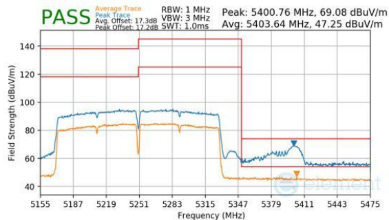
Plot 7-292. Antenna 3a (Peak & Average, Ch.50, 802.11ac, MCS9)
