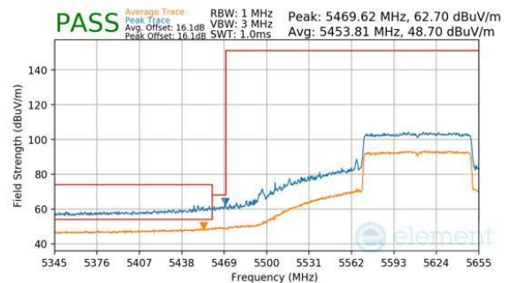
Plot 7-287. Antenna 3a (Peak & Average, Ch.122, 802.11be(SU), MCS11)
