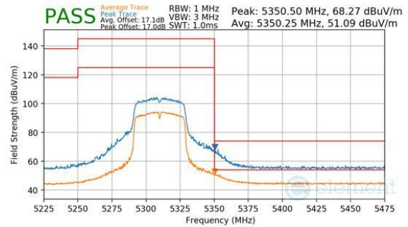
Plot 7-260. Antenna 3a (Peak & Average, Ch.62, 802.11n, MCS7)
