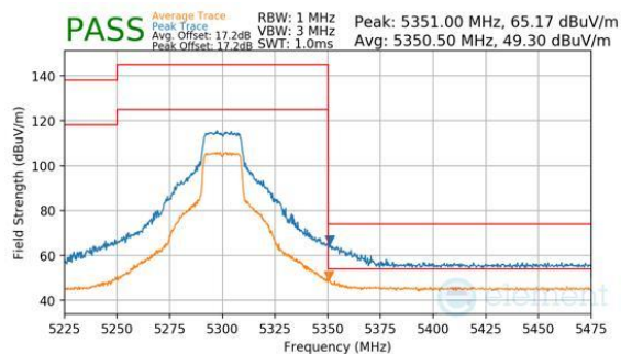
Plot 7-301. Antenna 1b (Peak & Average, Ch.60, 802.11n, MCS7)
