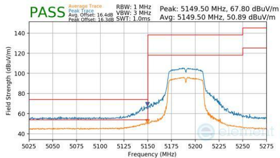
Plot 7-320. Antenna 1b (Peak & Average, Ch.38, 802.11n, MCS7)
