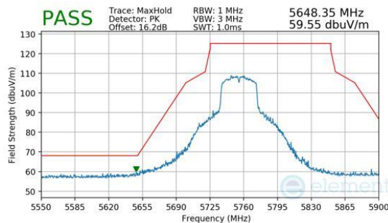
Plot 7-328. Antenna 1b (Peak, Ch.151, 802.11n, MCS7)
