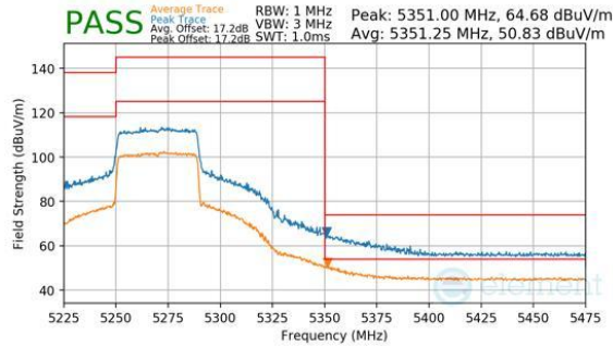
Plot 7-332. Antenna 1b (Peak & Average, Ch.54, 802.11be(SU), MCS11)
