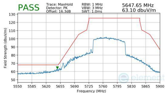
Plot 7-289. Antenna 3a (Peak, Ch.155, 802.11be(SU), MCS11)
