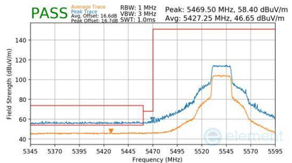
Plot 7-315. Antenna 1b (Peak & Average, Ch.108, 802.11be(SU), MCS11)
