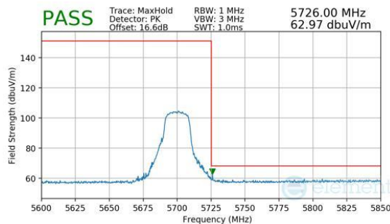
Plot 7-243. Antenna 3a (Peak, Ch.140, 802.11n, MCS7)
