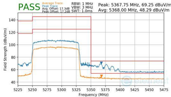
Plot 7-222. Antenna 3c (Peak & Average, Ch.58, 802.11be(SU), MCS11)
