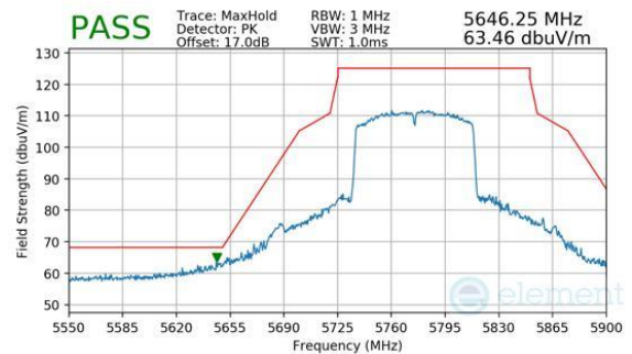
Plot 7-219. Antenna 3c (Peak, Ch.155, 802.11ac, MCS9)
