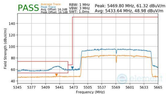
Plot 7-297. Antenna 3a (Peak & Average, Ch.114, 802.11be(SU), MCS11)
