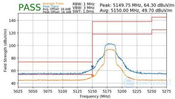
Plot 7-236. Antenna 3a (Peak & Average, Ch.36, 802.11n, MCS7)
