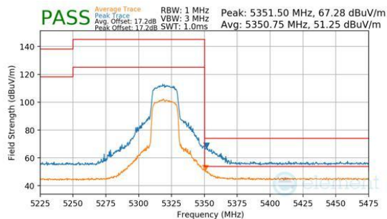
Plot 7-312. Antenna 1b (Peak & Average, Ch.64, 802.11be(SU), MCS11)
