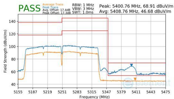
Plot 7-229. Antenna 3c (Peak & Average, Ch.50, 802.11ac, MCS9)
