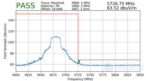
Plot 7-253. Antenna 3a (Peak, Ch.136, 802.11be(SU), MCS11)
