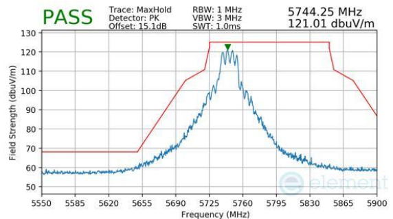
Plot 7-384. CDD Primary (Peak, Ch.149, 802.11be(SU), MCS11)
