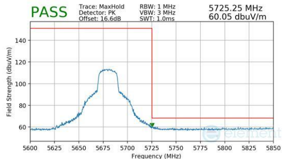
Plot 7-316. Antenna 1b (Peak, Ch.136, 802.11be(SU), MCS11)
