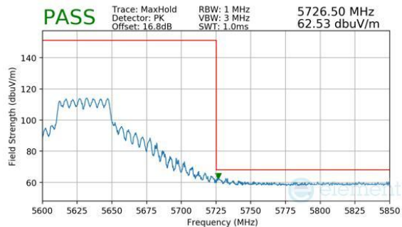
Plot 7-393. CDD Primary (Peak, Ch.126, 802.11n, MCS7)
