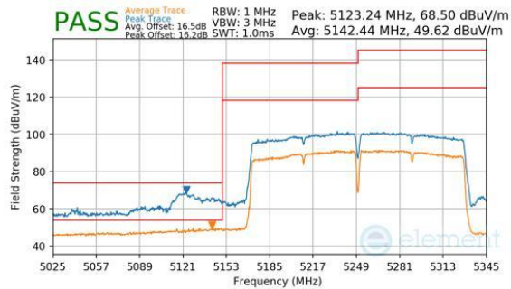
Plot 7-228. Antenna 3c (Peak & Average, Ch.50, 802.11ac, MCS9)
