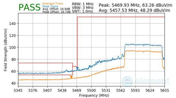
Plot 7-350. Antenna 1b (Peak & Average, Ch.122, 802.11be(SU), MCS11)
