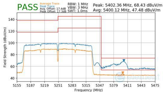
Plot 7-355. Antenna 1b (Peak & Average, Ch.50, 802.11ac, MCS9)
