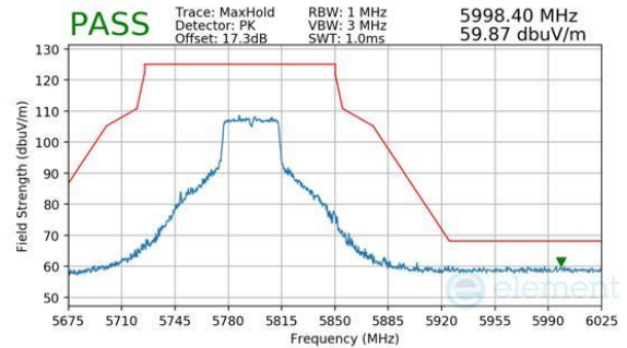
Plot 7-329. Antenna 1b (Peak, Ch.159, 802.11n, MCS7)
