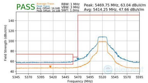
Plot 7-241. Antenna 3a (Peak & Average, Ch.104, 802.11n, MCS7)
