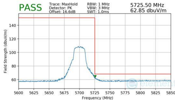
Plot 7-306. Antenna 1b (Peak, Ch.140, 802.11n, MCS7)
