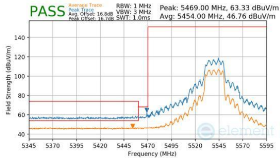
Plot 7-380. CDD Primary (Peak & Average, Ch.108, 802.11be(SU), MCS11)
