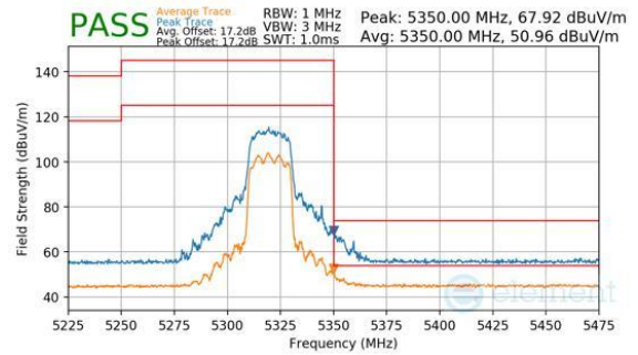
Plot 7-377. CDD Primary (Peak & Average, Ch.64, 802.11be(SU), MCS11)
