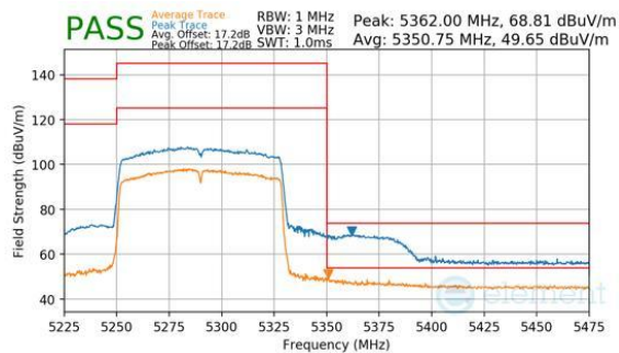
Plot 7-215. Antenna 3c (Peak & Average, Ch.58, 802.11ac, MCS9)
