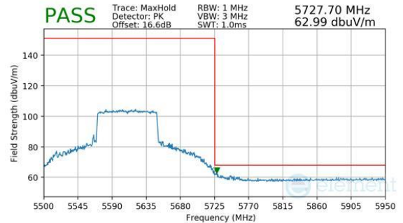
Plot 7-288. Antenna 3a (Peak, Ch.122, 802.11be(SU), MCS11)
