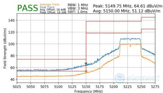
Plot 7-321. Antenna 1b (Peak & Average, Ch.46, 802.11n, MCS7)
