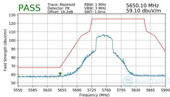
Plot 7-275. Antenna 3a (Peak, Ch.151, 802.11be(SU), MCS11)
