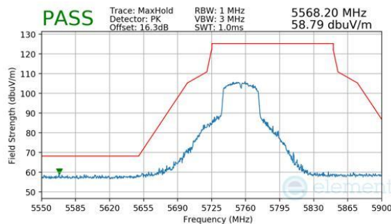
Plot 7-265. Antenna 3a (Peak, Ch.151, 802.11n, MCS7)
