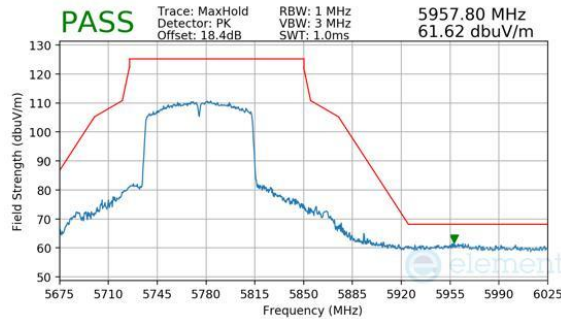
Plot 7-220. Antenna 3c (Peak, Ch.155, 802.11ac, MCS9)
