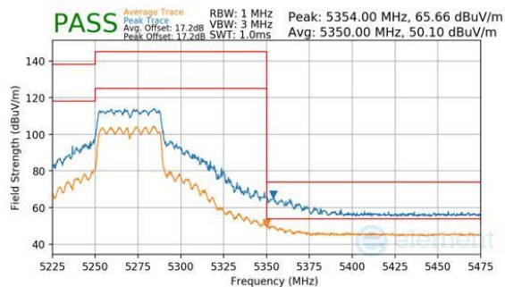
Plot 7-388. CDD Primary (Peak & Average, Ch.54, 802.11n, MCS7)
