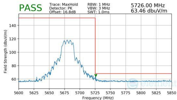
Plot 7-382. CDD Primary (Peak, Ch.136, 802.11be(SU), MCS11)
