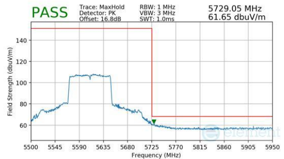
Plot 7-218. Antenna 3c (Peak, Ch.122, 802.11ac, MCS9)
