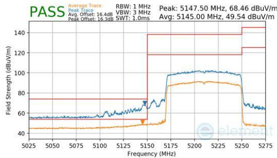
Plot 7-347. Antenna 1b (Peak & Average, Ch.42, 802.11be(SU), MCS11)
