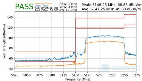
Plot 7-221. Antenna 3c (Peak & Average, Ch.42, 802.11be(SU), MCS11)
