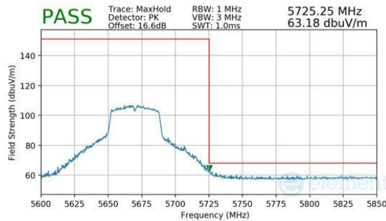
Plot 7-264. Antenna 3a (Peak, Ch.134, 802.11n, MCS7)
