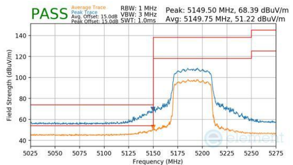
Plot 7-397. CDD Primary (Peak & Average, Ch.38, 802.11be(SU), MCS11)
