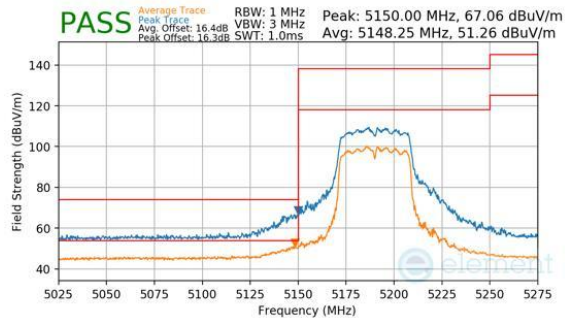
Plot 7-386. CDD Primary (Peak & Average, Ch.38, 802.11n, MCS7)
