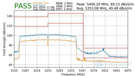
Plot 7-359. Antenna 1b (Peak & Average, Ch.50, 802.11be(SU), MCS11)
