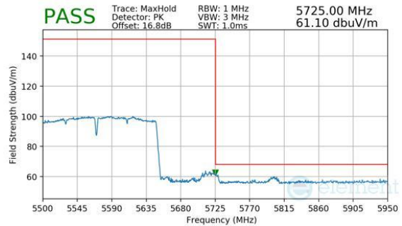
Plot 7-231. Antenna 3c (Peak, Ch.114, 802.11ac, MCS9)
