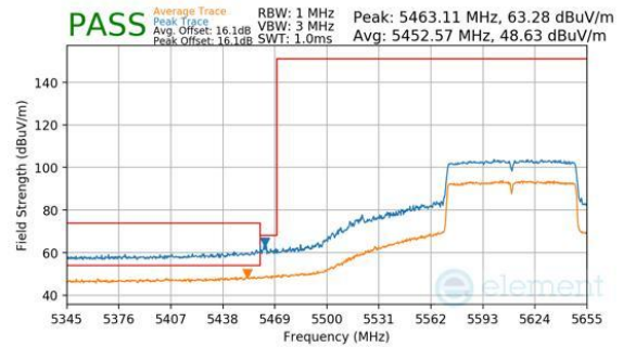
Plot 7-280. Antenna 3a (Peak & Average, Ch.122, 802.11ac, MCS9)
