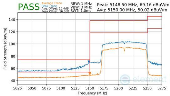
Plot 7-214. Antenna 3c (Peak & Average, Ch.42, 802.11ac, MCS9)
