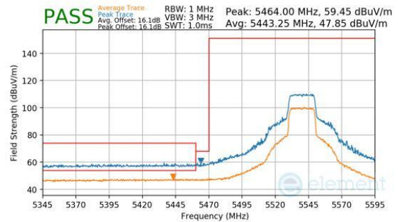
Plot 7-252. Antenna 3a (Peak & Average, Ch.108, 802.11be(SU), MCS11)
