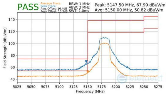
Plot 7-299. Antenna 1b (Peak & Average, Ch.36, 802.11n, MCS7)
