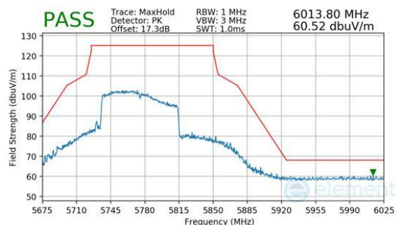
Plot 7-290. Antenna 3a (Peak, Ch.155, 802.11be(SU), MCS11)
