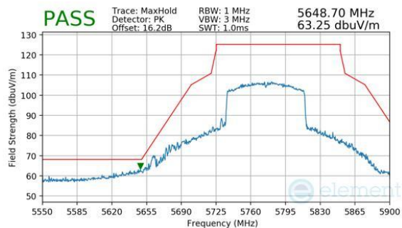
Plot 7-352. Antenna 1b (Peak, Ch.155, 802.11be(SU), MCS11)
