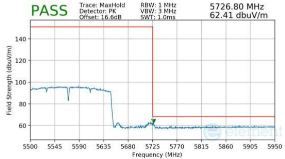
Plot 7-357. Antenna 1b (Peak, Ch.114, 802.11ac, MCS9)
