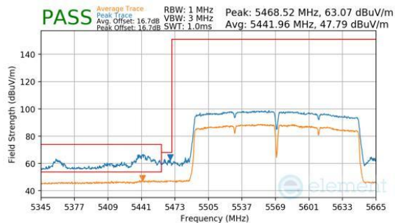
Plot 7-356. Antenna 1b (Peak & Average, Ch.114, 802.11ac, MCS9)
