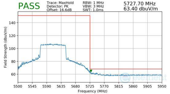
Plot 7-351. Antenna 1b (Peak, Ch.122, 802.11be(SU), MCS11)
