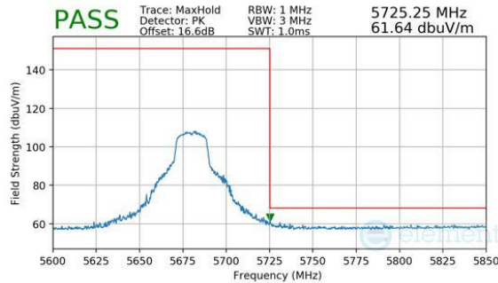
Plot 7-242. Antenna 3a (Peak, Ch.136, 802.11n, MCS7)
