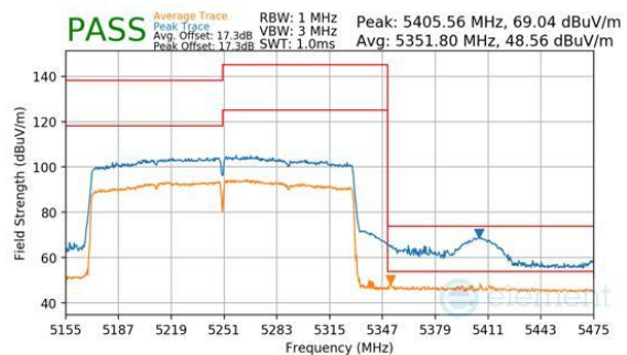
Plot 7-233. Antenna 3c (Peak & Average, Ch.50, 802.11be(SU), MCS11)
