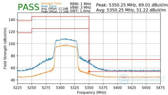
Plot 7-333. Antenna 1b (Peak & Average, Ch.62, 802.11be(SU), MCS11)
