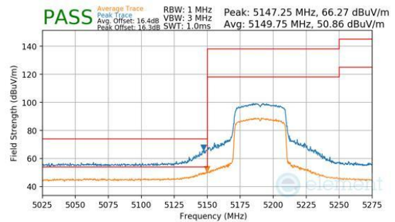
Plot 7-267. Antenna 3a (Peak & Average, Ch.38, 802.11be(SU), MCS11)
