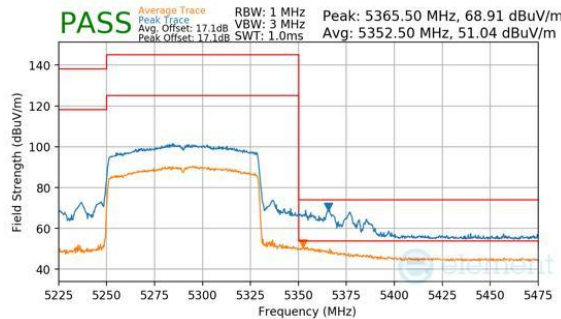
Plot 7-285. Antenna 3a (Peak & Average, Ch.58, 802.11be(SU), MCS11)
