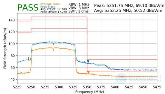
Plot 7-341. Antenna 1b (Peak & Average, Ch.58, 802.11ac, MCS9)
