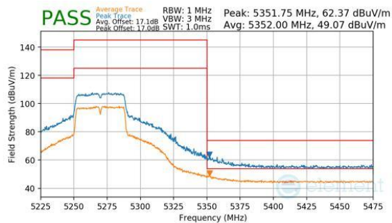
Plot 7-259. Antenna 3a (Peak & Average, Ch.54, 802.11n, MCS7)
