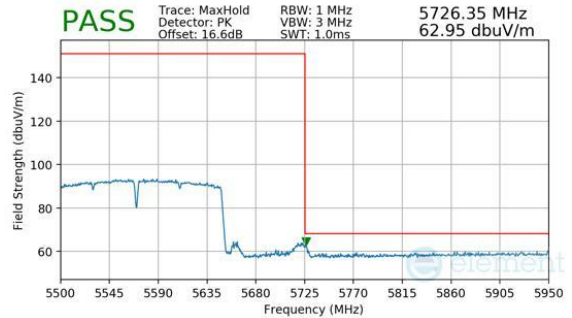
Plot 7-294. Antenna 3a (Peak, Ch.114, 802.11ac, MCS9)
