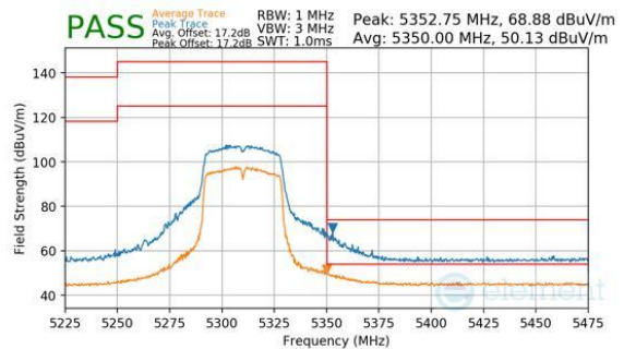
Plot 7-323. Antenna 1b (Peak & Average, Ch.62, 802.11n, MCS7)
