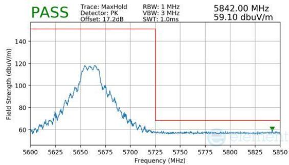
Plot 7-369. CDD Primary (Peak, Ch.132, 802.11n, MCS7)
