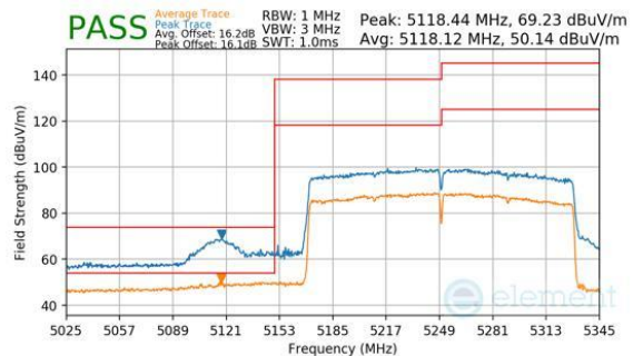
Plot 7-358. Antenna 1b (Peak & Average, Ch.50, 802.11be(SU), MCS11)
