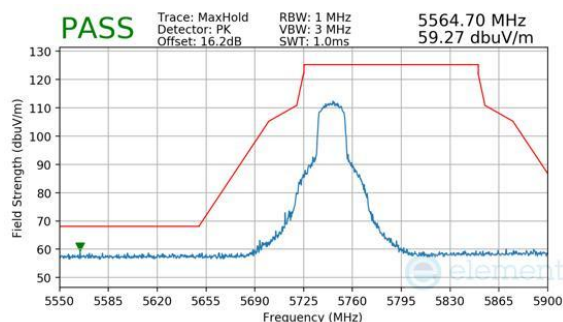
Plot 7-318. Antenna 1b (Peak, Ch.149, 802.11be(SU), MCS11)
