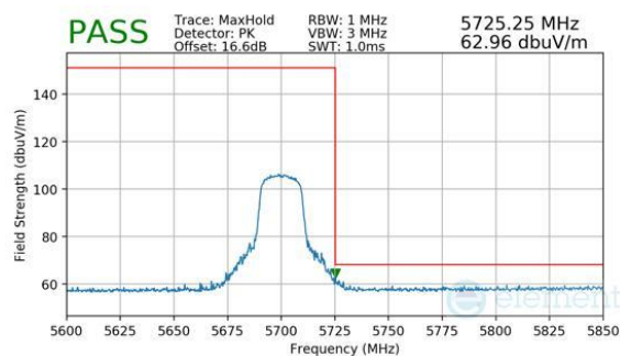
Plot 7-254. Antenna 3a (Peak, Ch.140, 802.11be(SU), MCS11)
