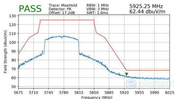
Plot 7-353. Antenna 1b (Peak, Ch.155, 802.11be(SU), MCS11)
