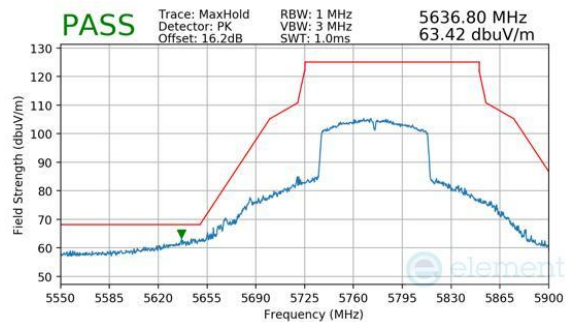
Plot 7-345. Antenna 1b (Peak, Ch.155, 802.11ac, MCS9)
