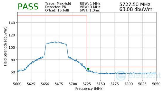
Plot 7-337. Antenna 1b (Peak, Ch.134, 802.11be(SU), MCS11)
