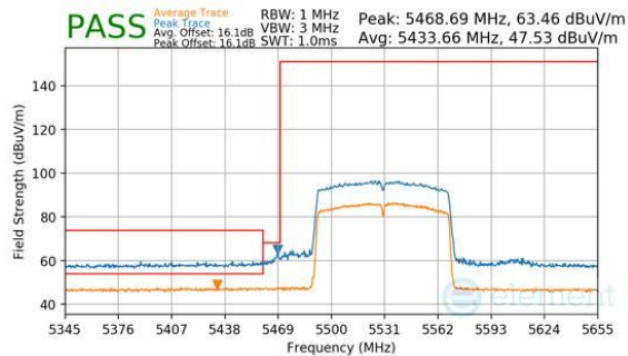
Plot 7-279. Antenna 3a (Peak & Average, Ch.106, 802.11ac, MCS9)
