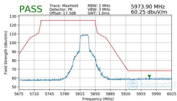
Plot 7-256. Antenna 3a (Peak, Ch.165, 802.11be(SU), MCS11)
