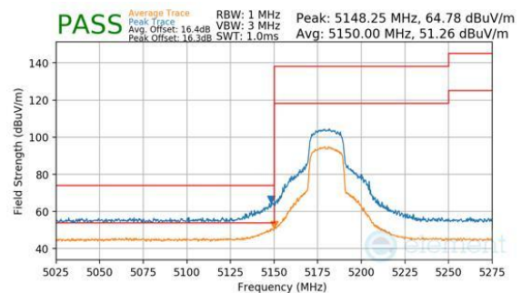
Plot 7-246. Antenna 3a (Peak & Average, Ch.36, 802.11be(SU), MCS11)
