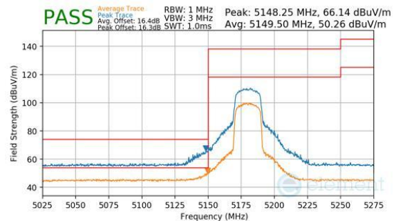
Plot 7-309. Antenna 1b (Peak & Average, Ch.36, 802.11be(SU), MCS11)
