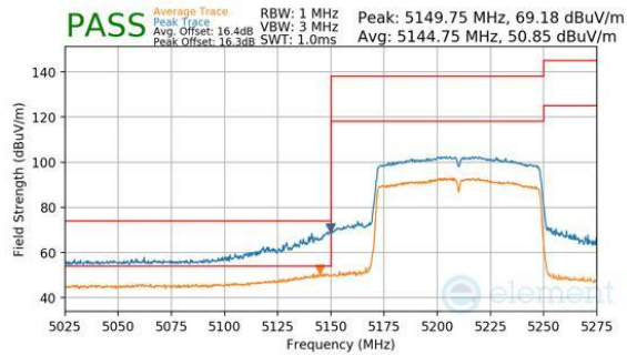
Plot 7-340. Antenna 1b (Peak & Average, Ch.42, 802.11ac, MCS9)
