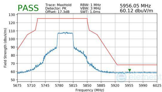
Plot 7-339. Antenna 1b (Peak, Ch.159, 802.11be(SU), MCS11)
