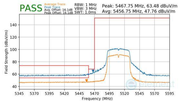
Plot 7-261. Antenna 3a (Peak & Average, Ch.102, 802.11n, MCS7)
