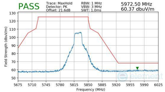
Plot 7-245. Antenna 3a (Peak, Ch.165, 802.11n, MCS7)
