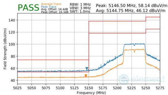
Plot 7-258. Antenna 3a (Peak & Average, Ch.46, 802.11n, MCS7)
