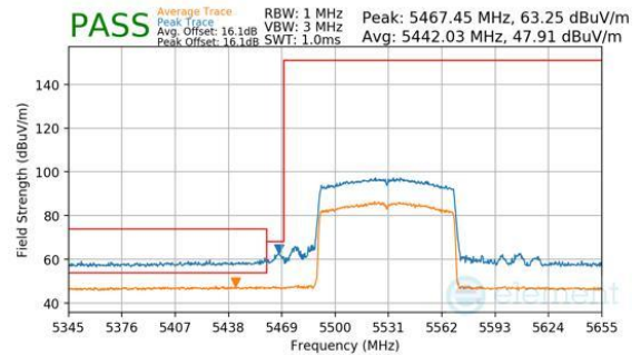
Plot 7-286. Antenna 3a (Peak & Average, Ch.106, 802.11be(SU), MCS11)
