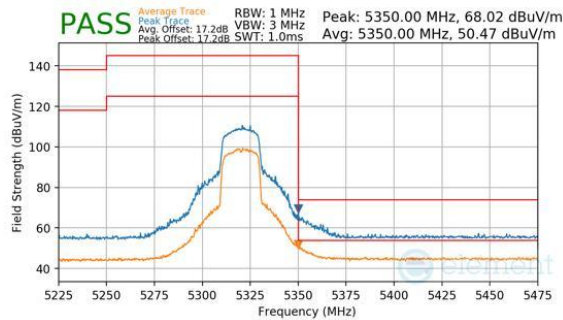
Plot 7-249. Antenna 3a (Peak & Average, Ch.64, 802.11be(SU), MCS11)
