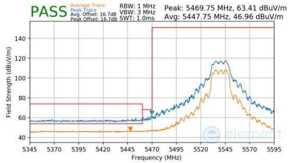
Plot 7-368. CDD Primary (Peak & Average, Ch.108, 802.11n, MCS7)
