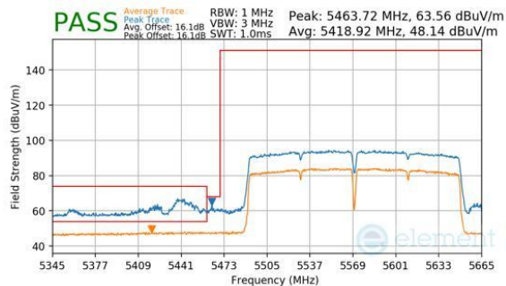
Plot 7-293. Antenna 3a (Peak & Average, Ch.114, 802.11ac, MCS9)
