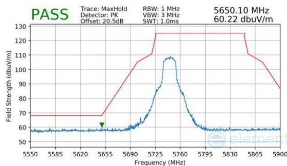
Plot 7-244. Antenna 3a (Peak, Ch.149, 802.11n, MCS7)
