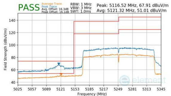
Plot 7-295. Antenna 3a (Peak & Average, Ch.50, 802.11be(SU), MCS11)
