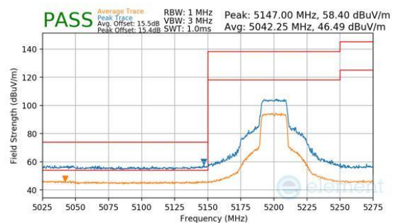
Plot 7-247. Antenna 3a (Peak & Average, Ch.40, 802.11be(SU), MCS11)
