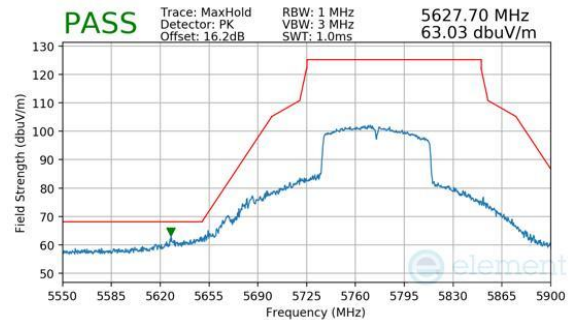
Plot 7-282. Antenna 3a (Peak, Ch.155, 802.11ac, MCS9)
