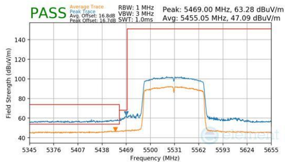
Plot 7-342. Antenna 1b (Peak & Average, Ch.106, 802.11ac, MCS9)
