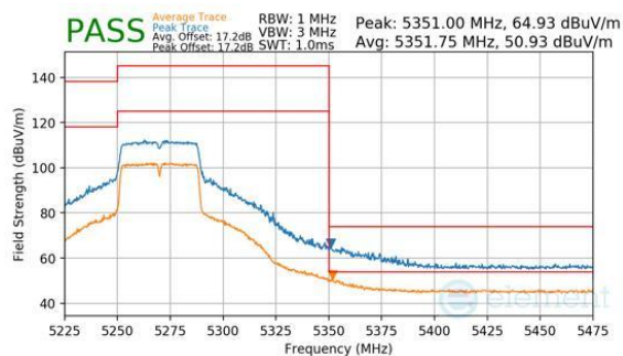
Plot 7-322. Antenna 1b (Peak & Average, Ch.54, 802.11n, MCS7)
