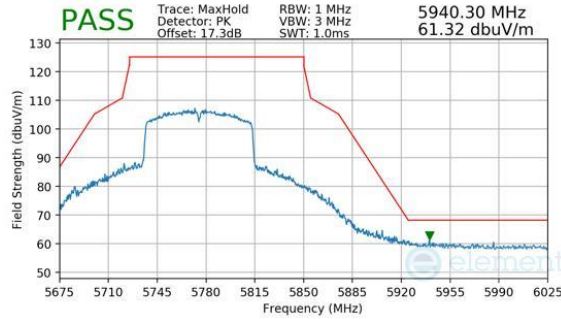
Plot 7-346. Antenna 1b (Peak, Ch.155, 802.11ac, MCS9)
