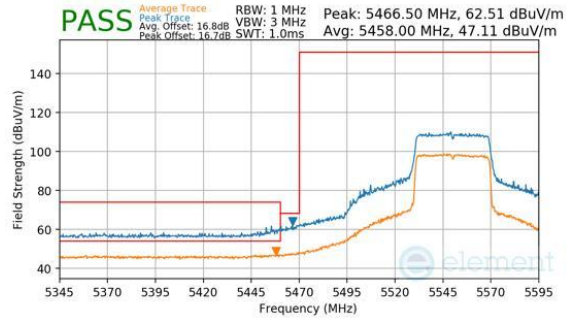
Plot 7-335. Antenna 1b (Peak & Average, Ch.110, 802.11be(SU), MCS11)
