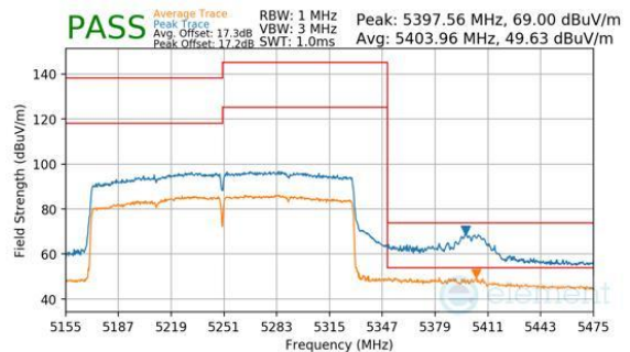
Plot 7-296. Antenna 3a (Peak & Average, Ch.50, 802.11be(SU), MCS11)
