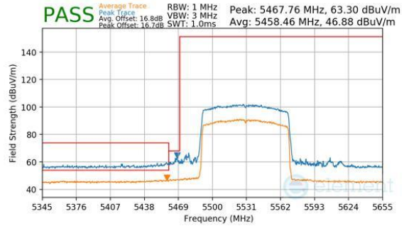
Plot 7-349. Antenna 1b (Peak & Average, Ch.106, 802.11be(SU), MCS11)
