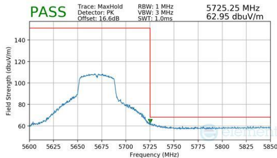
Plot 7-327. Antenna 1b (Peak, Ch.134, 802.11n, MCS7)
