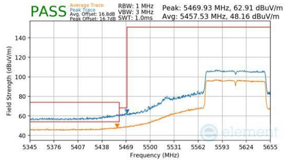
Plot 7-343. Antenna 1b (Peak & Average, Ch.122, 802.11ac, MCS9)
