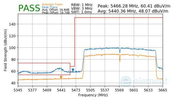
Plot 7-360. Antenna 1b (Peak & Average, Ch.114, 802.11be(SU), MCS11)
