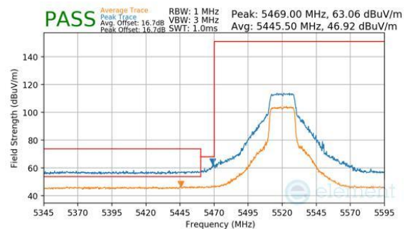
Plot 7-304. Antenna 1b (Peak & Average, Ch.104, 802.11n, MCS7)
