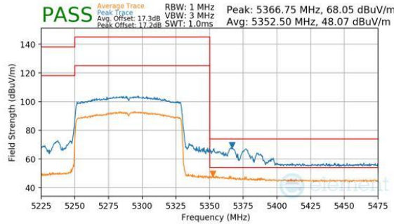
Plot 7-348. Antenna 1b (Peak & Average, Ch.58, 802.11be(SU), MCS11)
