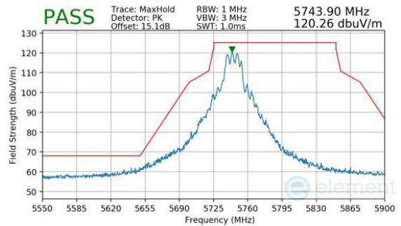
Plot 7-372. CDD Primary (Peak, Ch.149, 802.11n, MCS7)
