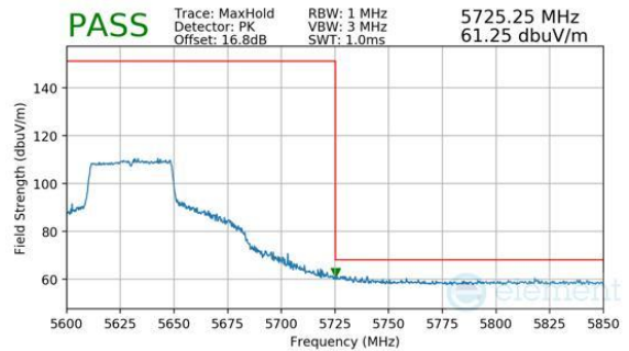
Plot 7-336. Antenna 1b (Peak, Ch.126, 802.11be(SU), MCS11)
