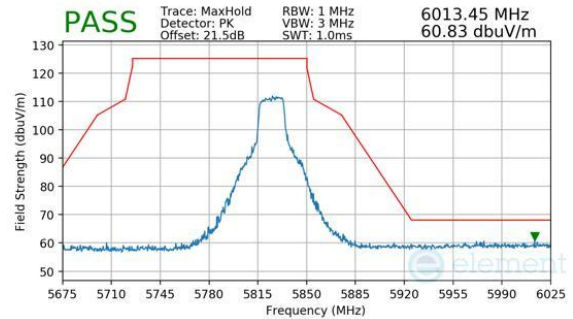
Plot 7-308. Antenna 1b (Peak, Ch.165, 802.11n, MCS7)
