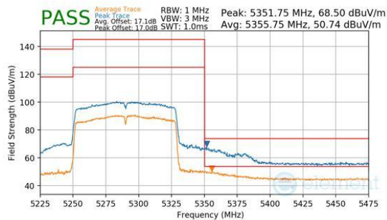
Plot 7-278. Antenna 3a (Peak & Average, Ch.58, 802.11ac, MCS9)
