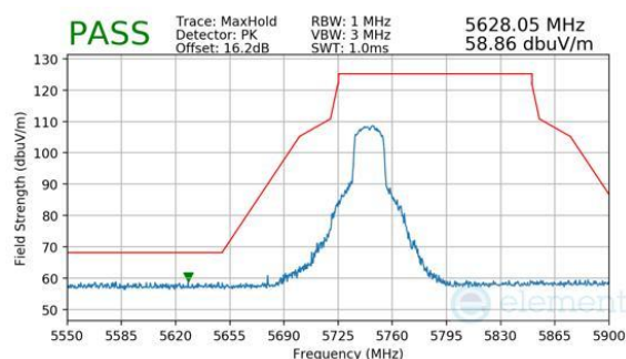
Plot 7-255. Antenna 3a (Peak, Ch.149, 802.11be(SU), MCS11)
