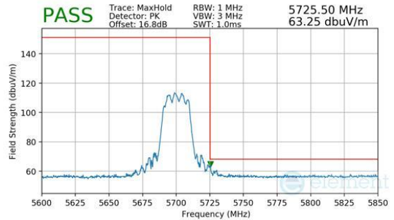
Plot 7-383. CDD Primary (Peak, Ch.140, 802.11be(SU), MCS11)
