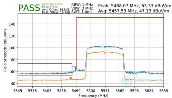
Plot 7-216. Antenna 3c (Peak & Average, Ch.106, 802.11ac, MCS9)
