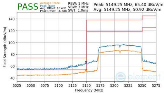
Plot 7-277. Antenna 3a (Peak & Average, Ch.42, 802.11ac, MCS9)
