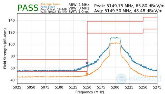
Plot 7-300. Antenna 1b (Peak & Average, Ch.40, 802.11n, MCS7)
