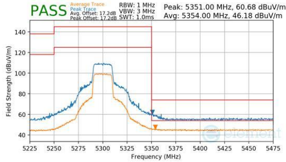
Plot 7-248. Antenna 3a (Peak & Average, Ch.60, 802.11be(SU), MCS11)
