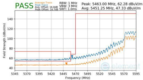
Plot 7-392. CDD Primary (Peak & Average, Ch.118, 802.11n, MCS7)
