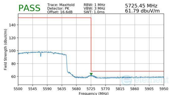
Plot 7-361. Antenna 1b (Peak, Ch.114, 802.11be(SU), MCS11)
