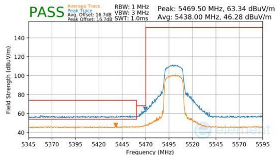
Plot 7-313. Antenna 1b (Peak & Average, Ch.100, 802.11be(SU), MCS11)
