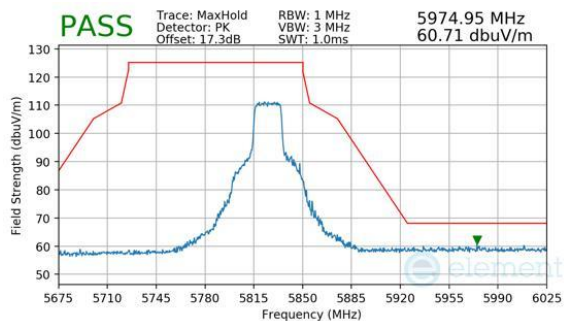
Plot 7-319. Antenna 1b (Peak, Ch.165, 802.11be(SU), MCS11)
