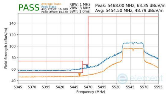
Plot 7-262. Antenna 3a (Peak & Average, Ch.110, 802.11n, MCS7)
