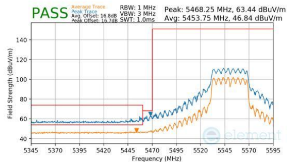
Plot 7-391. CDD Primary (Peak & Average, Ch.110, 802.11n, MCS7)
