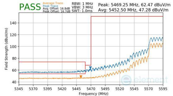
Plot 7-403. CDD Primary (Peak & Average, Ch.118, 802.11be(SU), MCS11)
