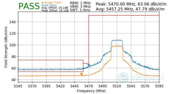
Plot 7-251. Antenna 3a (Peak & Average, Ch.104, 802.11be(SU), MCS11)
