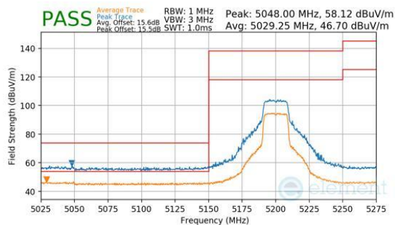
Plot 7-237. Antenna 3a (Peak & Average, Ch.40, 802.11n, MCS7)
