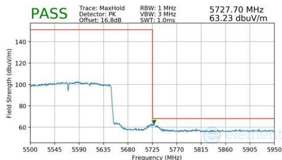
Plot 7-235. Antenna 3c (Peak, Ch.114, 802.11be(SU), MCS11)
