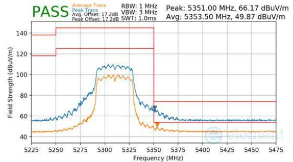
Plot 7-389. CDD Primary (Peak & Average, Ch.62, 802.11n, MCS7)
