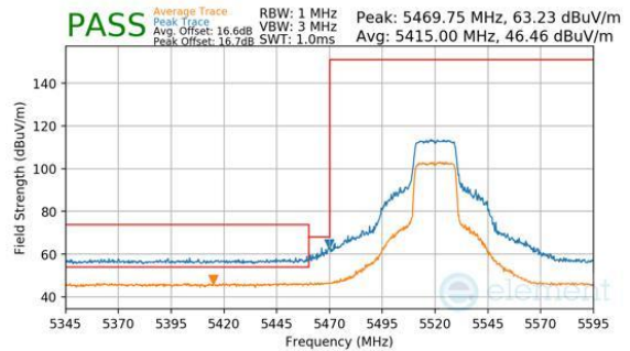
Plot 7-314. Antenna 1b (Peak & Average, Ch.104, 802.11be(SU), MCS11)
