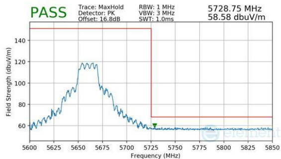
Plot 7-381. CDD Primary (Peak, Ch.132, 802.11be(SU), MCS11)
