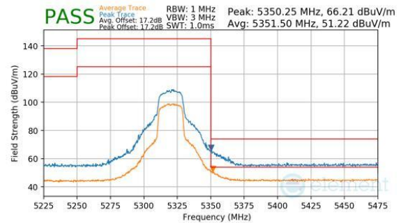
Plot 7-239. Antenna 3a (Peak & Average, Ch.64, 802.11n, MCS7)
