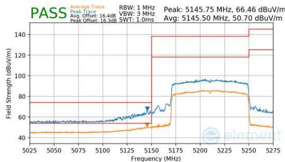
Plot 7-284. Antenna 3a (Peak & Average, Ch.42, 802.11be(SU), MCS11)
