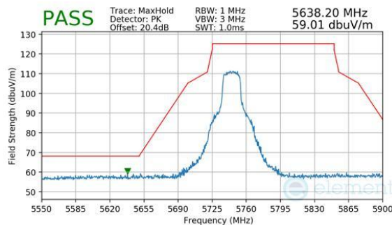
Plot 7-307. Antenna 1b (Peak, Ch.149, 802.11n, MCS7)
