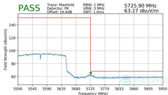
Plot 7-298. Antenna 3a (Peak, Ch.114, 802.11be(SU), MCS11)
