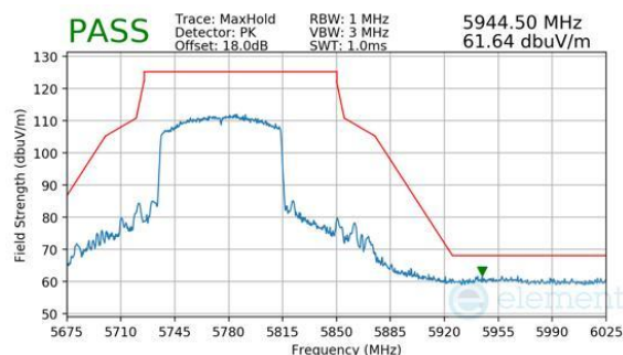
Plot 7-227. Antenna 3c (Peak, Ch.155, 802.11be(SU), MCS11)
