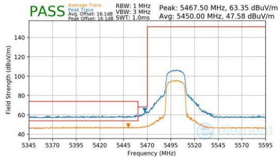
Plot 7-250. Antenna 3a (Peak & Average, Ch.100, 802.11be(SU), MCS11)
