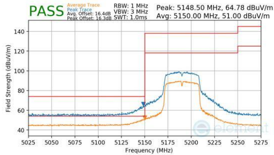
Plot 7-257. Antenna 3a (Peak & Average, Ch.38, 802.11n, MCS7)
