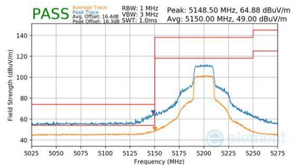
Plot 7-310. Antenna 1b (Peak & Average, Ch.40, 802.11be(SU), MCS11)
