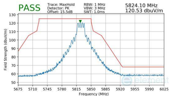
Plot 7-373. CDD Primary (Peak, Ch.165, 802.11n, MCS7)
