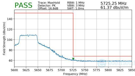
Plot 7-326. Antenna 1b (Peak, Ch.126, 802.11n, MCS7)
