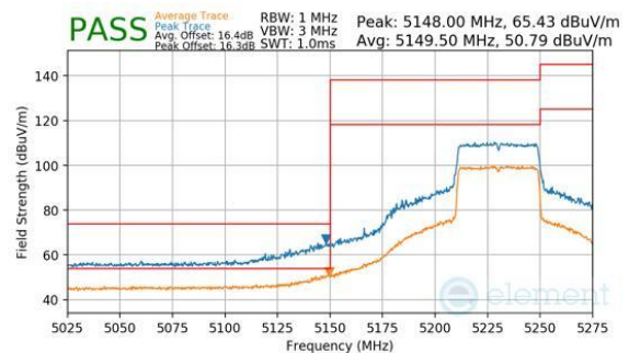
Plot 7-331. Antenna 1b (Peak & Average, Ch.46, 802.11be(SU), MCS11)
