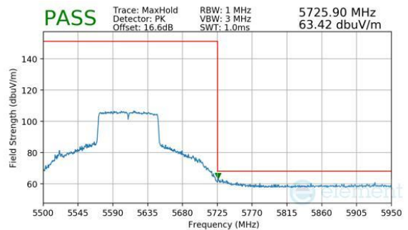
Plot 7-344. Antenna 1b (Peak, Ch.122, 802.11ac, MCS9)
