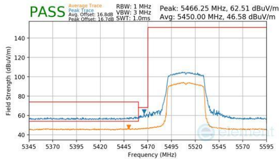
Plot 7-334. Antenna 1b (Peak & Average, Ch.102, 802.11be(SU), MCS11)
