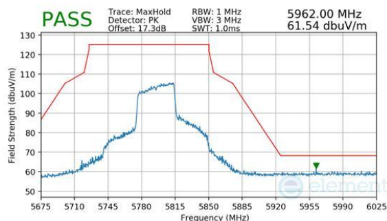
Plot 7-276. Antenna 3a (Peak, Ch.159, 802.11be(SU), MCS11)
