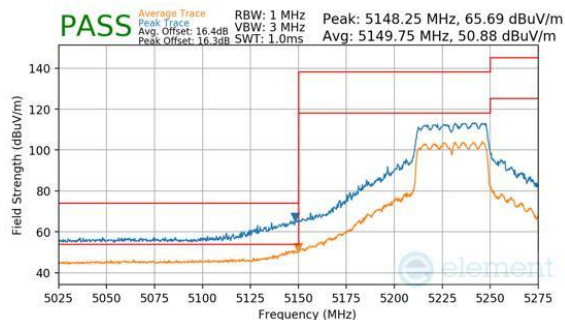
Plot 7-387. CDD Primary (Peak & Average, Ch.46, 802.11n, MCS7)
