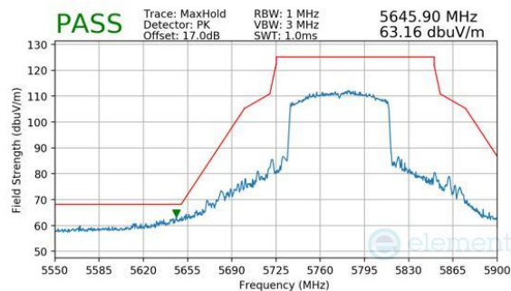
Plot 7-226. Antenna 3c (Peak, Ch.155, 802.11be(SU), MCS11)
