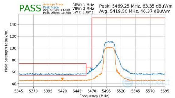
Plot 7-303. Antenna 1b (Peak & Average, Ch.100, 802.11n, MCS7)
