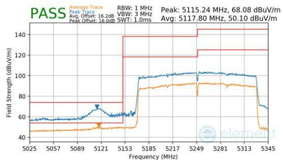
Plot 7-232. Antenna 3c (Peak & Average, Ch.50, 802.11be(SU), MCS11)
