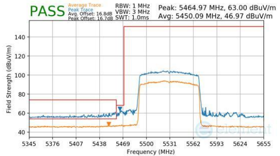
Plot 7-223. Antenna 3c (Peak & Average, Ch.106, 802.11be(SU), MCS11)
