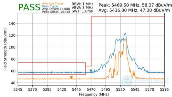
Plot 7-1068. CDD Diversity (Peak & Average, RU52, Index 40, Ch.104, MCS11)
