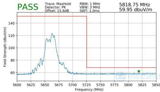
Plot 7-1100. CDD Diversity (Peak, RU52+26, Index 72, Ch.132, MCS11)
