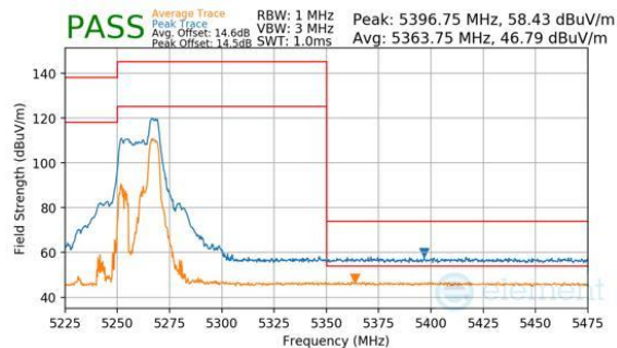
Plot 7-1127. CDD Diversity (Peak & Average, RU52, Index 40, Ch.54, MCS11)
