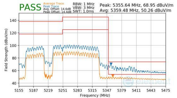
Plot 7-1031. CDD Primary (Peak & Average, RU996+484+242, Index 98 (L), Ch.50, MCS11)
