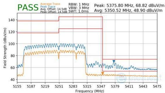
Plot 7-1034. CDD Primary (Peak & Average, RU996+484+242, Index 99 (H), Ch.50, MCS11)
