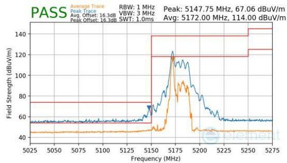
Plot 7-1055. CDD Diversity (Peak & Average, RU26, Index 0, Ch.36, MCS11)
