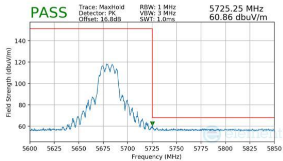
Plot 7-1116. CDD Diversity (Peak, RU242, Index 61, Ch.136, MCS11)
