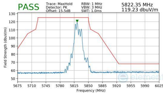
Plot 7-1106. CDD Diversity (Peak, RU52+26, Index 70, Ch.165, MCS11)
