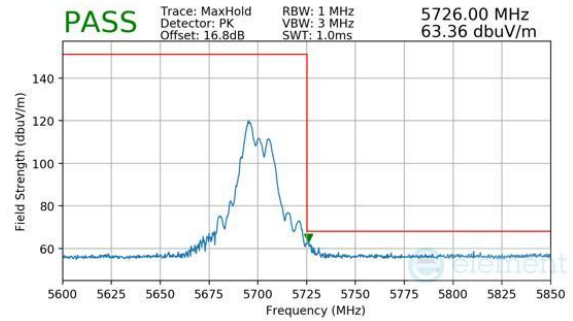
Plot 7-1102. CDD Diversity (Peak, RU52+26, Index 70, Ch.140, MCS11)
