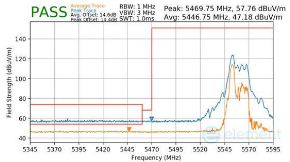
Plot 7-1071. CDD Diversity (Peak & Average, RU52, Index 37, Ch.112, MCS11)
