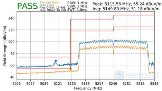
Plot 7-1051. CDD Primary (Peak & Average, RU996X2, Index 68, Ch.50, MCS11)
