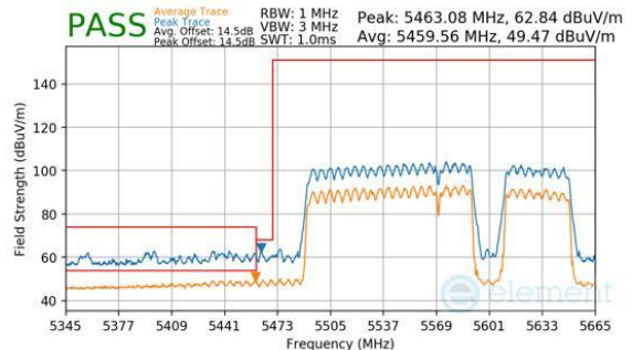
Plot 7-1038. CDD Primary (Peak & Average, RU996+484+242, Index 97 (H), Ch.114, MCS11)
