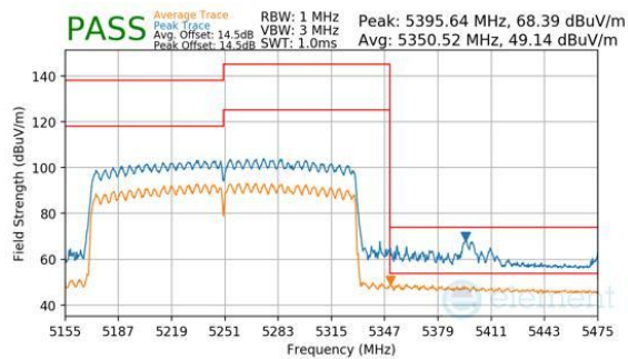
Plot 7-1052. CDD Primary (Peak & Average, RU996X2, Index 68, Ch.50, MCS11)
