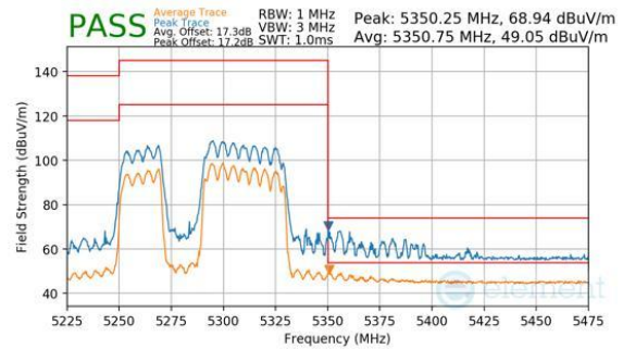
Plot 7-1168. CDD Diversity (Peak & Average, RU484+242, Index 91, Ch.58, MCS11)
