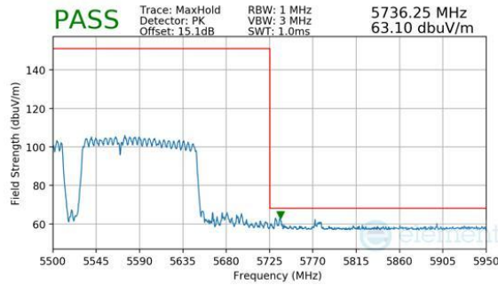
Plot 7-1045. CDD Primary (Peak, RU996+484+242, Index 97 (L), Ch.114, MCS11)
