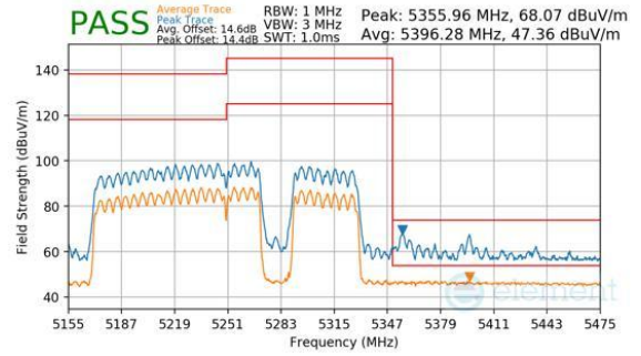
Plot 7-1030. CDD Primary (Peak & Average, RU996+484+242, Index 97 (H), Ch.50, MCS11)
