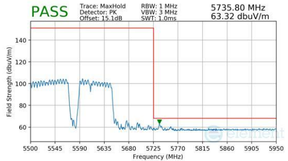
Plot 7-1043. CDD Primary (Peak, RU996+484+242, Index 96 (H), Ch.114, MCS11)
