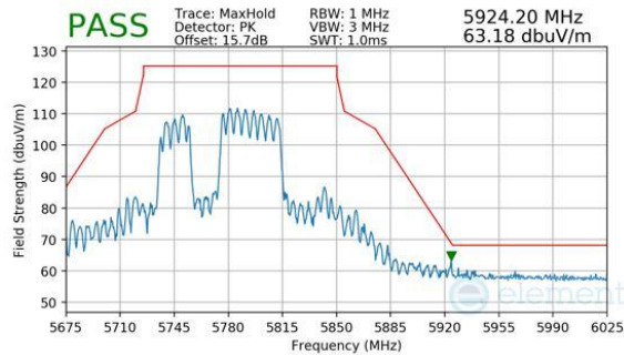
Plot 7-1188. CDD Diversity (Peak, RU484+242, Index 91, Ch.155, MCS11)
