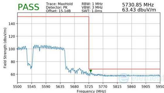
Plot 7-1047. CDD Primary (Peak, RU996+484+242, Index 98 (L), Ch.114, MCS11)
