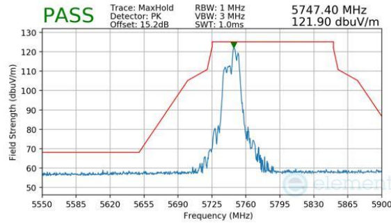
Plot 7-1105. CDD Diversity (Peak, RU52+26, Index 72, Ch.149, MCS11)
