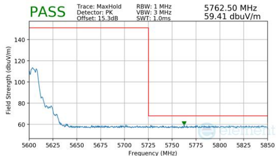
Plot 7-1075. CDD Diversity (Peak & Average, RU52, Index 37, Ch.120, MCS11)
