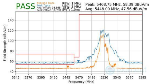
Plot 7-1097. CDD Diversity (Peak & Average, RU52+26, Index 70, Ch.104, MCS11)
