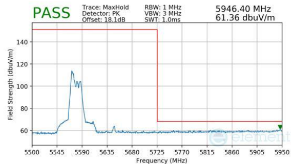
Plot 7-1161. CDD Diversity (Peak, RU52, Index 37, Ch.122, MCS11)
