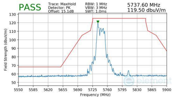
Plot 7-1122. CDD Diversity (Peak, RU26, Index 0, Ch.151, MCS11)
