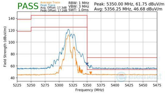
Plot 7-1093. CDD Diversity (Peak & Average, RU52+26, Index 70, Ch.64, MCS11)
