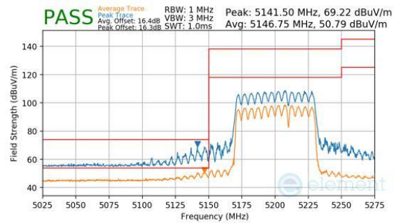
Plot 7-1166. CDD Diversity (Peak & Average, RU484+242, Index 93, Ch.42, MCS11)
