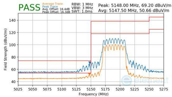
Plot 7-1140. CDD Diversity (Peak & Average, RU484, Index 65, Ch.38, MCS11)
