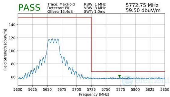
Plot 7-1115. CDD Diversity (Peak, RU242, Index 61, Ch.132, MCS11)
