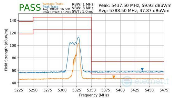
Plot 7-1064. CDD Diversity (Peak & Average, RU52, Index 40, Ch.64, MCS11)
