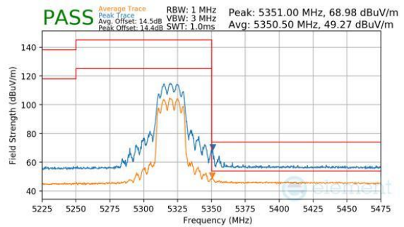
Plot 7-1111. CDD Diversity (Peak & Average, RU242, Index 61, Ch.64, MCS11)
