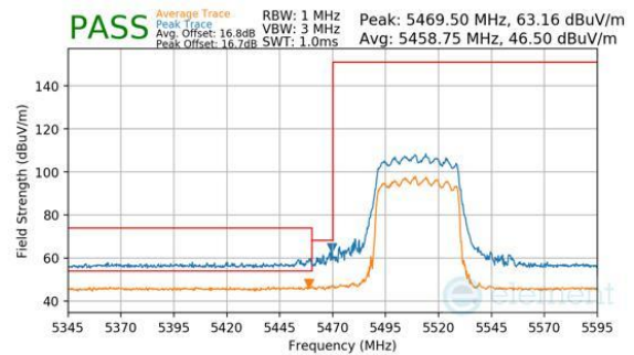
Plot 7-1144. CDD Diversity (Peak & Average, RU484, Index 65, Ch.102, MCS11)
