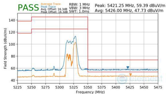
Plot 7-1158. CDD Diversity (Peak & Average, RU52, Index 52, Ch.58, MCS11)
