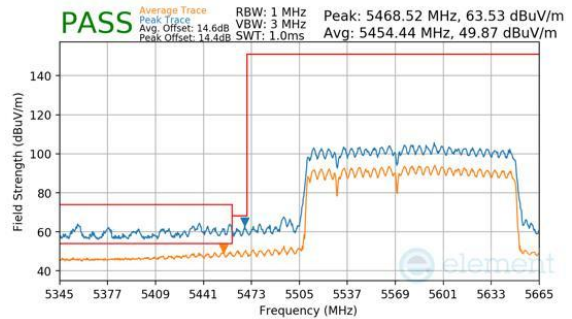
Plot 7-1036. CDD Primary (Peak & Average, RU996+484+242, Index 96 (L), Ch.114, MCS11)
