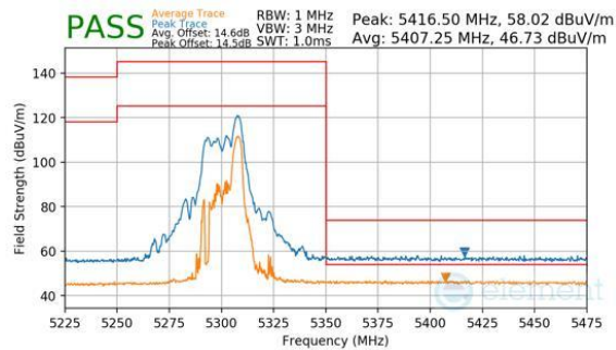
Plot 7-1062. CDD Diversity (Peak & Average, RU52, Index 40, Ch.60, MCS11)
