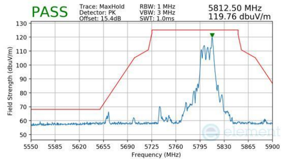
Plot 7-1154. CDD Diversity (Peak, RU26, Index 36, Ch.155, MCS11)
