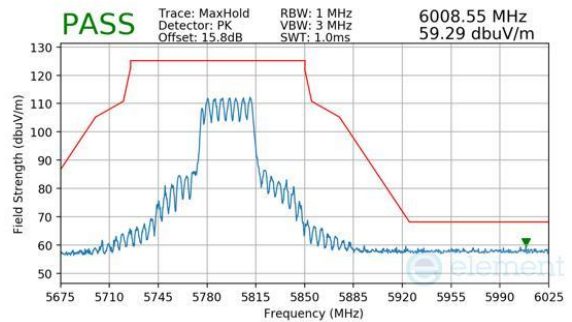
Plot 7-1150. CDD Diversity (Peak, RU484, Index 65, Ch.159, MCS11)
