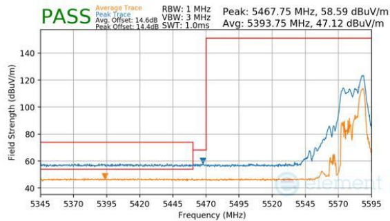
Plot 7-1074. CDD Diversity (Peak & Average, RU52, Index 40, Ch.116, MCS11)
