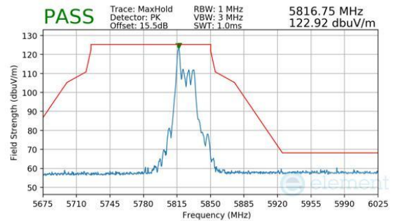
Plot 7-1059. CDD Diversity (Peak, RU26, Index 0, Ch.165, MCS11)
