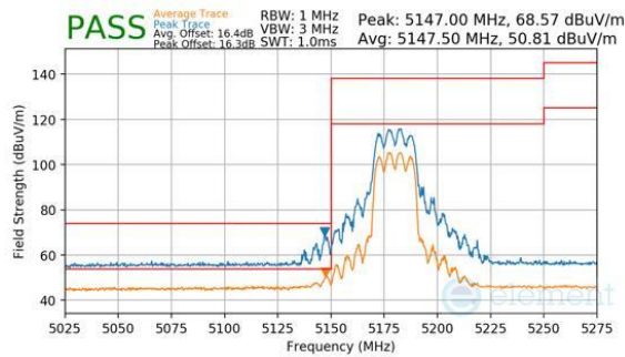
Plot 7-1108. CDD Diversity (Peak & Average, RU242, Index 61, Ch.36, MCS11)
