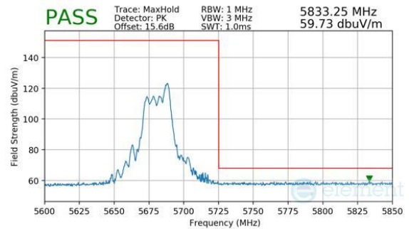
Plot 7-1084. CDD Diversity (Peak, RU52, Index 40, Ch.136, MCS11)
