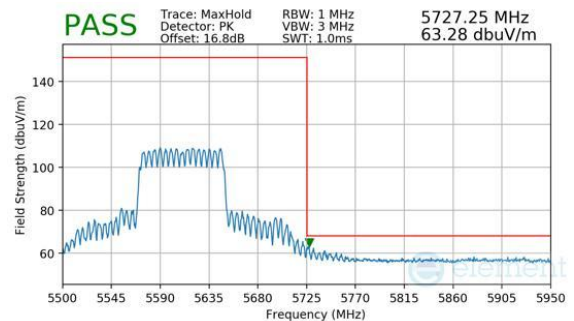
Plot 7-1195. CDD Diversity (Peak, RU996, Index 67, Ch.122, MCS11)
