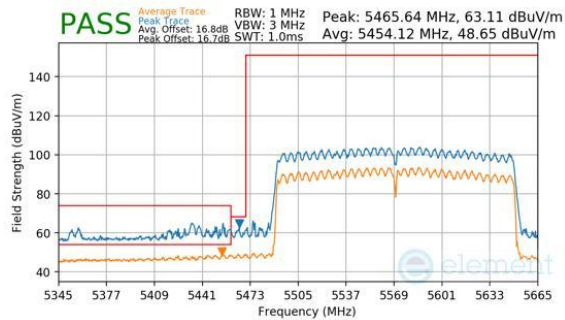
Plot 7-1053. CDD Primary (Peak & Average, RU996X2, Index 68, Ch.114, MCS11)
