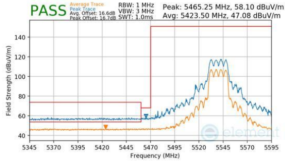
Plot 7-1114. CDD Diversity (Peak & Average, RU242, Index 61, Ch.108, MCS11)
