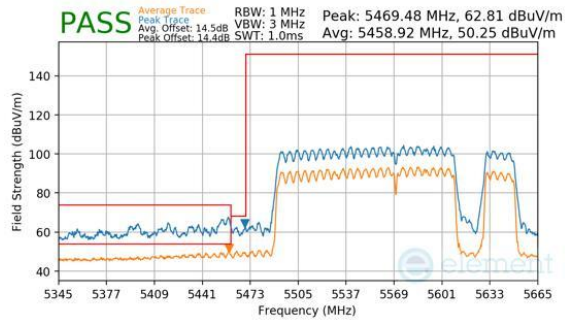
Plot 7-1039. CDD Primary (Peak & Average, RU996+484+242, Index 98 (H), Ch.114, MCS11)
