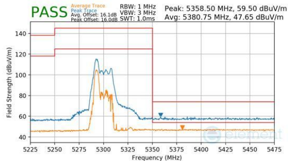
Plot 7-1128. CDD Diversity (Peak & Average, RU52, Index 37, Ch.62, MCS11)
