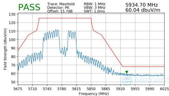
Plot 7-1189. CDD Diversity (Peak, RU484+242, Index 92, Ch.155, MCS11)
