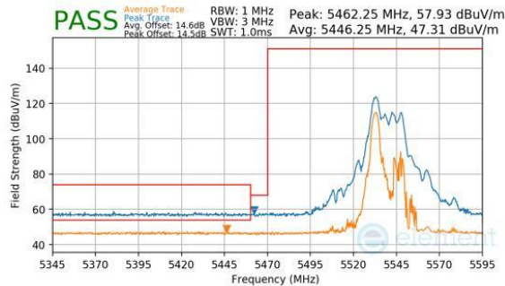
Plot 7-1069. CDD Diversity (Peak & Average, RU52, Index 37, Ch.108, MCS11)
