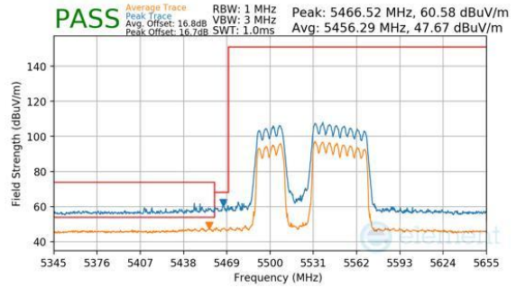
Plot 7-1172. CDD Diversity (Peak & Average, RU484+242, Index 91, Ch.106, MCS11)
