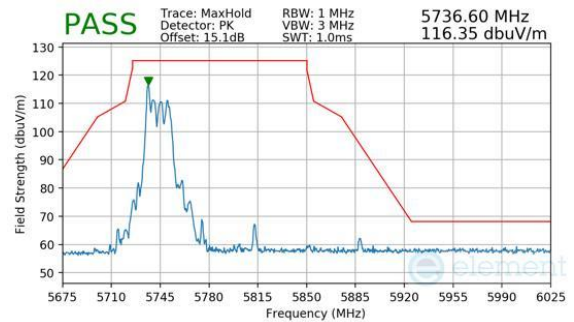
Plot 7-1155. CDD Diversity (Peak, RU26, Index 0, Ch.155, MCS11)
