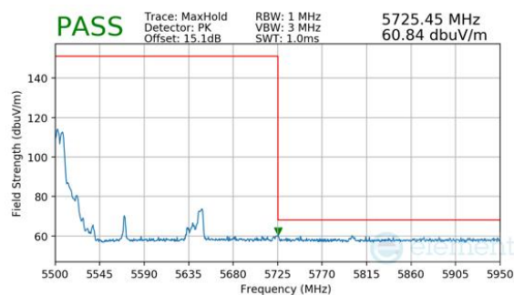
Plot 7-1204. CDD Diversity (Peak, RU52, Index 37 (L), Ch.114, MCS11)
