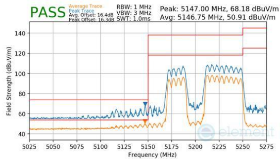
Plot 7-1164. CDD Diversity (Peak & Average, RU484+242, Index 91, Ch.42, MCS11)
