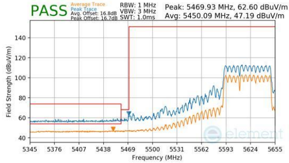
Plot 7-1175. CDD Diversity (Peak & Average, RU484+242, Index 90, Ch.122, MCS11)
