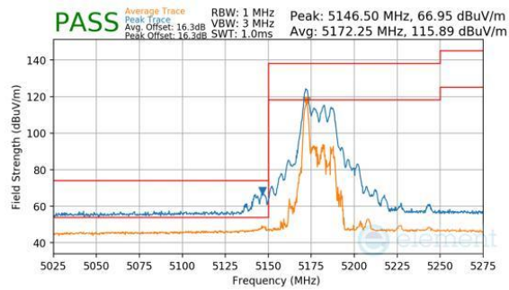
Plot 7-1120. CDD Diversity (Peak & Average, RU26, Index 0, Ch.38, MCS11)
