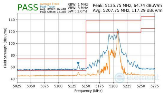
Plot 7-1121. CDD Diversity (Peak & Average, RU26, Index 17, Ch.38, MCS11)
