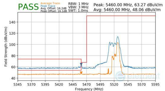
Plot 7-1131. CDD Diversity (Peak & Average, RU52, Index 44, Ch.102, MCS11)
