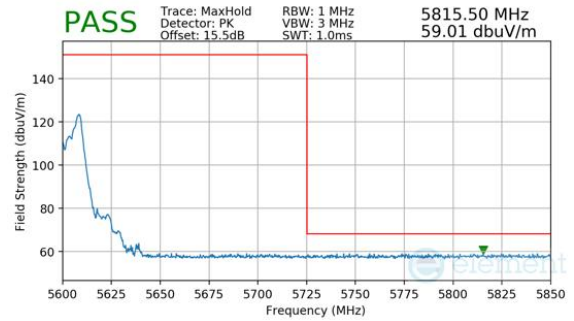
Plot 7-1076. CDD Diversity (Peak & Average, RU52, Index 40, Ch.120, MCS11)
