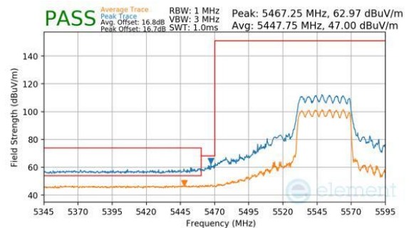
Plot 7-1145. CDD Diversity (Peak & Average, RU484, Index 65, Ch.110, MCS11)
