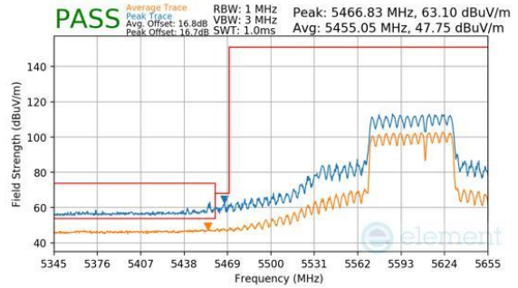
Plot 7-1178. CDD Diversity (Peak & Average, RU484+242, Index 93, Ch.122, MCS11)
