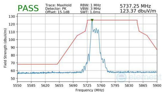
Plot 7-1057. CDD Diversity (Peak, RU26, Index 0, Ch.149, MCS11)
