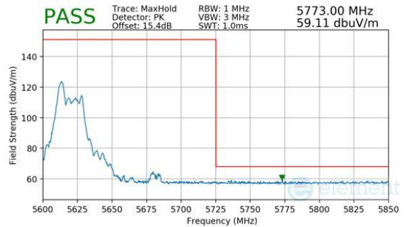
Plot 7-1136. CDD Diversity (Peak, RU52, Index 37, Ch.126, MCS11)
