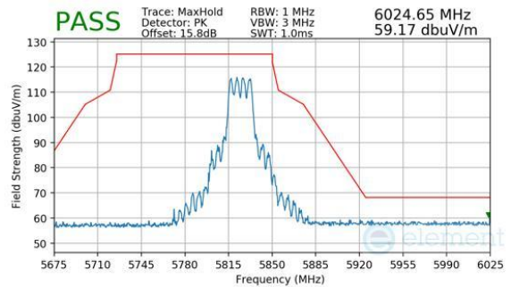
Plot 7-1119. CDD Diversity (Peak, RU242, Index 61, Ch.165, MCS11)
