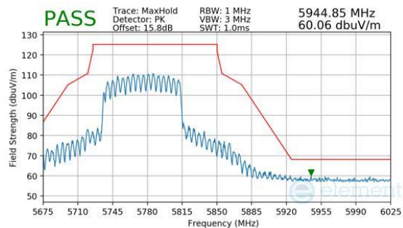
Plot 7-1197. CDD Diversity (Peak, RU996, Index 67, Ch.155, MCS11)
