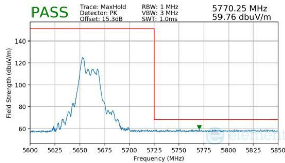
Plot 7-1081. CDD Diversity (Peak, RU52, Index 37, Ch.132, MCS11)
