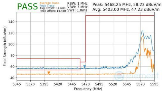
Plot 7-1134. CDD Diversity (Peak & Average, RU52, Index 37, Ch.118, MCS11)
