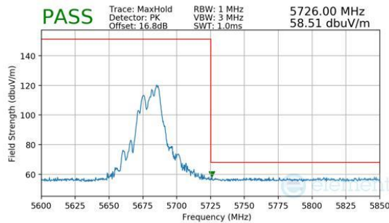
Plot 7-1101. CDD Diversity (Peak, RU52+26, Index 72, Ch.136, MCS11)
