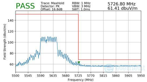
Plot 7-1179. CDD Diversity (Peak, RU484+242, Index 90, Ch.122, MCS11)
