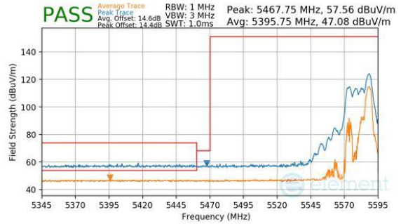
Plot 7-1135. CDD Diversity (Peak & Average, RU52, Index 40, Ch.118, MCS11)
