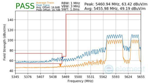
Plot 7-1177. CDD Diversity (Peak & Average, RU484+242, Index 92, Ch.122, MCS11)
