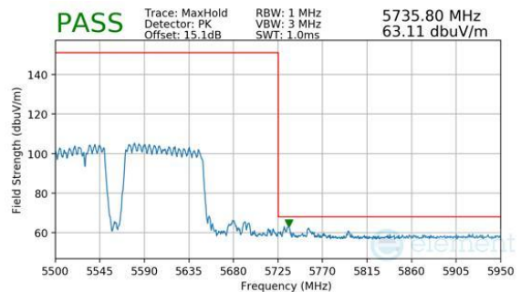
Plot 7-1049. CDD Primary (Peak, RU996+484+242, Index 99 (L), Ch.114, MCS11)
