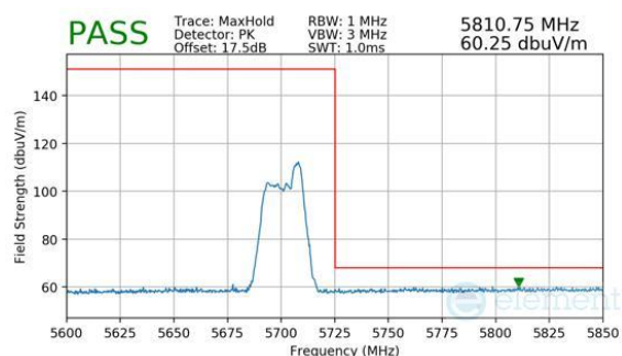
Plot 7-1086. CDD Diversity (Peak, RU52, Index 40, Ch.140, MCS11)
