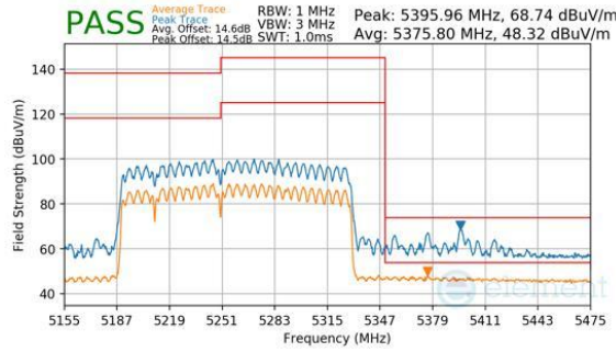
Plot 7-1027. CDD Primary (Peak & Average, RU996+484+242, Index 96 (L), Ch.50, MCS11)
