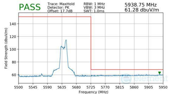
Plot 7-1162. CDD Diversity (Peak, RU52, Index 52, Ch.122, MCS11)
