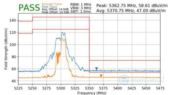
Plot 7-1092. CDD Diversity (Peak & Average, RU52+26, Index 72, Ch.60, MCS11)
