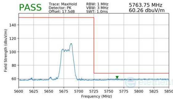
Plot 7-1139. CDD Diversity (Peak, RU52, Index 44, Ch.134, MCS11)
