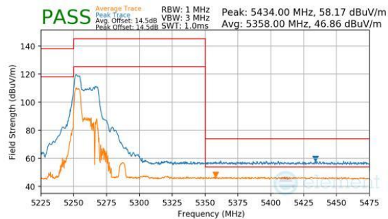
Plot 7-1126. CDD Diversity (Peak & Average, RU52, Index 37, Ch.54, MCS11)
