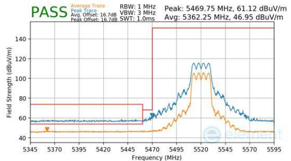
Plot 7-1113. CDD Diversity (Peak & Average, RU242, Index 61, Ch.104, MCS11)
