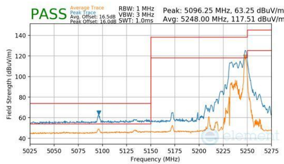
Plot 7-1152. CDD Diversity (Peak & Average, RU26, Index 36, Ch.42, MCS11)
