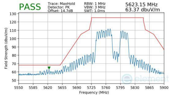
Plot 7-1185. CDD Diversity (Peak, RU484+242, Index 92, Ch.155, MCS11)
