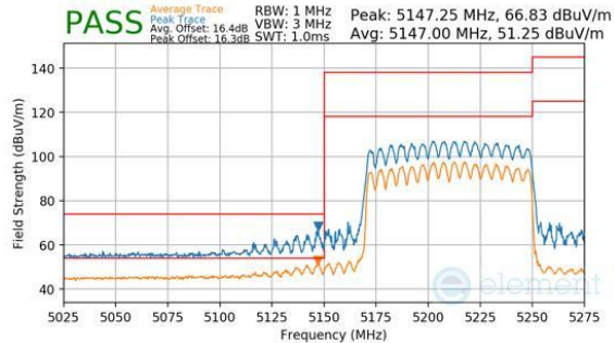
Plot 7-1191. CDD Diversity (Peak & Average, RU996, Index 67, Ch.42, MCS11)
