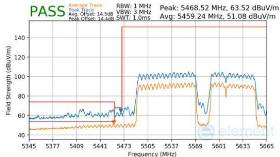
Plot 7-1035. CDD Primary (Peak & Average, RU996+484+242, Index 96 (H), Ch.114, MCS11)
