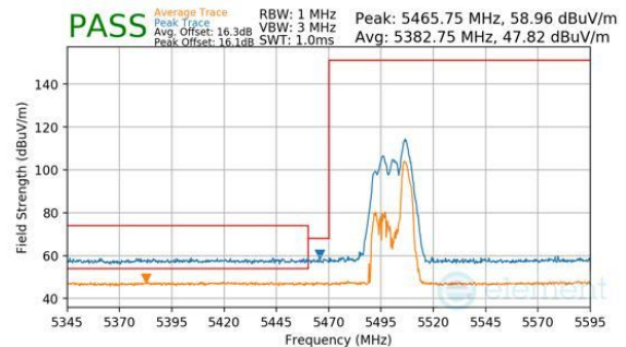
Plot 7-1066. CDD Diversity (Peak & Average, RU52, Index 40, Ch.100, MCS11)
