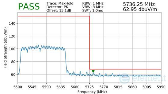
Plot 7-1044. CDD Primary (Peak, RU996+484+242, Index 96 (L), Ch.114, MCS11)
