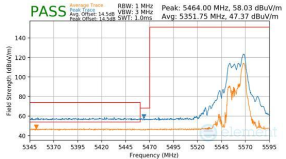
Plot 7-1072. CDD Diversity (Peak & Average, RU52, Index 40, Ch.112, MCS11)
