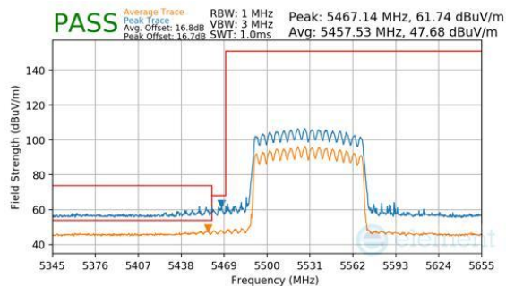
Plot 7-1193. CDD Diversity (Peak & Average, RU996, Index 67, Ch.106, MCS11)
