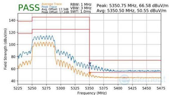
Plot 7-1142. CDD Diversity (Peak & Average, RU484, Index 65, Ch.54, MCS11)
