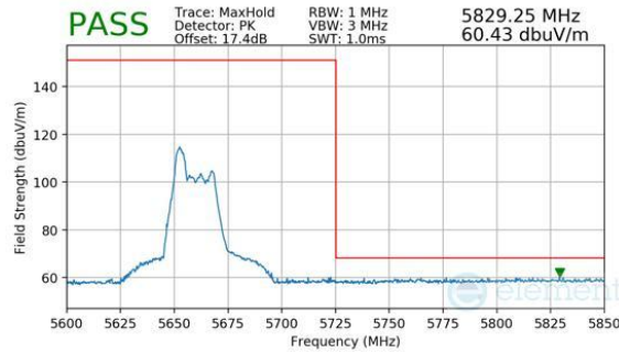
Plot 7-1138. CDD Diversity (Peak, RU52, Index 37, Ch.134, MCS11)
