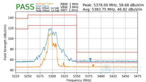
Plot 7-1091. CDD Diversity (Peak & Average, RU52+26, Index 70, Ch.60, MCS11)
