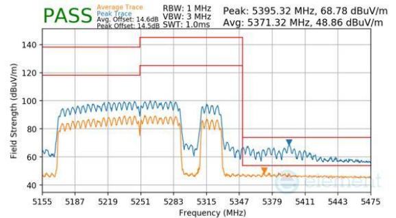
Plot 7-1032. CDD Primary (Peak & Average, RU996+484+242, Index 98 (H), Ch.50, MCS11)
