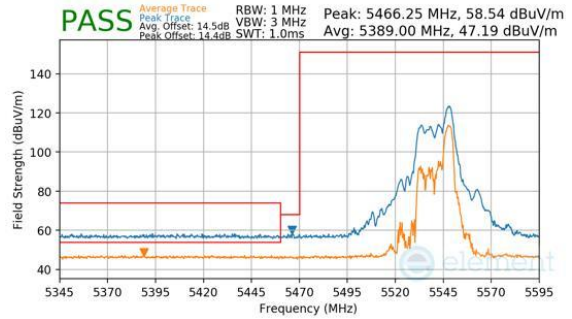
Plot 7-1070. CDD Diversity (Peak & Average, RU52, Index 40, Ch.108, MCS11)
