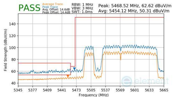
Plot 7-1037. CDD Primary (Peak & Average, RU996+484+242, Index 97 (L), Ch.114, MCS11)
