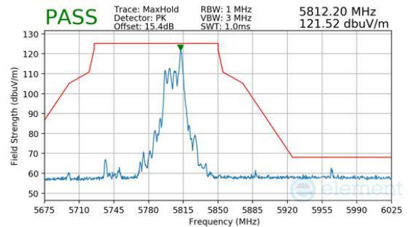
Plot 7-1156. CDD Diversity (Peak, RU26, Index 36, Ch.155, MCS11)
