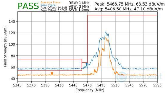
Plot 7-1096. CDD Diversity (Peak & Average, RU52+26, Index 72, Ch.100, MCS11)
