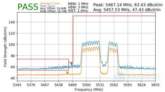
Plot 7-1173. CDD Diversity (Peak & Average, RU484+242, Index 92, Ch.106, MCS11)
