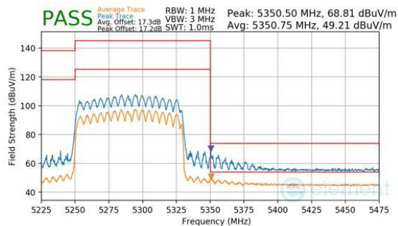
Plot 7-1192. CDD Diversity (Peak & Average, RU996, Index 67, Ch.58, MCS11)
