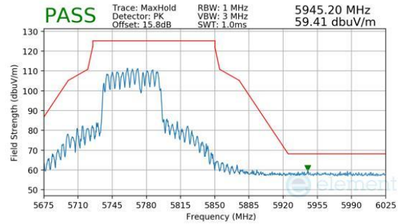
Plot 7-1190. CDD Diversity (Peak, RU484+242, Index 93, Ch.155, MCS11)
