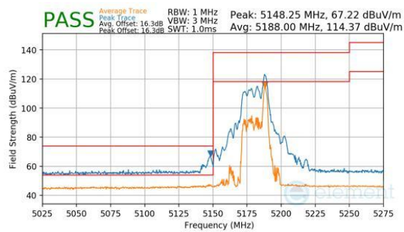
Plot 7-1056. CDD Diversity (Peak & Average, RU26, Index 8, Ch.36, MCS11)
