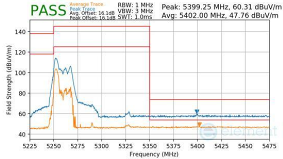
Plot 7-1157. CDD Diversity (Peak & Average, RU52, Index 37, Ch.58, MCS11)
