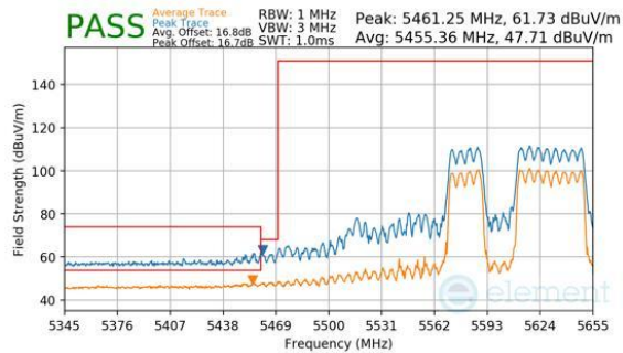
Plot 7-1176. CDD Diversity (Peak & Average, RU484+242, Index 91, Ch.122, MCS11)
