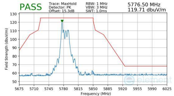
Plot 7-1124. CDD Diversity (Peak, RU26, Index 0, Ch.159, MCS11)
