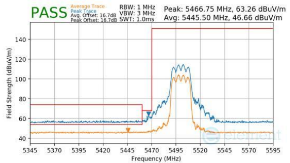
Plot 7-1112. CDD Diversity (Peak & Average, RU242, Index 61, Ch.100, MCS11)
