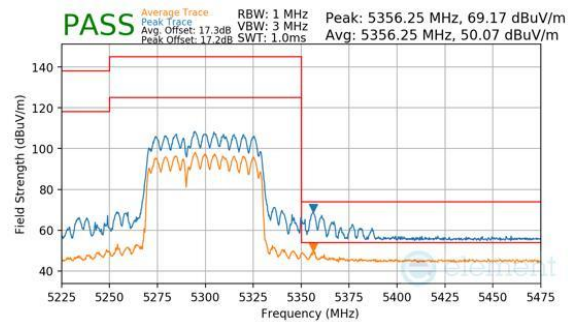
Plot 7-1167. CDD Diversity (Peak & Average, RU484+242, Index 90, Ch.58, MCS11)
