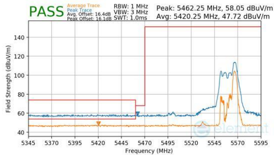
Plot 7-1133. CDD Diversity (Peak & Average, RU52, Index 44, Ch.110, MCS11)
