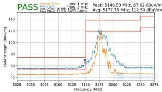
Plot 7-1087. CDD Diversity (Peak & Average, RU52+26, Index 70, Ch.36, MCS11)
