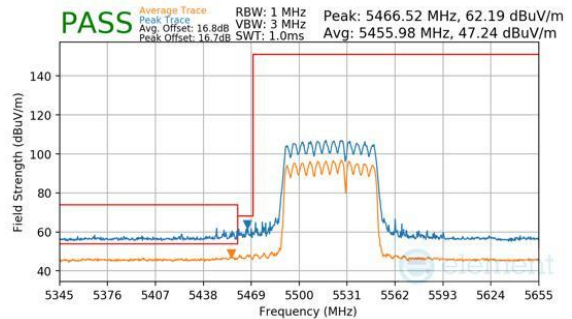
Plot 7-1174. CDD Diversity (Peak & Average, RU484+242, Index 93, Ch.106, MCS11)
