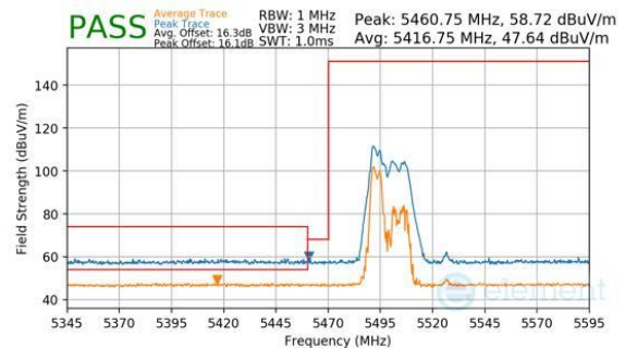
Plot 7-1130. CDD Diversity (Peak & Average, RU52, Index 37, Ch.102, MCS11)
