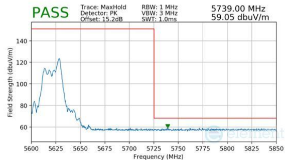
Plot 7-1078. CDD Diversity (Peak, RU52, Index 40, Ch.124, MCS11)
