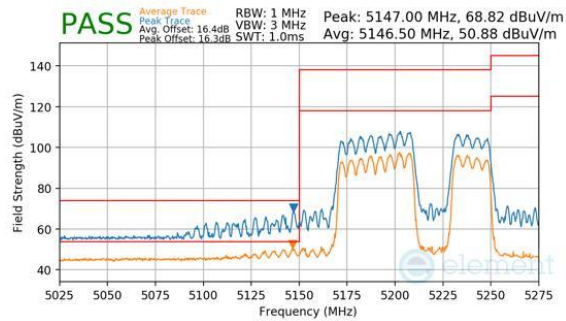
Plot 7-1165. CDD Diversity (Peak & Average, RU484+242, Index 92, Ch.42, MCS11)
