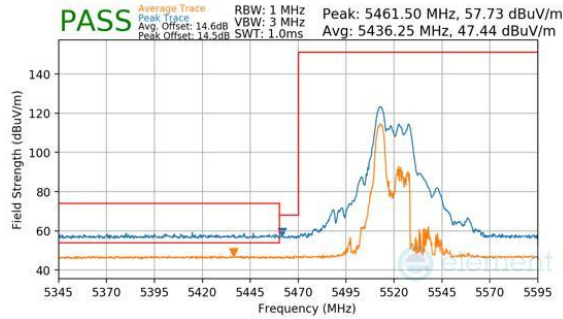
Plot 7-1067. CDD Diversity (Peak & Average, RU52, Index 37, Ch.104, MCS11)
