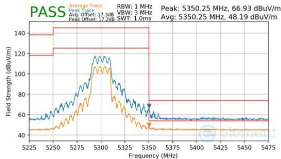
Plot 7-1110. CDD Diversity (Peak & Average, RU242, Index 61, Ch.60, MCS11)
