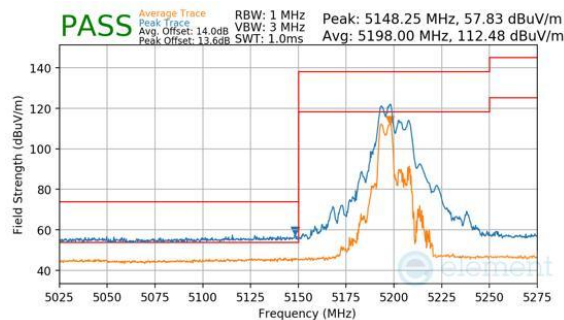
Plot 7-1089. CDD Diversity (Peak & Average, RU52+26, Index 70, Ch.40, MCS11)
