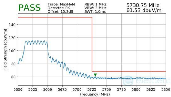
Plot 7-1147. CDD Diversity (Peak, RU484, Index 65, Ch.126, MCS11)
