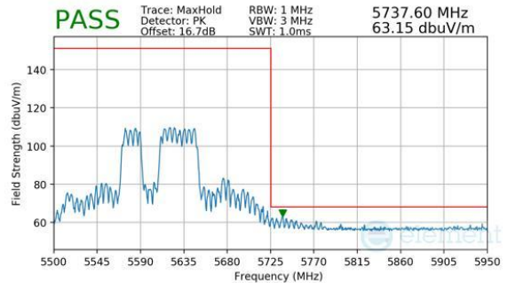
Plot 7-1180. CDD Diversity (Peak, RU484+242, Index 91, Ch.122, MCS11)
