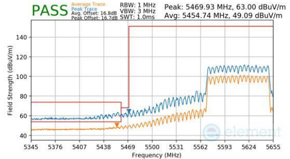
Plot 7-1194. CDD Diversity (Peak & Average, RU996, Index 67, Ch.122, MCS11)
