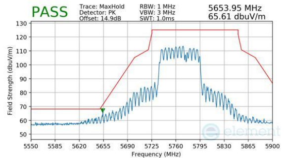
Plot 7-1186. CDD Diversity (Peak, RU484+242, Index 93, Ch.155, MCS11)
