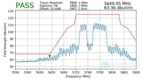
Plot 7-1184. CDD Diversity (Peak, RU484+242, Index 91, Ch.155, MCS11)
