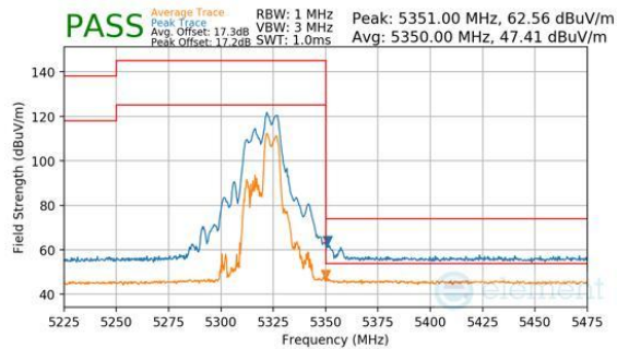
Plot 7-1094. CDD Diversity (Peak & Average, RU52+26, Index 72, Ch.64, MCS11)
