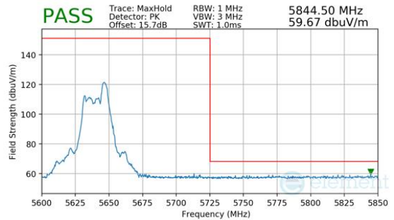
Plot 7-1137. CDD Diversity (Peak, RU52, Index 44, Ch.126, MCS11)
