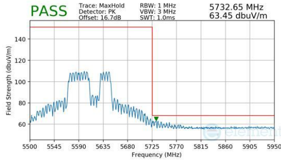
Plot 7-1181. CDD Diversity (Peak, RU484+242, Index 92, Ch.122, MCS11)
