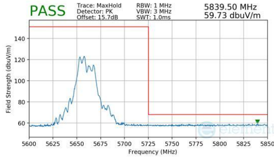
Plot 7-1099. CDD Diversity (Peak, RU52+26, Index 70, Ch.132, MCS11)
