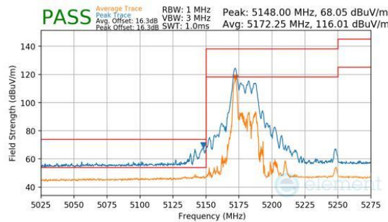
Plot 7-1151. CDD Diversity (Peak & Average, RU26, Index 0, Ch.42, MCS11)
