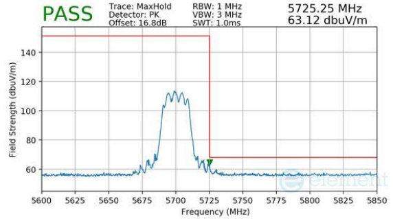
Plot 7-1117. CDD Diversity (Peak, RU242, Index 61, Ch.140, MCS11)
