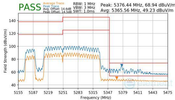
Plot 7-1029. CDD Primary (Peak & Average, RU996+484+242, Index 97 (L), Ch.50, MCS11)
