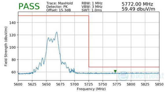
Plot 7-1082. CDD Diversity (Peak, RU52, Index 40, Ch.132, MCS11)
