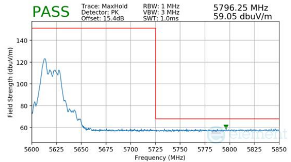
Plot 7-1077. CDD Diversity (Peak, RU52, Index 37, Ch.124, MCS11)
