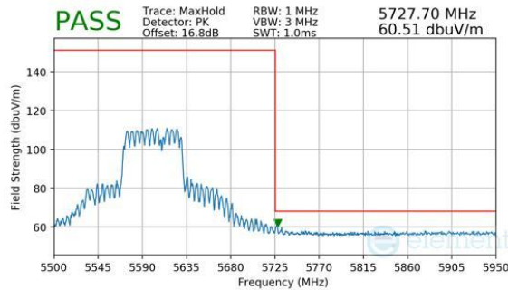
Plot 7-1182. CDD Diversity (Peak, RU484+242, Index 93, Ch.122, MCS11)
