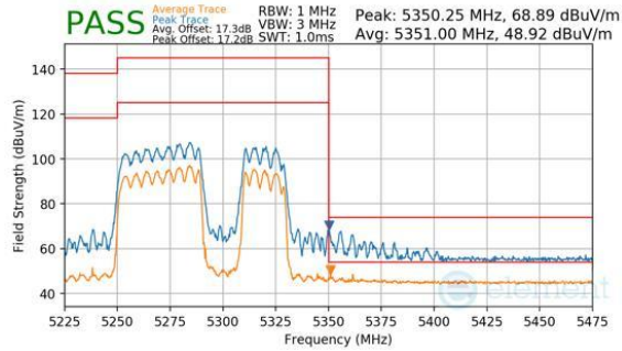
Plot 7-1169. CDD Diversity (Peak & Average, RU484+242, Index 92, Ch.58, MCS11)
