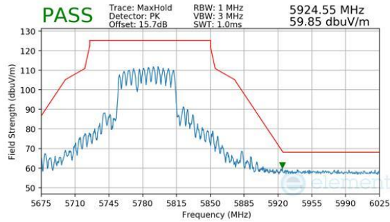
Plot 7-1187. CDD Diversity (Peak, RU484+242, Index 90, Ch.155, MCS11)
