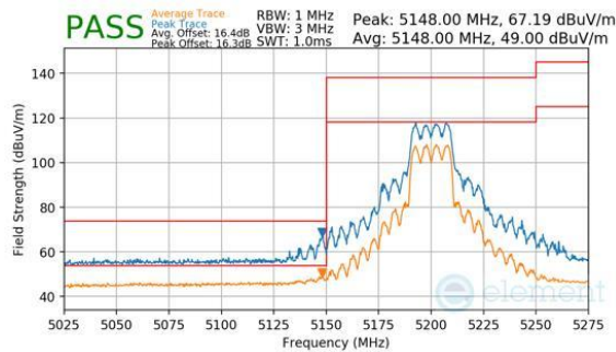
Plot 7-1109. CDD Diversity (Peak & Average, RU242, Index 61, Ch.40, MCS11)
