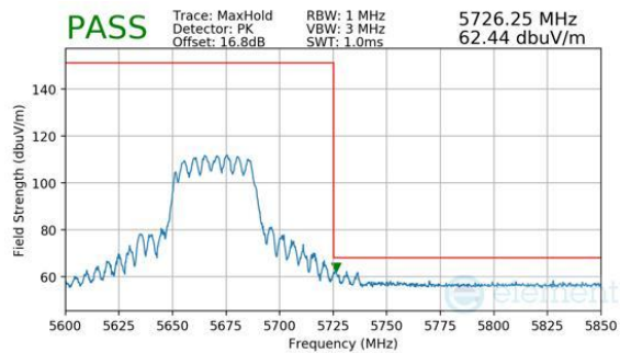
Plot 7-1148. CDD Diversity (Peak, RU484, Index 65, Ch.134, MCS11)
