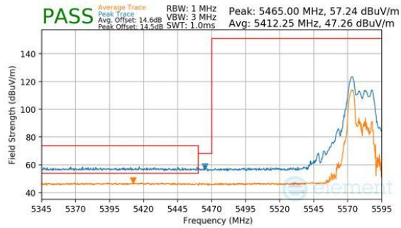
Plot 7-1073. CDD Diversity (Peak & Average, RU52, Index 37, Ch.116, MCS11)
