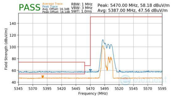
Plot 7-1065. CDD Diversity (Peak & Average, RU52, Index 37, Ch.100, MCS11)
