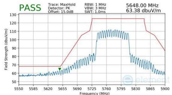
Plot 7-1196. CDD Diversity (Peak, RU996, Index 67, Ch.155, MCS11)
