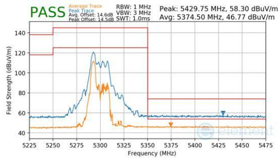
Plot 7-1061. CDD Diversity (Peak & Average, RU52, Index 37, Ch.60, MCS11)
