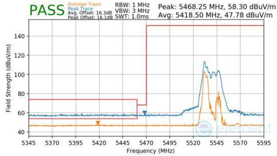
Plot 7-1132. CDD Diversity (Peak & Average, RU52, Index 37, Ch.110, MCS11)
