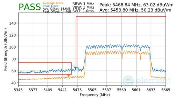
Plot 7-1042. CDD Primary (Peak & Average, RU996+484+242, Index 99 (H), Ch.114, MCS11)
