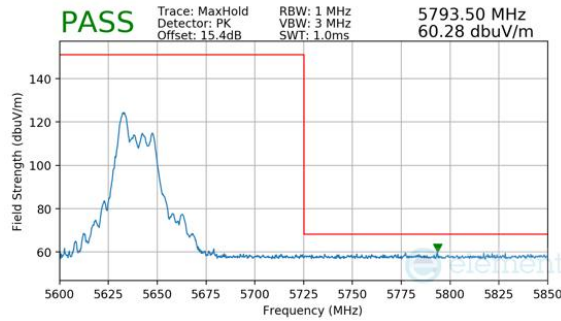
Plot 7-1079. CDD Diversity (Peak, RU52, Index 37, Ch.128, MCS11)
