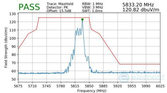
Plot 7-1060. CDD Diversity (Peak, RU26, Index 8, Ch.165, MCS11)
