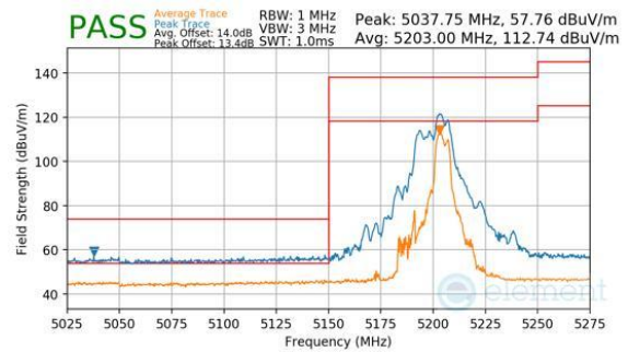
Plot 7-1090. CDD Diversity (Peak & Average, RU52+26, Index 72, Ch.40, MCS11)
