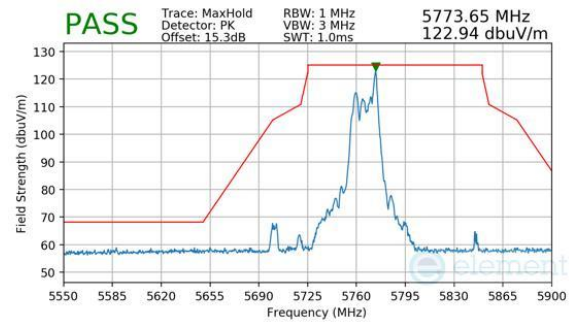
Plot 7-1123. CDD Diversity (Peak, RU26, Index 17, Ch.151, MCS11)
