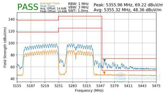
Plot 7-1028. CDD Primary (Peak & Average, RU996+484+242, Index 96 (H), Ch.50, MCS11)
