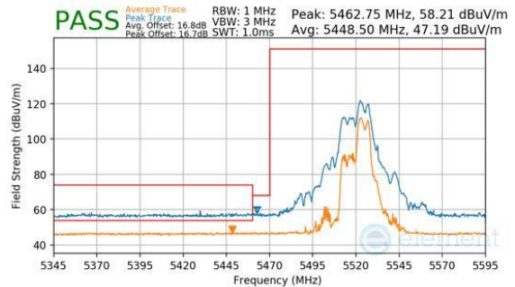
Plot 7-1098. CDD Diversity (Peak & Average, RU52+26, Index 72, Ch.104, MCS11)
