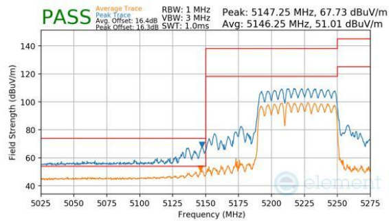
Plot 7-1163. CDD Diversity (Peak & Average, RU484+242, Index 90, Ch.42, MCS11)
