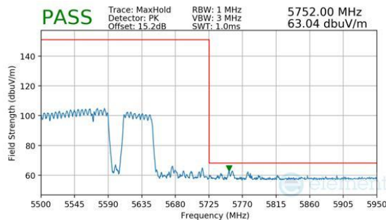
Plot 7-1046. CDD Primary (Peak, RU996+484+242, Index 97 (H), Ch.114, MCS11)
