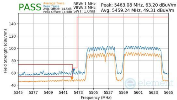
Plot 7-1041. CDD Primary (Peak & Average, RU996+484+242, Index 99 (L), Ch.114, MCS11)
