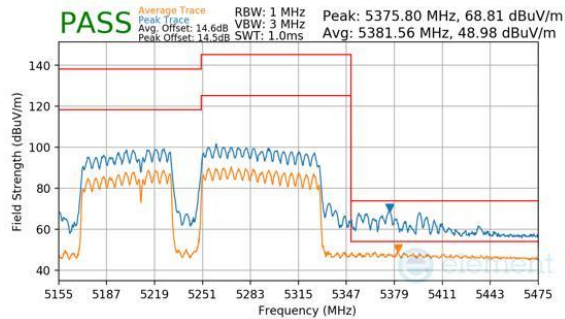
Plot 7-1033. CDD Primary (Peak & Average, RU996+484+242, Index 99 (L), Ch.50, MCS11)
