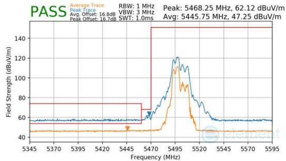
Plot 7-1095. CDD Diversity (Peak & Average, RU52+26, Index 70, Ch.100, MCS11)
