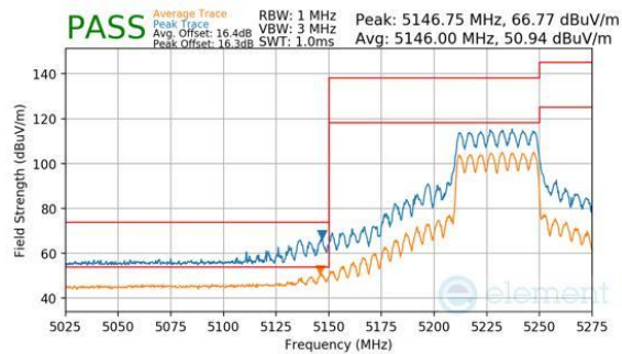
Plot 7-1141. CDD Diversity (Peak & Average, RU484, Index 65, Ch.46, MCS11)
