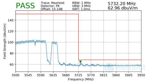
Plot 7-1048. CDD Primary (Peak, RU996+484+242, Index 98 (H), Ch.114, MCS11)
