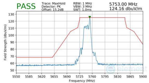
Plot 7-1058. CDD Diversity (Peak, RU26, Index 8, Ch.149, MCS11)
