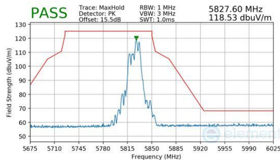
Plot 7-1107. CDD Diversity (Peak, RU52+26, Index 72, Ch.165, MCS11)
