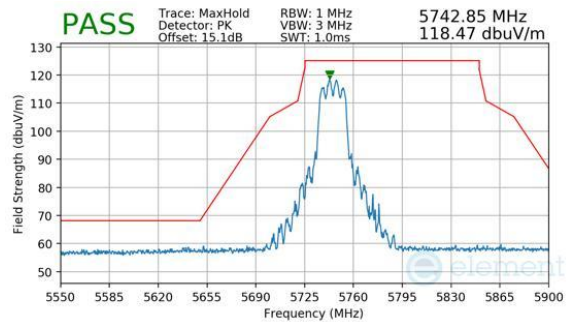
Plot 7-1118. CDD Diversity (Peak, RU242, Index 61, Ch.149, MCS11)
