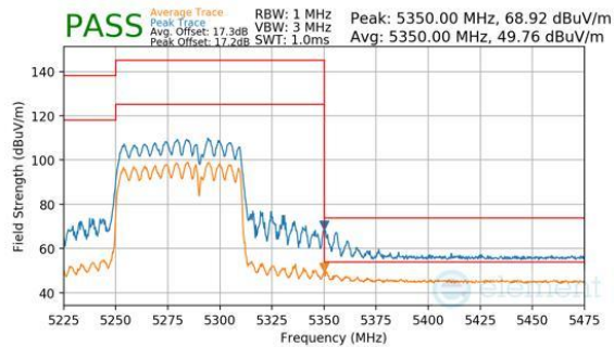
Plot 7-1170. CDD Diversity (Peak & Average, RU484+242, Index 93, Ch.58, MCS11)
