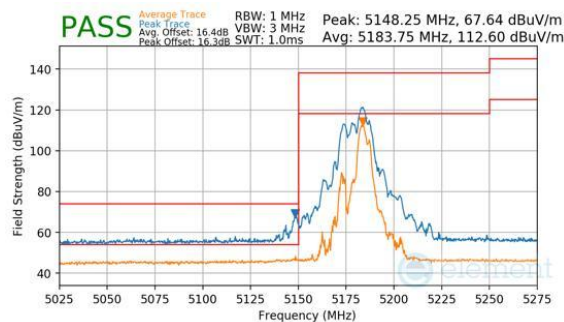
Plot 7-1088. CDD Diversity (Peak & Average, RU52+26, Index 72, Ch.36, MCS11)
