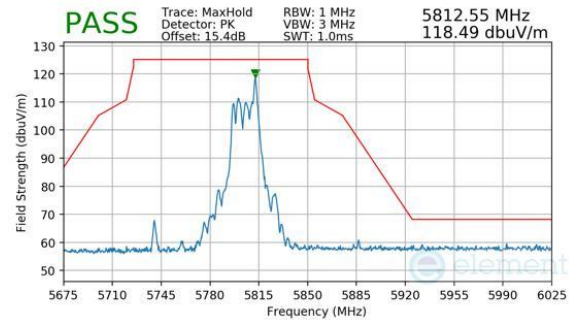
Plot 7-1125. CDD Diversity (Peak, RU26, Index 17, Ch.159, MCS11)
