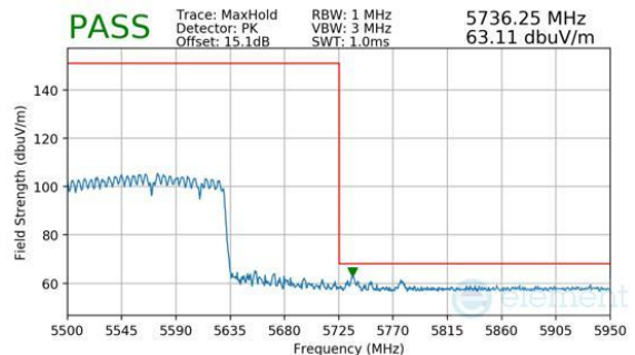
Plot 7-1050. CDD Primary (Peak, RU996+484+242, Index 99 (H), Ch.114, MCS11)
