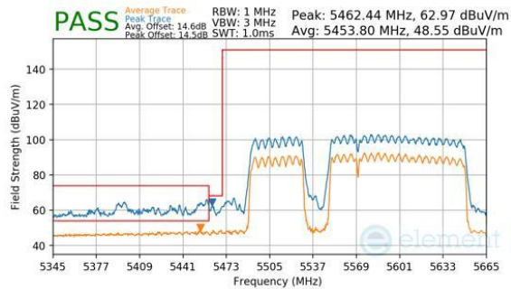
Plot 7-1040. CDD Primary (Peak & Average, RU996+484+242, Index 98 (L), Ch.114, MCS11)
