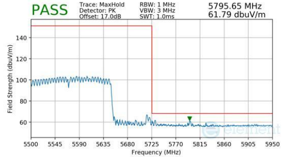
Plot 7-1054. CDD Primary (Peak, RU996X2, Index 68, Ch.114, MCS11)
