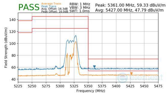
Plot 7-1129. CDD Diversity (Peak & Average, RU52, Index 44, Ch.62, MCS11)
