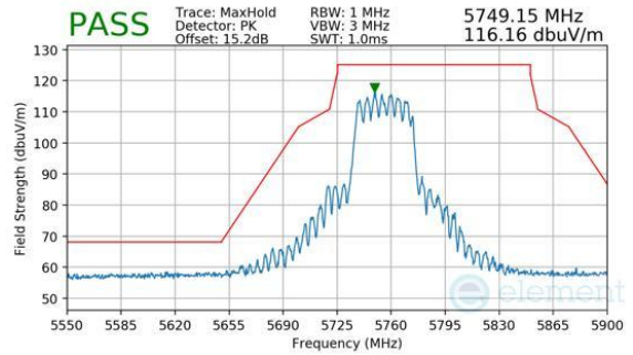
Plot 7-1149. CDD Diversity (Peak, RU484, Index 65, Ch.151, MCS11)
