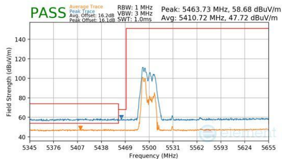
Plot 7-1159. CDD Diversity (Peak & Average, RU52, Index 37, Ch.106, MCS11)
