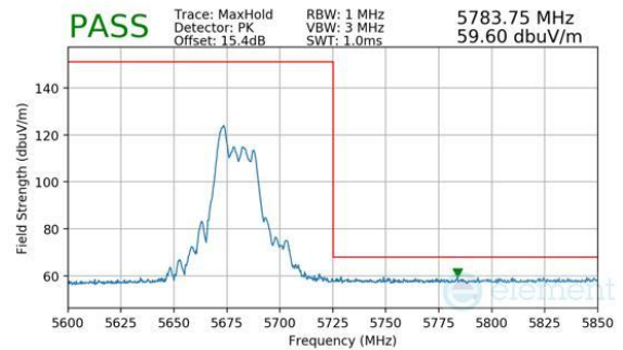
Plot 7-1083. CDD Diversity (Peak, RU52, Index 37, Ch.136, MCS11)
