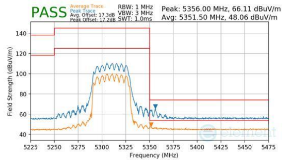
Plot 7-1143. CDD Diversity (Peak & Average, RU484, Index 65, Ch.62, MCS11)
