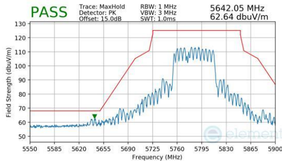
Plot 7-1183. CDD Diversity (Peak, RU484+242, Index 90, Ch.155, MCS11)
