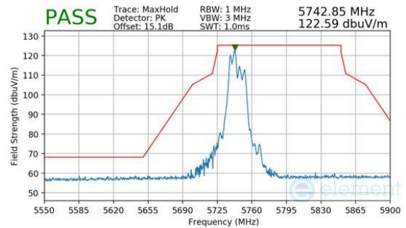
Plot 7-1104. CDD Diversity (Peak, RU52+26, Index 70, Ch.149, MCS11)
