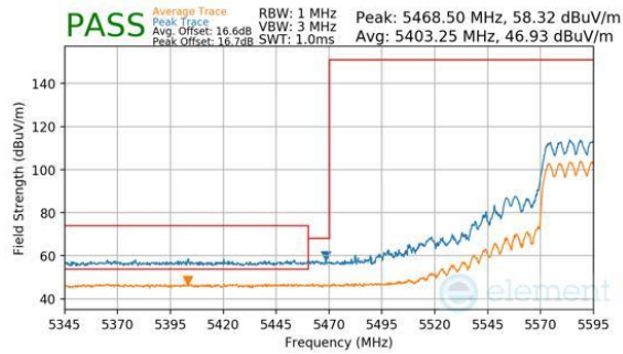
Plot 7-1146. CDD Diversity (Peak & Average, RU484, Index 65, Ch.118, MCS11)
