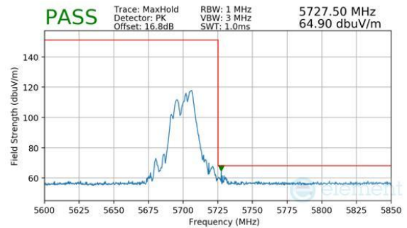
Plot 7-1103. CDD Diversity (Peak, RU52+26, Index 72, Ch.140, MCS11)
