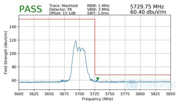
Plot 7-1085. CDD Diversity (Peak, RU52, Index 37, Ch.140, MCS11)
