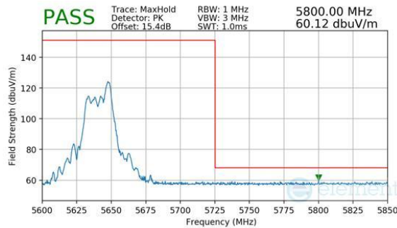
Plot 7-1080. CDD Diversity (Peak, RU52, Index 40, Ch.128, MCS11)
