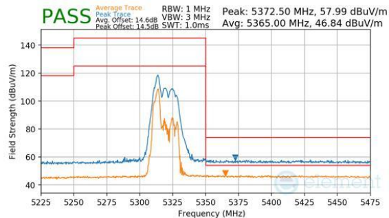
Plot 7-1063. CDD Diversity (Peak & Average, RU52, Index 37, Ch.64, MCS11)
