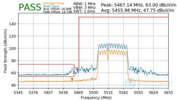
Plot 7-1171. CDD Diversity (Peak & Average, RU484+242, Index 90, Ch.106, MCS11)
