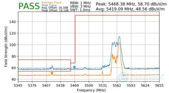
Plot 7-1160. CDD Diversity (Peak & Average, RU52, Index 52, Ch.106, MCS11)
