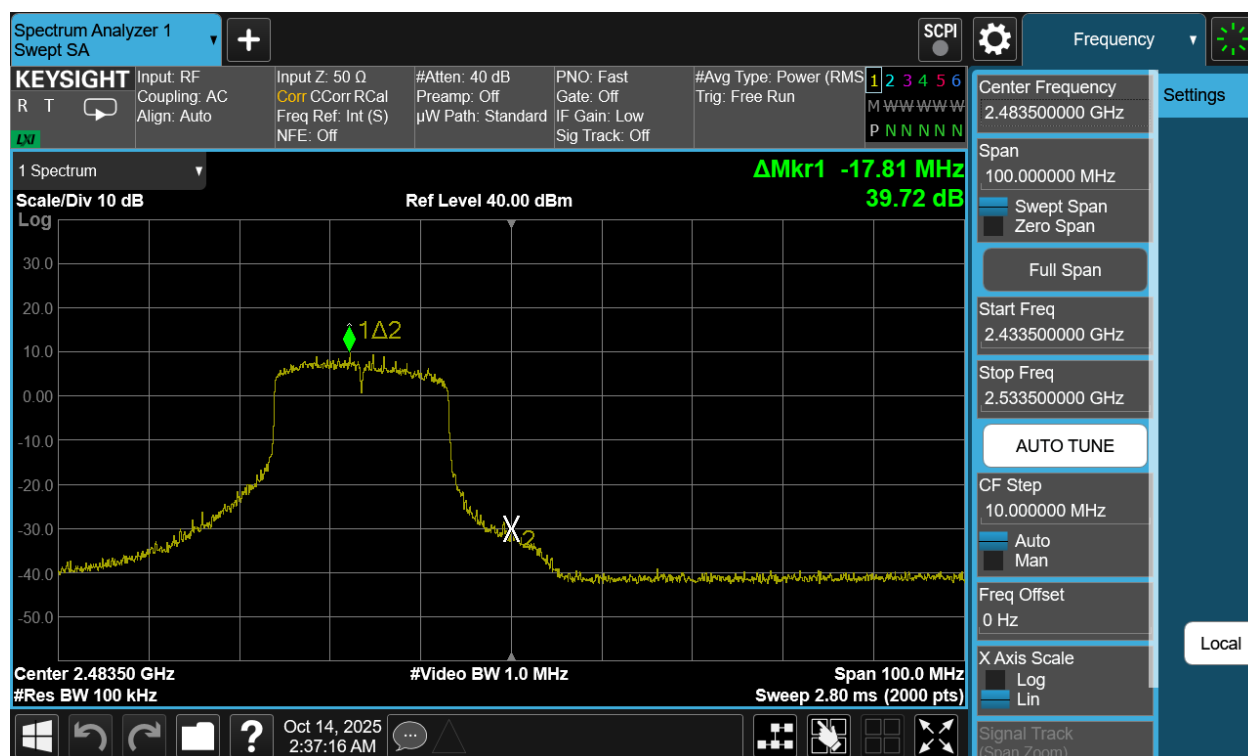
Plot 7-76. Band Edge Plot Antenna 3a (802.11be (SU - 2.4GHz) – Ch. 12)
