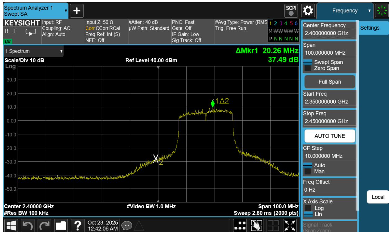
Plot 7-107. Band Edge Plot Antenna 1a (802.11be (SU - 2.4GHz) – Ch. 2)
