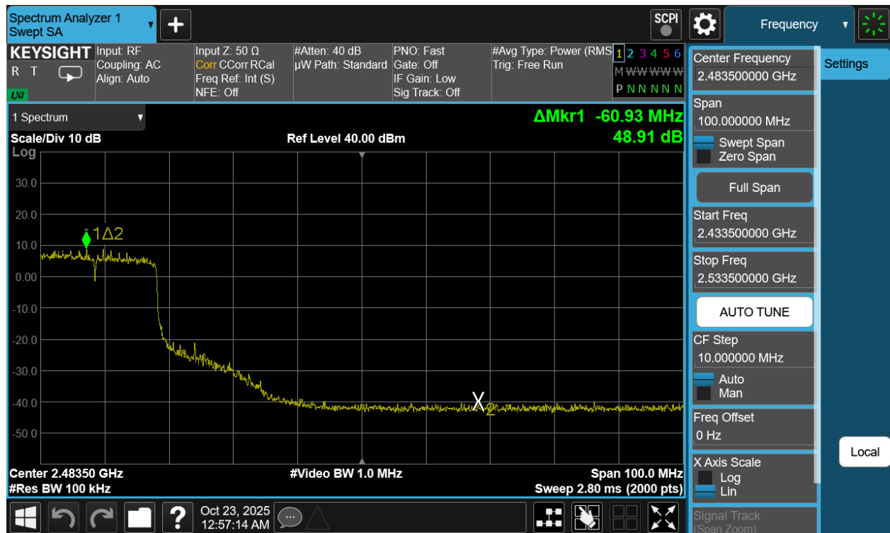
Plot 7-110. Band Edge Plot Antenna 1a (802.11be (SU - 2.4GHz) – Ch. 7)
