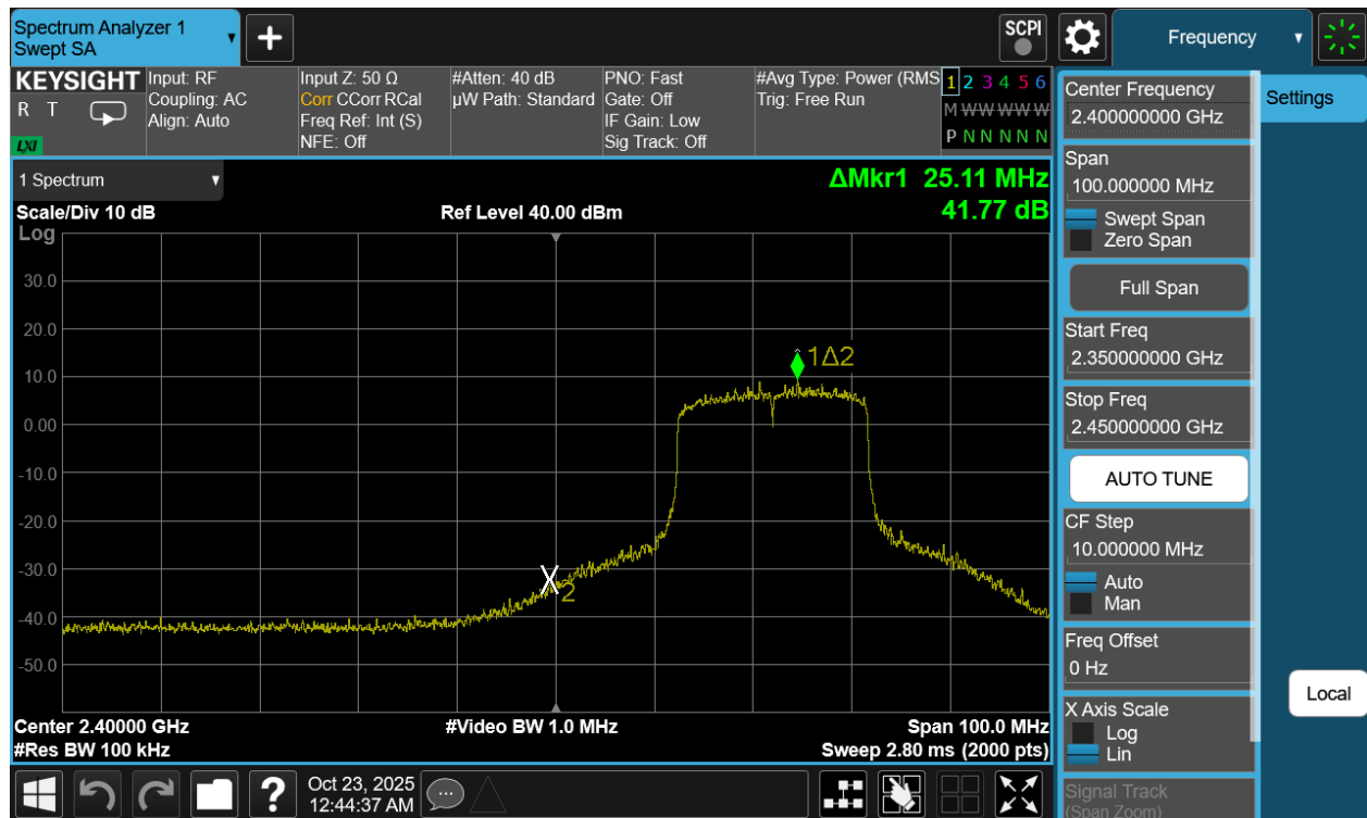
Plot 7-108. Band Edge Plot Antenna 1a (802.11be (SU - 2.4GHz) – Ch. 3)
