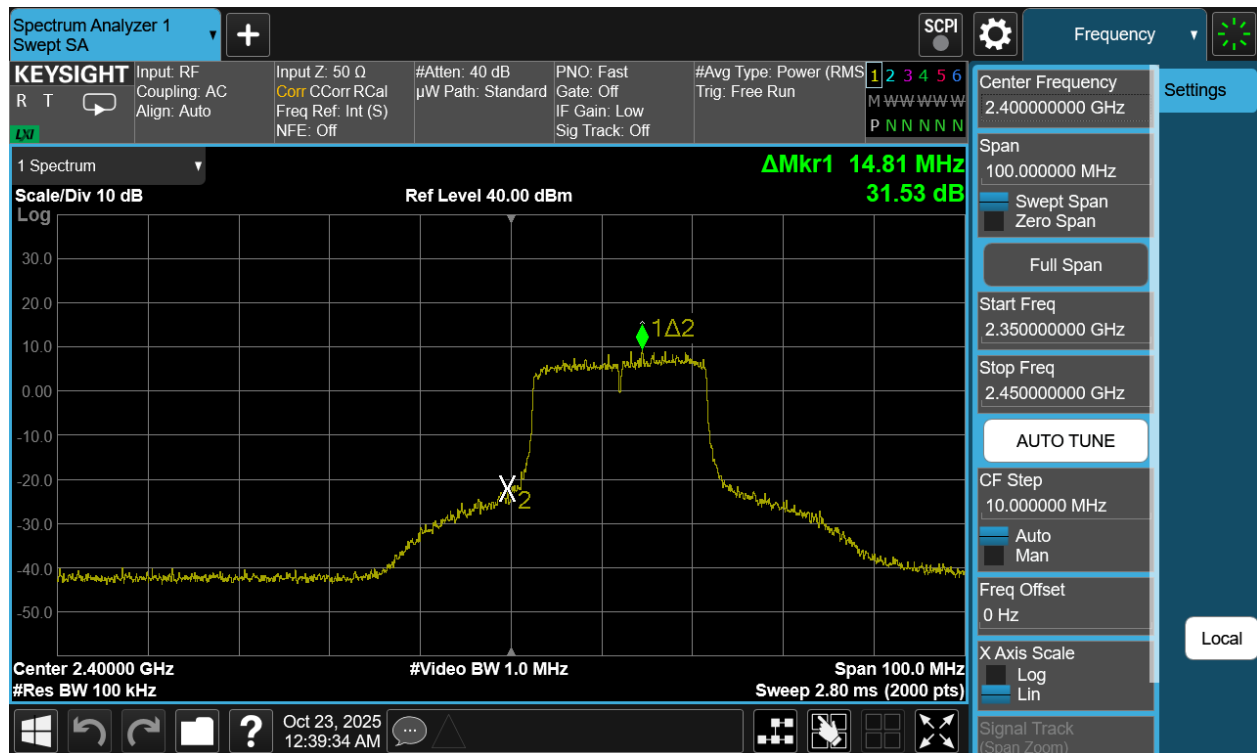
Plot 7-106. Band Edge Plot Antenna 1a (802.11be (SU - 2.4GHz) – Ch. 1)
