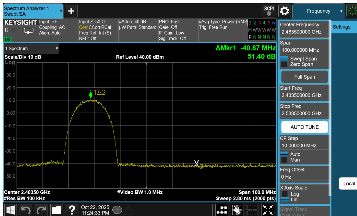
Plot 7-81. Band Edge Plot Antenna 1a (802.11b – Ch. 11)
