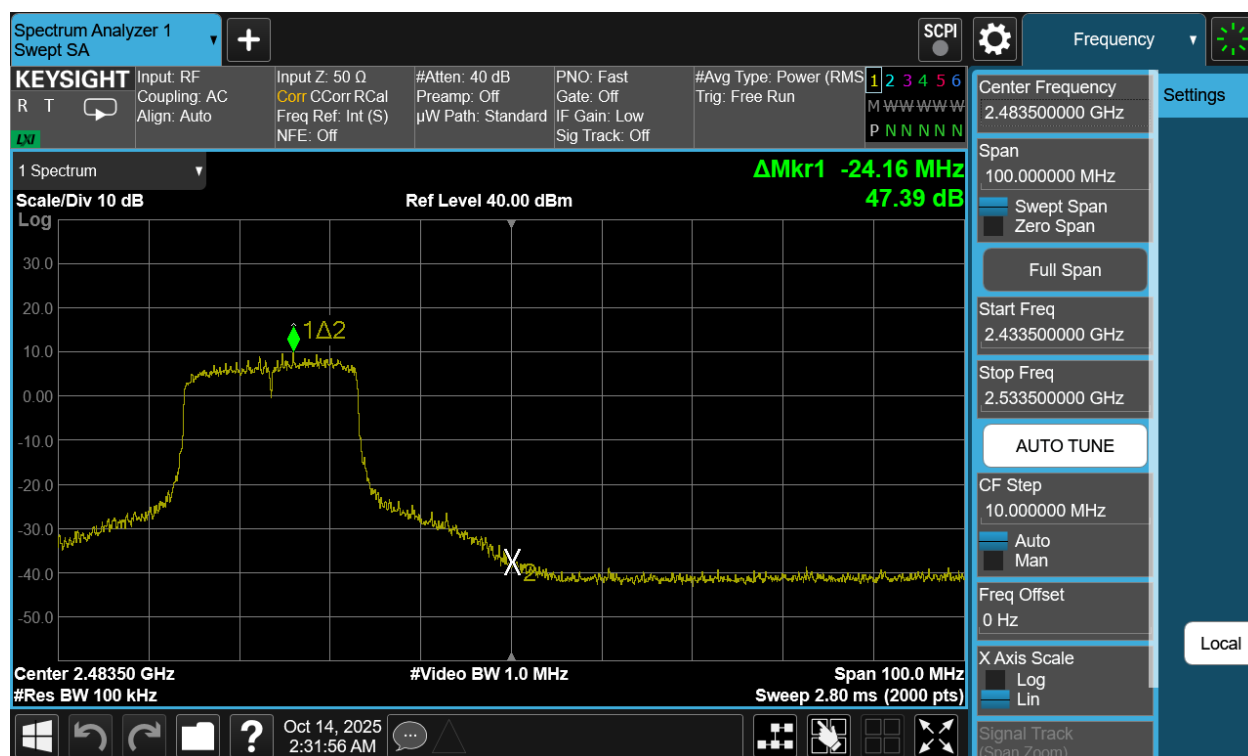
Plot 7-74. Band Edge Plot Antenna 3a (802.11be (SU - 2.4GHz) – Ch. 10)
