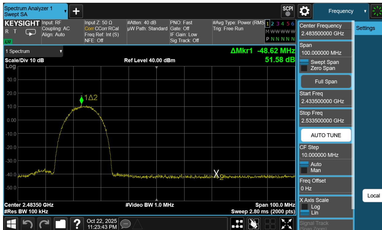
Plot 7-80. Band Edge Plot Antenna 1a (802.11b – Ch. 10)
