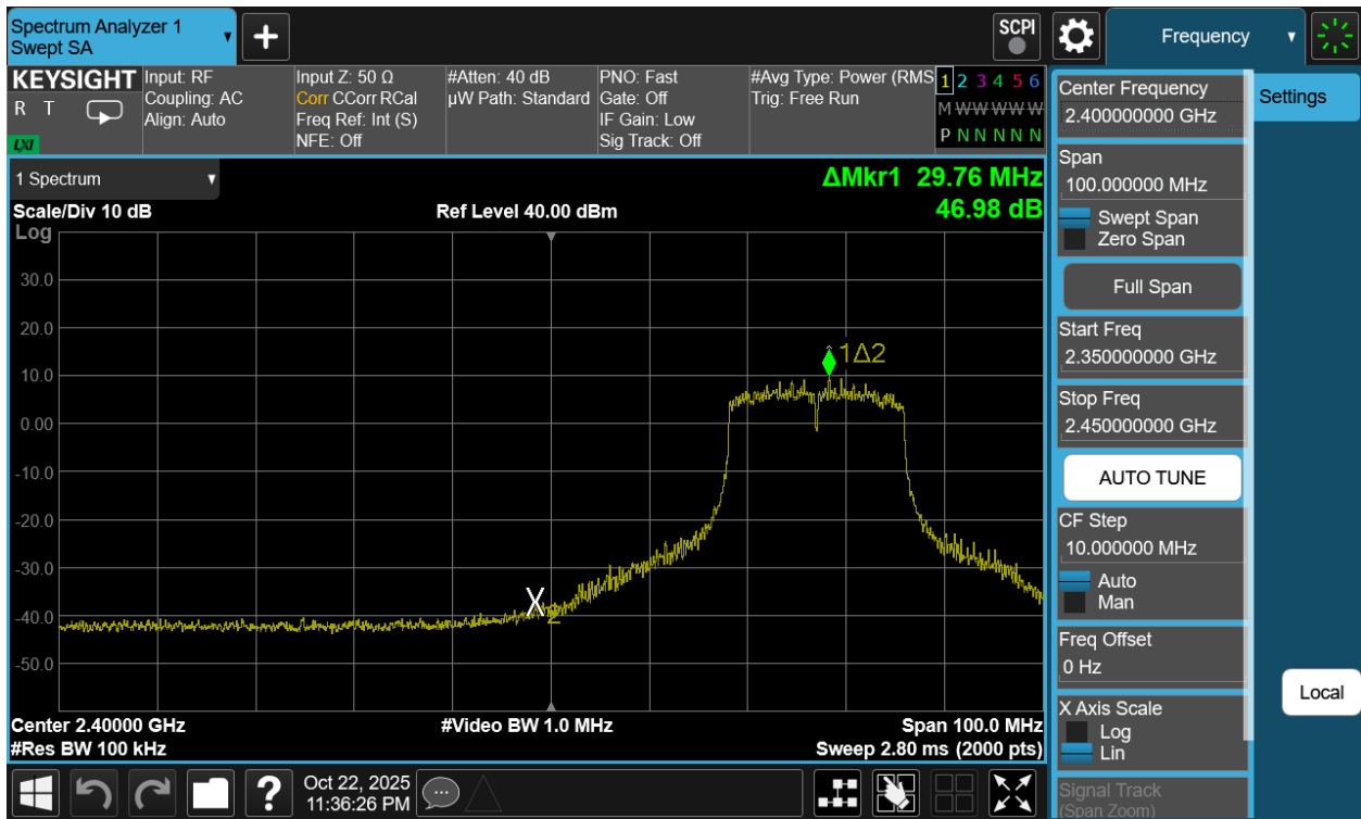
Plot 7-87. Band Edge Plot Antenna 1a (802.11g – Ch. 4)
