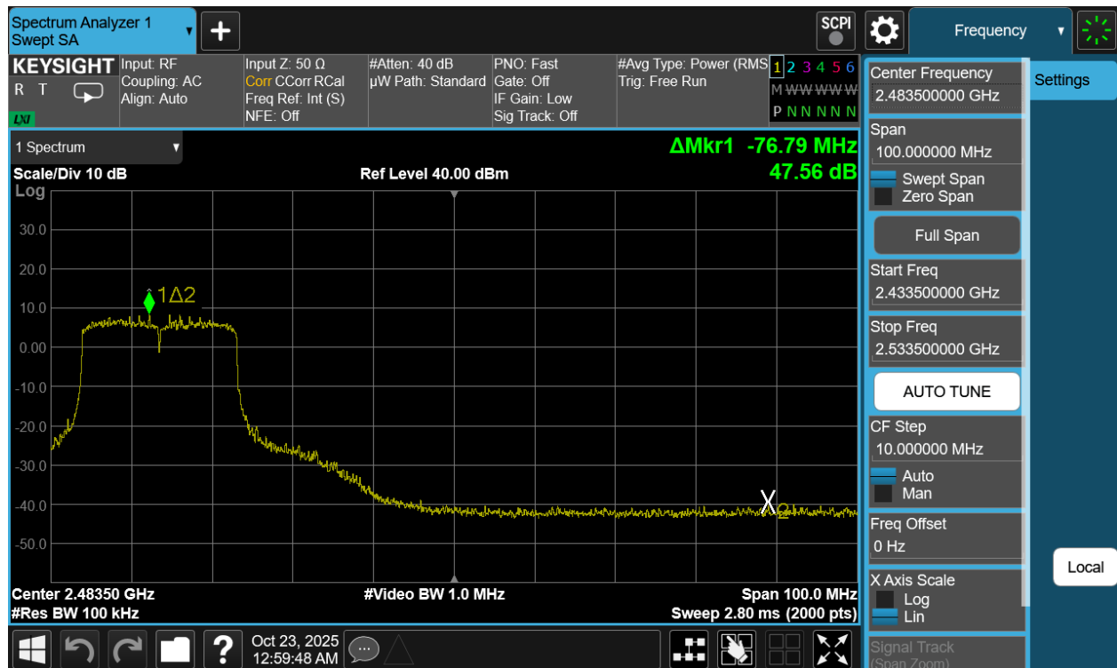
Plot 7-111. Band Edge Plot Antenna 1a (802.11be (SU - 2.4GHz) – Ch. 8)
