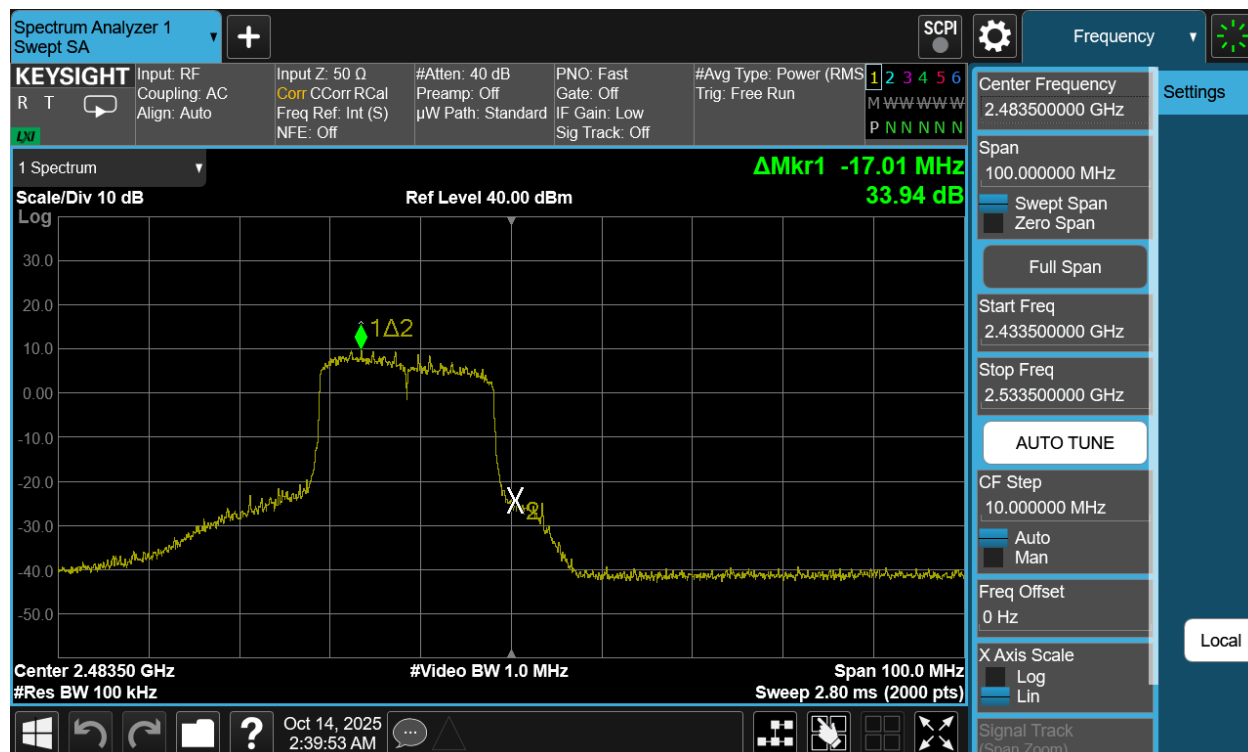
Plot 7-77. Band Edge Plot Antenna 3a (802.11be (SU - 2.4GHz) – Ch. 13)
