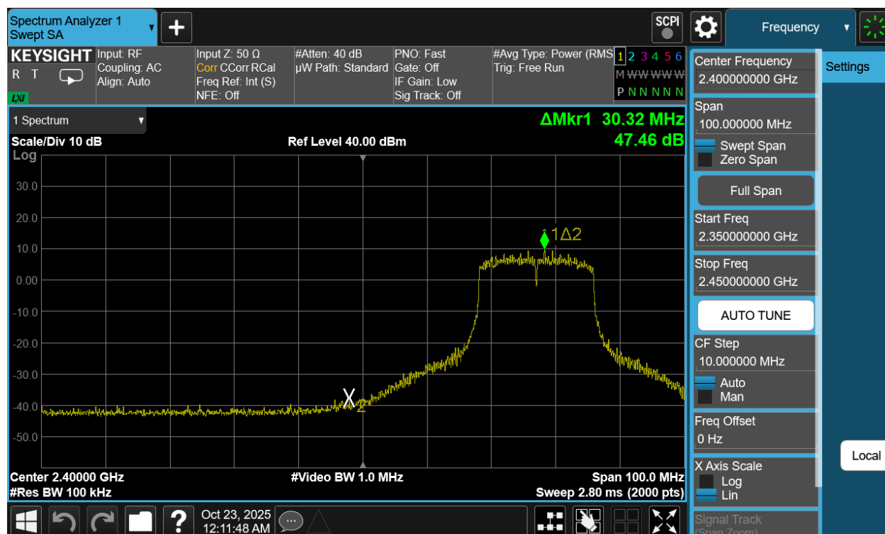
Plot 7-98. Band Edge Plot Antenna 1a (802.11n (2.4GHz) – Ch. 4)
