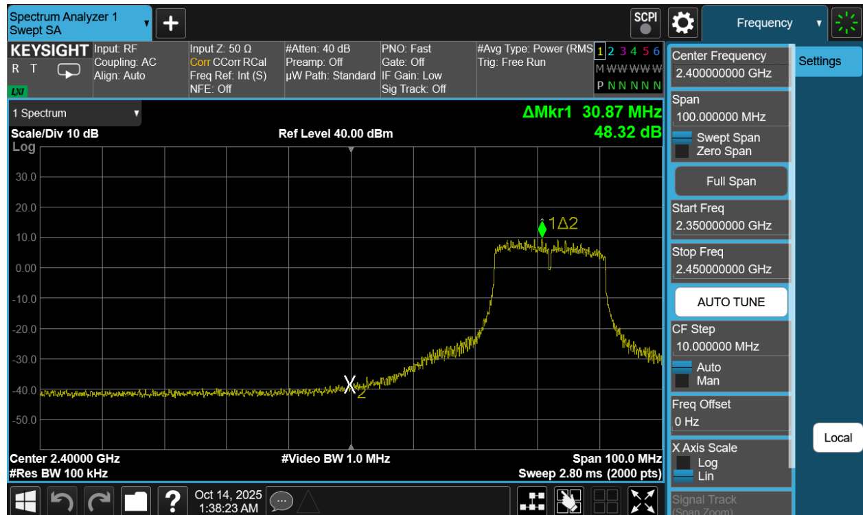
Plot 7-56. Band Edge Plot Antenna 3a (802.11n (2.4GHz) – Ch. 5)
