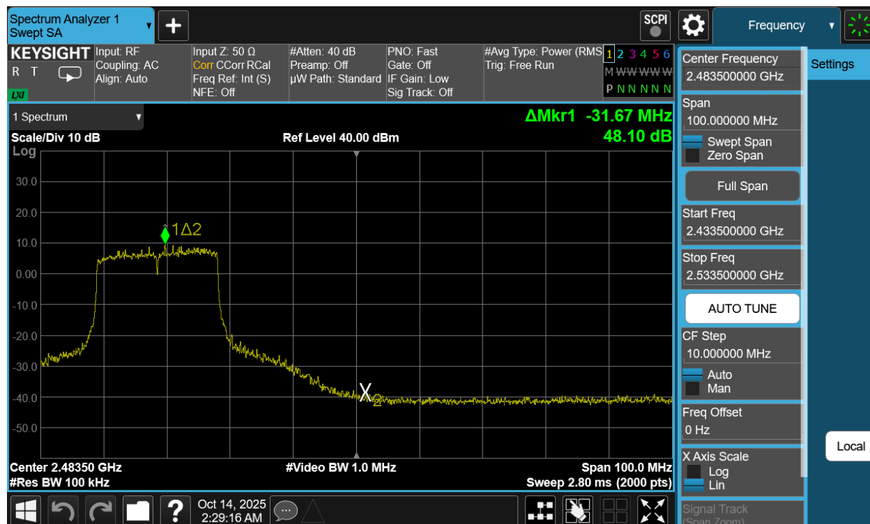
Plot 7-73. Band Edge Plot Antenna 3a (802.11be (SU - 2.4GHz) – Ch. 9)
