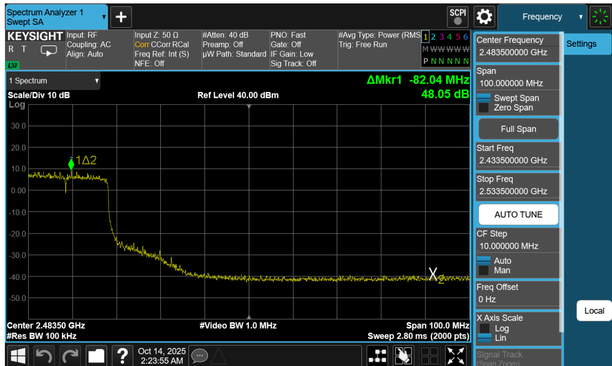
Plot 7-71. Band Edge Plot Antenna 3a (802.11be (SU - 2.4GHz) – Ch. 7)
