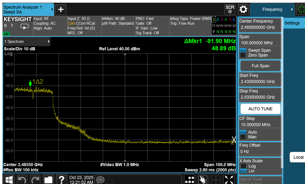
Plot 7-99. Band Edge Plot Antenna 1a (802.11n (2.4GHz) – Ch. 7)
