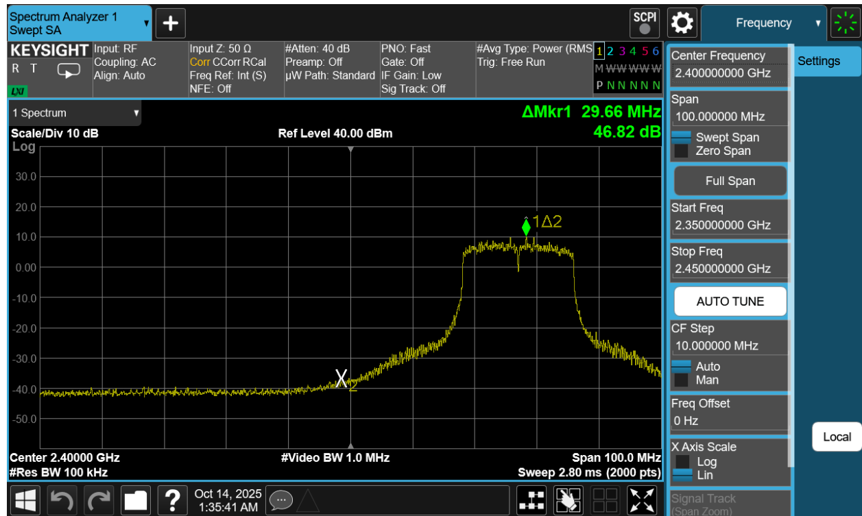
Plot 7-55. Band Edge Plot Antenna 3a (802.11n (2.4GHz) – Ch. 4)
