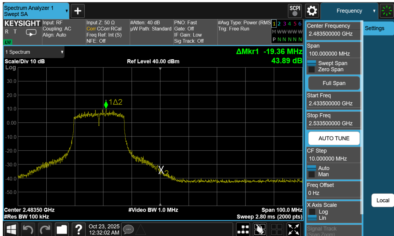
Plot 7-103. Band Edge Plot Antenna 1a (802.11n (2.4GHz) – Ch. 11)
