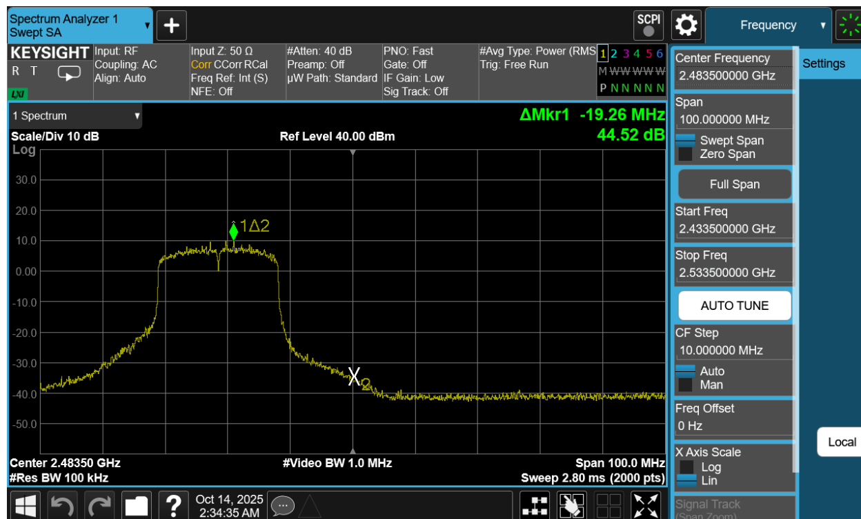
Plot 7-75. Band Edge Plot Antenna 3a (802.11be (SU - 2.4GHz) – Ch. 11)
