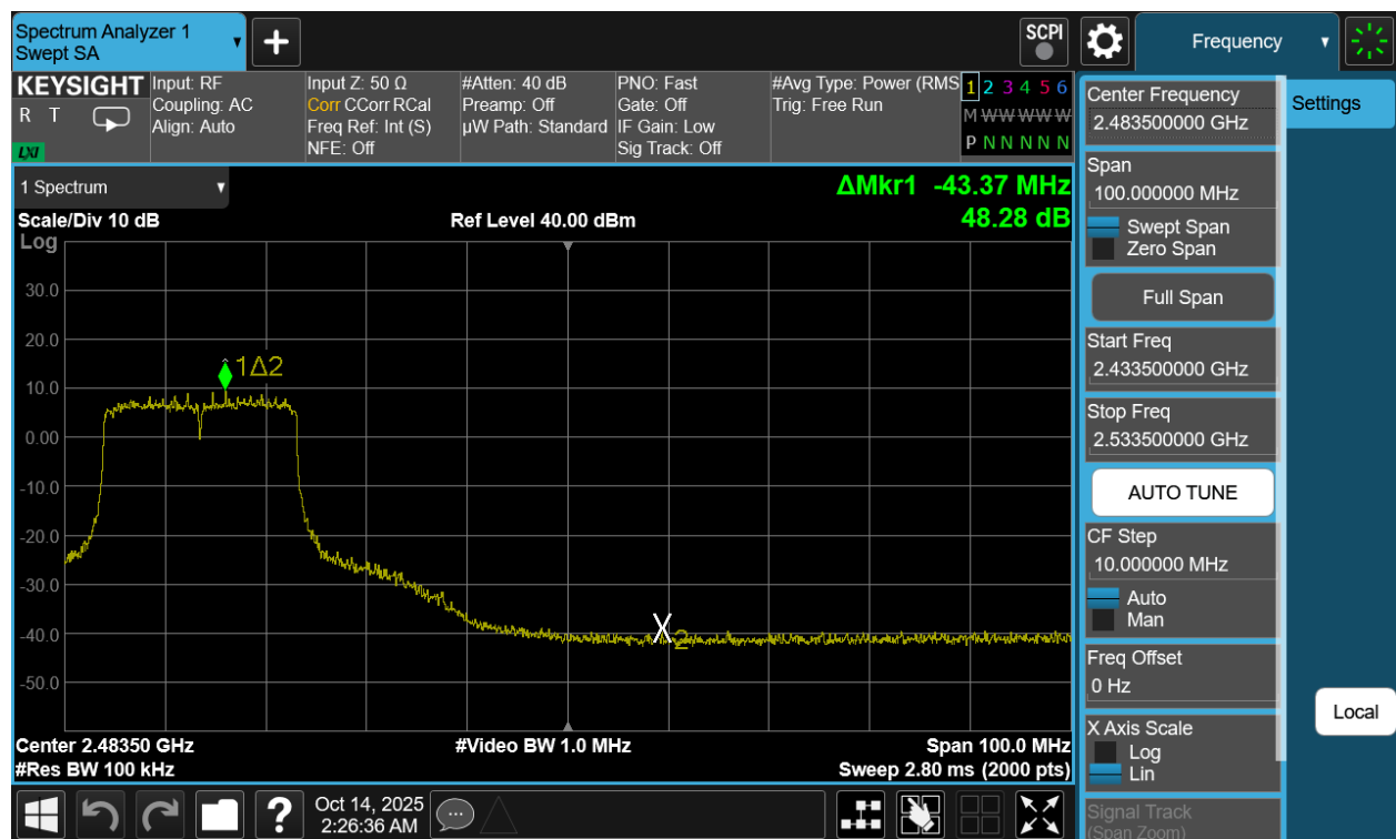
Plot 7-72. Band Edge Plot Antenna 3a (802.11be (SU - 2.4GHz) – Ch. 8)
