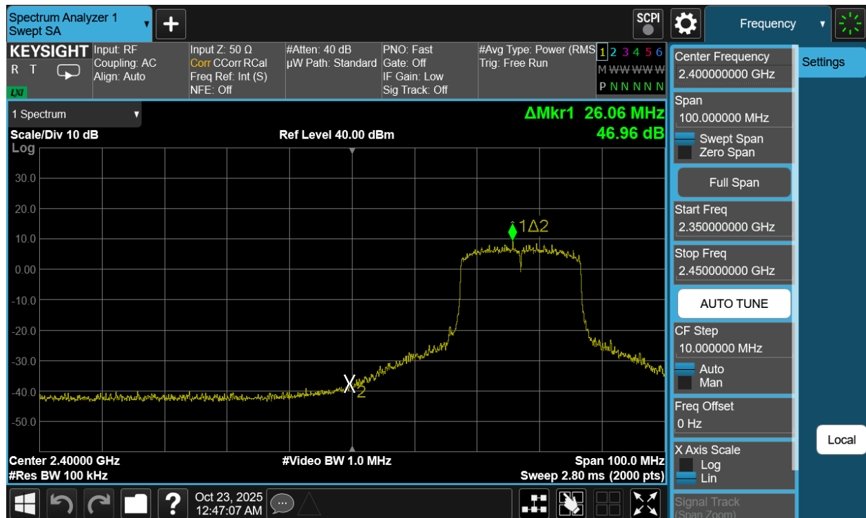
Plot 7-109. Band Edge Plot Antenna 1a (802.11be (SU - 2.4GHz) – Ch. 4)
