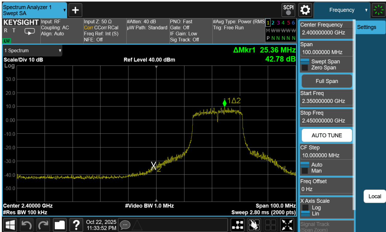
Plot 7-86. Band Edge Plot Antenna 1a (802.11g – Ch. 3)
