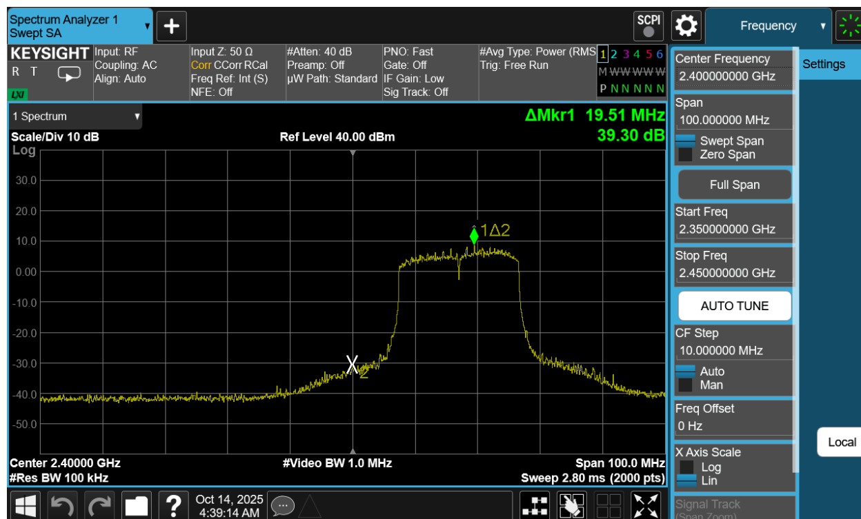
Plot 7-37. Band Edge Antenna 3a (802.11be OFDMA – RU242 – Ch. 2)
