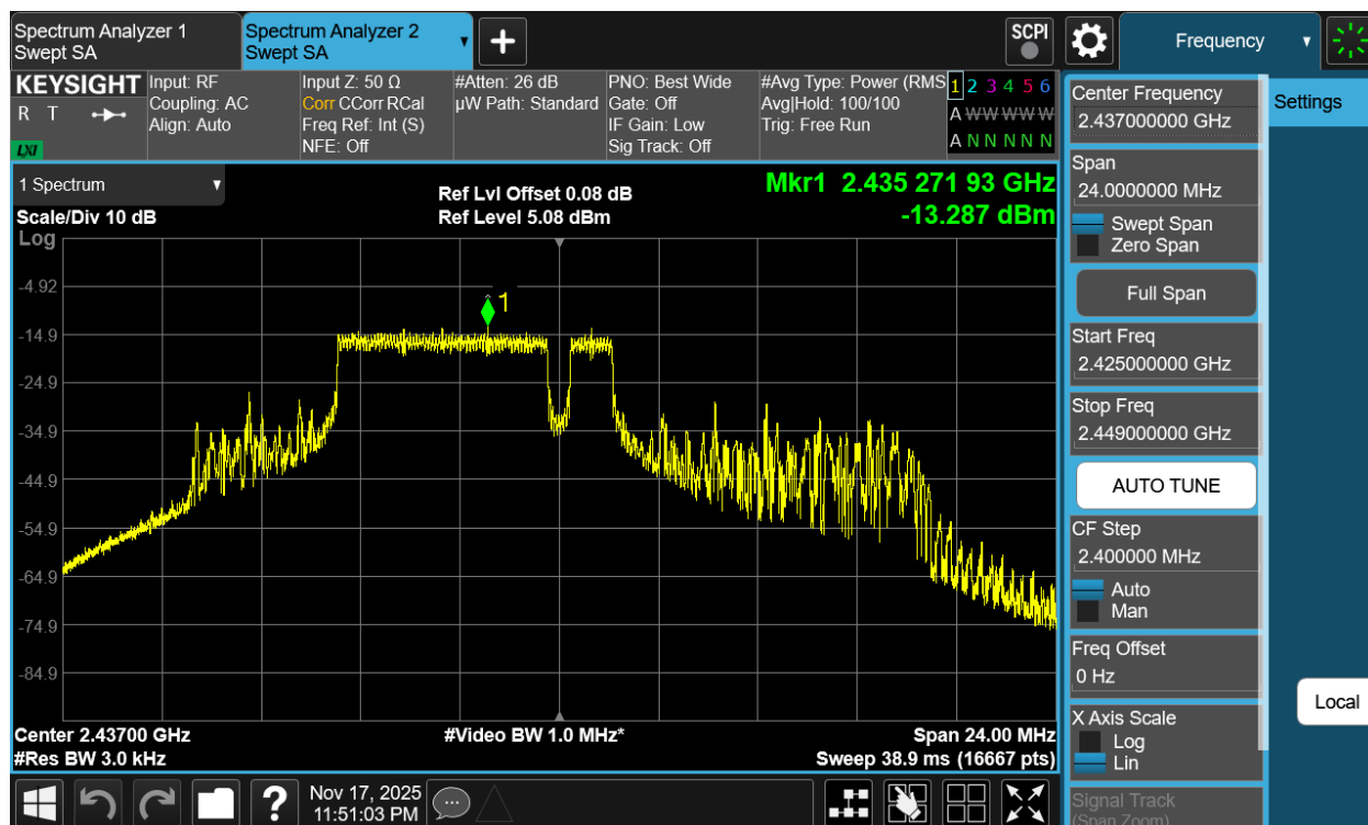
Plot 7-30 PSD CDD Antenna 1a (20MHz BW 802.11be(RU) RU52+26 Index71 - Ch.6)
