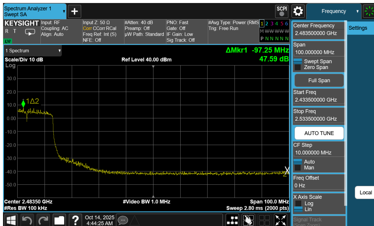
Plot 7-41. Band Edge Antenna 3a (802.11be OFDMA – RU242 – Ch. 6(High Channel))
