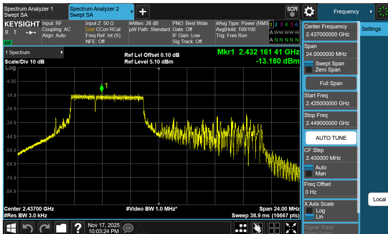
Plot 7-19 PSD Antenna 3a (20MHz BW 802.11be(RU) RU52+26 Index70 - Ch.6)
