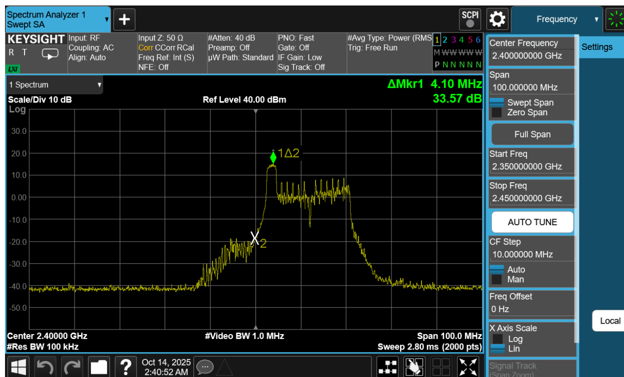
Plot 7-33. Band Edge Antenna 3a (802.11be OFDMA – RU26 Index 0 – Ch. 1)
