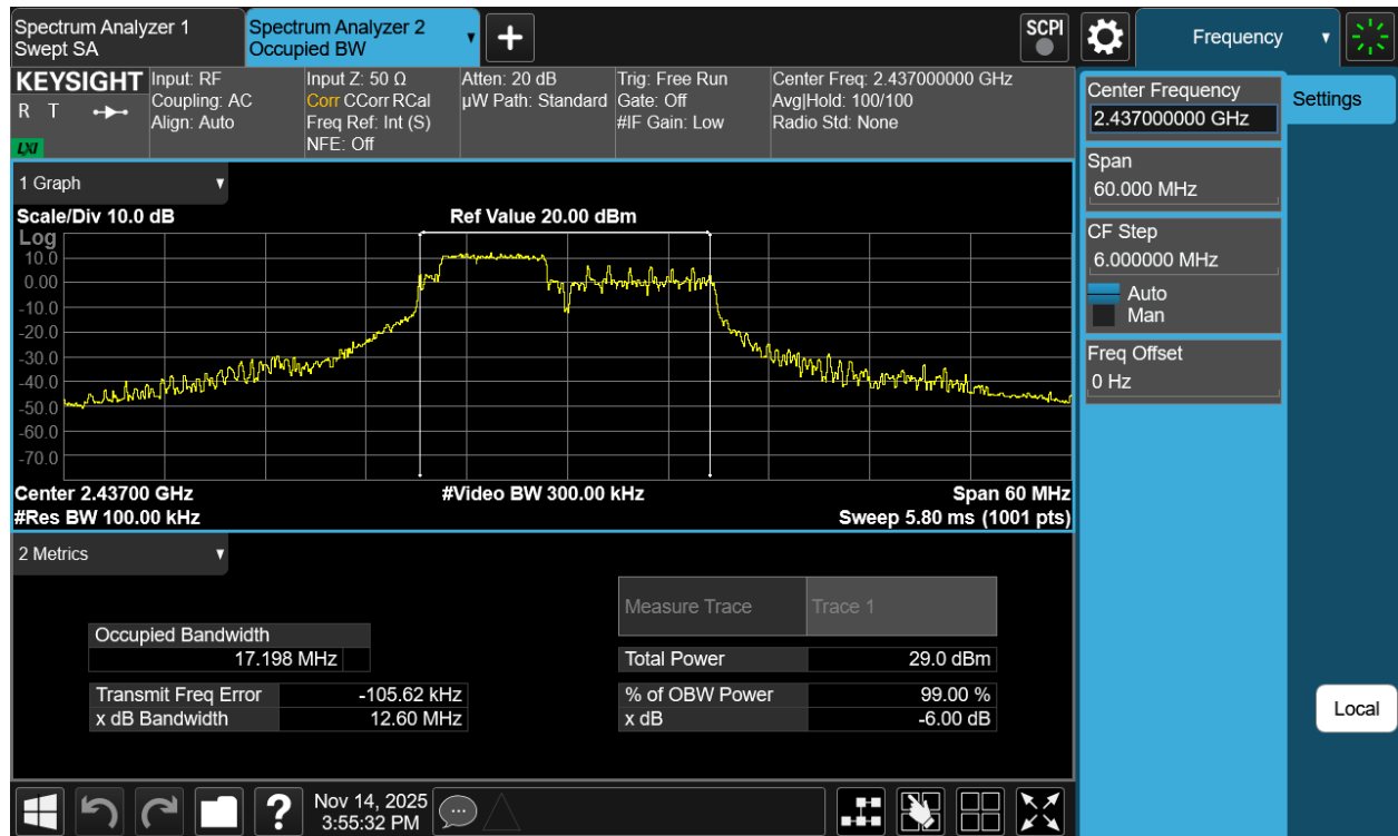
Plot 7-15 6dB BW Antenna 1a (20MHz BW 802.11be(RU) RU52+26 Index70 - Ch.6)
