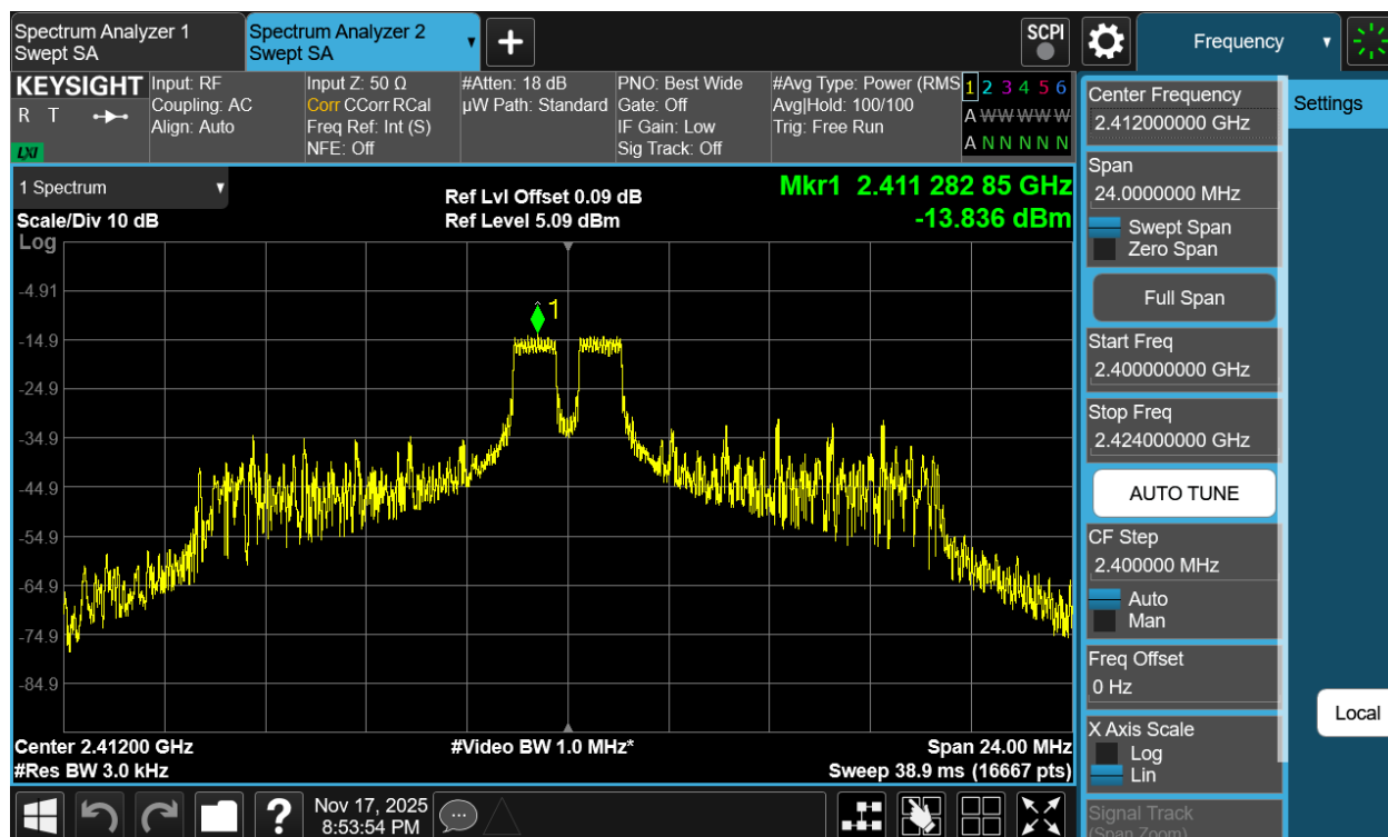
Plot 7-17 PSD Antenna 3a (20MHz BW 802.11be(RU) RU26 Index4 - Ch.1)
