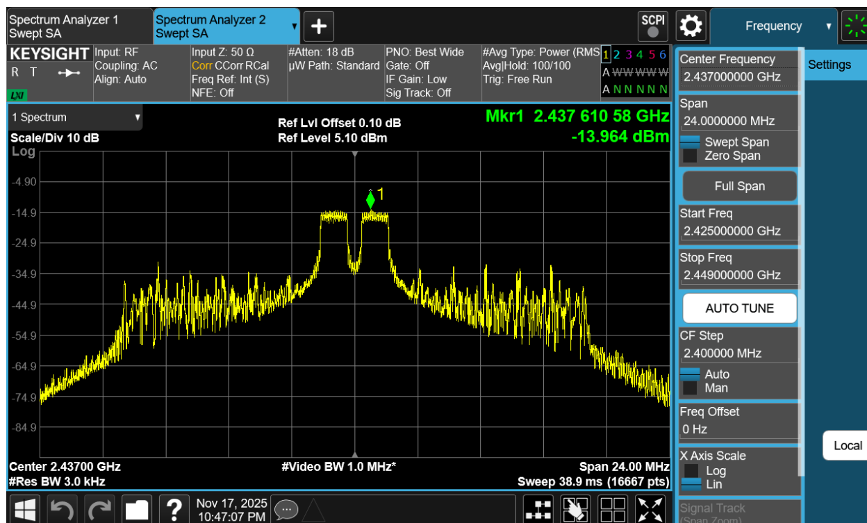
Plot 7-21 PSD Antenna 1a (20MHz BW 802.11be(RU) RU26 Index4 - Ch.6)
