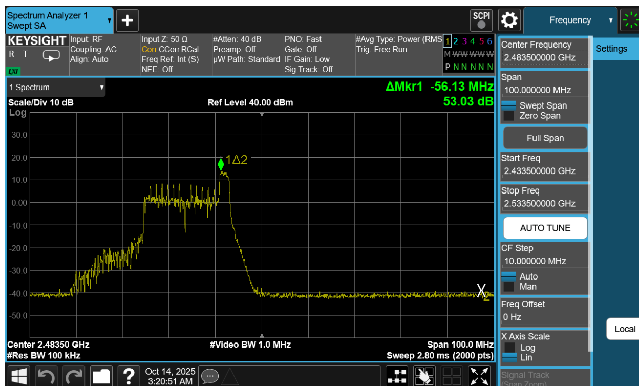
Plot 7-34. Band Edge Antenna 3a (802.11be OFDMA – RU26 Index 8 – Ch. 12)
