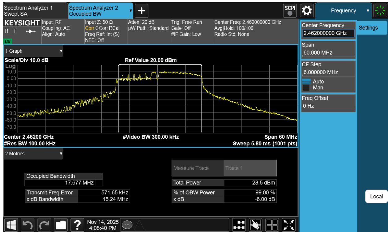
Plot 7-16 6dB BW Antenna 1a (20MHz BW 802.11be(RU) RU106+26 Index83 - Ch.11)
