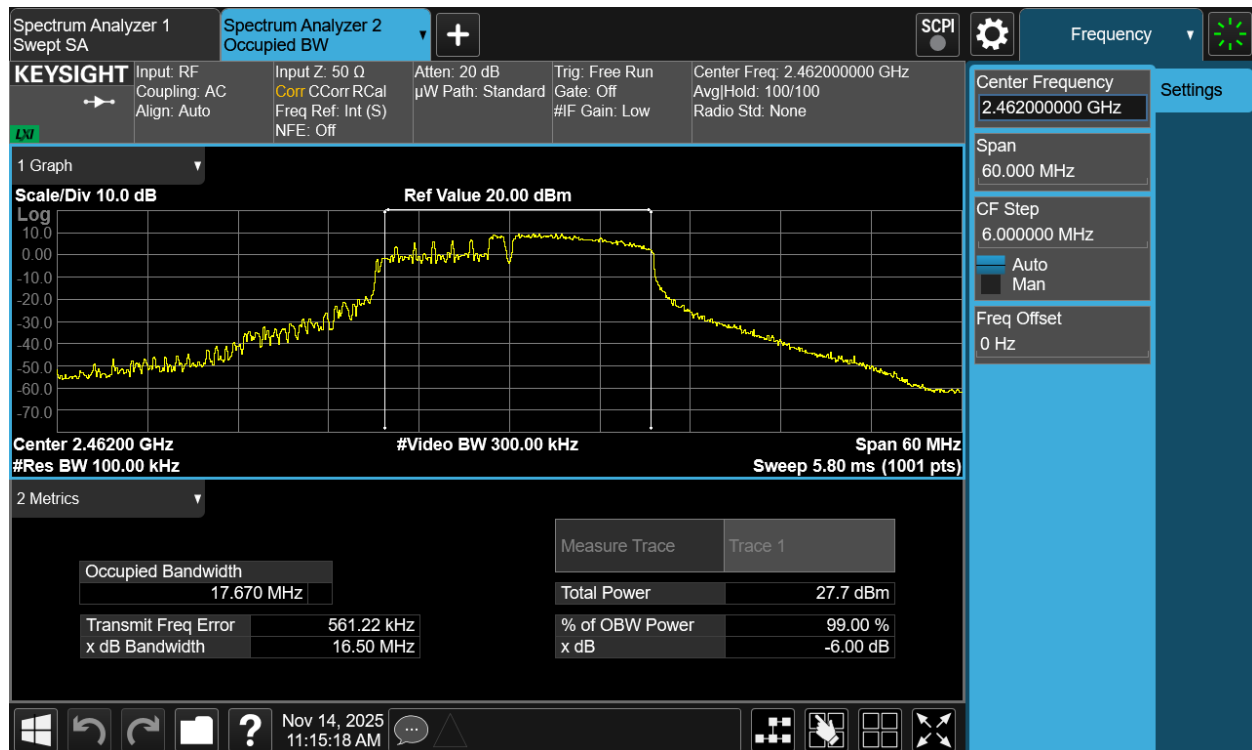
Plot 7-12 6dB BW Antenna 3a (20MHz BW 802.11be(RU) RU106+26 Index83 - Ch.11)
