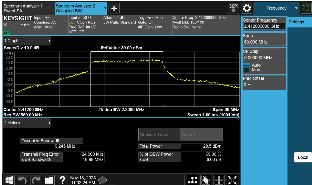
Plot 7-2 99% OBW Antenna 3a (20MHz BW 802.11be(RU) RU242 Index61 - Ch.1)
