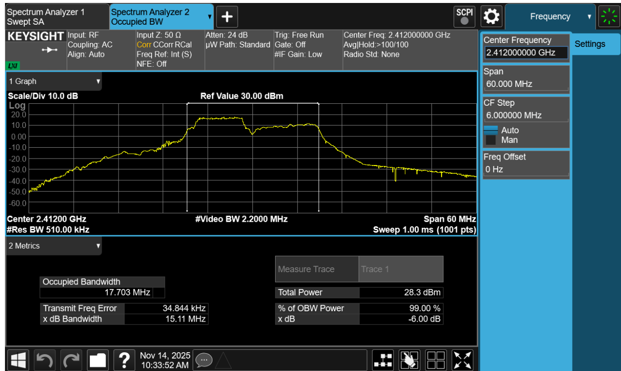
Plot 7-3 99% OBW Antenna 3a (20MHz BW 802.11be(RU) RU52+26 Index70 - Ch.1)
