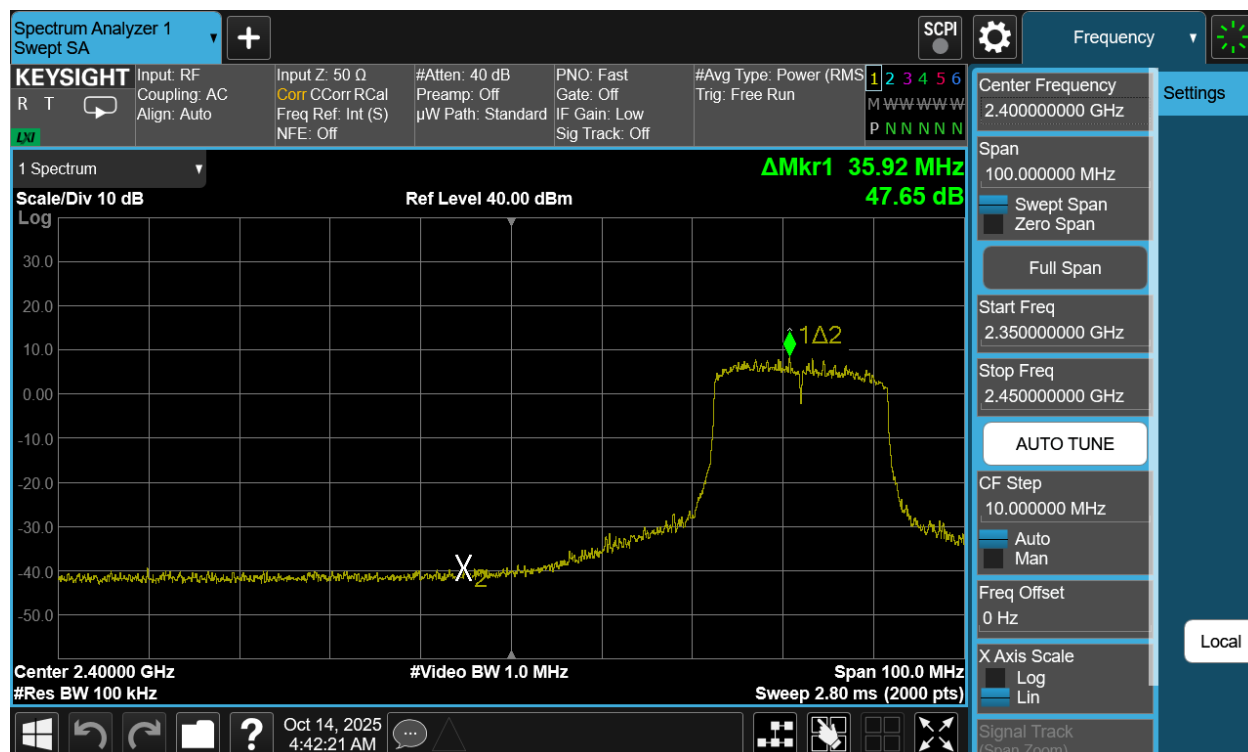
Plot 7-40. Band Edge Antenna 3a (802.11be OFDMA – RU242 – Ch. 5)
