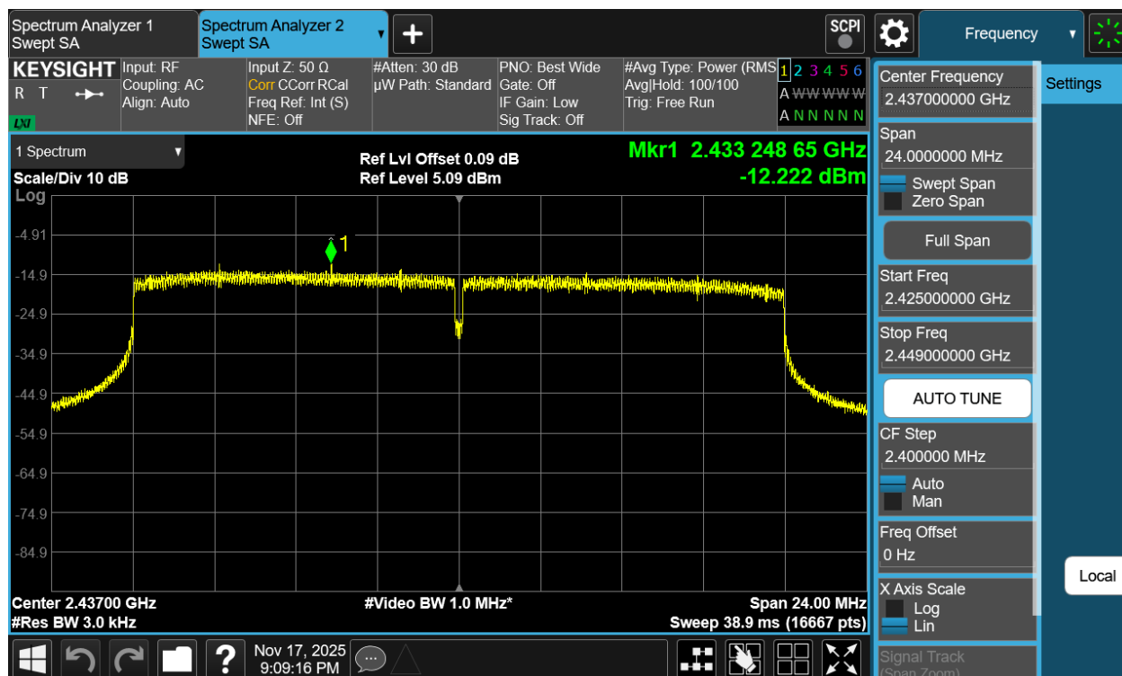
Plot 7-18 PSD Antenna 3a (20MHz BW 802.11be(RU) RU242 Index61 - Ch.6)
