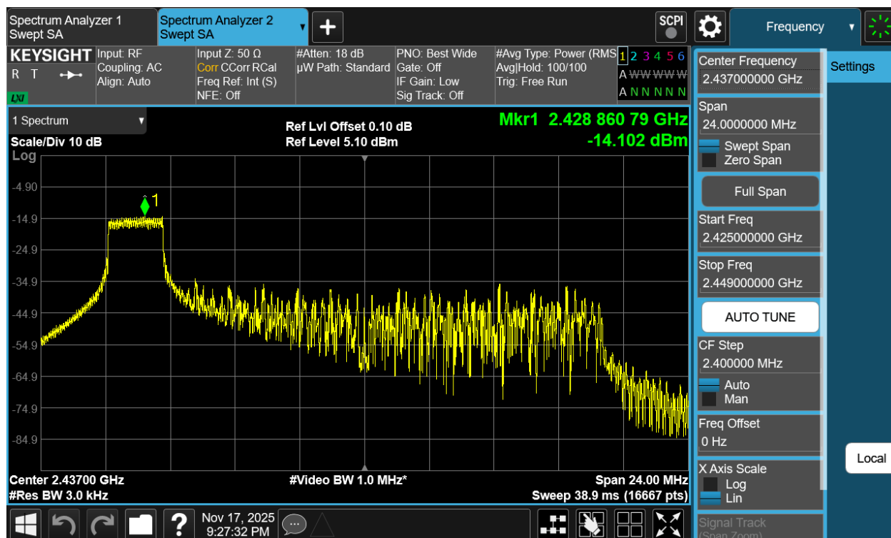
Plot 7-25 PSD CDD Antenna 3a (20MHz BW 802.11be(RU) RU26 Index0 - Ch.6)
