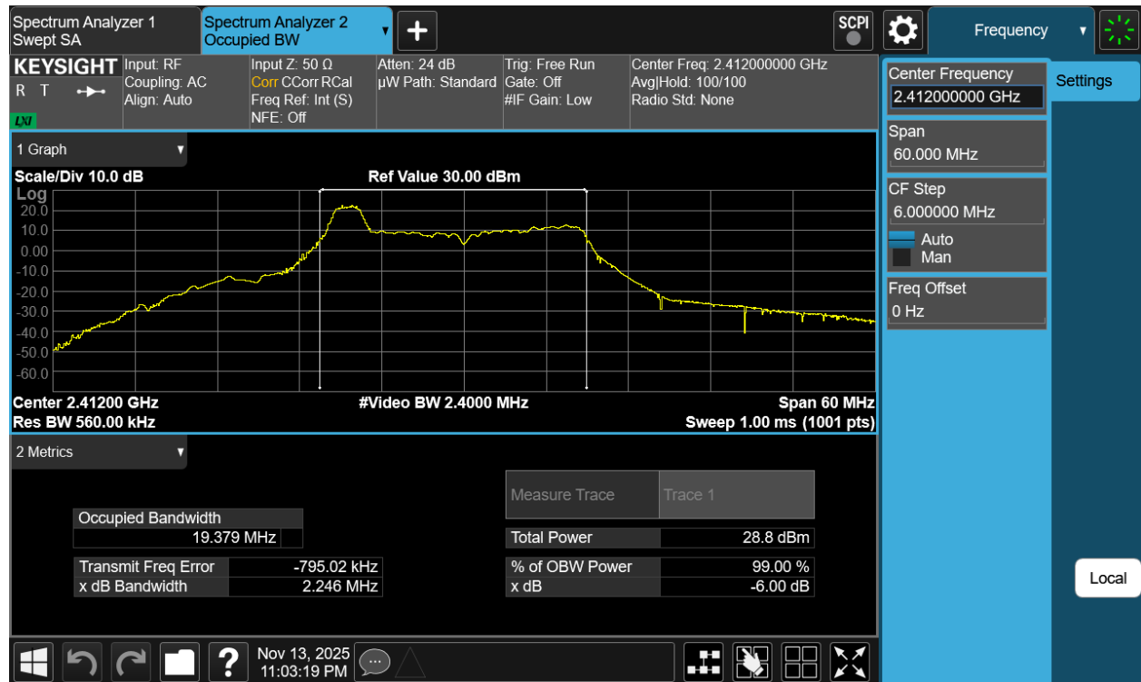
Plot 7-1 99% OBW Antenna 3a (20MHz BW 802.11be(RU) RU26 Index0 - Ch.1)
