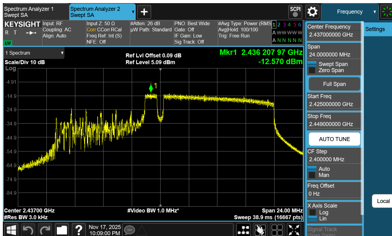
Plot 7-20 PSD Antenna 3a (20MHz BW 802.11be(RU) RU106+26 Index83 - Ch.6)
