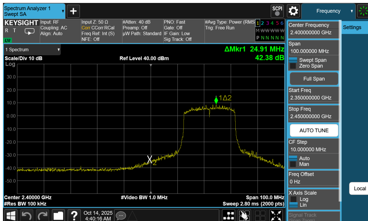
Plot 7-38. Band Edge Antenna 3a (802.11be OFDMA – RU242 – Ch. 3)
