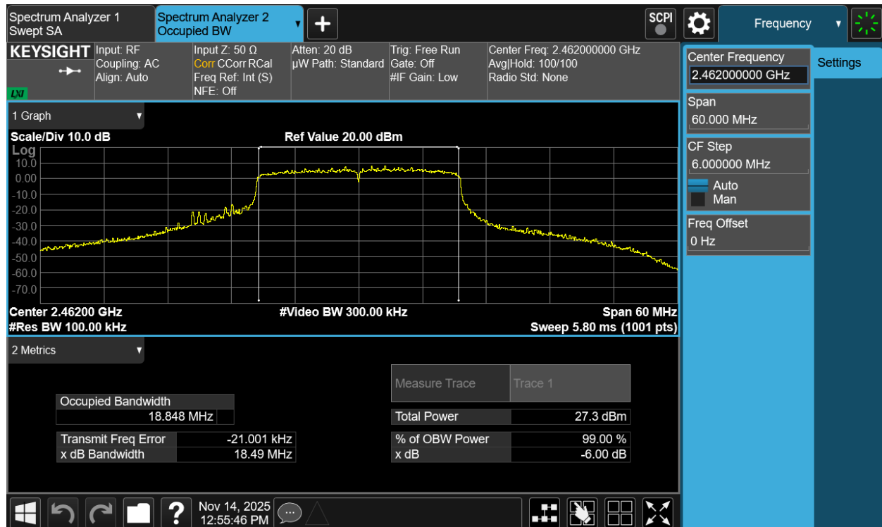
Plot 7-14 6dB BW Antenna 1a (20MHz BW 802.11be(RU) RU242 Index61 - Ch.11)
