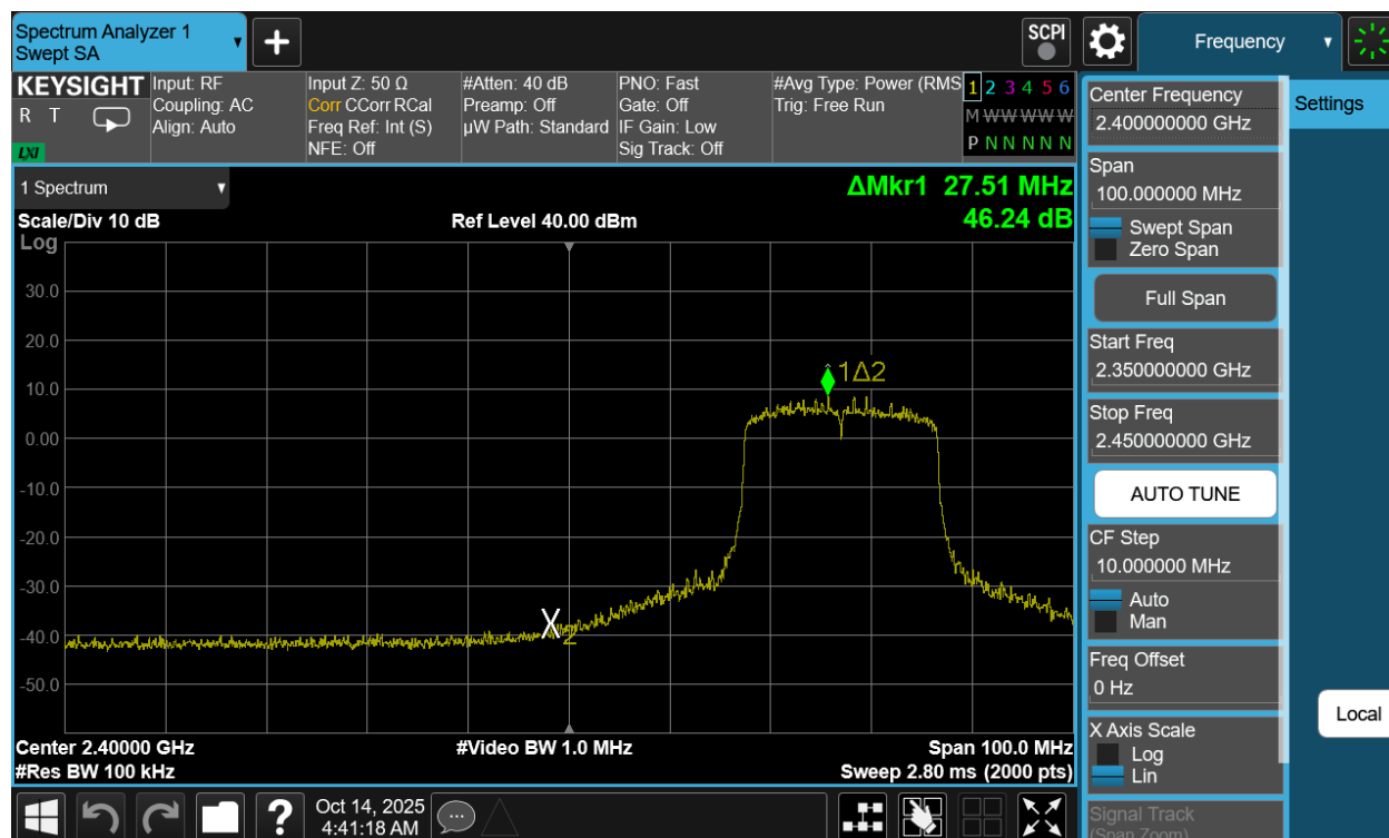
Plot 7-39. Band Edge Antenna 3a (802.11be OFDMA – RU242 – Ch. 4)
