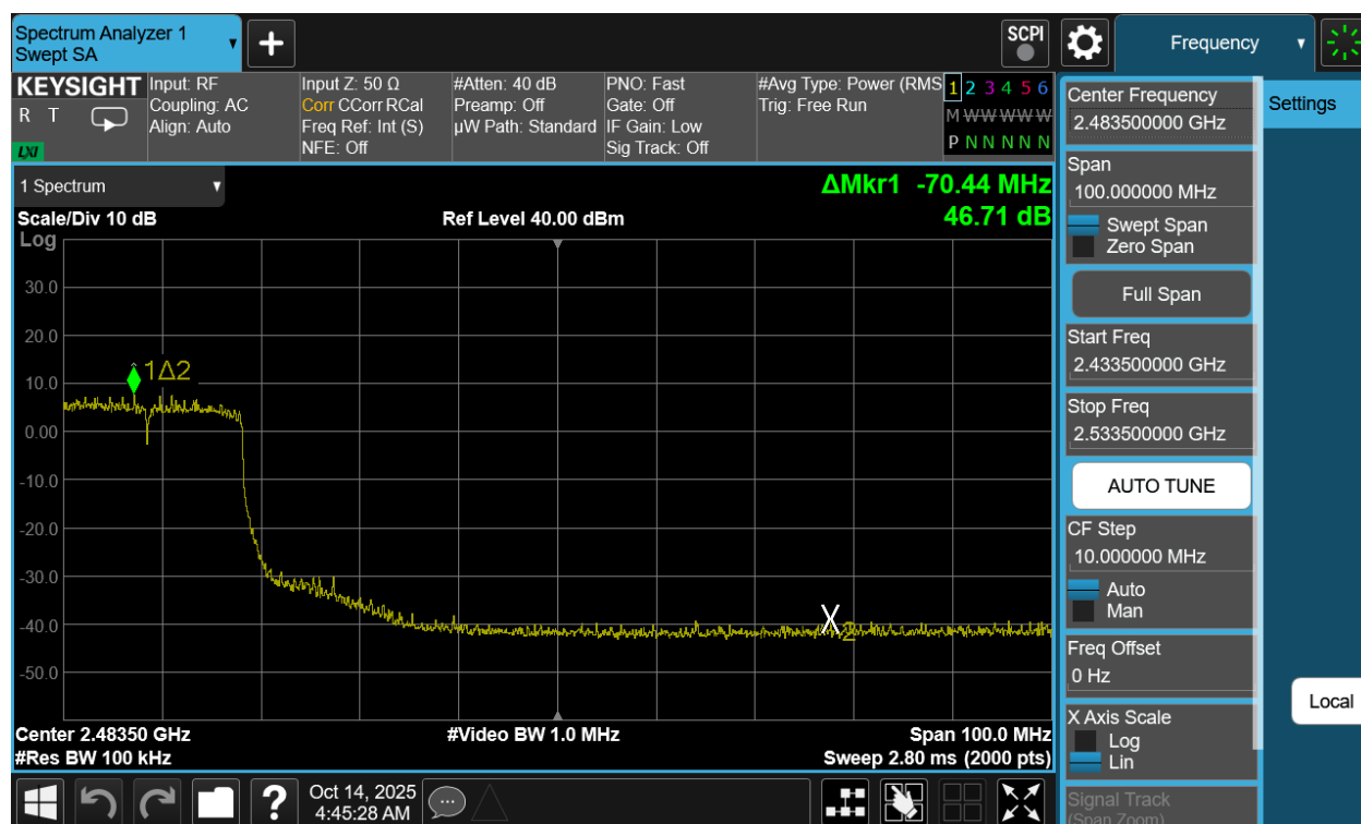
Plot 7-42. Band Edge Antenna 3a (802.11be OFDMA – RU242 – Ch. 7)
