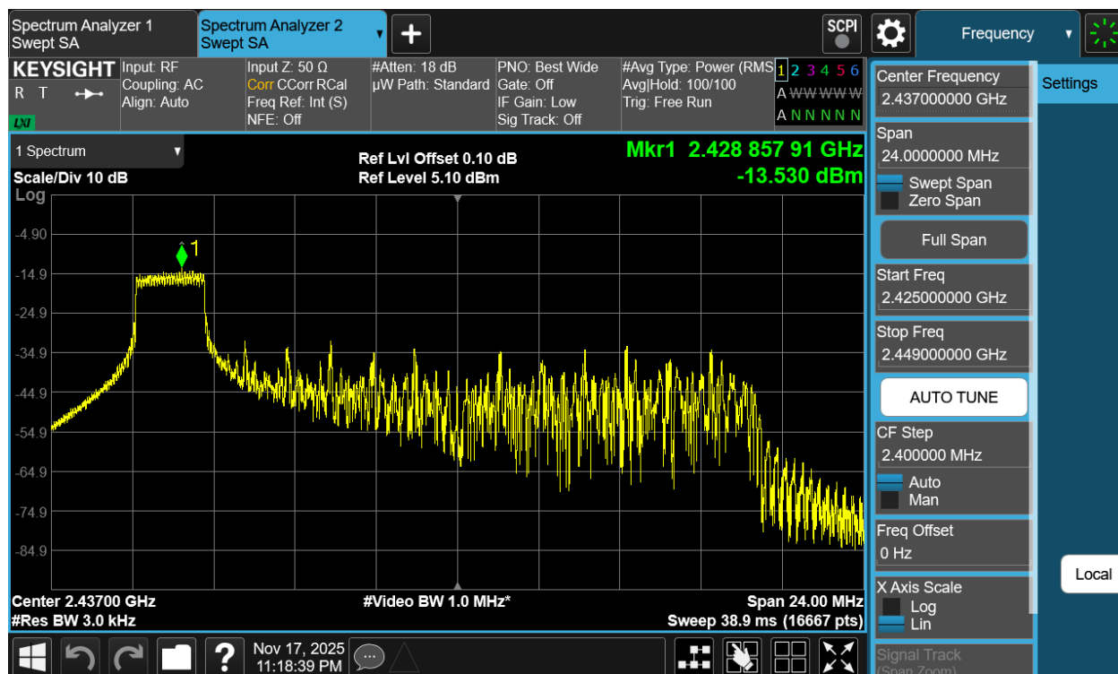
Plot 7-26 PSD CDD Antenna 1a (20MHz BW 802.11be(RU) RU26 Index0 - Ch.6)
