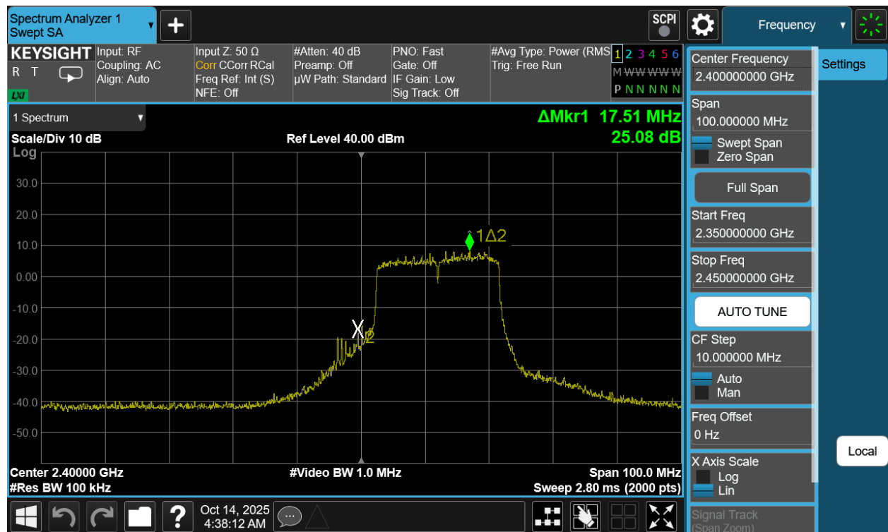
Plot 7-36. Band Edge Antenna 3a (802.11be OFDMA – RU242 – Ch. 1)
