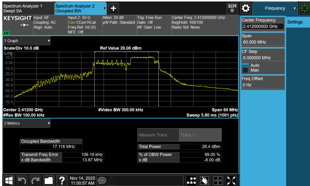
Plot 7-11 6dB BW Antenna 3a (20MHz BW 802.11be(RU) RU52+26 Index72 - Ch.1)
