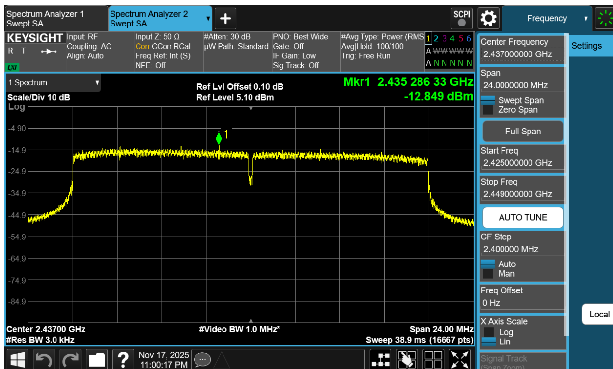
Plot 7-22 PSD Antenna 1a (20MHz BW 802.11be(RU) RU242 Index61 - Ch.6)
