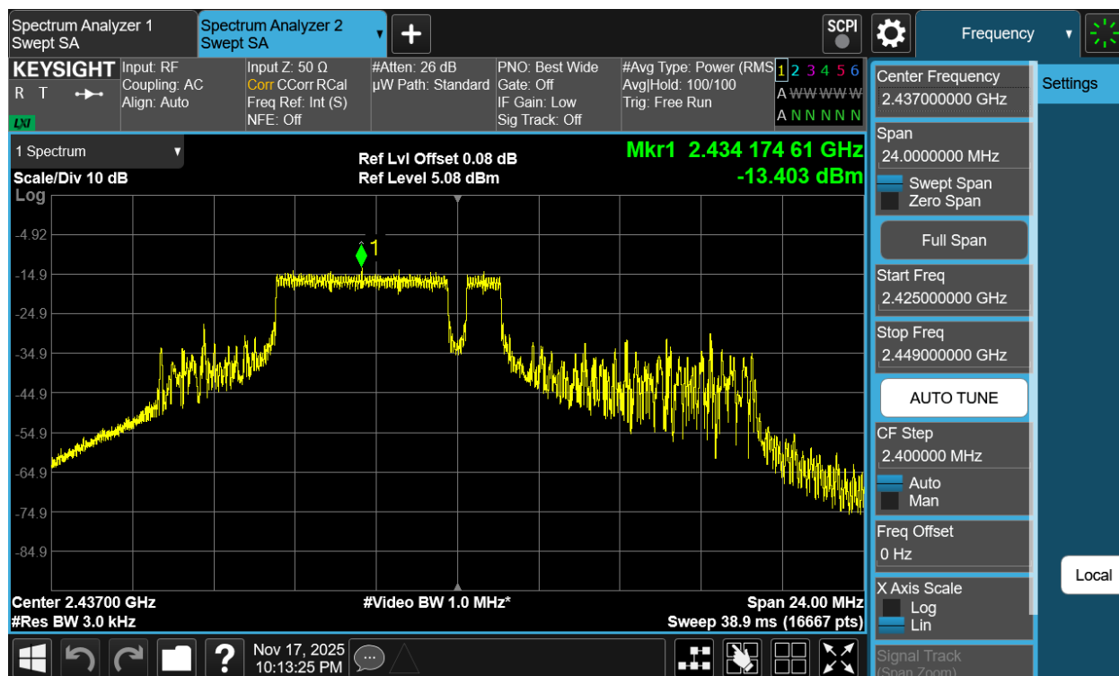
Plot 7-29 PSD CDD Antenna 3a (20MHz BW 802.11be(RU) RU52+26 Index71 - Ch.6)
