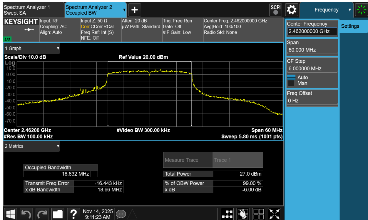
Plot 7-10 6dB BW Antenna 3a (20MHz BW 802.11be(RU) RU242 Index61 - Ch.11)
