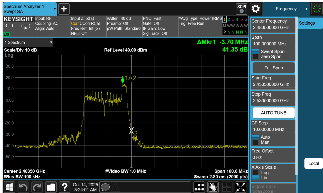
Plot 7-35. Band Edge Antenna 3a (802.11be OFDMA – RU26 Index 8 – Ch. 13)
