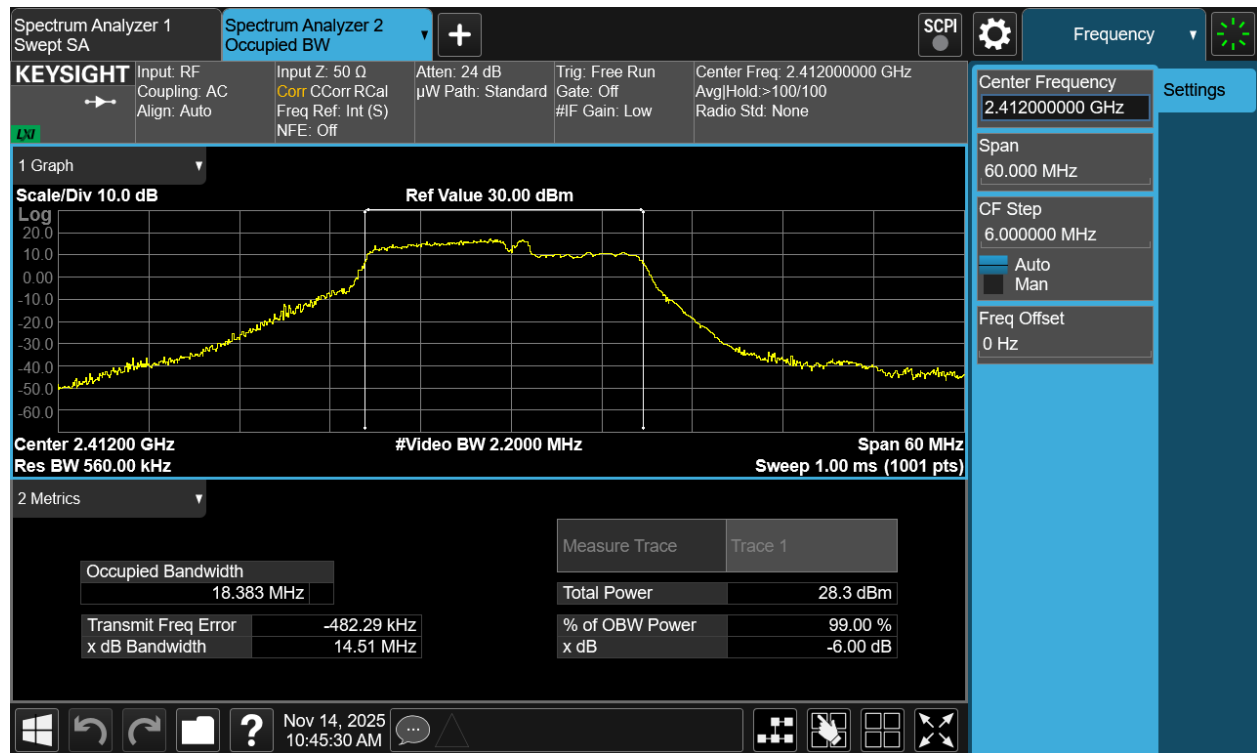
Plot 7-4 99% OBW Antenna 3a (20MHz BW 802.11be(RU) RU106+26 Index82 - Ch.1)
