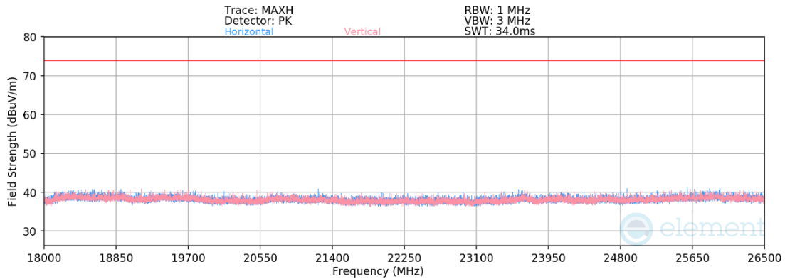
Plot 7-89. Radiated Spurious Emissions above 18GHz CDD (802.11be OFDMA – RU26 – Ch. 6)
