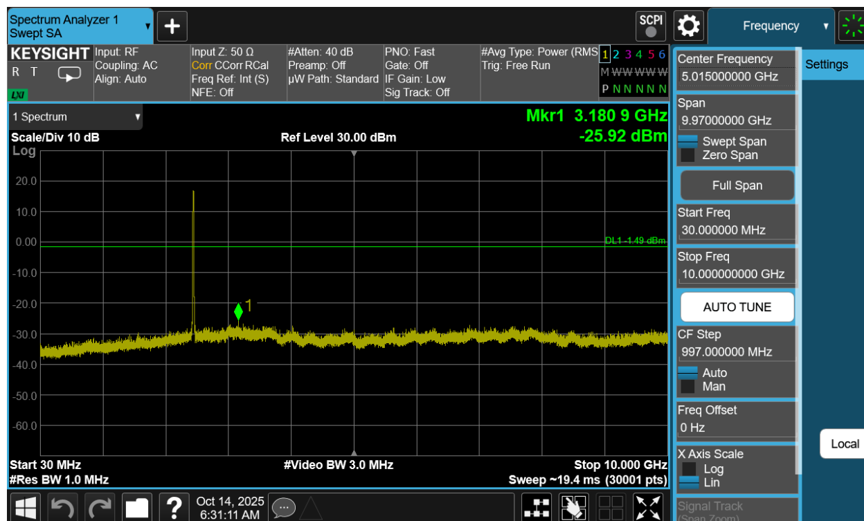
Plot 7-73. Conducted Spurious Plot Antenna 3a (802.11be OFDMA – RU242 – Ch. 11)
