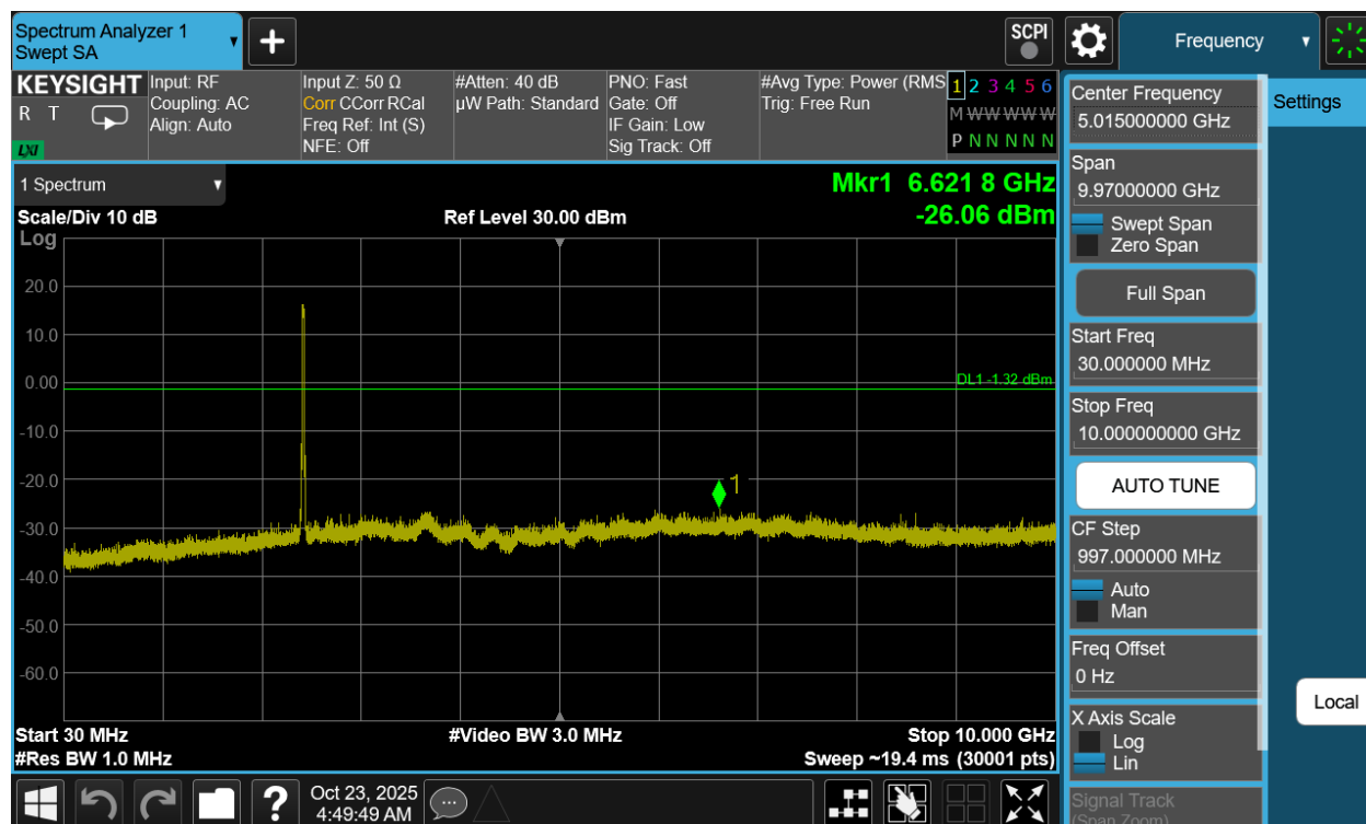
Plot 7-83. Conducted Spurious Plot Antenna 1a (802.11be OFDMA – RU242 – Ch. 6)
