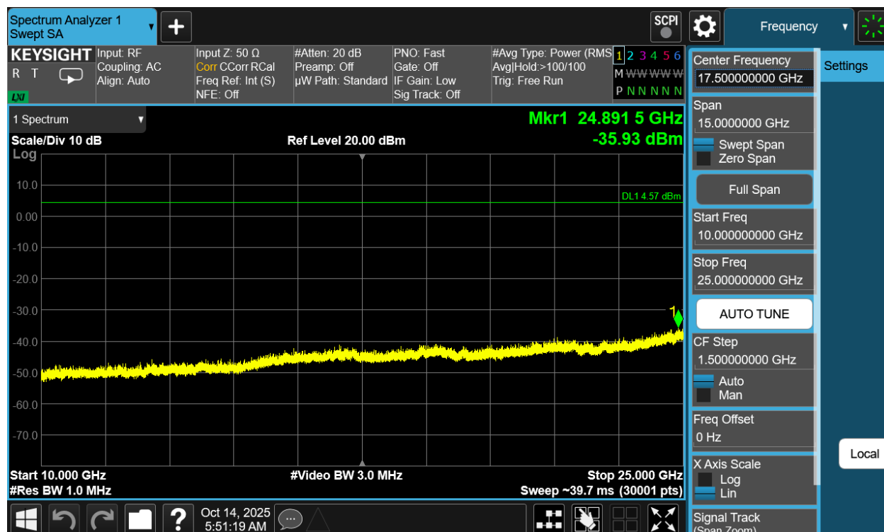
Plot 7-66. Conducted Spurious Plot Antenna 3a (802.11be OFDMA – RU26 – Ch. 6)
