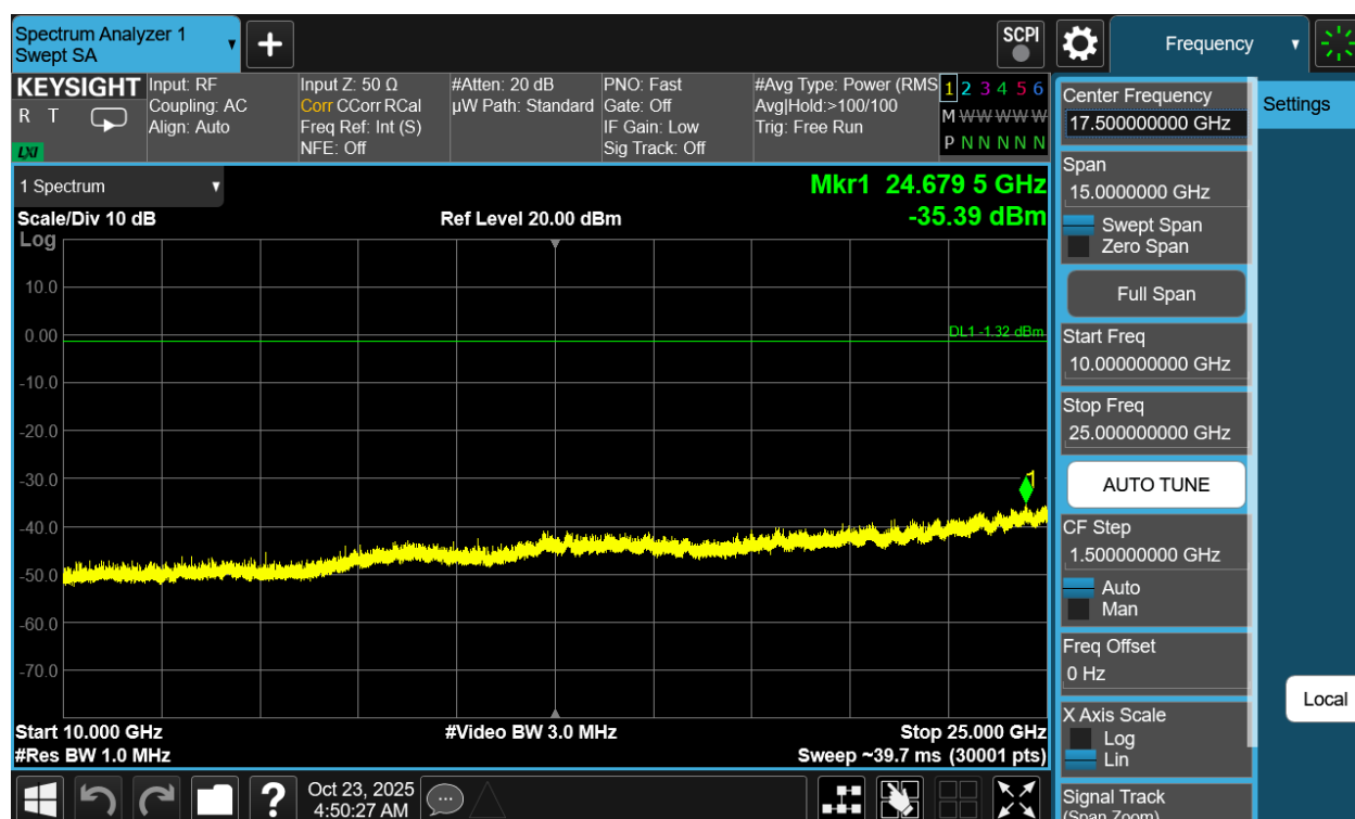
Plot 7-84. Conducted Spurious Plot Antenna 1a (802.11be OFDMA – RU242 – Ch. 6)
