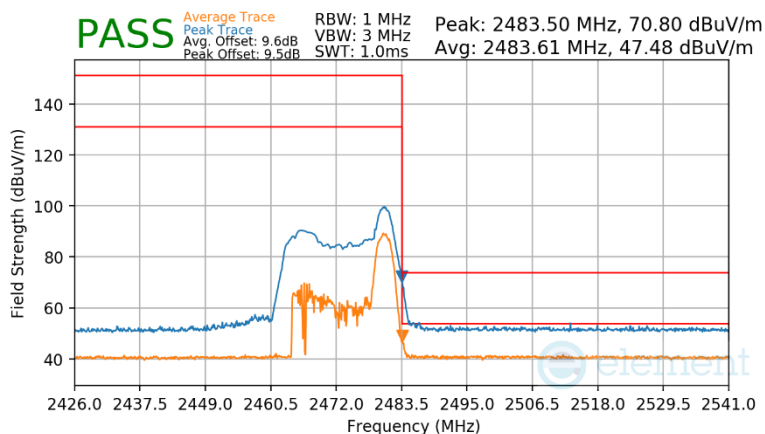
Plot 7-97 Radiated Restricted Upper Band Edge Measurement Antenna 3a (Peak & Average – RU26)
