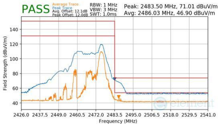
Plot 7-96 Radiated Restricted Upper Band Edge Measurement Antenna 3a (Peak & Average – RU26)
