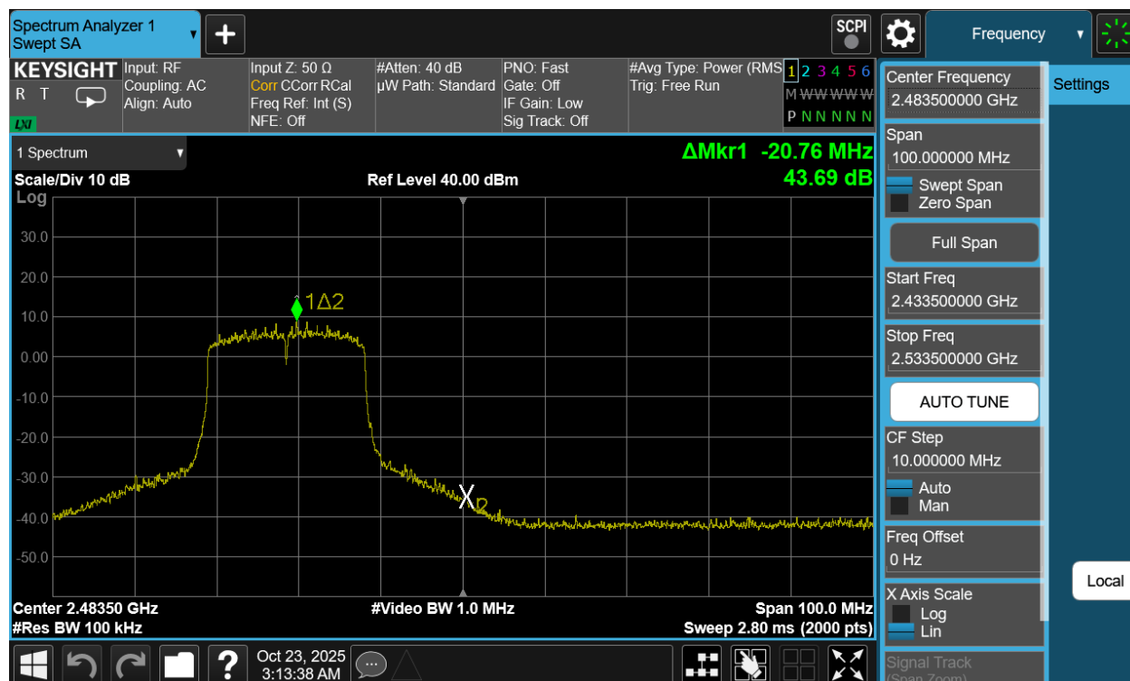
Plot 7-60. Band Edge Antenna 1a (802.11be OFDMA – RU242 – Ch. 11)
