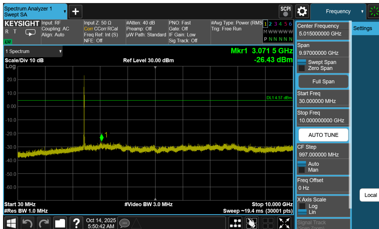
Plot 7-65. Conducted Spurious Plot Antenna 3a (802.11be OFDMA – RU26 – Ch. 6)
