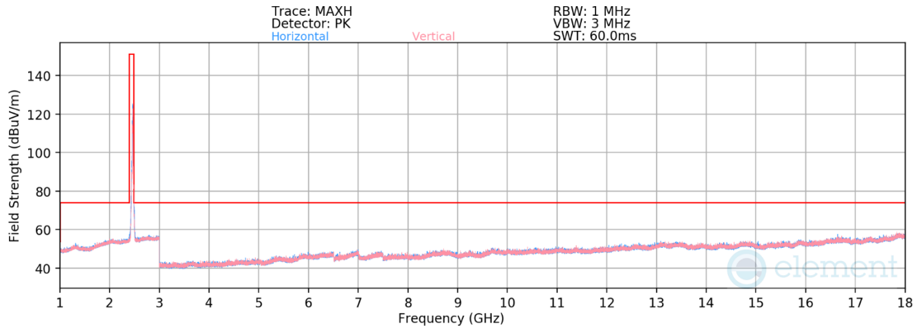
Plot 7-90. Radiated Spurious Emissions above 1GHz CDD (802.11be OFDMA – RU26 – Ch. 11)
