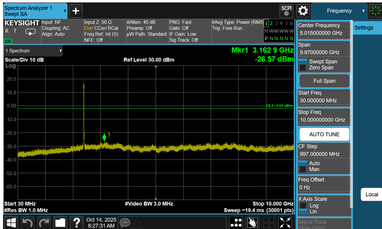
Plot 7-69. Conducted Spurious Plot Antenna 3a (802.11be OFDMA – RU242 – Ch. 1)
