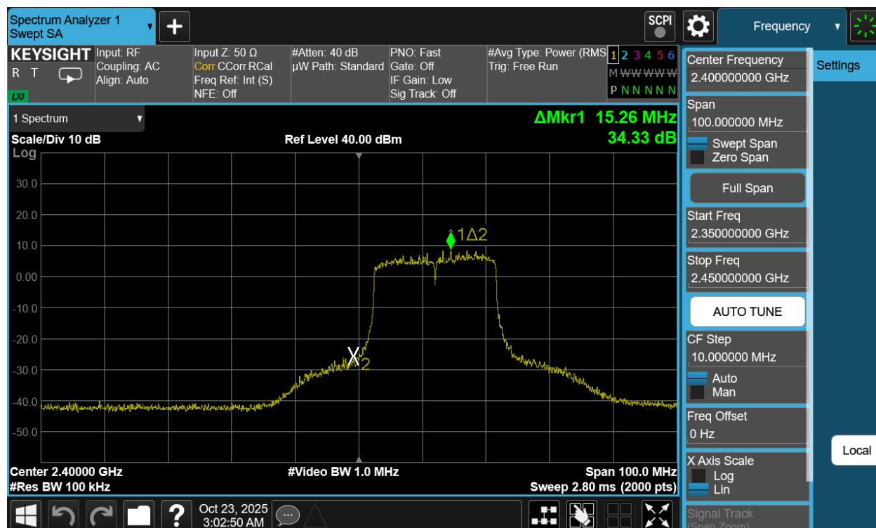
Plot 7-52. Band Edge Antenna 1a (802.11be OFDMA – RU242 – Ch. 1)
