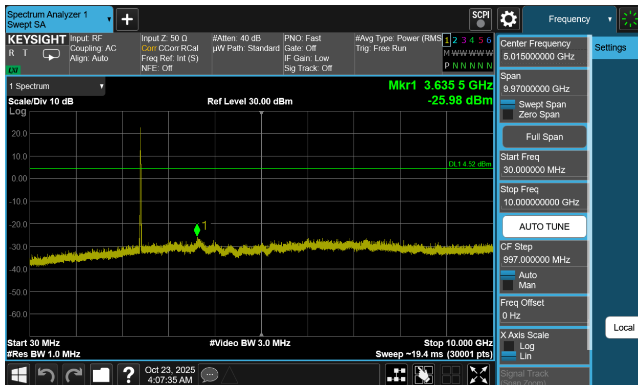
Plot 7-75. Conducted Spurious Plot Antenna 1a (802.11be OFDMA – RU26 – Ch. 1)
