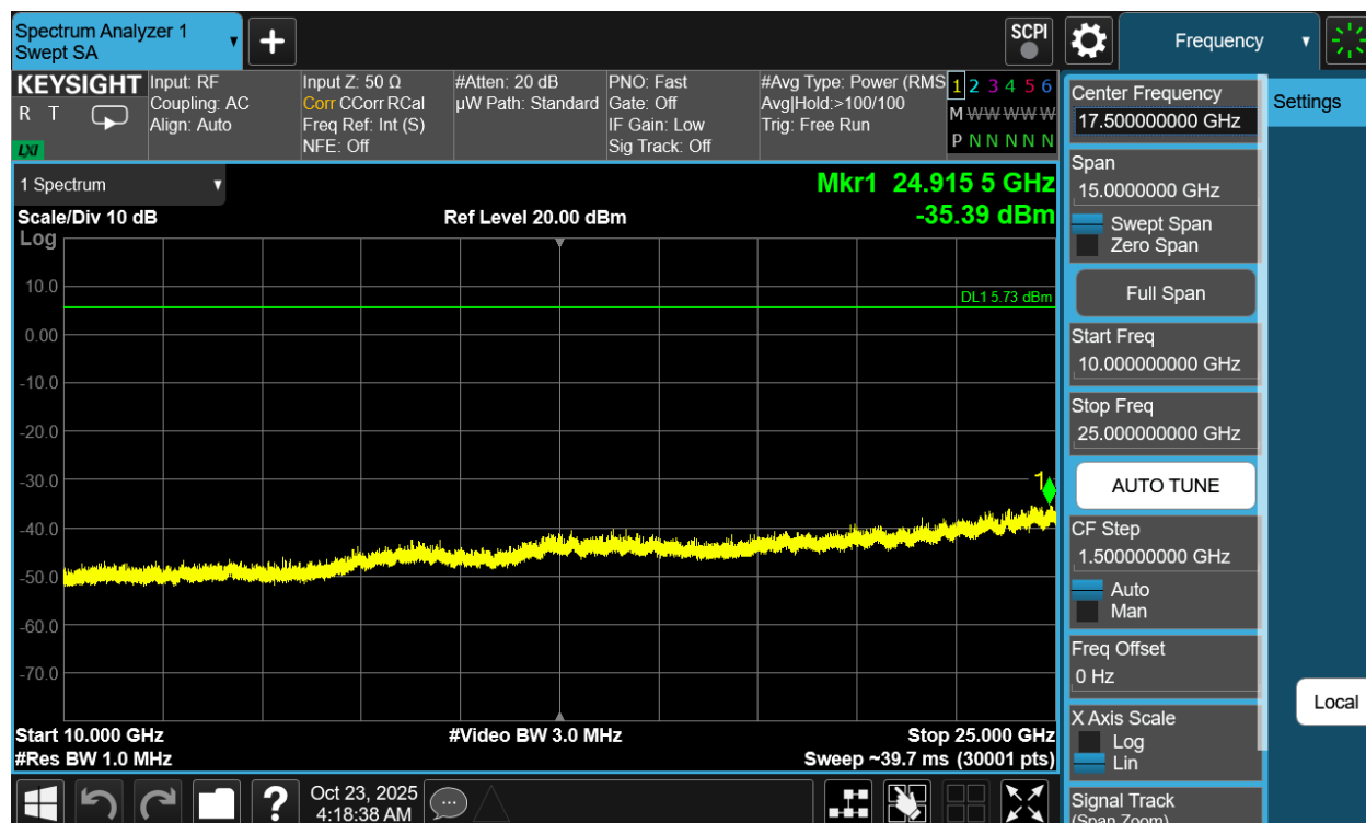
Plot 7-80. Conducted Spurious Plot Antenna 1a (802.11be OFDMA – RU26 – Ch. 11)
