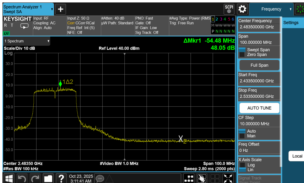
Plot 7-58. Band Edge Antenna 1a (802.11be OFDMA – RU242 – Ch. 9)
