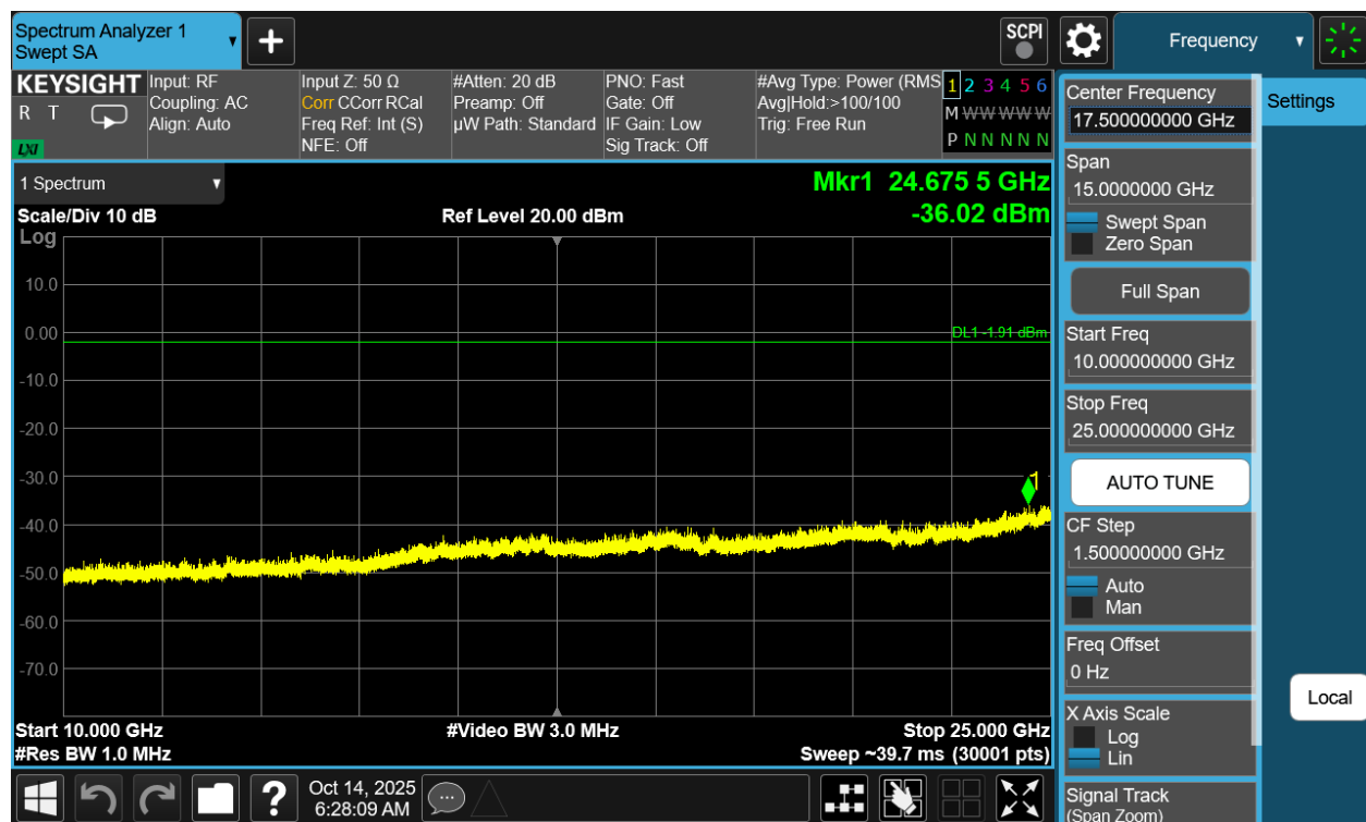
Plot 7-70. Conducted Spurious Plot Antenna 3a (802.11be OFDMA – RU242 – Ch. 1)
