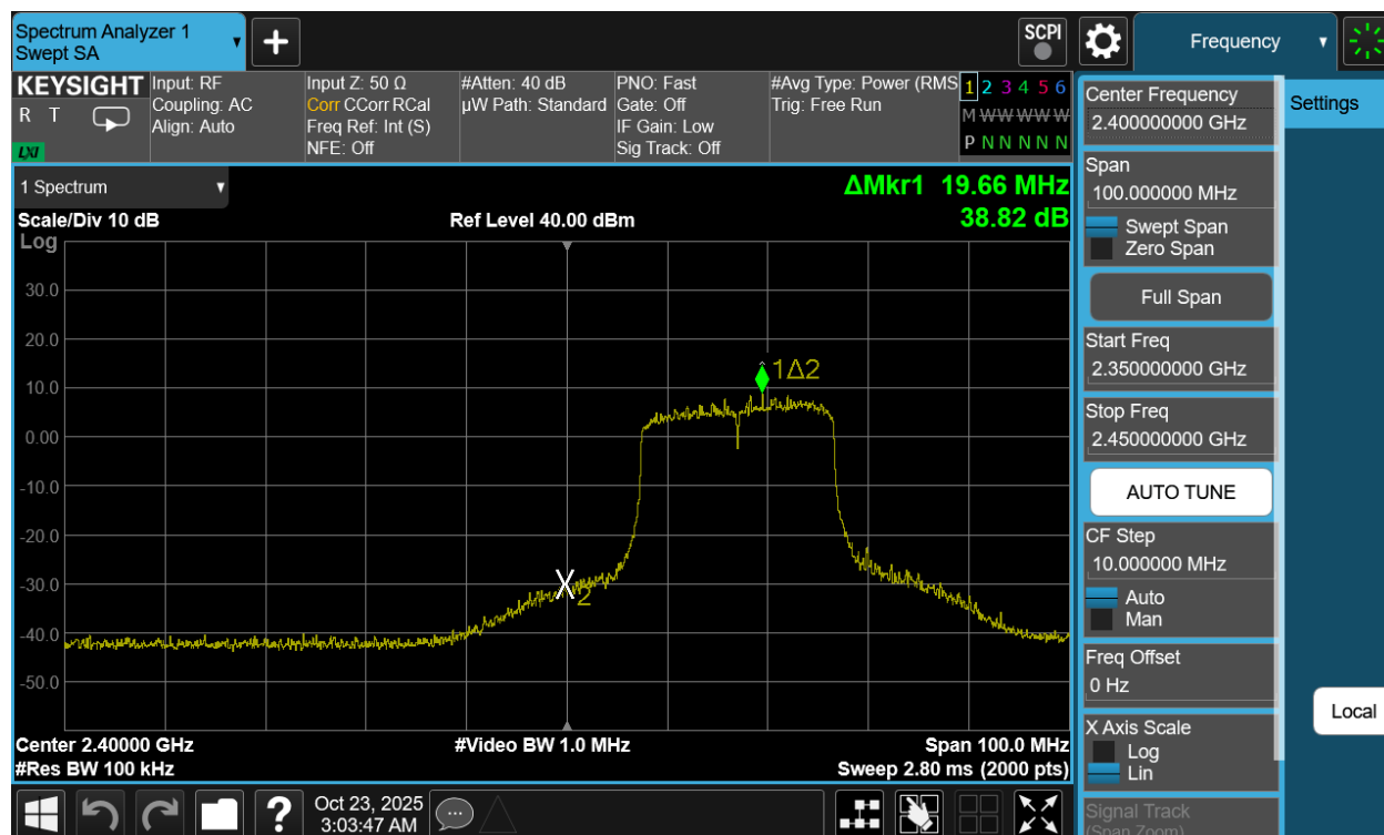
Plot 7-53. Band Edge Antenna 1a (802.11be OFDMA – RU242 – Ch. 2)
