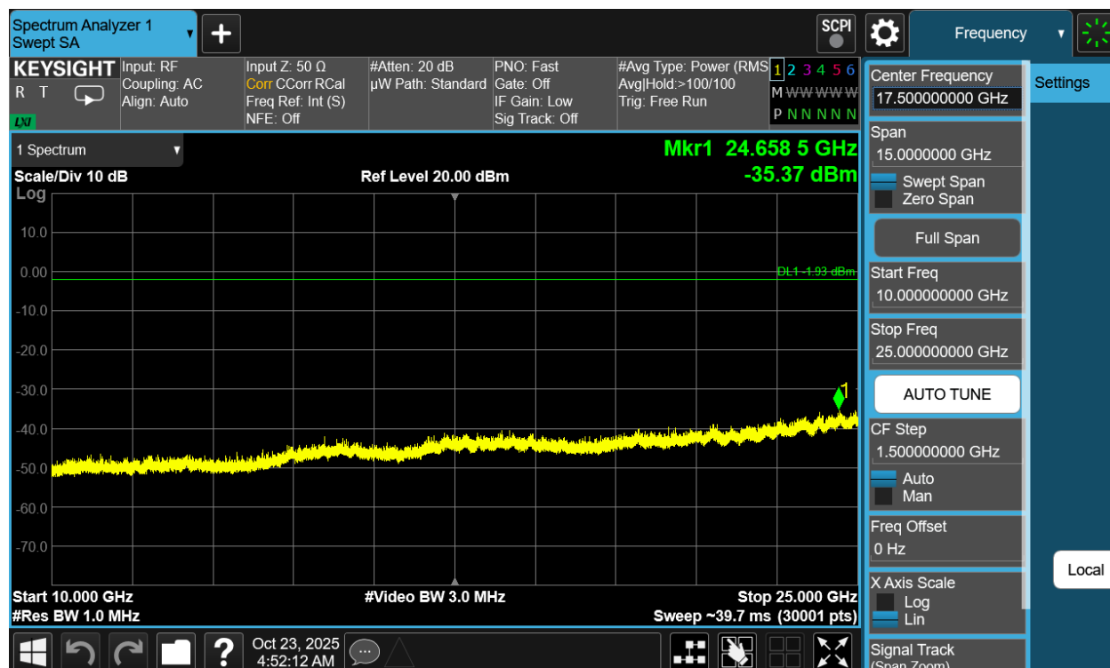
Plot 7-86. Conducted Spurious Plot Antenna 1a (802.11be OFDMA – RU242 – Ch. 11)
