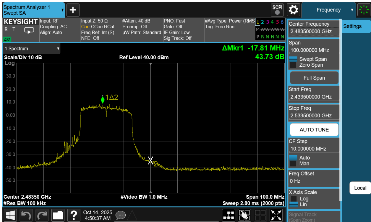
Plot 7-47. Band Edge Antenna 3a (802.11be OFDMA – RU242 – Ch. 12)
