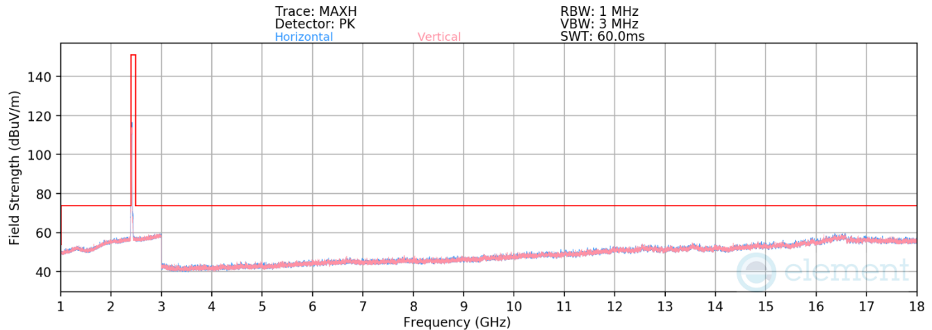
Plot 7-91. Radiated Spurious Emissions above 1GHz CDD (802.11be OFDMA – RU242 – Ch. 1)
