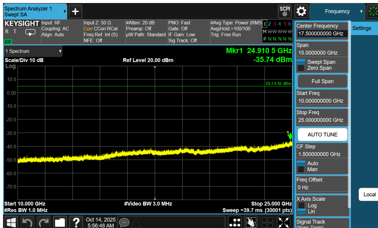
Plot 7-68. Conducted Spurious Plot Antenna 3a (802.11be OFDMA – RU26 – Ch. 11)
