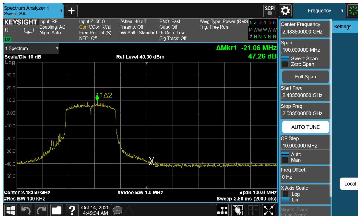
Plot 7-46. Band Edge Antenna 3a (802.11be OFDMA – RU242 – Ch. 11)
