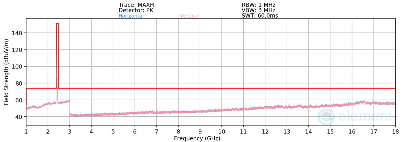
Plot 7-87. Radiated Spurious Emissions above 1GHz CDD (802.11be OFDMA – RU26 – Ch. 1)
