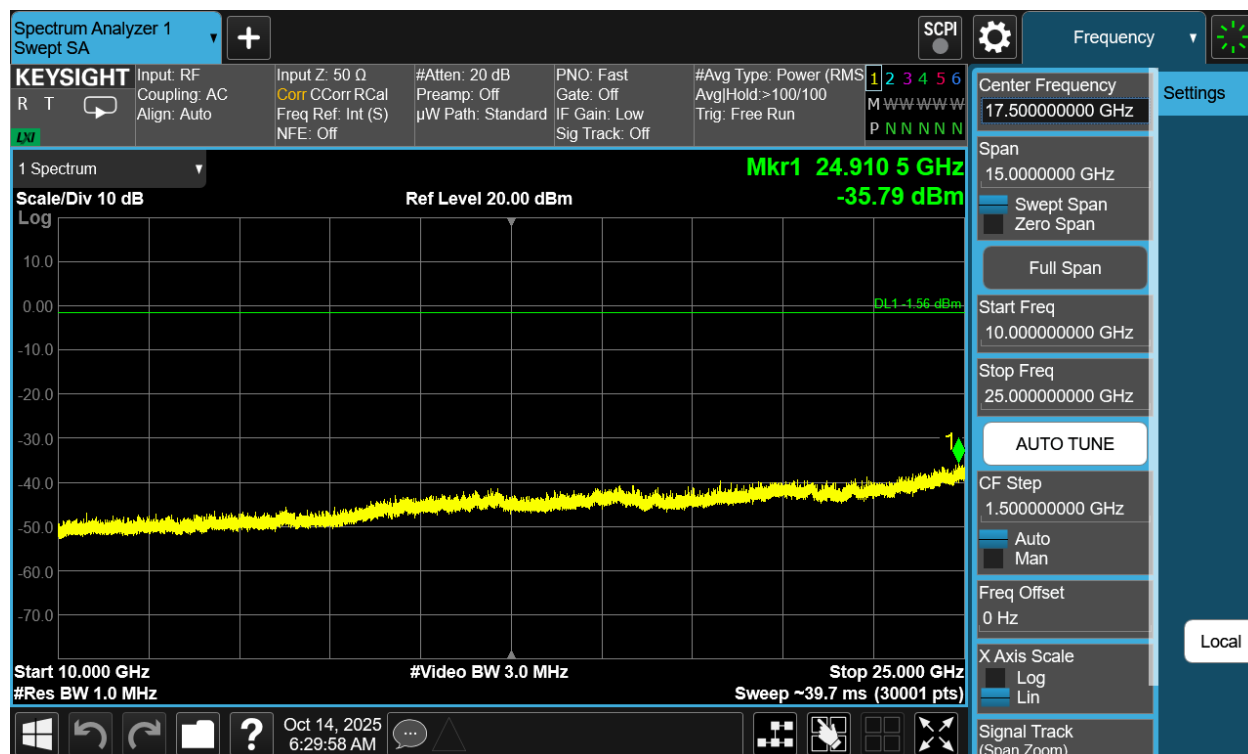
Plot 7-72. Conducted Spurious Plot Antenna 3a (802.11be OFDMA – RU242 – Ch. 6)
