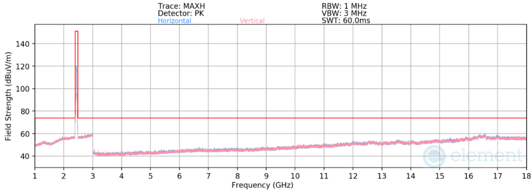
Plot 7-92. Radiated Spurious Emissions Above 1GHz CDD (802.11be OFDMA – RU242 – Ch. 6)
