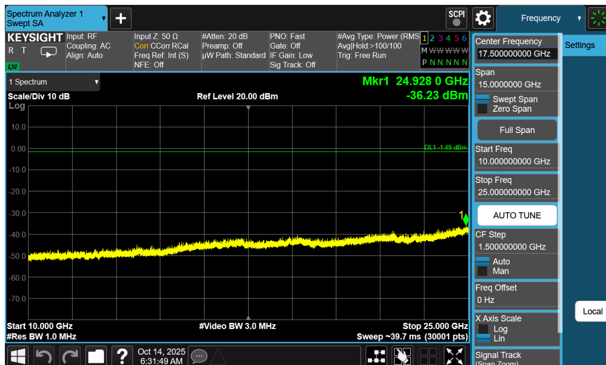
Plot 7-74. Conducted Spurious Plot Antenna 3a (802.11be OFDMA – RU242 – Ch. 11)
