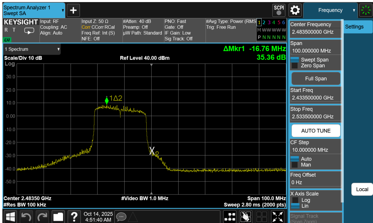
Plot 7-48. Band Edge Antenna 3a (802.11be OFDMA – RU242 – Ch. 13)
