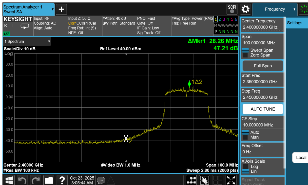
Plot 7-55. Band Edge Antenna 1a (802.11be OFDMA – RU242 – Ch. 4)
