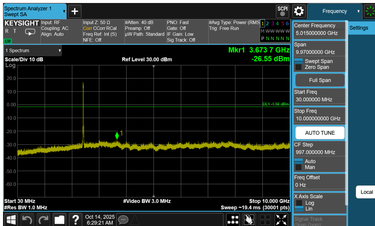
Plot 7-71. Conducted Spurious Plot Antenna 3a (802.11be OFDMA – RU242 – Ch. 6)
