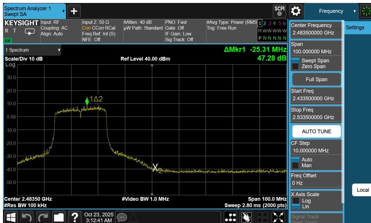
Plot 7-59. Band Edge Antenna 1a (802.11be OFDMA – RU242 – Ch. 10)
