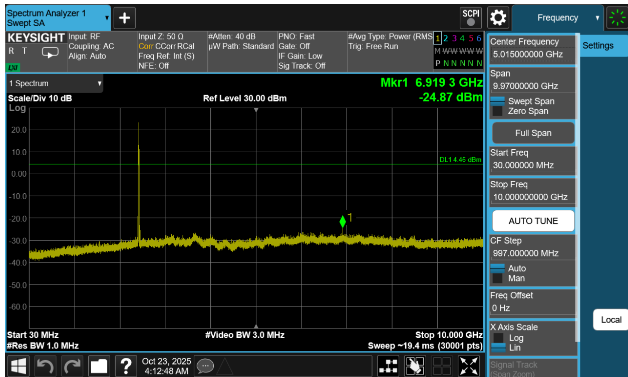
Plot 7-77. Conducted Spurious Plot Antenna 1a (802.11be OFDMA – RU26 – Ch. 6)
