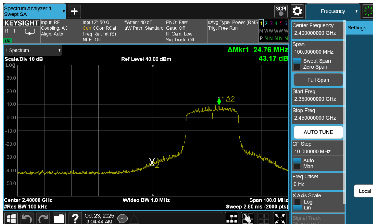
Plot 7-54. Band Edge Antenna 1a (802.11be OFDMA – RU242 – Ch. 3)
