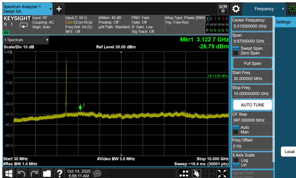
Plot 7-67. Conducted Spurious Plot Antenna 3a (802.11be OFDMA – RU26 – Ch. 11)
