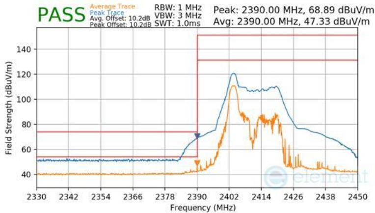
Plot 7-95 Radiated Restricted Lower Band Edge Measurement Antenna 3a (Peak & Average – RU26)
