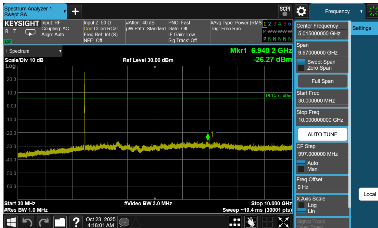
Plot 7-79. Conducted Spurious Plot Antenna 1a (802.11be OFDMA – RU26 – Ch. 11)
