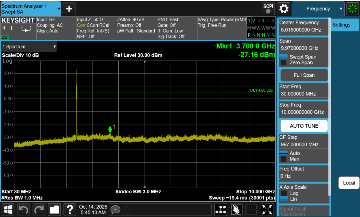
Plot 7-63. Conducted Spurious Plot Antenna 3a (802.11be OFDMA – RU26 – Ch. 1)
