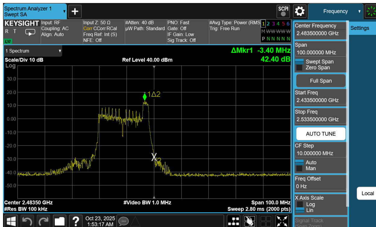
Plot 7-51. Band Edge Antenna 1a (802.11be OFDMA – RU26 Index 8 – Ch. 13)
