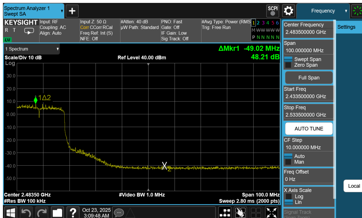
Plot 7-56. Band Edge Antenna 1a (802.11be OFDMA – RU242 – Ch. 7)
