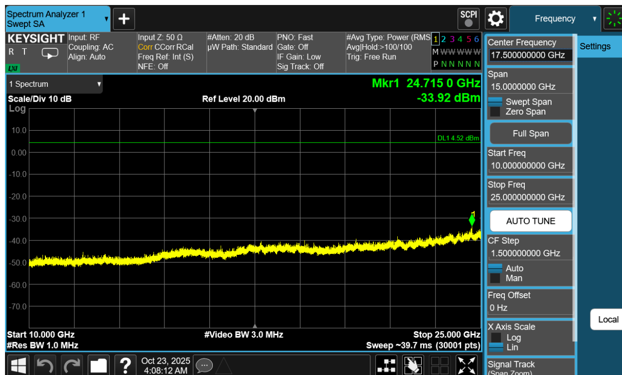
Plot 7-76. Conducted Spurious Plot Antenna 1a (802.11be OFDMA – RU26 – Ch. 1)
