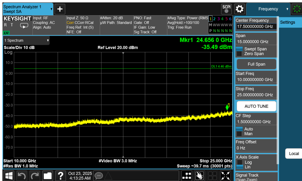
Plot 7-78. Conducted Spurious Plot Antenna 1a (802.11be OFDMA – RU26 – Ch. 6)
