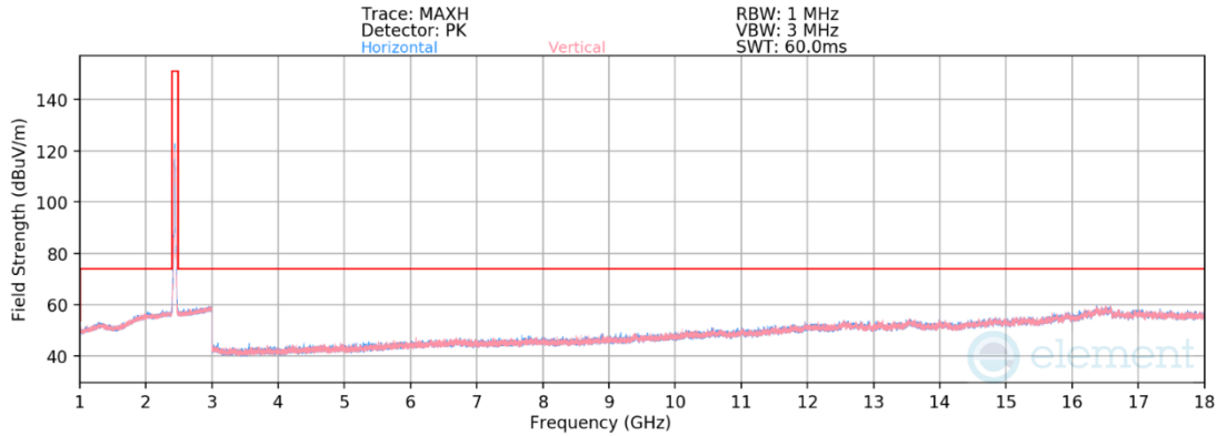
Plot 7-88. Radiated Spurious Emissions above 1GHz CDD (802.11be OFDMA – RU26 – Ch. 6)
