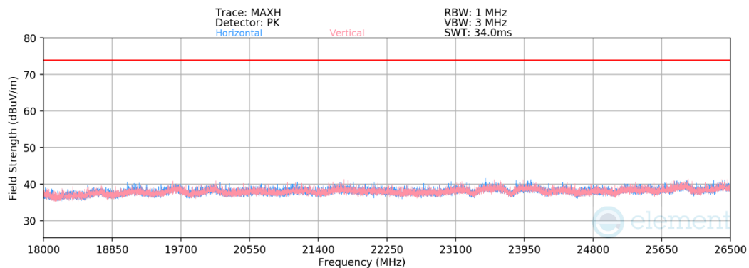
Plot 7-93. Radiated Spurious Emissions Above 1GHz CDD (802.11be OFDMA – RU242 – Ch. 6)
