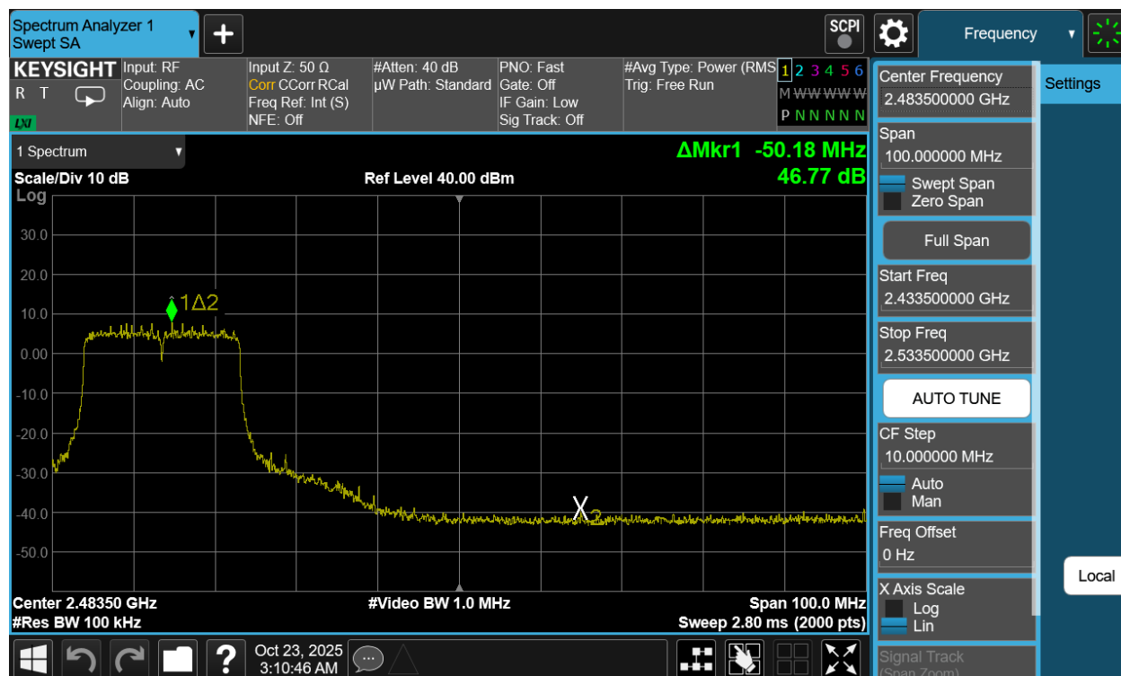
Plot 7-57. Band Edge Antenna 1a (802.11be OFDMA – RU242 – Ch. 8)
