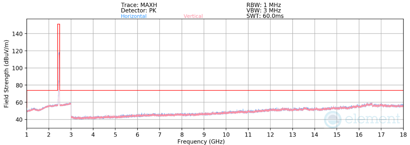
Plot 7-94. Radiated Spurious Emissions Above 1GHz CDD (802.11be OFDMA – RU242 – Ch. 11)
