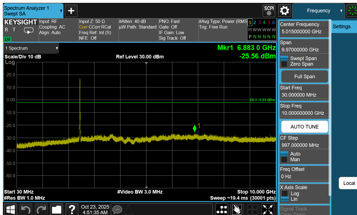
Plot 7-85. Conducted Spurious Plot Antenna 1a (802.11be OFDMA – RU242 – Ch. 11)
