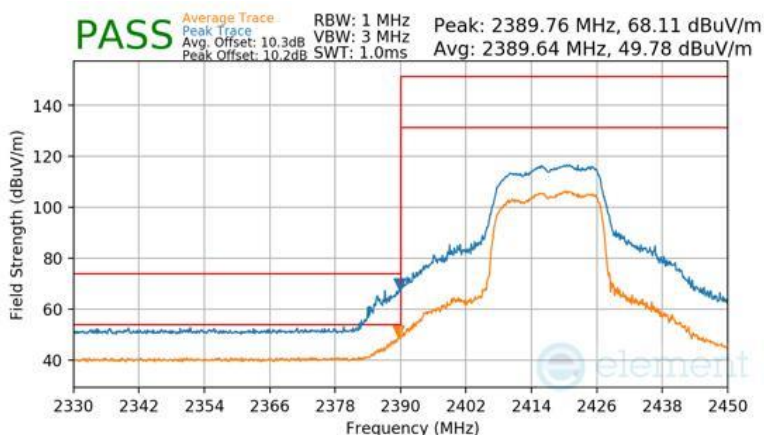
Plot 7-165 Radiated Restricted Lower Band Edge Measurement CDD (Peak & Average – RU242)
