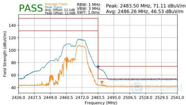
Plot 7-107 Radiated Restricted Upper Band Edge Measurement Antenna 3a (Peak & Average – RU52+26)
