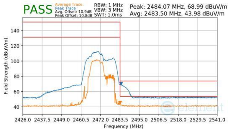
Plot 7-162 Radiated Restricted Upper Band Edge Measurement CDD (Peak & Average – RU52+26)
