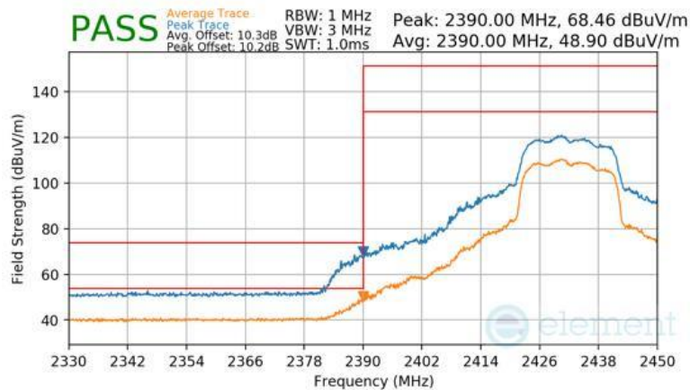
Plot 7-168 Radiated Restricted Lower Band Edge Measurement CDD (Peak & Average – RU242)
