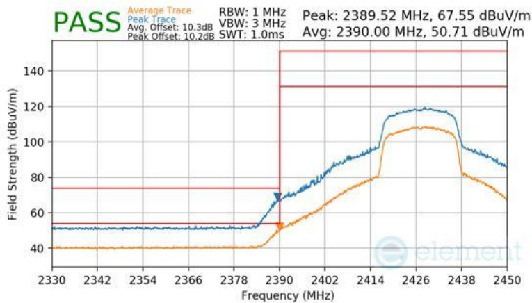
Plot 7-141 Radiated Restricted Lower Band Edge Measurement Antenna 1a (Peak & Average – RU242)
