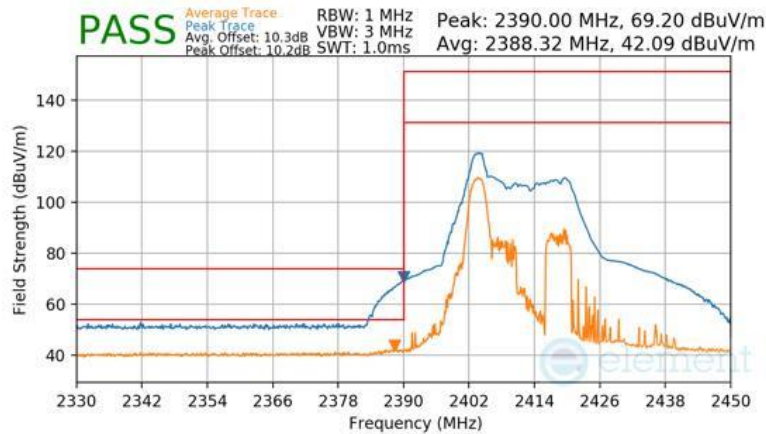
Plot 7-149 Radiated Restricted Lower Band Edge Measurement CDD (Peak & Average – RU26)
