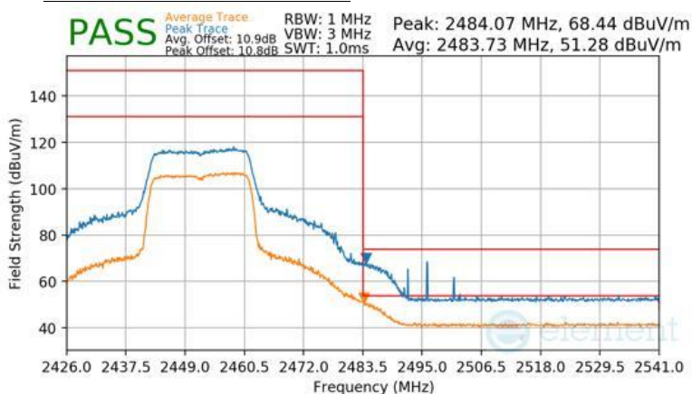
Plot 7-118 Radiated Restricted Upper Band Edge Measurement Antenna 3a (Peak & Average – RU242)
