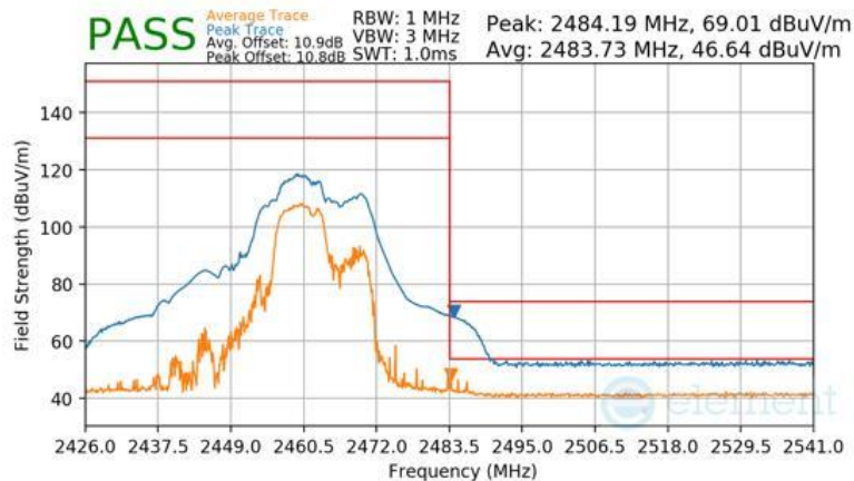
Plot 7-158 Radiated Restricted Upper Band Edge Measurement CDD (Peak & Average – RU52+26)
