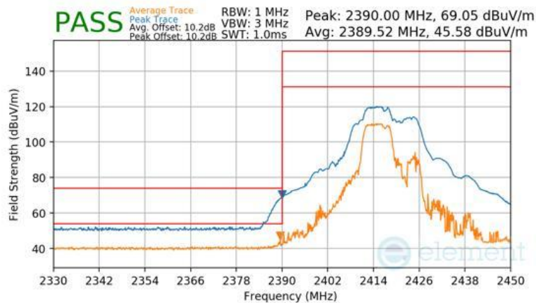
Plot 7-128 Radiated Restricted Lower Band Edge Measurement Antenna 1a (Peak & Average – RU52+26)
