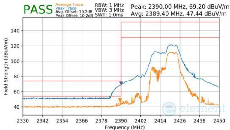
Plot 7-156 Radiated Restricted Lower Band Edge Measurement CDD (Peak & Average – RU52+26)
