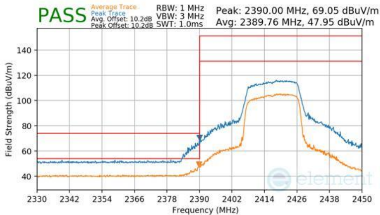
Plot 7-111 Radiated Restricted Lower Band Edge Measurement Antenna 3a (Peak & Average – RU242)
