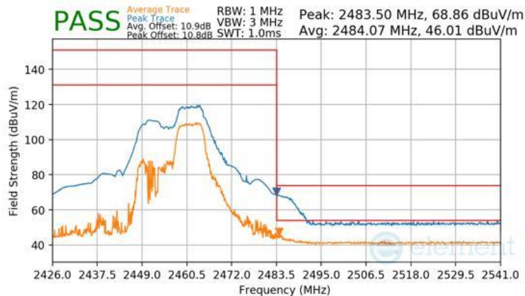
Plot 7-131 Radiated Restricted Upper Band Edge Measurement Antenna 1a (Peak & Average – RU52+26)
