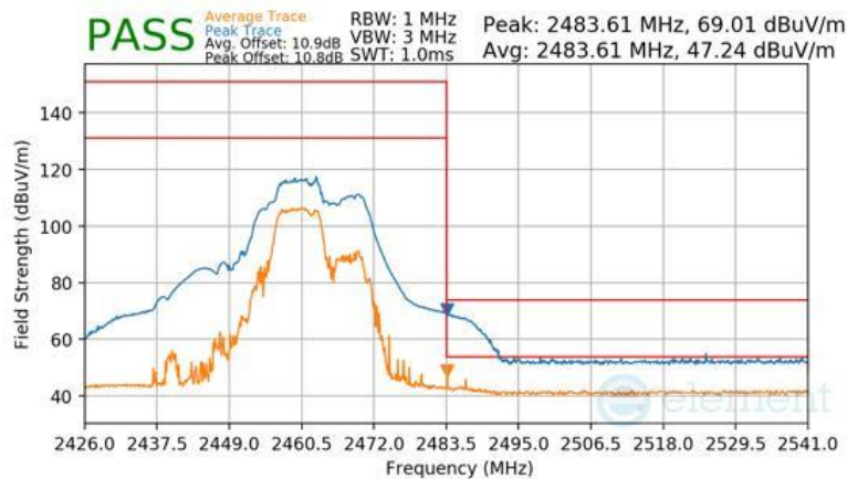
Plot 7-132 Radiated Restricted Upper Band Edge Measurement Antenna 1a (Peak & Average – RU52+26)
