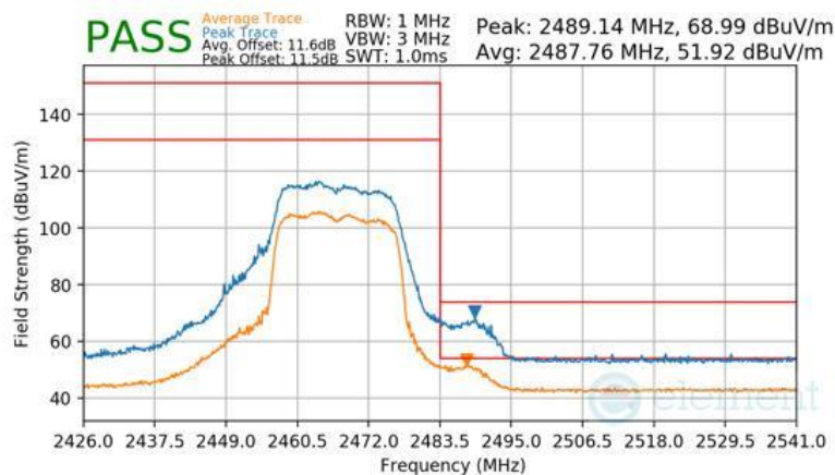
Plot 7-175 Radiated Restricted Upper Band Edge Measurement CDD (Peak & Average – RU242)
