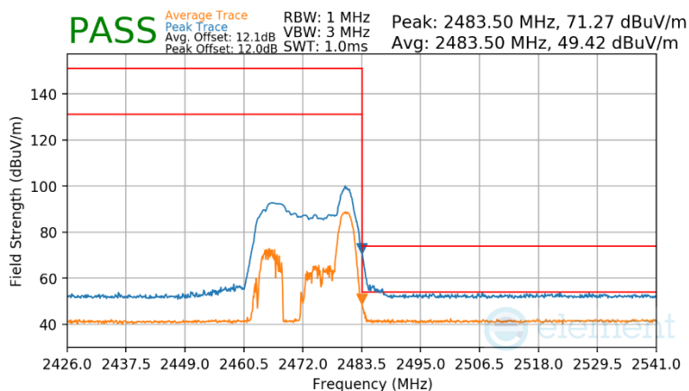
Plot 7-125 Radiated Restricted Upper Band Edge Measurement Antenna 1a (Peak & Average – RU26)
