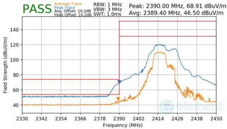
Plot 7-100 Radiated Restricted Lower Band Edge Measurement Antenna 3a (Peak & Average – RU52+26)
