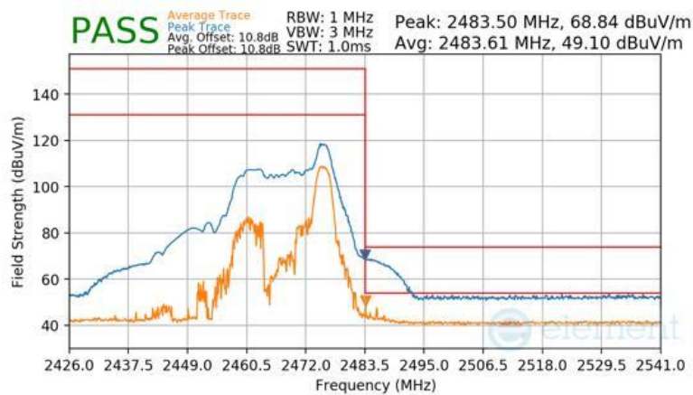
Plot 7-124 Radiated Restricted Upper Band Edge Measurement Antenna 1a (Peak & Average – RU26)
