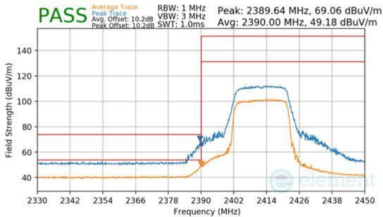
Plot 7-110 Radiated Restricted Lower Band Edge Measurement Antenna 3a (Peak & Average – RU242)
