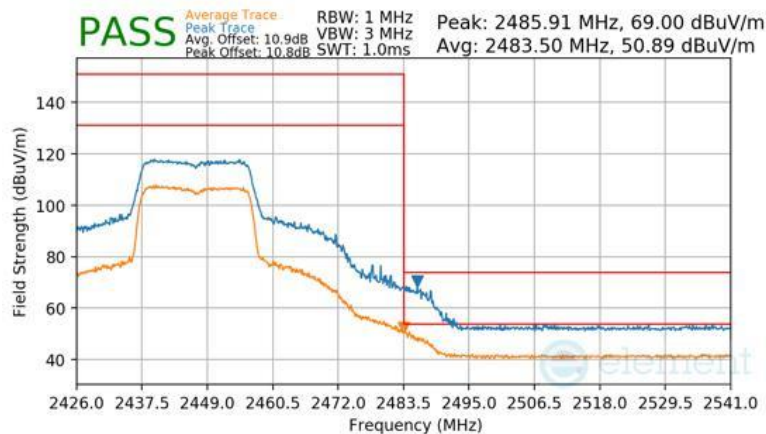
Plot 7-117 Radiated Restricted Upper Band Edge Measurement Antenna 3a (Peak & Average – RU242)
