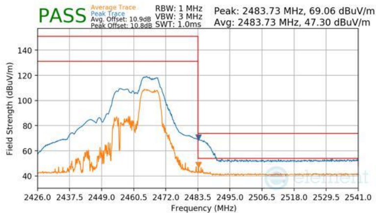
Plot 7-159 Radiated Restricted Upper Band Edge Measurement CDD (Peak & Average – RU52+26)
