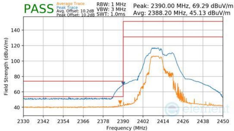
Plot 7-98 Radiated Restricted Lower Band Edge Measurement Antenna 3a (Peak & Average – RU52+26)
