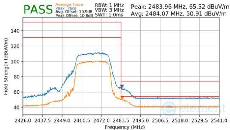
Plot 7-147 Radiated Restricted Upper Band Edge Measurement Antenna 1a (Peak & Average – RU242)
