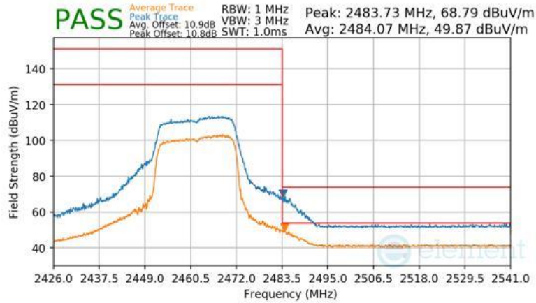
Plot 7-146 Radiated Restricted Upper Band Edge Measurement Antenna 1a (Peak & Average – RU242)
