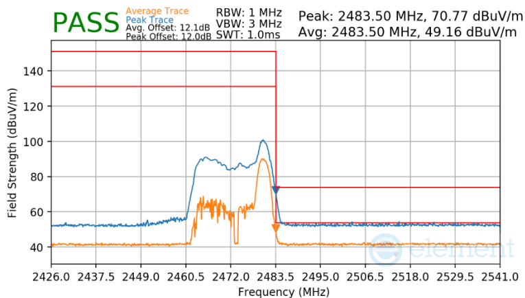
Plot 7-152 Radiated Restricted Upper Band Edge Measurement CDD (Peak & Average – RU26)
