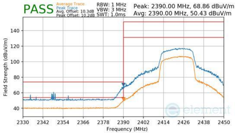
Plot 7-140 Radiated Restricted Lower Band Edge Measurement Antenna 1a (Peak & Average – RU242)
