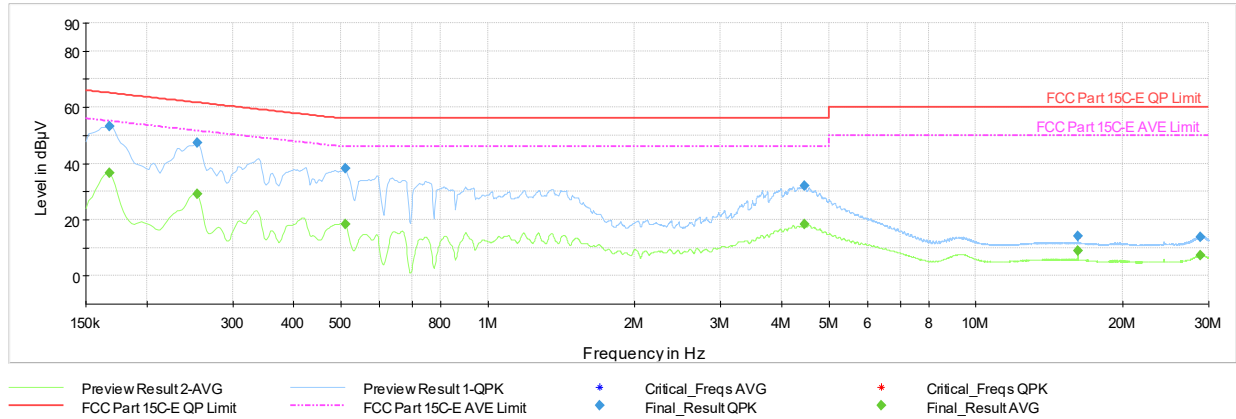
Plot 7-180. AC Line Conducted Emissions with 802.11be CDD (RU26) Ch.6 (N, with AC/DC Adapter)
