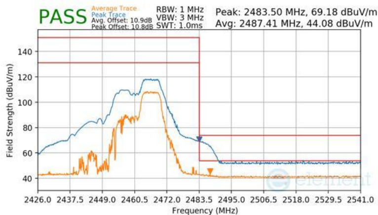
Plot 7-105 Radiated Restricted Upper Band Edge Measurement Antenna 3a (Peak & Average – RU52+26)
