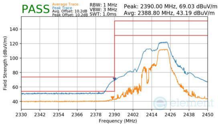
Plot 7-101 Radiated Restricted Lower Band Edge Measurement Antenna 3a (Peak & Average – RU52+26)
