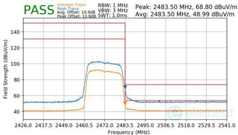
Plot 7-148 Radiated Restricted Upper Band Edge Measurement Antenna 1a (Peak & Average – RU242)
