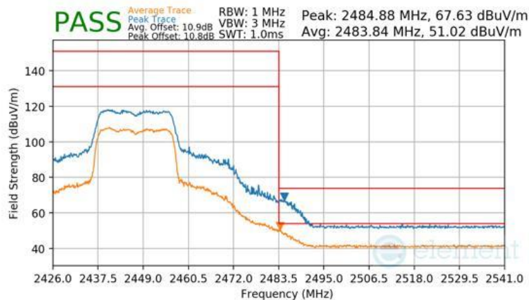
Plot 7-171 Radiated Restricted Upper Band Edge Measurement CDD (Peak & Average – RU242)
