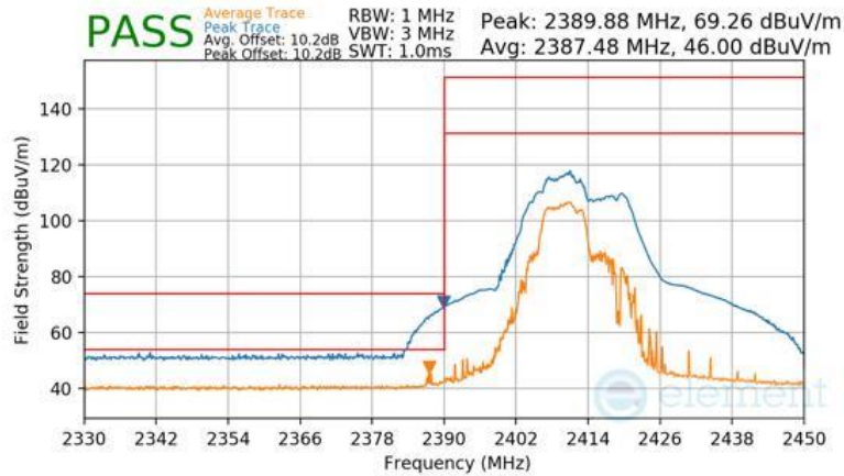
Plot 7-153 Radiated Restricted Lower Band Edge Measurement CDD (Peak & Average – RU52+26)
