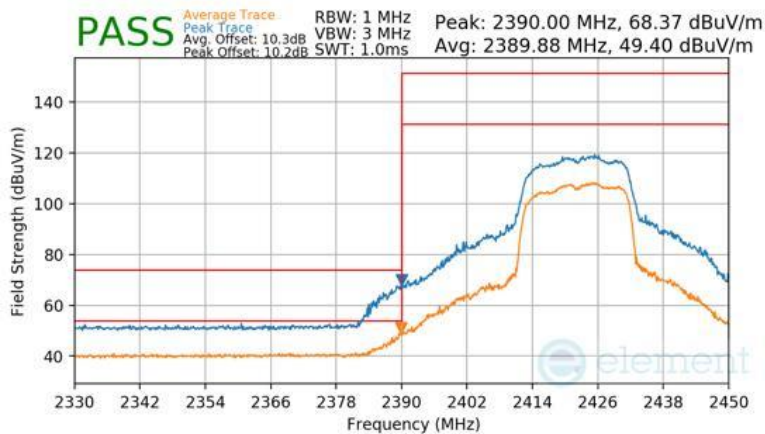
Plot 7-166 Radiated Restricted Lower Band Edge Measurement CDD (Peak & Average – RU242)
