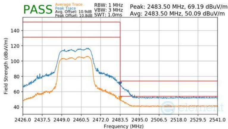
Plot 7-173 Radiated Restricted Upper Band Edge Measurement CDD (Peak & Average – RU242)
