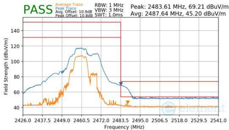
Plot 7-104 Radiated Restricted Upper Band Edge Measurement Antenna 3a (Peak & Average – RU52+26)
