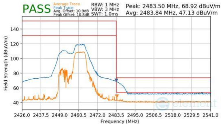
Plot 7-103 Radiated Restricted Upper Band Edge Measurement Antenna 3a (Peak & Average – RU52+26)
