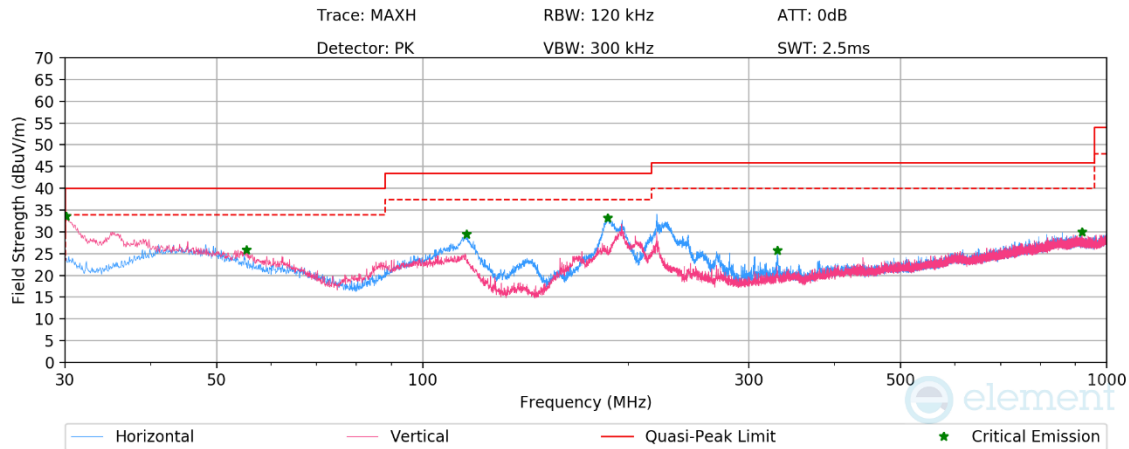
Plot 7-177. Radiated Spurious Emissions Below 1GHz CDD Ch.6 (RU26), with AC/DC Adapter
