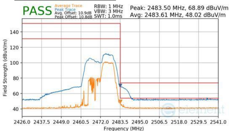
Plot 7-163 Radiated Restricted Upper Band Edge Measurement CDD (Peak & Average – RU52+26)
