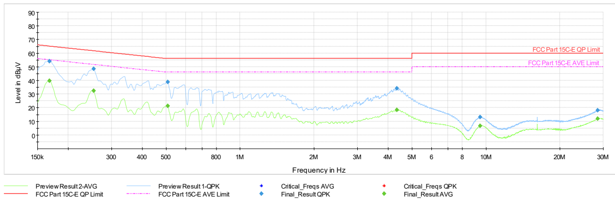
Plot 7-182. AC Line Conducted Emissions with 802.11be CDD (RU242) Ch.6 (N, with AC/DC Adapter)
