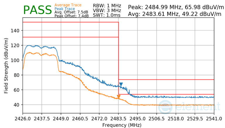
Plot 7-169 Radiated Restricted Upper Band Edge Measurement CDD (Peak & Average – RU242)
