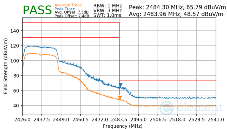
Plot 7-115 Radiated Restricted Upper Band Edge Measurement Antenna 3a (Peak & Average – RU242)
