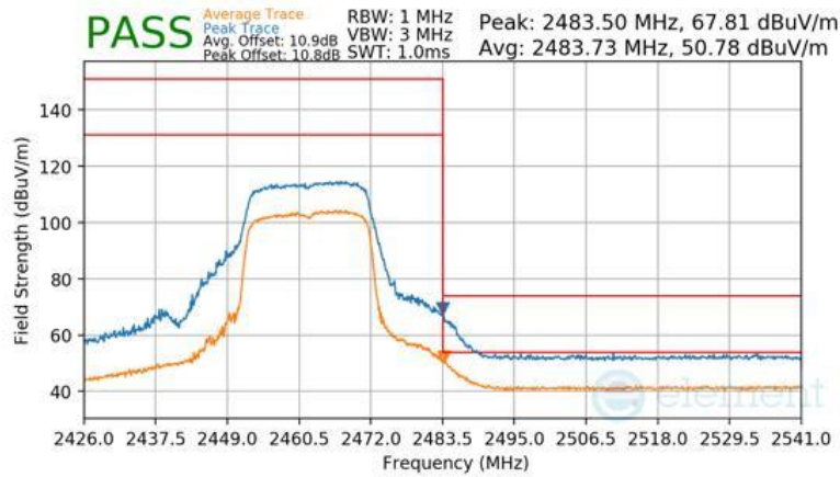
Plot 7-120 Radiated Restricted Upper Band Edge Measurement Antenna 3a (Peak & Average – RU242)
