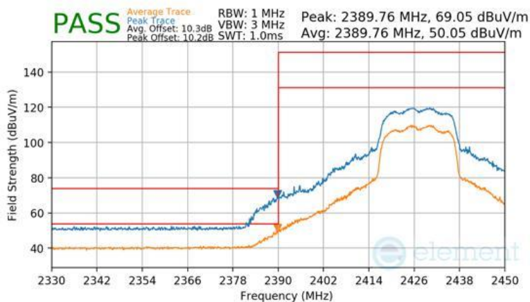
Plot 7-167 Radiated Restricted Lower Band Edge Measurement CDD (Peak & Average – RU242)
