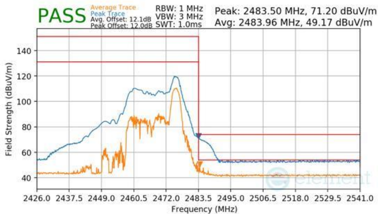
Plot 7-151 Radiated Restricted Upper Band Edge Measurement CDD (Peak & Average – RU26)
