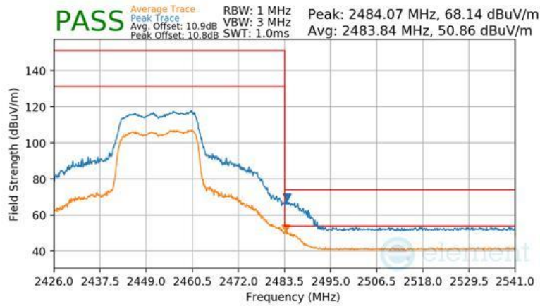
Plot 7-172 Radiated Restricted Upper Band Edge Measurement CDD (Peak & Average – RU242)
