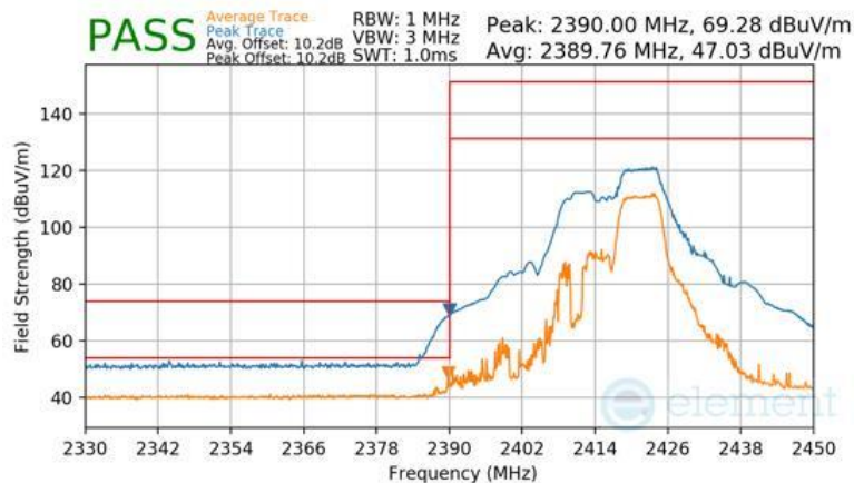
Plot 7-129 Radiated Restricted Lower Band Edge Measurement Antenna 1a (Peak & Average – RU52+26)
