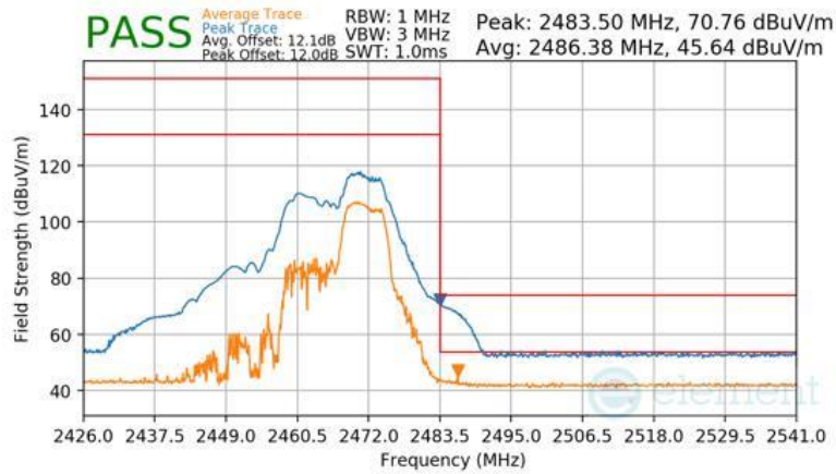
Plot 7-161 Radiated Restricted Upper Band Edge Measurement CDD (Peak & Average – RU52+26)
