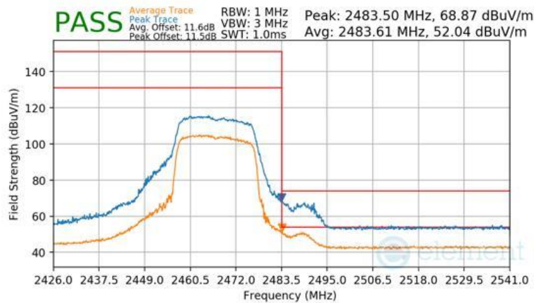
Plot 7-121 Radiated Restricted Upper Band Edge Measurement Antenna 3a (Peak & Average – RU242)
