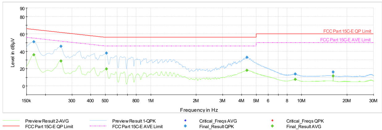
Plot 7-181. AC Line Conducted Emissions with 802.11be CDD (RU242) Ch.6 (L1, with AC/DC Adapter)
