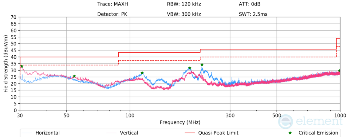
Plot 7-178. Radiated Spurious Emissions Below 1GHz CDD Ch.6 (RU242), with AC/DC Adapter
