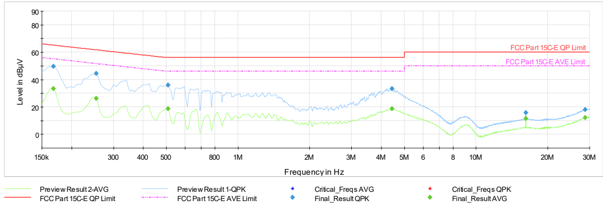
Plot 7-179. AC Line Conducted Emissions with 802.11be CDD (RU26) Ch.6 (L1, with AC/DC Adapter)
