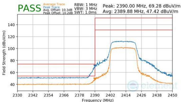
Plot 7-138 Radiated Restricted Lower Band Edge Measurement Antenna 1a (Peak & Average – RU242)
