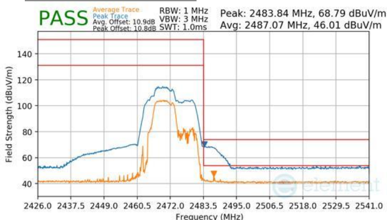
Plot 7-136 Radiated Restricted Upper Band Edge Measurement Antenna 1a (Peak & Average – RU52+26)
