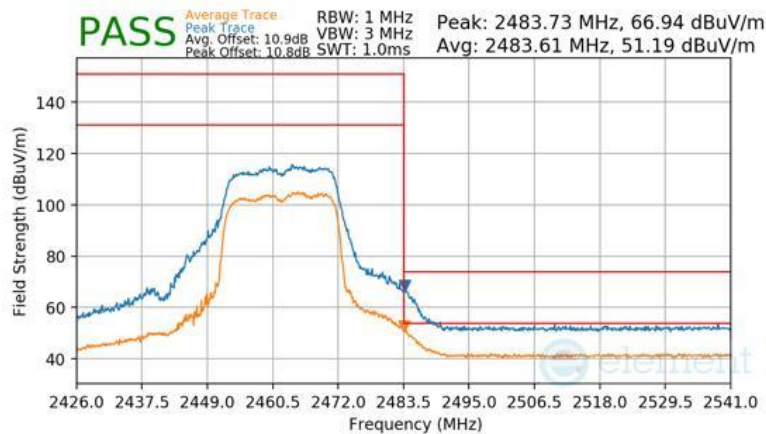
Plot 7-174 Radiated Restricted Upper Band Edge Measurement CDD (Peak & Average – RU242)
