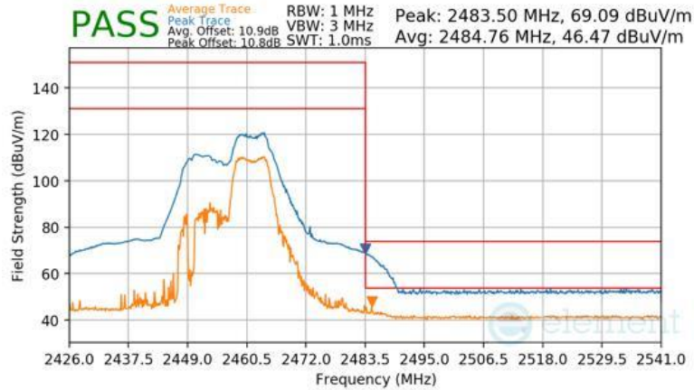
Plot 7-157 Radiated Restricted Upper Band Edge Measurement CDD (Peak & Average – RU52+26)
