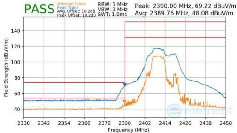
Plot 7-126 Radiated Restricted Lower Band Edge Measurement Antenna 1a (Peak & Average – RU52+26)
