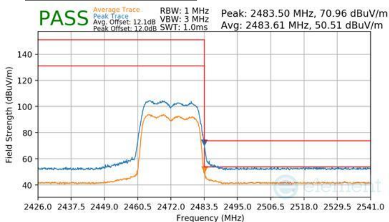
Plot 7-176 Radiated Restricted Upper Band Edge Measurement CDD (Peak & Average – RU242)
