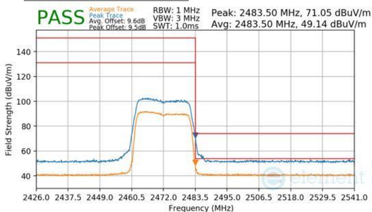
Plot 7-122 Radiated Restricted Upper Band Edge Measurement Antenna 3a (Peak & Average – RU242)
