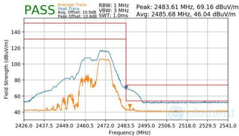
Plot 7-135 Radiated Restricted Upper Band Edge Measurement Antenna 1a (Peak & Average – RU52+26)
