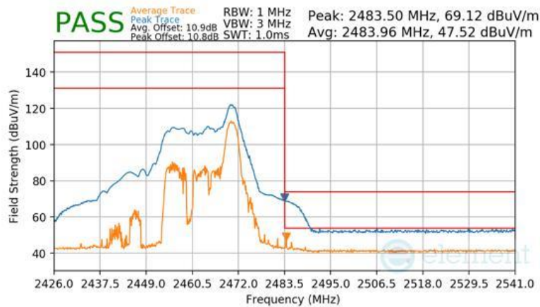
Plot 7-150 Radiated Restricted Upper Band Edge Measurement CDD (Peak & Average – RU26)
