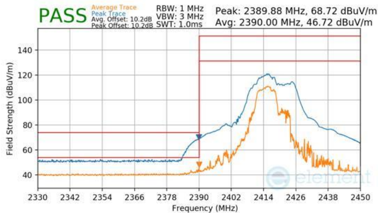
Plot 7-155 Radiated Restricted Lower Band Edge Measurement CDD (Peak & Average – RU52+26)
