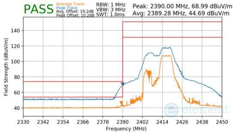
Plot 7-127 Radiated Restricted Lower Band Edge Measurement Antenna 1a (Peak & Average – RU52+26)
