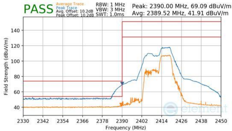
Plot 7-99 Radiated Restricted Lower Band Edge Measurement Antenna 3a (Peak & Average – RU52+26)
