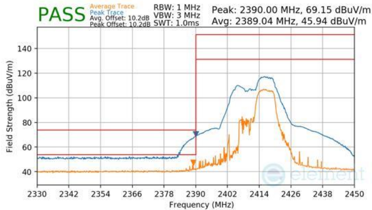
Plot 7-154 Radiated Restricted Lower Band Edge Measurement CDD (Peak & Average – RU52+26)
