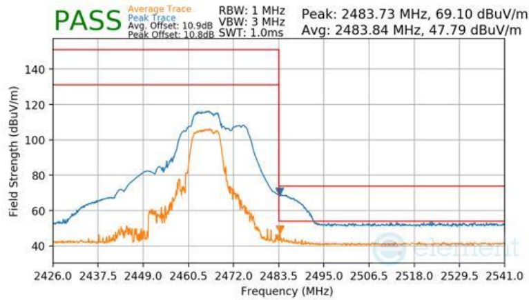
Plot 7-134 Radiated Restricted Upper Band Edge Measurement Antenna 1a (Peak & Average – RU52+26)
