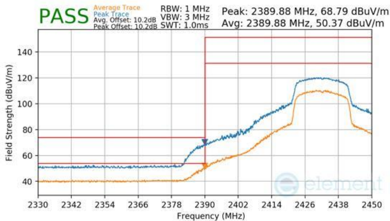
Plot 7-114 Radiated Restricted Lower Band Edge Measurement Antenna 3a (Peak & Average – RU242)
