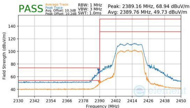
Plot 7-164 Radiated Restricted Lower Band Edge Measurement CDD (Peak & Average – RU242)
