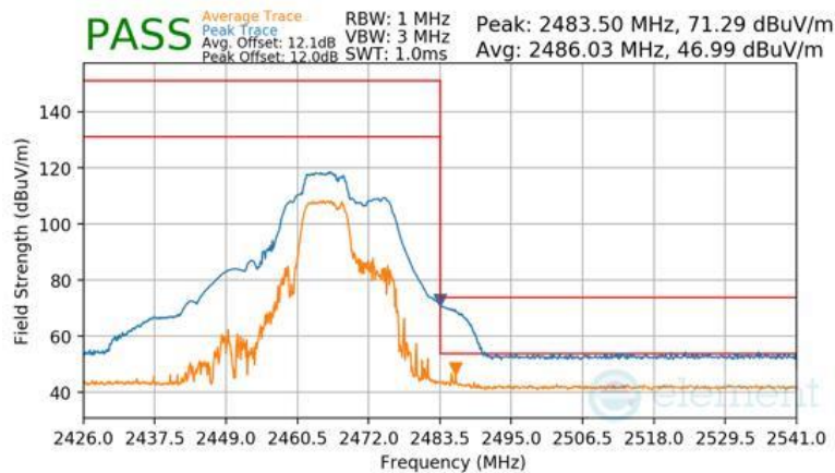
Plot 7-106 Radiated Restricted Upper Band Edge Measurement Antenna 3a (Peak & Average – RU52+26)
