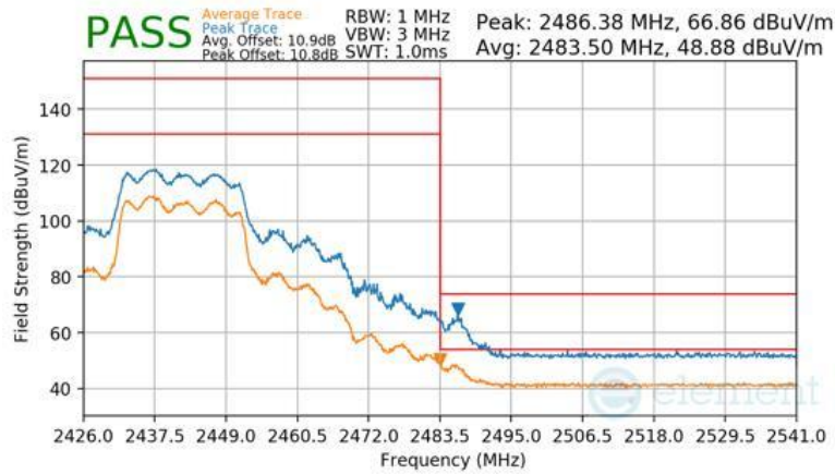
Plot 7-170 Radiated Restricted Upper Band Edge Measurement CDD (Peak & Average – RU242)
