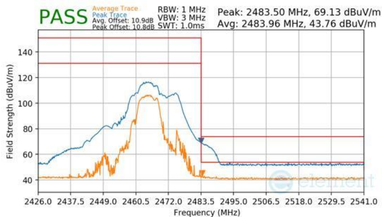
Plot 7-160 Radiated Restricted Upper Band Edge Measurement CDD (Peak & Average – RU52+26)
