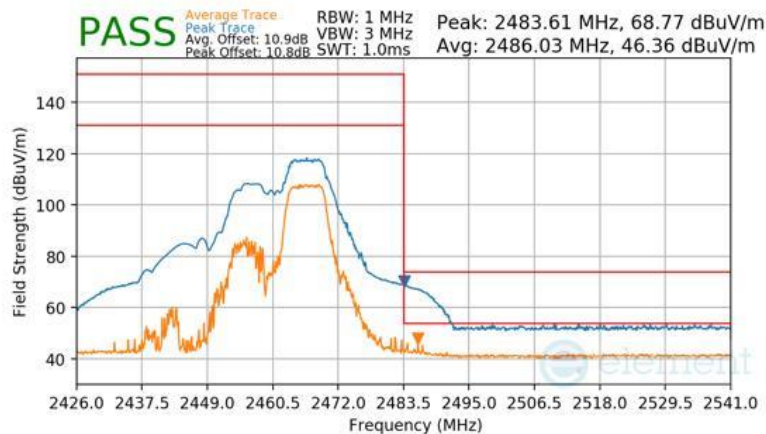
Plot 7-133 Radiated Restricted Upper Band Edge Measurement Antenna 1a (Peak & Average – RU52+26)
