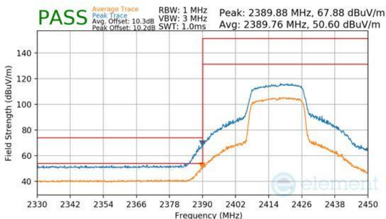
Plot 7-139 Radiated Restricted Lower Band Edge Measurement Antenna 1a (Peak & Average – RU242)
