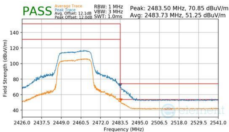
Plot 7-119 Radiated Restricted Upper Band Edge Measurement Antenna 3a (Peak & Average – RU242)
