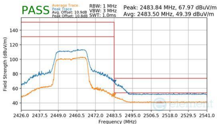
Plot 7-145 Radiated Restricted Upper Band Edge Measurement Antenna 1a (Peak & Average – RU242)
