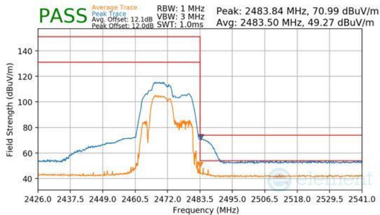
Plot 7-108 Radiated Restricted Upper Band Edge Measurement Antenna 3a (Peak & Average – RU52+26)
