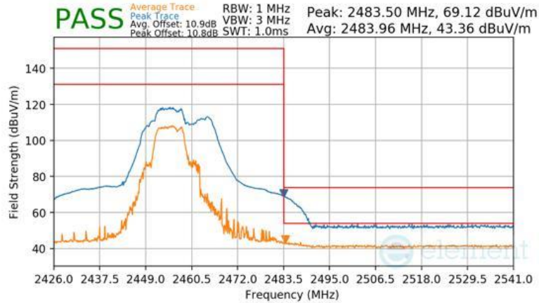
Plot 7-102 Radiated Restricted Upper Band Edge Measurement Antenna 3a (Peak & Average – RU52+26)
