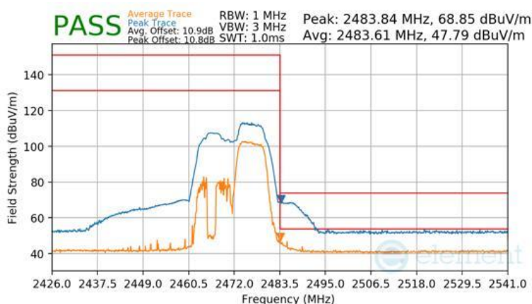
Plot 7-137 Radiated Restricted Upper Band Edge Measurement Antenna 1a (Peak & Average – RU52+26)
