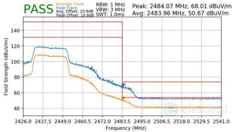
Plot 7-116 Radiated Restricted Upper Band Edge Measurement Antenna 3a (Peak & Average – RU242)
