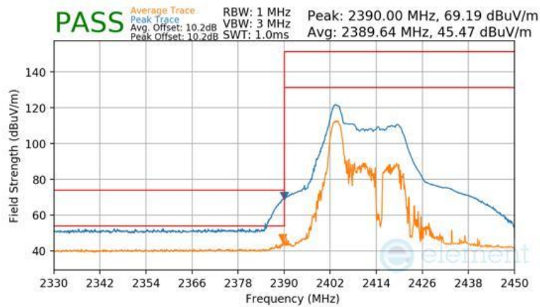
Plot 7-123 Radiated Restricted Lower Band Edge Measurement Antenna 1a (Peak & Average – RU26)
