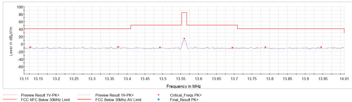
Plot 7-1. In Band Radiated Spurious Emissions (Charging Rate 2.6C, with AC/DC Adapter)
