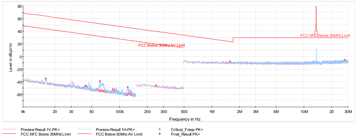
Plot 7-2. Radiated Spurious Plot 9kHz – 30MHz (Charging Rate 2.6C, with AC/DC Adapter)
