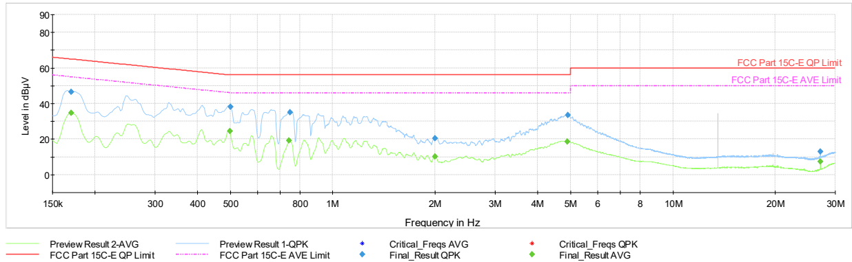
Plot 7-4. AC Line-Conducted Plot (L1, Charging Rate 2.6C, with AC/DC Adapter)
