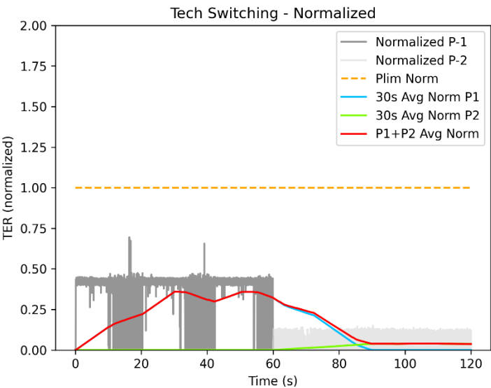
Figure 6-1 Technology Switch Normalized Time-averaged conducted TX power
