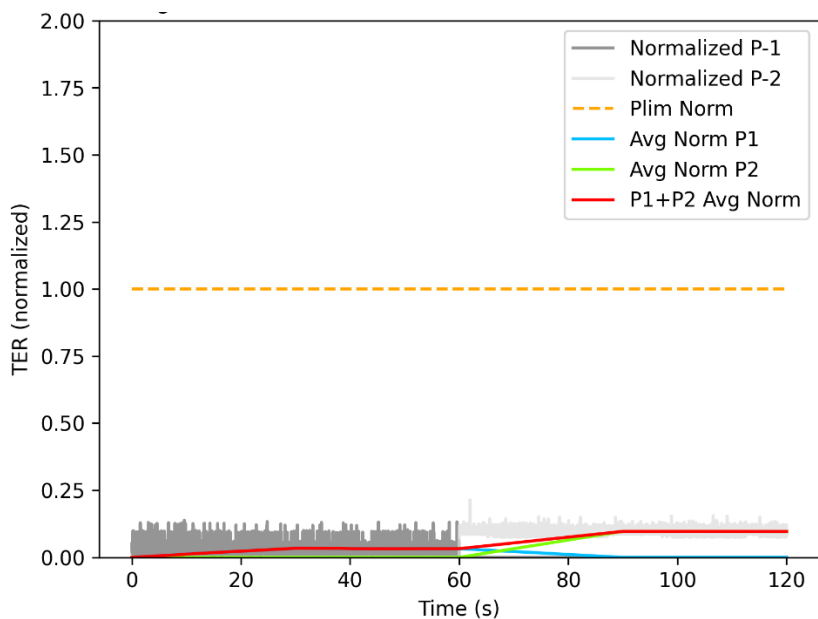
Figure 6-3 NB U-NII 3 Antenna Switch Normalized Time-averaged conducted TX power
