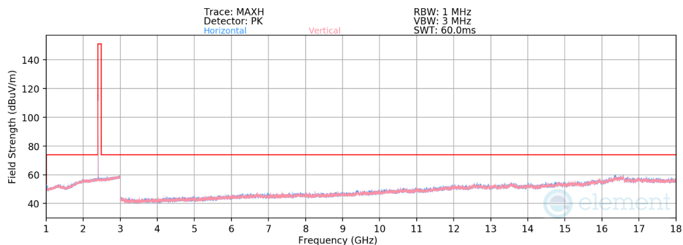
Plot 7-45. Radiated Spurious Emissions 1-18GHz Antenna WF2b (802.15.4 ePA – Ch. 11)
