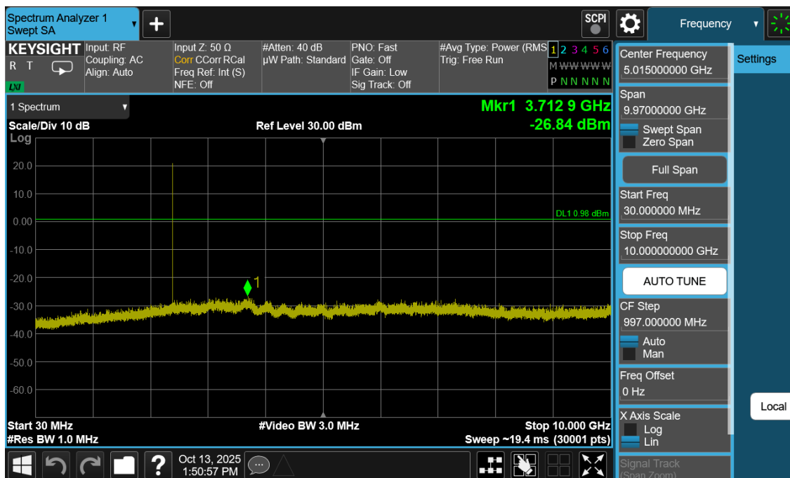
Plot 7-35. Conducted Spurious Antenna WF2b (802.15.4, ePA – Ch. 11)
