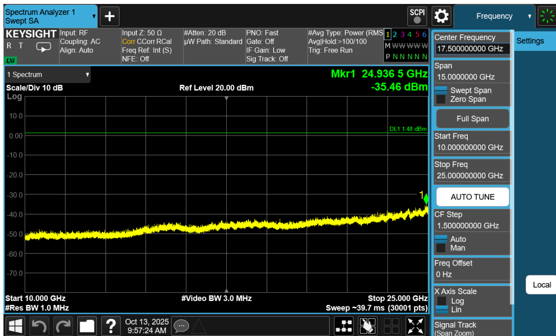
Plot 7-32. Conducted Spurious Antenna WF7b (802.15.4, ePA – Ch. 18)
