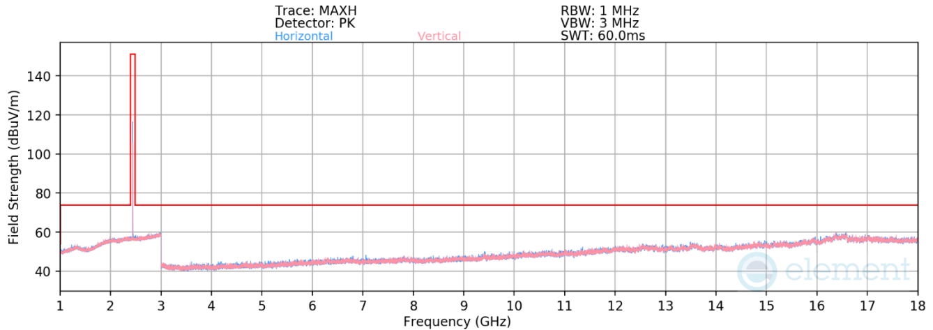
Plot 7-42. Radiated Spurious Emissions 1-18GHz Antenna WF7b (802.15.4 ePA – Ch. 18)
