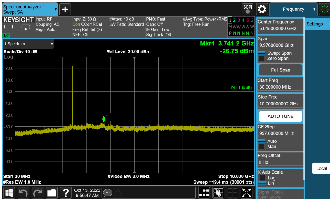
Plot 7-31. Conducted Spurious Antenna WF7b (802.15.4, ePA – Ch. 18)
