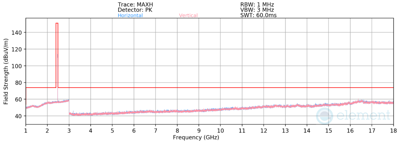
Plot 7-48. Radiated Spurious Emissions 1-18GHz Antenna WF2b (802.15.4 ePA – Ch. 25)
