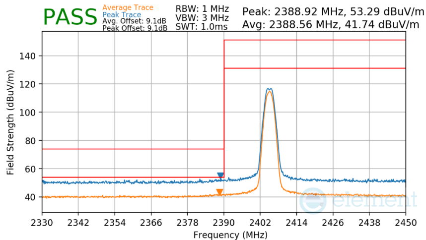
Plot 7-49. Radiated Restricted Lower Band Edge Measurement Antenna WF7b
