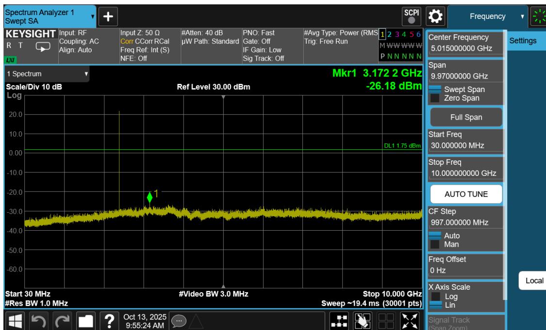
Plot 7-29. Conducted Spurious Antenna WF7b (802.15.4, ePA – Ch. 11)
