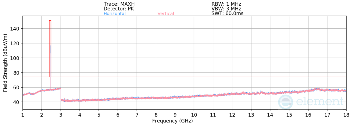
Plot 7-44. Radiated Spurious Emissions 1-18GHz Antenna WF7b (802.15.4 ePA – Ch. 25)
