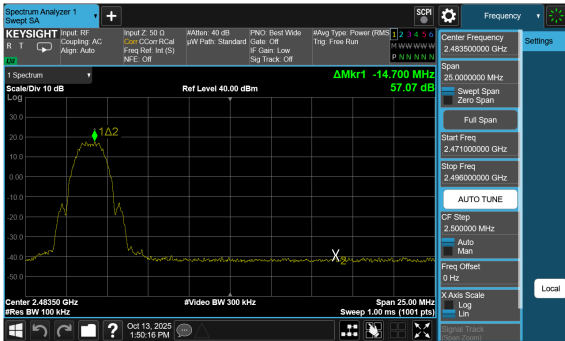
Plot 7-28. Band Edge Antenna WF2b (802.15.4, ePA – Ch. 25)
