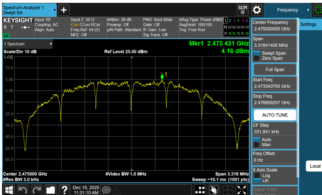
Plot 7-15. Power Spectral Density Antenna WF7b (802.15.4, ePA – Ch. 25)
