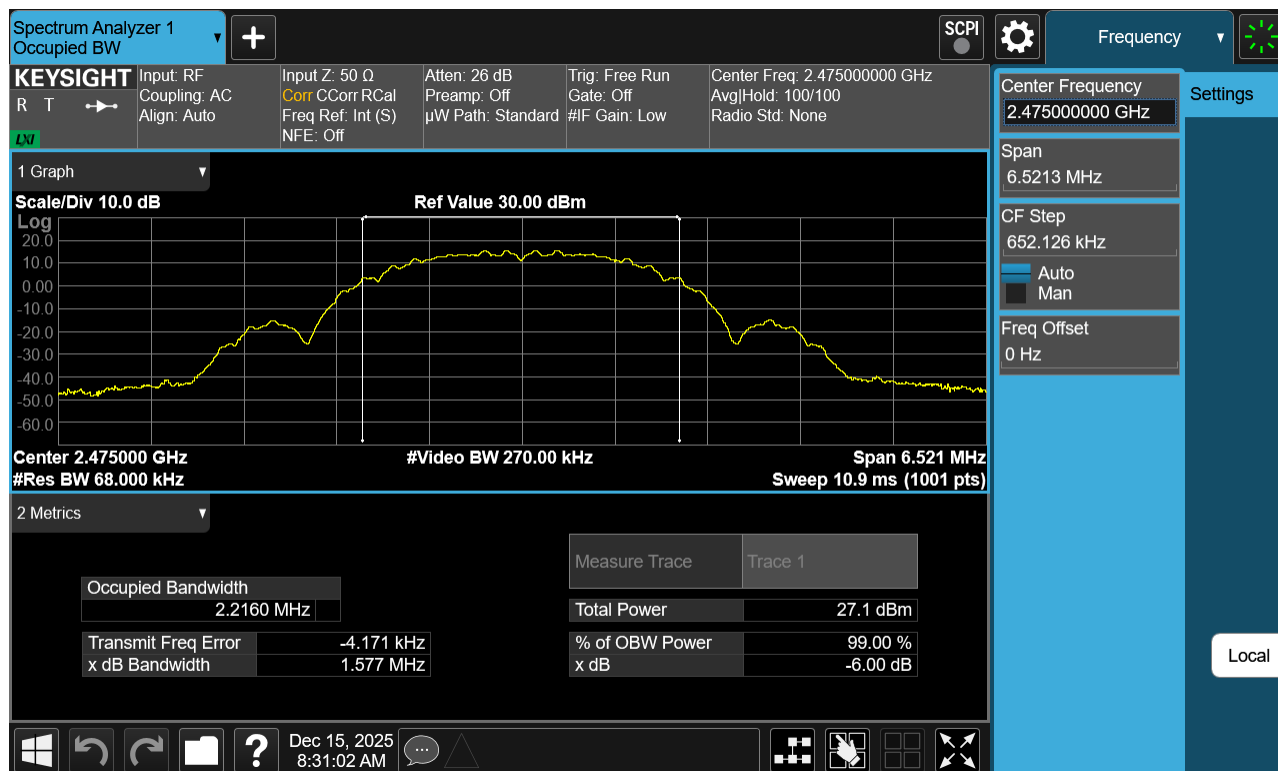
Plot 7-6. 99% OBW Antenna WF2b(802.15.4, Ch. 25)
