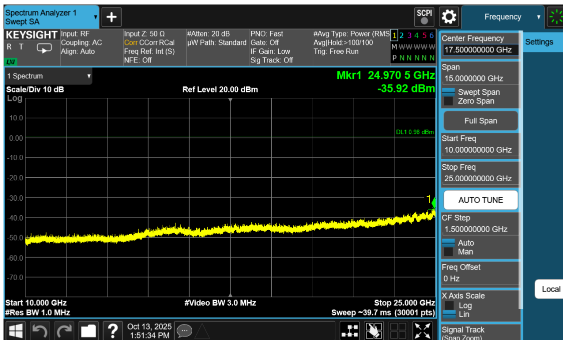
Plot 7-36. Conducted Spurious Antenna WF2b (802.15.4, ePA – Ch. 11)
