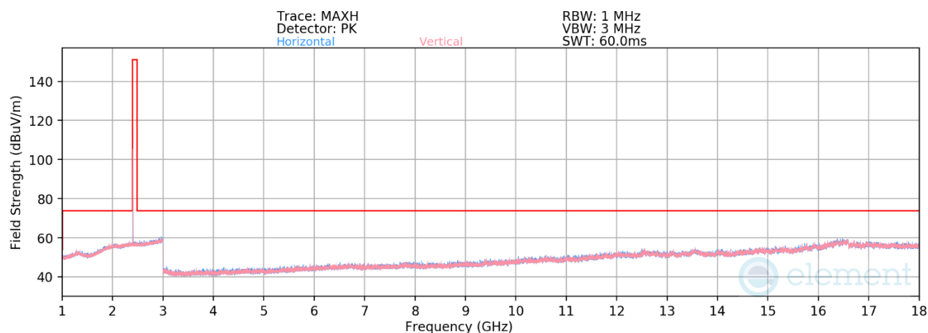
Plot 7-41. Radiated Spurious Emissions 1-18GHz Antenna WF7b (802.15.4 ePA – Ch. 11)
