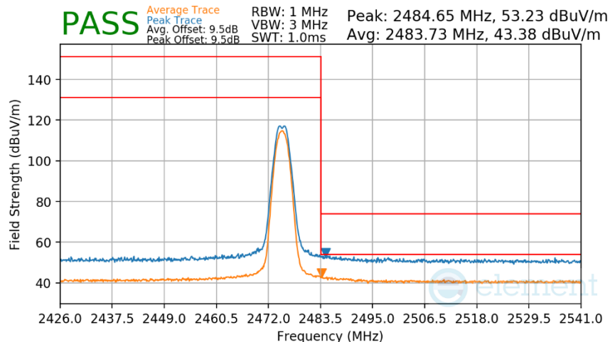
Plot 7-50. Radiated Restricted Upper Band Edge Measurement Antenna WF7b
