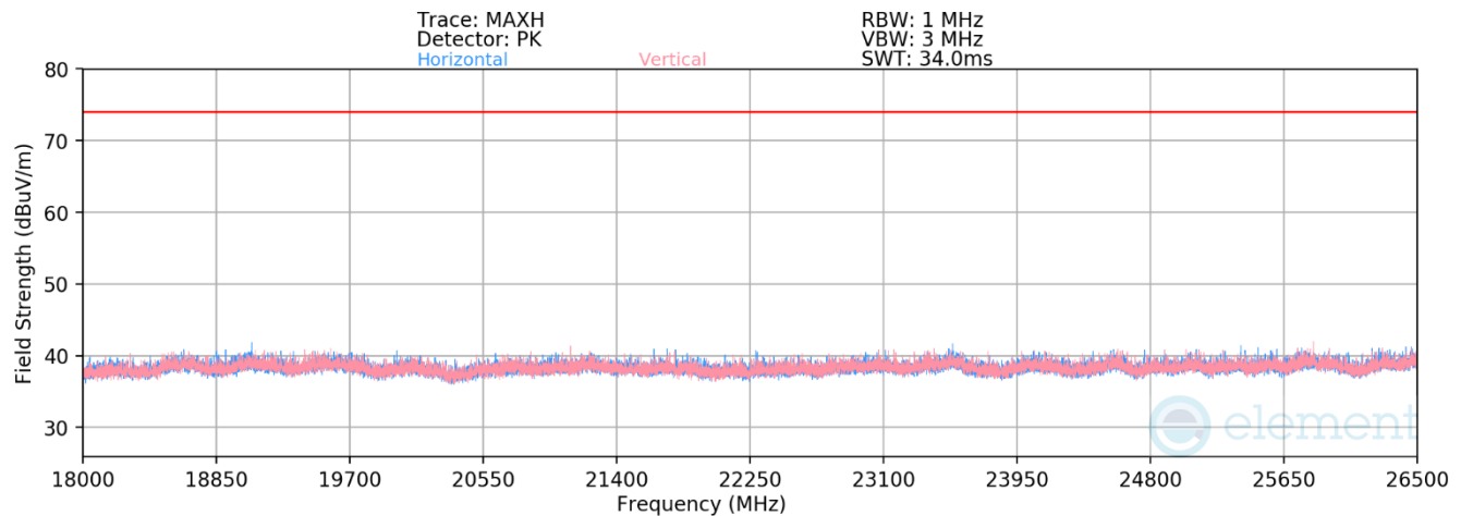
Plot 7-47. Radiated Spurious Emissions Above 18GHz Antenna WF2b (802.15.4 ePA – Ch. 18)
