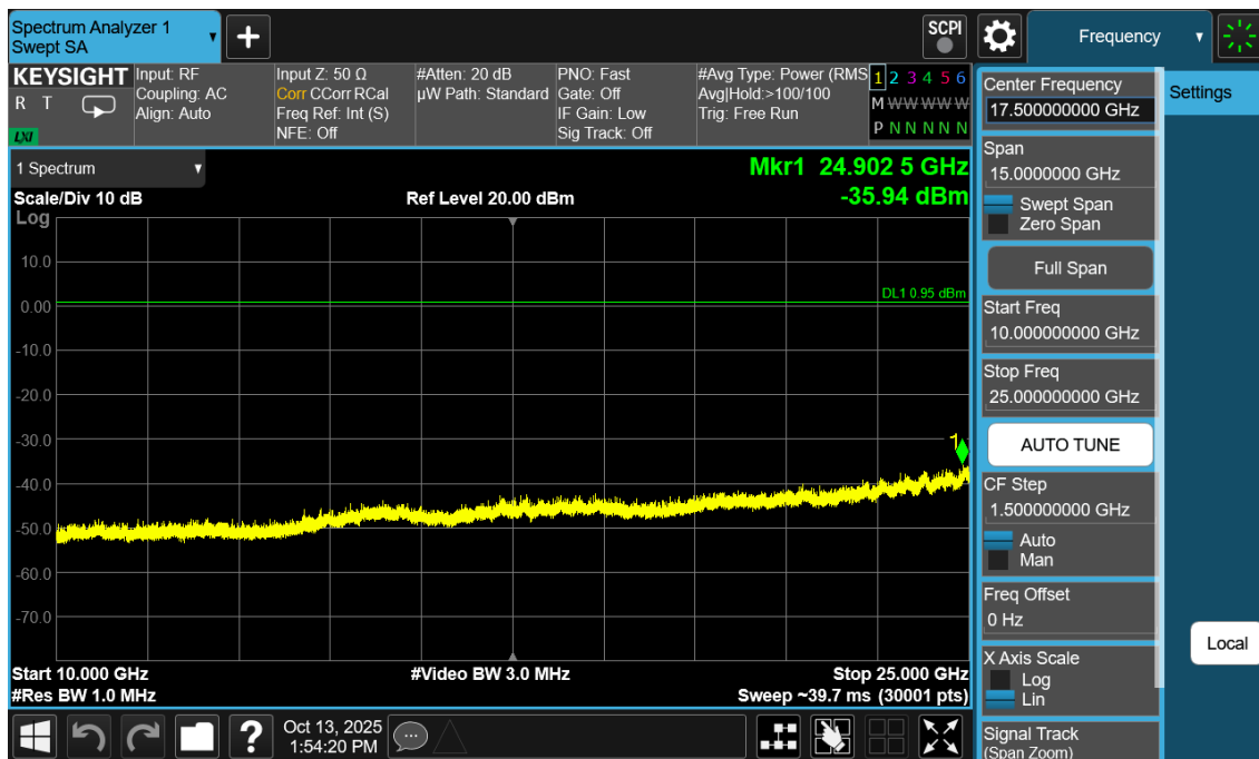
Plot 7-40. Conducted Spurious Antenna WF2b (802.15.4, ePA – Ch. 25)
