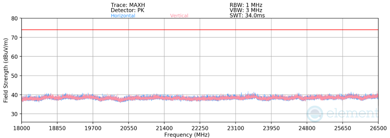
Plot 7-43. Radiated Spurious Emissions Above 18GHz Antenna WF7b (802.15.4 ePA – Ch. 18)
