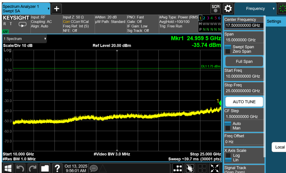
Plot 7-30. Conducted Spurious Antenna WF7b (802.15.4, ePA – Ch. 11)
