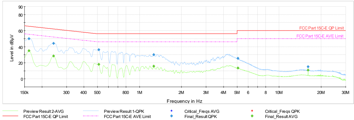
Plot 7-54. AC Line Conducted Emission with 802.15.4 Antenna WF7b (L1, Ch.18 - ePA, with AC/DC Adapter)
