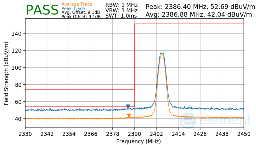
Plot 7-51. Radiated Restricted Lower Band Edge Measurement Antenna WF2b
