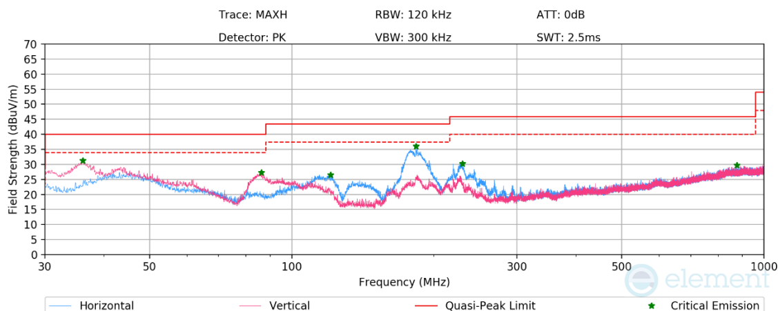
Plot 7-53. Radiated Spurious Emissions 30MHz-1GHz Antenna WF7b (ePA - Ch.18, with AC/DC Adapter)
