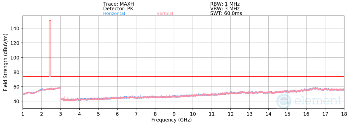
Plot 7-46. Radiated Spurious Emissions 1-18GHz Antenna WF2b (802.15.4 ePA – Ch. 18)
