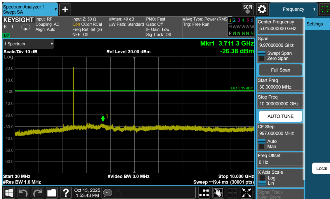
Plot 7-39. Conducted Spurious Antenna WF2b (802.15.4, ePA – Ch. 25)
