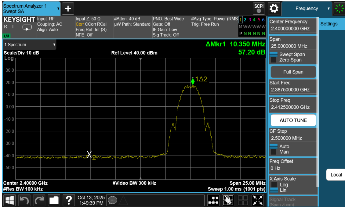
Plot 7-27. Band Edge Antenna WF2b (802.15.4, ePA – Ch. 11)
