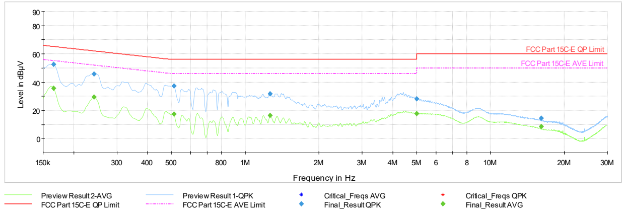
Plot 7-55. AC Line Conducted Emission with 802.15.4 Antenna WF7b (N, Ch.18 - ePA, with AC/DC Adapter)
