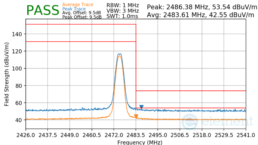
Plot 7-52. Radiated Restricted Upper Band Edge Measurement Antenna WF2b
