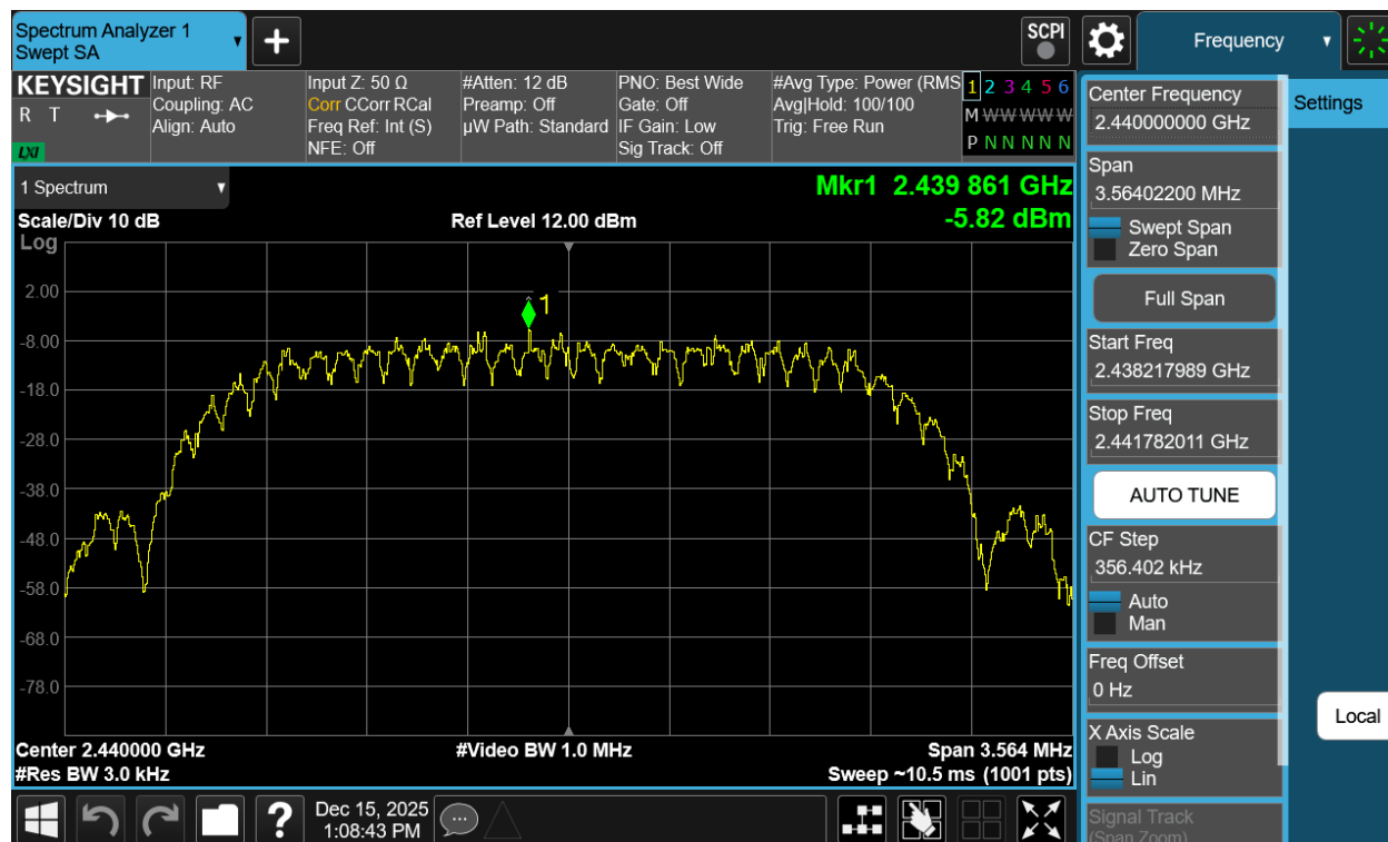
Plot 7-140. Power Spectral Density Plot Antenna WF2b (Bluetooth (HDT2), 2Mbps, ePA – Ch. 37)
