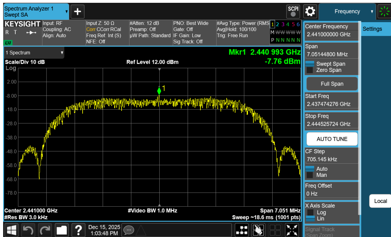
Plot 7-134. Power Spectral Density Plot Antenna WF2b (Bluetooth (HDRPM16), 16Mbps, ePA – Ch. 38)
