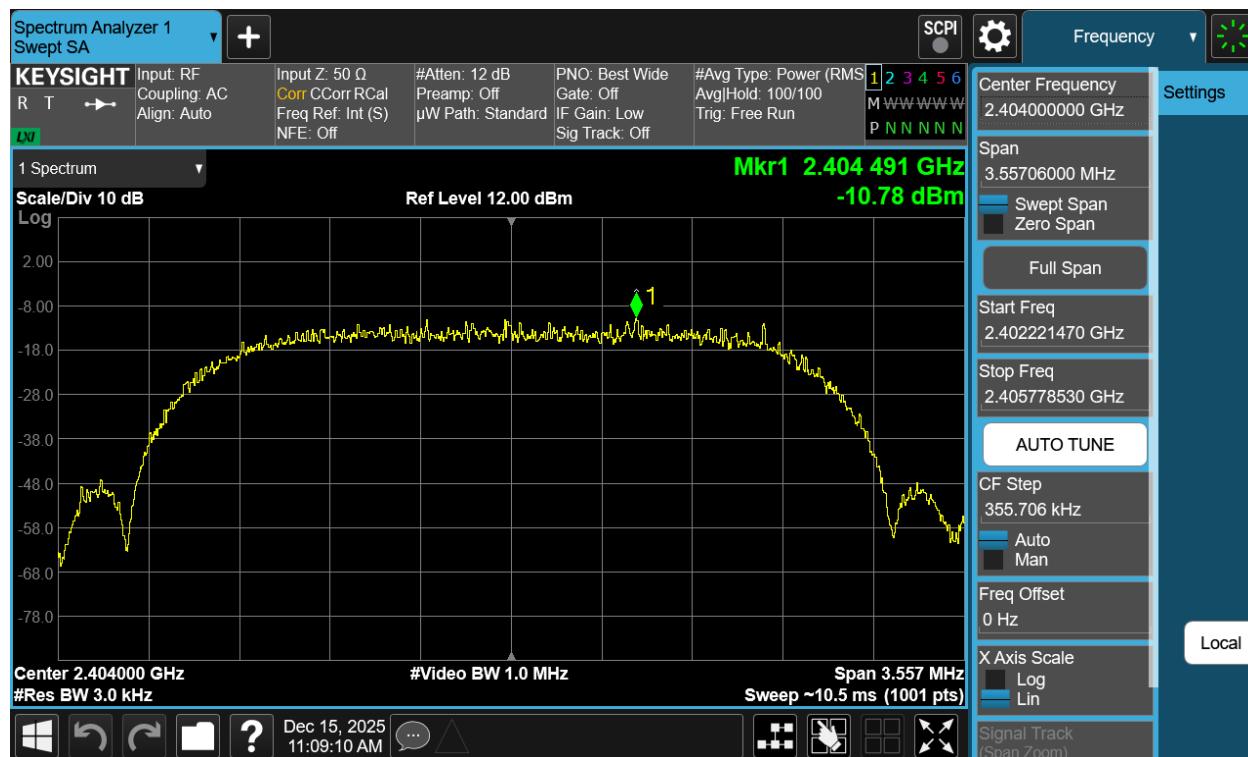
Plot 7-175. Power Spectral Density Plot TxBF Antenna WF7b (Bluetooth (HDRPS2), 8Mbps, iPA – Ch. 1)
