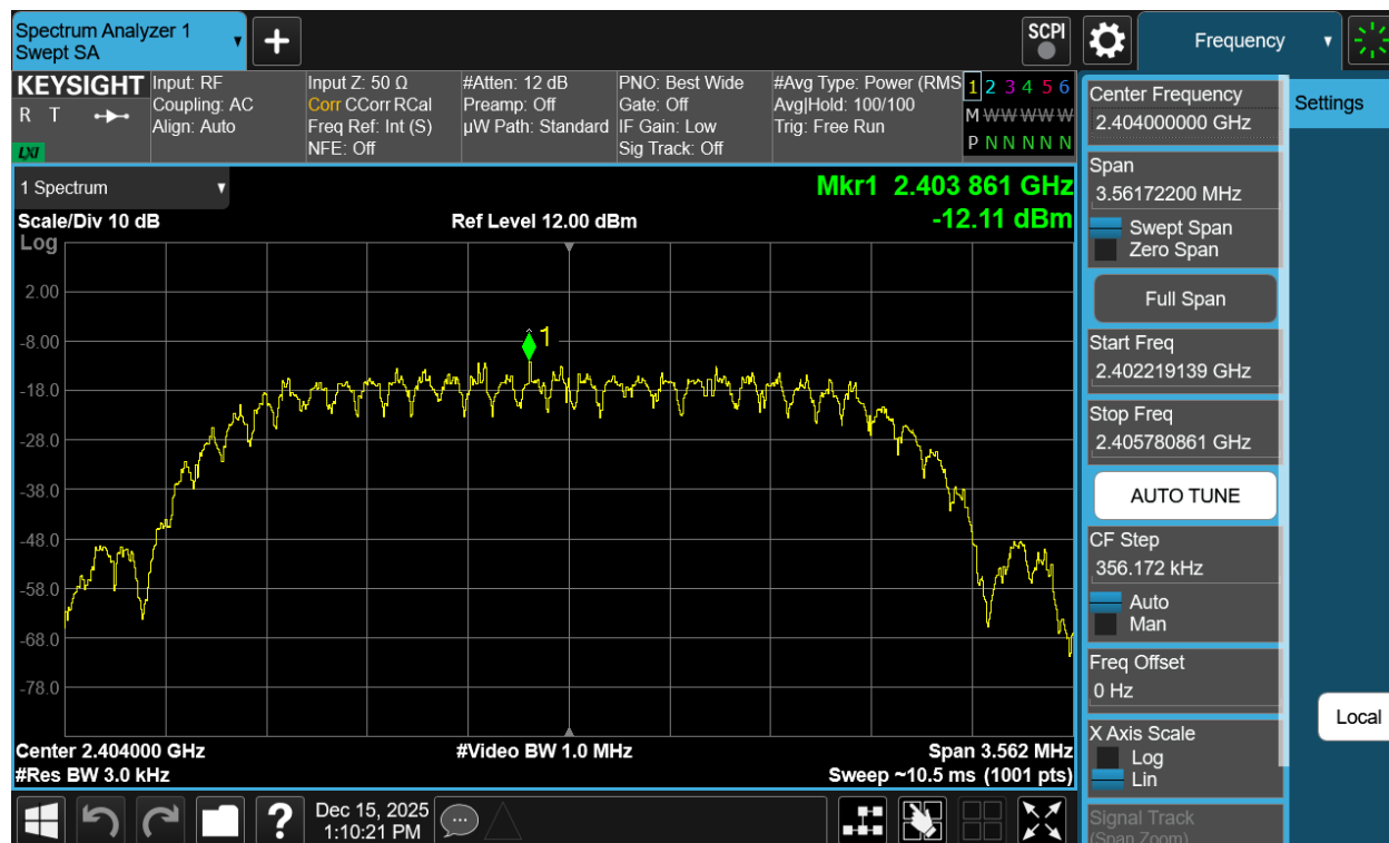
Plot 7-142. Power Spectral Density Plot Antenna WF2b (Bluetooth (HDT2), 2Mbps, iPA – Ch. 1)
