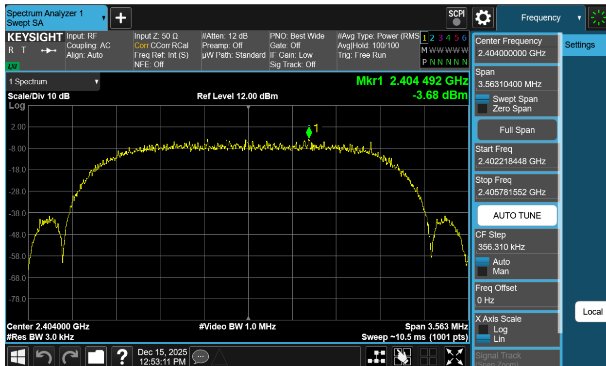
Plot 7-121. Power Spectral Density Plot Antenna WF2b (Bluetooth (HDRPS2), 2Mbps, ePA – Ch. 1)
