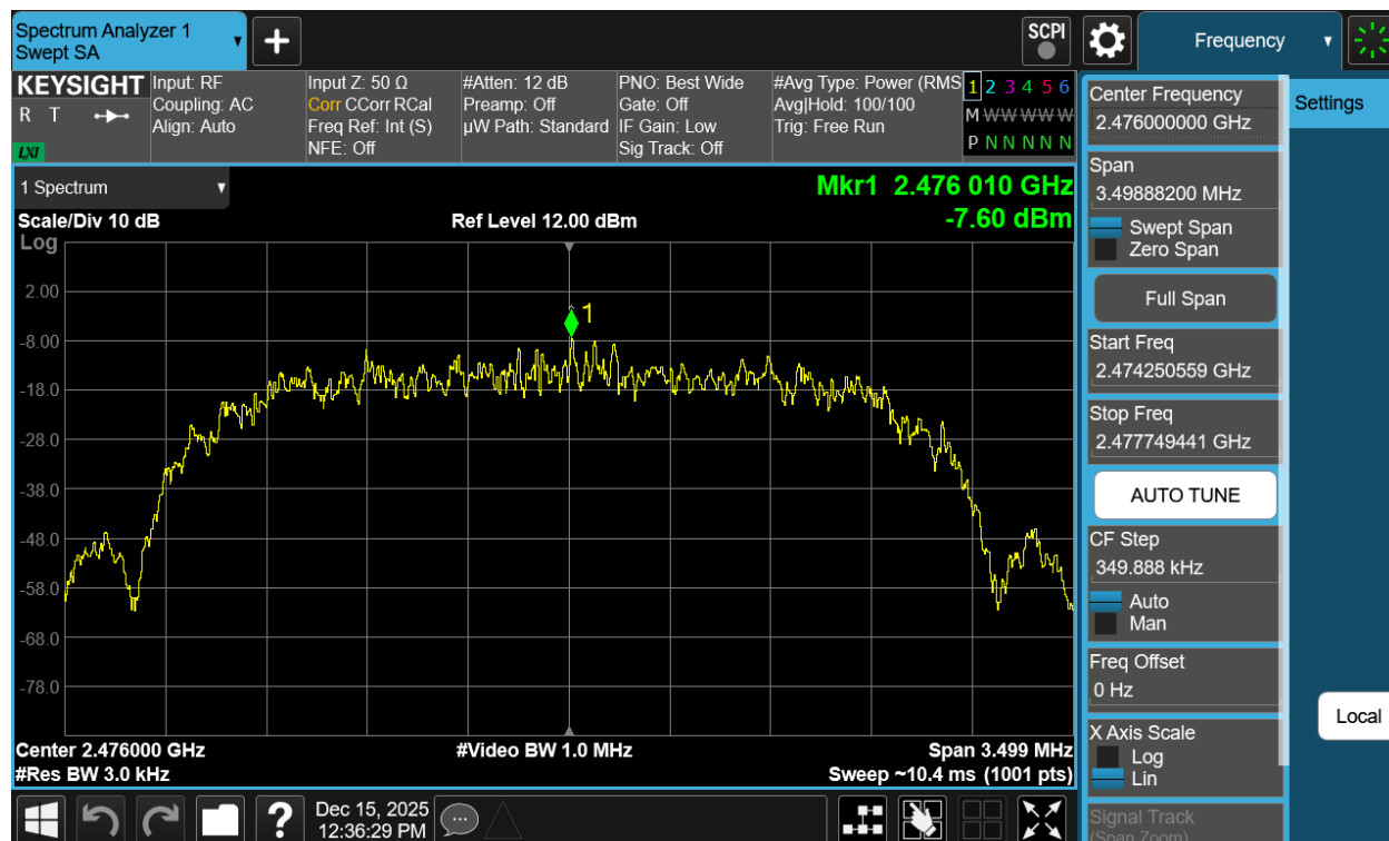
Plot 7-156. Power Spectral Density Plot Tx BF Antenna WF2b (Bluetooth (HDR4), 4Mbps, iPA – Ch. 73)
