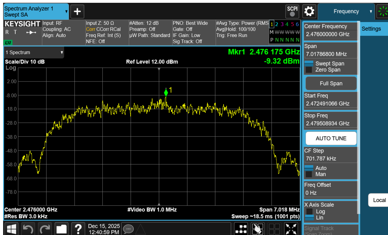
Plot 7-168. Power Spectral Density Plot Tx BF Antenna WF2b (Bluetooth (HDR8), 8Mbps, iPA – Ch. 73)
