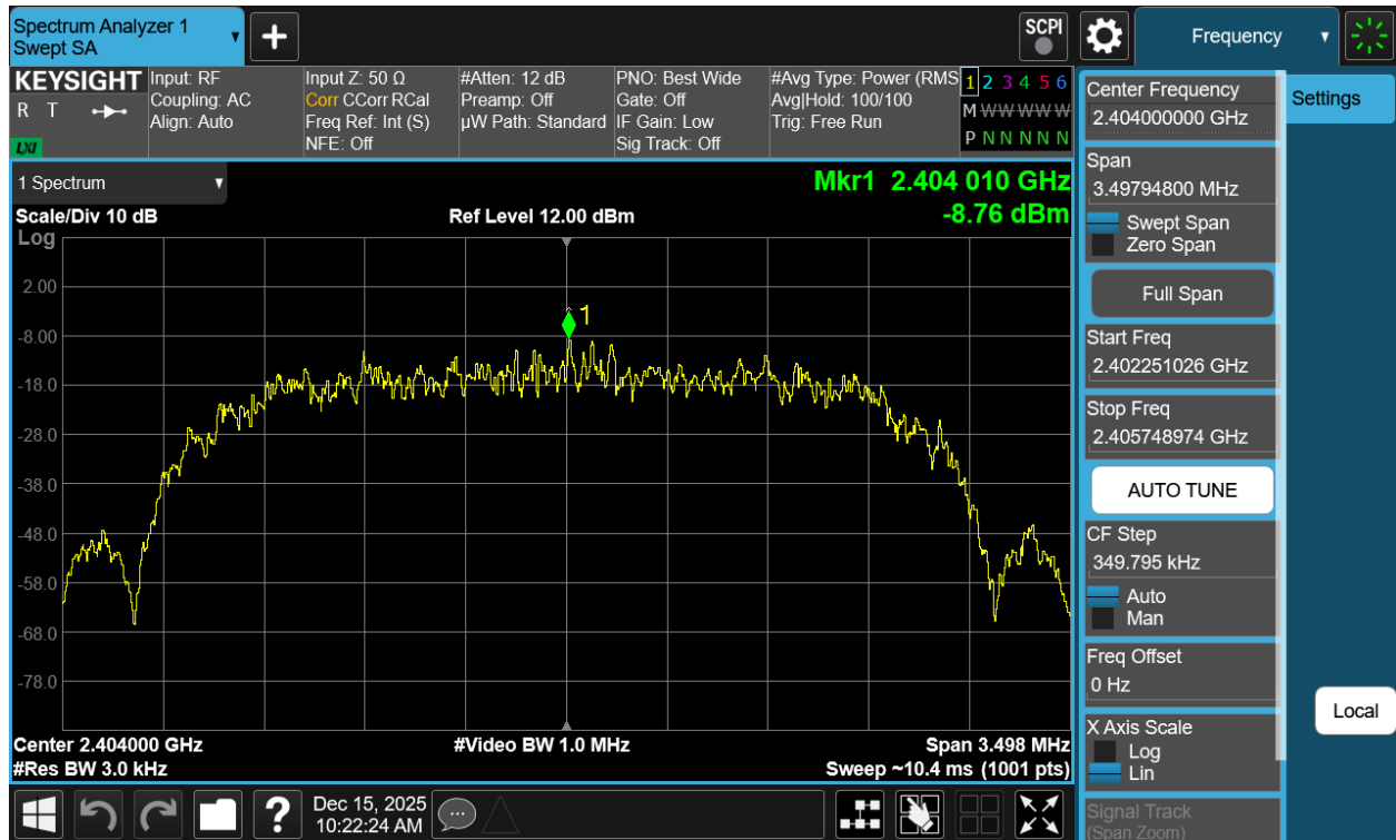
Plot 7-151. Power Spectral Density Plot TxBF Antenna WF7b (Bluetooth (HDR4), 4Mbps, iPA – Ch. 1)
