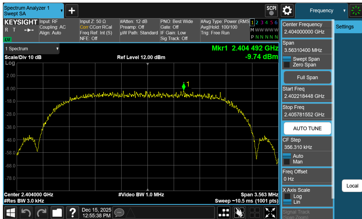
Plot 7-124. Power Spectral Density Plot Antenna WF2b (Bluetooth (HDRPS2), 2Mbps, iPA – Ch. 1)
