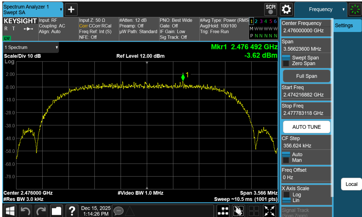
Plot 7-174. Power Spectral Density Plot Tx BF Antenna WF2b (Bluetooth (HDRPS2), 8Mbps, ePA – Ch. 73)
