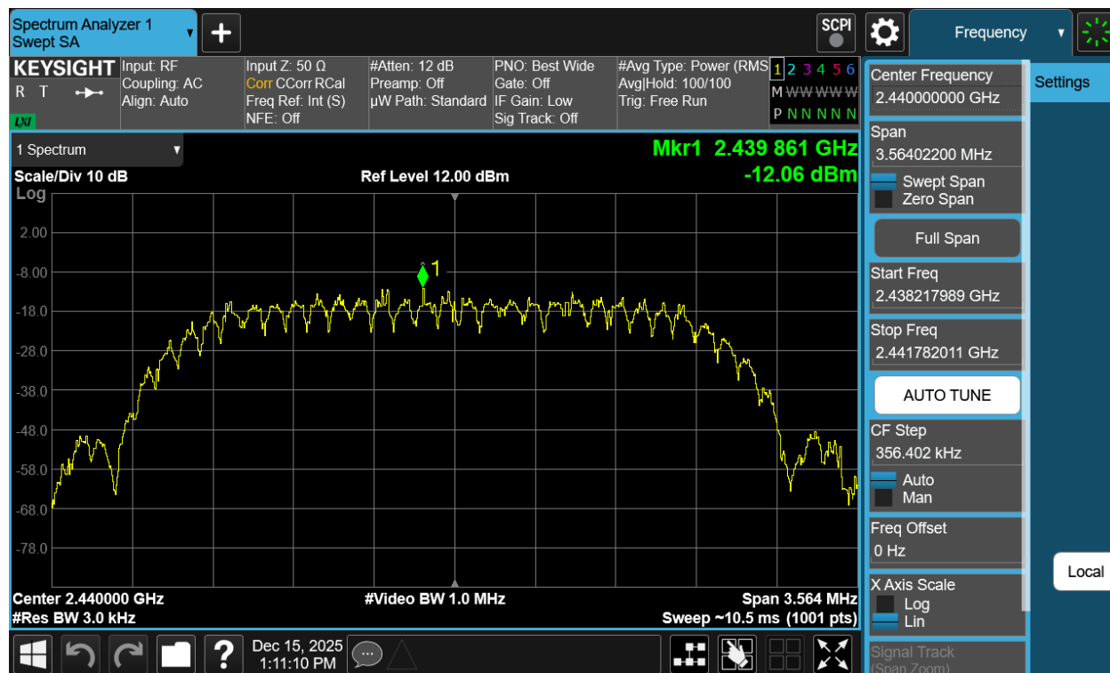
Plot 7-143. Power Spectral Density Plot Antenna WF2b (Bluetooth (HDT2), 2Mbps, iPA – Ch. 37)
