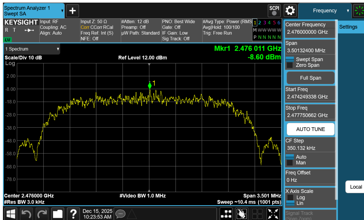
Plot 7-155. Power Spectral Density Plot Tx BF Antenna WF7b (Bluetooth (HDR4), 4Mbps, iPA – Ch. 73)
