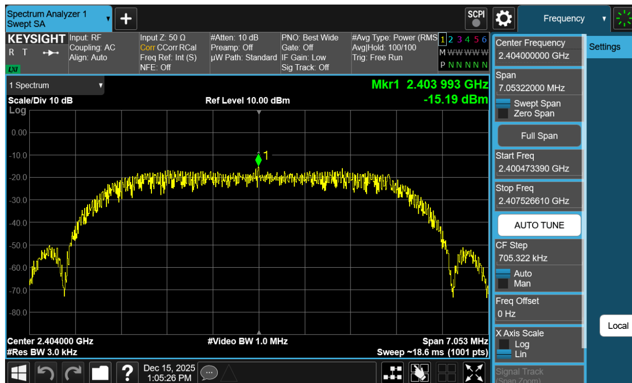
Plot 7-136. Power Spectral Density Plot Antenna WF2b (Bluetooth (HDRPM16), 16Mbps, iPA – Ch. 1)
