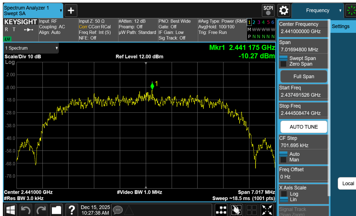
Plot 7-165. Power Spectral Density Plot Tx BF Antenna WF7b (Bluetooth (HDR8), 8Mbps, iPA – Ch. 38)
