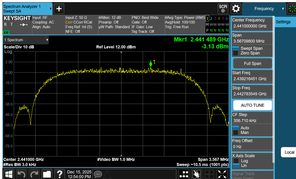
Plot 7-122. Power Spectral Density Plot Antenna WF2b (Bluetooth (HDRPS2), 2Mbps, ePA – Ch. 38)
