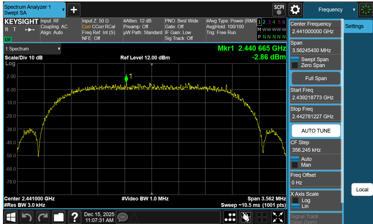
Plot 7-171. Power Spectral Density Plot Tx BF Antenna WF7b (Bluetooth (HDRPS2), 8Mbps, ePA – Ch. 38)
