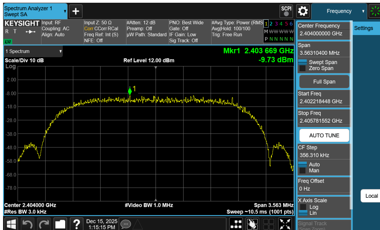
Plot 7-176. Power Spectral Density Plot TxBF Antenna WF2b (Bluetooth (HDRPS2), 8Mbps, iPA – Ch. 1)
