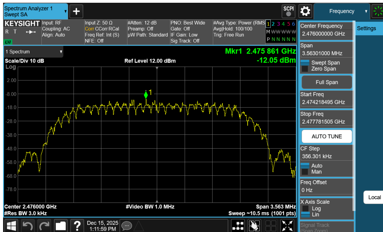
Plot 7-144. Power Spectral Density Plot Antenna WF2b (Bluetooth (HDT2), 2Mbps, iPA – Ch. 73)
