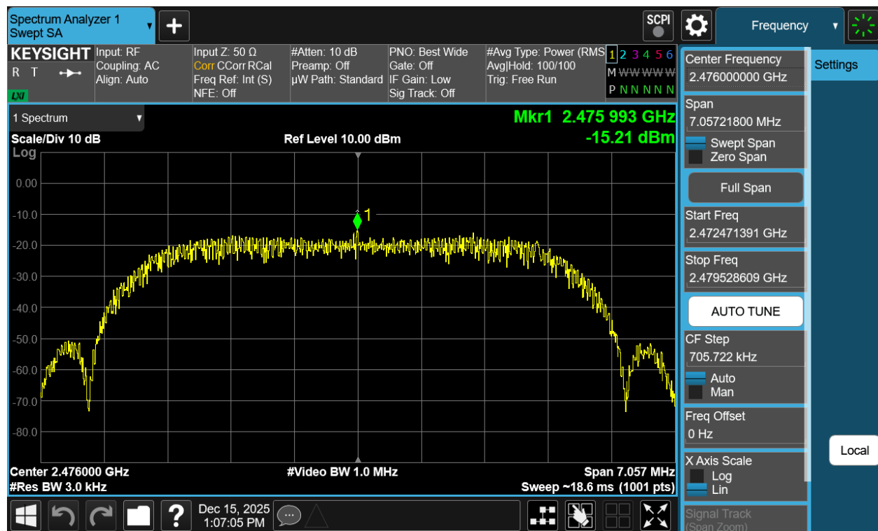
Plot 7-138. Power Spectral Density Plot Antenna WF2b (Bluetooth (HDRPM16), 16Mbps, iPA – Ch. 73)
