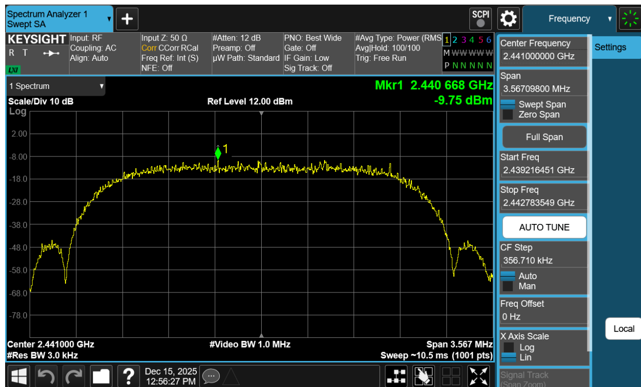
Plot 7-125. Power Spectral Density Plot Antenna WF2b (Bluetooth (HDRPS2), 2Mbps, iPA – Ch. 38)
