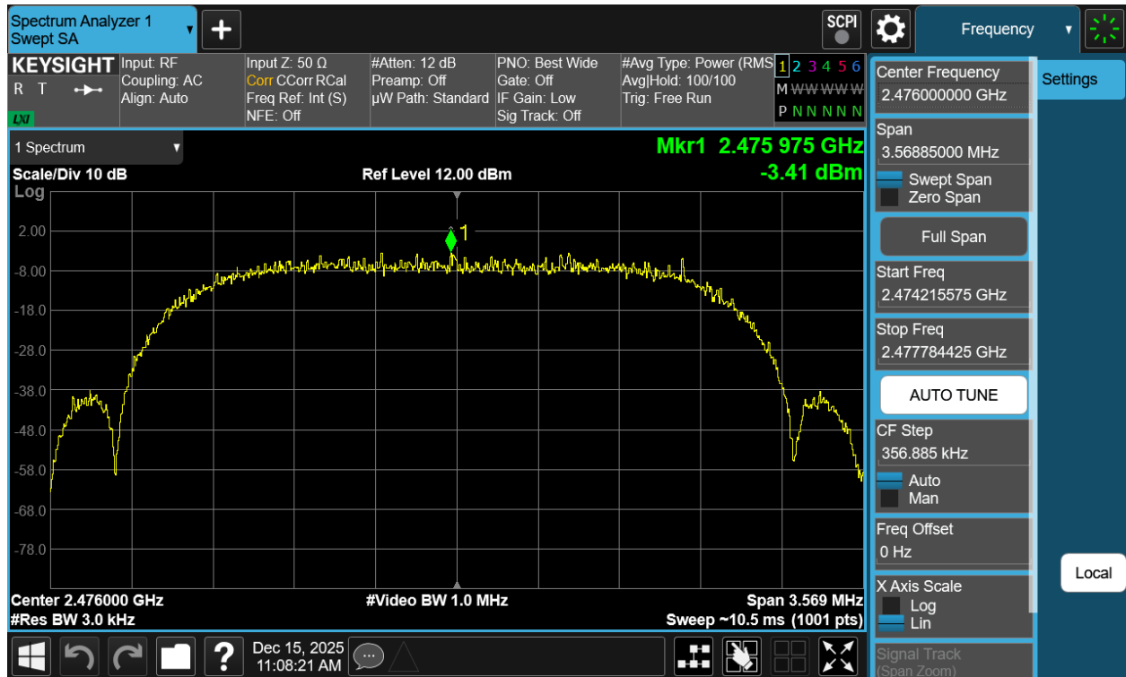
Plot 7-173. Power Spectral Density Plot Tx BF Antenna WF7b (Bluetooth (HDRPS2), 8Mbps, ePA – Ch. 73)
