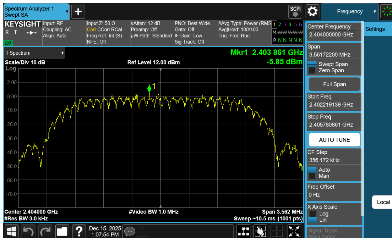
Plot 7-139. Power Spectral Density Plot Antenna WF2b (Bluetooth (HDT2), 2Mbps, ePA – Ch. 1)
