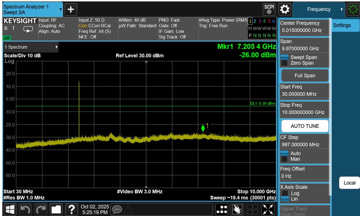
Plot 7-279. Conducted Spurious Plot Antenna WF2b (Bluetooth (HDRPS2), 8Mbps, ePA – Ch. 38)
