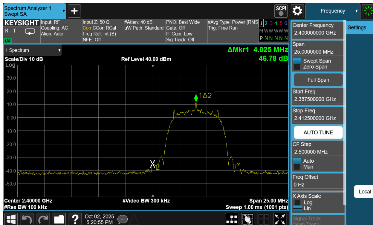
Plot 7-237. Band Edge Plot Antenna WF2b (Bluetooth (HDRPM16), 16Mbps, ePA – Ch. 1)
