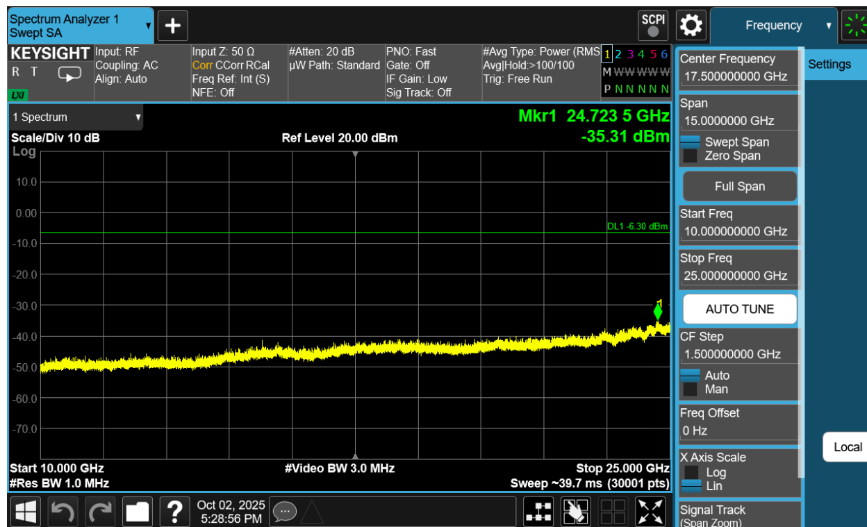
Plot 7-284. Conducted Spurious Plot Antenna WF2b (Bluetooth (XHDRPM6), 6Mbps, ePA – Ch. 1)
