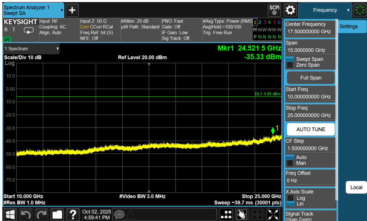
Plot 7-274. Conducted Spurious Plot Antenna WF2b (Bluetooth (HDR4), 4 Mbps, ePA – Ch. 38)
