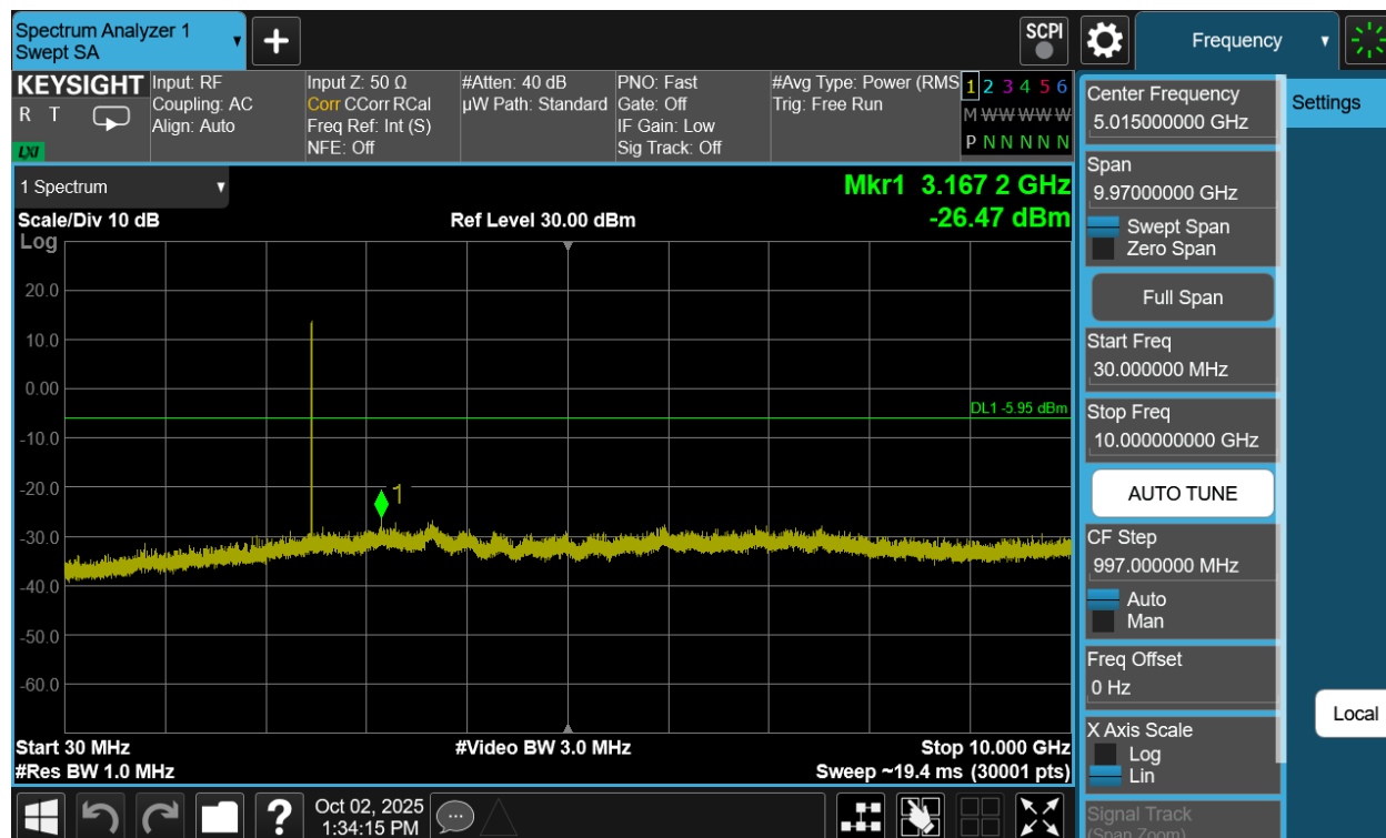
Plot 7-257. Conducted Spurious Plot Antenna WF7b (Bluetooth (XHDRPM6), 6Mbps, ePA – Ch. 73)
