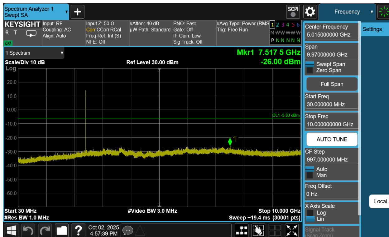
Plot 7-271. Conducted Spurious Plot Antenna WF2b (Bluetooth (HDR4), 4 Mbps, ePA – Ch. 1)
