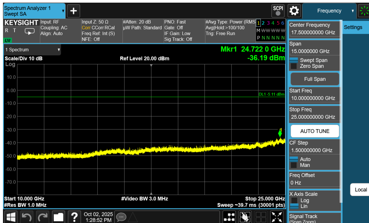
Plot 7-250. Conducted Spurious Plot Antenna WF7b (Bluetooth (HDRPS2), 8Mbps, ePA – Ch. 38)
