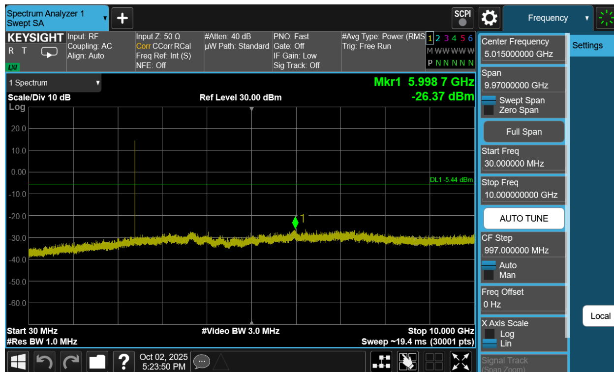
Plot 7-277. Conducted Spurious Plot Antenna WF2b (Bluetooth (HDRPS2), 8Mbps, ePA – Ch. 1)
