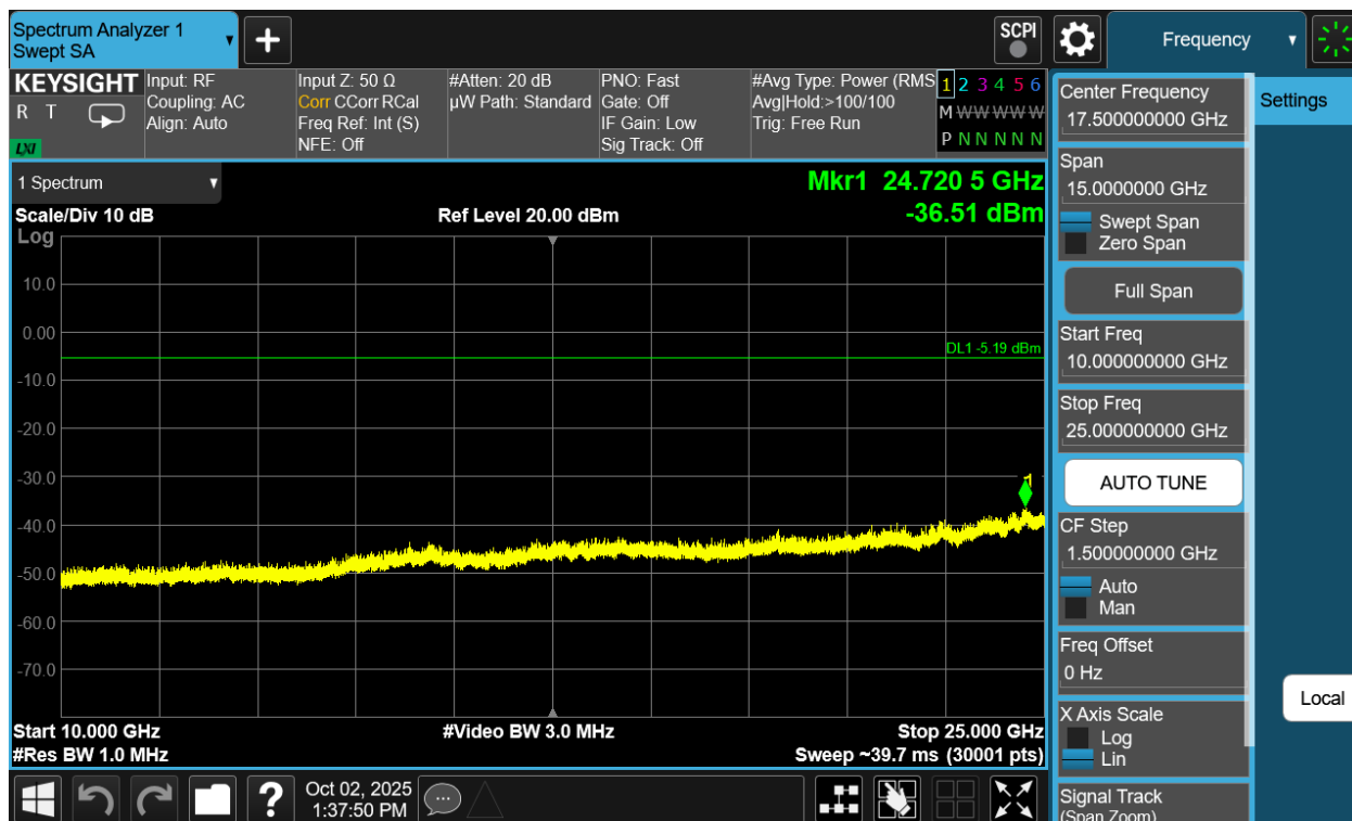
Plot 7-262. Conducted Spurious Plot Antenna WF7b (Bluetooth (HDRPM16), 16Mbps, ePA – Ch. 38)
