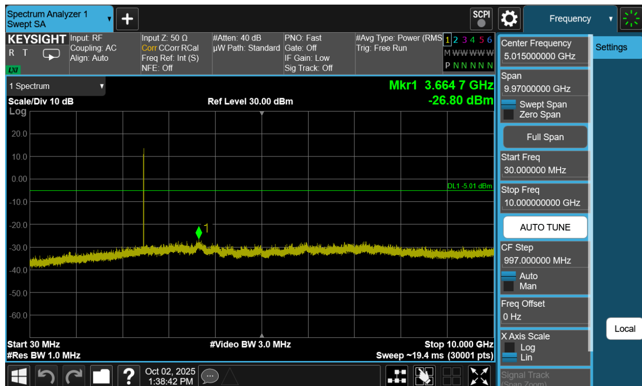
Plot 7-263. Conducted Spurious Plot Antenna WF7b (Bluetooth (HDRPM16), 16Mbps, ePA – Ch. 73)
