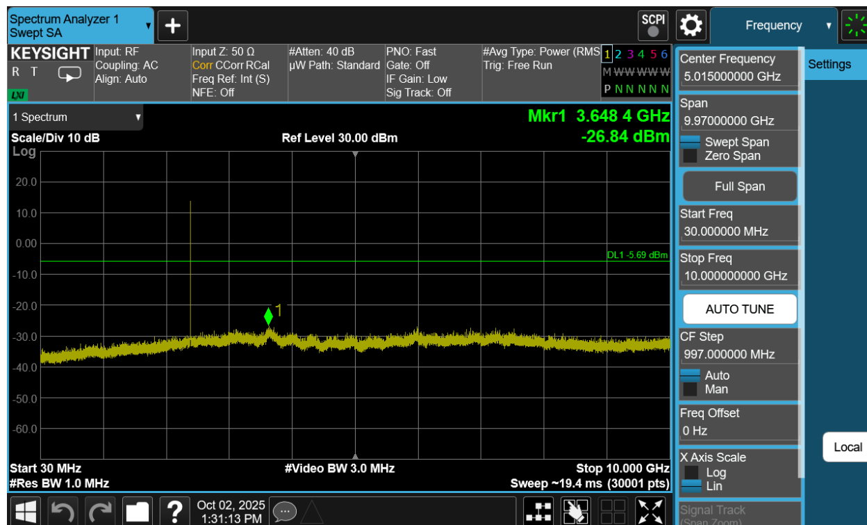
Plot 7-253. Conducted Spurious Plot Antenna WF7b (Bluetooth (XHDRPM6), 6Mbps, ePA – Ch. 1)
