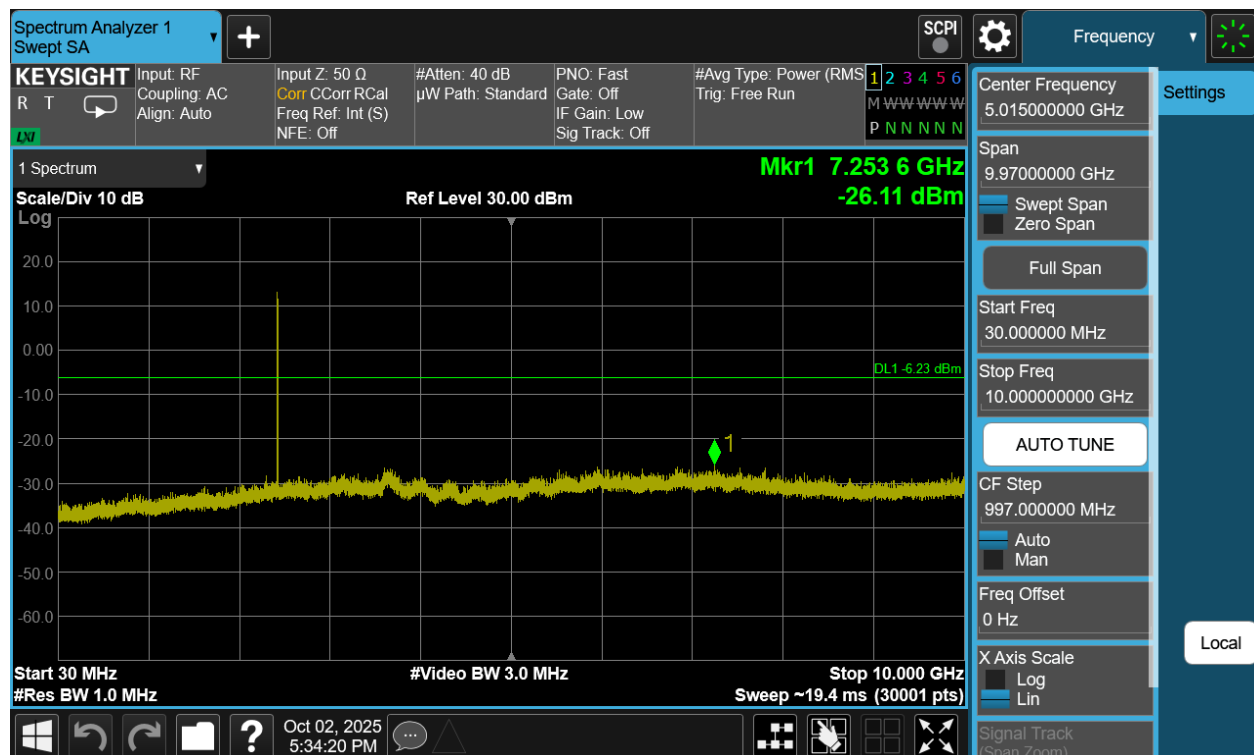
Plot 7-291. Conducted Spurious Plot Antenna WF2b (Bluetooth (HDRPM16), 16Mbps, ePA – Ch. 38)
