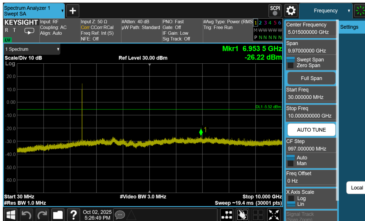
Plot 7-281. Conducted Spurious Plot Antenna WF2b (Bluetooth (HDRPS2), 8Mbps, ePA – Ch. 73)
