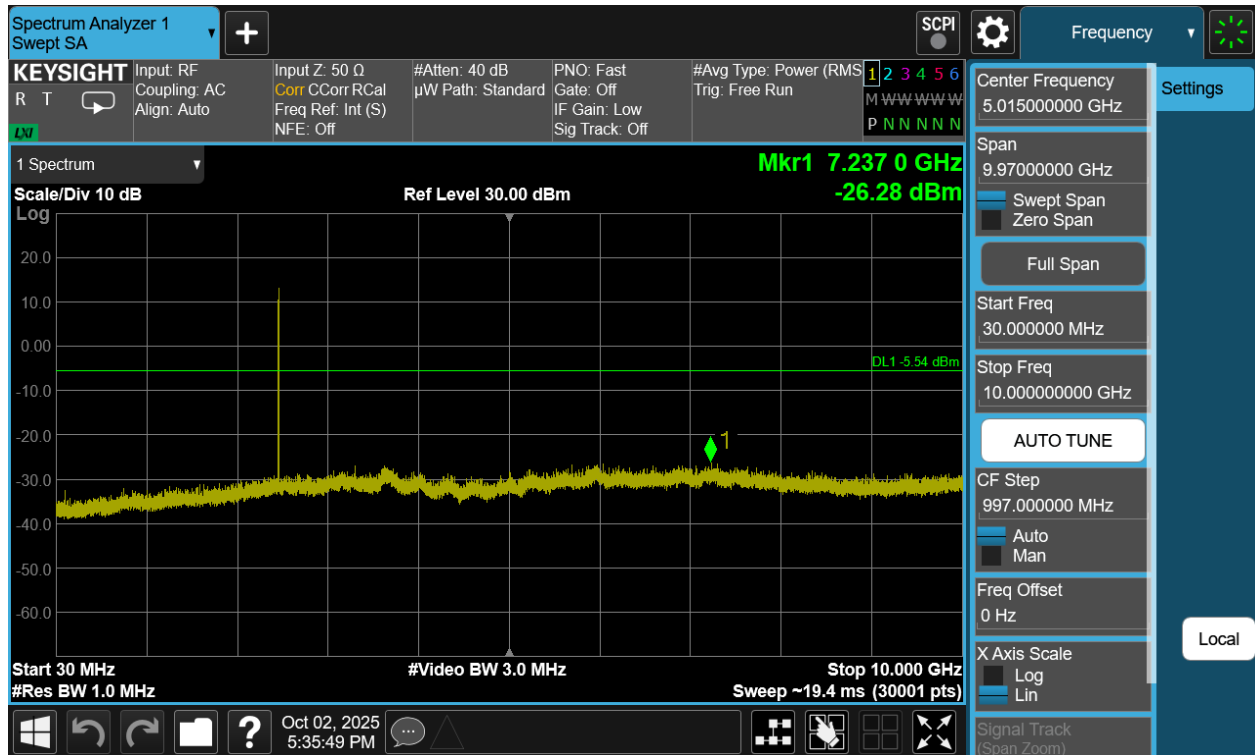
Plot 7-293. Conducted Spurious Plot Antenna WF2b (Bluetooth (HDRPM16), 16Mbps, ePA – Ch. 73)
