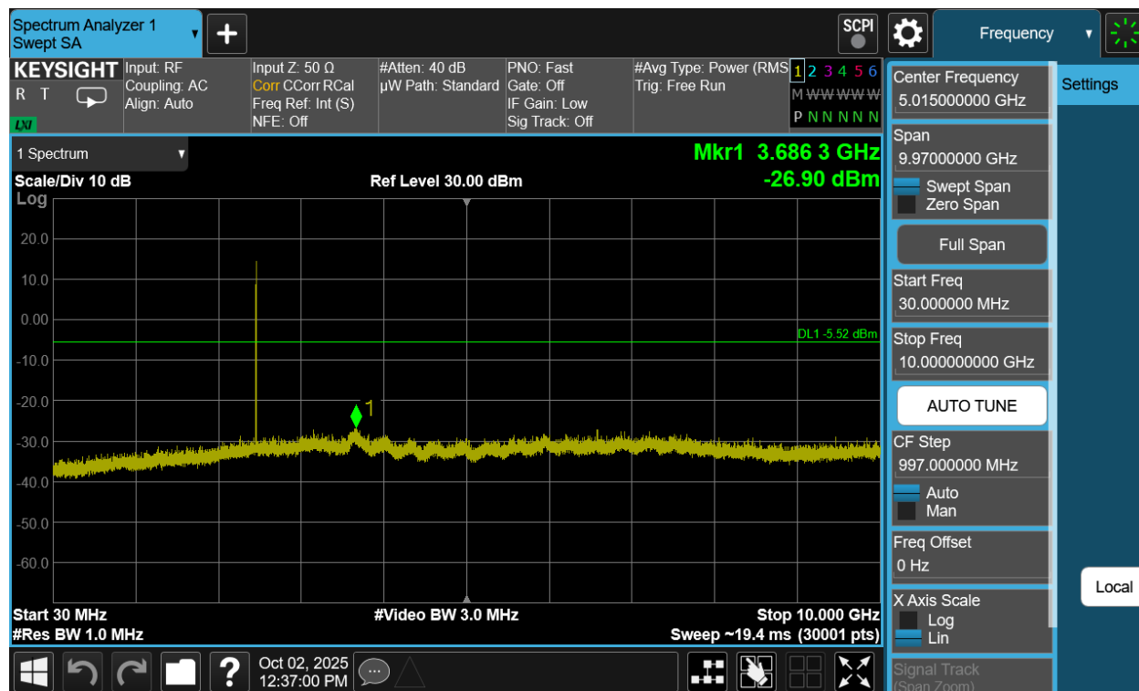
Plot 7-245. Conducted Spurious Plot Antenna WF7b (Bluetooth (HDR4), 4 Mbps, ePA – Ch. 73)
