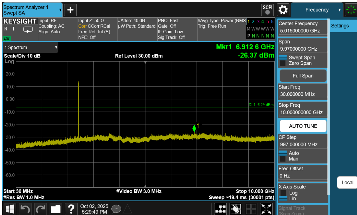
Plot 7-285. Conducted Spurious Plot Antenna WF2b (Bluetooth (XHDRPM6), 6Mbps, ePA – Ch. 38)
