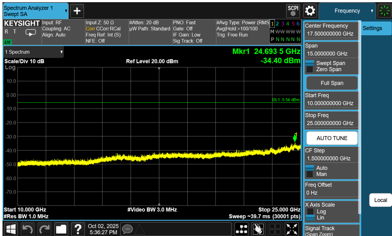
Plot 7-294. Conducted Spurious Plot Antenna WF2b (Bluetooth (HDRPM16), 16Mbps, ePA – Ch. 73)
