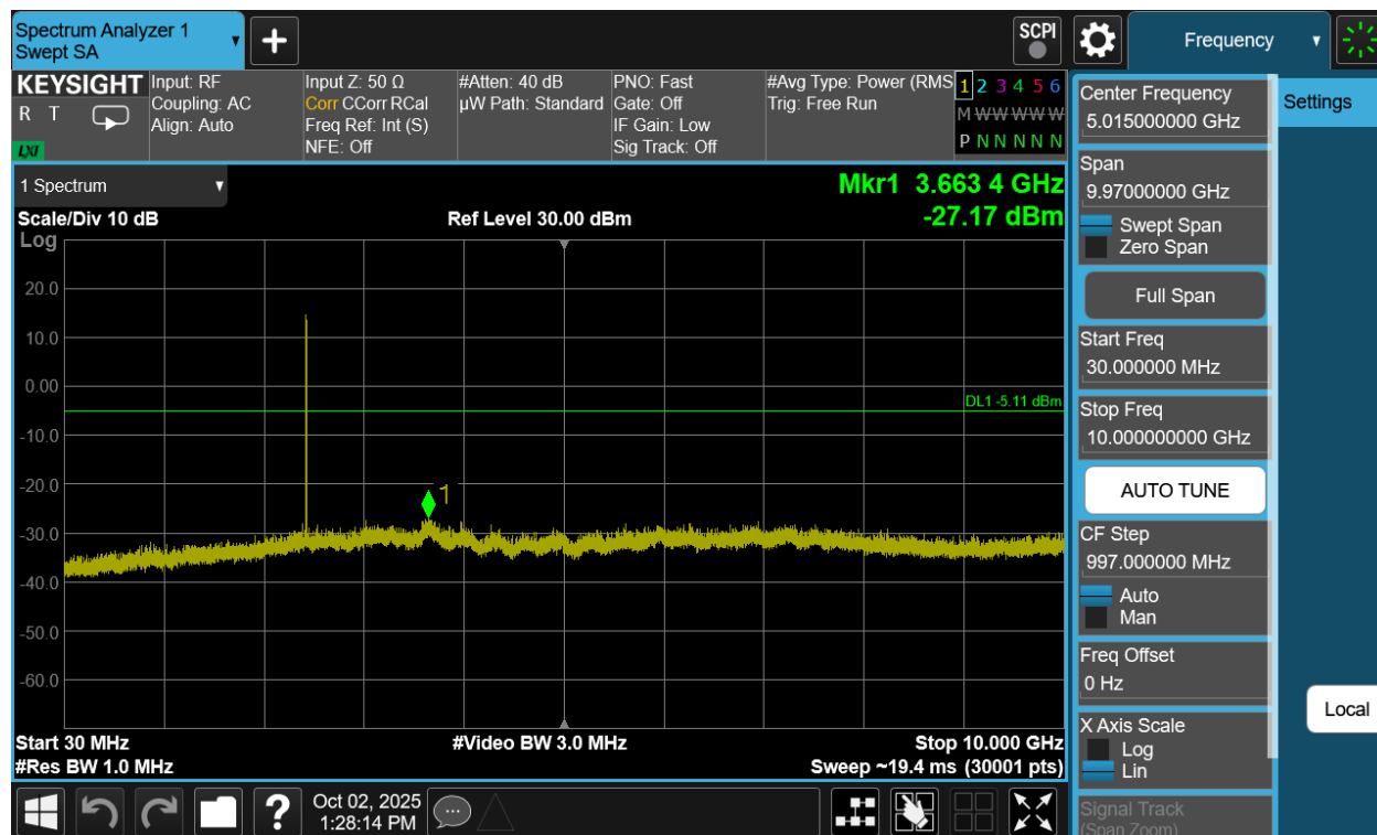
Plot 7-249. Conducted Spurious Plot Antenna WF7b (Bluetooth (HDRPS2), 8Mbps, ePA – Ch. 38)
