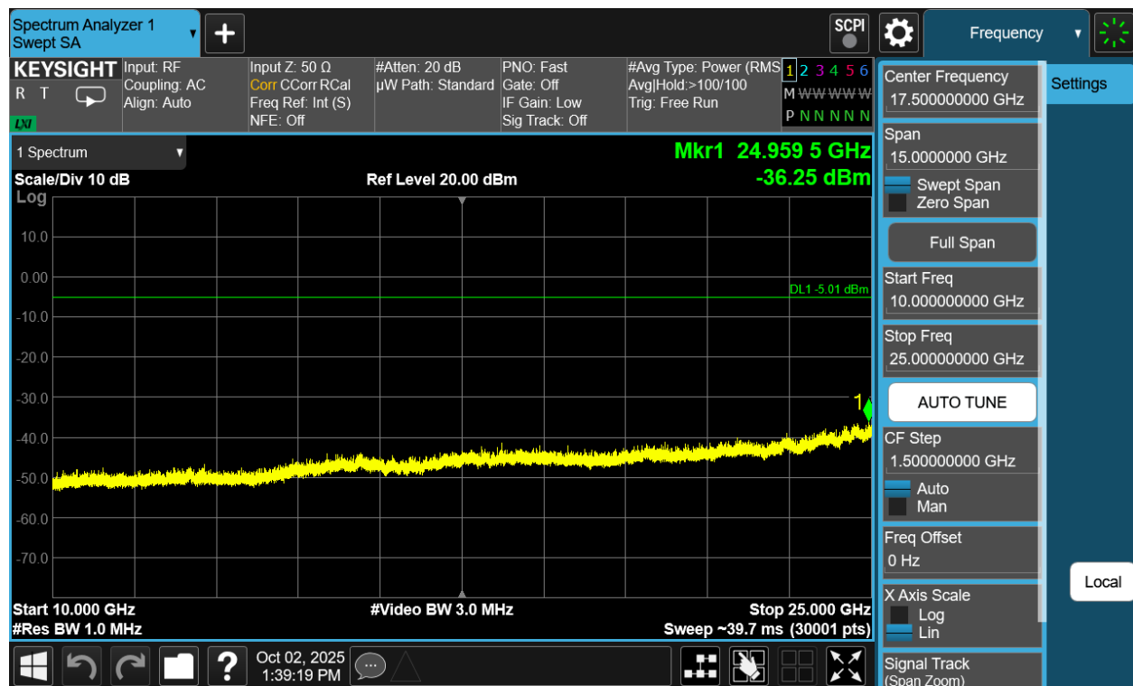
Plot 7-264. Conducted Spurious Plot Antenna WF7b (Bluetooth (HDRPM16), 16Mbps, ePA – Ch. 73)
