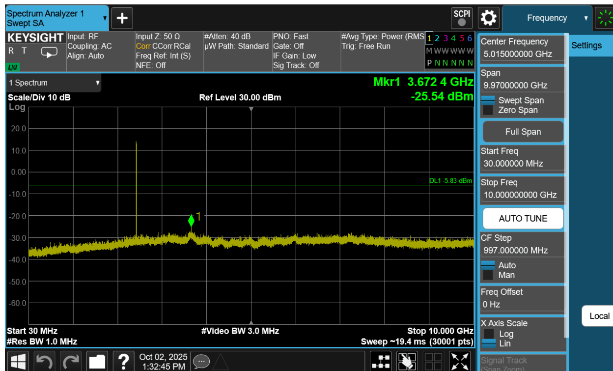
Plot 7-255. Conducted Spurious Plot Antenna WF7b (Bluetooth (XHDRPM6), 6Mbps, ePA – Ch. 38)
