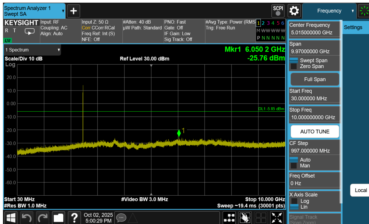
Plot 7-275. Conducted Spurious Plot Antenna WF2b (Bluetooth (HDR4), 4 Mbps, ePA – Ch. 73)
