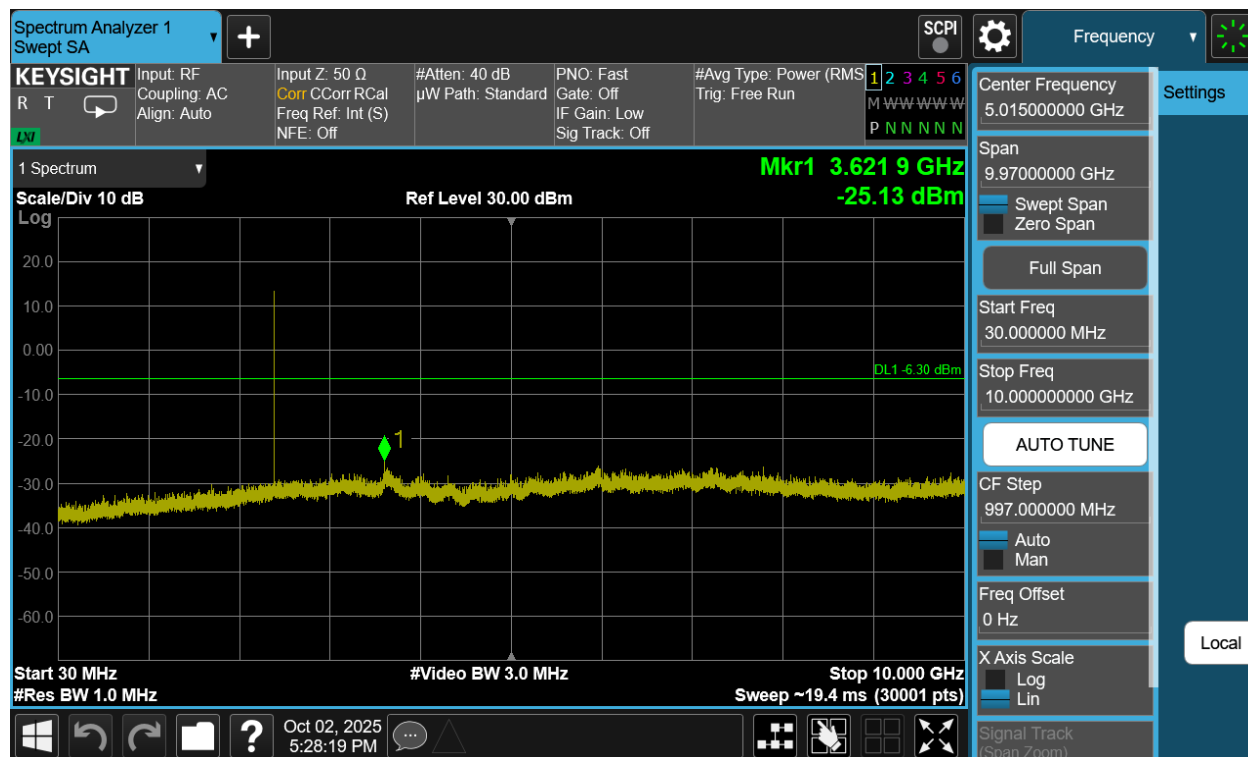
Plot 7-283. Conducted Spurious Plot Antenna WF2b (Bluetooth (XHDRPM6), 6Mbps, ePA – Ch. 1)
