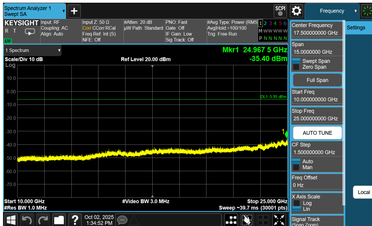
Plot 7-258. Conducted Spurious Plot Antenna WF7b (Bluetooth (XHDRPM6), 6Mbps, ePA – Ch. 73)
