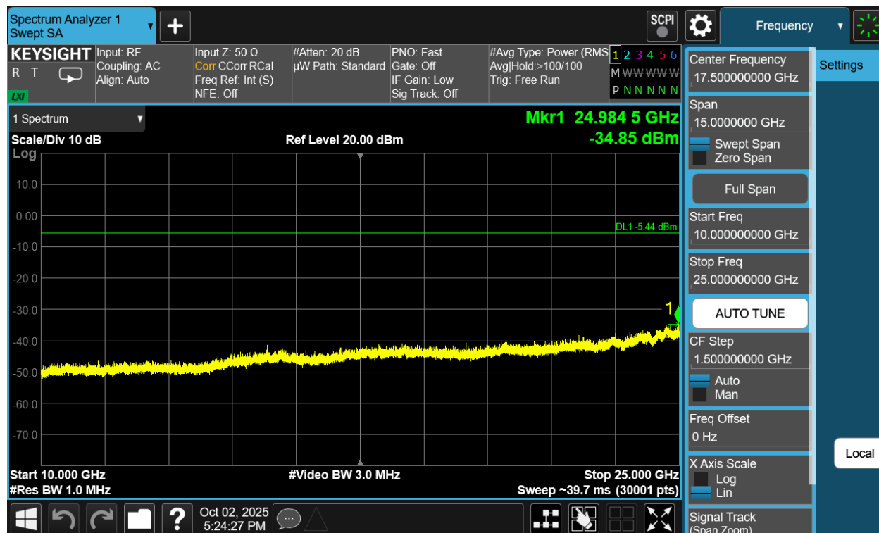
Plot 7-278. Conducted Spurious Plot Antenna WF2b (Bluetooth (HDRPS2), 8Mbps, ePA – Ch. 1)
