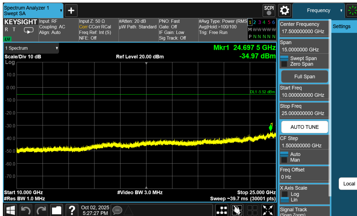
Plot 7-282. Conducted Spurious Plot Antenna WF2b (Bluetooth (HDRPS2), 8Mbps, ePA – Ch. 73)
