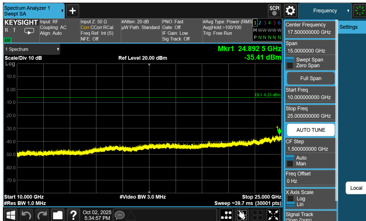
Plot 7-292. Conducted Spurious Plot Antenna WF2b (Bluetooth (HDRPM16), 16Mbps, ePA – Ch. 38)
