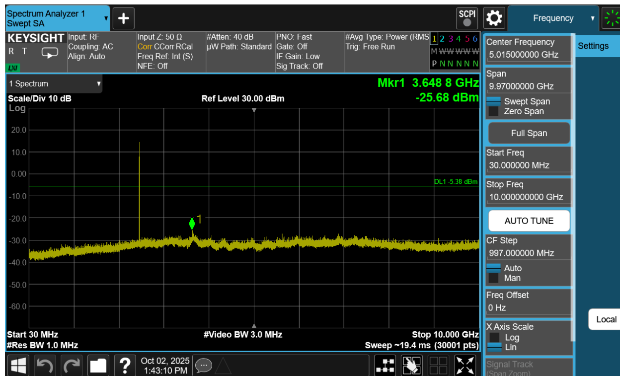
Plot 7-269. Conducted Spurious Plot Antenna WF7b (Bluetooth (HDT2), 2Mbps, ePA – Ch. 73)
