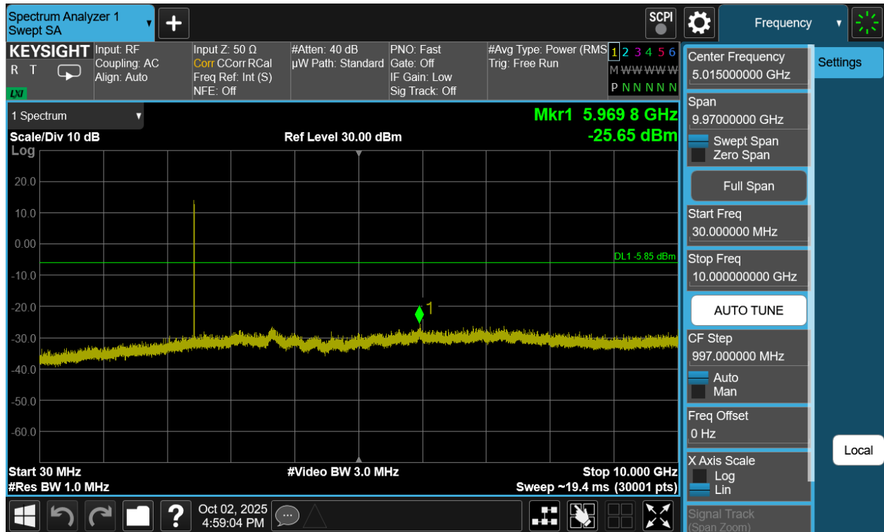
Plot 7-273. Conducted Spurious Plot Antenna WF2b (Bluetooth (HDR4), 4 Mbps, ePA – Ch. 38)
