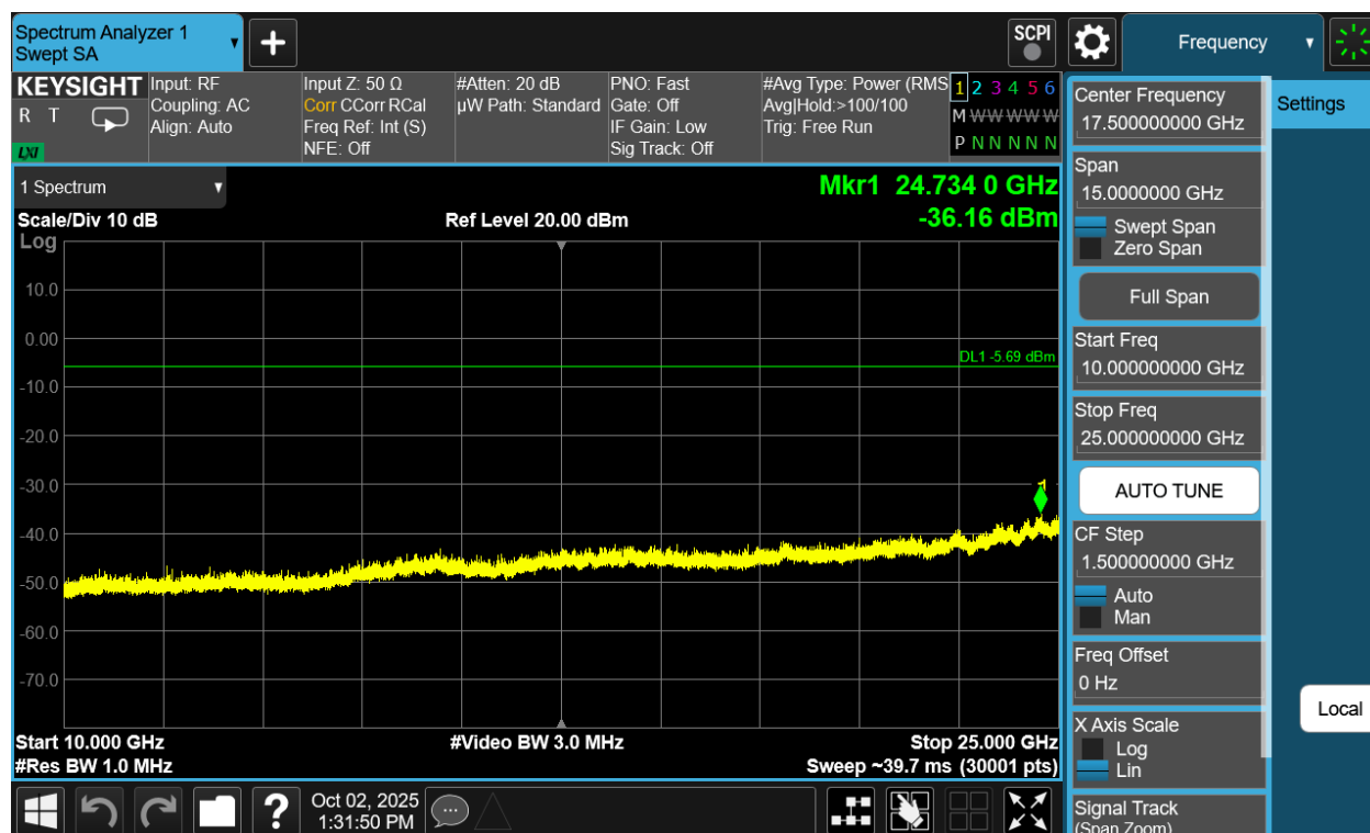
Plot 7-254. Conducted Spurious Plot Antenna WF7b (Bluetooth (XHDRPM6), 6Mbps, ePA – Ch. 1)
