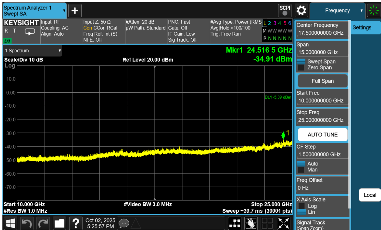
Plot 7-280. Conducted Spurious Plot Antenna WF2b (Bluetooth (HDRPS2), 8Mbps, ePA – Ch. 38)
