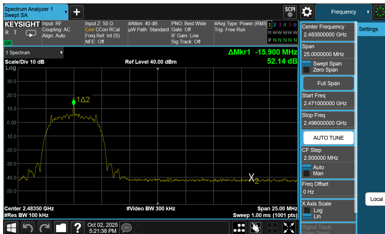
Plot 7-238. Band Edge Plot Antenna WF2b (Bluetooth (HDRPM16), 16Mbps, ePA – Ch. 73)
