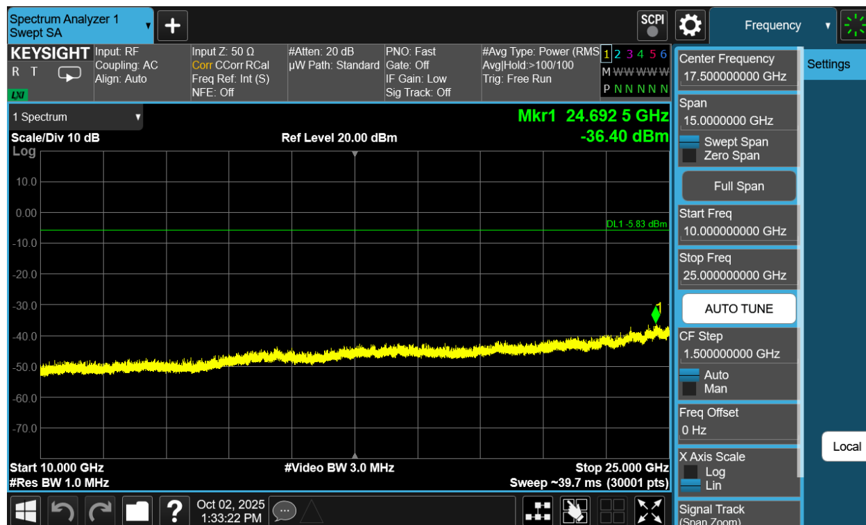
Plot 7-256. Conducted Spurious Plot Antenna WF7b (Bluetooth (XHDRPM6), 6Mbps, ePA – Ch. 38)
