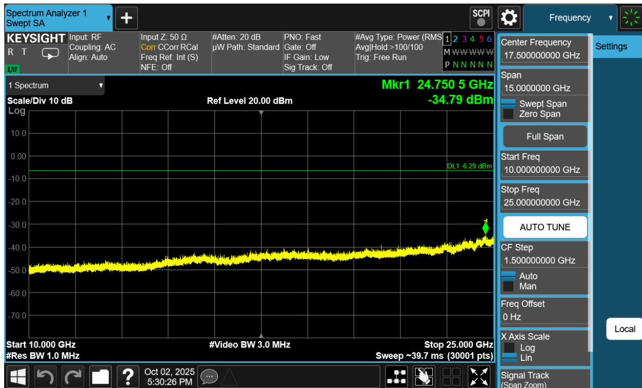
Plot 7-286. Conducted Spurious Plot Antenna WF2b (Bluetooth (XHDRPM6), 6Mbps, ePA – Ch. 38)
