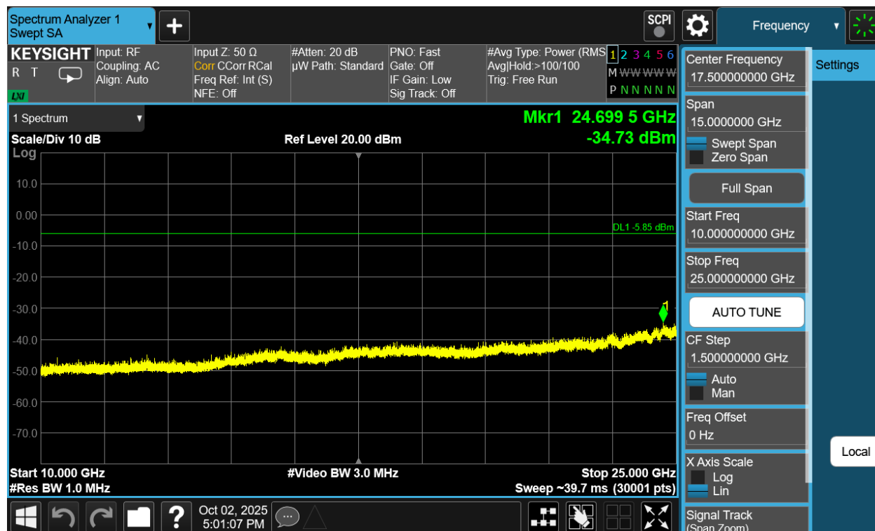
Plot 7-276. Conducted Spurious Plot Antenna WF2b (Bluetooth (HDR4), 4 Mbps, ePA – Ch. 73)
