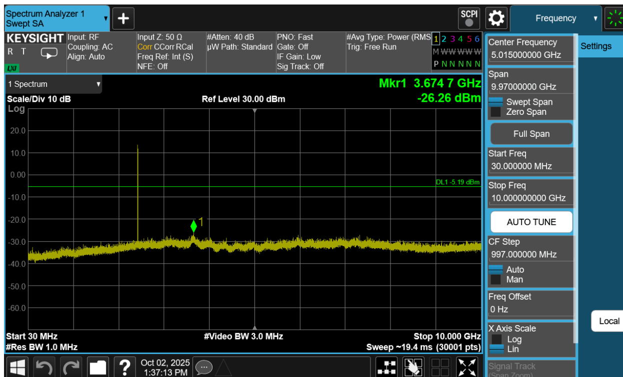
Plot 7-261. Conducted Spurious Plot Antenna WF7b (Bluetooth (HDRPM16), 16Mbps, ePA – Ch. 38)
