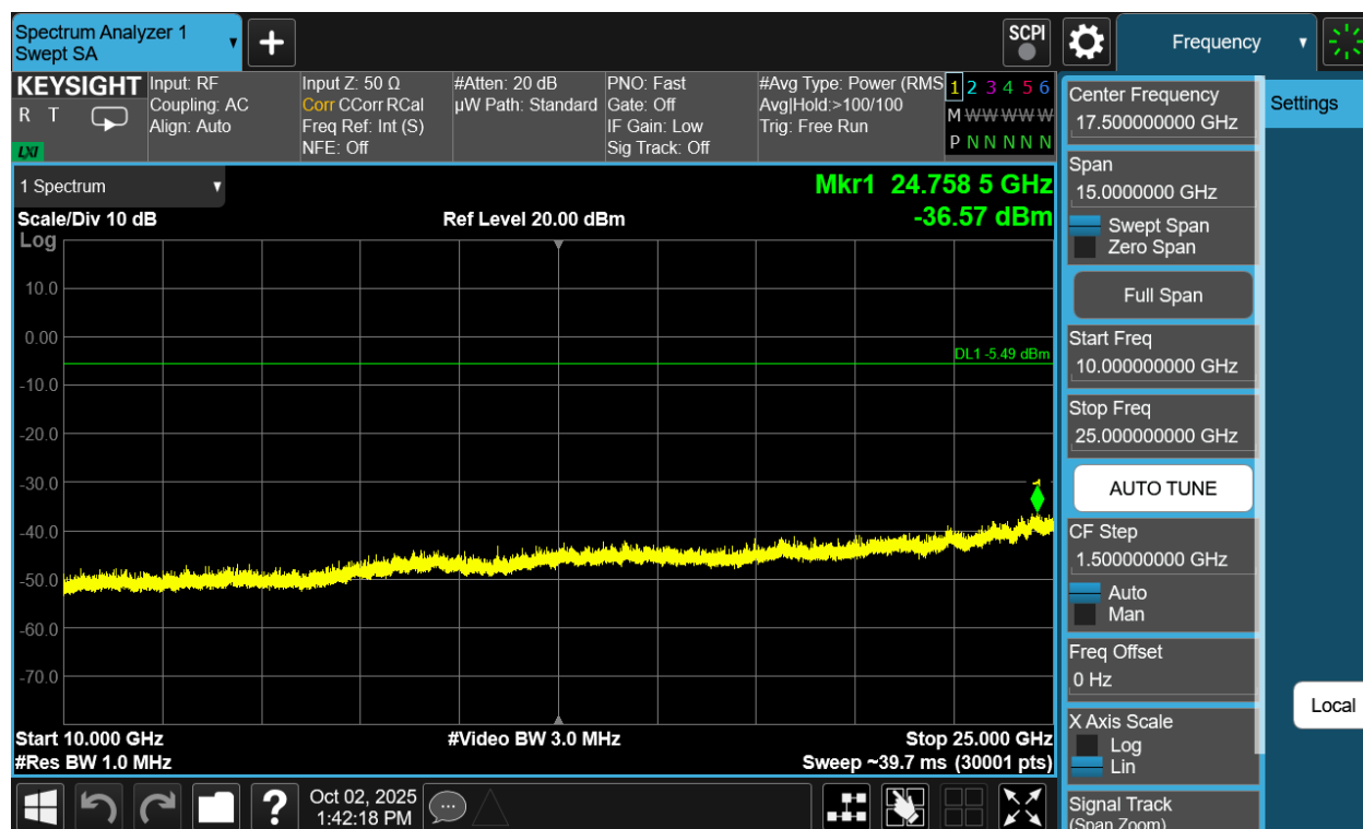
Plot 7-268. Conducted Spurious Plot Antenna WF7b (Bluetooth (HDT2), 2Mbps, ePA – Ch. 37)
