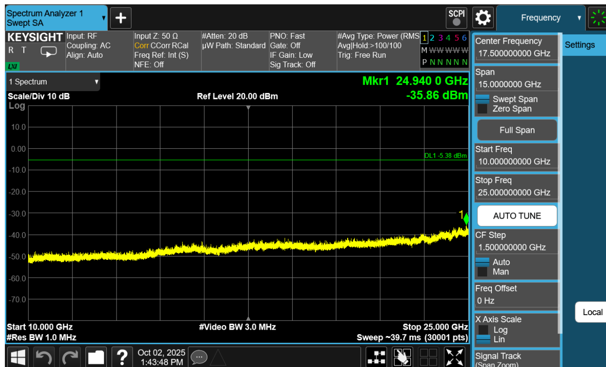
Plot 7-270. Conducted Spurious Plot Antenna WF7b (Bluetooth (HDT2), 2Mbps, ePA – Ch. 73)
