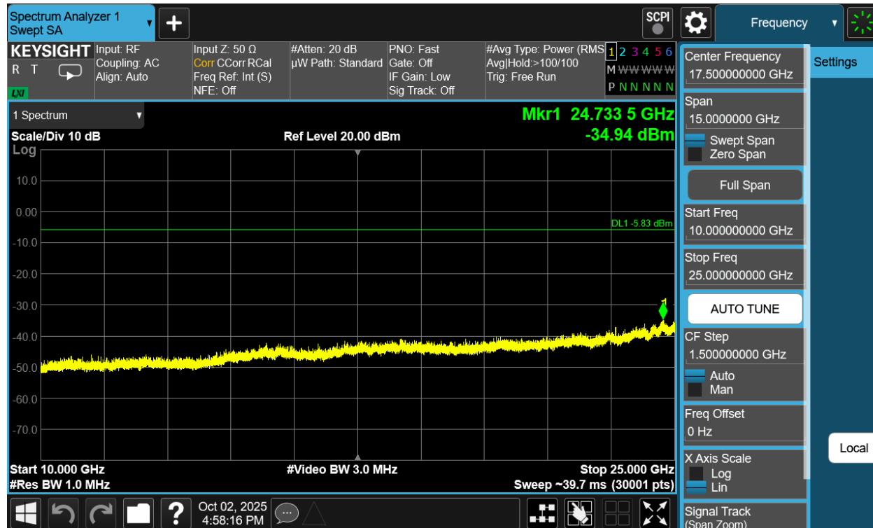
Plot 7-272. Conducted Spurious Plot Antenna WF2b (Bluetooth (HDR4), 4 Mbps, ePA – Ch. 1)
