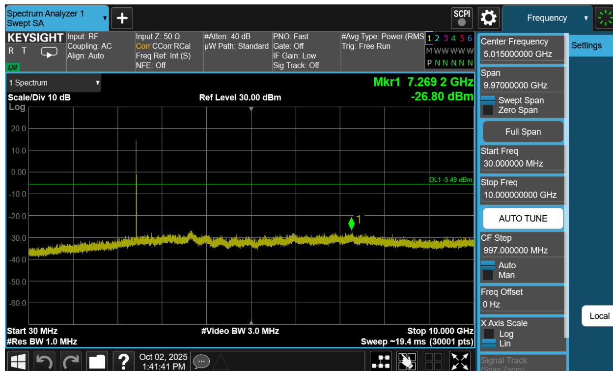
Plot 7-267. Conducted Spurious Plot Antenna WF7b (Bluetooth (HDT2), 2Mbps, ePA – Ch. 37)
