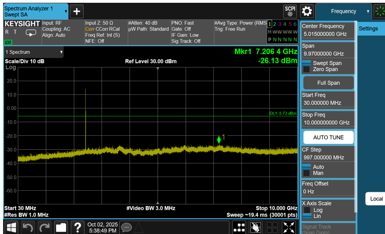
Plot 7-297. Conducted Spurious Plot Antenna WF2b (Bluetooth (HDT2), 2Mbps, ePA – Ch. 37)
