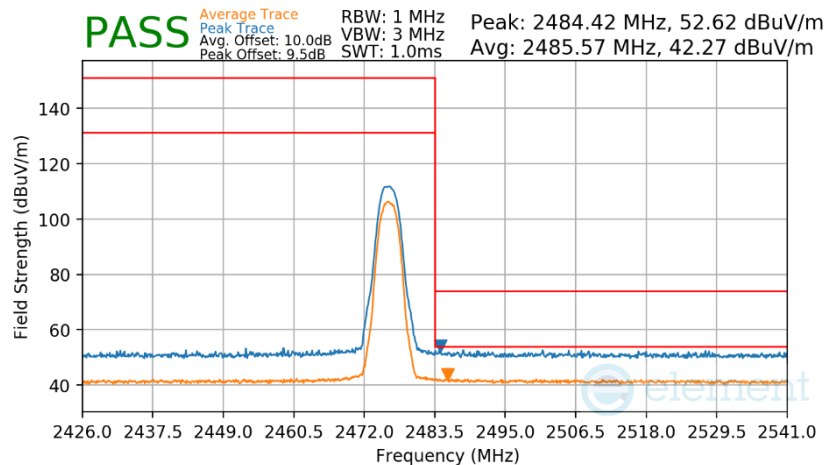
Plot 7-316. Radiated Restricted Upper Band Edge Measurement Antenna WF7b
