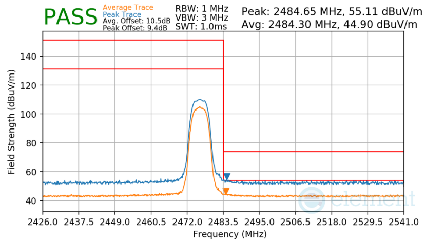
Plot 7-324. Radiated Restricted Upper Band Edge Measurement Antenna WF2b
