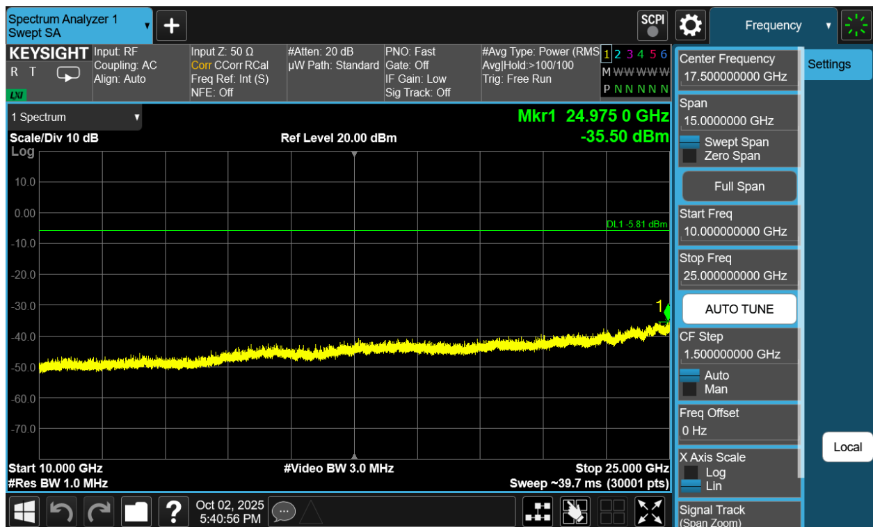
Plot 7-300. Conducted Spurious Plot Antenna WF2b (Bluetooth (HDT2), 2Mbps, ePA – Ch. 73)
