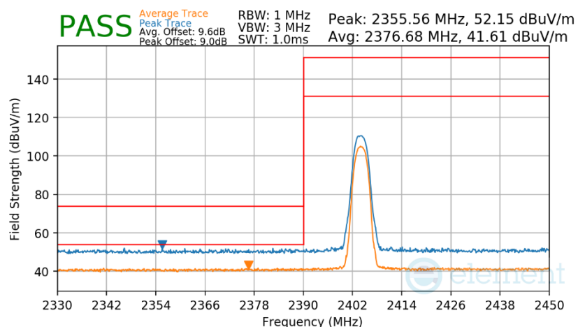
Plot 7-322. Radiated Restricted Lower Band Edge Measurement Antenna WF2b
