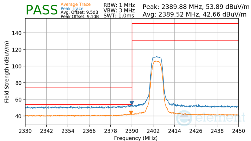
Plot 7-308. Radiated Restricted Lower Band Edge Measurement Antenna WF7b
