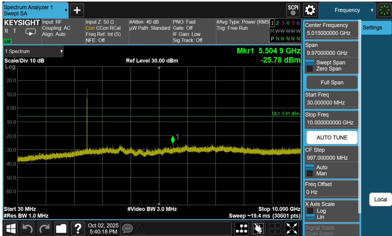
Plot 7-299. Conducted Spurious Plot Antenna WF2b (Bluetooth (HDT2), 2Mbps, ePA – Ch. 73)
