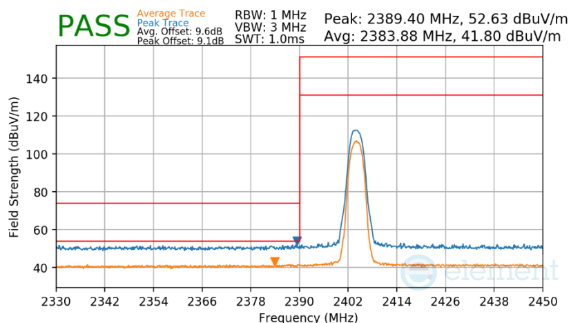
Plot 7-310. Radiated Restricted Lower Band Edge Measurement Antenna WF7b
