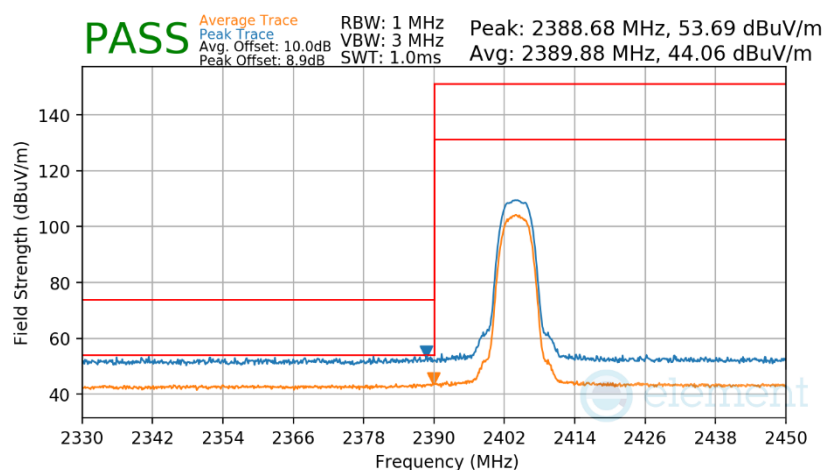
Plot 7-306. Radiated Restricted Lower Band Edge Measurement Antenna WF7b
