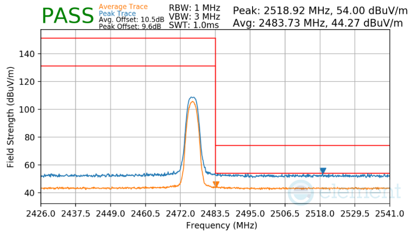
Plot 7-311. Radiated Restricted Upper Band Edge Measurement Antenna WF7b
