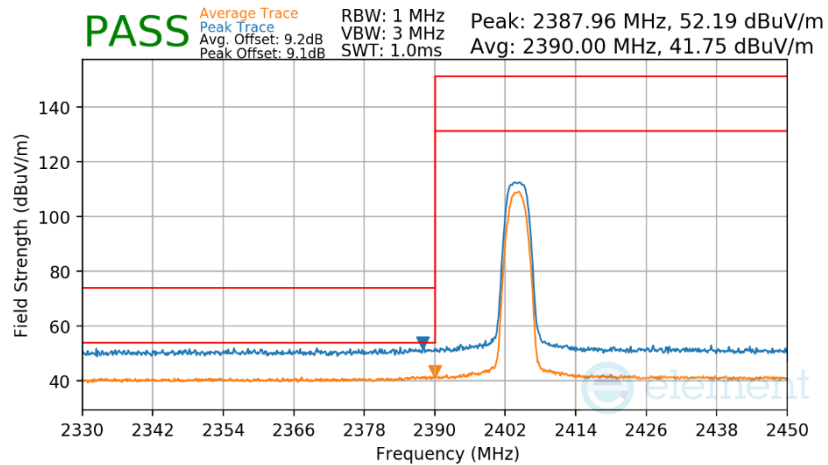
Plot 7-331. Radiated Restricted Lower Band Edge Measurement TxBF
