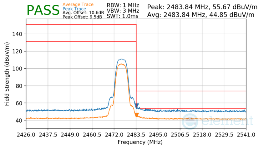
Plot 7-312. Radiated Restricted Upper Band Edge Measurement Antenna WF7b
