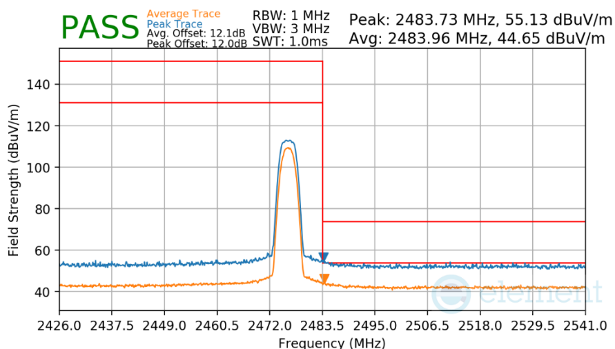
Plot 7-313. Radiated Restricted Upper Band Edge Measurement Antenna WF7b
