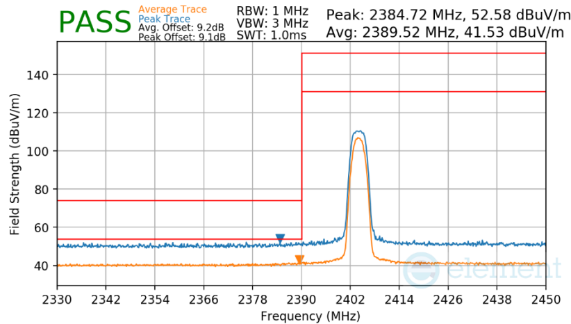
Plot 7-319. Radiated Restricted Lower Band Edge Measurement Antenna WF2b
