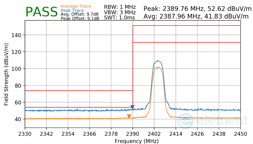
Plot 7-321. Radiated Restricted Lower Band Edge Measurement Antenna WF2b
