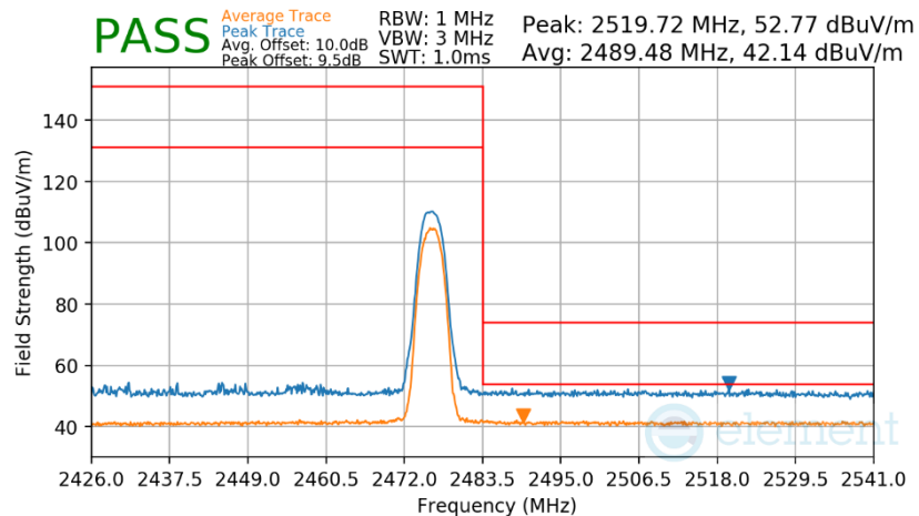
Plot 7-328. Radiated Restricted Upper Band Edge Measurement Antenna WF2b
