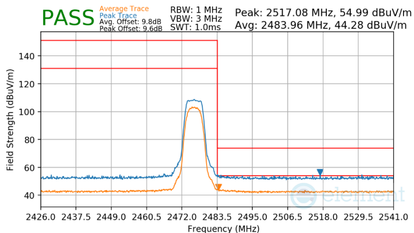
Plot 7-314. Radiated Restricted Upper Band Edge Measurement Antenna WF7b
