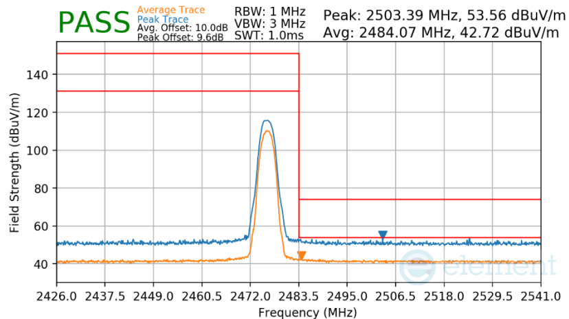
Plot 7-340. Radiated Restricted Upper Band Edge Measurement TxBF
