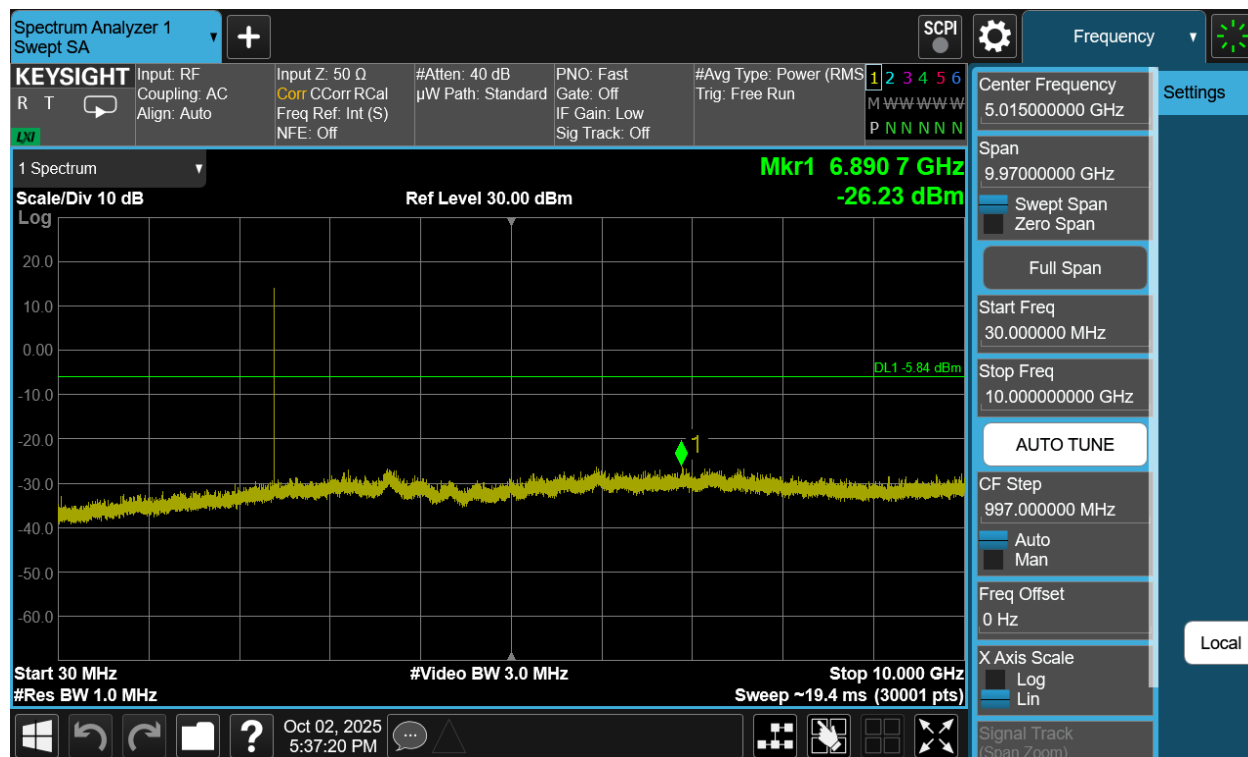
Plot 7-295. Conducted Spurious Plot Antenna WF2b (Bluetooth (HDT2), 2Mbps, ePA – Ch. 1)
