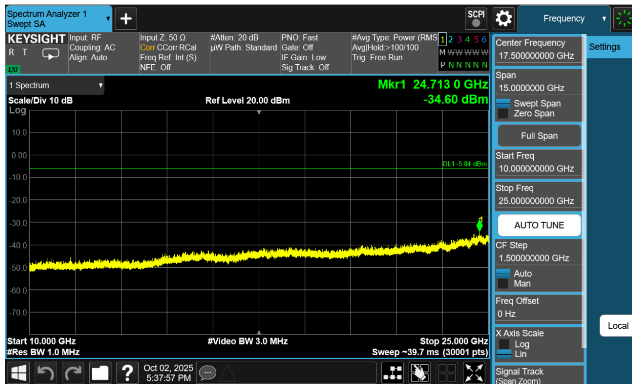
Plot 7-296. Conducted Spurious Plot Antenna WF2b (Bluetooth (HDT2), 2Mbps, ePA – Ch. 1)
