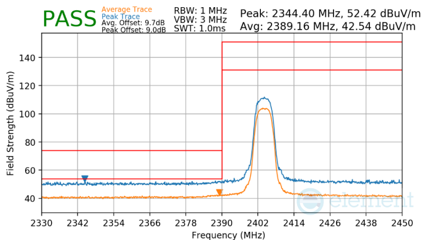
Plot 7-309. Radiated Restricted Lower Band Edge Measurement Antenna WF7b
