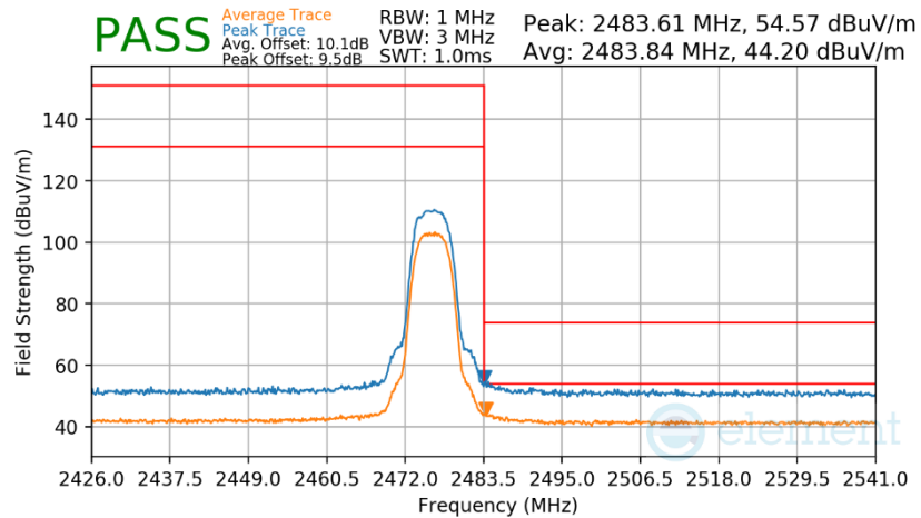
Plot 7-315. Radiated Restricted Upper Band Edge Measurement Antenna WF7b
