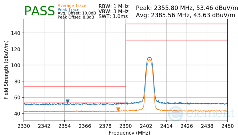
Plot 7-305. Radiated Restricted Lower Band Edge Measurement Antenna WF7b
