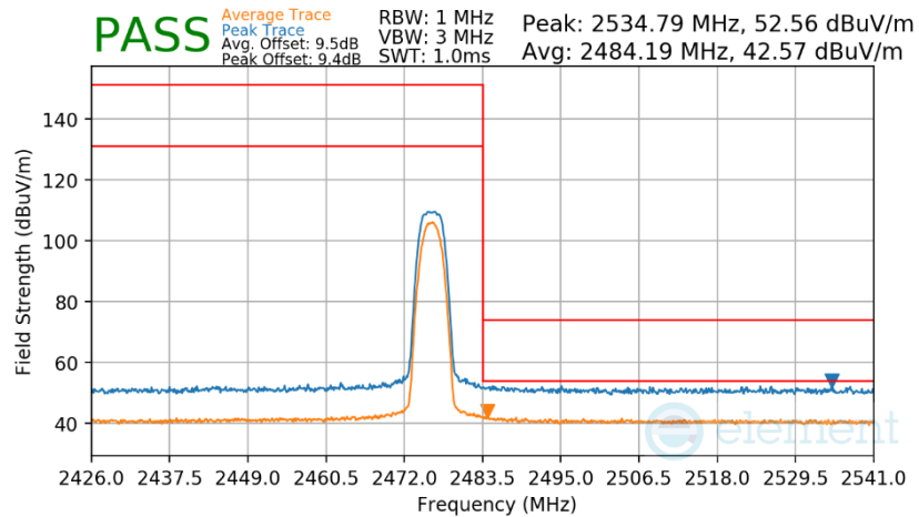
Plot 7-325. Radiated Restricted Upper Band Edge Measurement Antenna WF2b
