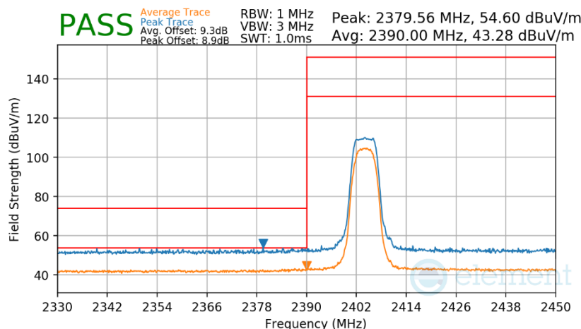
Plot 7-320. Radiated Restricted Lower Band Edge Measurement Antenna WF2b
