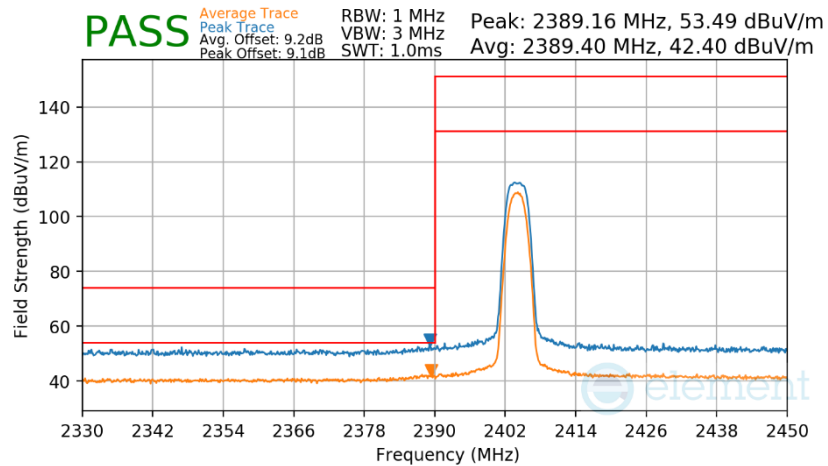
Plot 7-307. Radiated Restricted Lower Band Edge Measurement Antenna WF7b
