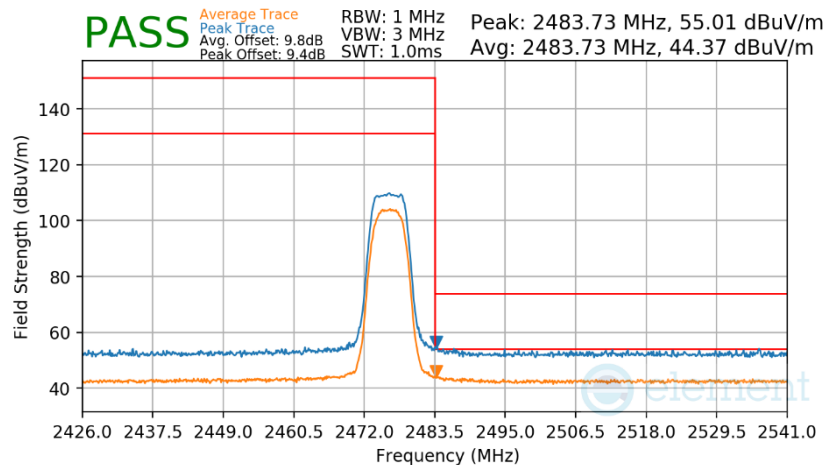
Plot 7-326. Radiated Restricted Upper Band Edge Measurement Antenna WF2b
