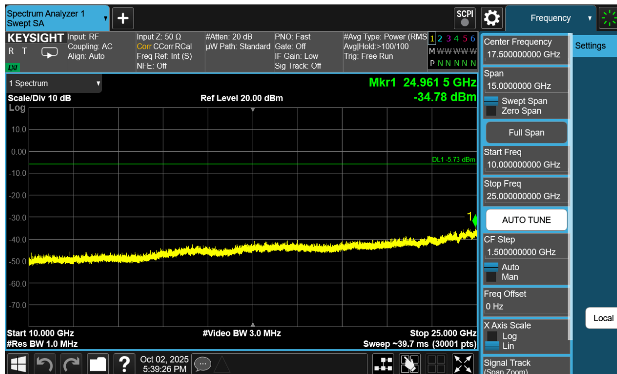
Plot 7-298. Conducted Spurious Plot Antenna WF2b (Bluetooth (HDT2), 2Mbps, ePA – Ch. 37)
