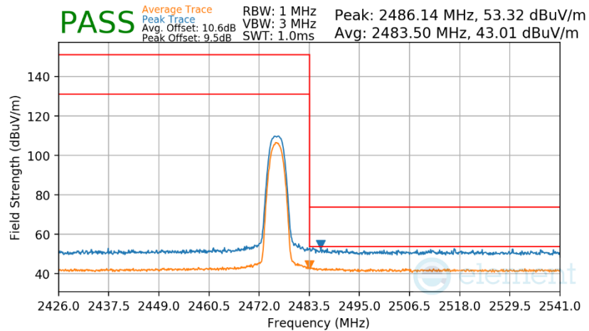
Plot 7-323. Radiated Restricted Upper Band Edge Measurement Antenna WF2b
