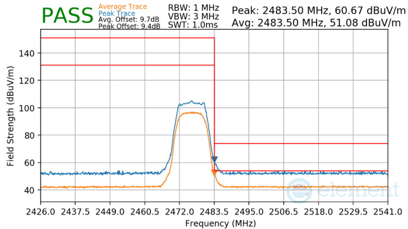
Plot 7-327. Radiated Restricted Upper Band Edge Measurement Antenna WF2b
