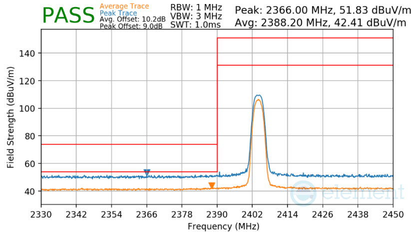
Plot 7-317. Radiated Restricted Lower Band Edge Measurement Antenna WF2b
