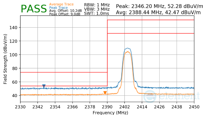
Plot 7-318. Radiated Restricted Lower Band Edge Measurement Antenna WF2b
