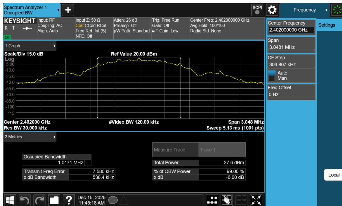
Plot 7-16. 99% OBW Plot Antenna WF2b (Bluetooth (LE), 500kbps, ePA – Ch. 0)
