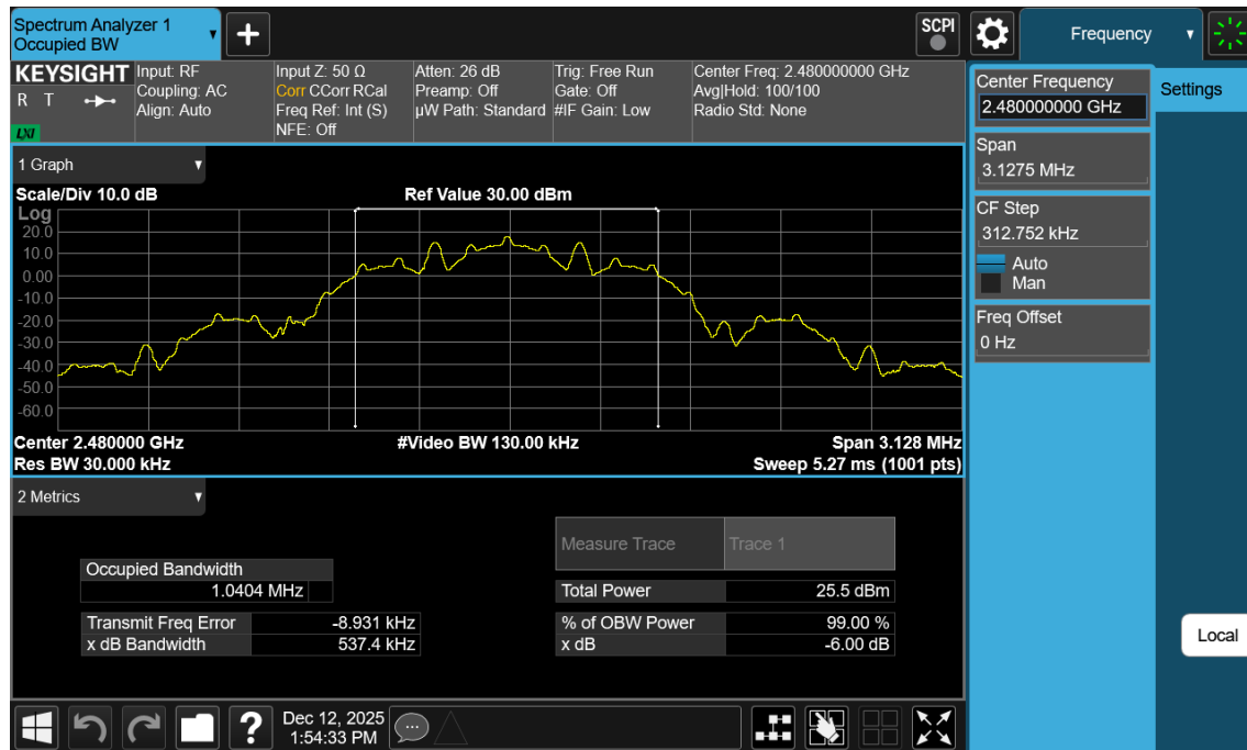
Plot 7-3. 99% OBW Plot Antenna WF7b (Bluetooth (LE), 125kbps, ePA – Ch. 39)
