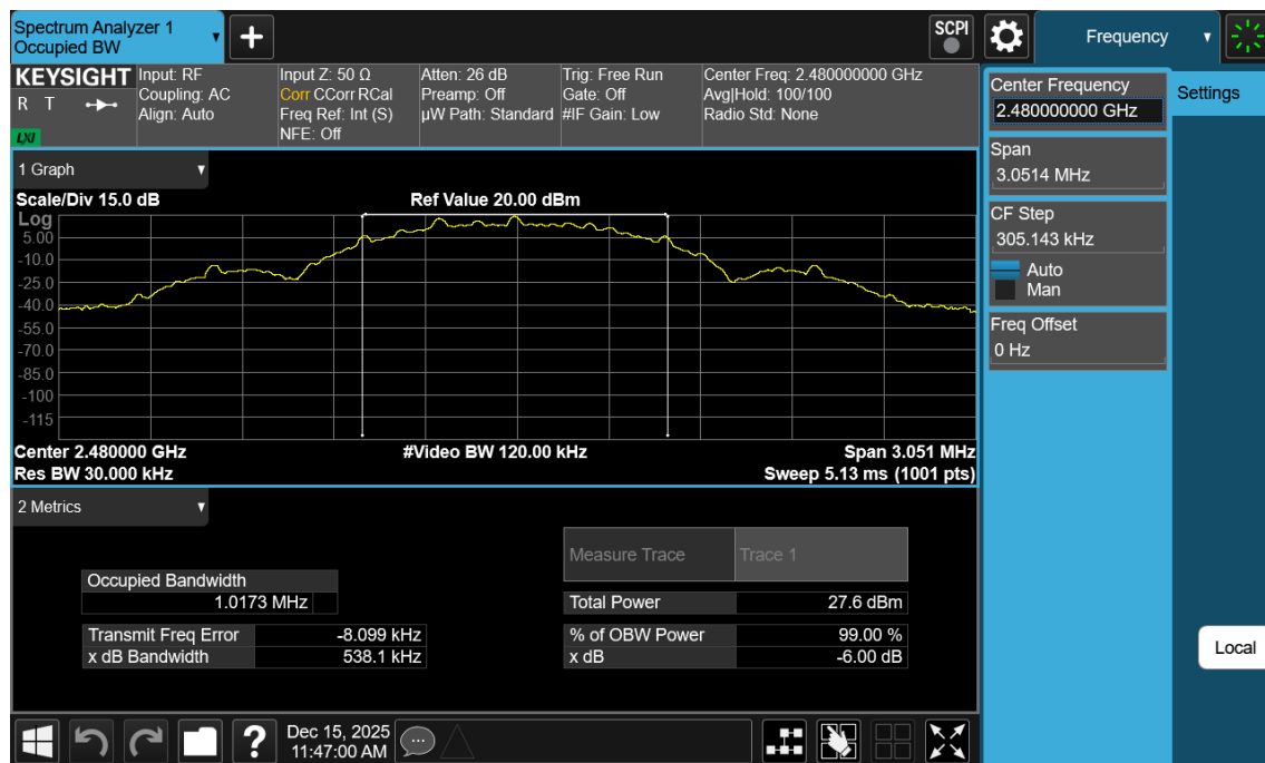
Plot 7-18. 99% OBW Plot Antenna WF2b (Bluetooth (LE), 500kbps, ePA – Ch. 39)
