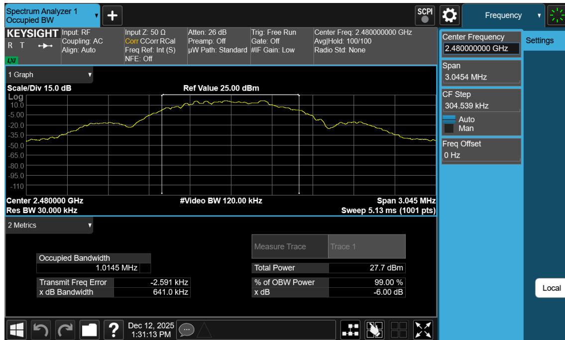
Plot 7-9. 99% OBW Plot Antenna WF7b (Bluetooth (LE), 1Mbps, ePA – Ch. 39)
