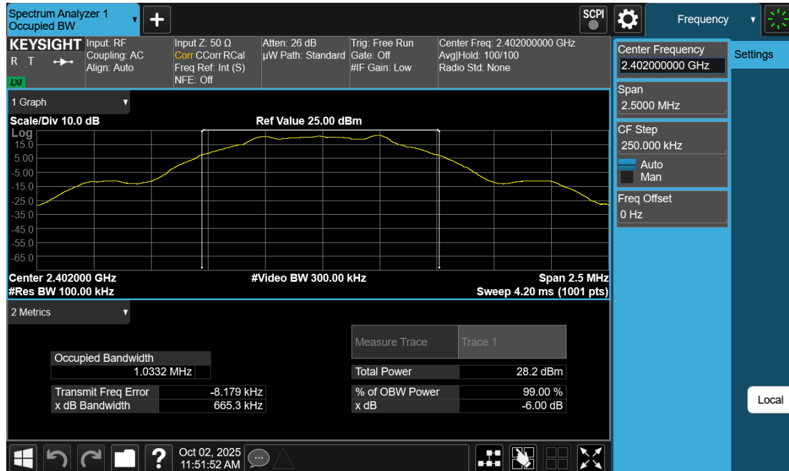
Plot 7-31. 6dB BW Plot Antenna WF7b (Bluetooth (LE), 1Mbps, ePA – Ch. 0)
