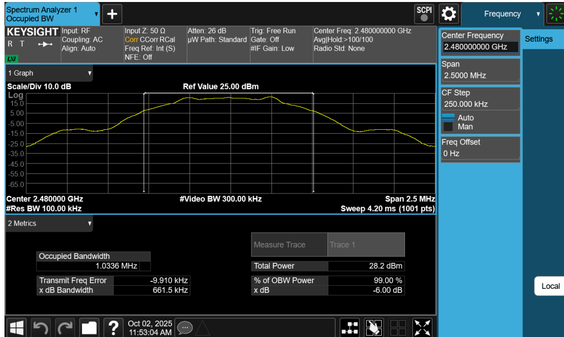
Plot 7-33. 6dB BW Plot Antenna WF7b (Bluetooth (LE), 1Mbps, ePA – Ch. 39)
