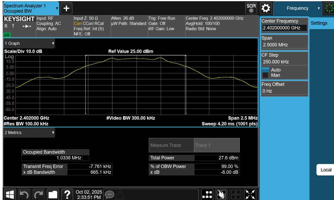
Plot 7-43. 6dB BW Plot Antenna WF2b (Bluetooth (LE), 1Mbps, ePA – Ch. 0)
