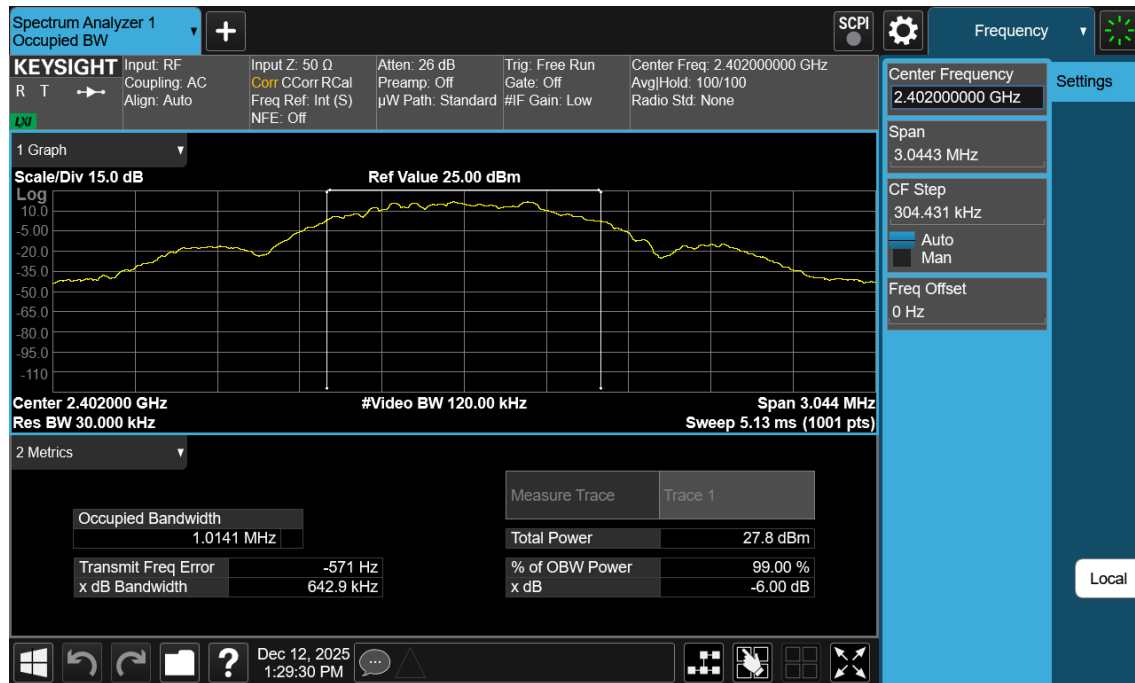
Plot 7-7. 99% OBW Plot Antenna WF7b (Bluetooth (LE), 1Mbps, ePA – Ch. 0)
