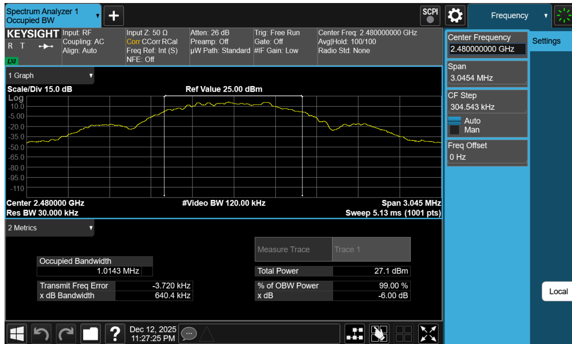
Plot 7-21. 99% OBW Plot Antenna WF2b (Bluetooth (LE), 1Mbps, ePA – Ch. 39)
