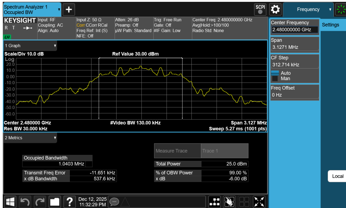
Plot 7-15. 99% OBW Plot Antenna WF2b (Bluetooth (LE), 125kbps, ePA – Ch. 39)
