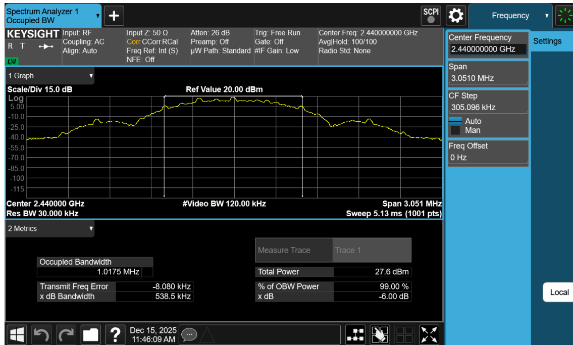
Plot 7-17. 99% OBW Plot Antenna WF2b (Bluetooth (LE), 500kbps, ePA – Ch. 19)
