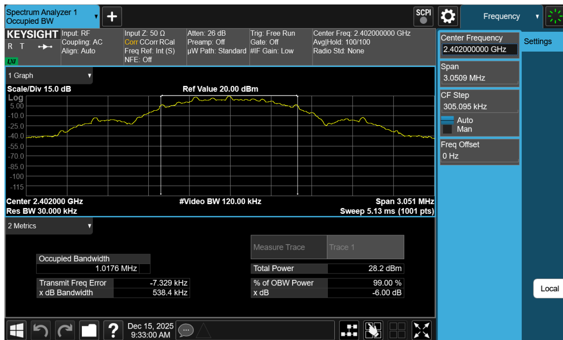
Plot 7-4. 99% OBW Plot Antenna WF7b (Bluetooth (LE), 500kbps, ePA – Ch. 0)
