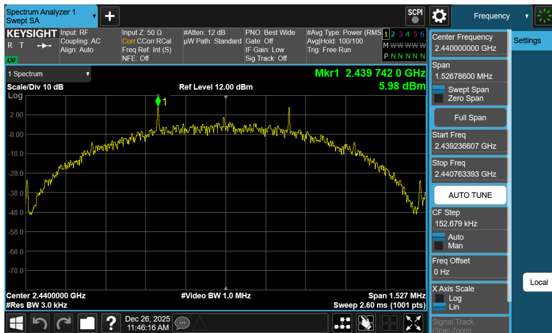
Plot 7-56. Power Spectral Density Plot Antenna WF7b (Bluetooth (LE), 500kbps, ePA – Ch. 19)
