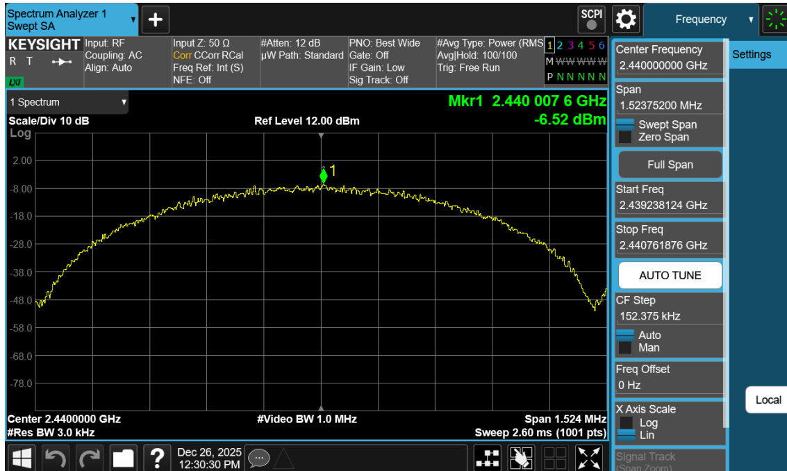
Plot 7-89. Power Spectral Density Plot Antenna WF2b (Bluetooth (LE), 1Mbps, iPA – Ch. 19)
