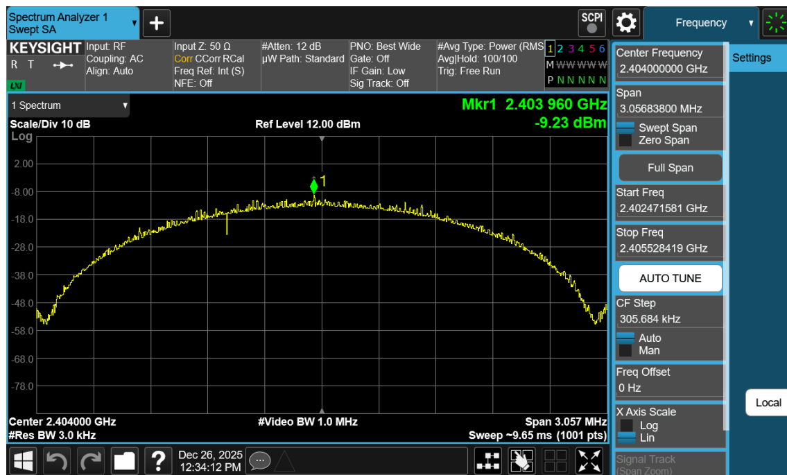
Plot 7-94. Power Spectral Density Plot Antenna WF2b (Bluetooth (LE), 2Mbps, iPA – Ch. 1)
