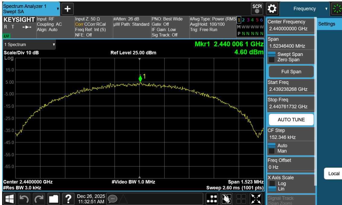
Plot 7-62. Power Spectral Density Plot Antenna WF7b (Bluetooth (LE), 1Mbps, ePA – Ch. 19)
