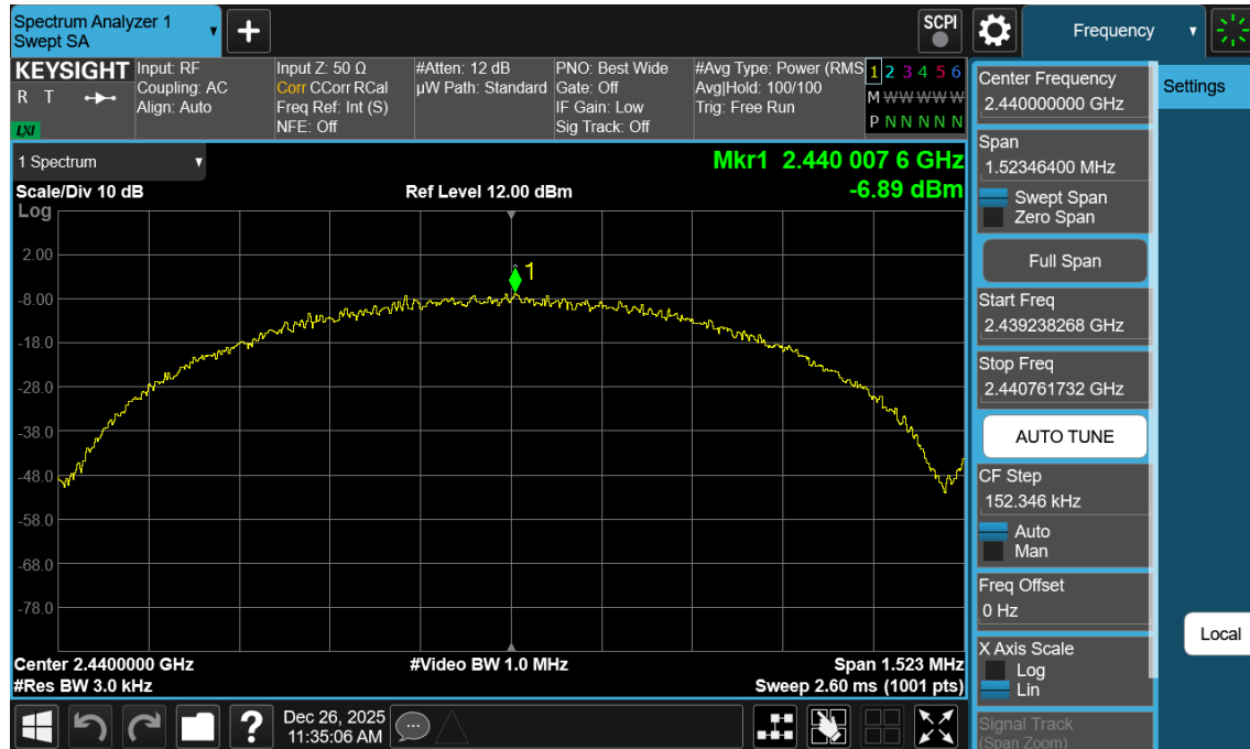
Plot 7-65. Power Spectral Density Plot Antenna WF7b (Bluetooth (LE), 1Mbps, iPA – Ch. 19)
