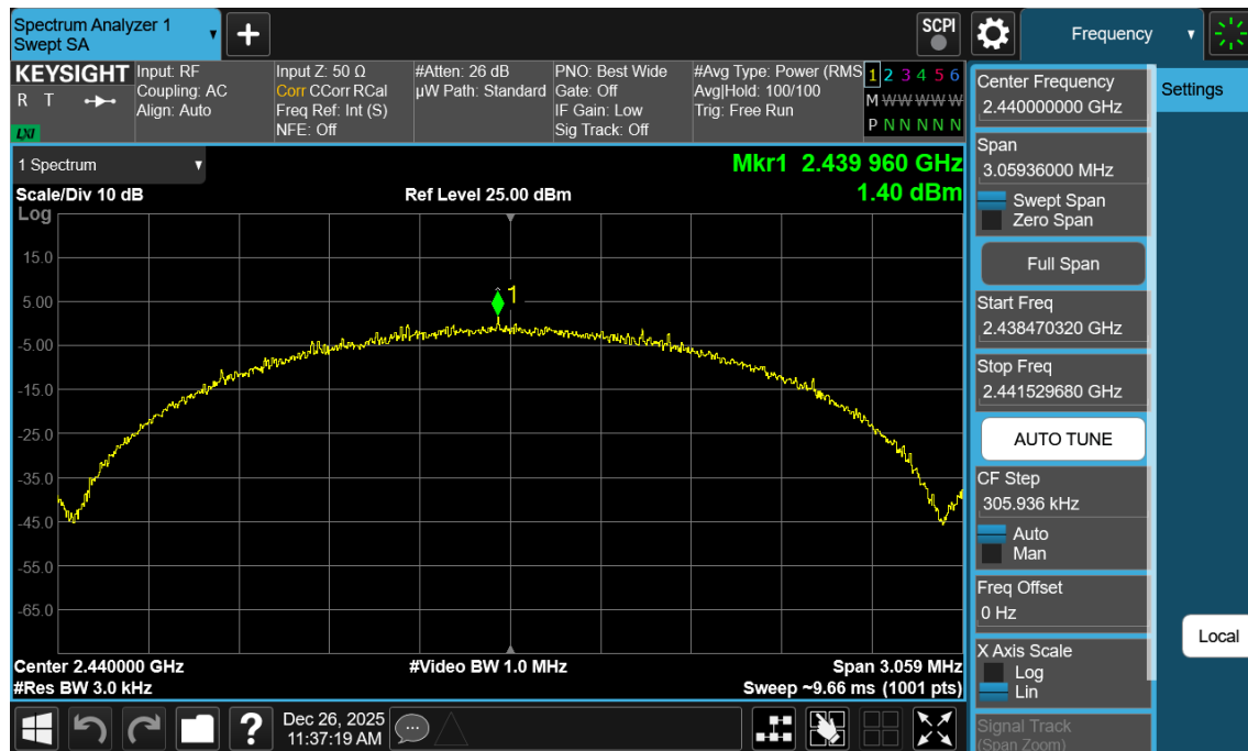
Plot 7-68. Power Spectral Density Plot Antenna WF7b (Bluetooth (LE), 2Mbps, ePA – Ch. 19)
