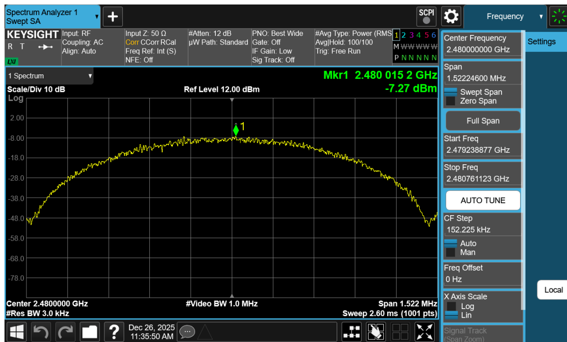
Plot 7-66. Power Spectral Density Plot Antenna WF7b (Bluetooth (LE), 1Mbps, iPA – Ch. 39)
