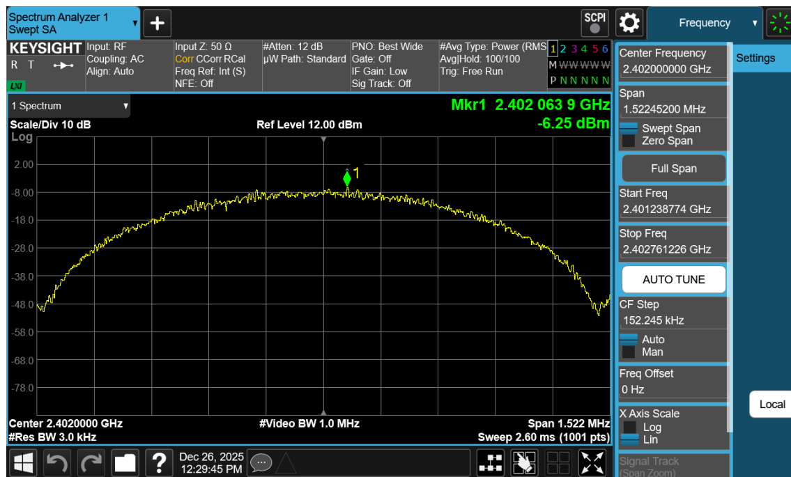
Plot 7-88. Power Spectral Density Plot Antenna WF2b (Bluetooth (LE), 1Mbps, iPA – Ch. 0)
