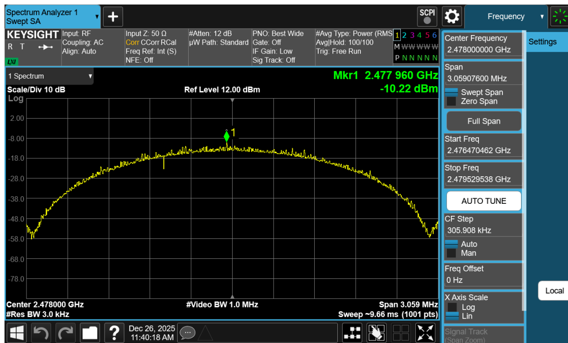
Plot 7-72. Power Spectral Density Plot Antenna WF7b (Bluetooth (LE), 2Mbps, iPA – Ch. 38)
