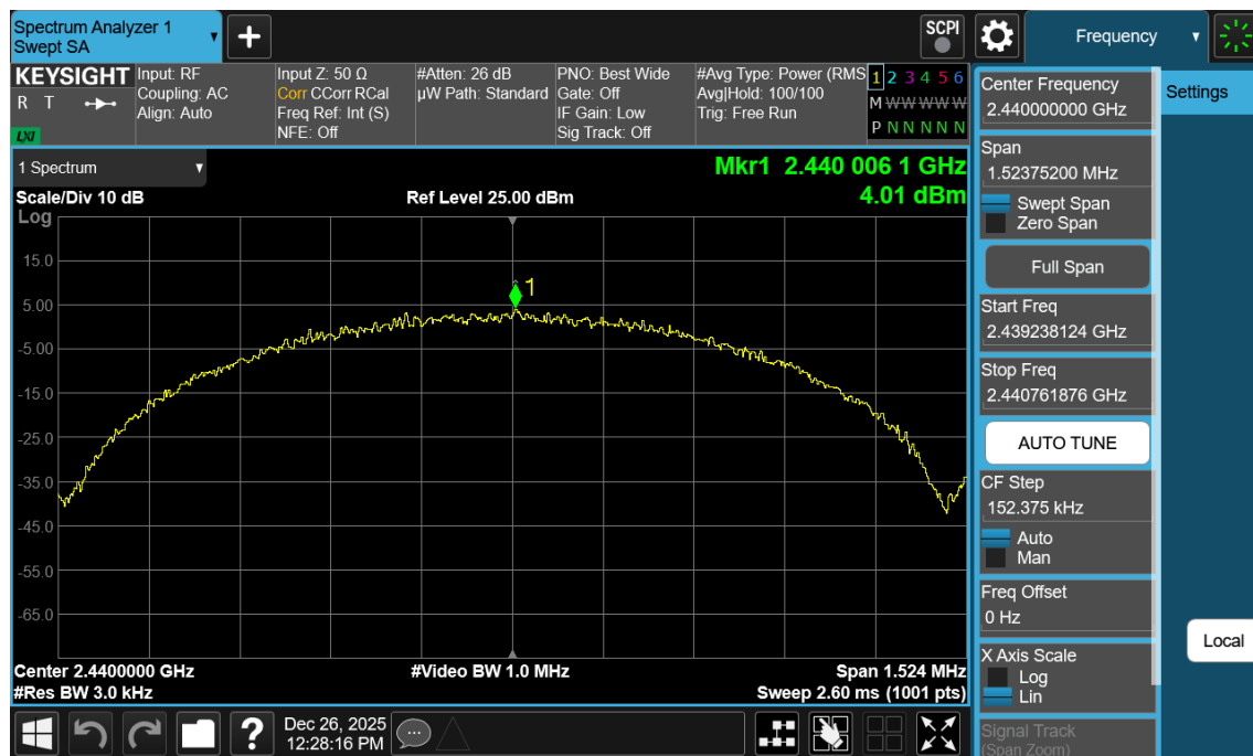
Plot 7-86. Power Spectral Density Plot Antenna WF2b (Bluetooth (LE), 1Mbps, ePA – Ch. 19)
