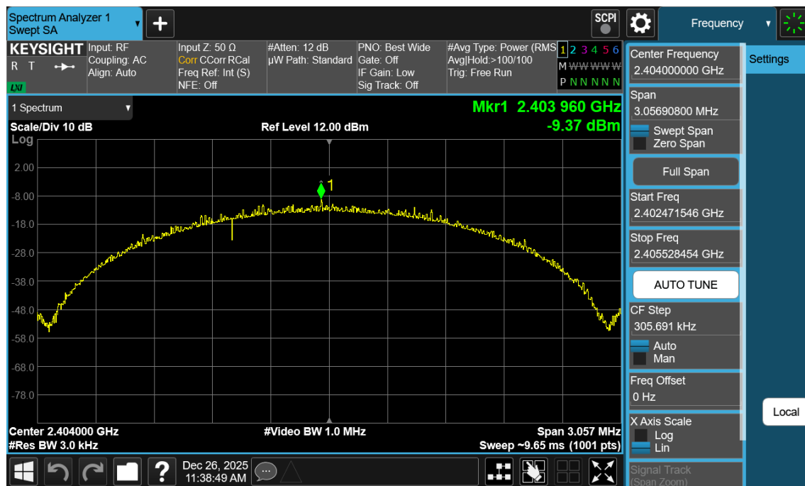
Plot 7-70. Power Spectral Density Plot Antenna WF7b (Bluetooth (LE), 2Mbps, iPA – Ch. 1)
