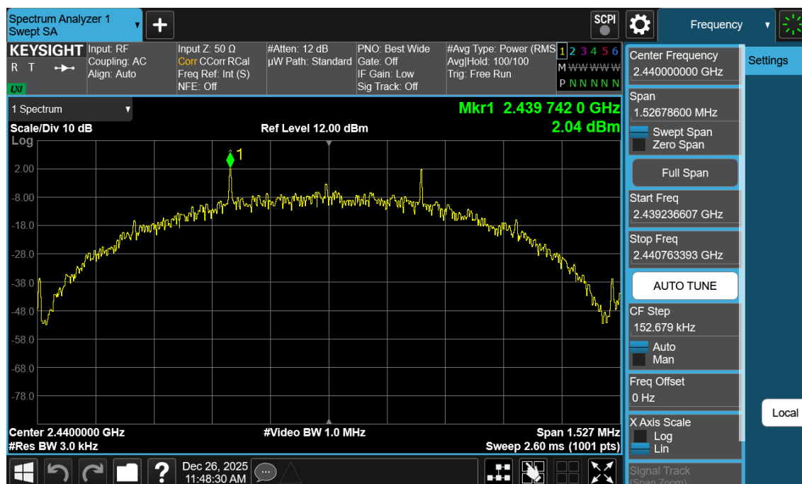
Plot 7-59. Power Spectral Density Plot Antenna WF7b (Bluetooth (LE), 500kbps, iPA – Ch. 19)
