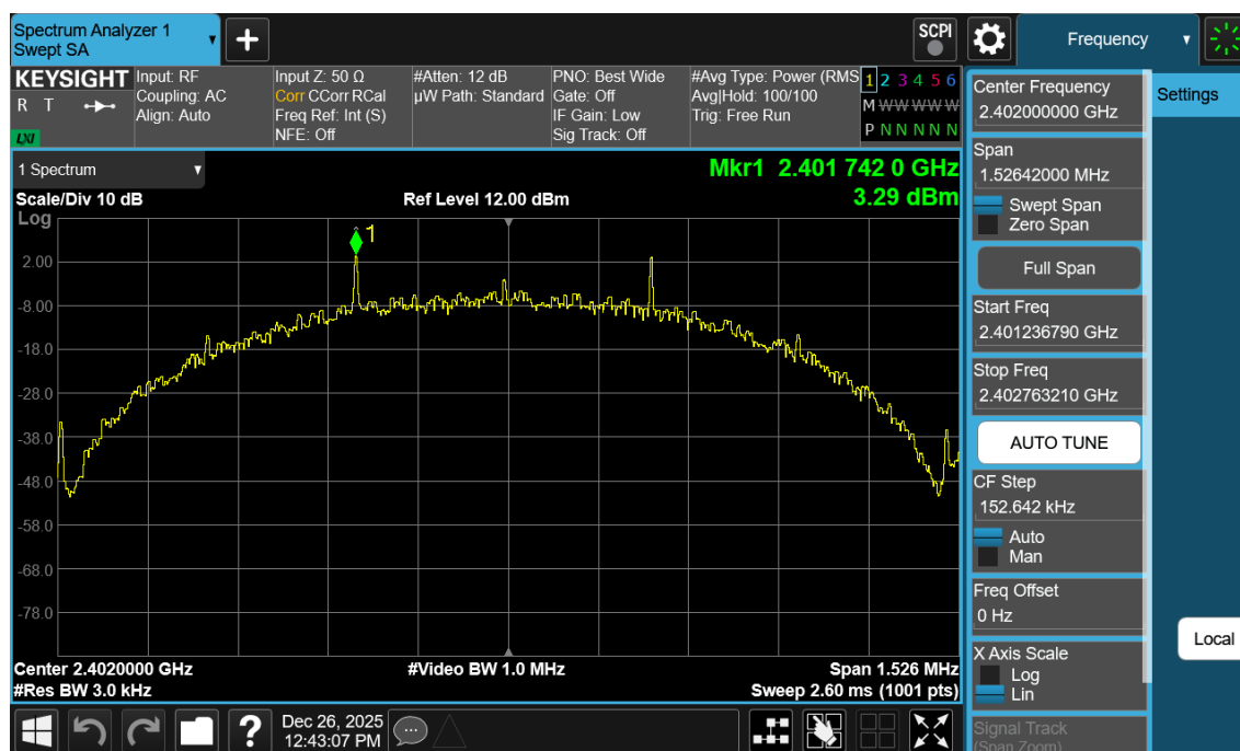
Plot 7-82. Power Spectral Density Plot Antenna WF2b (Bluetooth (LE), 500kbps, iPA – Ch. 0)
