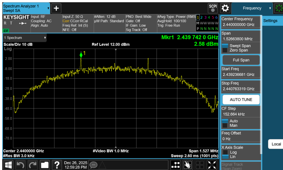
Plot 7-112. Power Spectral Density Plot Antenna WF2b (Bluetooth (LE), 500kbps, ePA – Ch. 19)
