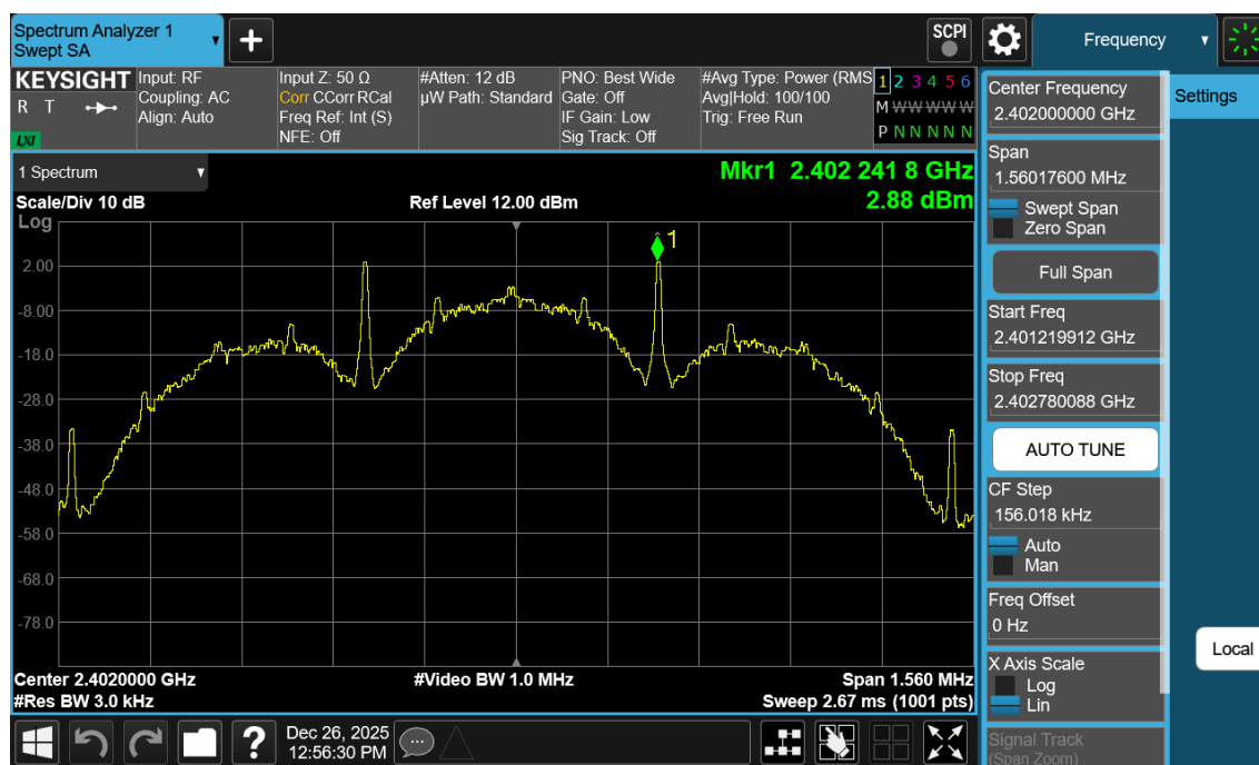
Plot 7-104. Power Spectral Density Plot Antenna WF2b (Bluetooth (LE), 125kbps, iPA – Ch. 0)
