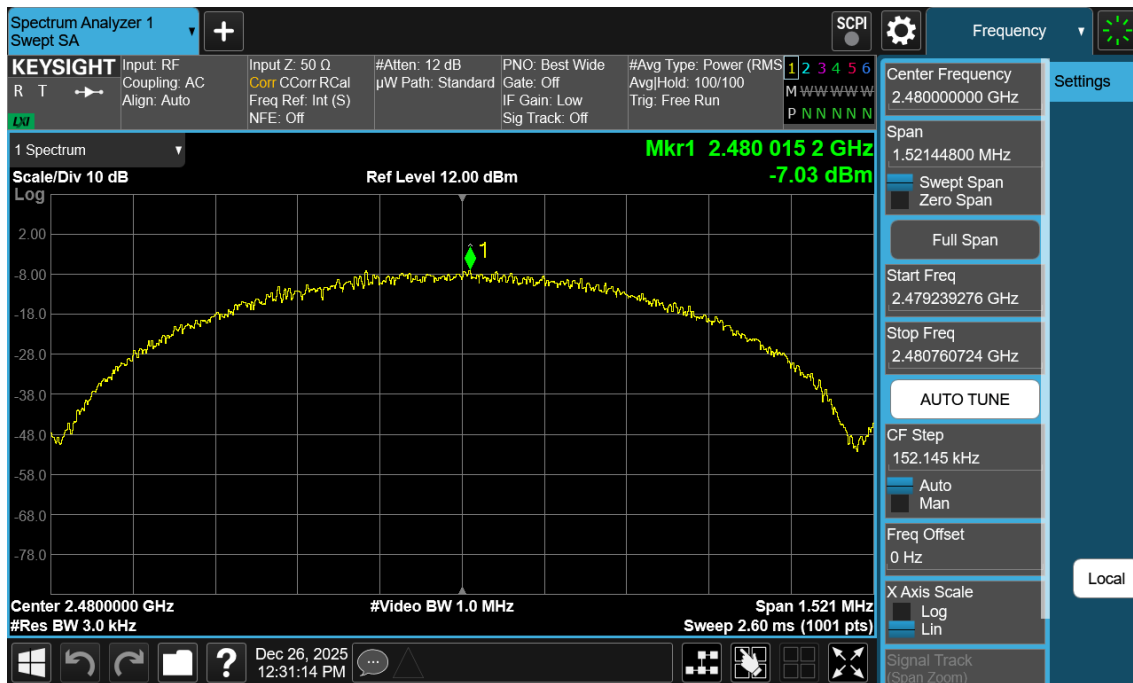
Plot 7-90. Power Spectral Density Plot Antenna WF2b (Bluetooth (LE), 1Mbps, iPA – Ch. 39)
