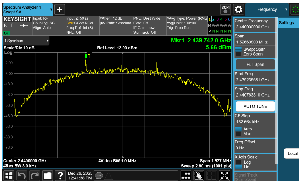
Plot 7-80. Power Spectral Density Plot Antenna WF2b (Bluetooth (LE), 500kbps, ePA – Ch. 19)
