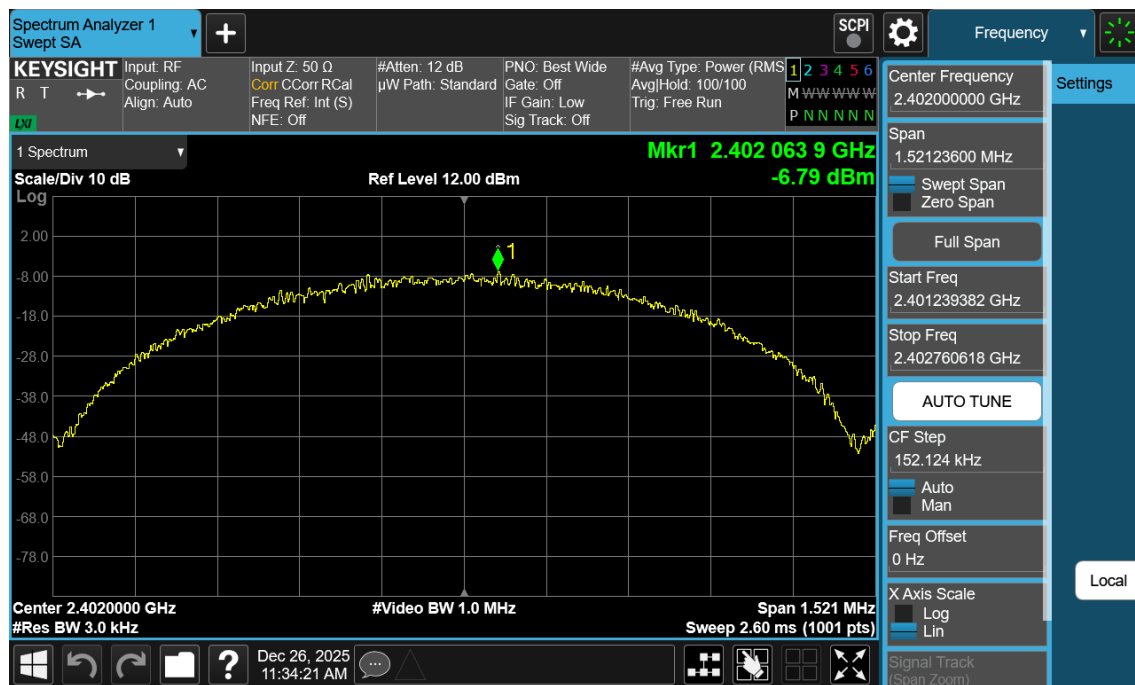
Plot 7-64. Power Spectral Density Plot Antenna WF7b (Bluetooth (LE), 1Mbps, iPA – Ch. 0)
