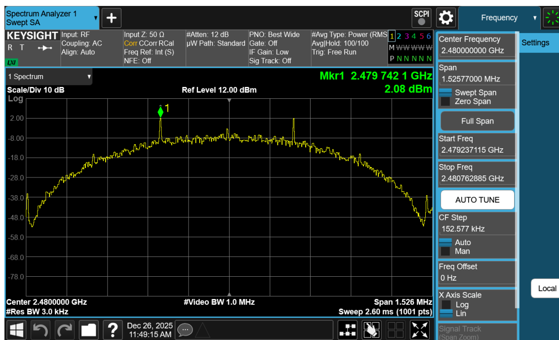
Plot 7-60. Power Spectral Density Plot Antenna WF7b (Bluetooth (LE), 500kbps, iPA – Ch. 39)
