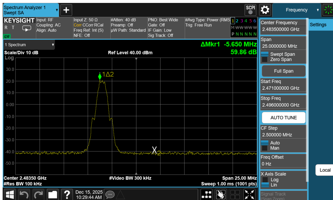
Plot 7-148. Band Edge Plot Antenna WF7b (Bluetooth (LE), 500kbps, ePA – Ch. 39)
