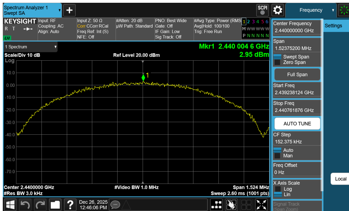
Plot 7-124. Power Spectral Density Plot Antenna WF2b (Bluetooth (LE), 1Mbps, ePA – Ch. 19)
