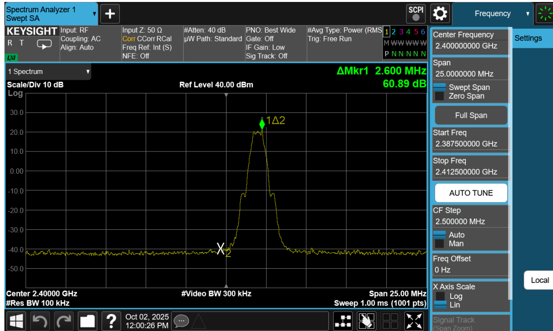
Plot 7-149. Band Edge Plot Antenna WF7b (Bluetooth (LE), 1Mbps, ePA – Ch.0)
