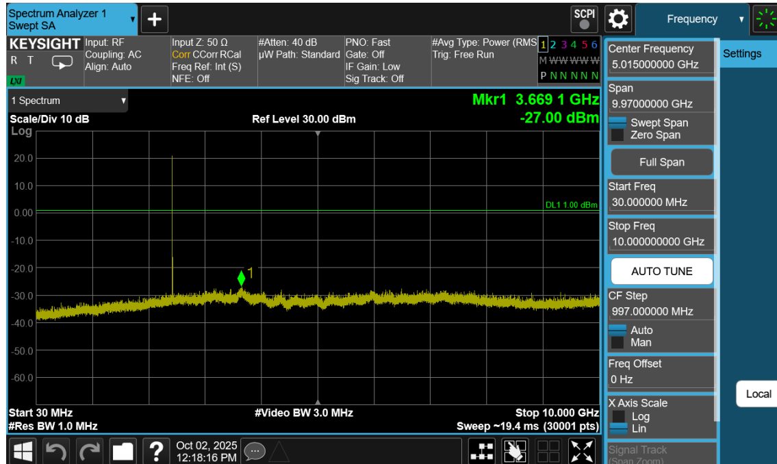
Plot 7-163. Conducted Spurious Plot Antenna WF7b (Bluetooth (LE), 1Mbps, ePA – Ch. 19)
