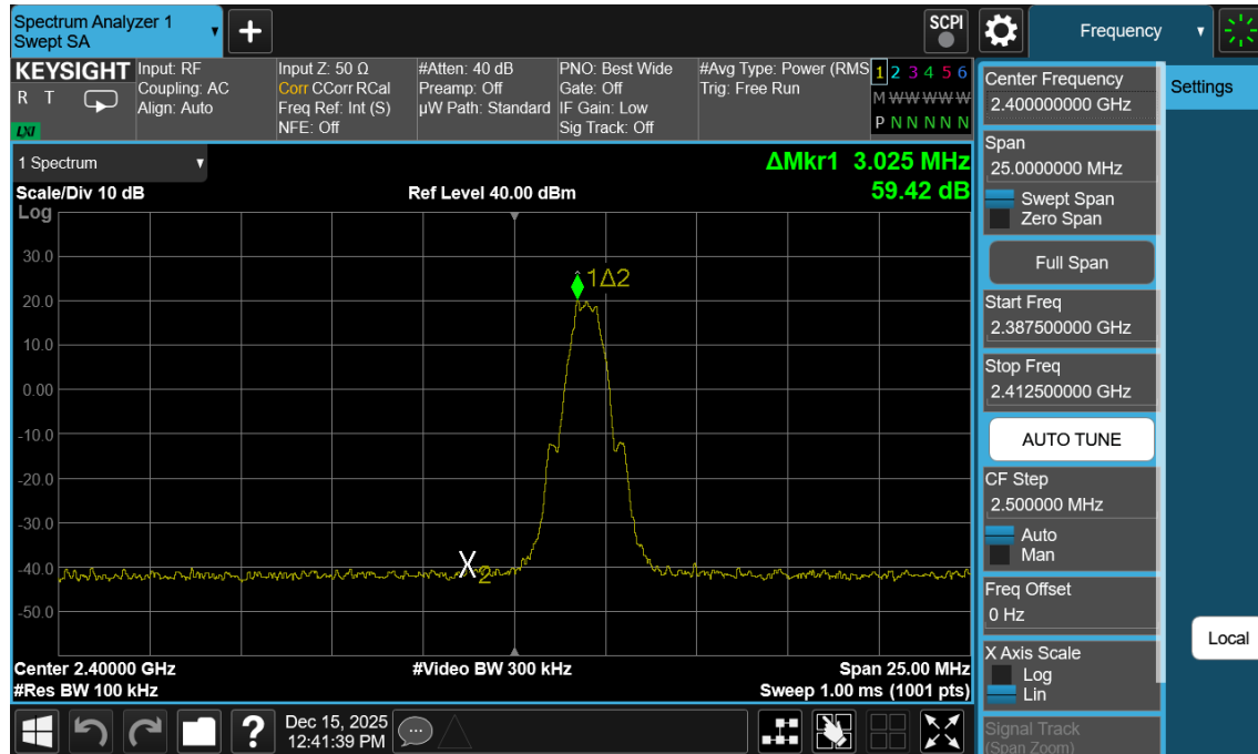
Plot 7-155. Band Edge Plot Antenna WF2b (Bluetooth (LE), 500kbps, ePA – Ch.0)
