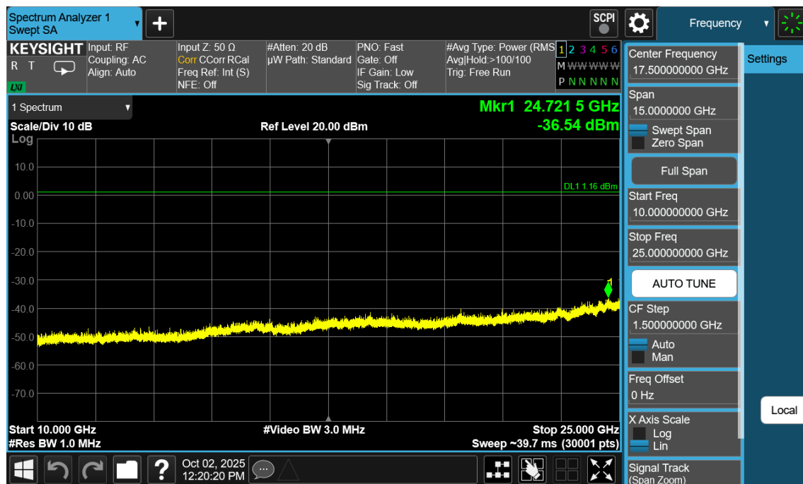
Plot 7-166. Conducted Spurious Plot Antenna WF7b (Bluetooth) (LE), 1Mbps, ePA – Ch. 39)
