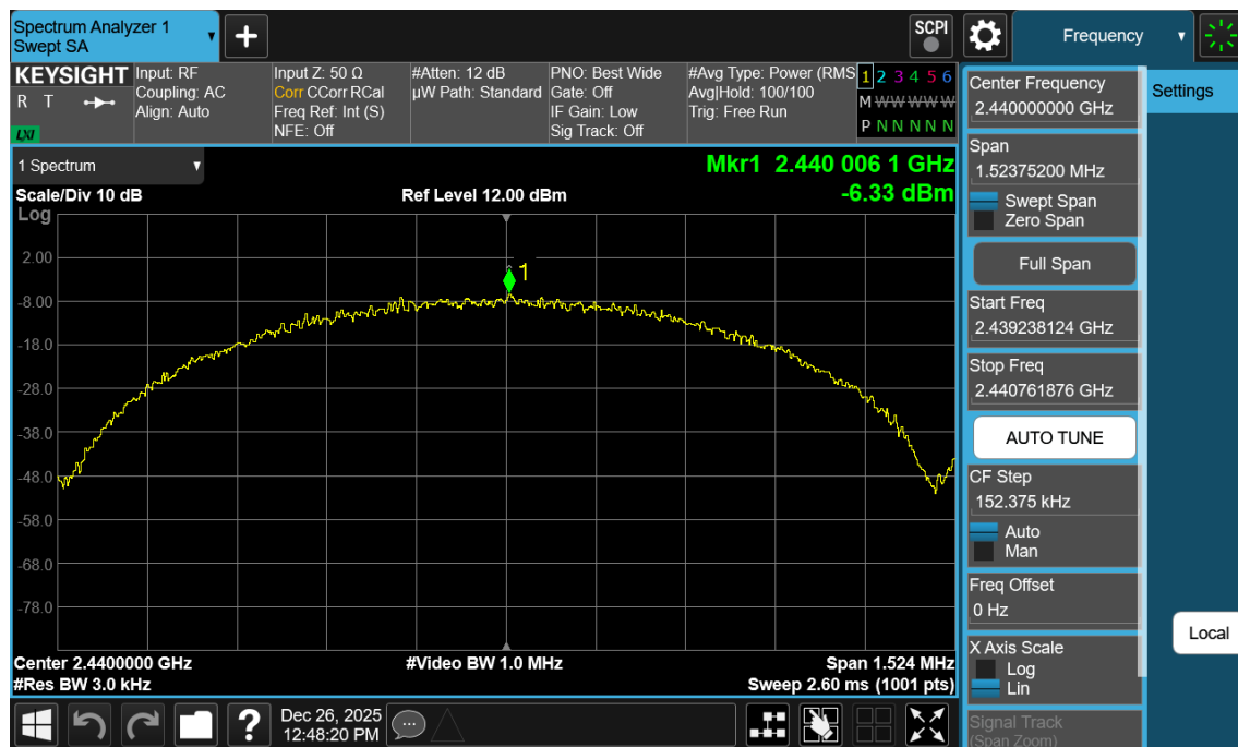
Plot 7-130. Power Spectral Density Plot Antenna WF2b (Bluetooth (LE), 1Mbps, iPA – Ch. 19)
