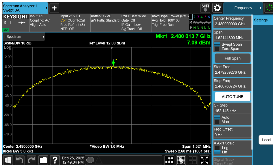
Plot 7-132. Power Spectral Density Plot Antenna WF2b (Bluetooth (LE), 1Mbps, iPA – Ch. 39)
