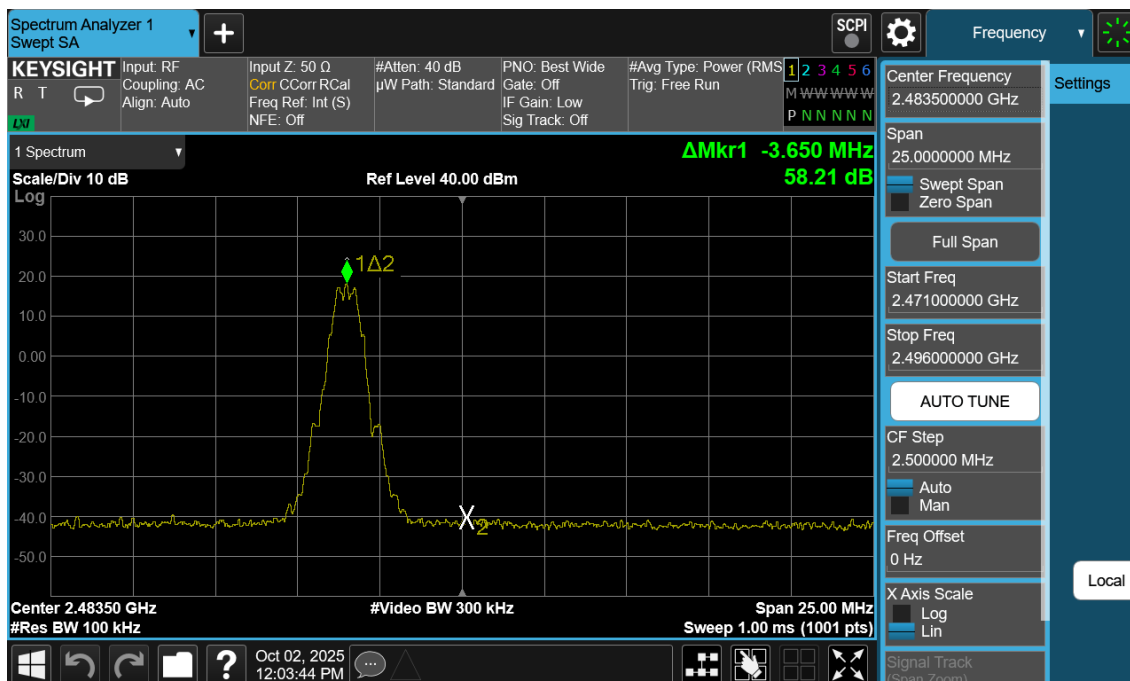
Plot 7-146. Band Edge Plot Antenna WF7b (Bluetooth (LE), 125kbps, ePA – Ch. 39)
