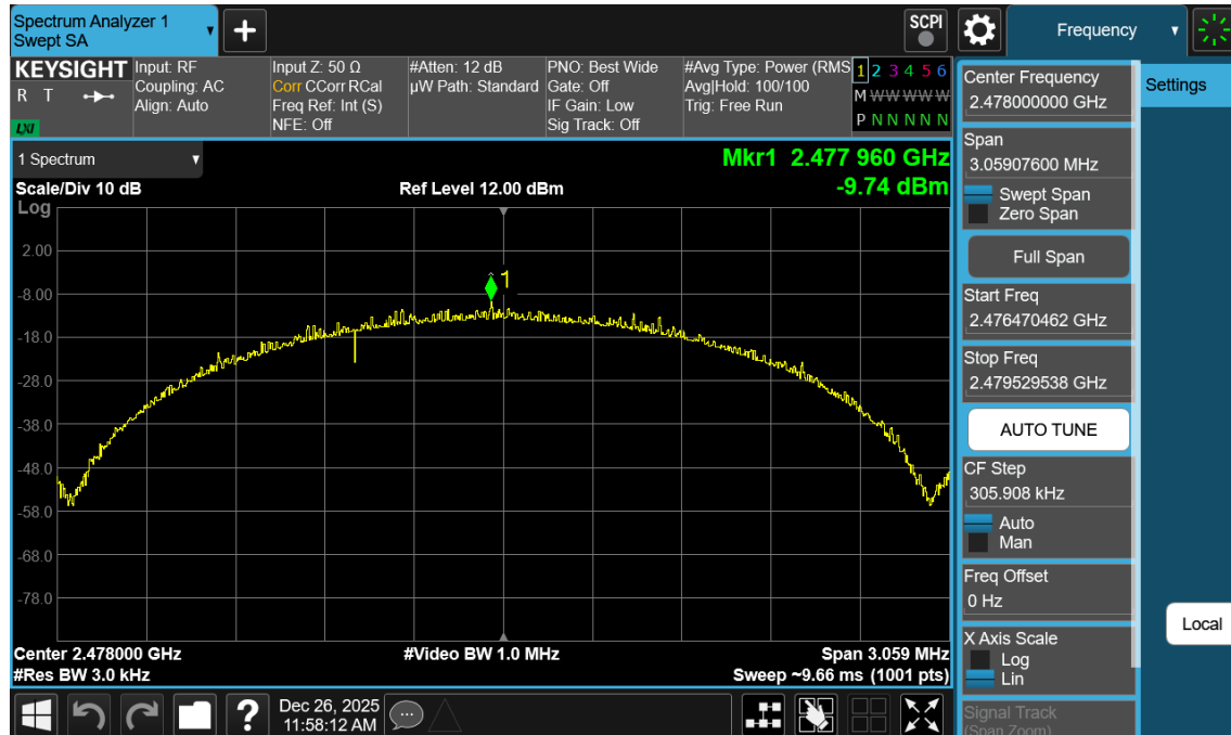
Plot 7-143. Power Spectral Density Plot Antenna WF7b (Bluetooth (LE), 2Mbps, iPA – Ch. 38)
