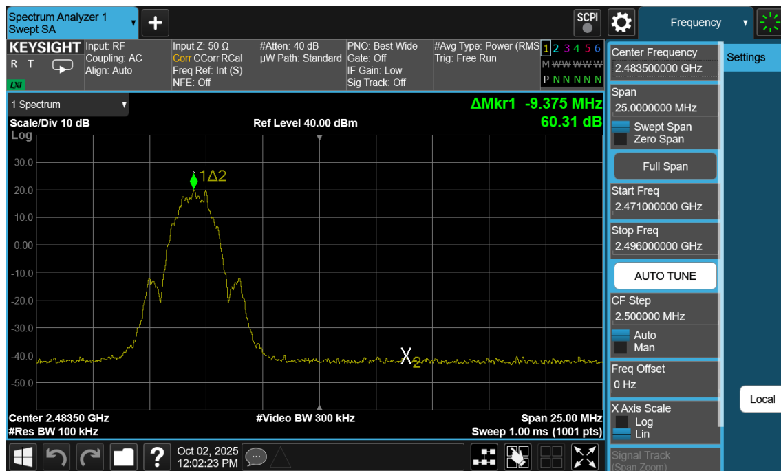
Plot 7-152. Band Edge Plot Antenna WF7b (Bluetooth (LE), 2Mbps, ePA – Ch. 38)
