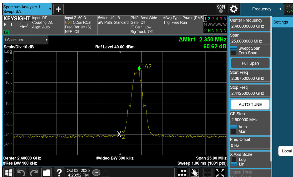
Plot 7-157. Band Edge Plot Antenna WF2b (Bluetooth (LE), 1Mbps, ePA – Ch.0)
