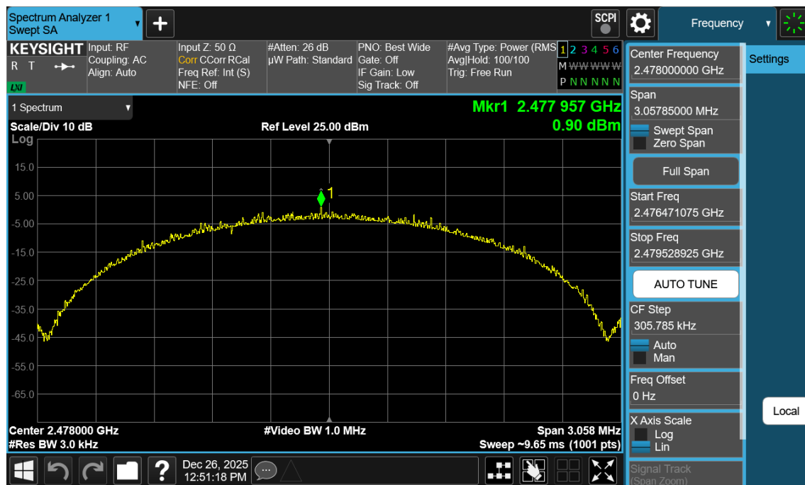
Plot 7-138. Power Spectral Density Plot Antenna WF2b (Bluetooth (LE), 2Mbps, ePA – Ch. 38)
