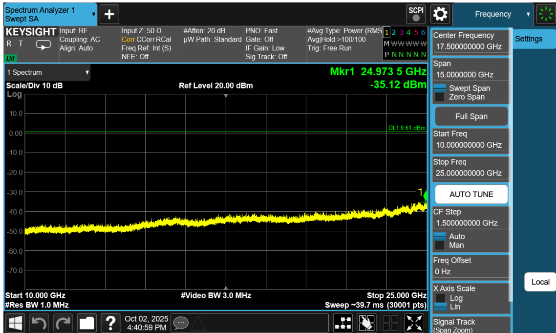
Plot 7-168. Conducted Spurious Plot Antenna WF2b (Bluetooth (LE), 1Mbps, ePA – Ch. 0)
