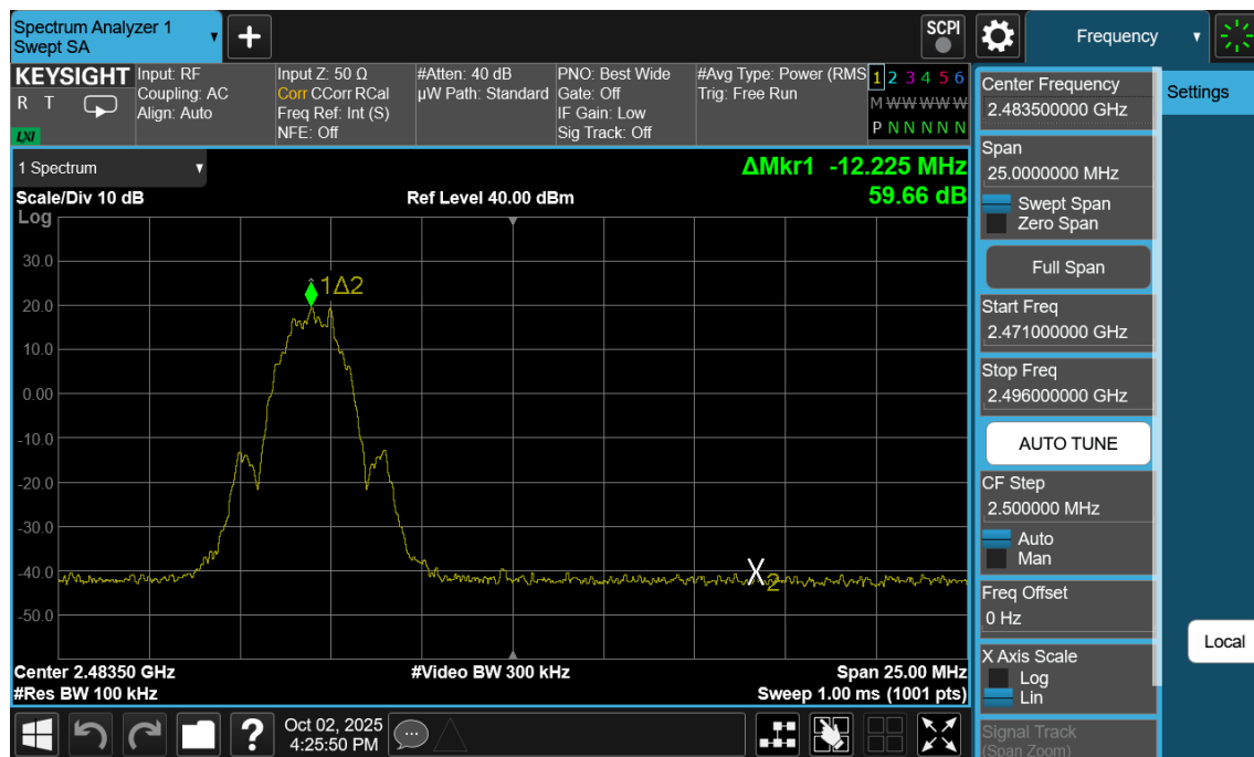
Plot 7-160. Band Edge Plot Antenna WF2b (Bluetooth (LE), 2Mbps, ePA – Ch. 38)
