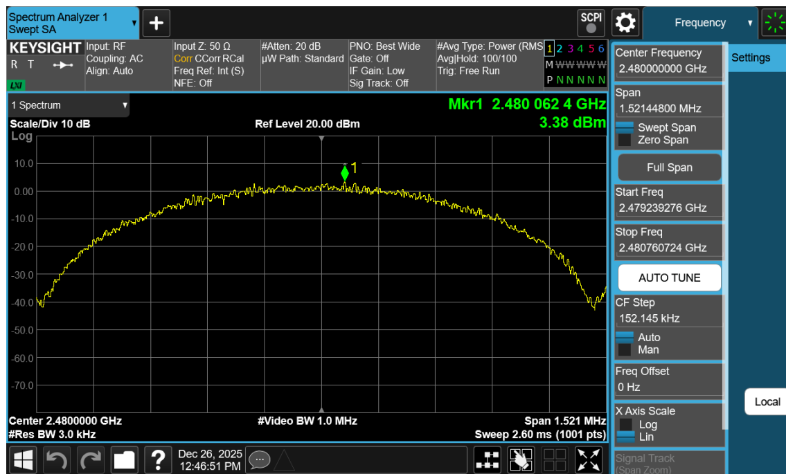
Plot 7-126. Power Spectral Density Plot Antenna WF2b (Bluetooth (LE), 1Mbps, ePA – Ch. 39)
