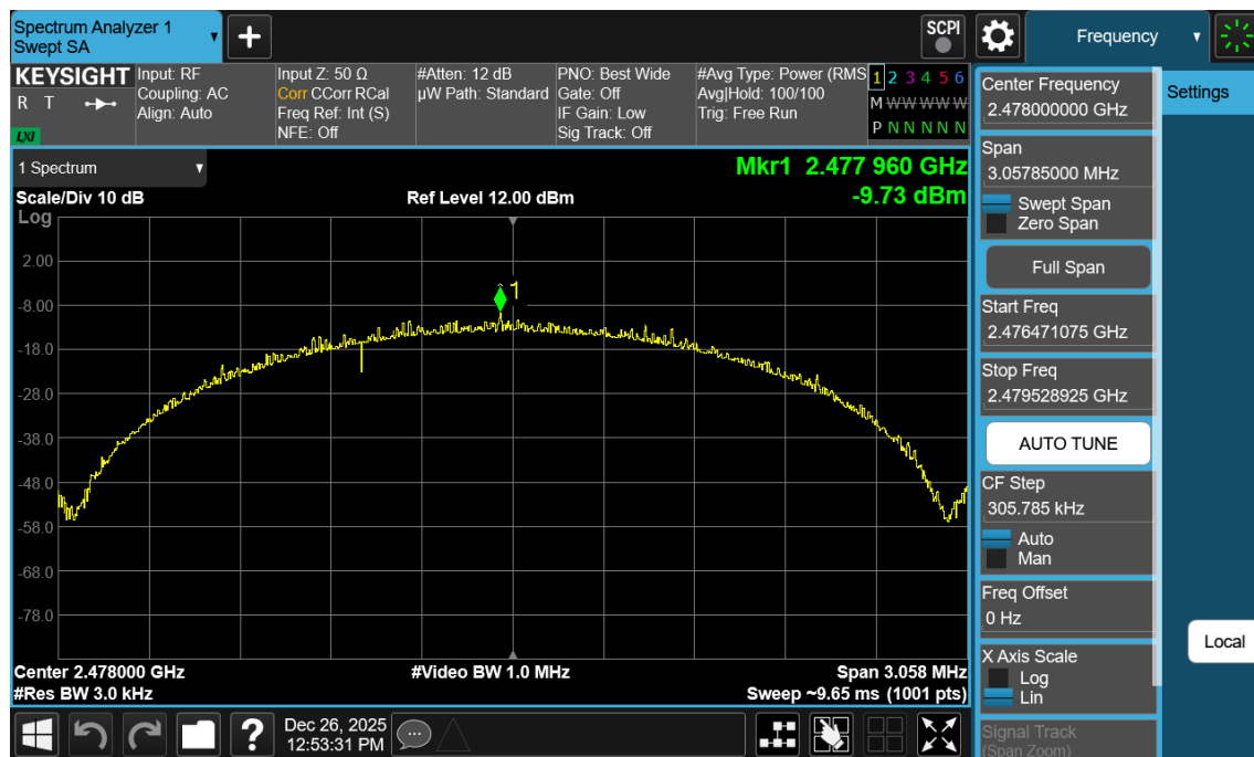
Plot 7-144. Power Spectral Density Plot Antenna WF2b (Bluetooth (LE), 2Mbps, iPA – Ch. 38)
