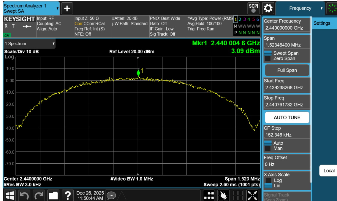
Plot 7-123. Power Spectral Density Plot Antenna WF7b (Bluetooth (LE), 1Mbps, ePA – Ch. 19)
