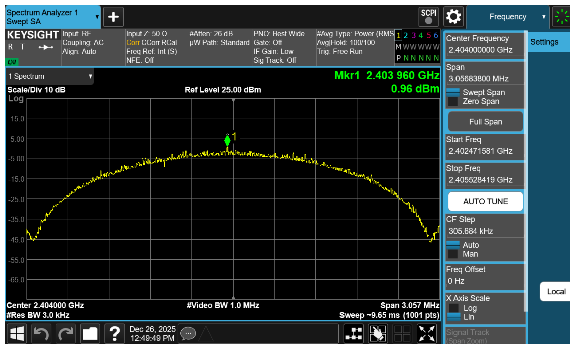
Plot 7-134. Power Spectral Density Plot Antenna WF2b (Bluetooth (LE), 2Mbps, ePA – Ch. 1)
