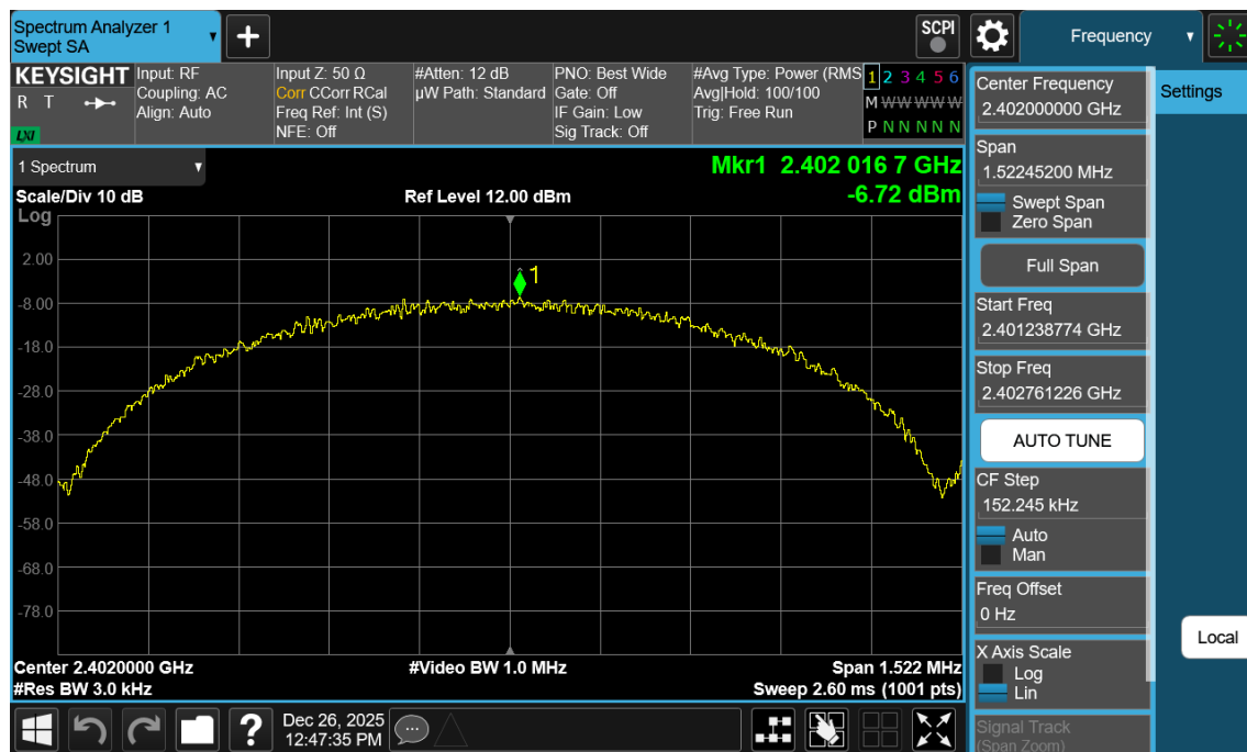
Plot 7-128. Power Spectral Density Plot Antenna WF2b (Bluetooth (LE), 1Mbps, iPA – Ch. 0)
