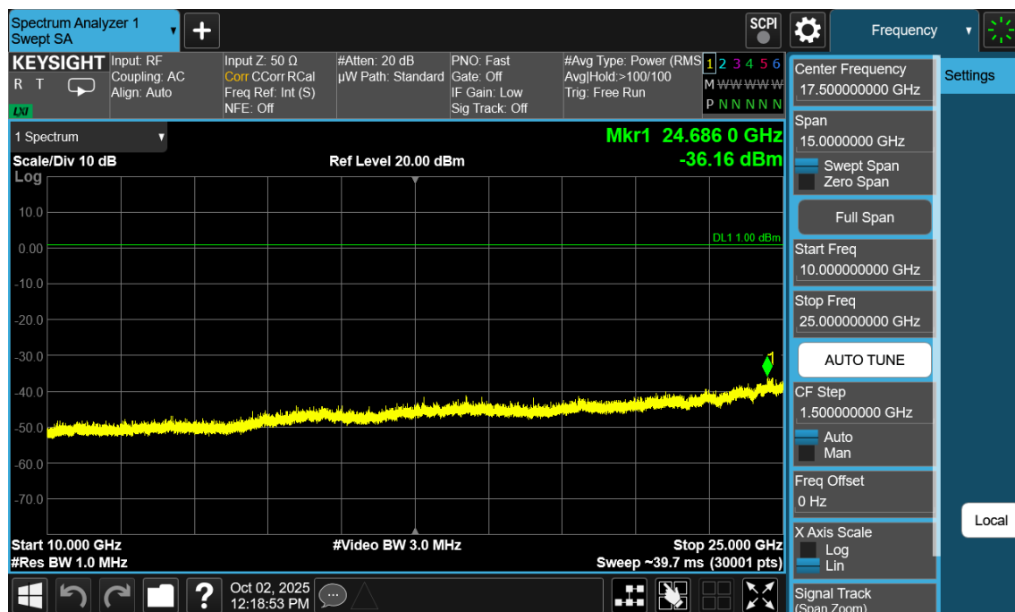
Plot 7-164. Conducted Spurious Plot Antenna WF7b (Bluetooth (LE), 1Mbps, ePA – Ch. 19)
