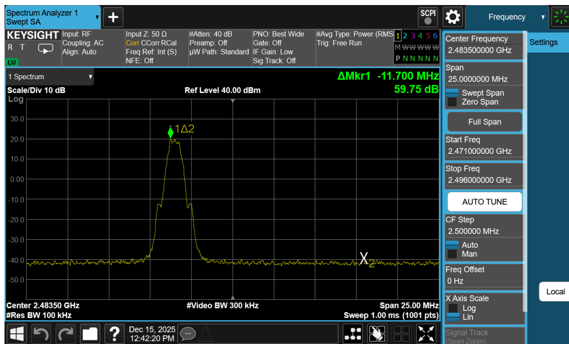
Plot 7-156. Band Edge Plot Antenna WF2b (Bluetooth (LE), 500kbps, ePA – Ch. 39)
