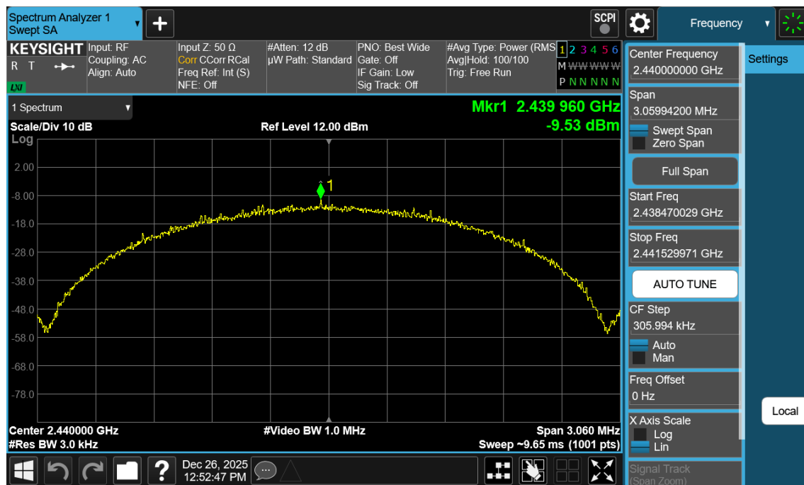
Plot 7-142. Power Spectral Density Plot Antenna WF2b (Bluetooth (LE), 2Mbps, iPA – Ch. 19)
