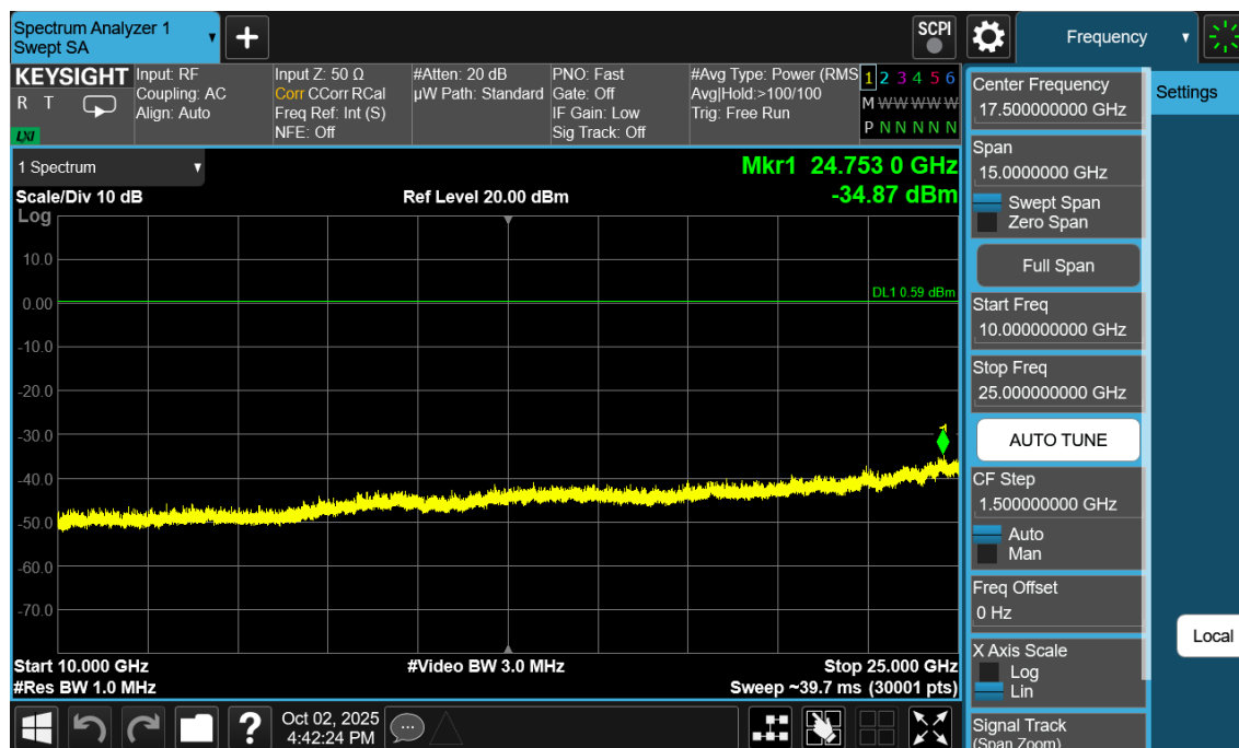
Plot 7-170. Conducted Spurious Plot Antenna WF2b (Bluetooth (LE), 1Mbps, ePA – Ch. 19)
