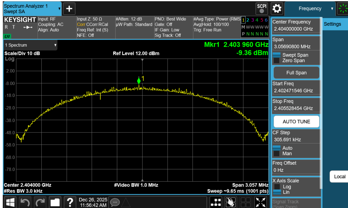
Plot 7-139. Power Spectral Density Plot Antenna WF7b (Bluetooth (LE), 2Mbps, iPA – Ch. 1)
