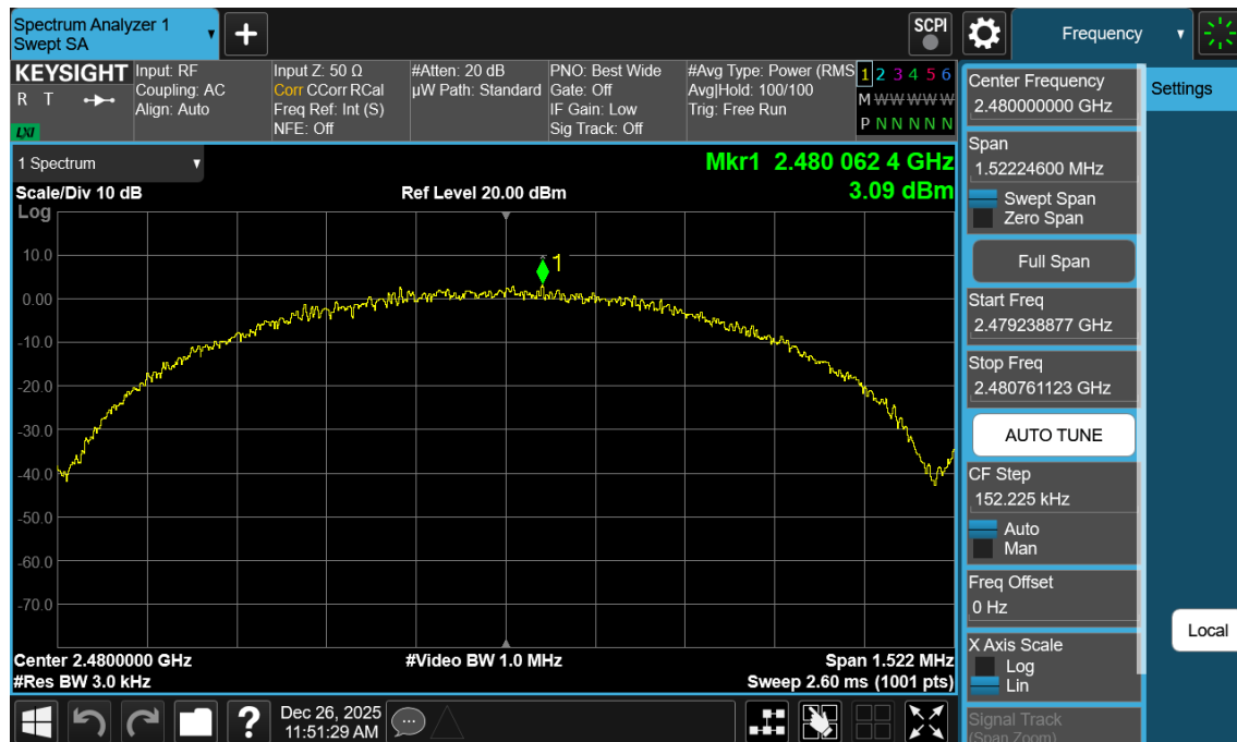
Plot 7-125. Power Spectral Density Plot Antenna WF7b (Bluetooth (LE), 1Mbps, ePA – Ch. 39)
