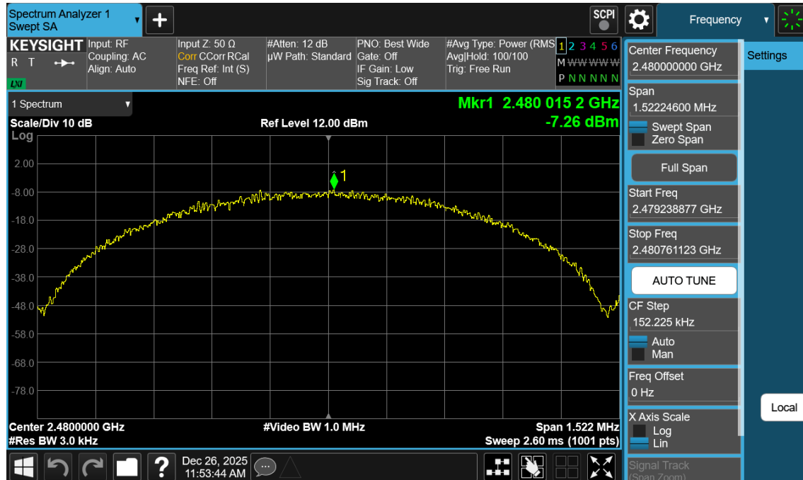
Plot 7-131. Power Spectral Density Plot Antenna WF7b (Bluetooth (LE), 1Mbps, iPA – Ch. 39)
