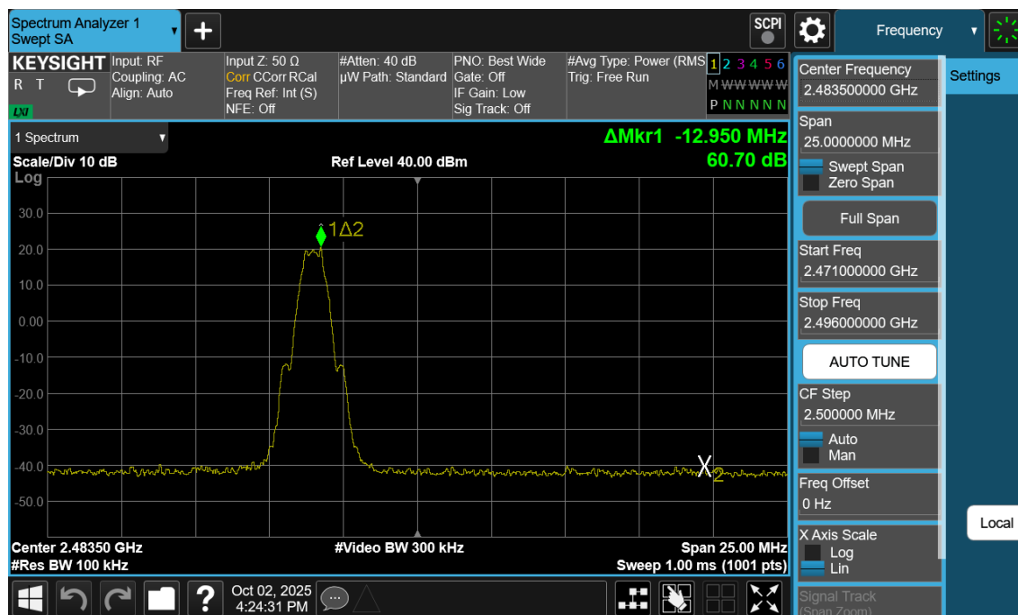
Plot 7-158. Band Edge Plot Antenna WF2b (Bluetooth (LE), 1Mbps, ePA – Ch. 39)
