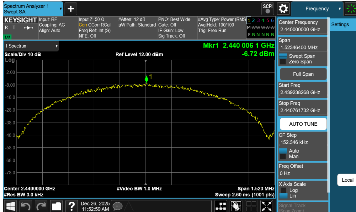
Plot 7-129. Power Spectral Density Plot Antenna WF7b (Bluetooth (LE), 1Mbps, iPA – Ch. 19)
