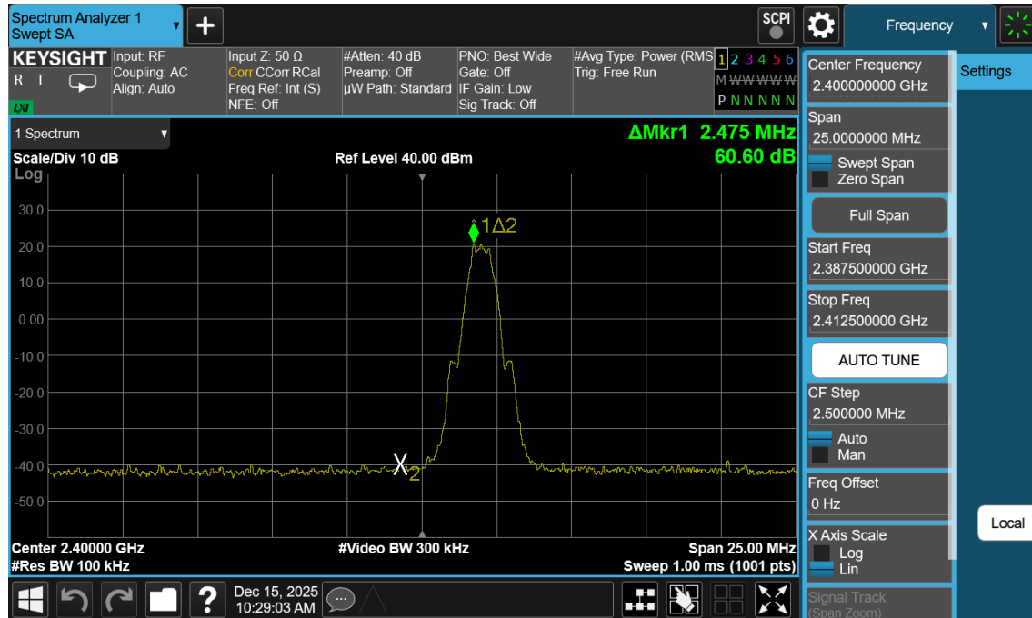
Plot 7-147. Band Edge Plot Antenna WF7b (Bluetooth (LE), 500kbps, ePA – Ch.0)
