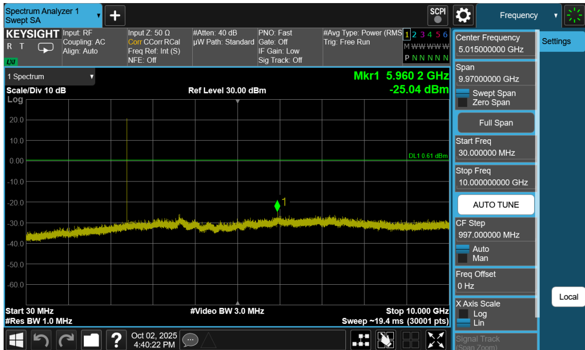
Plot 7-167. Conducted Spurious Plot Antenna WF2b (Bluetooth (LE), 1Mbps, ePA – Ch. 0)
