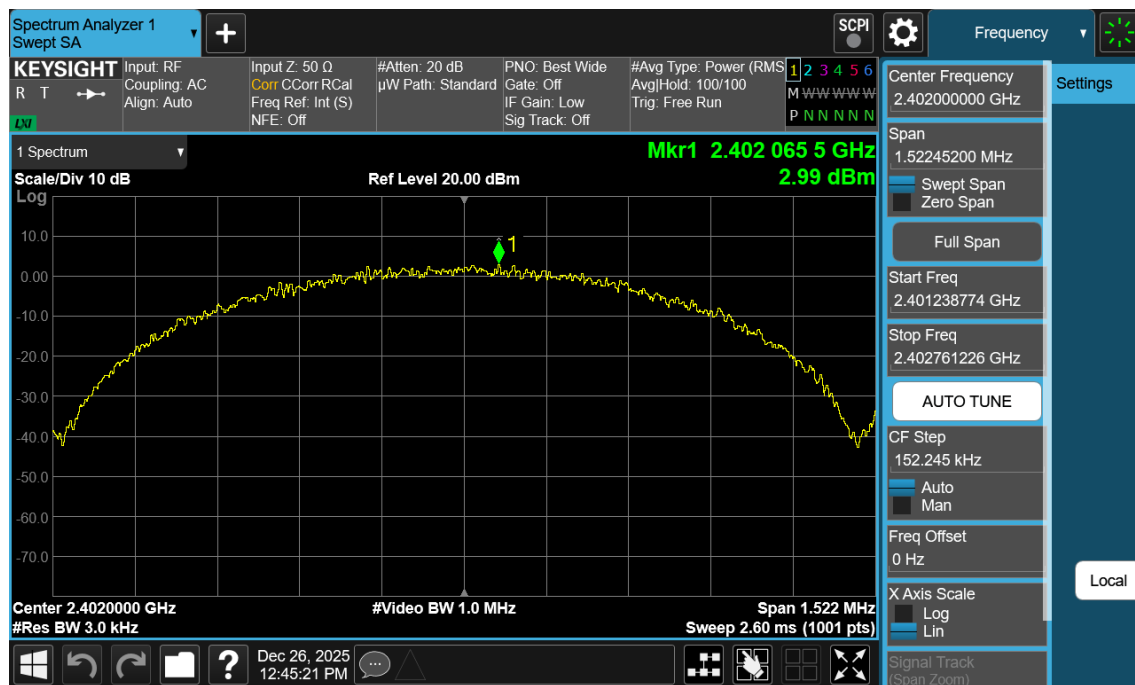
Plot 7-122. Power Spectral Density Plot Antenna WF2b (Bluetooth (LE), 1Mbps, ePA – Ch. 0)
