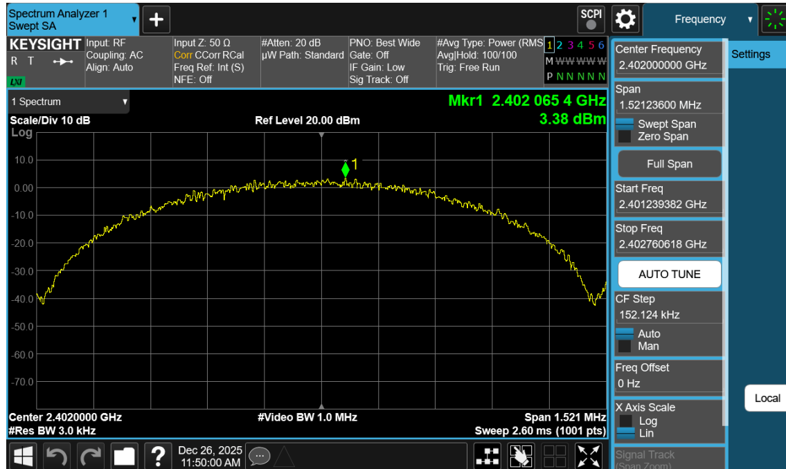
Plot 7-121. Power Spectral Density Plot Antenna WF7b (Bluetooth (LE), 1Mbps, ePA – Ch. 0)
