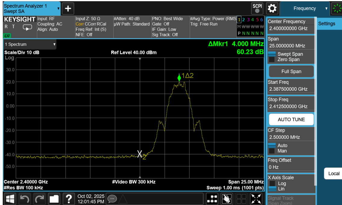
Plot 7-151. Band Edge Plot Antenna WF7b (Bluetooth (LE), 2Mbps, ePA – Ch. 1)
