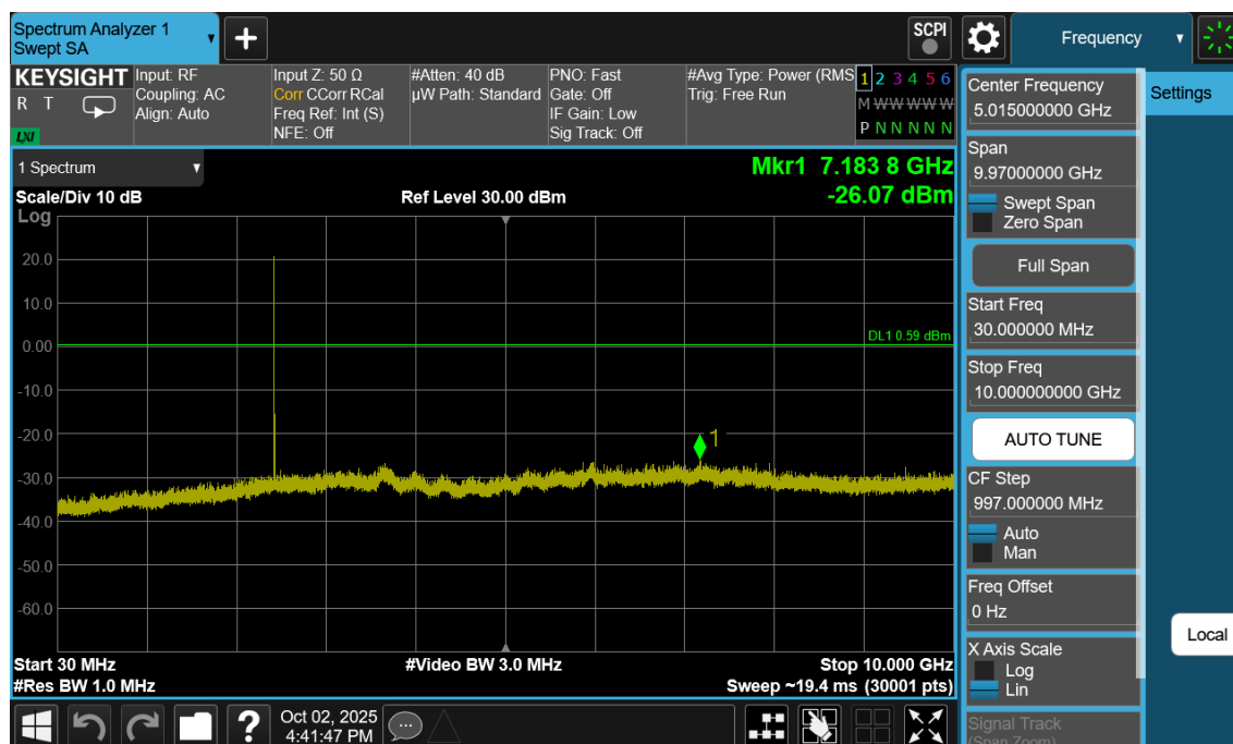
Plot 7-169. Conducted Spurious Plot Antenna WF2b (Bluetooth (LE), 1Mbps, ePA – Ch. 19)
