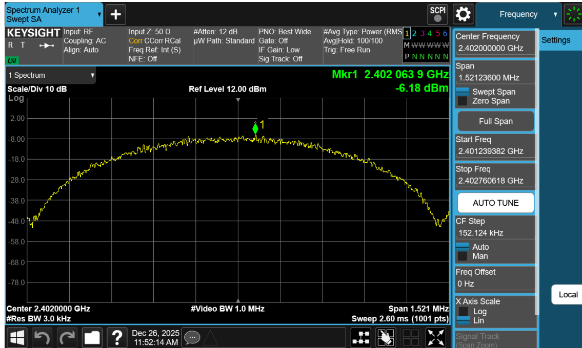
Plot 7-127. Power Spectral Density Plot Antenna WF7b (Bluetooth (LE), 1Mbps, iPA – Ch. 0)
