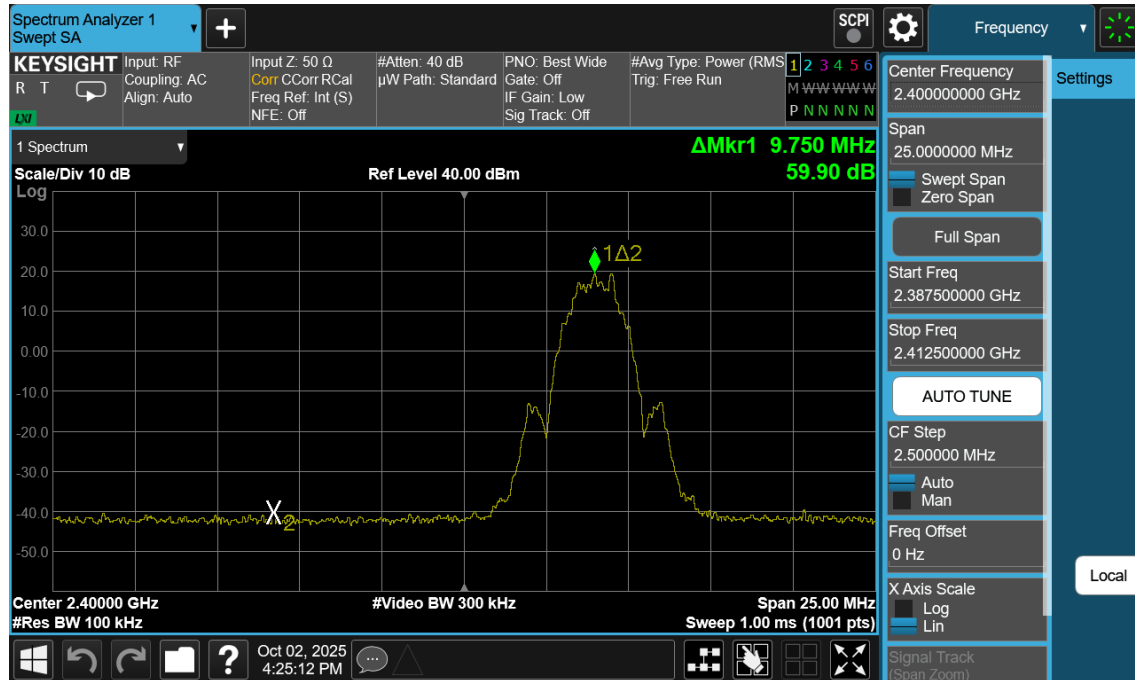
Plot 7-159. Band Edge Plot Antenna WF2b (Bluetooth (LE), 2Mbps, ePA – Ch. 1)
