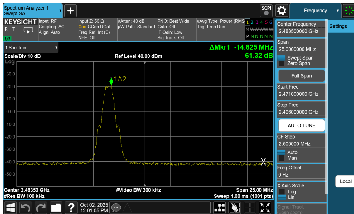
Plot 7-150. Band Edge Plot Antenna WF7b (Bluetooth (LE), 1Mbps, ePA – Ch. 39)
