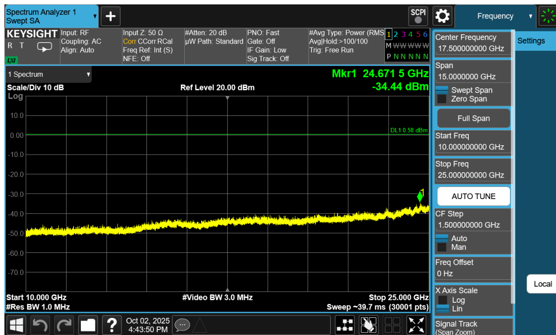
Plot 7-172. Conducted Spurious Plot Antenna WF2b (Bluetooth (LE), 1Mbps, ePA – Ch. 39)
