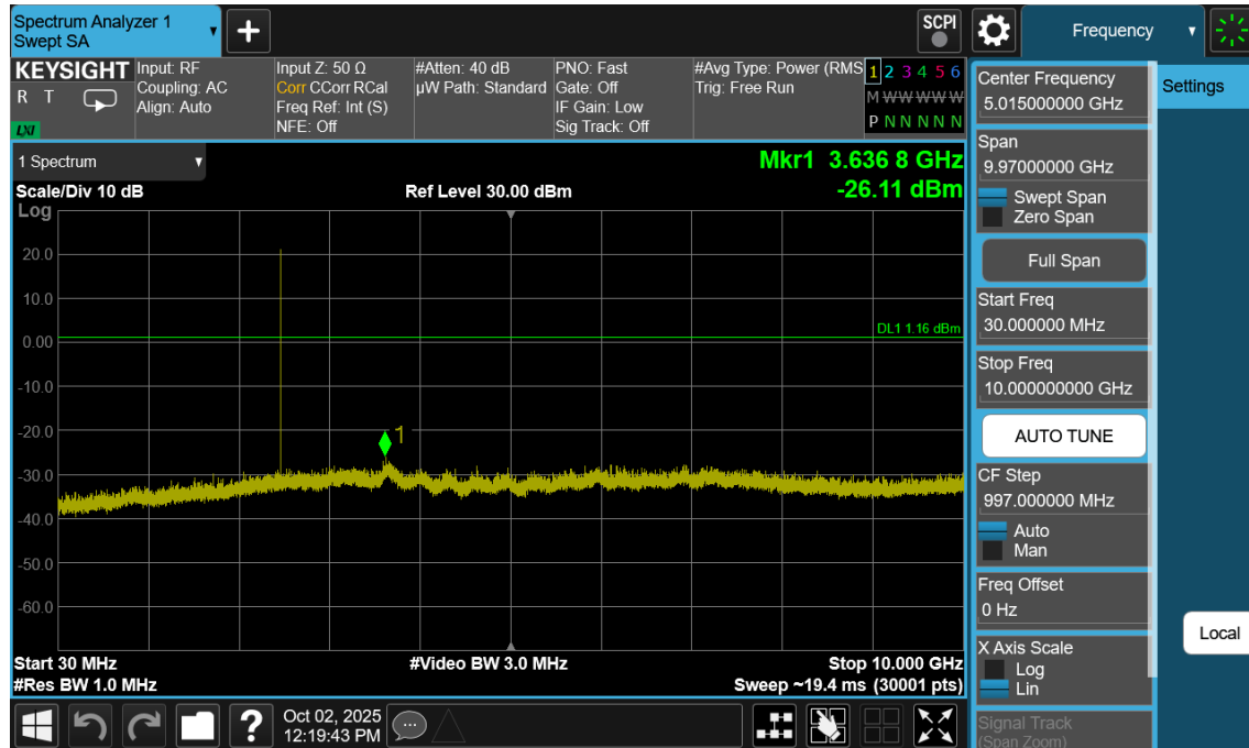
Plot 7-165. Conducted Spurious Plot Antenna WF7b (Bluetooth) (LE), 1Mbps, ePA – Ch. 39)
