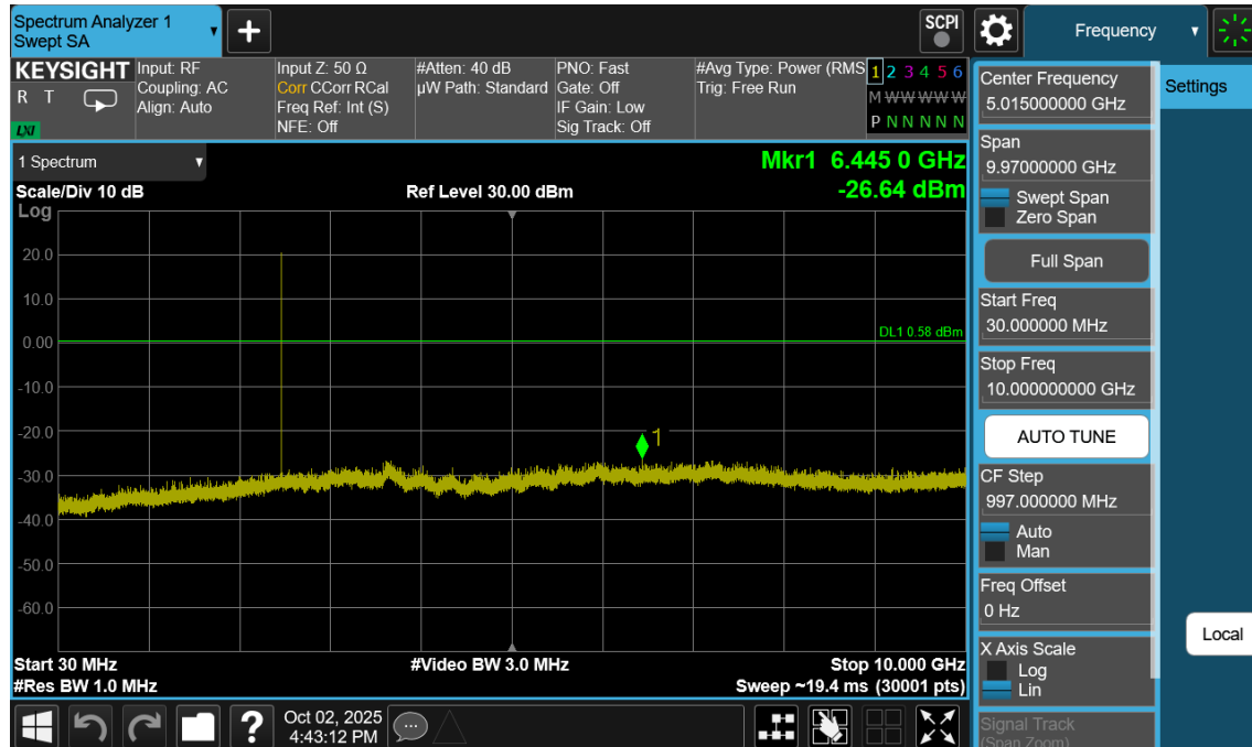
Plot 7-171. Conducted Spurious Plot Antenna WF2b (Bluetooth (LE), 1Mbps, ePA – Ch. 39)
