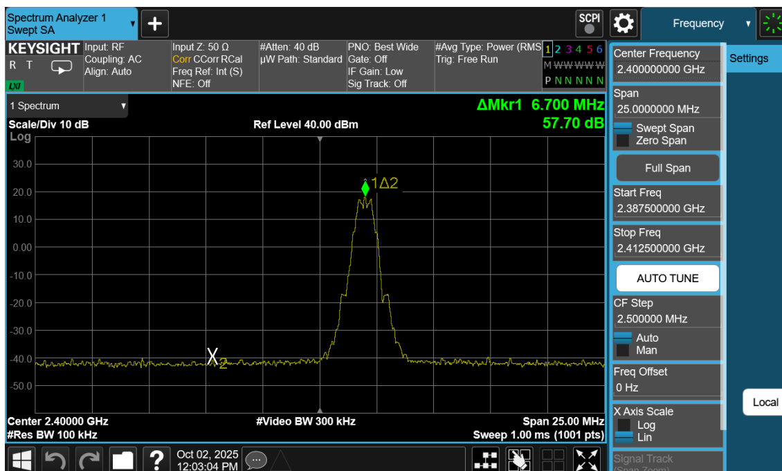
Plot 7-145. Band Edge Plot Antenna WF7b (Bluetooth (LE), 125kbps, ePA – Ch.0)
