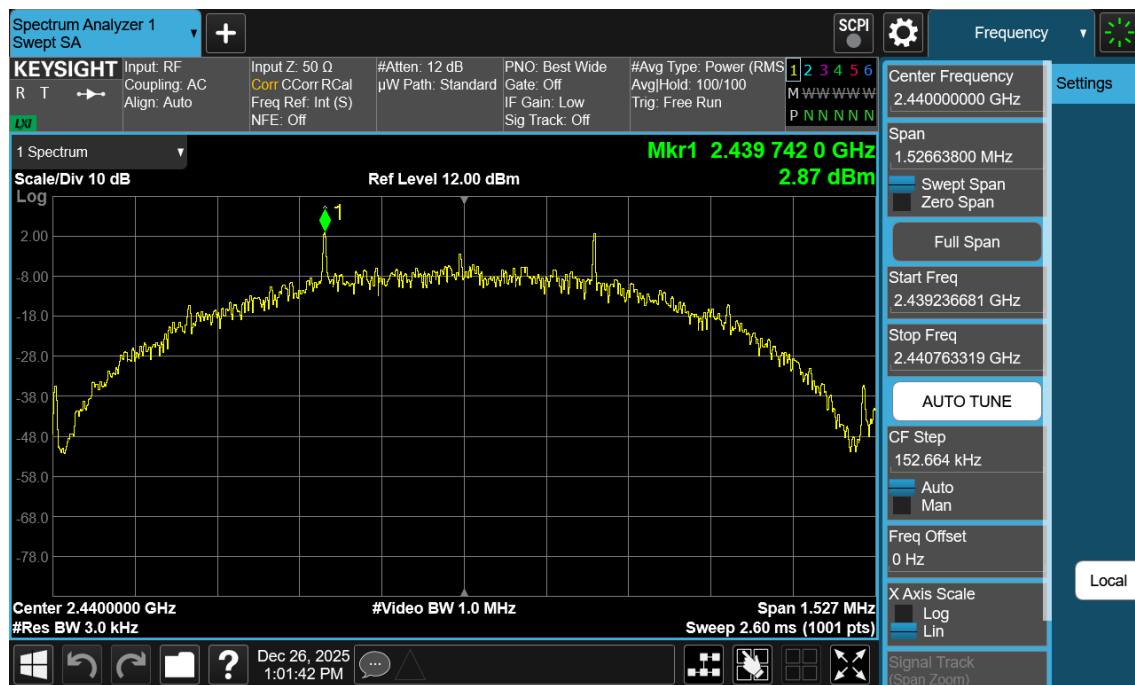
Plot 7-118. Power Spectral Density Plot Antenna WF2b (Bluetooth (LE), 500kbps, iPA – Ch. 19)
