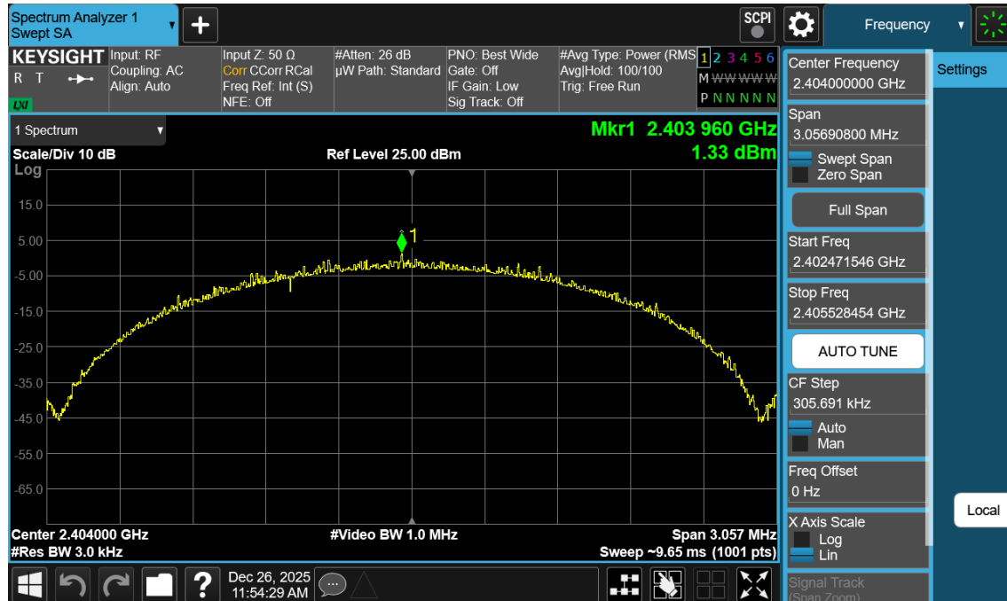
Plot 7-133. Power Spectral Density Plot Antenna WF7b (Bluetooth (LE), 2Mbps, ePA – Ch. 1)
