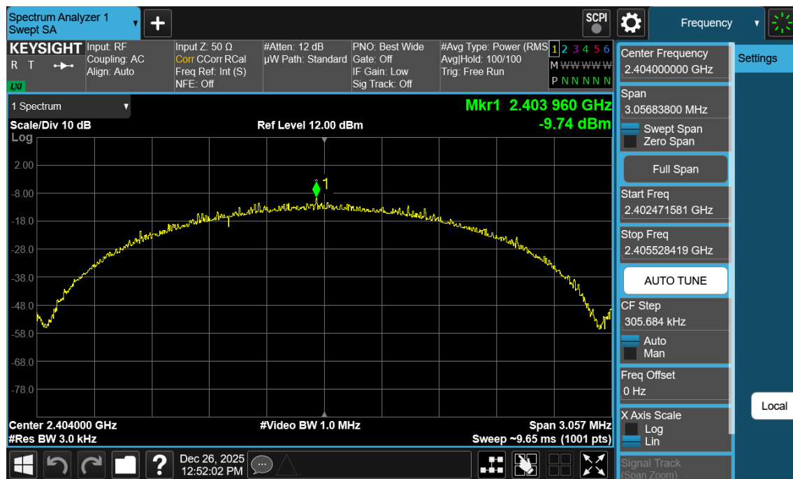
Plot 7-140. Power Spectral Density Plot Antenna WF2b (Bluetooth (LE), 2Mbps, iPA – Ch. 1)
