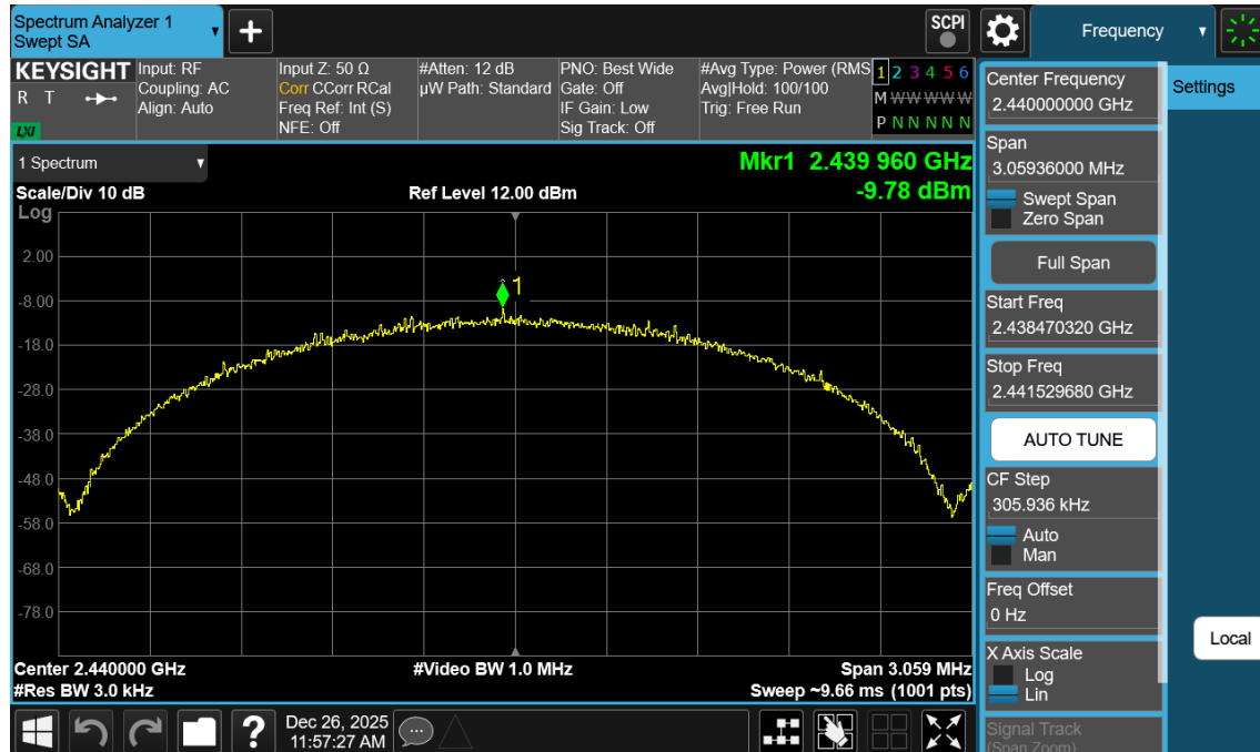
Plot 7-141. Power Spectral Density Plot Antenna WF7b (Bluetooth (LE), 2Mbps, iPA – Ch. 19)
