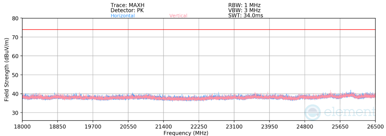
Plot 7-175. Radiated Spurious Emissions Above 18GHz TxBF (1Mbps ePA – Ch. 39)
