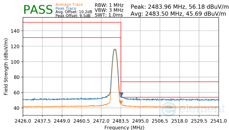
Plot 7-182. Radiated Restricted Upper Band Edge Measurement Antenna WF2b (Average & Peak)
