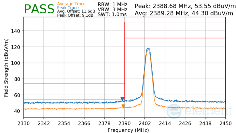
Plot 7-179. Radiated Restricted Lower Band Edge Measurement Antenna WF7b (Average & Peak)
