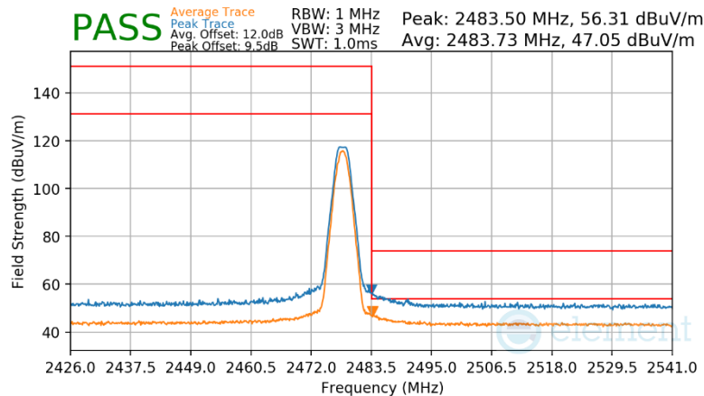
Plot 7-180. Radiated Restricted Upper Band Edge Measurement Antenna WF7b (Average & Peak)
