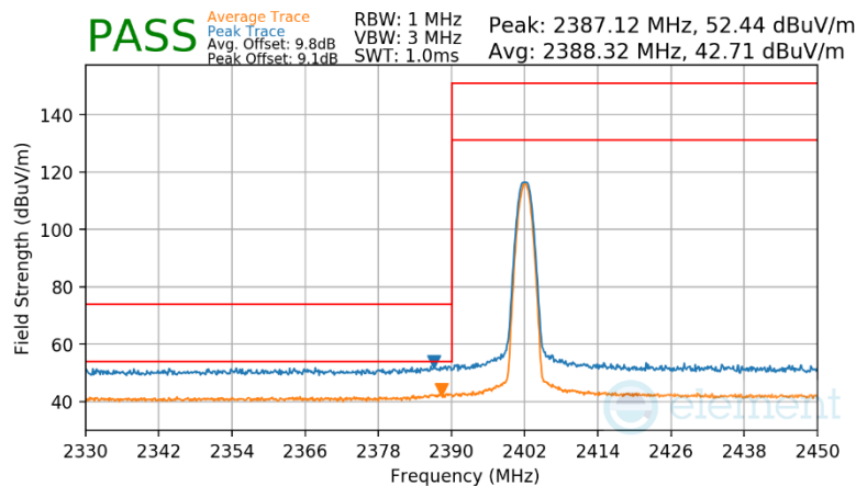
Plot 7-181. Radiated Restricted Lower Band Edge Measurement Antenna WF2b (Average & Peak)
