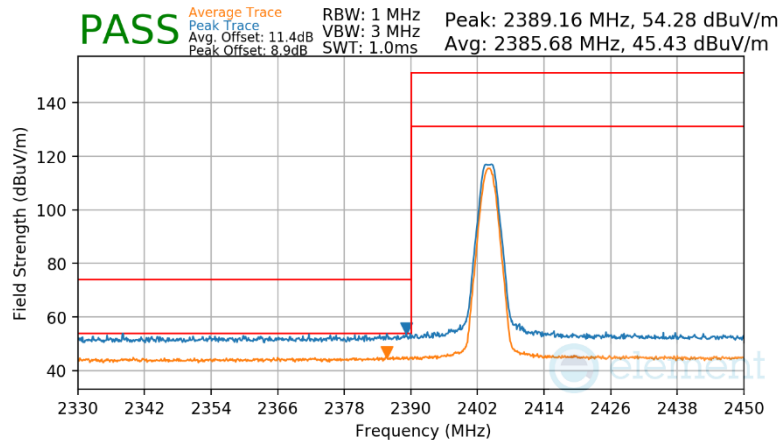
Plot 7-183. Radiated Restricted Lower Band Edge Measurement Antenna WF2b (Average & Peak)
