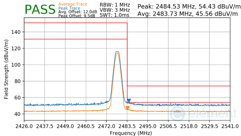
Plot 7-184. Radiated Restricted Upper Band Edge Measurement Antenna WF2b (Average & Peak)
