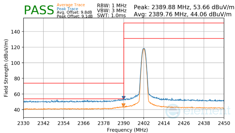
Plot 7-177. Radiated Restricted Lower Band Edge Measurement Antenna WF7b (Average & Peak)
