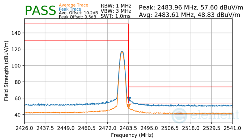
Plot 7-178. Radiated Restricted Upper Band Edge Measurement Antenna WF7b (Average & Peak)
