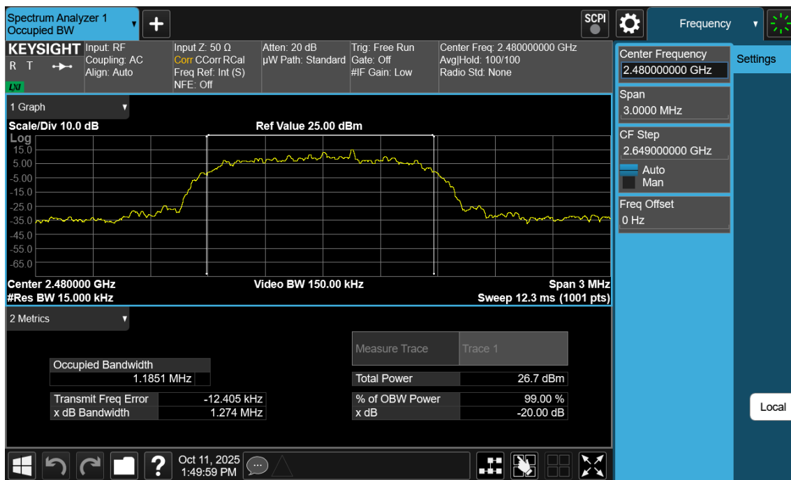
Plot 7-6. 20dB BW and 99% OBW Plot Antenna WF7b (Bluetooth, 8DPSK, ePA – Ch. 78)
