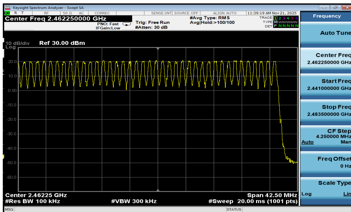
Plot 7-42. High End Spectrum Channel Hopping Plot Antenna WF2b (Bluetooth, GFSK, ePA)
