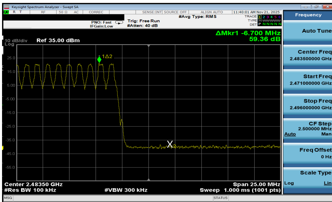
Plot 7-24. Band Edge Plot Antenna WF2b (Bluetooth with Hopping Enabled, GFSK, ePA)
