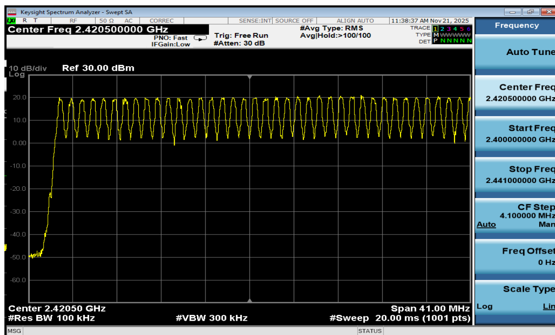
Plot 7-41. Low End Spectrum Channel Hopping Plot Antenna WF2b (Bluetooth, GFSK, ePA)
