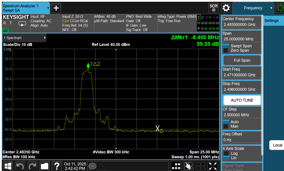
Plot 7-18. Band Edge Plot Antenna WF7b (Bluetooth with Hopping Disabled, 8DPSK, ePA – Ch. 78)
