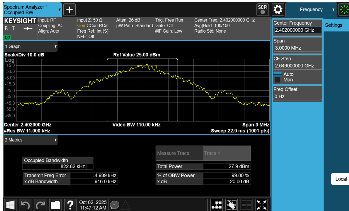
Plot 7-1. 20dB BW and 99% OBW Plot Antenna WF7b (Bluetooth, GFSK, ePA – Ch. 0)
