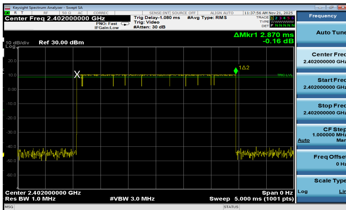
Plot 7-35. Time of Occupancy Plot Antenna WF2b (Bluetooth, GFSK, ePA)
