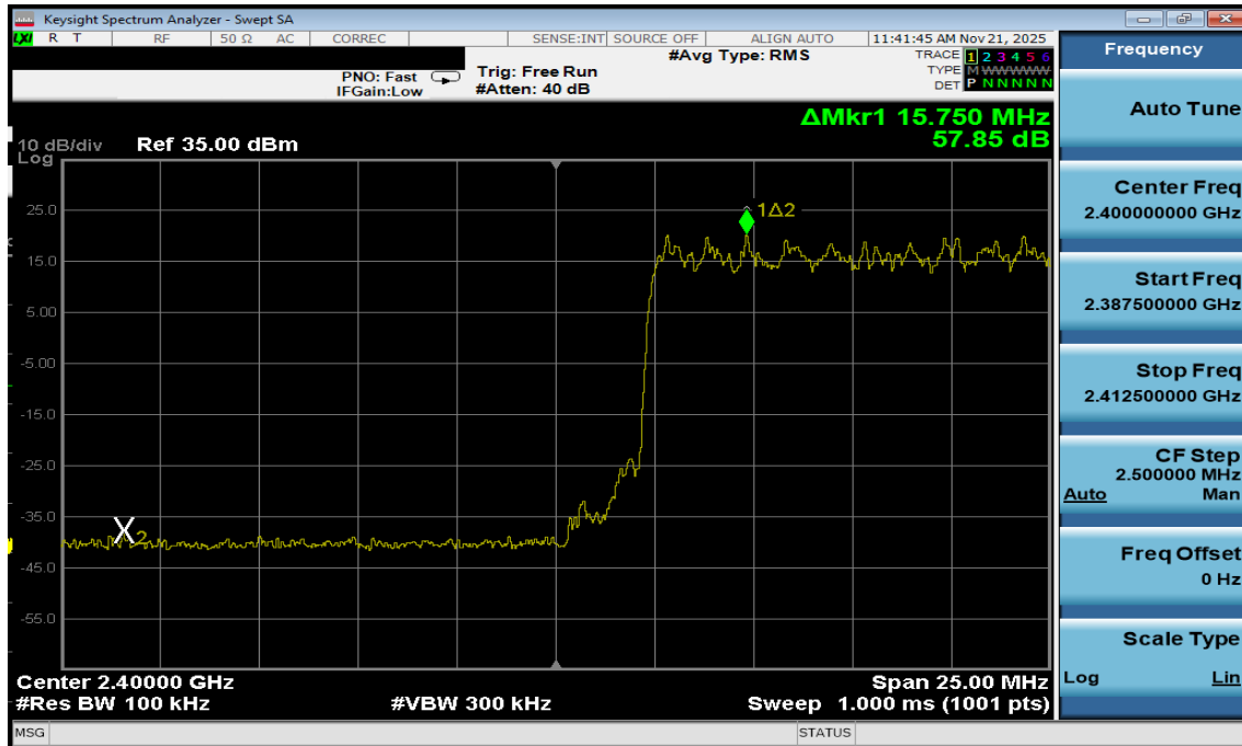
Plot 7-27. Band Edge Plot Antenna WF2b (Bluetooth with Hopping Enabled, 8DPSK, ePA)
