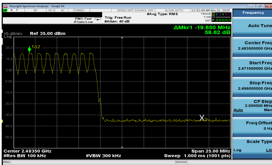
Plot 7-16. Band Edge Plot Antenna WF7b (Bluetooth with Hopping Enabled, GFSK, ePA)
