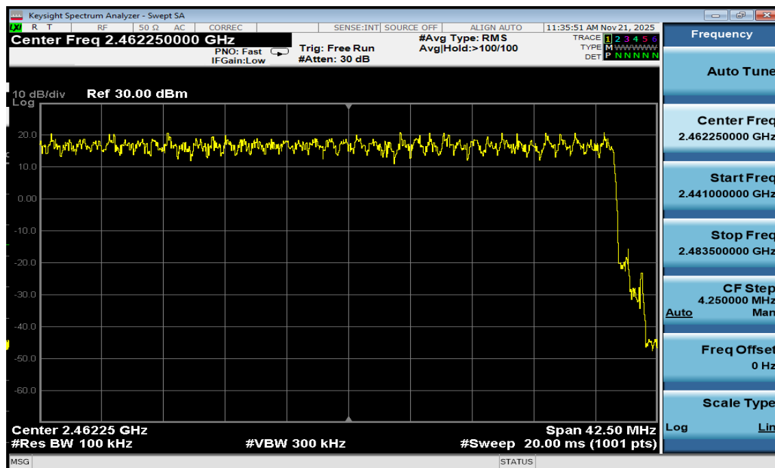
Plot 7-40. High End Spectrum Channel Hopping Plot Antenna WF7b (Bluetooth, 8DPSK, ePA)
