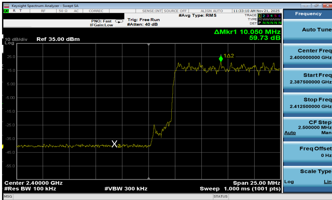
Plot 7-19. Band Edge Plot Antenna WF7b (Bluetooth with Hopping Enabled, 8DPSK, ePA)
