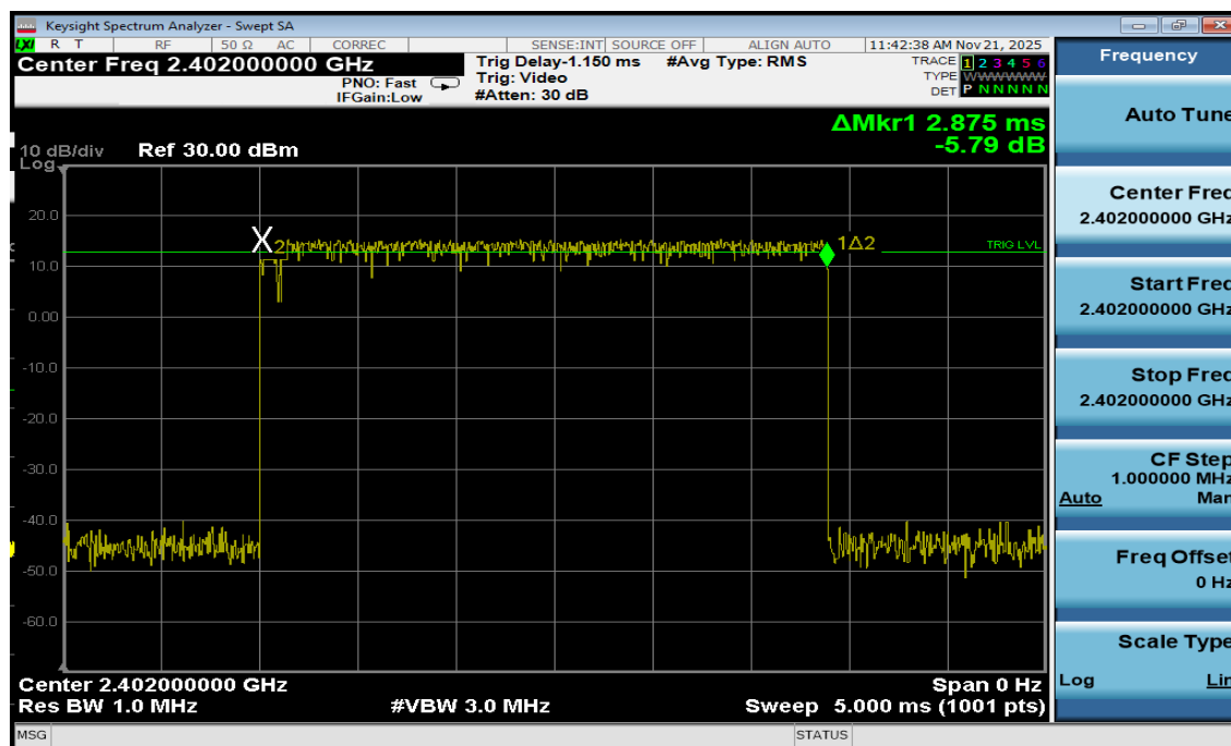
Plot 7-36. Time of Occupancy Plot Antenna WF2b (Bluetooth, 8DPSK, ePA)
