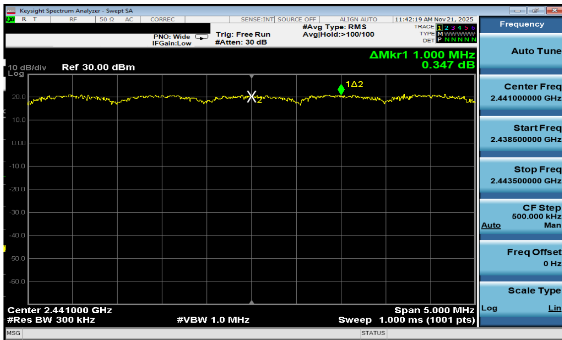
Plot 7-32. Channel Spacing Plot Antenna WF2b (Bluetooth, 8DPSK, ePA)
