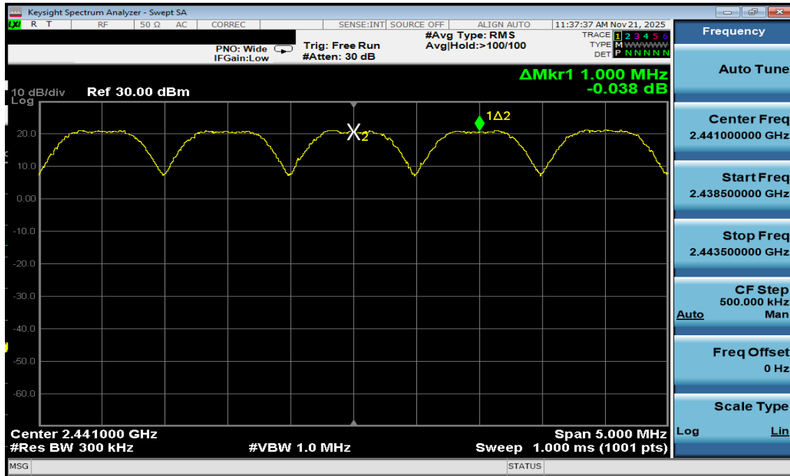
Plot 7-31. Channel Spacing Plot Antenna WF2b (Bluetooth, GFSK, ePA)
