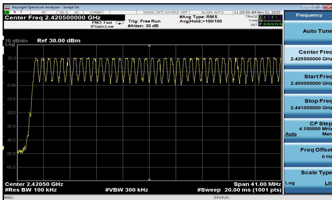
Plot 7-37. Low End Spectrum Channel Hopping Plot Antenna WF7b (Bluetooth, GFSK, ePA)
