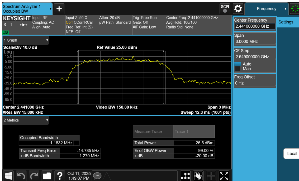
Plot 7-5. 20dB BW and 99% OBW Plot Antenna WF7b (Bluetooth, 8DPSK, ePA – Ch. 39)
