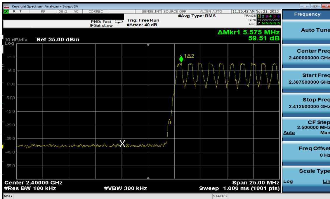
Plot 7-15. Band Edge Plot Antenna WF7b (Bluetooth with Hopping Enabled, GFSK, ePA)
