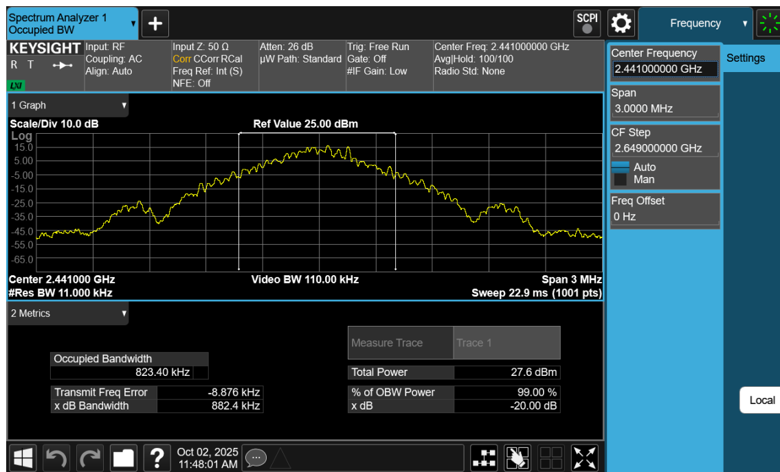
Plot 7-2. 20dB BW and 99% OBW Plot Antenna WF7b (Bluetooth, GFSK, ePA – Ch. 39)
