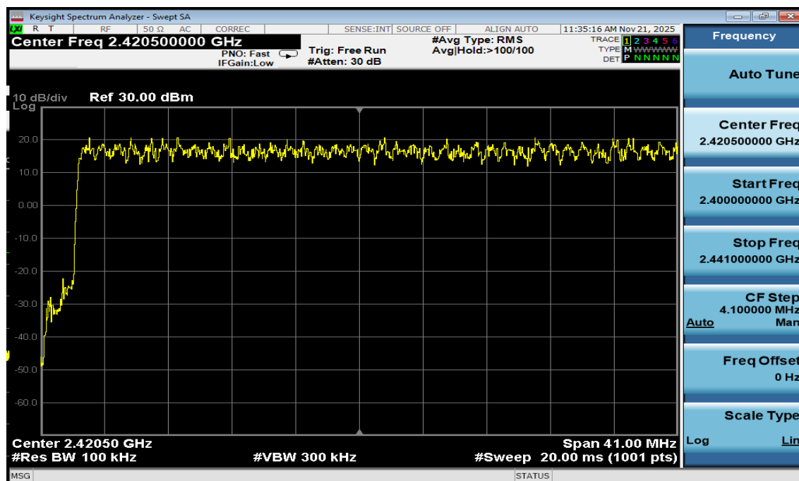
Plot 7-39. Low End Spectrum Channel Hopping Plot Antenna WF7b (Bluetooth, 8DPSK, ePA)
