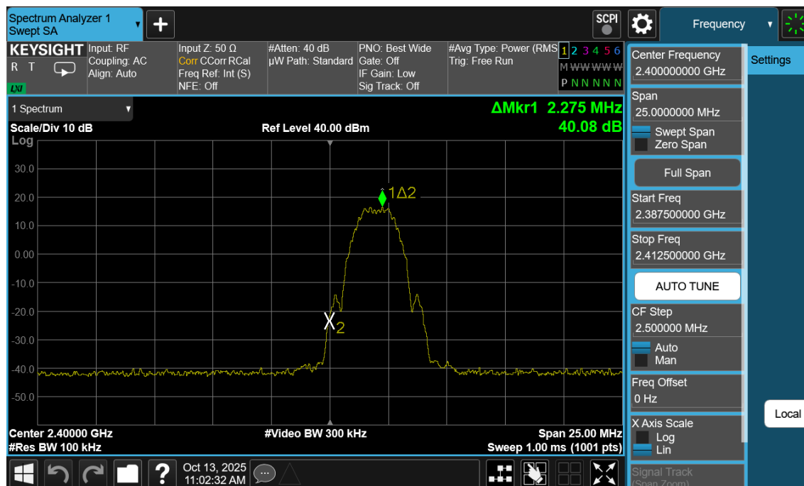
Plot 7-25. Band Edge Plot Antenna WF2b (Bluetooth with Hopping Disabled, 8DPSK, ePA – Ch. 0)
