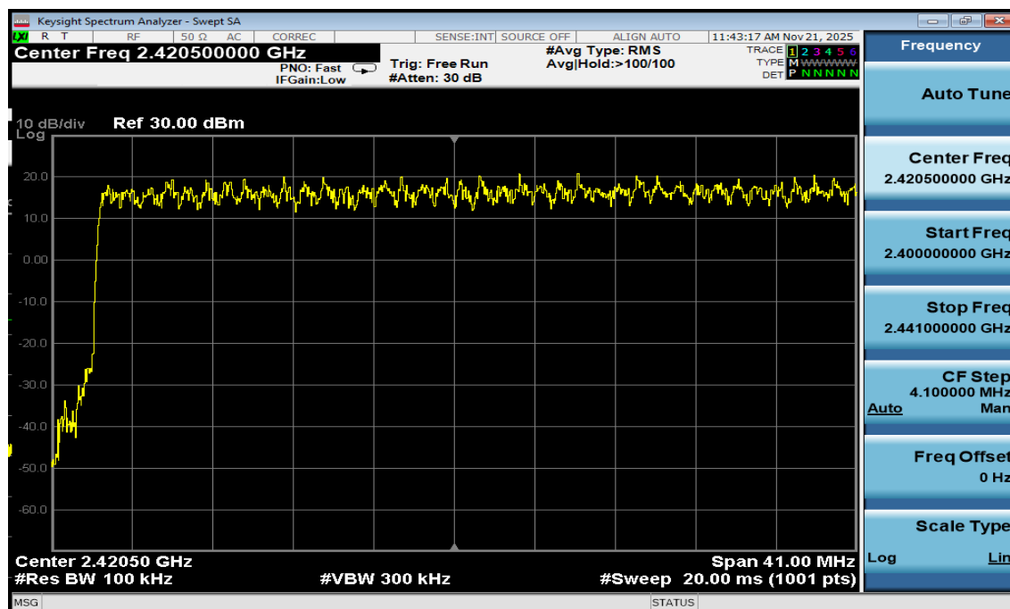
Plot 7-43. Low End Spectrum Channel Hopping Plot Antenna WF2b (Bluetooth, 8DPSK, ePA)
