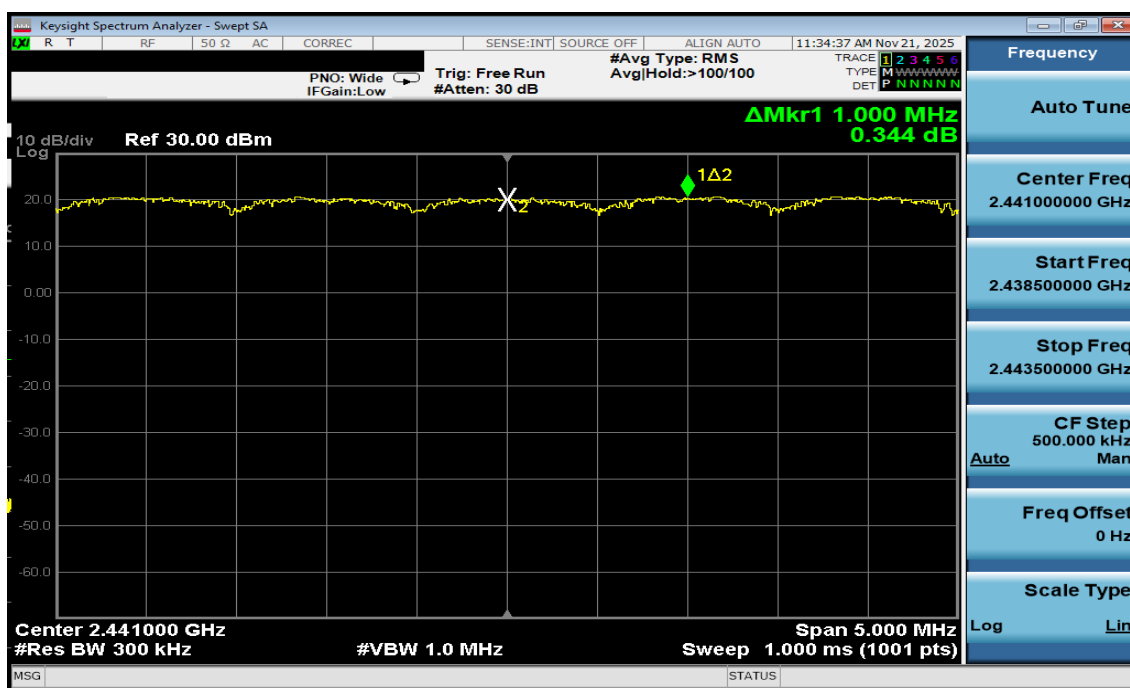
Plot 7-30. Channel Spacing Plot Antenna WF7b (Bluetooth, 8DPSK, ePA)
