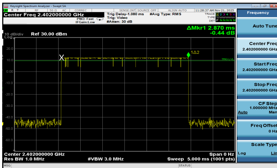
Plot 7-33. Time of Occupancy Plot Antenna WF7b (Bluetooth, GFSK, ePA)
