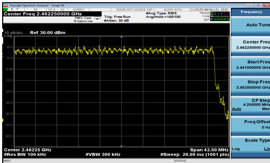
Plot 7-44. High End Spectrum Channel Hopping Plot Antenna WF2b (Bluetooth, 8DPSK, ePA)
