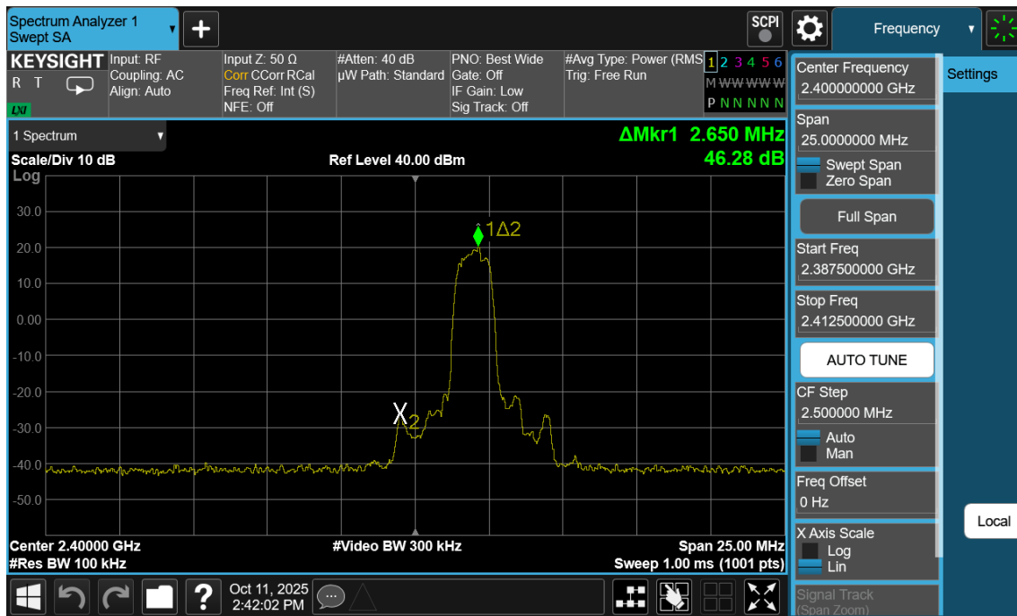
Plot 7-17. Band Edge Plot Antenna WF7b (Bluetooth with Hopping Disabled, 8DPSK, ePA – Ch. 0)
