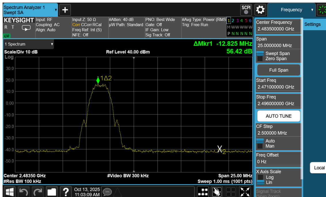
Plot 7-26. Band Edge Plot Antenna WF2b (Bluetooth with Hopping Disabled, 8DPSK, ePA – Ch. 78)
