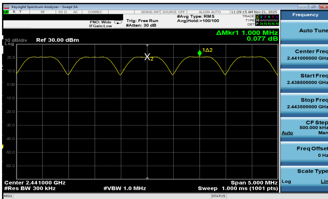
Plot 7-29. Channel Spacing Plot Antenna WF7b (Bluetooth, GFSK, ePA)
