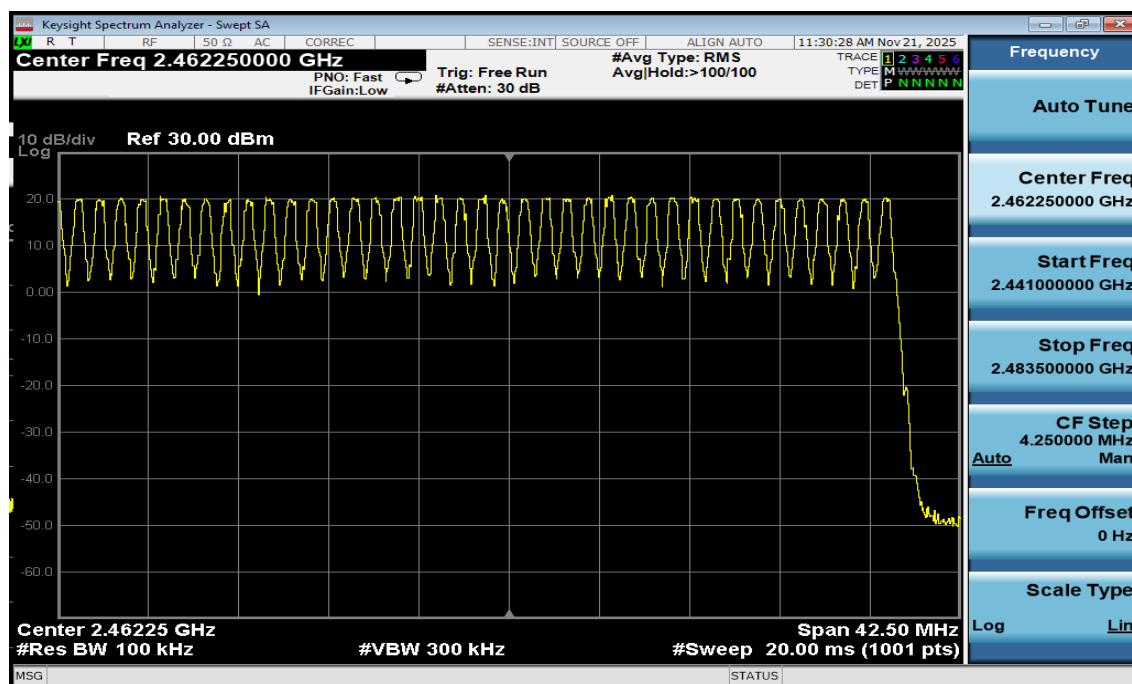
Plot 7-38. High End Spectrum Channel Hopping Plot Antenna WF7b (Bluetooth, GFSK, ePA)
