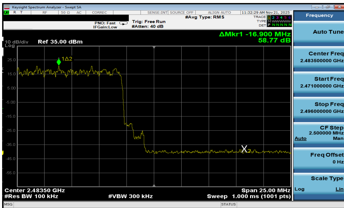
Plot 7-20. Band Edge Plot Antenna WF7b (Bluetooth with Hopping Enabled, 8DPSK, ePA)
