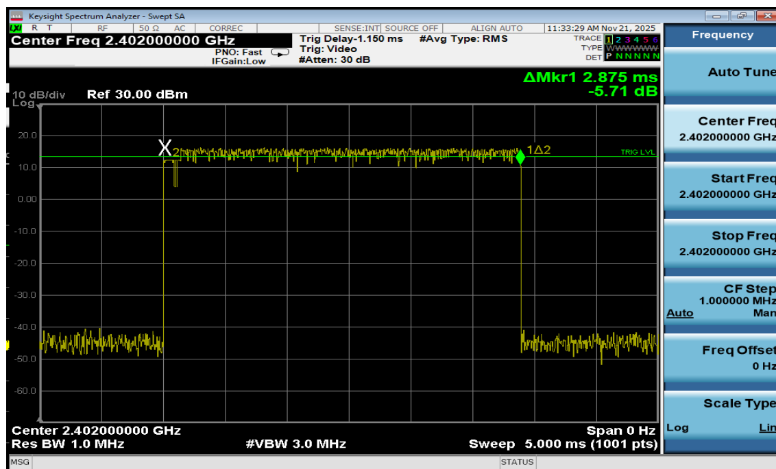
Plot 7-34. Time of Occupancy Plot Antenna WF7b (Bluetooth, 8DPSK, ePA)
