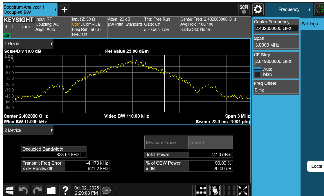
Plot 7-7. 20dB BW and 99% OBW Plot Antenna WF2b (Bluetooth, GFSK, ePA – Ch. 0)
