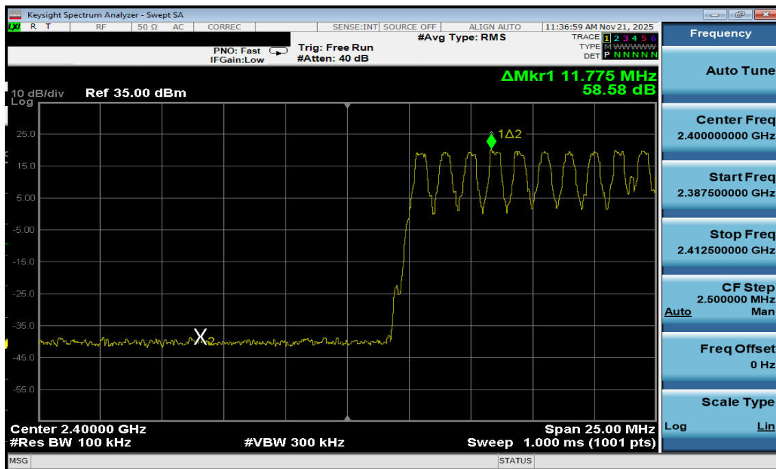
Plot 7-23. Band Edge Plot Antenna WF2b (Bluetooth with Hopping Enabled, GFSK, ePA)
