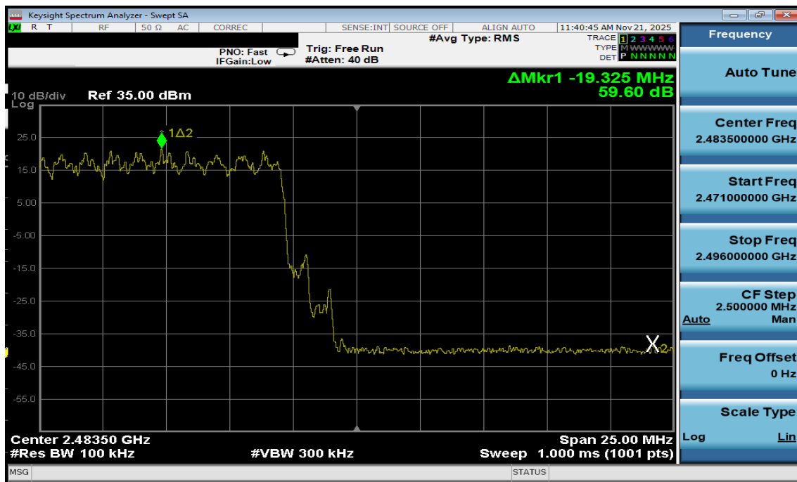
Plot 7-28. Band Edge Plot Antenna WF2b (Bluetooth with Hopping Enabled, 8DPSK, ePA)
