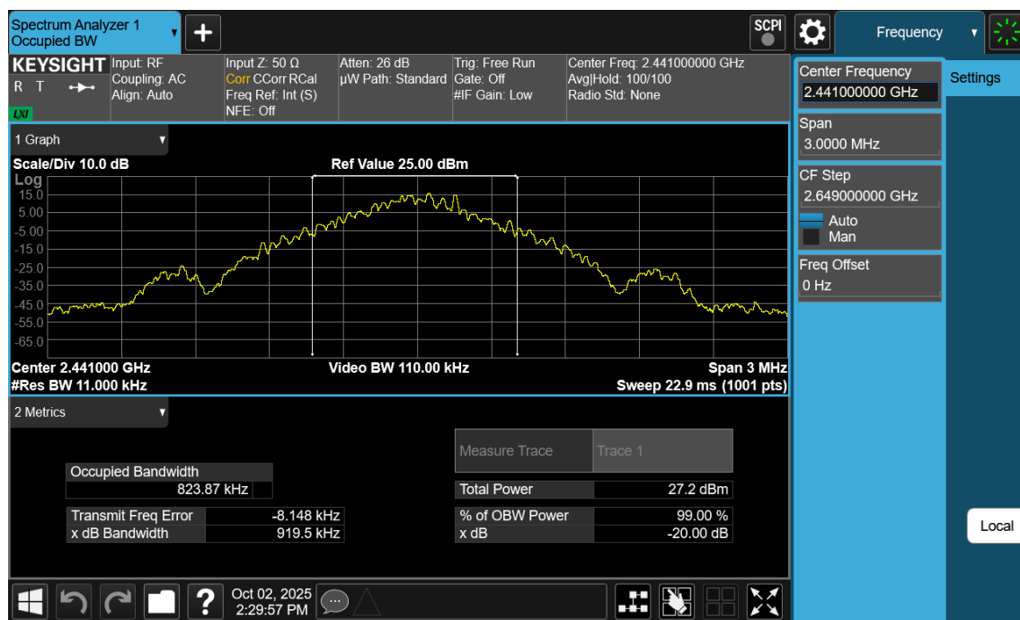
Plot 7-8. 20dB BW and 99% OBW Plot Antenna WF2b (Bluetooth, GFSK, ePA – Ch. 39)
