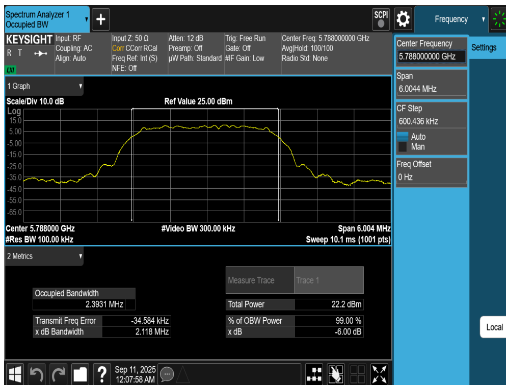
Plot 7-89. 6dB BW Antenna WF7a (NB UNII HDT2, ePA– 5788MHz)
