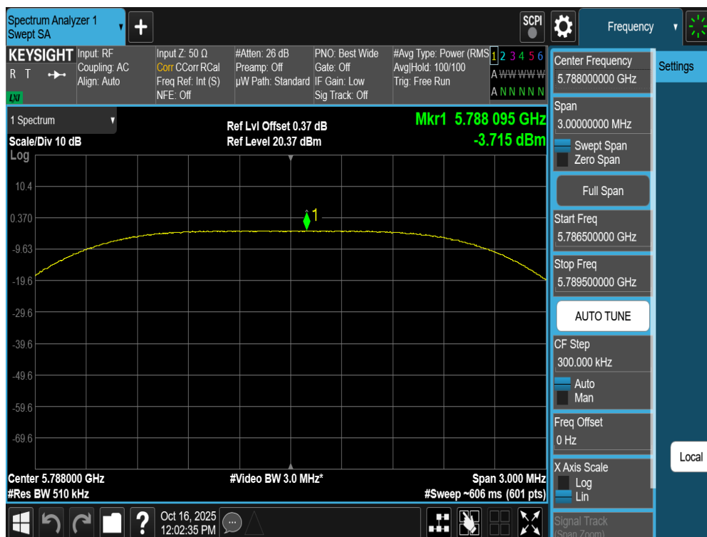
Plot 7-155. PSD Antenna WF7a (NB UNII HDRPS2, iPA – 5788MHz)
