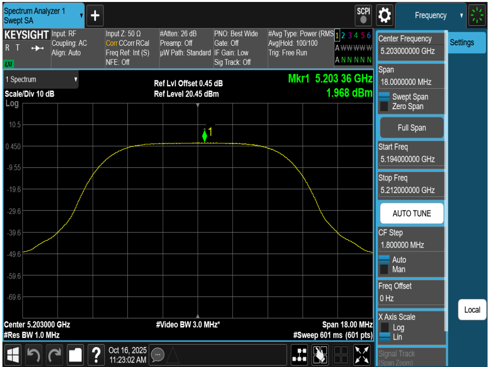
Plot 7-134. PSD Antenna WF7a (NB UNII HDRPL12, ePA – 5203MHz)
