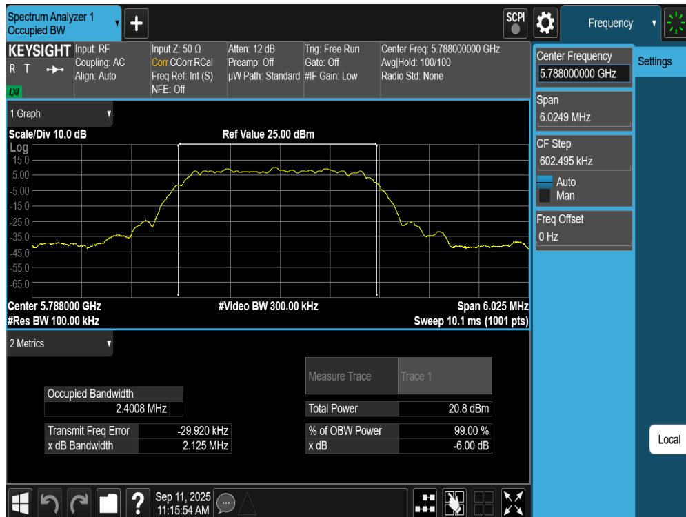
Plot 7-103. 6dB BW Antenna WF2a (NB UNII HDT4, ePA- 5788MHz)
