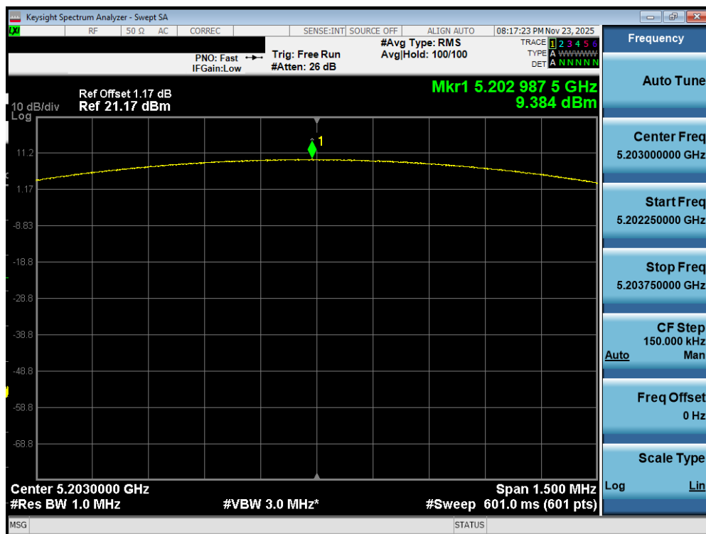
Plot 7-170. PSD Antenna WF2a (NB UNII BDR, ePA – 5203MHz)
