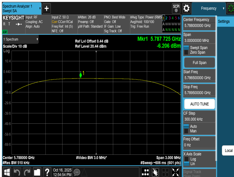
Plot 7-169. PSD Antenna WF7a (NB UNII HDT6, iPA – 5788MHz)
