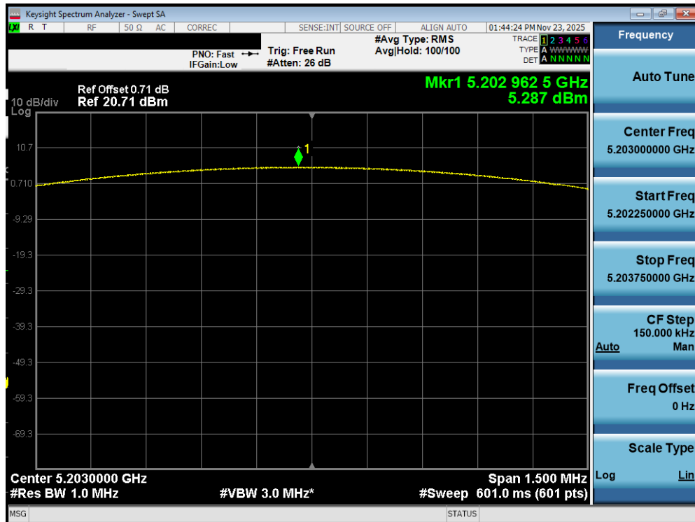
Plot 7-121. PSD Antenna WF7a (NB UNII LE1M, iPA – 5203MHz)
