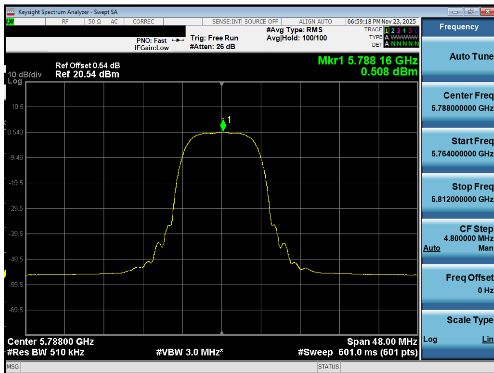
Plot 7-162. PSD Antenna WF7a (NB UNII HDRPL32, ePA – 5788MHz)
