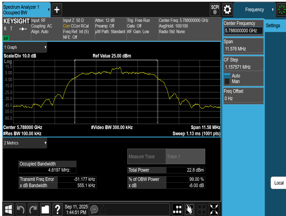
Plot 7-96. 6dB BW Antenna WF2a (NB UNII HDR8, ePA – 5788MHz)
