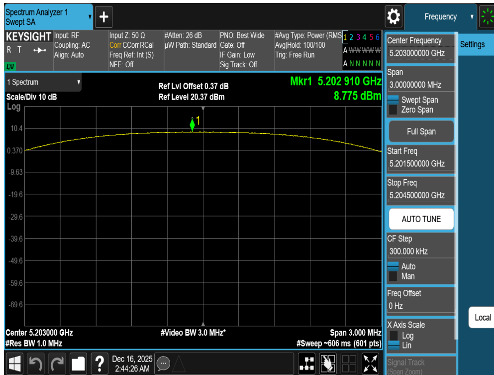
Plot 7-128. PSD Antenna WF7a (NB UNII HDRPS2, ePA – 5203MHz)
