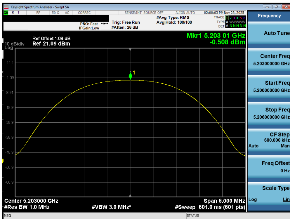
Plot 7-125. PSD Antenna WF7a (NB UNII HDR4, iPA – 5203MHz)
