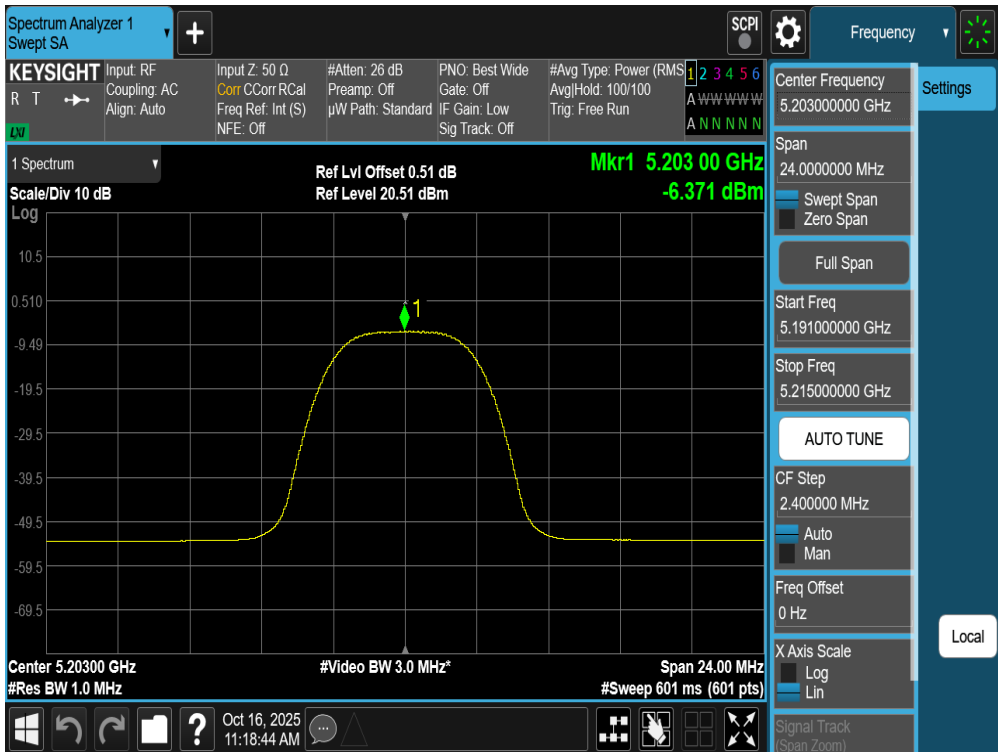
Plot 7-133. PSD Antenna WF7a (NB UNII HDRPM16, iPA – 5203MHz)
