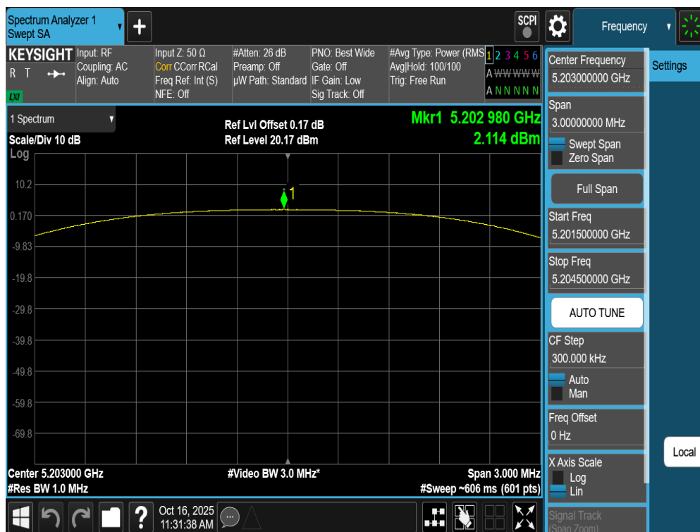
Plot 7-138. PSD Antenna WF7a (NB UNII HDT2, ePA – 5203MHz)
