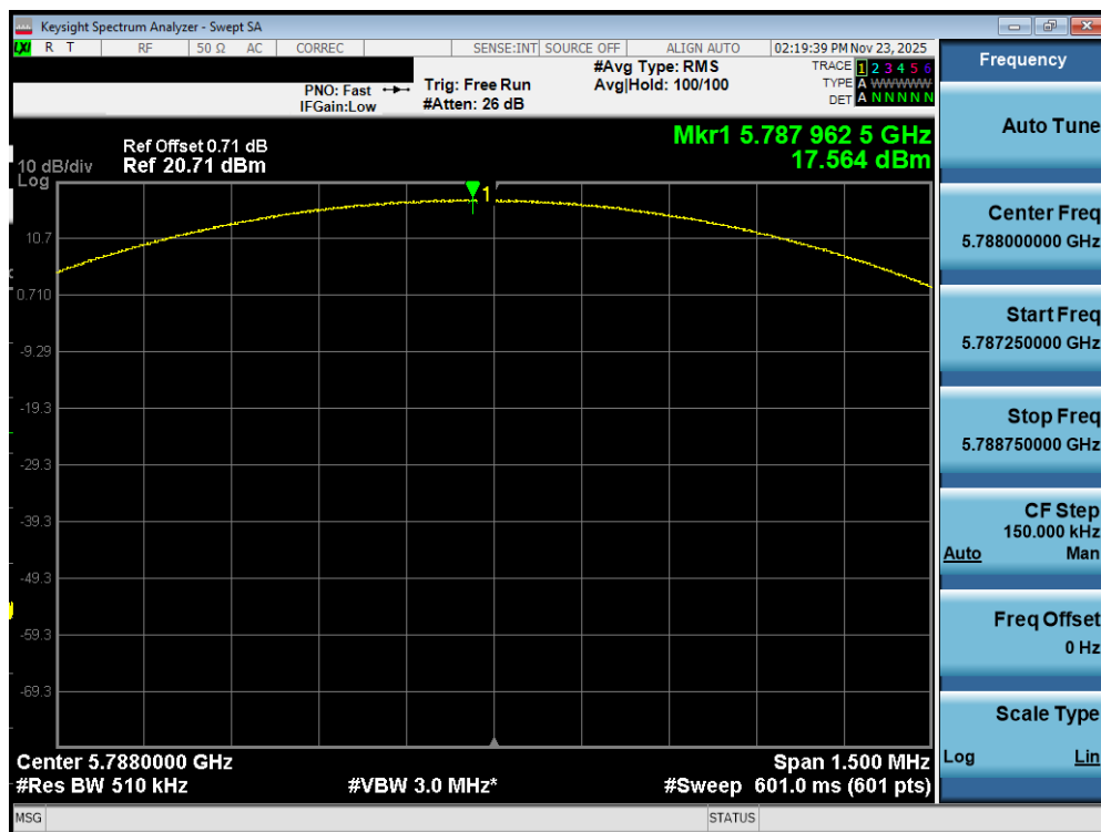
Plot 7-146. PSD Antenna WF7a (NB UNII LE1M, ePA – 5788MHz)
