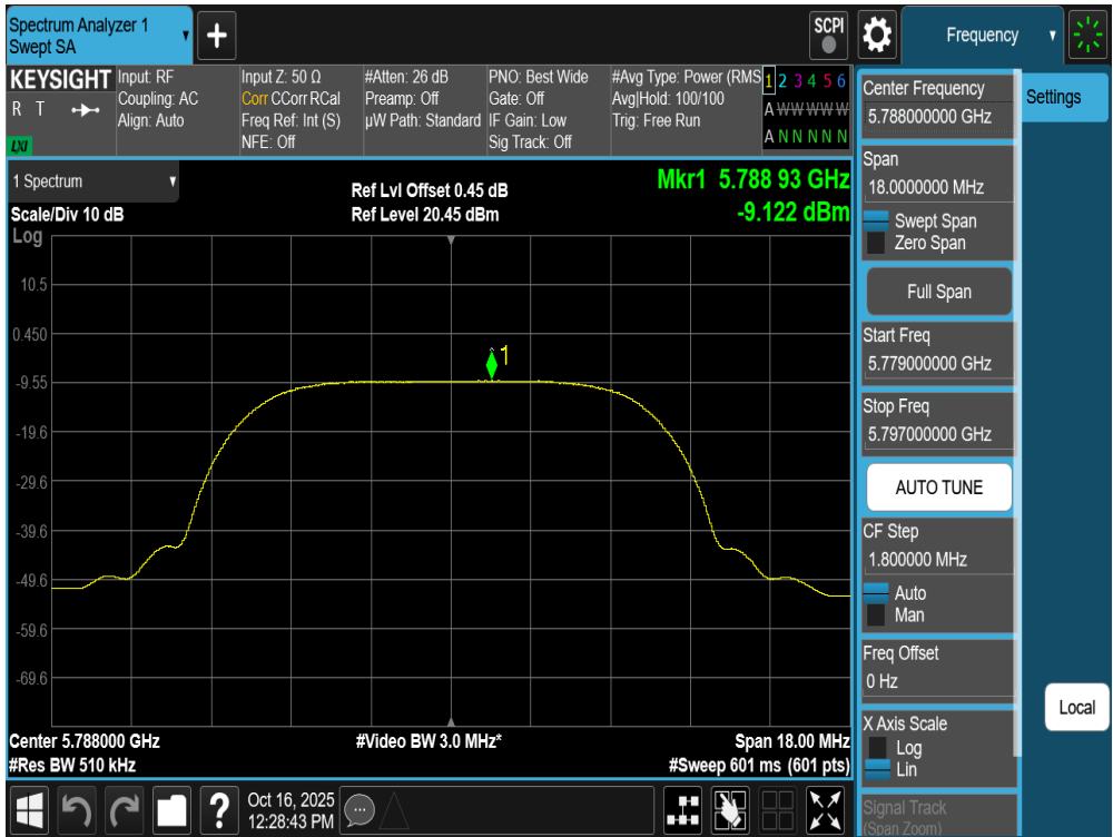
Plot 7-161. PSD Antenna WF7a (NB UNII HDRPL12, iPA – 5788MHz)
