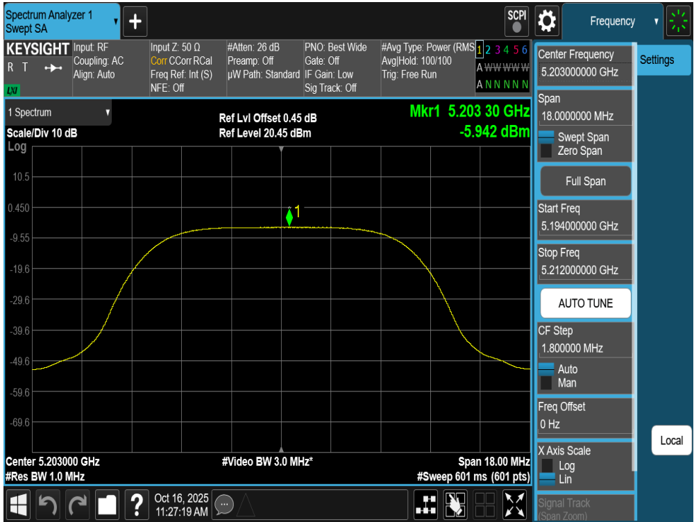
Plot 7-135. PSD Antenna WF7a (NB UNII HDRPL12, iPA – 5203MHz)
