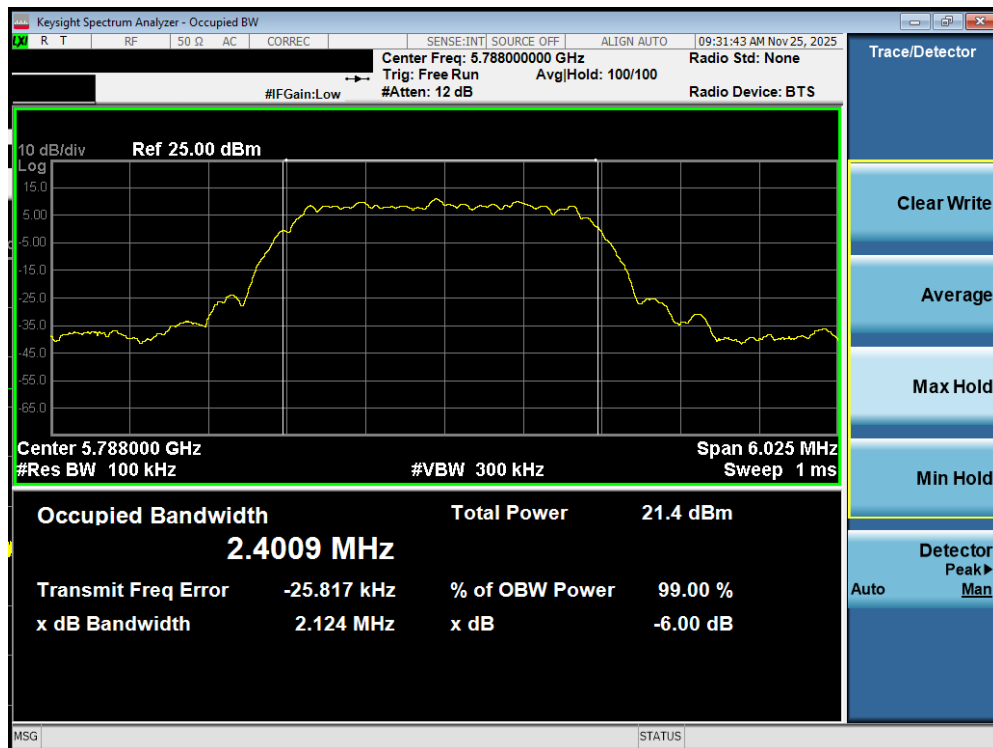
Plot 7-116. 6dB BW Antenna WF7b (NB UNII HDT4, ePA- 5788MHz)
