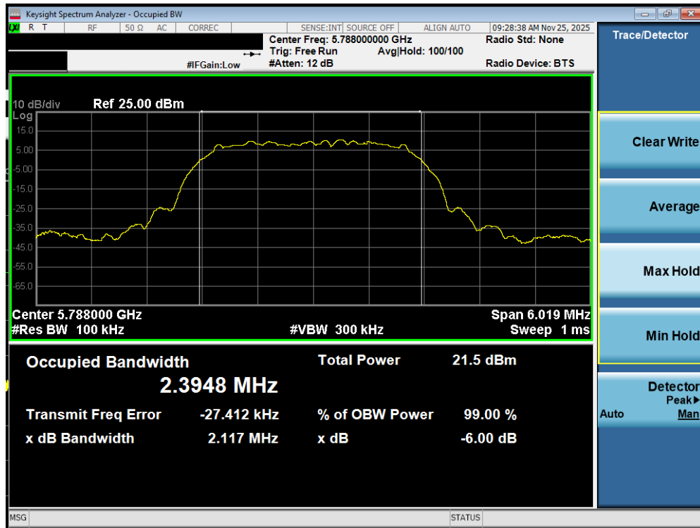
Plot 7-115. 6dB BW Antenna WF7b (NB UNII HDT2, ePA- 5788MHz)
