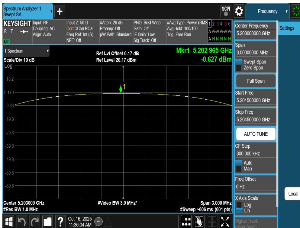
Plot 7-139. PSD Antenna WF7a (NB UNII HDT2, iPA – 5203MHz)
