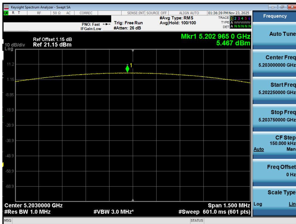
Plot 7-119. PSD Antenna WF7a (NB UNII BDR, iPA – 5203MHz)
