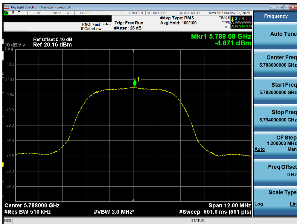
Plot 7-153. PSD Antenna WF7a (NB UNII HDR8, iPA – 5788MHz)
