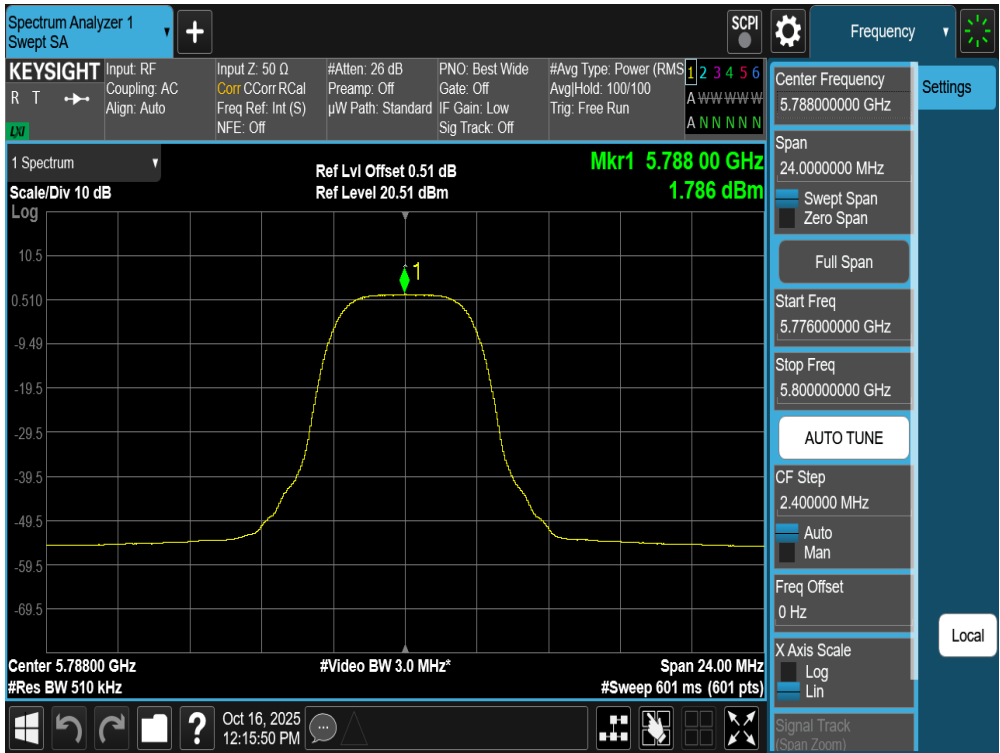
Plot 7-158. PSD Antenna WF7a (NB UNII HDRPM16, ePA – 5788MHz)
