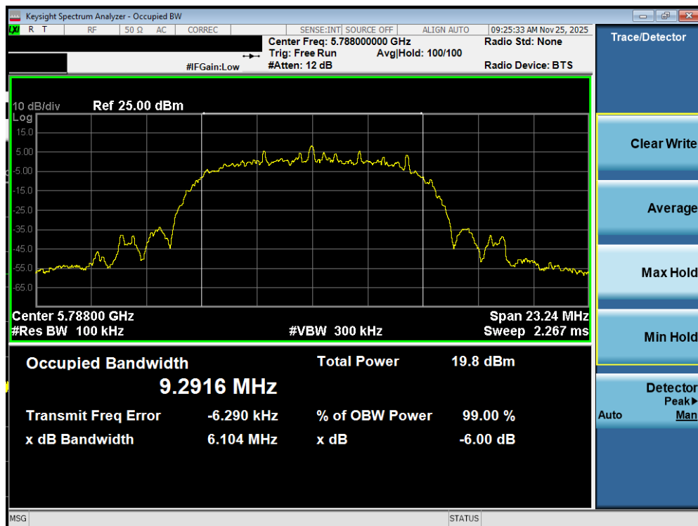
Plot 7-114. 6dB BW Antenna WF7b (NB UNII HDRPL32, ePA – 5788MHz)
