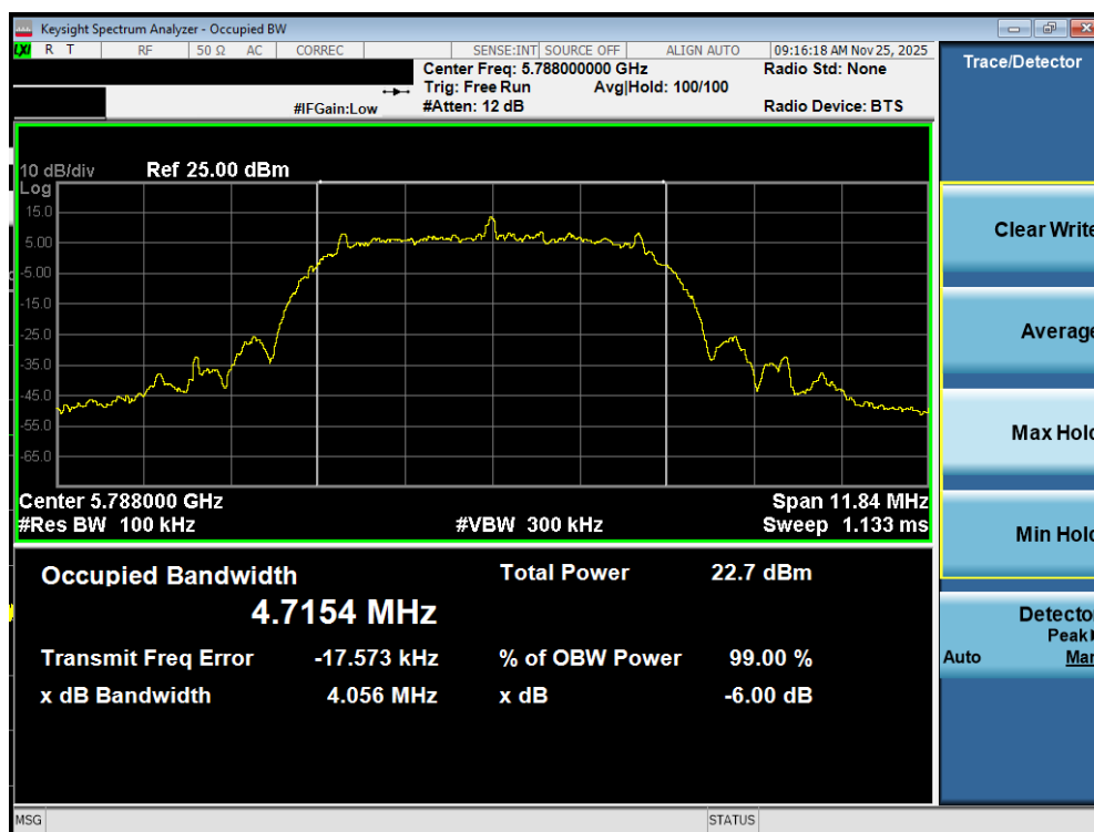
Plot 7-111. 6dB BW Antenna WF7b (NB UNII XHDRPM6, ePA – 5788MHz)
