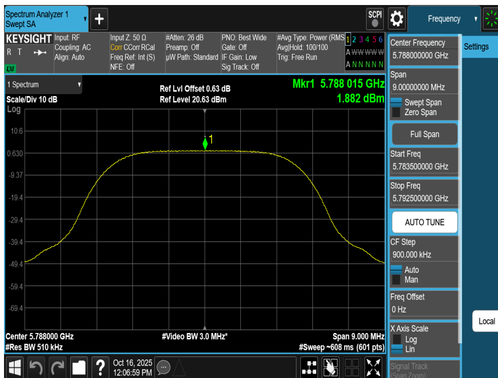
Plot 7-156. PSD Antenna WF7a (NB UNII XHDRPM6, ePA – 5788MHz)
