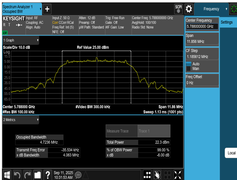
Plot 7-98. 6dB BW Antenna WF2a (NB UNII XHDRPM6, ePA – 5788MHz)
