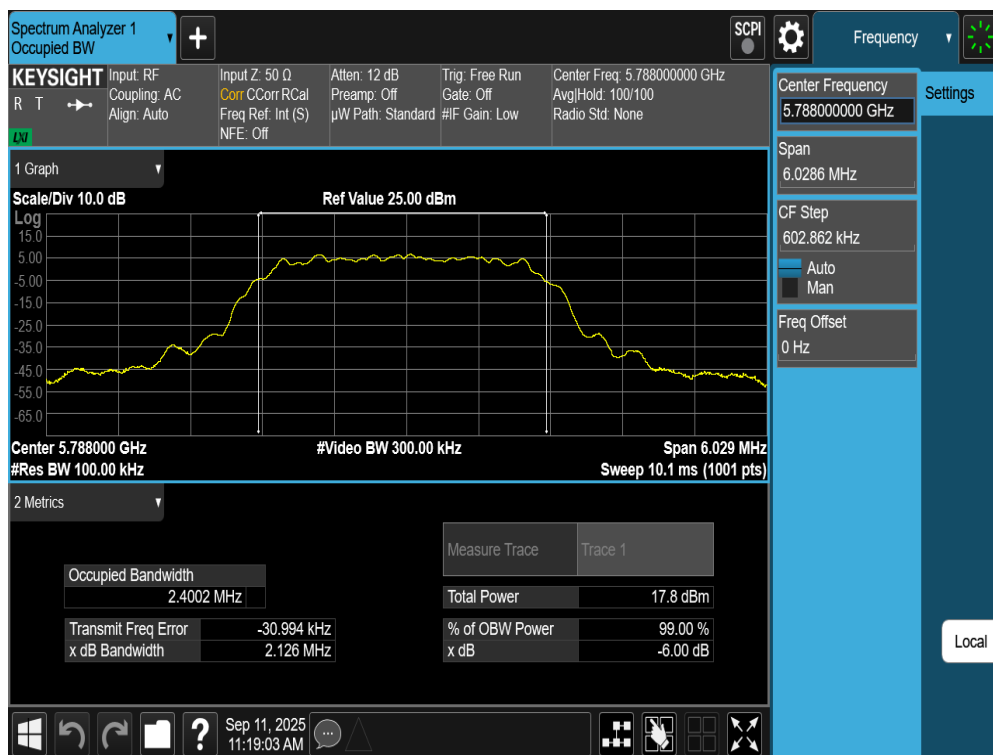
Plot 7-104. 6dB BW Antenna WF2a (NB UNII HDT6, ePA– 5788MHz)
