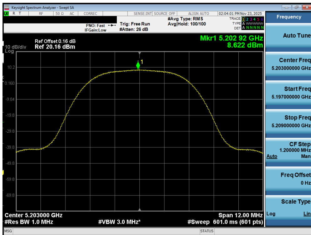
Plot 7-126. PSD Antenna WF7a (NB UNII HDR8, ePA – 5203MHz)
