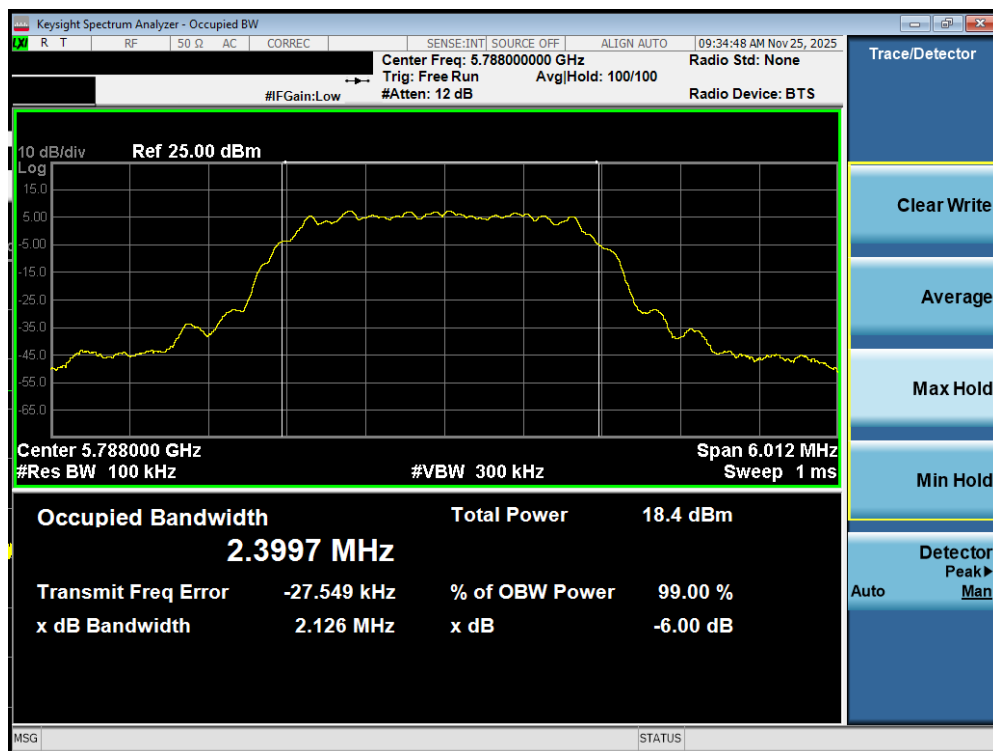
Plot 7-117. 6dB BW Antenna WF7b (NB UNII HDT6, ePA- 5788MHz)
