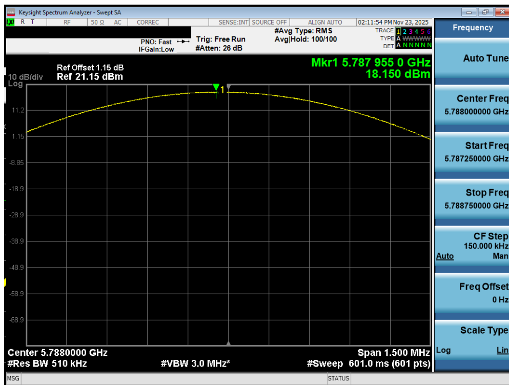
Plot 7-144. PSD Antenna WF7a (NB UNII BDR, ePA – 5788MHz)
