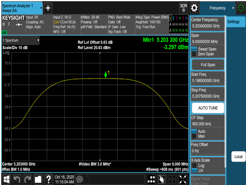
Plot 7-131. PSD Antenna WF7a (NB UNII XHDRPM6, iPA – 5203MHz)
