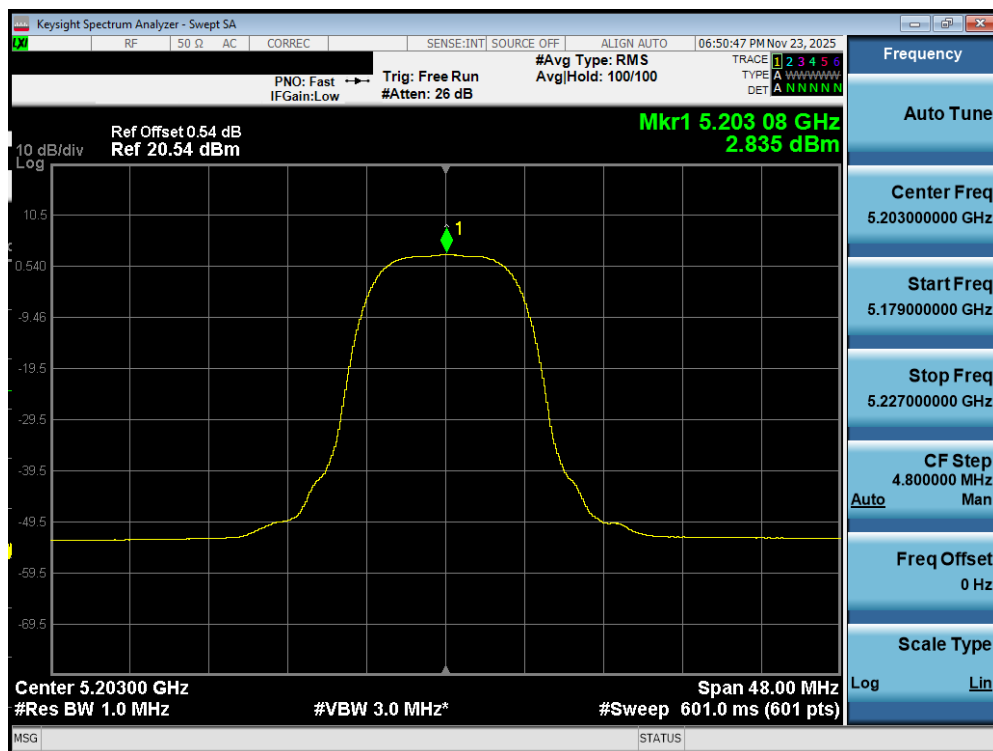
Plot 7-136. PSD Antenna WF7a (NB UNII HDRPL32, ePA – 5203MHz)
