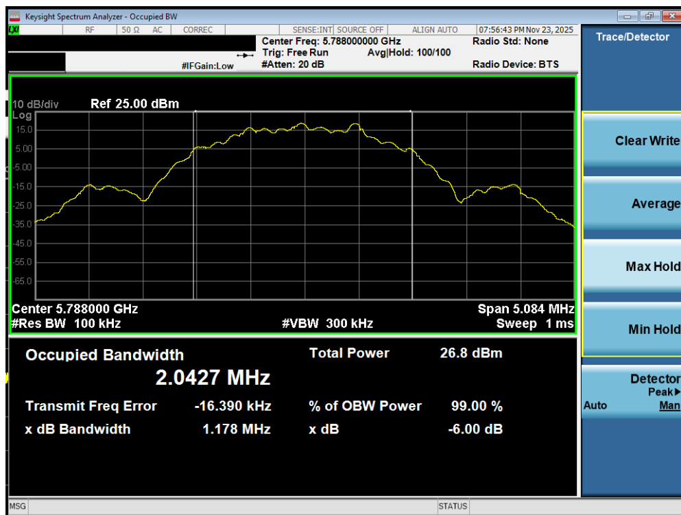
Plot 7-94. 6dB BW Antenna WF2a (NB UNII LE2M, ePA– 5788MHz)
