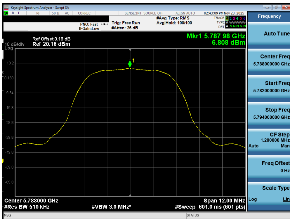
Plot 7-152. PSD Antenna WF7a (NB UNII HDR8, ePA – 5788MHz)
