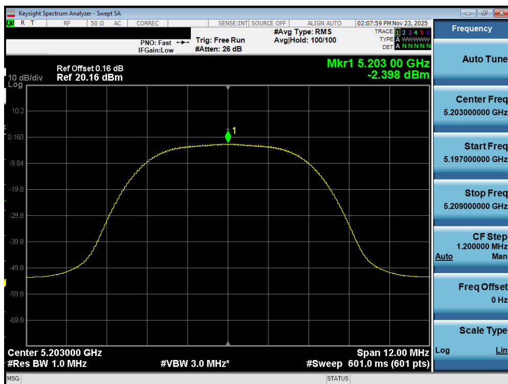
Plot 7-127. PSD Antenna WF7a (NB UNII HDR8, iPA – 5203MHz)
