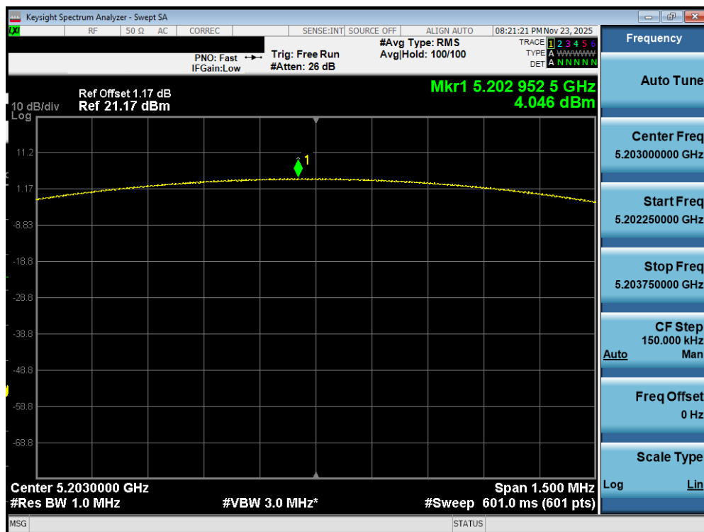
Plot 7-171. PSD Antenna WF2a (NB UNII BDR, iPA – 5203MHz)
