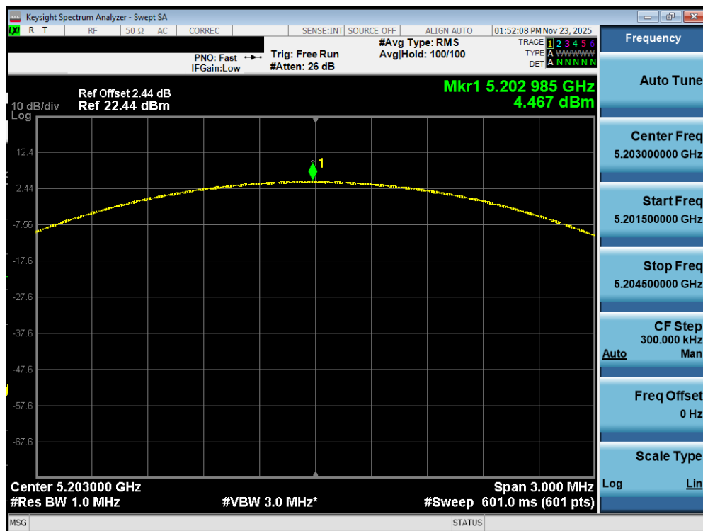
Plot 7-123. PSD Antenna WF7a (NB UNII LE2M, iPA – 5203MHz)
