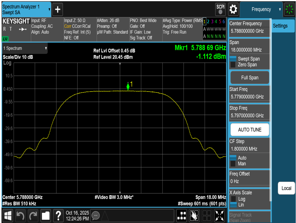
Plot 7-160. PSD Antenna WF7a (NB UNII HDRPL12, ePA – 5788MHz)
