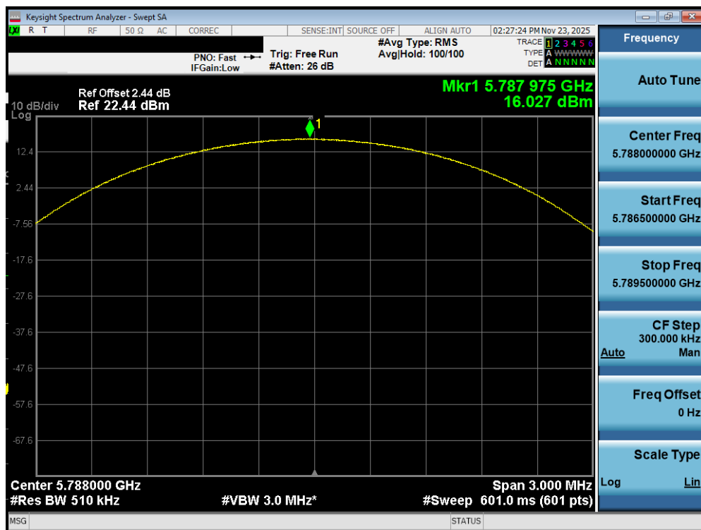
Plot 7-148. PSD Antenna WF7a (NB UNII LE2M, ePA - 5788MHz)
