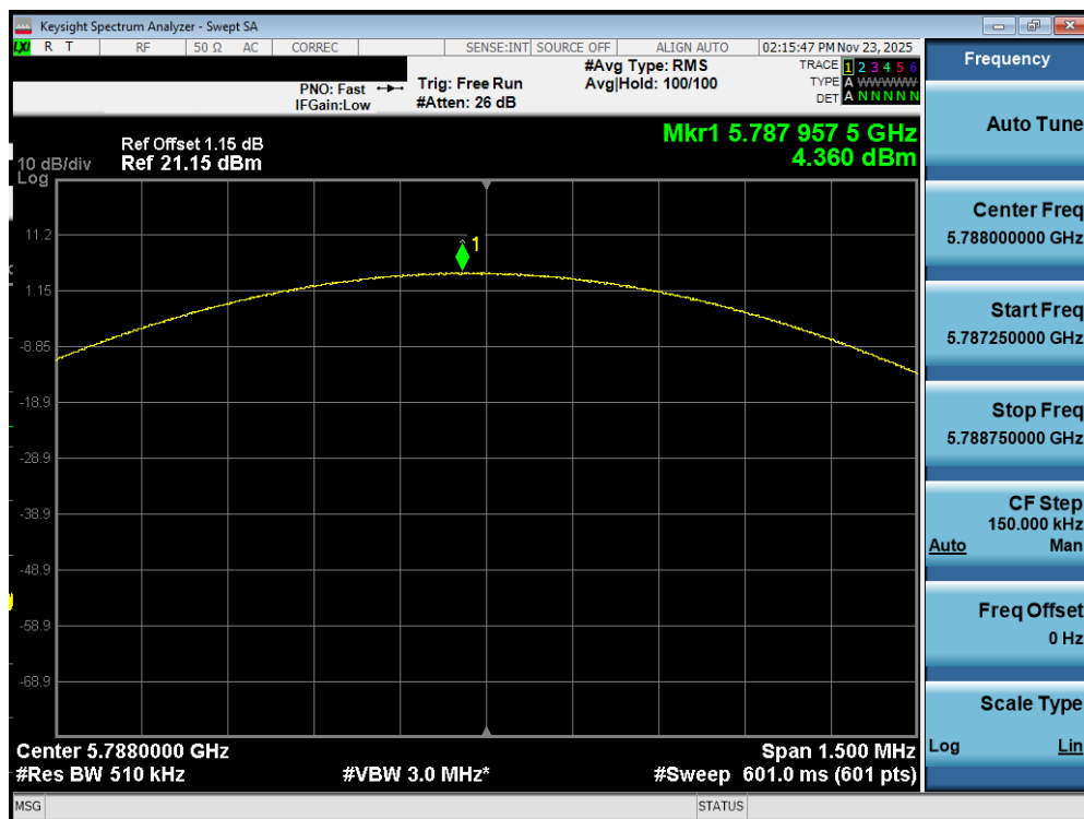
Plot 7-145. PSD Antenna WF7a (NB UNII BDR, iPA – 5788MHz)
