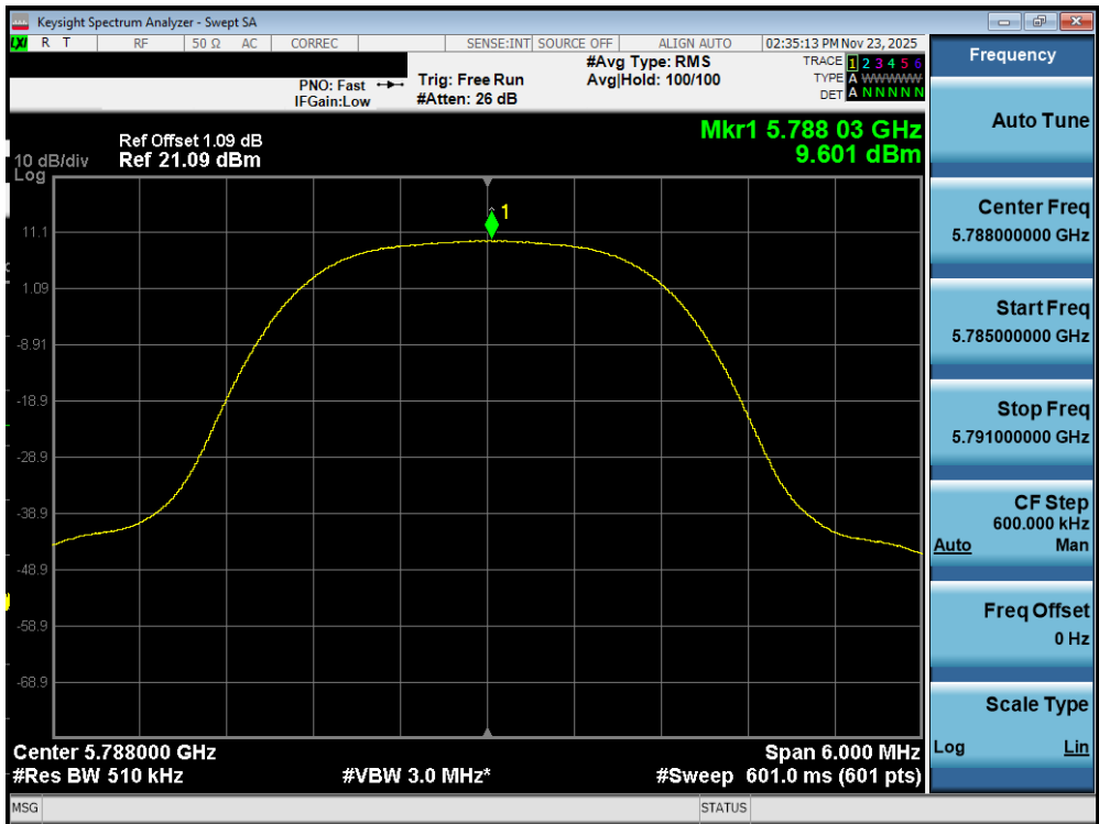
Plot 7-150. PSD Antenna WF7a (NB UNII HDR4, ePA - 5788MHz)
