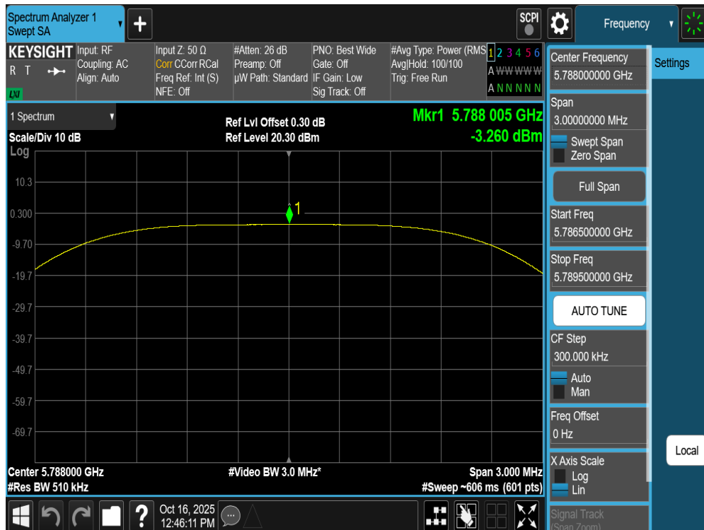
Plot 7-167. PSD Antenna WF7a (NB UNII HDT4, iPA – 5788MHz)
