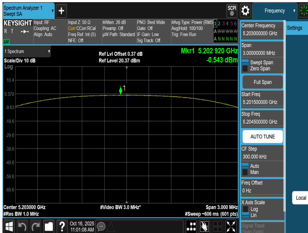
Plot 7-129. PSD Antenna WF7a (NB UNII HDRPS2, iPA – 5203MHz)
