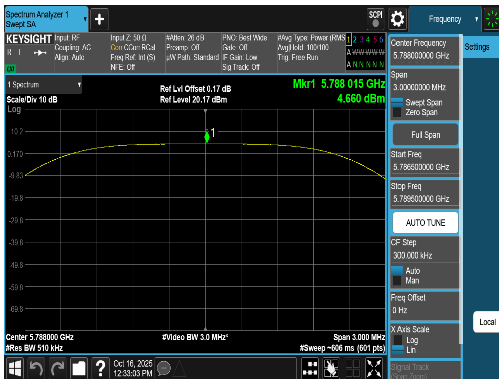
Plot 7-164. PSD Antenna WF7a (NB UNII HDT2, ePA – 5788MHz)
