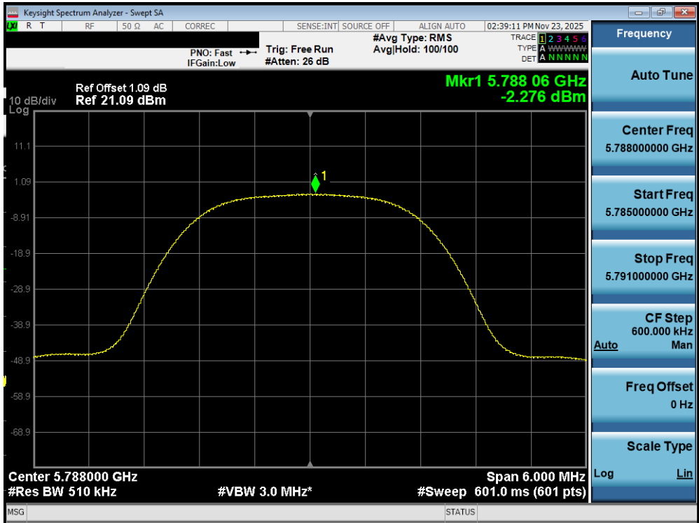
Plot 7-151. PSD Antenna WF7a (NB UNII HDR4, iPA - 5788MHz)
