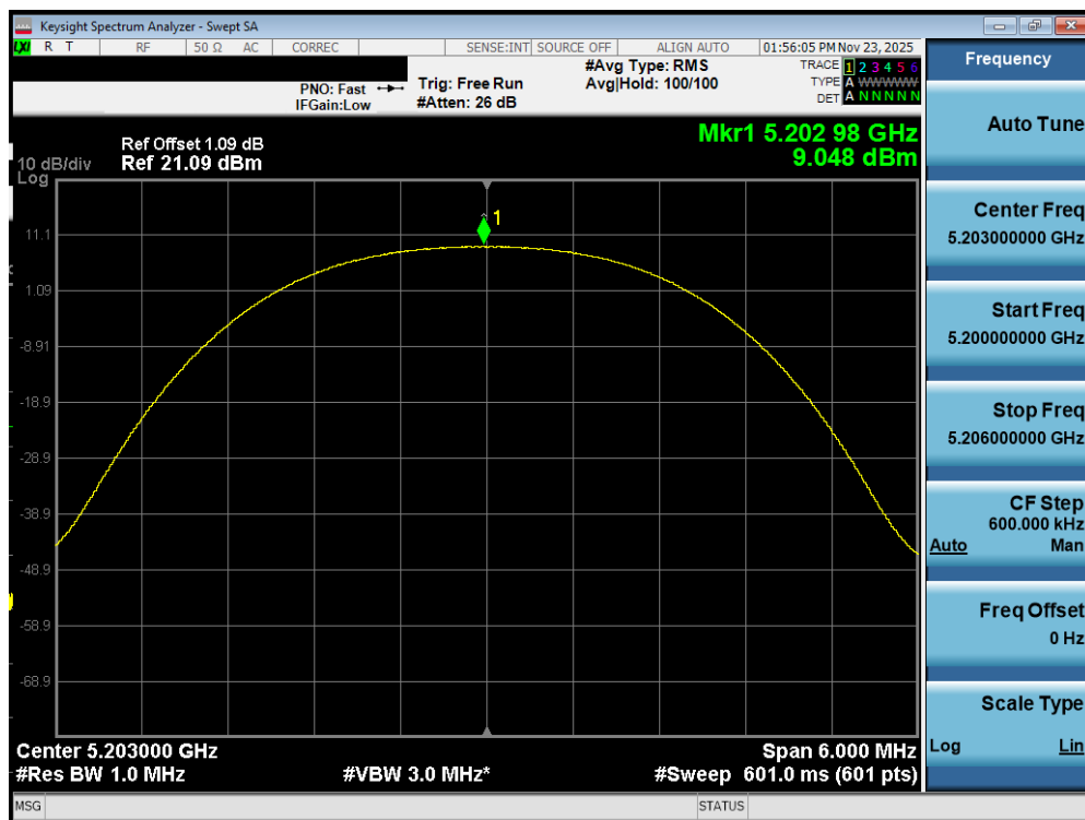
Plot 7-124. PSD Antenna WF7a (NB UNII HDR4, ePA – 5203MHz)
