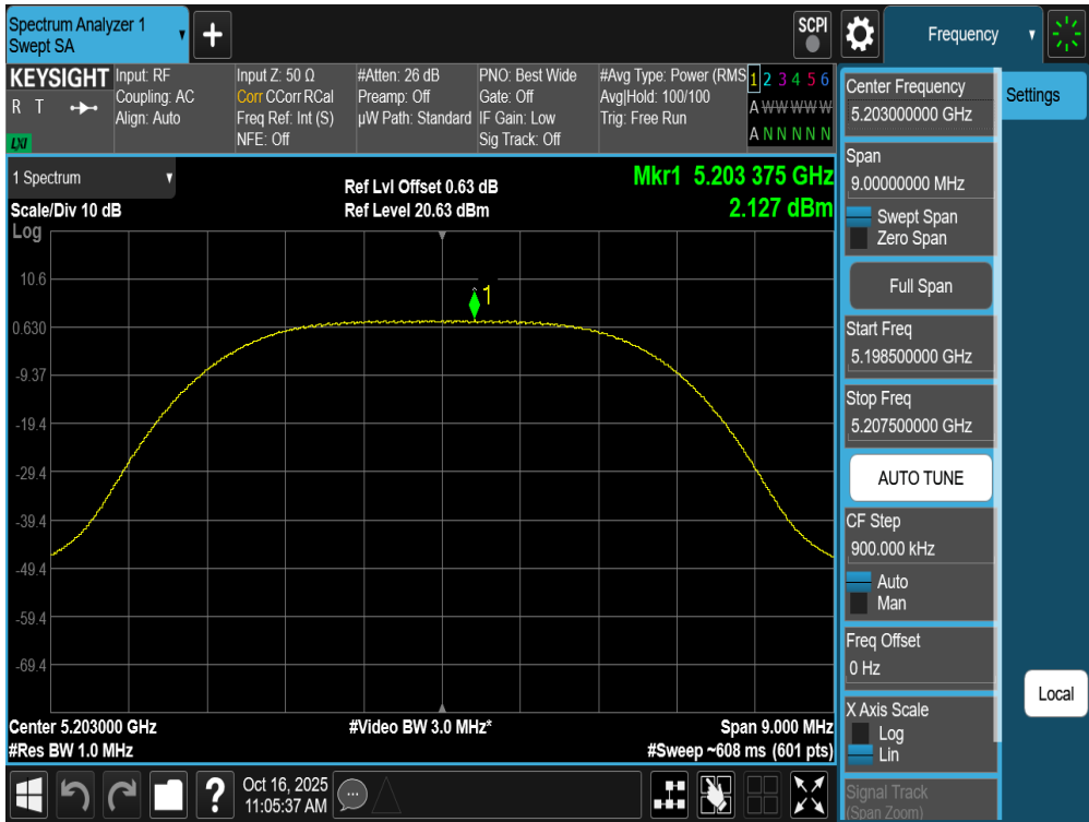
Plot 7-130. PSD Antenna WF7a (NB UNII XHDRPM6, ePA – 5203MHz)
