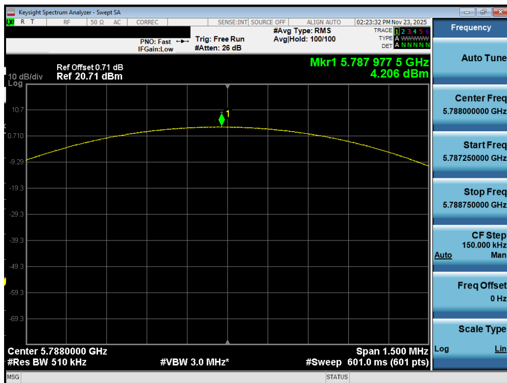
Plot 7-147. PSD Antenna WF7a (NB UNII LE1M, iPA – 5788MHz)
