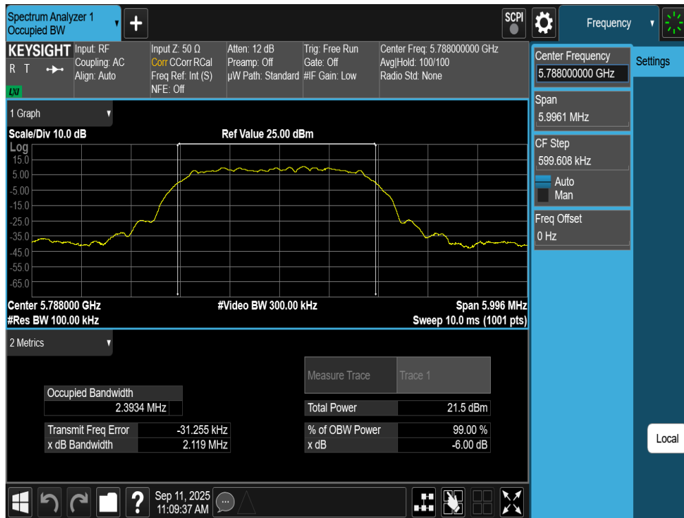
Plot 7-102. 6dB BW Antenna WF2a (NB UNII HDT2, ePA- 5788MHz)
