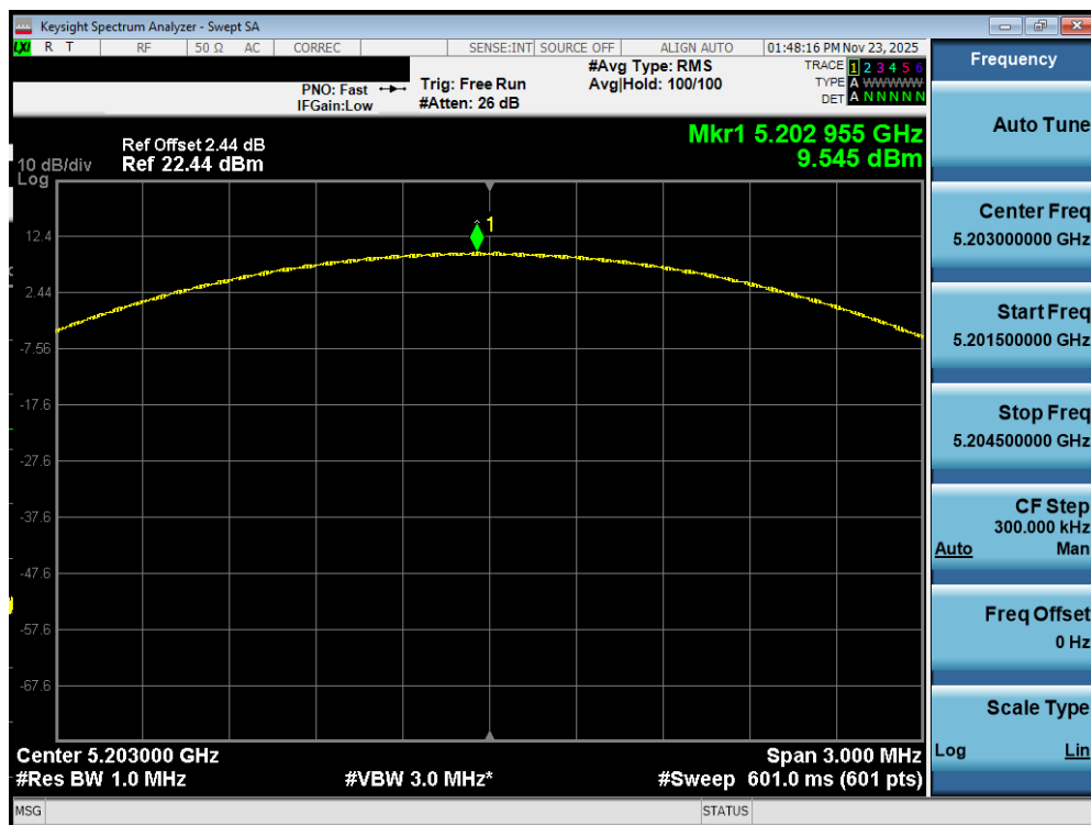
Plot 7-122. PSD Antenna WF7a (NB UNII LE2M, ePA – 5203MHz)
