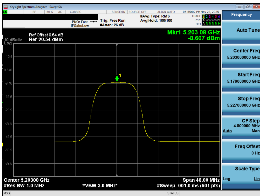
Plot 7-137. PSD Antenna WF7a (NB UNII HDRPL32, iPA – 5203MHz)
