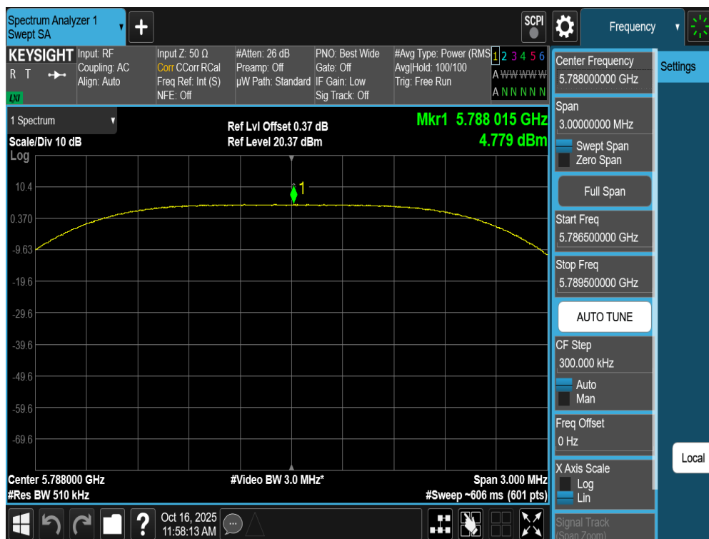
Plot 7-154. PSD Antenna WF7a (NB UNII HDRPS2, ePA – 5788MHz)
