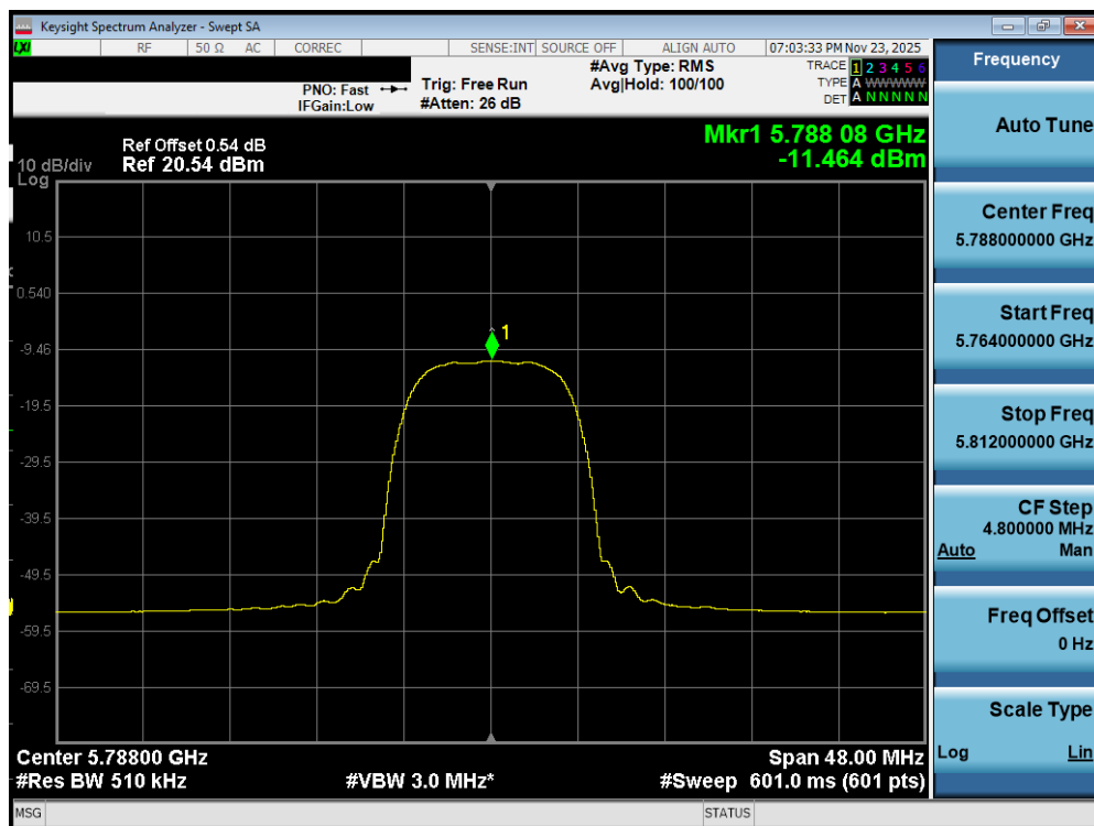
Plot 7-163. PSD Antenna WF7a (NB UNII HDRPL32, iPA – 5788MHz)
