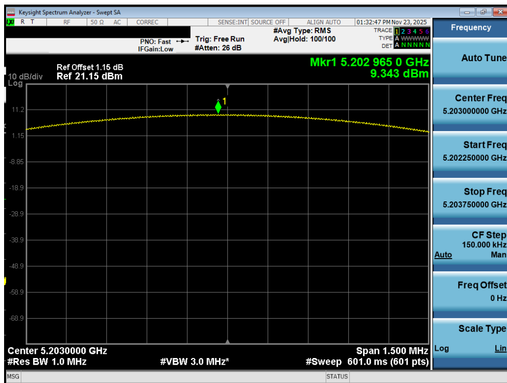
Plot 7-118. PSD Antenna WF7a (NB UNII BDR, ePA – 5203MHz)
