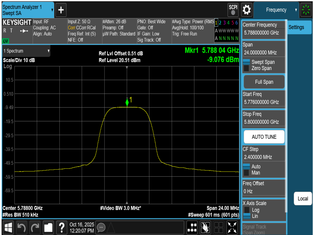
Plot 7-159. PSD Antenna WF7a (NB UNII HDRPM16, iPA – 5788MHz)
