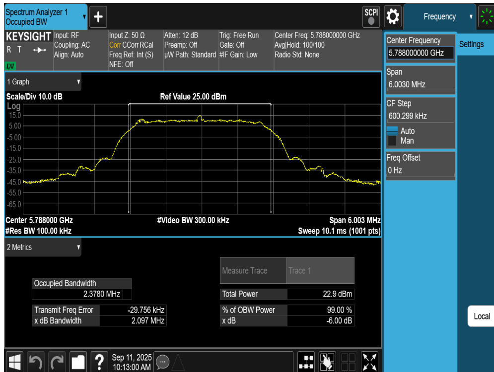
Plot 7-97. 6dB BW Antenna WF2a (NB UNII HDRPS2, ePA – 5788MHz)
