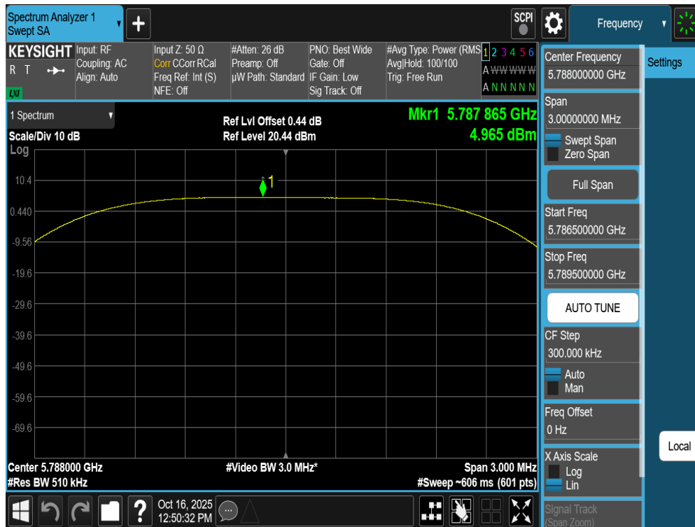
Plot 7-168. PSD Antenna WF7a (NB UNII HDT6, ePA – 5788MHz)
