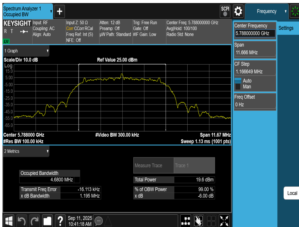
Plot 7-99. 6dB BW Antenna WF2a (NB UNII HDRPM16, ePA – 5788MHz)
