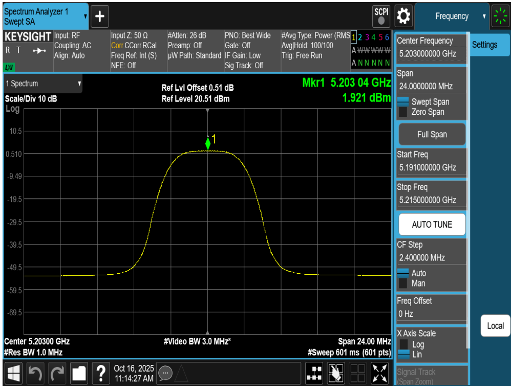
Plot 7-132. PSD Antenna WF7a (NB UNII HDRPM16, ePA – 5203MHz)
