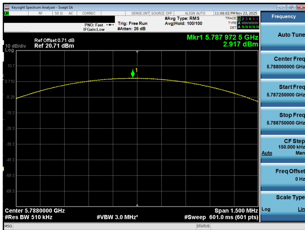
Plot 7-436. PSD TxBF Diversity Antenna WF2a (NB UNII LE1M, iPA – 5788MHz)
