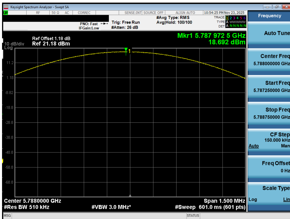
Plot 7-430. PSD TxBF Diversity Antenna WF2a (NB UNII BDR, ePA – 5788MHz)
