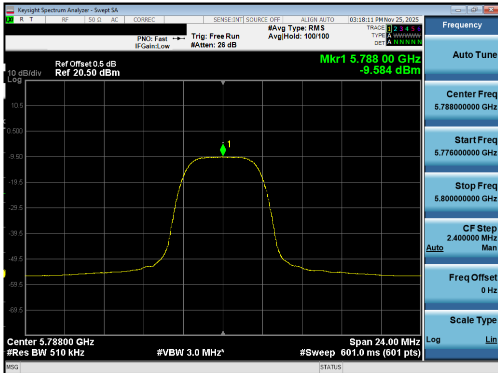
Plot 7-461. PSD TxBF Diversity Antenna WF7b (NB UNII HDRPM16, iPA – 5788MHz)
