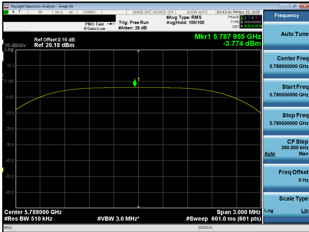
Plot 7-473. PSD TxBF Diversity Antenna WF7b (NB UNII HDT2, iPA - 5788MHz)
