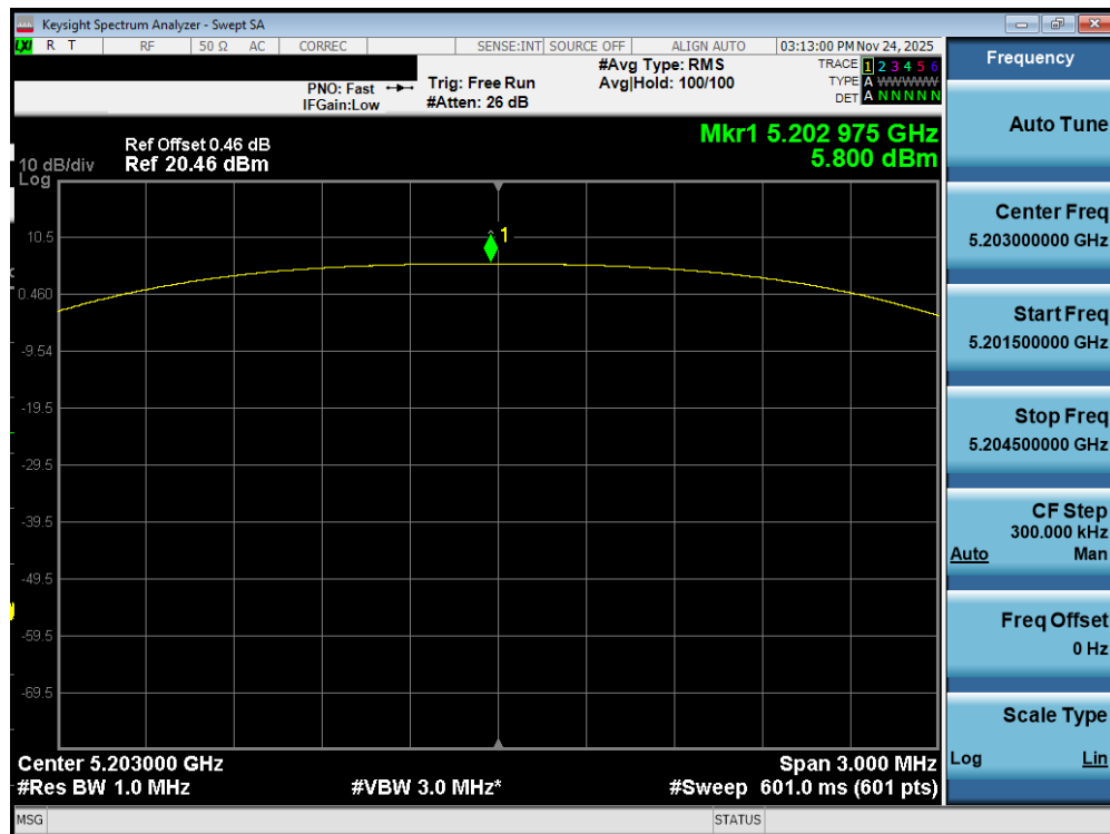
Plot 7-426. PSD TxBF Diversity Antenna WF2a (NB UNII HDT6, ePA – 5203MHz)
