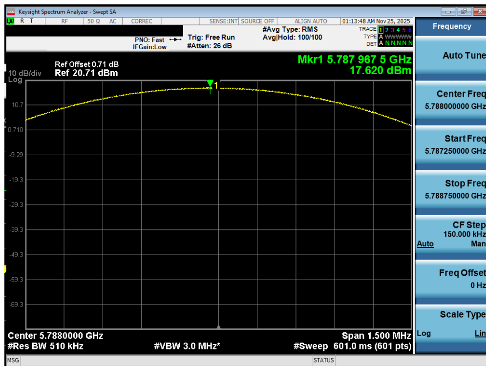
Plot 7-435. PSD TxBF Diversity Antenna WF7b (NB UNII LE1M, ePA – 5788MHz)
