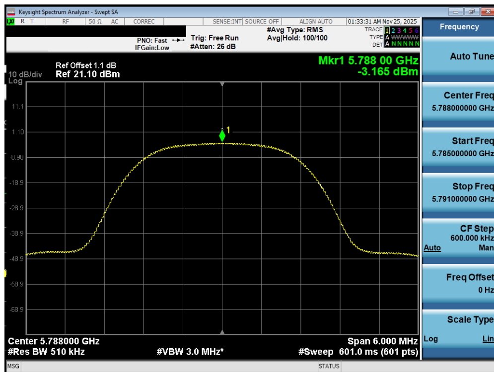
Plot 7-445. PSD TxBF Diversity Antenna WF7b (NB UNII HDR4, iPA – 5788MHz)
