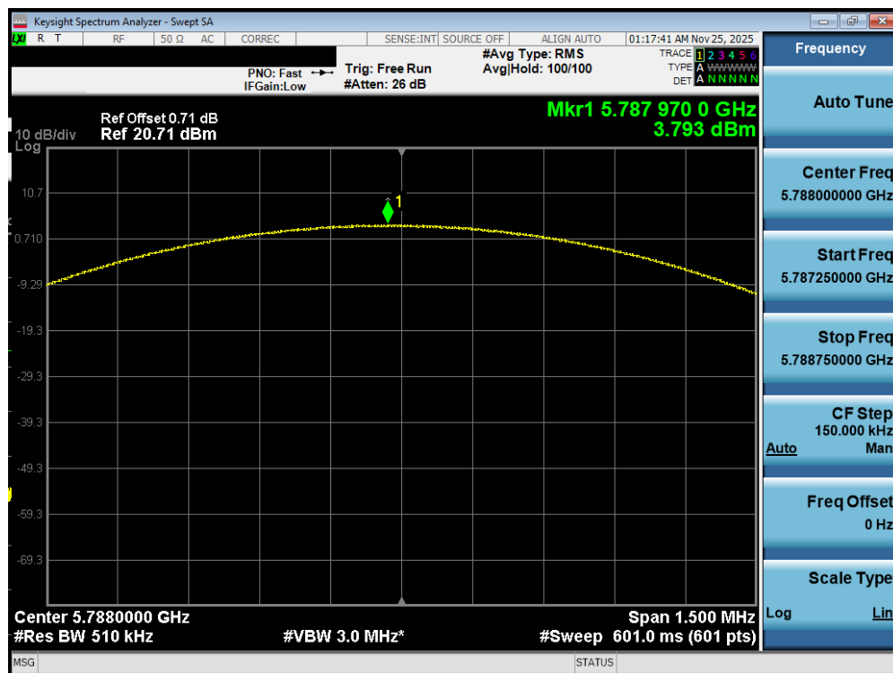
Plot 7-437. PSD TxBF Diversity Antenna WF7b (NB UNII LE1M, iPA – 5788MHz)
