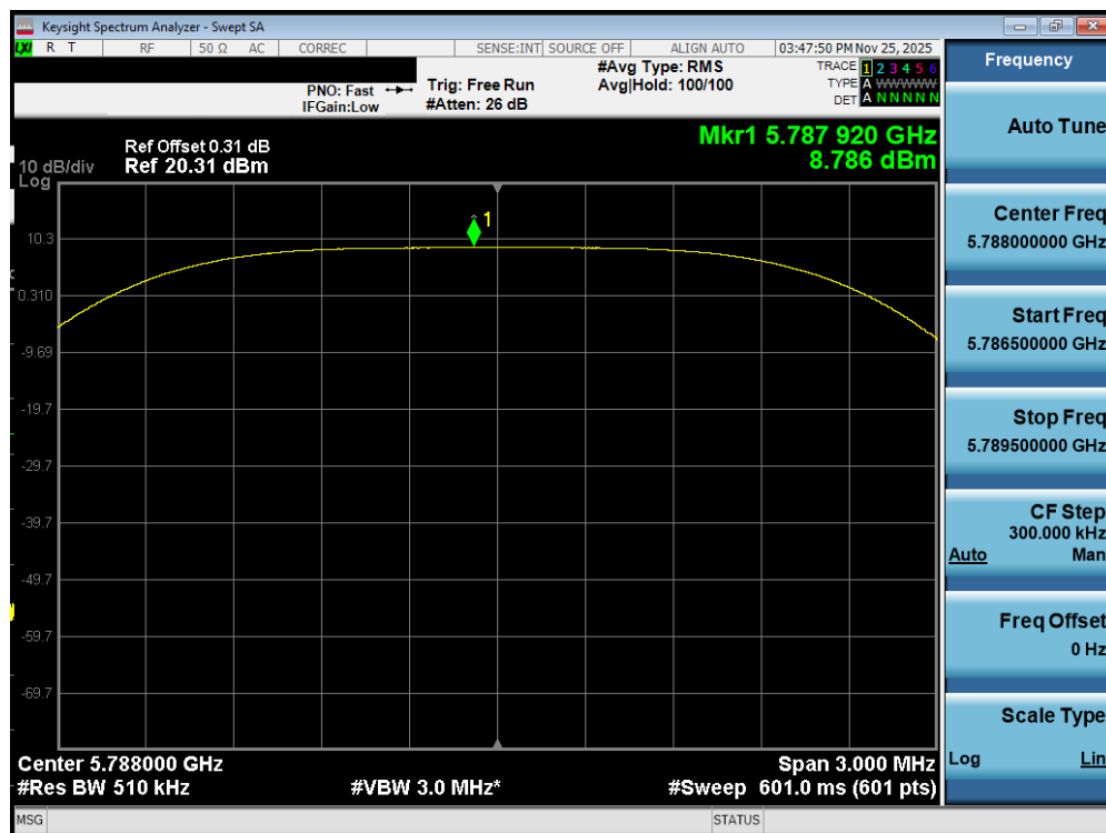
Plot 7-475. PSD TxBF Diversity Antenna WF7b (NB UNII HDT4, ePA - 5788MHz)
