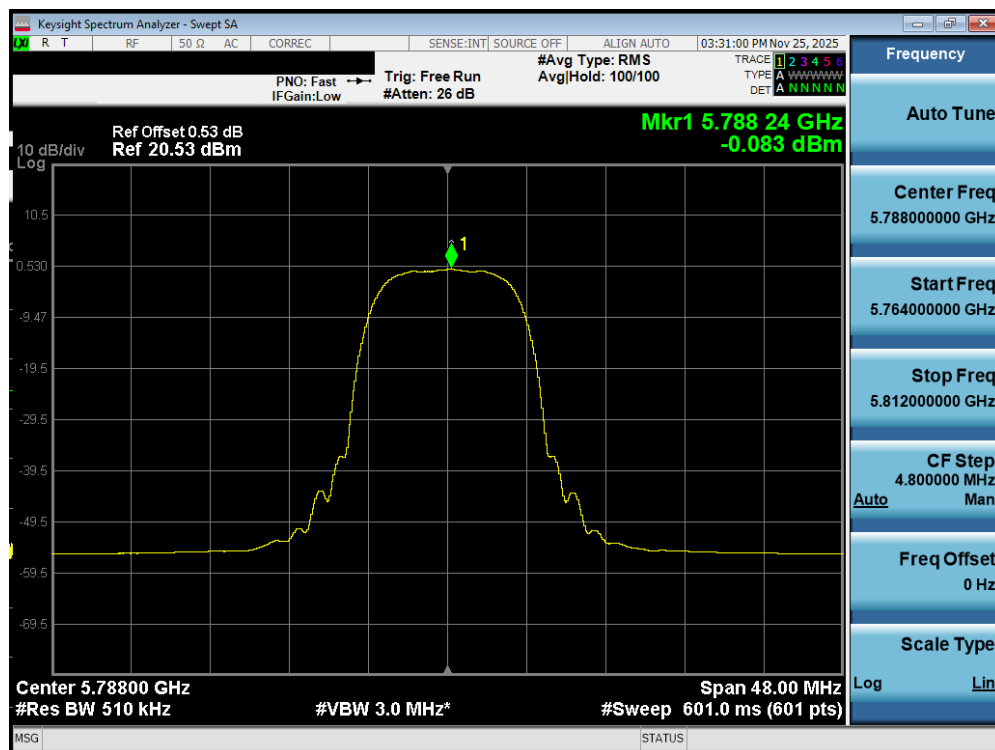
Plot 7-467. PSD TxBF Diversity Antenna WF7b (NB UNII HDRPL32, ePA – 5788MHz)
