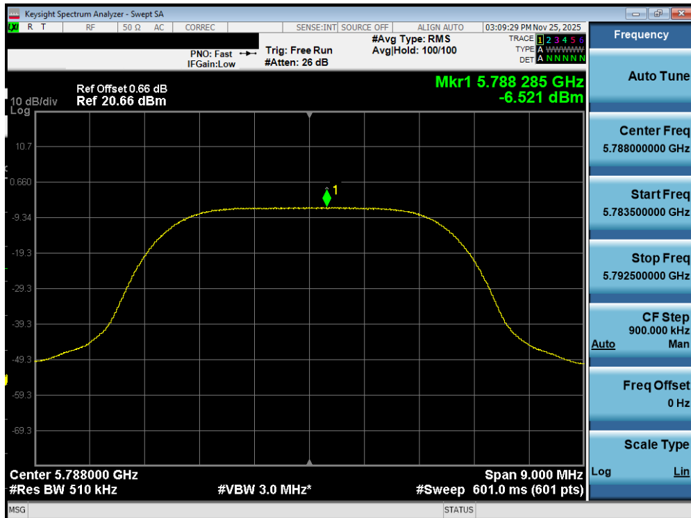
Plot 7-457. PSD TxBF Diversity Antenna WF7b (NB UNII XHDRPM6, iPA – 5788MHz)
