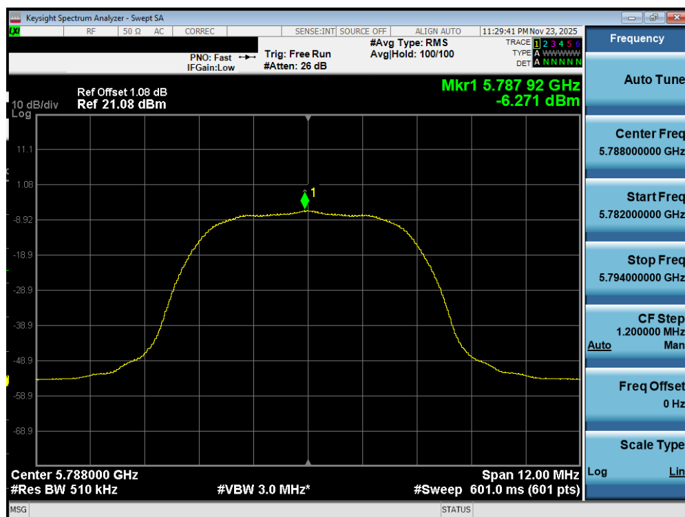
Plot 7-448. PSD TxBF Diversity Antenna WF2a (NB UNII HDR8, iPA – 5788MHz)
