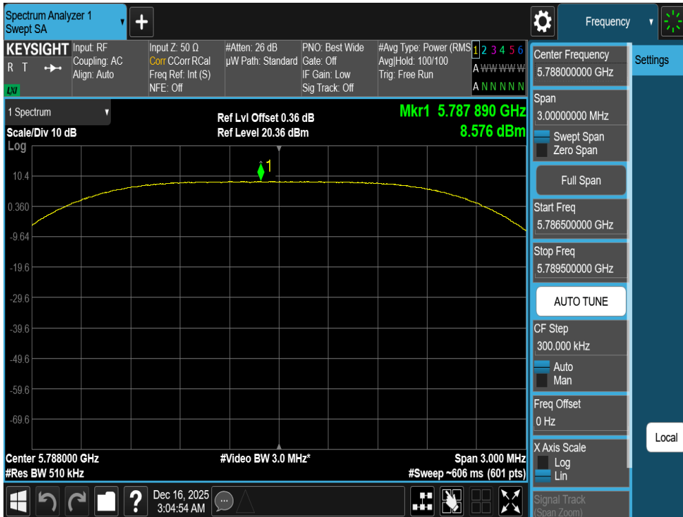
Plot 7-450. PSD Tx BF Diversity Antenna WF2a (NB UNII HDRPS2, ePA – 5788MHz)
