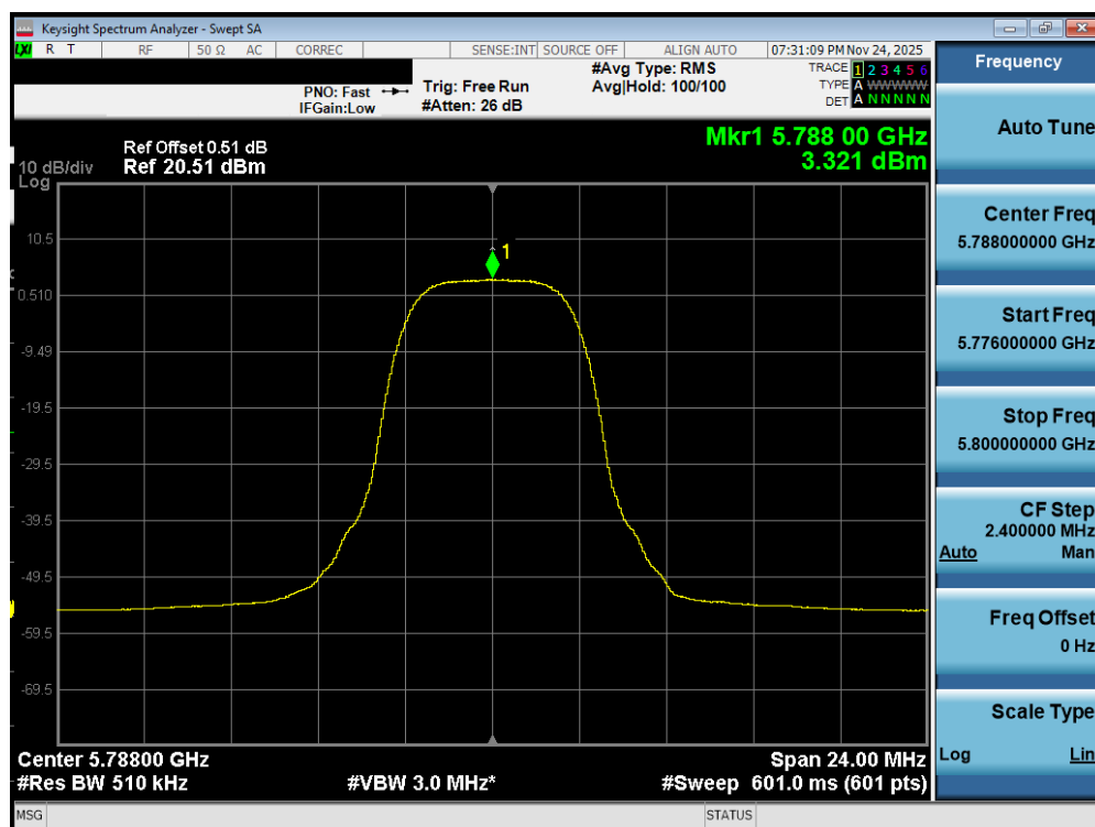
Plot 7-458. PSD TxBF Diversity Antenna WF2a (NB UNII HDRPM16, ePA – 5788MHz)
