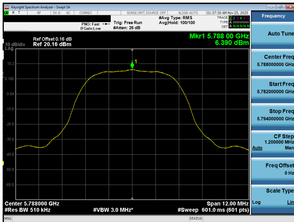
Plot 7-447. PSD TxBF Diversity Antenna WF7b (NB UNII HDR8, ePA – 5788MHz)
