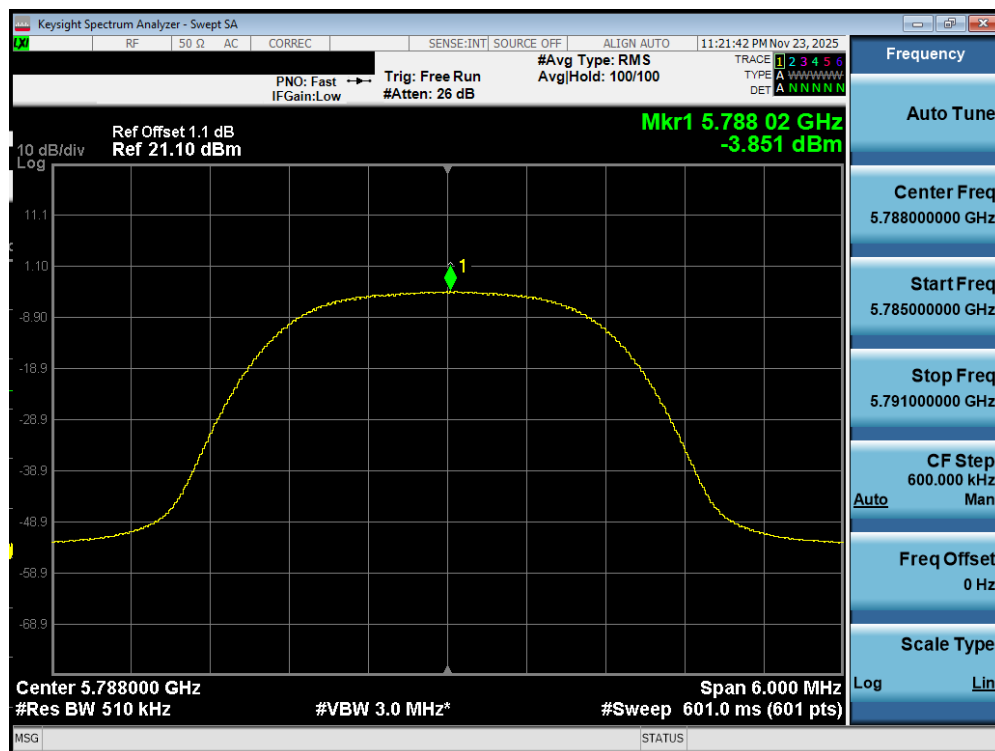
Plot 7-444. PSD TxBF Diversity Antenna WF2a (NB UNII HDR4, iPA – 5788MHz)
