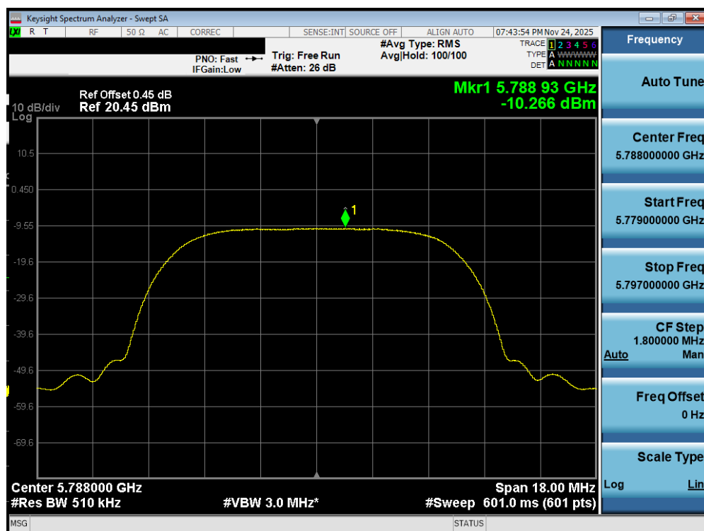
Plot 7-464. PSD TxBF Diversity Antenna WF2a (NB UNII HDRPL12, iPA – 5788MHz)
