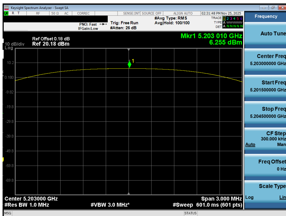
Plot 7-419. PSD TxBF Diversity Antenna WF7b (NB UNII HDT2, ePA – 5203MHz)
