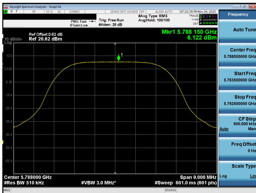
Plot 7-454. PSD TxBF Diversity Antenna WF2a (NB UNII XHDRPM6, ePA – 5788MHz)
