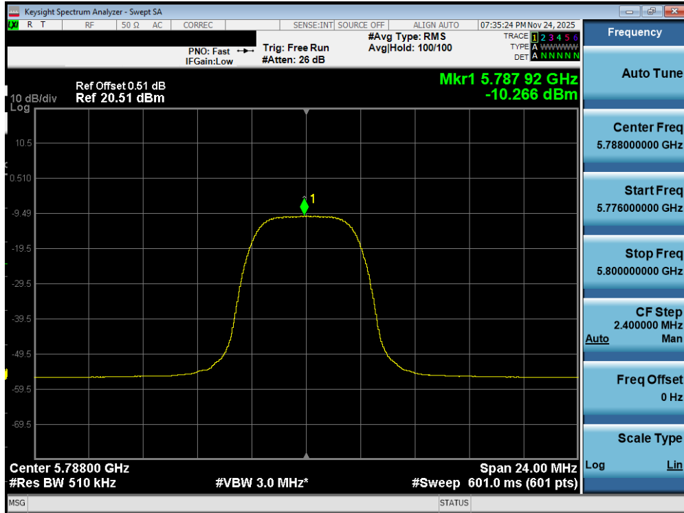
Plot 7-460. PSD TxBF Diversity Antenna WF2a (NB UNII HDRPM16, iPA – 5788MHz)
