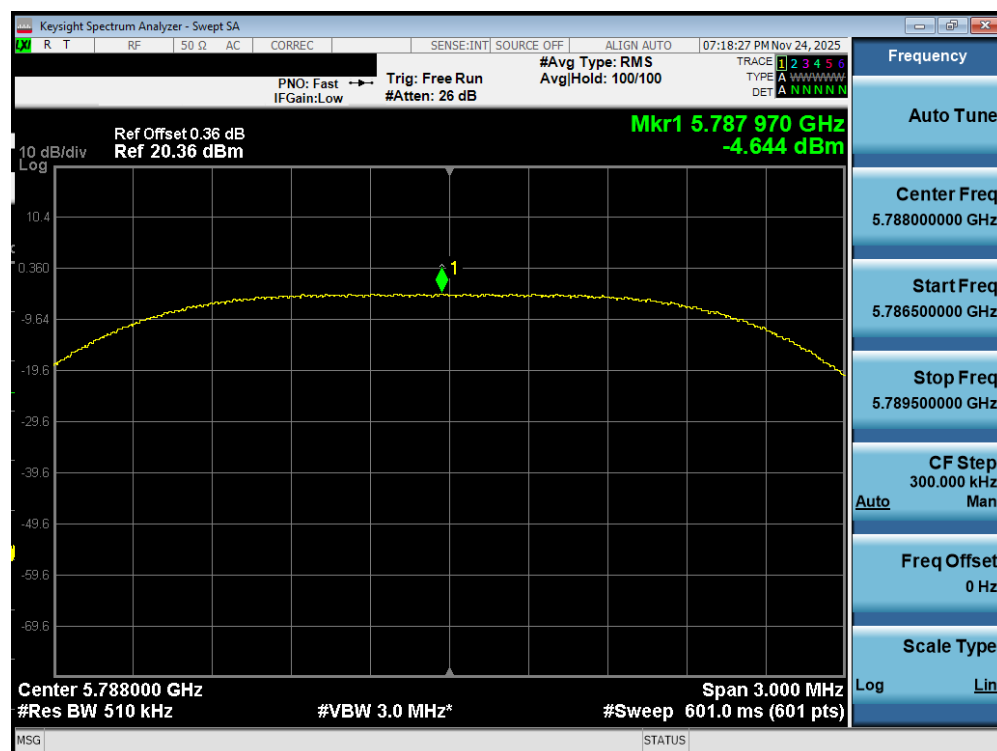
Plot 7-452. PSD TxBF Diversity Antenna WF2a (NB UNII HDRPS2, iPA – 5788MHz)
