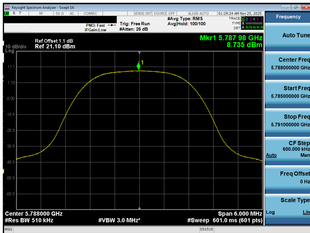
Plot 7-443. PSD TxBF Diversity Antenna WF7b (NB UNII HDR4, ePA – 5788MHz)
