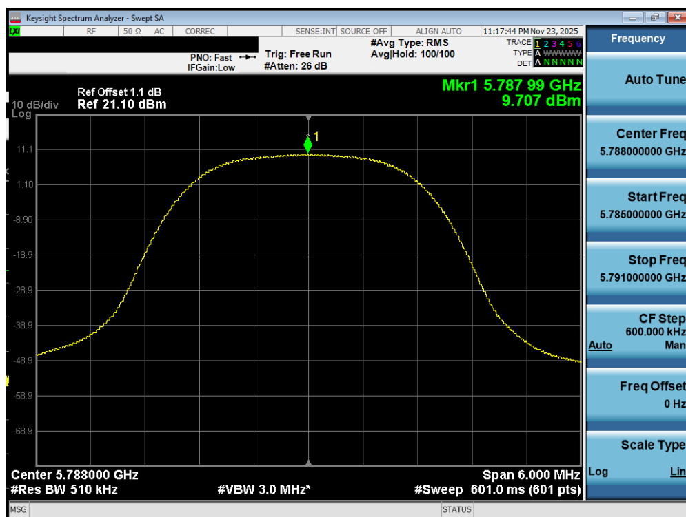
Plot 7-442. PSD TxBF Diversity Antenna WF2a (NB UNII HDR4, ePA – 5788MHz)
