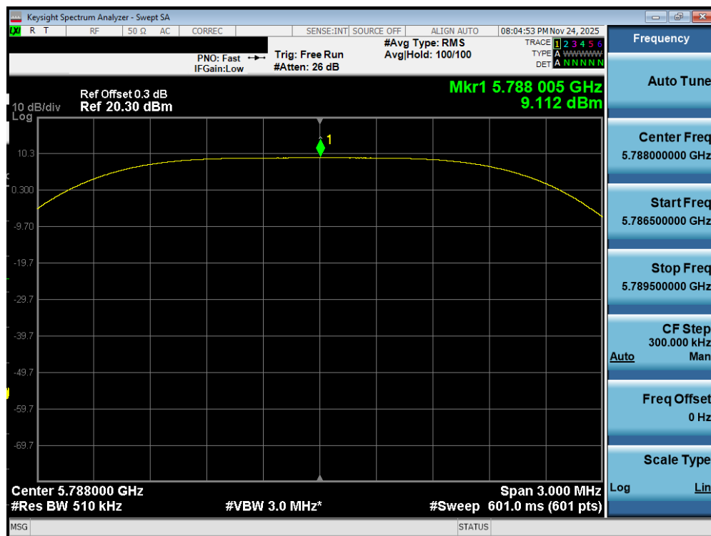
Plot 7-474. PSD TxBF Diversity Antenna WF2a (NB UNII HDT4, ePA - 5788MHz)
