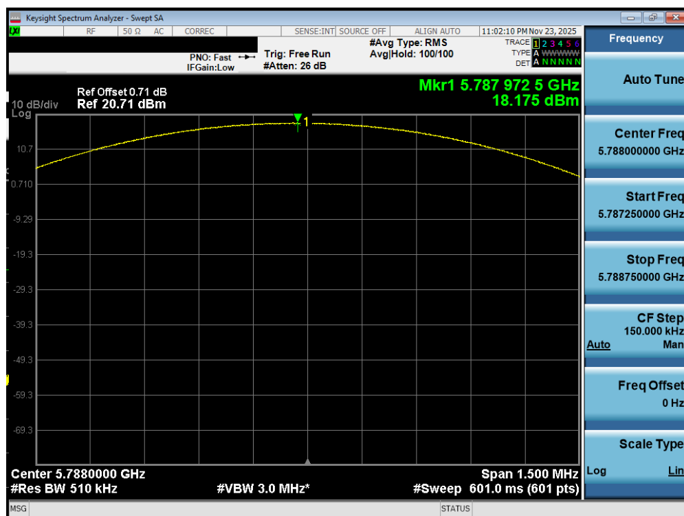
Plot 7-434. PSD TxBF Diversity Antenna WF2a (NB UNII LE1M, ePA – 5788MHz)
