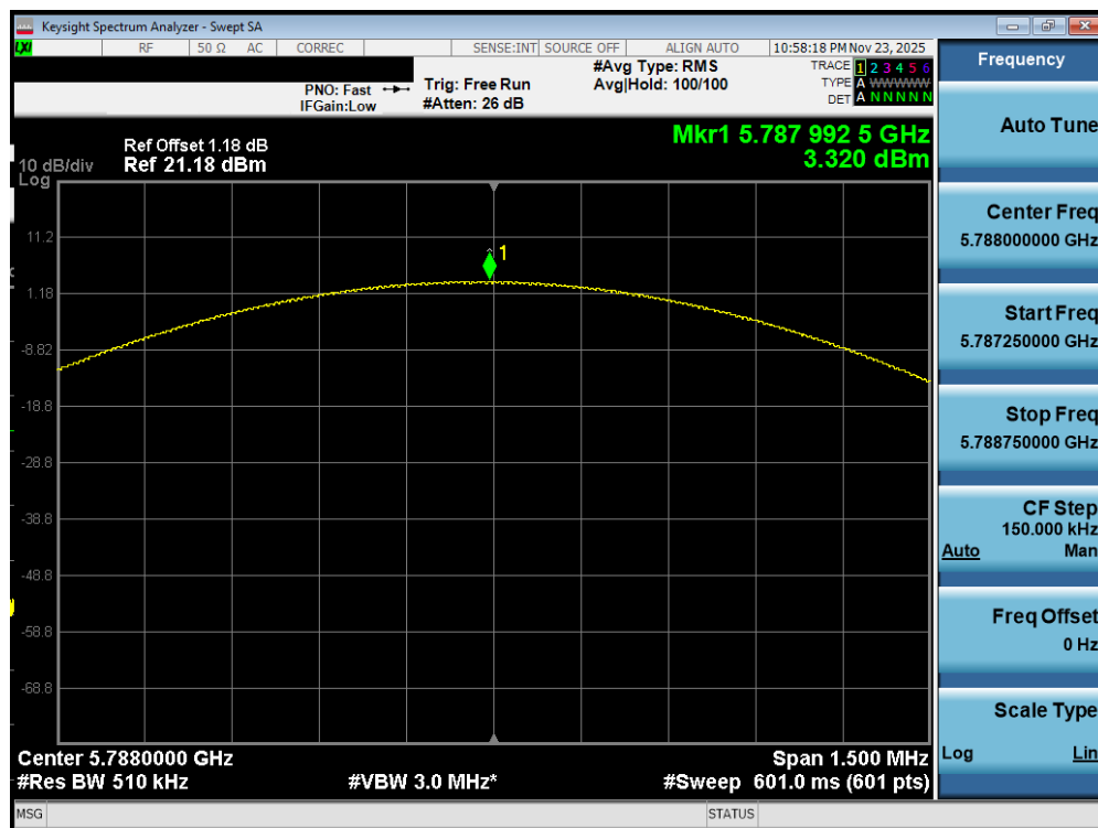
Plot 7-432. PSD TxBF Diversity Antenna WF2a (NB UNII BDR, iPA – 5788MHz)
