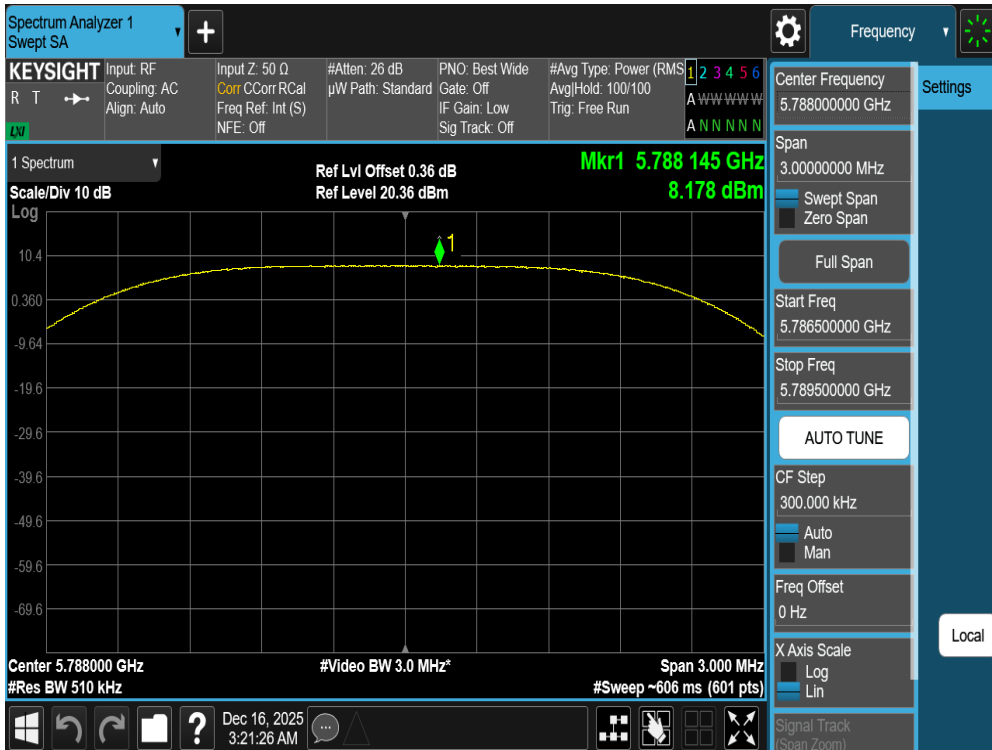
Plot 7-451. PSD Tx BF Diversity Antenna WF7b (NB UNII HDRPS2, ePA – 5788MHz)
