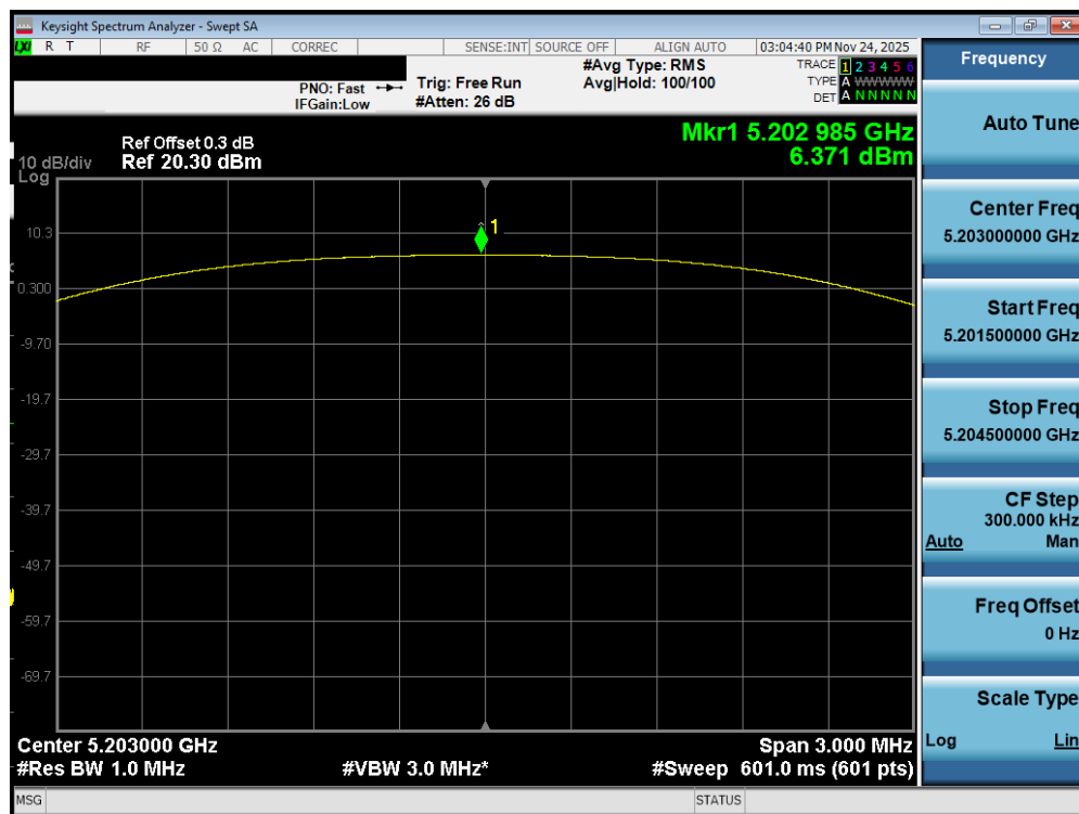
Plot 7-422. PSD TxBF Diversity Antenna WF2a (NB UNII HDT4, ePA – 5203MHz)
