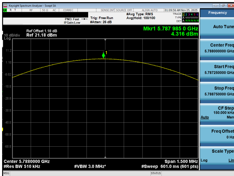
Plot 7-433. PSD TxBF Diversity Antenna WF7b (NB UNII BDR, iPA – 5788MHz)
