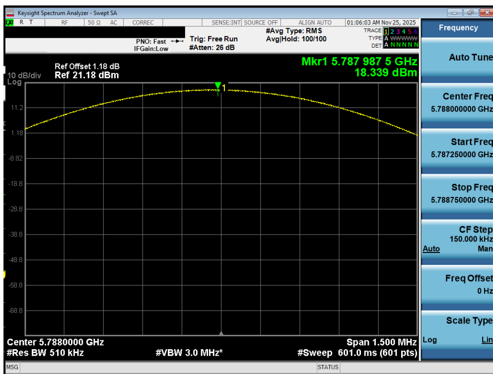
Plot 7-431. PSD TxBF Diversity Antenna WF7b (NB UNII BDR, ePA – 5788MHz)
