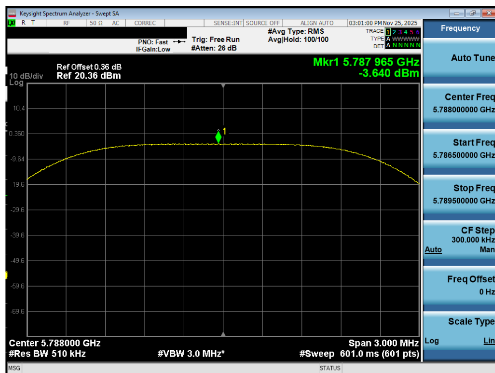
Plot 7-453. PSD TxBF Diversity Antenna WF7b (NB UNII HDRPS2, iPA – 5788MHz)
