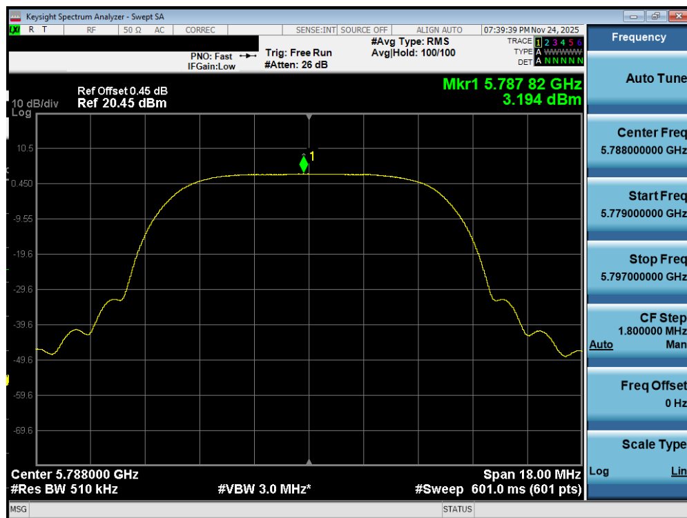
Plot 7-462. PSD TxBF Diversity Antenna WF2a (NB UNII HDRPL12, ePA – 5788MHz)
