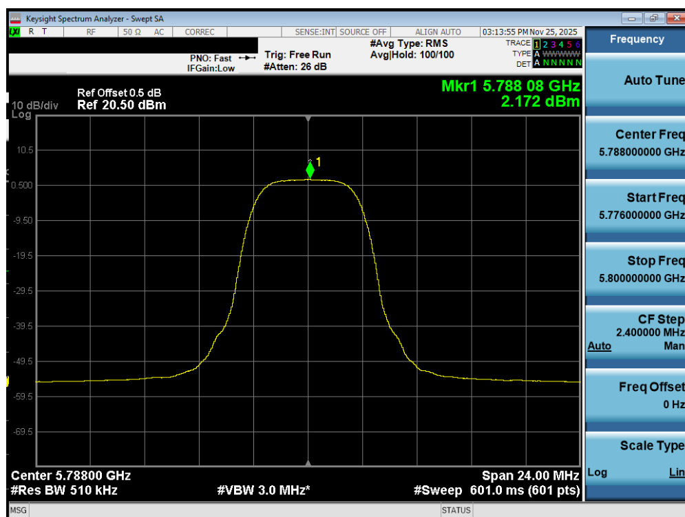
Plot 7-459. PSD TxBF Diversity Antenna WF7b (NB UNII HDRPM16, ePA – 5788MHz)
