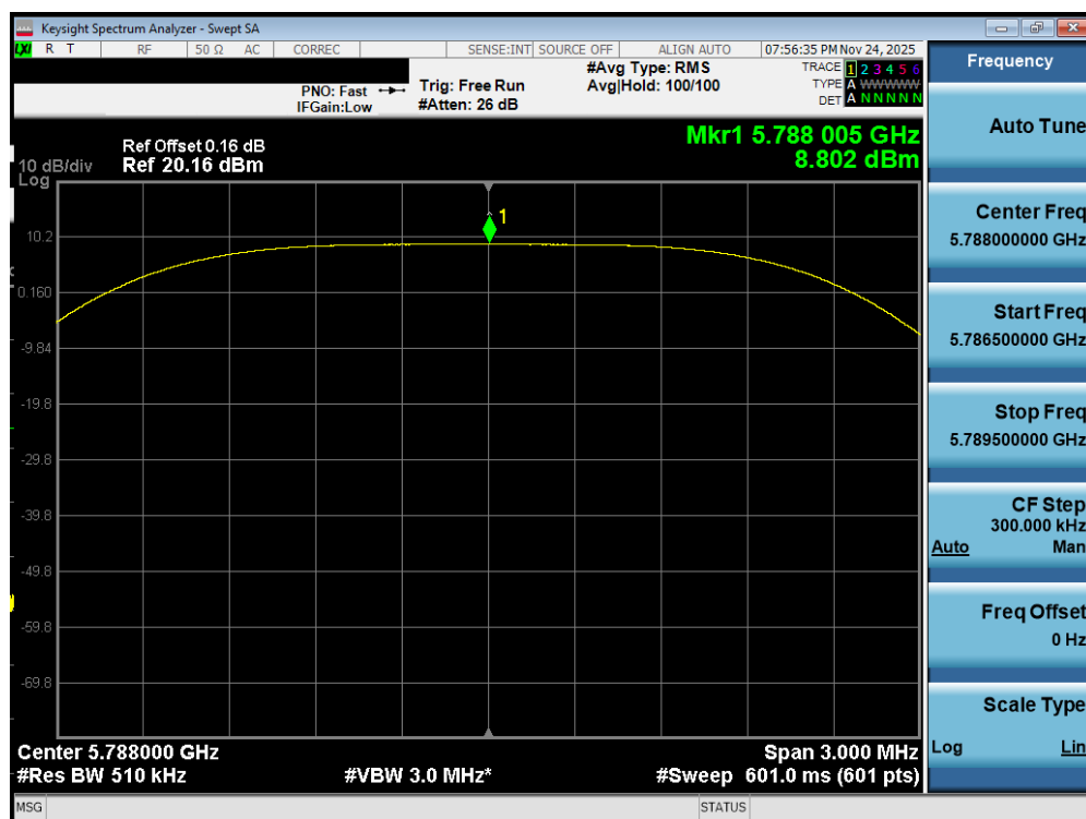
Plot 7-470. PSD Tx BF Diversity Antenna WF2a (NB UNII HDT2, ePA – 5788MHz)
