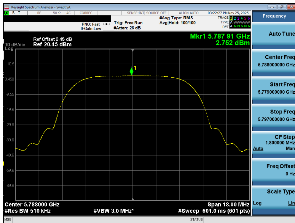
Plot 7-463. PSD TxBF Diversity Antenna WF7b (NB UNII HDRPL12, ePA – 5788MHz)
