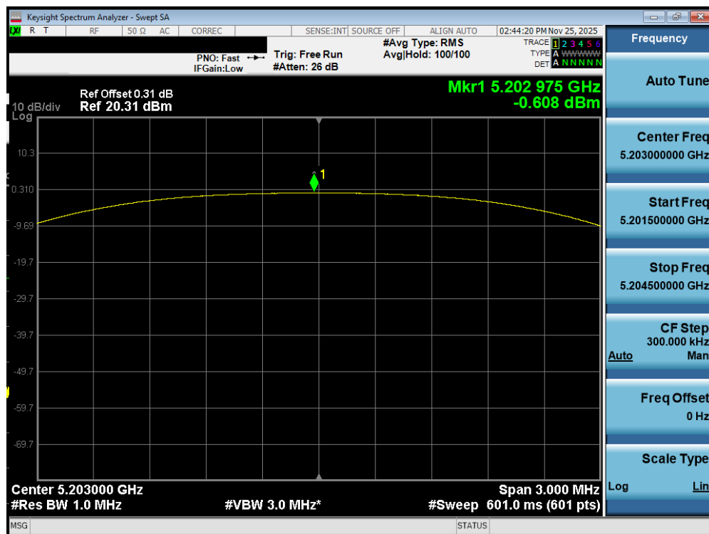
Plot 7-425. PSD TxBF Diversity Antenna WF7b (NB UNII HDT4, iPA – 5203MHz)
