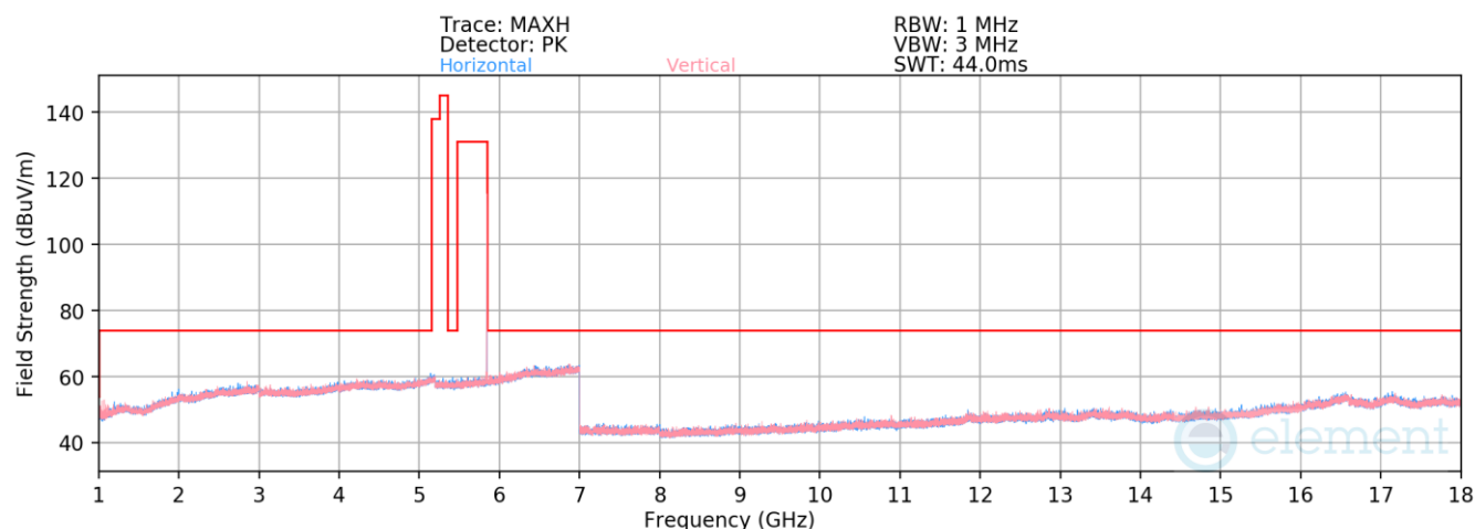
Plot 7-497. Radiated Spurious Emissions 1-18GHz TxBF Primary (HDR HDR4 ePA – 5844MHz)
