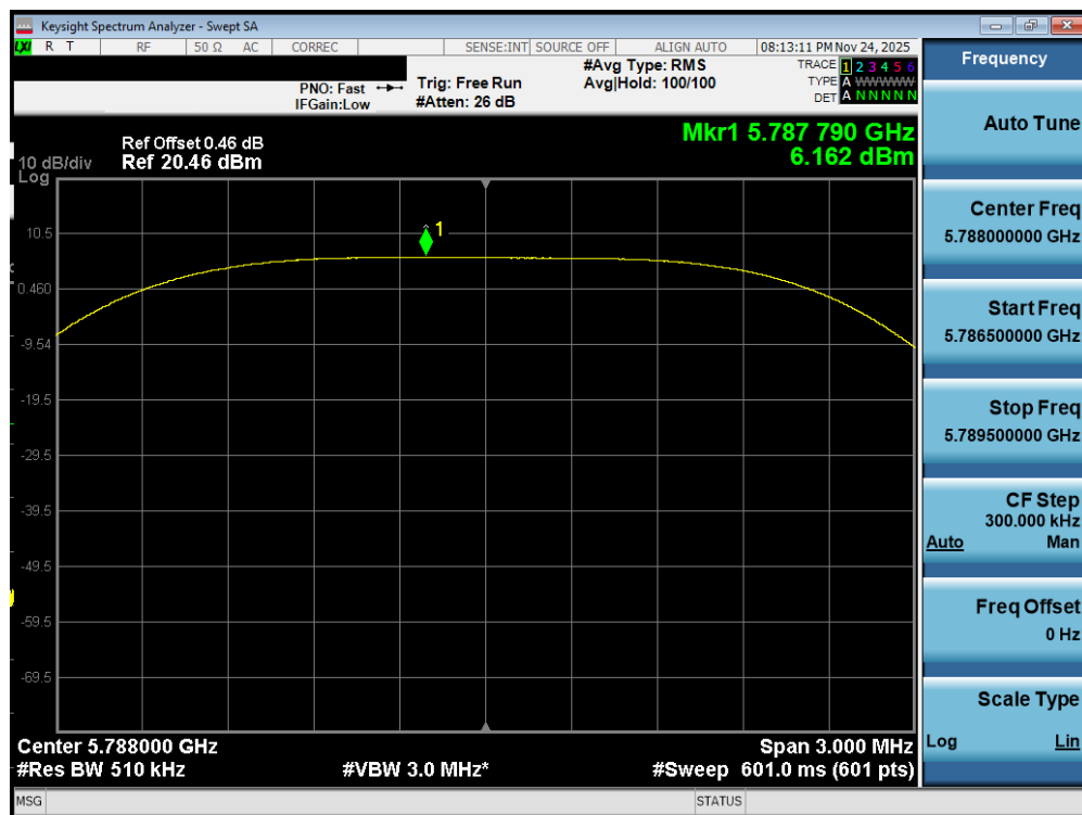
Plot 7-478. PSD TxBF Diversity Antenna WF2a (NB UNII HDT6, ePA – 5788MHz)
