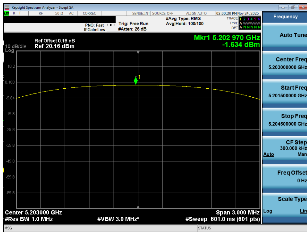
Plot 7-420. PSD TxBF Diversity Antenna WF2a (NB UNII HDT2, iPA – 5203MHz)
