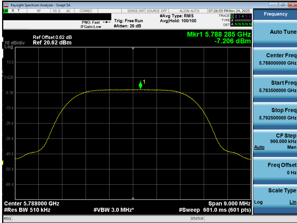
Plot 7-456. PSD TxBF Diversity Antenna WF2a (NB UNII XHDRPM6, iPA – 5788MHz)
