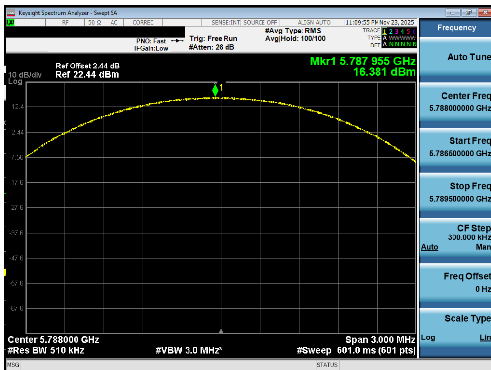
Plot 7-438. PSD TxBF Diversity Antenna WF2a (NB UNII LE2M, ePA - 5788MHz)
