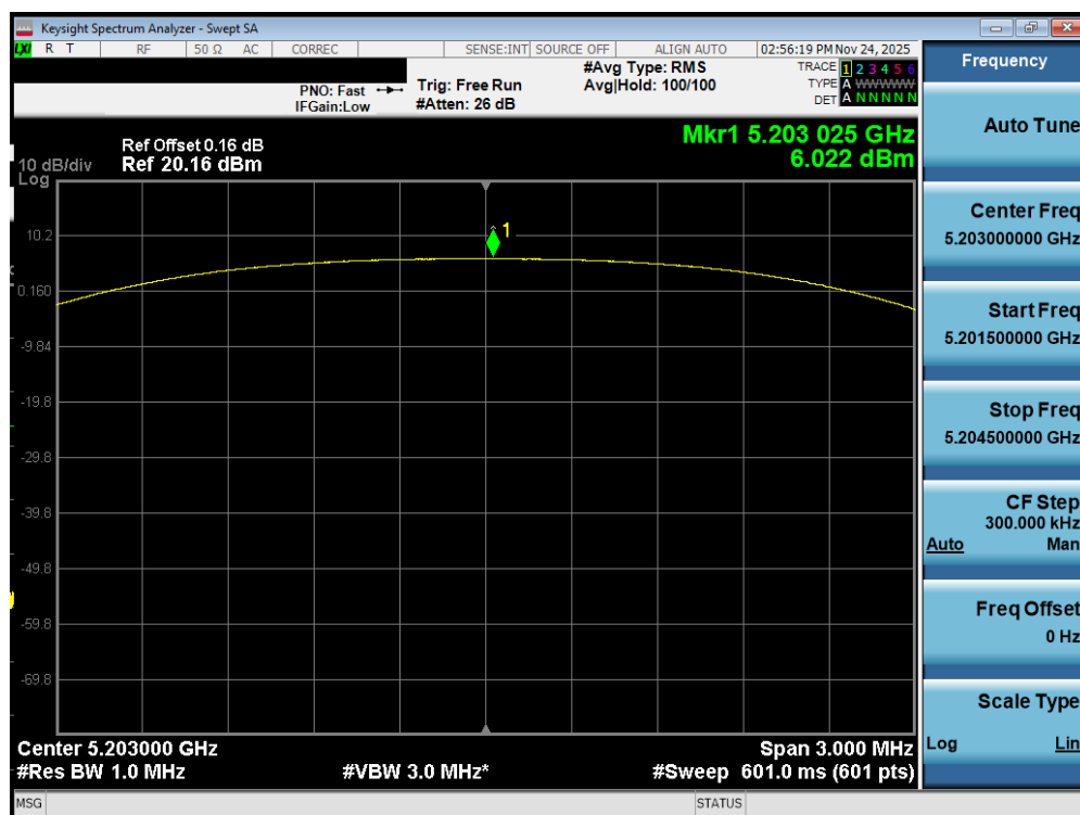
Plot 7-418. PSD TxBF Diversity Antenna WF2a (NB UNII HDT2, ePA – 5203MHz)
