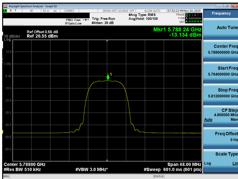
Plot 7-468. PSD TxBF Diversity Antenna WF2a (NB UNII HDRPL32, iPA – 5788MHz)
