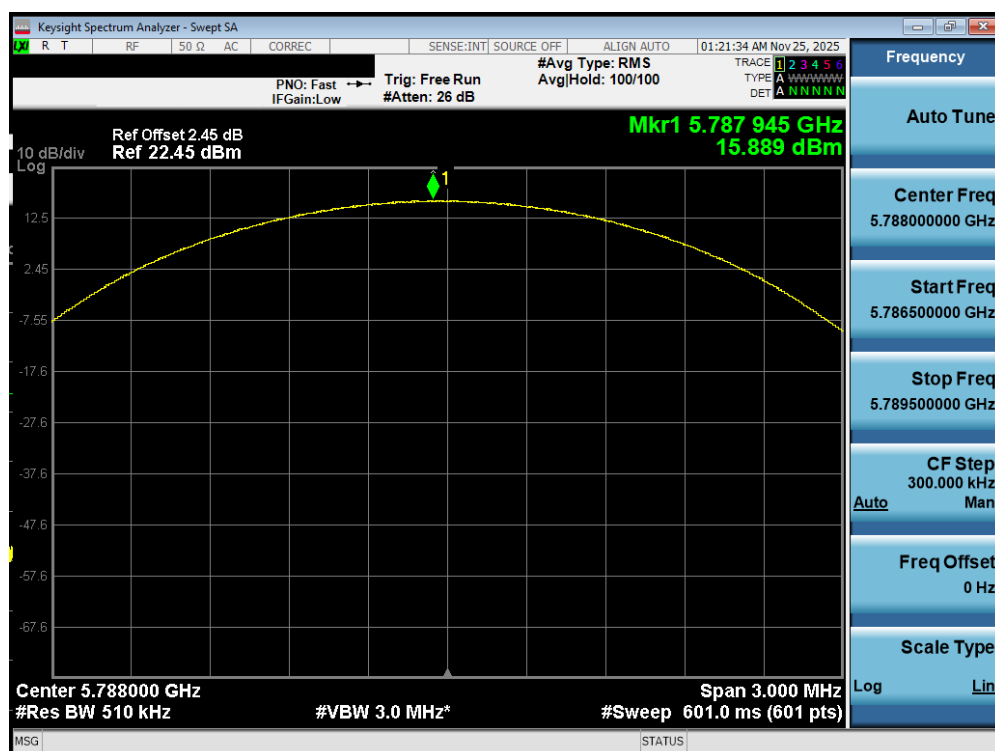
Plot 7-439. PSD TxBF Diversity Antenna WF7b (NB UNII LE2M, ePA - 5788MHz)
