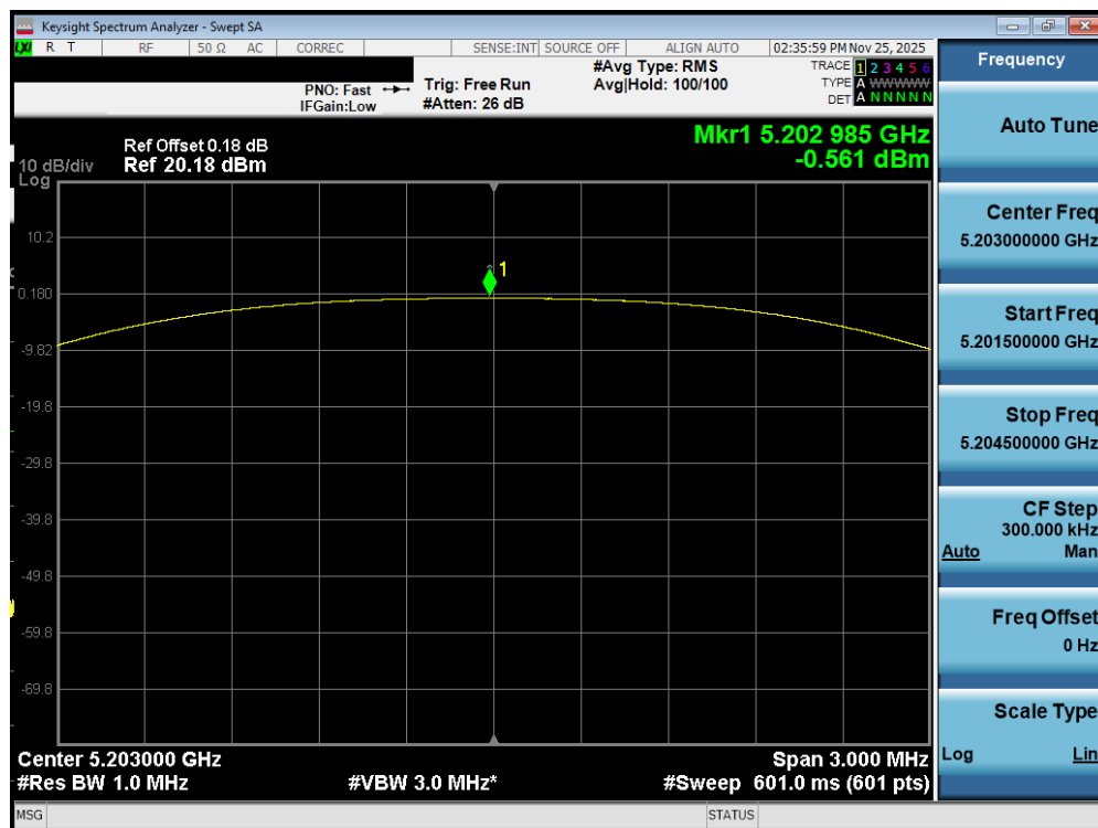
Plot 7-421. PSD TxBF Diversity Antenna WF7b (NB UNII HDT2, iPA – 5203MHz)
