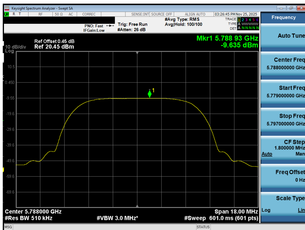
Plot 7-465. PSD TxBF Diversity Antenna WF7b (NB UNII HDRPL12, iPA – 5788MHz)
