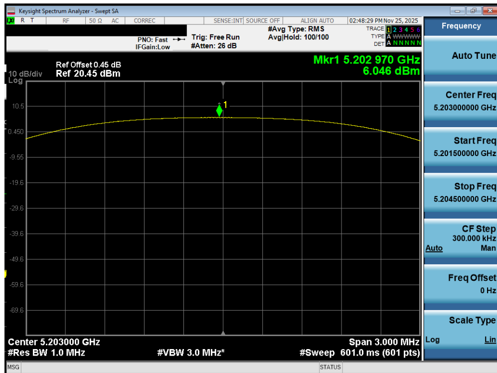
Plot 7-427. PSD TxBF Diversity Antenna WF7b (NB UNII HDT6, ePA – 5203MHz)
