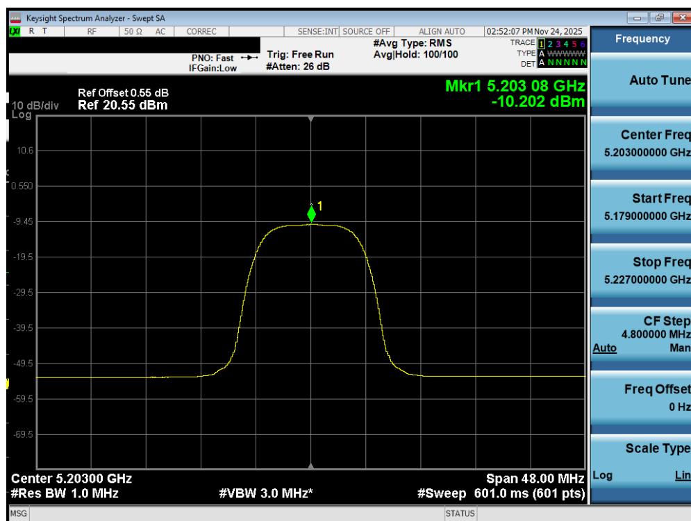
Plot 7-416. PSD TxBF Diversity Antenna WF2a (NB UNII HDRPL32, iPA – 5203MHz)
