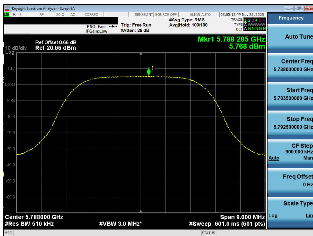
Plot 7-455. PSD TxBF Diversity Antenna WF7b (NB UNII XHDRPM6, ePA – 5788MHz)
