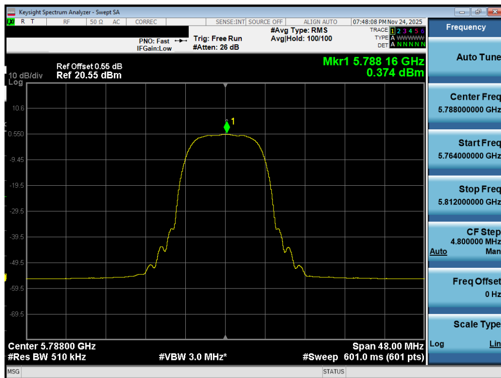
Plot 7-466. PSD TxBF Diversity Antenna WF2a (NB UNII HDRPL32, ePA – 5788MHz)
