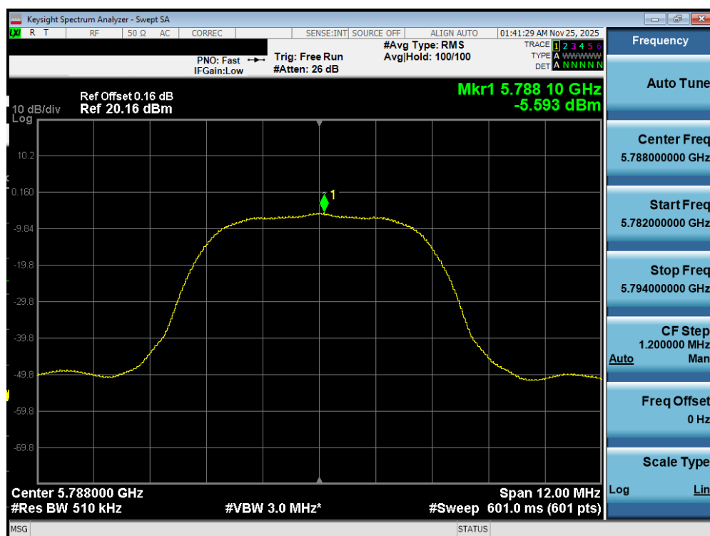
Plot 7-449. PSD TxBF Diversity Antenna WF7b (NB UNII HDR8, iPA – 5788MHz)
