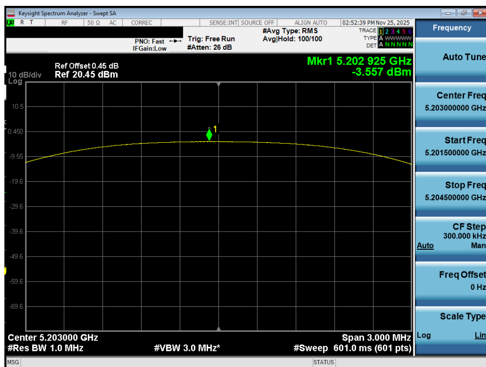
Plot 7-429. PSD TxBF Diversity Antenna WF7b (NB UNII HDT6, iPA – 5203MHz)
