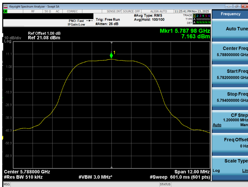
Plot 7-446. PSD TxBF Diversity Antenna WF2a (NB UNII HDR8, ePA – 5788MHz)
