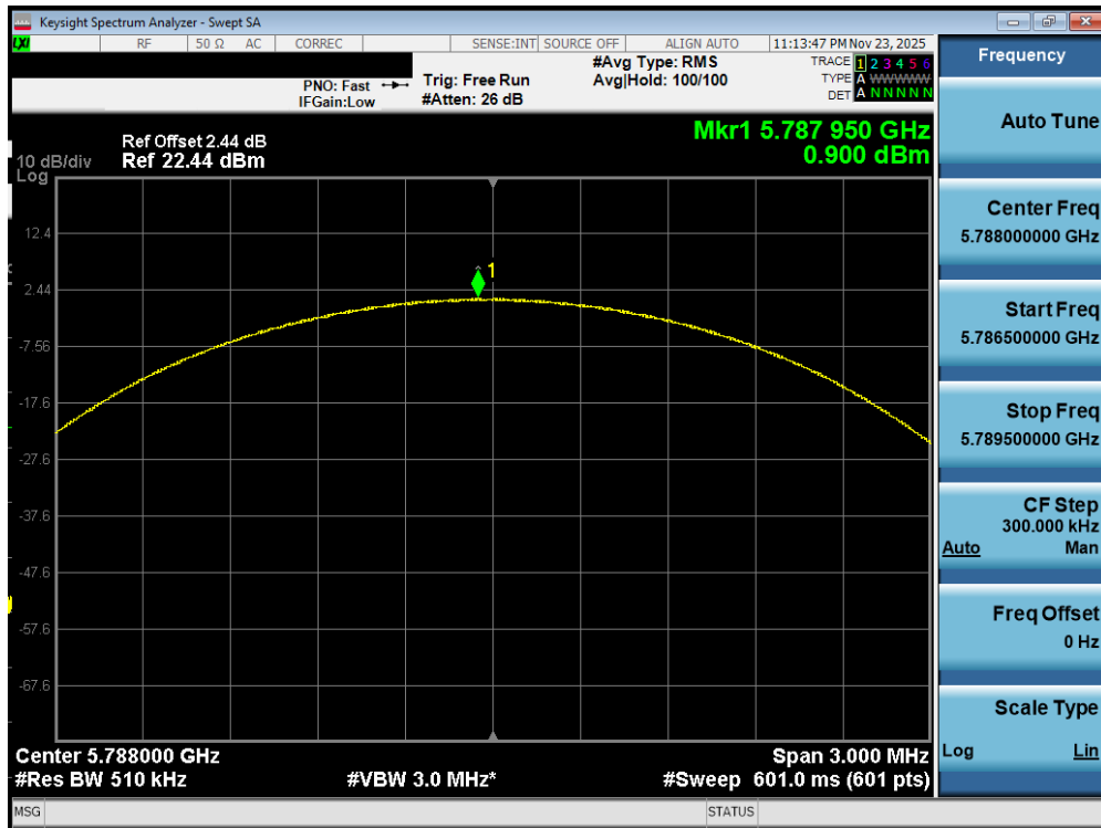
Plot 7-440. PSD TxBF Diversity Antenna WF2a (NB UNII LE2M, iPA - 5788MHz)
