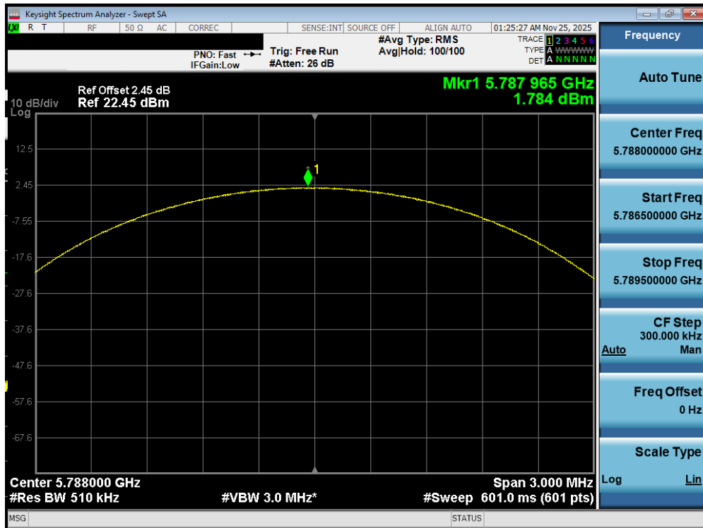
Plot 7-441. PSD TxBF Diversity Antenna WF7b (NB UNII LE2M, iPA - 5788MHz)
