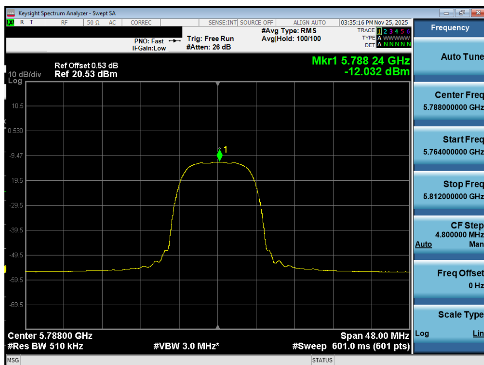
Plot 7-469. PSD TxBF Diversity Antenna WF7b (NB UNII HDRPL32, iPA – 5788MHz)
