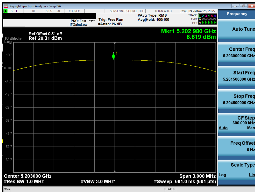
Plot 7-423. PSD TxBF Diversity Antenna WF7b (NB UNII HDT4, ePA – 5203MHz)
