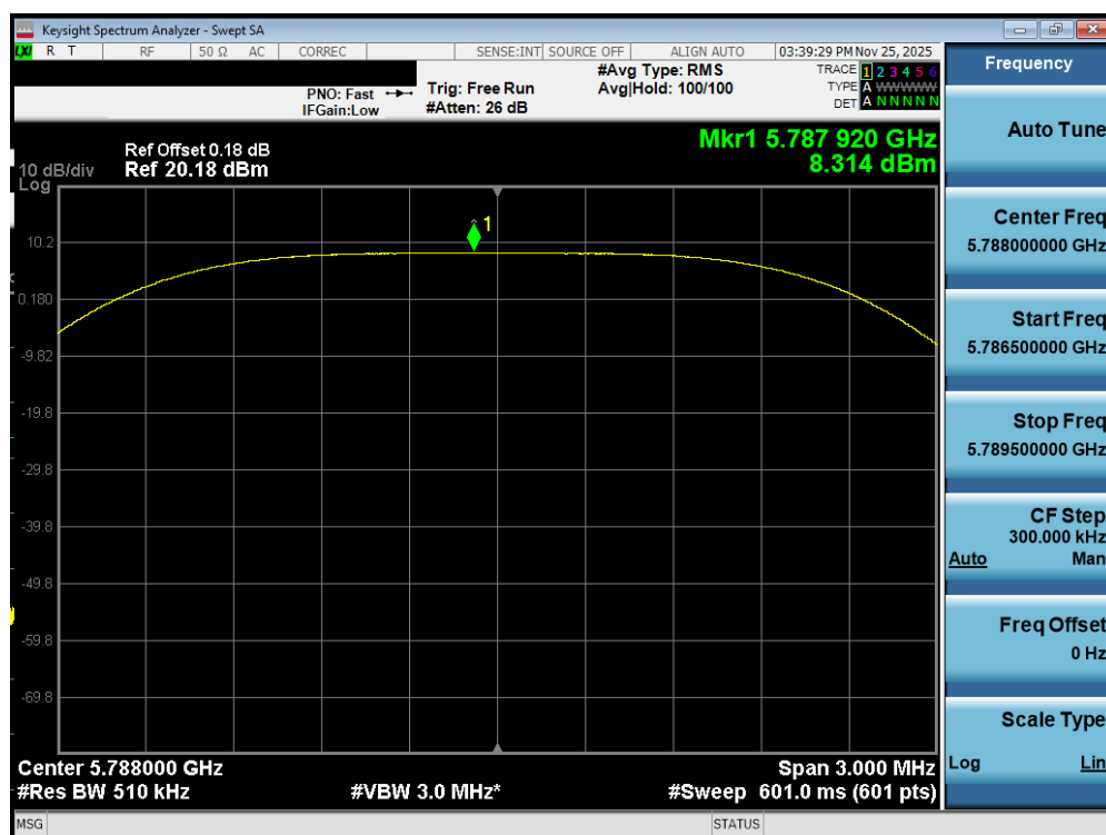
Plot 7-471. PSD Tx BF Diversity Antenna WF7b (NB UNII HDT2, ePA – 5788MHz)
