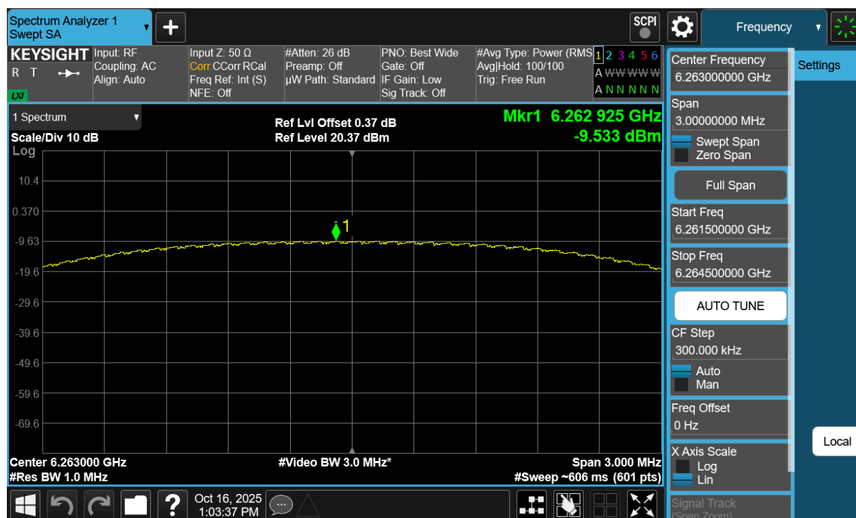
Plot 7-51. PSD Antenna WF7a (NB UNII HDRPS2, iPA – 6263MHz)
