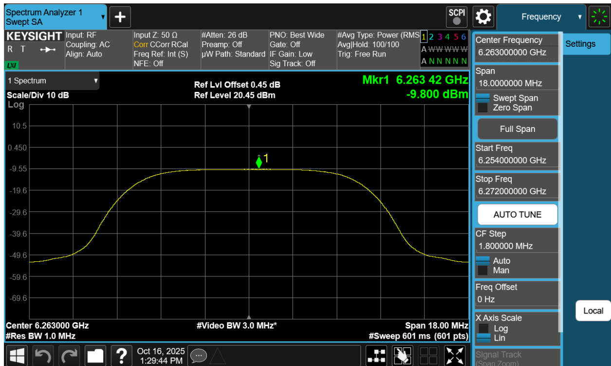
Plot 7-57. PSD Antenna WF7a (NB UNII HDRPL12, iPA – 6263MHz)
