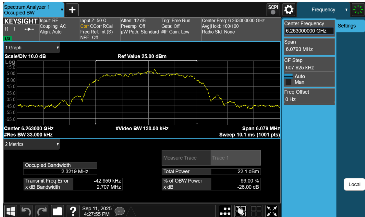
Plot 7-30. 26dB BW & 99% OBW Antenna WF7b (NB UNII HDR4, ePA- 6263MHz)
