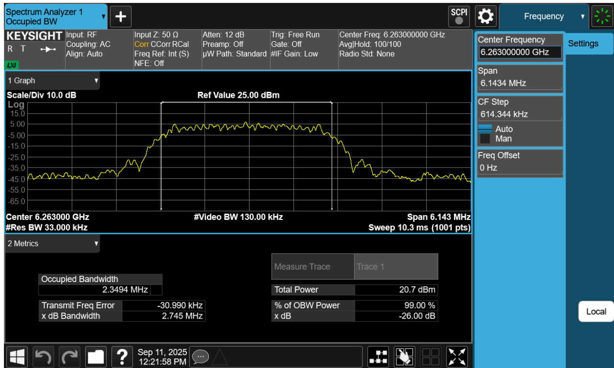
Plot 7-24. 26dB BW & 99% OBW Antenna WF2a (NB UNII HDT2, ePA- 6263MHz)
