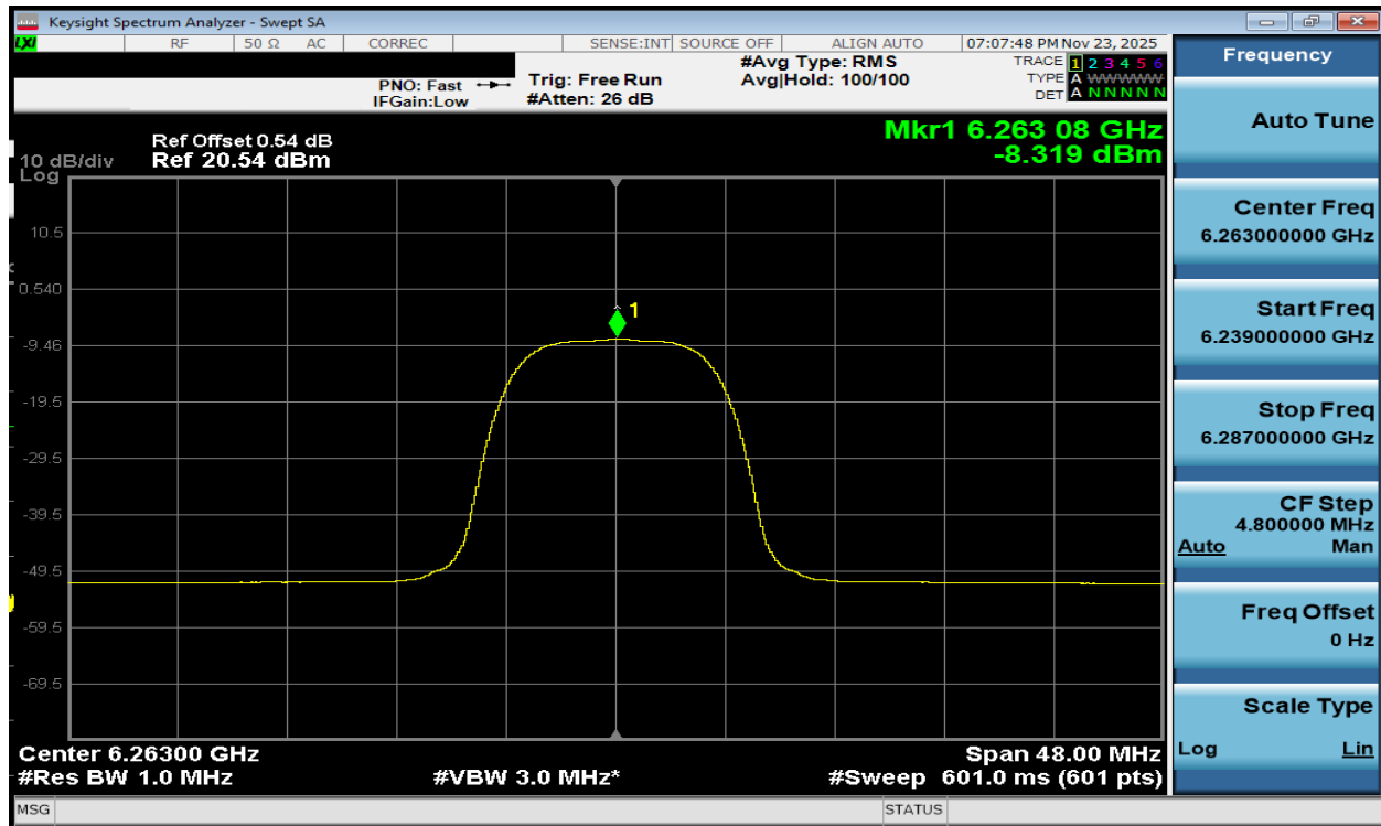
Plot 7-58. PSD Antenna WF7a (NB UNII HDRPL32, ePA – 6263MHz)
