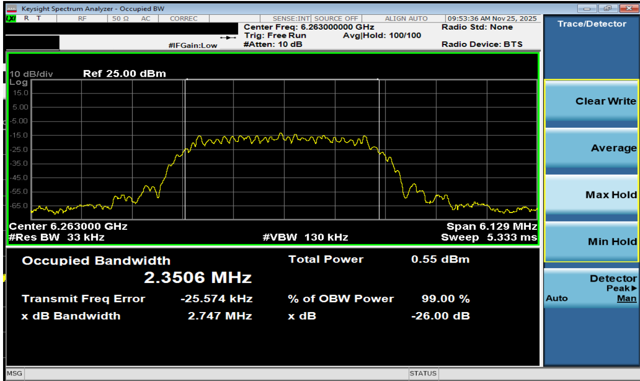
Plot 7-37. 26dB BW & 99% OBW Antenna WF7b (NB UNII HDT2, ePA- 6263MHz)
