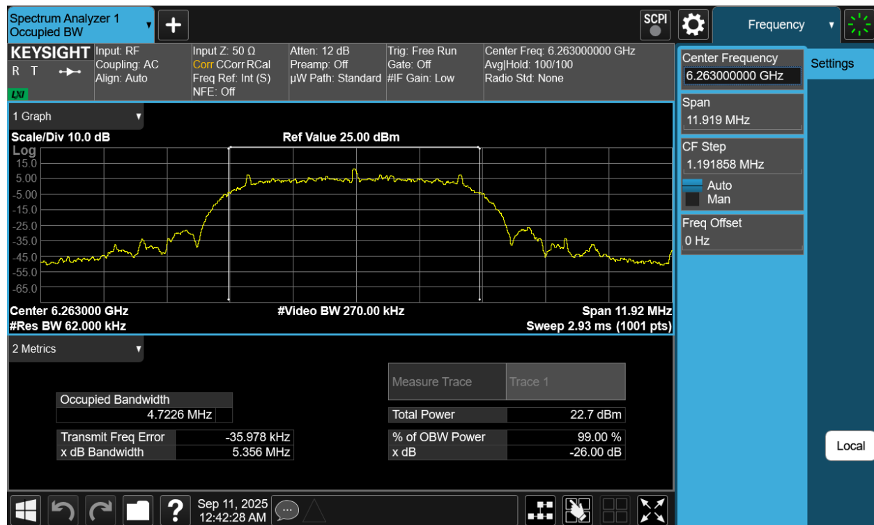
Plot 7-7. 26dB BW & 99% OBW Antenna WF7a (NB UNII XHDRPM6, ePA- 6263MHz)
