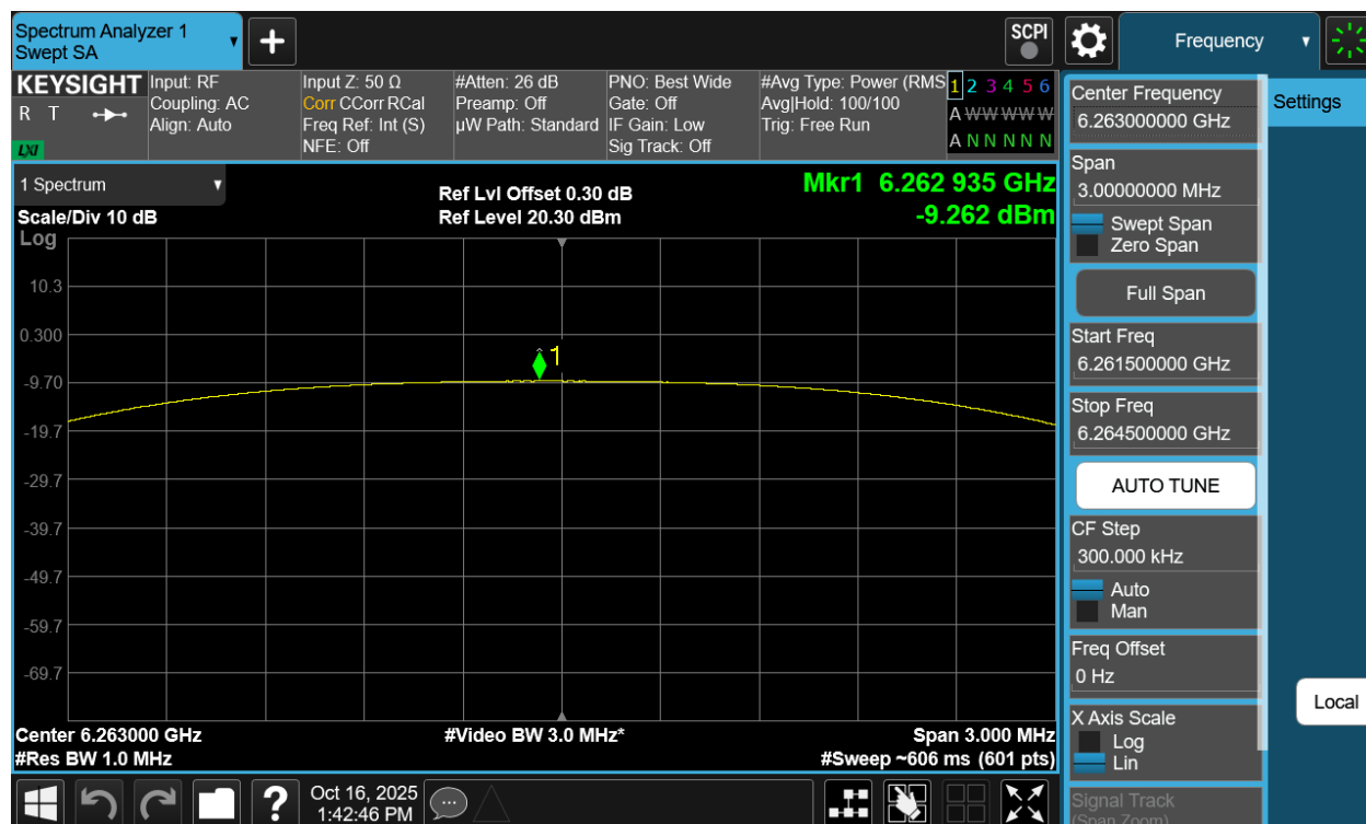
Plot 7-62. PSD Antenna WF7a (NB UNII HDT4, ePA – 6263MHz)
