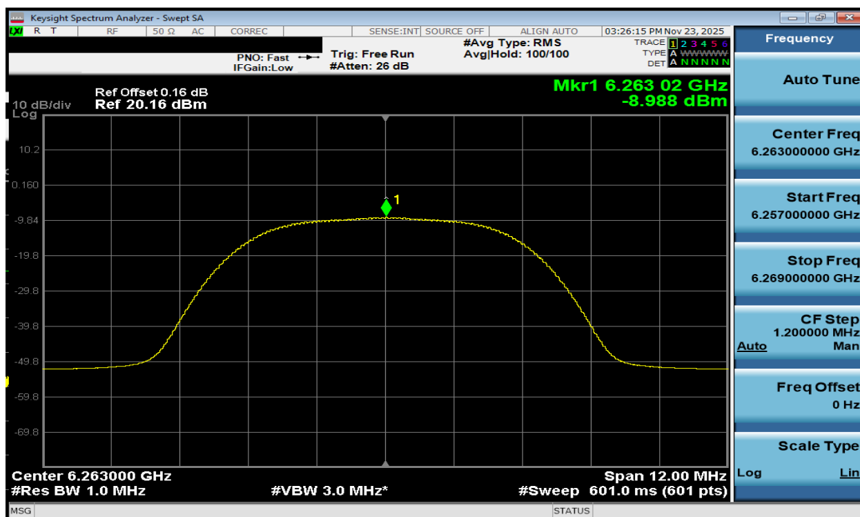
Plot 7-49. PSD Antenna WF7a (NB UNII HDR8, iPA - 6263MHz)
