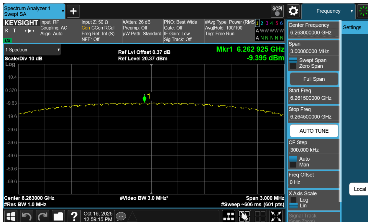
Plot 7-50. PSD Antenna WF7a (NB UNII HDRPS2, ePA – 6263MHz)
