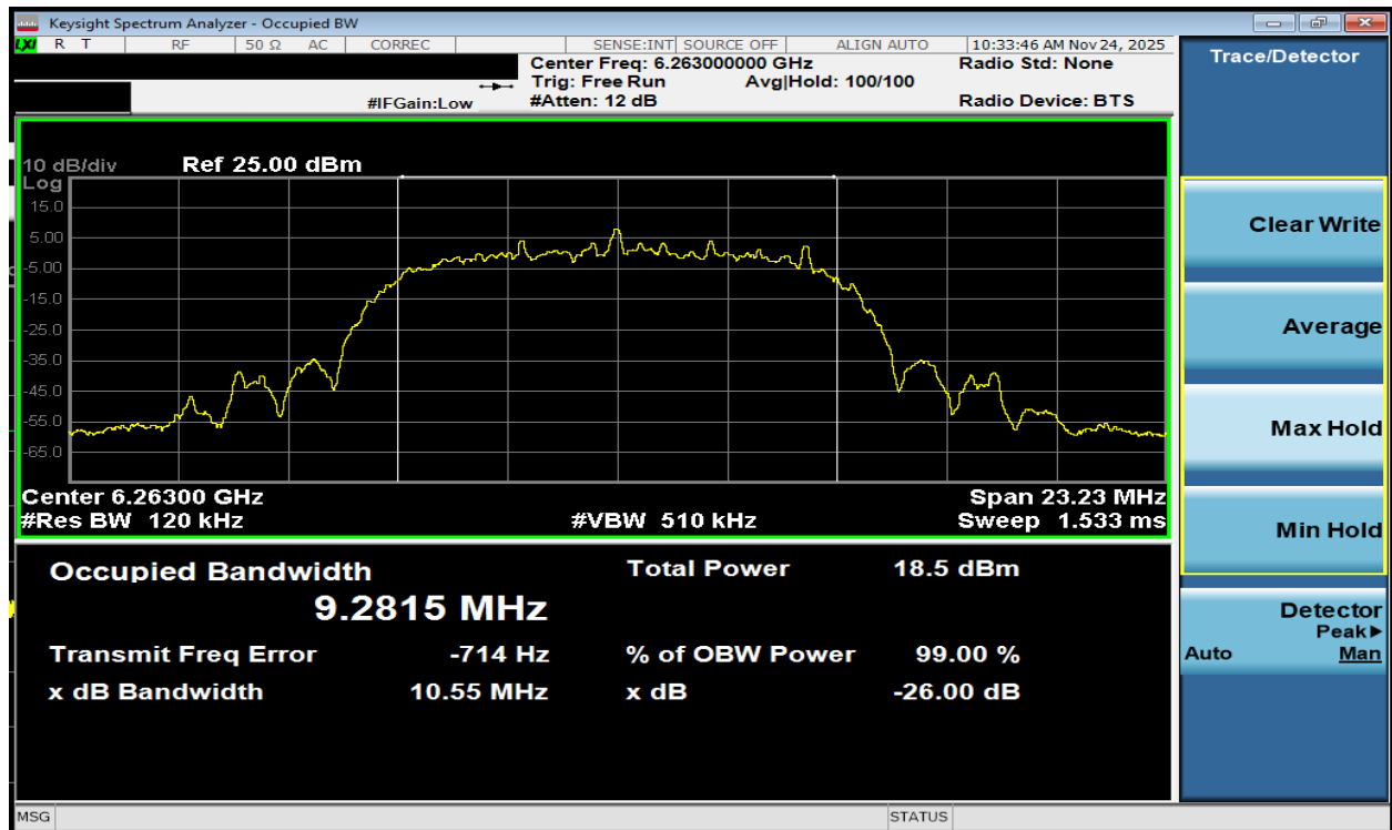
Plot 7-23. 26dB BW & 99% OBW Antenna WF2a (NB UNII HDRPL32, ePA- 6263MHz)
