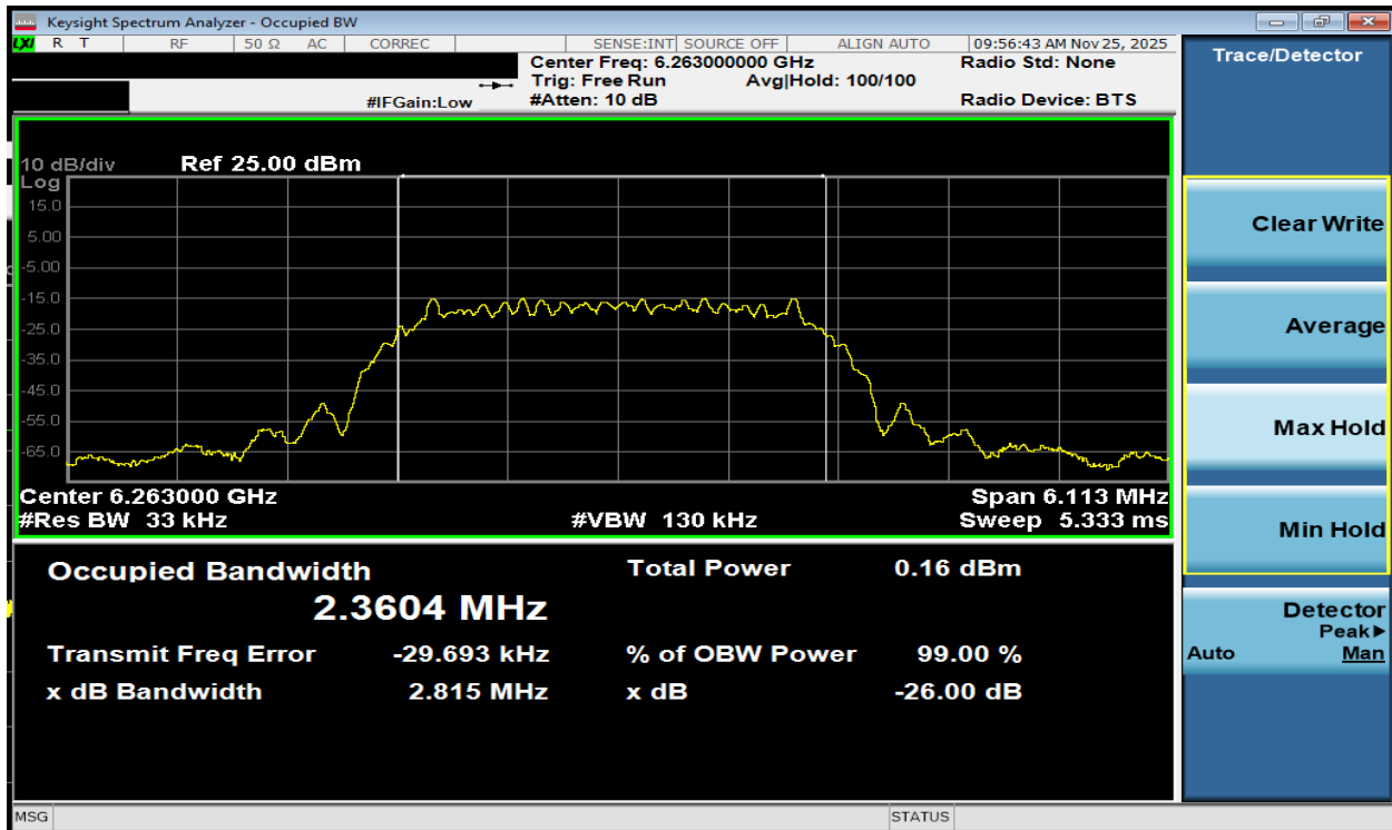
Plot 7-38. 26dB BW & 99% OBW Antenna WF7b (NB UNII HDT4, ePA- 6263MHz)
