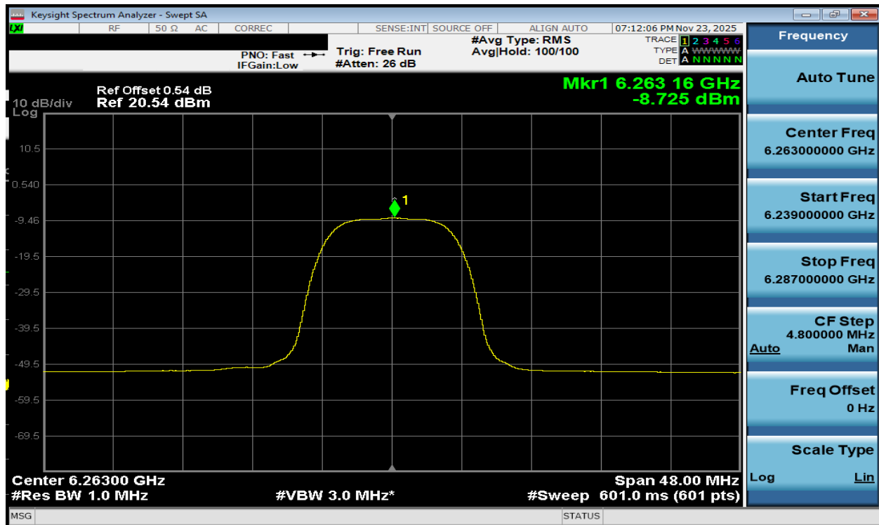
Plot 7-59. PSD Antenna WF7a (NB UNII HDRPL32, iPA – 6263MHz)
