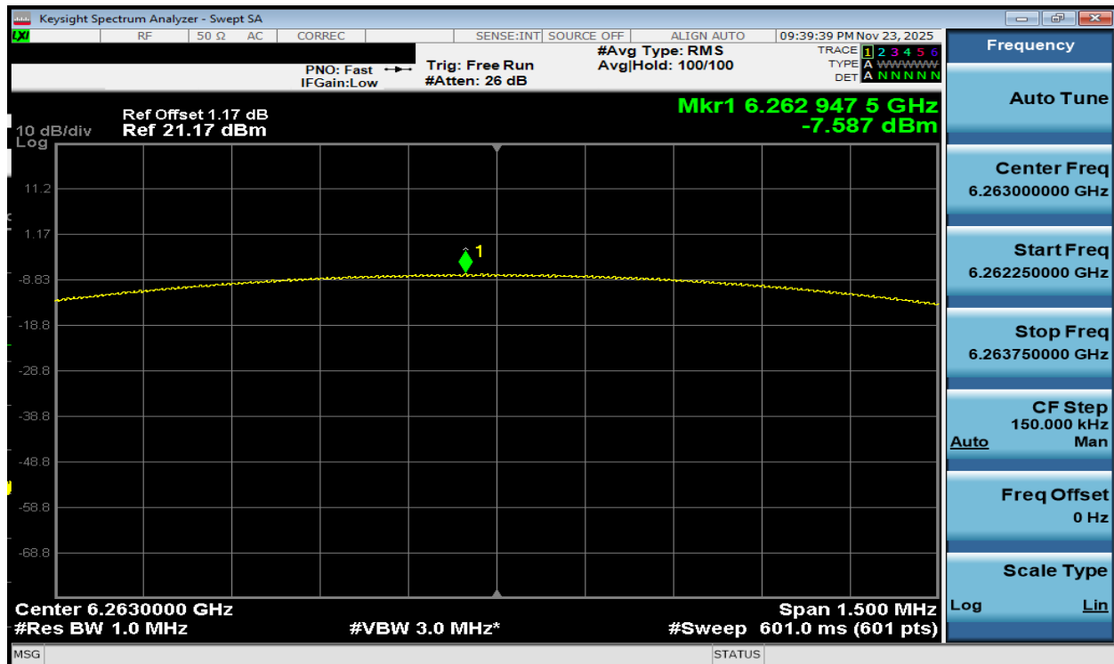
Plot 7-67. PSD Antenna WF2a (NB UNII BDR, iPA – 6263MHz)
