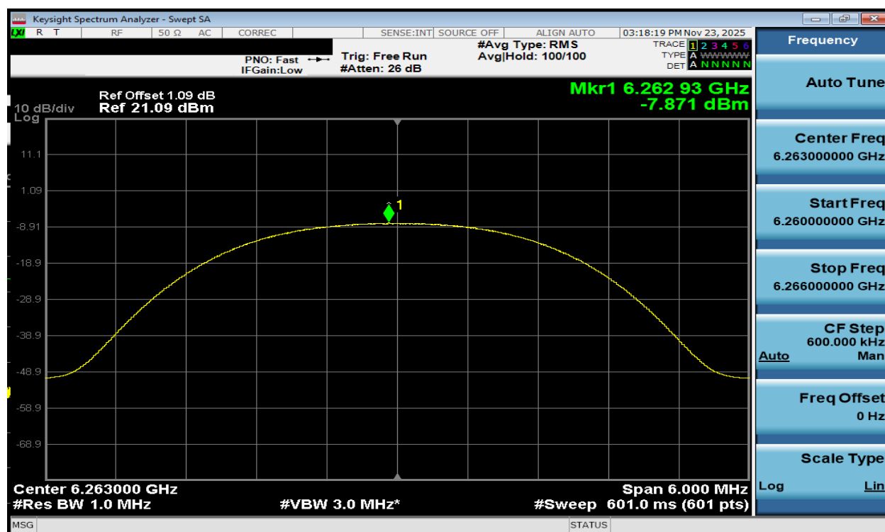
Plot 7-47. PSD Antenna WF7a (NB UNII HDR4, iPA – 6263MHz)
