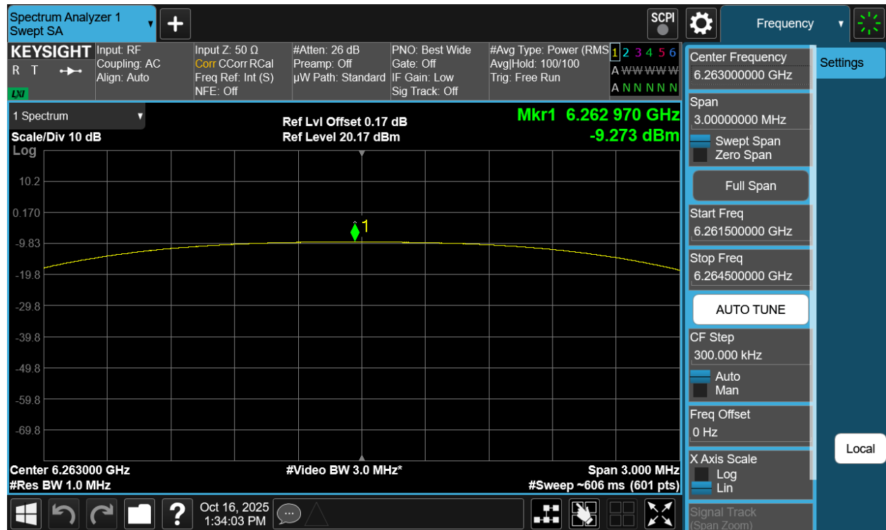
Plot 7-60. PSD Antenna WF7a (NB UNII HDT2, ePA – 6263MHz)
