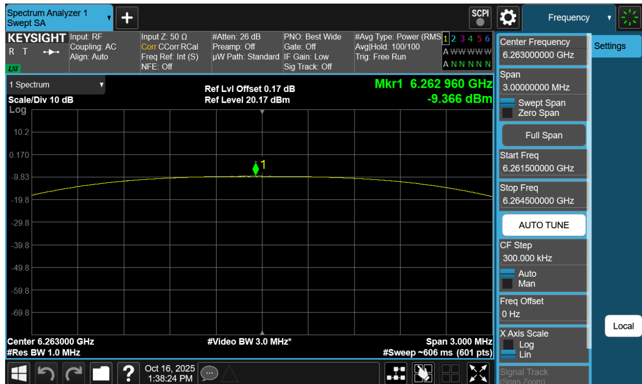
Plot 7-61. PSD Antenna WF7a (NB UNII HDT2, iPA – 6263MHz)
