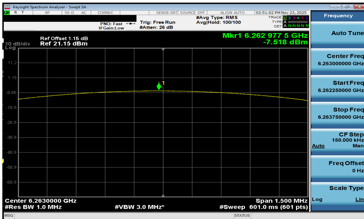
Plot 7-40. PSD Antenna WF7a (NB UNII BDR, ePA – 6263MHz)
