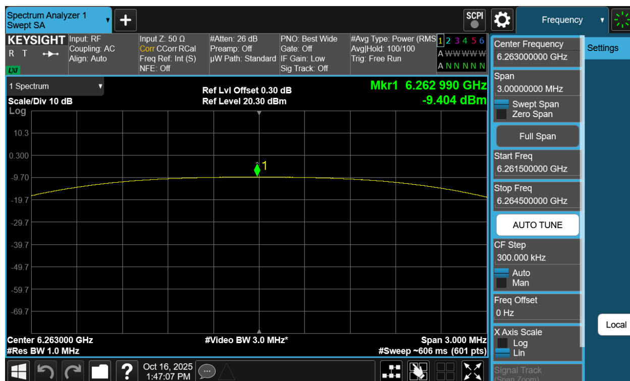
Plot 7-63. PSD Antenna WF7a (NB UNII HDT4, iPA – 6263MHz)
