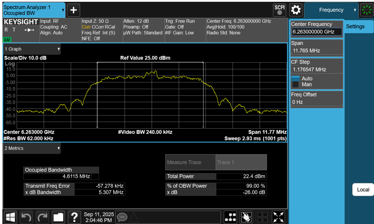
Plot 7-18. 26dB BW & 99% OBW Antenna WF2a (NB UNII HDR8, ePA- 6263MHz)
