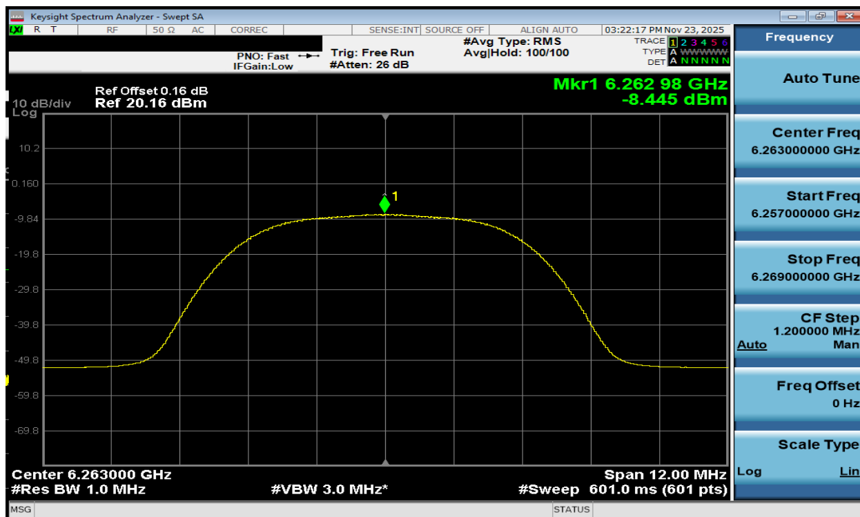
Plot 7-48. PSD Antenna WF7a (NB UNII HDR8, ePA - 6263MHz)
