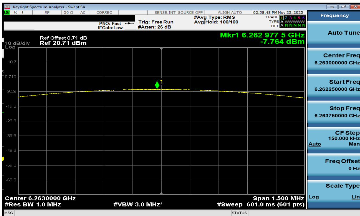
Plot 7-42. PSD Antenna WF7a (NB UNII LE1M, ePA – 6263MHz)
