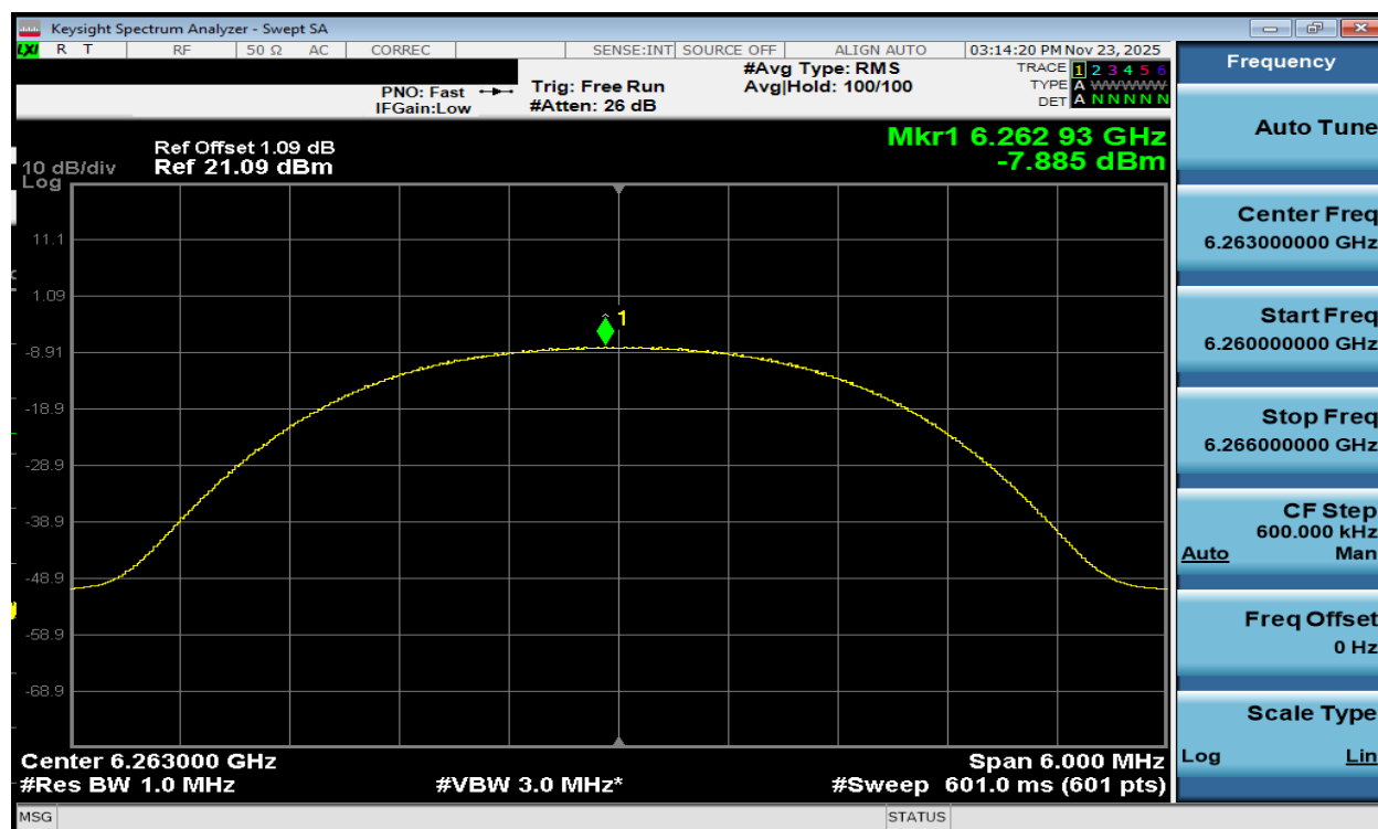
Plot 7-46. PSD Antenna WF7a (NB UNII HDR4, ePA – 6263MHz)
