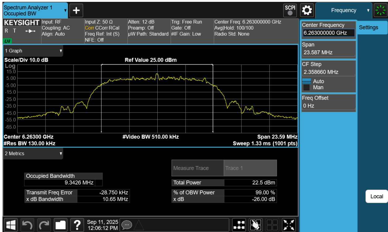
Plot 7-22. 26dB BW & 99% OBW Antenna WF2a (NB UNII HDRPL12, ePA- 6263MHz)
