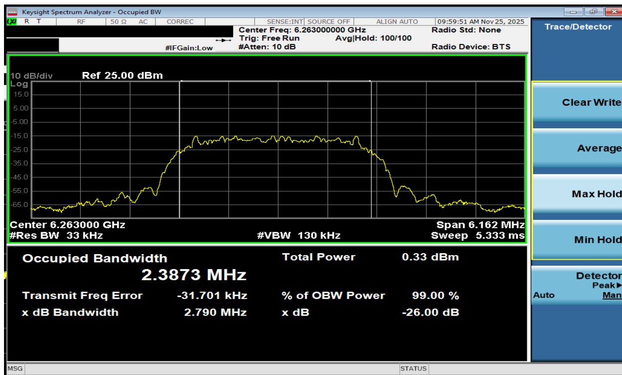
Plot 7-39. 26dB BW & 99% OBW Antenna WF7b (NB UNII HDT6, ePA- 6263MHz)
