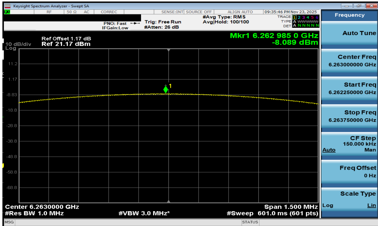
Plot 7-66. PSD Antenna WF2a (NB UNII BDR, ePA – 6263MHz)
