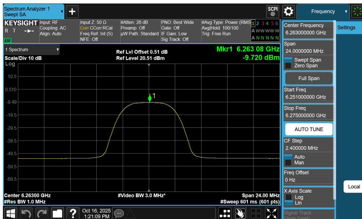
Plot 7-55. PSD Antenna WF7a (NB UNII HDRPM16, iPA – 6263MHz)
