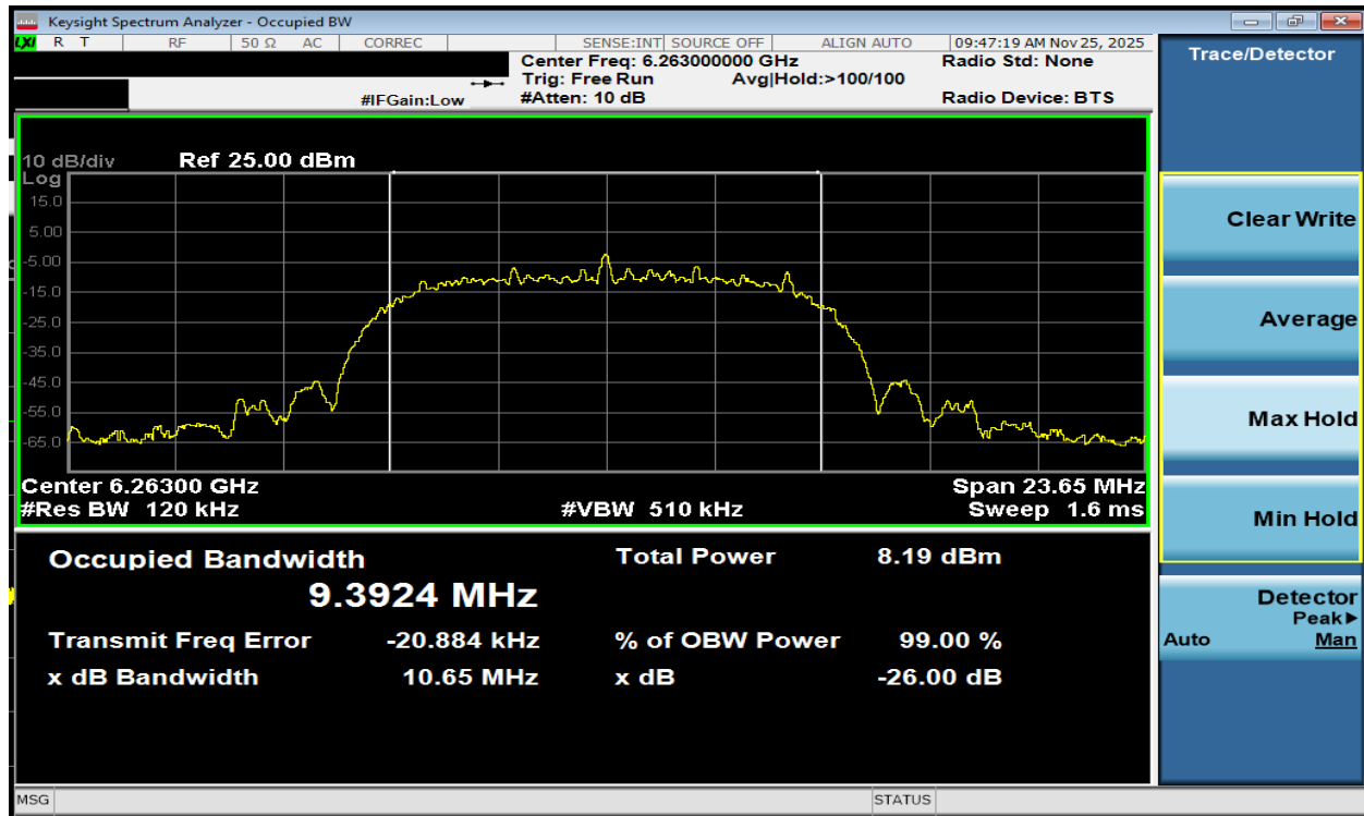
Plot 7-35. 26dB BW & 99% OBW Antenna WF7b (NB UNII HDRPL12, ePA- 6263MHz)
