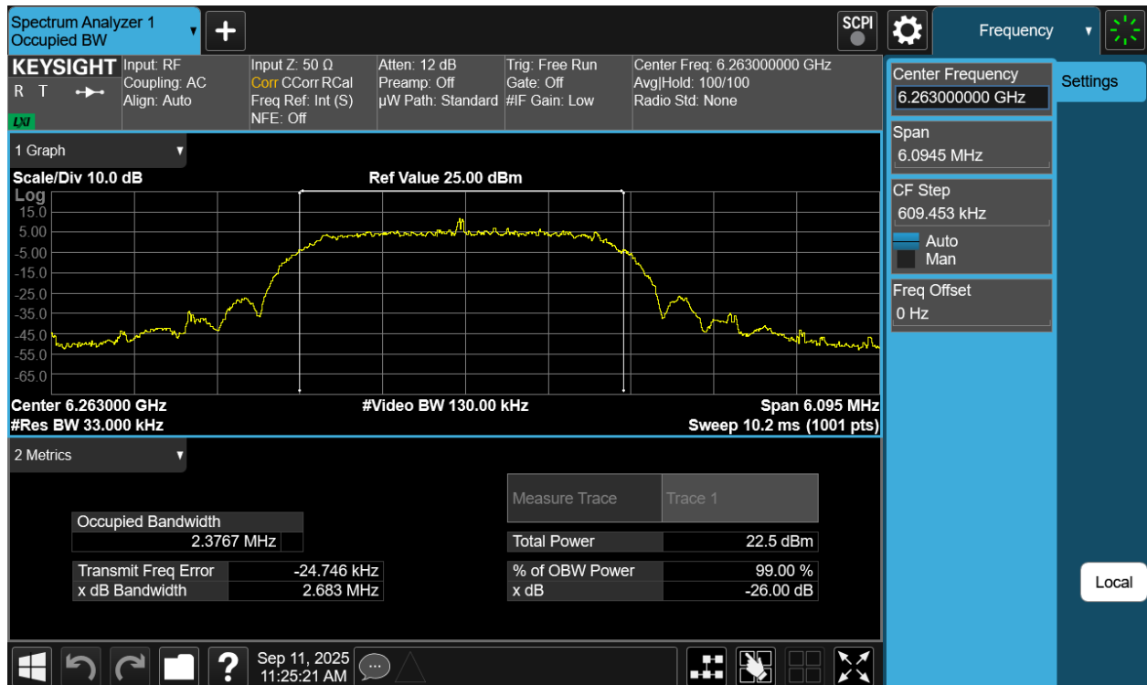
Plot 7-19. 26dB BW & 99% OBW Antenna WF2a (NB UNII HDRPS2, ePA- 6263MHz)
