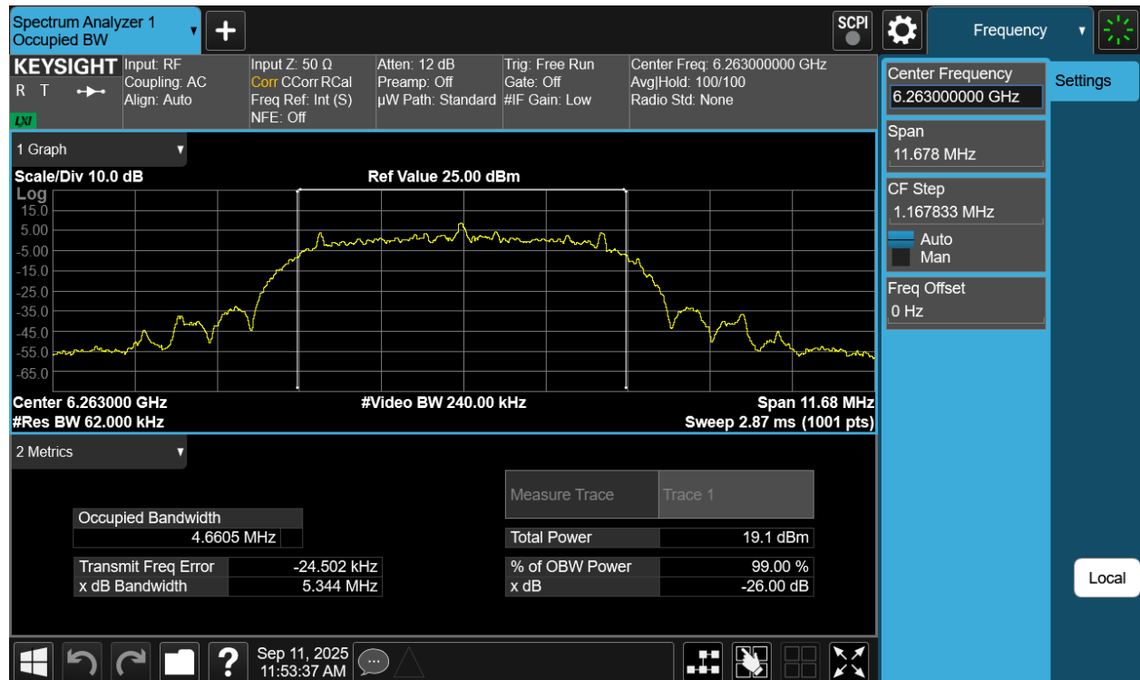
Plot 7-21. 26dB BW & 99% OBW Antenna WF2a (NB UNII HDRPM16, ePA- 6263MHz)
