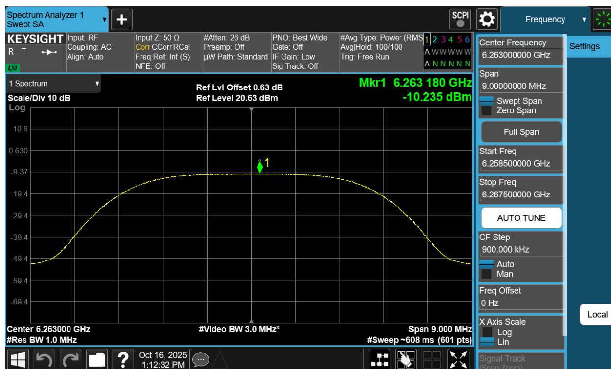
Plot 7-53. PSD Antenna WF7a (NB UNII XHDRPM6, iPA – 6263MHz)
