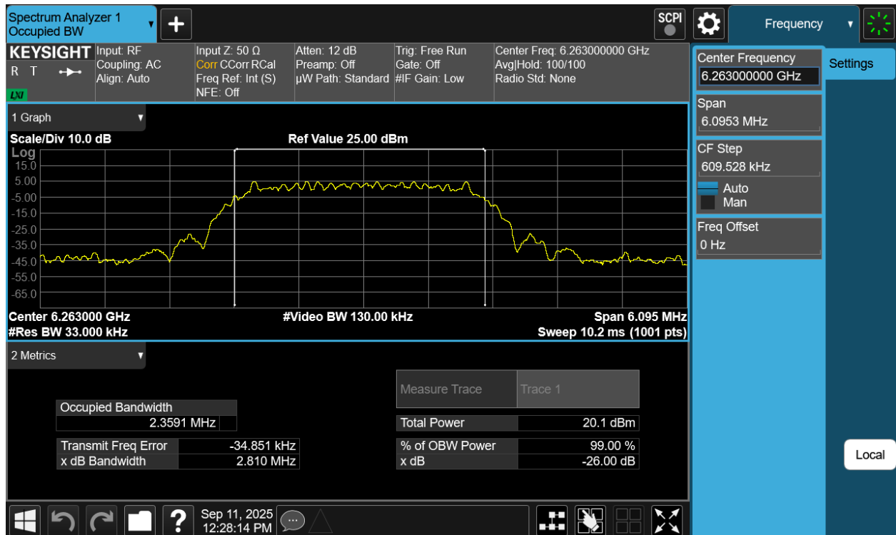
Plot 7-25. 26dB BW & 99% OBW Antenna WF2a (NB UNII HDT4, ePA- 6263MHz)
