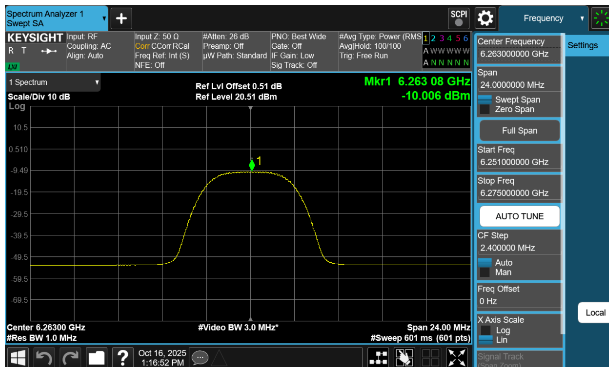
Plot 7-54. PSD Antenna WF7a (NB UNII HDRPM16, ePA – 6263MHz)
