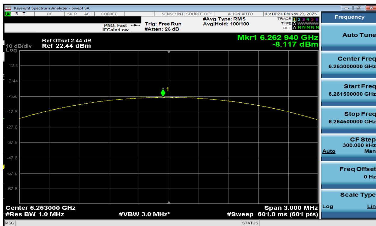
Plot 7-45. PSD Antenna WF7a (NB UNII LE2M, iPA – 6263MHz)
