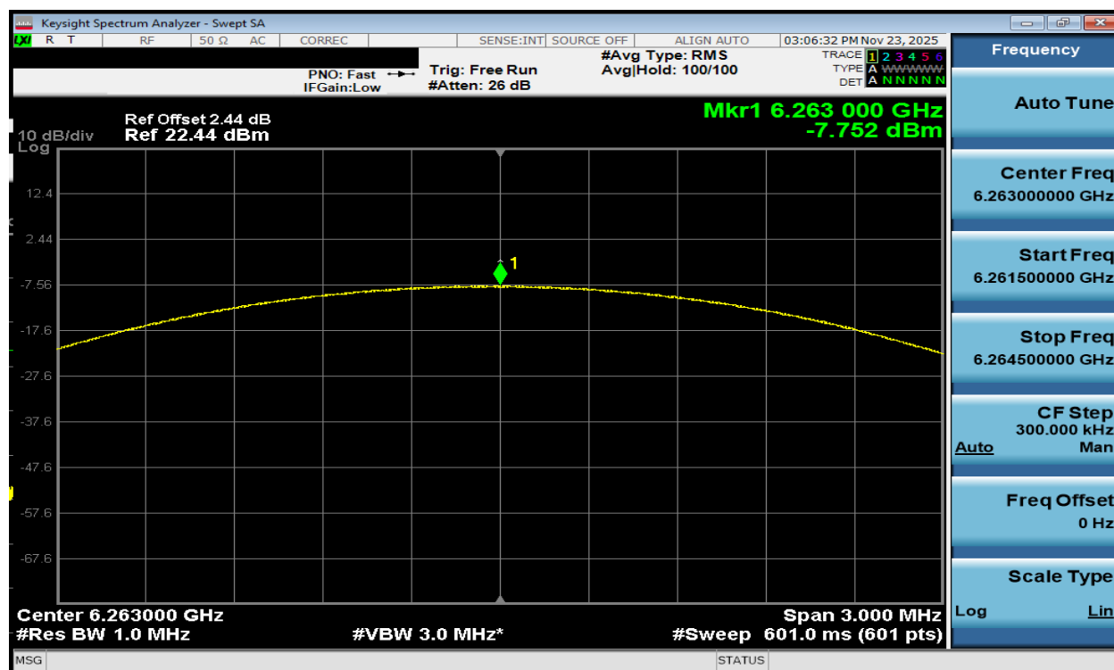
Plot 7-44. PSD Antenna WF7a (NB UNII LE2M, ePA – 6263MHz)
