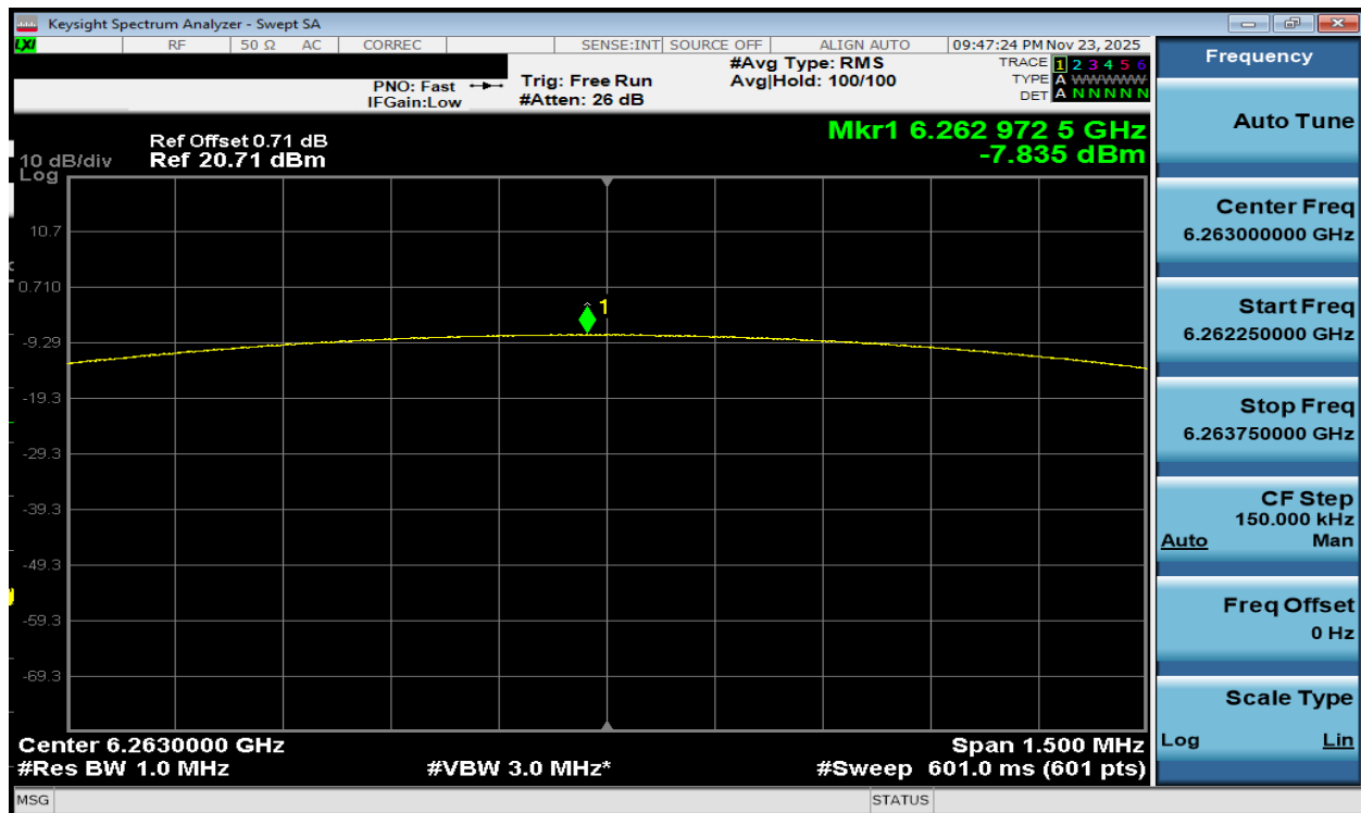
Plot 7-69. PSD Antenna WF2a (NB UNII LE1M, iPA – 6263MHz)
