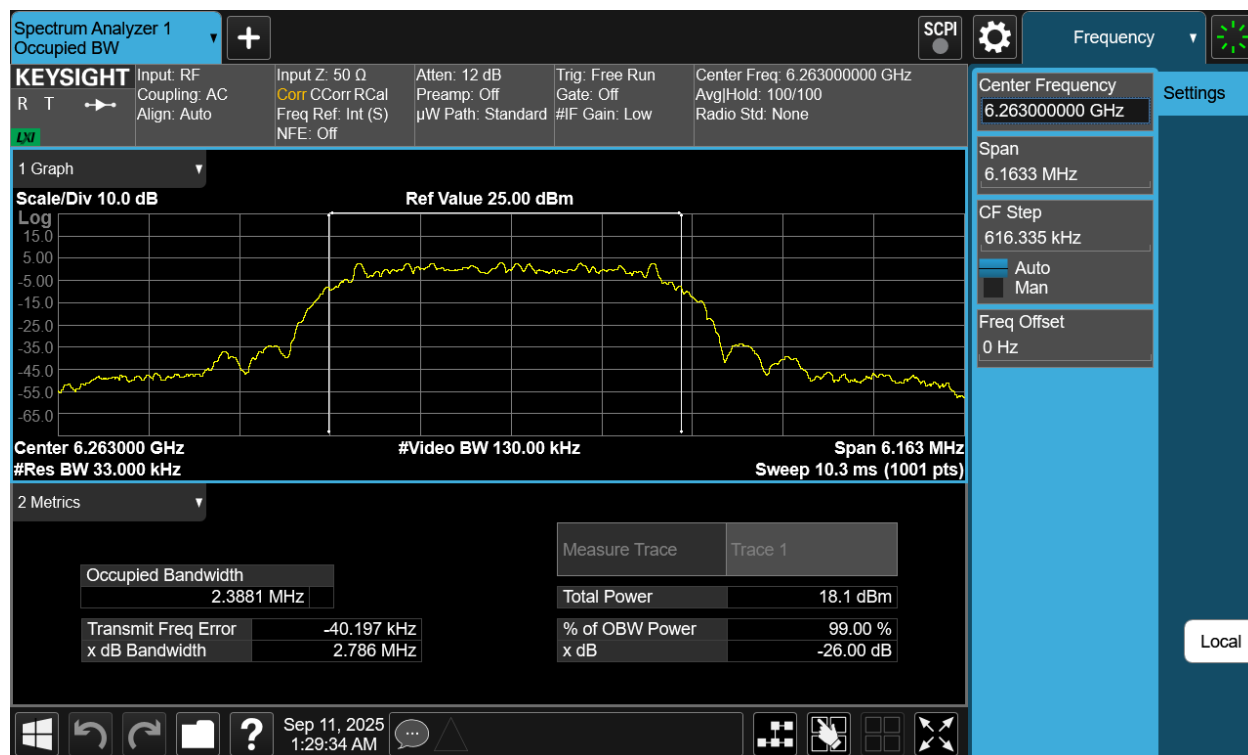
Plot 7-13. 26dB BW & 99% OBW Antenna WF7a (NB UNII HDT6, ePA- 6263MHz)
