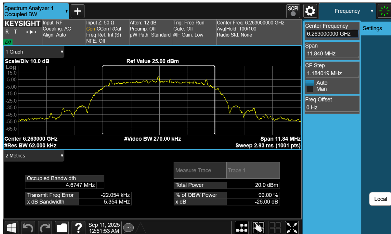
Plot 7-8. 26dB BW & 99% OBW Antenna WF7a (NB UNII HDRPM16, ePA- 6263MHz)
