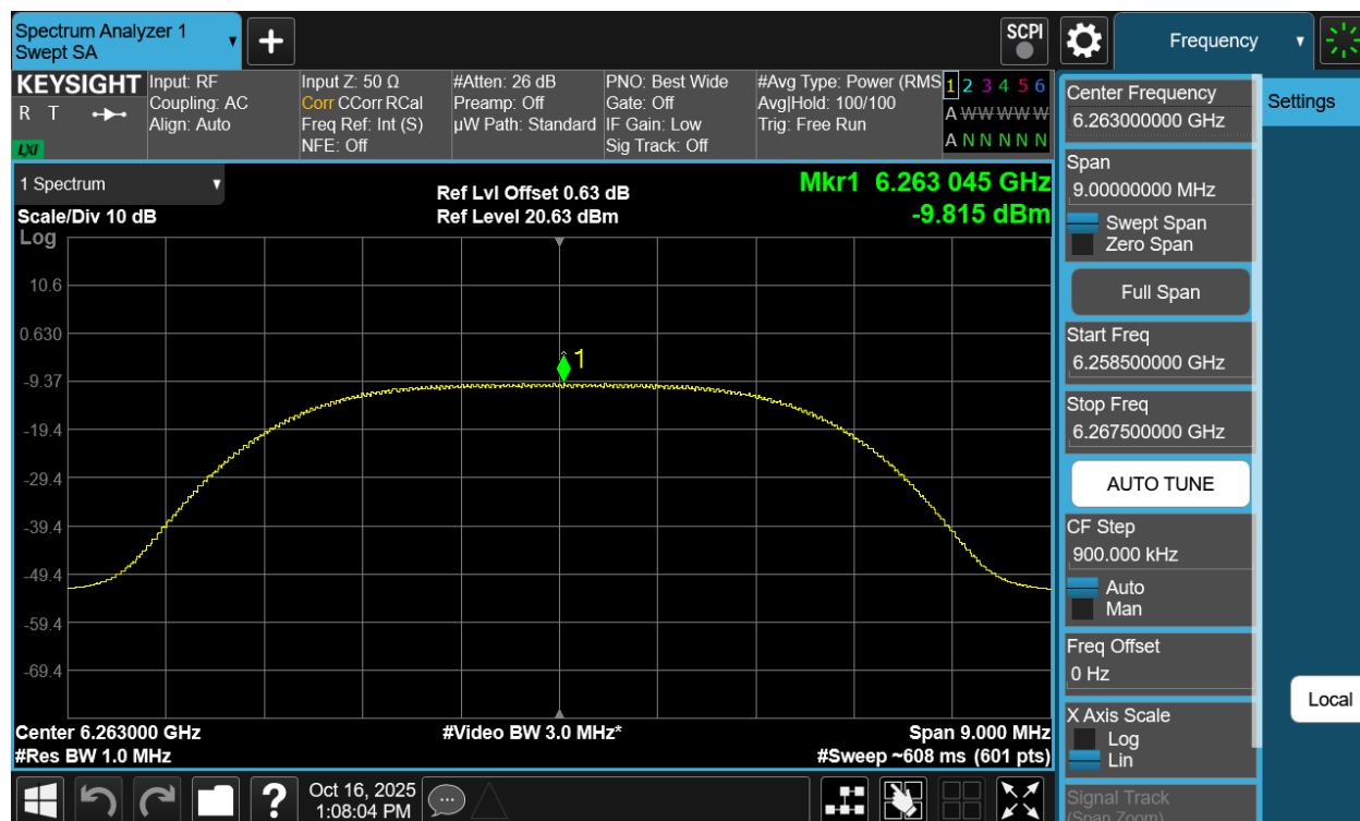
Plot 7-52. PSD Antenna WF7a (NB UNII XHDRPM6, ePA – 6263MHz)
