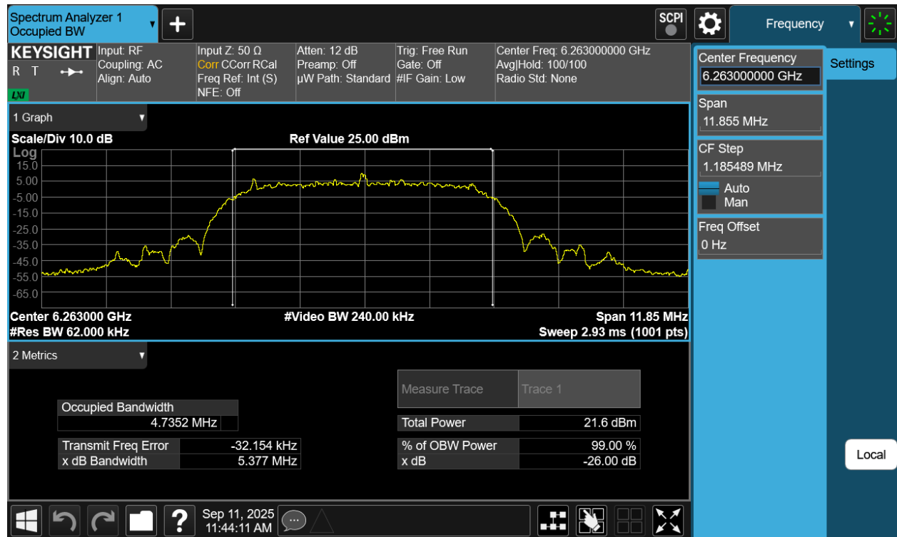
Plot 7-20. 26dB BW & 99% OBW Antenna WF2a (NB UNII XHDRPM6, ePA- 6263MHz)
