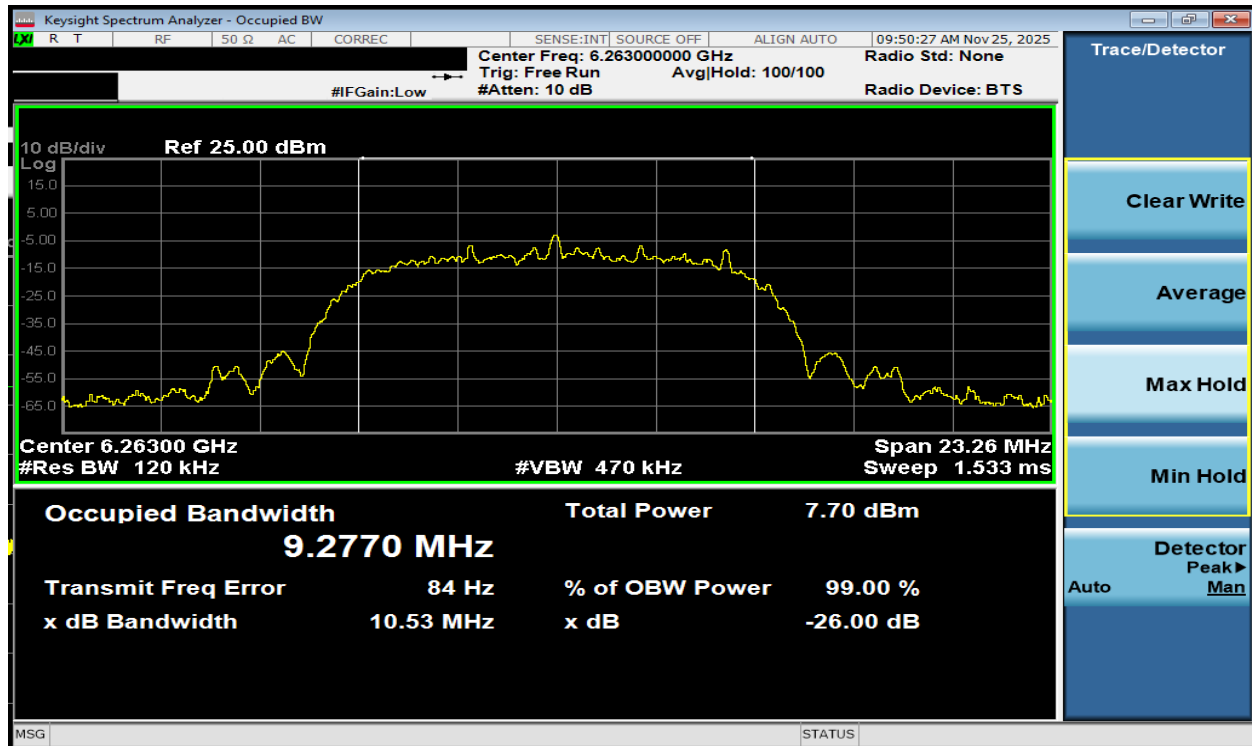
Plot 7-36. 26dB BW & 99% OBW Antenna WF7b (NB UNII HDRPL32, ePA- 6263MHz)
