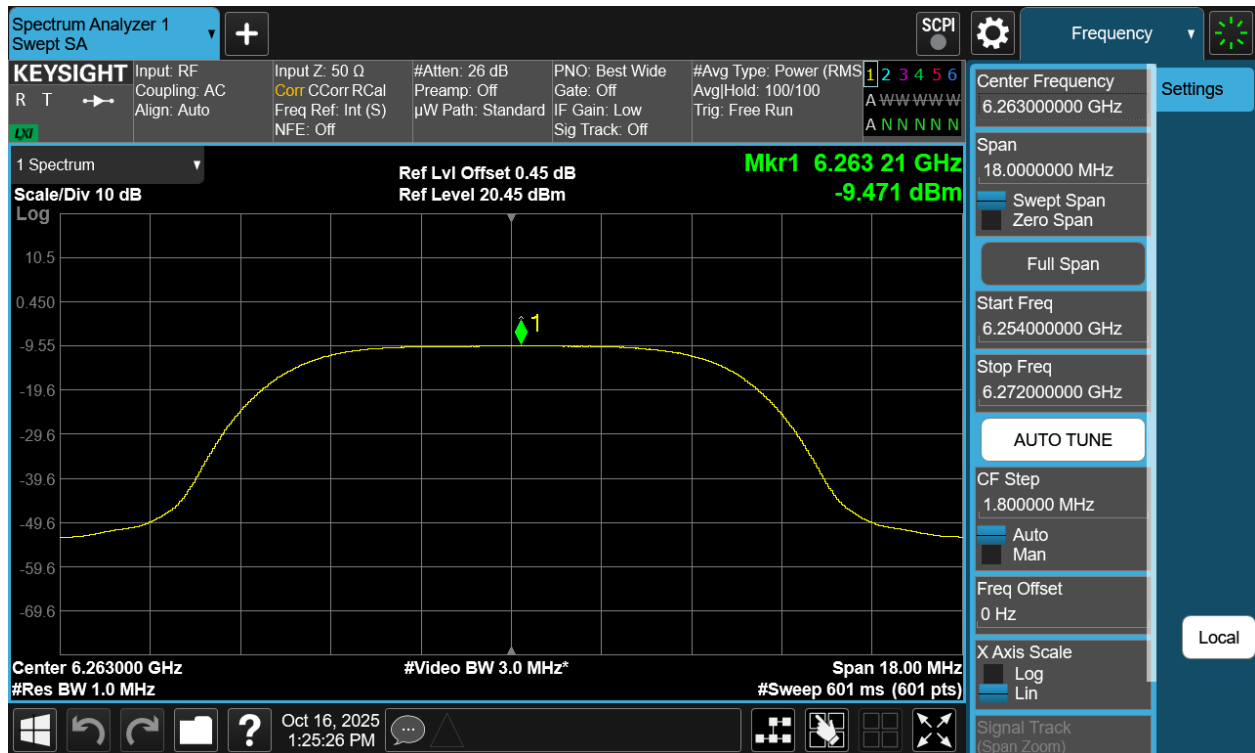
Plot 7-56. PSD Antenna WF7a (NB UNII HDRPL12, ePA – 6263MHz)
