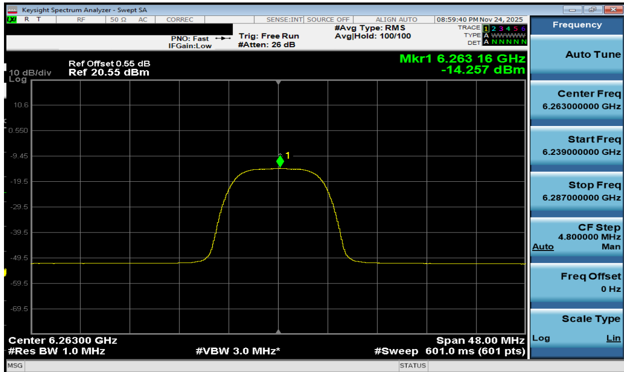
Plot 7-208. PSD TxBF Diversity Antenna WF2a (NB UNII HDRPL32, iPA – 6263MHz)
