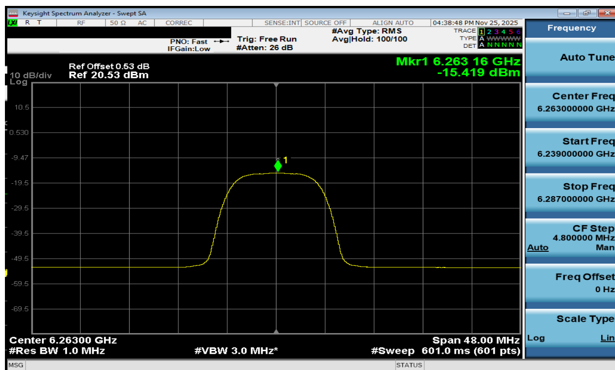
Plot 7-207. PSD TxBF Diversity Antenna WF7b (NB UNII HDRPL32, ePA – 6263MHz)
