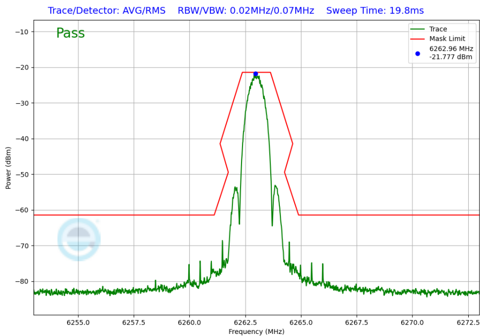
Plot 7-224. In-Band Emission Antenna WF7a (NB UNII LE1M, ePA – 6263MHz)
