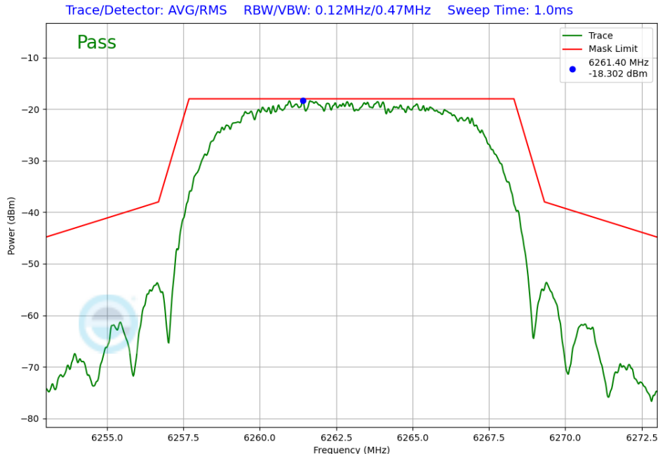
Plot 7-239. In-Band Emission Antenna WF7a (NB UNII HDRPL12, iPA – 6263MHz)
