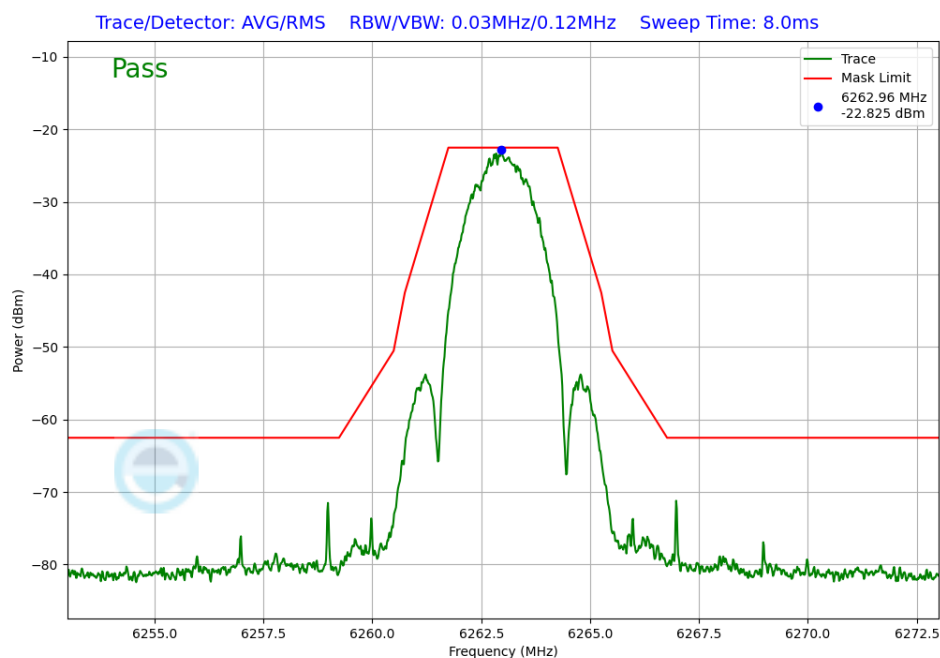
Plot 7-226. In-Band Emission Antenna WF7a (NB UNII LE2M, ePA – 6263MHz)
