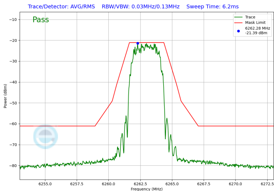
Plot 7-228. In-Band Emission Antenna WF7a (NB UNII HDR4, ePA – 6263MHz)
