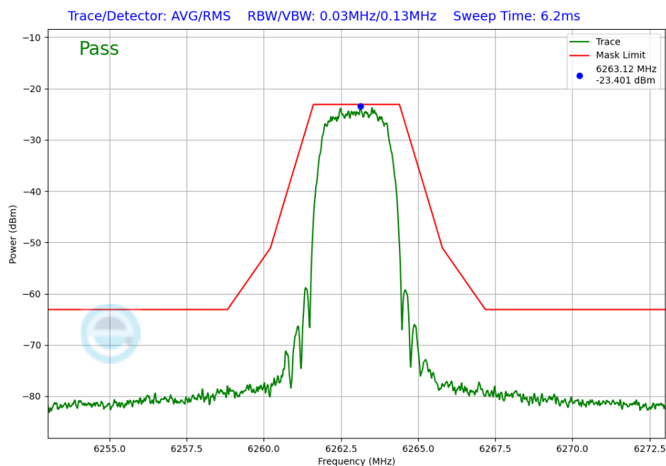
Plot 7-246. In-Band Emission Antenna WF7a (NB UNII HDT6, ePA – 6263MHz)
