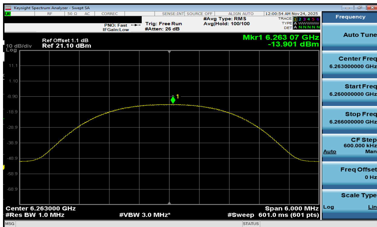
Plot 7-184. PSD TxBF Diversity Antenna WF2a (NB UNII HDR4, iPA - 6263MHz)
