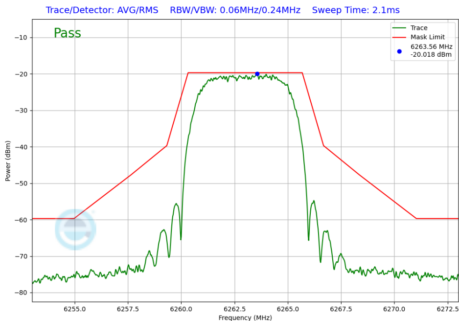
Plot 7-236. In-Band Emission Antenna WF7a (NB UNII HDRPM16, ePA – 6263MHz)
