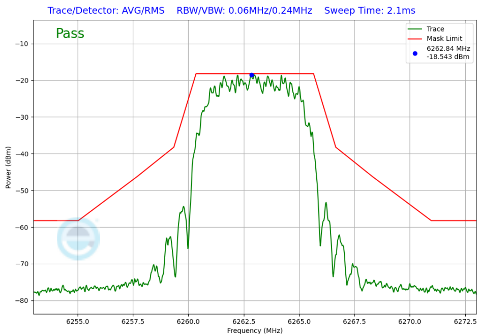
Plot 7-230. In-Band Emission Antenna WF7a (NB UNII HDR8, ePA – 6263MHz)
