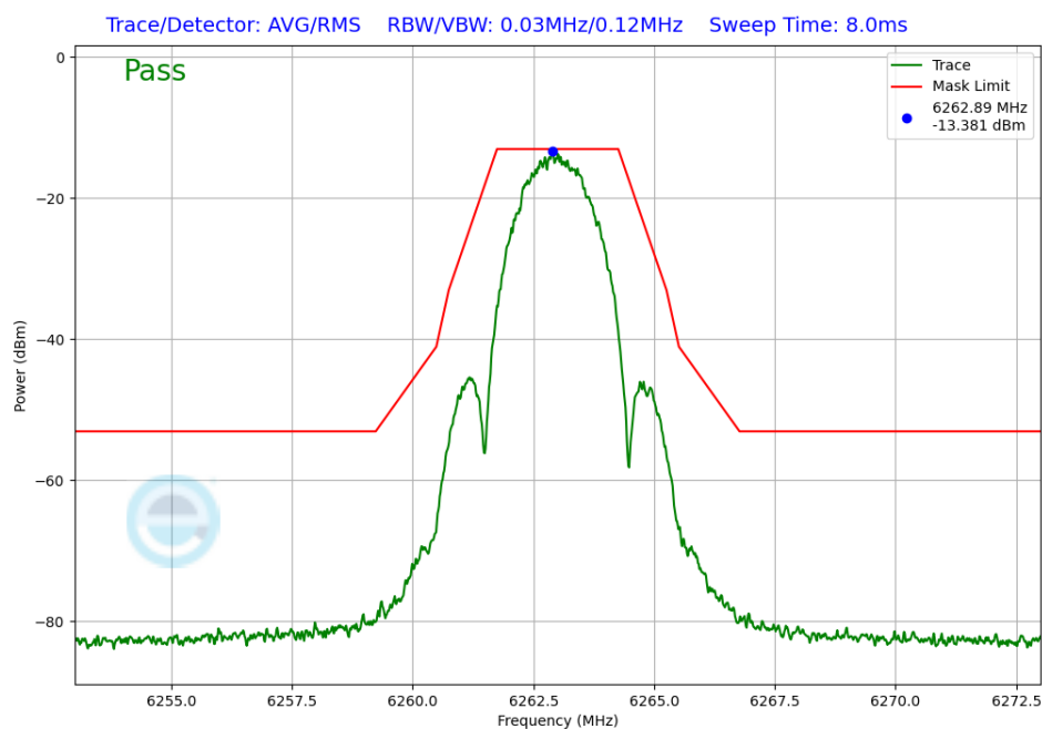
Plot 7-253. In-Band Emission Antenna WF2a (NB UNII LE2M, iPA – 6263MHz)
