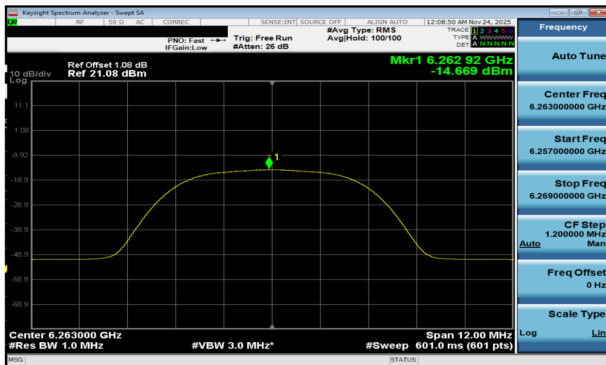
Plot 7-188. PSD TxBF Diversity Antenna WF2a (NB UNII HDR8, iPA – 6263MHz)
