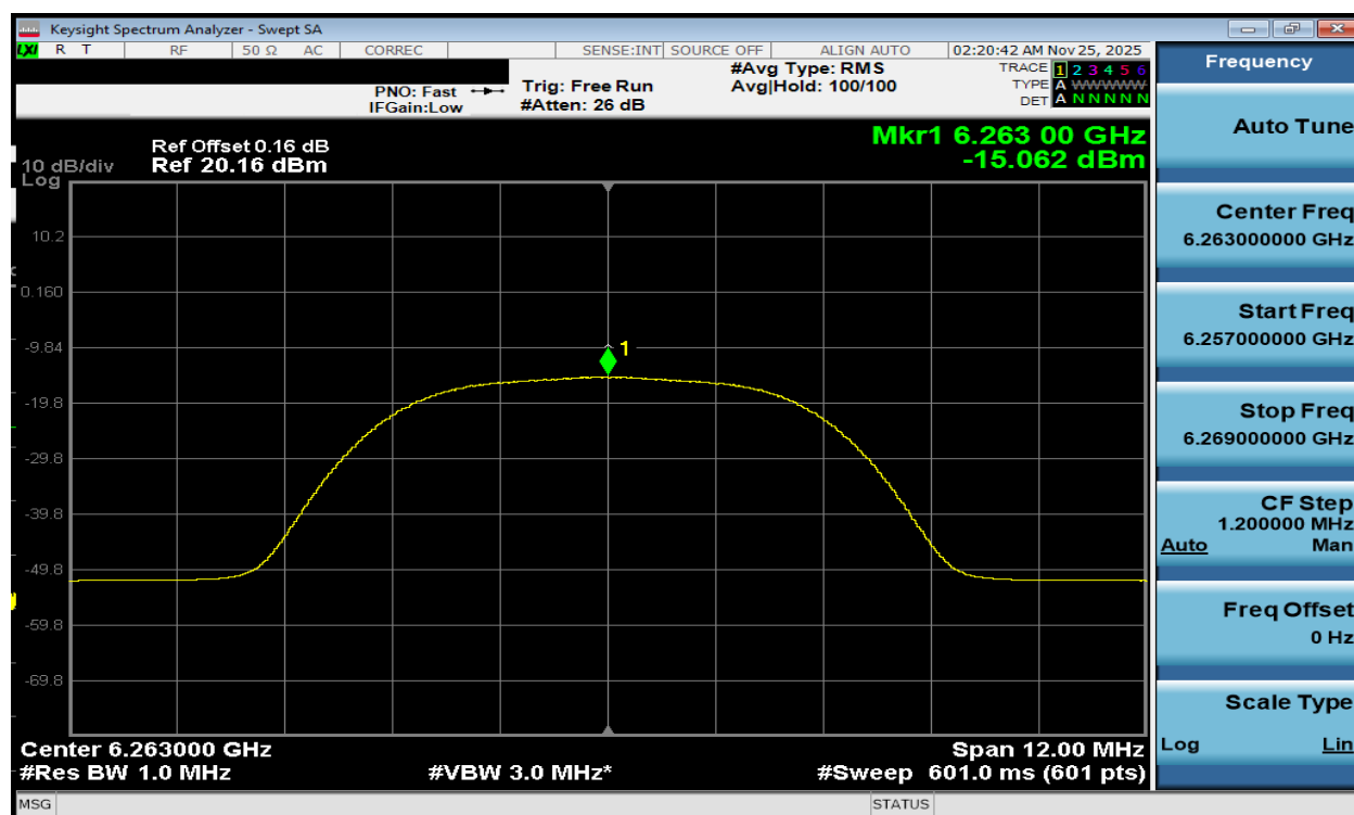
Plot 7-189. PSD TxBF Diversity Antenna WF7b (NB UNII HDR8, iPA – 6263MHz)
