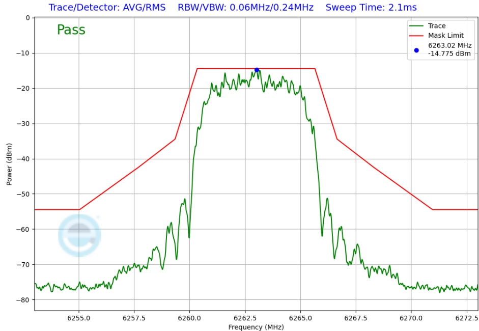
Plot 7-257. In-Band Emission Antenna WF2a (NB UNII HDR8, iPA – 6263MHz)
