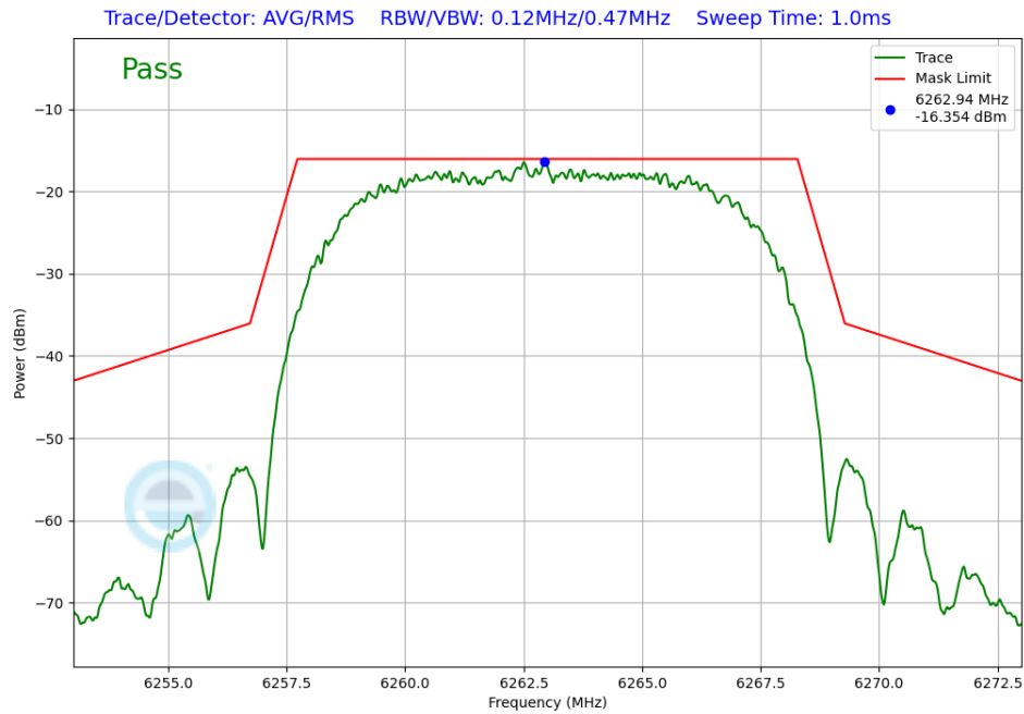
Plot 7-240. In-Band Emission Antenna WF7a (NB UNII HDRPL32, ePA – 6263MHz)
