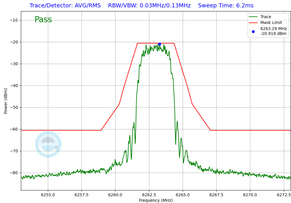
Plot 7-229. In-Band Emission Antenna WF7a (NB UNII HDR4, iPA – 6263MHz)
