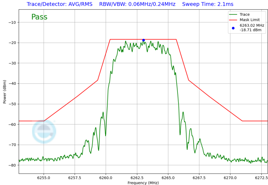
Plot 7-231. In-Band Emission Antenna WF7a (NB UNII HDR8, iPA – 6263MHz)
