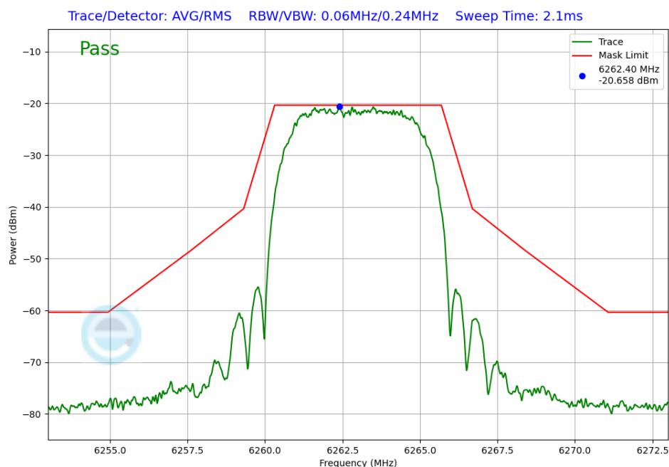
Plot 7-261. In-Band Emission Antenna WF2a (NB UNII XHDRPM6, iPA – 6263MHz)
