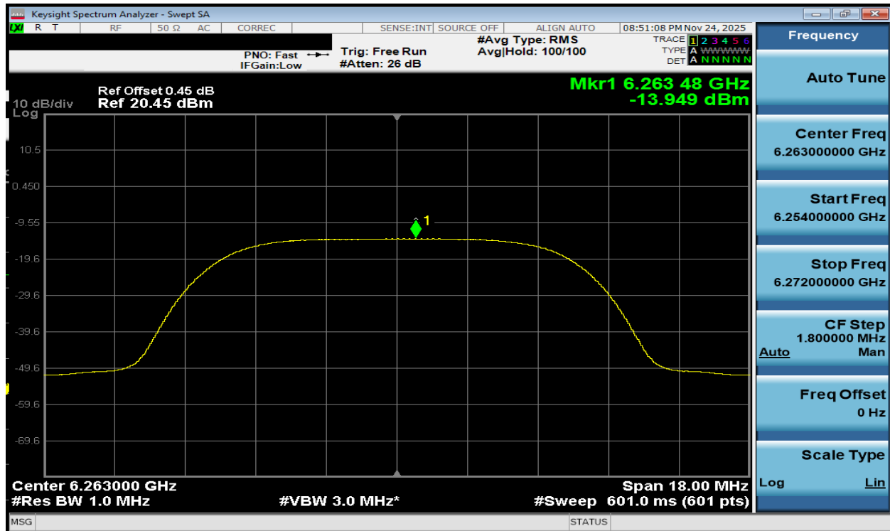
Plot 7-204. PSD TxBF Diversity Antenna WF2a (NB UNII HDRPL12, iPA – 6263MHz)
