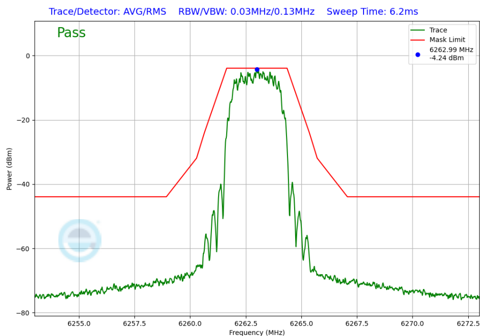
Plot 7-254. In-Band Emission Antenna WF2a (NB UNII HDR4, ePA – 6263MHz)
