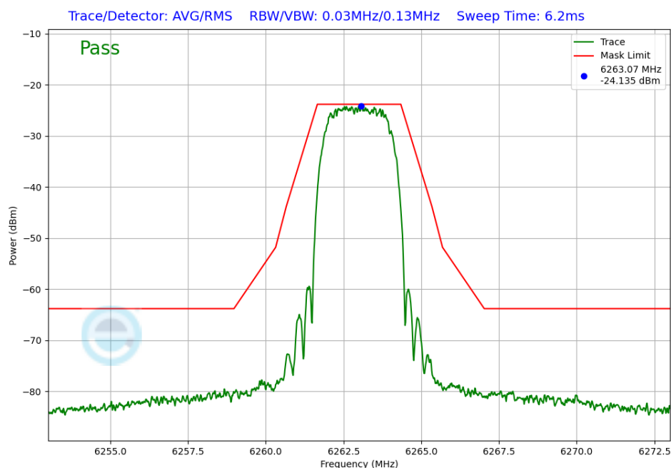
Plot 7-233. In-Band Emission Antenna WF7a (NB UNII HDRPS2, iPA – 6263MHz)
