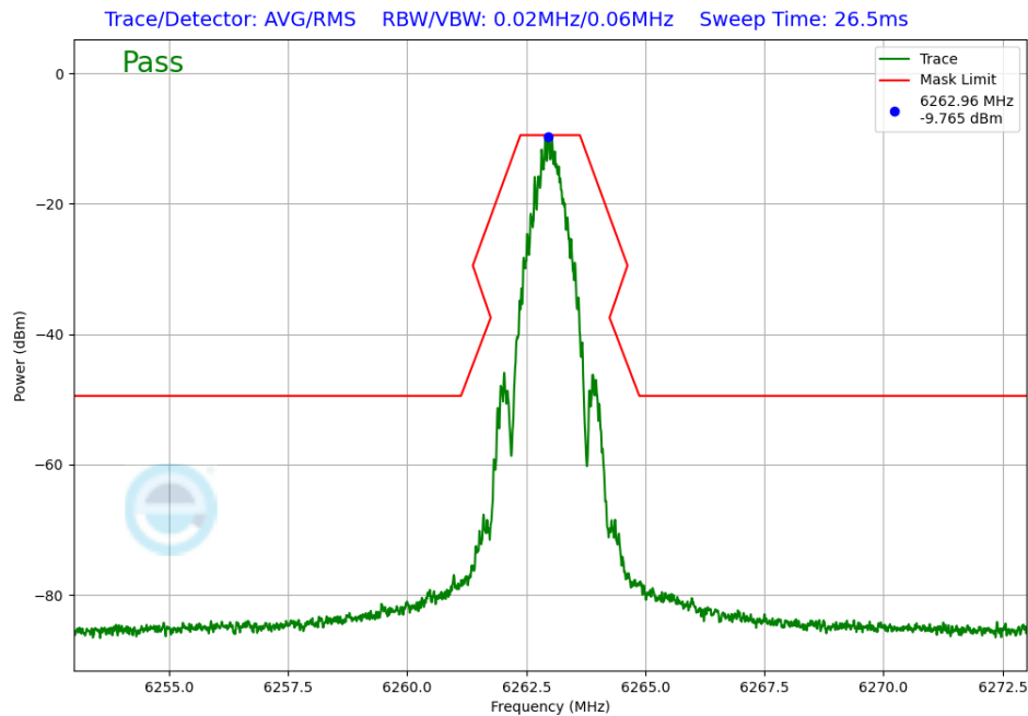
Plot 7-249. In-Band Emission Antenna WF2a (NB UNII BDR, iPA – 6263MHz)
