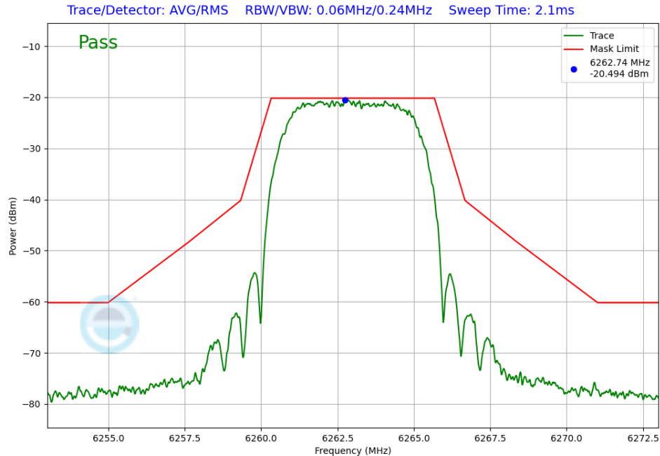
Plot 7-263. In-Band Emission Antenna WF2a (NB UNII HDRPM16, iPA – 6263MHz)
