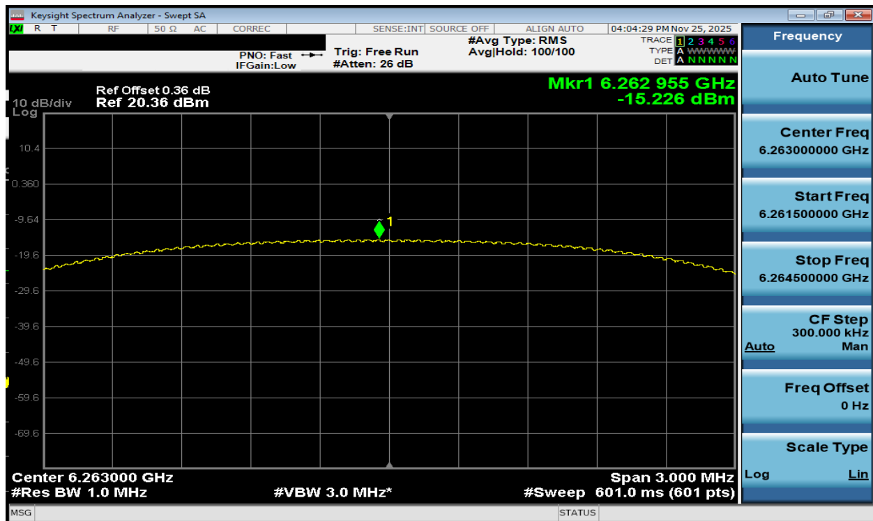
Plot 7-191. PSD TxBF Diversity Antenna WF7b (NB UNII HDRPS2, ePA – 6263MHz)
