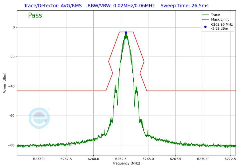
Plot 7-248. In-Band Emission Antenna WF2a (NB UNII BDR, ePA – 6263MHz)
