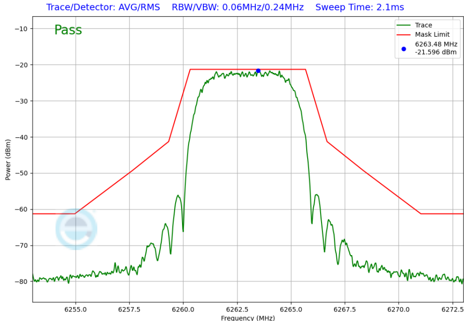
Plot 7-237. In-Band Emission Antenna WF7a (NB UNII HDRPM16, iPA – 6263MHz)
