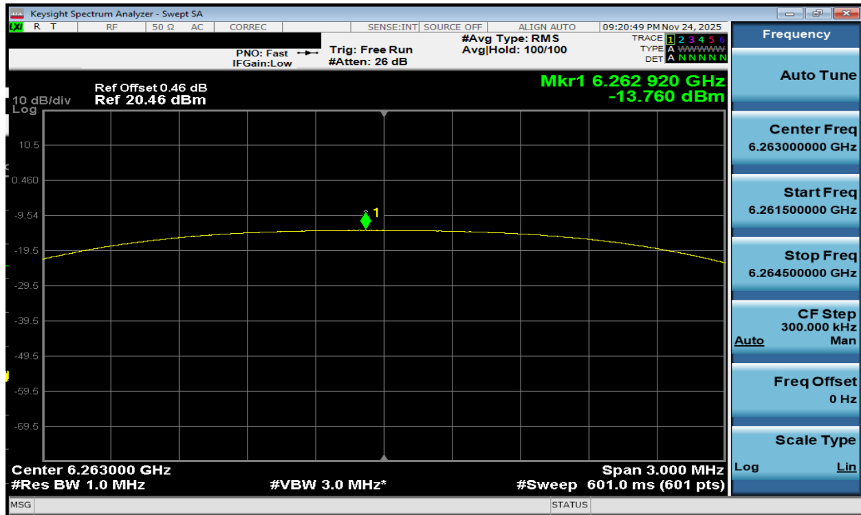
Plot 7-218. PSD TxBF Diversity Antenna WF2a (NB UNII HDT6, ePA – 6263MHz)
