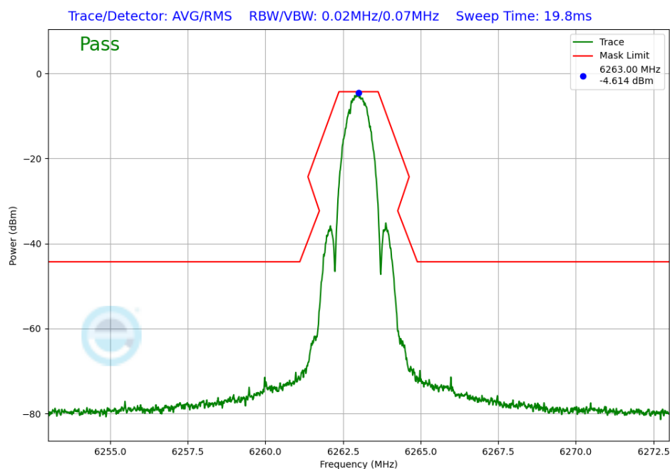
Plot 7-250. In-Band Emission Antenna WF2a (NB UNII LE1M, ePA – 6263MHz)
