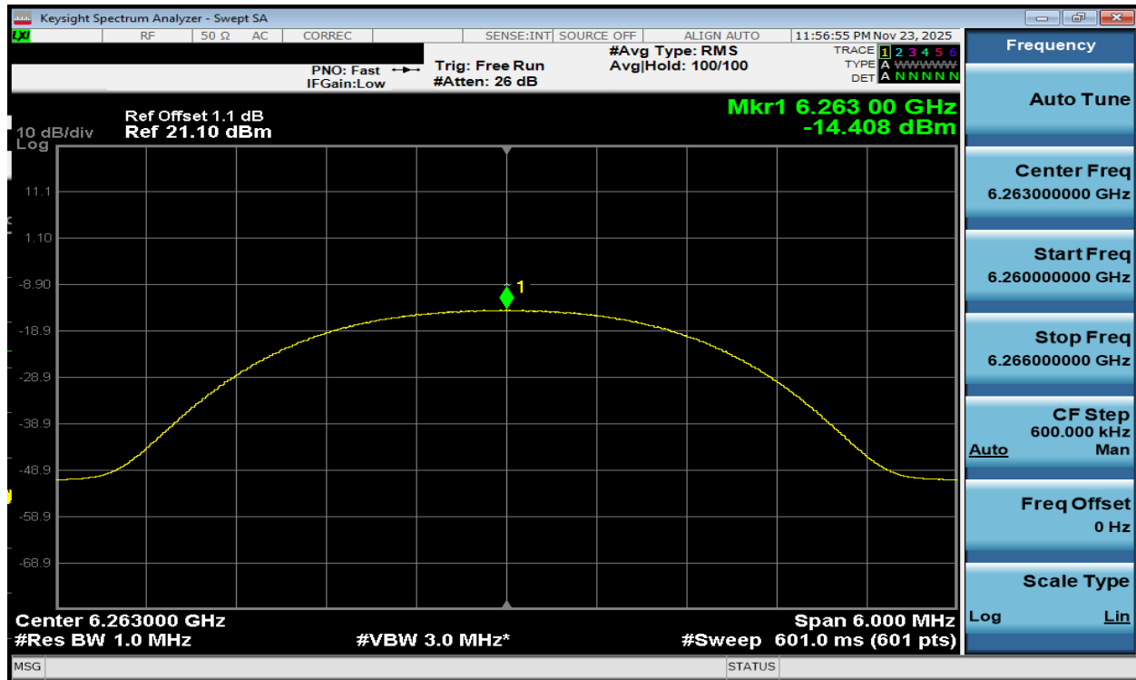
Plot 7-182. PSD TxBF Diversity Antenna WF2a (NB UNII HDR4, ePA – 6263MHz)
