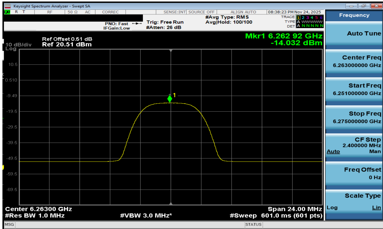
Plot 7-198. PSD TxBF Diversity Antenna WF2a (NB UNII HDRPM16, ePA – 6263MHz)
