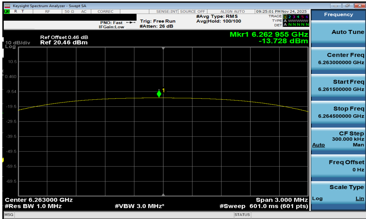
Plot 7-220. PSD TxBF Diversity Antenna WF2a (NB UNII HDT6, iPA – 6263MHz)
