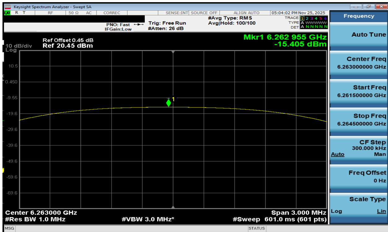
Plot 7-219. PSD TxBF Diversity Antenna WF7b (NB UNII HDT6, ePA – 6263MHz)
