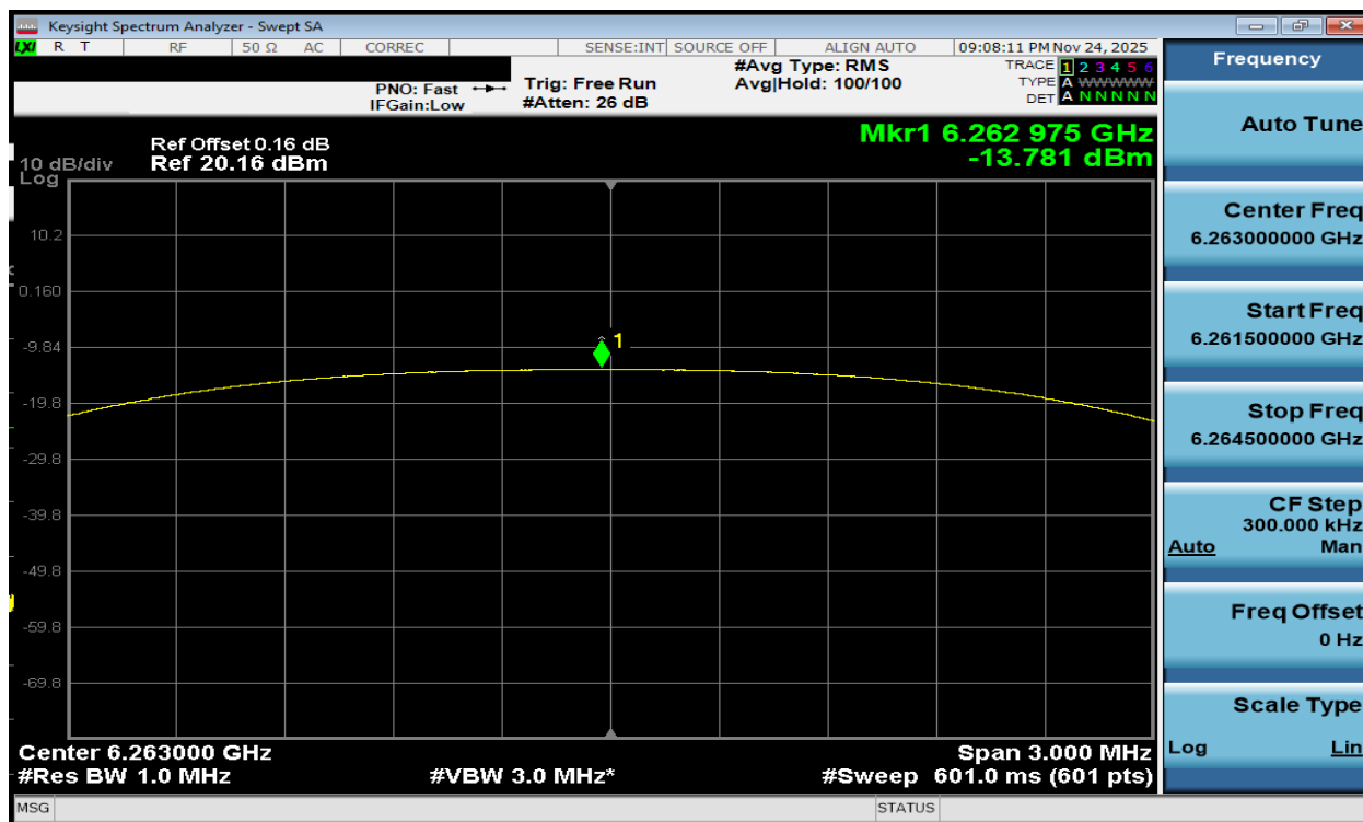
Plot 7-212. PSD TxBF Diversity Antenna WF2a (NB UNII HDT2, iPA – 6263MHz)
