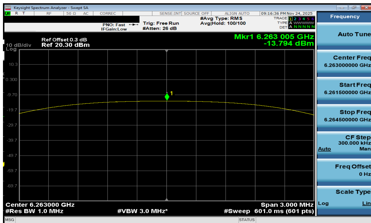
Plot 7-216. PSD TxBF Diversity Antenna WF2a (NB UNII HDT4, iPA – 6263MHz)
