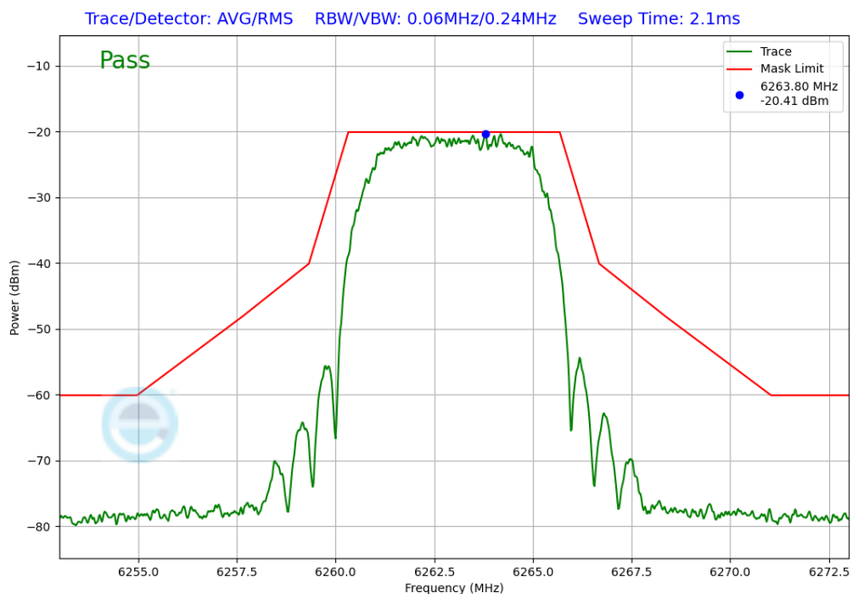
Plot 7-234. In-Band Emission Antenna WF7a (NB UNII XHDRPM6, ePA – 6263MHz)
