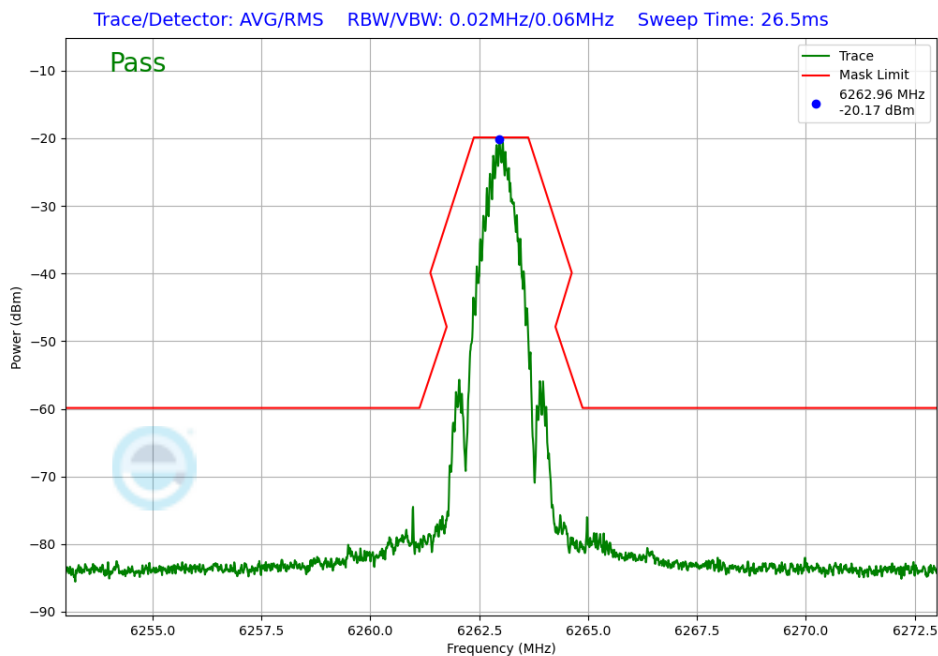
Plot 7-222. In-Band Emission Antenna WF7a (NB UNII BDR, ePA – 6263MHz)
