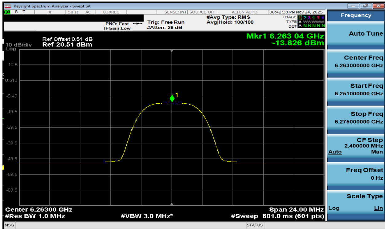
Plot 7-200. PSD TxBF Diversity Antenna WF2a (NB UNII HDRPM16, iPA – 6263MHz)
