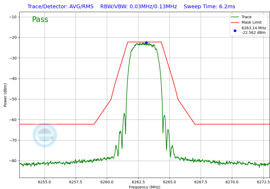
Plot 7-232. In-Band Emission Antenna WF7a (NB UNII HDRPS2, ePA – 6263MHz)
