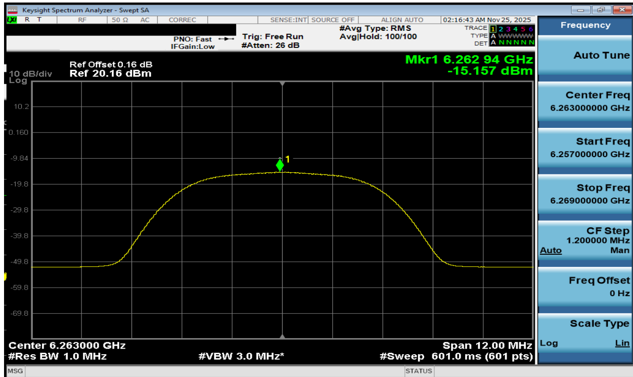
Plot 7-187. PSD TxBF Diversity Antenna WF7b (NB UNII HDR8, ePA - 6263MHz)
