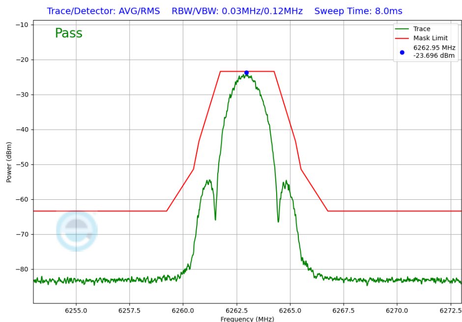
Plot 7-227. In-Band Emission Antenna WF7a (NB UNII LE2M, iPA – 6263MHz)
