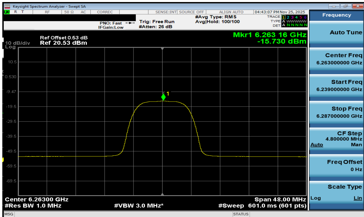
Plot 7-209. PSD TxBF Diversity Antenna WF7b (NB UNII HDRPL32, iPA – 6263MHz)
