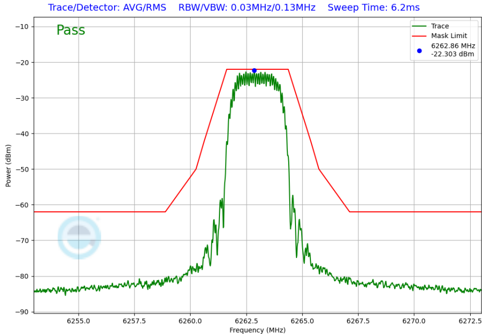
Plot 7-243. In-Band Emission Antenna WF7a (NB UNII HDT2, iPA – 6263MHz)
