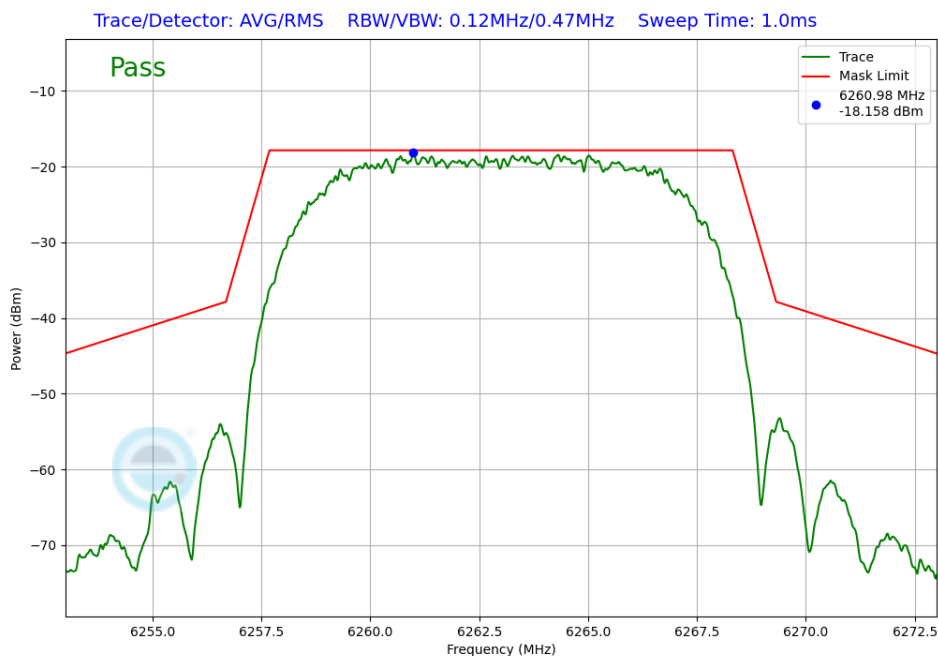
Plot 7-238. In-Band Emission Antenna WF7a (NB UNII HDRPL12, ePA – 6263MHz)
