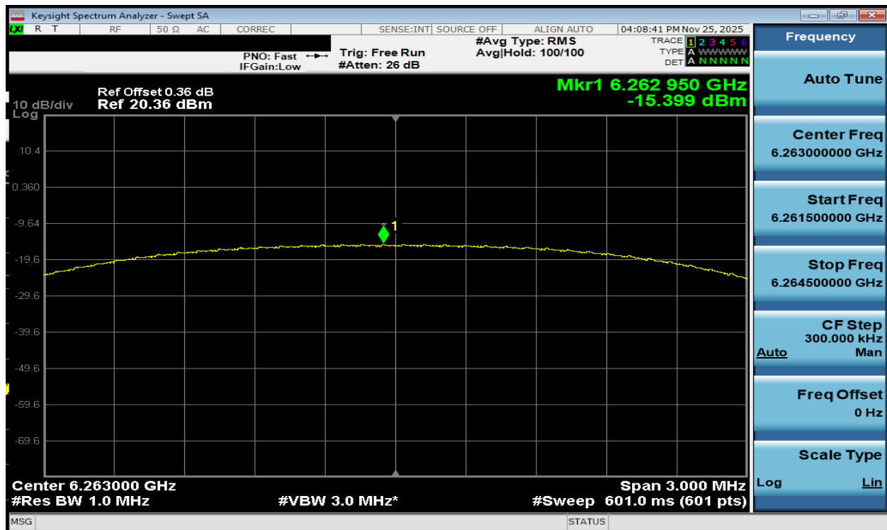
Plot 7-193. PSD TxBF Diversity Antenna WF7b (NB UNII HDRPS2, iPA – 6263MHz)
