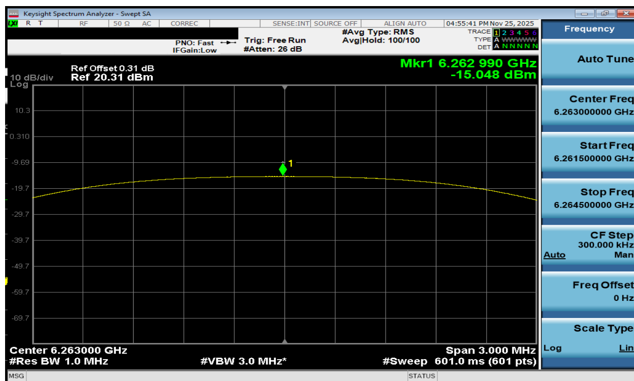
Plot 7-215. PSD TxBF Diversity Antenna WF7b (NB UNII HDT4, ePA – 6263MHz)
