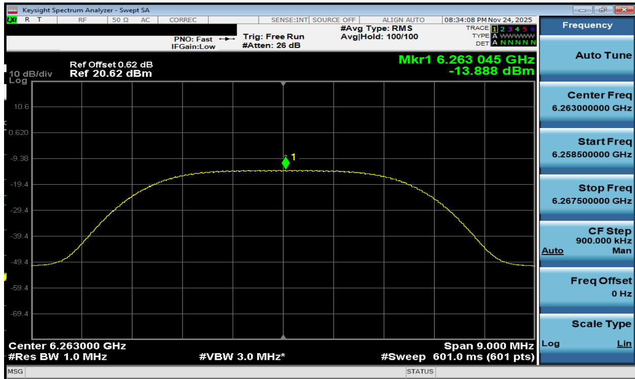
Plot 7-196. PSD TxBF Diversity Antenna WF2a (NB UNII XHDRPM6, iPA – 6263MHz)
