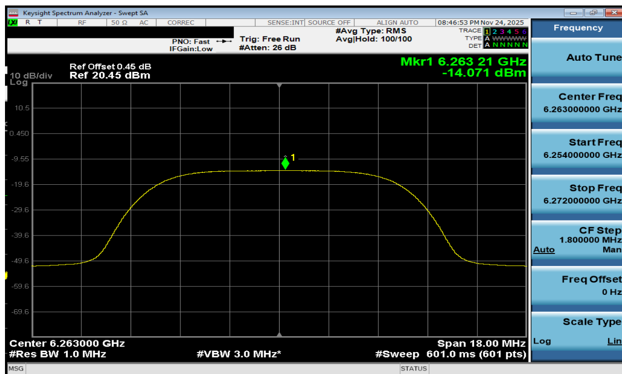
Plot 7-202. PSD Tx BF Diversity Antenna WF2a (NB UNII HDRPL12, ePA – 6263MHz)
