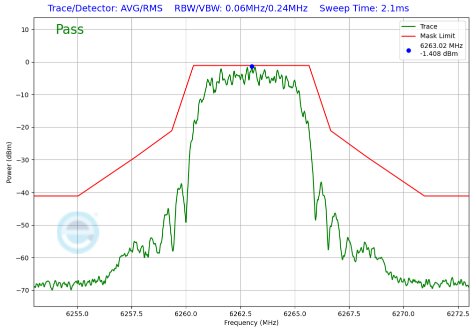
Plot 7-256. In-Band Emission Antenna WF2a (NB UNII HDR8, ePA – 6263MHz)
