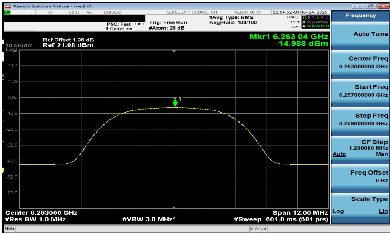
Plot 7-186. PSD TxBF Diversity Antenna WF2a (NB UNII HDR8, ePA - 6263MHz)
