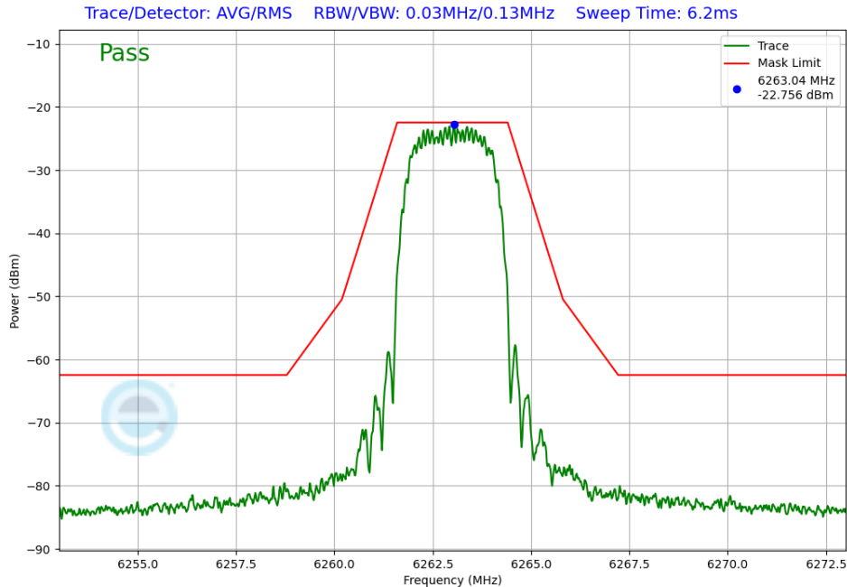
Plot 7-245. In-Band Emission Antenna WF7a (NB UNII HDT4, iPA – 6263MHz)
