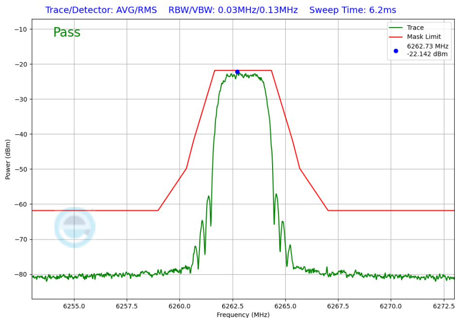
Plot 7-258. In-Band Emission Antenna WF2a (NB UNII HDRPS2, ePA – 6263MHz)
