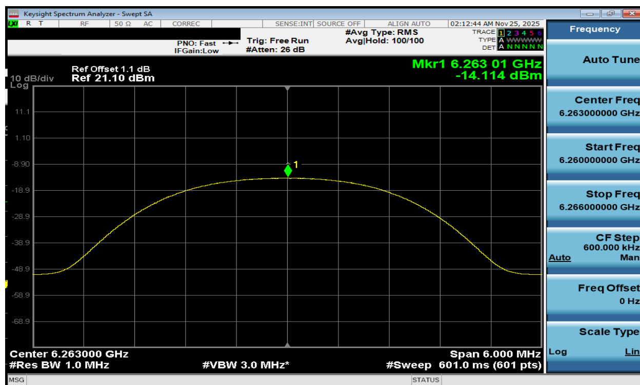
Plot 7-185. PSD TxBF Diversity Antenna WF7b (NB UNII HDR4, iPA - 6263MHz)
