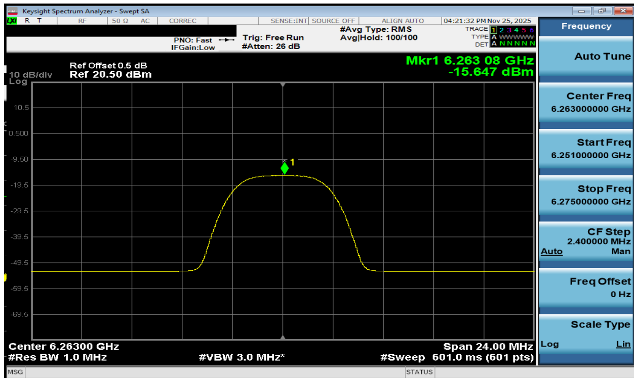
Plot 7-199. PSD TxBF Diversity Antenna WF7b (NB UNII HDRPM16, ePA – 6263MHz)
