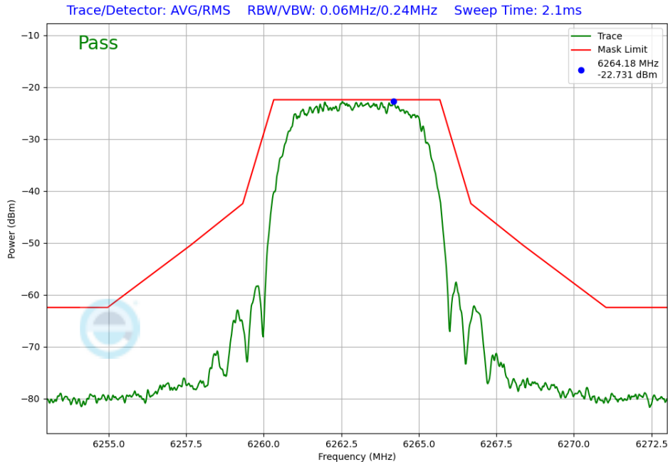
Plot 7-235. In-Band Emission Antenna WF7a (NB UNII XHDRPM6, iPA – 6263MHz)
