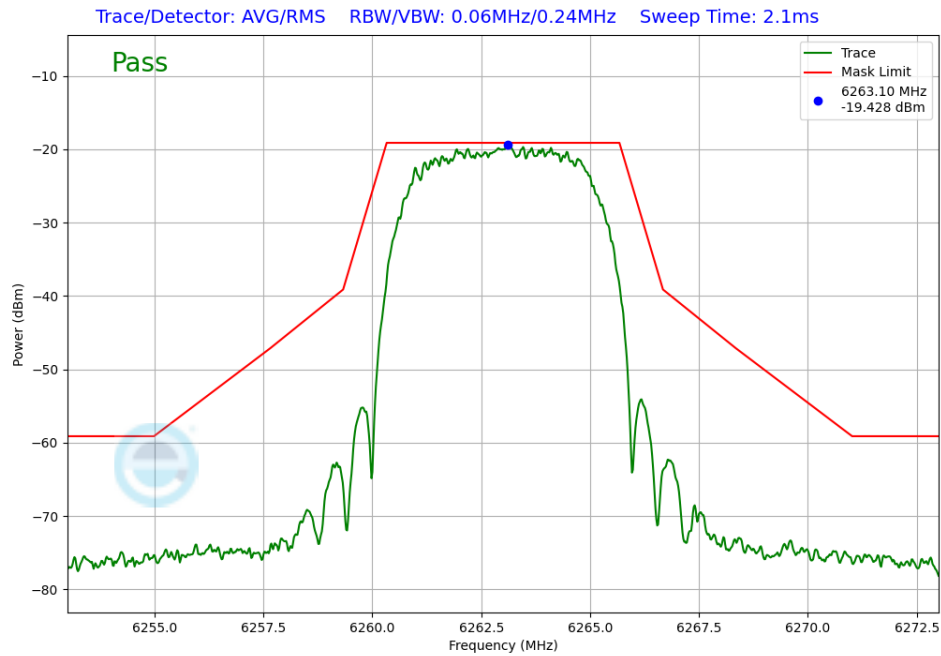
Plot 7-262. In-Band Emission Antenna WF2a (NB UNII HDRPM16, ePA – 6263MHz)
