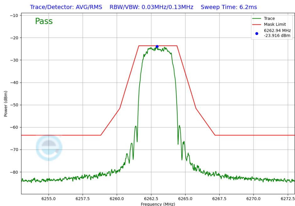
Plot 7-247. In-Band Emission Antenna WF7a (NB UNII HDT6, iPA – 6263MHz)
