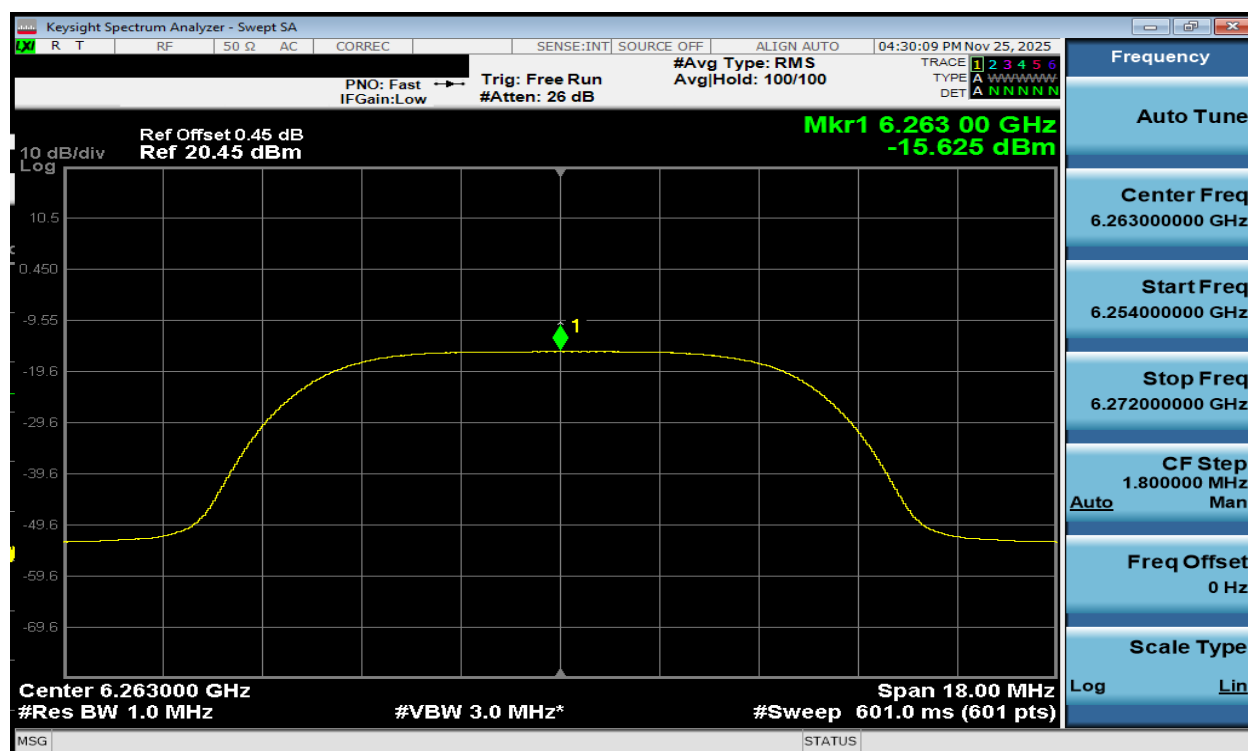
Plot 7-203. PSD Tx BF Diversity Antenna WF7b (NB UNII HDRPL12, ePA – 6263MHz)
