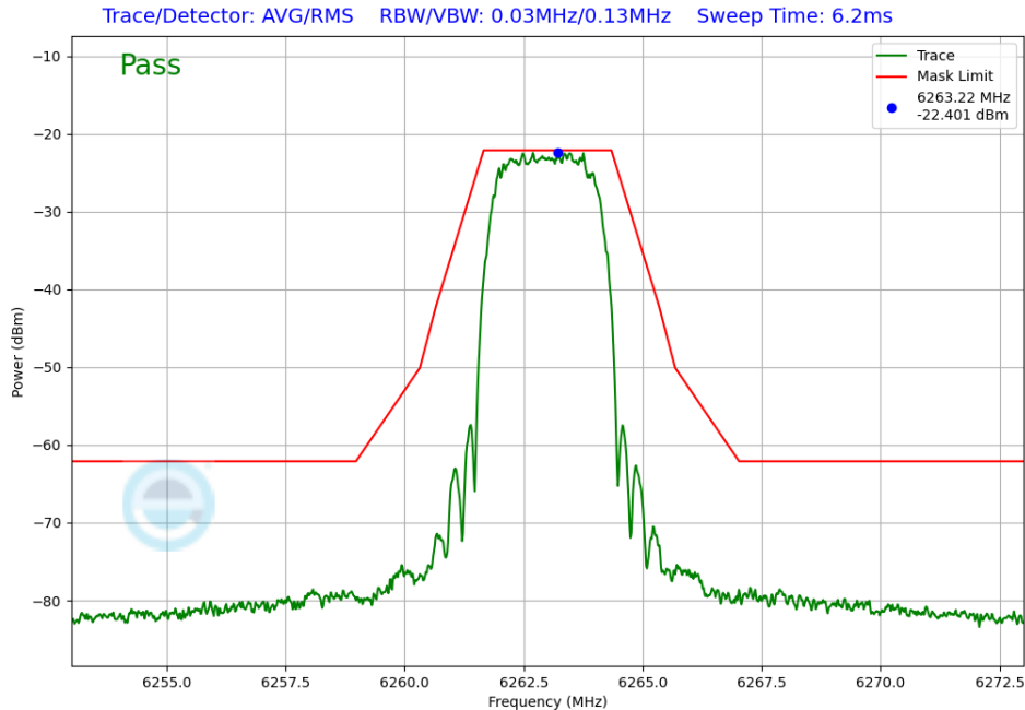
Plot 7-259. In-Band Emission Antenna WF2a (NB UNII HDRPS2, iPA – 6263MHz)
