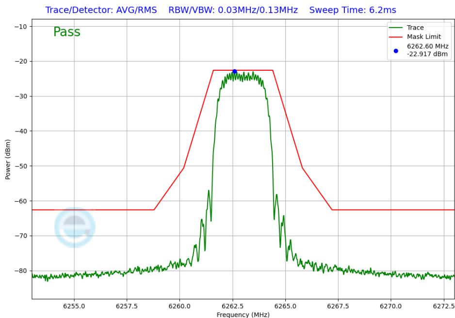
Plot 7-244. In-Band Emission Antenna WF7a (NB UNII HDT4, ePA – 6263MHz)
