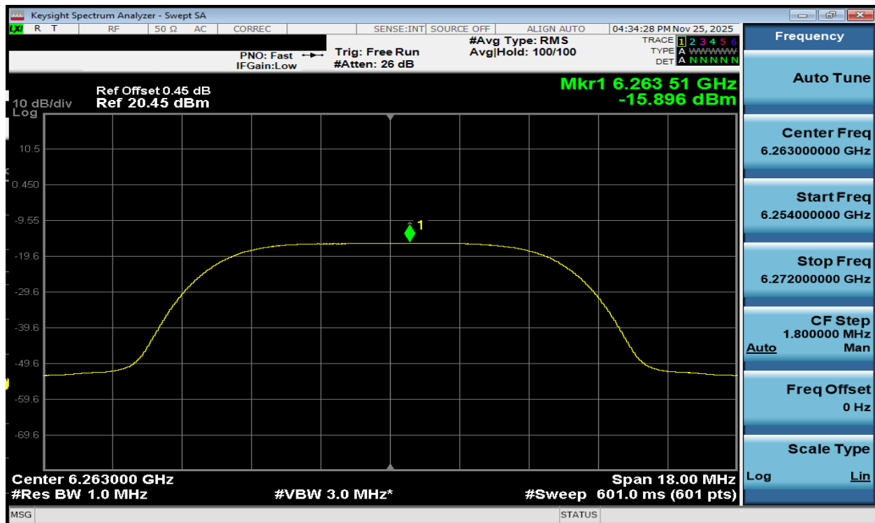
Plot 7-205. PSD TxBF Diversity Antenna WF7b (NB UNII HDRPL12, iPA – 6263MHz)
