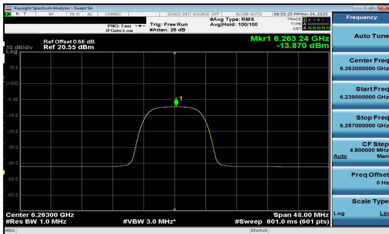
Plot 7-206. PSD TxBF Diversity Antenna WF2a (NB UNII HDRPL32, ePA – 6263MHz)
