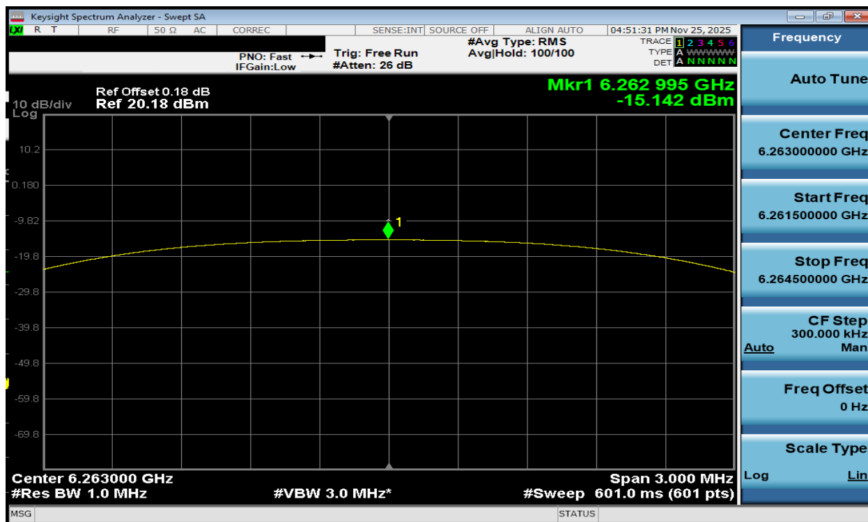
Plot 7-213. PSD TxBF Diversity Antenna WF7b (NB UNII HDT2, iPA – 6263MHz)
