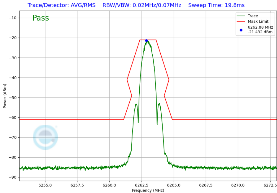
Plot 7-225. In-Band Emission Antenna WF7a (NB UNII LE1M, iPA – 6263MHz)
