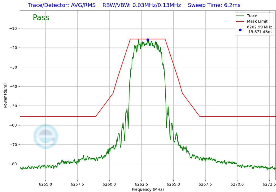
Plot 7-255. In-Band Emission Antenna WF2a (NB UNII HDR4, iPA – 6263MHz)
