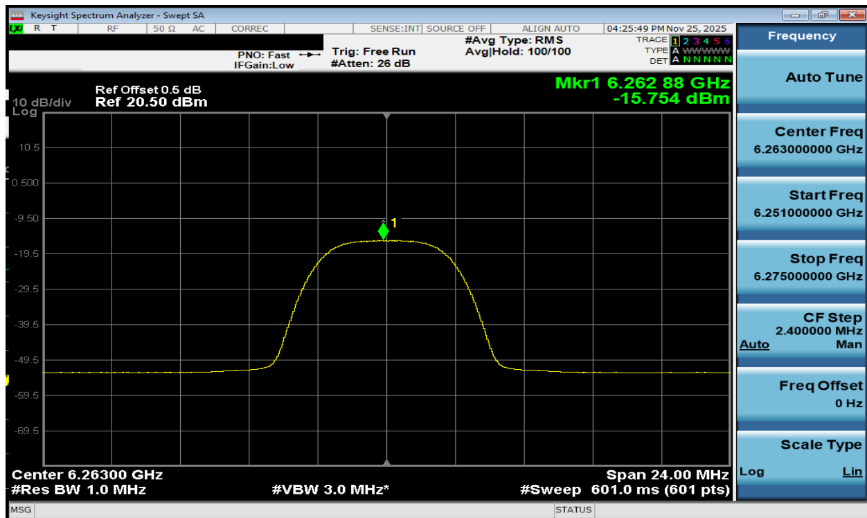
Plot 7-201. PSD TxBF Diversity Antenna WF7b (NB UNII HDRPM16, iPA – 6263MHz)
