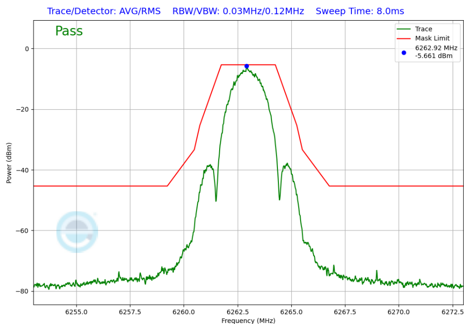
Plot 7-252. In-Band Emission Antenna WF2a (NB UNII LE2M, ePA – 6263MHz)
