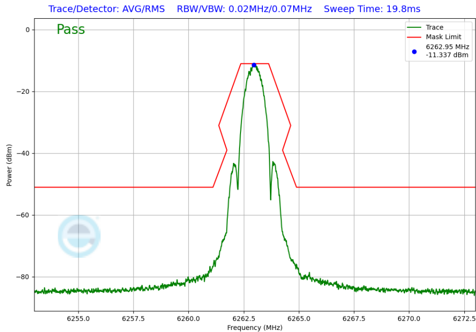
Plot 7-251. In-Band Emission Antenna WF2a (NB UNII LE1M, iPA – 6263MHz)
