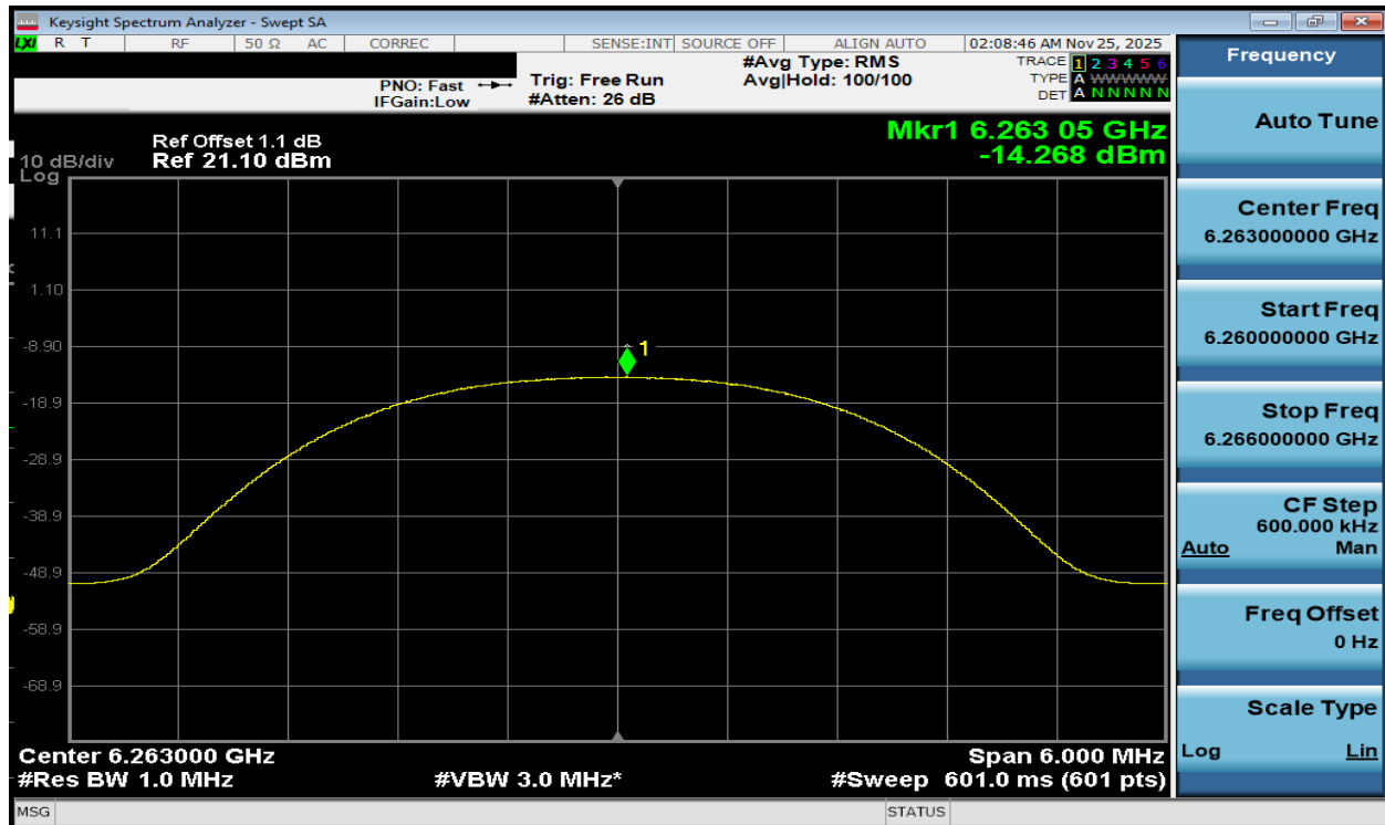
Plot 7-183. PSD TxBF Diversity Antenna WF7b (NB UNII HDR4, ePA – 6263MHz)
