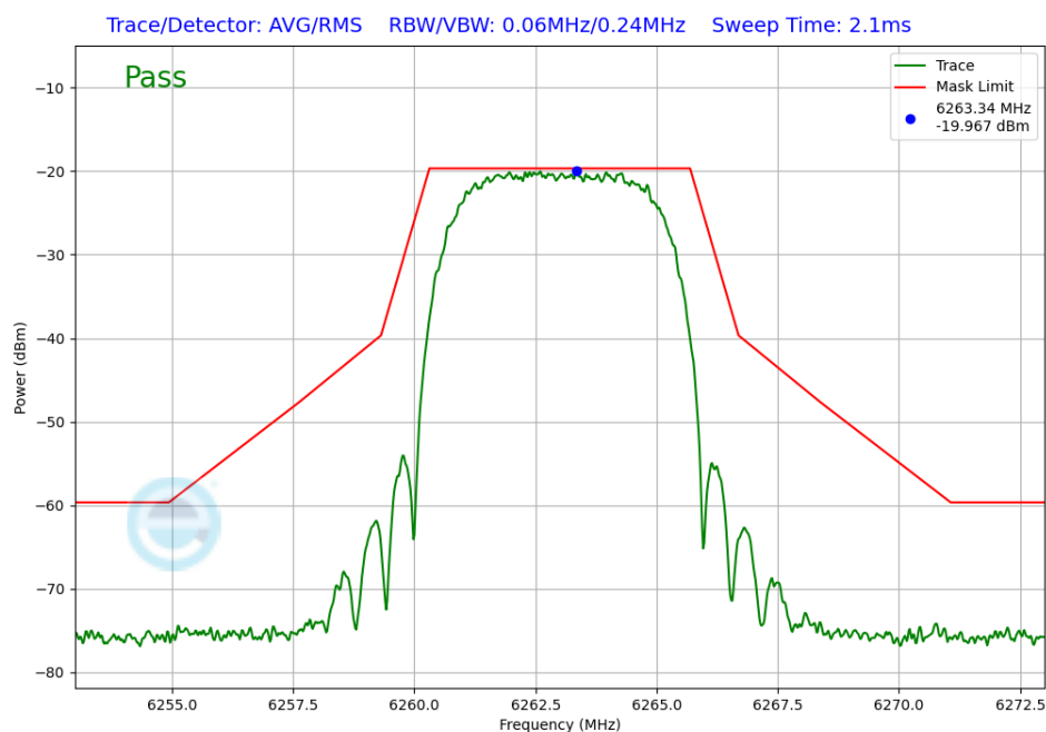
Plot 7-260. In-Band Emission Antenna WF2a (NB UNII XHDRPM6, ePA – 6263MHz)
