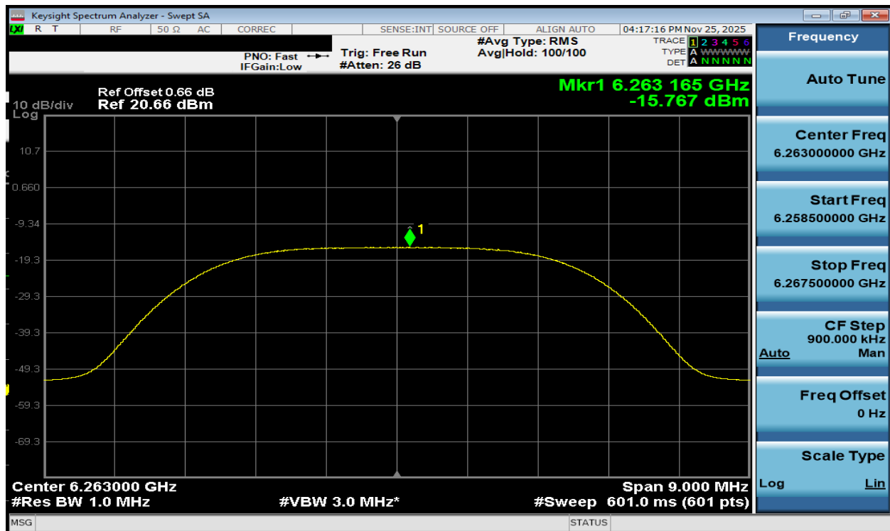
Plot 7-197. PSD TxBF Diversity Antenna WF7b (NB UNII XHDRPM6, iPA – 6263MHz)
