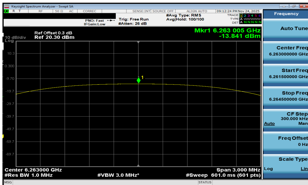
Plot 7-214. PSD TxBF Diversity Antenna WF2a (NB UNII HDT4, ePA – 6263MHz)
