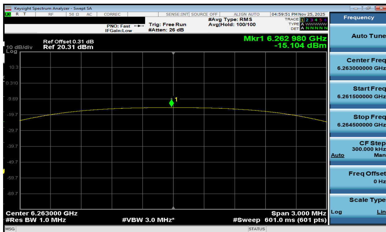
Plot 7-217. PSD TxBF Diversity Antenna WF7b (NB UNII HDT4, iPA – 6263MHz)
