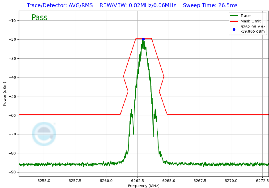
Plot 7-223. In-Band Emission Antenna WF7a (NB UNII BDR, iPA – 6263MHz)
