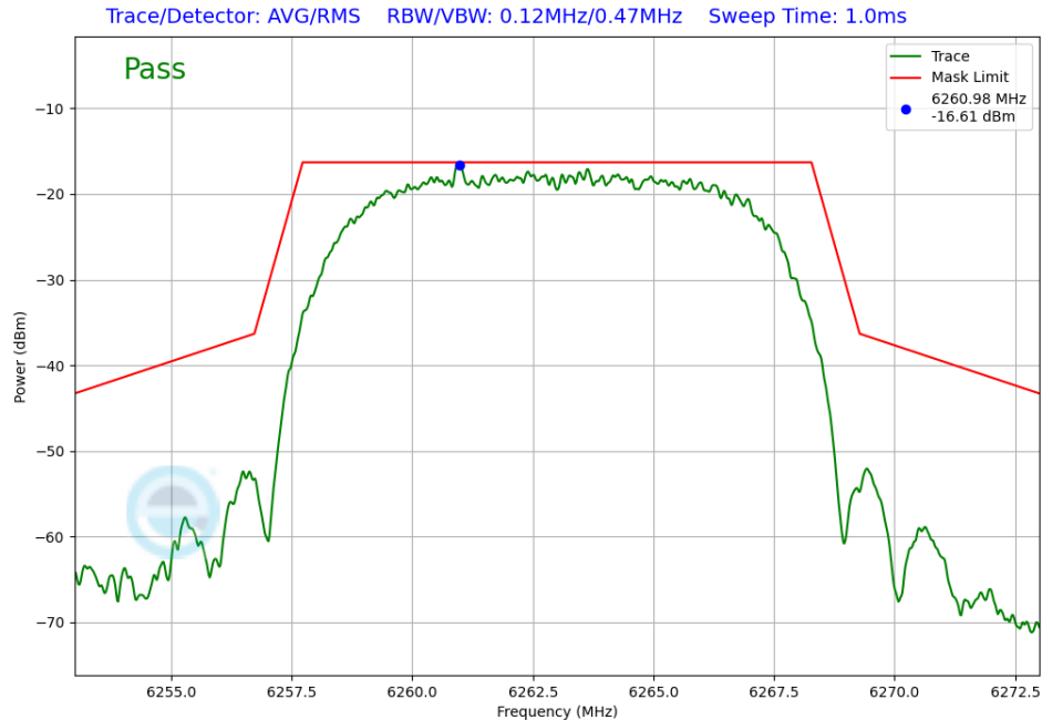
Plot 7-241. In-Band Emission Antenna WF7a (NB UNII HDRPL32, iPA – 6263MHz)
