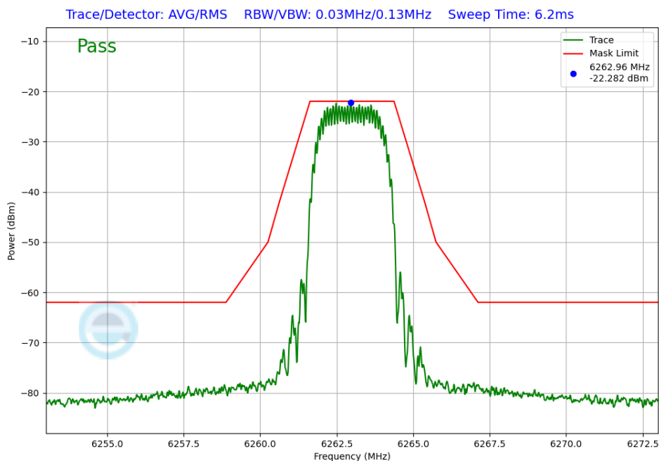
Plot 7-242. In-Band Emission Antenna WF7a (NB UNII HDT2, ePA – 6263MHz)
