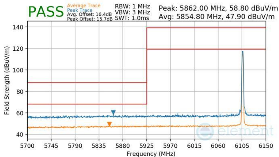
Plot 7-460 Radiated Lower Band Edge Measurement Antenna WF7b
