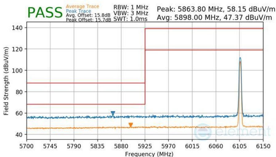
Plot 7-445 Radiated Lower Band Edge Measurement Antenna WF7a
