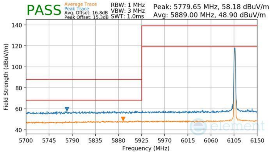
Plot 7-447 Radiated Lower Band Edge Measurement Antenna WF2a
