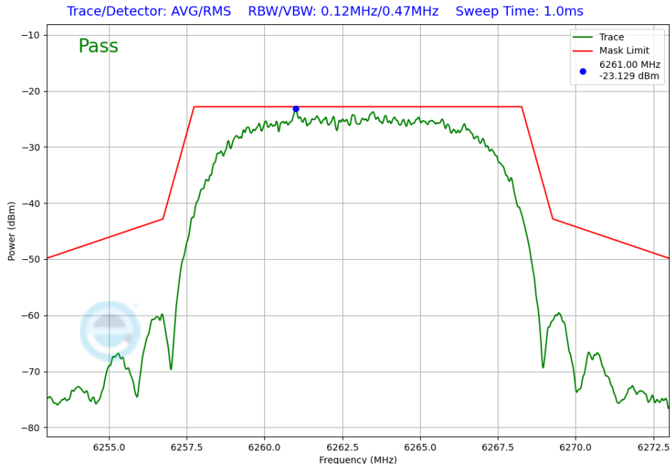
Plot 7-389. In-Band Emission TxBF Diversity Antenna WF7b (NB UNII HDRPL32, ePA – 6263MHz)
