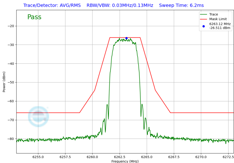
Plot 7-400. In-Band Emission Tx BF Diversity Antenna WF2a (NB UNII HDT6, ePA – 6263MHz)
