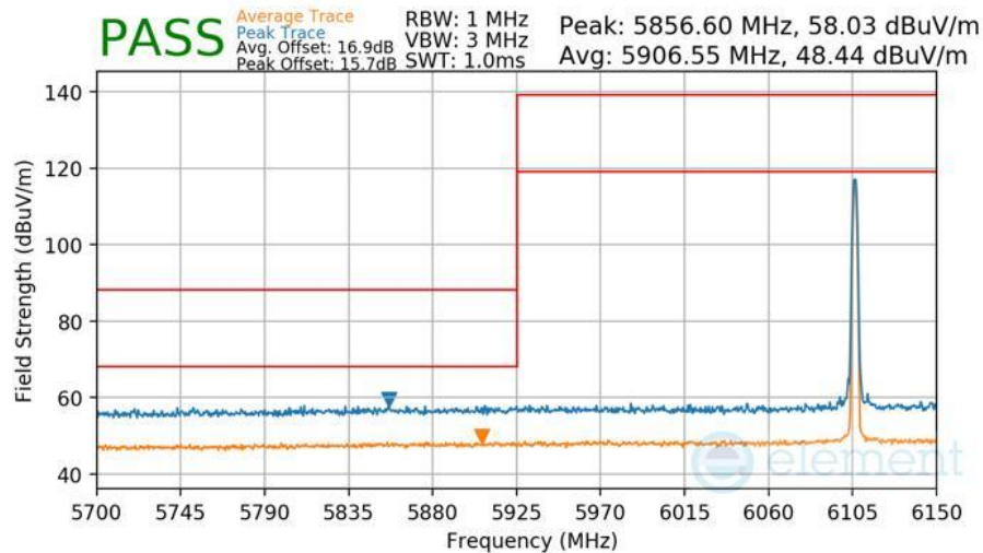
Plot 7-459 Radiated Lower Band Edge Measurement Antenna WF7b
