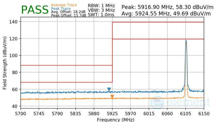
Plot 7-449 Radiated Lower Band Edge Measurement Antenna WF2a
