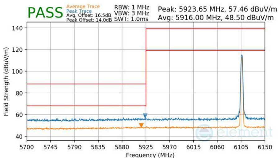
Plot 7-437 Radiated Lower Band Edge Measurement Antenna WF7a
