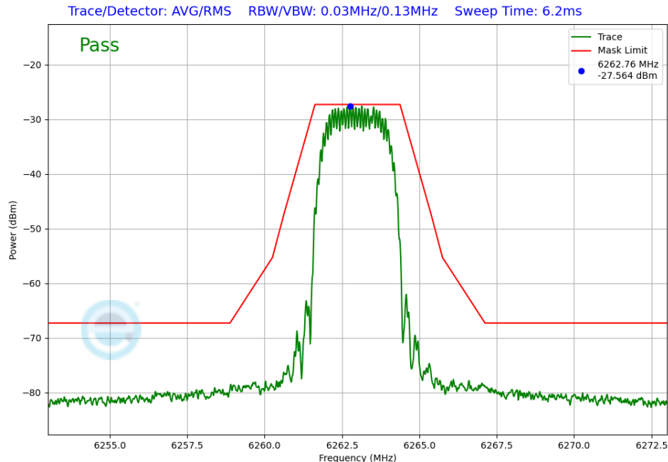
Plot 7-393. In-Band Emission Tx BF Diversity Antenna WF7b (NB UNII HDT2, ePA – 6263MHz)
