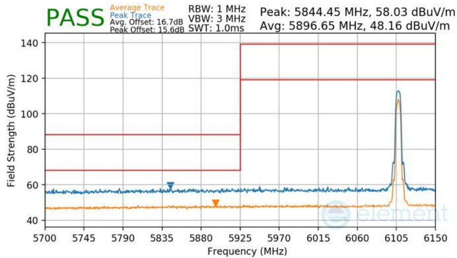
Plot 7-463 Radiated Lower Band Edge Measurement Antenna WF7b
