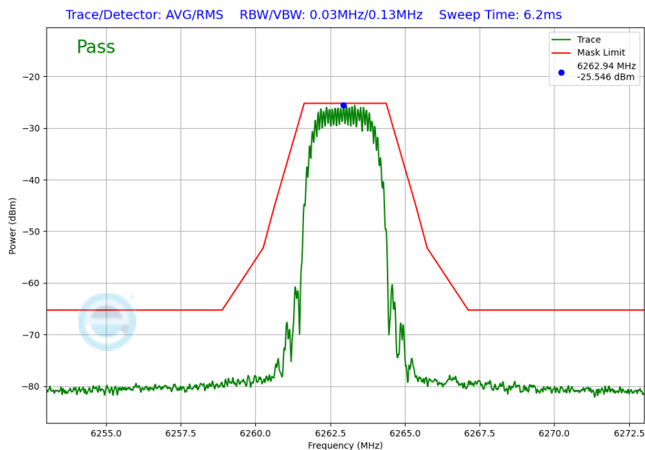
Plot 7-392. In-Band Emission Tx BF Diversity Antenna WF2a (NB UNII HDT2, ePA – 6263MHz)
