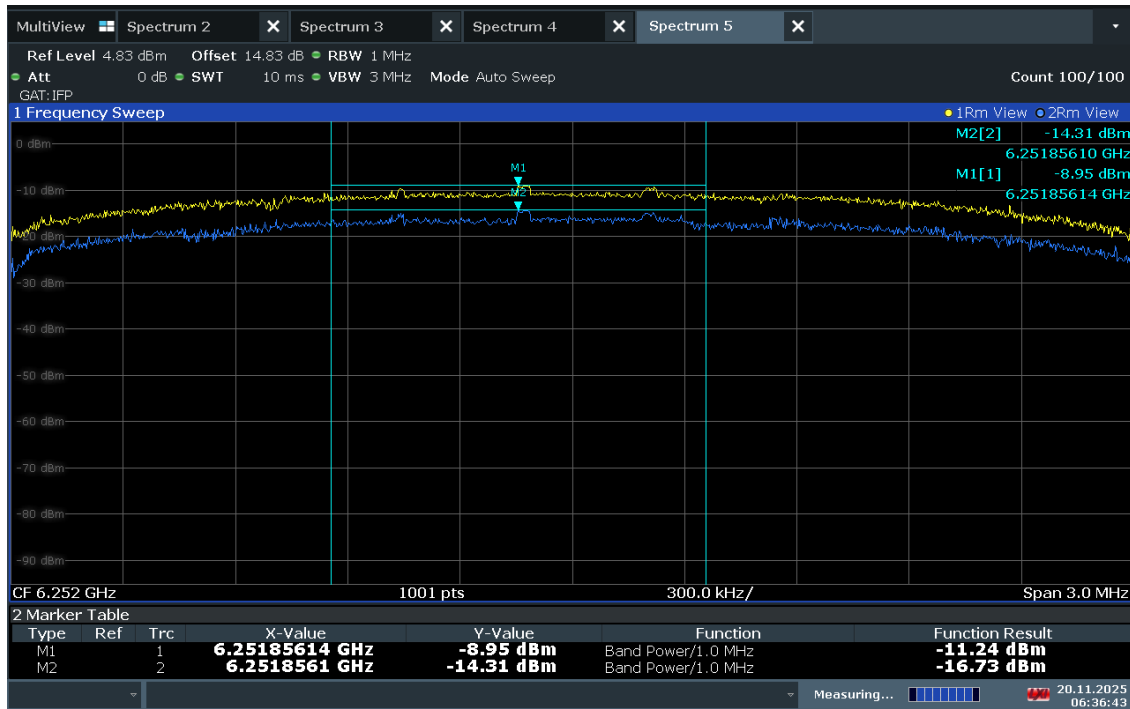
Plot 7-409. Power Density Plot – 6252MHz Antenna WF7a
