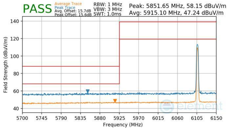
Plot 7-464 Radiated Lower Band Edge Measurement Antenna WF7b
