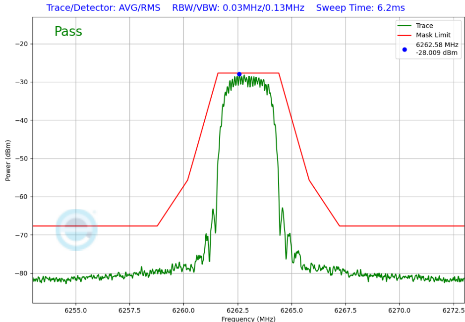
Plot 7-397. In-Band Emission Tx BF Diversity Antenna WF7b (NB UNII HDT4, ePA – 6263MHz)
