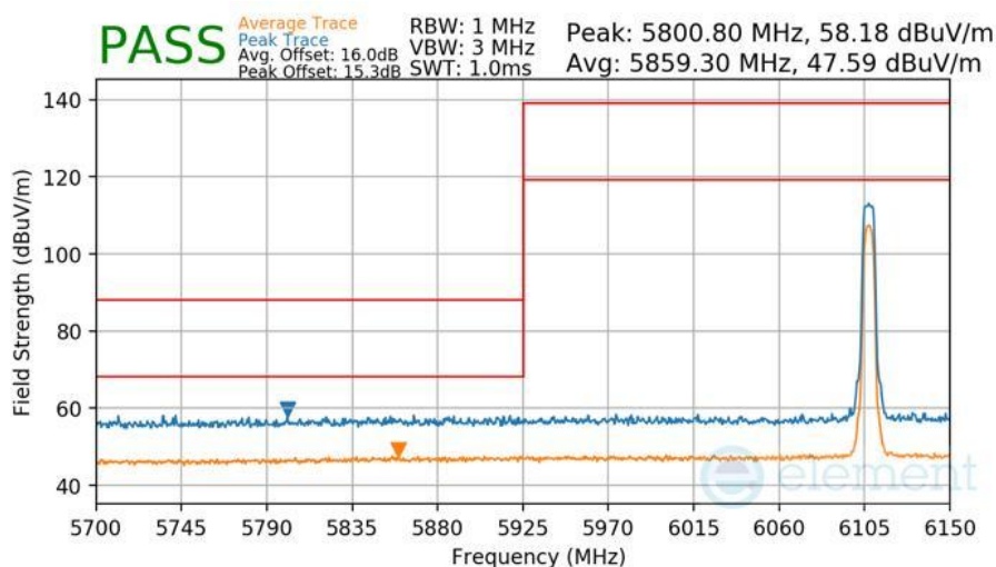
Plot 7-453 Radiated Lower Band Edge Measurement Antenna WF2a
