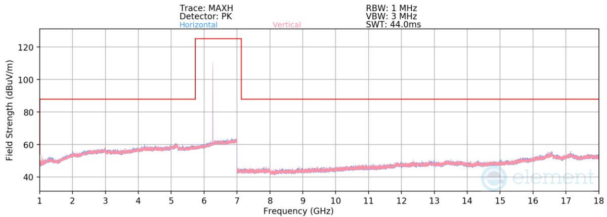
Plot 7-428. Radiated Spurious Emissions 1-18GHz TxBF Diversity (HDR4 ePA – 6263MHz)
