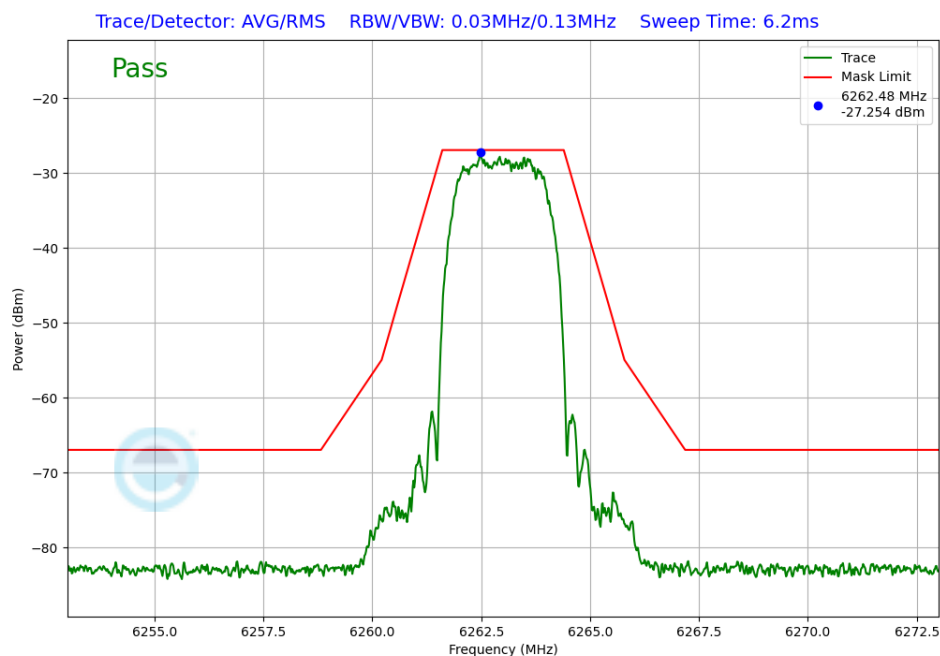
Plot 7-402. In-Band Emission TxBF Diversity Antenna WF2a (NB UNII HDT6, iPA – 6263MHz)
