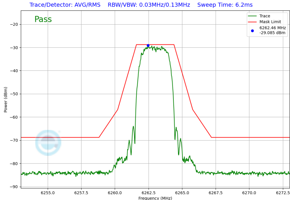
Plot 7-403. In-Band Emission TxBF Diversity Antenna WF7b (NB UNII HDT6, iPA – 6263MHz)
