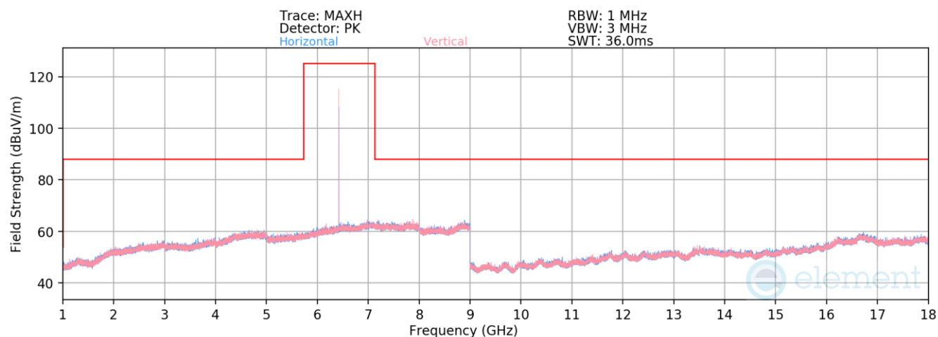
Plot 7-422. Radiated Spurious Emissions 1-18GHz TxBF Primary (LE1M GFSK ePA – 6420MHz)
