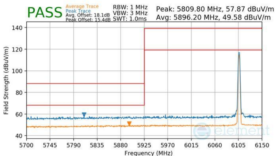
Plot 7-461 Radiated Lower Band Edge Measurement Antenna WF7b
