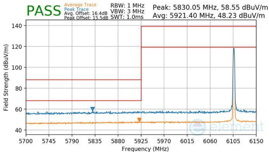
Plot 7-448 Radiated Lower Band Edge Measurement Antenna WF2a
