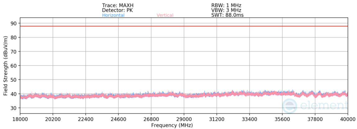
Plot 7-433. Radiated Spurious Emissions Above 18GHz TxBF Diversity (LE1M ePA – 6263MHz)
