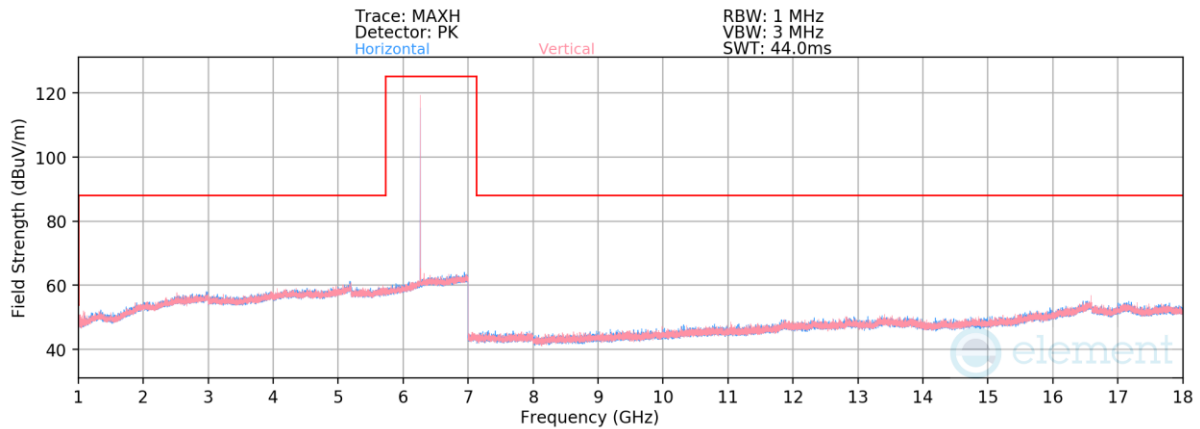
Plot 7-420. Radiated Spurious Emissions 1-18GHz TxBF Primary (LE1M GFSK ePA – 6263MHz)
