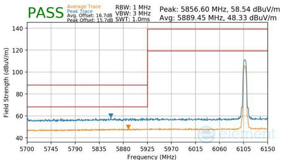
Plot 7-439 Radiated Lower Band Edge Measurement Antenna WF7a
