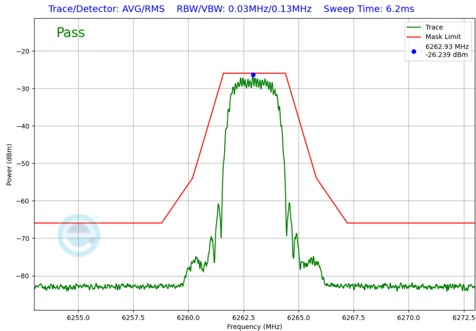
Plot 7-398. In-Band Emission TxBF Diversity Antenna WF2a (NB UNII HDT4, iPA – 6263MHz)
