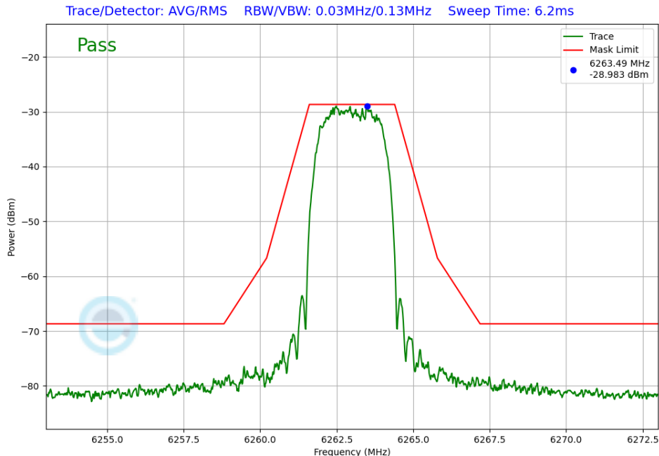
Plot 7-401. In-Band Emission Tx BF Diversity Antenna WF7b (NB UNII HDT6, ePA – 6263MHz)
