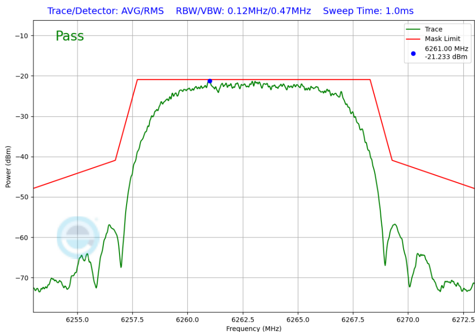
Plot 7-388. In-Band Emission TxBF Diversity Antenna WF2a (NB UNII HDRPL32, ePA – 6263MHz)
