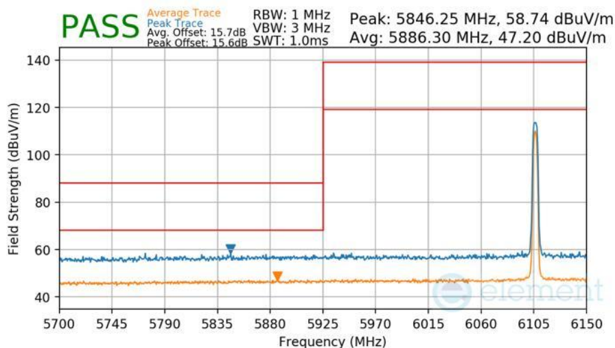
Plot 7-452 Radiated Lower Band Edge Measurement Antenna WF2a
