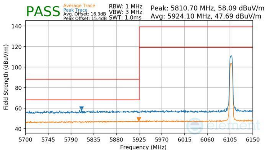
Plot 7-454 Radiated Lower Band Edge Measurement Antenna WF2a
