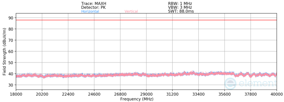
Plot 7-417. Radiated Spurious Emissions Above 18GHz (HDR4 GFSK ePA – 6263MHz)
