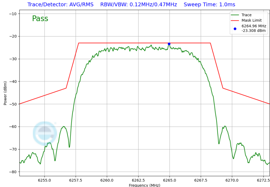
Plot 7-391. In-Band Emission TxBF Diversity Antenna WF7b (NB UNII HDRPL32, iPA – 6263MHz)
