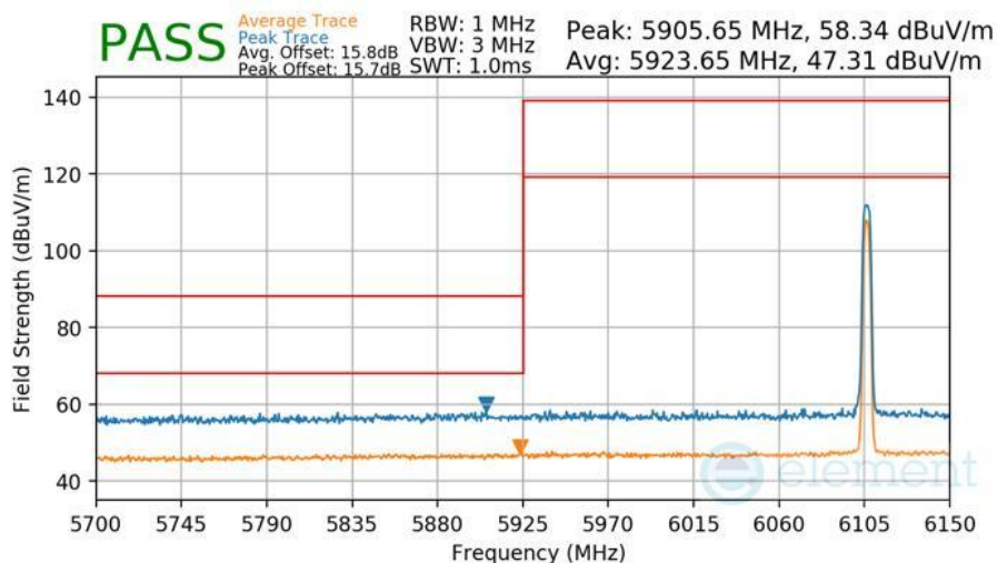
Plot 7-440 Radiated Lower Band Edge Measurement Antenna WF7a
