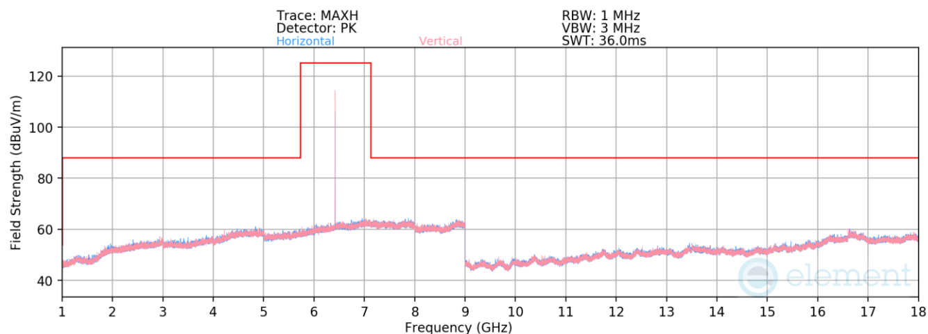
Plot 7-418. Radiated Spurious Emissions 1-18GHz TxBF Primary (HDR4 GFSK ePA – 6420MHz)
