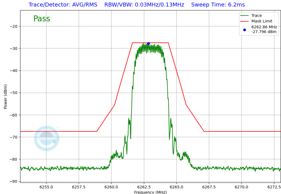
Plot 7-395. In-Band Emission TxBF Diversity Antenna WF7b (NB UNII HDT2, iPA – 6263MHz)
