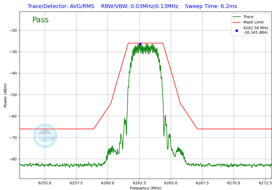
Plot 7-394. In-Band Emission TxBF Diversity Antenna WF2a (NB UNII HDT2, iPA – 6263MHz)
