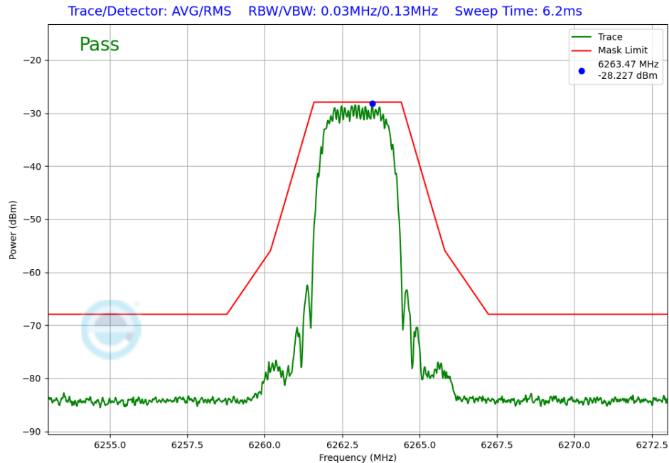
Plot 7-399. In-Band Emission TxBF Diversity Antenna WF7b (NB UNII HDT4, iPA – 6263MHz)
