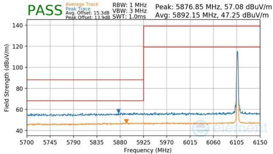
Plot 7-435 Radiated Lower Band Edge Measurement Antenna WF7a
