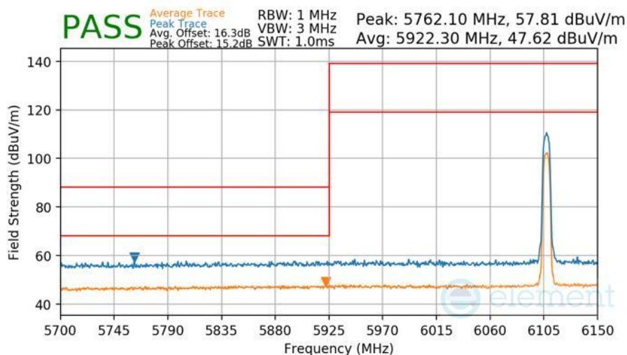
Plot 7-442 Radiated Lower Band Edge Measurement Antenna WF7a
