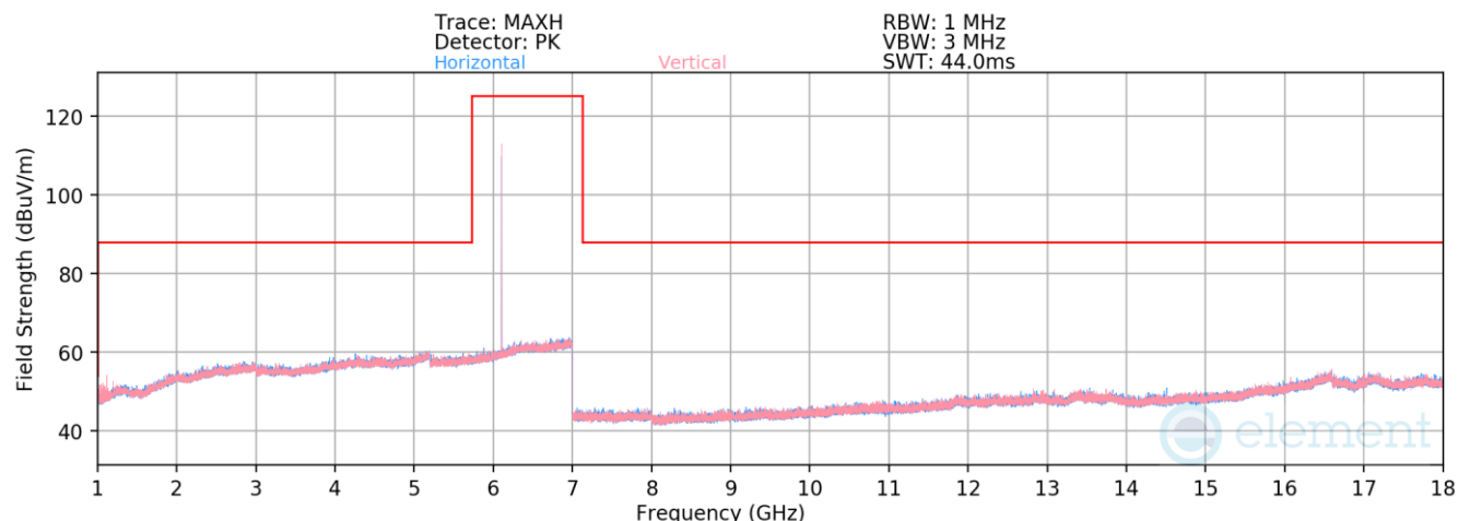
Plot 7-431. Radiated Spurious Emissions 1-18GHz TxBF Diversity (LE1M ePA – 6106MHz)
