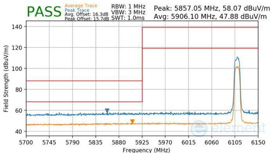
Plot 7-456 Radiated Lower Band Edge Measurement Antenna WF2a
