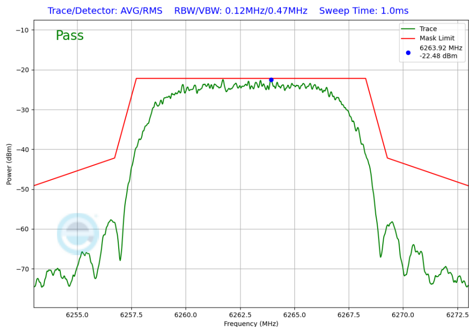
Plot 7-390. In-Band Emission TxBF Diversity Antenna WF2a (NB UNII HDRPL32, iPA – 6263MHz)
