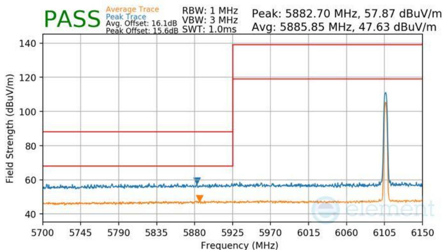
Plot 7-446 Radiated Lower Band Edge Measurement Antenna WF7a
