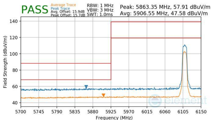
Plot 7-443 Radiated Lower Band Edge Measurement Antenna WF7a
