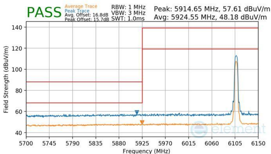
Plot 7-451 Radiated Lower Band Edge Measurement Antenna WF2a
