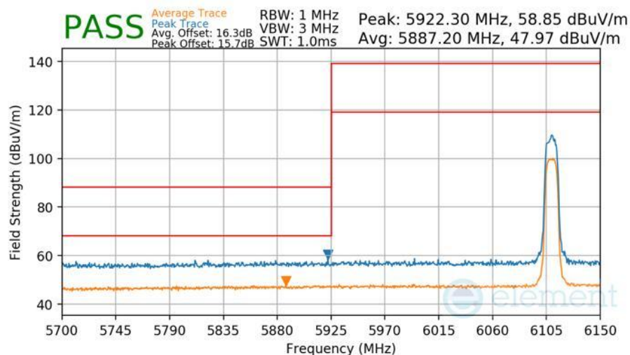
Plot 7-444 Radiated Lower Band Edge Measurement Antenna WF7a
