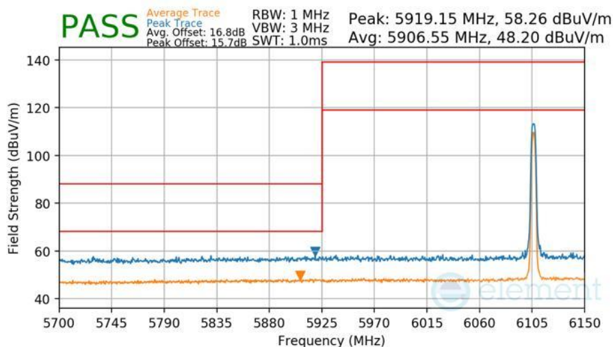
Plot 7-450 Radiated Lower Band Edge Measurement Antenna WF2a
