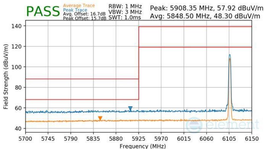
Plot 7-438 Radiated Lower Band Edge Measurement Antenna WF7a
