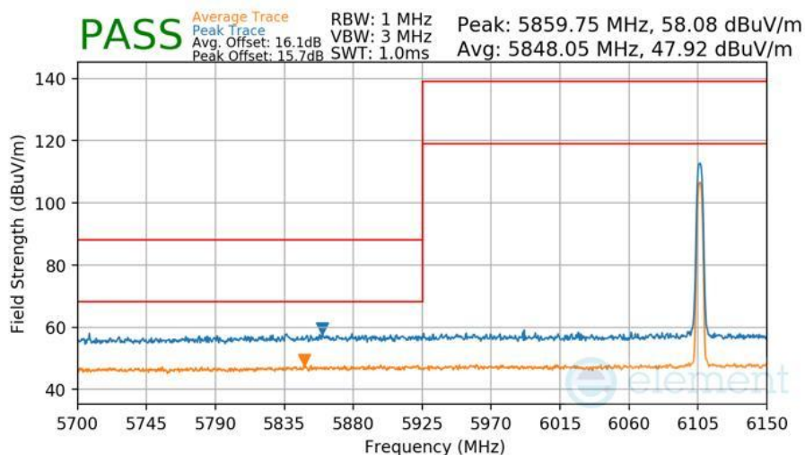
Plot 7-458 Radiated Lower Band Edge Measurement Antenna WF2a
