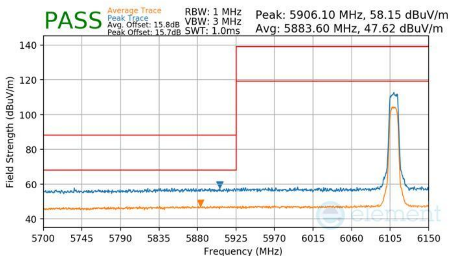
Plot 7-455 Radiated Lower Band Edge Measurement Antenna WF2a
