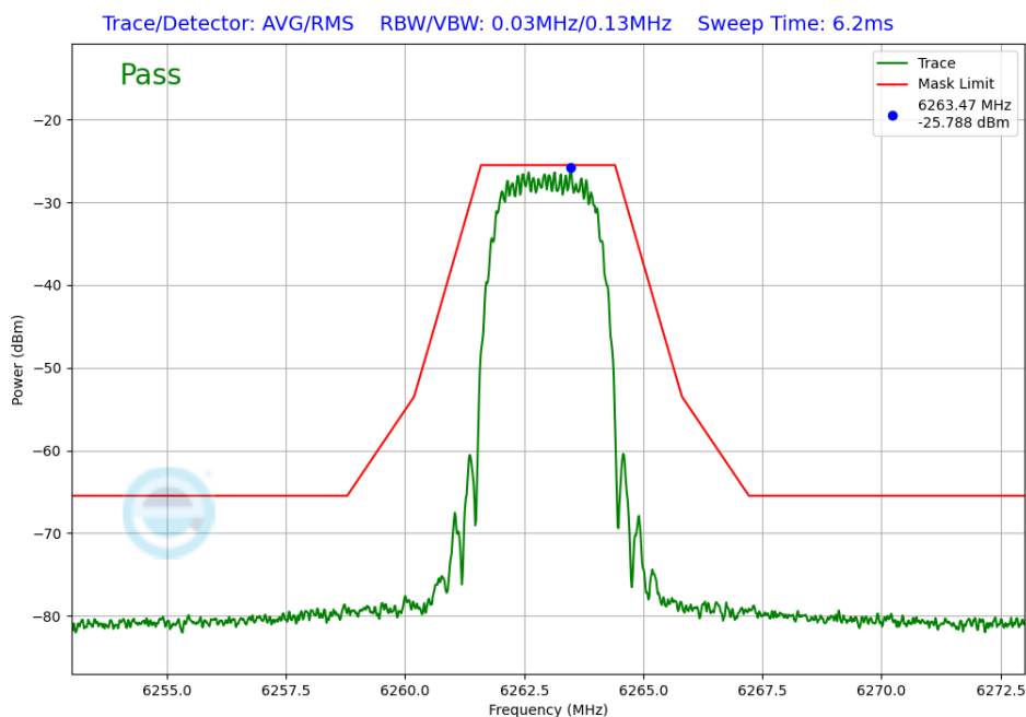
Plot 7-396. In-Band Emission Tx BF Diversity Antenna WF2a (NB UNII HDT4, ePA – 6263MHz)
