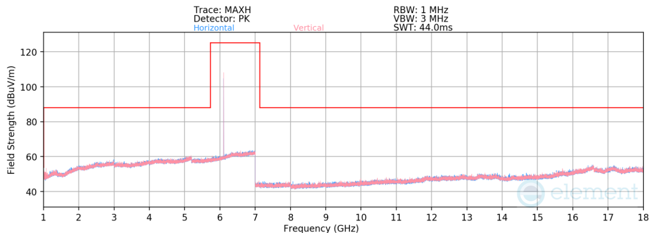
Plot 7-427. Radiated Spurious Emissions 1-18GHz TxBF Diversity (HDR4 ePA – 6106MHz)
