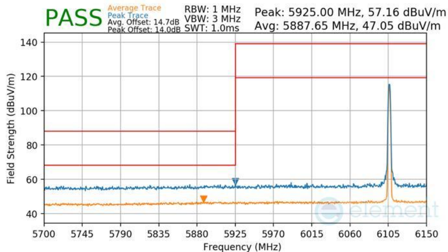
Plot 7-436 Radiated Lower Band Edge Measurement Antenna WF7a
