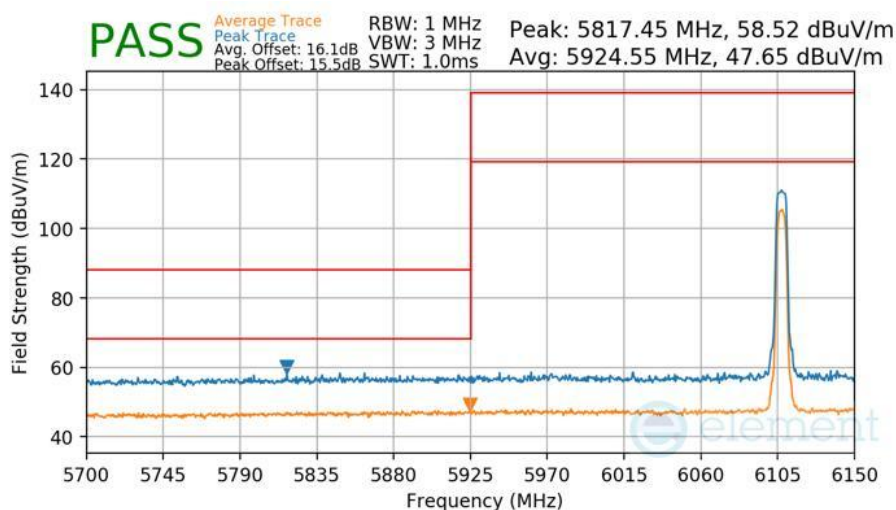
Plot 7-441 Radiated Lower Band Edge Measurement Antenna WF7a
