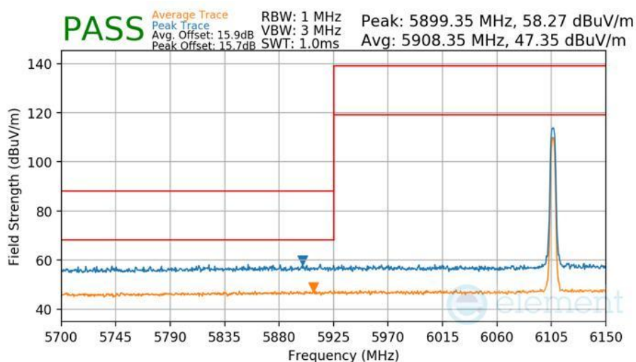
Plot 7-457 Radiated Lower Band Edge Measurement Antenna WF2a
