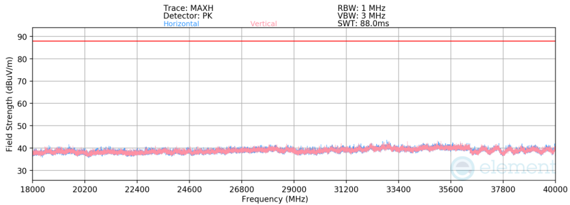
Plot 7-421. Radiated Spurious Emissions Above 18GHz (LE1M GFSK ePA – 6263MHz)
