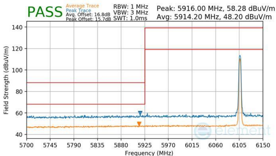
Plot 7-462 Radiated Lower Band Edge Measurement Antenna WF7b
