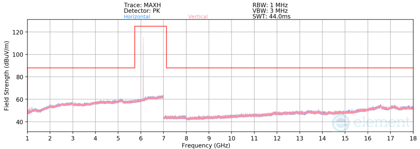
Plot 7-415. Radiated Spurious Emissions 1-18GHz TxBF Primary (HDR4 GFSK ePA – 6106MHz)
