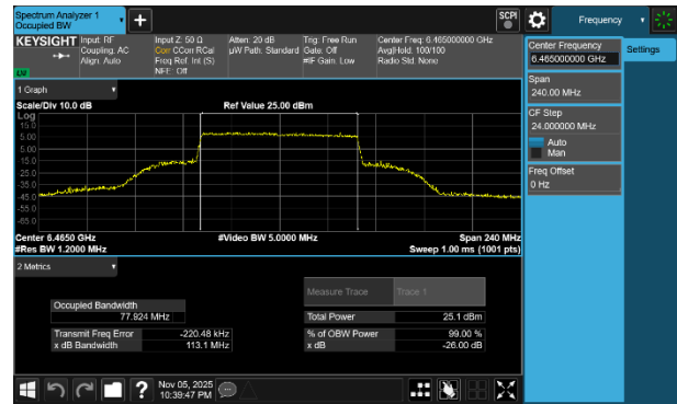
Plot 7-47 26dB BW & 99% OBW Antenna WF2a (80MHz BW 802.11be(SU) - Ch.103)
