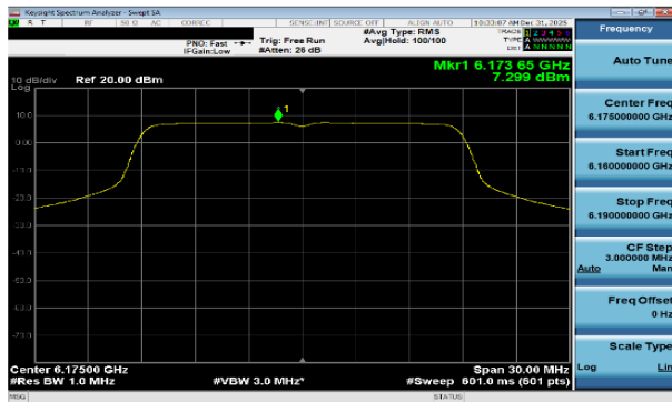
Plot 7-85 PSD Antenna WF7a (20MHz BW 802.11a - Ch.45)
