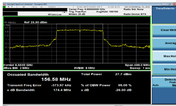
Plot 7-68 26dB BW & 99% OBW Antenna WF7b (160MHz BW 802.11be(SU) - Ch.143)
