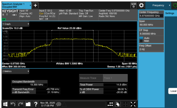
Plot 7-77 26dB BW & 99% OBW Antenna WF7b (20MHz BW 802.11be(SU) - Ch.185)
