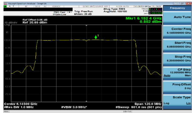
Plot 7-87 PSD Antenna WF7a (80MHz BW 802.11be(SU) - Ch.39)
