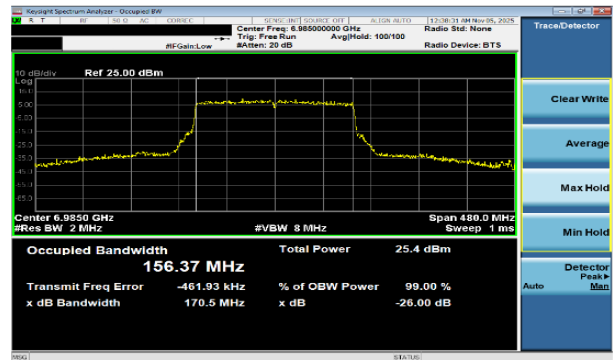
Plot 7-28 26dB BW & 99% OBW Antenna WF7a (160MHz BW 802.11be(SU) - Ch.207)
