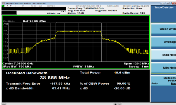
Plot 7-26 26dB BW & 99% OBW Antenna WF7a (40MHz BW 802.11be(SU) - Ch.227)
