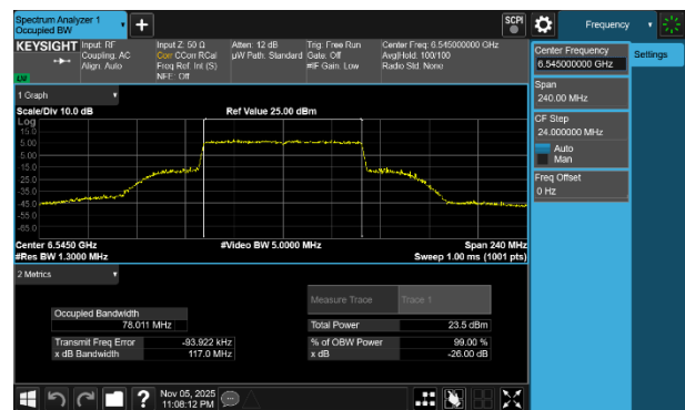
Plot 7-51 26dB BW & 99% OBW Antenna WF2a (80MHz BW 802.11be(SU) - Ch.119)
