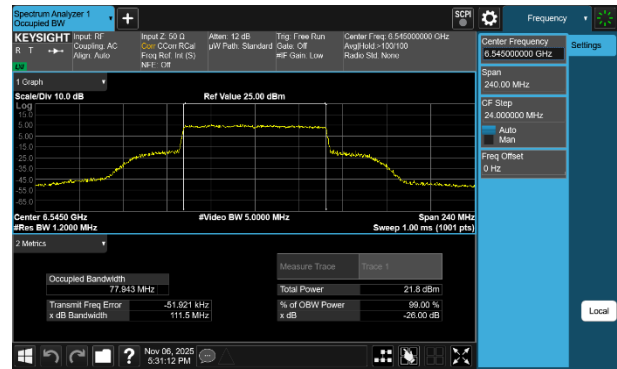
Plot 7-79 26dB BW & 99% OBW Antenna WF7b (80MHz BW 802.11be(SU) - Ch.119)
