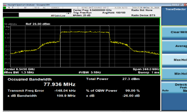
Plot 7-11 26dB BW & 99% OBW Antenna WF7a (80MHz BW 802.11be(SU) - Ch.119)
