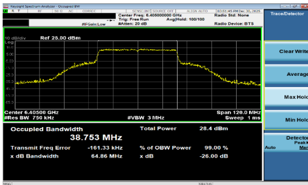
Plot 7-58 26dB BW & 99% OBW Antenna WF7b (40MHz BW 802.11be(SU) - Ch.91)
