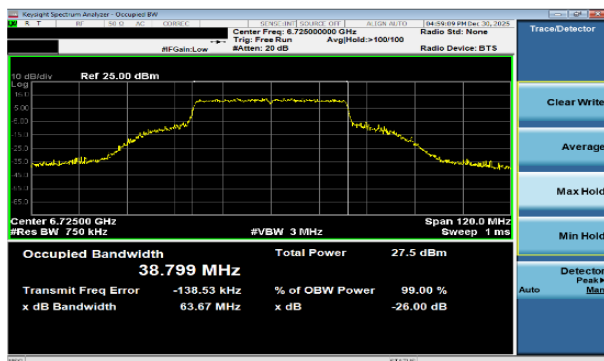
Plot 7-66 26dB BW & 99% OBW Antenna WF7b (40MHz BW 802.11be(SU) - Ch.155)
