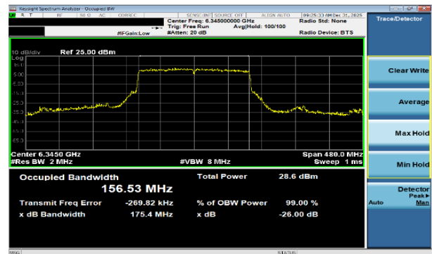
Plot 7-4 26dB BW & 99% OBW Antenna WF7a (160MHz BW 802.11be(SU) - Ch.79)
