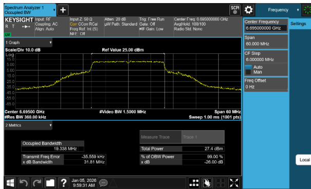
Plot 7-37 26dB BW & 99% OBW Antenna WF2a (20MHz BW 802.11be(SU) - Ch.149)
