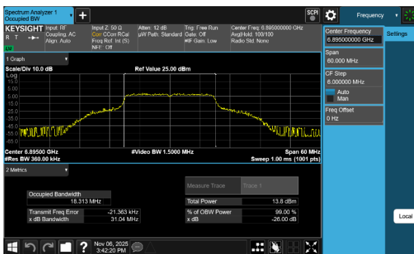
Plot 7-81 26dB BW & 99% OBW Antenna WF7b (20MHz BW 802.11a - Ch.189)
