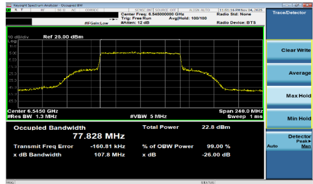
Plot 7-23 26dB BW & 99% OBW Antenna WF7a (80MHz BW 802.11be(SU) - Ch.119)
