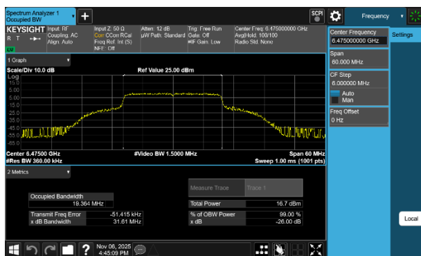
Plot 7-73 26dB BW & 99% OBW Antenna WF7b (20MHz BW 802.11be(SU) - Ch.105)
