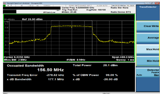
Plot 7-60 26dB BW & 99% OBW Antenna WF7b (160MHz BW 802.11be(SU) - Ch.15)
