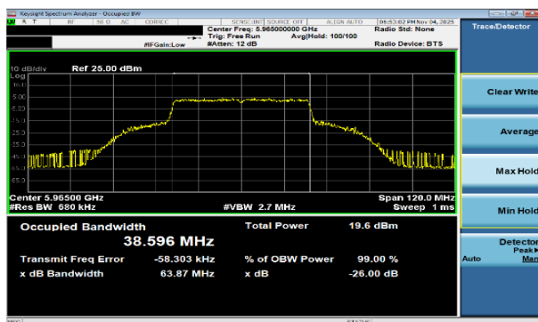
Plot 7-14 26dB BW & 99% OBW Antenna WF7a (40MHz BW 802.11be(SU) - Ch.3)
