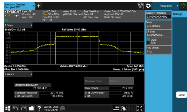
Plot 7-39 26dB BW & 99% OBW Antenna WF2a (80MHz BW 802.11be(SU) - Ch.151)
