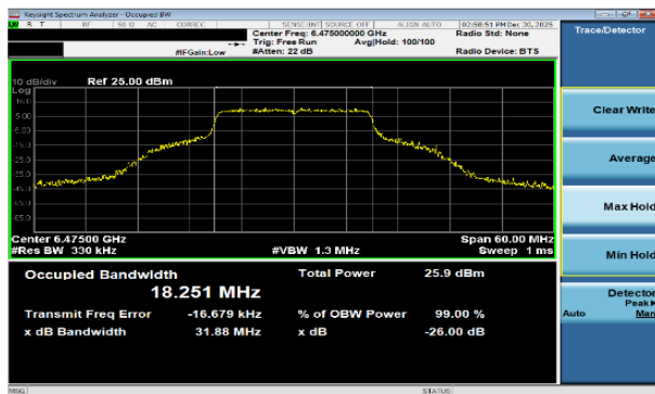
Plot 7-61 26dB BW & 99% OBW Antenna WF7b (20MHz BW 802.11a - Ch.105)
