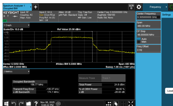
Plot 7-76 26dB BW & 99% OBW Antenna WF7b (160MHz BW 802.11be(SU) - Ch.111)
