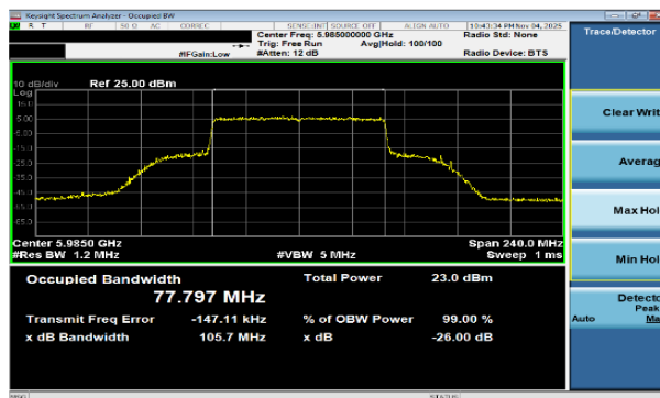
Plot 7-15 26dB BW & 99% OBW Antenna WF7a (80MHz BW 802.11be(SU) - Ch.7)
