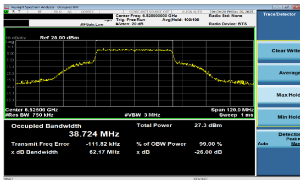
Plot 7-62 26dB BW & 99% OBW Antenna WF7b (40MHz BW 802.11be(SU) - Ch.115)
