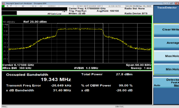
Plot 7-57 26dB BW & 99% OBW Antenna WF7b (20MHz BW 802.11be(SU) - Ch.45)
