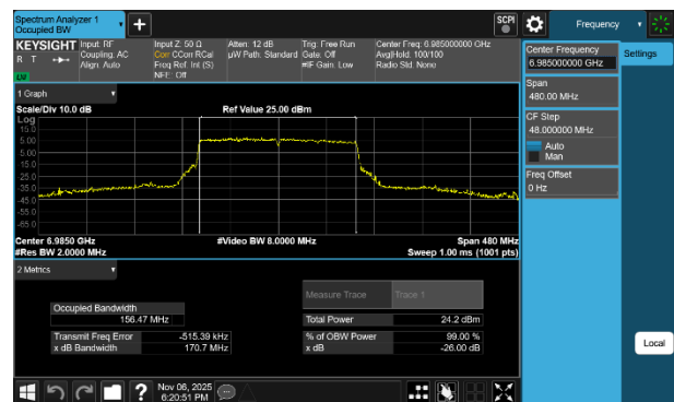
Plot 7-84 26dB BW & 99% OBW Antenna WF7b (160MHz BW 802.11be(SU) - Ch.207)
