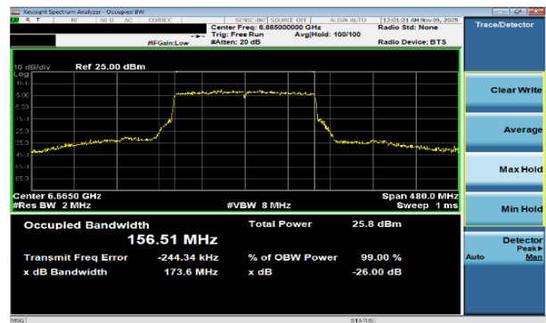
Plot 7-24 26dB BW & 99% OBW Antenna WF7a (160MHz BW 802.11be(SU) - Ch.143)
