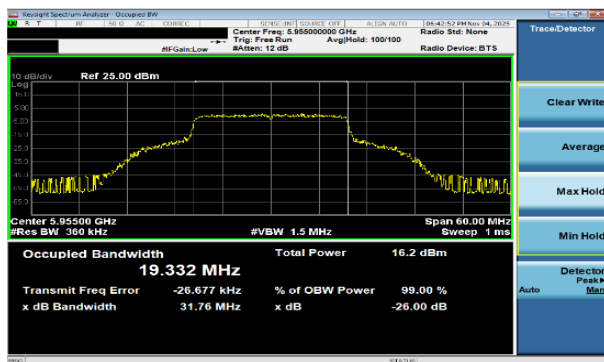
Plot 7-13 26dB BW & 99% OBW Antenna WF7a (20MHz BW 802.11be(SU) - Ch.1)
