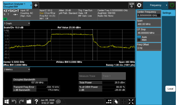
Plot 7-36 26dB BW & 99% OBW Antenna WF2a (160MHz BW 802.11be(SU) - Ch.111)
