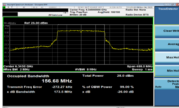
Plot 7-16 26dB BW & 99% OBW Antenna WF7a (160MHz BW 802.11be(SU) - Ch.79)
