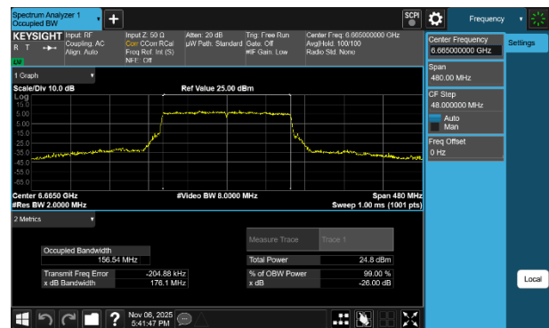
Plot 7-80 26dB BW & 99% OBW Antenna WF7b (160MHz BW 802.11be(SU) - Ch.143)
