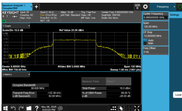
Plot 7-82 26dB BW & 99% OBW Antenna WF7b (40MHz BW 802.11be(SU) - Ch.187)
