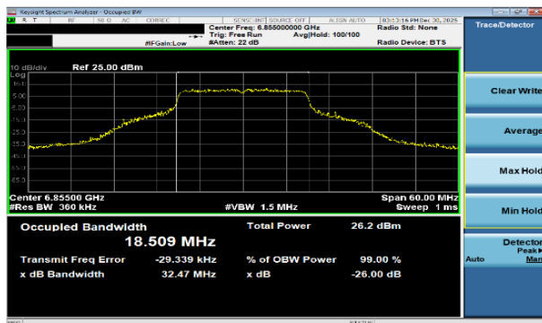
Plot 7-65 26dB BW & 99% OBW Antenna WF7b (20MHz BW 802.11a - Ch.181)
