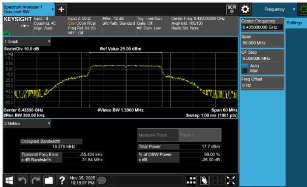
Plot 7-45 26dB BW & 99% OBW Antenna WF2a (20MHz BW 802.11be(SU) - Ch.97)
