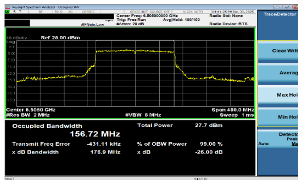
Plot 7-64 26dB BW & 99% OBW Antenna WF7b (160MHz BW 802.11be(SU) - Ch.111)
