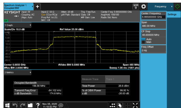
Plot 7-52 26dB BW & 99% OBW Antenna WF2a (160MHz BW 802.11be(SU) - Ch.143)
