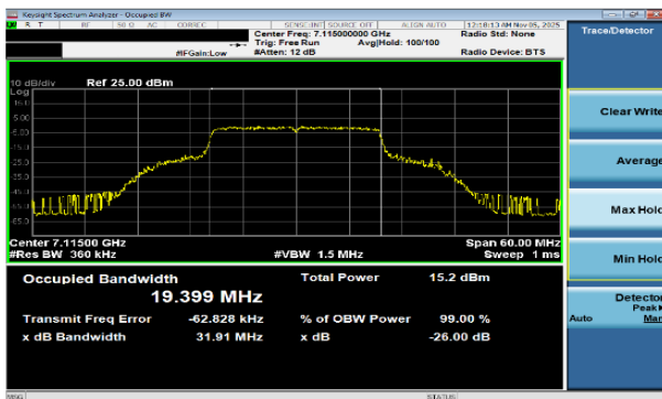
Plot 7-25 26dB BW & 99% OBW Antenna WF7a (20MHz BW 802.11be(SU) - Ch.233)
