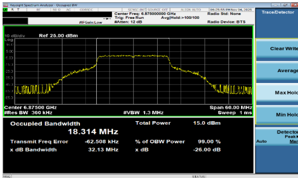
Plot 7-21 26dB BW & 99% OBW Antenna WF7a (20MHz BW 802.11a - Ch.185)
