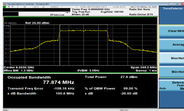
Plot 7-63 26dB BW & 99% OBW Antenna WF7b (80MHz BW 802.11be(SU) - Ch.103)
