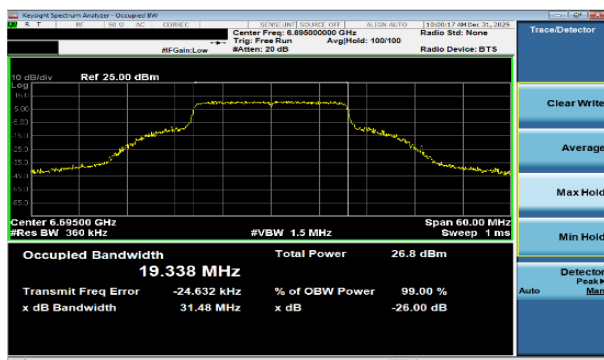
Plot 7-9 26dB BW & 99% OBW Antenna WF7a (20MHz BW 802.11be(SU) - Ch.149)
