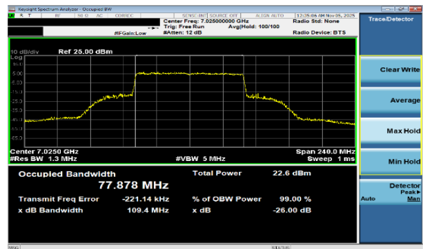
Plot 7-27 26dB BW & 99% OBW Antenna WF7a (80MHz BW 802.11be(SU) - Ch.215)
