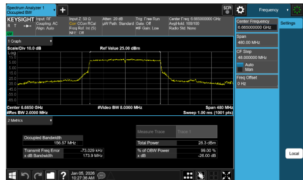
Plot 7-40 26dB BW & 99% OBW Antenna WF2a (160MHz BW 802.11be(SU) - Ch.143)
