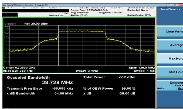
Plot 7-10 26dB BW & 99% OBW Antenna WF7a (40MHz BW 802.11be(SU) - Ch.155)
