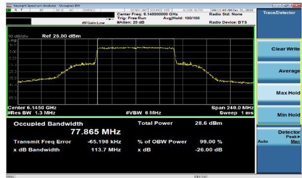
Plot 7-3 26dB BW & 99% OBW Antenna WF7a (80MHz BW 802.11be(SU) - Ch.39)
