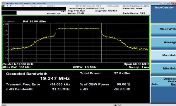
Plot 7-1 26dB BW & 99% OBW Antenna WF7a (20MHz BW 802.11be(SU) - Ch.45)
