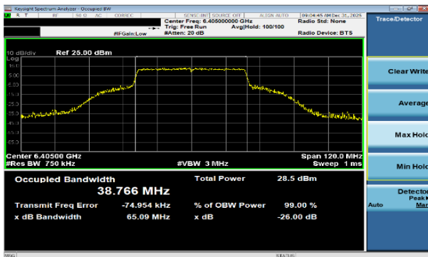
Plot 7-2 26dB BW & 99% OBW Antenna WF7a (40MHz BW 802.11be(SU) - Ch.91)
