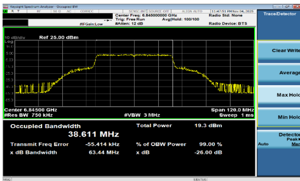
Plot 7-22 26dB BW & 99% OBW Antenna WF7a (40MHz BW 802.11be(SU) - Ch.179)
