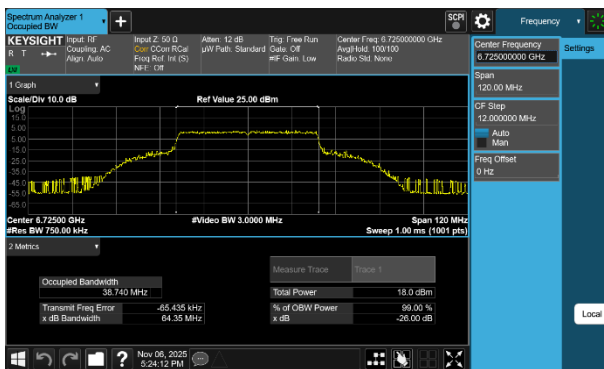
Plot 7-78 26dB BW & 99% OBW Antenna WF7b (40MHz BW 802.11be(SU) - Ch.155)
