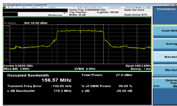
Plot 7-12 26dB BW & 99% OBW Antenna WF7a (160MHz BW 802.11be(SU) - Ch.143)
