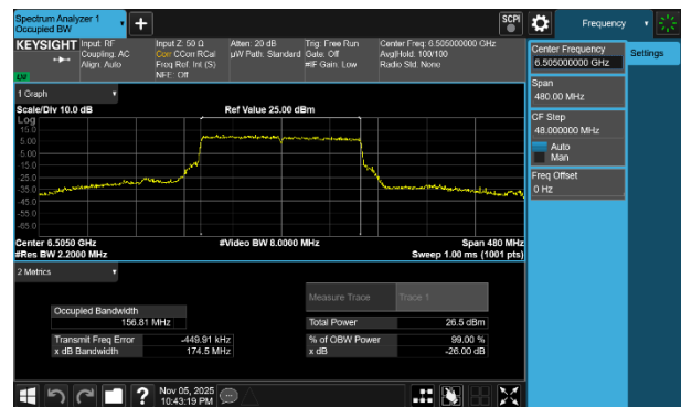
Plot 7-48 26dB BW & 99% OBW Antenna WF2a (160MHz BW 802.11be(SU) - Ch.111)
