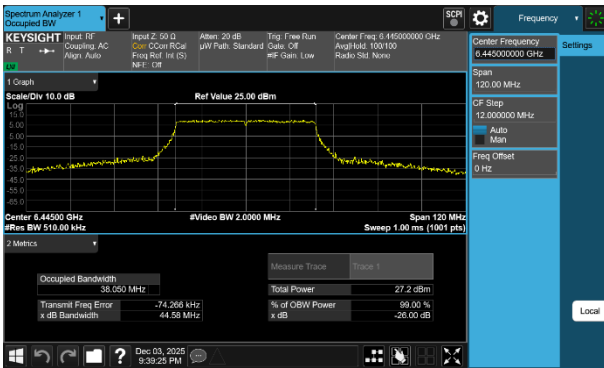
Plot 7-34 26dB BW & 99% OBW Antenna WF2a (40MHz BW 802.11be(SU) - Ch.99)
