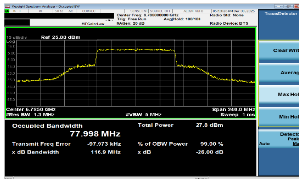
Plot 7-67 26dB BW & 99% OBW Antenna WF7b (80MHz BW 802.11be(SU) - Ch.167)
