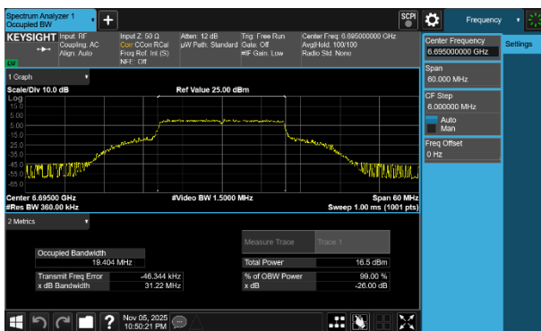
Plot 7-49 26dB BW & 99% OBW Antenna WF2a (20MHz BW 802.11be(SU) - Ch.149)
