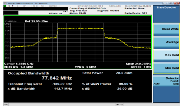
Plot 7-59 26dB BW & 99% OBW Antenna WF7b (80MHz BW 802.11be(SU) - Ch.87)
