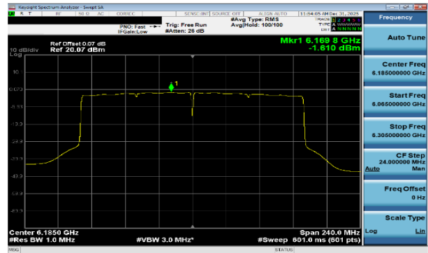
Plot 7-88 PSD Antenna WF7a (160MHz BW 802.11be(SU) - Ch.47)
