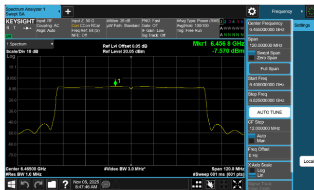
Plot 7-55 PSD Antenna WF7a (80MHz BW 802.11b(SU) - Ch.103)
