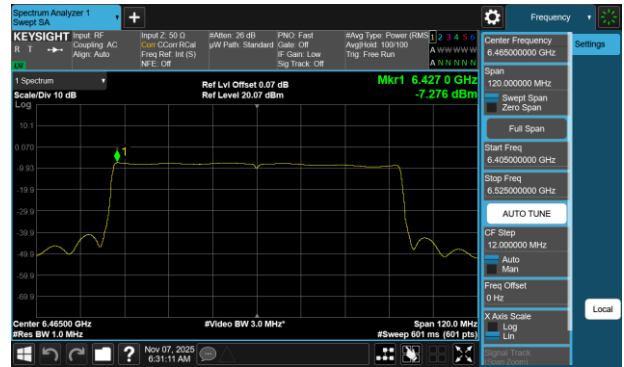
Plot 7-71 PSD Antenna WF2a (80MHz BW 802.11be(SU) - Ch.103)
