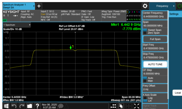
Plot 7-54 PSD Antenna WF7a (40MHz BW 802.11b(SU) - Ch.99)
