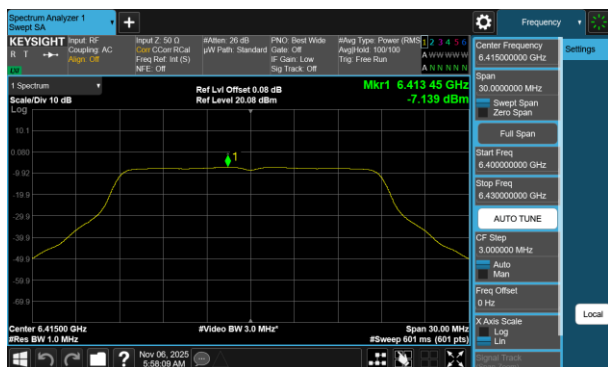
Plot 7-49 PSD Antenna WF7a (20MHz BW 802.11a - Ch.93)
