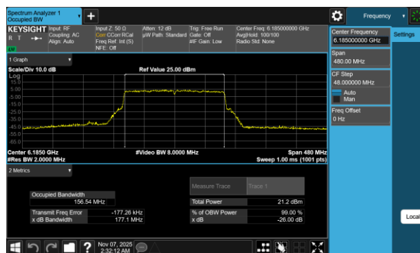
Plot 7-20 26dB BW & 99% OBW Antenna WF2a (160MHz BW 802.11be(SU) - Ch.47)
