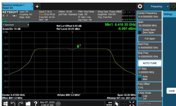
Plot 7-65 PSD Antenna WF2a (20MHz BW 802.11a - Ch.93)
