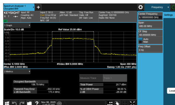
Plot 7-4 26dB BW & 99% OBW Antenna WF7a (160MHz BW 802.11be(SU) - Ch.47)
