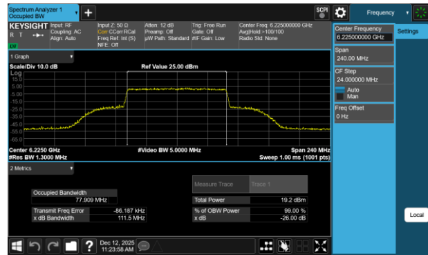
Plot 7-35 26dB BW & 99% OBW Antenna WF7b (80MHz BW 802.11be(SU) - Ch.55)
