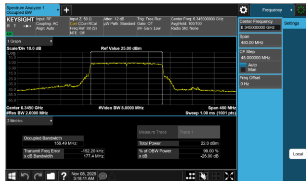
Plot 7-36 26dB BW & 99% OBW Antenna WF7b (160MHz BW 802.11be(SU) - Ch.79)
