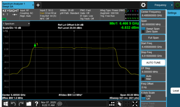
Plot 7-70 PSD Antenna WF2a (40MHz BW 802.11be(SU) - Ch.107)
