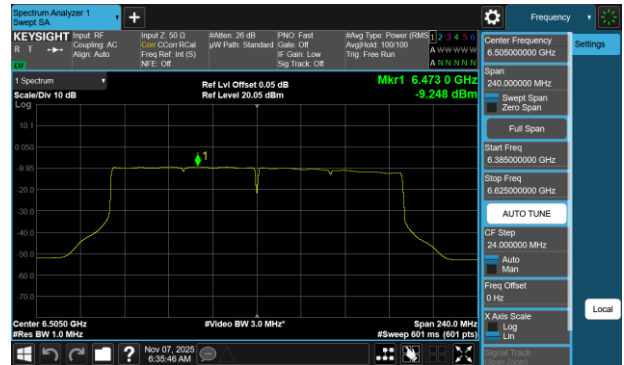
Plot 7-72 PSD Antenna WF2a (160MHz BW 802.11be(SU) - Ch.111)
