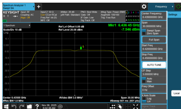
Plot 7-53 PSD Antenna WF7a (20MHz BW 802.11a - Ch.97)
