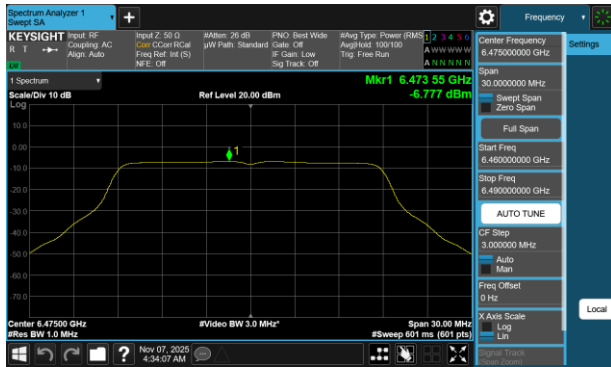
Plot 7-69 PSD Antenna WF2a (20MHz BW 802.11a - Ch.105)
