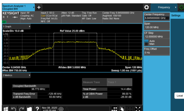
Plot 7-42 26dB BW & 99% OBW Antenna WF7b (40MHz BW 802.11be(SU) - Ch.179)
