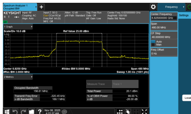
Plot 7-44 26dB BW & 99% OBW Antenna WF7b (160MHz BW 802.11be(SU) - Ch.175)
