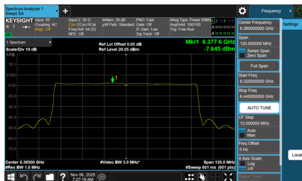
Plot 7-51 PSD Antenna WF7a (80MHz BW 802.11b(SU) - Ch.87)
