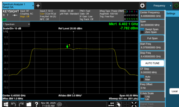
Plot 7-50 PSD Antenna WF7a (40MHz BW 802.11b(SU) - Ch.91)
