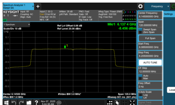
Plot 7-67 PSD Antenna WF2a (80MHz BW 802.11b(SU) - Ch.39)
