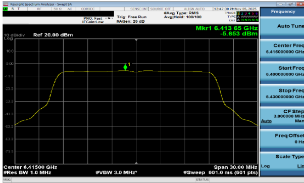
Plot 7-193 PSD SDM Primary Antenna WF7a (20MHz BW 802.11be(SU) - Ch.93)
