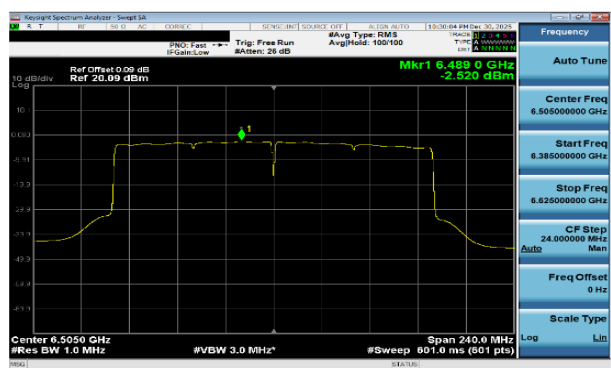
Plot 7-240 PSD CDD Diversity Antenna WF7b (160MHz BW 802.11b(SU) - Ch.111)
