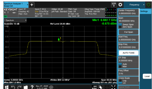
Plot 7-278 PSD SDM Diversity Antenna WF7b (40MHz BW 802.11be(SU) - Ch.187)
