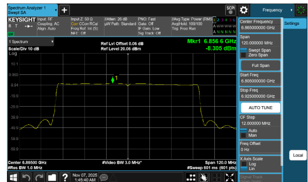
Plot 7-271 PSD SDM Diversity Antenna WF7b (80MHz BW 802.11be(SU) - Ch.183)
