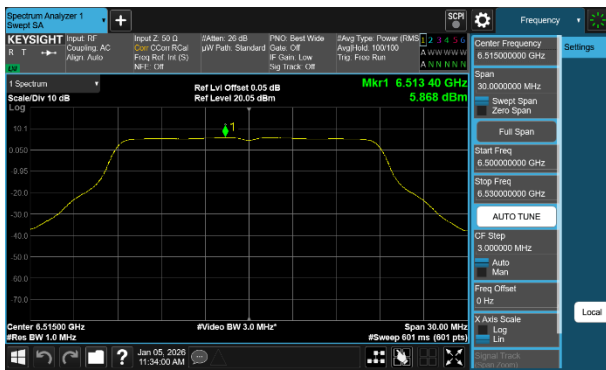
Plot 7-233 PSD CDD Diversity Antenna WF2a (20MHz BW 802.11a - Ch.113)
