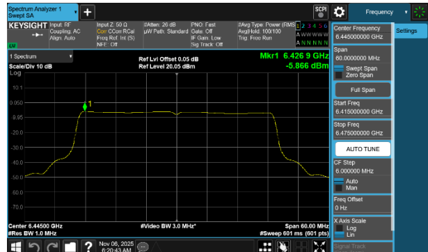
Plot 7-206 PSD SDM Primary Antenna WF2a (40MHz BW 802.11be(SU) - Ch.99)
