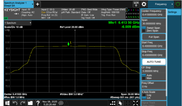
Plot 7-197 PSD SDM Primary Antenna WF2a (20MHz BW 802.11be(SU) - Ch.93)
