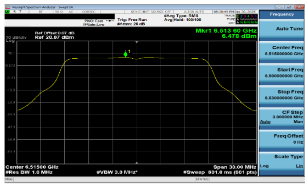
Plot 7-237 PSD CDD Diversity Antenna WF7b (20MHz BW 802.11a - Ch.113)
