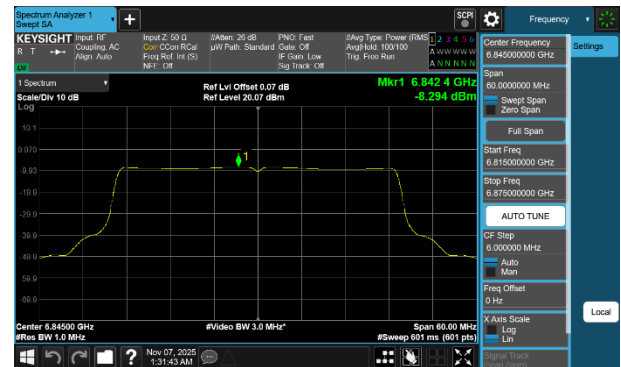
Plot 7-270 PSD SDM Diversity Antenna WF7b (40MHz BW 802.11be(SU) - Ch.179)
