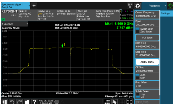
Plot 7-276 PSD SDM Diversity Antenna WF2a (160MHz BW 802.11be(SU) - Ch.207)
