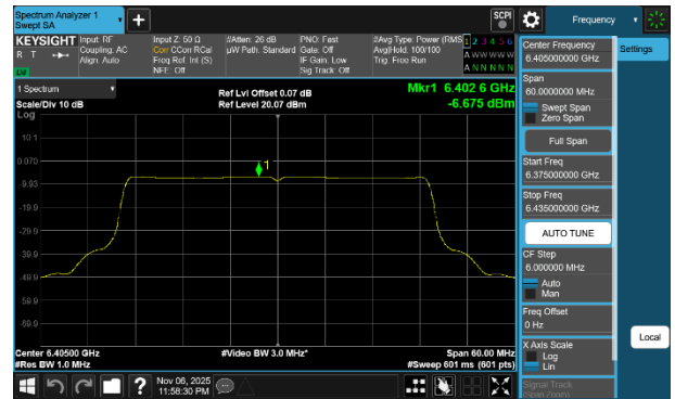
Plot 7-254 PSD SDM Diversity Antenna WF7b (40MHz BW 802.11be(SU) - Ch.91)
