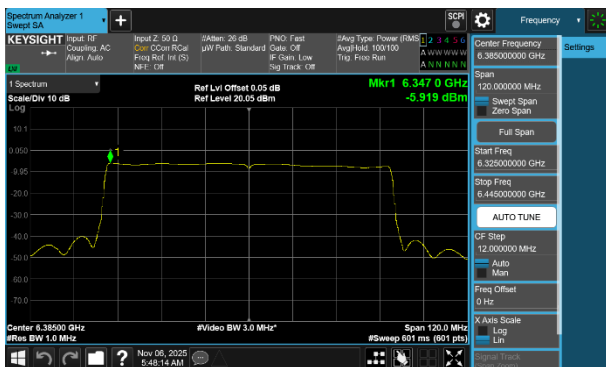
Plot 7-251 PSD SDM Diversity Antenna WF2a (80MHz BW 802.11be(SU) - Ch.87)
