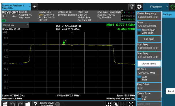
Plot 7-243 PSD CDD Diversity Antenna WF2a (80MHz BW 802.11b(SU) - Ch.167)
