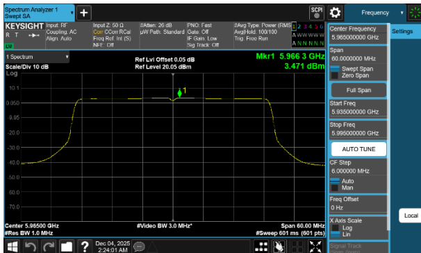
Plot 7-226 PSD CDD Diversity Antenna WF2a (40MHz BW 802.11be(SU) - Ch.3)
