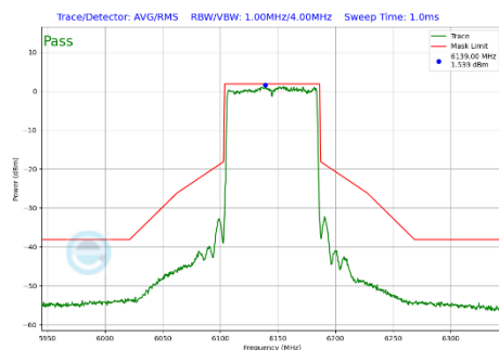
Plot 7-283 In-Band Emission Plot Antenna WF7a (80MHz BW 802.11be(SU) (UNII Band 5) - Ch.39)
