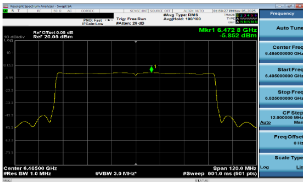
Plot 7-203 PSD SDM Primary Antenna WF7a (80MHz BW 802.11be(SU) - Ch.103)
