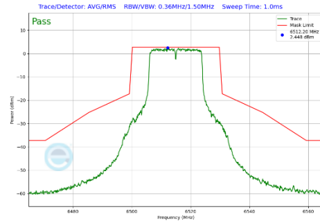
Plot 7-285 In-Band Emission Plot Antenna WF7a (20MHz BW 802.11a (UNII Band 6) - Ch.113)
