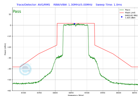
Plot 7-287 In-Band Emission Plot Antenna WF7a (80MHz BW 802.11be(SU) (UNII Band 6) - Ch.103)
