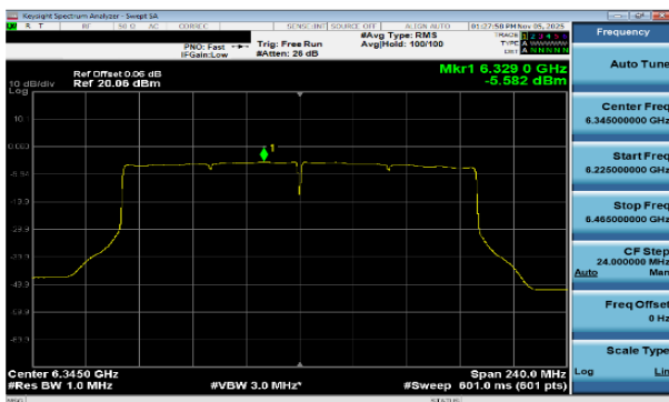
Plot 7-196 PSD SDM Primary Antenna WF7a (160MHz BW 802.11be(SU) - Ch.79)
