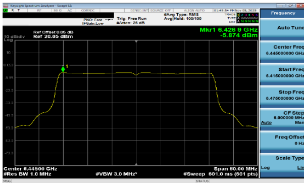
Plot 7-202 PSD SDM Primary Antenna WF7a (40MHz BW 802.11be(SU) - Ch.99)
