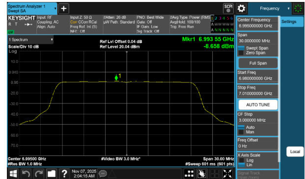
Plot 7-277 PSD SDM Diversity Antenna WF7b (20MHz BW 802.11be(SU) - Ch.209)
