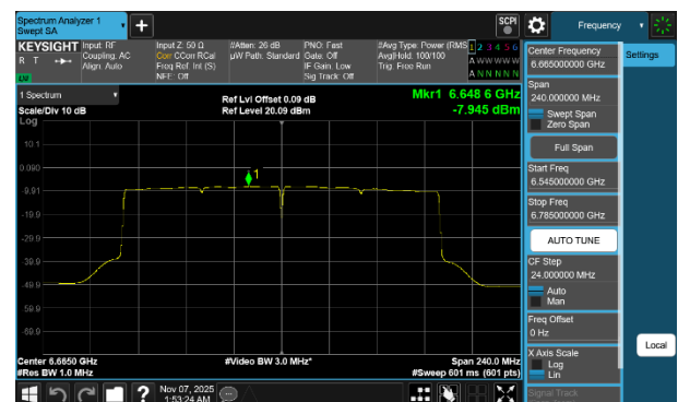
Plot 7-272 PSD SDM Diversity Antenna WF7b (160MHz BW 802.11be(SU) - Ch.143)
