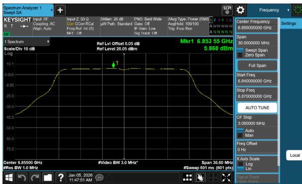
Plot 7-241 PSD CDD Diversity Antenna WF2a (20MHz BW 802.11a - Ch.181)
