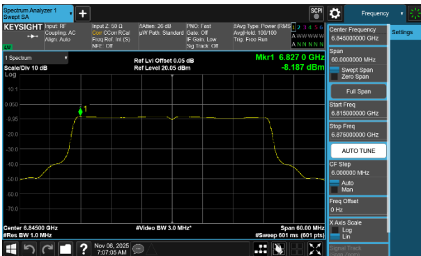
Plot 7-266 PSD SDM Diversity Antenna WF2a (40MHz BW 802.11be(SU) - Ch.179)
