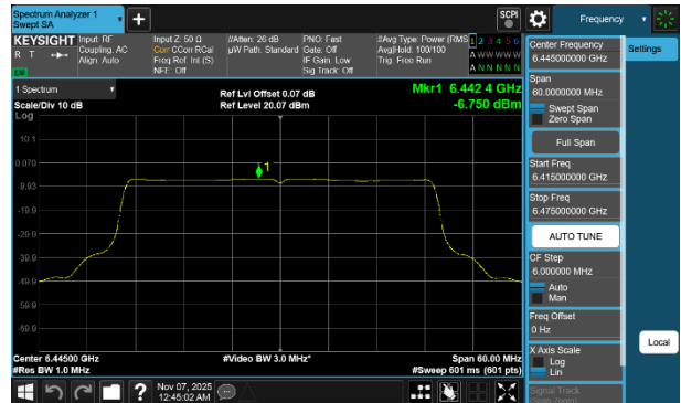
Plot 7-262 PSD SDM Diversity Antenna WF7b (40MHz BW 802.11be(SU) - Ch.99)
