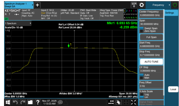
Plot 7-269 PSD SDM Diversity Antenna WF7b (20MHz BW 802.11be(SU) - Ch.149)
