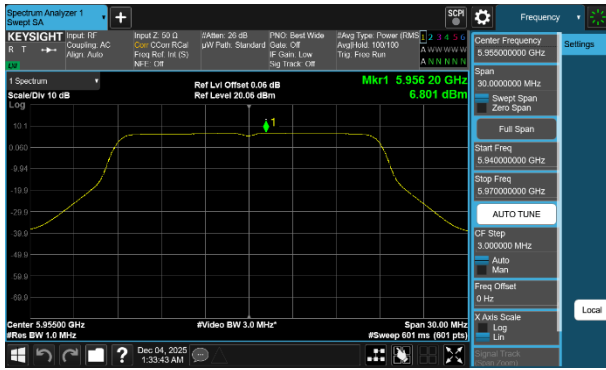
Plot 7-225 PSD CDD Diversity Antenna WF2a (20MHz BW 802.11a - Ch.1)
