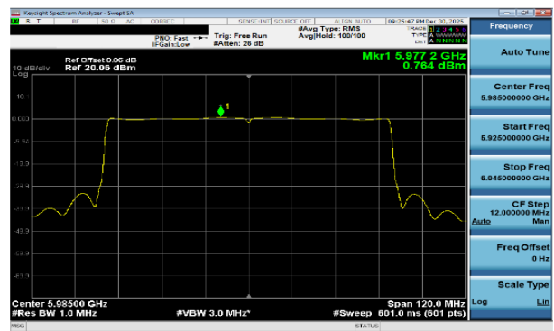
Plot 7-231 PSD CDD Diversity Antenna WF7b (80MHz BW 802.11be(SU) - Ch.7)
