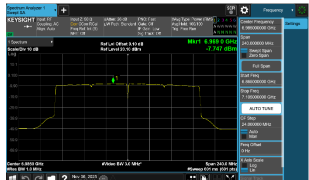
Plot 7-224 PSD SDM Primary Antenna WF2a (160MHz BW 802.11be(SU) - Ch.207)
