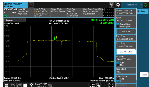
Plot 7-280 PSD SDM Diversity Antenna WF7b (160MHz BW 802.11be(SU) - Ch.207)
