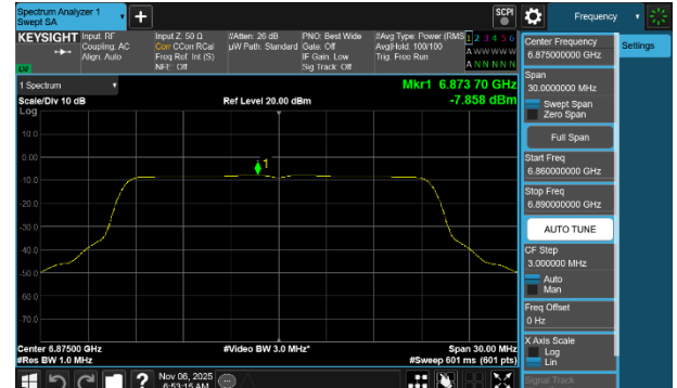
Plot 7-213 PSD SDM Primary Antenna WF2a (20MHz BW 802.11be(SU) - Ch.185)
