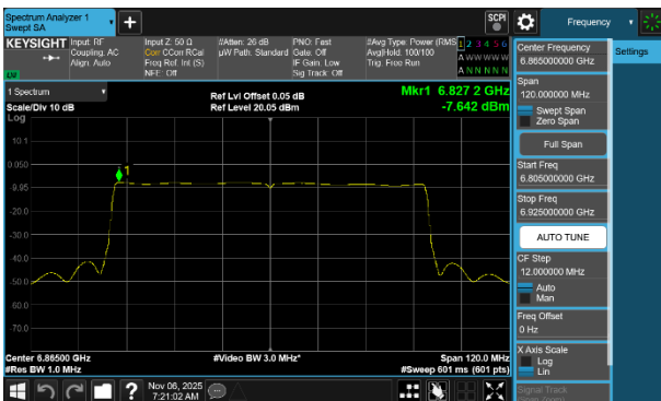
Plot 7-267 PSD SDM Diversity Antenna WF2a (80MHz BW 802.11be(SU) - Ch.183)
