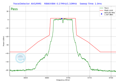
Plot 7-289 In-Band Emission Plot Antenna WF7a (20MHz BW 802.11a (UNII Band 7) - Ch.149)
