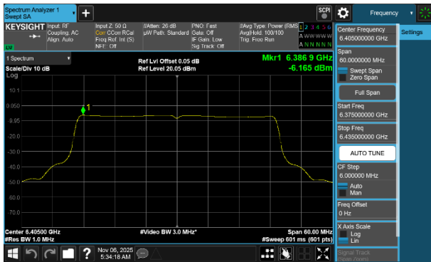
Plot 7-250 PSD SDM Diversity Antenna WF2a (40MHz BW 802.11be(SU) - Ch.91)
