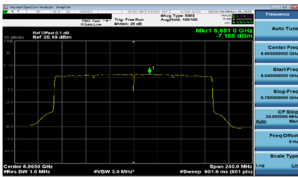
Plot 7-212 PSD SDM Primary Antenna WF7a (160MHz BW 802.11be(SU) - Ch.143)
