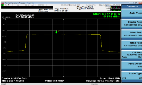
Plot 7-195 PSD SDM Primary Antenna WF7a (80MHz BW 802.11be(SU) - Ch.87)
