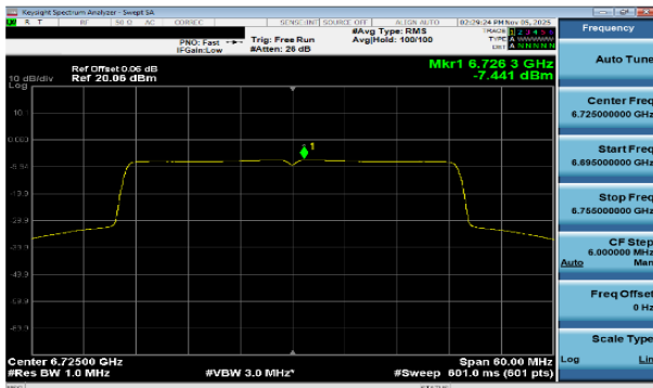
Plot 7-210 PSD SDM Primary Antenna WF7a (40MHz BW 802.11be(SU) - Ch.155)
