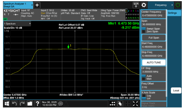
Plot 7-261 PSD CDD Diversity Antenna WF7b (20MHz BW 802.11a - Ch.105)
