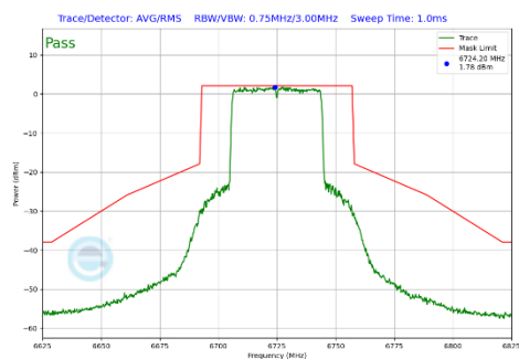
Plot 7-290 In-Band Emission Plot Antenna WF7a (40MHz BW 802.11be(SU) (UNII Band 7) - Ch.155)
