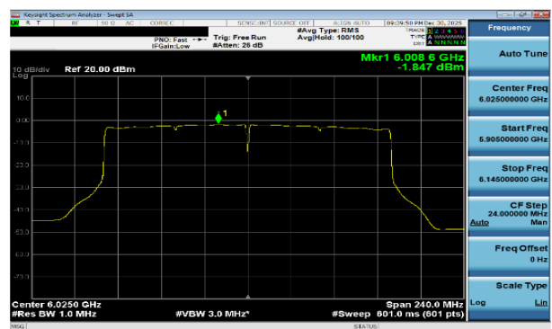
Plot 7-232 PSD CDD Diversity Antenna WF7b (160MHz BW 802.11be(SU) - Ch.15)
