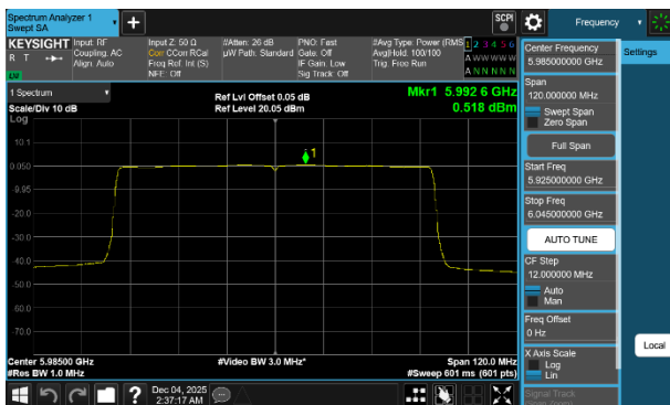
Plot 7-227 PSD CDD Diversity Antenna WF2a (80MHz BW 802.11be(SU) - Ch.7)
