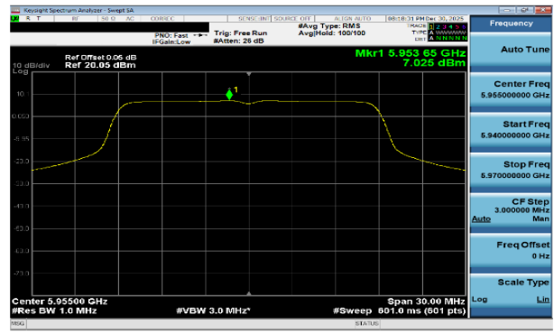
Plot 7-229 PSD CDD Diversity Antenna WF7b (20MHz BW 802.11a - Ch.1)
