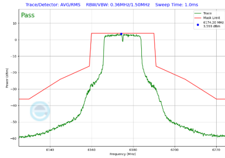
Plot 7-281 In-Band Emission Plot Antenna WF7a (20MHz BW 802.11a (UNII Band 5) - Ch.45)
