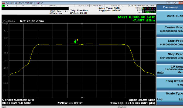
Plot 7-217 PSD SDM Primary Antenna WF7a (20MHz BW 802.11be(SU) - Ch.189)
