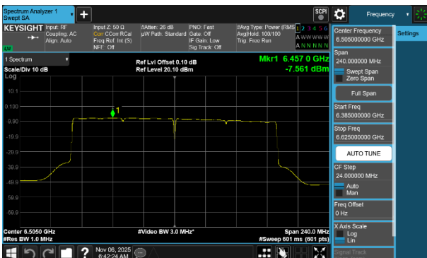
Plot 7-260 PSD SDM Diversity Antenna WF2a (160MHz BW 802.11be(SU) - Ch.111)
