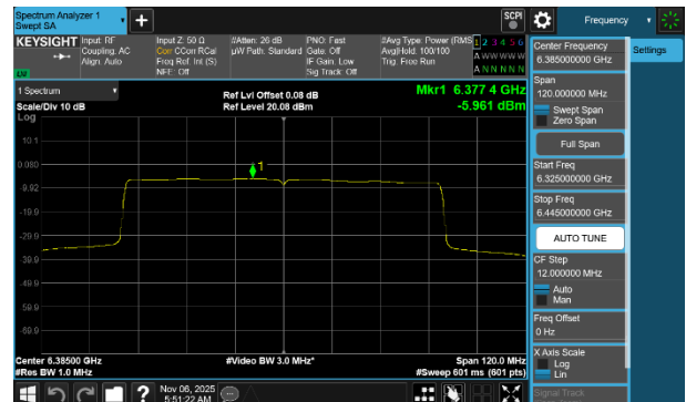
Plot 7-199 PSD SDM Primary Antenna WF2a (80MHz BW 802.11be(SU) - Ch.87)
