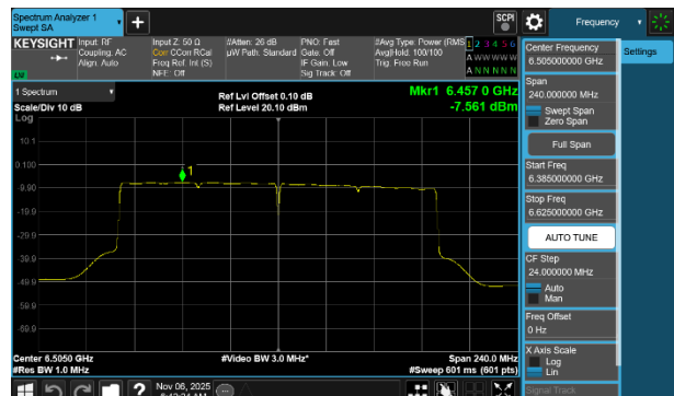
Plot 7-208 PSD SDM Primary Antenna WF2a (160MHz BW 802.11be(SU) - Ch.111)
