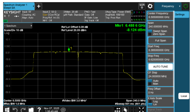
Plot 7-264 PSD SDM Diversity Antenna WF7b (160MHz BW 802.11be(SU) - Ch.111)
