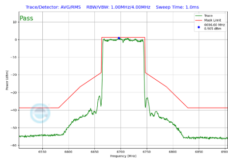
Plot 7-291 In-Band Emission Plot Antenna WF7a (80MHz BW 802.11be(SU) (UNII Band 7) - Ch.151)
