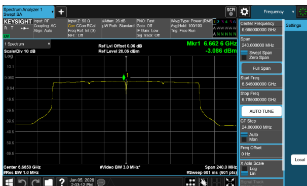
Plot 7-244 PSD CDD Diversity Antenna WF2a (160MHz BW 802.11b(SU) - Ch.143)
