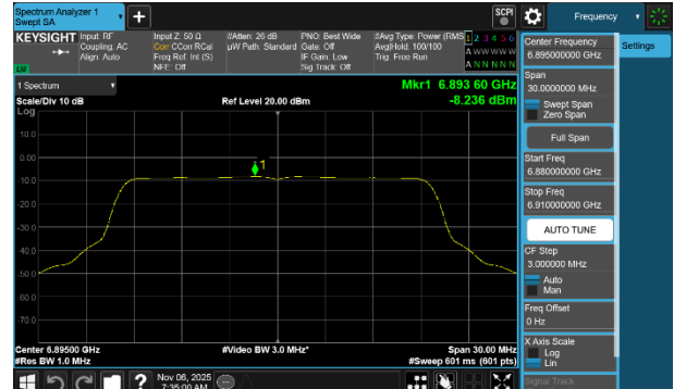
Plot 7-221 PSD SDM Primary Antenna WF2a (20MHz BW 802.11be(SU) - Ch.189)
