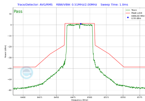
Plot 7-286 In-Band Emission Plot Antenna WF7a (40MHz BW 802.11be(SU) (UNII Band 6) - Ch.107)
