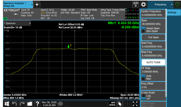
Plot 7-205 PSD CDD Primary Antenna WF2a (20MHz BW 802.11a - Ch.97)
