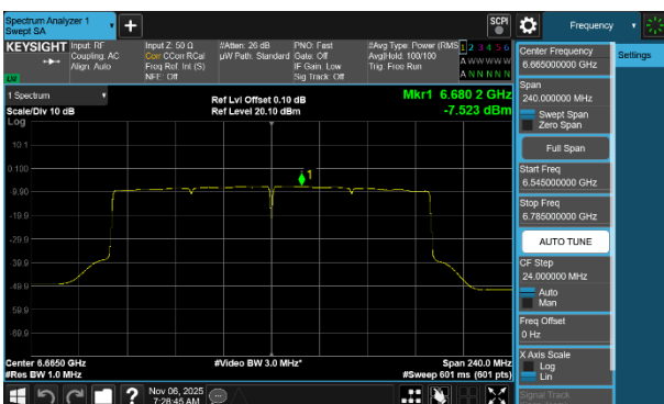
Plot 7-268 PSD SDM Diversity Antenna WF2a (160MHz BW 802.11be(SU) - Ch.143)
