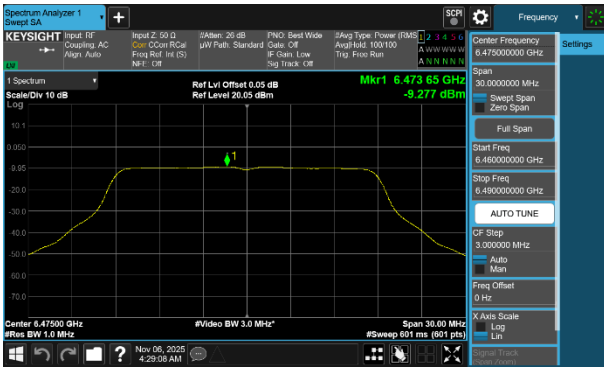
Plot 7-257 PSD CDD Diversity Antenna WF2a (20MHz BW 802.11a - Ch.105)
