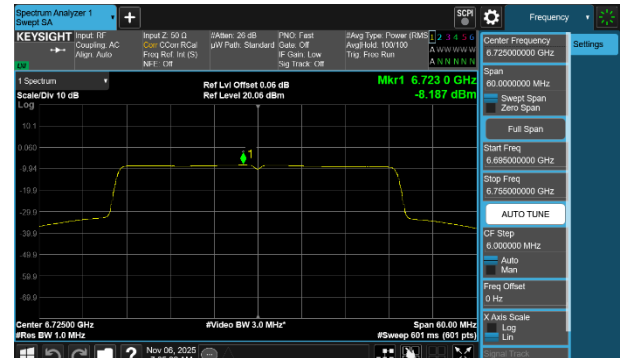
Plot 7-214 PSD SDM Primary Antenna WF2a (40MHz BW 802.11be(SU) - Ch.155)
