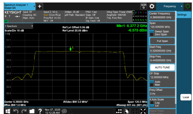
Plot 7-255 PSD SDM Diversity Antenna WF7b (80MHz BW 802.11be(SU) - Ch.87)
