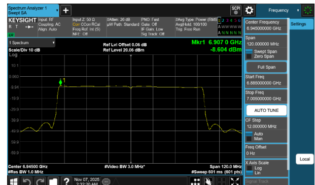
Plot 7-279 PSD SDM Diversity Antenna WF7b (80MHz BW 802.11be(SU) - Ch.199)
