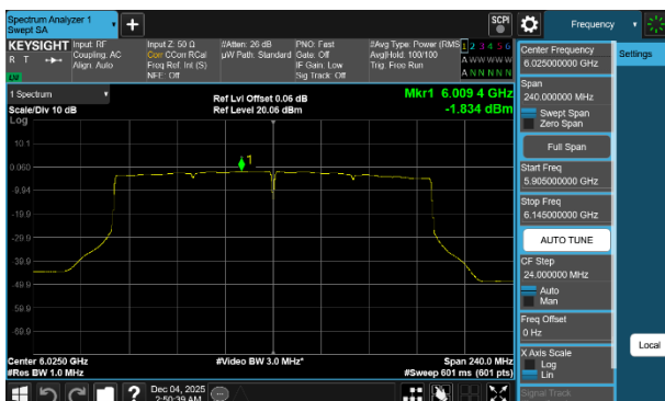
Plot 7-228 PSD CDD Diversity Antenna WF2a (160MHz BW 802.11be(SU) - Ch.15)
