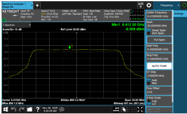
Plot 7-249 PSD SDM Diversity Antenna WF2a (20MHz BW 802.11be(SU) - Ch.93)
