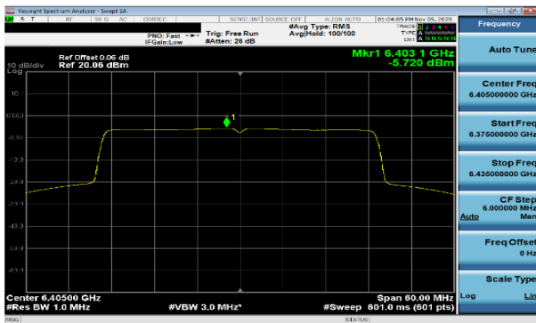
Plot 7-194 PSD SDM Primary Antenna WF7a (40MHz BW 802.11be(SU) - Ch.91)
