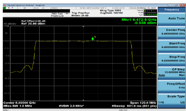
Plot 7-239 PSD CDD Diversity Antenna WF7b (80MHz BW 802.11b(SU) - Ch.103)
