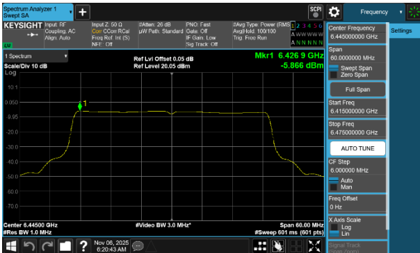
Plot 7-258 PSD SDM Diversity Antenna WF2a (40MHz BW 802.11be(SU) - Ch.99)
