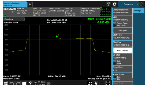
Plot 7-198 PSD SDM Primary Antenna WF2a (40MHz BW 802.11be(SU) - Ch.91)
