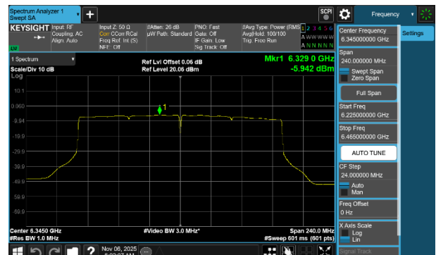
Plot 7-200 PSD SDM Primary Antenna WF2a (160MHz BW 802.11be(SU) - Ch.79)
