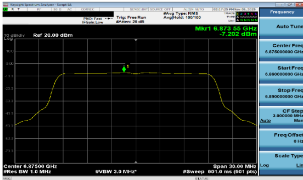
Plot 7-209 PSD SDM Primary Antenna WF7a (20MHz BW 802.11be(SU) - Ch.185)
