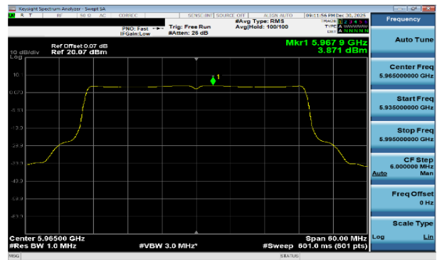
Plot 7-230 PSD CDD Diversity Antenna WF7b (40MHz BW 802.11be(SU) - Ch.3)
