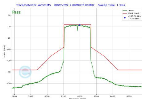
Plot 7-284 In-Band Emission Plot Antenna WF7a (160MHz BW 802.11be(SU) (UNII Band 5) - Ch.47)
