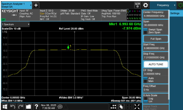
Plot 7-273 PSD SDM Diversity Antenna WF2a (20MHz BW 802.11be(SU) - Ch.209)
