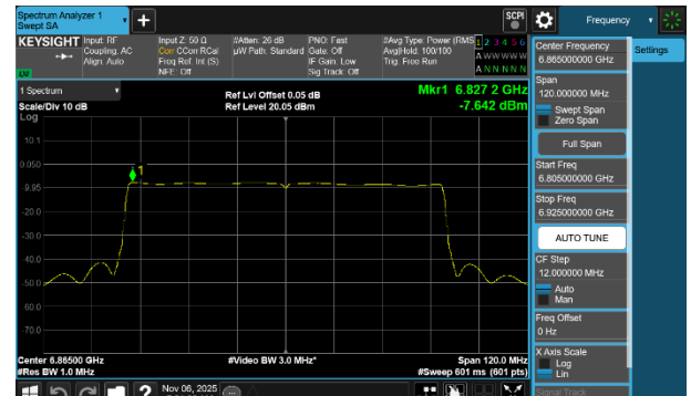
Plot 7-215 PSD SDM Primary Antenna WF2a (80MHz BW 802.11be(SU) - Ch.183)
