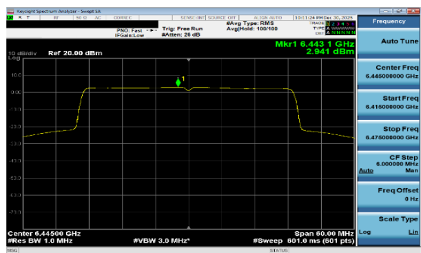
Plot 7-238 PSD CDD Diversity Antenna WF7b (40MHz BW 802.11b(SU) - Ch.99)
