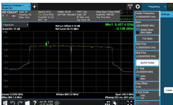
Plot 7-236 PSD CDD Diversity Antenna WF2a (160MHz BW 802.11b(SU) - Ch.111)
