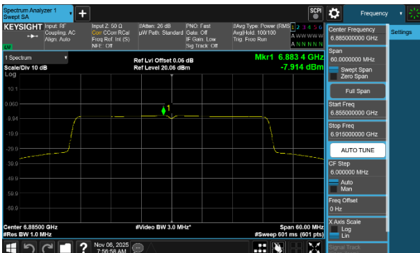
Plot 7-274 PSD SDM Diversity Antenna WF2a (40MHz BW 802.11be(SU) - Ch.187)
