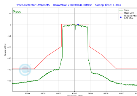
Plot 7-288 In-Band Emission Plot Antenna WF7a (160MHz BW 802.11be(SU) (UNII Band 6) - Ch.111)
