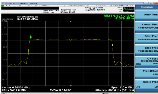
Plot 7-219 PSD SDM Primary Antenna WF7a (80MHz BW 802.11be(SU) - Ch.199)
