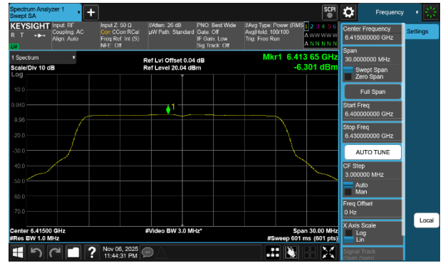
Plot 7-253 PSD SDM Diversity Antenna WF7b (20MHz BW 802.11be(SU) - Ch.93)
