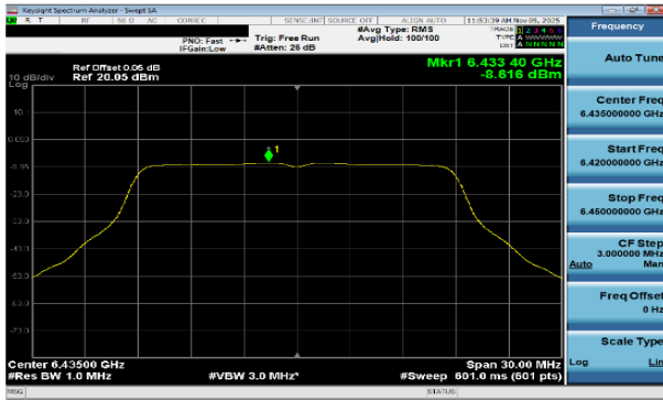
Plot 7-201 PSD CDD Primary Antenna WF7a (20MHz BW 802.11a - Ch.97)
