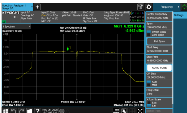
Plot 7-252 PSD SDM Diversity Antenna WF2a (160MHz BW 802.11be(SU) - Ch.79)
