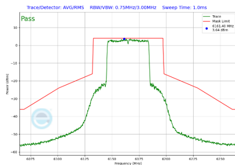
Plot 7-282 In-Band Emission Plot Antenna WF7a (40MHz BW 802.11be(SU) (UNII Band 5) - Ch.43)
