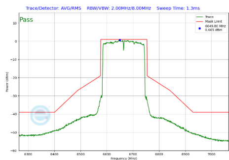
Plot 7-292 In-Band Emission Plot Antenna WF7a (160MHz BW 802.11be(SU) (UNII Band 7) - Ch.143)
