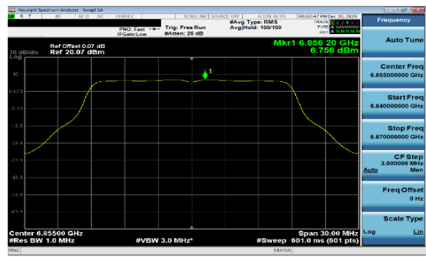
Plot 7-245 PSD CDD Diversity Antenna WF7b (20MHz BW 802.11a - Ch.181)
