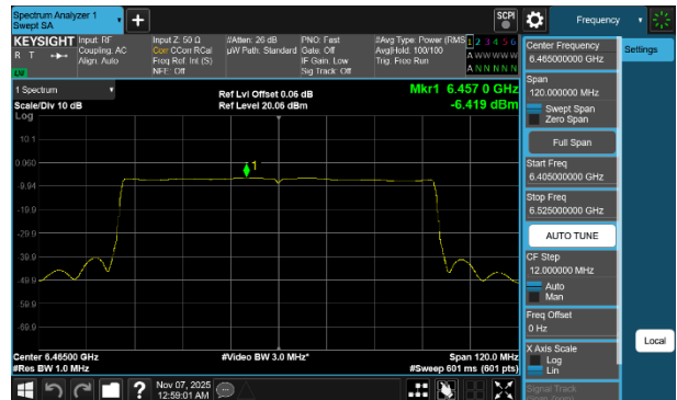
Plot 7-263 PSD SDM Diversity Antenna WF7b (80MHz BW 802.11be(SU) - Ch.103)
