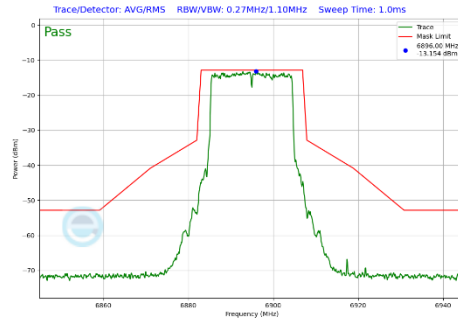
Plot 7-417 In-Band Emission Plot CDD Primary Antenna WF2a (20MHz BW 802.11be(SU) (UNII Band 8) - Ch.189)
