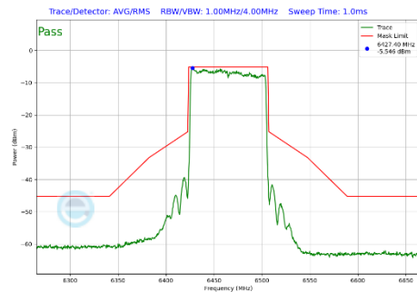
Plot 7-411 In-Band Emission Plot CDD Primary Antenna WF2a (80MHz BW 802.11be(SU) (UNII Band 6) - Ch.103)
