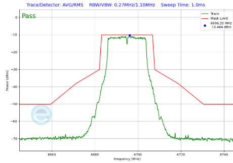
Plot 7-357 In-Band Emission Plot Antenna WF7b (20MHz BW 802.11a (UNII Band 7) - Ch.149)
