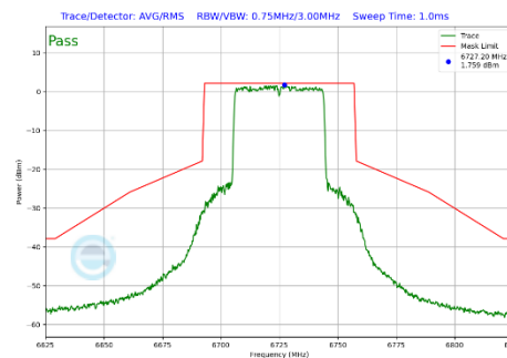
Plot 7-442 In-Band Emission Plot CDD Diversity Antenna WF2a (40MHz BW 802.11be(SU) (UNII Band 7) - Ch.155)
