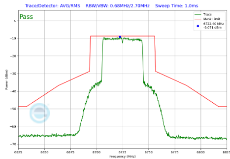
Plot 7-414 In-Band Emission Plot CDD Primary Antenna WF2a (40MHz BW 802.11be(SU) (UNII Band 7) - Ch.155)
