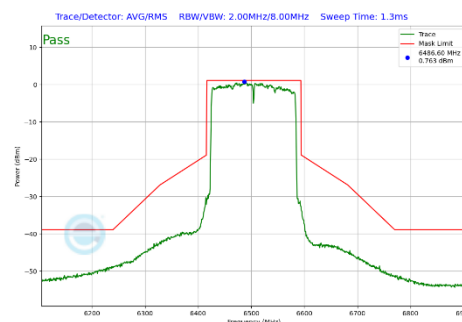
Plot 7-344 In-Band Emission Plot Antenna WF7b (160MHz BW 802.11be(SU) (UNII Band 6) - Ch.111)
