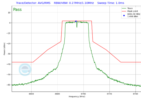
Plot 7-373 In-Band Emission Plot CDD Primary Antenna WF7a (20MHz BW 802.11a (UNII Band 7) - Ch.149)
