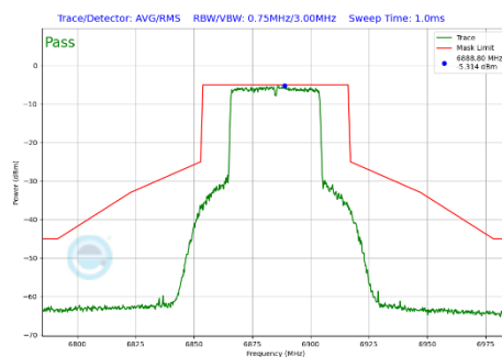
Plot 7-306 In-Band Emission Plot Antenna WF7a (40MHz BW 802.11be(SU) (UNII Band 8) - Ch.187)
