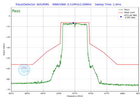
Plot 7-330 In-Band Emission Plot Antenna WF2a (40MHz BW 802.11be(SU) (UNII Band 7) - Ch.155)
