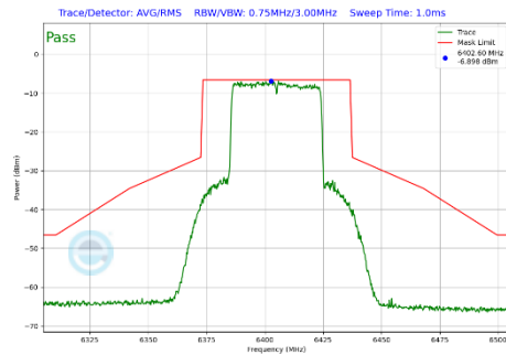
Plot 7-406 In-Band Emission Plot CDD Primary Antenna WF2a (40MHz BW 802.11be(SU) (UNII Band 5) - Ch.91)
