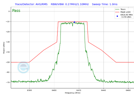
Plot 7-389 In-Band Emission Plot CDD Primary Antenna WF7a (20MHz BW 802.11be(SU) (UNII Band 5) - Ch.93)
