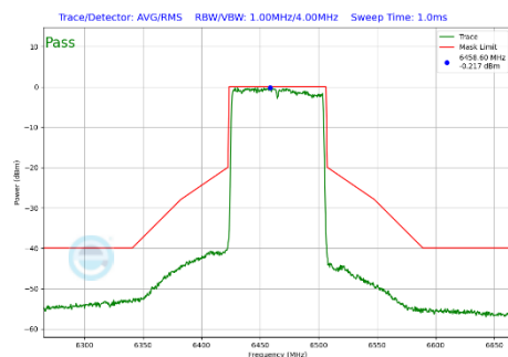
Plot 7-439 In-Band Emission Plot CDD Diversity Antenna WF2a (80MHz BW 802.11be(SU) (UNII Band 6) - Ch.103)
