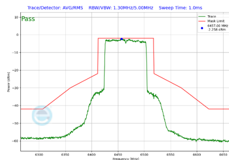
Plot 7-355 In-Band Emission Plot Antenna WF7b (80MHz BW 802.11be(SU) (UNII Band 6) - Ch.103)
