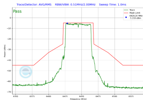
Plot 7-326 In-Band Emission Plot Antenna WF2a (40MHz BW 802.11be(SU) (UNII Band 6) - Ch.99)
