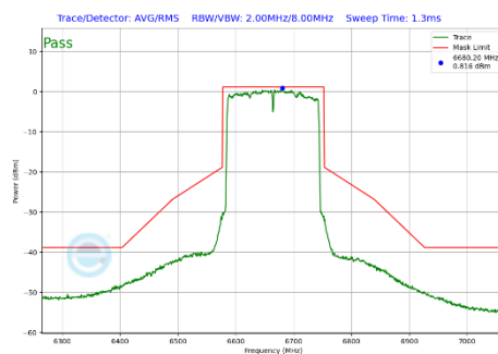
Plot 7-348 In-Band Emission Plot Antenna WF7b (160MHz BW 802.11be(SU) (UNII Band 7) - Ch.143)
