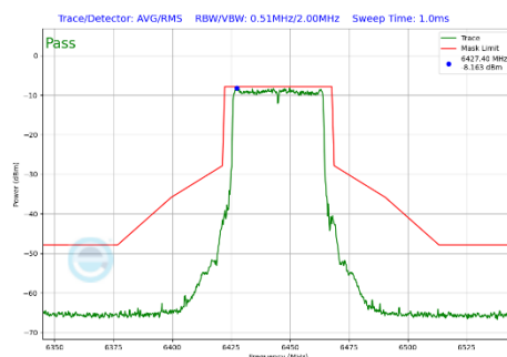
Plot 7-394 In-Band Emission Plot CDD Primary Antenna WF7a (40MHz BW 802.11be(SU) (UNII Band 6) - Ch.99)
