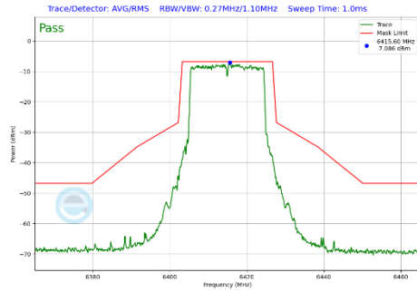
Plot 7-293 In-Band Emission Plot Antenna WF7a (20MHz BW 802.11be(SU) (UNII Band 5) - Ch.93)
