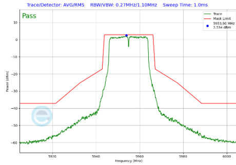
Plot 7-309 In-Band Emission Plot Antenna WF2a (20MHz BW 802.11a (UNII Band 5) - Ch.1)
