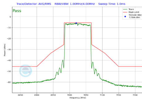
Plot 7-363 In-Band Emission Plot Antenna WF7b (80MHz BW 802.11be(SU) (UNII Band 8) - Ch.215)
