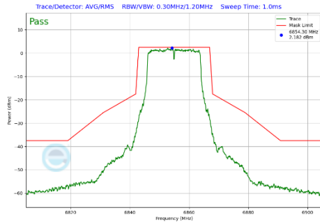
Plot 7-429 In-Band Emission Plot CDD Diversity Antenna WF7b (20MHz BW 802.11a (UNII Band 7) - Ch.181)
