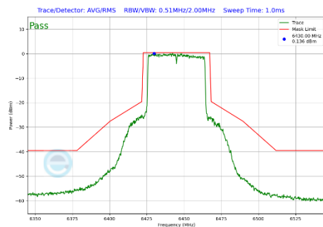
Plot 7-438 In-Band Emission Plot CDD Diversity Antenna WF2a (40MHz BW 802.11be(SU) (UNII Band 6) - Ch.99)
