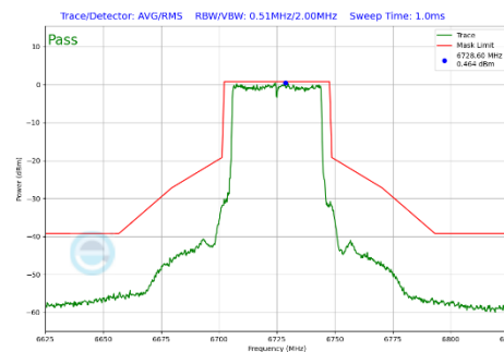
Plot 7-386 In-Band Emission Plot CDD Primary Antenna WF2a (40MHz BW 802.11be(SU) (UNII Band 7) - Ch.155)
