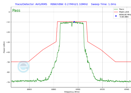
Plot 7-305 In-Band Emission Plot Antenna WF7a (20MHz BW 802.11be(SU) (UNII Band 8) - Ch.189)
