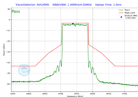
Plot 7-331 In-Band Emission Plot Antenna WF2a (80MHz BW 802.11be(SU) (UNII Band 7) - Ch.119)
