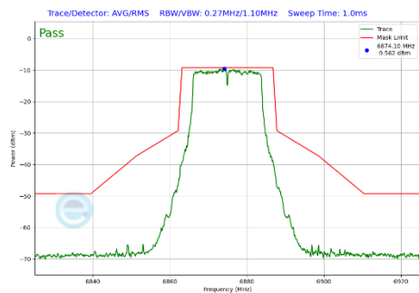
Plot 7-301 In-Band Emission Plot Antenna WF7a (20MHz BW 802.11a (UNII Band 7) - Ch.185)
