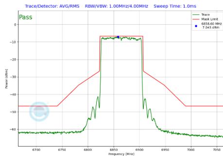
Plot 7-399 In-Band Emission Plot CDD Primary Antenna WF7a (80MHz BW 802.11be(SU) (UNII Band 7) - Ch.183)
