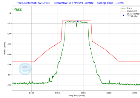
Plot 7-325 In-Band Emission Plot Antenna WF2a (20MHz BW 802.11a (UNII Band 6) - Ch.105)
