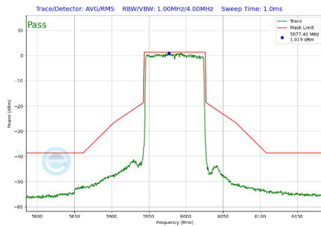
Plot 7-367 In-Band Emission Plot CDD Primary Antenna WF7a (80MHz BW 802.11be(SU) (UNII Band 5) - Ch.7)
