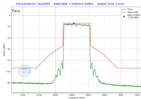
Plot 7-415 In-Band Emission Plot CDD Primary Antenna WF2a (80MHz BW 802.11be(SU) (UNII Band 7) - Ch.183)
