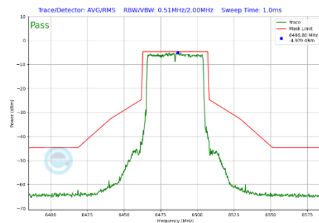
Plot 7-298 In-Band Emission Plot Antenna WF7a (40MHz BW 802.11be(SU) (UNII Band 6) - Ch.107)
