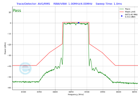
Plot 7-427 In-Band Emission Plot CDD Diversity Antenna WF7b (80MHz BW 802.11be(SU) (UNII Band 6) - Ch.103)
