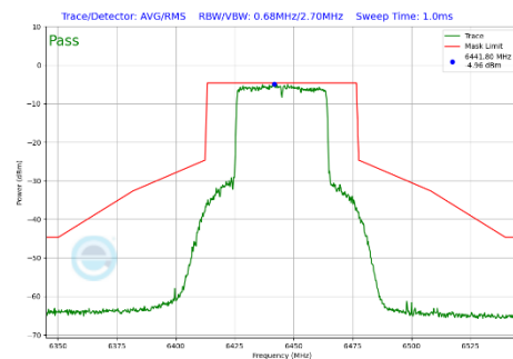
Plot 7-354 In-Band Emission Plot Antenna WF7b (40MHz BW 802.11be(SU) (UNII Band 6) - Ch.99)
