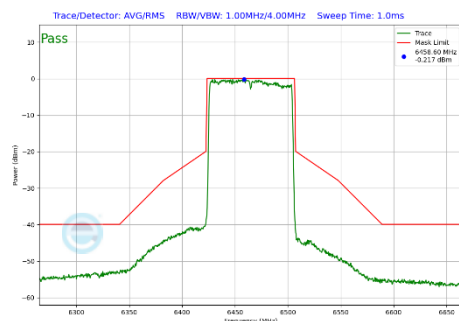
Plot 7-383 In-Band Emission Plot CDD Primary Antenna WF2a (80MHz BW 802.11be(SU) (UNII Band 6) - Ch.103)
