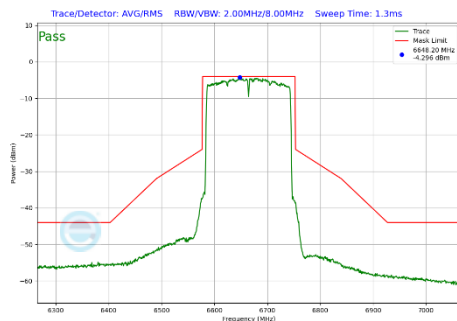
Plot 7-416 In-Band Emission Plot CDD Primary Antenna WF2a (160MHz BW 802.11be(SU) (UNII Band 7) - Ch.143)
