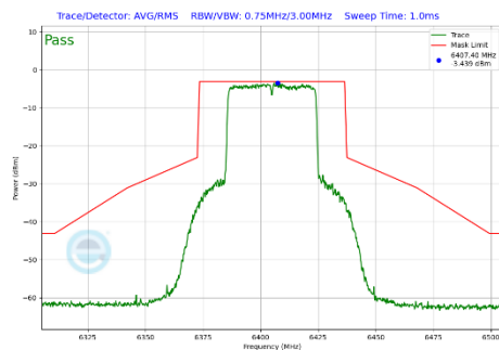
Plot 7-294 In-Band Emission Plot Antenna WF7a (40MHz BW 802.11be(SU) (UNII Band 5) - Ch.91)
