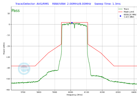
Plot 7-368 In-Band Emission Plot CDD Primary Antenna WF7a (160MHz BW 802.11be(SU) (UNII Band 5) - Ch.15)
