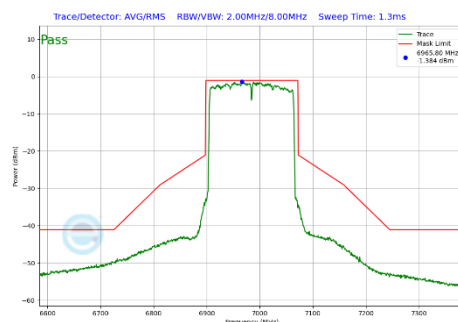
Plot 7-336 In-Band Emission Plot Antenna WF2a (160MHz BW 802.11be(SU) (UNII Band 8) - Ch.207)
