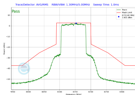
Plot 7-339 In-Band Emission Plot Antenna WF7b (80MHz BW 802.11be(SU) (UNII Band 5) - Ch.39)
