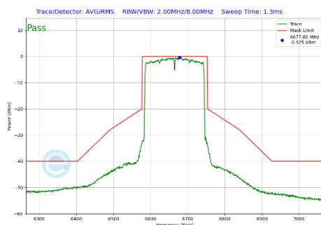
Plot 7-332 In-Band Emission Plot Antenna WF2a (160MHz BW 802.11be(SU) (UNII Band 7) - Ch.143)
