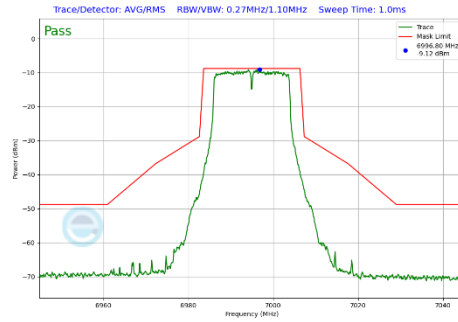
Plot 7-333 In-Band Emission Plot Antenna WF2a (20MHz BW 802.11a (UNII Band 8) - Ch.209)
