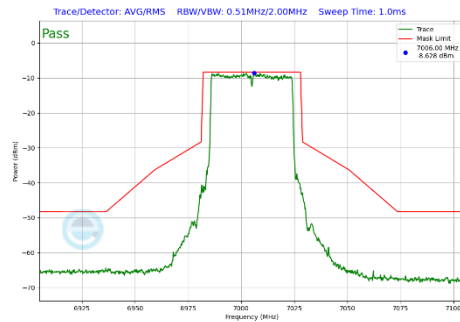
Plot 7-362 In-Band Emission Plot Antenna WF7b (40MHz BW 802.11be(SU) (UNII Band 8) - Ch.211)
