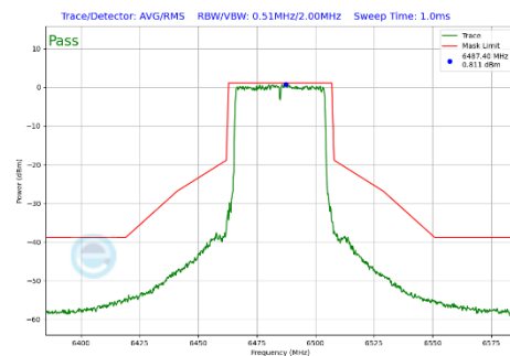
Plot 7-342 In-Band Emission Plot Antenna WF7b (40MHz BW 802.11be(SU) (UNII Band 6) - Ch.107)
