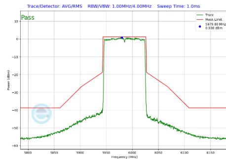
Plot 7-435 In-Band Emission Plot CDD Diversity Antenna WF2a (80MHz BW 802.11be(SU) (UNII Band 5) - Ch.7)
