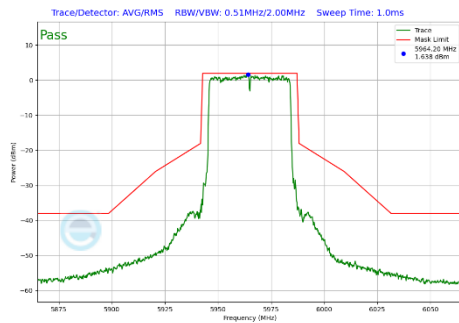
Plot 7-366 In-Band Emission Plot CDD Primary Antenna WF7a (40MHz BW 802.11be(SU) (UNII Band 5) - Ch.3)
