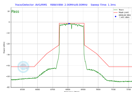
Plot 7-304 In-Band Emission Plot Antenna WF7a (160MHz BW 802.11be(SU) (UNII Band 7) - Ch.175)
