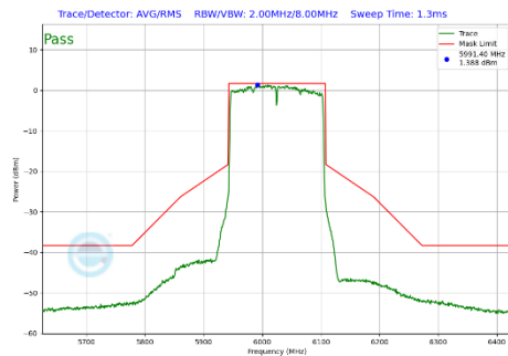
Plot 7-424 In-Band Emission Plot CDD Diversity Antenna WF7b (160MHz BW 802.11be(SU) (UNII Band 5) - Ch.15)
