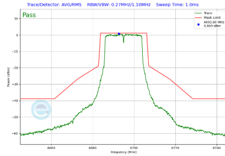
Plot 7-385 In-Band Emission Plot CDD Primary Antenna WF2a (20MHz BW 802.11a (UNII Band 7) - Ch.149)
