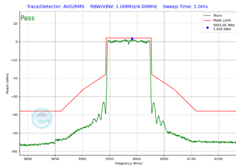
Plot 7-423 In-Band Emission Plot CDD Diversity Antenna WF7b (80MHz BW 802.11be(SU) (UNII Band 5) - Ch.7)
