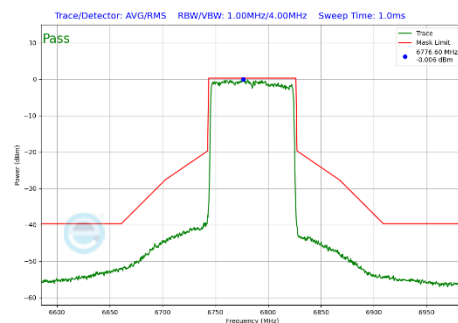
Plot 7-443 In-Band Emission Plot CDD Diversity Antenna WF2a (80MHz BW 802.11be(SU) (UNII Band 7) - Ch.167)
