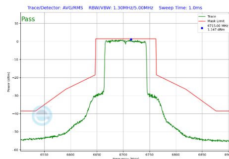
Plot 7-387 In-Band Emission Plot CDD Primary Antenna WF2a (80MHz BW 802.11be(SU) (UNII Band 7) - Ch.151)
