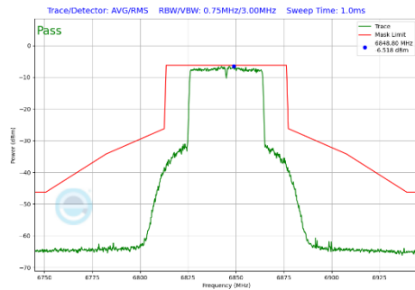
Plot 7-358 In-Band Emission Plot Antenna WF7b (40MHz BW 802.11be(SU) (UNII Band 7) - Ch.179)
