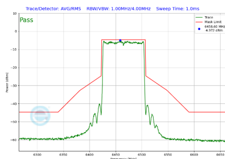
Plot 7-395 In-Band Emission Plot CDD Primary Antenna WF7a (80MHz BW 802.11be(SU) (UNII Band 6) - Ch.103)
