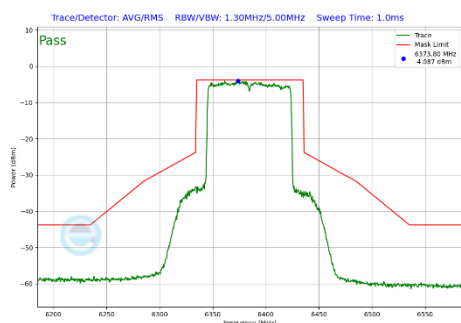
Plot 7-391 In-Band Emission Plot CDD Primary Antenna WF7a (80MHz BW 802.11be(SU) (UNII Band 5) - Ch.87)
