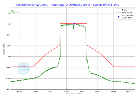
Plot 7-324 In-Band Emission Plot Antenna WF2a (160MHz BW 802.11be(SU) (UNII Band 5) - Ch.79)
