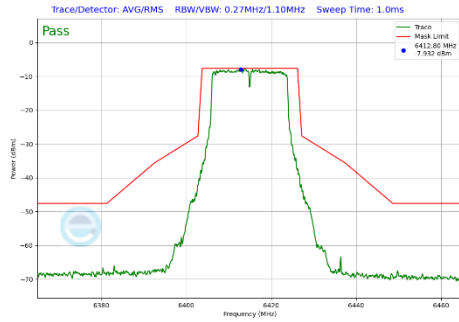
Plot 7-321 In-Band Emission Plot Antenna WF2a (20MHz BW 802.11a (UNII Band 5) - Ch.93)
