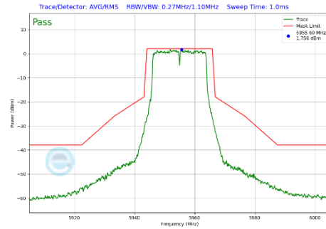
Plot 7-433 In-Band Emission Plot CDD Diversity Antenna WF2a (20MHz BW 802.11a (UNII Band 5) - Ch.1)
