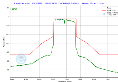
Plot 7-364 In-Band Emission Plot Antenna WF7b (160MHz BW 802.11be(SU) (UNII Band 8) - Ch.207)
