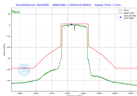
Plot 7-296 In-Band Emission Plot Antenna WF7a (160MHz BW 802.11be(SU) (UNII Band 5) - Ch.79)
