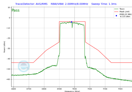
Plot 7-404 In-Band Emission Plot CDD Primary Antenna WF7a (160MHz BW 802.11be(SU) (UNII Band 8) - Ch.207)
