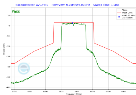
Plot 7-346 In-Band Emission Plot Antenna WF7b (40MHz BW 802.11be(SU) (UNII Band 7) - Ch.179)
