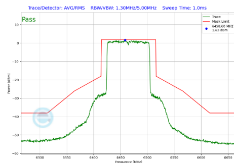
Plot 7-343 In-Band Emission Plot Antenna WF7b (80MHz BW 802.11be(SU) (UNII Band 6) - Ch.103)
