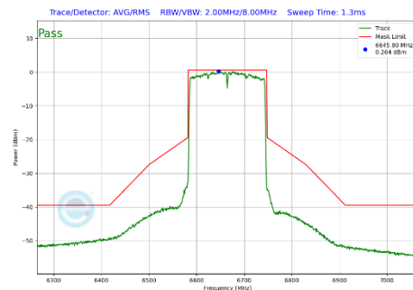
Plot 7-444 In-Band Emission Plot CDD Diversity Antenna WF2a (160MHz BW 802.11be(SU) (UNII Band 7) - Ch.143)
