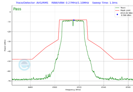
Plot 7-297 In-Band Emission Plot Antenna WF7a (20MHz BW 802.11a (UNII Band 6) - Ch.113)
