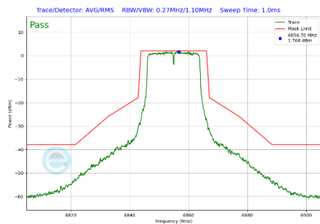
Plot 7-317 In-Band Emission Plot Antenna WF2a (20MHz BW 802.11a (UNII Band 7) - Ch.181)
