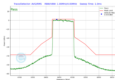
Plot 7-315 In-Band Emission Plot Antenna WF2a (80MHz BW 802.11be(SU) (UNII Band 6) - Ch.103)
