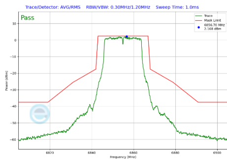
Plot 7-345 In-Band Emission Plot Antenna WF7b (20MHz BW 802.11a (UNII Band 7) - Ch.181)
