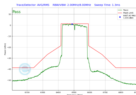
Plot 7-316 In-Band Emission Plot Antenna WF2a (160MHz BW 802.11be(SU) (UNII Band 6) - Ch.111)
