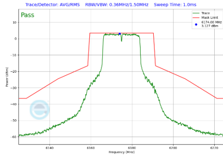
Plot 7-337 In-Band Emission Plot Antenna WF7b (20MHz BW 802.11a (UNII Band 5) - Ch.45)
