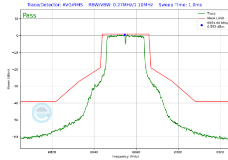
Plot 7-441 In-Band Emission Plot CDD Diversity Antenna WF2a (20MHz BW 802.11a (UNII Band 7) - Ch.181)
