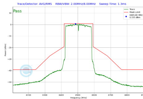
Plot 7-372 In-Band Emission Plot CDD Primary Antenna WF7a (160MHz BW 802.11be(SU) (UNII Band 6) - Ch.111)
