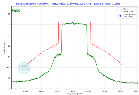
Plot 7-375 In-Band Emission Plot CDD Primary Antenna WF7a (80MHz BW 802.11be(SU) (UNII Band 7) - Ch.151)
