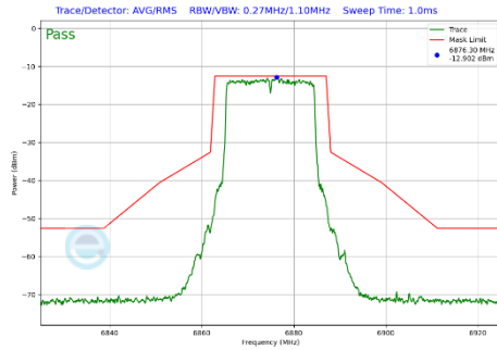
Plot 7-413 In-Band Emission Plot CDD Primary Antenna WF2a (20MHz BW 802.11be(SU) (UNII Band 7) - Ch.185)
