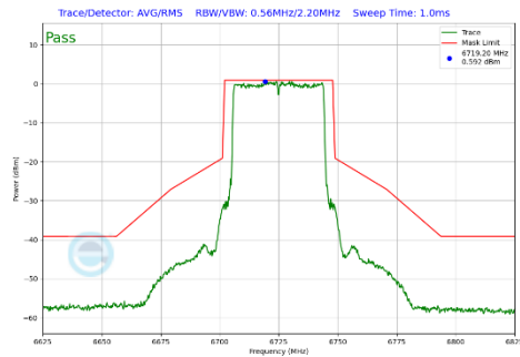
Plot 7-374 In-Band Emission Plot CDD Primary Antenna WF7a (40MHz BW 802.11be(SU) (UNII Band 7) - Ch.155)
