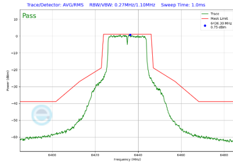
Plot 7-381 In-Band Emission Plot CDD Primary Antenna WF2a (20MHz BW 802.11a (UNII Band 6) - Ch.97)
