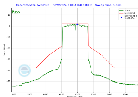
Plot 7-340 In-Band Emission Plot Antenna WF7b (160MHz BW 802.11be(SU) (UNII Band 5) - Ch.47)
