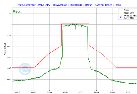
Plot 7-388 In-Band Emission Plot CDD Primary Antenna WF2a (160MHz BW 802.11be(SU) (UNII Band 7) - Ch.143)
