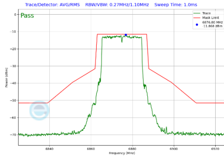
Plot 7-397 In-Band Emission Plot CDD Primary Antenna WF7a (20MHz BW 802.11be(SU) (UNII Band 7) - Ch.185)
