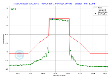
Plot 7-327 In-Band Emission Plot Antenna WF2a (80MHz BW 802.11be(SU) (UNII Band 6) - Ch.103)
