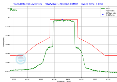
Plot 7-351 In-Band Emission Plot Antenna WF7b (80MHz BW 802.11be(SU) (UNII Band 5) - Ch.87)
