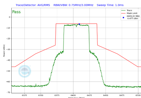
Plot 7-390 In-Band Emission Plot CDD Primary Antenna WF7a (40MHz BW 802.11be(SU) (UNII Band 5) - Ch.91)
