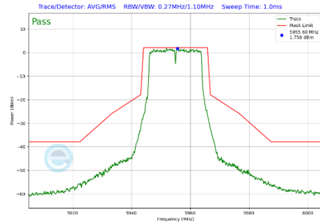
Plot 7-377 In-Band Emission Plot CDD Primary Antenna WF2a (20MHz BW 802.11a (UNII Band 5) - Ch.1)
