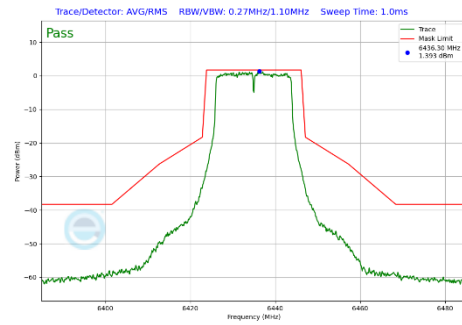
Plot 7-369 In-Band Emission Plot CDD Primary Antenna WF7a (20MHz BW 802.11a (UNII Band 6) - Ch.97)
