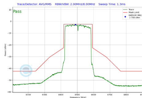
Plot 7-356 In-Band Emission Plot Antenna WF7b (160MHz BW 802.11be(SU) (UNII Band 6) - Ch.111)
