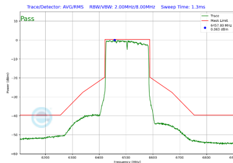
Plot 7-440 In-Band Emission Plot CDD Diversity Antenna WF2a (160MHz BW 802.11be(SU) (UNII Band 6) - Ch.111)
