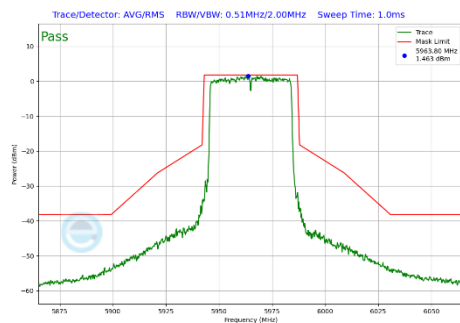
Plot 7-310 In-Band Emission Plot Antenna WF2a (40MHz BW 802.11be(SU) (UNII Band 5) - Ch.3)
