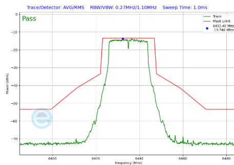
Plot 7-393 In-Band Emission Plot CDD Primary Antenna WF7a (20MHz BW 802.11a (UNII Band 6) - Ch.97)
