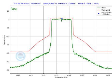
Plot 7-314 In-Band Emission Plot Antenna WF2a (40MHz BW 802.11be(SU) (UNII Band 6) - Ch.107)
