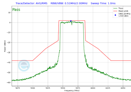
Plot 7-378 In-Band Emission Plot CDD Primary Antenna WF2a (40MHz BW 802.11be(SU) (UNII Band 5) - Ch.3)
