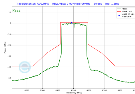
Plot 7-428 In-Band Emission Plot CDD Diversity Antenna WF7b (160MHz BW 802.11be(SU) (UNII Band 6) - Ch.111)
