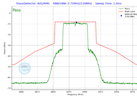
Plot 7-418 In-Band Emission Plot CDD Primary Antenna WF2a (40MHz BW 802.11be(SU) (UNII Band 8) - Ch.187)
