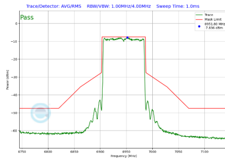
Plot 7-419 In-Band Emission Plot CDD Primary Antenna WF2a (80MHz BW 802.11be(SU) (UNII Band 8) - Ch.199)
