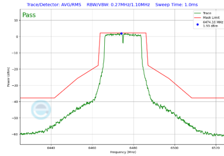
Plot 7-313 In-Band Emission Plot Antenna WF2a (20MHz BW 802.11a (UNII Band 6) - Ch.105)
