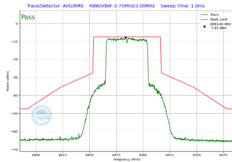
Plot 7-402 In-Band Emission Plot CDD Primary Antenna WF7a (40MHz BW 802.11be(SU) (UNII Band 8) - Ch.187)
