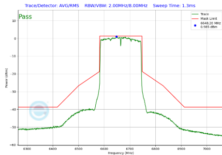
Plot 7-432 In-Band Emission Plot CDD Diversity Antenna WF7b (160MHz BW 802.11be(SU) (UNII Band 7) - Ch.143)
