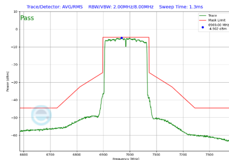
Plot 7-420 In-Band Emission Plot CDD Primary Antenna WF2a (160MHz BW 802.11be(SU) (UNII Band 8) - Ch.207)
