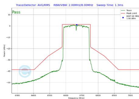
Plot 7-320 In-Band Emission Plot Antenna WF2a (160MHz BW 802.11be(SU) (UNII Band 7) - Ch.143)
