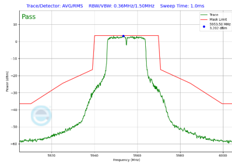
Plot 7-421 In-Band Emission Plot CDD Diversity Antenna WF7b (20MHz BW 802.11a (UNII Band 5) - Ch.1)
