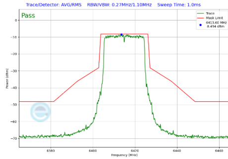
Plot 7-349 In-Band Emission Plot Antenna WF7b (20MHz BW 802.11be(SU) (UNII Band 5) - Ch.93)
