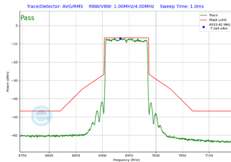
Plot 7-403 In-Band Emission Plot CDD Primary Antenna WF7a (80MHz BW 802.11be(SU) (UNII Band 8) - Ch.199)
