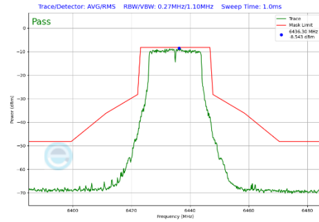
Plot 7-353 In-Band Emission Plot Antenna WF7b (20MHz BW 802.11a (UNII Band 6) - Ch.97)
