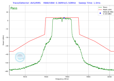
Plot 7-365 In-Band Emission Plot CDD Primary Antenna WF7a (20MHz BW 802.11a (UNII Band 5) - Ch.1)
