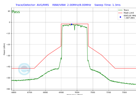
Plot 7-308 In-Band Emission Plot Antenna WF7a (160MHz BW 802.11be(SU) (UNII Band 8) - Ch.207)
