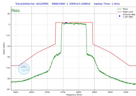
Plot 7-431 In-Band Emission Plot CDD Diversity Antenna WF7b (80MHz BW 802.11be(SU) (UNII Band 7) - Ch.167)
