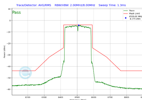
Plot 7-396 In-Band Emission Plot CDD Primary Antenna WF7a (160MHz BW 802.11be(SU) (UNII Band 6) - Ch.111)
