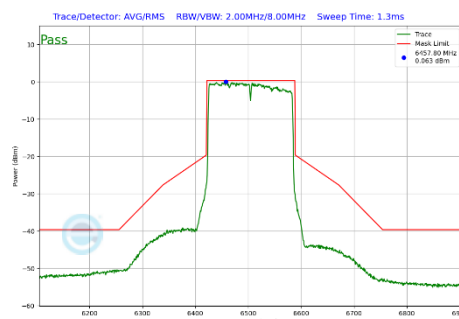
Plot 7-384 In-Band Emission Plot CDD Primary Antenna WF2a (160MHz BW 802.11be(SU) (UNII Band 6) - Ch.111)
