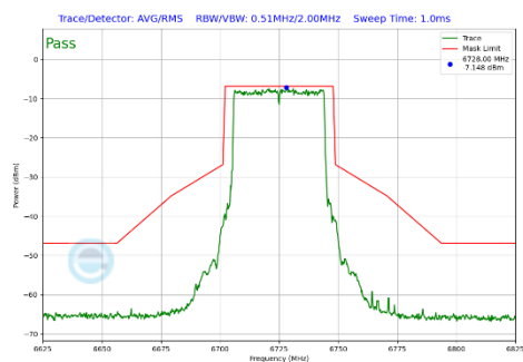
Plot 7-302 In-Band Emission Plot Antenna WF7a (40MHz BW 802.11be(SU) (UNII Band 7) - Ch.155)
