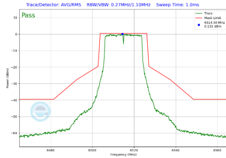
Plot 7-437 In-Band Emission Plot CDD Diversity Antenna WF2a (20MHz BW 802.11a (UNII Band 6) - Ch.113)
