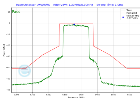
Plot 7-323 In-Band Emission Plot Antenna WF2a (80MHz BW 802.11be(SU) (UNII Band 5) - Ch.87)
