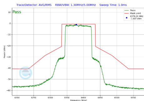
Plot 7-295 In-Band Emission Plot Antenna WF7a (80MHz BW 802.11be(SU) (UNII Band 5) - Ch.87)
