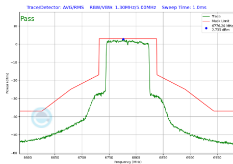
Plot 7-319 In-Band Emission Plot Antenna WF2a (80MHz BW 802.11be(SU) (UNII Band 7) - Ch.167)
