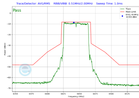
Plot 7-410 In-Band Emission Plot CDD Primary Antenna WF2a (40MHz BW 802.11be(SU) (UNII Band 6) - Ch.99)
