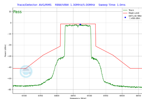
Plot 7-299 In-Band Emission Plot Antenna WF7a (80MHz BW 802.11be(SU) (UNII Band 6) - Ch.103)
