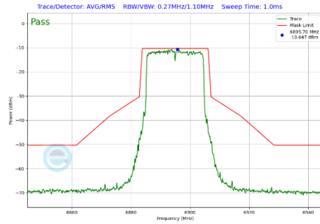
Plot 7-361 In-Band Emission Plot Antenna WF7b (20MHz BW 802.11be(SU) (UNII Band 8) - Ch.189)
