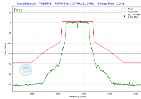
Plot 7-425 In-Band Emission Plot CDD Diversity Antenna WF7b (20MHz BW 802.11a (UNII Band 6) - Ch.113)
