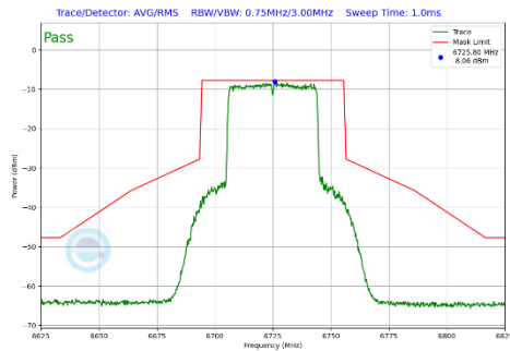
Plot 7-398 In-Band Emission Plot CDD Primary Antenna WF7a (40MHz BW 802.11be(SU) (UNII Band 7) - Ch.155)
