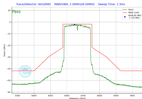
Plot 7-360 In-Band Emission Plot Antenna WF7b (160MHz BW 802.11be(SU) (UNII Band 7) - Ch.143)
