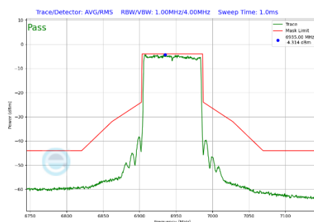
Plot 7-307 In-Band Emission Plot Antenna WF7a (80MHz BW 802.11be(SU) (UNII Band 8) - Ch.199)
