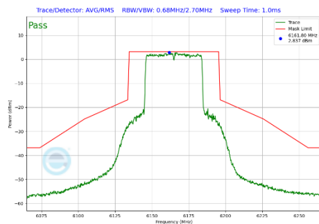
Plot 7-338 In-Band Emission Plot Antenna WF7b (40MHz BW 802.11be(SU) (UNII Band 5) - Ch.43)
