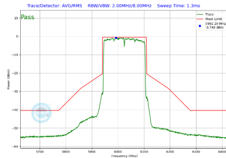
Plot 7-436 In-Band Emission Plot CDD Diversity Antenna WF2a (160MHz BW 802.11be(SU) (UNII Band 5) - Ch.15)
