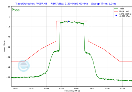
Plot 7-407 In-Band Emission Plot CDD Primary Antenna WF2a (80MHz BW 802.11be(SU) (UNII Band 5) - Ch.87)
