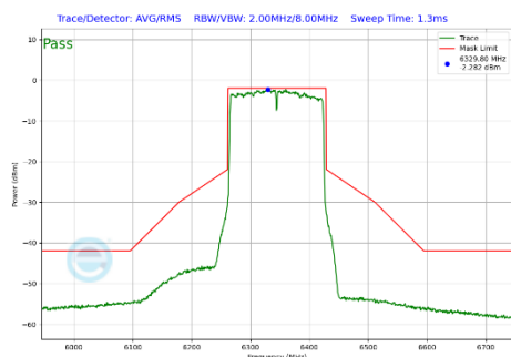
Plot 7-392 In-Band Emission Plot CDD Primary Antenna WF7a (160MHz BW 802.11be(SU) (UNII Band 5) - Ch.79)
