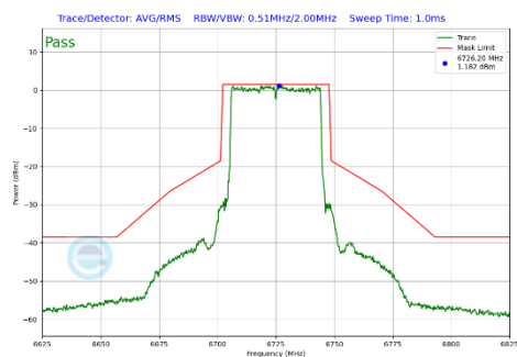
Plot 7-318 In-Band Emission Plot Antenna WF2a (40MHz BW 802.11be(SU) (UNII Band 7) - Ch.155)
