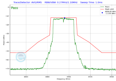
Plot 7-401 In-Band Emission Plot CDD Primary Antenna WF7a (20MHz BW 802.11be(SU) (UNII Band 8) - Ch.189)
