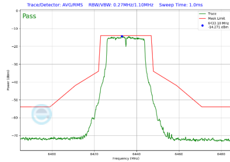
Plot 7-409 In-Band Emission Plot CDD Primary Antenna WF2a (20MHz BW 802.11a (UNII Band 6) - Ch.97)
