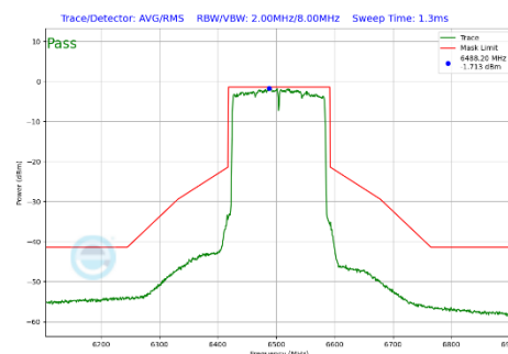
Plot 7-300 In-Band Emission Plot Antenna WF7a (160MHz BW 802.11be(SU) (UNII Band 6) - Ch.111)
