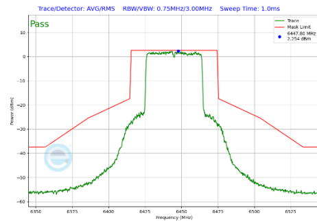
Plot 7-426 In-Band Emission Plot CDD Diversity Antenna WF7b (40MHz BW 802.11be(SU) (UNII Band 6) - Ch.99)
