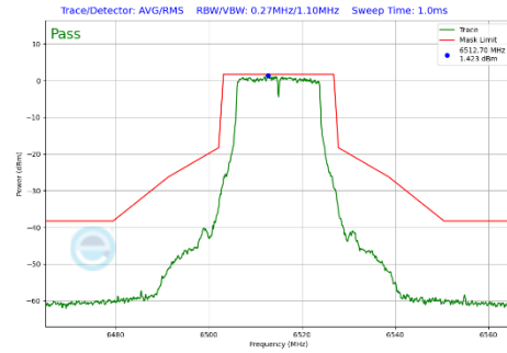
Plot 7-341 In-Band Emission Plot Antenna WF7b (20MHz BW 802.11a (UNII Band 6) - Ch.113)
