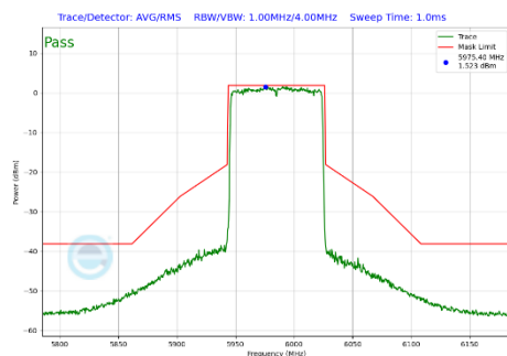
Plot 7-311 In-Band Emission Plot Antenna WF2a (80MHz BW 802.11be(SU) (UNII Band 5) - Ch.7)
