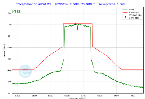
Plot 7-376 In-Band Emission Plot CDD Primary Antenna WF7a (160MHz BW 802.11be(SU) (UNII Band 7) - Ch.143)
