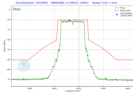
Plot 7-405 In-Band Emission Plot CDD Primary Antenna WF2a (20MHz BW 802.11be(SU) (UNII Band 5) - Ch.93)
