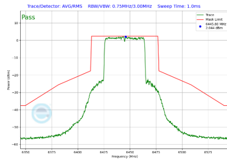
Plot 7-370 In-Band Emission Plot CDD Primary Antenna WF7a (40MHz BW 802.11be(SU) (UNII Band 6) - Ch.99)
