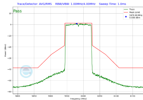
Plot 7-379 In-Band Emission Plot CDD Primary Antenna WF2a (80MHz BW 802.11be(SU) (UNII Band 5) - Ch.7)
