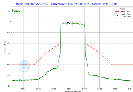
Plot 7-380 In-Band Emission Plot CDD Primary Antenna WF2a (160MHz BW 802.11be(SU) (UNII Band 5) - Ch.15)
