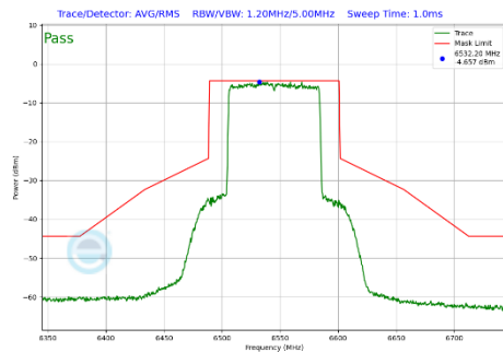
Plot 7-359 In-Band Emission Plot Antenna WF7b (80MHz BW 802.11be(SU) (UNII Band 7) - Ch.119)
