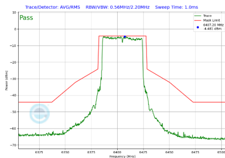
Plot 7-322 In-Band Emission Plot Antenna WF2a (40MHz BW 802.11be(SU) (UNII Band 5) - Ch.91)
