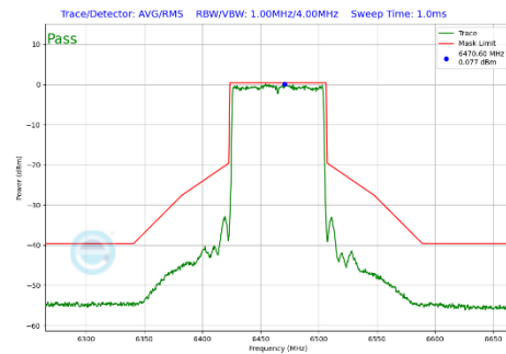
Plot 7-371 In-Band Emission Plot CDD Primary Antenna WF7a (80MHz BW 802.11be(SU) (UNII Band 6) - Ch.103)
