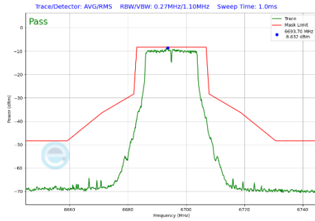
Plot 7-329 In-Band Emission Plot Antenna WF2a (20MHz BW 802.11a (UNII Band 7) - Ch.149)
