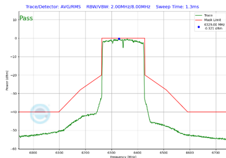
Plot 7-352 In-Band Emission Plot Antenna WF7b (160MHz BW 802.11be(SU) (UNII Band 5) - Ch.79)
