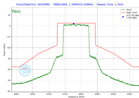
Plot 7-347 In-Band Emission Plot Antenna WF7b (80MHz BW 802.11be(SU) (UNII Band 7) - Ch.167)
