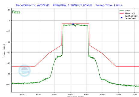
Plot 7-303 In-Band Emission Plot Antenna WF7a (80MHz BW 802.11be(SU) (UNII Band 7) - Ch.183)
