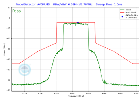
Plot 7-350 In-Band Emission Plot Antenna WF7b (40MHz BW 802.11be(SU) (UNII Band 5) - Ch.91)
