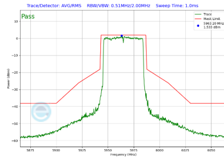
Plot 7-434 In-Band Emission Plot CDD Diversity Antenna WF2a (40MHz BW 802.11be(SU) (UNII Band 5) - Ch.3)
