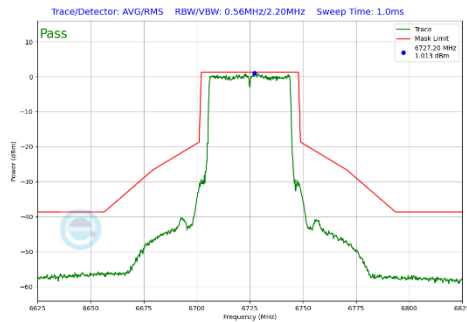
Plot 7-430 In-Band Emission Plot CDD Diversity Antenna WF7b (40MHz BW 802.11be(SU) (UNII Band 7) - Ch.155)
