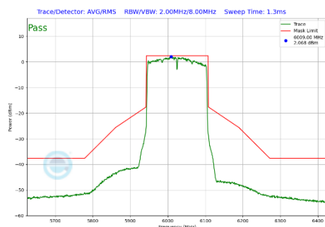
Plot 7-312 In-Band Emission Plot Antenna WF2a (160MHz BW 802.11be(SU) (UNII Band 5) - Ch.15)
