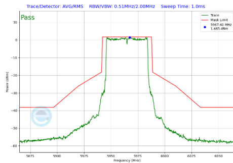
Plot 7-422 In-Band Emission Plot CDD Diversity Antenna WF7b (40MHz BW 802.11be(SU) (UNII Band 5) - Ch.3)
