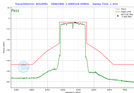
Plot 7-400 In-Band Emission Plot CDD Primary Antenna WF7a (160MHz BW 802.11be(SU) (UNII Band 7) - Ch.143)
