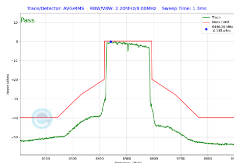
Plot 7-328 In-Band Emission Plot Antenna WF2a (160MHz BW 802.11be(SU) (UNII Band 6) - Ch.111)
