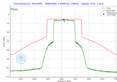
Plot 7-334 In-Band Emission Plot Antenna WF2a (40MHz BW 802.11be(SU) (UNII Band 8) - Ch.211)
