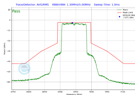
Plot 7-335 In-Band Emission Plot Antenna WF2a (80MHz BW 802.11be(SU) (UNII Band 8) - Ch.199)
