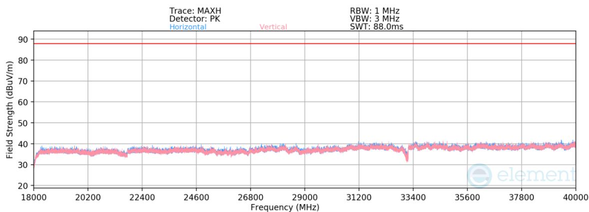
Plot 7-328. Radiated Spurious Emissions 18-40GHz SDM Primary (802.11be – Ch. 61)
