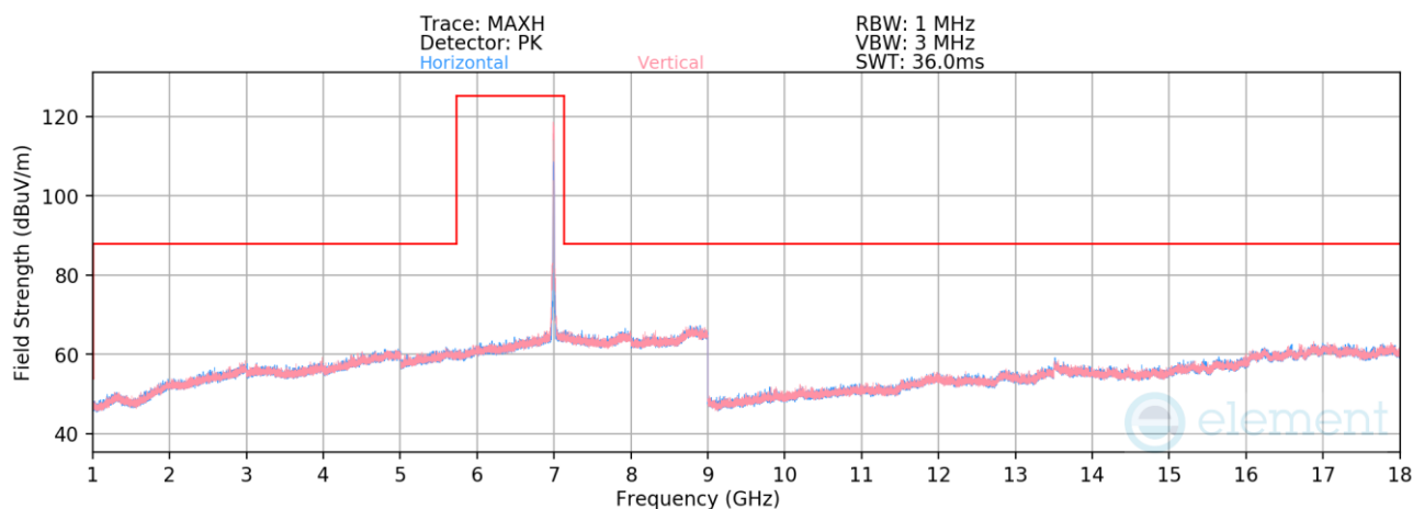
Plot 7-355. Radiated Spurious Emissions 1-18GHz SDM Diversity (802.11be – Ch. 209)
