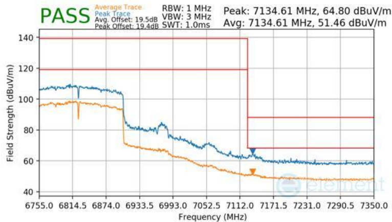
Plot 7-371 Antenna WF7a Radiated Upper Band Edge (Peak & Average – UNII Band 7)
