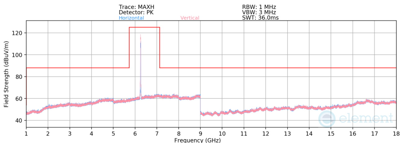
Plot 7-327. Radiated Spurious Emissions 1-18GHz SDM Primary (802.11be – Ch. 61)
