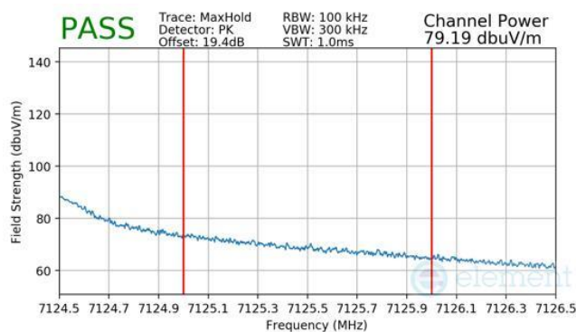
Plot 7-364 Antenna WF7a Radiated Integrated Band Edge (Peak – UNII Band 8)
