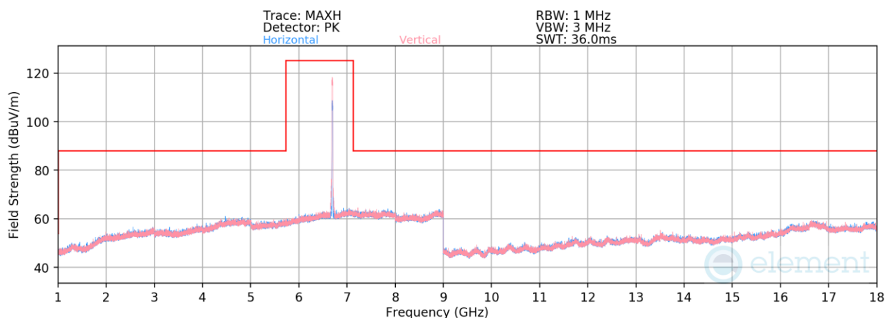
Plot 7-335. Radiated Spurious Emissions 1-18GHz SDM Primary (802.11be – Ch. 149)
