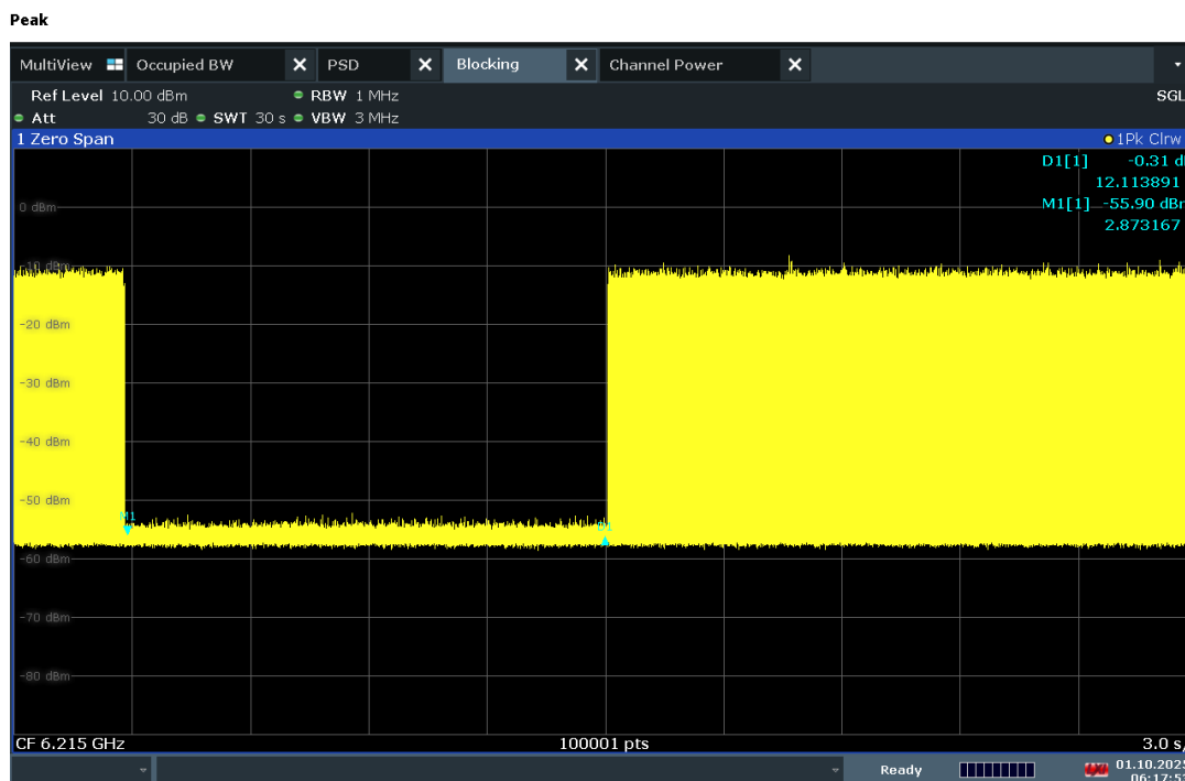
Plot 7-305. Contention Based Protocol Timing Plot – UNII 5 – 20MHz Channel 53
