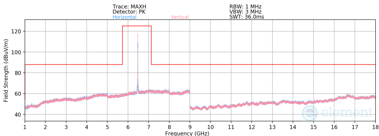
Plot 7-331. Radiated Spurious Emissions 1-18GHz SDM Primary (802.11be – Ch. 105)
