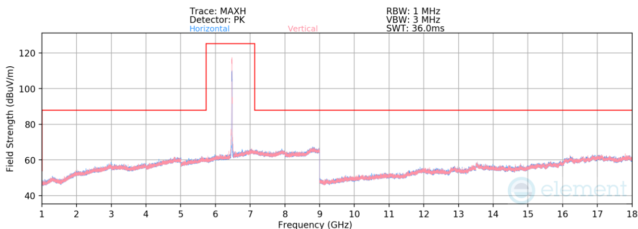
Plot 7-347. Radiated Spurious Emissions 1-18GHz SDM Diversity (802.11be – Ch. 105)
