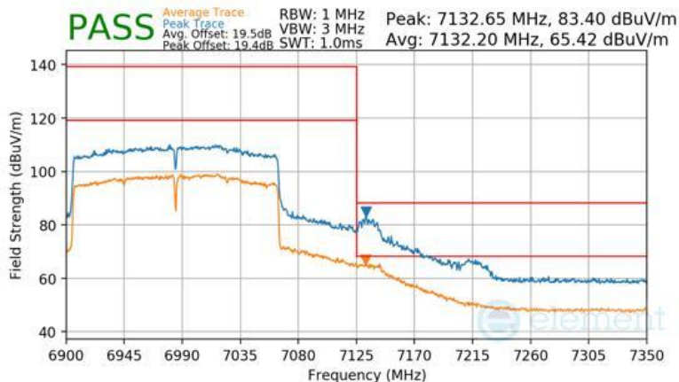
Plot 7-372 Antenna WF7a Radiated Upper Band Edge (Peak & Average – UNII Band 8)
