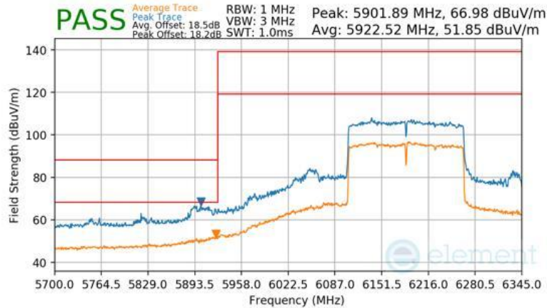
Plot 7-370 Antenna WF7a Radiated Lower Band Edge (Peak & Average – UNII Band 5)
