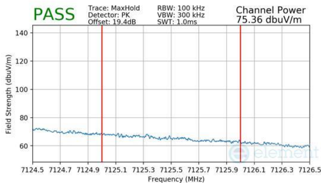
Plot 7-360 Antenna WF7a Radiated Integrated Band Edge (Peak – UNII Band 8)
