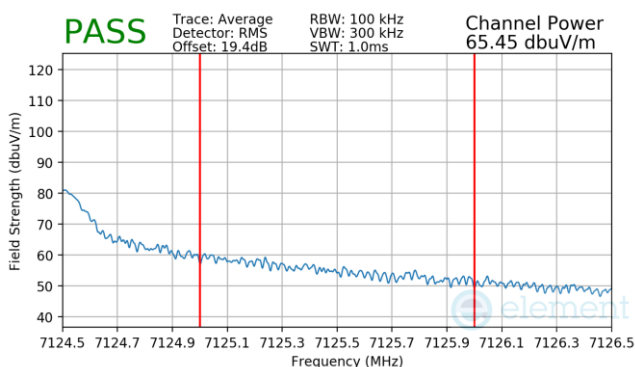
Plot 7-365 Antenna WF7a Radiated Integrated Band Edge (Average – UNII Band 8)
