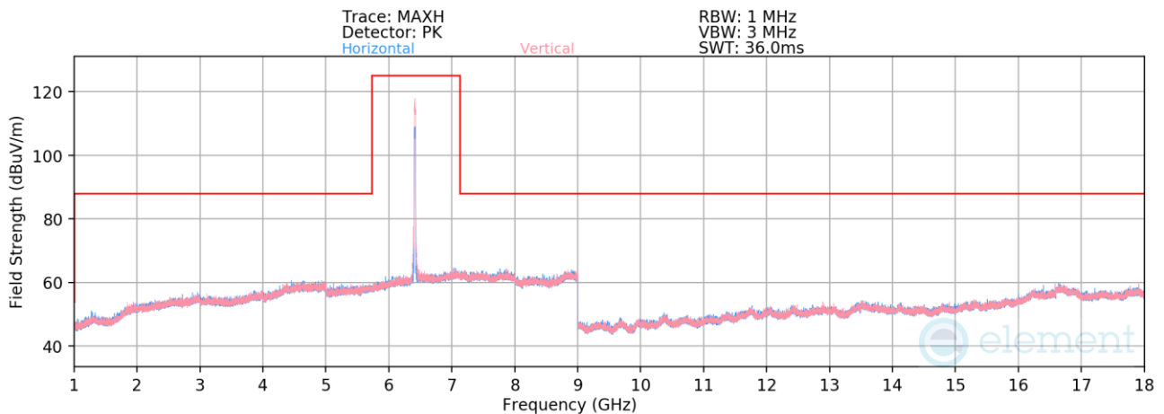
Plot 7-329. Radiated Spurious Emissions 1-18GHz SDM (802.11be – Ch. 93)
