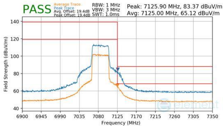
Plot 7-367 Antenna WF7a Radiated Upper Band Edge (Peak & Average – UNII Band 8)
