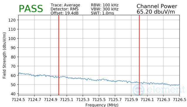
Plot 7-361 Antenna WF7a Radiated Integrated Band Edge (Average – UNII Band 8)
