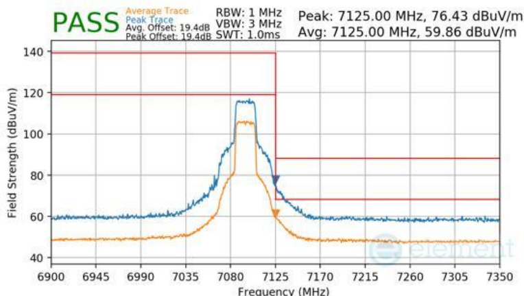
Plot 7-363 Antenna WF7a Radiated Upper Band Edge (Peak & Average – UNII Band 8)
