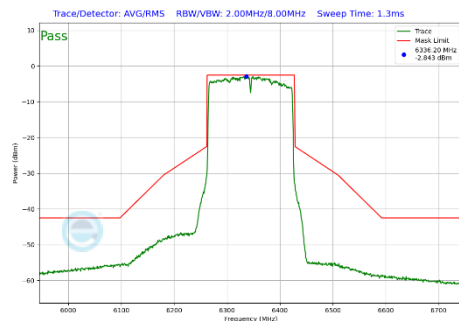
Plot 7-464 In-Band Emission Plot CDD Diversity Antenna WF2a (160MHz BW 802.11be(SU) (UNII Band 5) - Ch.79)
