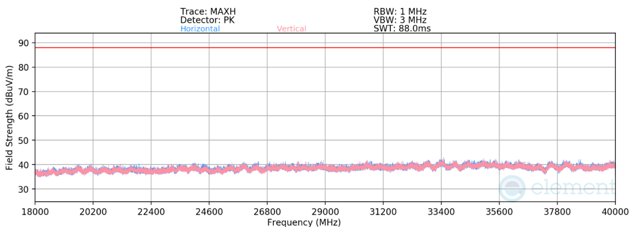
Plot 7-542. Radiated Spurious Emissions 18-40GHz SDM Primary (802.11be – Ch. 209)
