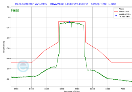
Plot 7-456 In-Band Emission Plot CDD Diversity Antenna WF7b (160MHz BW 802.11be(SU) (UNII Band 7) - Ch.143)
