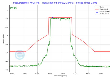
Plot 7-450 In-Band Emission Plot CDD Diversity Antenna WF7b (40MHz BW 802.11be(SU) (UNII Band 6) - Ch.99)
