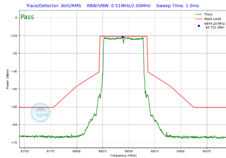
Plot 7-470 In-Band Emission Plot CDD Diversity Antenna WF2a (40MHz BW 802.11be(SU) (UNII Band 7) - Ch.179)
