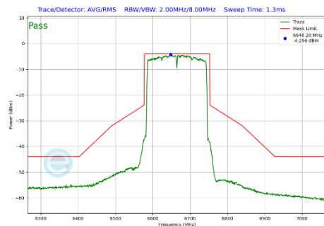
Plot 7-472 In-Band Emission Plot CDD Diversity Antenna WF2a (160MHz BW 802.11be(SU) (UNII Band 7) - Ch.143)
