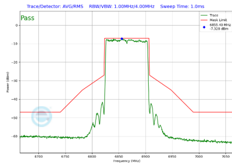
Plot 7-471 In-Band Emission Plot CDD Diversity Antenna WF2a (80MHz BW 802.11be(SU) (UNII Band 7) - Ch.183)
