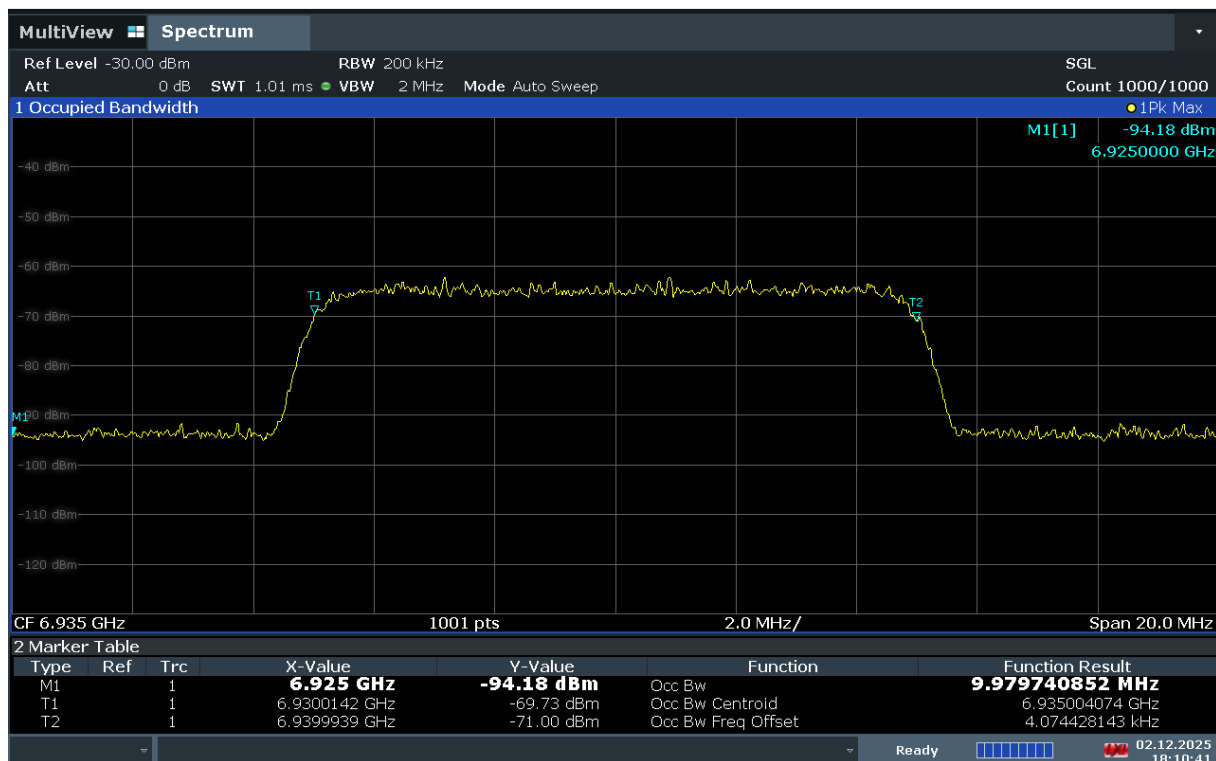
Plot 7-489. AWGN Signal – UNII 8 – 20MHz
