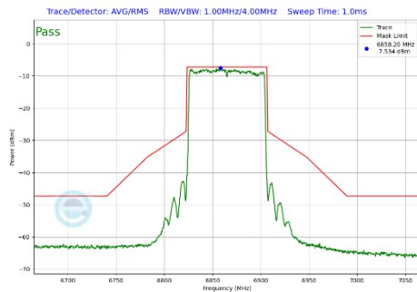
Plot 7-455 In-Band Emission Plot CDD Diversity Antenna WF7b (80MHz BW 802.11be(SU) (UNII Band 7) - Ch.183)
