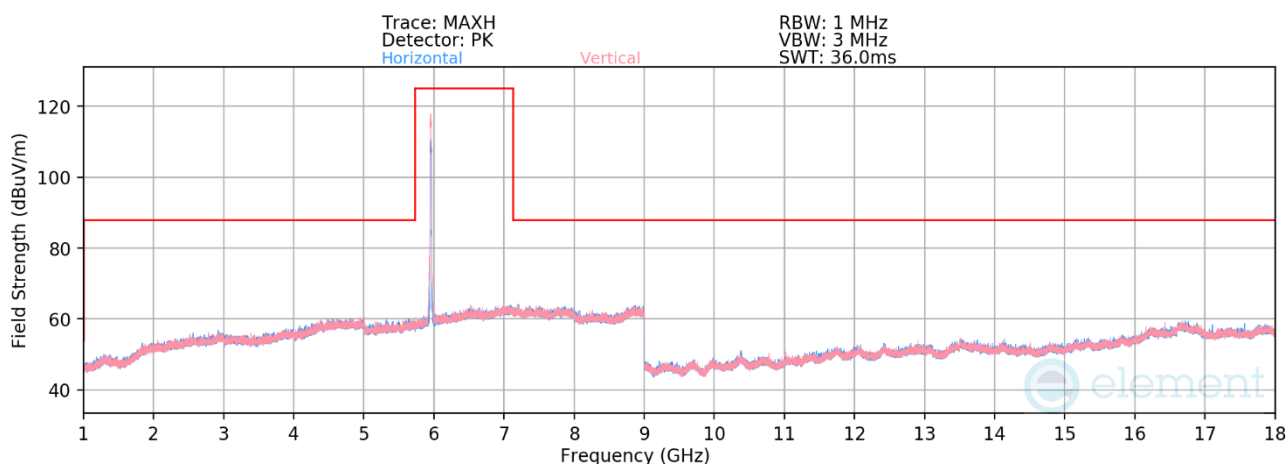
Plot 7-528. Radiated Spurious Emissions 1-18GHz CDD Primary (802.11be – Ch. 1)
