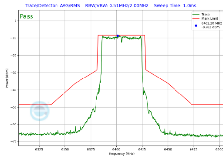
Plot 7-446 In-Band Emission Plot CDD Diversity Antenna WF7b (40MHz BW 802.11be(SU) (UNII Band 5) - Ch.91)
