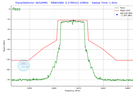
Plot 7-445 In-Band Emission Plot CDD Diversity Antenna WF7b (20MHz BW 802.11be(SU) (UNII Band 5) - Ch.93)
