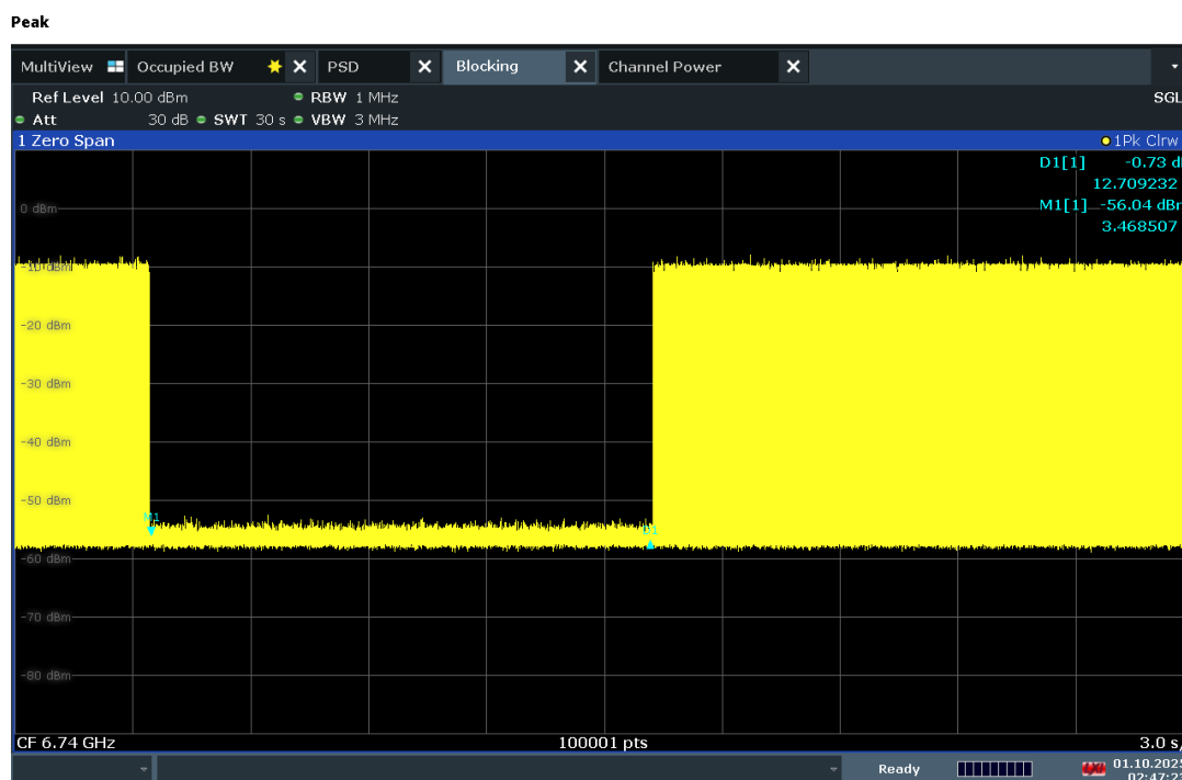
Plot 7-520. Contention Based Protocol Timing Plot – UNII 7 – 160MHz Channel 143 – High
