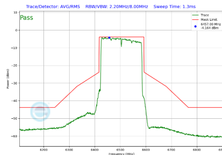
Plot 7-468 In-Band Emission Plot CDD Diversity Antenna WF2a (160MHz BW 802.11be(SU) (UNII Band 6) - Ch.111)
