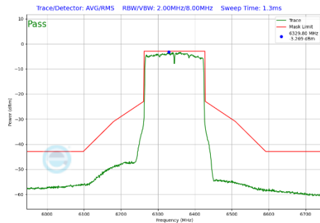
Plot 7-448 In-Band Emission Plot CDD Diversity Antenna WF7b (160MHz BW 802.11be(SU) (UNII Band 5) - Ch.79)
