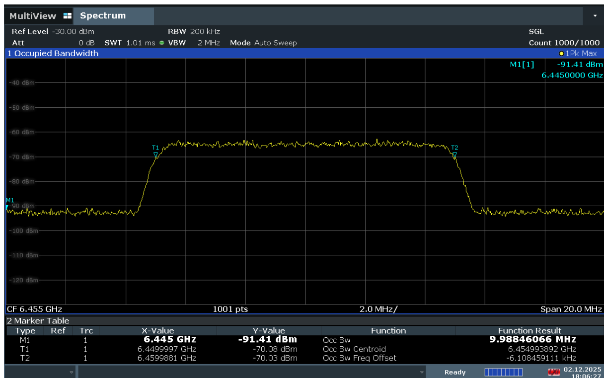
Plot 7-481. AWGN Signal – UNII 6 – 20MHz
