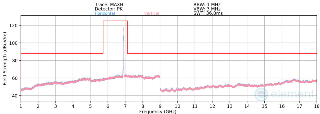
Plot 7-540. Radiated Spurious Emissions 1-18GHz SDM Primary (802.11be – Ch. 189)
