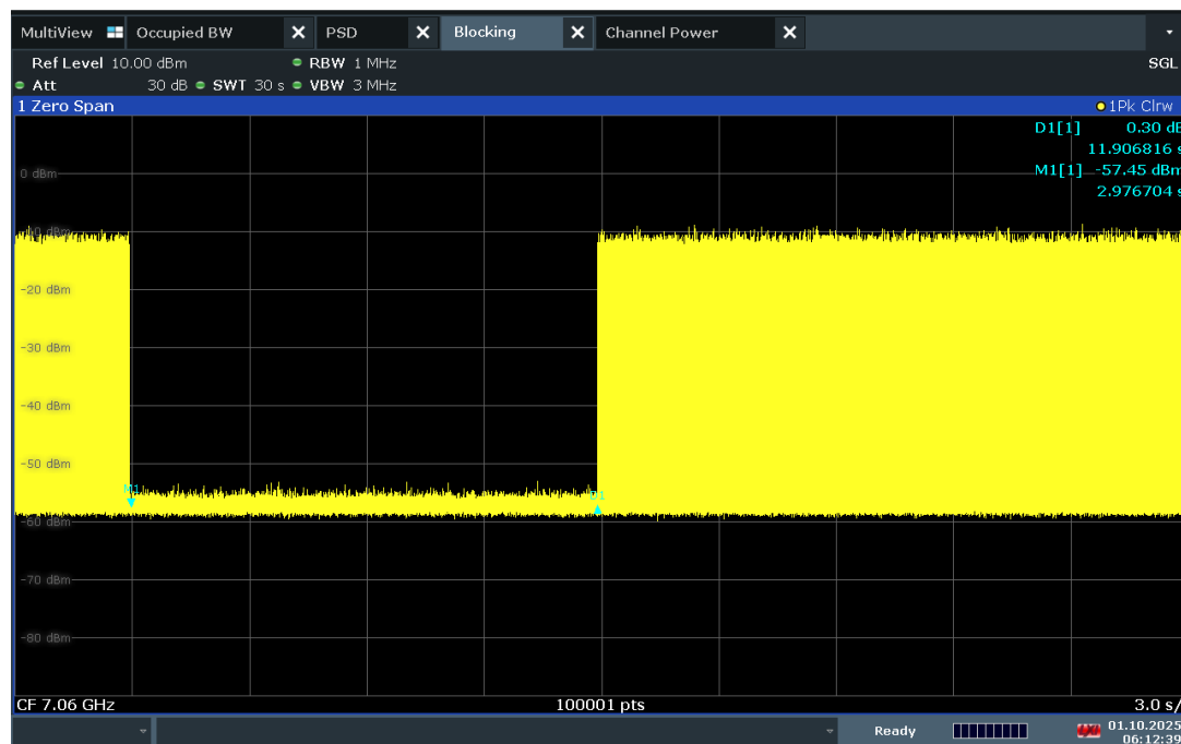
Plot 7-524. Contention Based Protocol Timing Plot – UNII 8 – 160MHz Channel 207 – High
