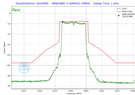
Plot 7-462 In-Band Emission Plot CDD Diversity Antenna WF2a (40MHz BW 802.11be(SU) (UNII Band 5) - Ch.91)
