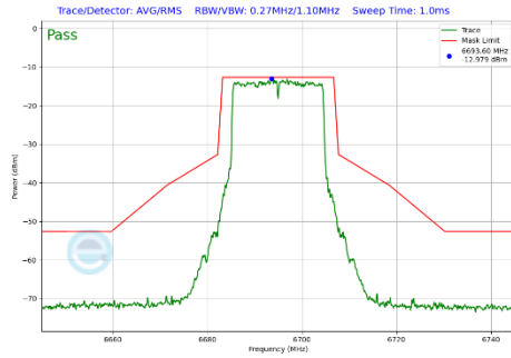
Plot 7-453 In-Band Emission Plot CDD Diversity Antenna WF7b (20MHz BW 802.11be(SU) (UNII Band 7) - Ch.149)
