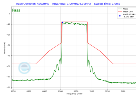
Plot 7-459 In-Band Emission Plot CDD Diversity Antenna WF7b (80MHz BW 802.11be(SU) (UNII Band 8) - Ch.199)
