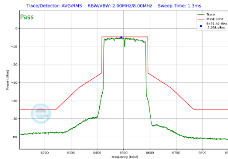
Plot 7-452 In-Band Emission Plot CDD Diversity Antenna WF7b (160MHz BW 802.11be(SU) (UNII Band 6) - Ch.111)
