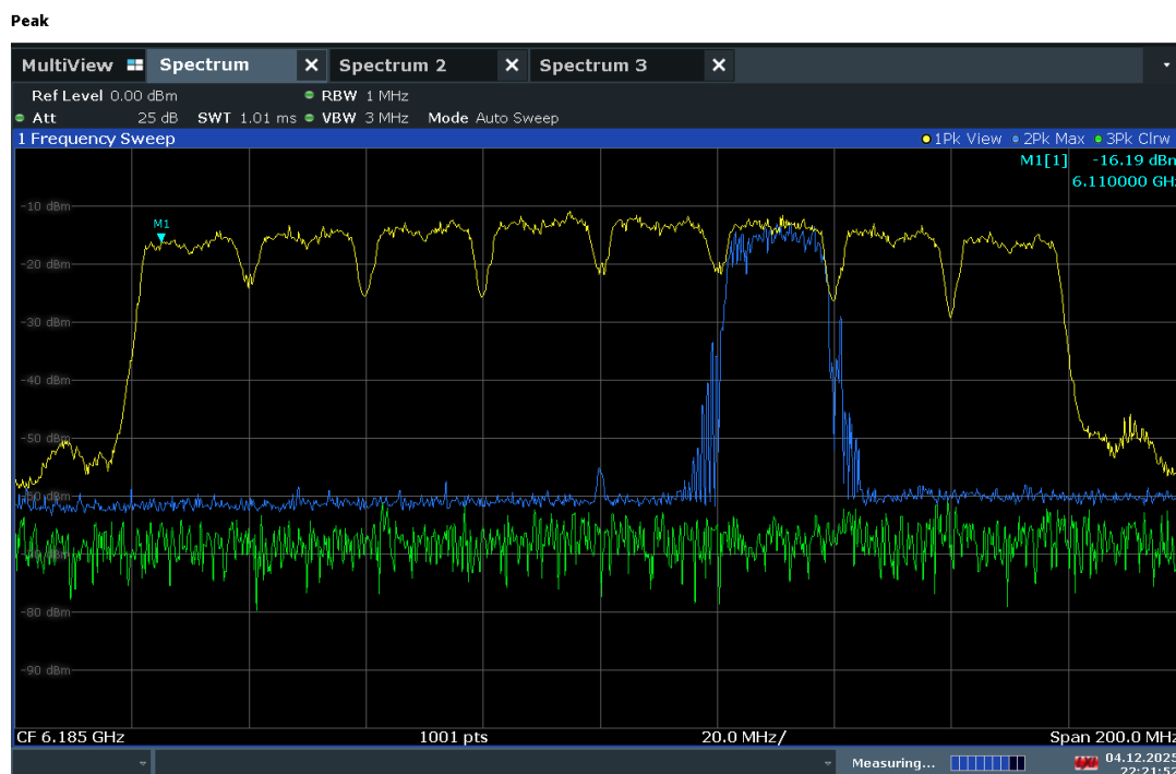
Plot 7-525. 160MHz Bandwidth, AWGN Signal Injected – 6110Mhz
