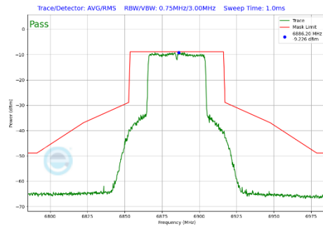
Plot 7-458 In-Band Emission Plot CDD Diversity Antenna WF7b (40MHz BW 802.11be(SU) (UNII Band 8) - Ch.187)
