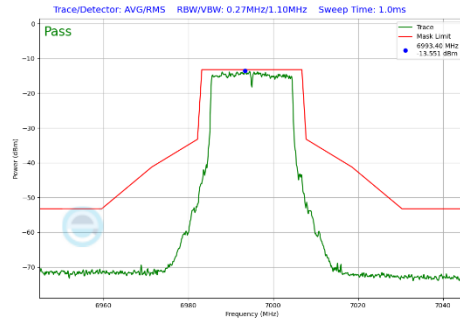
Plot 7-457 In-Band Emission Plot CDD Diversity Antenna WF7b (20MHz BW 802.11be(SU) (UNII Band 8) - Ch.209)
