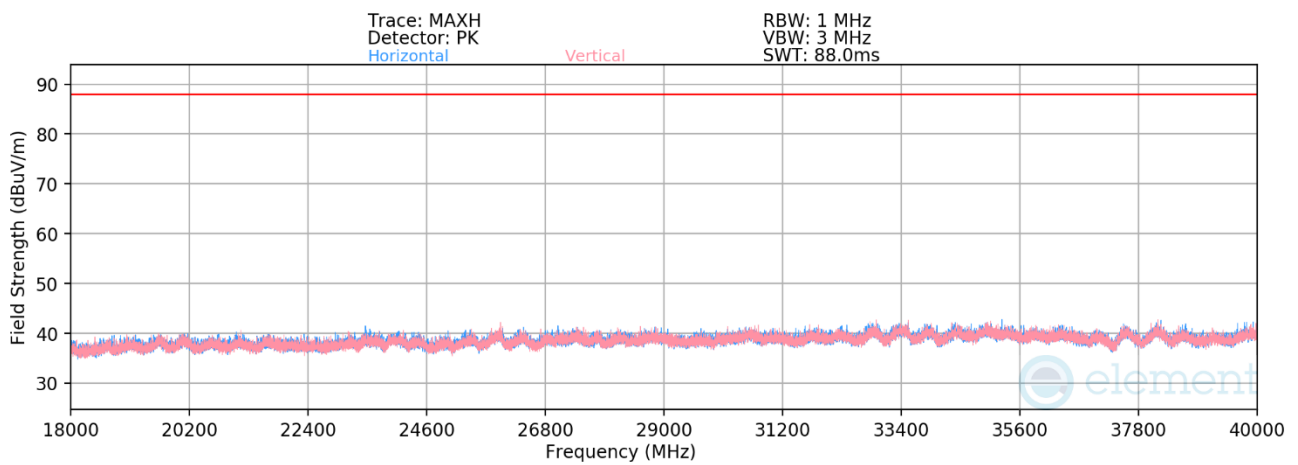
Plot 7-534. Radiated Spurious Emissions 18-40GHz CDD Primary (802.11be – Ch. 105)
