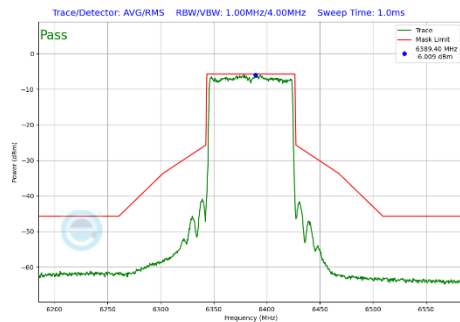
Plot 7-447 In-Band Emission Plot CDD Diversity Antenna WF7b (80MHz BW 802.11be(SU) (UNII Band 5) - Ch.87)
