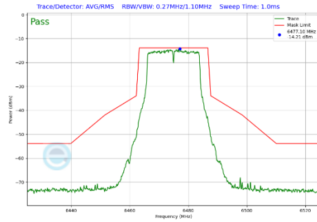
Plot 7-449 In-Band Emission Plot CDD Diversity Antenna WF7b (20MHz BW 802.11a (UNII Band 6) - Ch.105)
