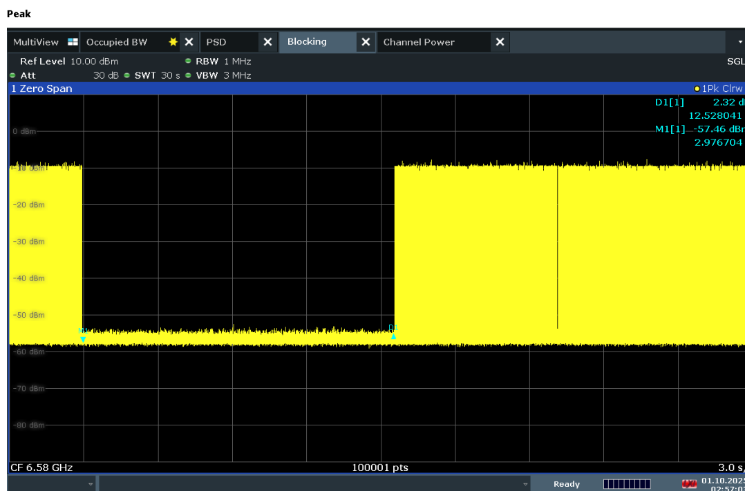
Plot 7-516. Contention Based Protocol Timing Plot – UNII 6 – 160MHz Channel 111 – High
