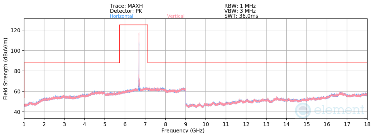
Plot 7-537. Radiated Spurious Emissions 1-18GHz CDD Primary (802.11be – Ch. 149)
