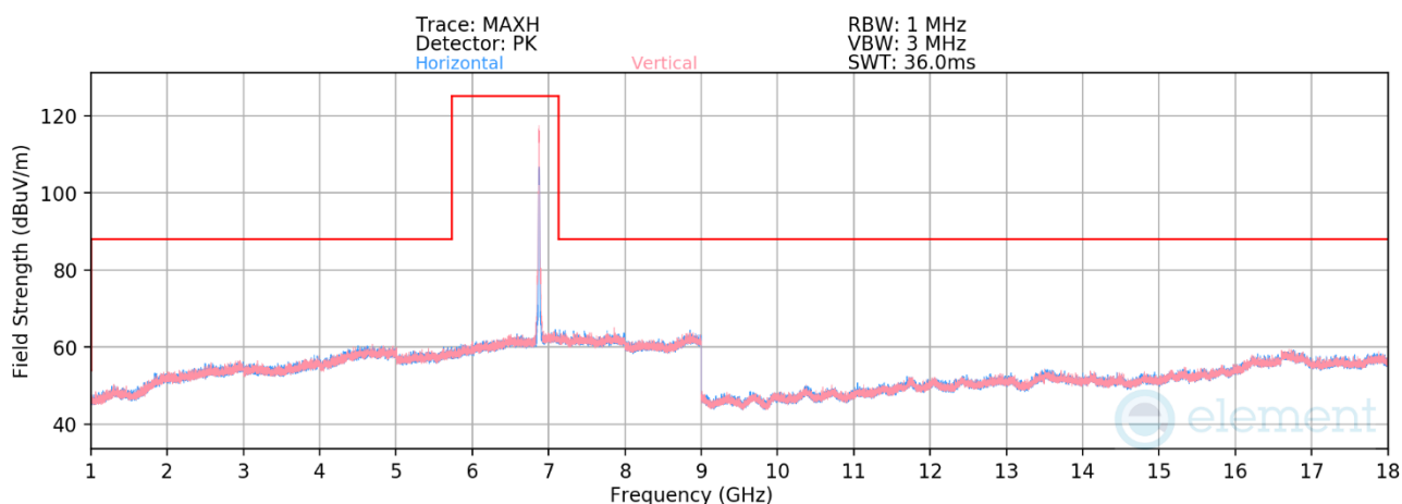
Plot 7-539. Radiated Spurious Emissions 1-18GHz CDD Primary (802.11be – Ch. 185)
