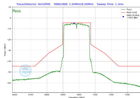
Plot 7-476 In-Band Emission Plot CDD Diversity Antenna WF2a (160MHz BW 802.11be(SU) (UNII Band 8) - Ch.207)
