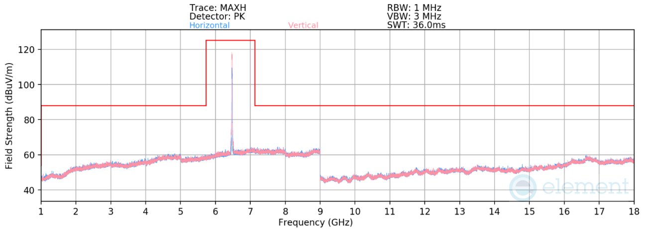
Plot 7-533. Radiated Spurious Emissions 1-18GHz CDD Primary (802.11be – Ch. 105)
