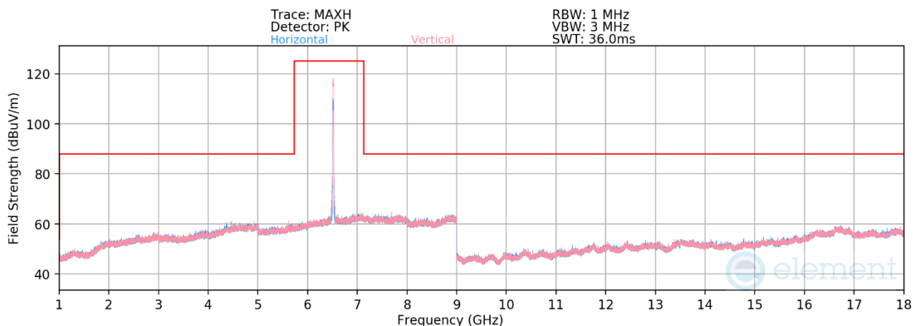
Plot 7-535. Radiated Spurious Emissions 1-18GHz CDD Primary (802.11be – Ch. 113)
