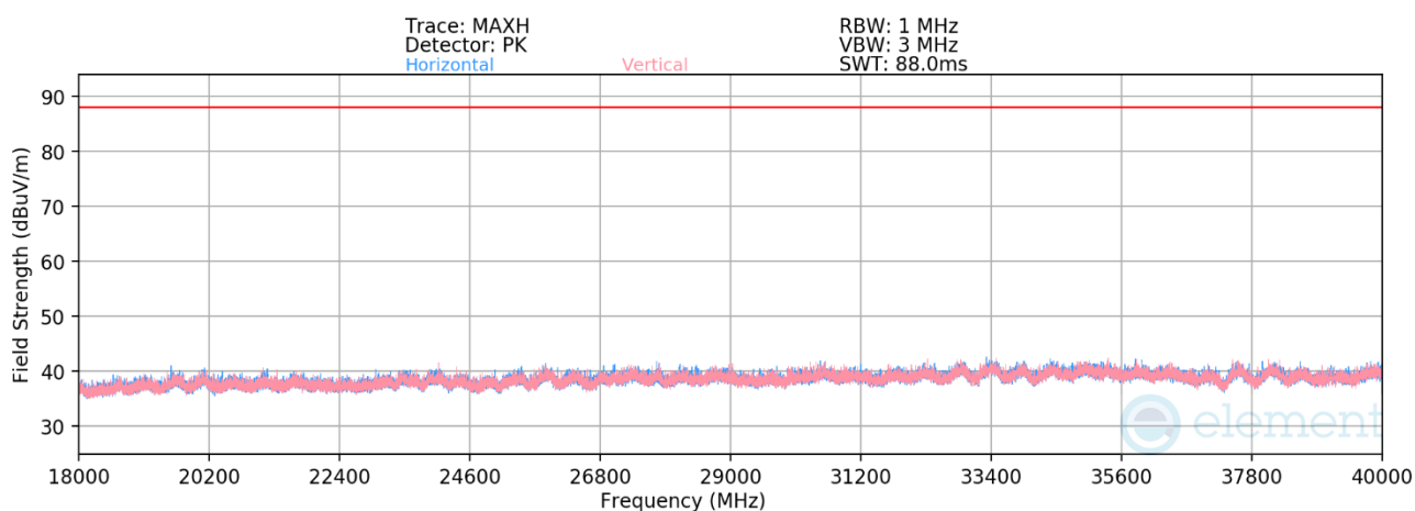
Plot 7-538. Radiated Spurious Emissions 18-40GHz CDD Primary (802.11be – Ch. 149)
