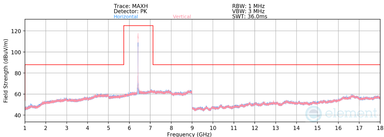
Plot 7-531. Radiated Spurious Emissions 1-18GHz CDD Primary (802.11be – Ch. 93)
