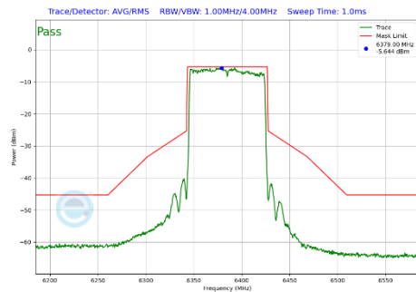
Plot 7-463 In-Band Emission Plot CDD Diversity Antenna WF2a (80MHz BW 802.11be(SU) (UNII Band 5) - Ch.87)
