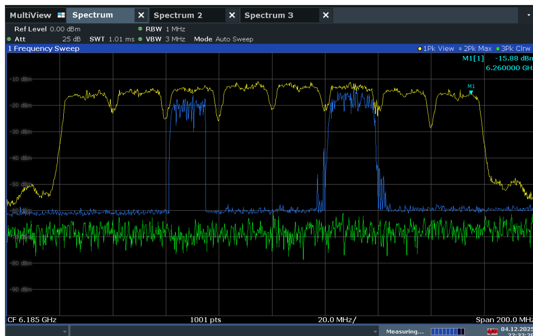
Plot 7-527. 160MHz Bandwidth, AWGN Signal Injected – 6260MHz
