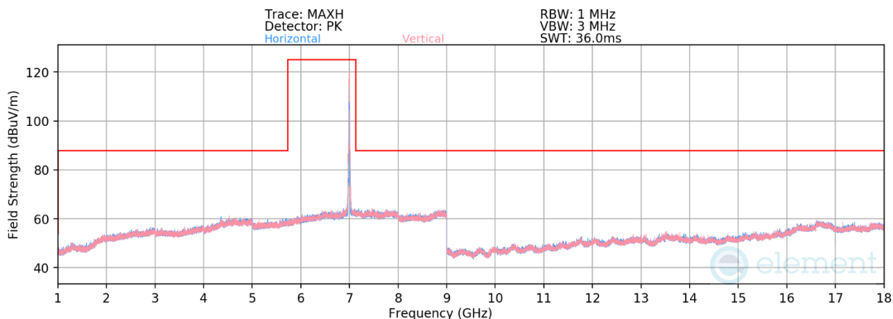
Plot 7-541. Radiated Spurious Emissions 1-18GHz SDM Primary (802.11be – Ch. 209)
