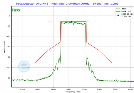
Plot 7-451 In-Band Emission Plot CDD Diversity Antenna WF7b (80MHz BW 802.11be(SU) (UNII Band 6) - Ch.103)
