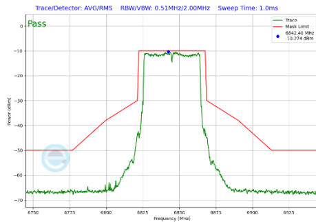
Plot 7-454 In-Band Emission Plot CDD Diversity Antenna WF7b (40MHz BW 802.11be(SU) (UNII Band 7) - Ch.179)
