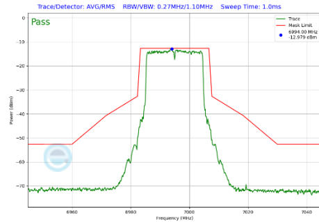
Plot 7-473 In-Band Emission Plot CDD Diversity Antenna WF2a (20MHz BW 802.11be(SU) (UNII Band 8) - Ch.209)
