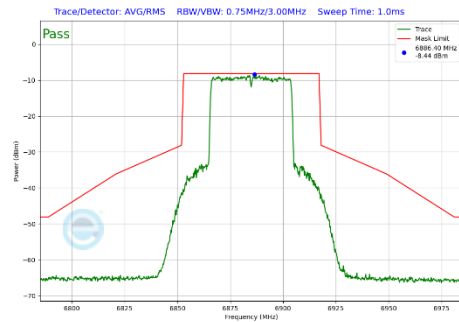
Plot 7-474 In-Band Emission Plot CDD Diversity Antenna WF2a (40MHz BW 802.11be(SU) (UNII Band 8) - Ch.187)
