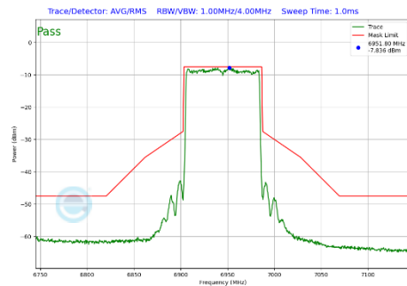
Plot 7-475 In-Band Emission Plot CDD Diversity Antenna WF2a (80MHz BW 802.11be(SU) (UNII Band 8) - Ch.199)
