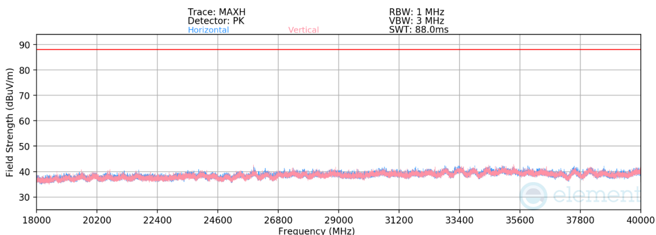
Plot 7-530. Radiated Spurious Emissions 18-40GHz CDD Primary (802.11be – Ch. 45)
