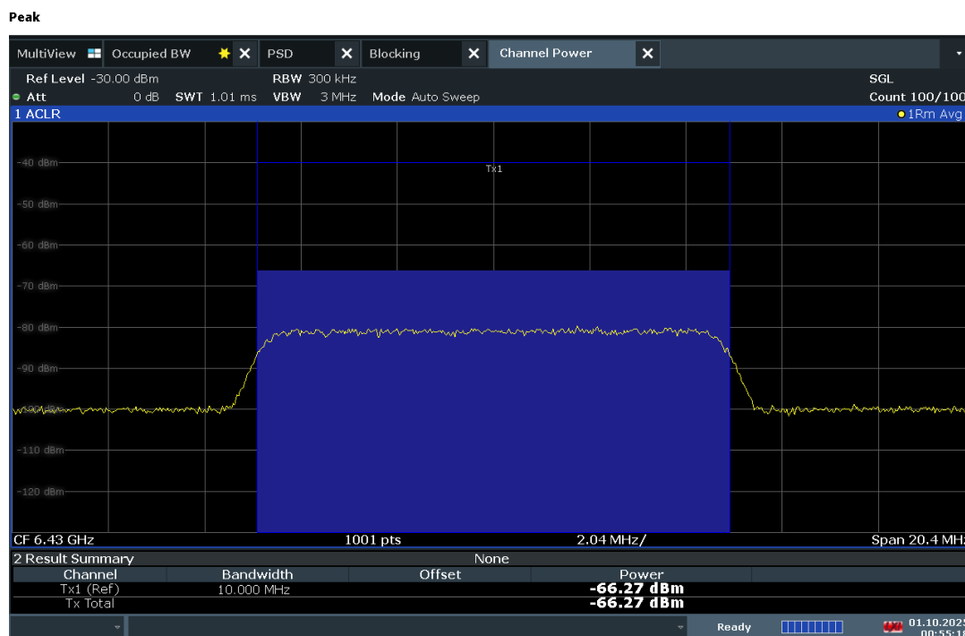
Plot 7-498. Channel Power – UNII 6 – 160MHz - Low
