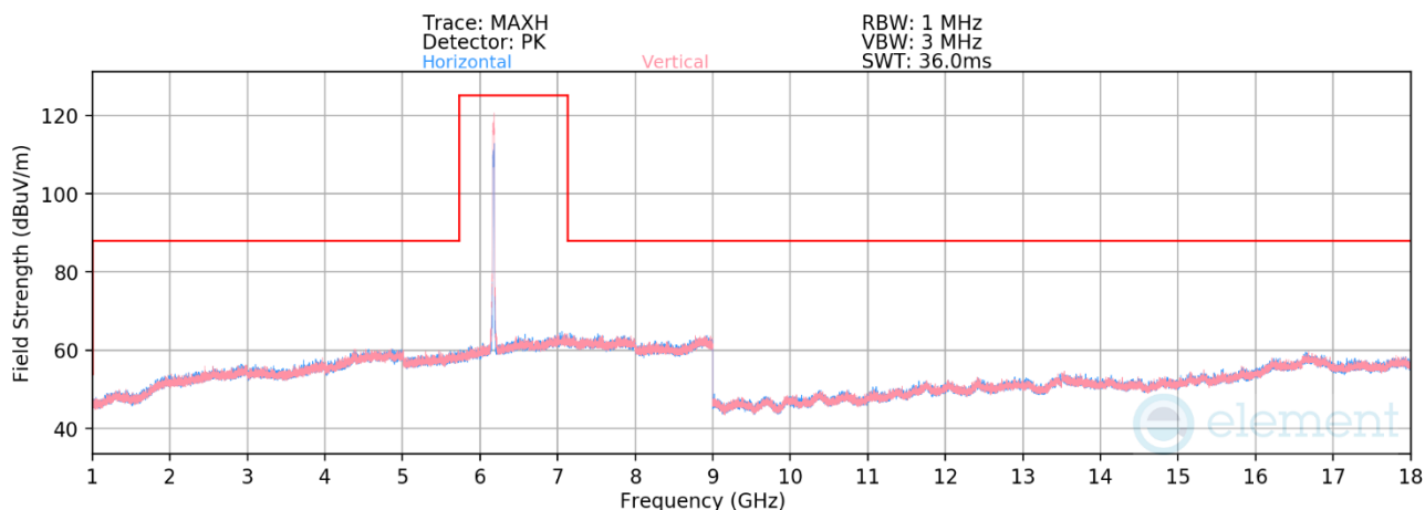
Plot 7-529. Radiated Spurious Emissions 1-18GHz CDD Primary (802.11be – Ch. 45)
