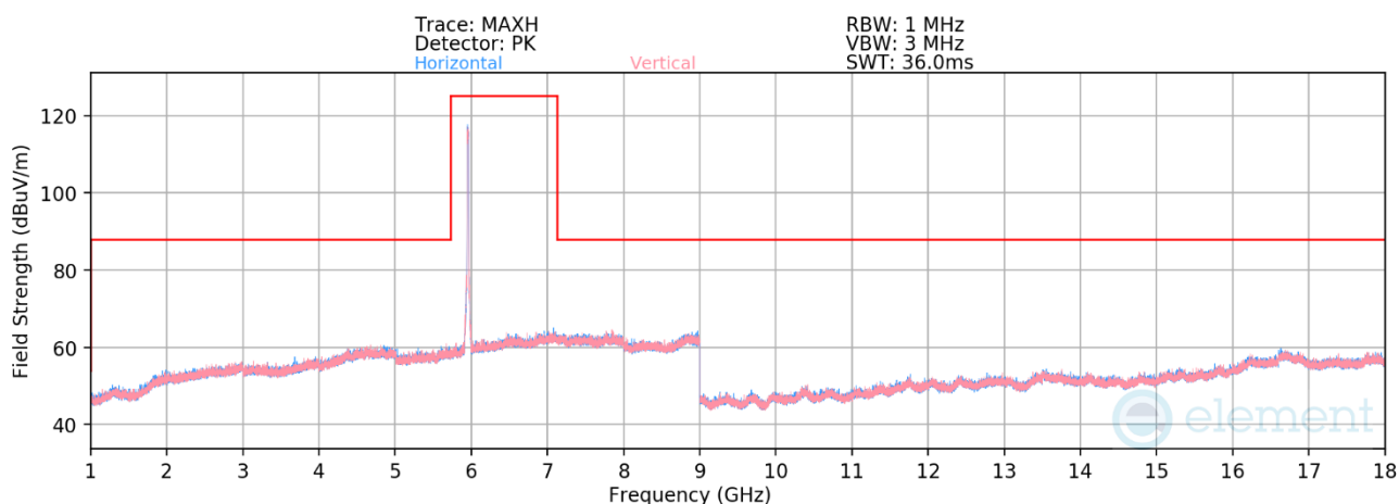
Plot 7-544. Radiated Spurious Emissions 1-18GHz CDD Diversity (802.11be – Ch. 1)
