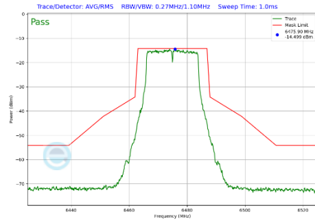
Plot 7-465 In-Band Emission Plot CDD Diversity Antenna WF2a (20MHz BW 802.11a (UNII Band 6) - Ch.105)
