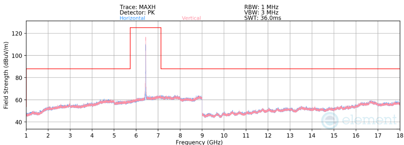
Plot 7-532. Radiated Spurious Emissions 1-18GHz CDD Primary (802.11be – Ch. 97)
