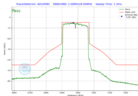
Plot 7-460 In-Band Emission Plot CDD Diversity Antenna WF7b (160MHz BW 802.11be(SU) (UNII Band 8) - Ch.207)
