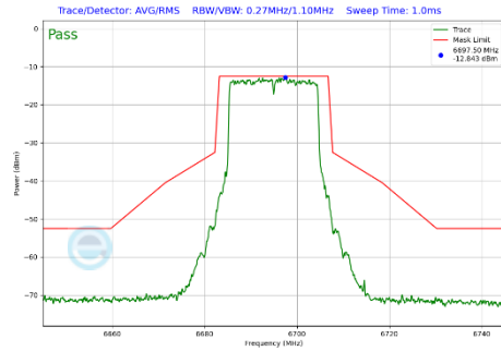
Plot 7-469 In-Band Emission Plot CDD Diversity Antenna WF2a (20MHz BW 802.11be(SU) (UNII Band 7) - Ch.149)
