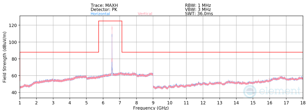
Plot 7-536. Radiated Spurious Emissions 1-18GHz CDD Primary (802.11be – Ch. 117)
