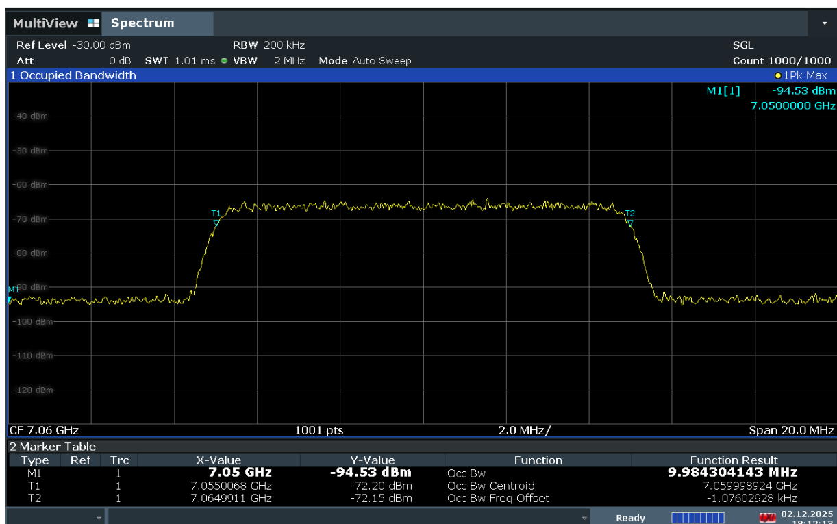
Plot 7-492. AWGN Signal – UNII 8 – 160MHz - High
