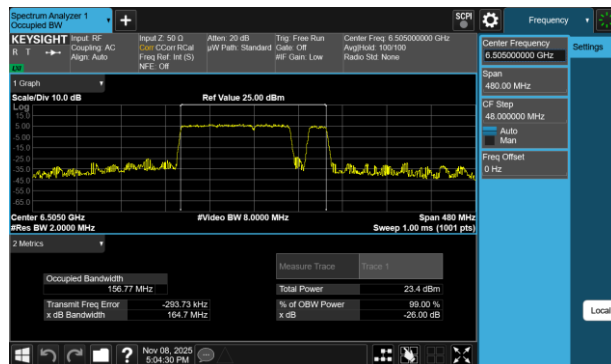
Plot 7-51 26dB BW & 99% OBW Antenna WF7a (160MHz BW 802.11be(RU) RU996+484+242 Index98 - Ch.111)
