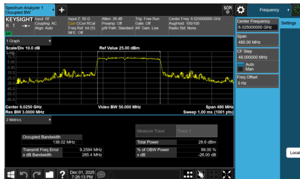
Plot 7-84 26dB BW & 99% OBW Antenna WF2a (160MHz BW 802.11be(RU) RU996+484+242 Index96 - Ch.15)
