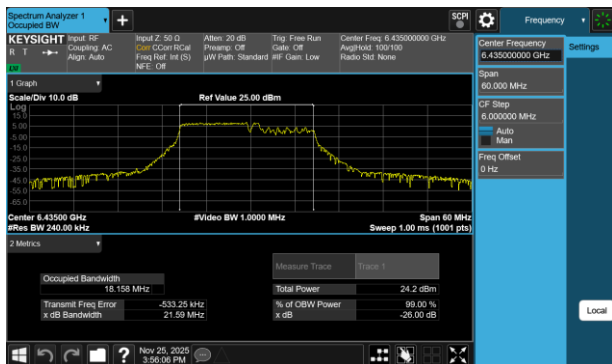
Plot 7-16 26dB BW & 99% OBW Antenna WF7a (20MHz BW 802.11be(RU) RU106+26 Index82 - Ch.97)
