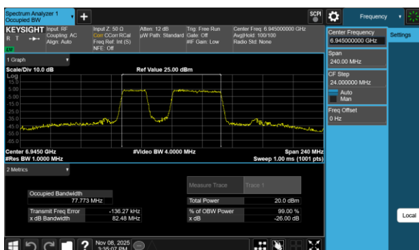
Plot 7-72 26dB BW & 99% OBW Antenna WF7a (80MHz BW 802.11be(RU) RU484+242 Index91 - Ch.199)
