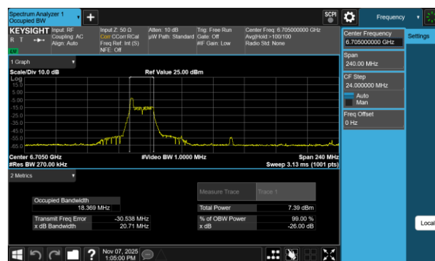
Plot 7-58 26dB BW & 99% OBW Antenna WF7a (80MHz BW 802.11be(RU) RU26 Index0 - Ch.151)
