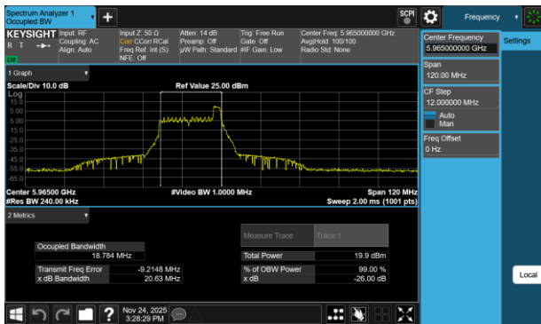
Plot 7-2 26dB BW & 99% OBW Antenna WF7a (40MHz BW 802.11be(RU) RU26 Index8 - Ch.3)
