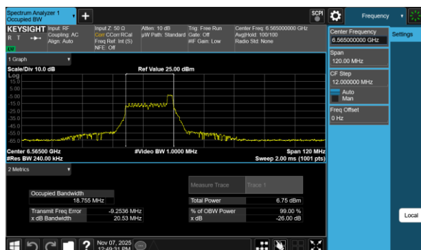
Plot 7-57 26dB BW & 99% OBW Antenna WF7a (40MHz BW 802.11be(RU) RU26 Index8 - Ch.123)
