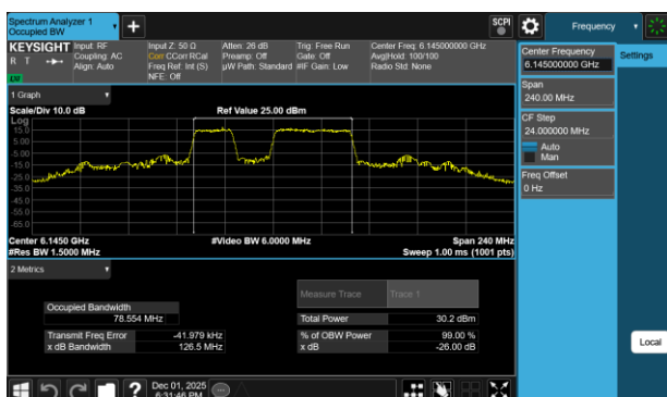
Plot 7-83 26dB BW & 99% OBW Antenna WF2a (80MHz BW 802.11be(RU) RU484+242 Index91 - Ch.39)
