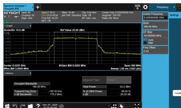
Plot 7-44 26dB BW & 99% OBW Antenna WF7a (160MHz BW 802.11be(RU) RU996X2 Index68 - Ch.15)
