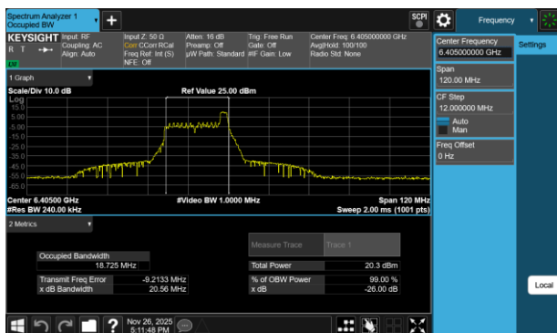
Plot 7-79 26dB BW & 99% OBW Antenna WF2a (40MHz BW 802.11be(RU) RU26 Index8 - Ch.91)
