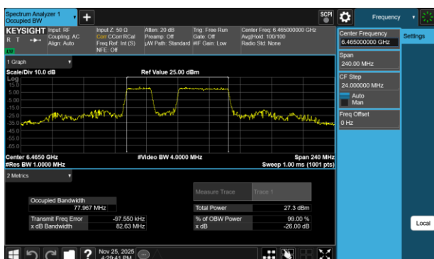
Plot 7-17 26dB BW & 99% OBW Antenna WF7a (80MHz BW 802.11be(RU) RU484+242 Index91 - Ch.103)
