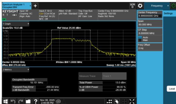
Plot 7-71 26dB BW & 99% OBW Antenna WF7a (20MHz BW 802.11be(RU) RU106+26 Index82 - Ch.209)
