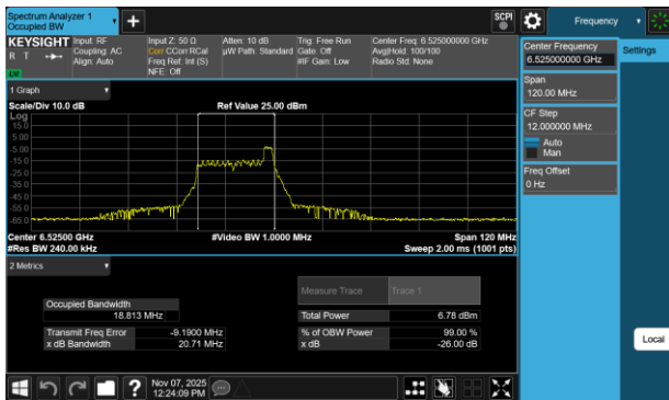
Plot 7-46 26dB BW & 99% OBW Antenna WF7a (40MHz BW 802.11be(RU) RU26 Index8 - Ch.115)
