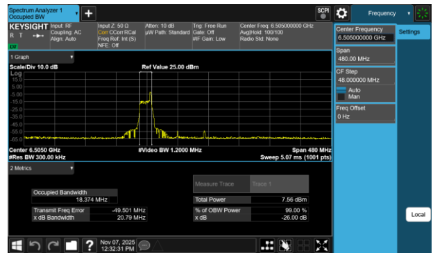
Plot 7-48 26dB BW & 99% OBW Antenna WF7a (160MHz BW 802.11be(RU) RU26 Index17 - Ch.111)
