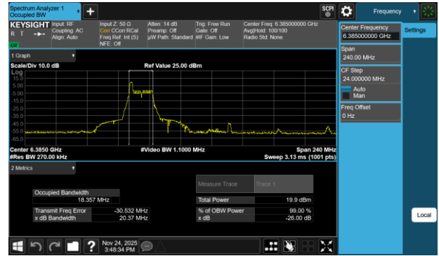
Plot 7-3 26dB BW & 99% OBW Antenna WF7a (80MHz BW 802.11be(RU) RU26 Index0 - Ch.87)
