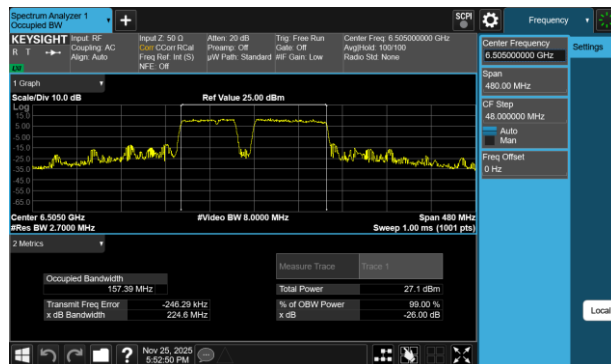
Plot 7-18 26dB BW & 99% OBW Antenna WF7a (160MHz BW 802.11be(RU) RU996+484+242 Index99 - Ch.111)
