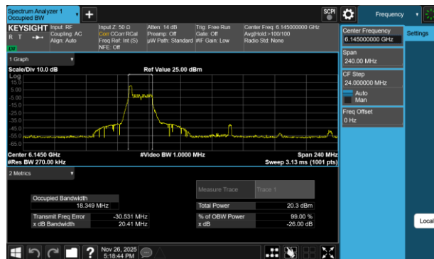
Plot 7-80 26dB BW & 99% OBW Antenna WF2a (80MHz BW 802.11be(RU) RU26 Index0 - Ch.39)
