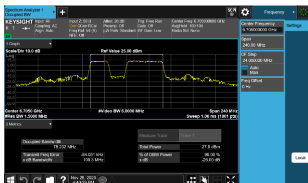
Plot 7-28 26dB BW & 99% OBW Antenna WF7a (80MHz BW 802.11be(RU) RU484+242 Index91 - Ch.151)
