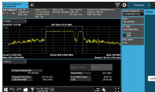
Plot 7-40 26dB BW & 99% OBW Antenna WF7a (160MHz BW 802.11be(RU) RU996+484+242 Index98 - Ch.79)
