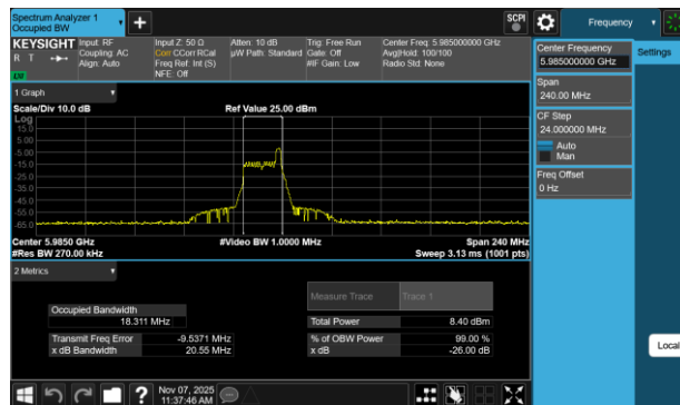
Plot 7-36 26dB BW & 99% OBW Antenna WF7a (80MHz BW 802.11be(RU) RU26 Index17 - Ch.7)
