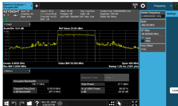
Plot 7-29 26dB BW & 99% OBW Antenna WF7a (160MHz BW 802.11be(RU) RU996+484+242 Index96 - Ch.143)
