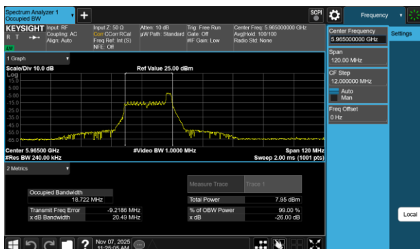
Plot 7-35 26dB BW & 99% OBW Antenna WF7a (40MHz BW 802.11be(RU) RU26 Index8 - Ch.3)
