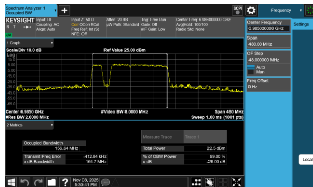
Plot 7-73 26dB BW & 99% OBW Antenna WF7a (160MHz BW 802.11be(RU) RU996+484+242 Index97 - Ch.207)
