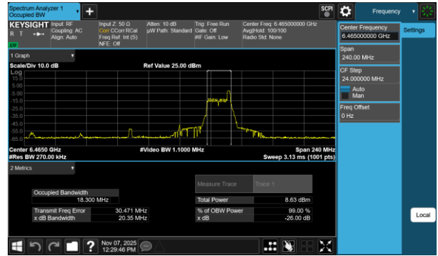
Plot 7-47 26dB BW & 99% OBW Antenna WF7a (80MHz BW 802.11be(RU) RU26 Index36 - Ch.103)
