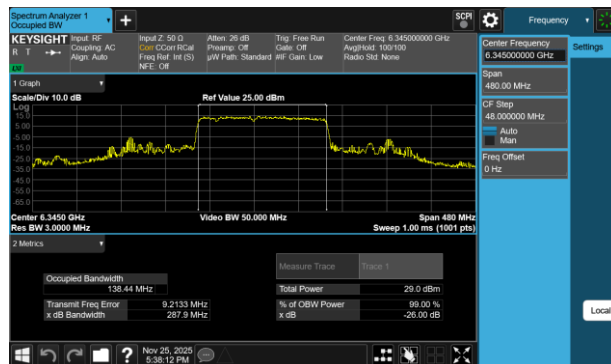
Plot 7-7 26dB BW & 99% OBW Antenna WF7a (160MHz BW 802.11be(RU) RU996+484+242 Index96 - Ch.79)
