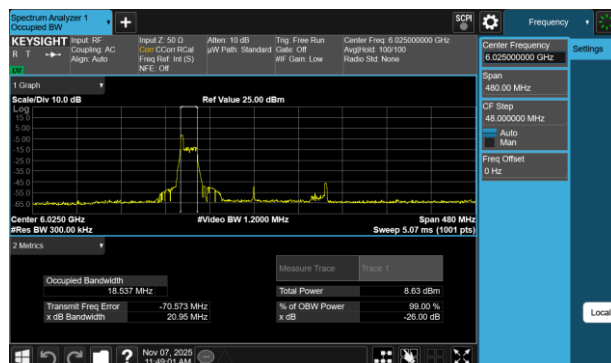
Plot 7-37 26dB BW & 99% OBW Antenna WF7a (160MHz BW 802.11be(RU) RU26 Index0 - Ch.15)
