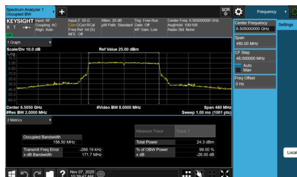
Plot 7-55 26dB BW & 99% OBW Antenna WF7a (160MHz BW 802.11be(RU) RU996X2 Index68 - Ch.111)
