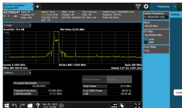
Plot 7-81 26dB BW & 99% OBW Antenna WF2a (160MHz BW 802.11be(RU) RU26 Index0 - Ch.47)
