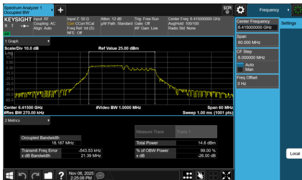
Plot 7-38 26dB BW & 99% OBW Antenna WF7a (20MHz BW 802.11be(RU) RU106+26 Index82 - Ch.93)
