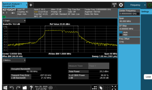
Plot 7-5 26dB BW & 99% OBW Antenna WF7a (20MHz BW 802.11be(RU) RU106+26 Index82 - Ch.1)
