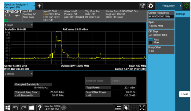
Plot 7-4 26dB BW & 99% OBW Antenna WF7a (160MHz BW 802.11be(RU) RU26 Index0 - Ch.79)
