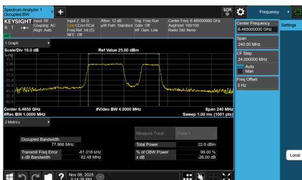
Plot 7-50 26dB BW & 99% OBW Antenna WF7a (80MHz BW 802.11be(RU) RU484+242 Index92 - Ch.103)
