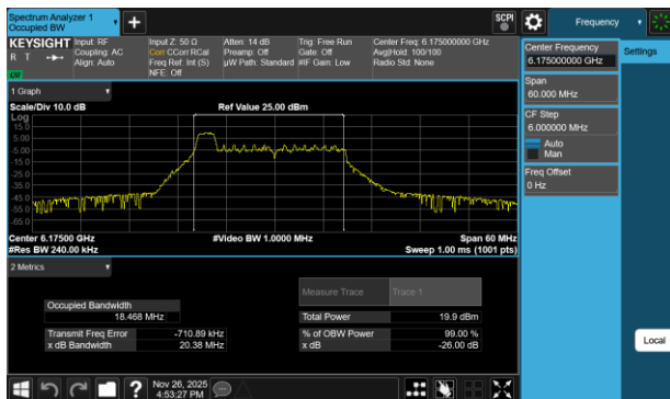
Plot 7-78 26dB BW & 99% OBW Antenna WF2a (20MHz BW 802.11be(RU) RU26 Index0 - Ch.45)
