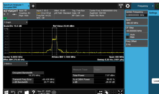
Plot 7-59 26dB BW & 99% OBW Antenna WF7a (160MHz BW 802.11be(RU) RU26 Index17 - Ch.143)
