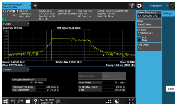
Plot 7-49 26dB BW & 99% OBW Antenna WF7a (20MHz BW 802.11be(RU) RU106+26 Index82 - Ch.105)
