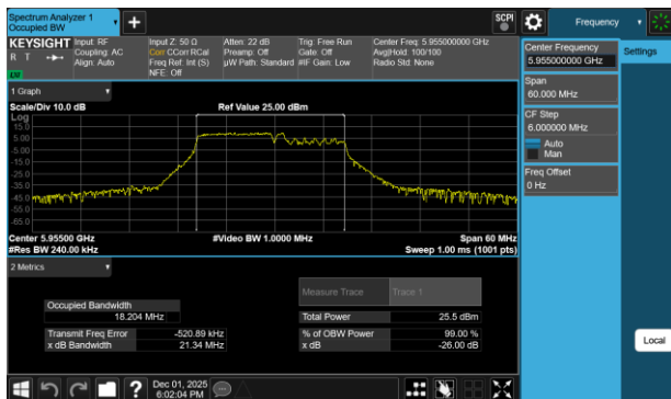
Plot 7-82 26dB BW & 99% OBW Antenna WF2a (20MHz BW 802.11be(RU) RU106+26 Index82 - Ch.1)
