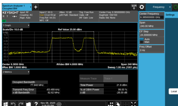
Plot 7-39 26dB BW & 99% OBW Antenna WF7a (80MHz BW 802.11be(RU) RU484+242 Index92 - Ch.87)
