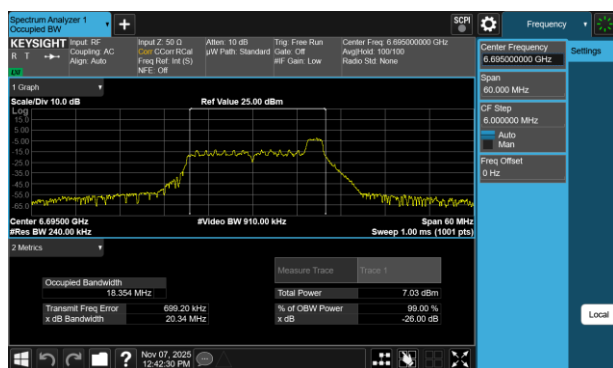
Plot 7-56 26dB BW & 99% OBW Antenna WF7a (20MHz BW 802.11be(RU) RU26 Index8 - Ch.149)
