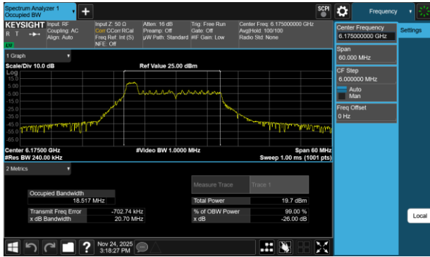
Plot 7-1 26dB BW & 99% OBW Antenna WF7a (20MHz BW 802.11be(RU) RU26 Index0 - Ch.45)
