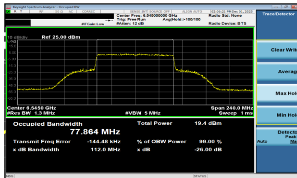
Plot 7-76 26dB BW & 99% OBW Antenna WF2a (80MHz BW 802.11be(RU) RU996 Index67 - Ch.119)
