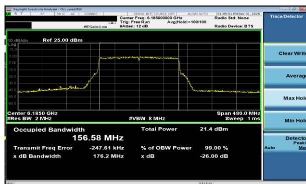
Plot 7-55 26dB BW & 99% OBW Antenna WF2a (160MHz BW 802.11be(RU) RU996X2 Index68 - Ch.47)
