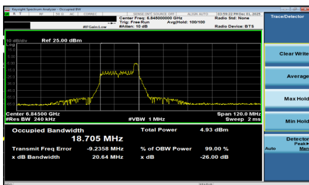
Plot 7-68 26dB BW & 99% OBW Antenna WF2a (40MHz BW 802.11be(RU) RU26 Index8 - Ch.179)
