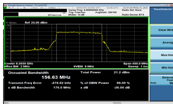
Plot 7-66 26dB BW & 99% OBW Antenna WF2a (160MHz BW 802.11be(RU) RU996X2 Index68 - Ch.111)
