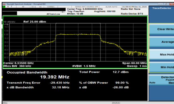
Plot 7-74 26dB BW & 99% OBW Antenna WF2a (20MHz BW 802.11be(RU) RU242 Index61 - Ch.117)
