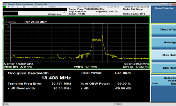
Plot 7-80 26dB BW & 99% OBW Antenna WF2a (80MHz BW 802.11be(RU) RU26 Index36 - Ch.215)
