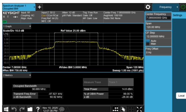
Plot 7-42 26dB BW & 99% OBW Antenna WF7a (40MHz BW 802.11be(RU) RU484 Index65 - Ch.227)
