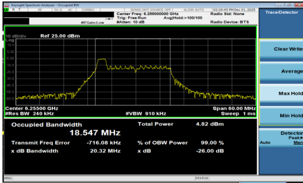
Plot 7-45 26dB BW & 99% OBW Antenna WF2a (20MHz BW 802.11be(RU) RU26 Index0 - Ch.61)
