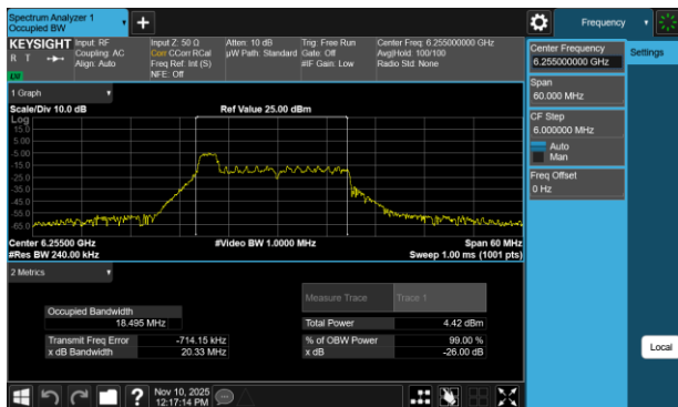
Plot 7-1 26dB BW & 99% OBW Antenna WF7a (20MHz BW 802.11be(RU) RU26 Index0 - Ch.61)
