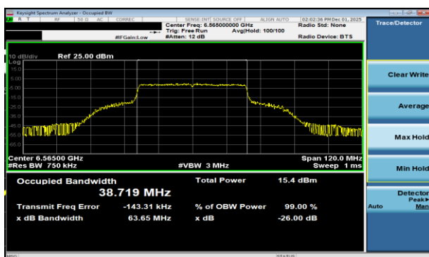
Plot 7-75 26dB BW & 99% OBW Antenna WF2a (40MHz BW 802.11be(RU) RU484 Index65 - Ch.123)
