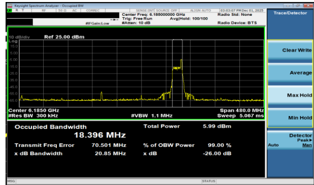
Plot 7-48 26dB BW & 99% OBW Antenna WF2a (160MHz BW 802.11be(RU) RU26 Index36 - Ch.47)
