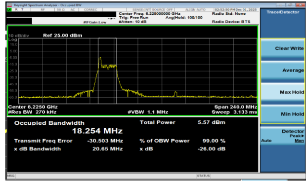
Plot 7-47 26dB BW & 99% OBW Antenna WF2a (80MHz BW 802.11be(RU) RU26 Index0 - Ch.55)
