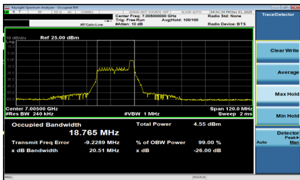
Plot 7-79 26dB BW & 99% OBW Antenna WF2a (40MHz BW 802.11be(RU) RU26 Index8 - Ch.211)
