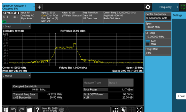
Plot 7-2 26dB BW & 99% OBW Antenna WF7a (40MHz BW 802.11be(RU) RU26 Index8 - Ch.35)
