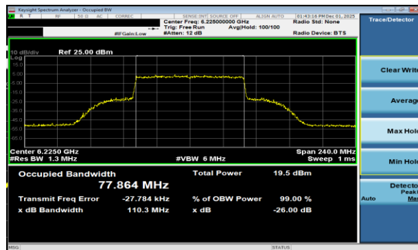
Plot 7-54 26dB BW & 99% OBW Antenna WF2a (80MHz BW 802.11be(RU) RU996 Index67 - Ch.55)
