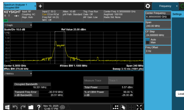
Plot 7-3 26dB BW & 99% OBW Antenna WF7a (80MHz BW 802.11be(RU) RU26 Index0 - Ch.87)
