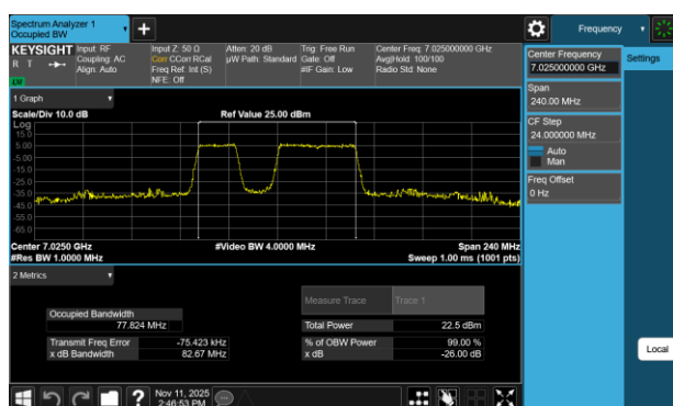
Plot 7-39 26dB BW & 99% OBW Antenna WF7a (80MHz BW 802.11be(RU) RU484+242 Index91 - Ch.215)
