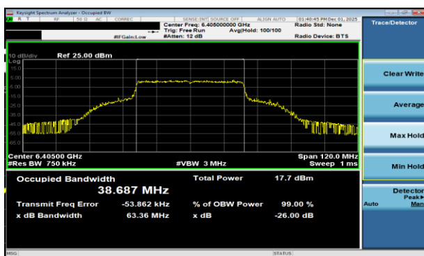
Plot 7-53 26dB BW & 99% OBW Antenna WF2a (40MHz BW 802.11be(RU) RU484 Index65 - Ch.91)
