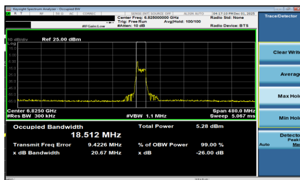
Plot 7-70 26dB BW & 99% OBW Antenna WF2a (160MHz BW 802.11be(RU) RU26 Index0 - Ch.175)
