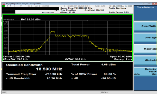
Plot 7-78 26dB BW & 99% OBW Antenna WF2a (20MHz BW 802.11be(RU) RU26 Index0 - Ch.229)
