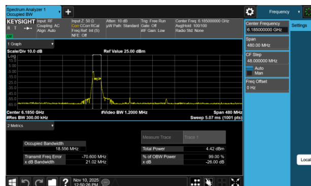
Plot 7-4 26dB BW & 99% OBW Antenna WF7a (160MHz BW 802.11be(RU) RU26 Index0 - Ch.47)
