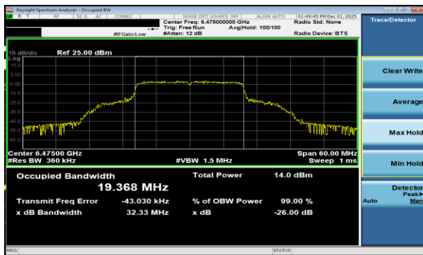
Plot 7-63 26dB BW & 99% OBW Antenna WF2a (20MHz BW 802.11be(RU) RU242 Index61 - Ch.105)
