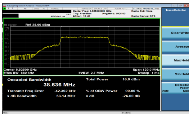
Plot 7-64 26dB BW & 99% OBW Antenna WF2a (40MHz BW 802.11be(RU) RU484 Index65 - Ch.115)
