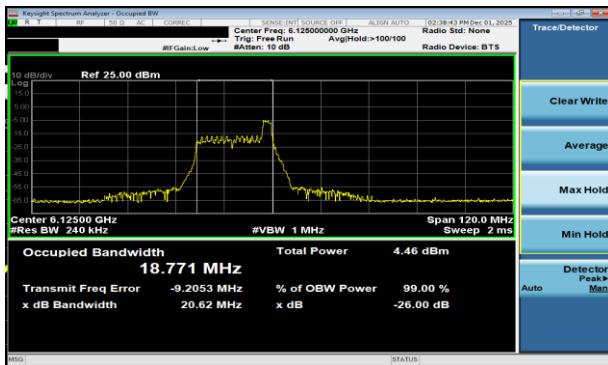
Plot 7-46 26dB BW & 99% OBW Antenna WF2a (40MHz BW 802.11be(RU) RU26 Index8 - Ch.35)
