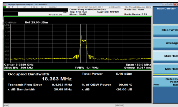
Plot 7-81 26dB BW & 99% OBW Antenna WF2a (160MHz BW 802.11be(RU) RU26 Index0 - Ch.207)
