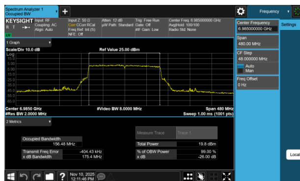
Plot 7-44 26dB BW & 99% OBW Antenna WF7a (160MHz BW 802.11be(RU) RU996X2 Index68 - Ch.207)
