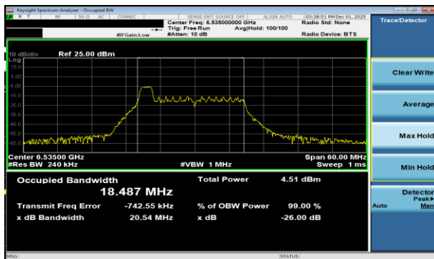
Plot 7-67 26dB BW & 99% OBW Antenna WF2a (20MHz BW 802.11be(RU) RU26 Index0 - Ch.117)
