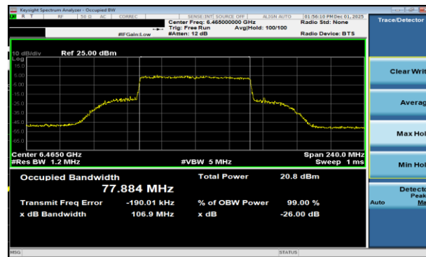
Plot 7-65 26dB BW & 99% OBW Antenna WF2a (80MHz BW 802.11be(RU) RU996 Index67 - Ch.103)
