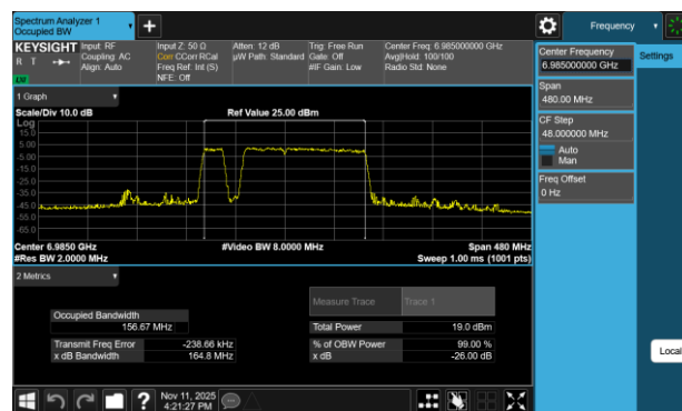
Plot 7-40 26dB BW & 99% OBW Antenna WF7a (160MHz BW 802.11be(RU) RU996+484+242 Index97 - Ch.207)
