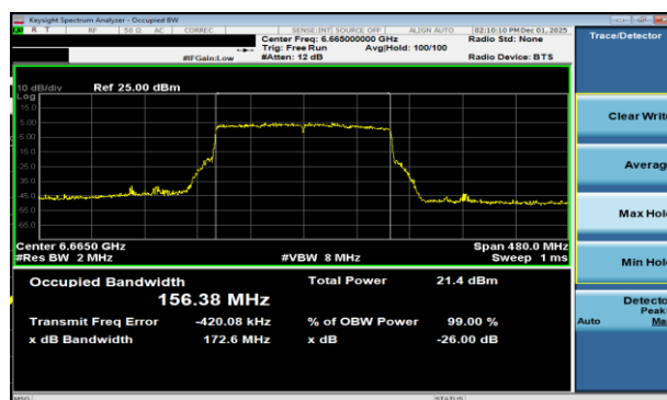
Plot 7-77 26dB BW & 99% OBW Antenna WF2a (160MHz BW 802.11be(RU) RU996X2 Index68 - Ch.143)
