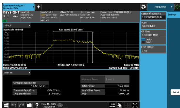
Plot 7-38 26dB BW & 99% OBW Antenna WF7a (20MHz BW 802.11be(RU) RU106+26 Index82 - Ch.209)
