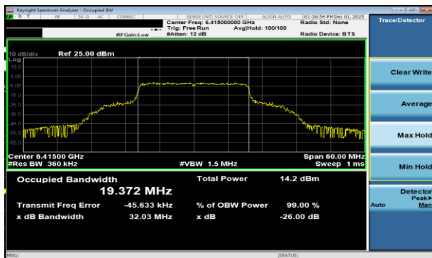
Plot 7-52 26dB BW & 99% OBW Antenna WF2a (20MHz BW 802.11be(RU) RU242 Index61 - Ch.93)
