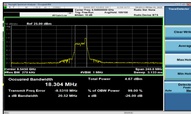
Plot 7-69 26dB BW & 99% OBW Antenna WF2a (80MHz BW 802.11be(RU) RU26 Index17 - Ch.119)
